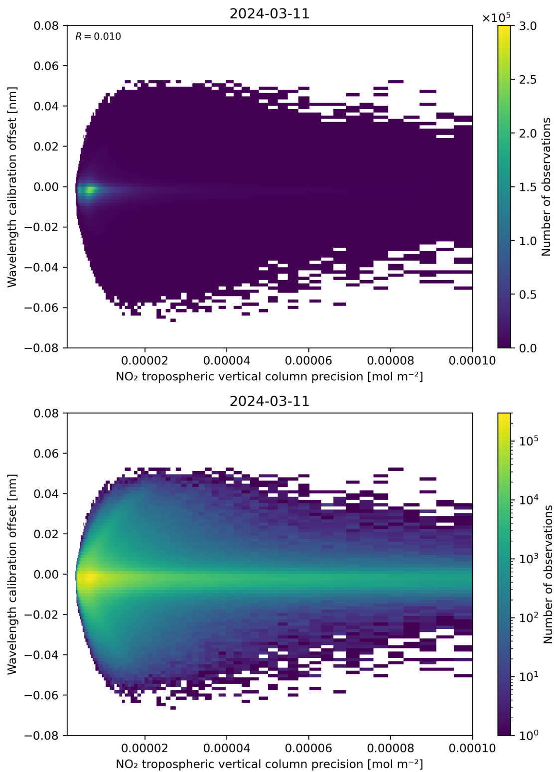
Figure 141: Scatter density plot of “NO 2 tropospheric vertical column precision” against “Wavelength calibration offset” for 2024-03-10 to 2024-03-12.
