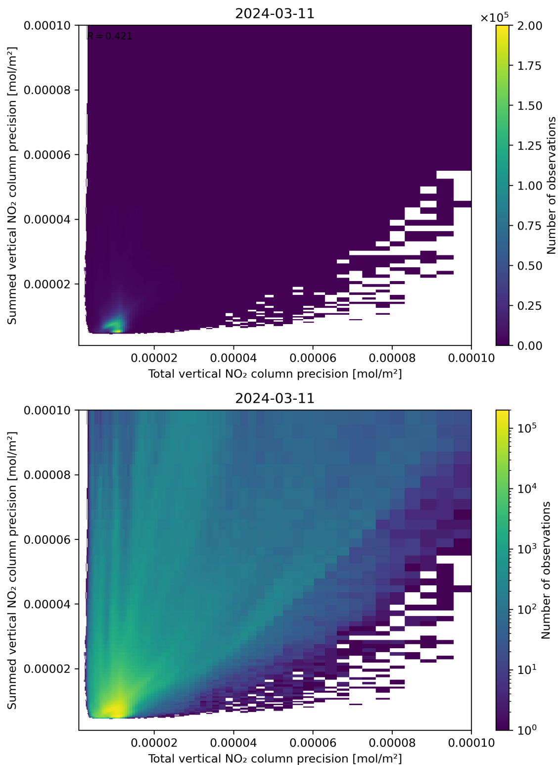
Figure 118: Scatter density plot of “Total vertical NO 2 column precision” against “Summed vertical NO 2 column precision” for 2024-03-10 to 2024-03-12.
