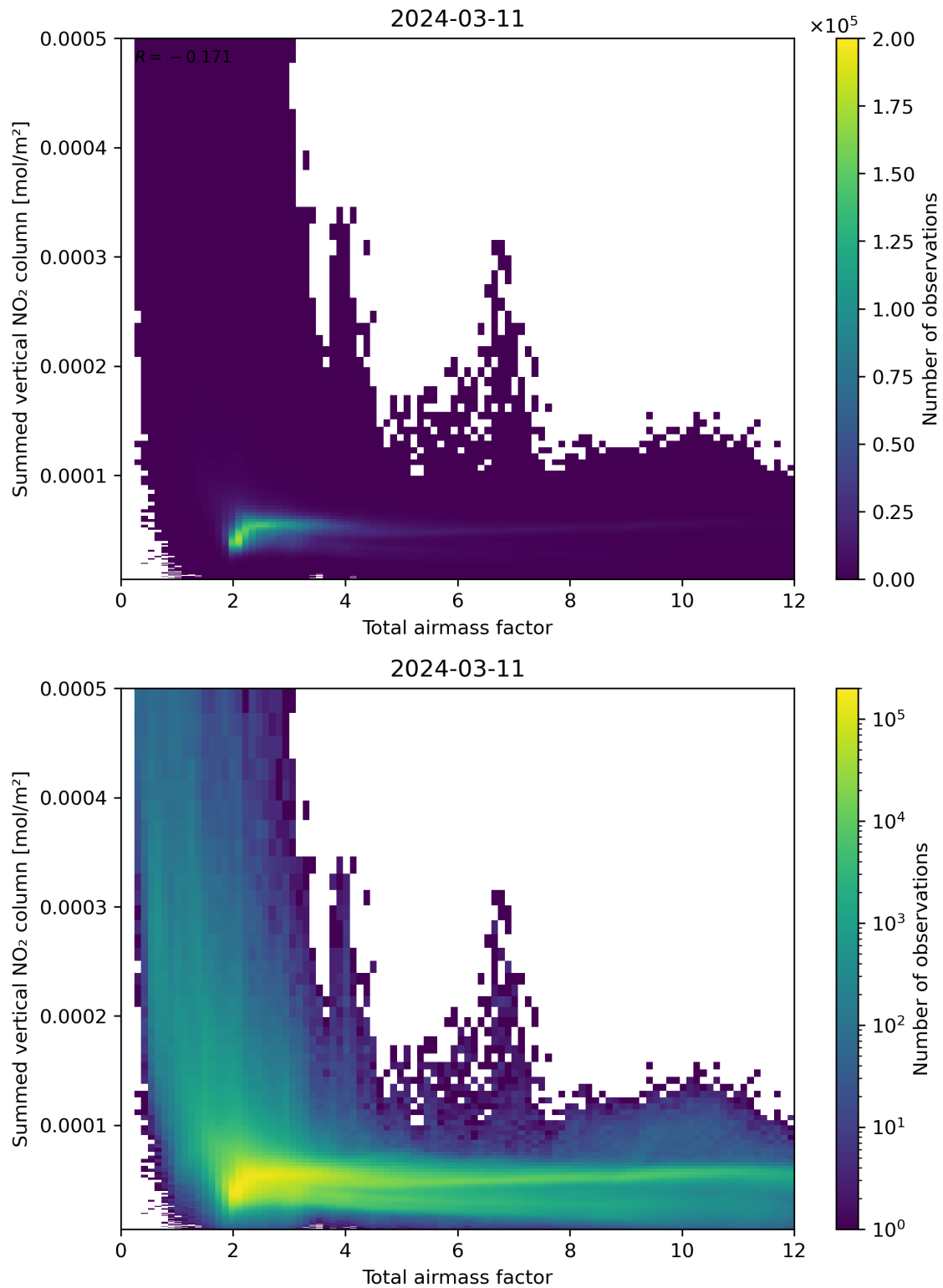
Figure 65: Scatter density plot of “Total airmass factor” against “Summed vertical NO 2 column” for 2024-03-10 to 2024-03-12.
