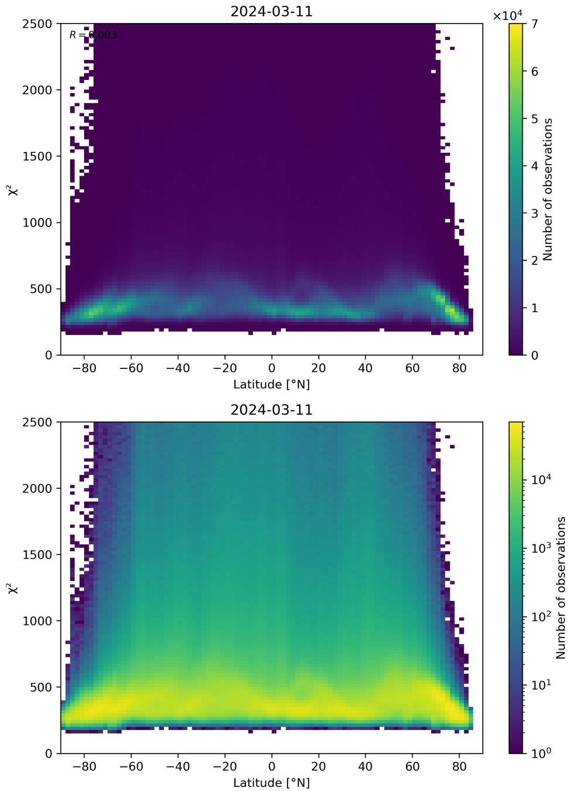
Figure 86: Scatter density plot of “Latitude” against “ \chi^2 ” for 2024-03-10 to 2024-03-12.
