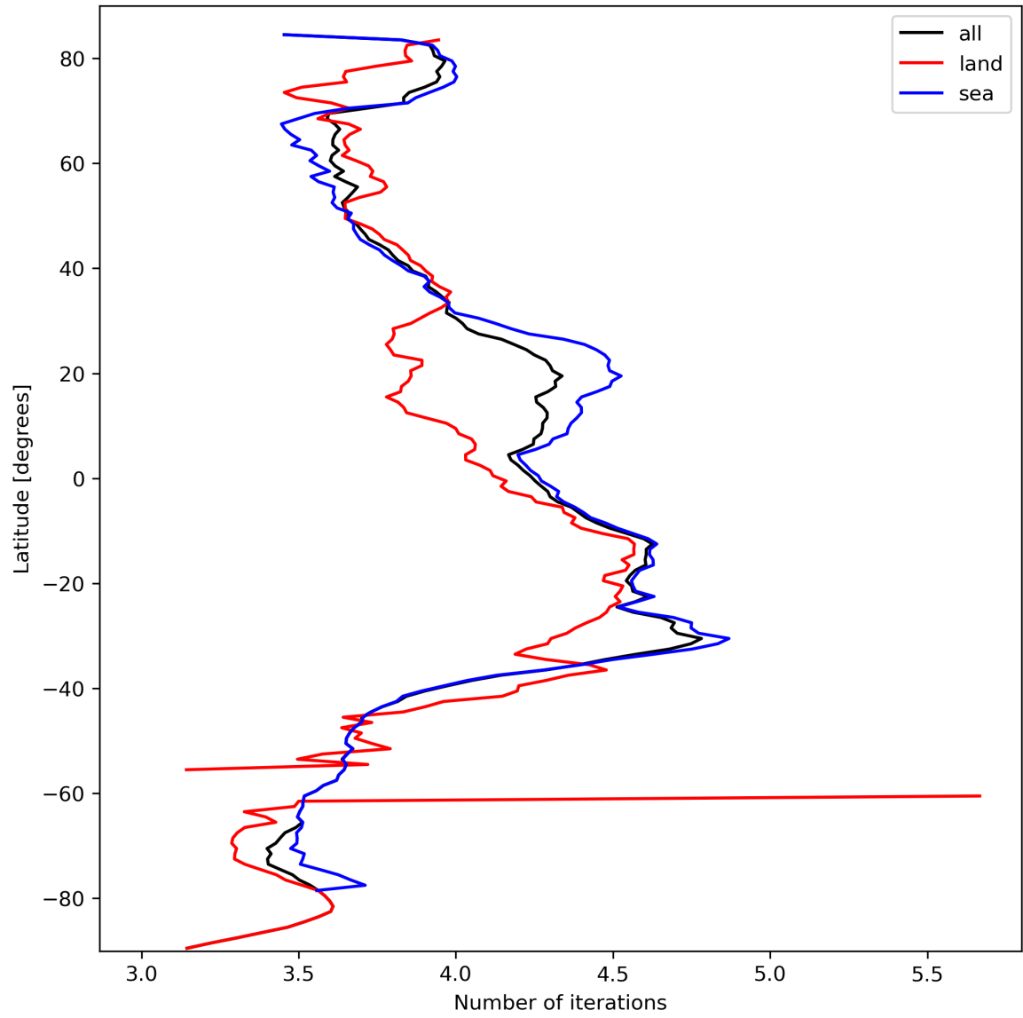
Figure 17: Zonal average of “Number of iterations” for 2024-03-10 to 2024-03-12.
