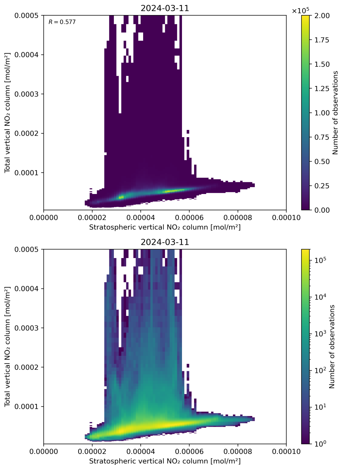
Figure 100: Scatter density plot of “Stratospheric vertical NO 2 column” against “Total vertical NO 2 column” for 2024-03-10 to 2024-03-12.
