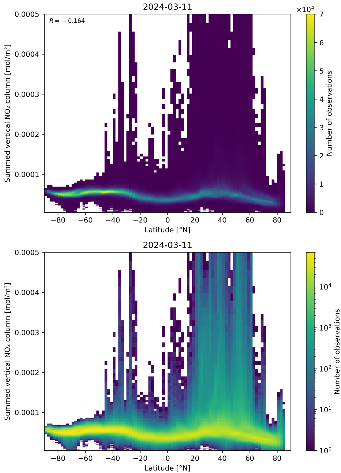
Figure 88: Scatter density plot of “Latitude” against “Summed vertical NO 2 column” for 2024-03-10 to 2024-03-12.
