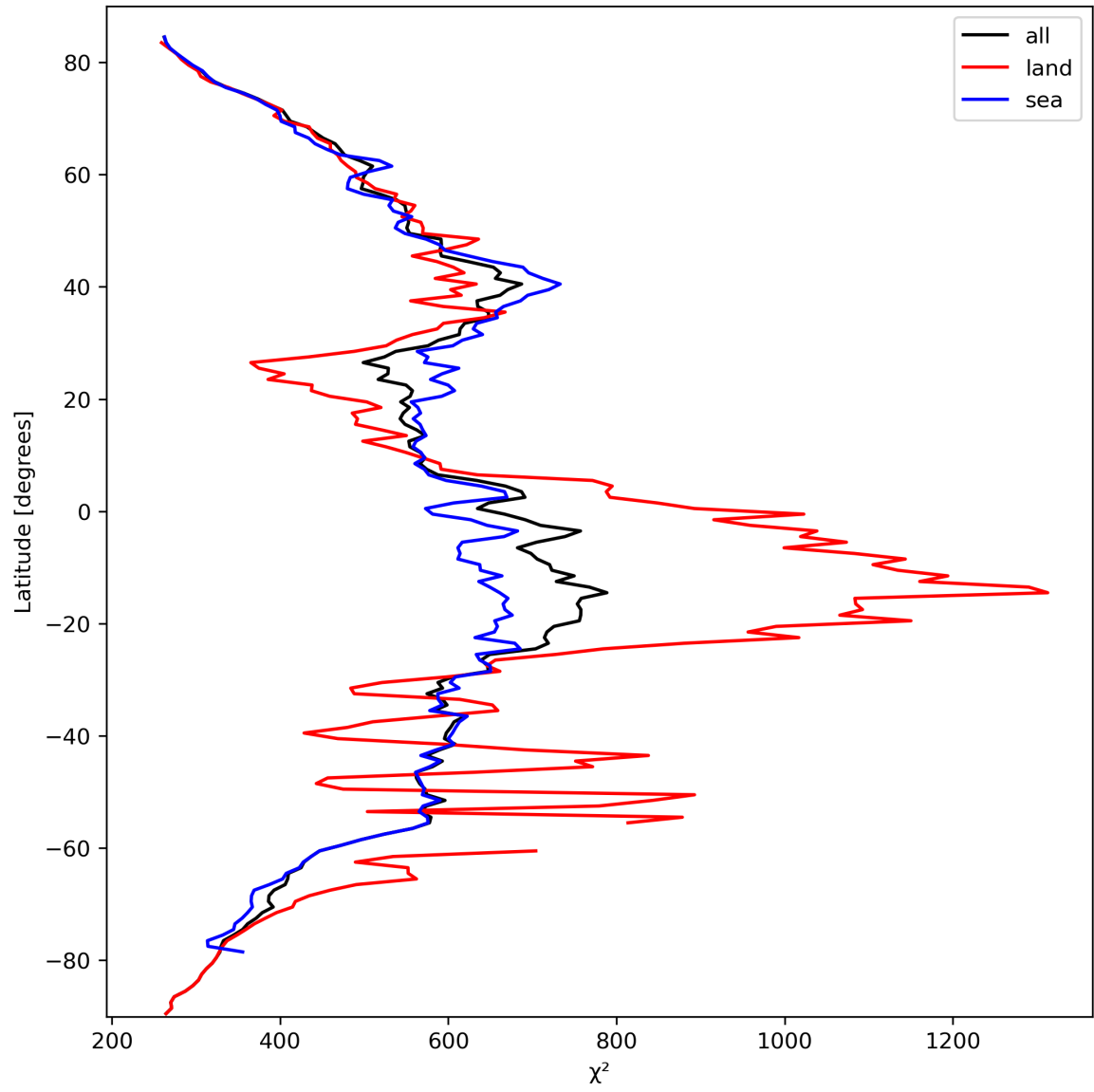
Figure 25: Zonal average of “ \chi^2 ” for 2024-03-10 to 2024-03-12.
