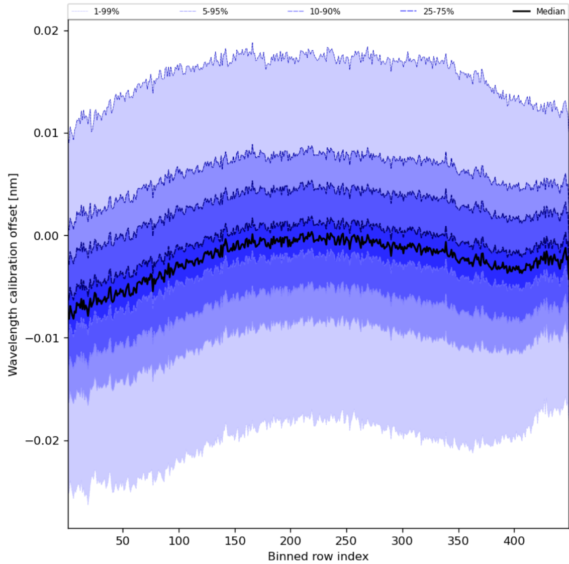
Figure 52: Along track statistics of “Wavelength calibration offset” for 2024-03-10 to 2024-03-12
