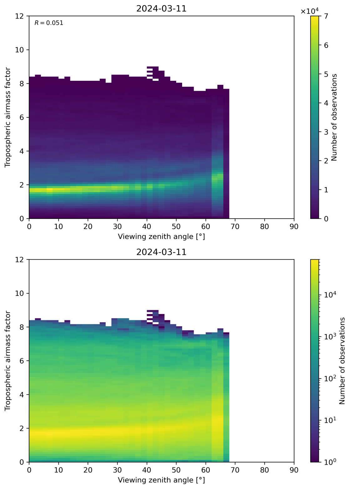
Figure 161: Scatter density plot of “Viewing zenith angle” against “Tropospheric airmass factor” for 2024-03-10 to 2024-03-12.
