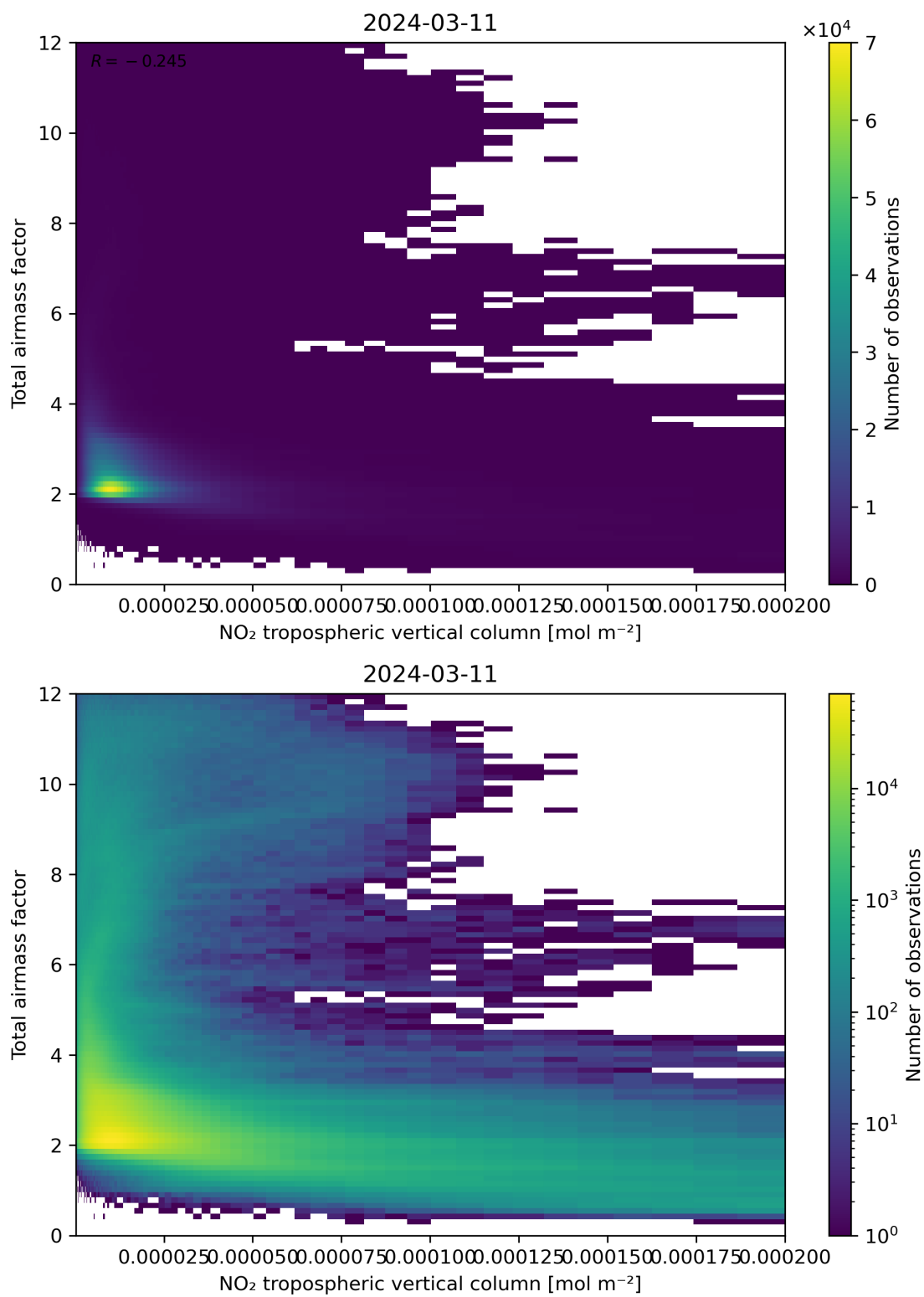
Figure 122: Scatter density plot of “NO 2 tropospheric vertical column” against “Total air mass factor” for 2024-03-10 to 2024-03-12.
