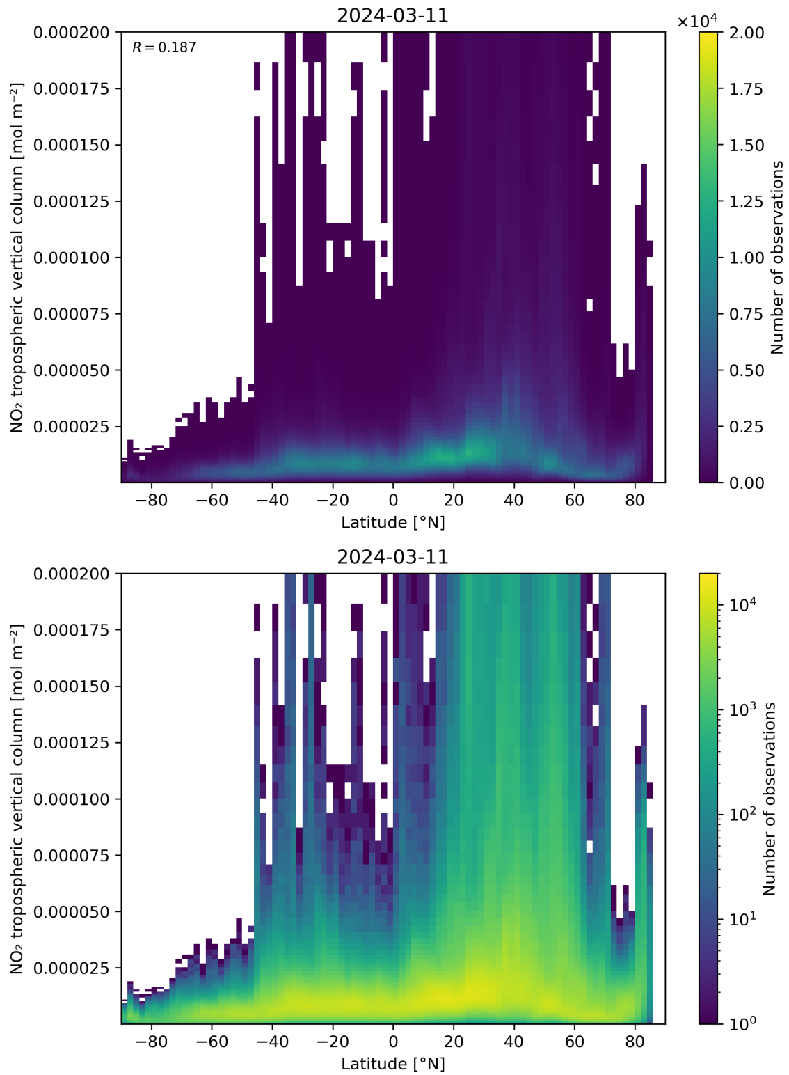
Figure 92: Scatter density plot of “Latitude” against “NO 2 tropospheric vertical column” for 2024-03-10 to 2024-03-12.
