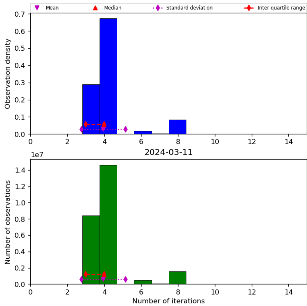
Figure 34: Histogram of “Number of iterations” for 2024-03-10 to 2024-03-12
