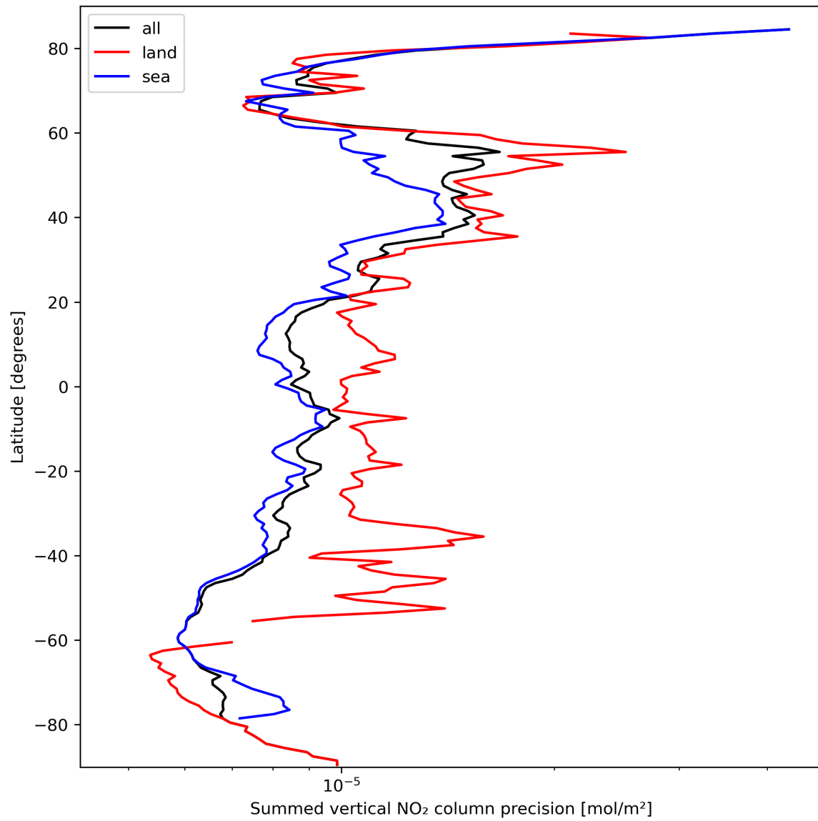
Figure 24: Zonal average of “Summed vertical NO 2 column precision” for 2024-03-10 to 2024-03-12.
