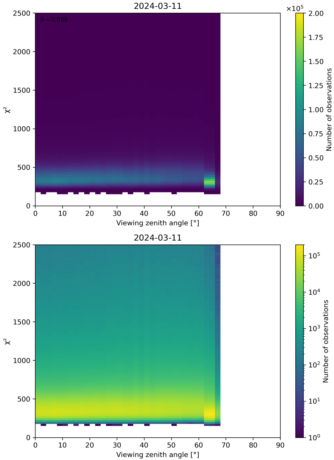
Figure 162: Scatter density plot of “Viewing zenith angle” against “ \chi^2 ” for 2024-03-10 to 2024-03-12.
