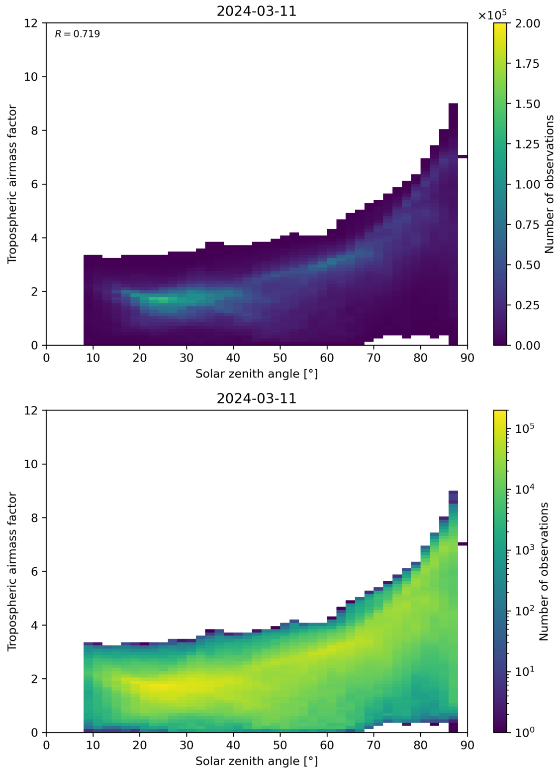
Figure 147: Scatter density plot of “Solar zenith angle” against “Tropospheric airmass factor” for 2024-03-10 to 2024-03-12.
