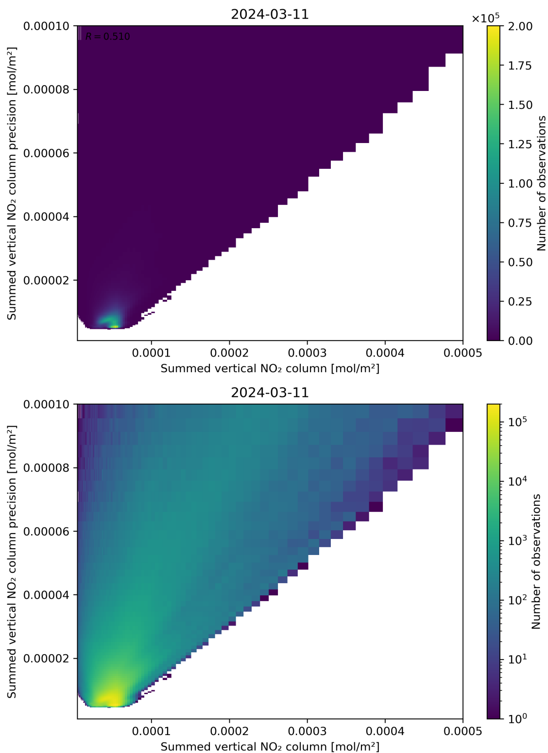
Figure 105: Scatter density plot of “Summed vertical NO 2 column” against “Summed vertical NO 2 column precision” for 2024-03-10 to 2024-03-12.
