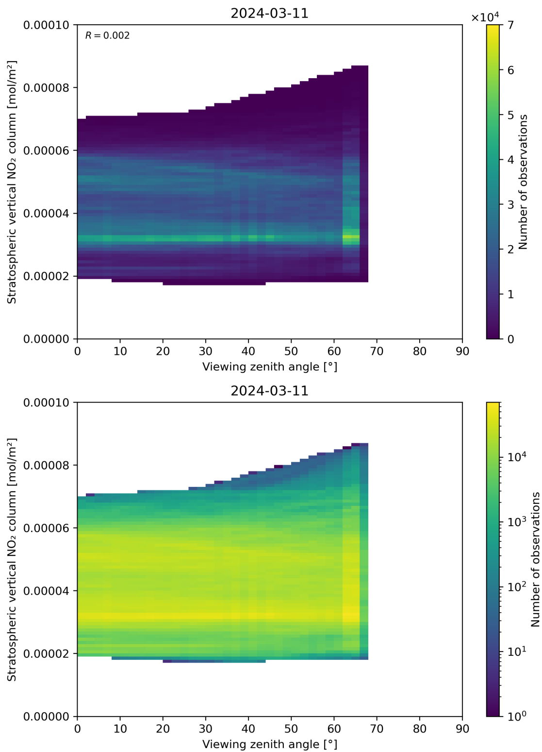
Figure 164: Scatter density plot of “Viewing zenith angle” against “Stratospheric vertical NO 2 column” for 2024-03-10 to 2024-03-12.
