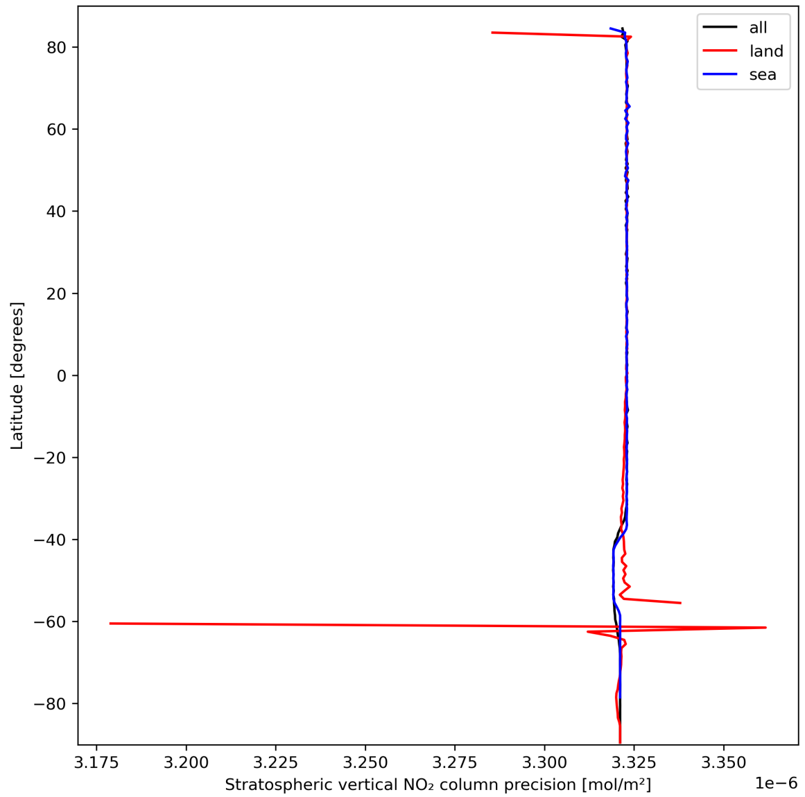
Figure 20: Zonal average of "Stratospheric vertical NO 2 column precision" for 2024-03-10 to 2024-03-12.
