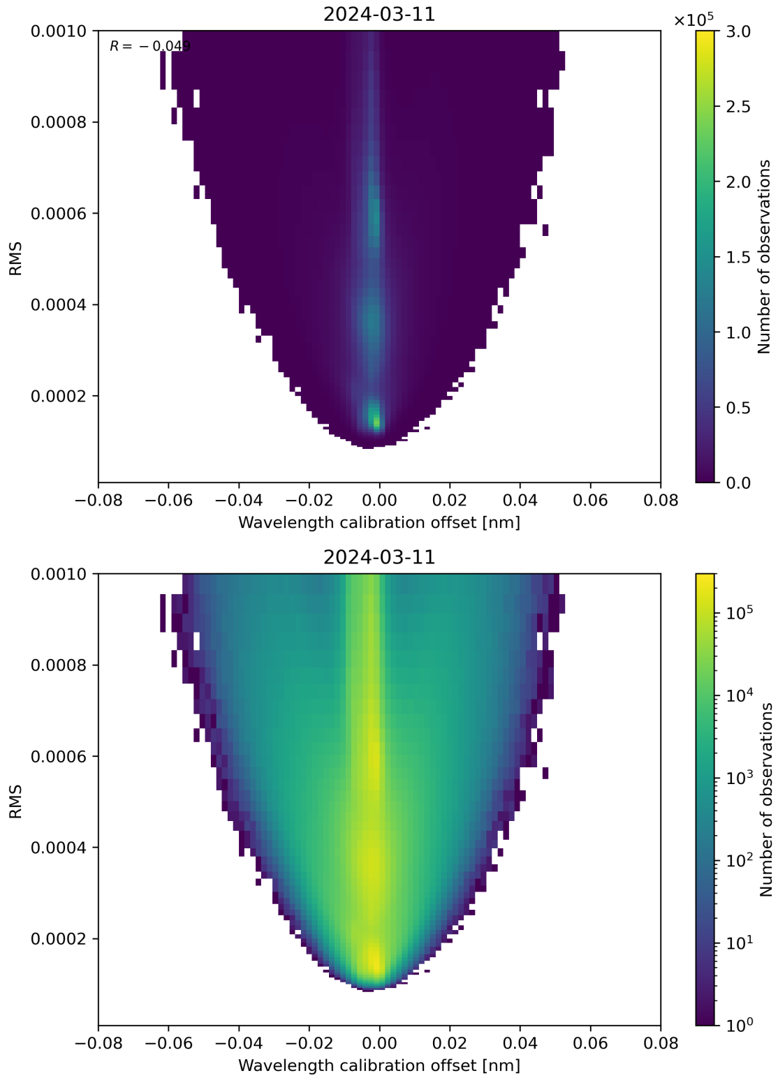
Figure 181: Scatter density plot of “Wavelength calibration offset” against “RMS” for 2024-03-10 to 2024-03-12.
