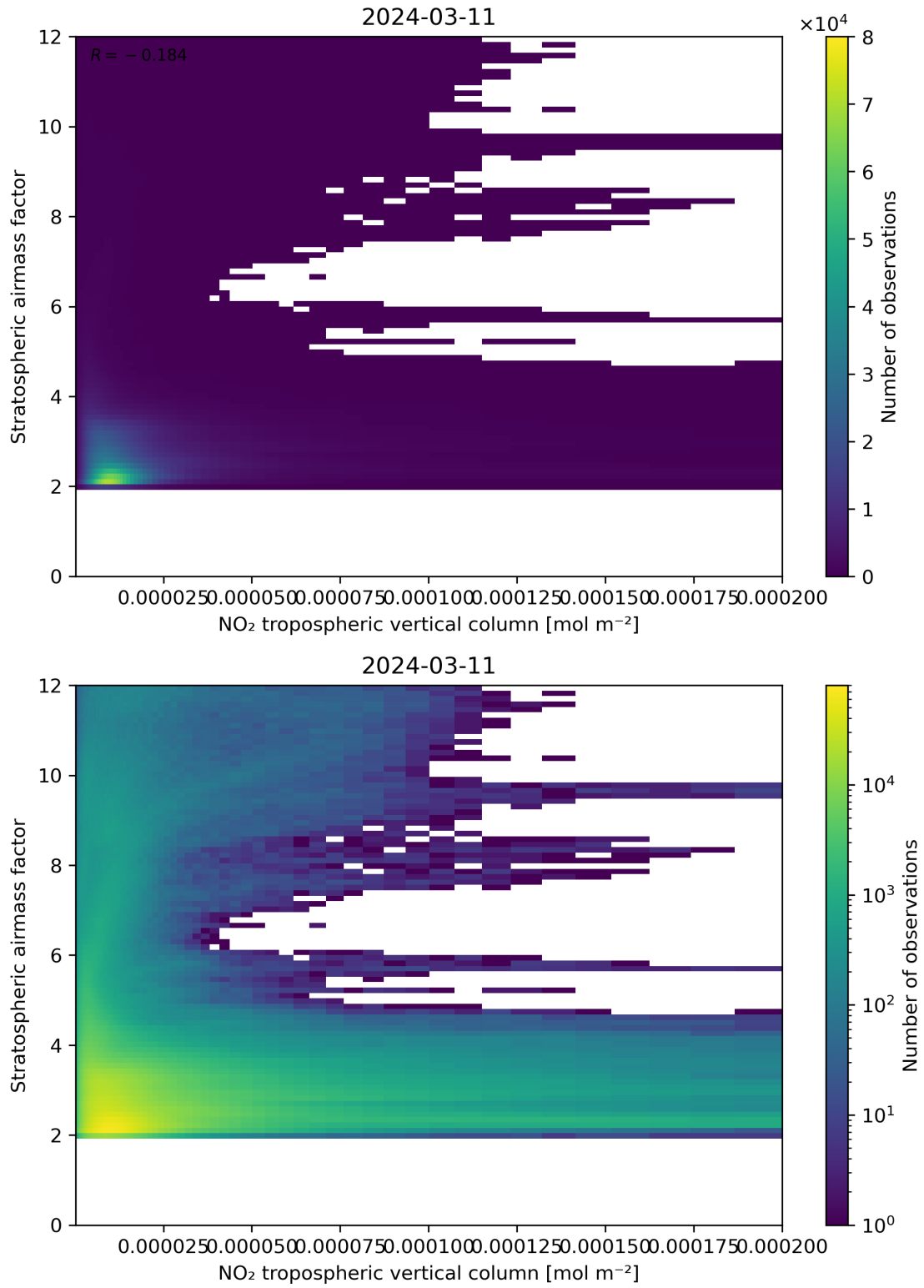
Figure 121: Scatter density plot of “NO 2 tropospheric vertical column” against “Stratospheric air mass factor” for 2024-03-10 to 2024-03-12.
