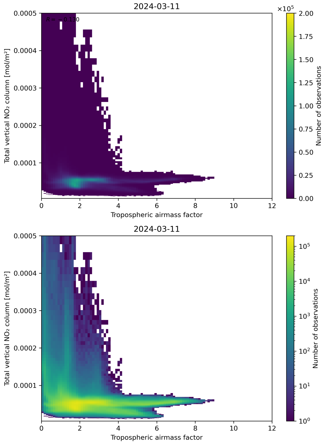
Figure 77: Scatter density plot of “Tropospheric airmass factor” against “Total vertical NO 2 column” for 2024-03-10 to 2024-03-12.
