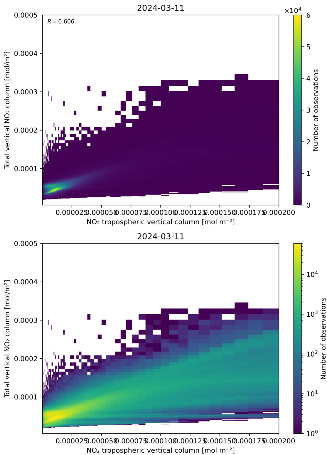
Figure 128: Scatter density plot of “NO 2 tropospheric vertical column” against “Total vertical NO 2 column” for 2024-03-10 to 2024-03-12.
