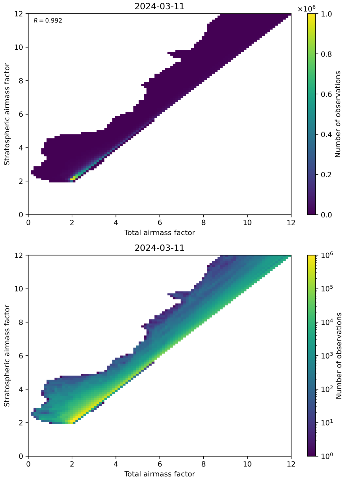
Figure 62: Scatter density plot of “Total airmass factor” against “Stratospheric airmass factor” for 2024-03-10 to 2024-03-12.
