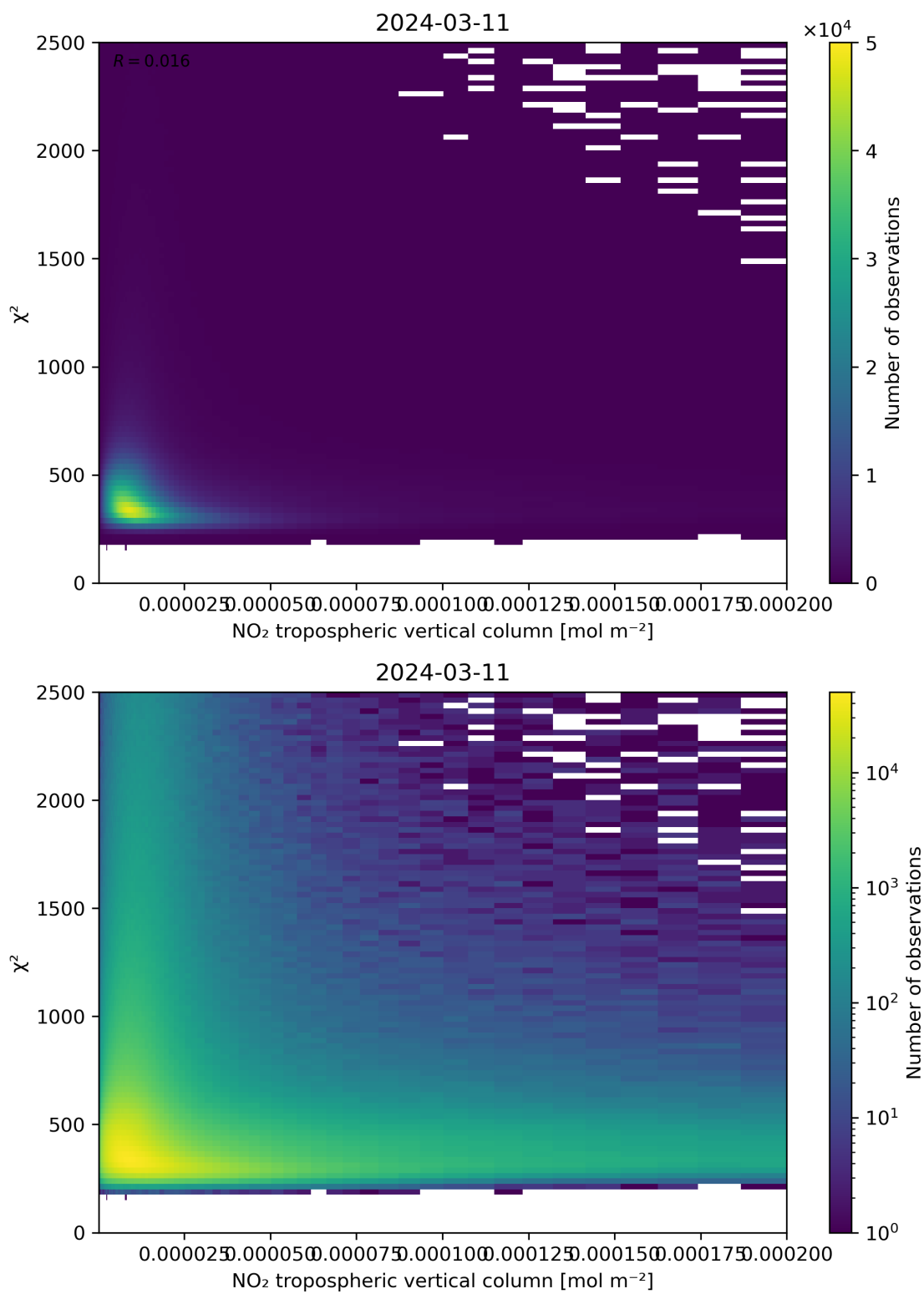
Figure 124: Scatter density plot of “NO 2 tropospheric vertical column” against “ \chi^2 ” for 2024-03-10 to 2024-03-12.
