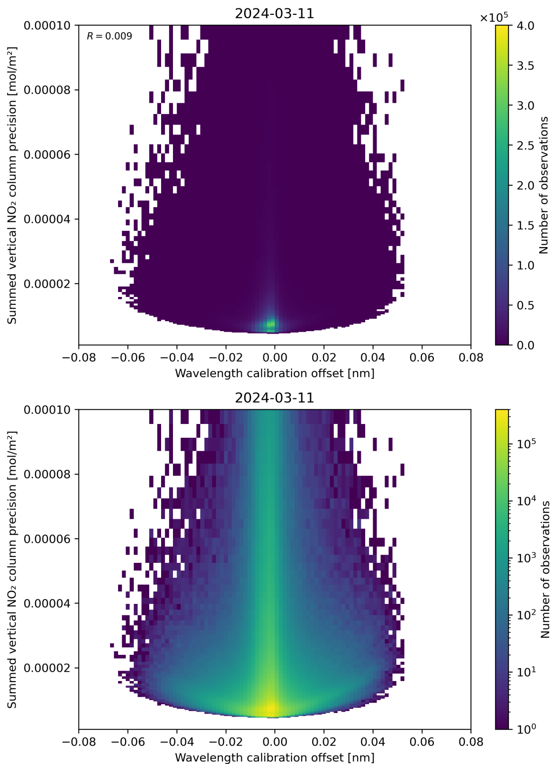
Figure 178: Scatter density plot of “Wavelength calibration offset” against “Summed vertical NO 2 column precision” for 2024-03-10 to 2024-03-12.
