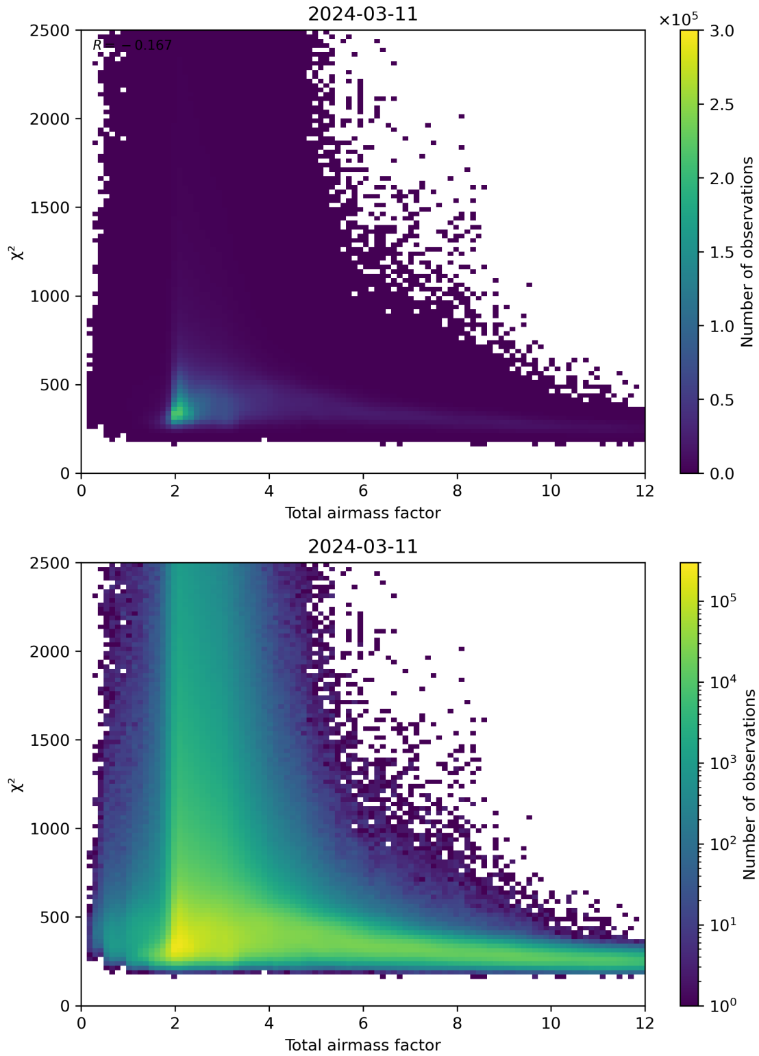
Figure 63: Scatter density plot of “Total airmass factor” against “ \chi^2 ” for 2024-03-10 to 2024-03-12.
