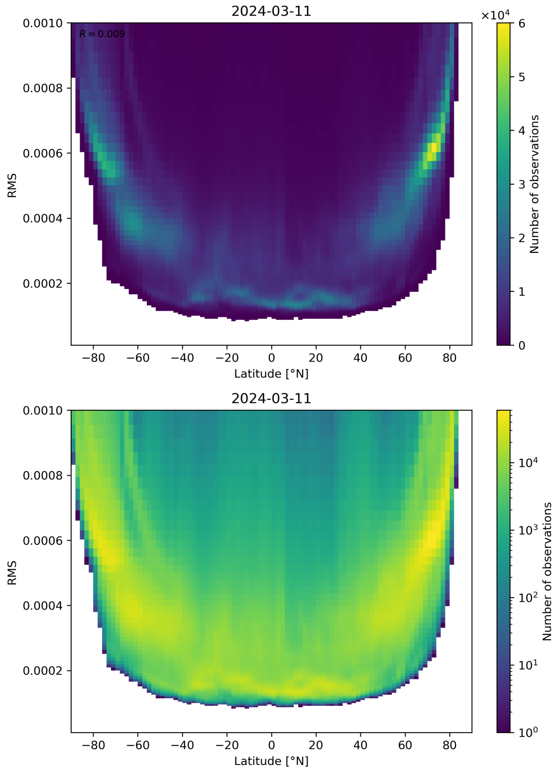
Figure 94: Scatter density plot of “Latitude” against “RMS” for 2024-03-10 to 2024-03-12.
