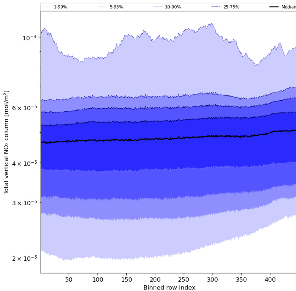
Figure 55: Along track statistics of “Total vertical NO 2 column” for 2024-03-10 to 2024-03-12
