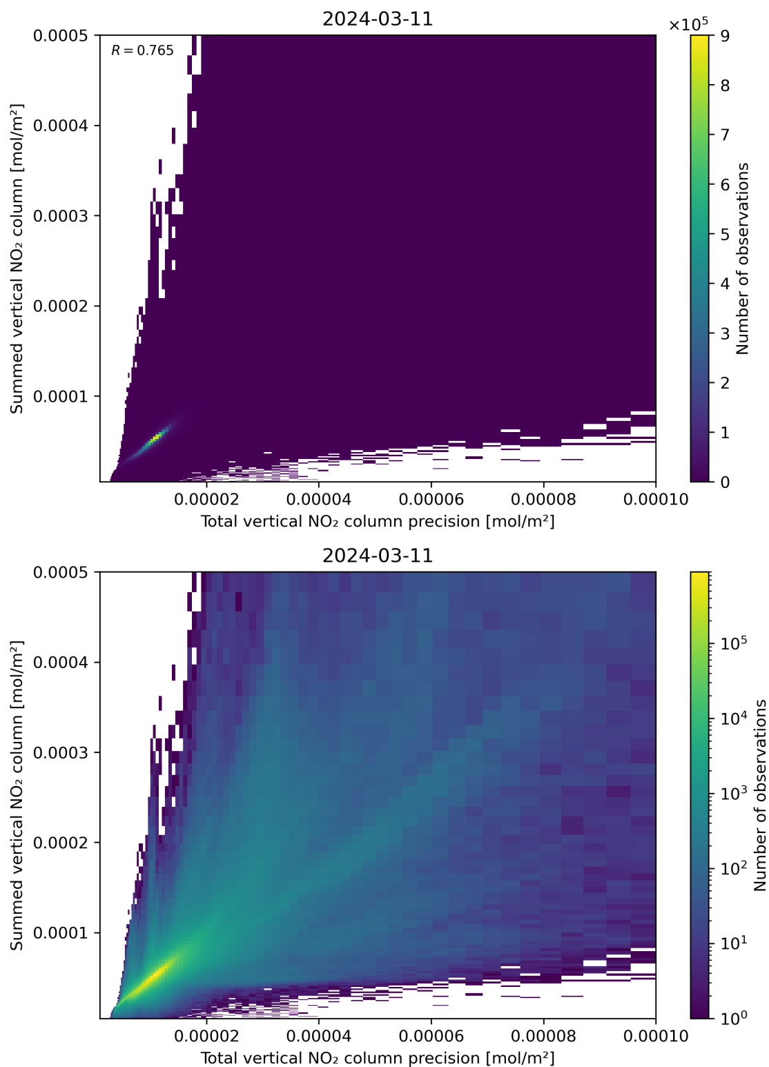
Figure 117: Scatter density plot of “Total vertical NO 2 column precision” against “Summed vertical NO 2 column” for 2024-03-10 to 2024-03-12.
