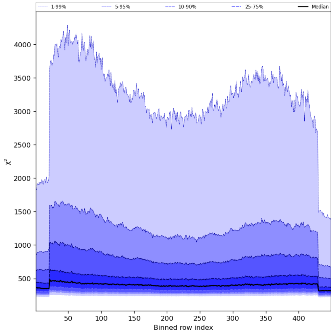
Figure 59: Along track statistics of “ \chi^2 ” for 2024-03-10 to 2024-03-12
