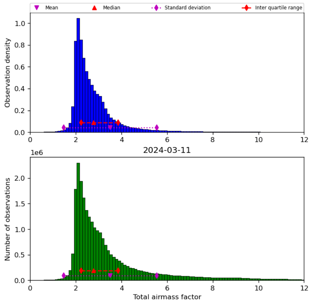
Figure 32: Histogram of “Total airmass factor” for 2024-03-10 to 2024-03-12
