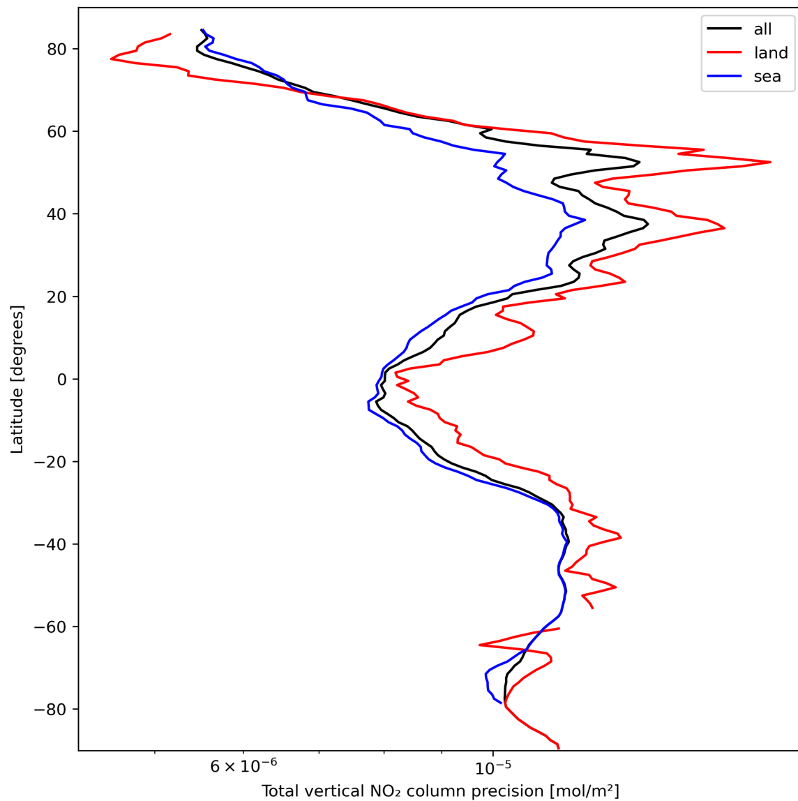
Figure 22: Zonal average of “Total vertical NO 2 column precision” for 2024-03-10 to 2024-03-12.
