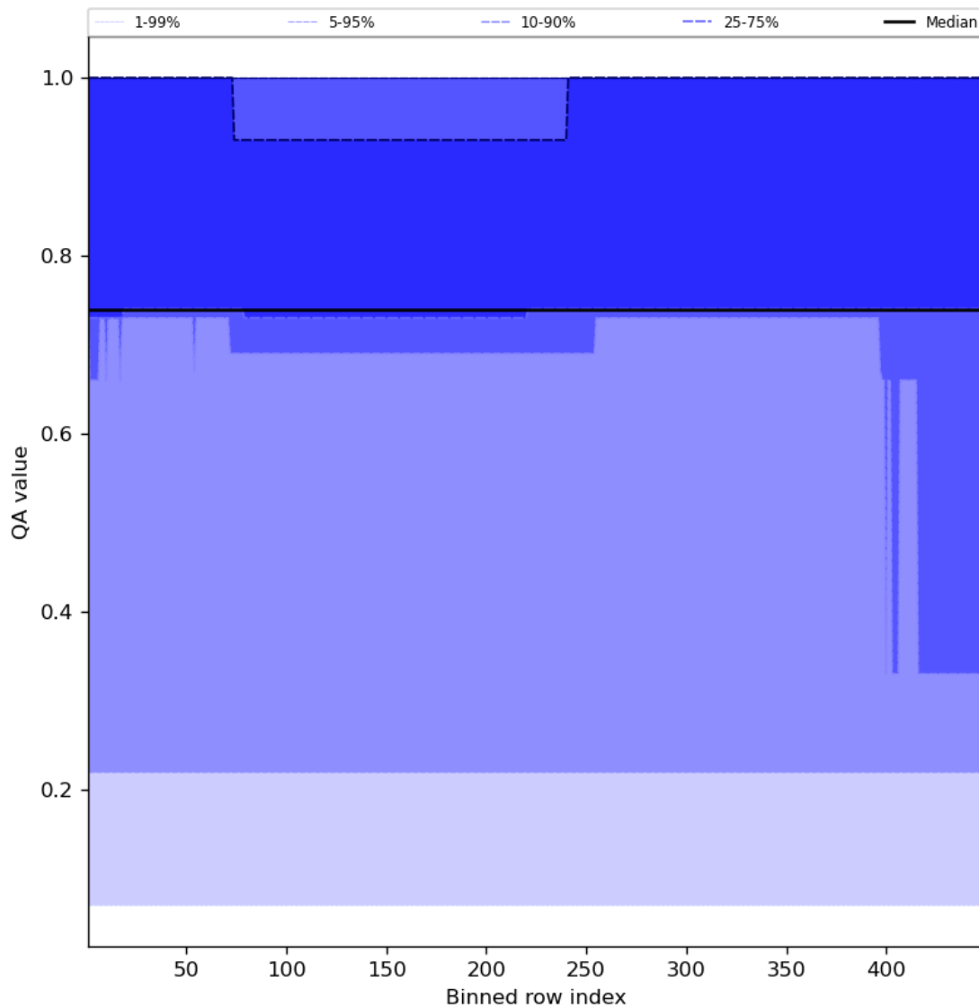
Figure 45: Along track statistics of “QA value” for 2024-03-10 to 2024-03-12
