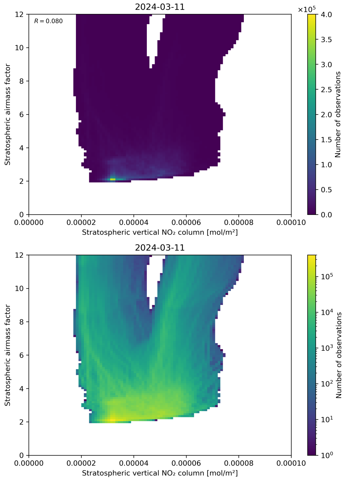
Figure 96: Scatter density plot of “Stratospheric vertical NO 2 column” against “Stratospheric airmass factor” for 2024-03-10 to 2024-03-12.
