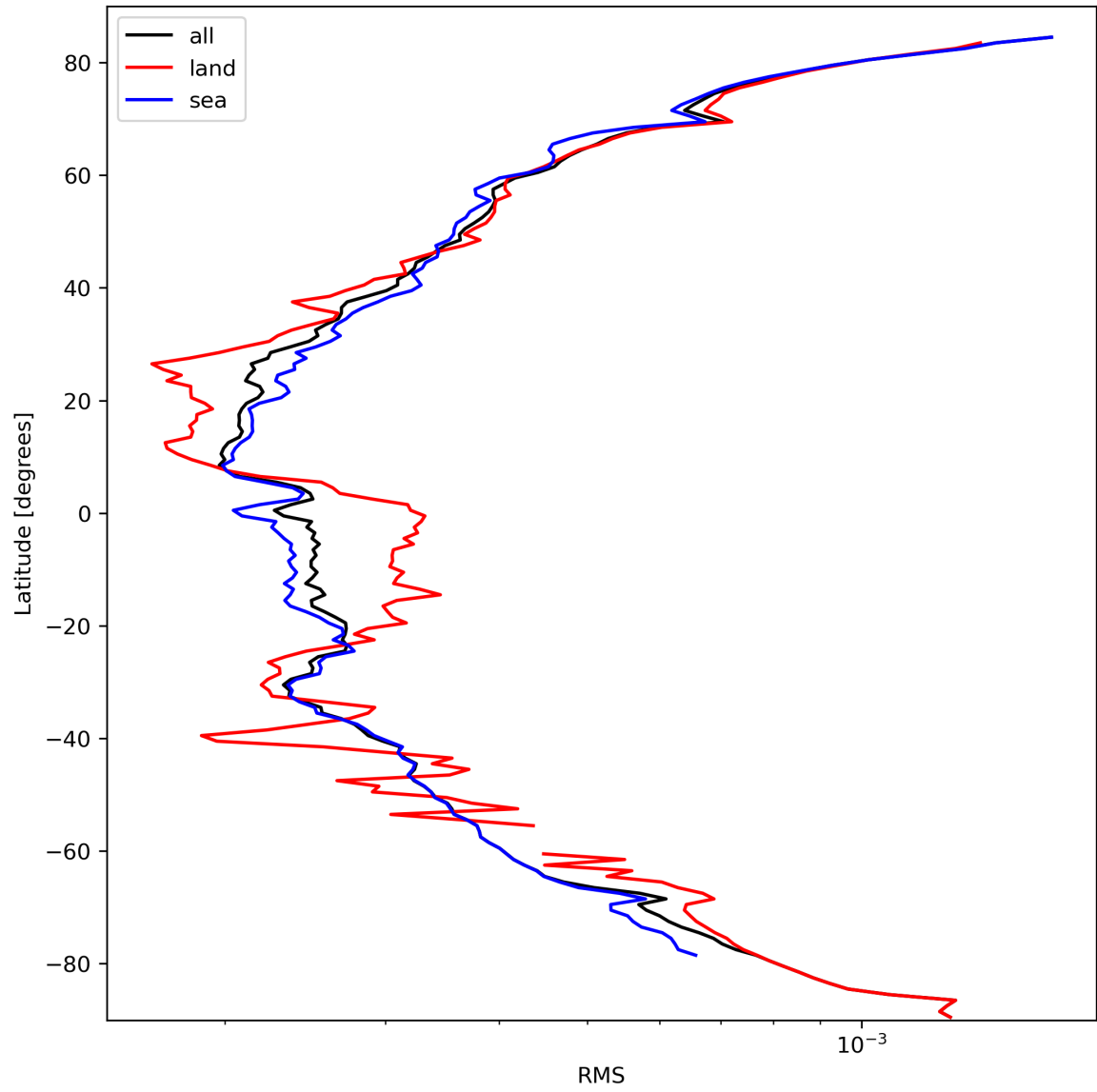
Figure 26: Zonal average of “RMS” for 2024-03-10 to 2024-03-12.
