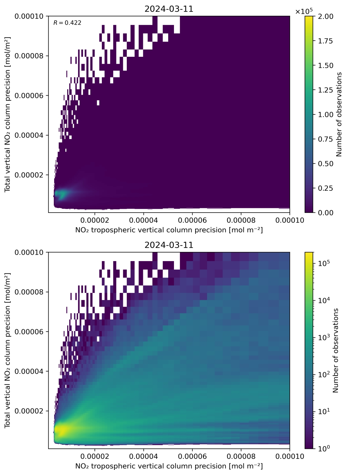
Figure 139: Scatter density plot of “NO 2 tropospheric vertical column precision” against “Total vertical NO 2 column precision” for 2024-03-10 to 2024-03-12.
