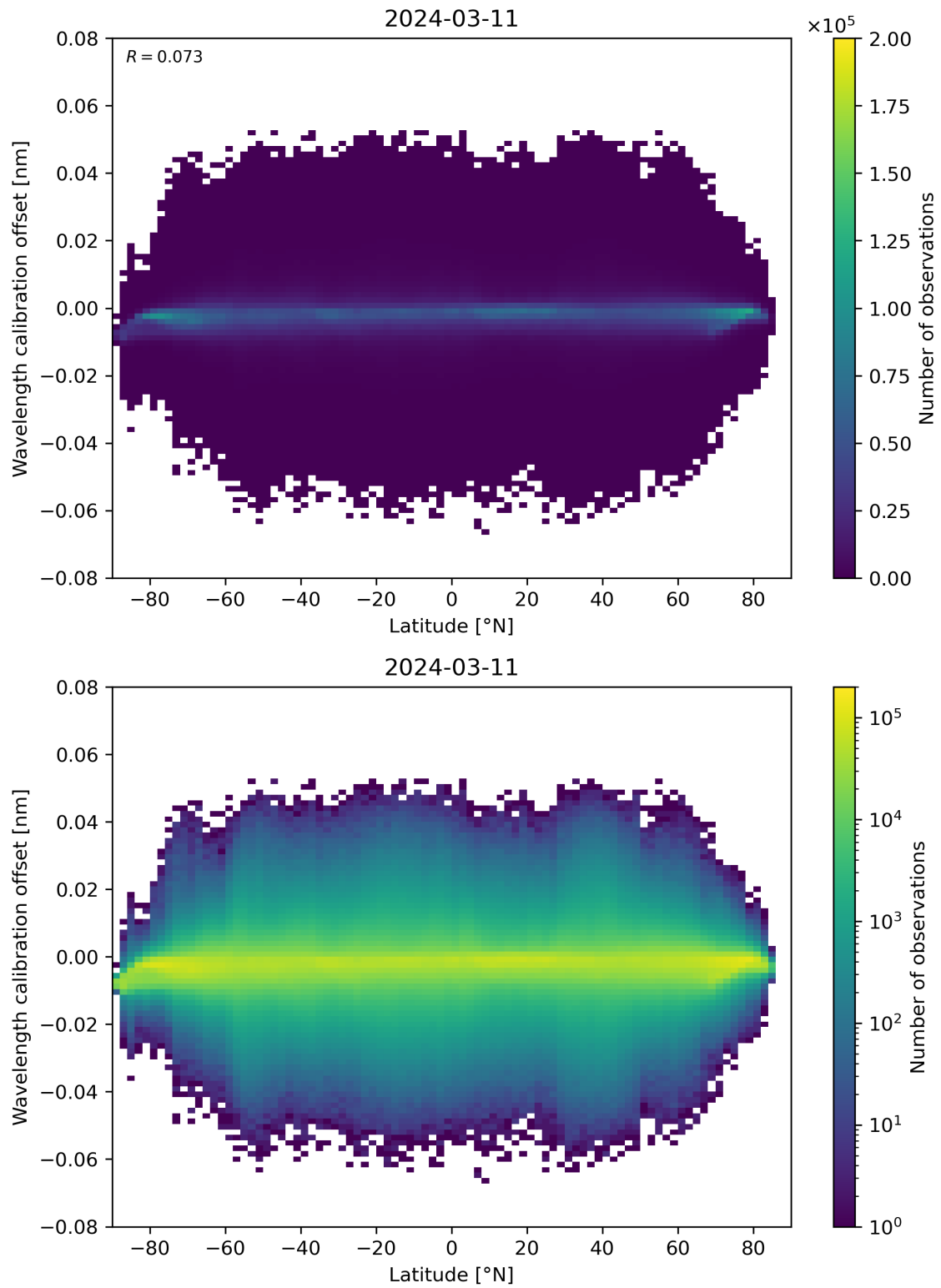
Figure 95: Scatter density plot of “Latitude” against “Wavelength calibration offset” for 2024-03-10 to 2024-03-12.
