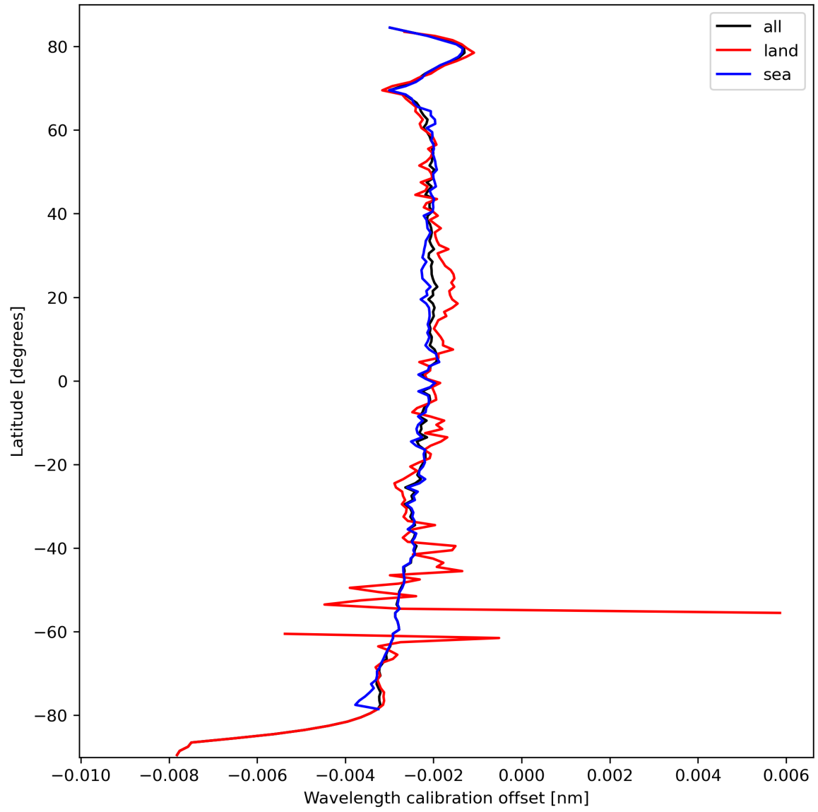
Figure 18: Zonal average of “Wavelength calibration offset” for 2024-03-10 to 2024-03-12.
