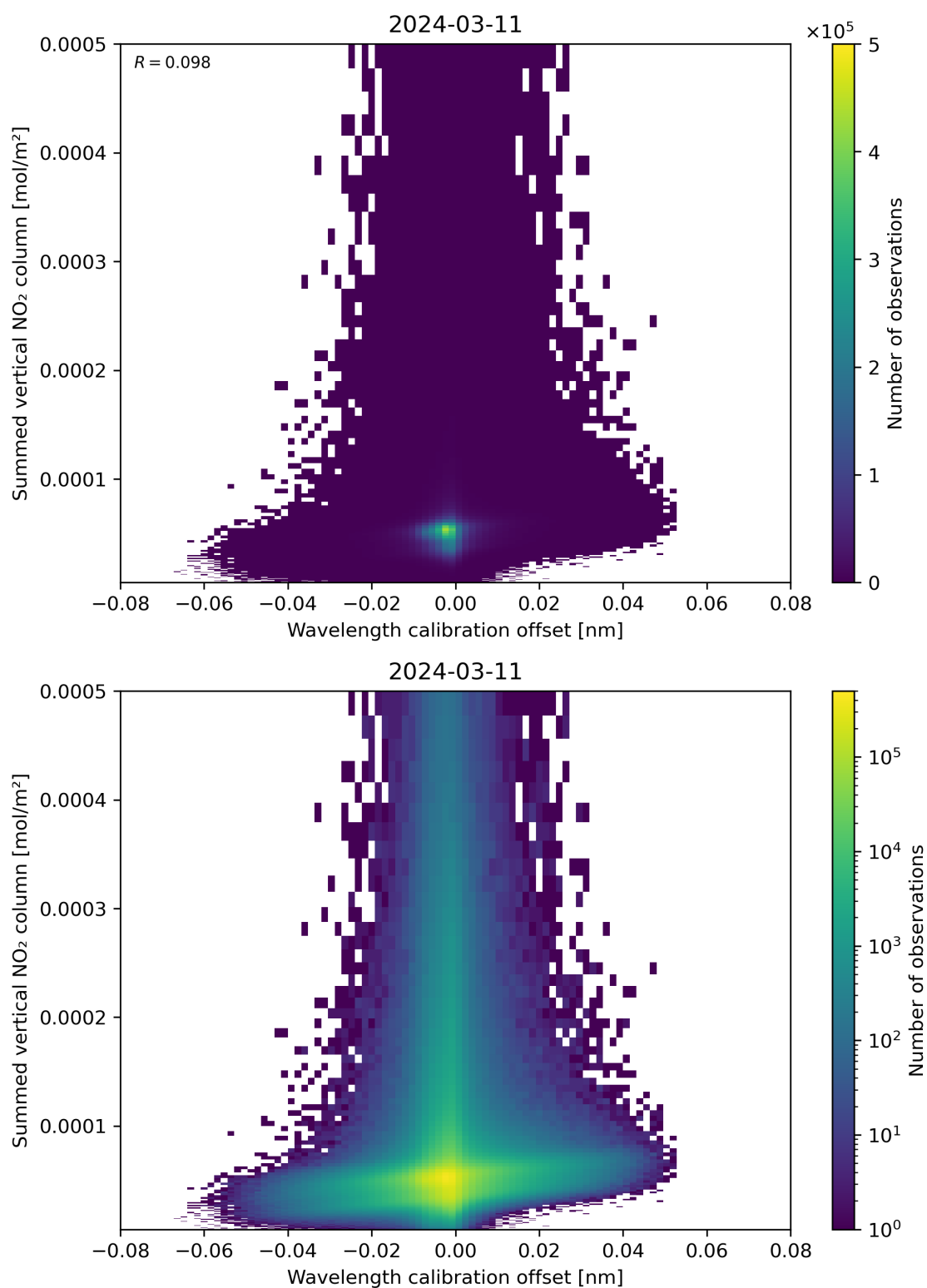
Figure 177: Scatter density plot of “Wavelength calibration offset” against “Summed vertical NO 2 column” for 2024-03-10 to 2024-03-12.
