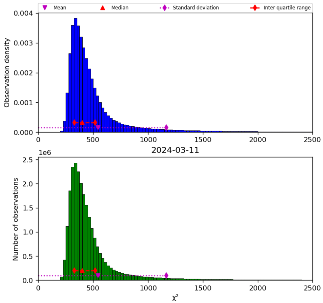
Figure 42: Histogram of “ \chi^2 ” for 2024-03-10 to 2024-03-12
