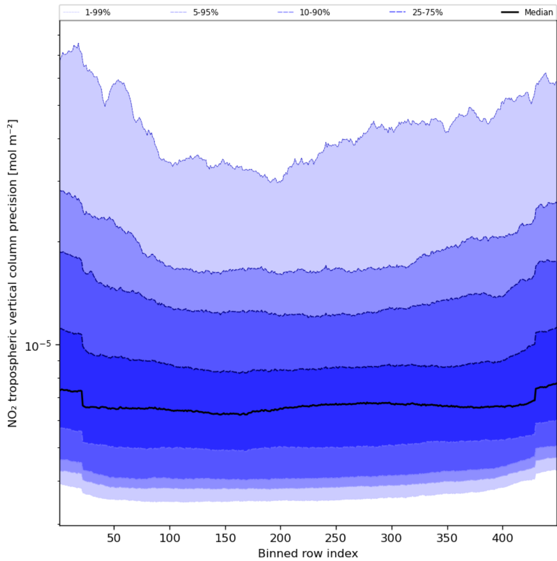
Figure 47: Along track statistics of “NO 2 tropospheric vertical column precision” for 2024-03-10 to 2024-03-12
