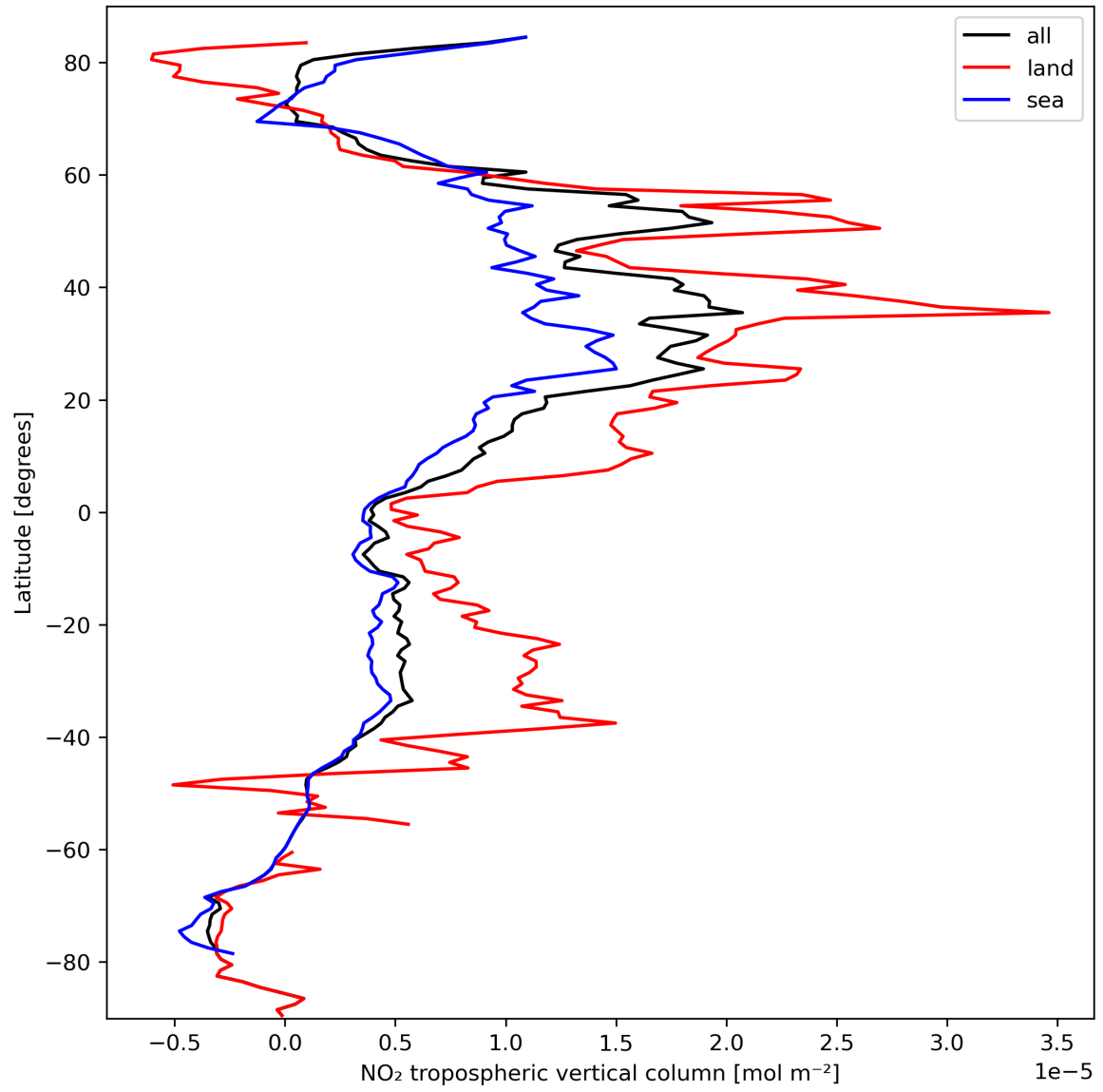
Figure 12: Zonal average of “NO 2 tropospheric vertical column” for 2024-03-10 to 2024-03-12.
