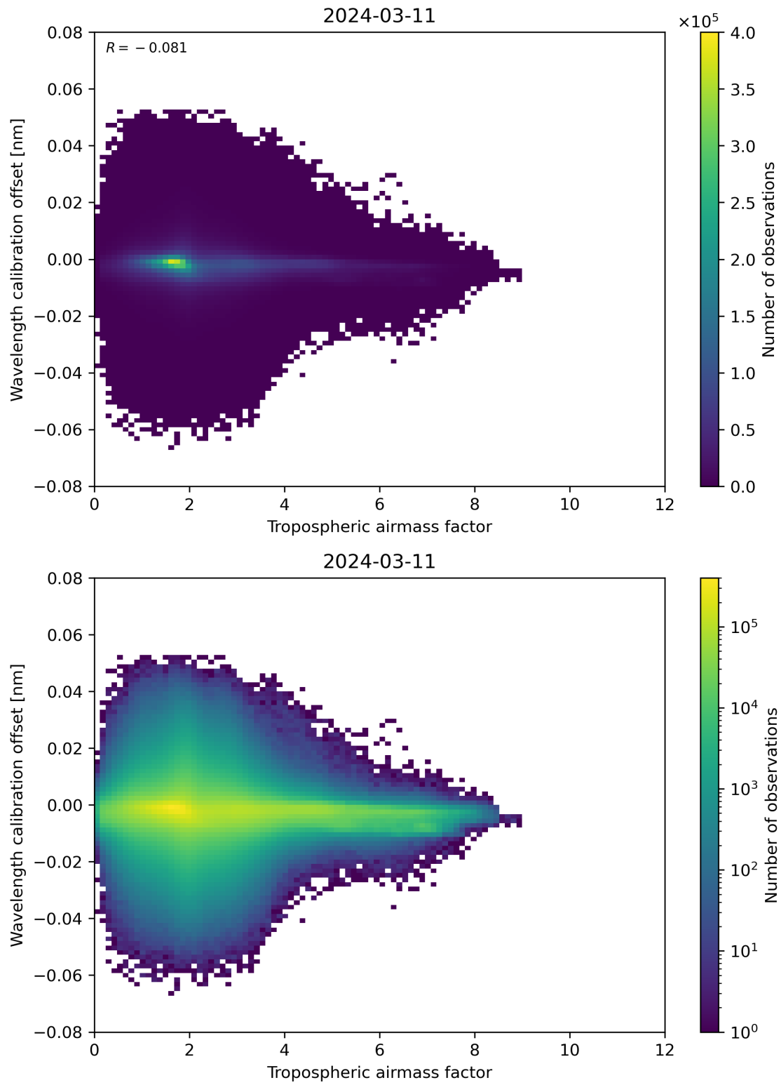
Figure 80: Scatter density plot of “Tropospheric airmass factor” against “Wavelength calibration offset” for 2024-03-10 to 2024-03-12.
