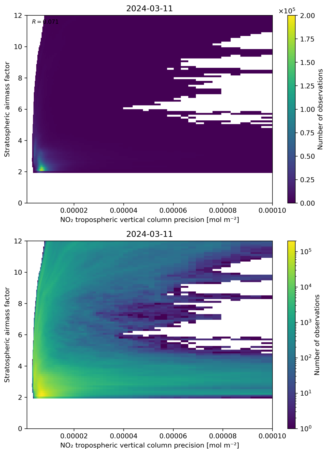
Figure 131: Scatter density plot of “NO 2 tropospheric vertical column precision” against “Stratospheric airmass factor” for 2024-03-10 to 2024-03-12.
