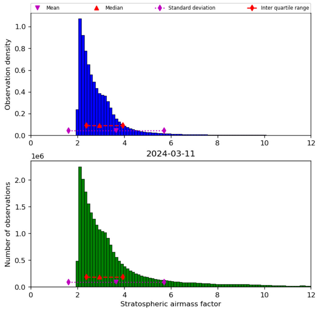
Figure 44: Histogram of “Stratospheric airmass factor” for 2024-03-10 to 2024-03-12
