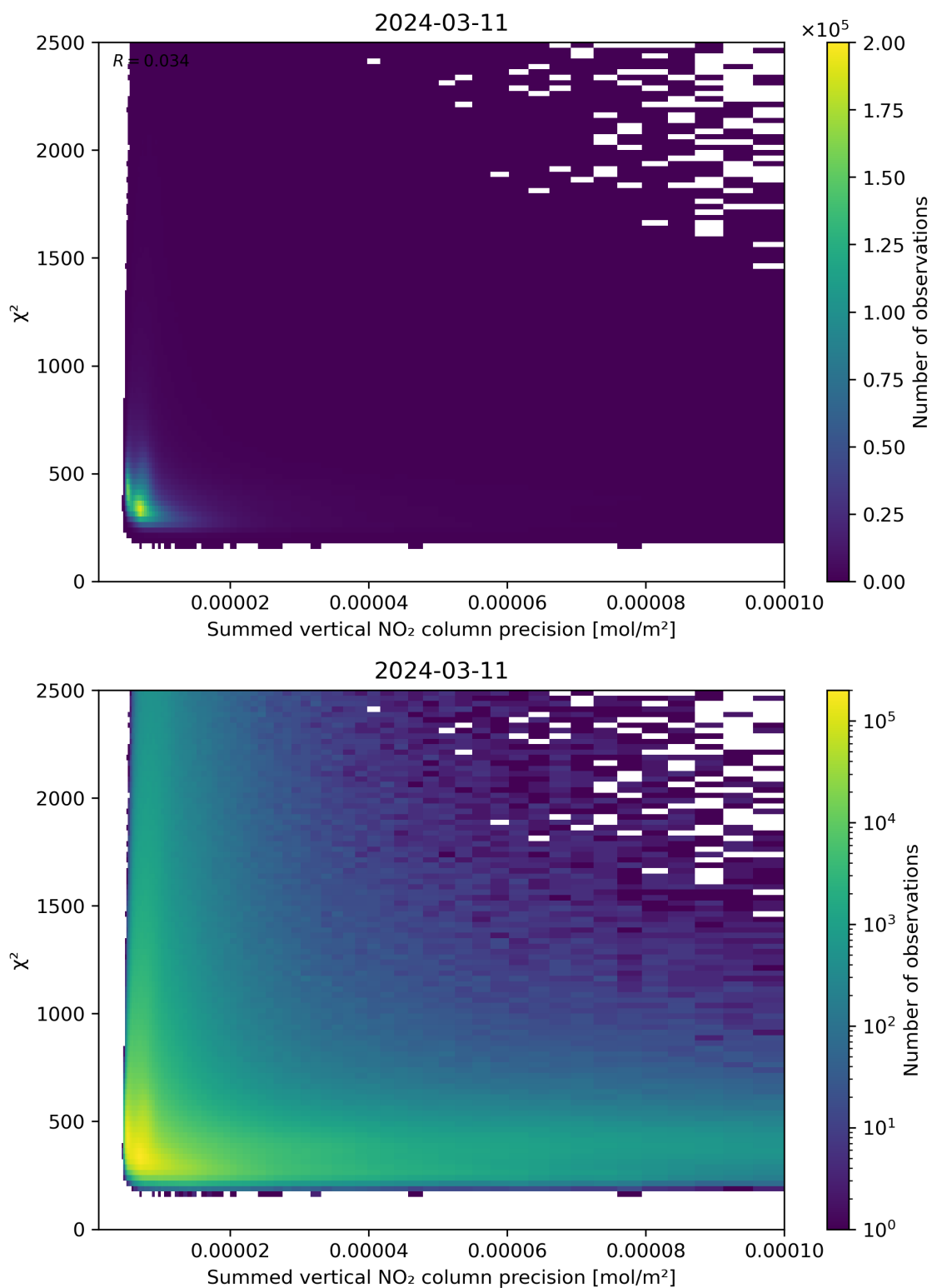
Figure 107: Scatter density plot of “Summed vertical NO 2 column precision” against “ \chi^2 ” for 2024-03-10 to 2024-03-12.
