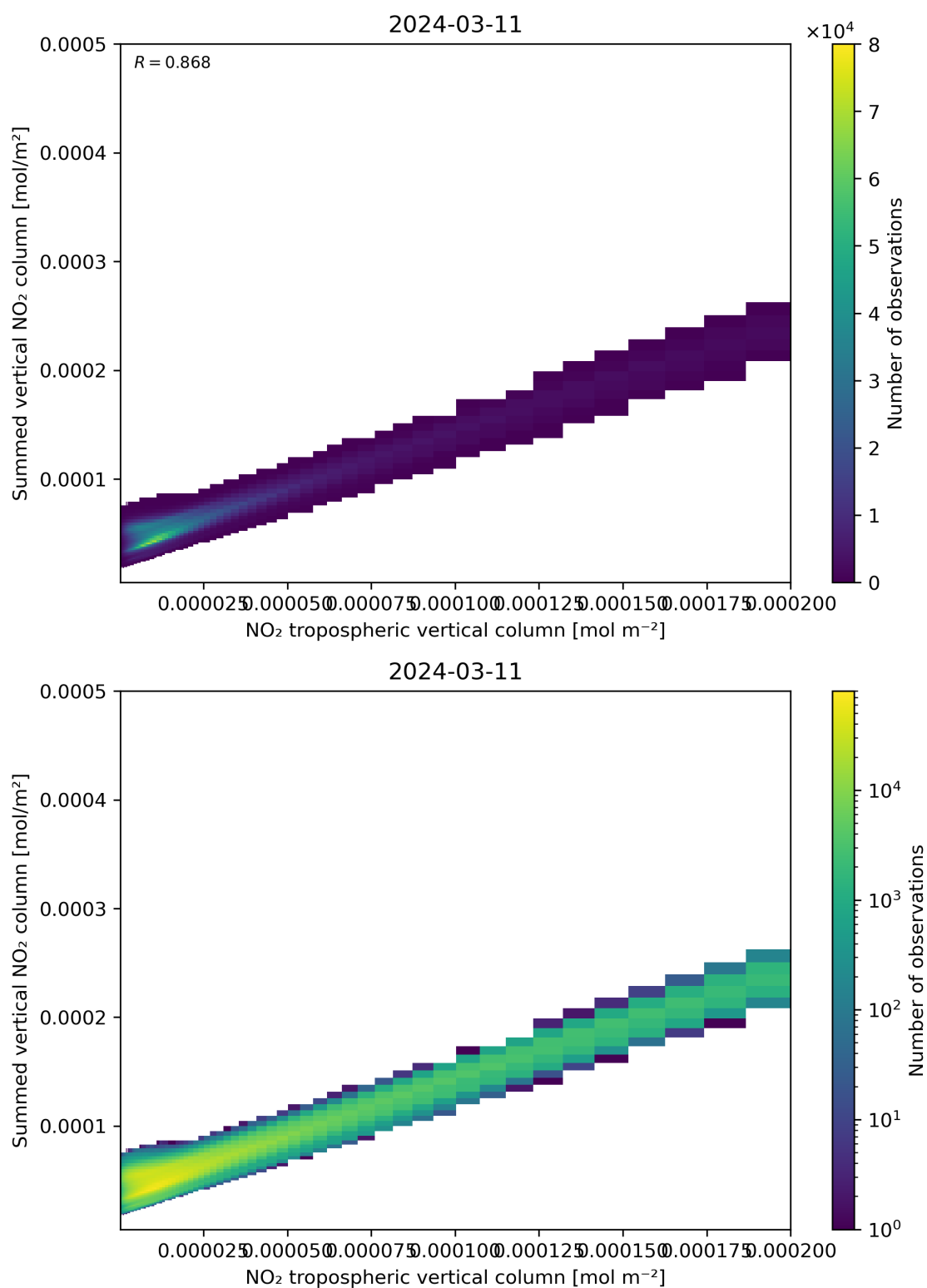
Figure 126: Scatter density plot of “NO 2 tropospheric vertical column” against “Summed vertical NO 2 column” for 2024-03-10 to 2024-03-12.
