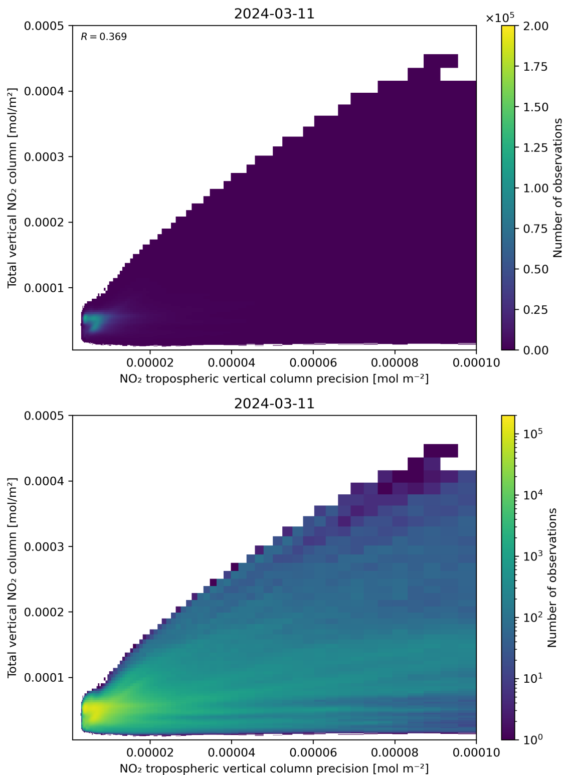
Figure 138: Scatter density plot of “NO 2 tropospheric vertical column precision” against “Total vertical NO 2 column” for 2024-03-10 to 2024-03-12.
