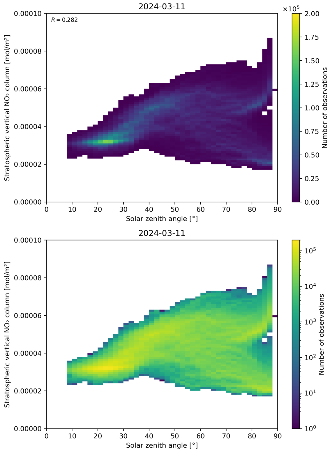
Figure 150: Scatter density plot of “Solar zenith angle” against “Stratospheric vertical NO 2 column” for 2024-03-10 to 2024-03-12.
