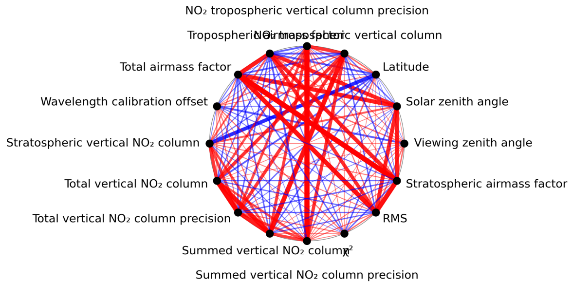
Figure 1: Map of correlation graph for 2024-03-10 to 2024-03-12.
