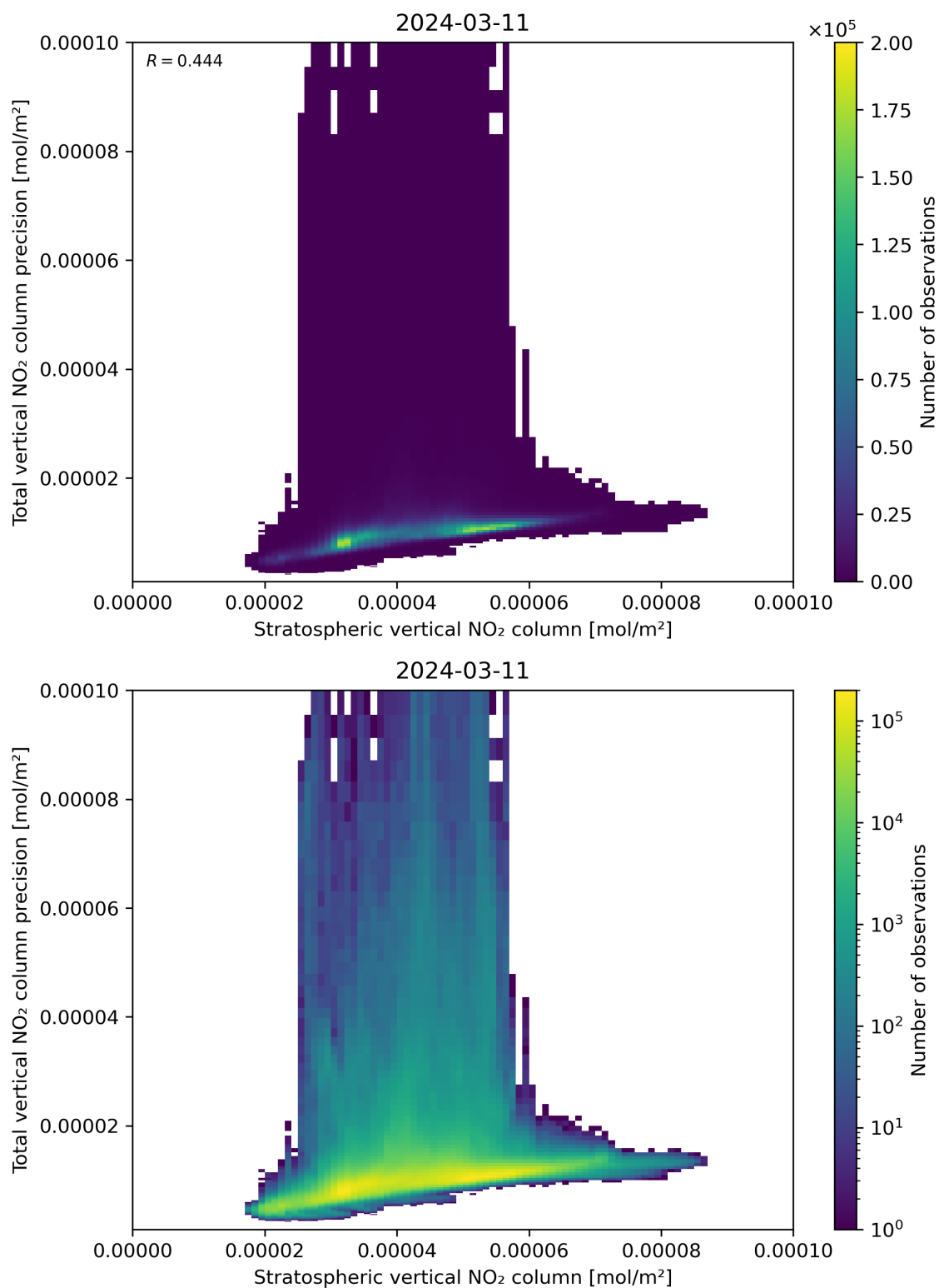
Figure 101: Scatter density plot of “Stratospheric vertical NO 2 column” against “Total vertical NO 2 column precision” for 2024-03-10 to 2024-03-12.
