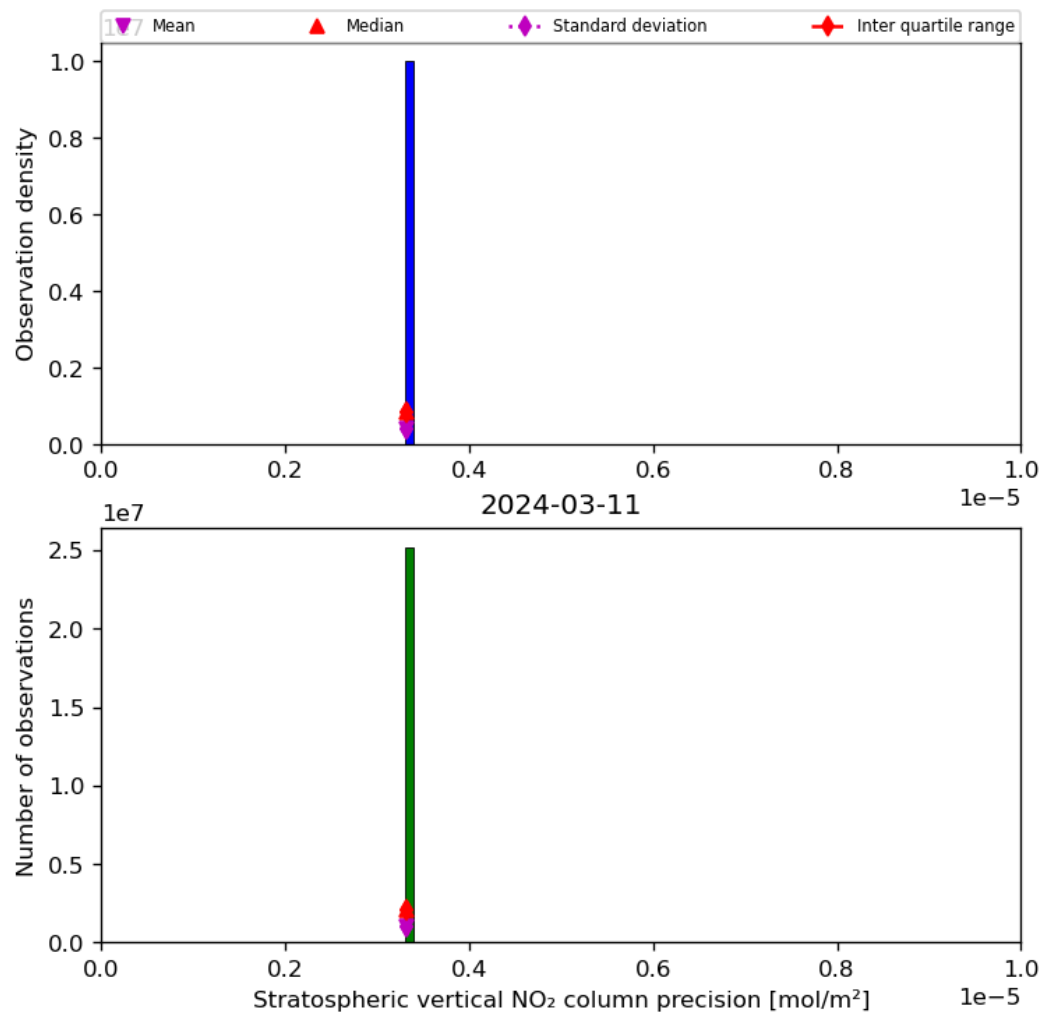
Figure 37: Histogram of “Stratospheric vertical NO 2 column precision” for 2024-03-10 to 2024-03-12
