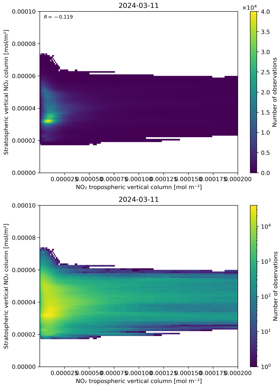
Figure 125: Scatter density plot of “NO 2 tropospheric vertical column” against “Stratospheric vertical NO 2 column” for 2024-03-10 to 2024-03-12.
