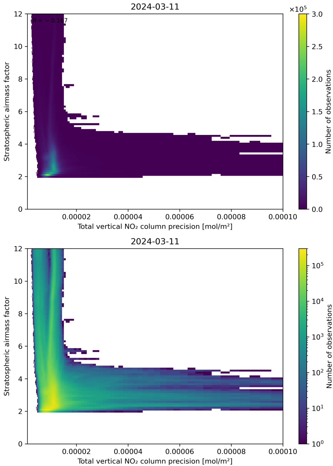
Figure 115: Scatter density plot of “Total vertical NO 2 column precision” against “Stratospheric airmass factor” for 2024-03-10 to 2024-03-12.
