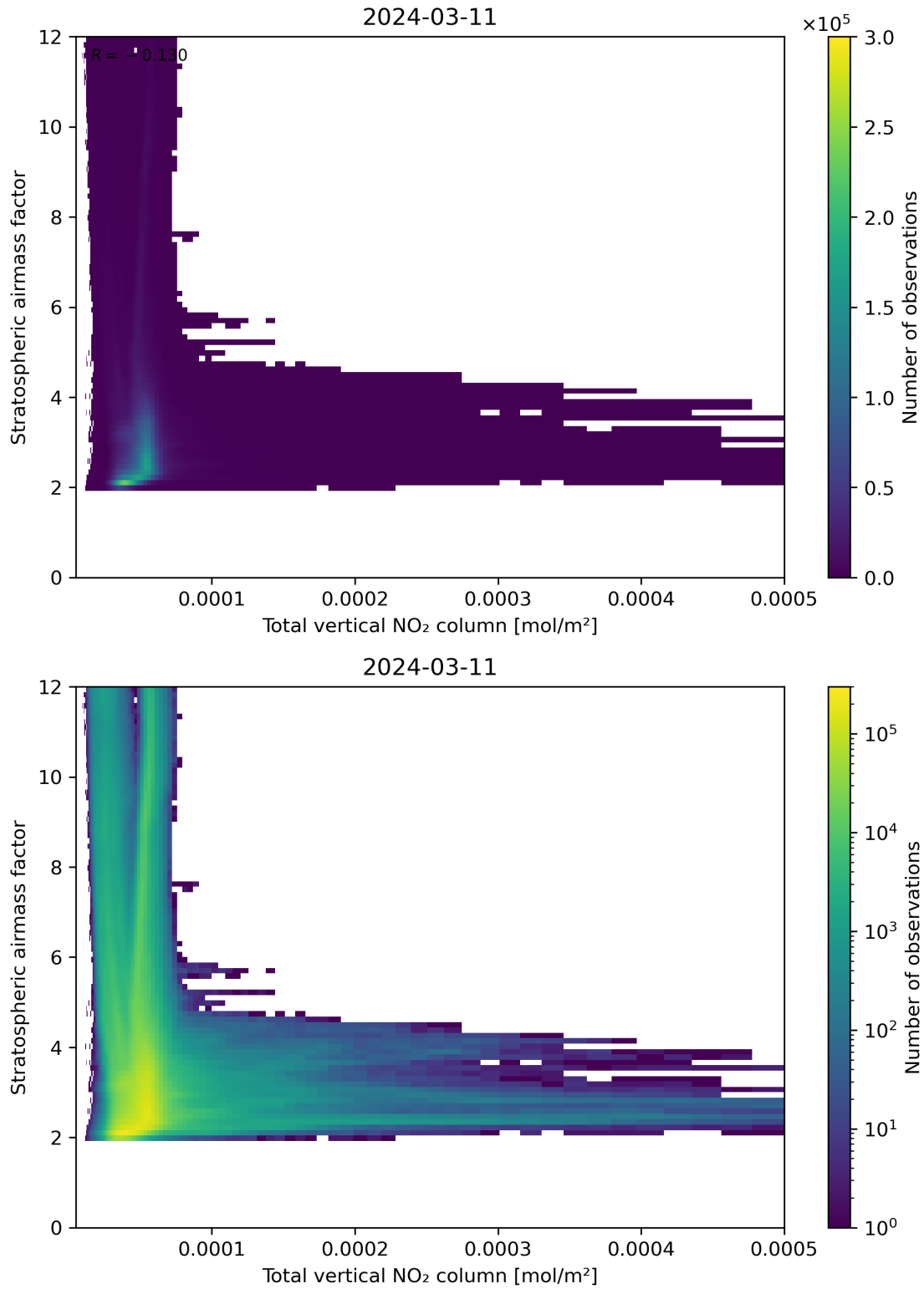
Figure 110: Scatter density plot of “Total vertical NO 2 column” against “Stratospheric airmass factor” for 2024-03-10 to 2024-03-12.
