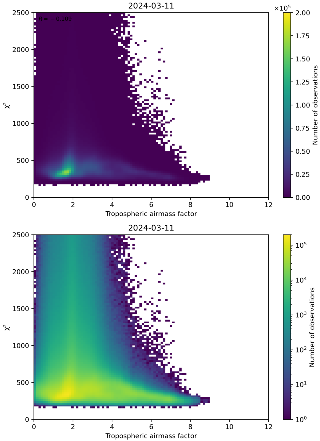
Figure 73: Scatter density plot of “Tropospheric airmass factor” against “ \chi^2 ” for 2024-03-10 to 2024-03-12.
