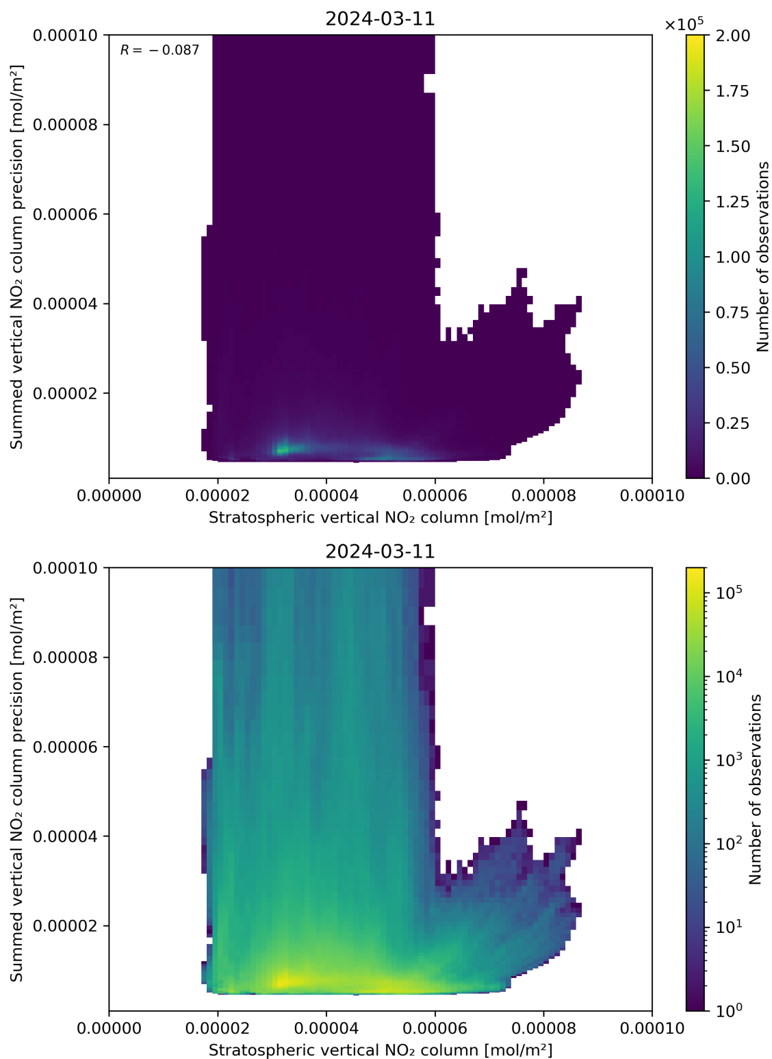
Figure 99: Scatter density plot of “Stratospheric vertical NO 2 column” against “Summed vertical NO 2 column precision” for 2024-03-10 to 2024-03-12.
