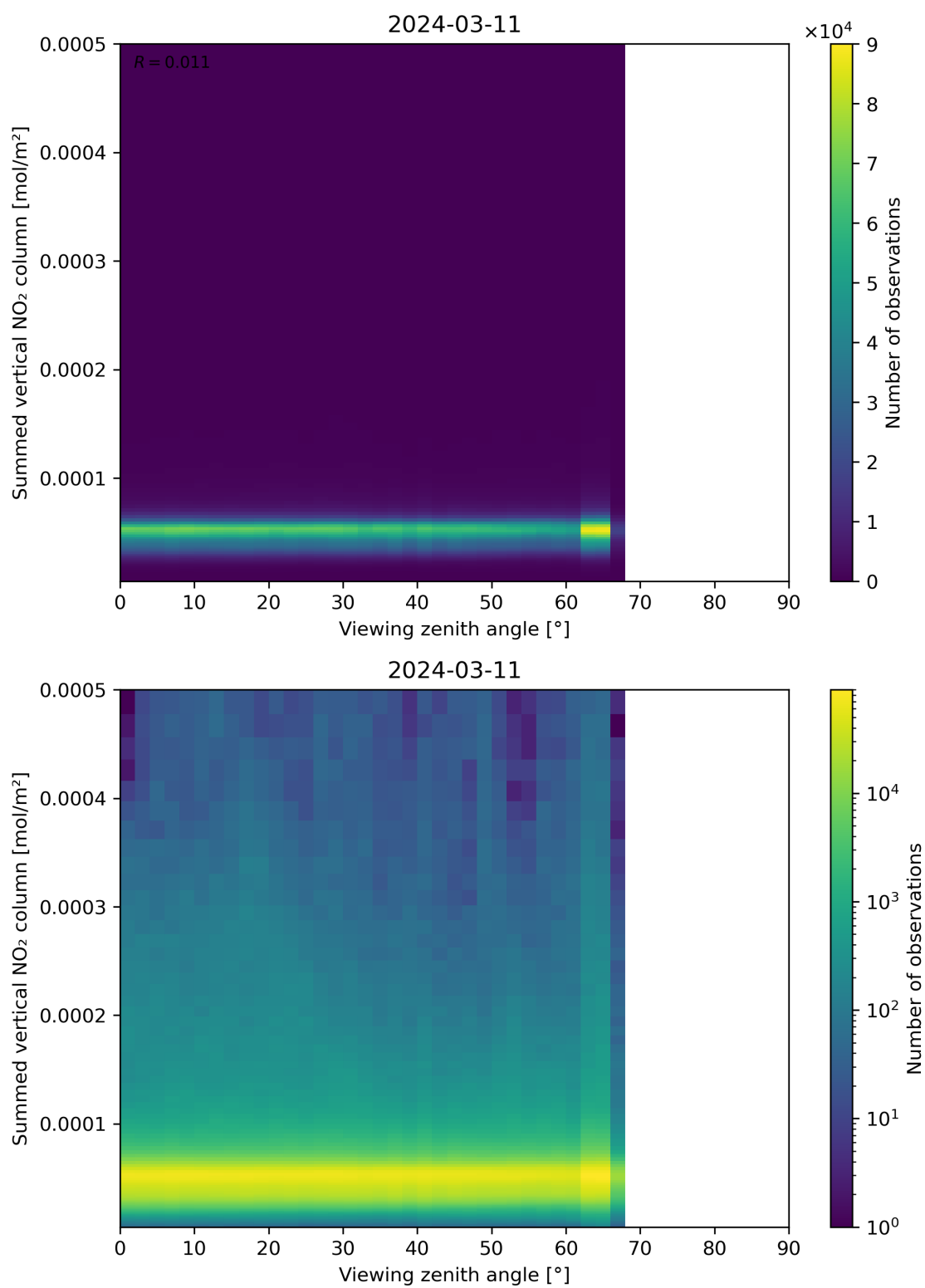
Figure 165: Scatter density plot of “Viewing zenith angle” against “Summed vertical NO 2 column” for 2024-03-10 to 2024-03-12.
