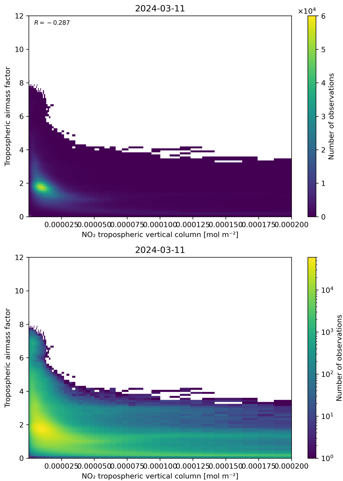
Figure 123: Scatter density plot of “NO 2 tropospheric vertical column” against “Tropospheric airmass factor” for 2024-03-10 to 2024-03-12.
