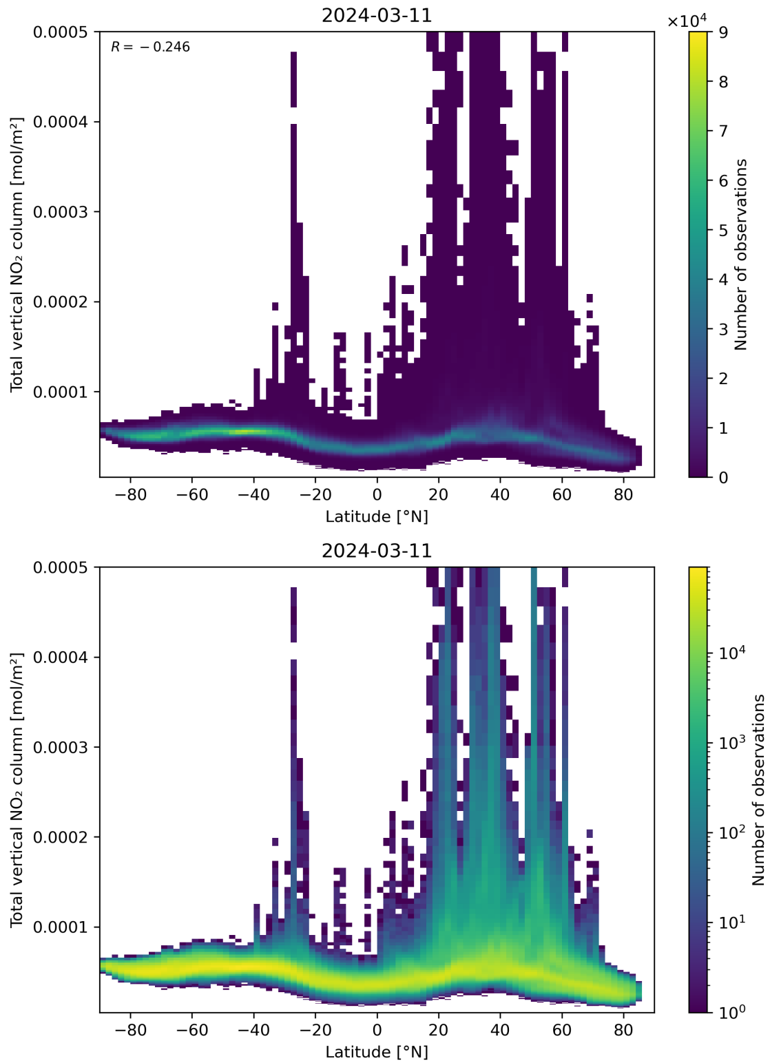
Figure 90: Scatter density plot of “Latitude” against “Total vertical NO 2 column” for 2024-03-10 to 2024-03-12.
