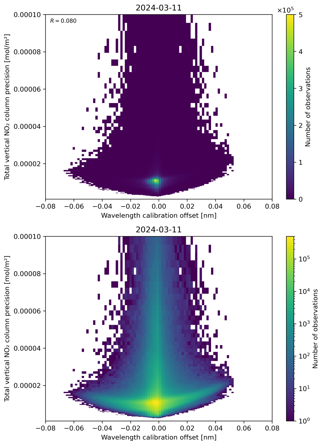
Figure 180: Scatter density plot of “Wavelength calibration offset” against “Total vertical NO 2 column precision” for 2024-03-10 to 2024-03-12.
