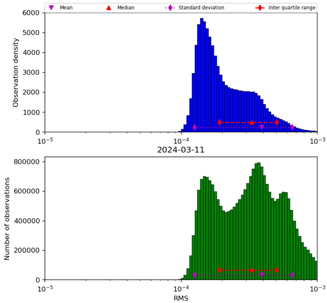
Figure 43: Histogram of “RMS” for 2024-03-10 to 2024-03-12
