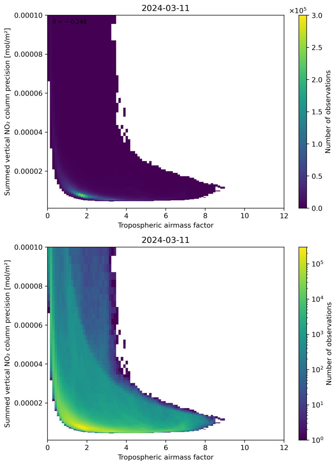
Figure 76: Scatter density plot of “Tropospheric air mass factor” against “Summed vertical NO 2 column precision” for 2024-03-10 to 2024-03-12.
