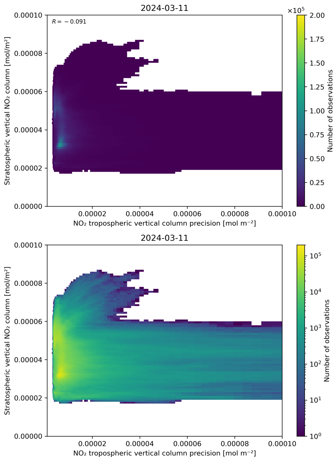
Figure 135: Scatter density plot of “NO 2 tropospheric vertical column precision” against “Stratospheric vertical NO 2 column” for 2024-03-10 to 2024-03-12.
