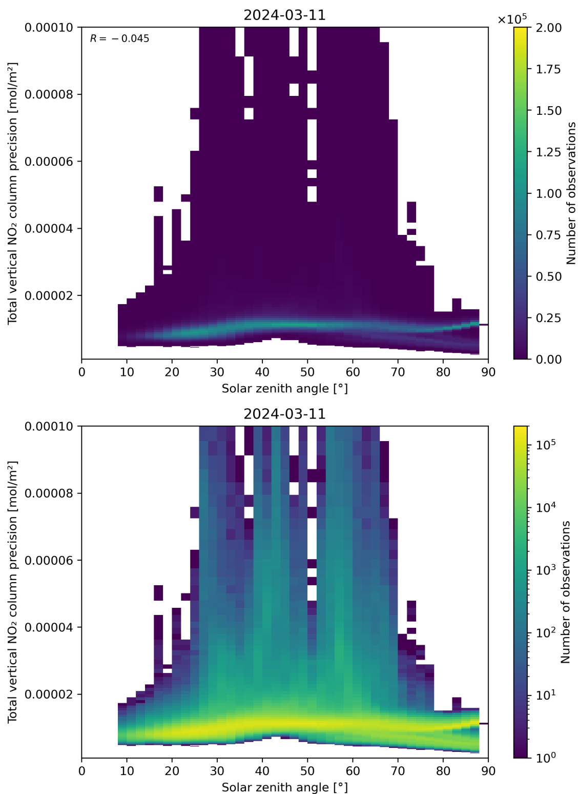
Figure 154: Scatter density plot of “Solar zenith angle” against “Total vertical NO 2 column precision” for 2024-03-10 to 2024-03-12.
