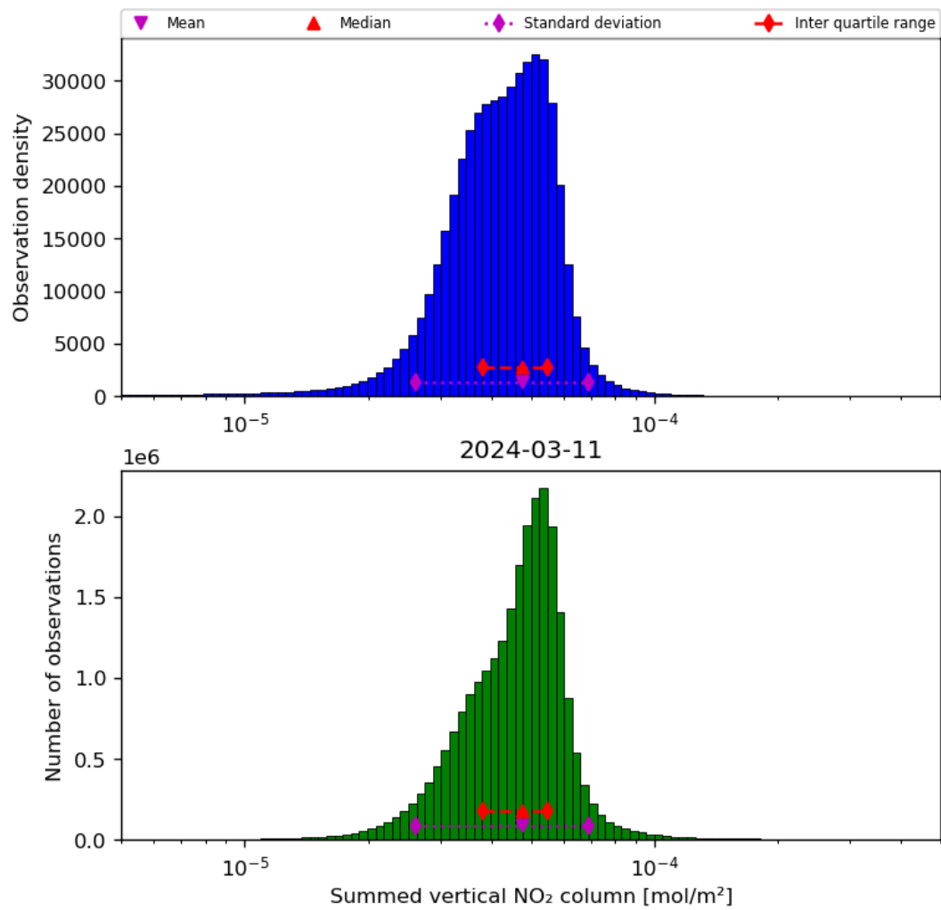
Figure 40: Histogram of “Summed vertical NO 2 column” for 2024-03-10 to 2024-03-12
