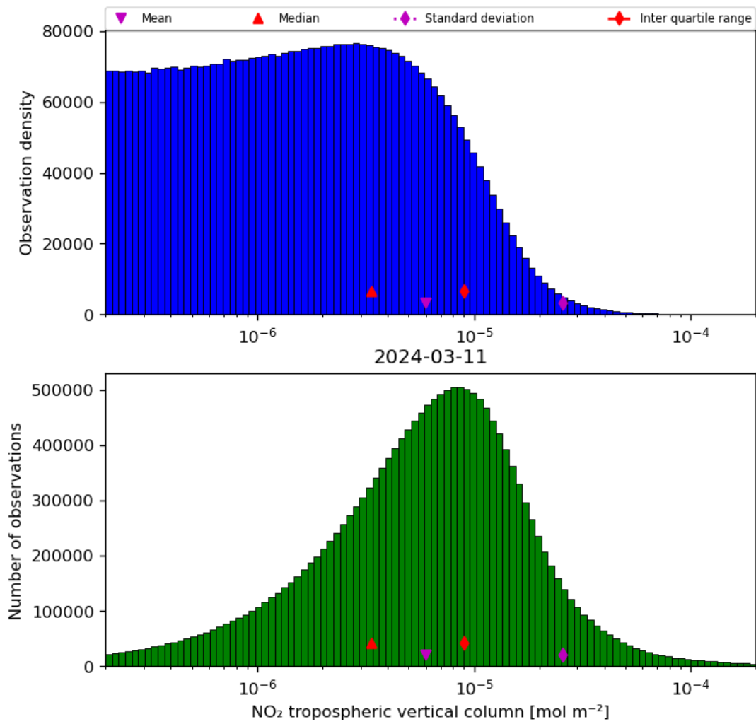
Figure 29: Histogram of “NO 2 tropospheric vertical column” for 2024-03-10 to 2024-03-12
