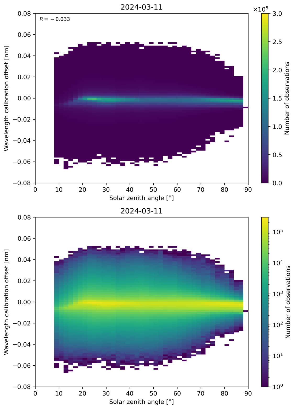
Figure 158: Scatter density plot of “Solar zenith angle” against “Wavelength calibration offset” for 2024-03-10 to 2024-03-12.
