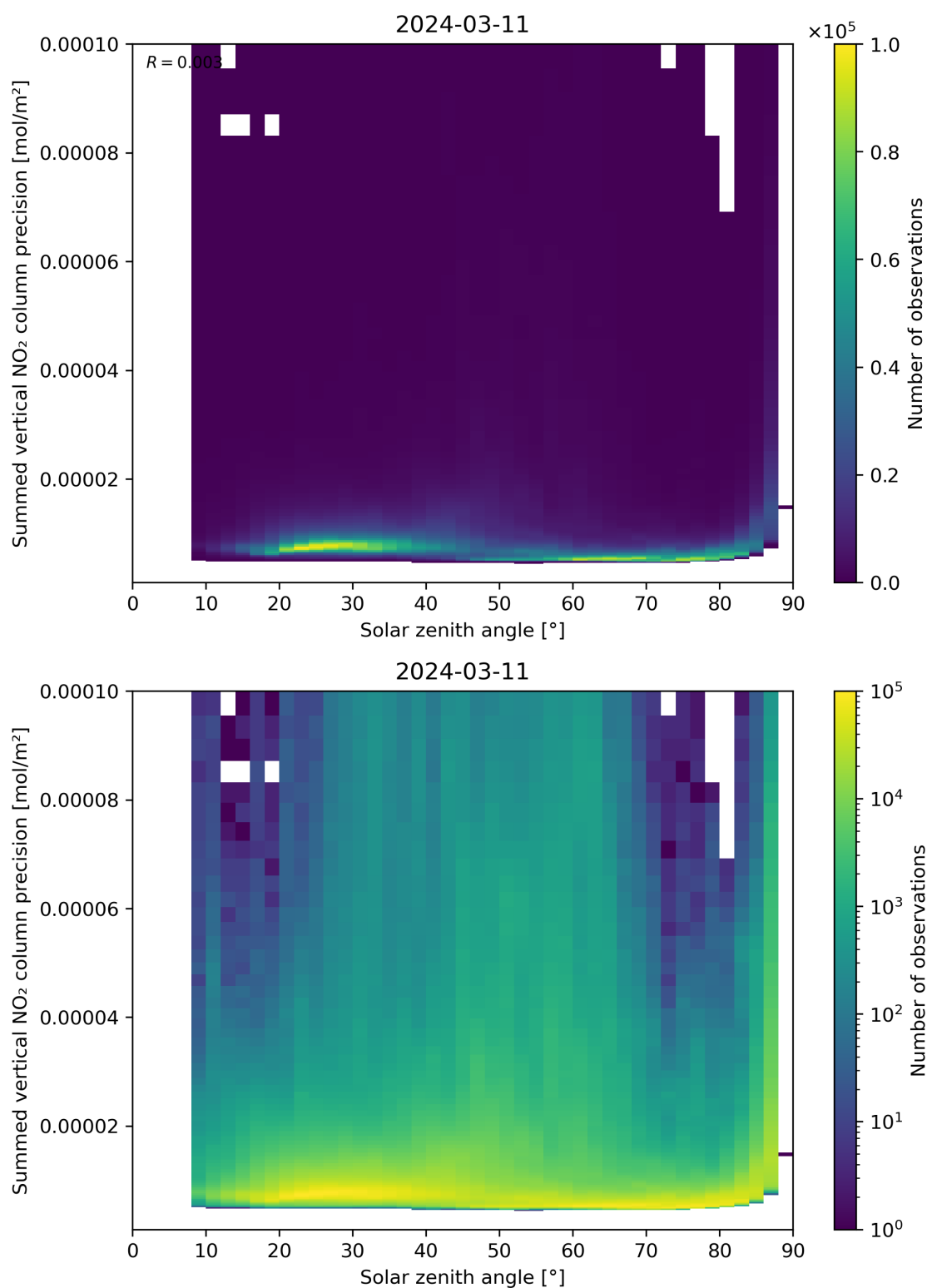
Figure 152: Scatter density plot of “Solar zenith angle” against “Summed vertical NO 2 column precision” for 2024-03-10 to 2024-03-12.
