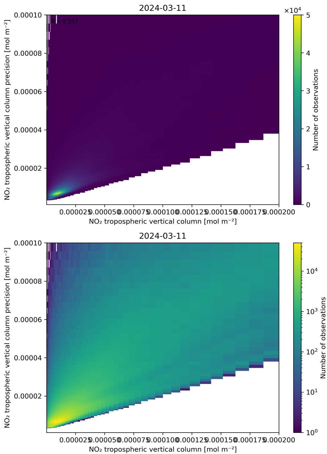
Figure 130: Scatter density plot of “NO 2 tropospheric vertical column” against “NO 2 tropospheric vertical column precision” for 2024-03-10 to 2024-03-12.
