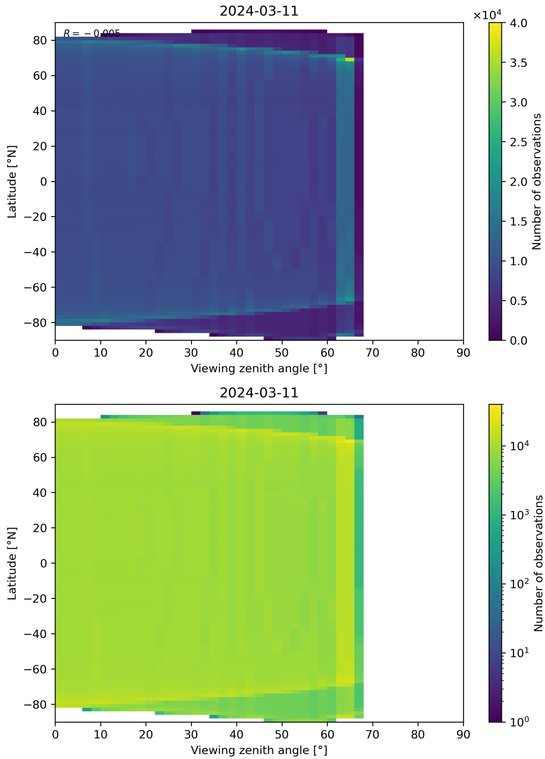
Figure 163: Scatter density plot of “Viewing zenith angle” against “Latitude” for 2024-03-10 to 2024-03-12.
