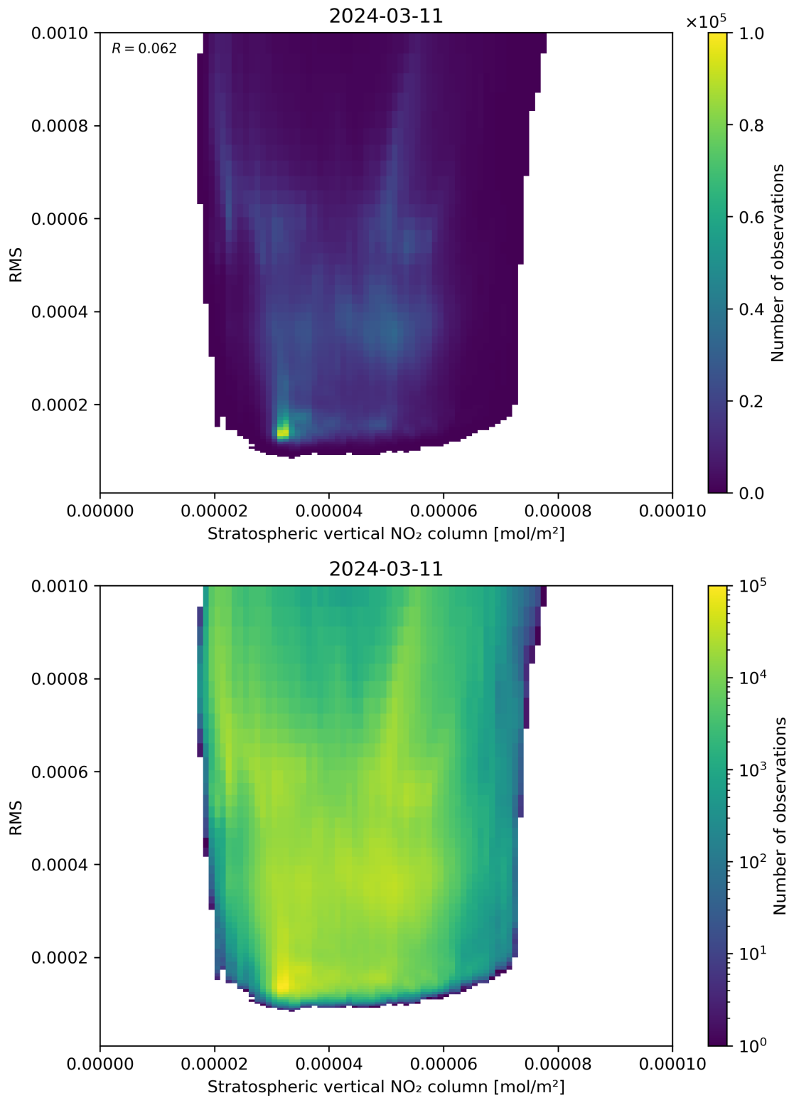
Figure 102: Scatter density plot of “Stratospheric vertical NO 2 column” against “RMS” for 2024-03-10 to 2024-03-12.
