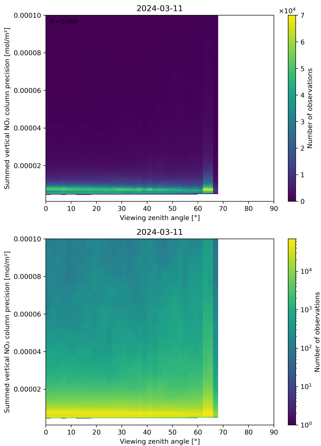
Figure 166: Scatter density plot of “Viewing zenith angle” against “Summed vertical NO 2 column precision” for 2024-03-10 to 2024-03-12.
