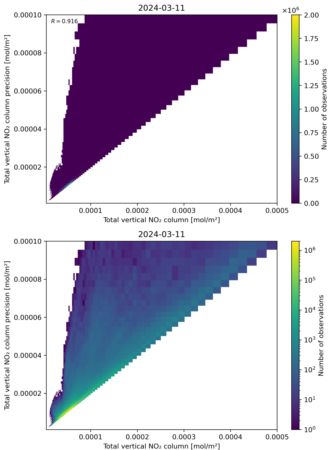
Figure 114: Scatter density plot of “Total vertical NO 2 column” against “Total vertical NO 2 column precision” for 2024-03-10 to 2024-03-12.
