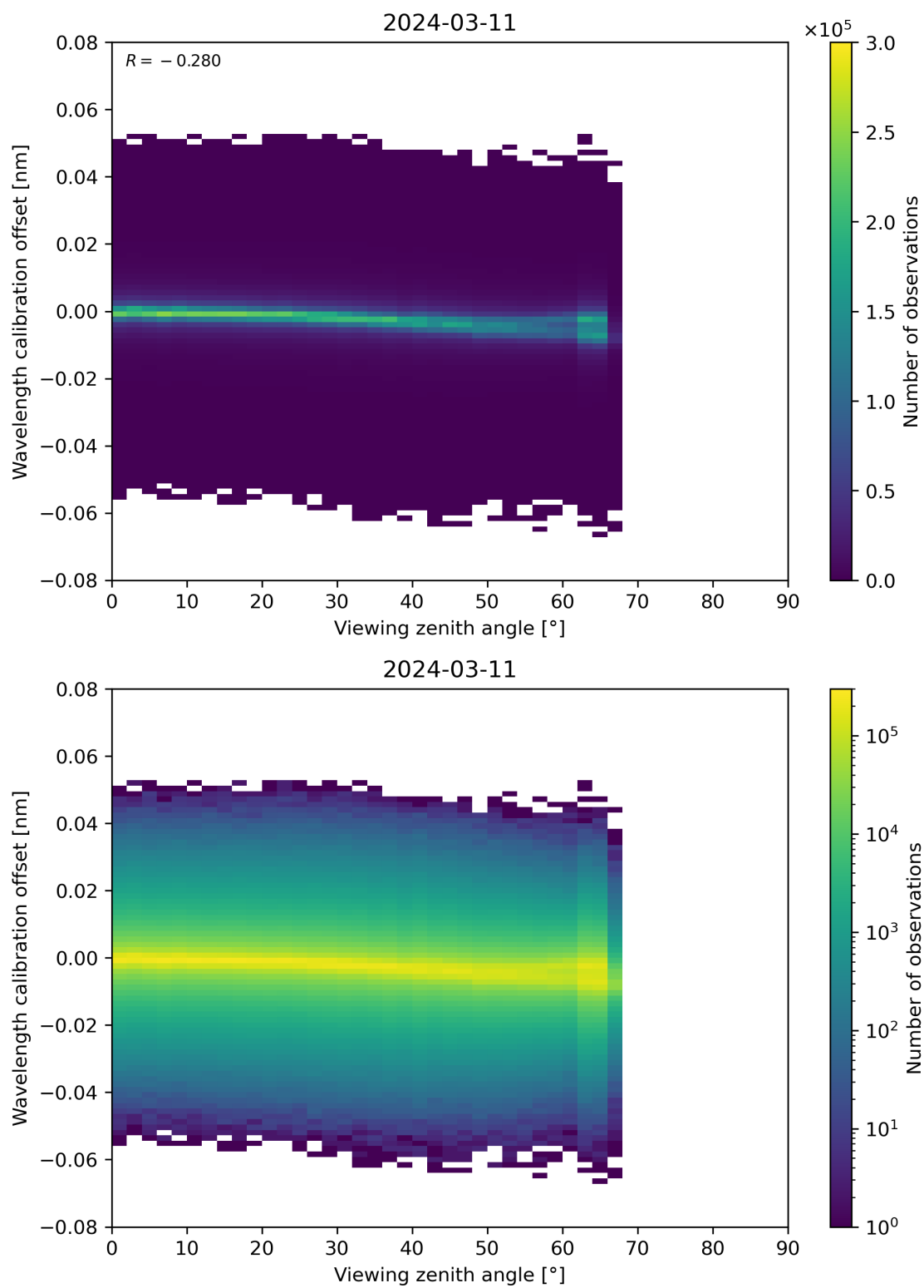
Figure 173: Scatter density plot of “Viewing zenith angle” against “Wavelength calibration offset” for 2024-03-10 to 2024-03-12.
