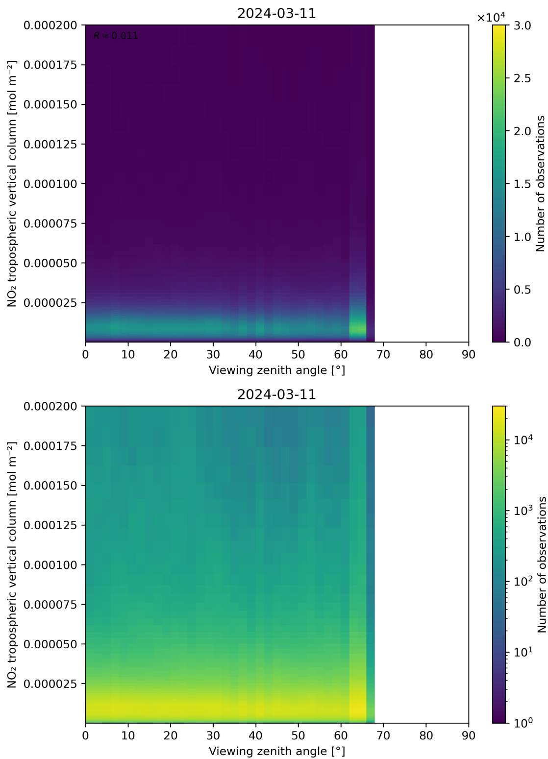
Figure 169: Scatter density plot of “Viewing zenith angle” against “NO 2 tropospheric vertical column” for 2024-03-10 to 2024-03-12.
