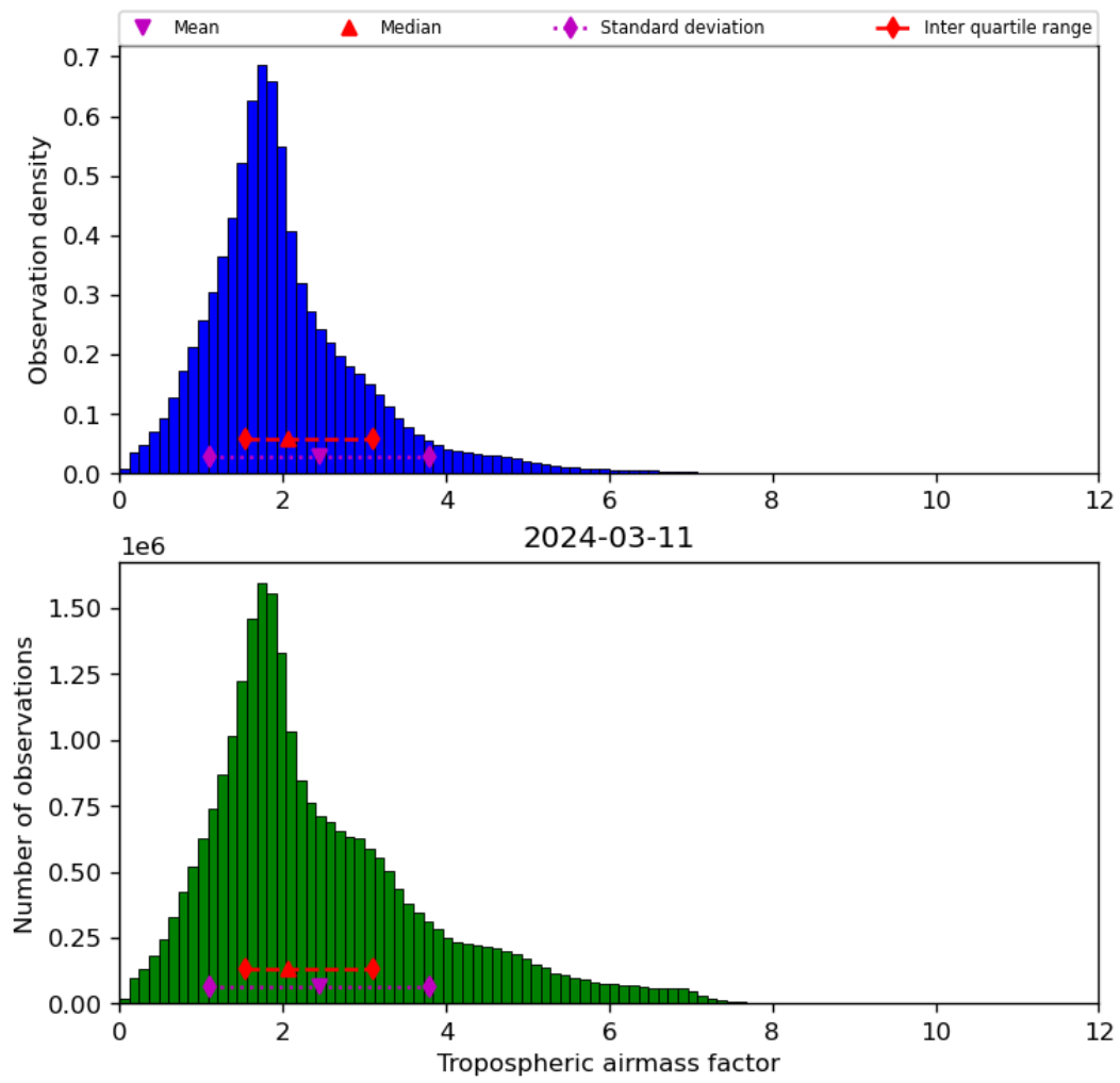
Figure 31: Histogram of “Tropospheric airmass factor” for 2024-03-10 to 2024-03-12
