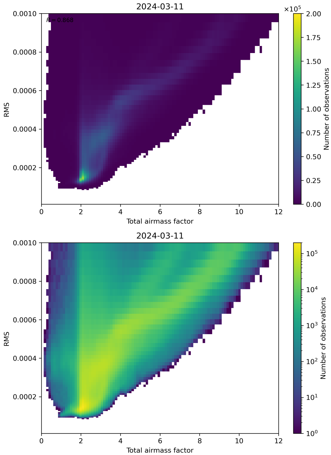
Figure 69: Scatter density plot of “Total airmass factor” against “RMS” for 2024-03-10 to 2024-03-12.
