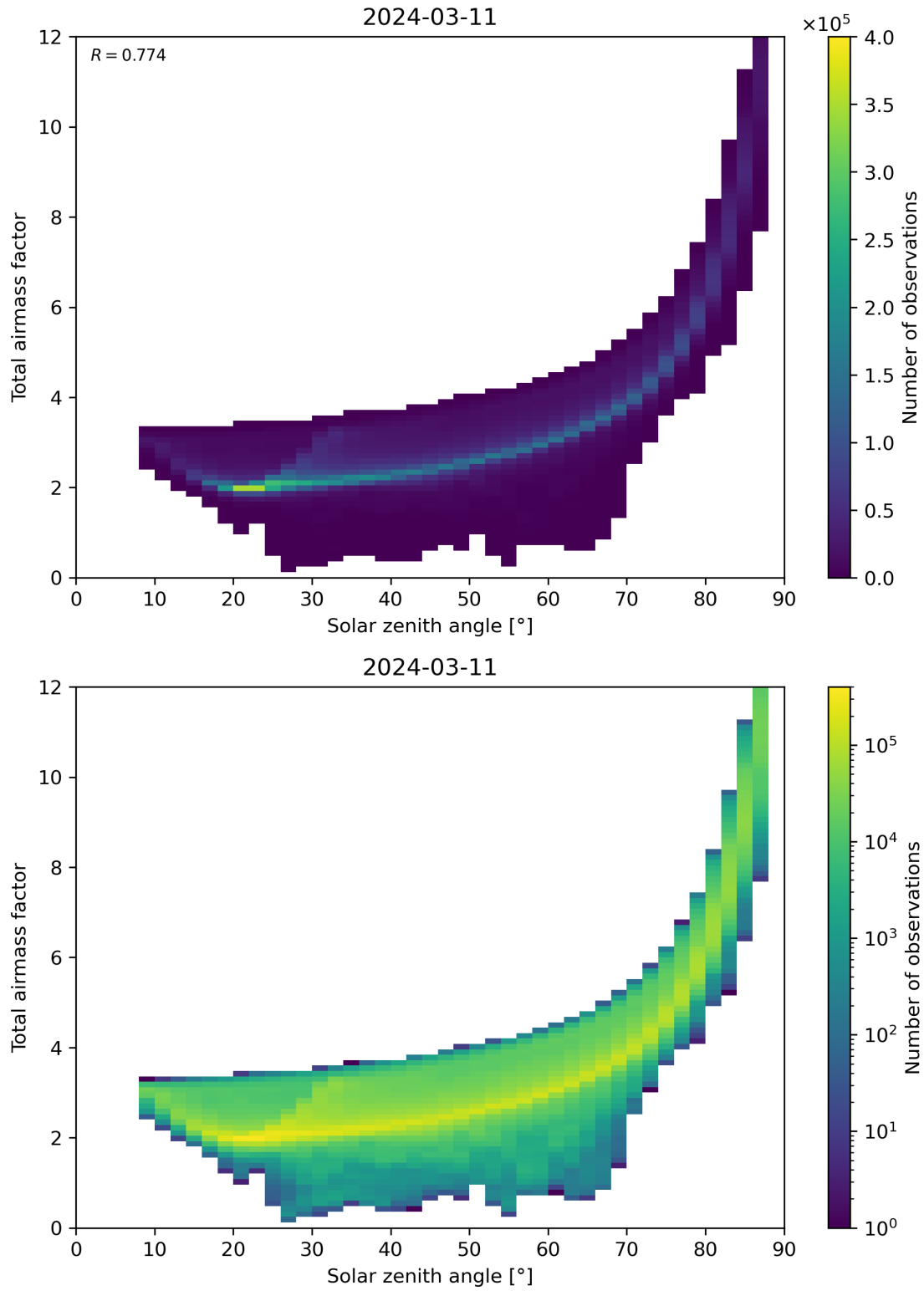
Figure 146: Scatter density plot of “Solar zenith angle” against “Total air mass factor” for 2024-03-10 to 2024-03-12.
