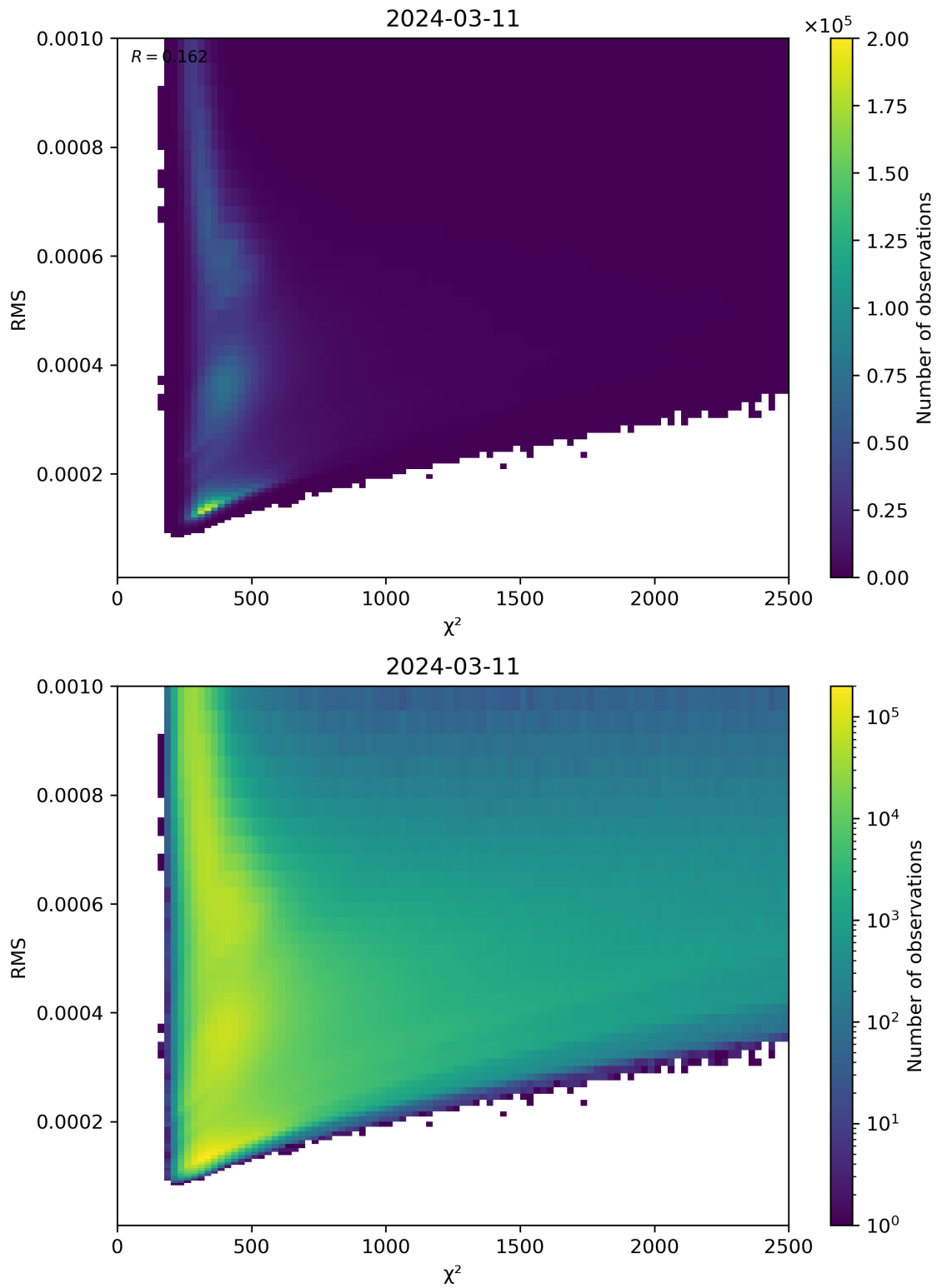
Figure 82: Scatter density plot of “ \chi^2 ” against “RMS” for 2024-03-10 to 2024-03-12.
