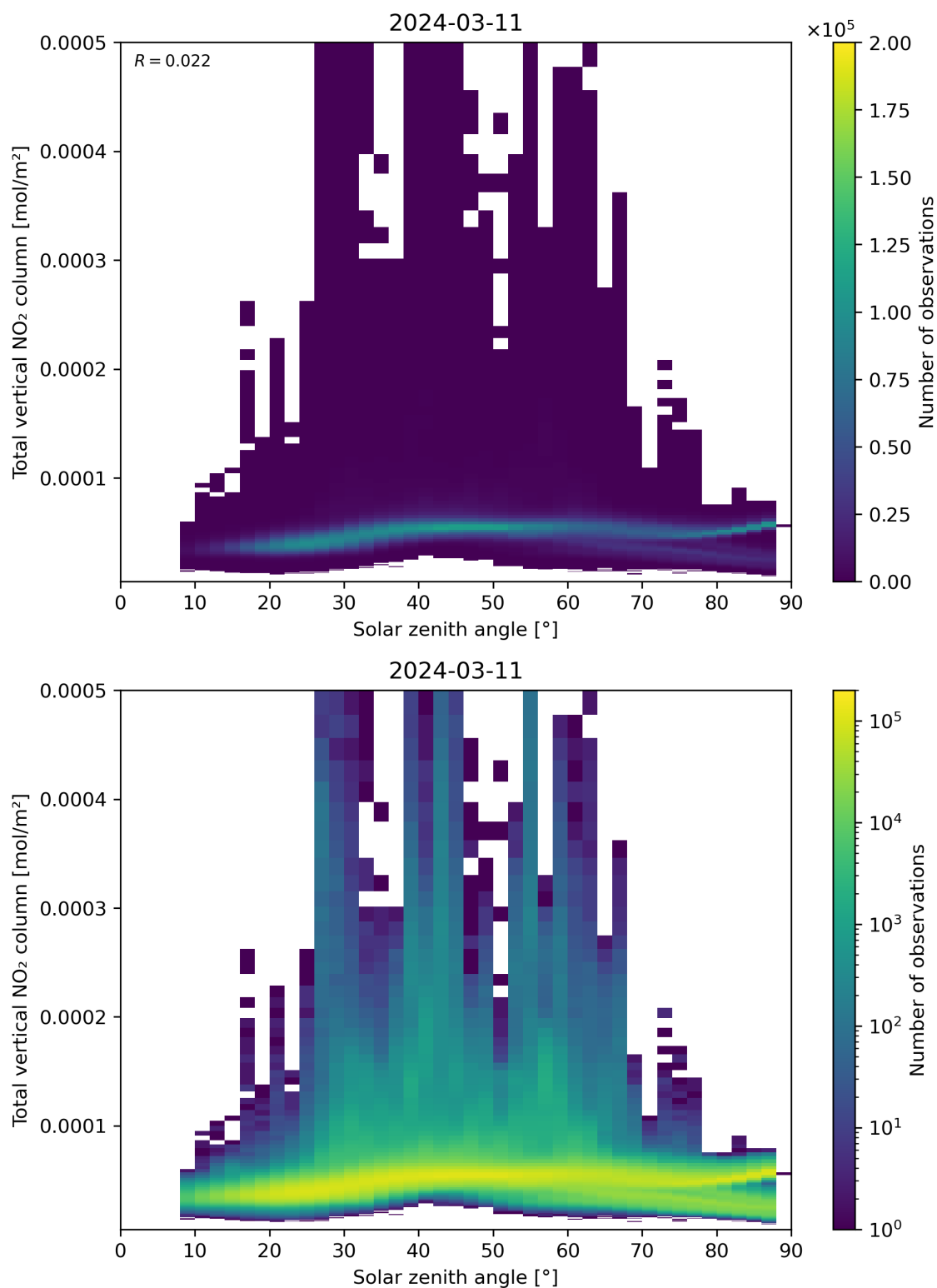
Figure 153: Scatter density plot of “Solar zenith angle” against “Total vertical NO 2 column” for 2024-03-10 to 2024-03-12.
