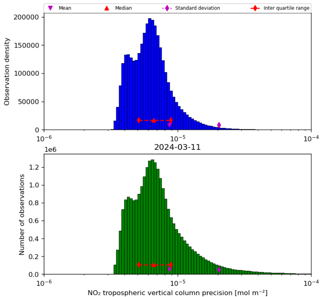
Figure 30: Histogram of “NO 2 tropospheric vertical column precision” for 2024-03-10 to 2024-03-12
