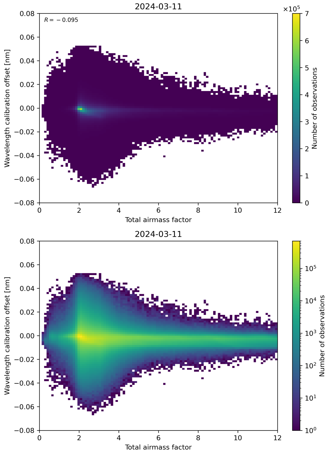
Figure 70: Scatter density plot of “Total airmass factor” against “Wavelength calibration offset” for 2024-03-10 to 2024-03-12.
