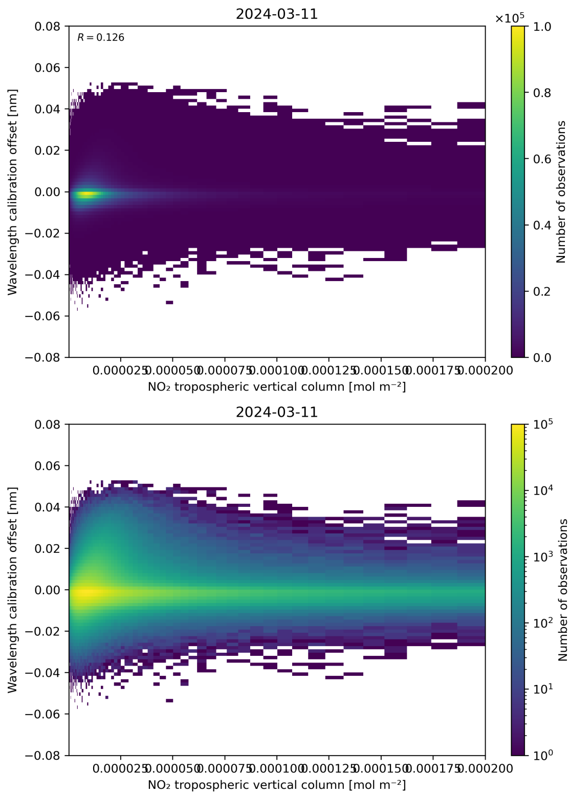
Figure 143: Scatter density plot of “NO 2 tropospheric vertical column” against “Wavelength calibration offset” for 2024-03-10 to 2024-03-12.
