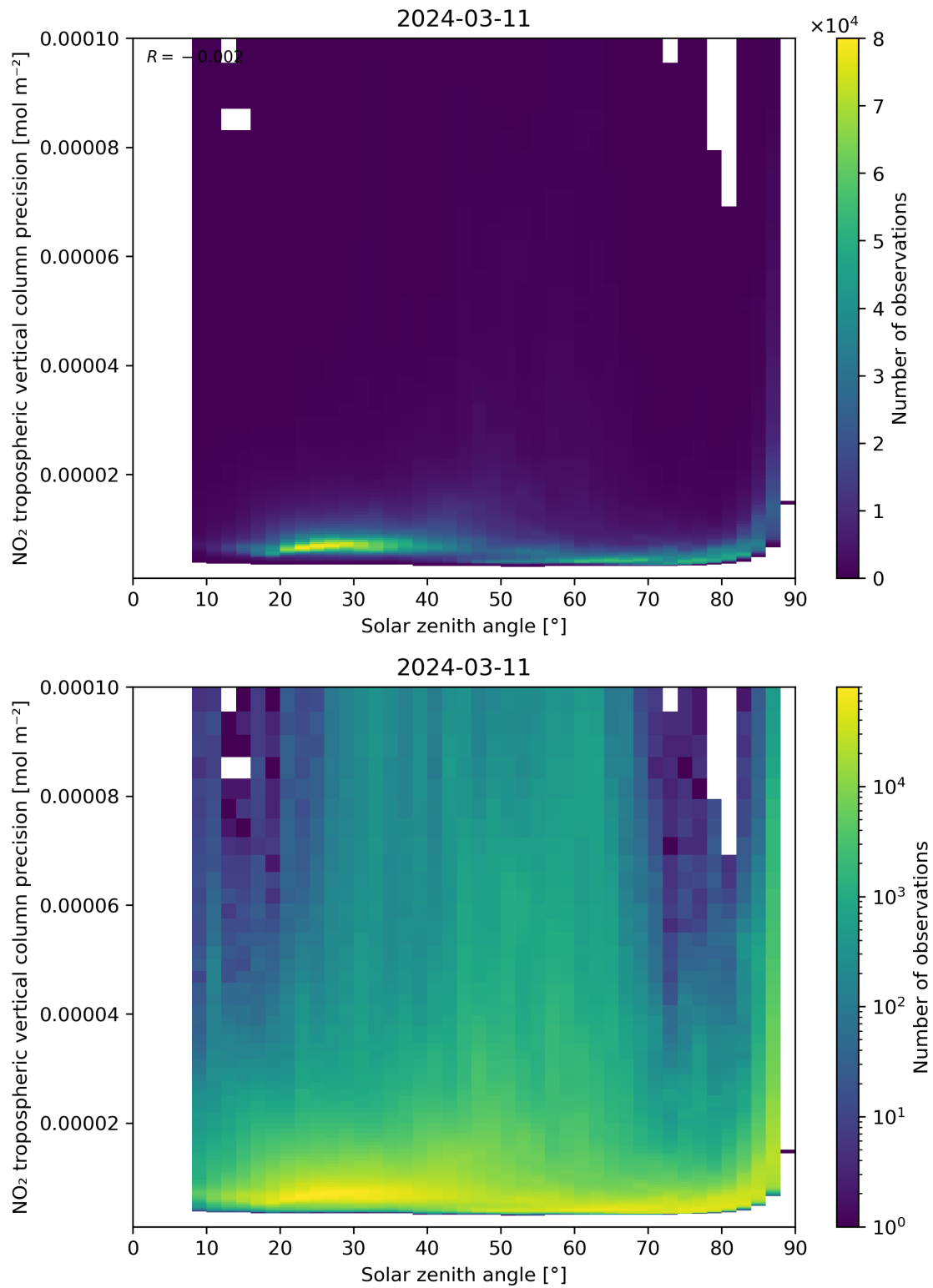
Figure 156: Scatter density plot of “Solar zenith angle” against “NO 2 tropospheric vertical column precision” for 2024-03-10 to 2024-03-12.
