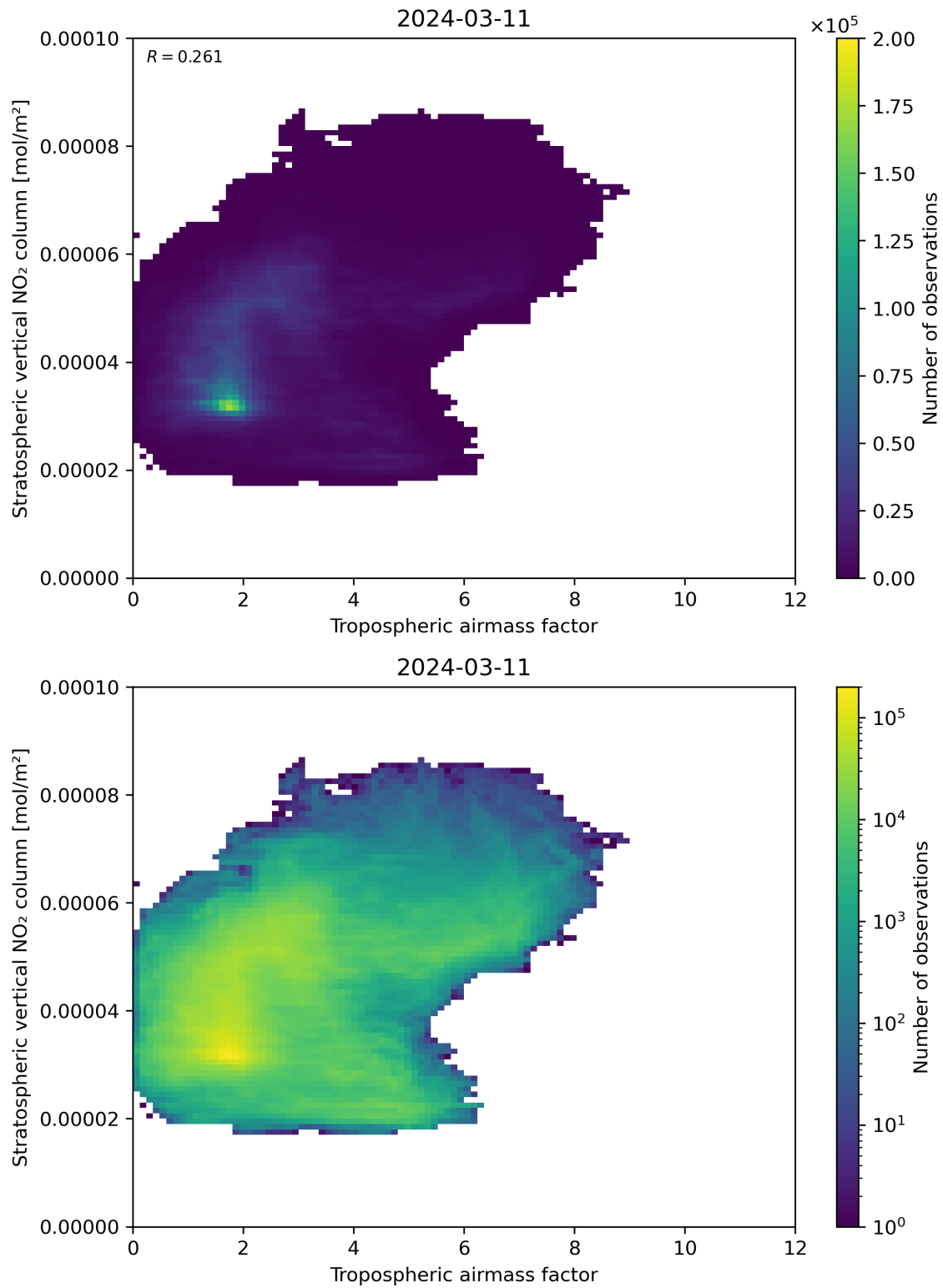
Figure 74: Scatter density plot of “Tropospheric air mass factor” against “Stratospheric vertical NO 2 column” for 2024-03-10 to 2024-03-12.
