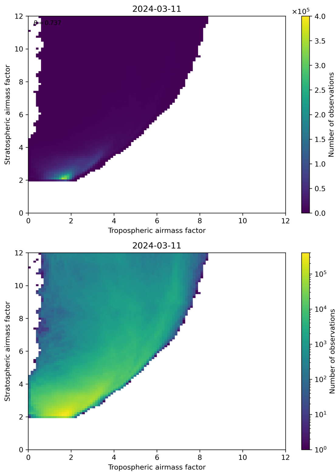
Figure 71: Scatter density plot of “Tropospheric airmass factor” against “Stratospheric airmass factor” for 2024-03-10 to 2024-03-12.
