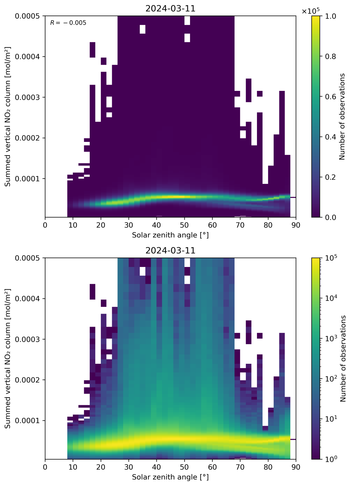
Figure 151: Scatter density plot of “Solar zenith angle” against “Summed vertical NO 2 column” for 2024-03-10 to 2024-03-12.
