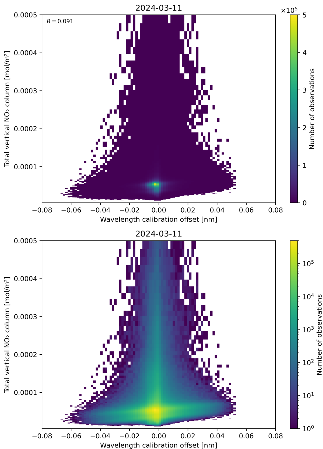
Figure 179: Scatter density plot of “Wavelength calibration offset” against “Total vertical NO 2 column” for 2024-03-10 to 2024-03-12.
