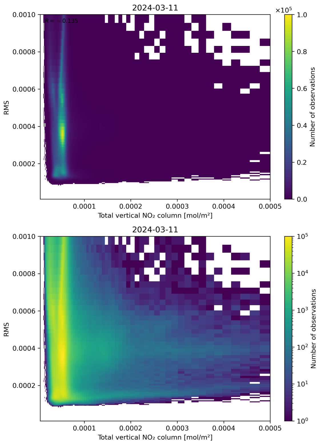
Figure 120: Scatter density plot of “Total vertical NO 2 column” against “RMS” for 2024-03-10 to 2024-03-12.
