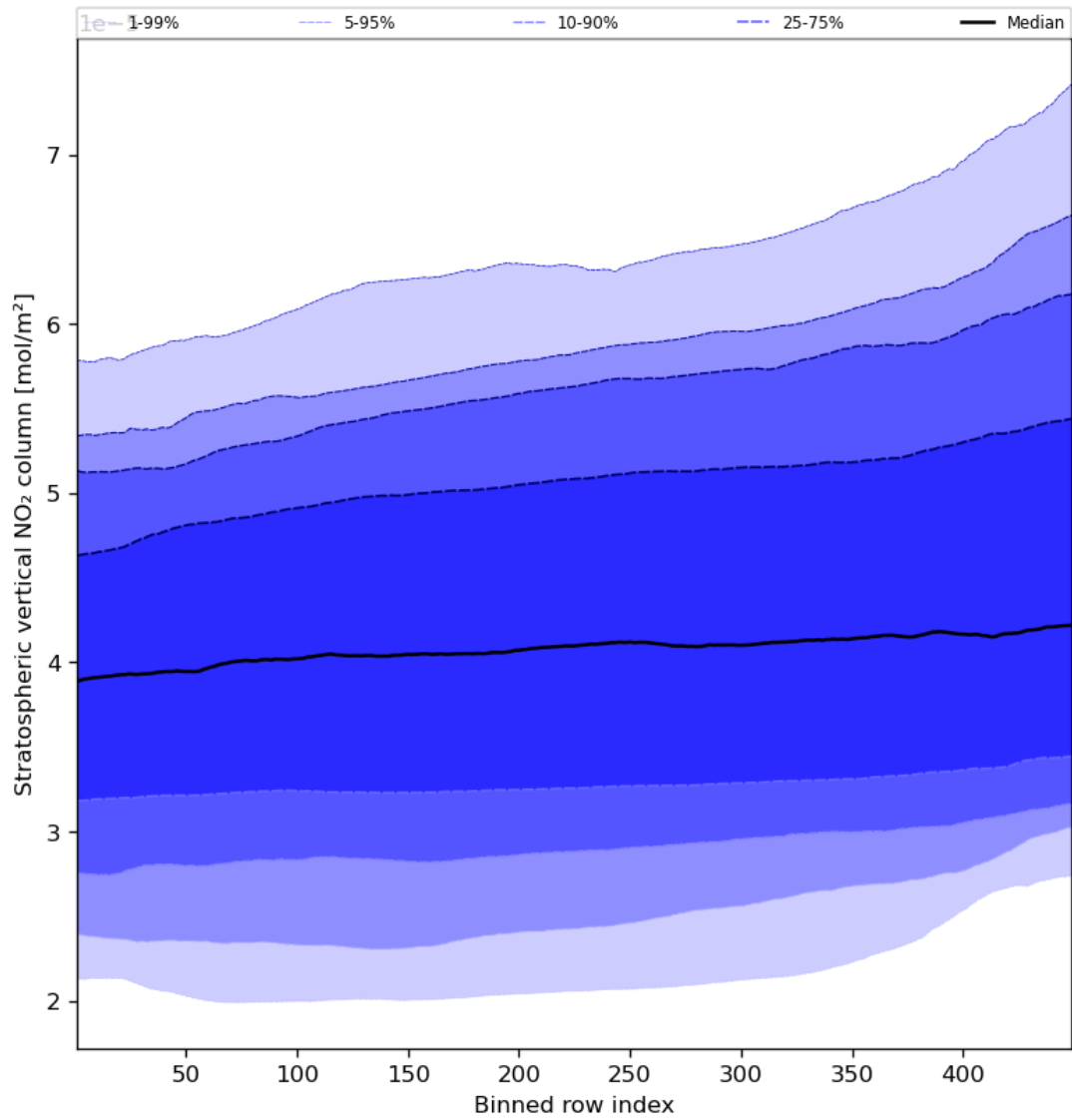
Figure 53: Along track statistics of “Stratospheric vertical NO 2 column” for 2024-03-10 to 2024-03-12
