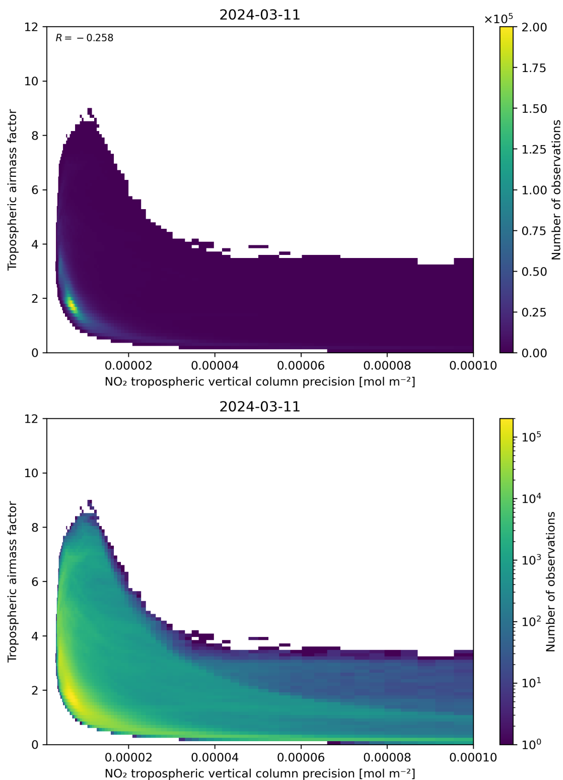
Figure 133: Scatter density plot of “NO 2 tropospheric vertical column precision” against “Tropospheric airmass factor” for 2024-03-10 to 2024-03-12.
