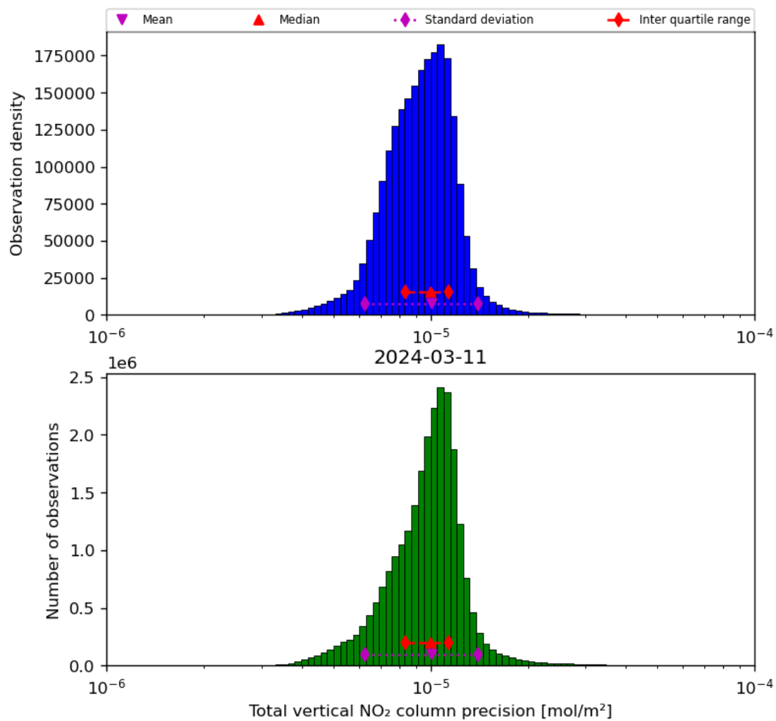
Figure 39: Histogram of “Total vertical NO 2 column precision” for 2024-03-10 to 2024-03-12
