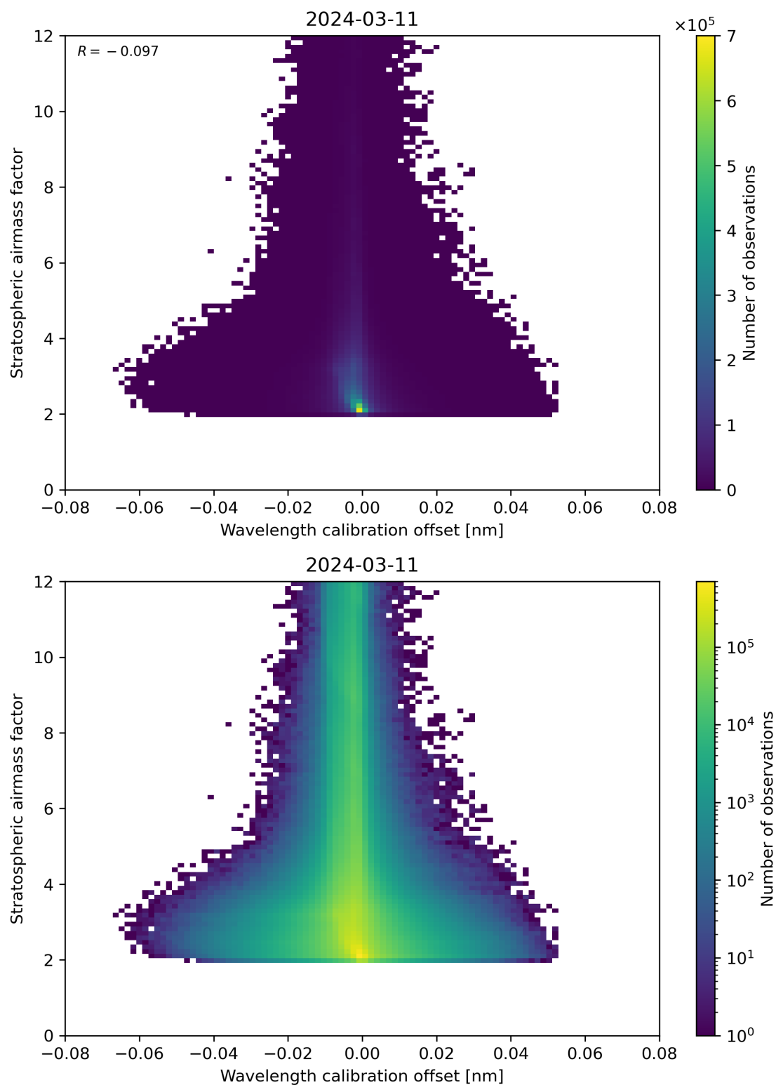
Figure 174: Scatter density plot of “Wavelength calibration offset” against “Stratospheric airmass factor” for 2024-03-10 to 2024-03-12.
