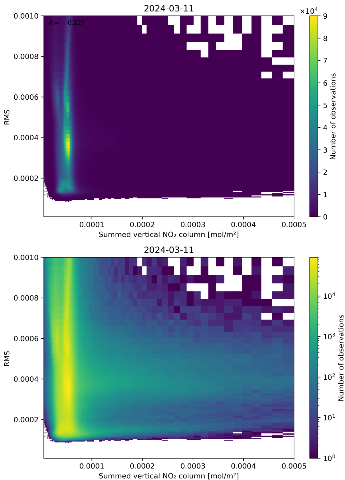
Figure 109: Scatter density plot of “Summed vertical NO 2 column” against “RMS” for 2024-03-10 to 2024-03-12.
