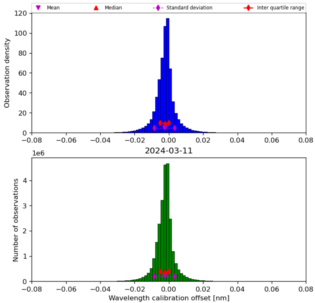
Figure 35: Histogram of “Wavelength calibration offset” for 2024-03-10 to 2024-03-12
