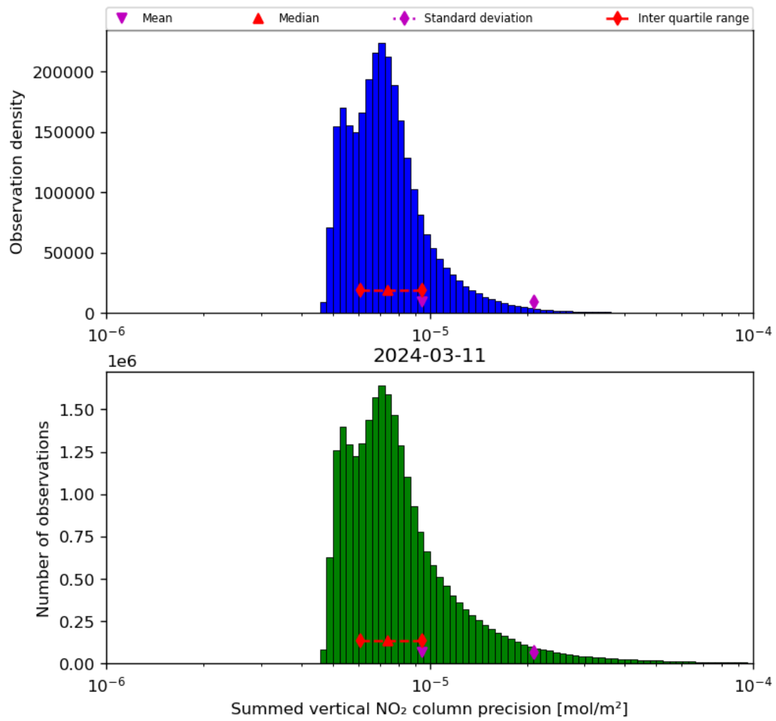
Figure 41: Histogram of “Summed vertical NO 2 column precision” for 2024-03-10 to 2024-03-12
