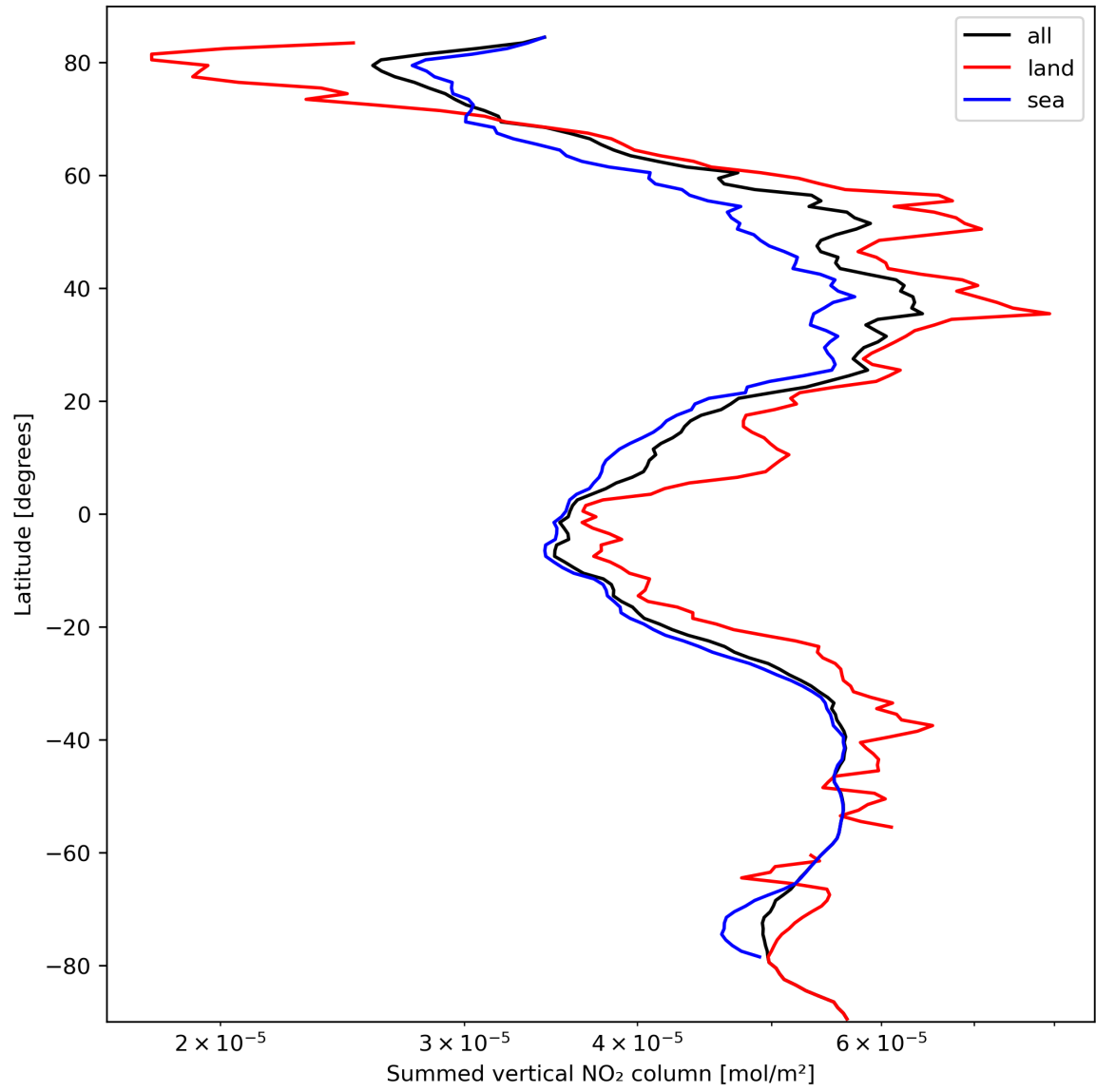
Figure 23: Zonal average of “Summed vertical NO 2 column” for 2024-03-10 to 2024-03-12.
