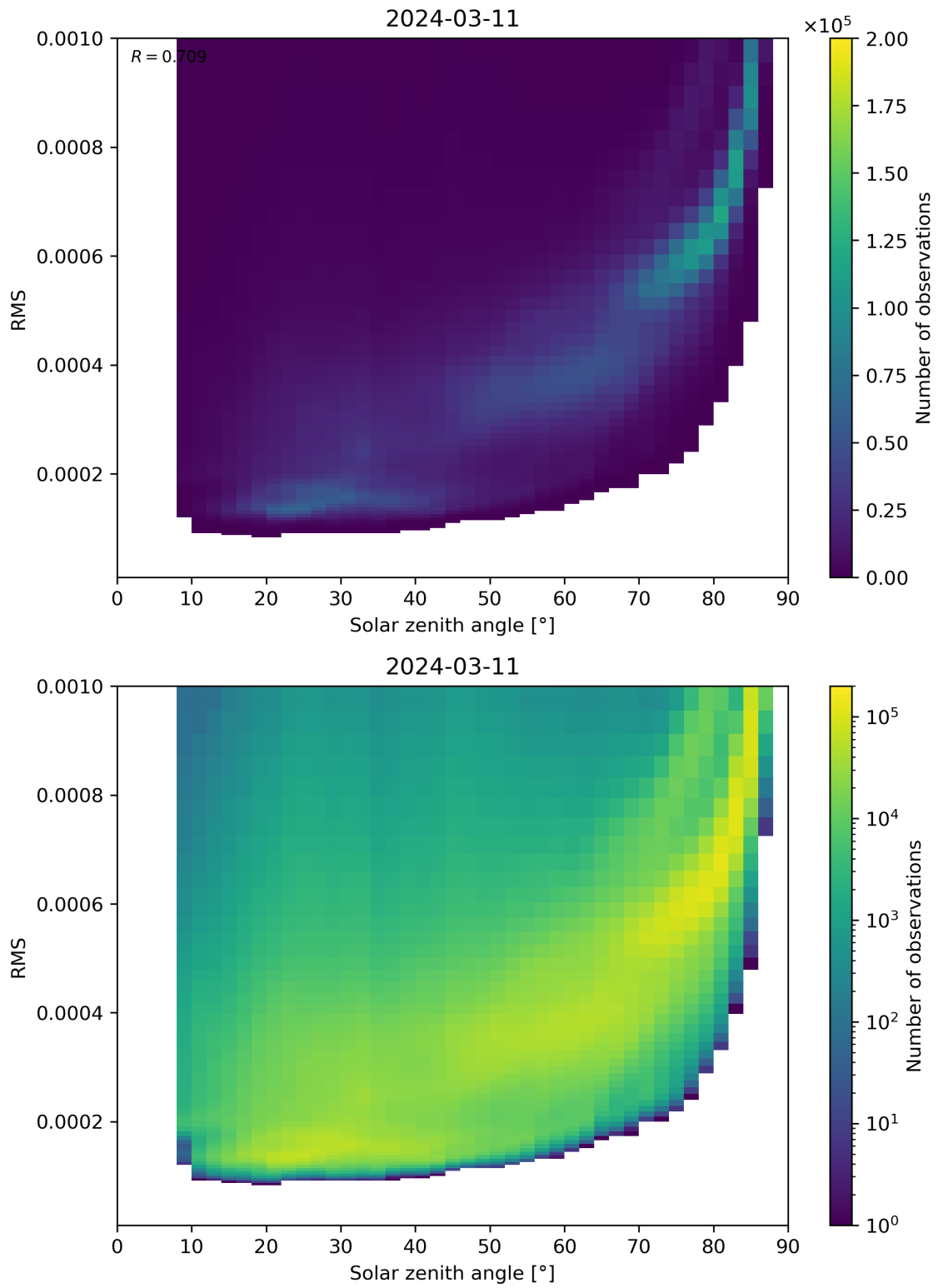
Figure 157: Scatter density plot of “Solar zenith angle” against “RMS” for 2024-03-10 to 2024-03-12.
