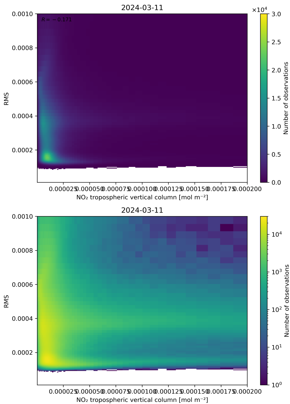
Figure 142: Scatter density plot of “NO 2 tropospheric vertical column” against “RMS” for 2024-03-10 to 2024-03-12.
