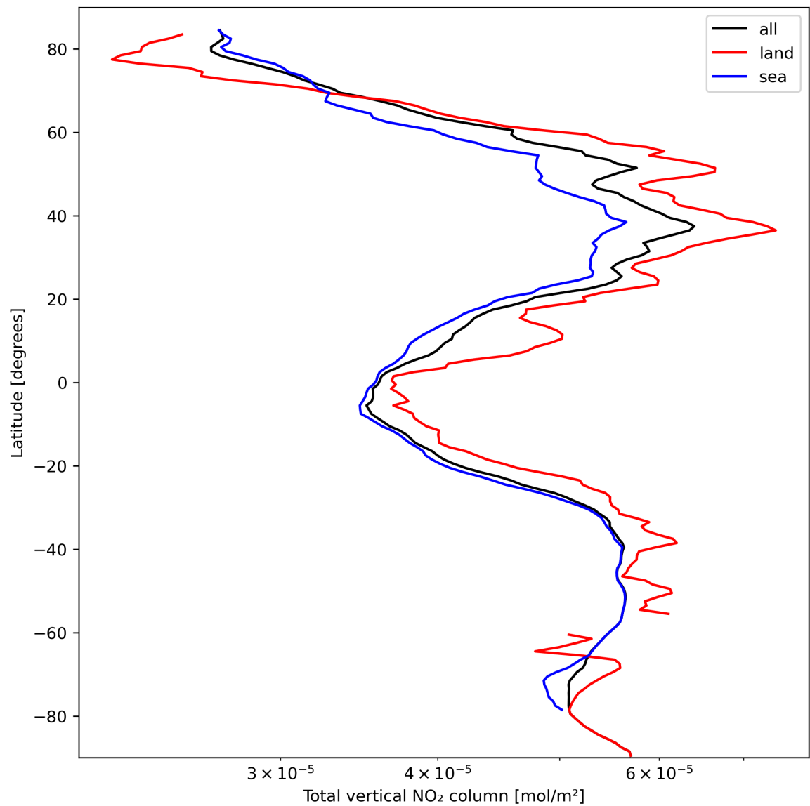
Figure 21: Zonal average of “Total vertical NO 2 column” for 2024-03-10 to 2024-03-12.
