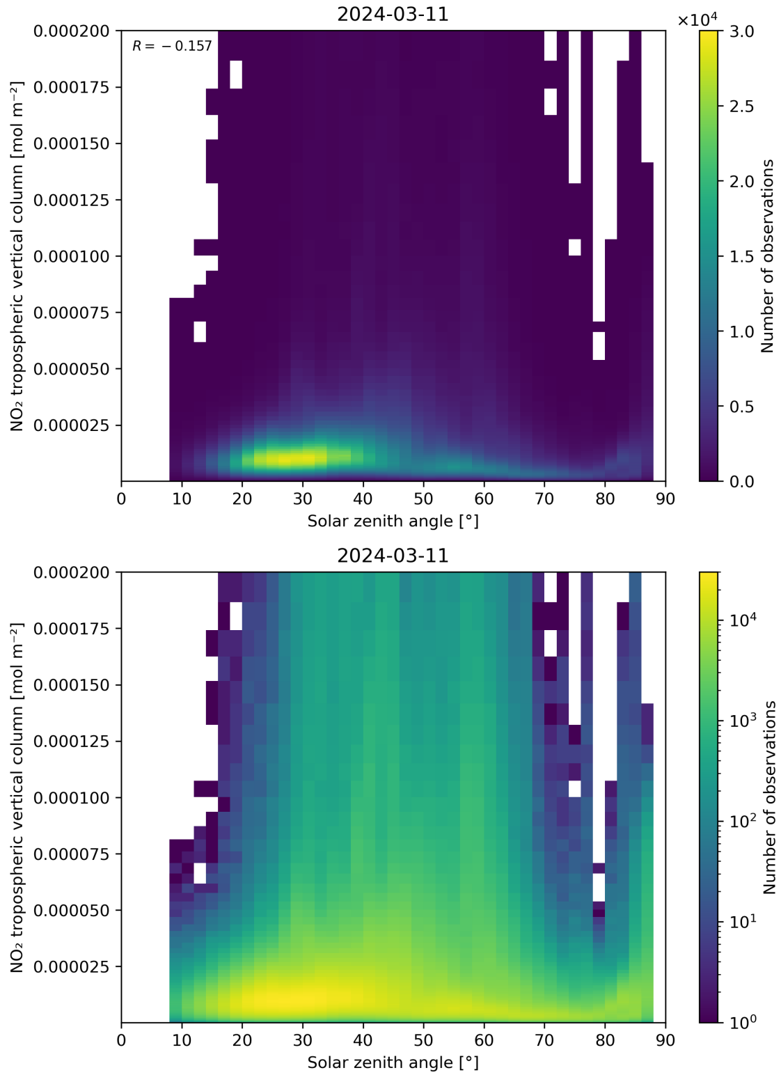
Figure 155: Scatter density plot of “Solar zenith angle” against “NO 2 tropospheric vertical column” for 2024-03-10 to 2024-03-12.
