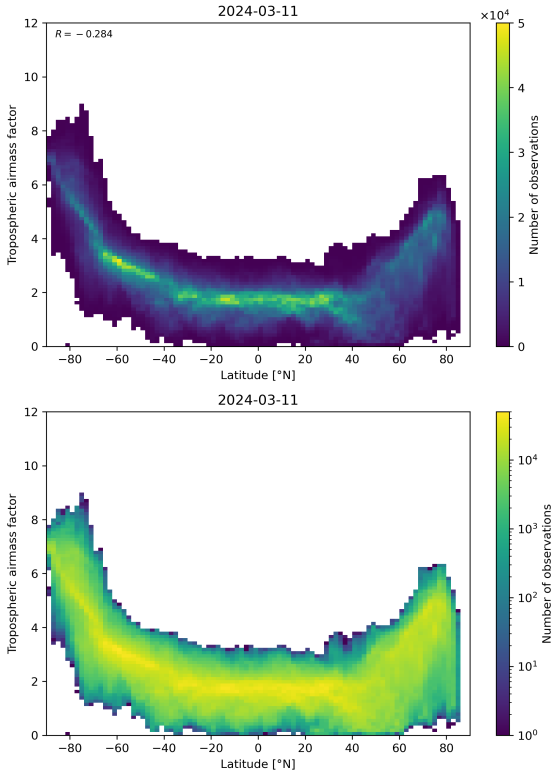
Figure 85: Scatter density plot of “Latitude” against “Tropospheric airmass factor” for 2024-03-10 to 2024-03-12.
