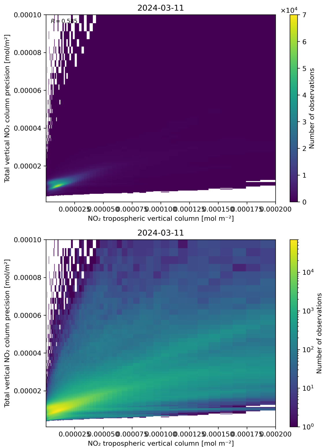
Figure 129: Scatter density plot of “NO 2 tropospheric vertical column” against “Total vertical NO 2 column precision” for 2024-03-10 to 2024-03-12.
