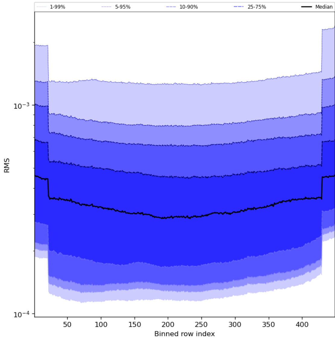
Figure 60: Along track statistics of “RMS” for 2024-03-10 to 2024-03-12
