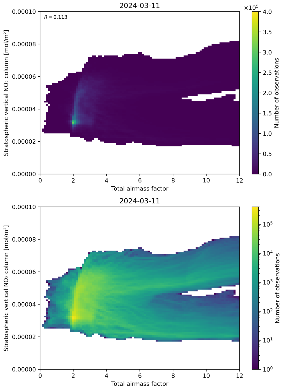
Figure 64: Scatter density plot of “Total airmass factor” against “Stratospheric vertical \text{NO}_2 column” for 2024-03-10 to 2024-03-12.
