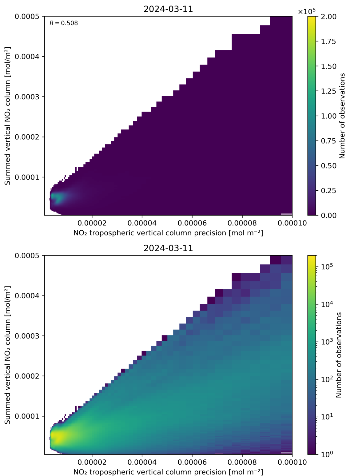
Figure 136: Scatter density plot of “NO 2 tropospheric vertical column precision” against “Summed vertical NO 2 column” for 2024-03-10 to 2024-03-12.
