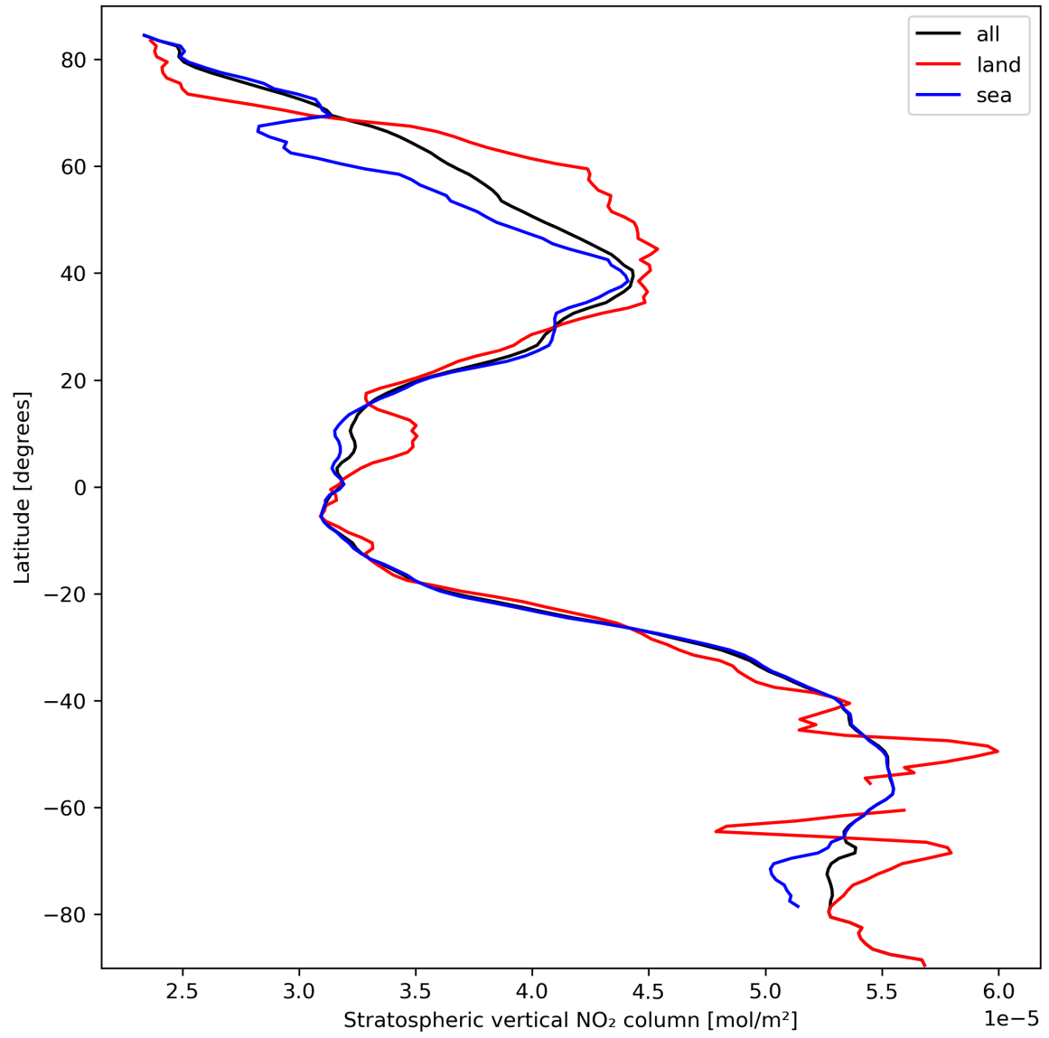
Figure 19: Zonal average of “Stratospheric vertical NO 2 column” for 2024-03-10 to 2024-03-12.
