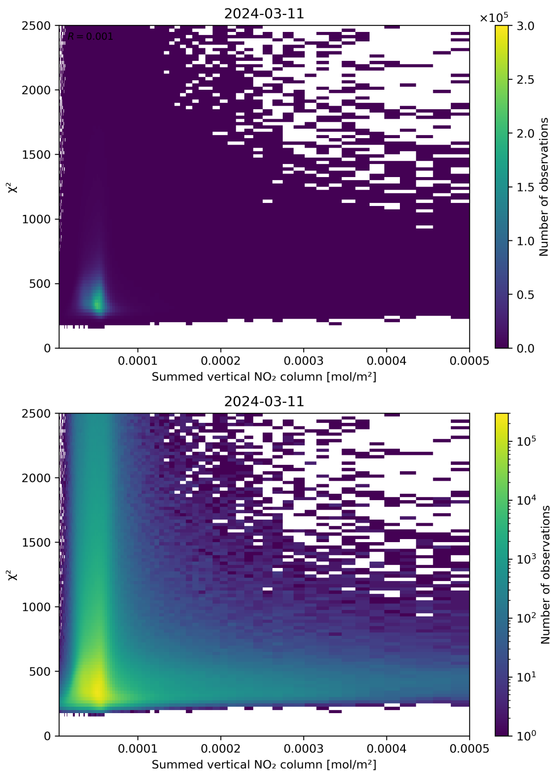
Figure 104: Scatter density plot of “Summed vertical NO 2 column” against “ \chi^2 ” for 2024-03-10 to 2024-03-12.
