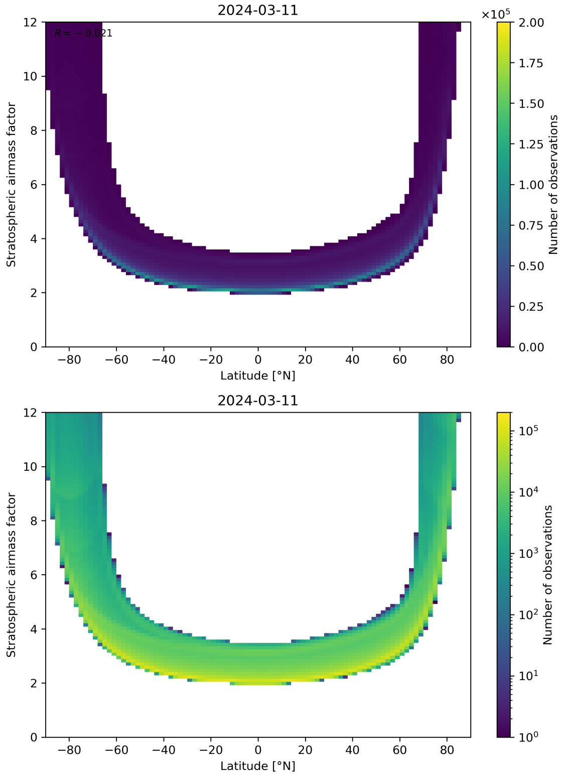
Figure 83: Scatter density plot of “Latitude” against “Stratospheric airmass factor” for 2024-03-10 to 2024-03-12.
