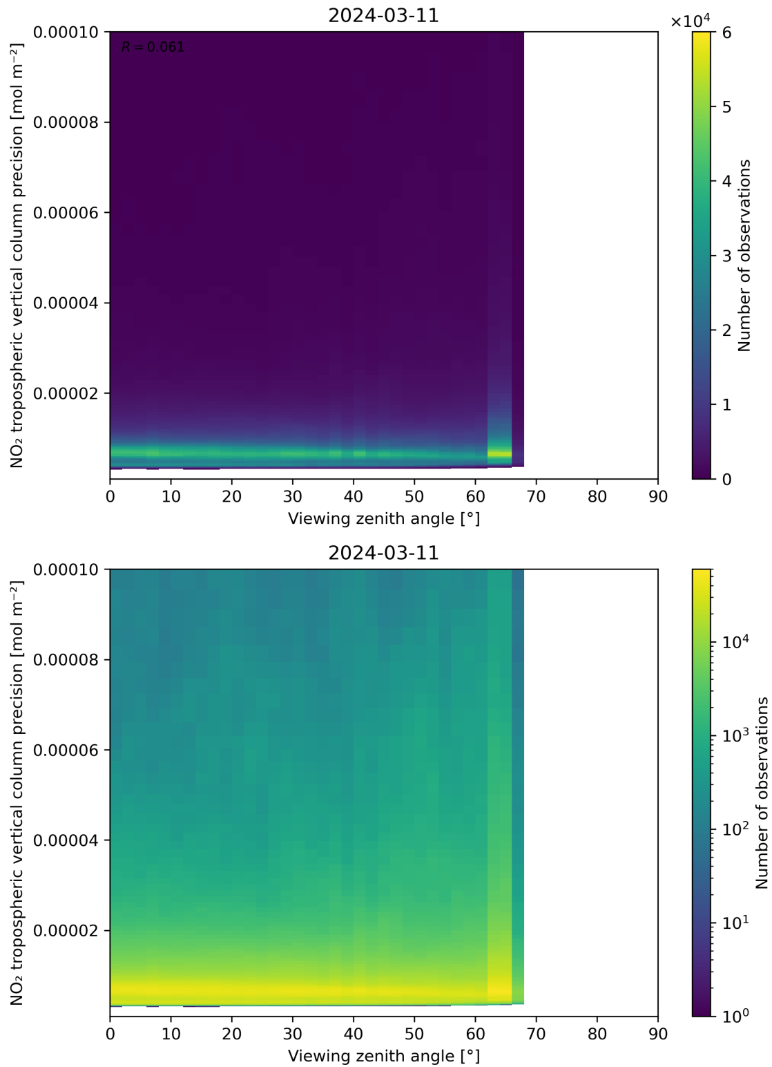
Figure 170: Scatter density plot of “Viewing zenith angle” against “NO 2 tropospheric vertical column precision” for 2024-03-10 to 2024-03-12.
