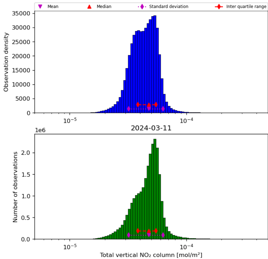
Figure 38: Histogram of “Total vertical NO 2 column” for 2024-03-10 to 2024-03-12
