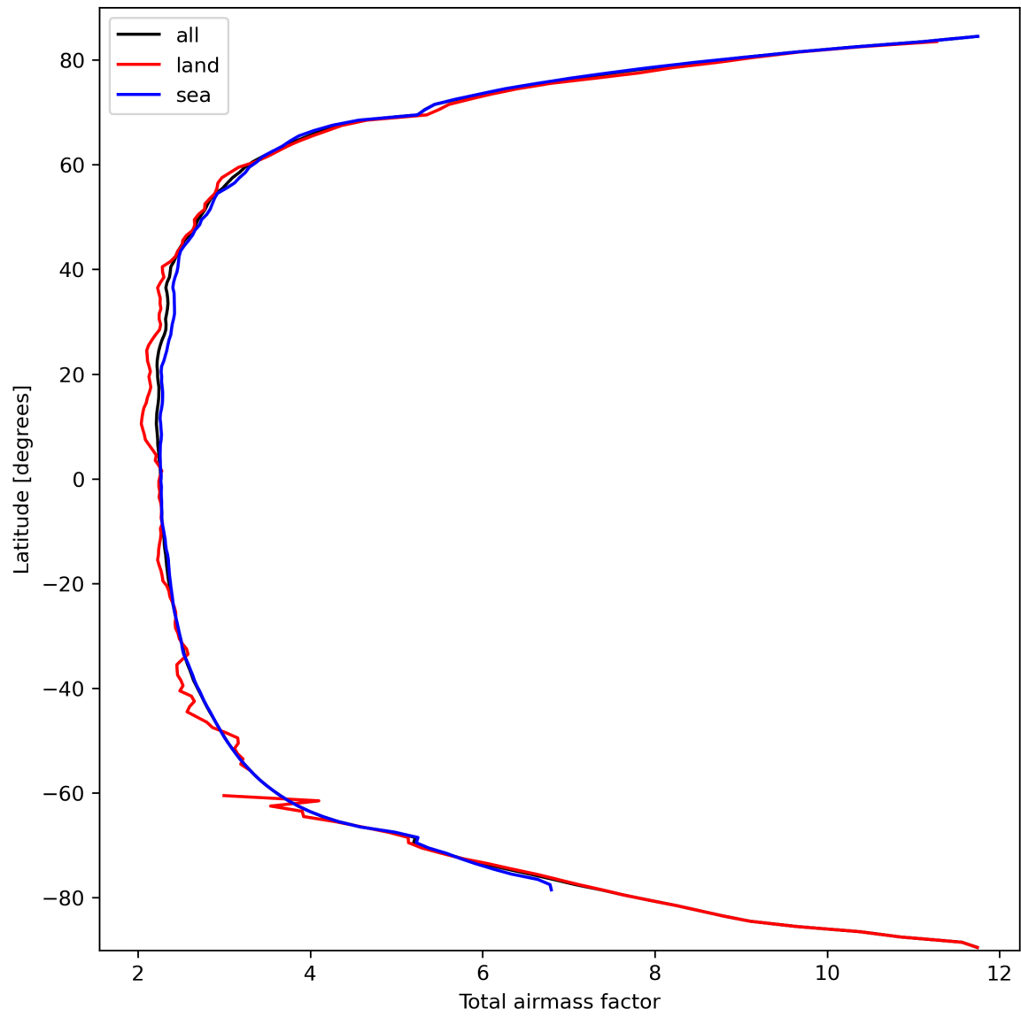
Figure 15: Zonal average of “Total airmass factor” for 2024-03-10 to 2024-03-12.
