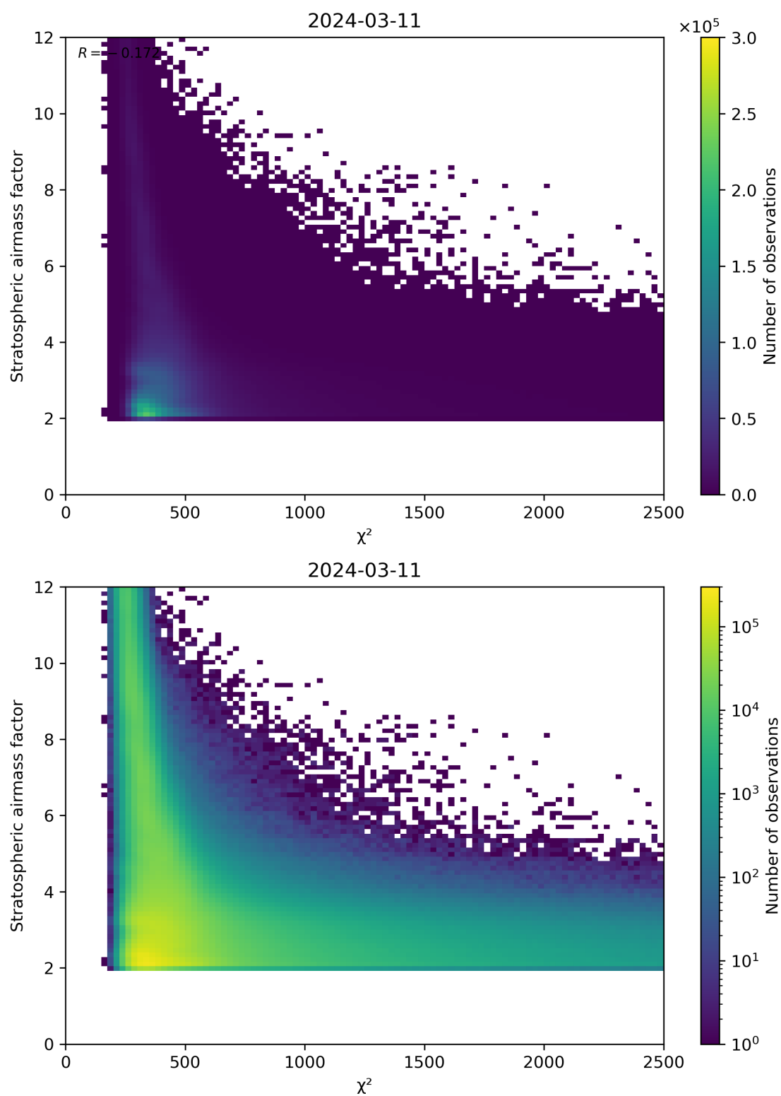
Figure 81: Scatter density plot of “ \chi^2 ” against “Stratospheric airmass factor” for 2024-03-10 to 2024-03-12.
