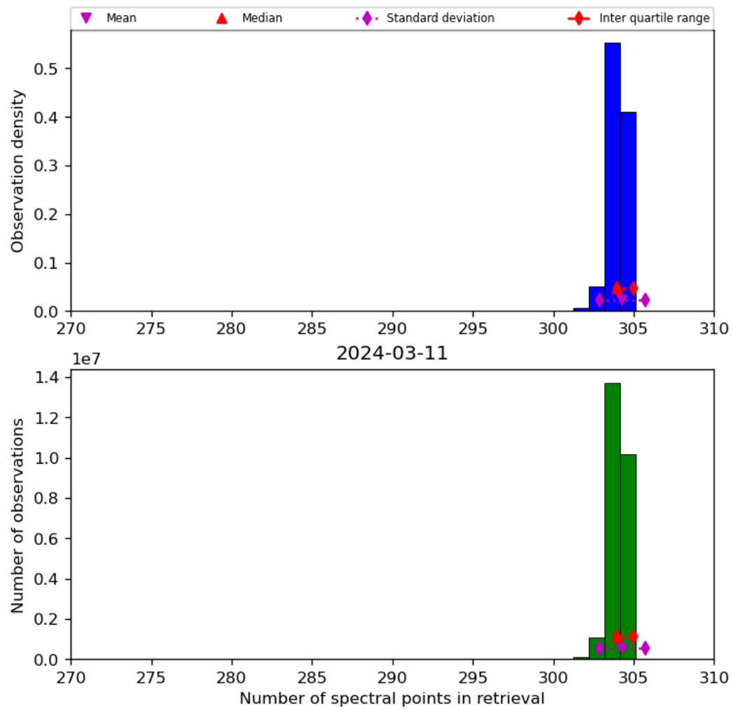
Figure 33: Histogram of “Number of spectral points in retrieval” for 2024-03-10 to 2024-03-12
