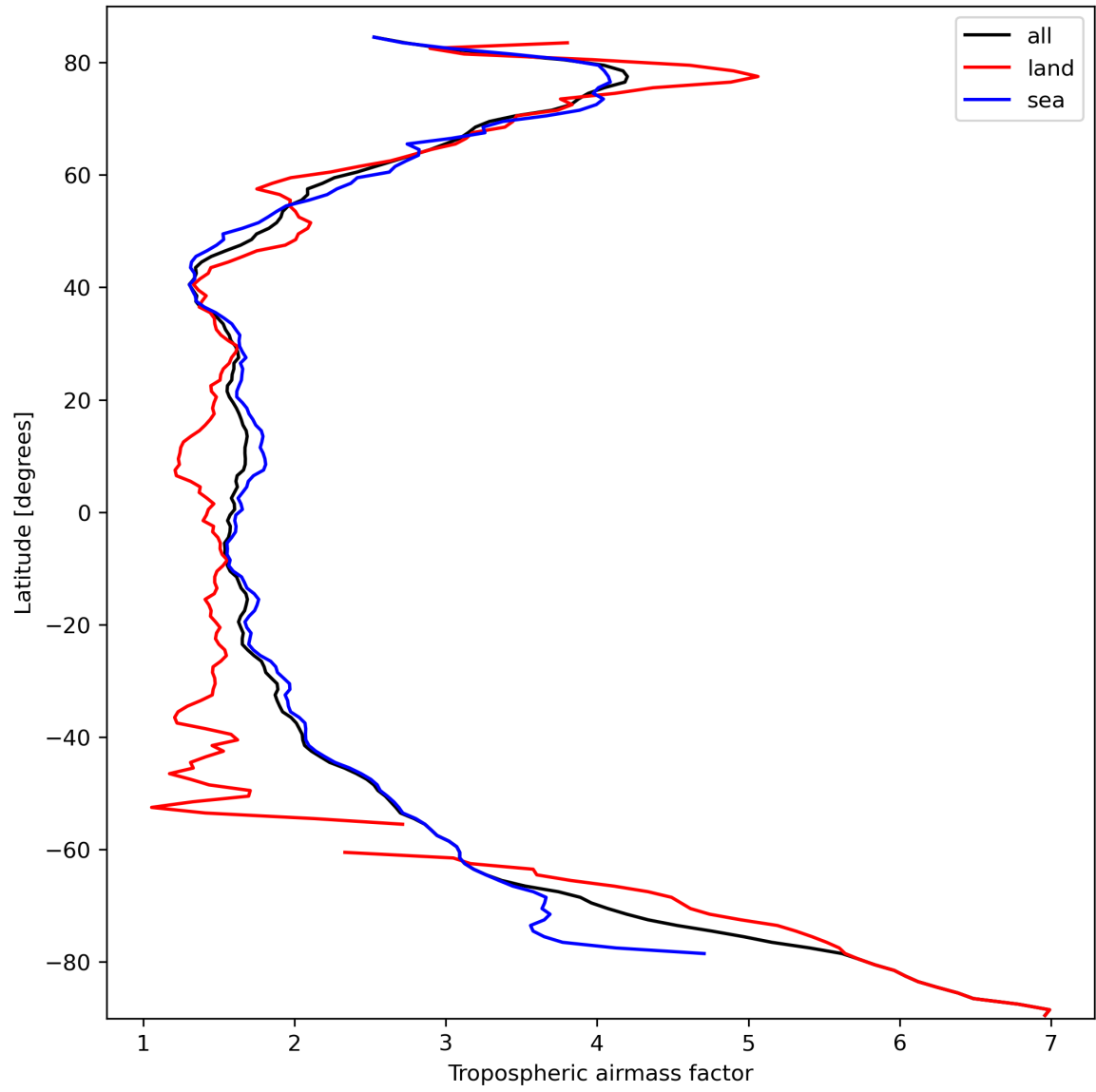
Figure 14: Zonal average of “Tropospheric air mass factor” for 2024-03-10 to 2024-03-12.
