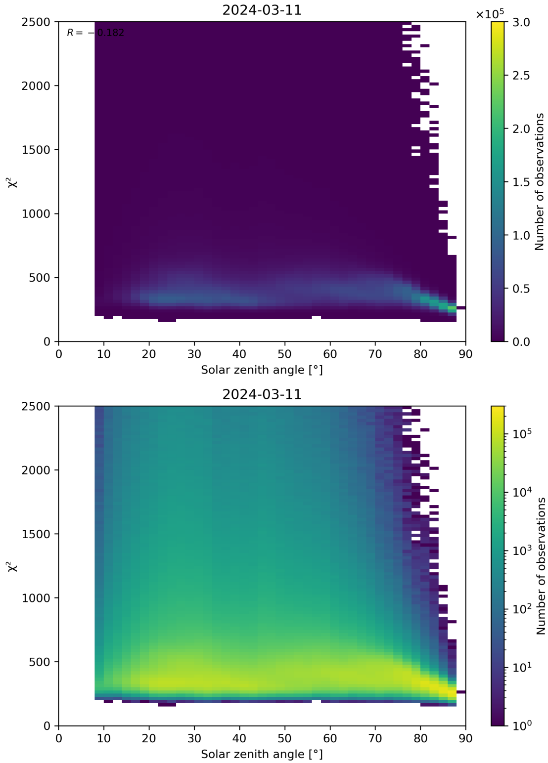
Figure 148: Scatter density plot of “Solar zenith angle” against “ \chi^2 ” for 2024-03-10 to 2024-03-12.
