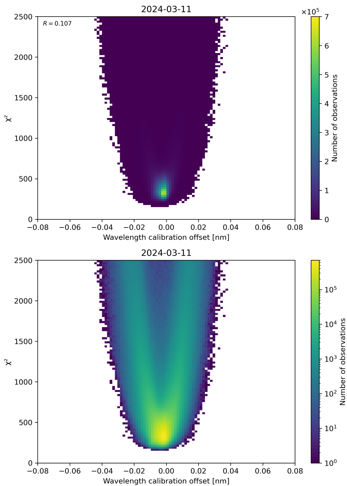
Figure 175: Scatter density plot of “Wavelength calibration offset” against “ \chi^2 ” for 2024-03-10 to 2024-03-12.
