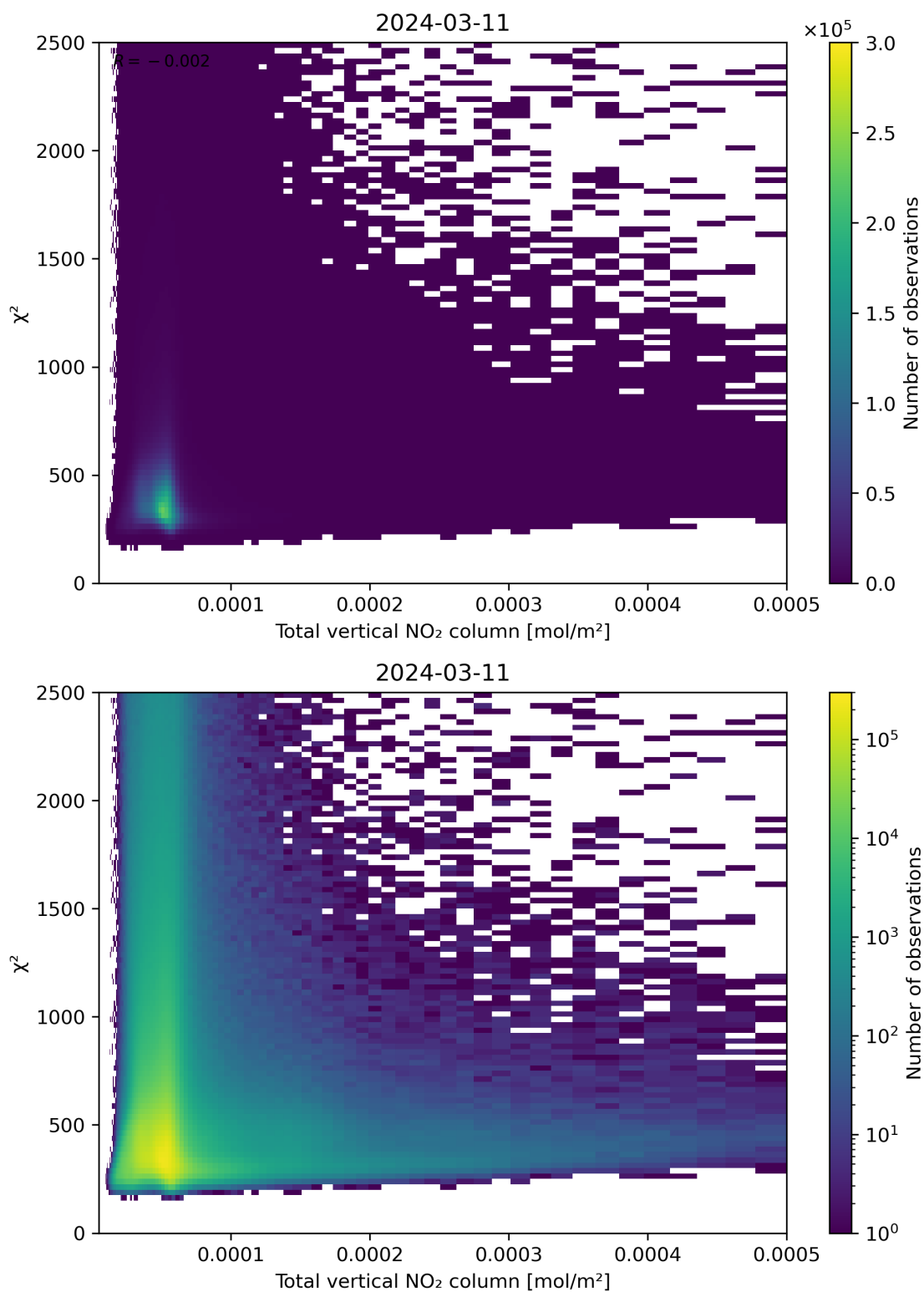
Figure 111: Scatter density plot of “Total vertical NO 2 column” against “ \chi^2 ” for 2024-03-10 to 2024-03-12.
