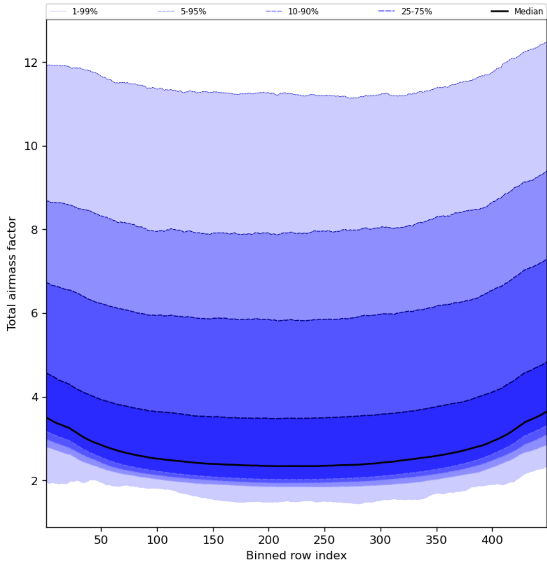
Figure 49: Along track statistics of “Total airmass factor” for 2024-03-10 to 2024-03-12
