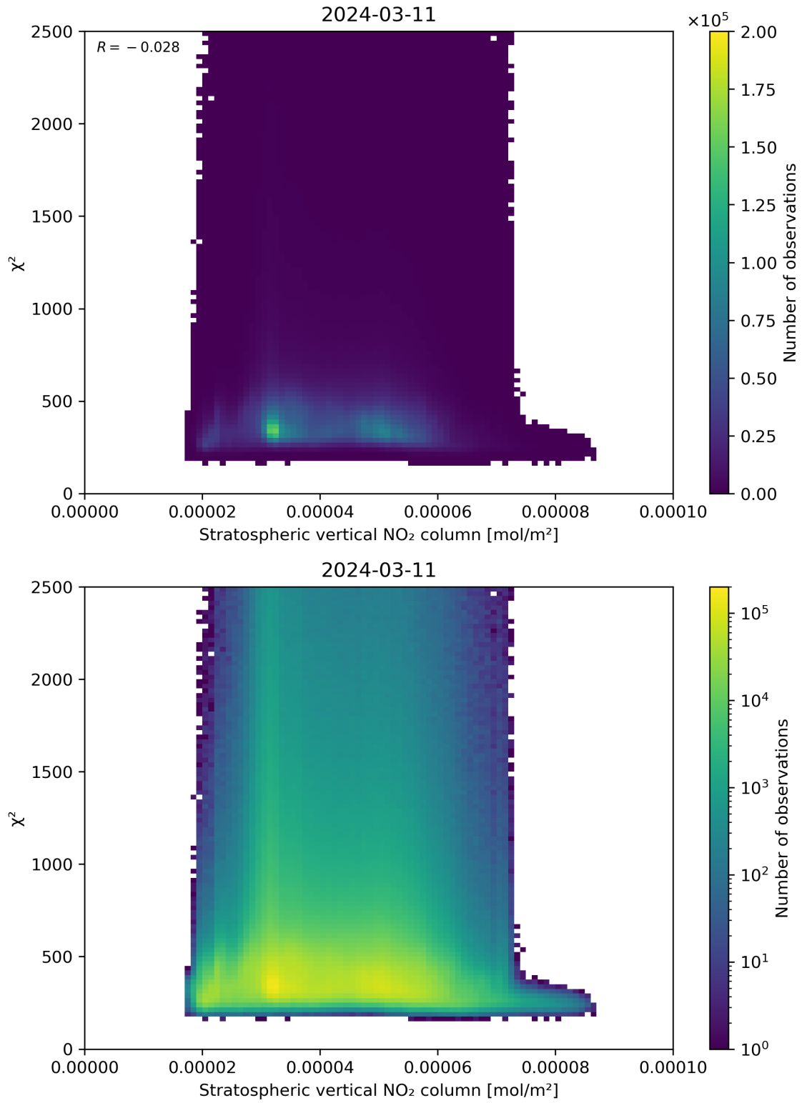
Figure 97: Scatter density plot of “Stratospheric vertical NO 2 column” against “ \chi^2 ” for 2024-03-10 to 2024-03-12.
