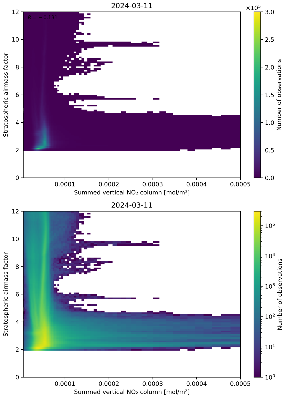
Figure 103: Scatter density plot of “Summed vertical NO 2 column” against “Stratospheric airmass factor” for 2024-03-10 to 2024-03-12.
