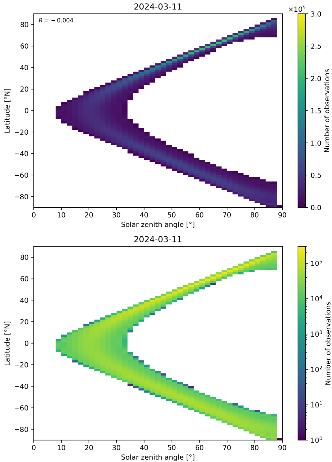
Figure 149: Scatter density plot of “Solar zenith angle” against “Latitude” for 2024-03-10 to 2024-03-12.
