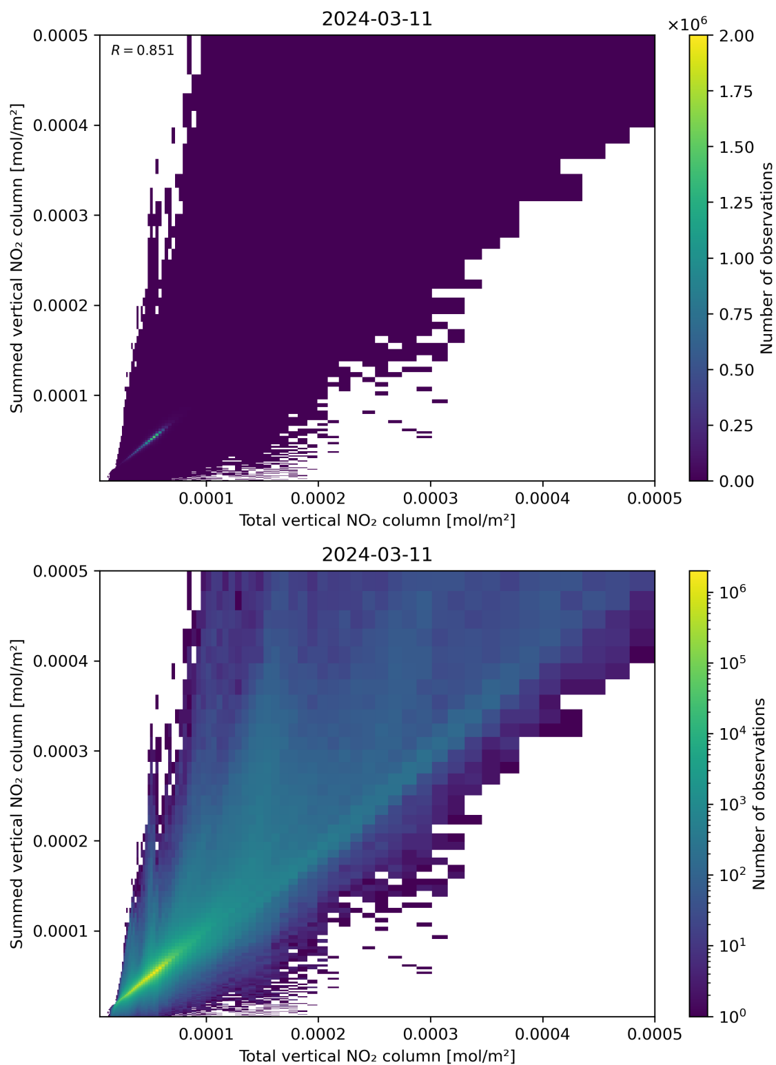
Figure 112: Scatter density plot of “Total vertical NO 2 column” against “Summed vertical NO 2 column” for 2024-03-10 to 2024-03-12.
