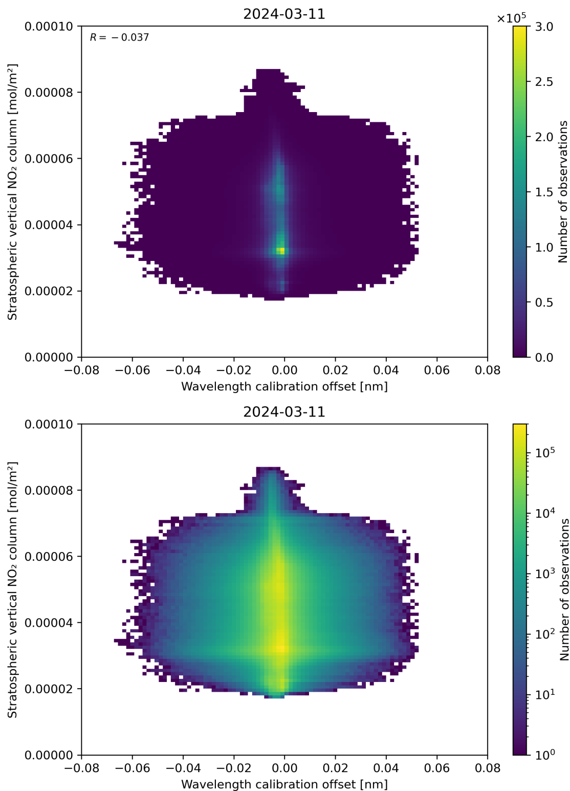
Figure 176: Scatter density plot of “Wavelength calibration offset” against “Stratospheric vertical NO 2 column” for 2024-03-10 to 2024-03-12.
