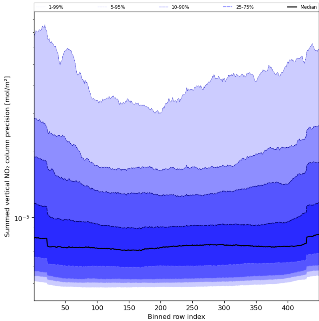
Figure 58: Along track statistics of “Summed vertical NO 2 column precision” for 2024-03-10 to 2024-03-12
