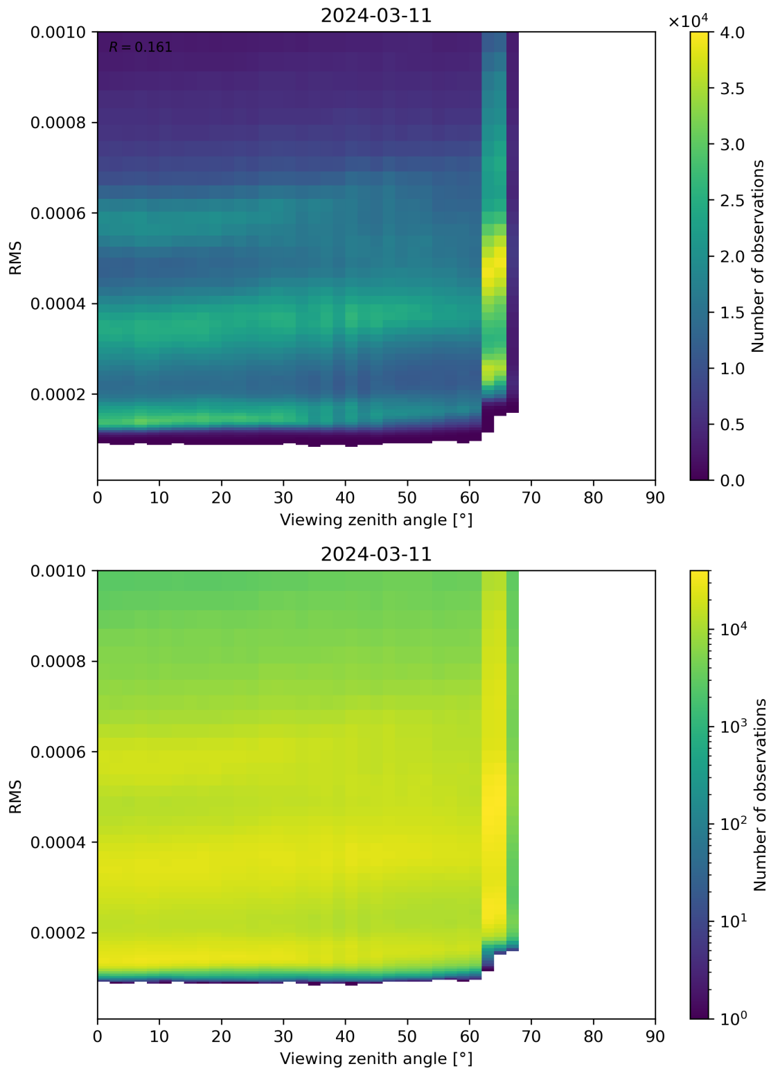
Figure 171: Scatter density plot of “Viewing zenith angle” against “RMS” for 2024-03-10 to 2024-03-12.
