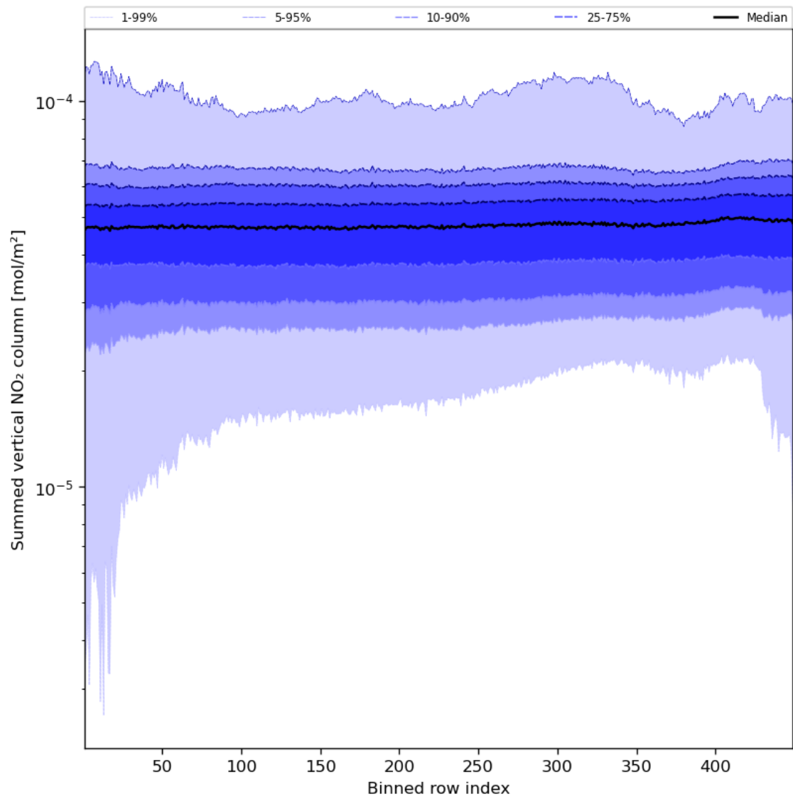
Figure 57: Along track statistics of “Summed vertical NO 2 column” for 2024-03-10 to 2024-03-12
