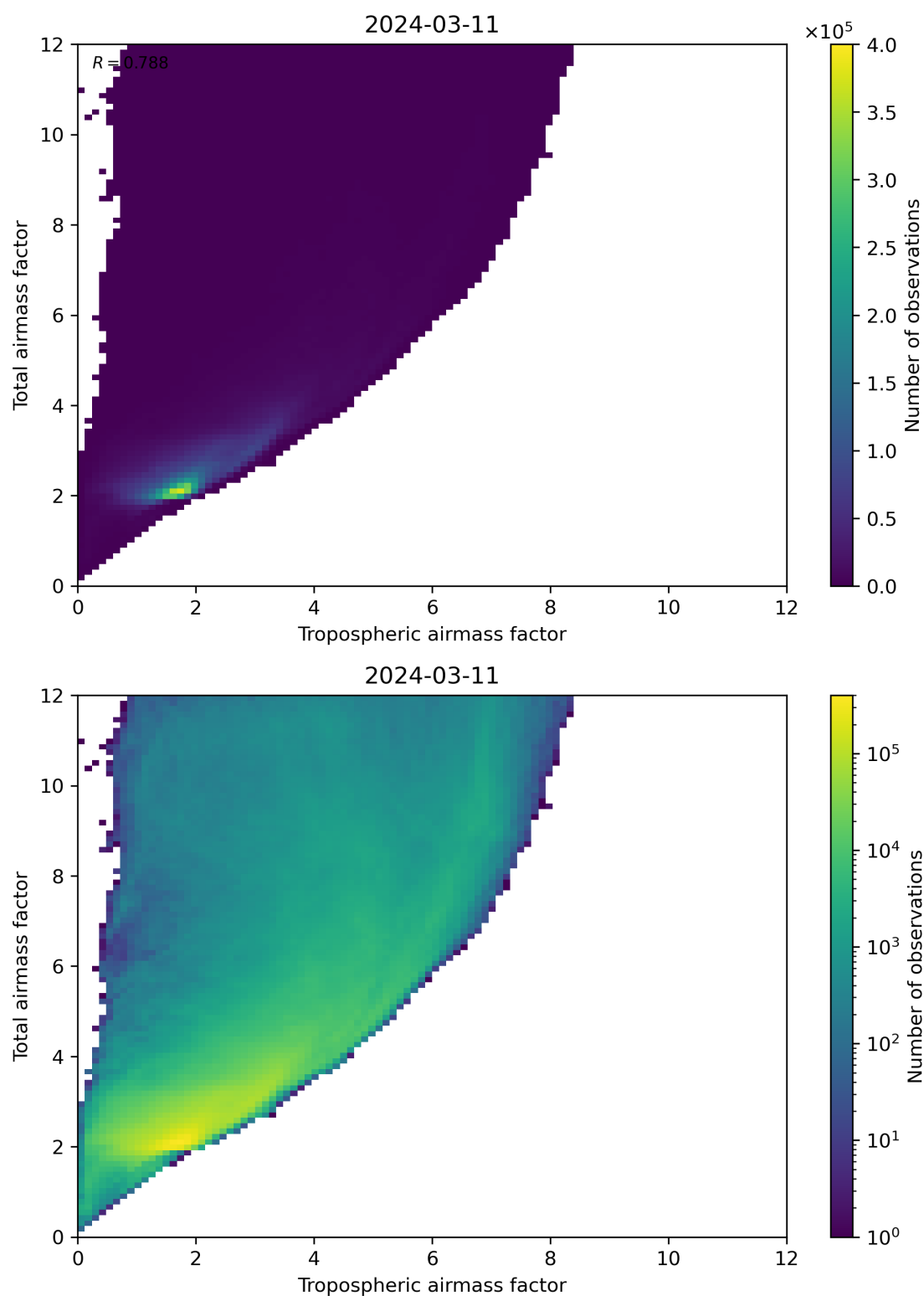
Figure 72: Scatter density plot of “Tropospheric airmass factor” against “Total airmass factor” for 2024-03-10 to 2024-03-12.
