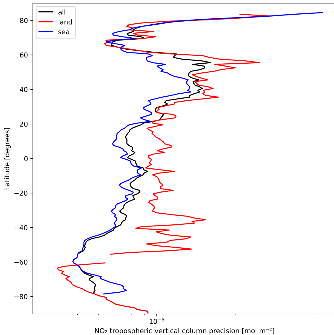
Figure 13: Zonal average of “NO 2 tropospheric vertical column precision” for 2024-03-10 to 2024-03-12.
