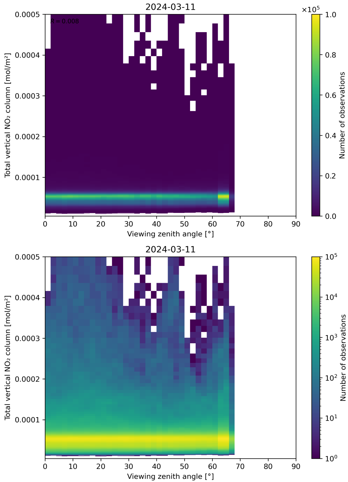
Figure 167: Scatter density plot of “Viewing zenith angle” against “Total vertical NO 2 column” for 2024-03-10 to 2024-03-12.
