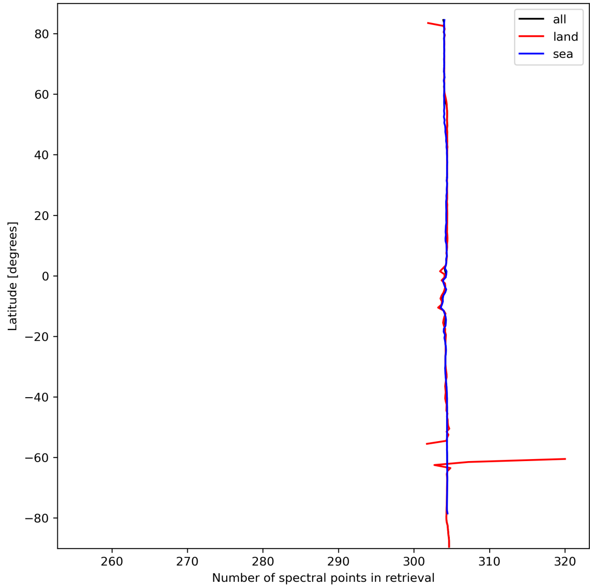
Figure 16: Zonal average of “Number of spectral points in retrieval” for 2024-03-10 to 2024-03-12.
