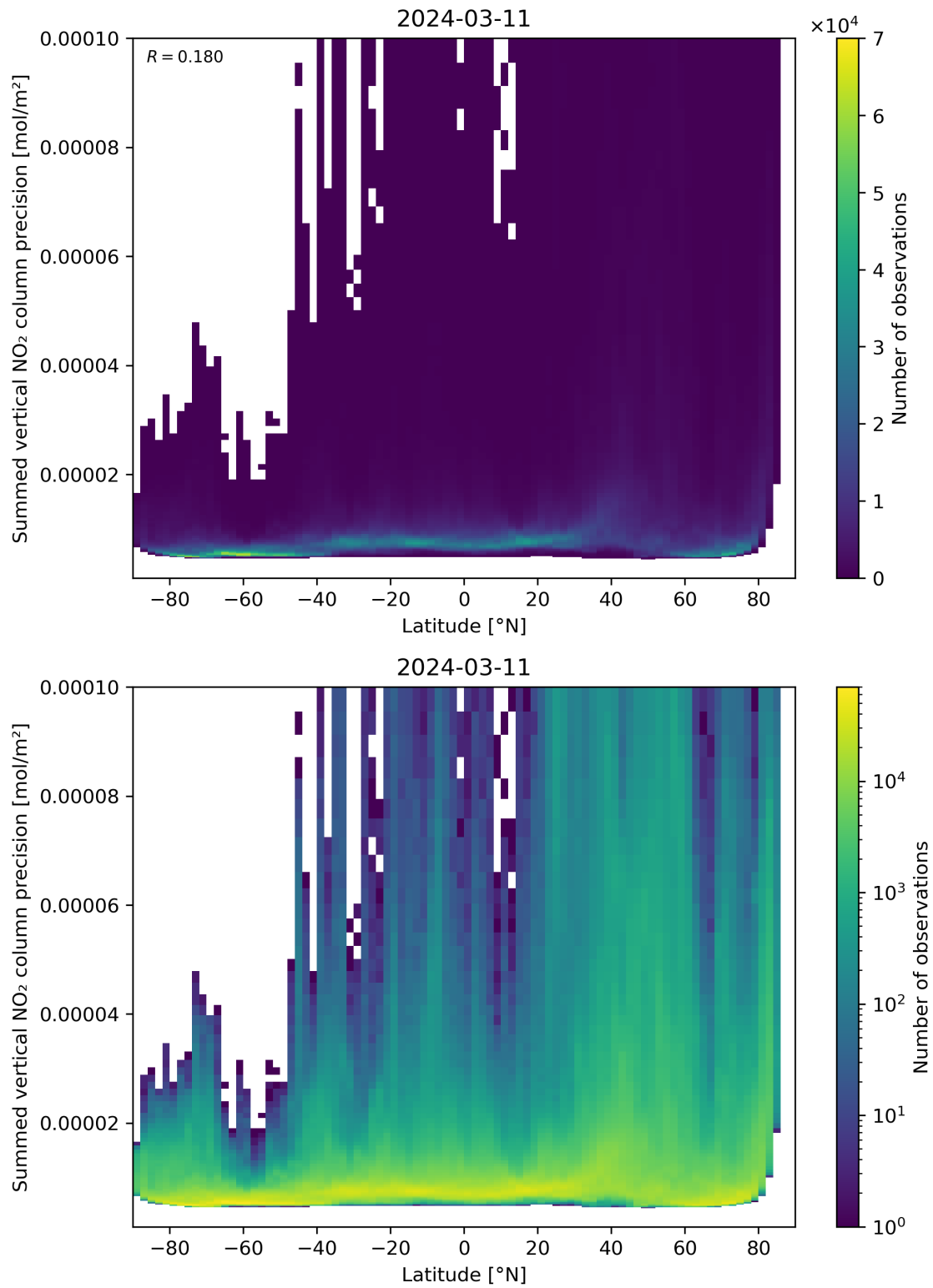
Figure 89: Scatter density plot of “Latitude” against “Summed vertical NO 2 column precision” for 2024-03-10 to 2024-03-12.
