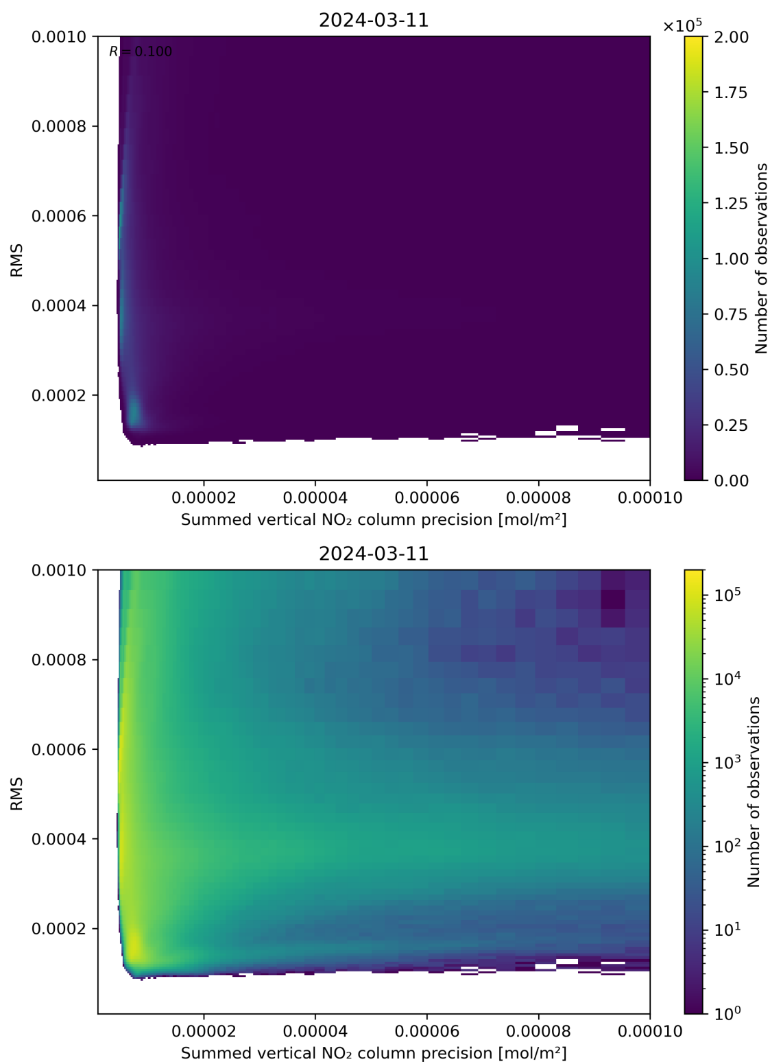
Figure 108: Scatter density plot of “Summed vertical NO 2 column precision” against “RMS” for 2024-03-10 to 2024-03-12.
