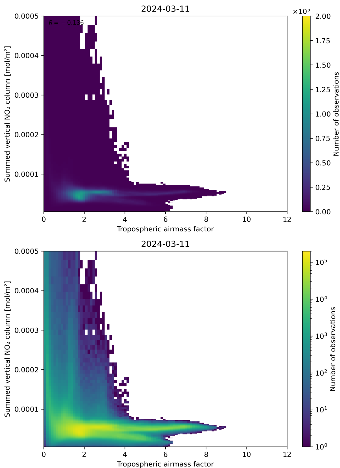
Figure 75: Scatter density plot of “Tropospheric airmass factor” against “Summed vertical NO 2 column” for 2024-03-10 to 2024-03-12.
