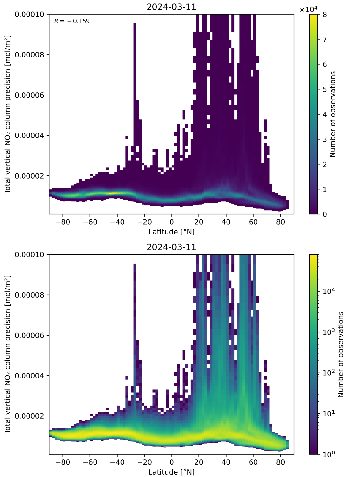
Figure 91: Scatter density plot of “Latitude” against “Total vertical NO 2 column precision” for 2024-03-10 to 2024-03-12.
