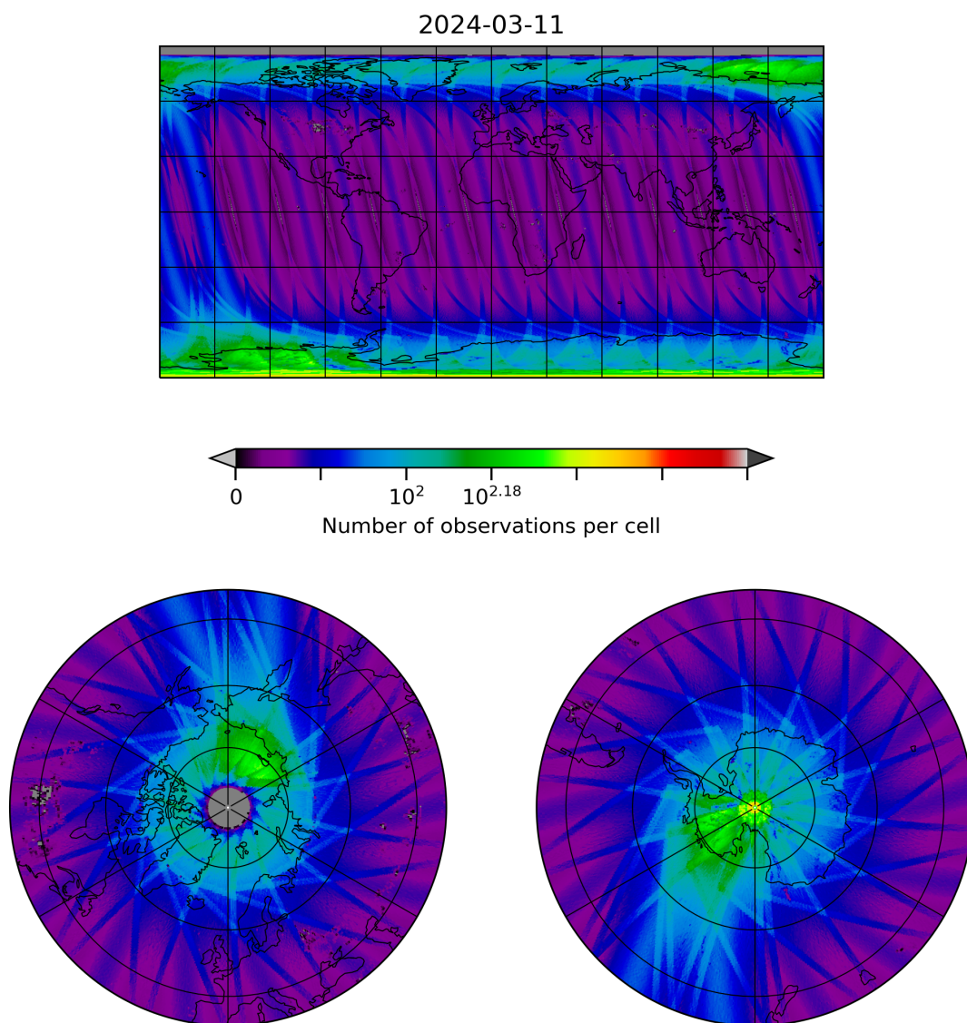
Figure 10: Map of the number of observations for 2024-03-10 to 2024-03-12
