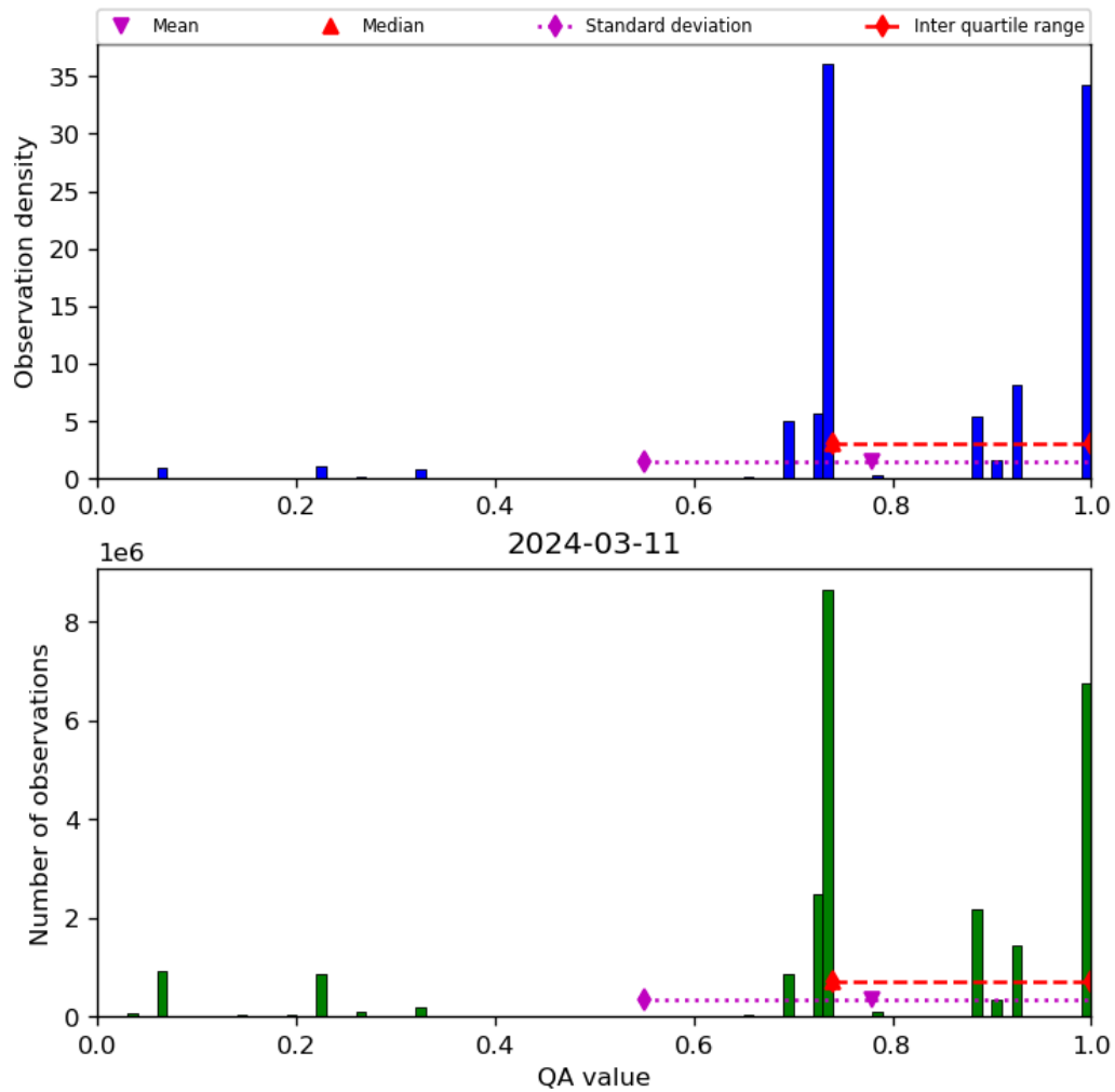
Figure 28: Histogram of “QA value” for 2024-03-10 to 2024-03-12
