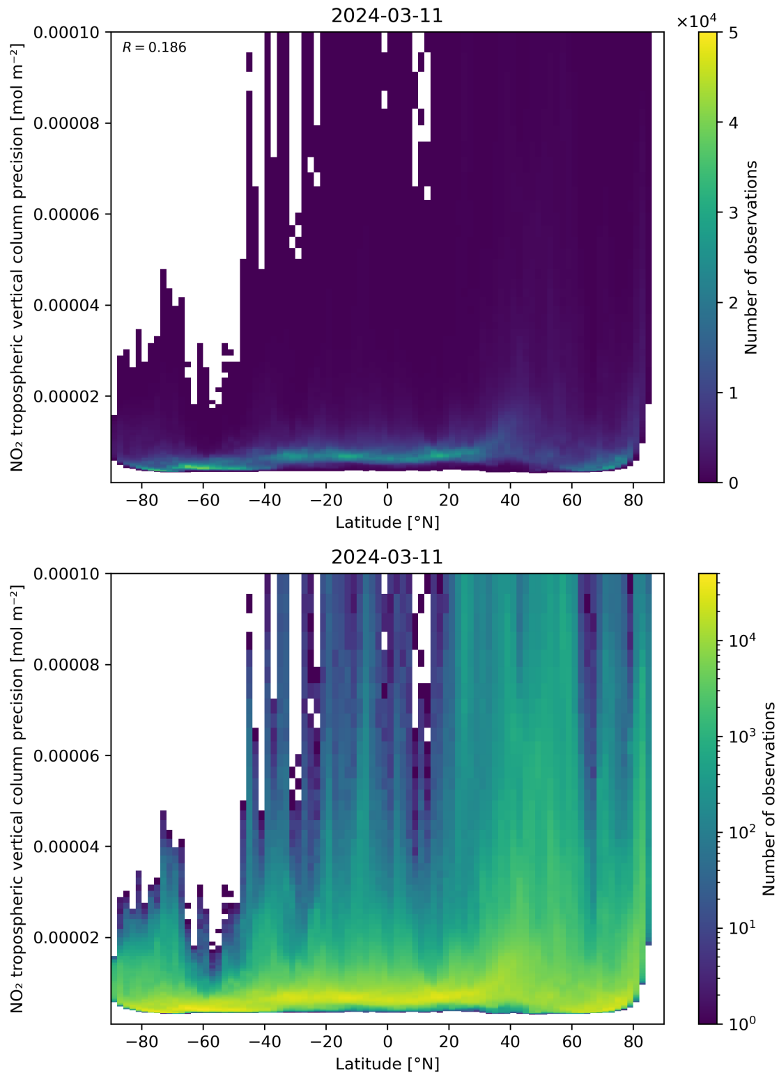
Figure 93: Scatter density plot of “Latitude” against “NO 2 tropospheric vertical column precision” for 2024-03-10 to 2024-03-12.
