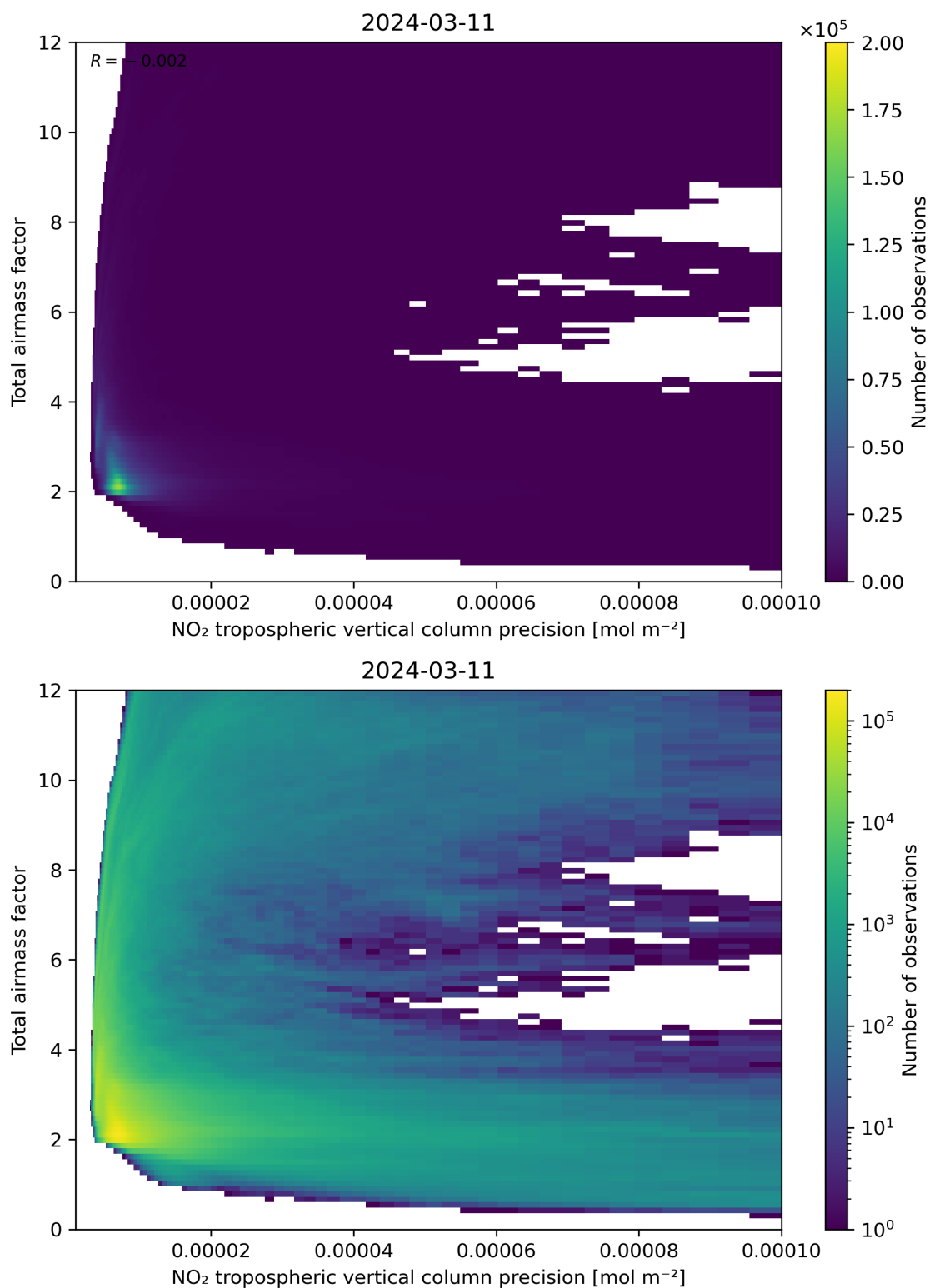
Figure 132: Scatter density plot of “NO 2 tropospheric vertical column precision” against “Total air mass factor” for 2024-03-10 to 2024-03-12.
