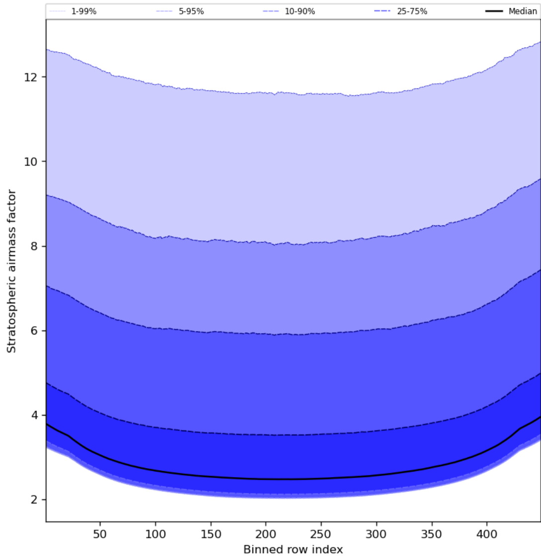
Figure 61: Along track statistics of “Stratospheric airmass factor” for 2024-03-10 to 2024-03-12
