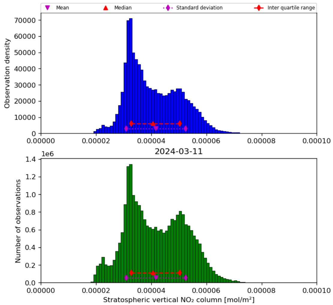
Figure 36: Histogram of “Stratospheric vertical NO 2 column” for 2024-03-10 to 2024-03-12
