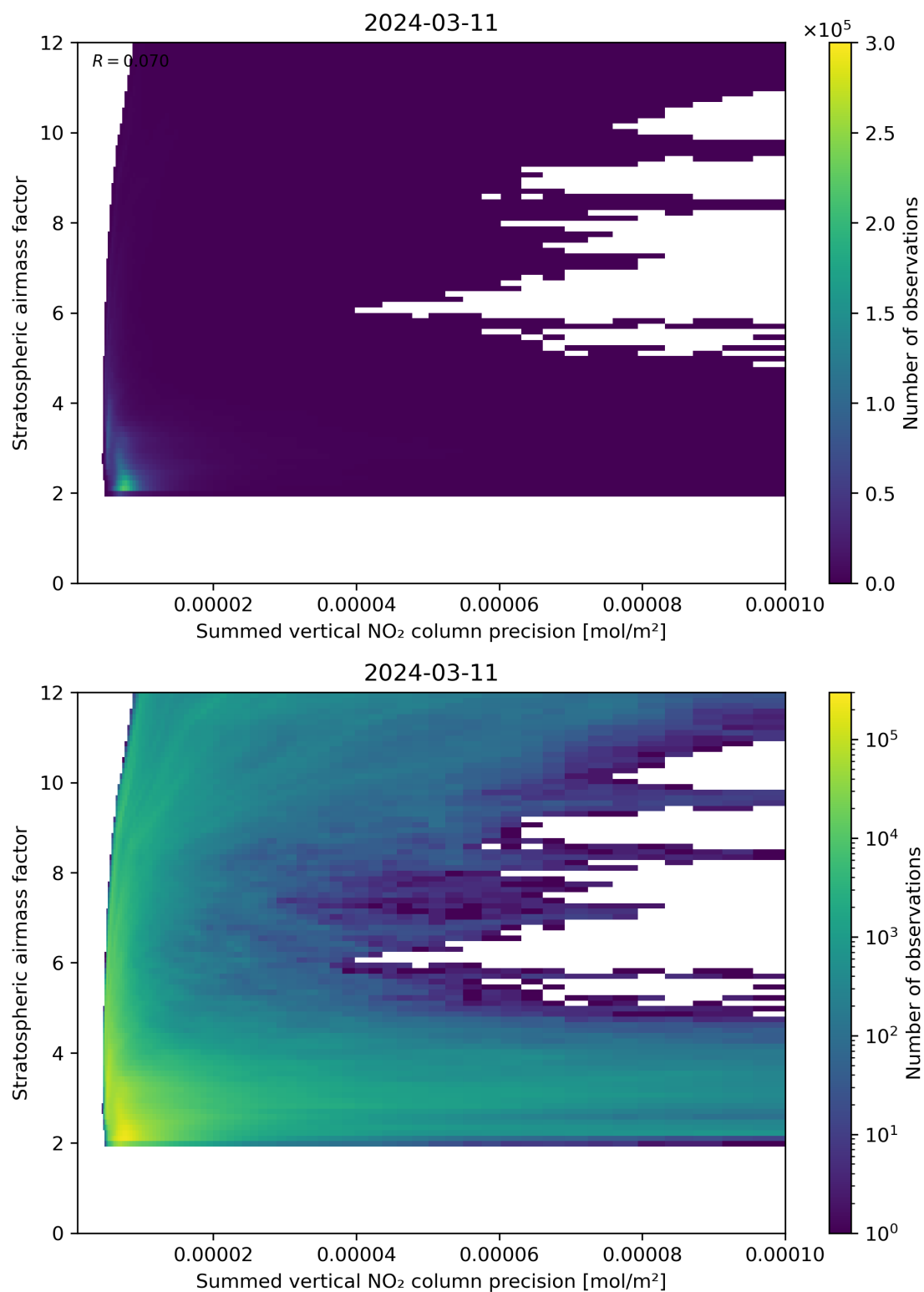
Figure 106: Scatter density plot of “Summed vertical NO 2 column precision” against “Stratospheric airmass factor” for 2024-03-10 to 2024-03-12.
