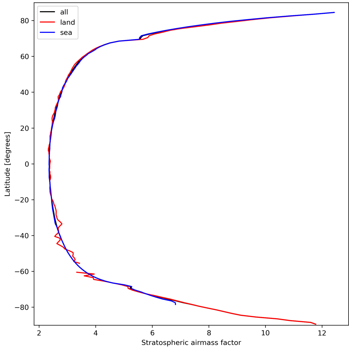
Figure 27: Zonal average of “Stratospheric air mass factor” for 2024-03-10 to 2024-03-12.
