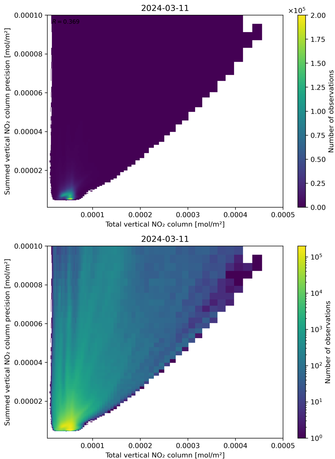
Figure 113: Scatter density plot of “Total vertical NO 2 column” against “Summed vertical NO 2 column precision” for 2024-03-10 to 2024-03-12.
