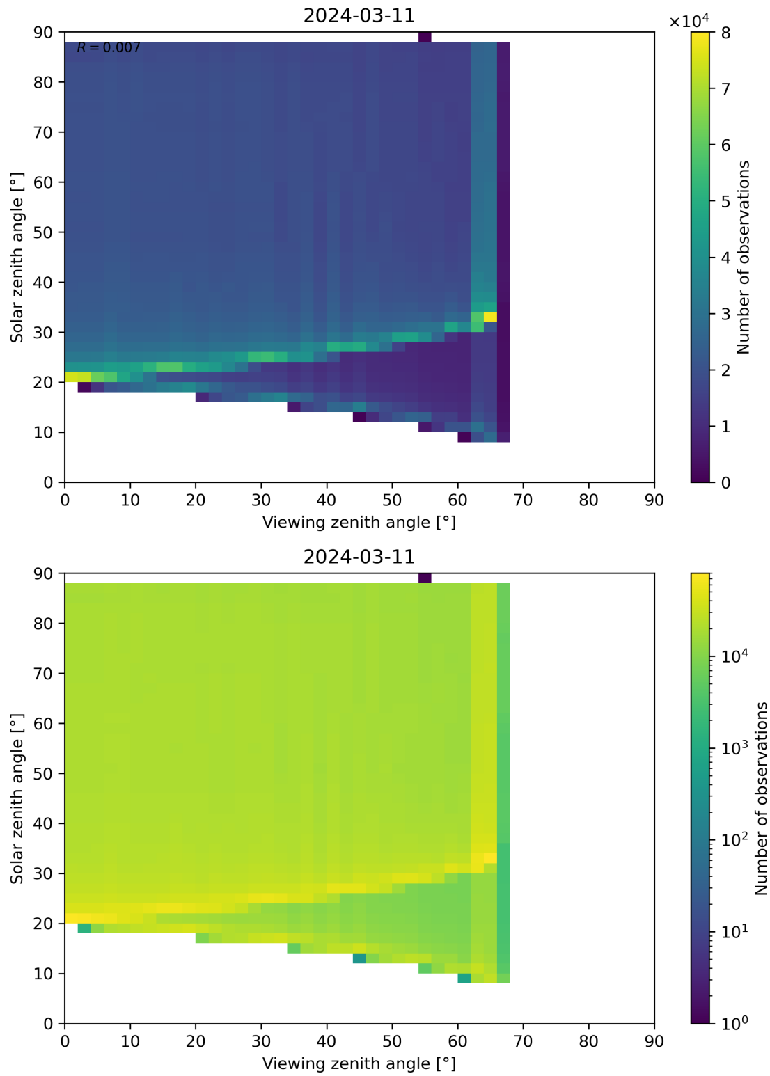
Figure 172: Scatter density plot of “Viewing zenith angle” against “Solar zenith angle” for 2024-03-10 to 2024-03-12.
