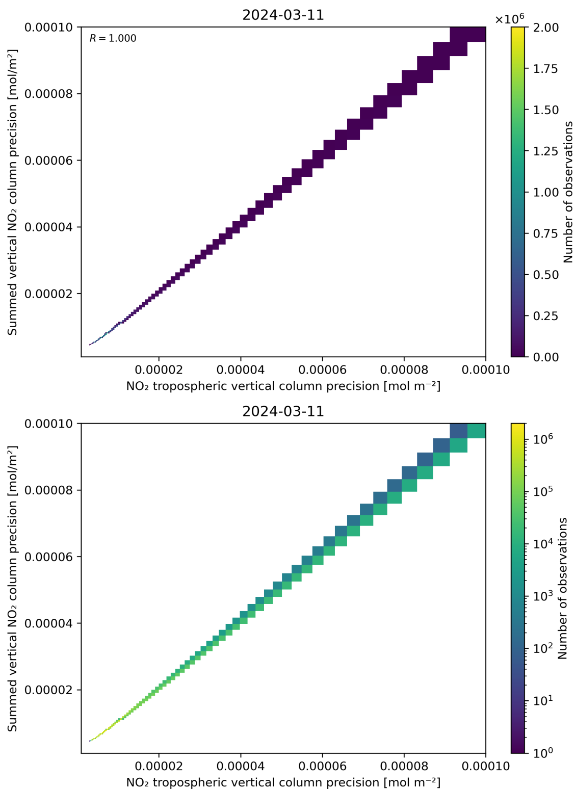
Figure 137: Scatter density plot of “NO 2 tropospheric vertical column precision” against “Summed vertical NO 2 column precision” for 2024-03-10 to 2024-03-12.
