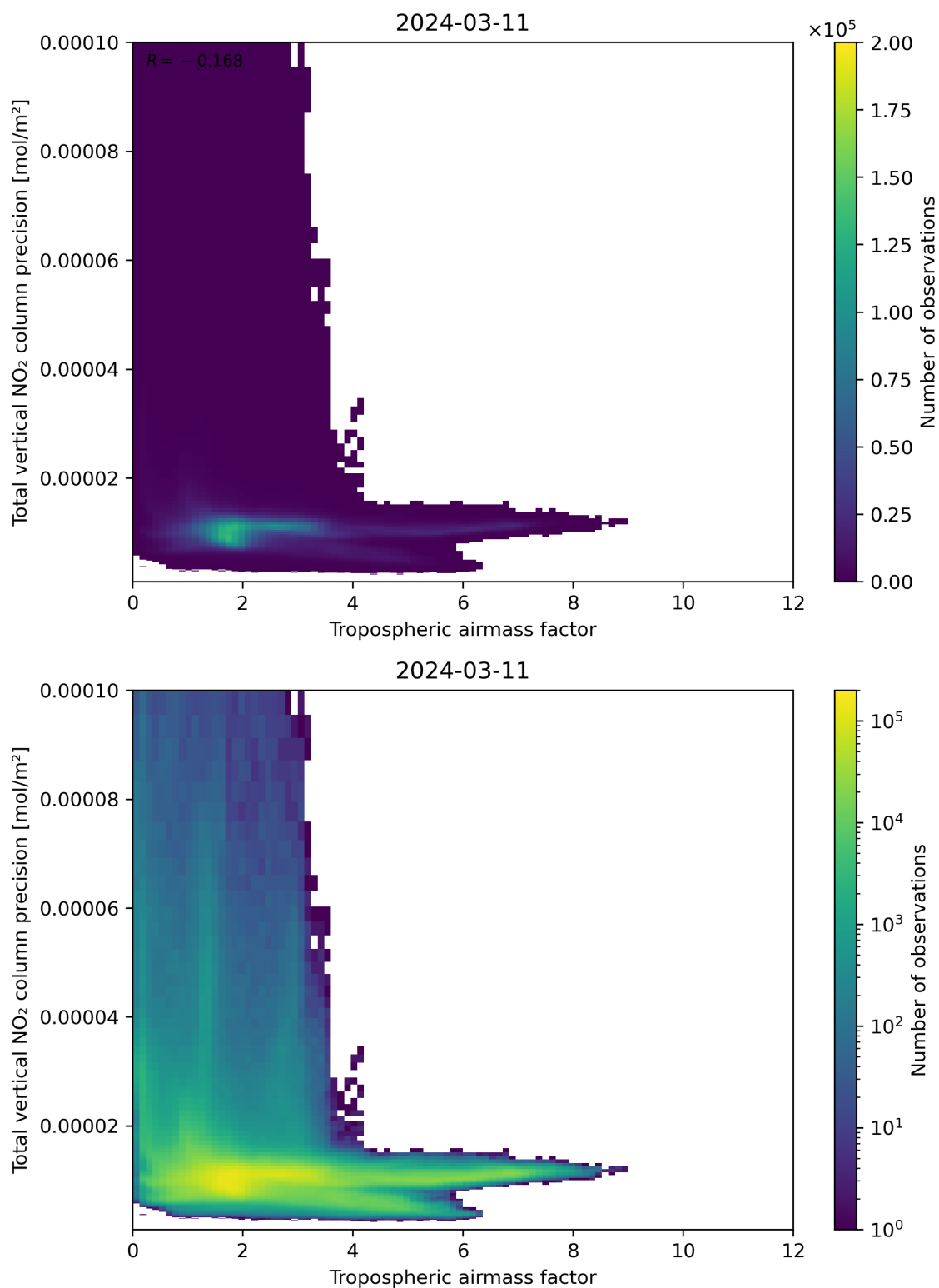
Figure 78: Scatter density plot of “Tropospheric airmass factor” against “Total vertical NO 2 column precision” for 2024-03-10 to 2024-03-12.
