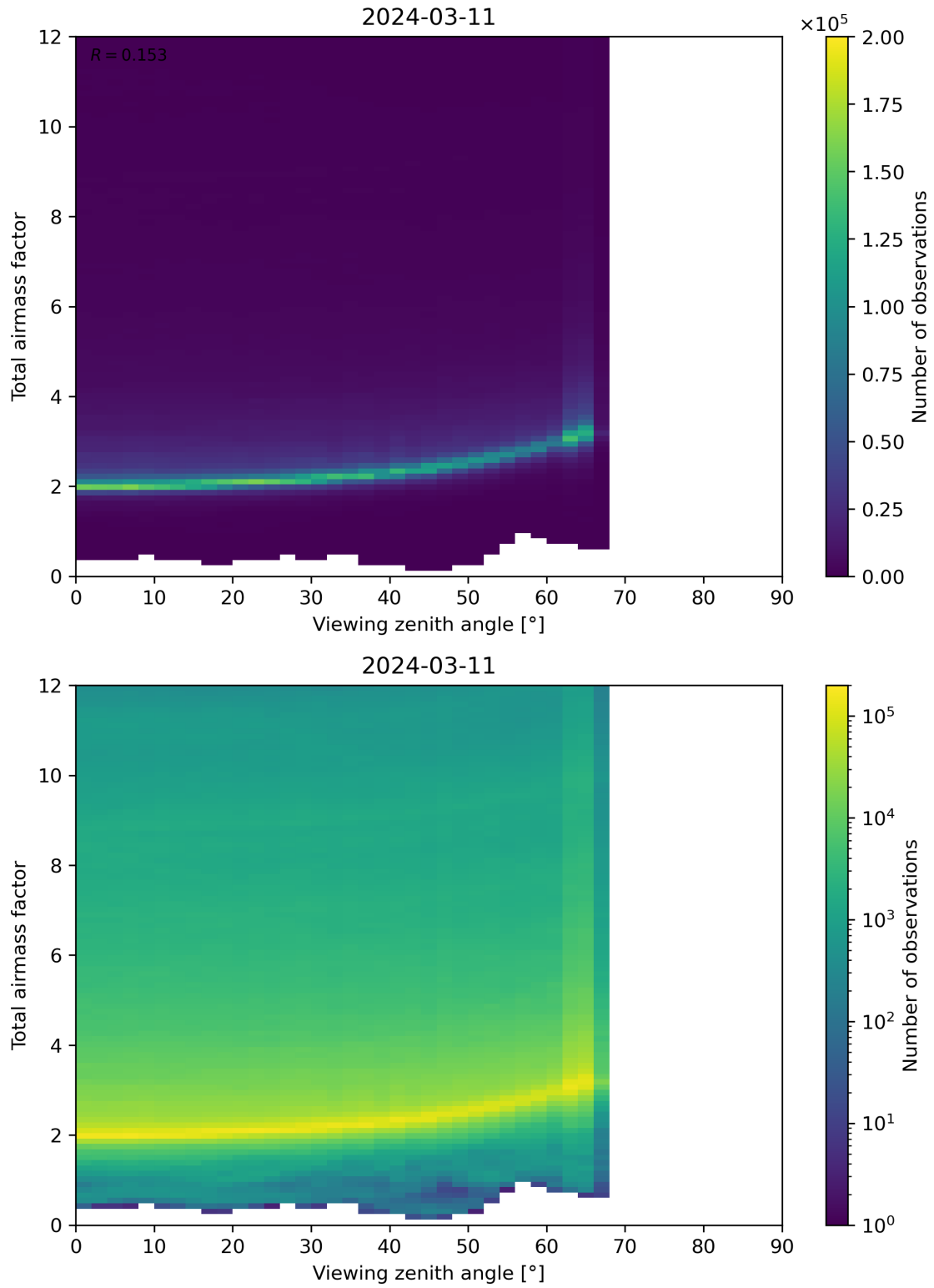
Figure 160: Scatter density plot of “Viewing zenith angle” against “Total airmass factor” for 2024-03-10 to 2024-03-12.
