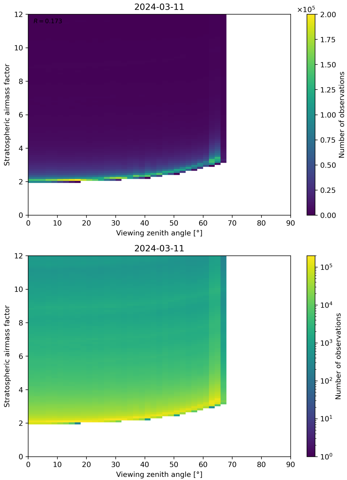
Figure 159: Scatter density plot of “Viewing zenith angle” against “Stratospheric airmass factor” for 2024-03-10 to 2024-03-12.
