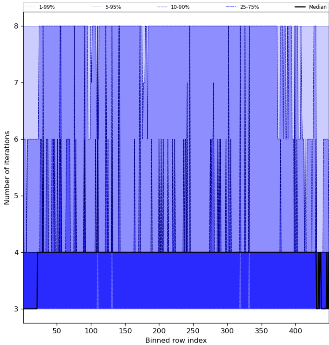
Figure 51: Along track statistics of “Number of iterations” for 2024-03-10 to 2024-03-12
