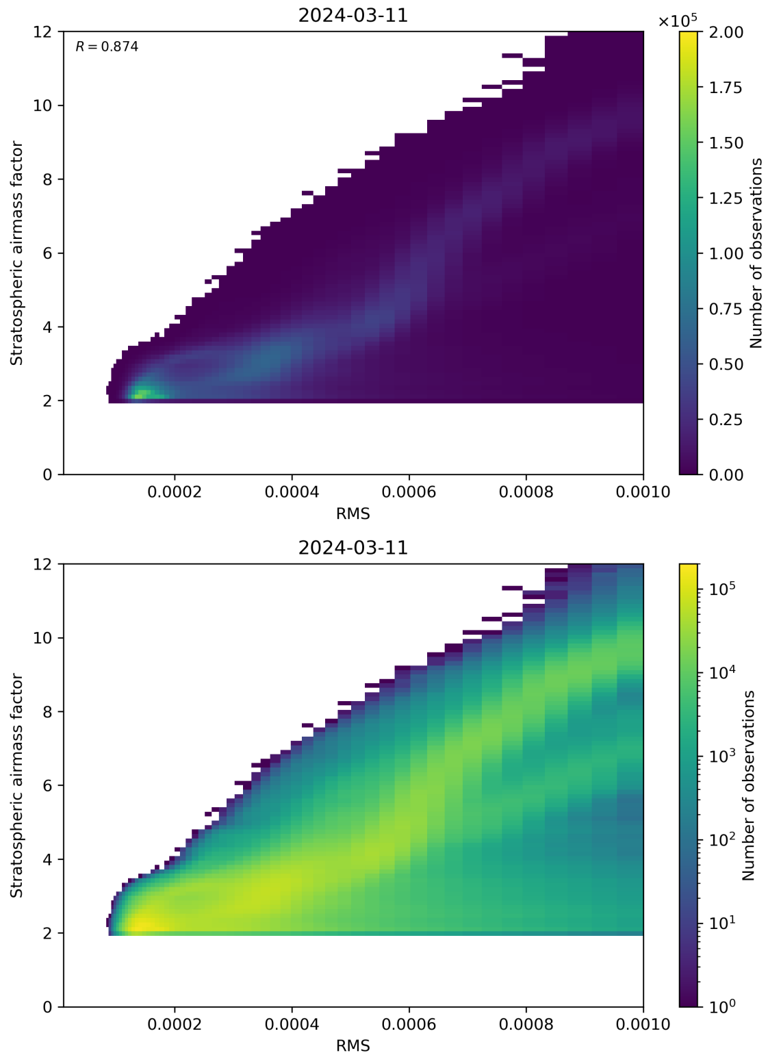
Figure 144: Scatter density plot of “RMS” against “Stratospheric airmass factor” for 2024-03-10 to 2024-03-12.
