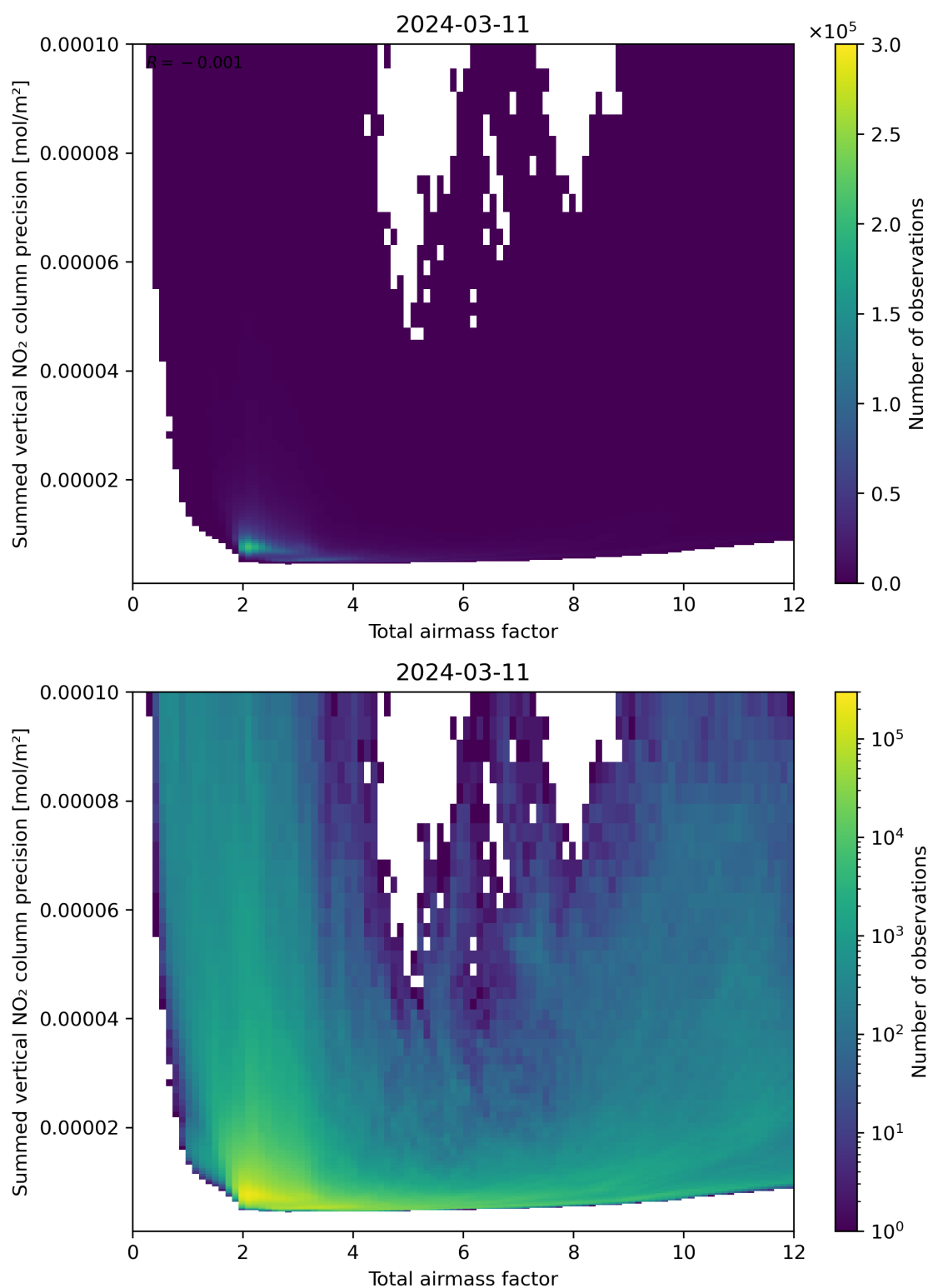
Figure 66: Scatter density plot of “Total airmass factor” against “Summed vertical NO 2 column precision” for 2024-03-10 to 2024-03-12.
