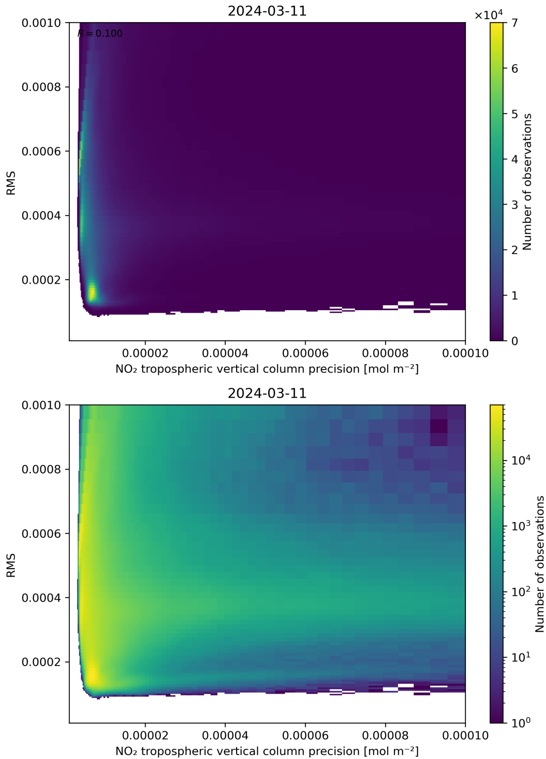
Figure 140: Scatter density plot of “NO 2 tropospheric vertical column precision” against “RMS” for 2024-03-10 to 2024-03-12.
