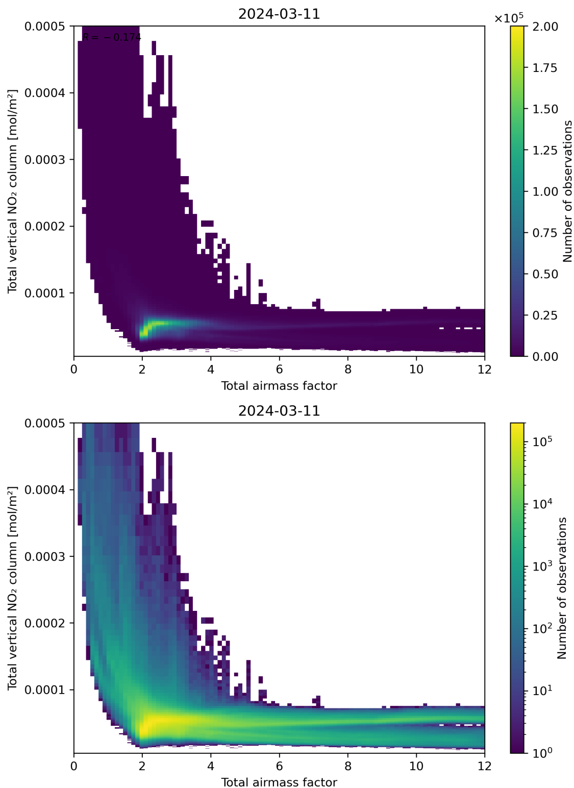
Figure 67: Scatter density plot of “Total airmass factor” against “Total vertical NO 2 column” for 2024-03-10 to 2024-03-12.
