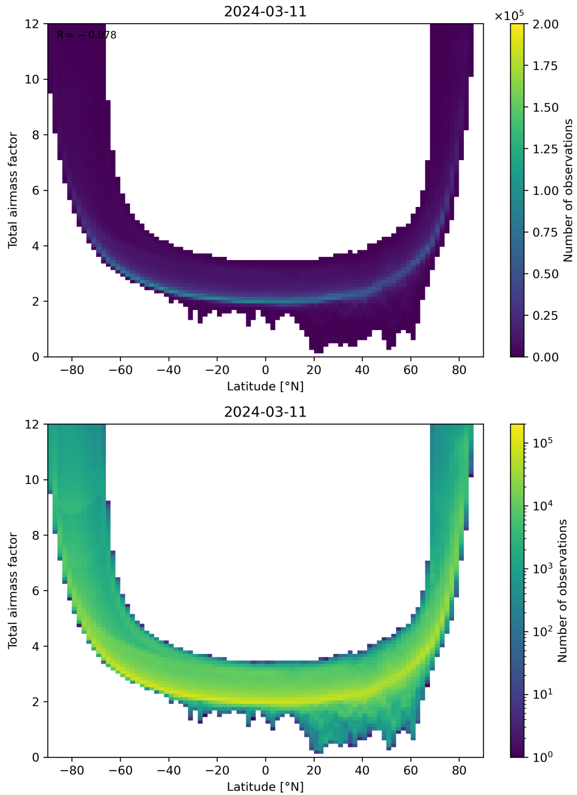
Figure 84: Scatter density plot of “Latitude” against “Total airmass factor” for 2024-03-10 to 2024-03-12.
