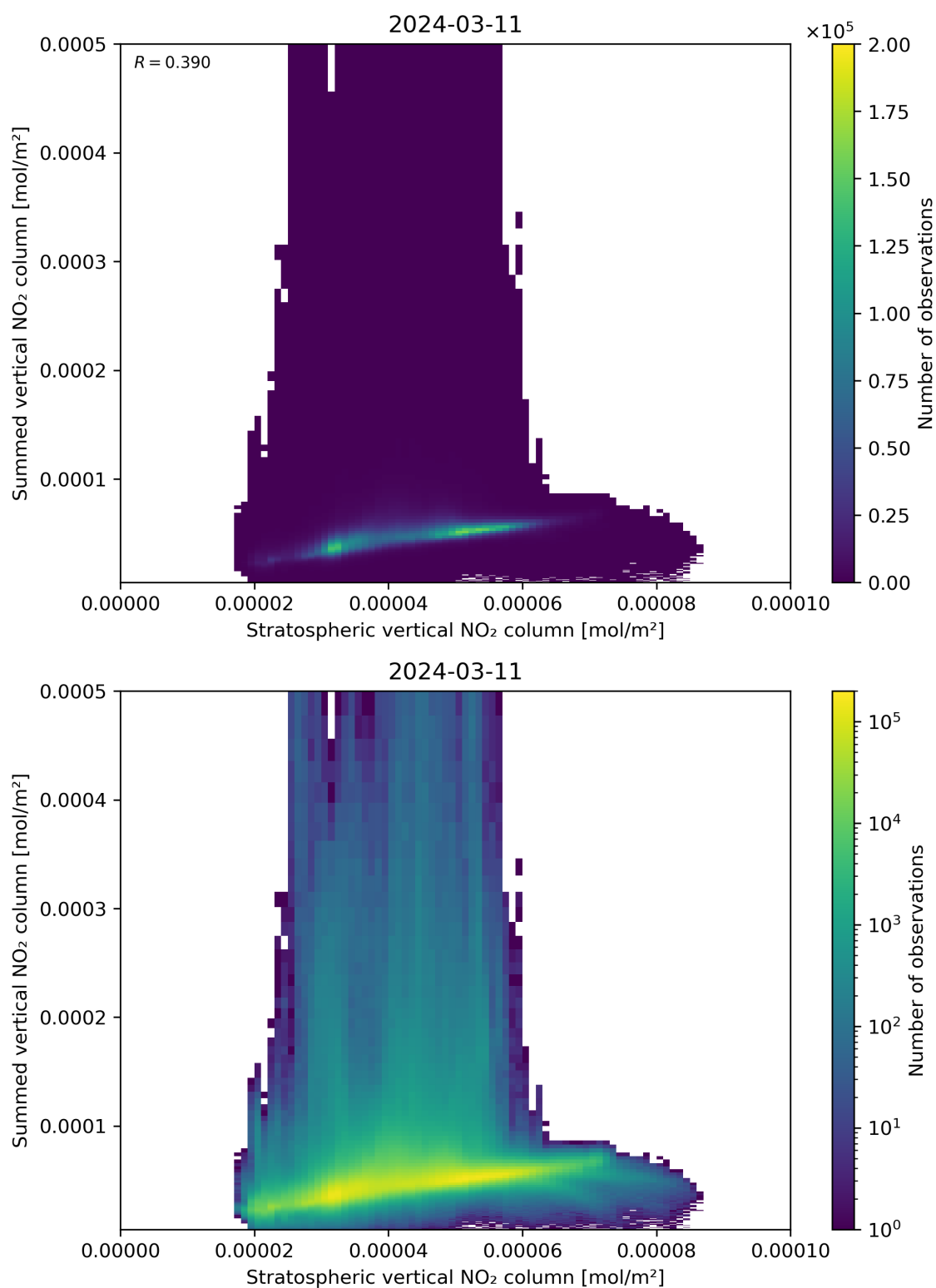
Figure 98: Scatter density plot of “Stratospheric vertical NO 2 column” against “Summed vertical NO 2 column” for 2024-03-10 to 2024-03-12.
