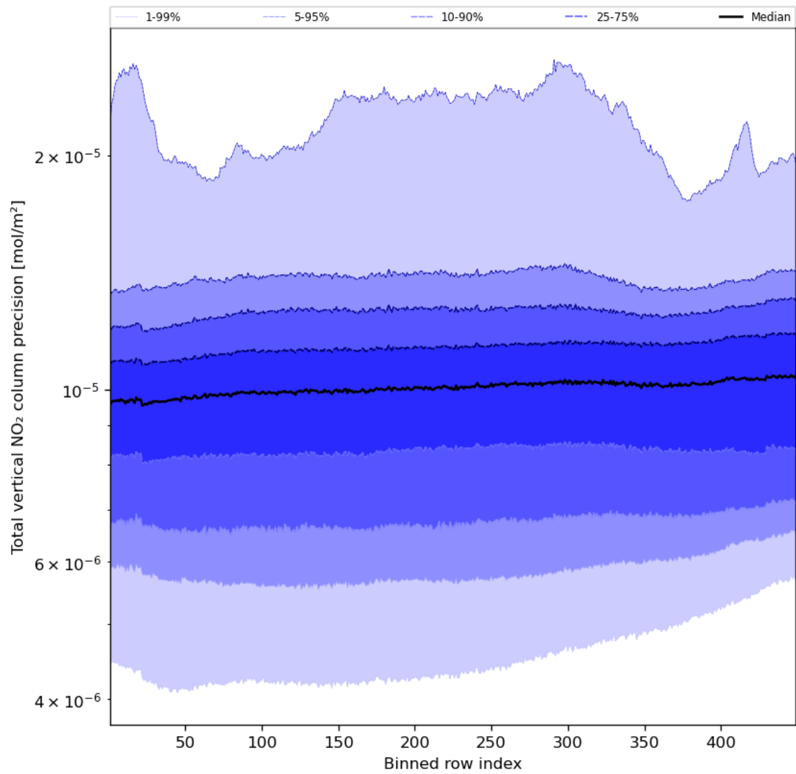
Figure 56: Along track statistics of “Total vertical NO 2 column precision” for 2024-03-10 to 2024-03-12
