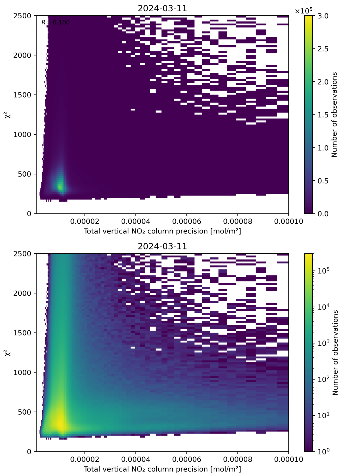
Figure 116: Scatter density plot of “Total vertical NO 2 column precision” against “ \chi^2 ” for 2024-03-10 to 2024-03-12.
