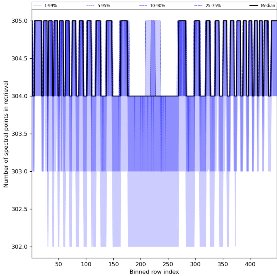
Figure 50: Along track statistics of “Number of spectral points in retrieval” for 2024-03-10 to 2024-03-12
