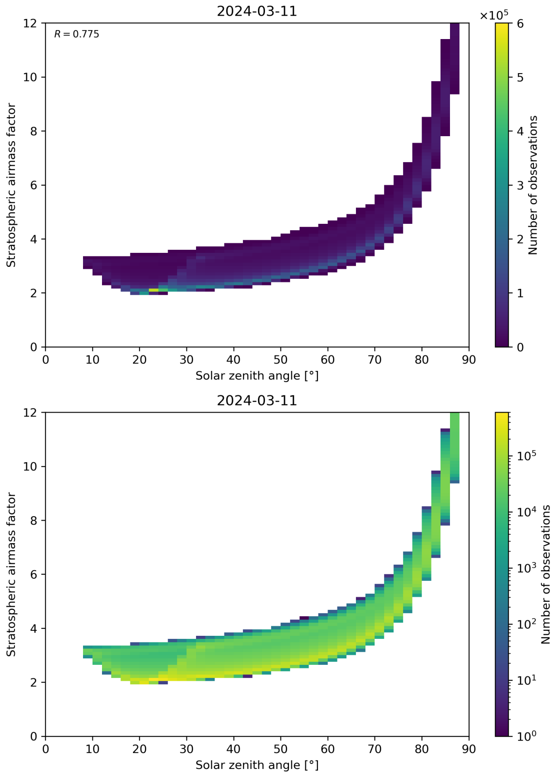
Figure 145: Scatter density plot of “Solar zenith angle” against “Stratospheric airmass factor” for 2024-03-10 to 2024-03-12.
