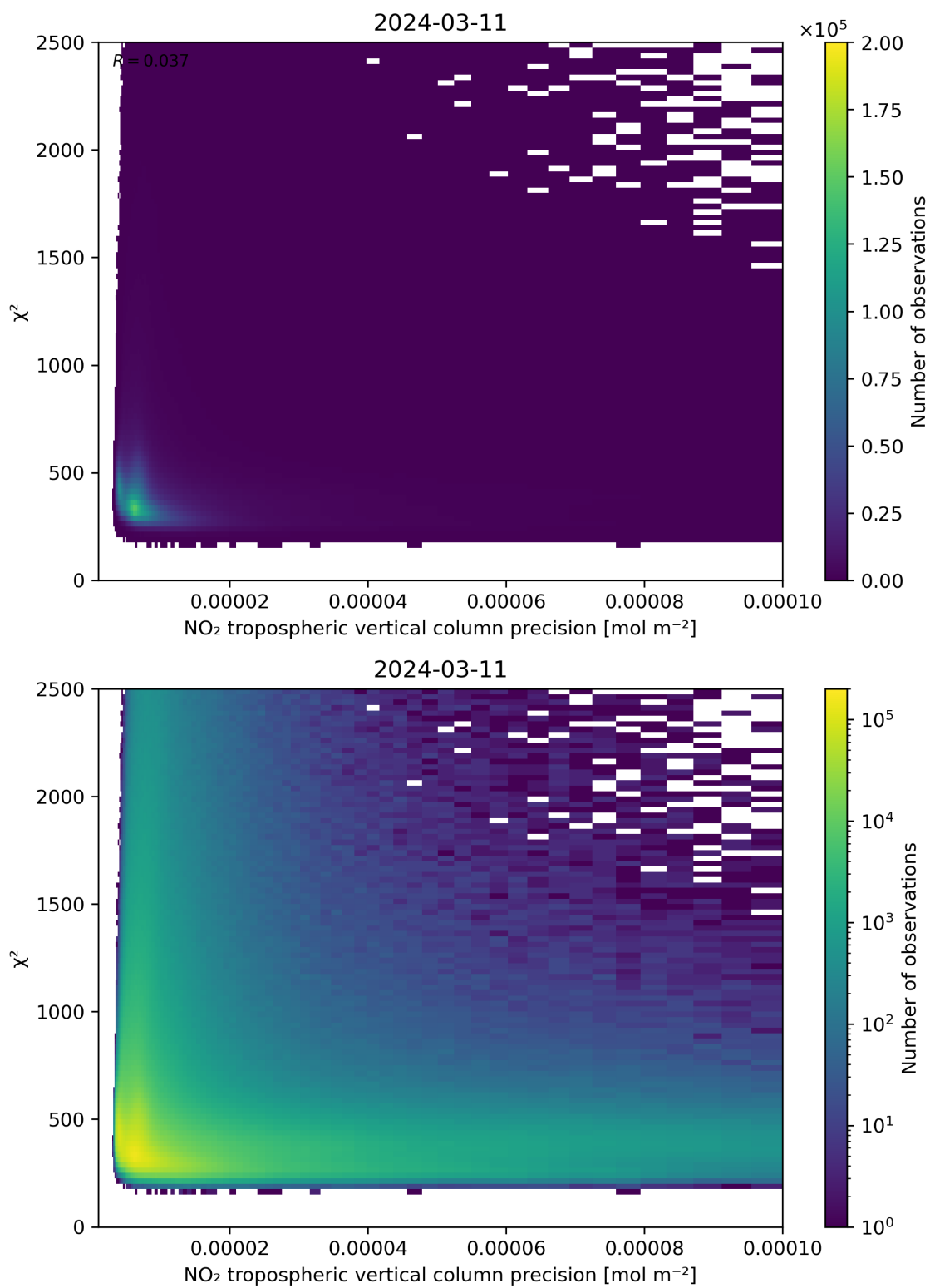
Figure 134: Scatter density plot of “NO 2 tropospheric vertical column precision” against “ \chi^2 ” for 2024-03-10 to 2024-03-12.
