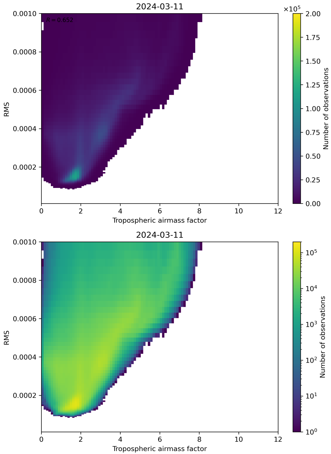
Figure 79: Scatter density plot of “Tropospheric airmass factor” against “RMS” for 2024-03-10 to 2024-03-12.
