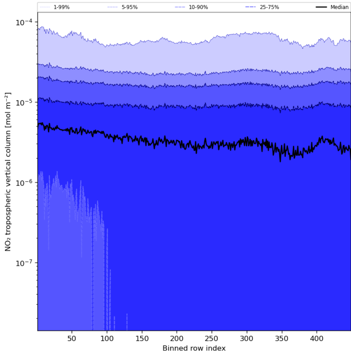
Figure 46: Along track statistics of “NO 2 tropospheric vertical column” for 2024-03-10 to 2024-03-12
