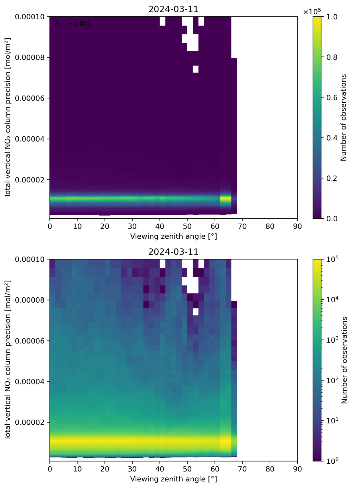
Figure 168: Scatter density plot of “Viewing zenith angle” against “Total vertical NO 2 column precision” for 2024-03-10 to 2024-03-12.
