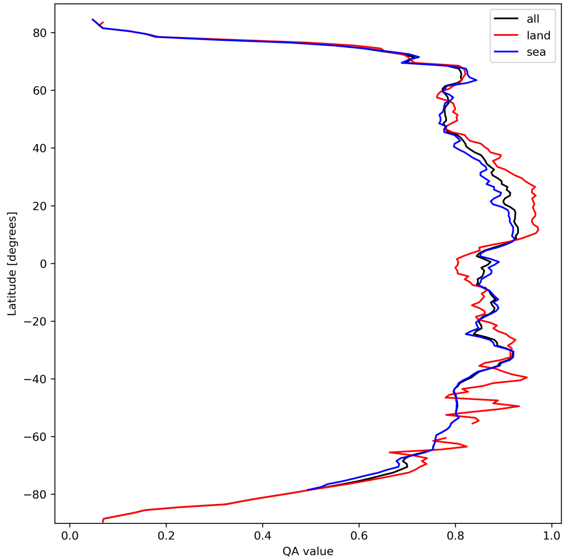
Figure 11: Zonal average of “QA value” for 2024-03-10 to 2024-03-12.
