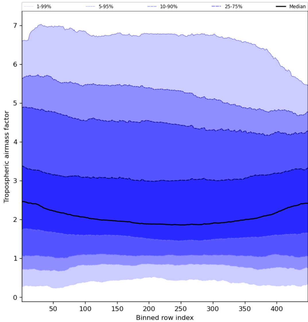
Figure 48: Along track statistics of “Tropospheric airmass factor” for 2024-03-10 to 2024-03-12
