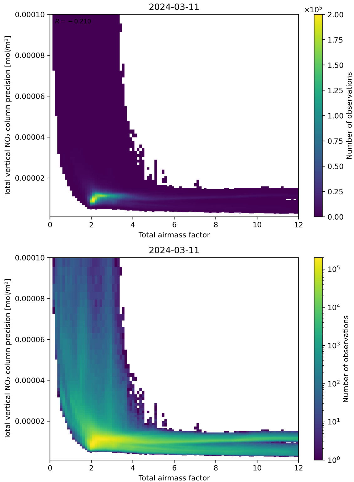
Figure 68: Scatter density plot of “Total airmass factor” against “Total vertical NO 2 column precision” for 2024-03-10 to 2024-03-12.
