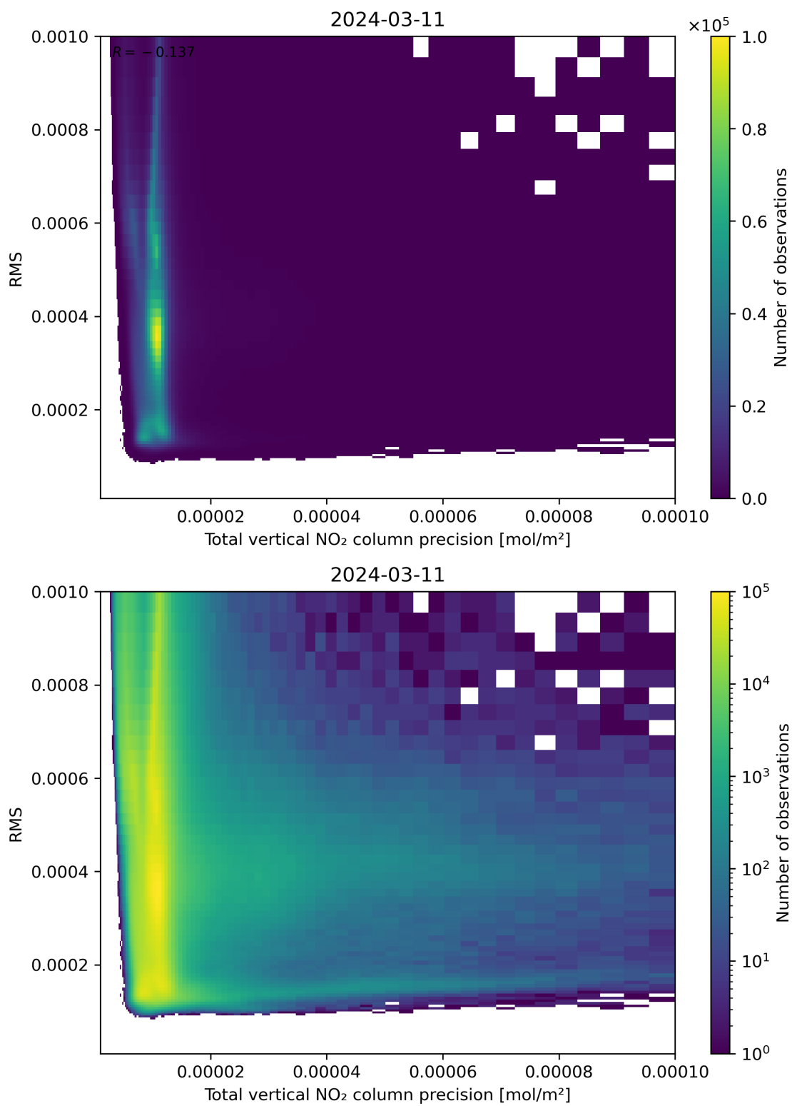
Figure 119: Scatter density plot of “Total vertical NO 2 column precision” against “RMS” for 2024-03-10 to 2024-03-12.
