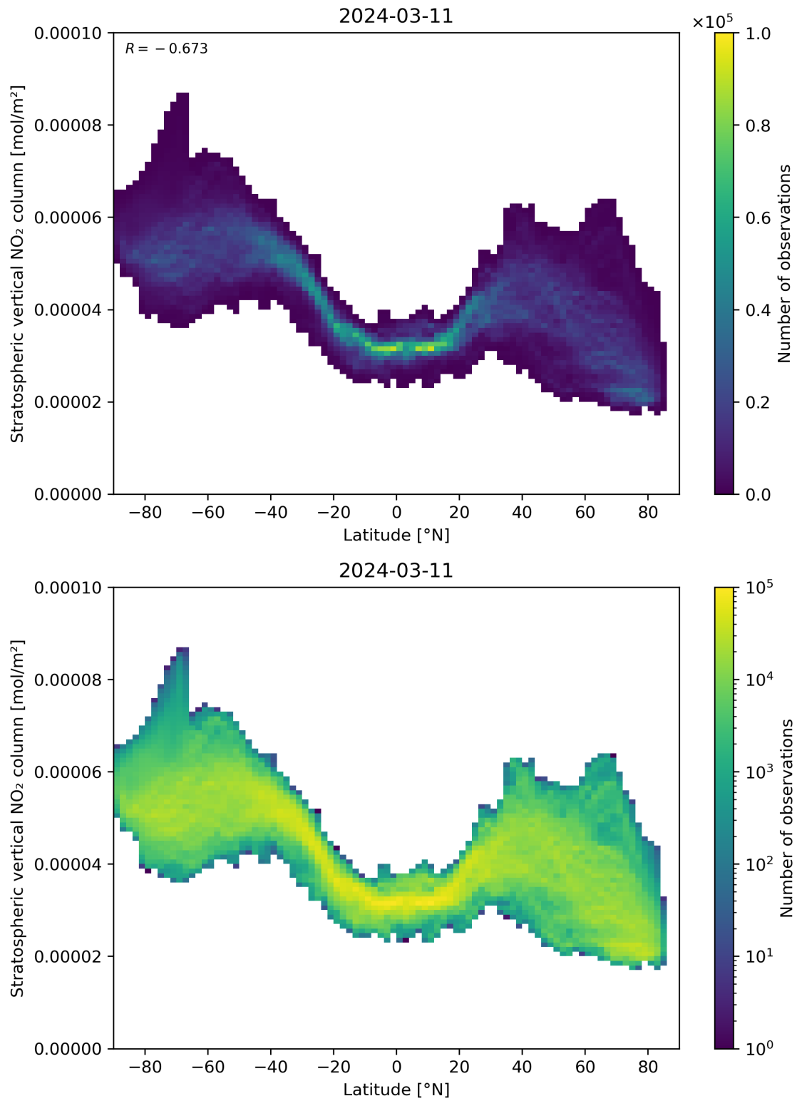
Figure 87: Scatter density plot of “Latitude” against “Stratospheric vertical NO 2 column” for 2024-03-10 to 2024-03-12.
