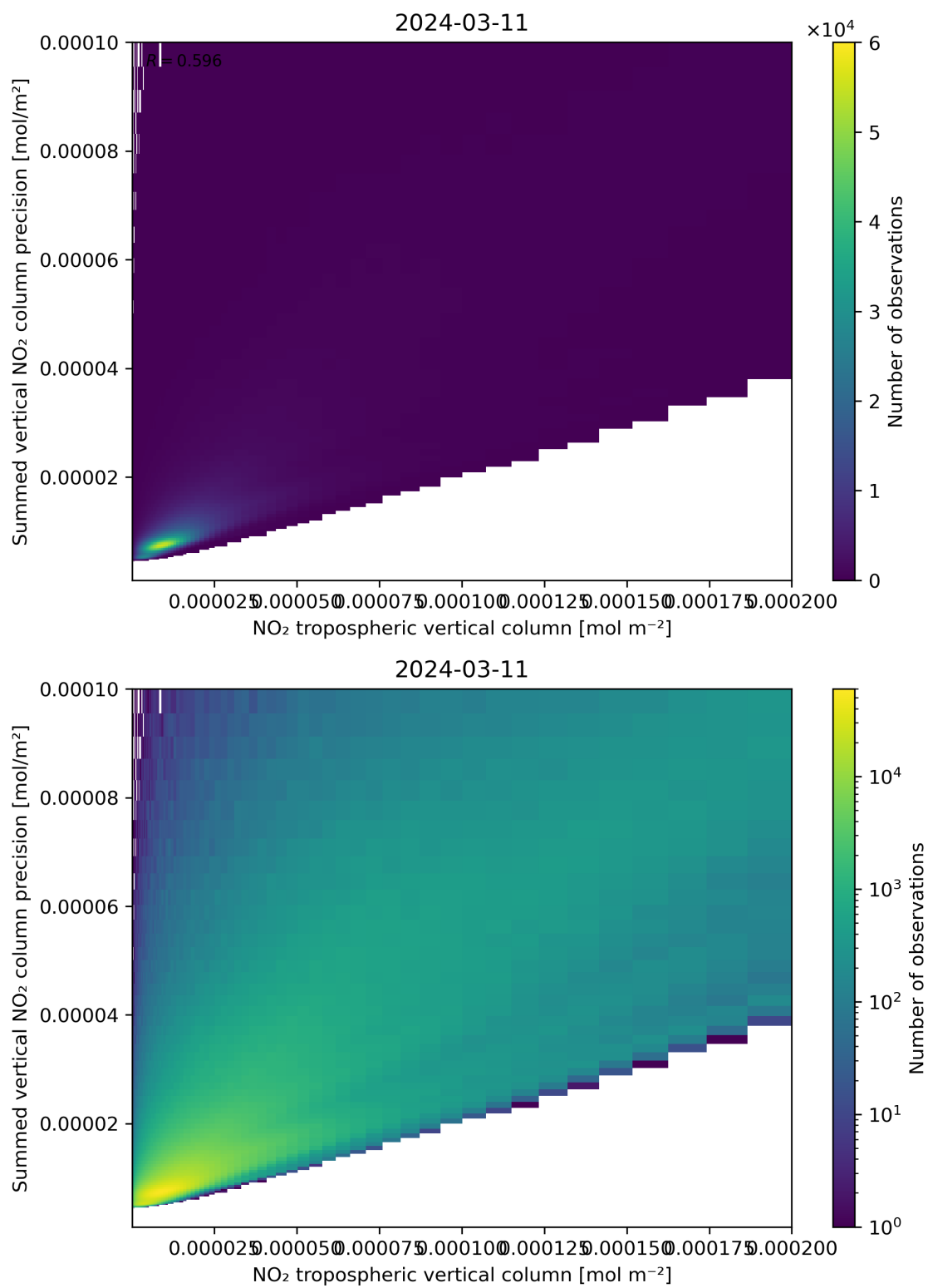
Figure 127: Scatter density plot of “NO 2 tropospheric vertical column” against “Summed vertical NO 2 column precision” for 2024-03-10 to 2024-03-12.
