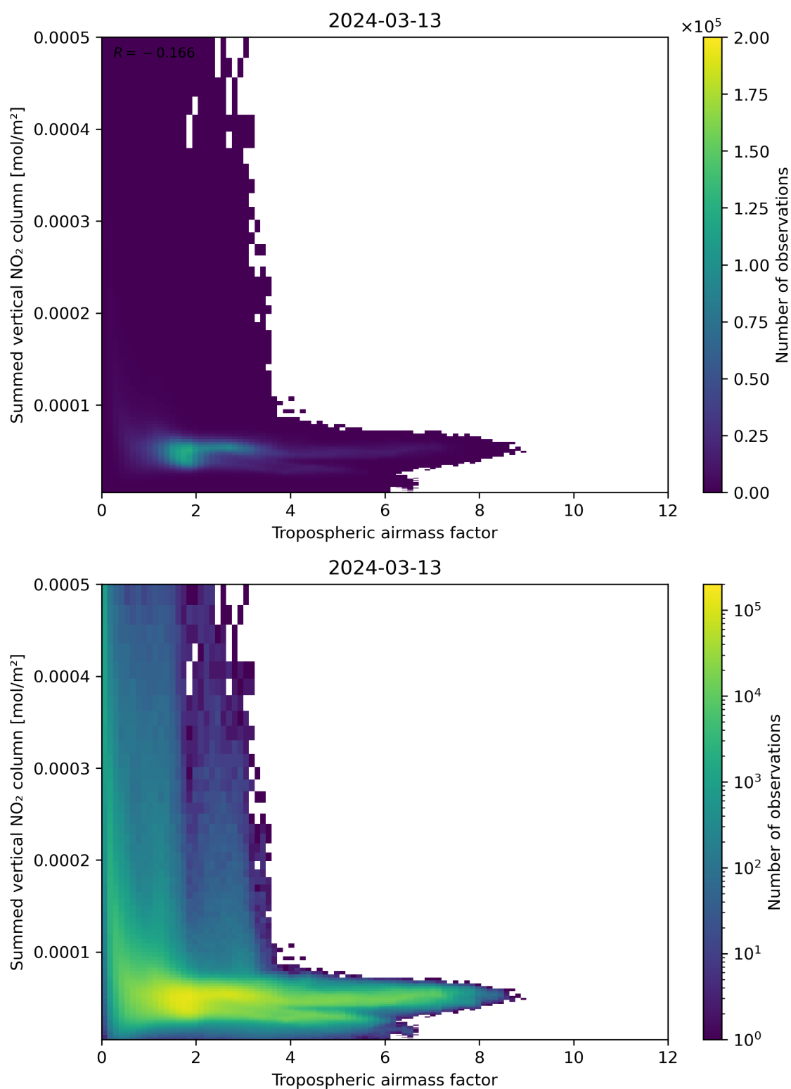
Figure 75: Scatter density plot of “Tropospheric airmass factor” against “Summed vertical NO 2 column” for 2024-03-12 to 2024-03-14.
