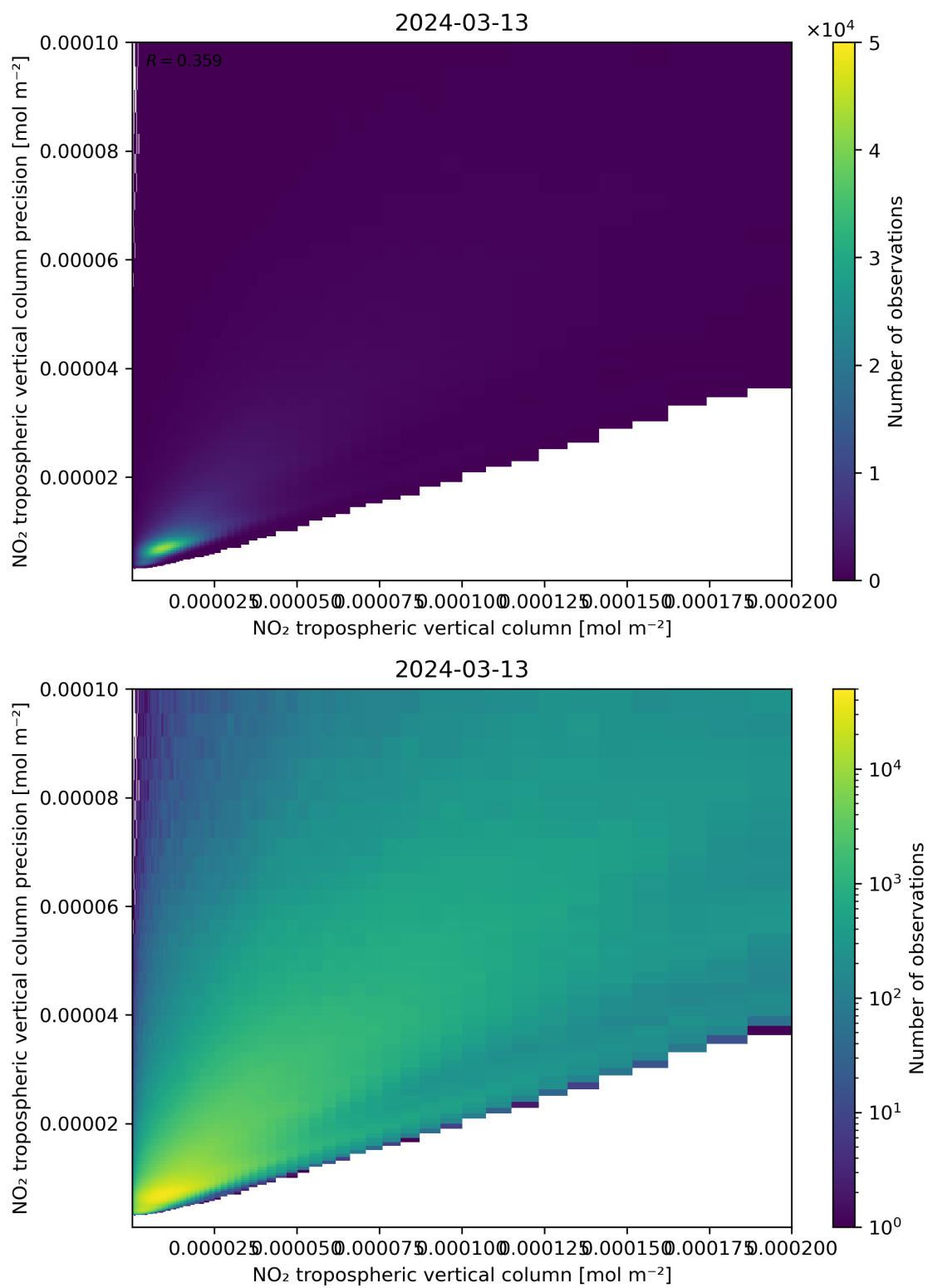
Figure 130: Scatter density plot of “NO 2 tropospheric vertical column” against “NO 2 tropospheric vertical column precision” for 2024-03-12 to 2024-03-14.
