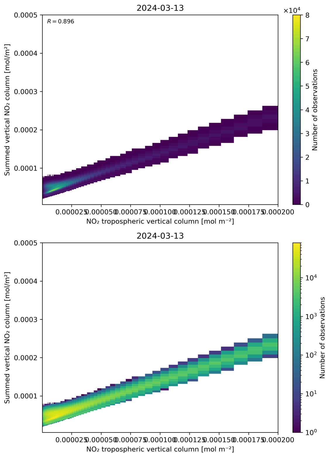
Figure 126: Scatter density plot of “NO 2 tropospheric vertical column” against “Summed vertical NO 2 column” for 2024-03-12 to 2024-03-14.
