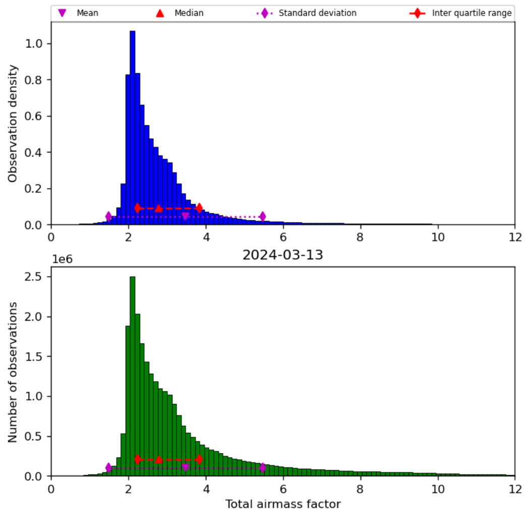
Figure 32: Histogram of “Total airmass factor” for 2024-03-12 to 2024-03-14
