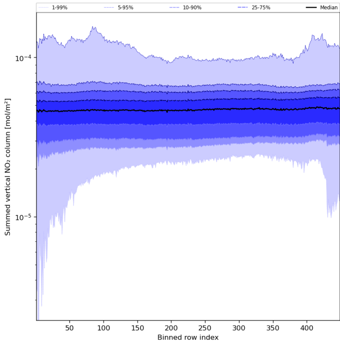
Figure 57: Along track statistics of “Summed vertical NO 2 column” for 2024-03-12 to 2024-03-14
