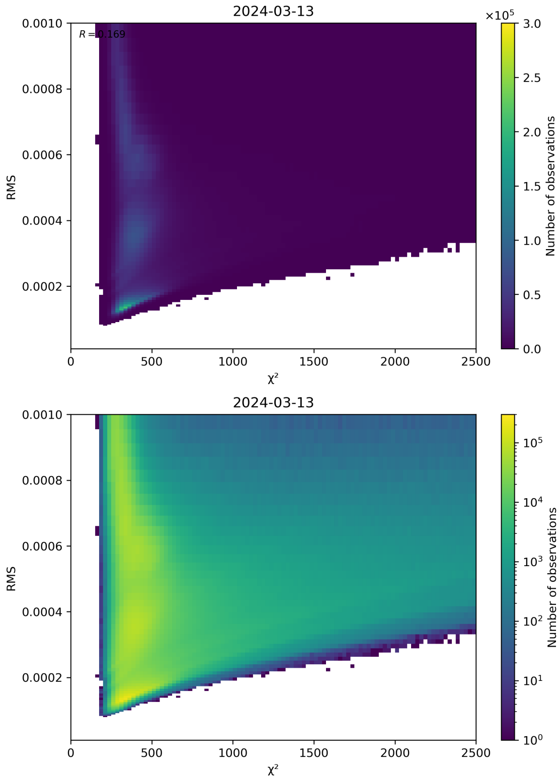
Figure 82: Scatter density plot of “ \chi^2 ” against “RMS” for 2024-03-12 to 2024-03-14.
