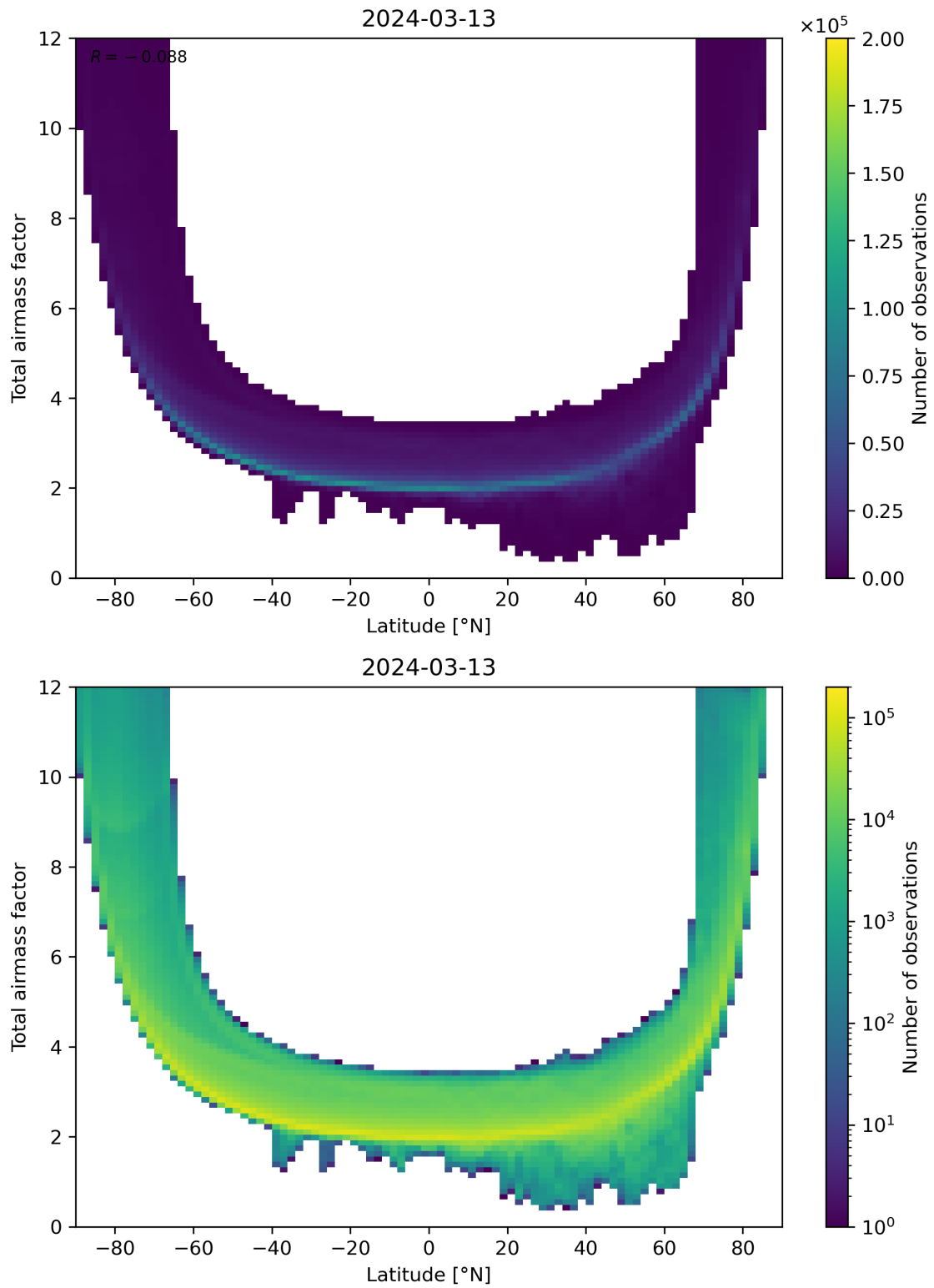
Figure 84: Scatter density plot of “Latitude” against “Total airmass factor” for 2024-03-12 to 2024-03-14.
