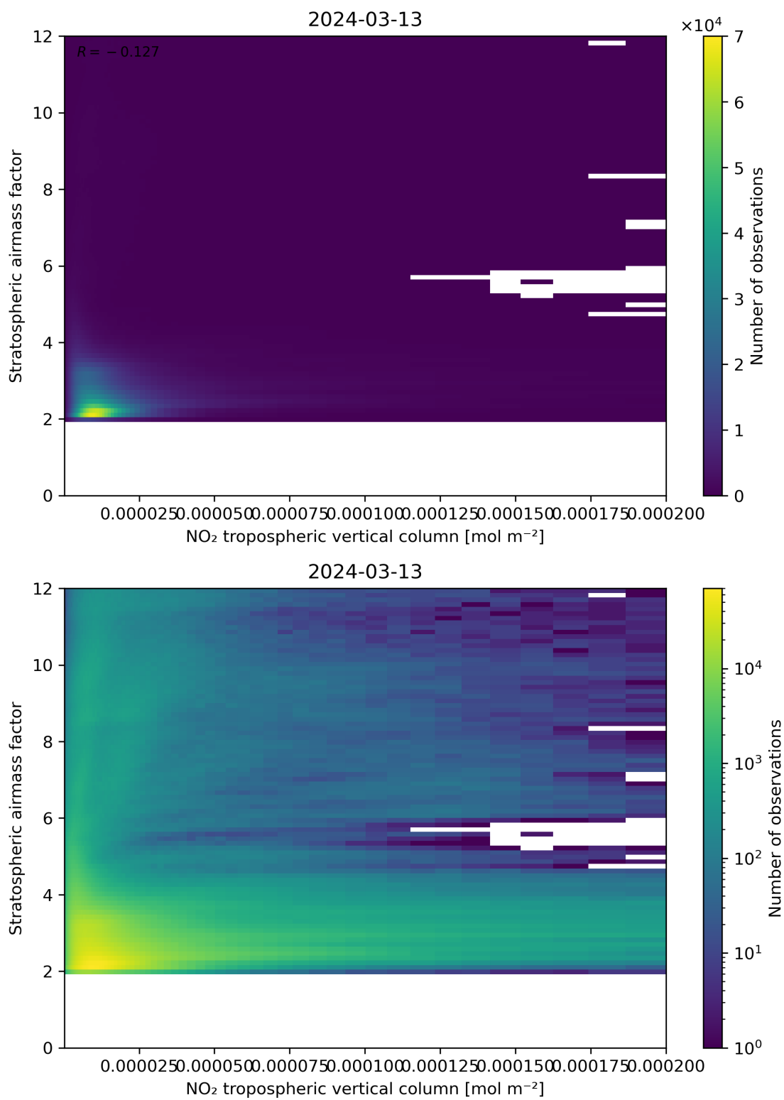
Figure 121: Scatter density plot of “NO 2 tropospheric vertical column” against “Stratospheric airmass factor” for 2024-03-12 to 2024-03-14.
