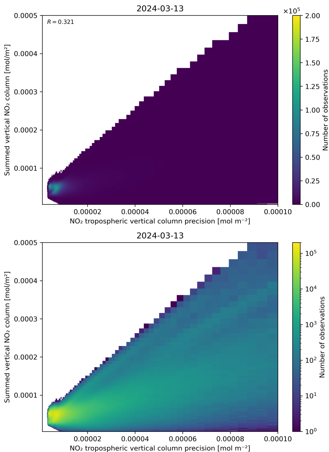
Figure 136: Scatter density plot of “NO 2 tropospheric vertical column precision” against “Summed vertical NO 2 column” for 2024-03-12 to 2024-03-14.
