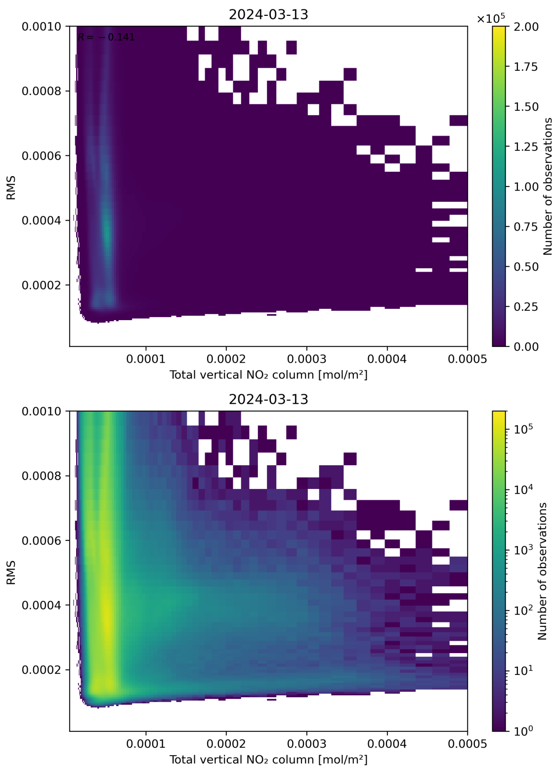
Figure 120: Scatter density plot of “Total vertical NO 2 column” against “RMS” for 2024-03-12 to 2024-03-14.
