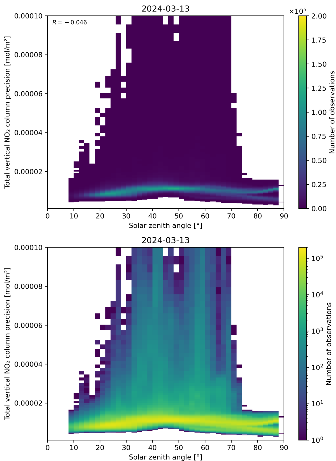
Figure 154: Scatter density plot of “Solar zenith angle” against “Total vertical NO 2 column precision” for 2024-03-12 to 2024-03-14.
