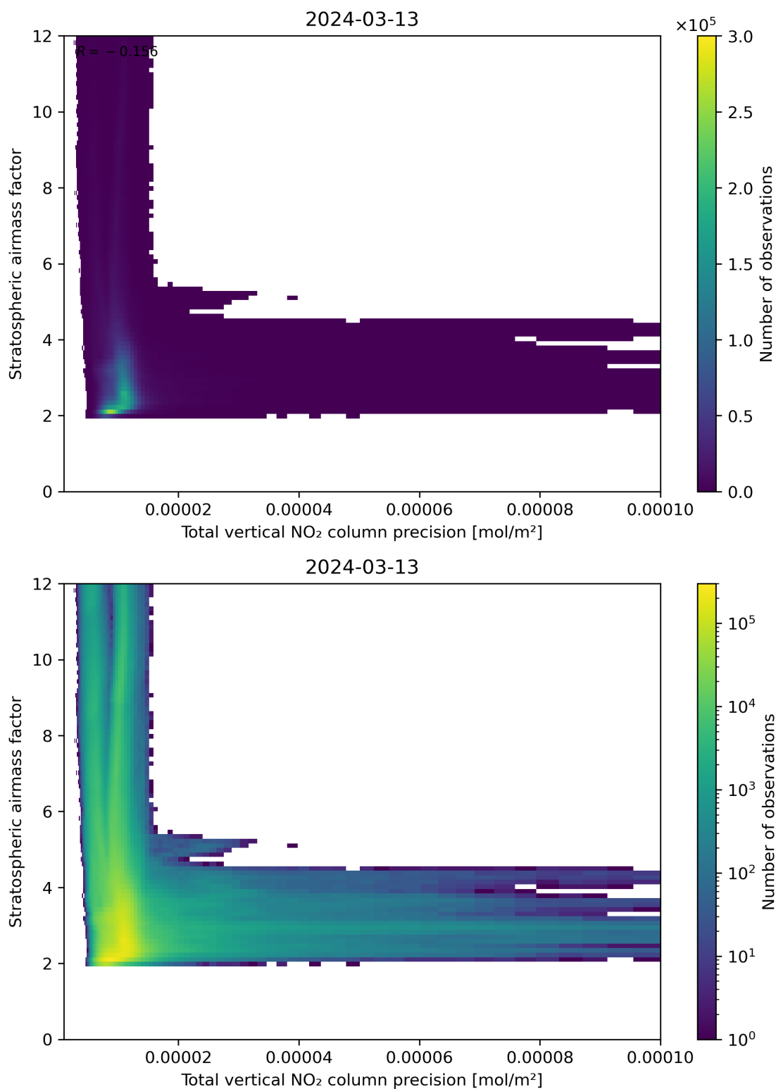
Figure 115: Scatter density plot of “Total vertical NO 2 column precision” against “Stratospheric airmass factor” for 2024-03-12 to 2024-03-14.
