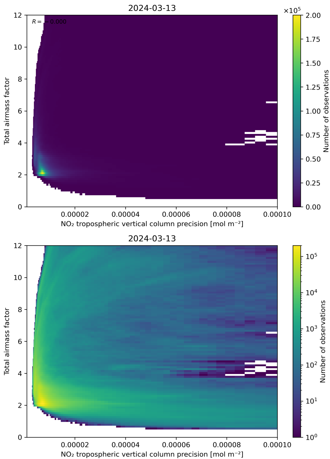
Figure 132: Scatter density plot of “NO 2 tropospheric vertical column precision” against “Total air mass factor” for 2024-03-12 to 2024-03-14.
