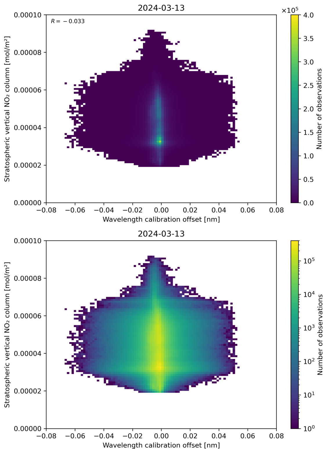
Figure 176: Scatter density plot of “Wavelength calibration offset” against “Stratospheric vertical NO 2 column” for 2024-03-12 to 2024-03-14.
