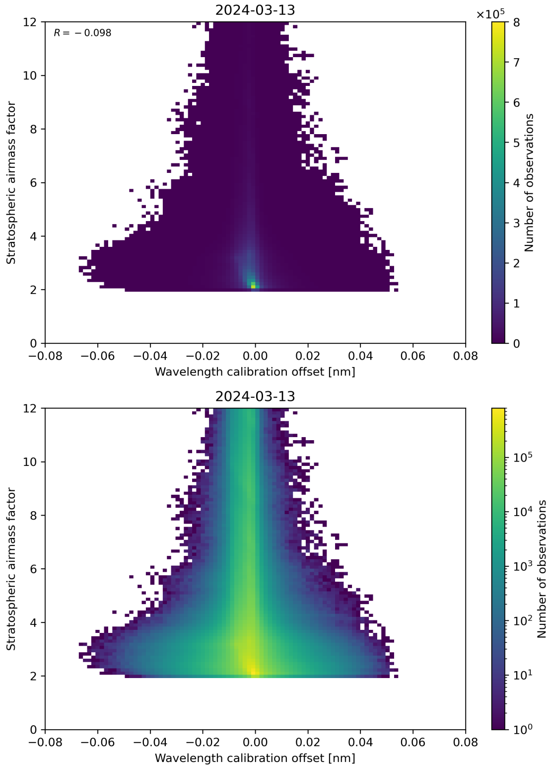
Figure 174: Scatter density plot of “Wavelength calibration offset” against “Stratospheric air mass factor” for 2024-03-12 to 2024-03-14.
