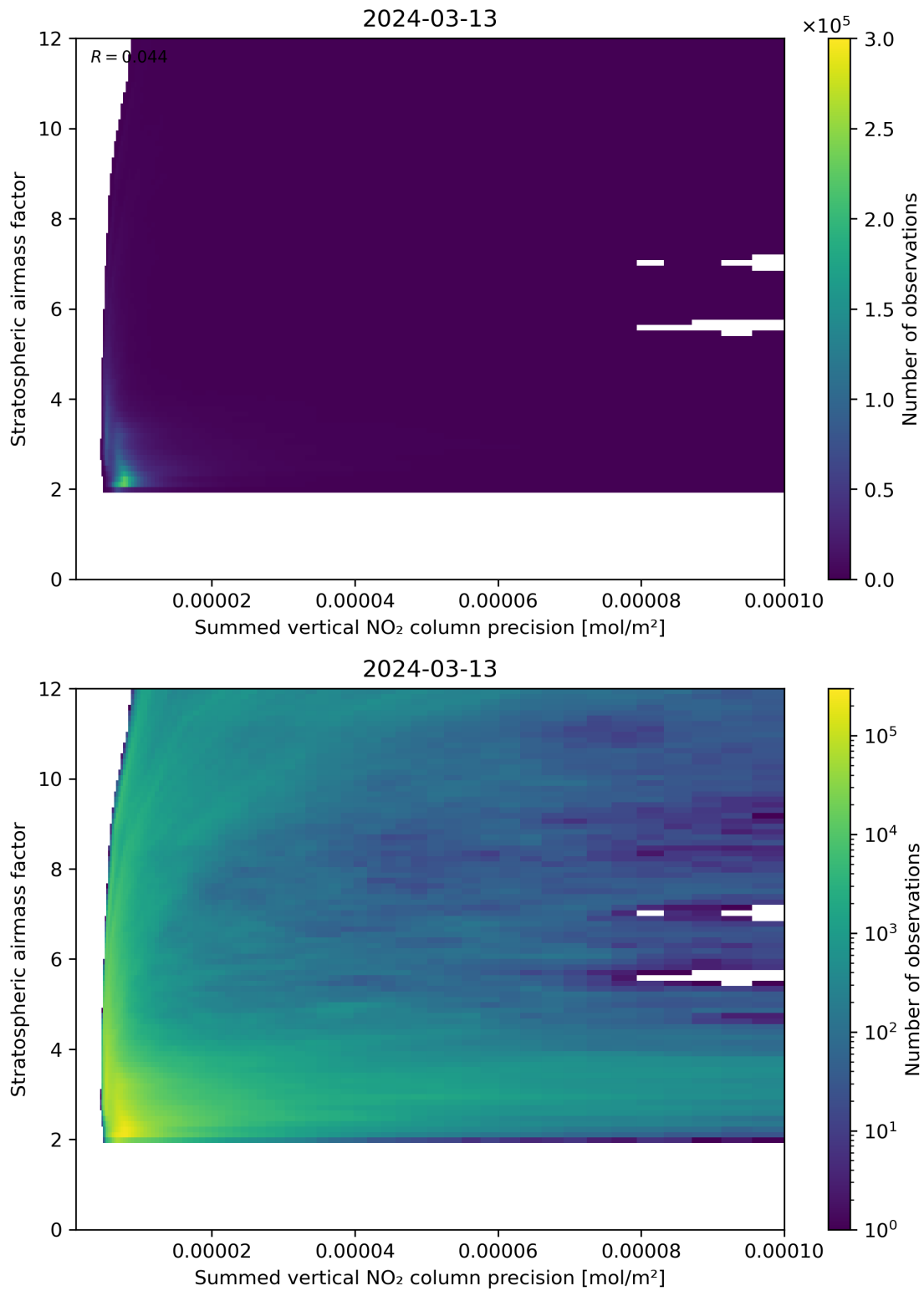
Figure 106: Scatter density plot of “Summed vertical NO 2 column precision” against “Stratospheric airmass factor” for 2024-03-12 to 2024-03-14.
