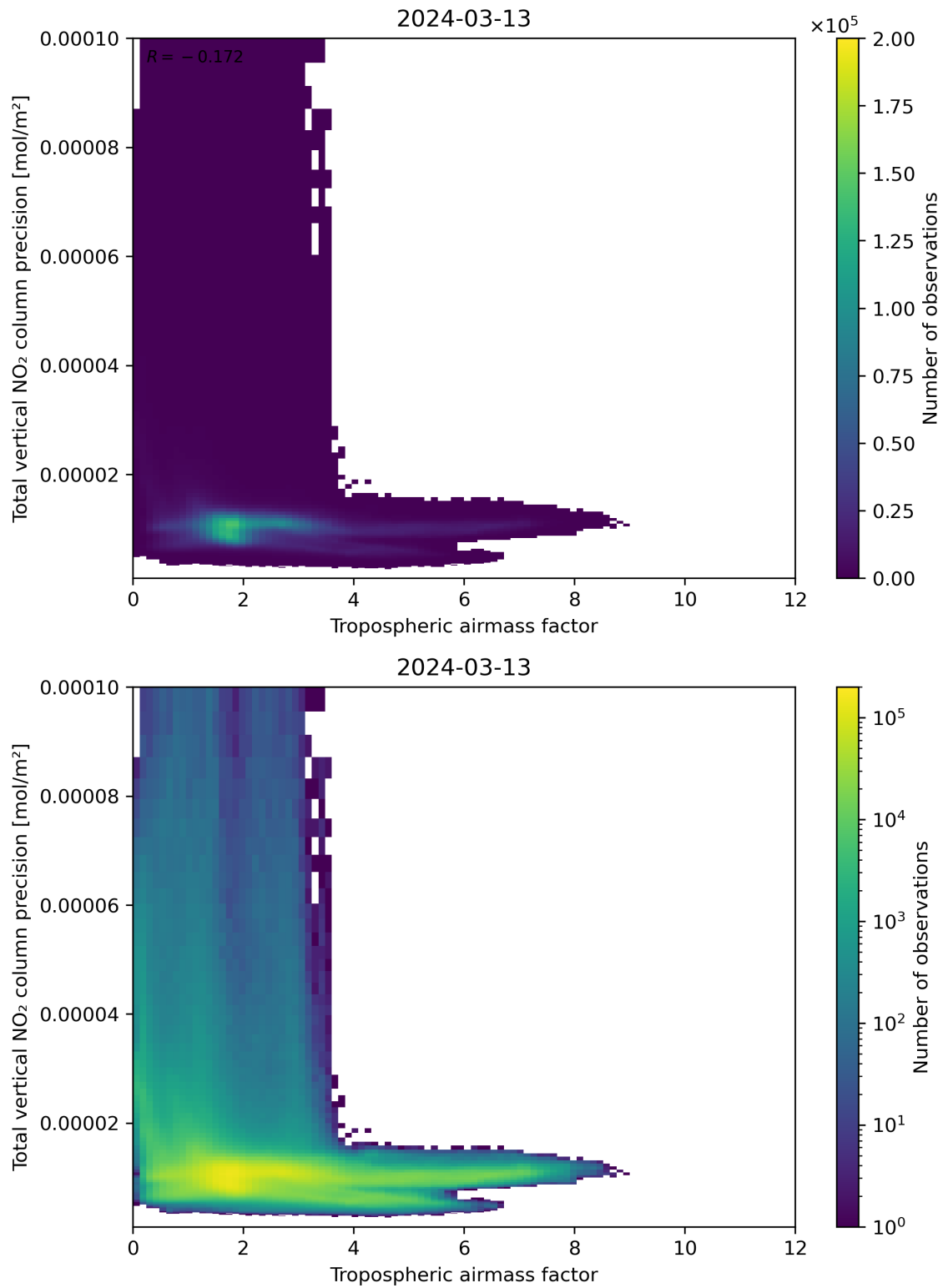
Figure 78: Scatter density plot of “Tropospheric air mass factor” against “Total vertical NO 2 column precision” for 2024-03-12 to 2024-03-14.
