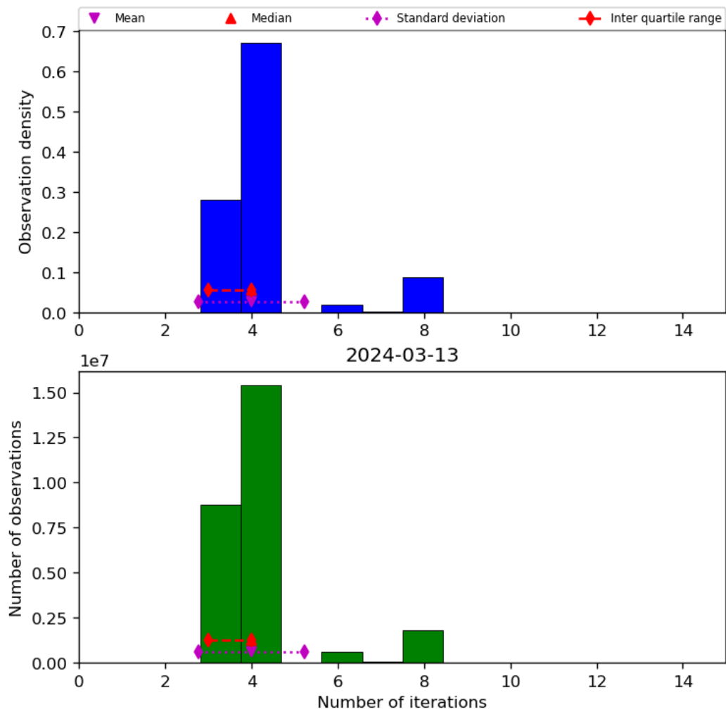
Figure 34: Histogram of “Number of iterations” for 2024-03-12 to 2024-03-14
