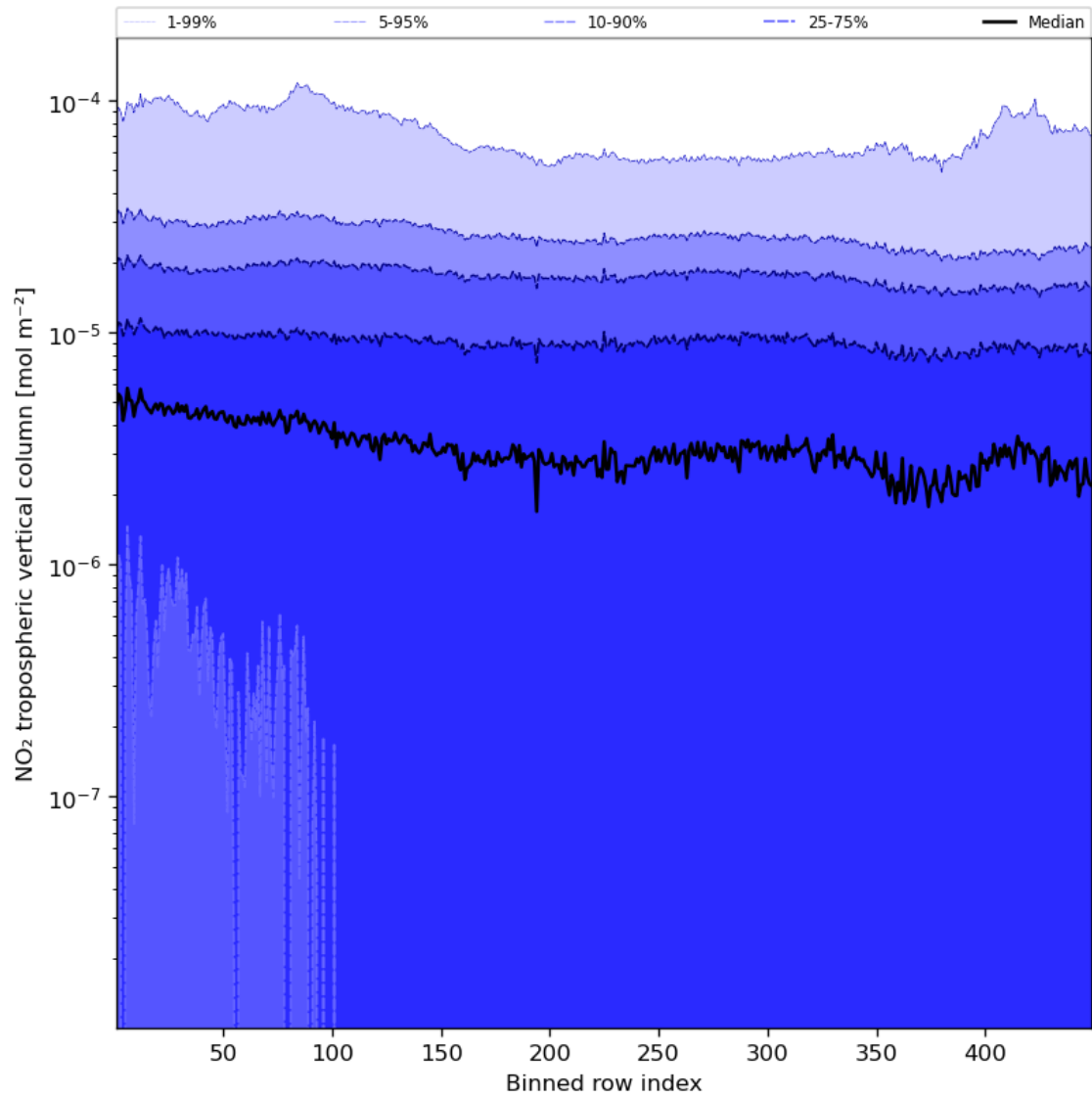
Figure 46: Along track statistics of “NO 2 tropospheric vertical column” for 2024-03-12 to 2024-03-14
