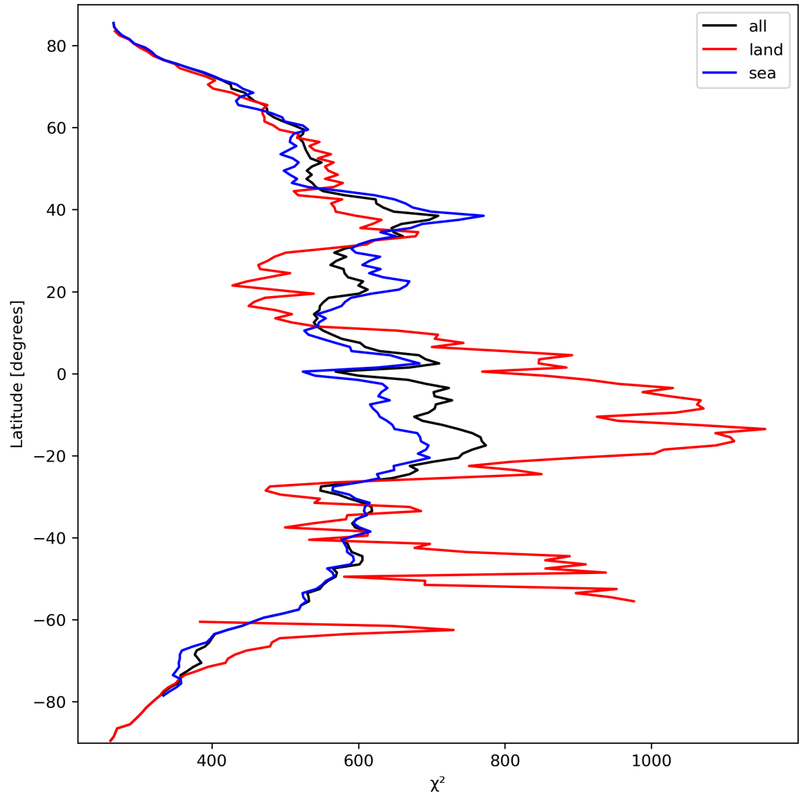
Figure 25: Zonal average of “ \chi^2 ” for 2024-03-12 to 2024-03-14.
