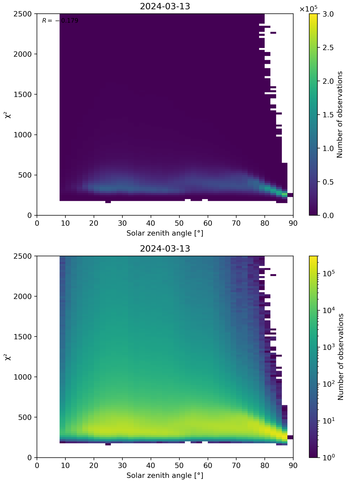
Figure 148: Scatter density plot of “Solar zenith angle” against “ \chi^2 ” for 2024-03-12 to 2024-03-14.
