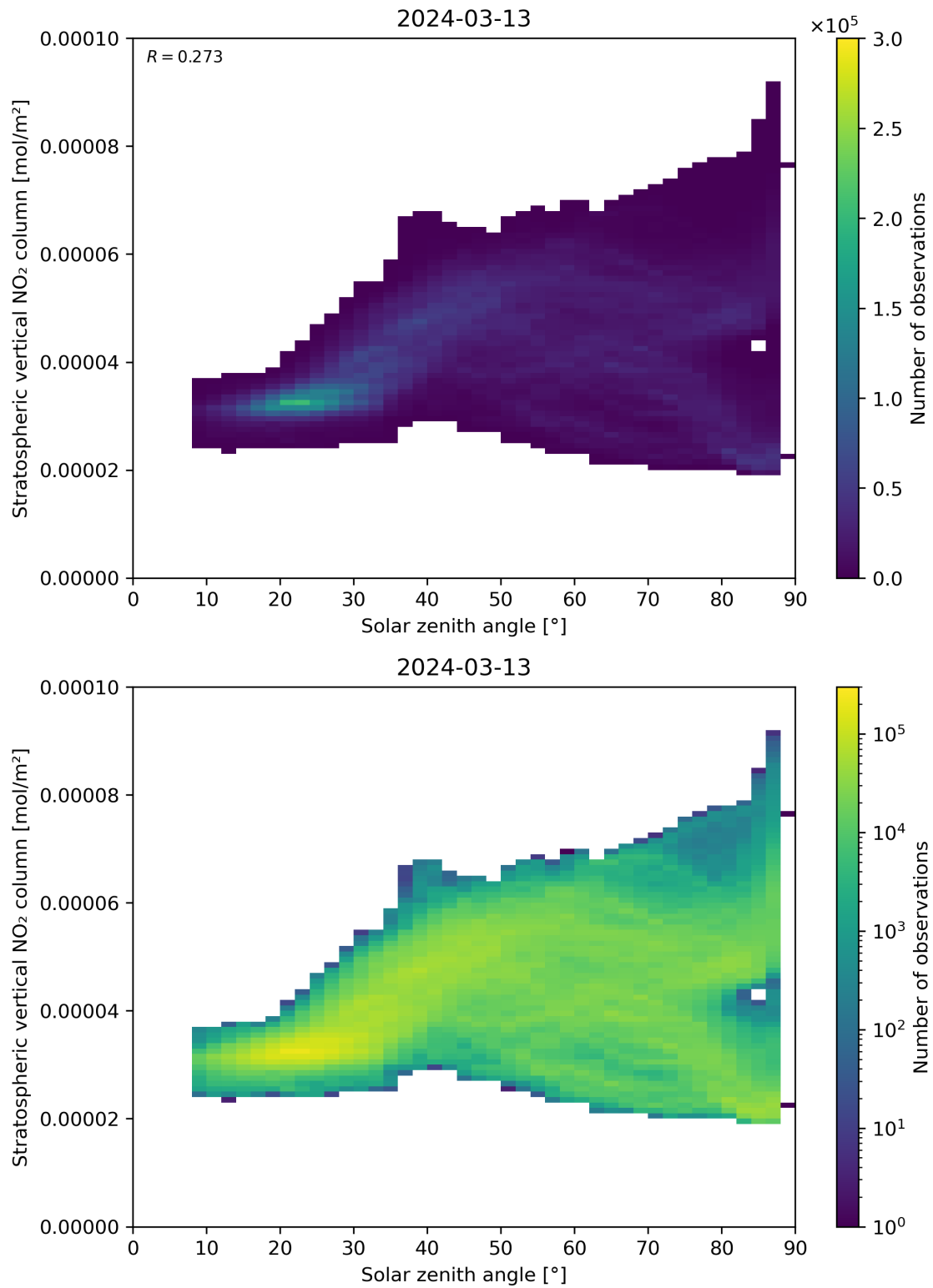
Figure 150: Scatter density plot of “Solar zenith angle” against “Stratospheric vertical NO 2 column” for 2024-03-12 to 2024-03-14.
