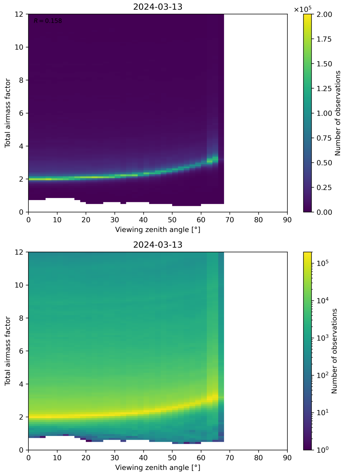
Figure 160: Scatter density plot of “Viewing zenith angle” against “Total airmass factor” for 2024-03-12 to 2024-03-14.
