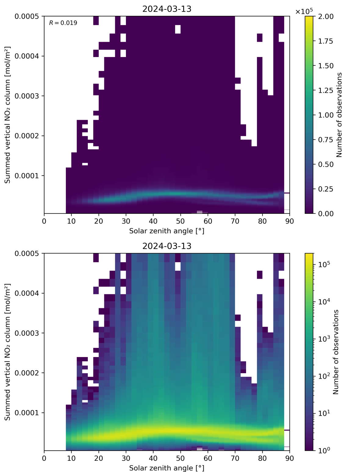
Figure 151: Scatter density plot of “Solar zenith angle” against “Summed vertical NO 2 column” for 2024-03-12 to 2024-03-14.
