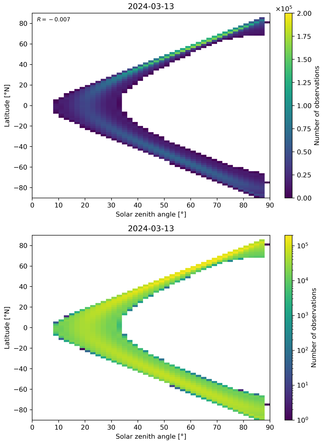
Figure 149: Scatter density plot of “Solar zenith angle” against “Latitude” for 2024-03-12 to 2024-03-14.
