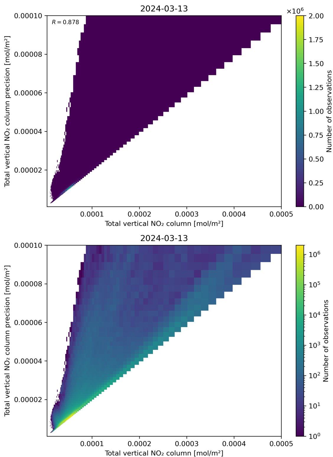
Figure 114: Scatter density plot of “Total vertical NO 2 column” against “Total vertical NO 2 column precision” for 2024-03-12 to 2024-03-14.
