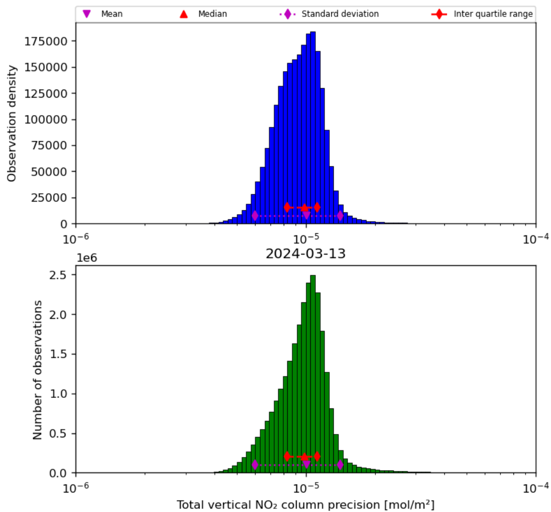
Figure 39: Histogram of “Total vertical NO 2 column precision” for 2024-03-12 to 2024-03-14
