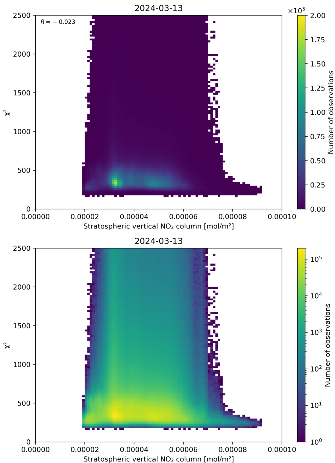
Figure 97: Scatter density plot of “Stratospheric vertical NO 2 column” against “ \chi^2 ” for 2024-03-12 to 2024-03-14.
