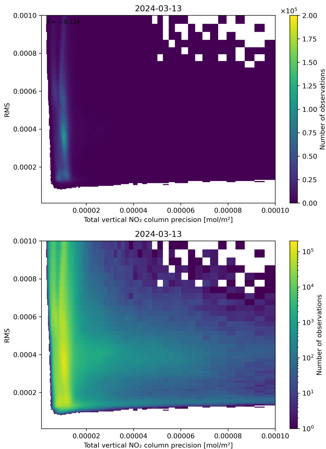
Figure 119: Scatter density plot of “Total vertical NO 2 column precision” against “RMS” for 2024-03-12 to 2024-03-14.
