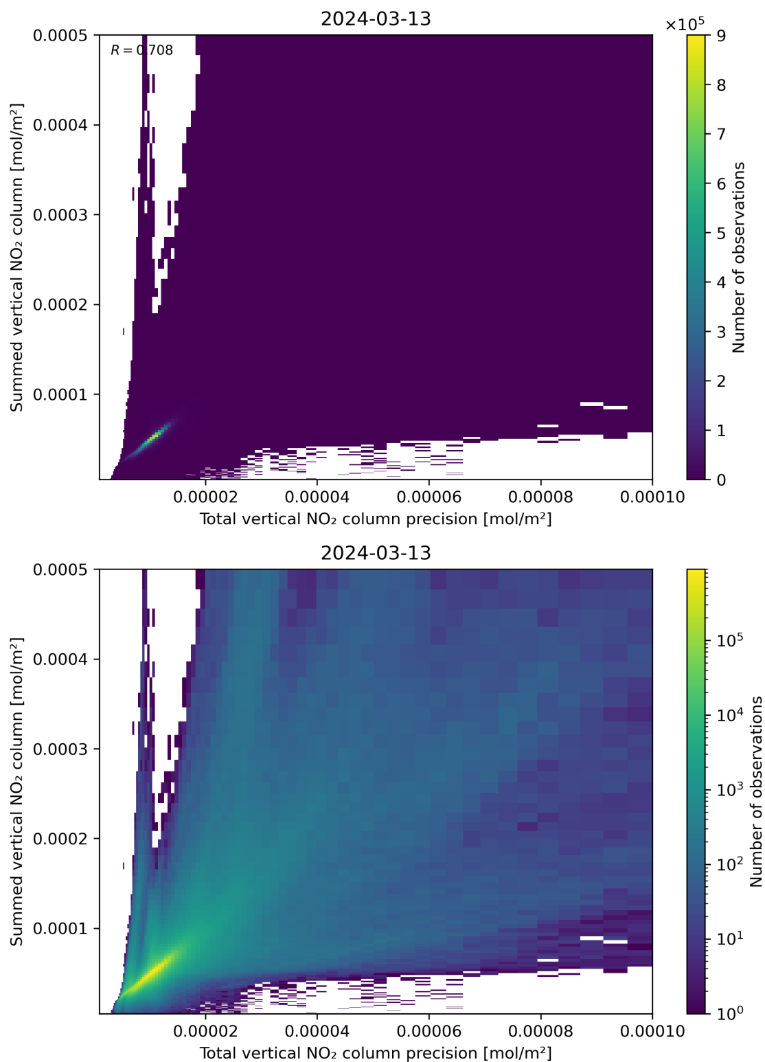
Figure 117: Scatter density plot of “Total vertical NO 2 column precision” against “Summed vertical NO 2 column” for 2024-03-12 to 2024-03-14.
