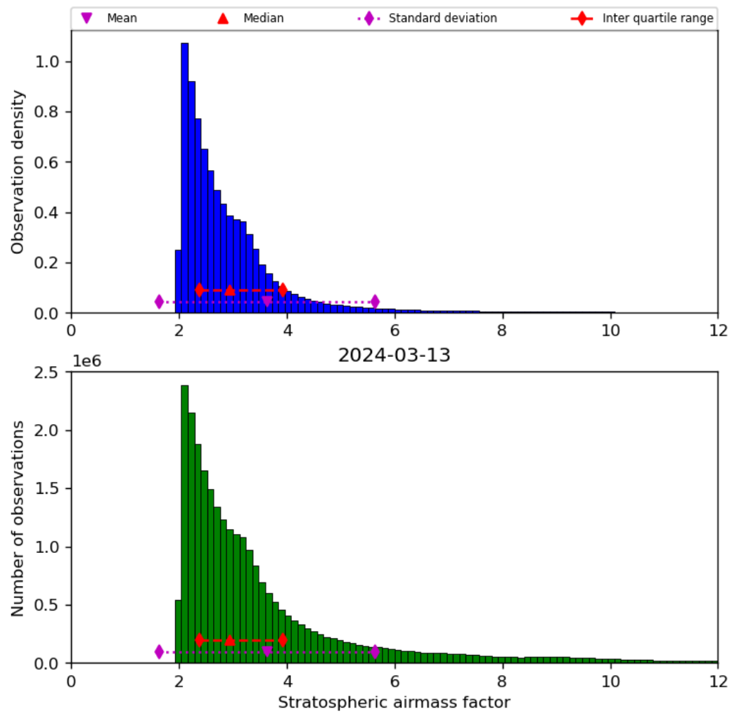
Figure 44: Histogram of “Stratospheric airmass factor” for 2024-03-12 to 2024-03-14
