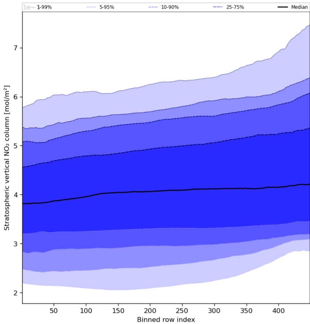
Figure 53: Along track statistics of “Stratospheric vertical NO 2 column” for 2024-03-12 to 2024-03-14
