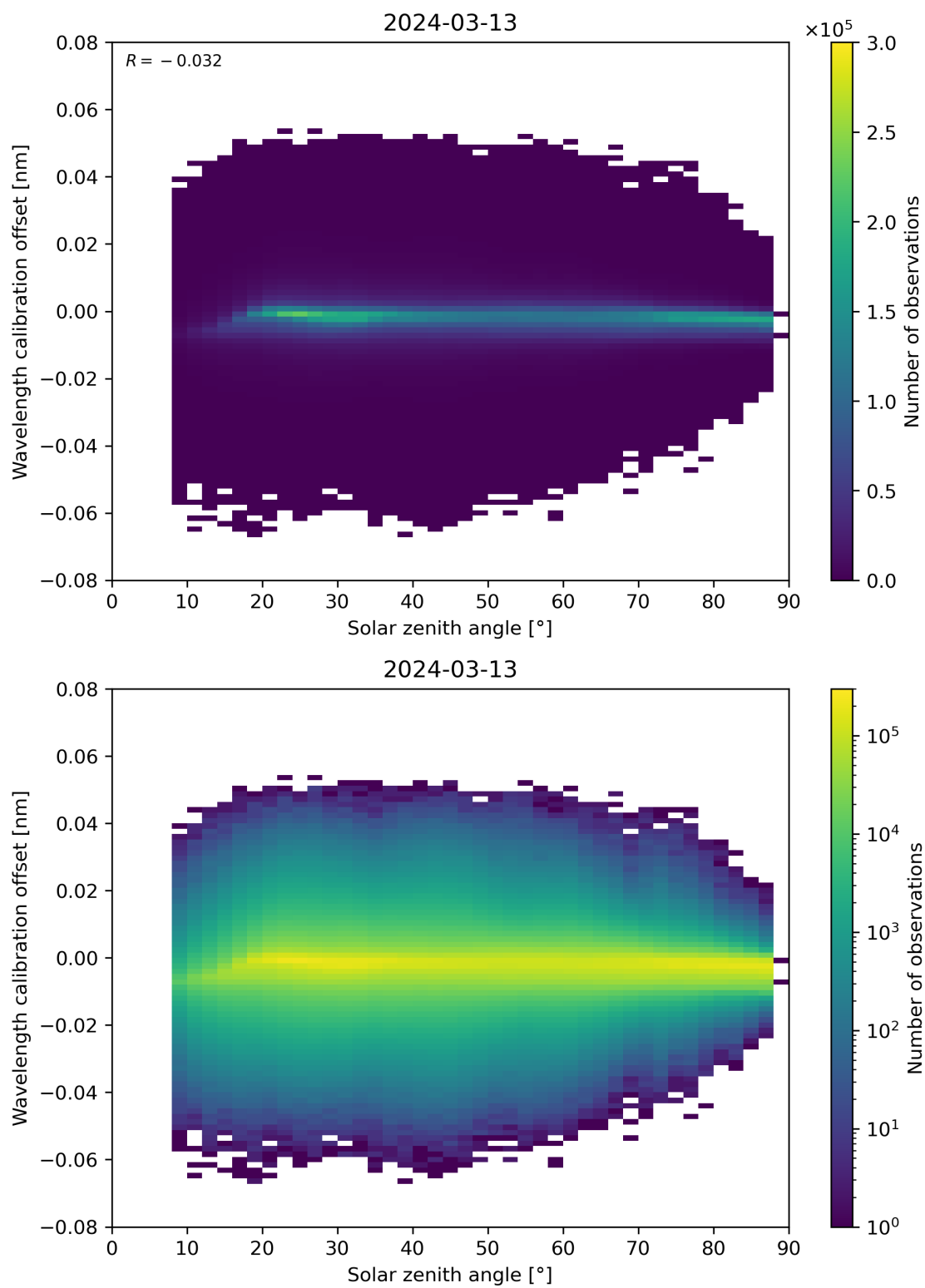
Figure 158: Scatter density plot of “Solar zenith angle” against “Wavelength calibration offset” for 2024-03-12 to 2024-03-14.
