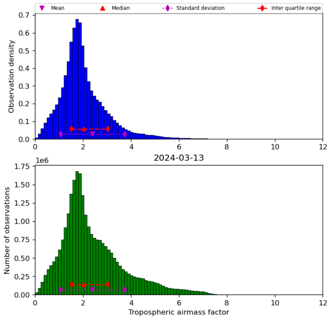
Figure 31: Histogram of “Tropospheric airmass factor” for 2024-03-12 to 2024-03-14
