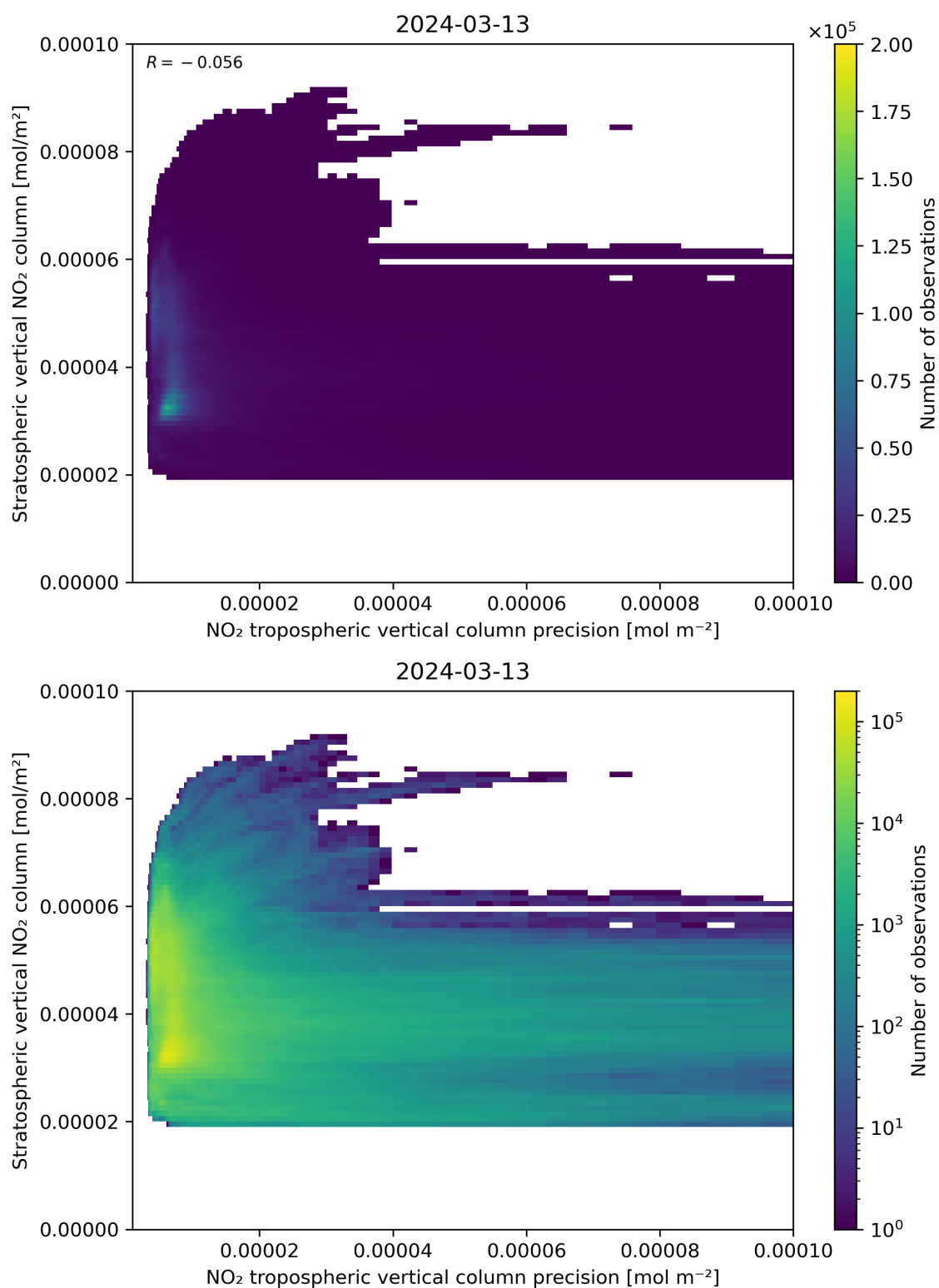
Figure 135: Scatter density plot of “NO 2 tropospheric vertical column precision” against “Stratospheric vertical NO 2 column” for 2024-03-12 to 2024-03-14.
