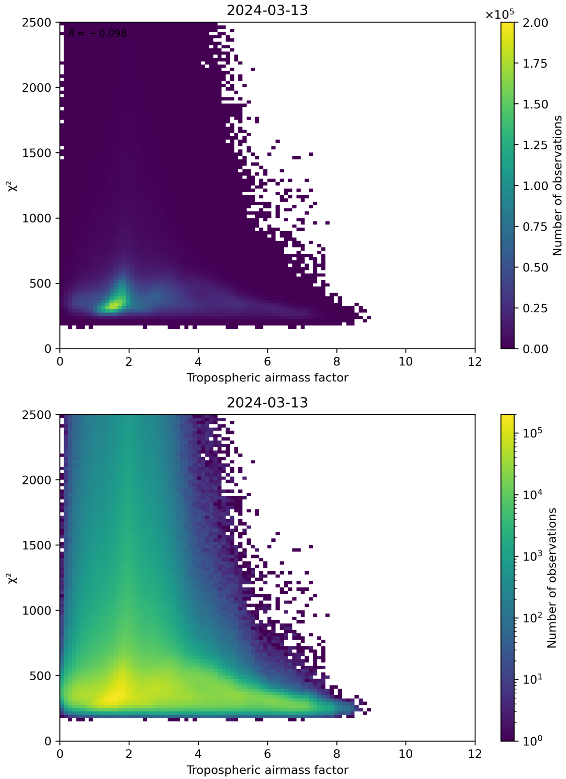
Figure 73: Scatter density plot of “Tropospheric airmass factor” against “ \chi^2 ” for 2024-03-12 to 2024-03-14.
