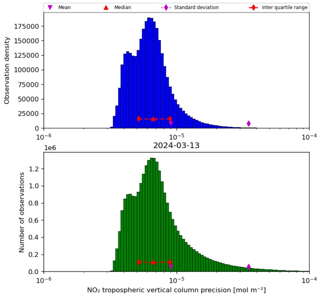
Figure 30: Histogram of “NO 2 tropospheric vertical column precision” for 2024-03-12 to 2024-03-14
