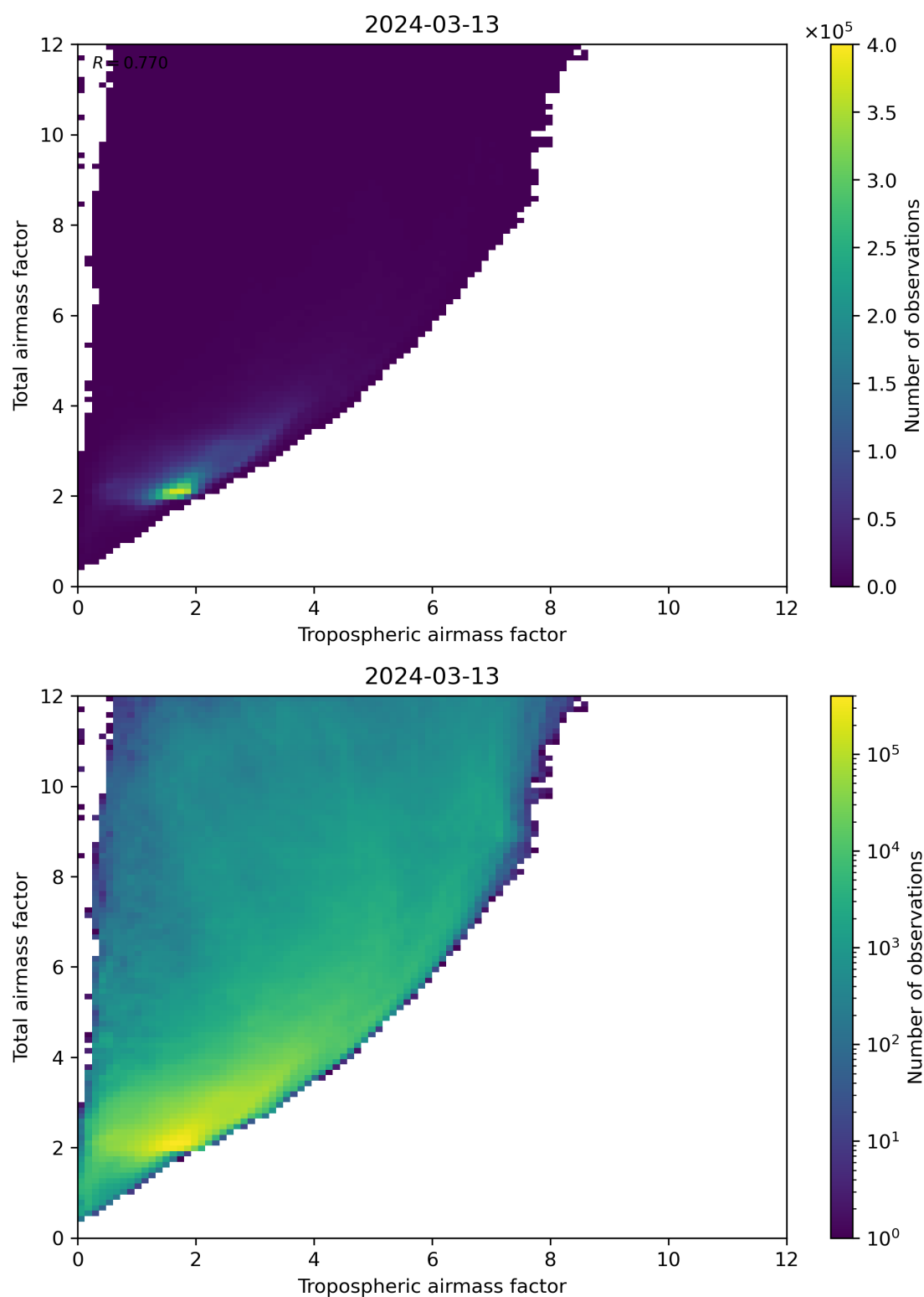
Figure 72: Scatter density plot of “Tropospheric airmass factor” against “Total airmass factor” for 2024-03-12 to 2024-03-14.
