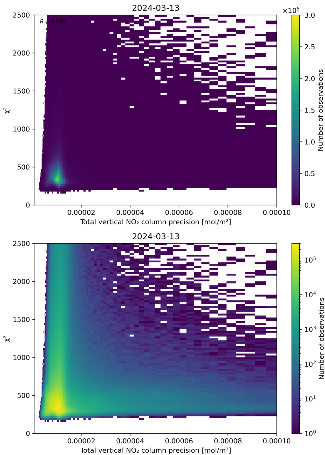
Figure 116: Scatter density plot of “Total vertical NO 2 column precision” against “ \chi^2 ” for 2024-03-12 to 2024-03-14.
