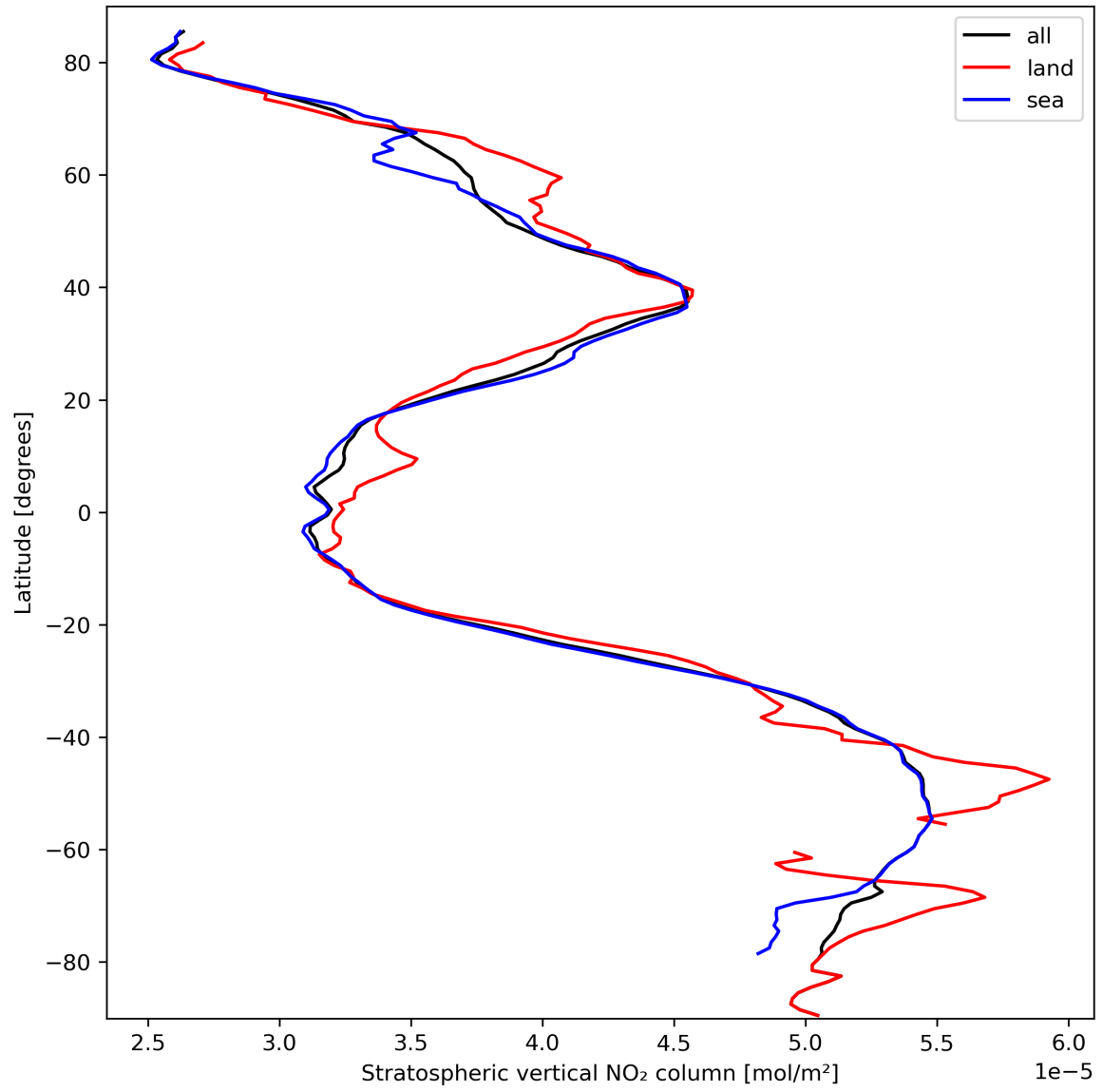
Figure 19: Zonal average of “Stratospheric vertical NO 2 column” for 2024-03-12 to 2024-03-14.
