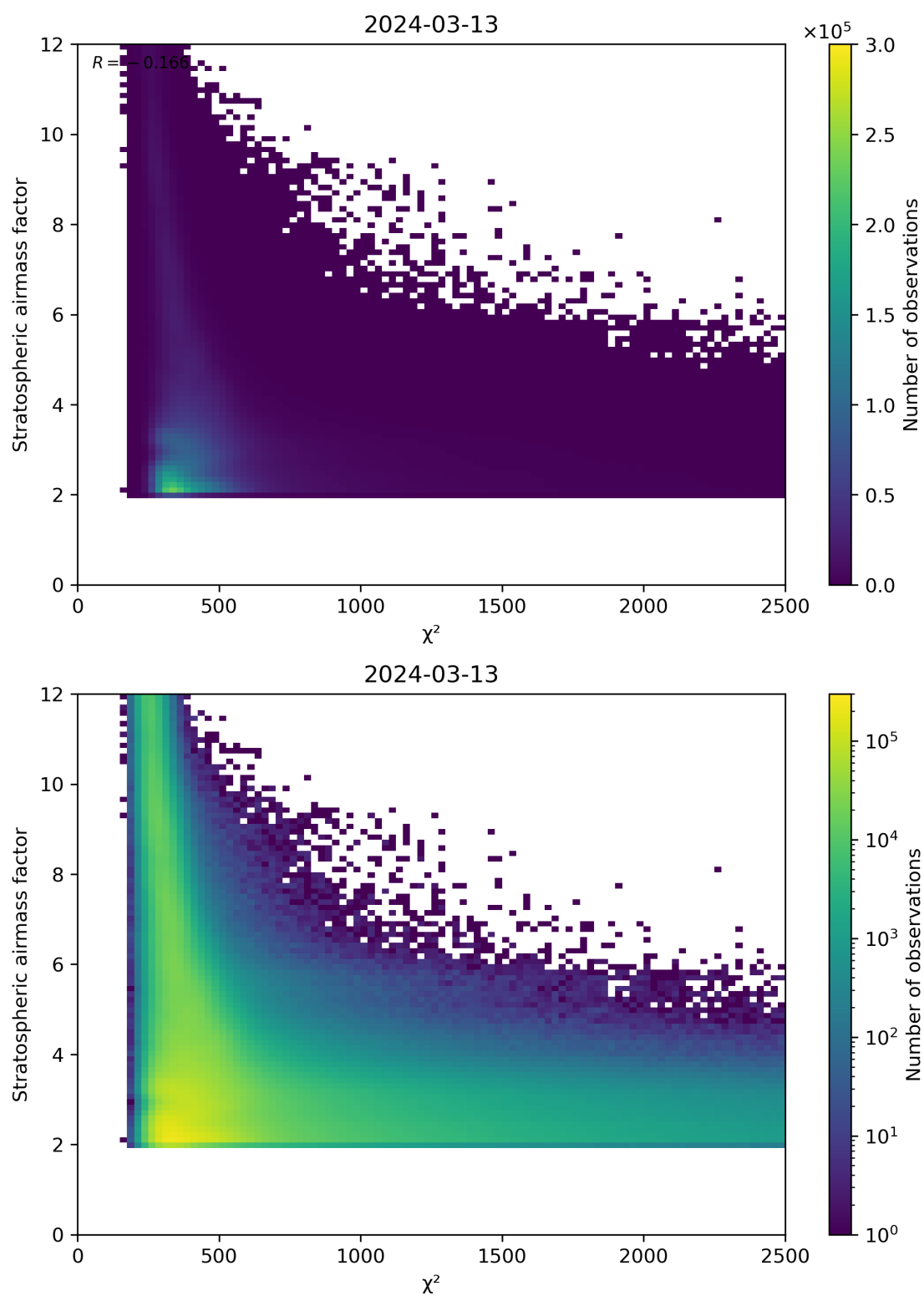
Figure 81: Scatter density plot of “ \chi^2 ” against “Stratospheric airmass factor” for 2024-03-12 to 2024-03-14.
