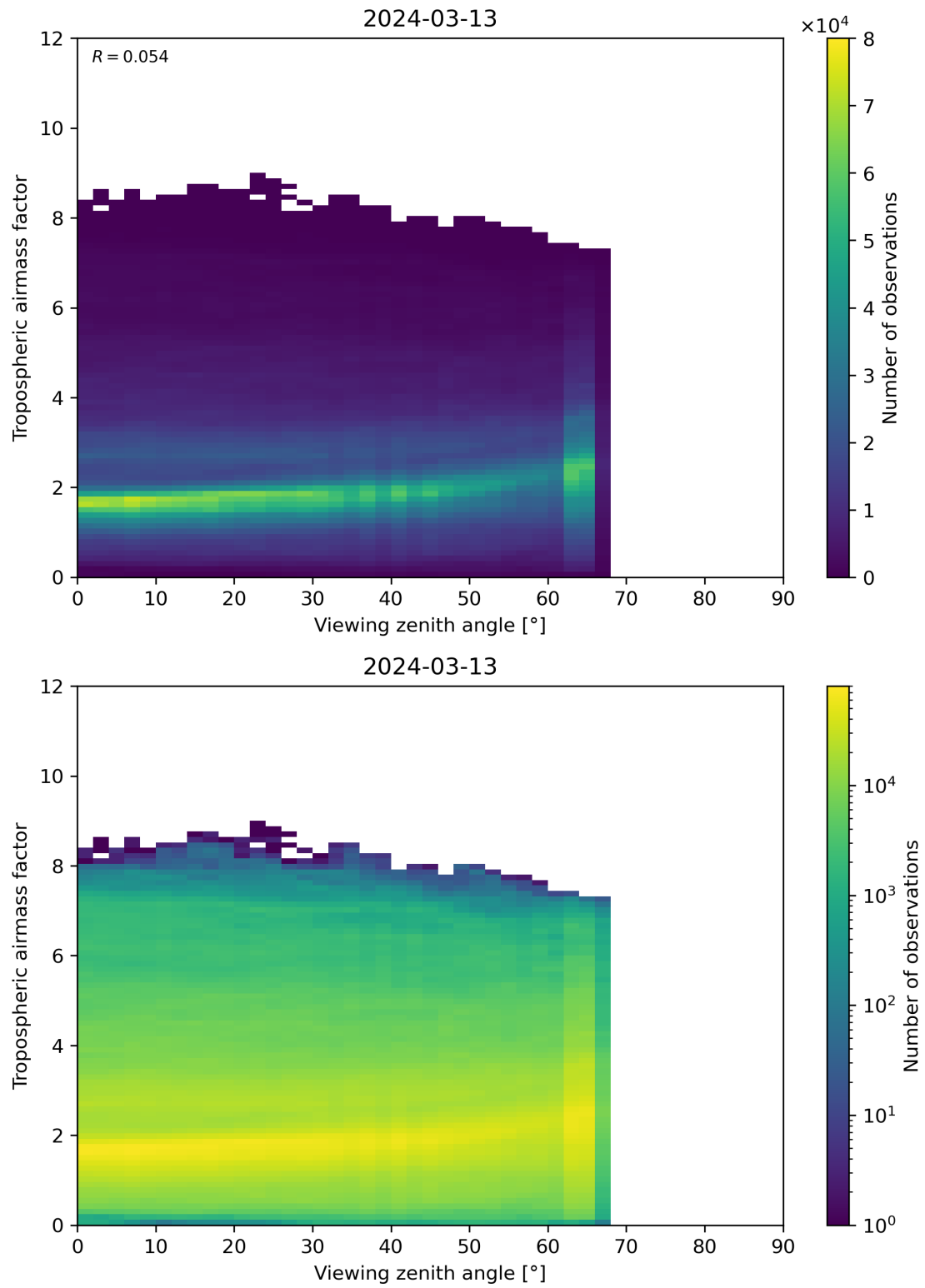
Figure 161: Scatter density plot of “Viewing zenith angle” against “Tropospheric airmass factor” for 2024-03-12 to 2024-03-14.
