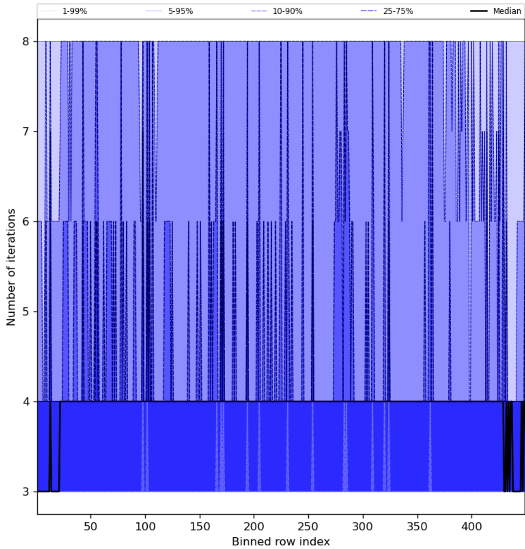
Figure 51: Along track statistics of “Number of iterations” for 2024-03-12 to 2024-03-14
