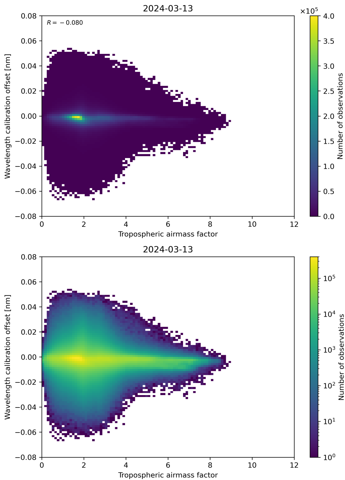
Figure 80: Scatter density plot of “Tropospheric airmass factor” against “Wavelength calibration offset” for 2024-03-12 to 2024-03-14.
