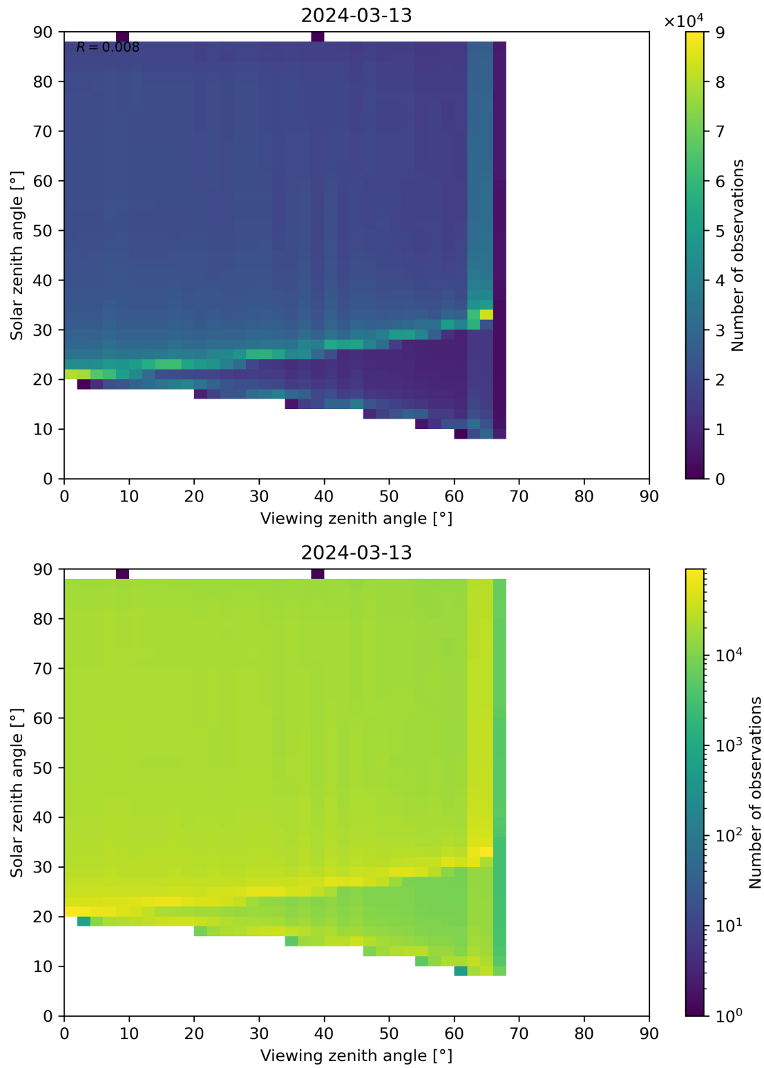
Figure 172: Scatter density plot of “Viewing zenith angle” against “Solar zenith angle” for 2024-03-12 to 2024-03-14.
