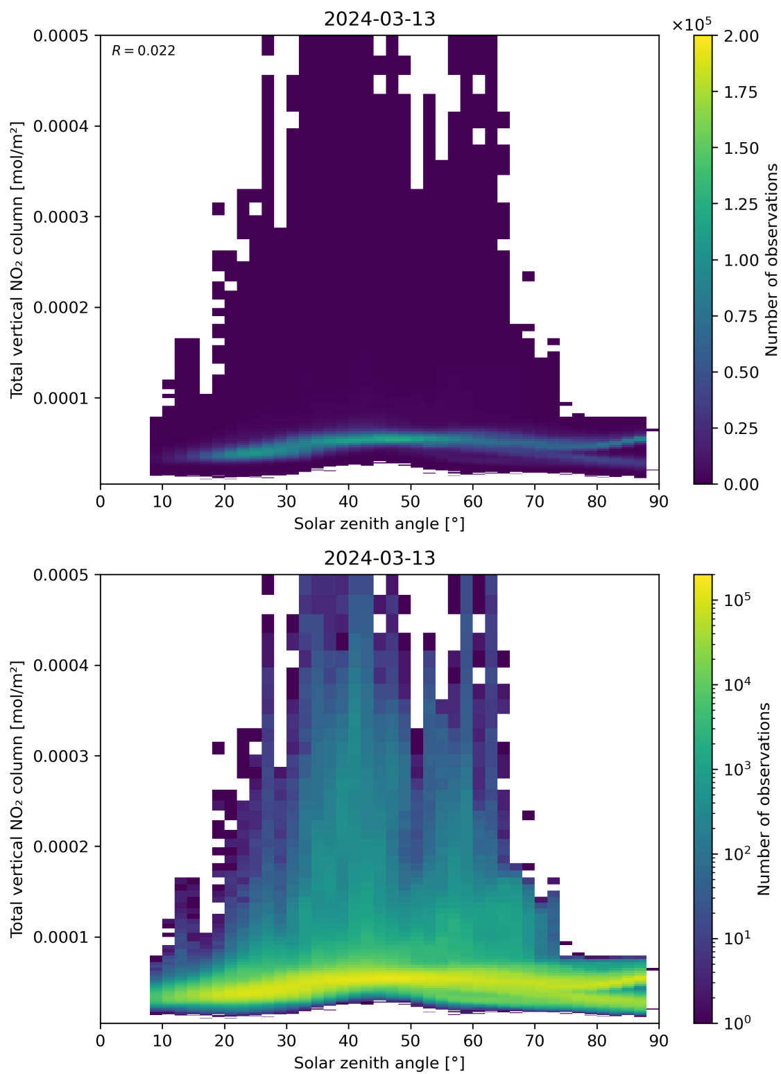
Figure 153: Scatter density plot of “Solar zenith angle” against “Total vertical NO 2 column” for 2024-03-12 to 2024-03-14.
