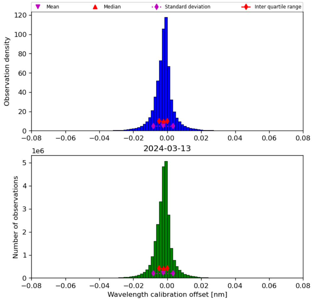
Figure 35: Histogram of “Wavelength calibration offset” for 2024-03-12 to 2024-03-14
