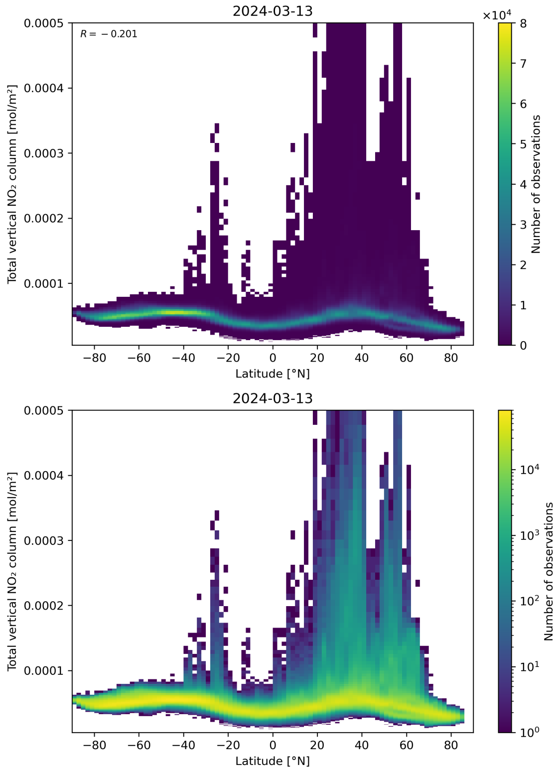
Figure 90: Scatter density plot of “Latitude” against “Total vertical NO 2 column” for 2024-03-12 to 2024-03-14.
