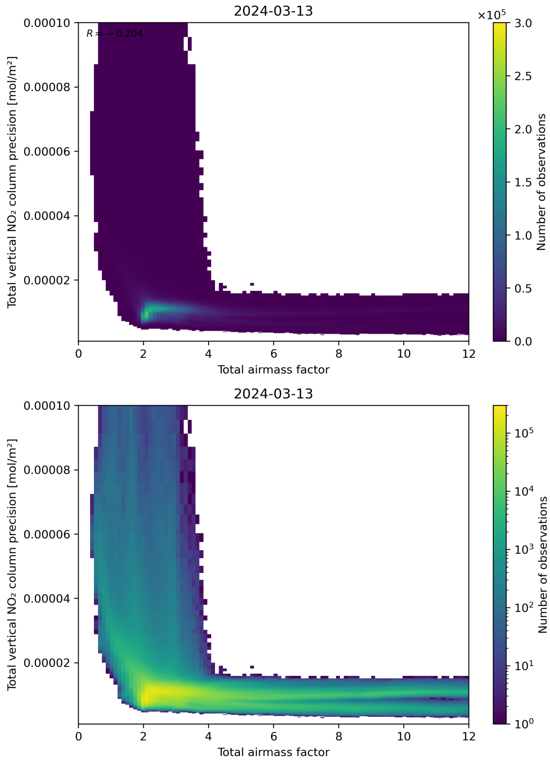
Figure 68: Scatter density plot of “Total airmass factor” against “Total vertical NO 2 column precision” for 2024-03-12 to 2024-03-14.
