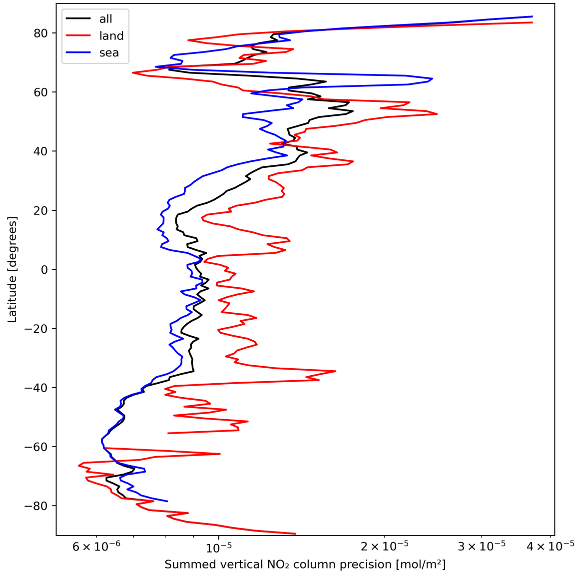
Figure 24: Zonal average of “Summed vertical NO 2 column precision” for 2024-03-12 to 2024-03-14.
