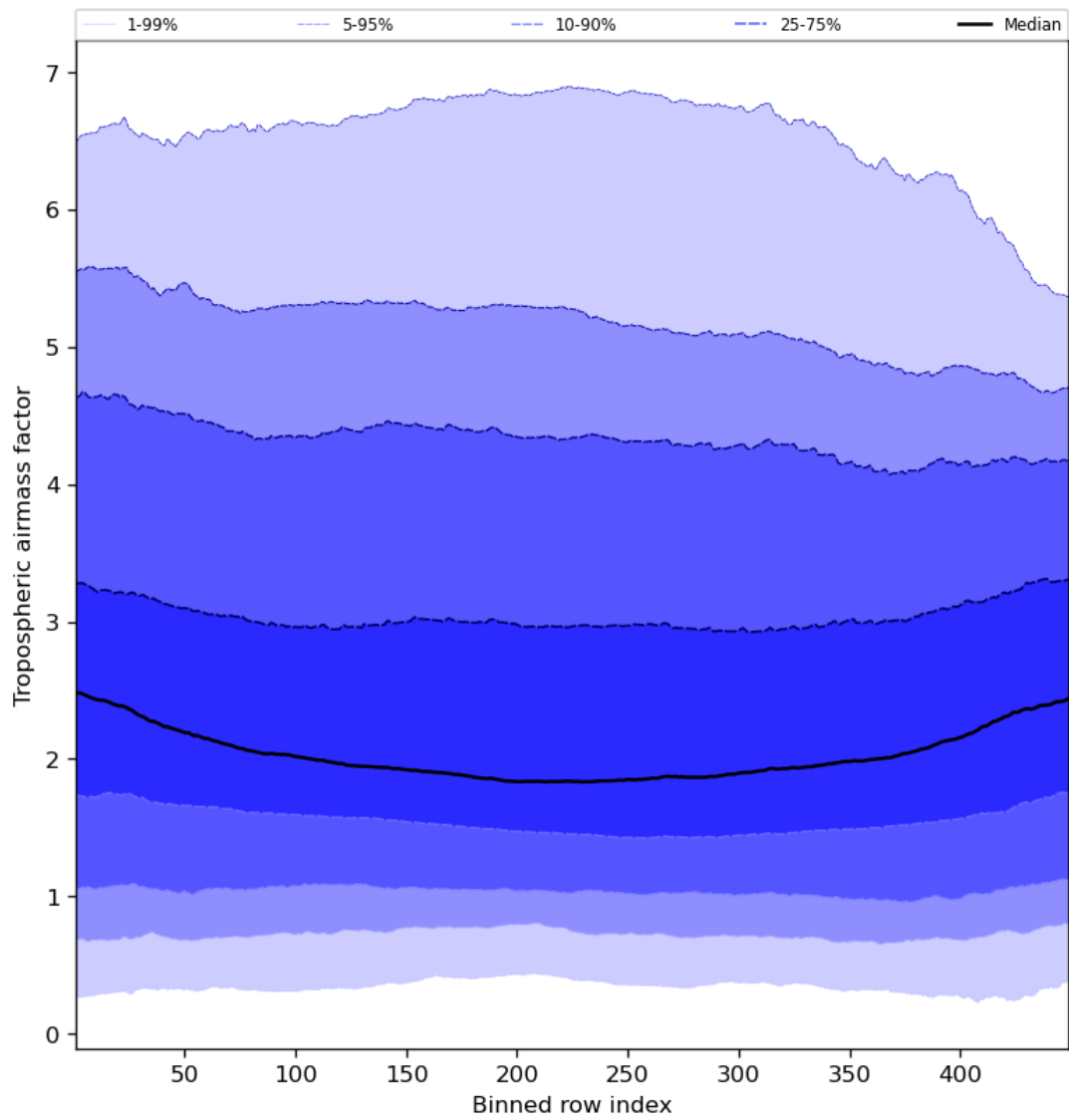
Figure 48: Along track statistics of “Tropospheric air mass factor” for 2024-03-12 to 2024-03-14
