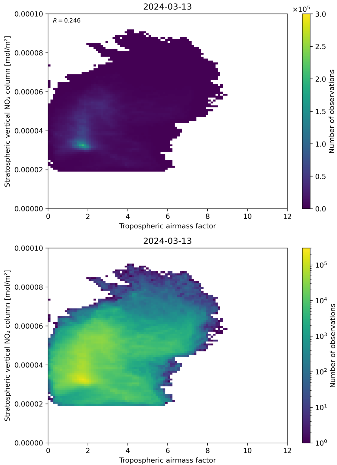
Figure 74: Scatter density plot of “Tropospheric air mass factor” against “Stratospheric vertical NO 2 column” for 2024-03-12 to 2024-03-14.
