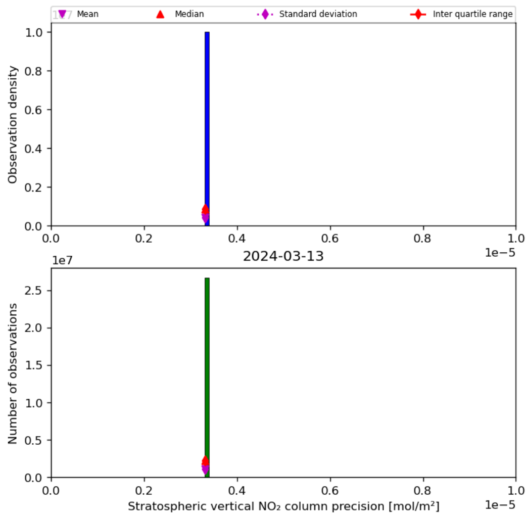
Figure 37: Histogram of “Stratospheric vertical NO 2 column precision” for 2024-03-12 to 2024-03-14
