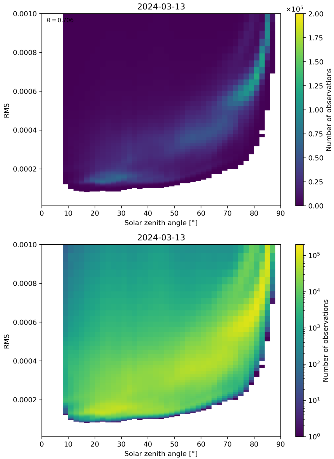
Figure 157: Scatter density plot of “Solar zenith angle” against “RMS” for 2024-03-12 to 2024-03-14.
