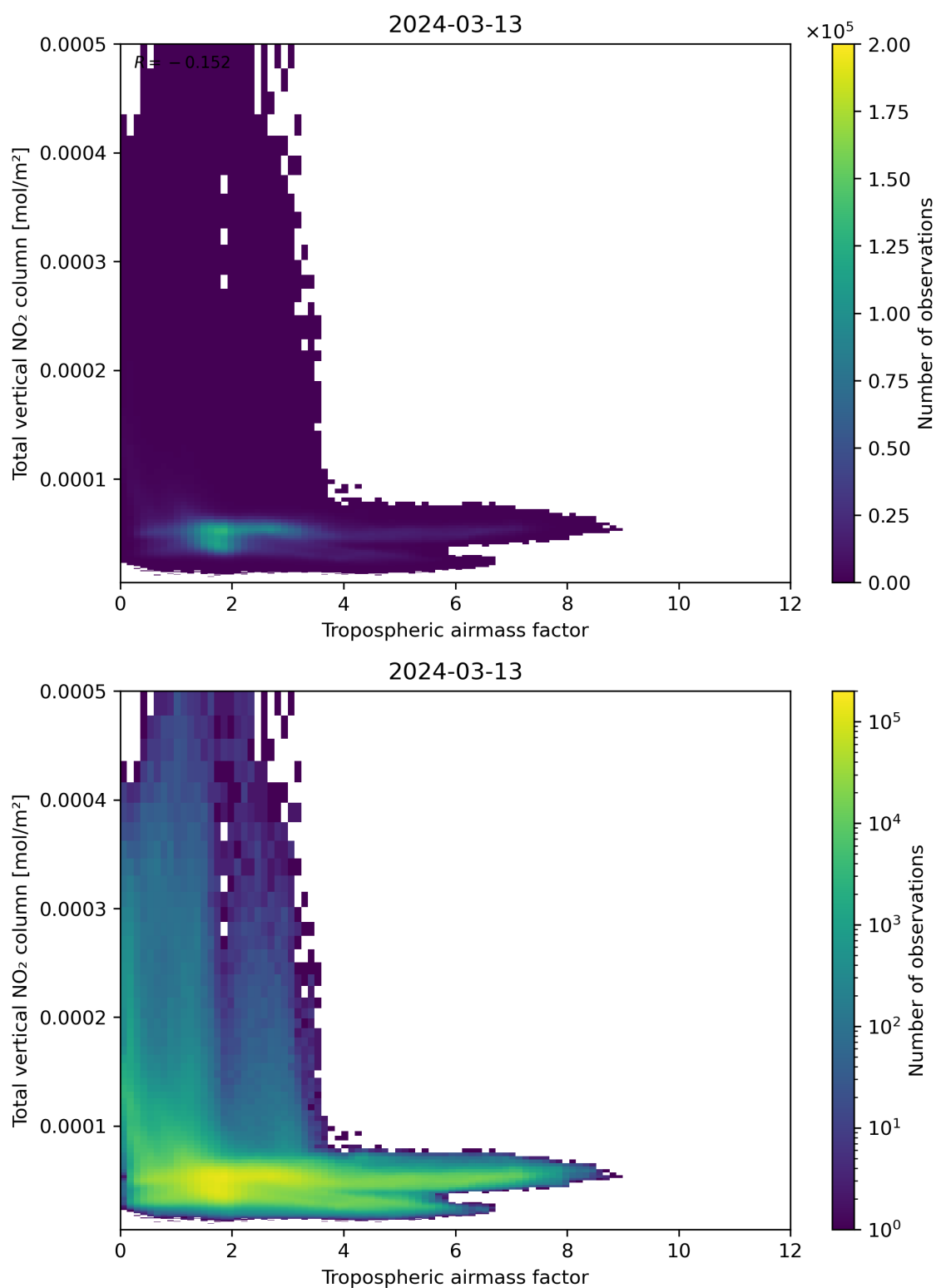
Figure 77: Scatter density plot of “Tropospheric airmass factor” against “Total vertical NO 2 column” for 2024-03-12 to 2024-03-14.
