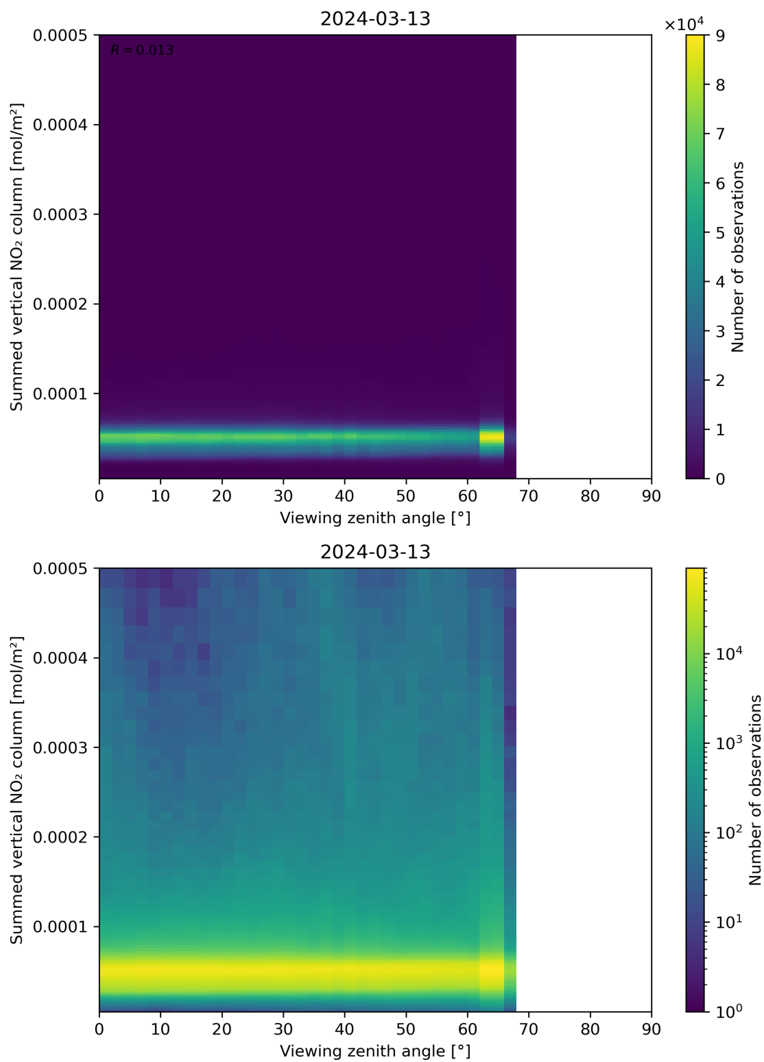
Figure 165: Scatter density plot of “Viewing zenith angle” against “Summed vertical NO 2 column” for 2024-03-12 to 2024-03-14.
