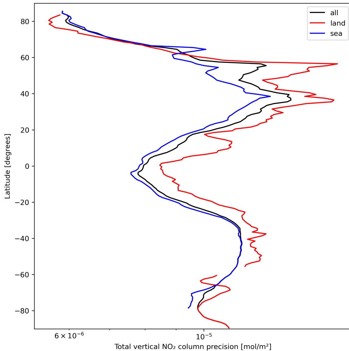
Figure 22: Zonal average of “Total vertical NO 2 column precision” for 2024-03-12 to 2024-03-14.
