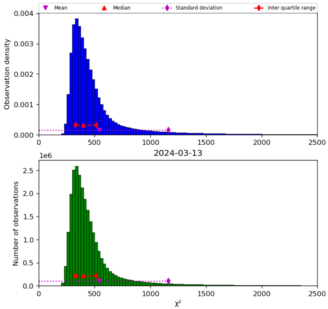
Figure 42: Histogram of “ \chi^2 ” for 2024-03-12 to 2024-03-14
