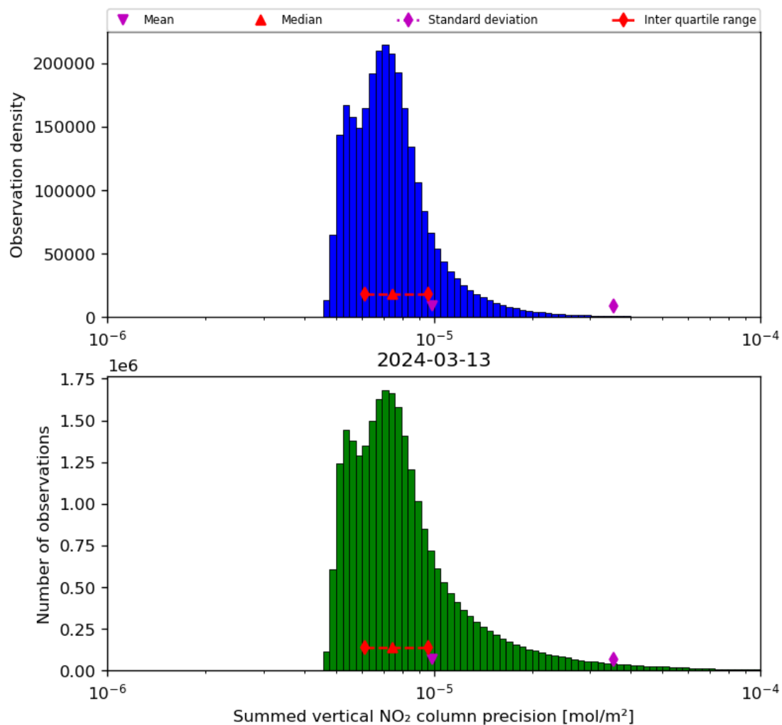
Figure 41: Histogram of "Summed vertical NO 2 column precision" for 2024-03-12 to 2024-03-14
