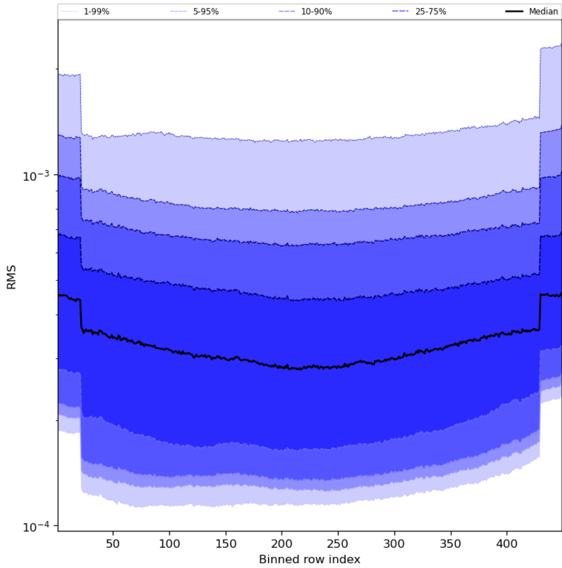
Figure 60: Along track statistics of “RMS” for 2024-03-12 to 2024-03-14
