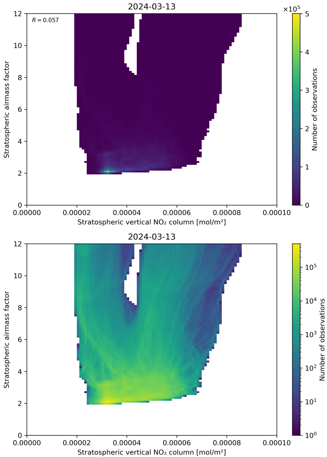
Figure 96: Scatter density plot of “Stratospheric vertical NO 2 column” against “Stratospheric airmass factor” for 2024-03-12 to 2024-03-14.
