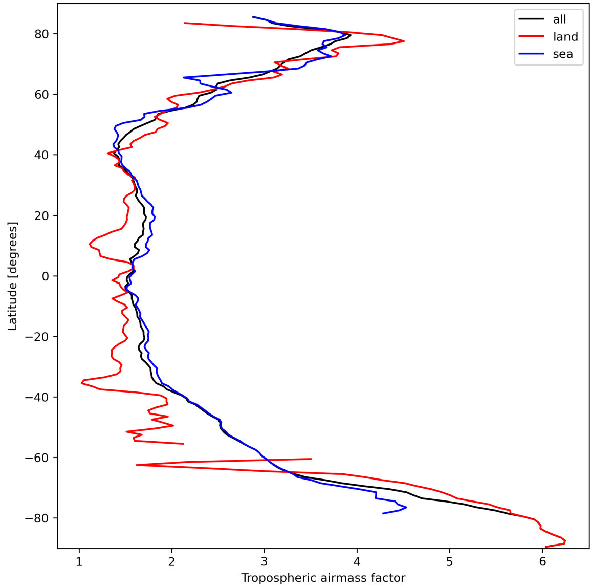
Figure 14: Zonal average of “Tropospheric airmass factor” for 2024-03-12 to 2024-03-14.
