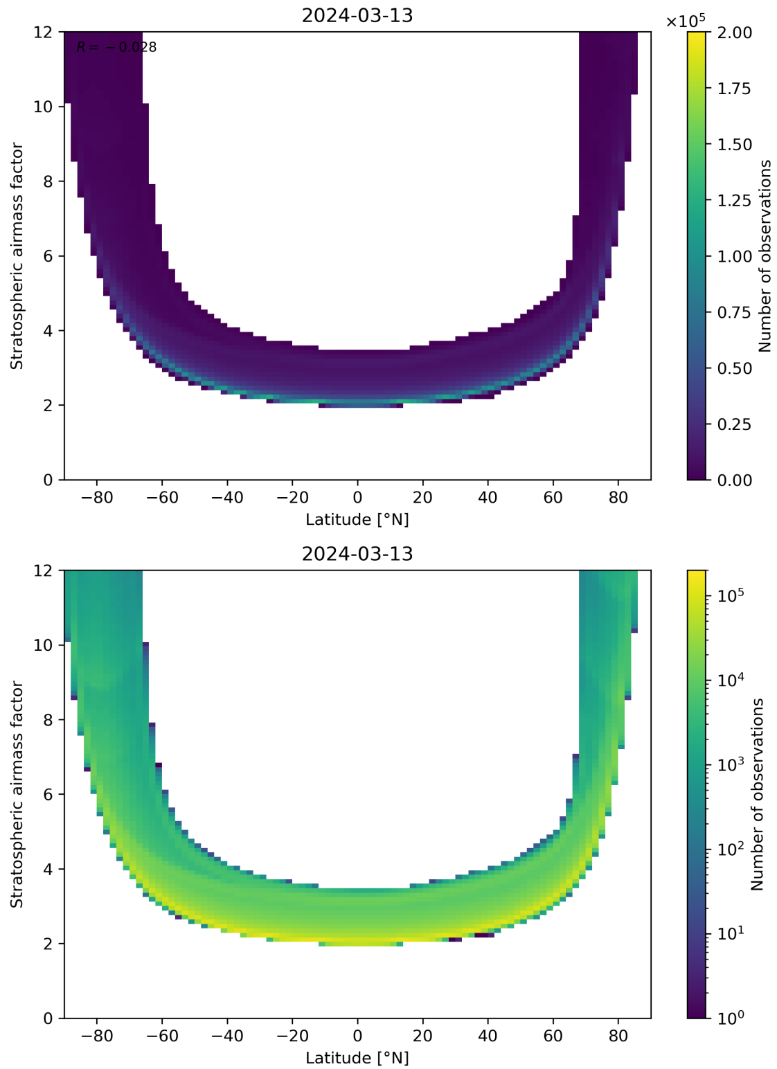
Figure 83: Scatter density plot of “Latitude” against “Stratospheric airmass factor” for 2024-03-12 to 2024-03-14.
