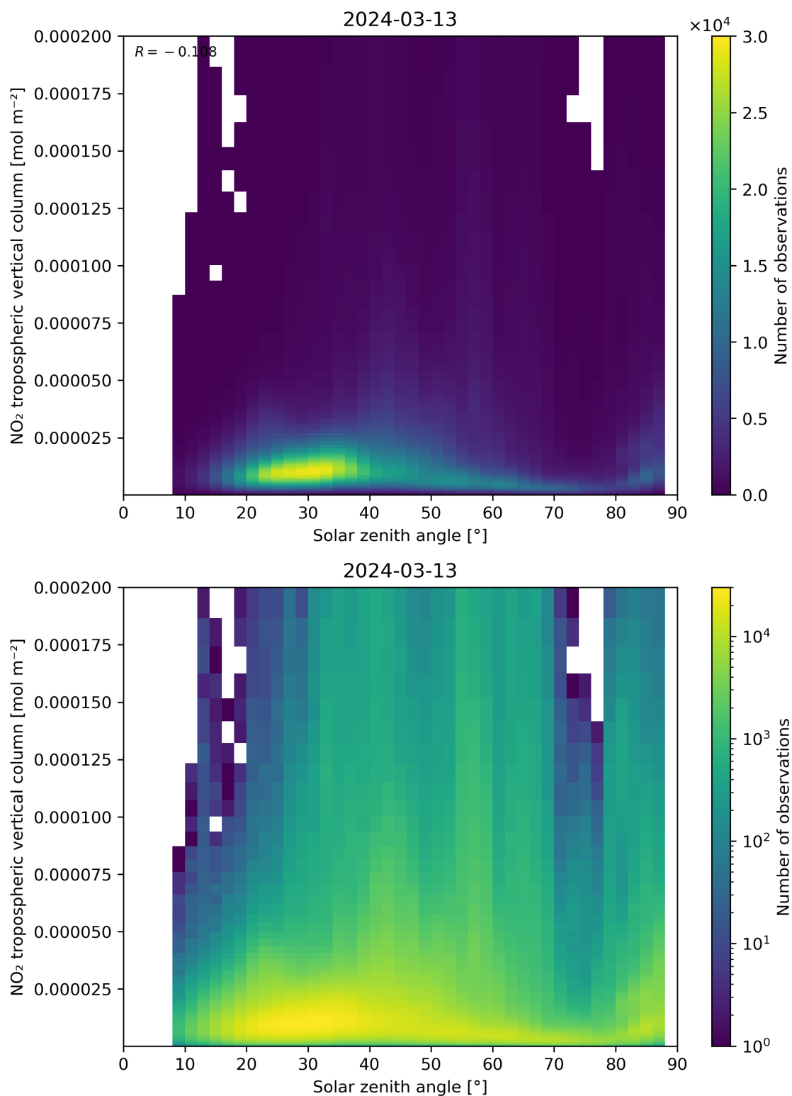
Figure 155: Scatter density plot of “Solar zenith angle” against “NO 2 tropospheric vertical column” for 2024-03-12 to 2024-03-14.
