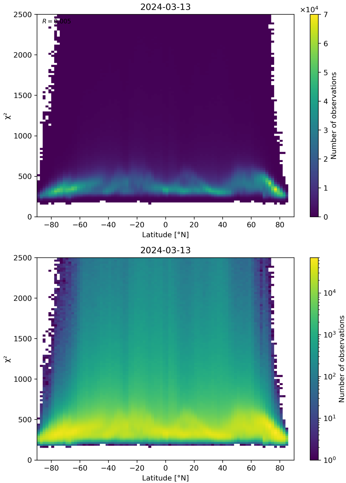
Figure 86: Scatter density plot of “Latitude” against “ \chi^2 ” for 2024-03-12 to 2024-03-14.
