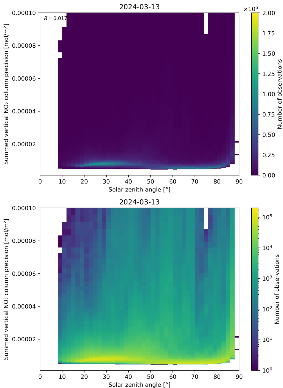
Figure 152: Scatter density plot of “Solar zenith angle” against “Summed vertical NO 2 column precision” for 2024-03-12 to 2024-03-14.
