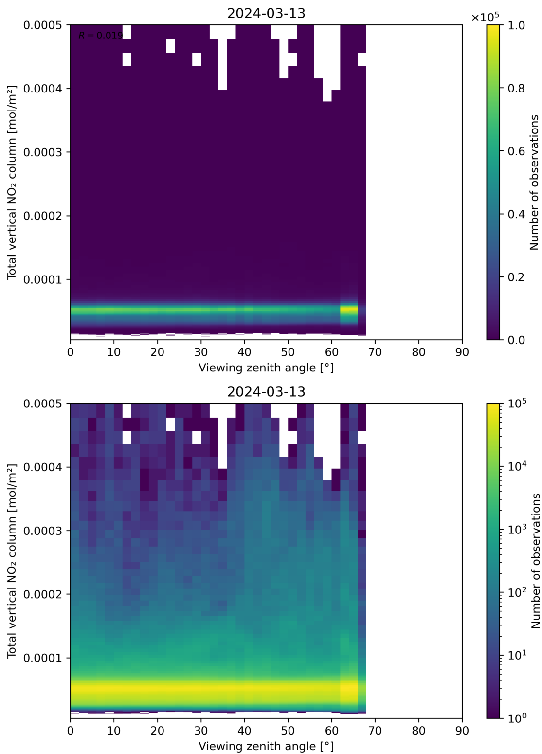
Figure 167: Scatter density plot of “Viewing zenith angle” against “Total vertical NO 2 column” for 2024-03-12 to 2024-03-14.
