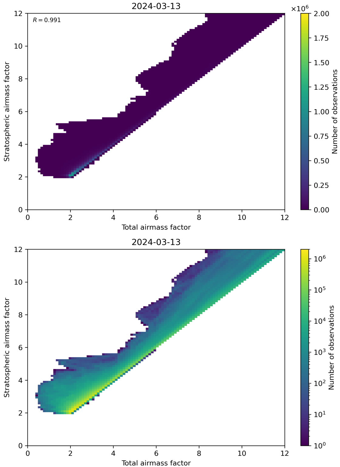
Figure 62: Scatter density plot of “Total airmass factor” against “Stratospheric airmass factor” for 2024-03-12 to 2024-03-14.
