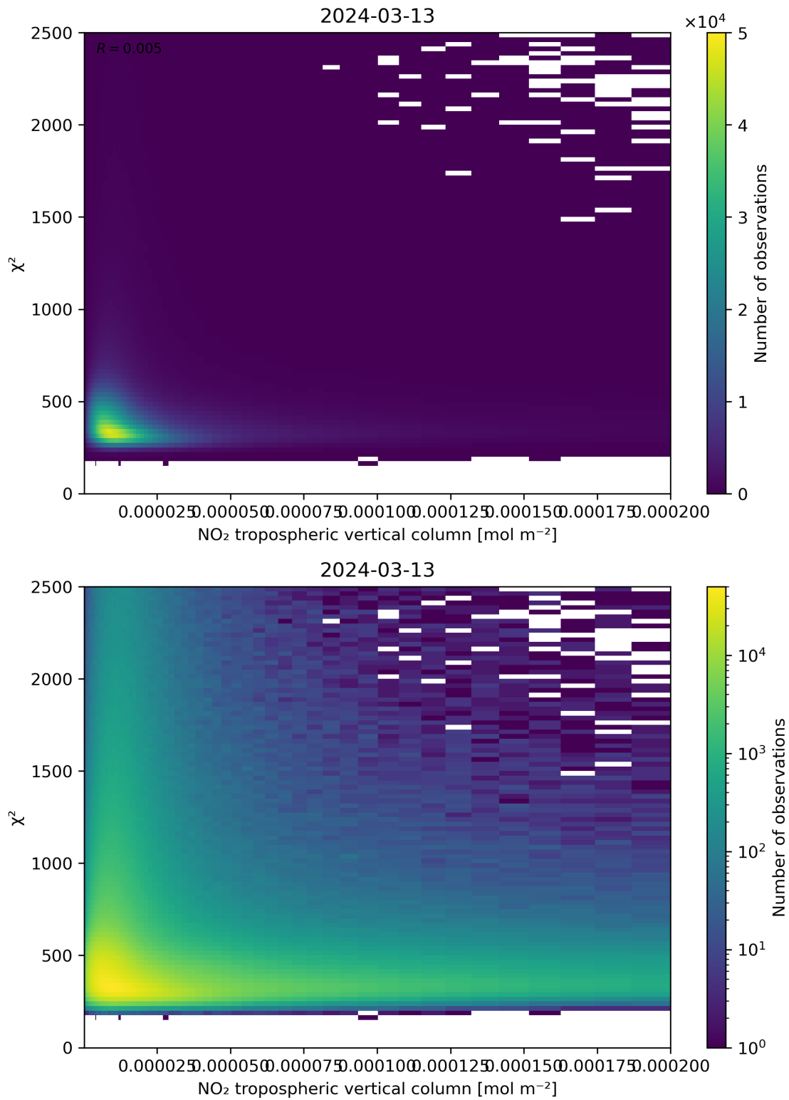
Figure 124: Scatter density plot of “NO 2 tropospheric vertical column” against “ \chi^2 ” for 2024-03-12 to 2024-03-14.
