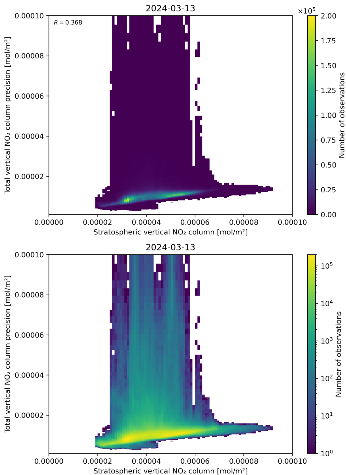
Figure 101: Scatter density plot of “Stratospheric vertical NO 2 column” against “Total vertical NO 2 column precision” for 2024-03-12 to 2024-03-14.
