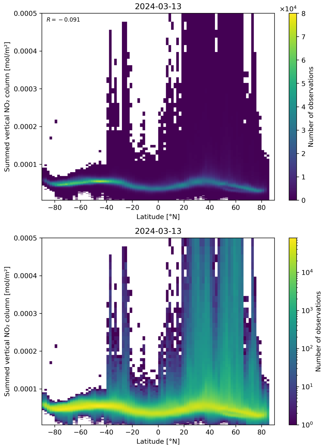
Figure 88: Scatter density plot of “Latitude” against “Summed vertical NO 2 column” for 2024-03-12 to 2024-03-14.
