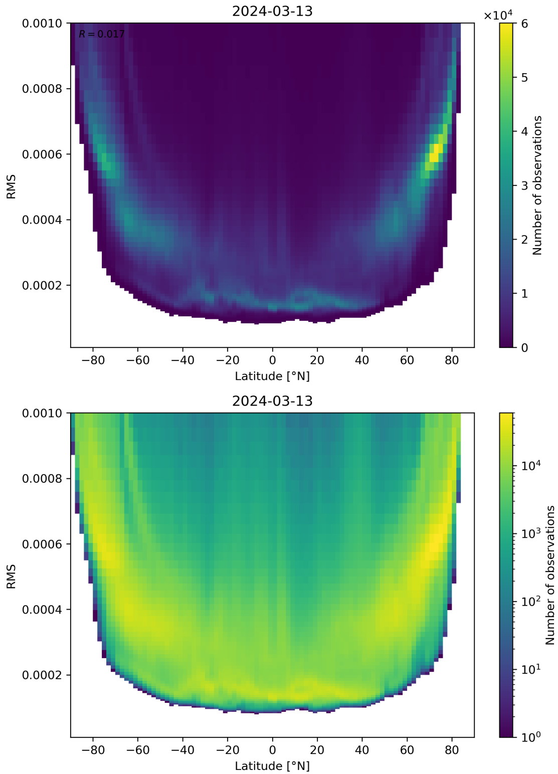
Figure 94: Scatter density plot of “Latitude” against “RMS” for 2024-03-12 to 2024-03-14.
