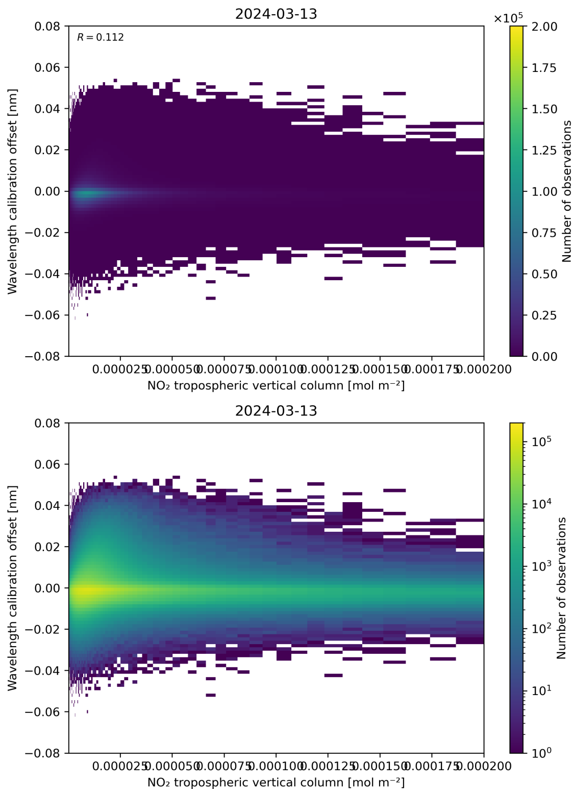
Figure 143: Scatter density plot of “NO 2 tropospheric vertical column” against “Wavelength calibration offset” for 2024-03-12 to 2024-03-14.
