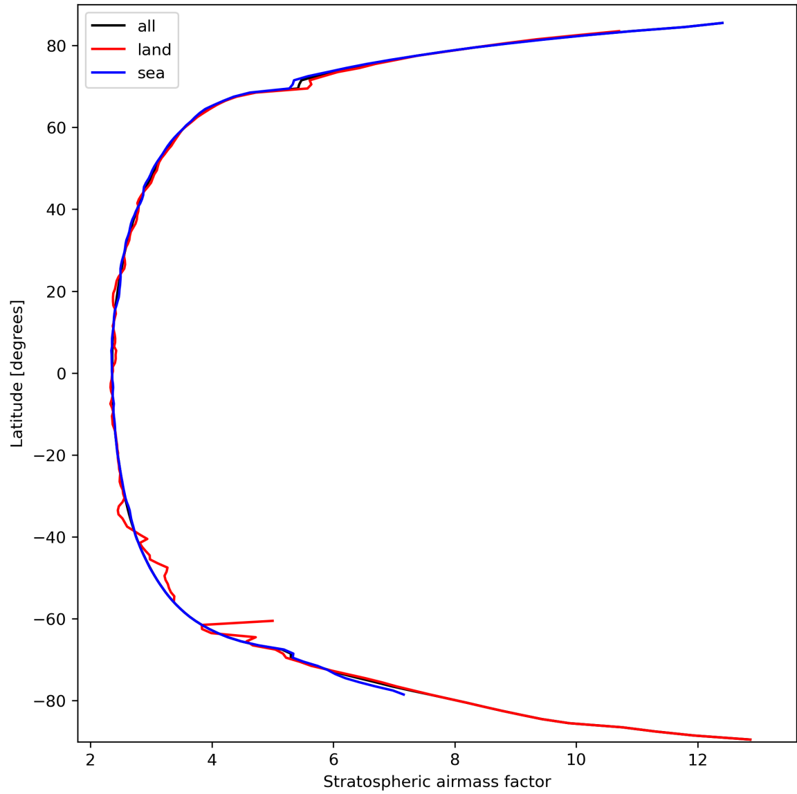
Figure 27: Zonal average of “Stratospheric air mass factor” for 2024-03-12 to 2024-03-14.
