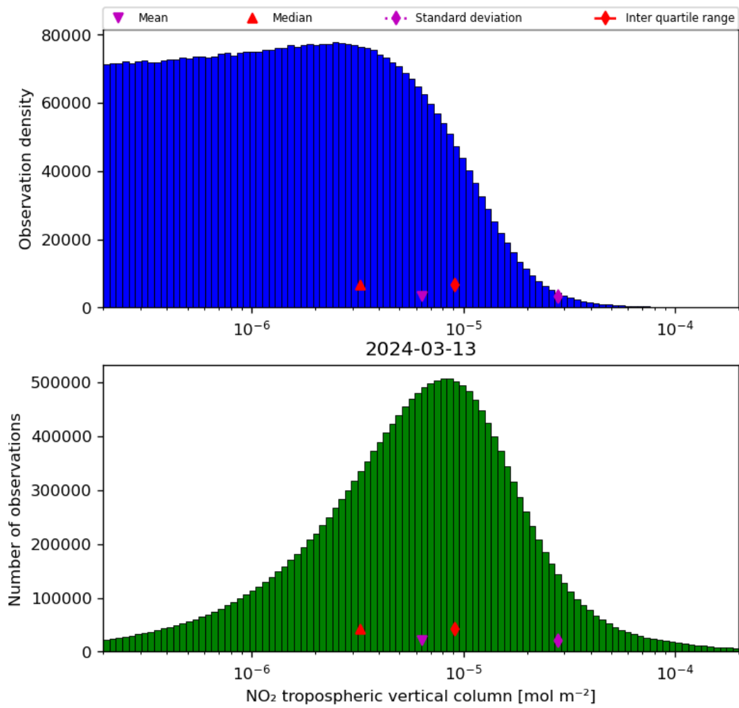
Figure 29: Histogram of “NO 2 tropospheric vertical column” for 2024-03-12 to 2024-03-14
