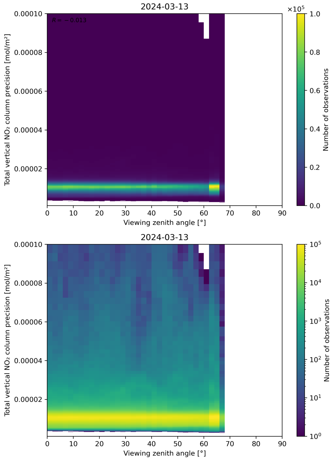
Figure 168: Scatter density plot of “Viewing zenith angle” against “Total vertical NO 2 column precision” for 2024-03-12 to 2024-03-14.
