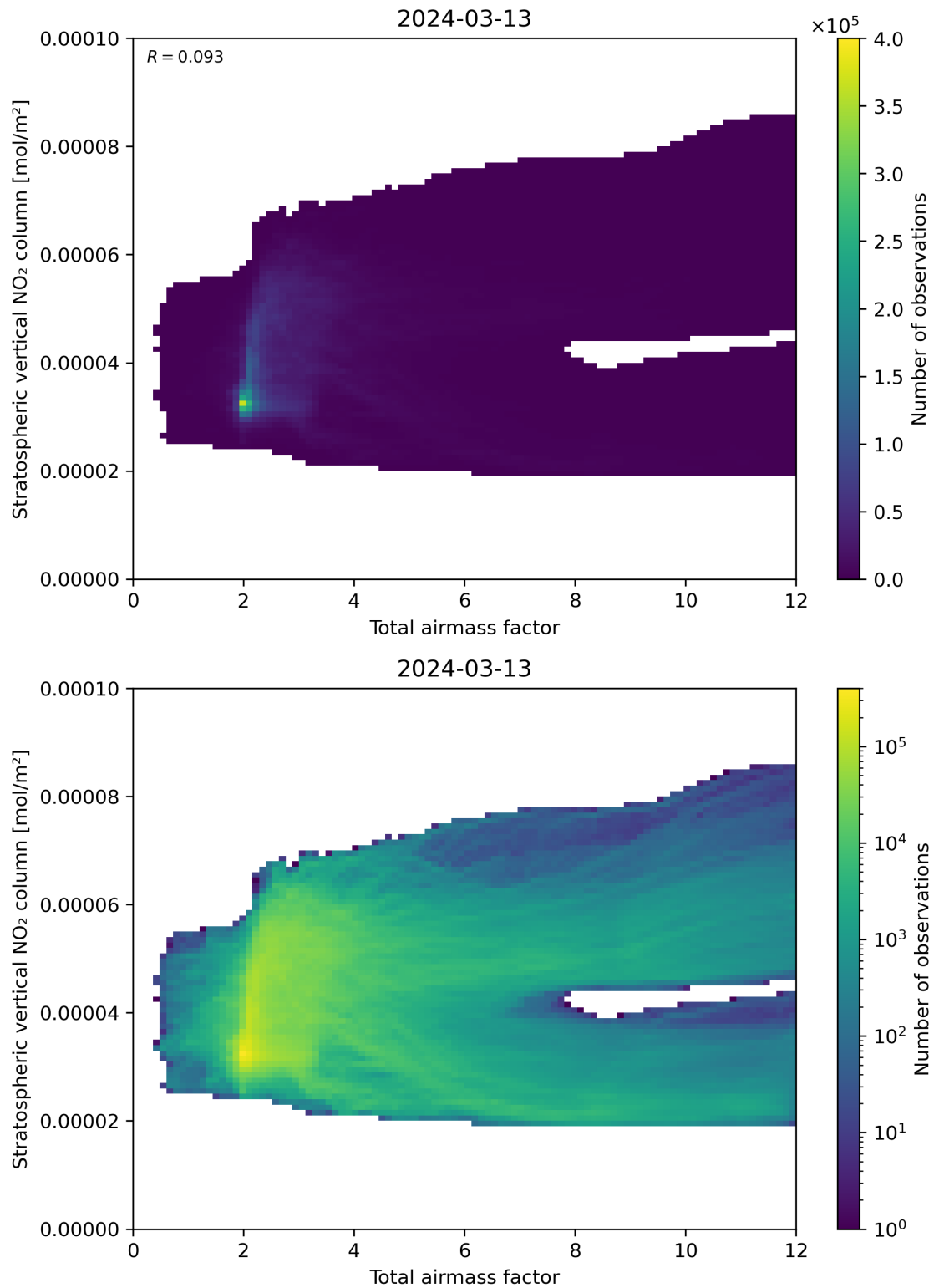
Figure 64: Scatter density plot of “Total airmass factor” against “Stratospheric vertical NO 2 column” for 2024-03-12 to 2024-03-14.
