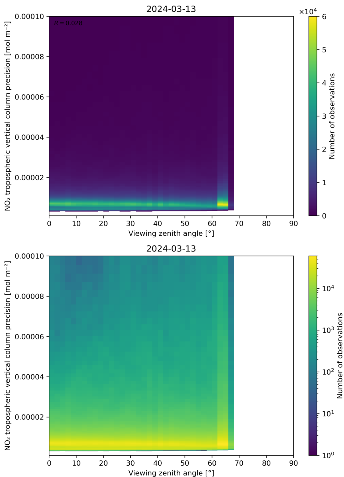
Figure 170: Scatter density plot of “Viewing zenith angle” against “NO 2 tropospheric vertical column precision” for 2024-03-12 to 2024-03-14.
