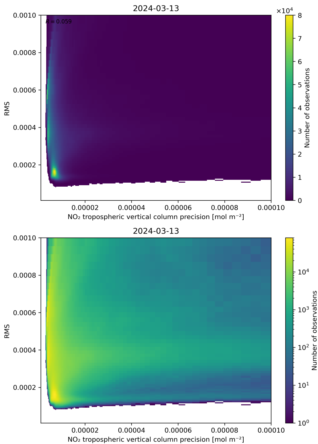
Figure 140: Scatter density plot of “NO 2 tropospheric vertical column precision” against “RMS” for 2024-03-12 to 2024-03-14.
