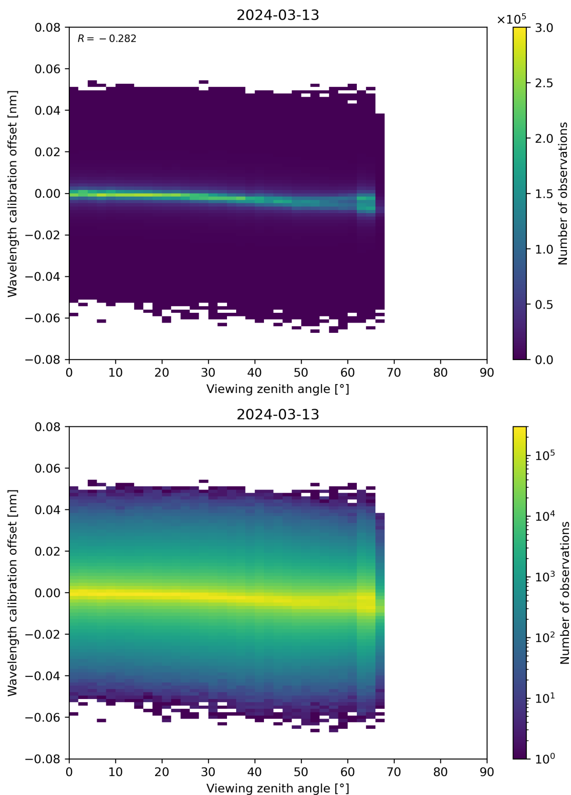
Figure 173: Scatter density plot of “Viewing zenith angle” against “Wavelength calibration offset” for 2024-03-12 to 2024-03-14.
