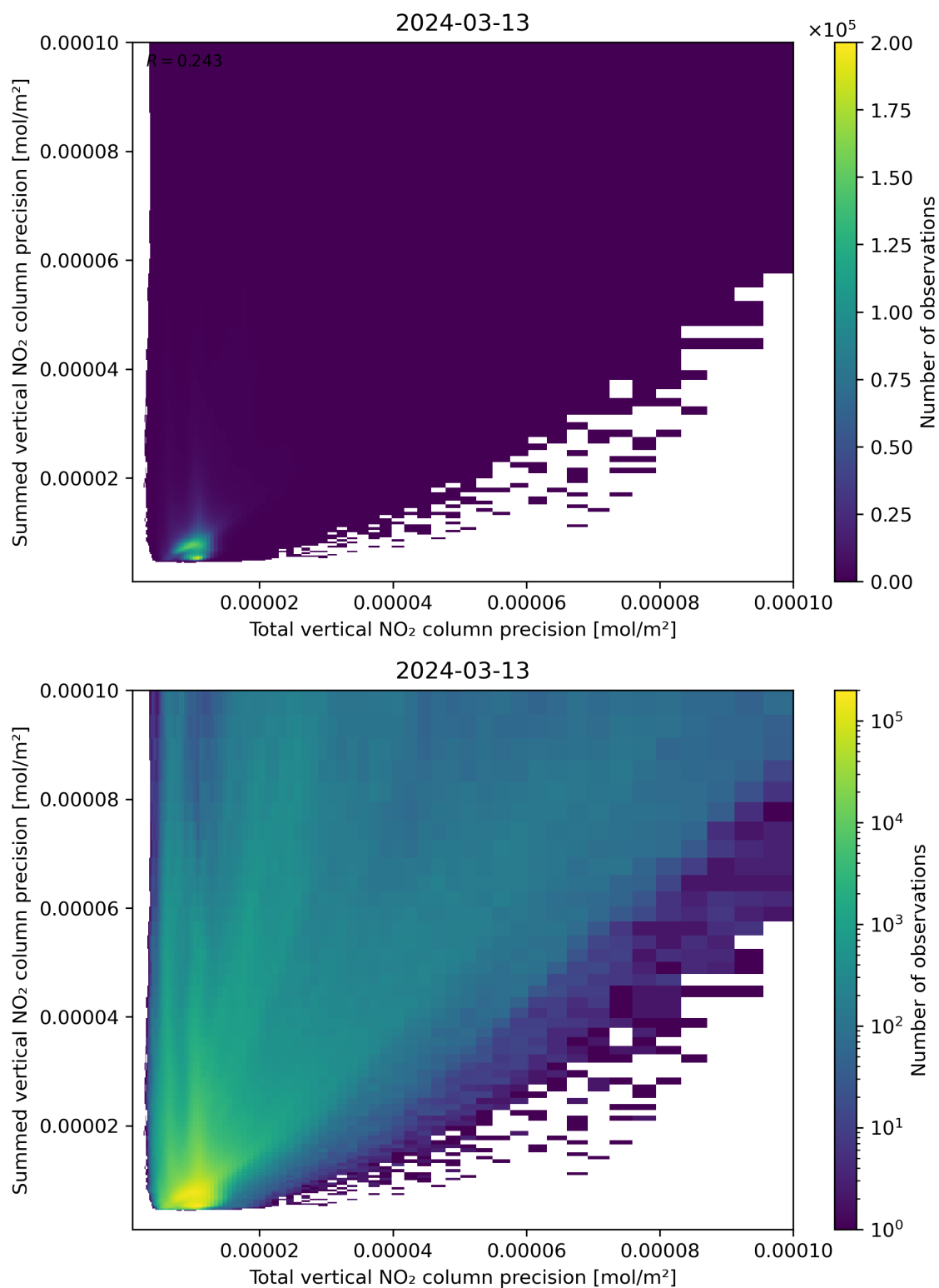
Figure 118: Scatter density plot of “Total vertical NO 2 column precision” against “Summed vertical NO 2 column precision” for 2024-03-12 to 2024-03-14.
