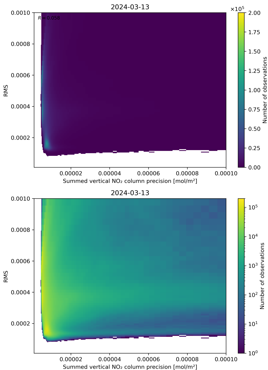
Figure 108: Scatter density plot of “Summed vertical NO 2 column precision” against “RMS” for 2024-03-12 to 2024-03-14.
