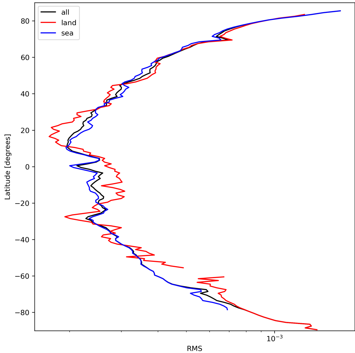
Figure 26: Zonal average of “RMS” for 2024-03-12 to 2024-03-14.
