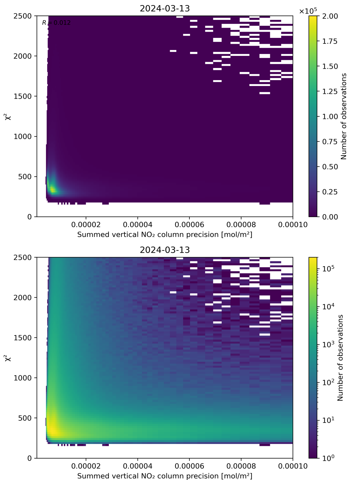
Figure 107: Scatter density plot of “Summed vertical NO 2 column precision” against “ \chi^2 ” for 2024-03-12 to 2024-03-14.
