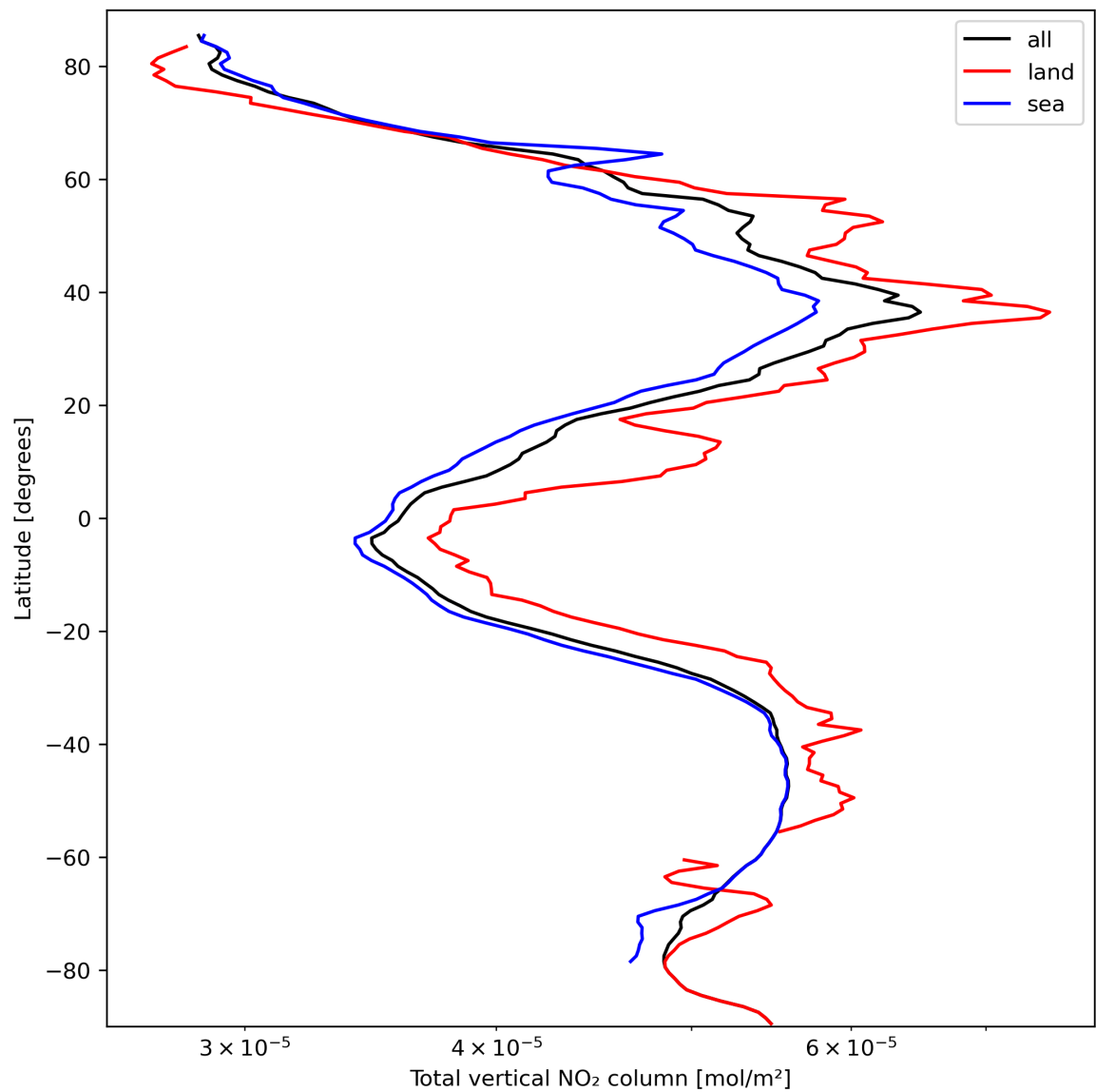
Figure 21: Zonal average of “Total vertical NO 2 column” for 2024-03-12 to 2024-03-14.
