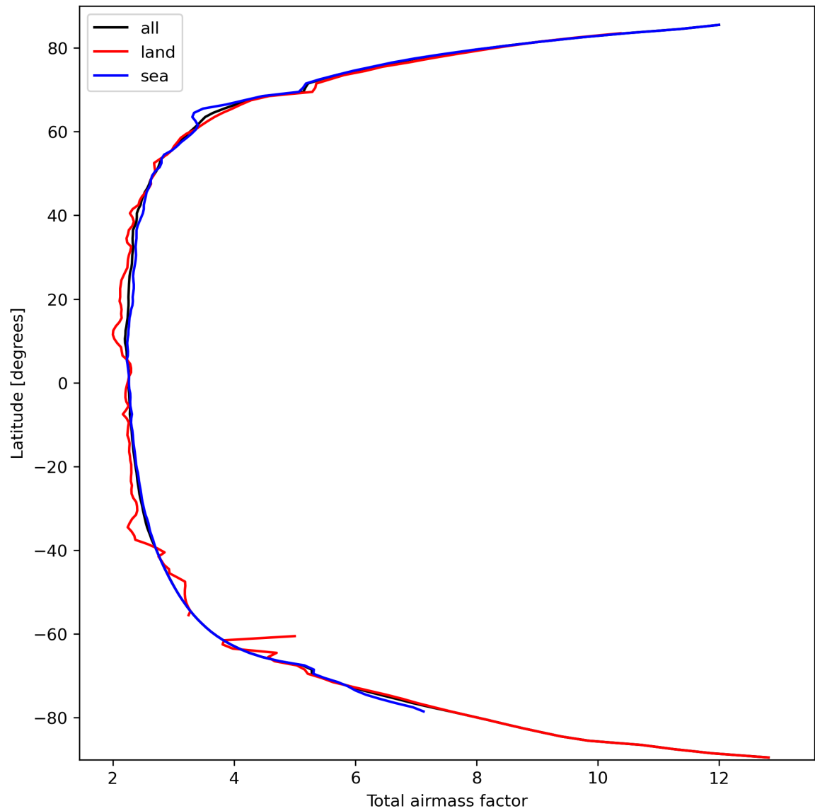
Figure 15: Zonal average of “Total airmass factor” for 2024-03-12 to 2024-03-14.
