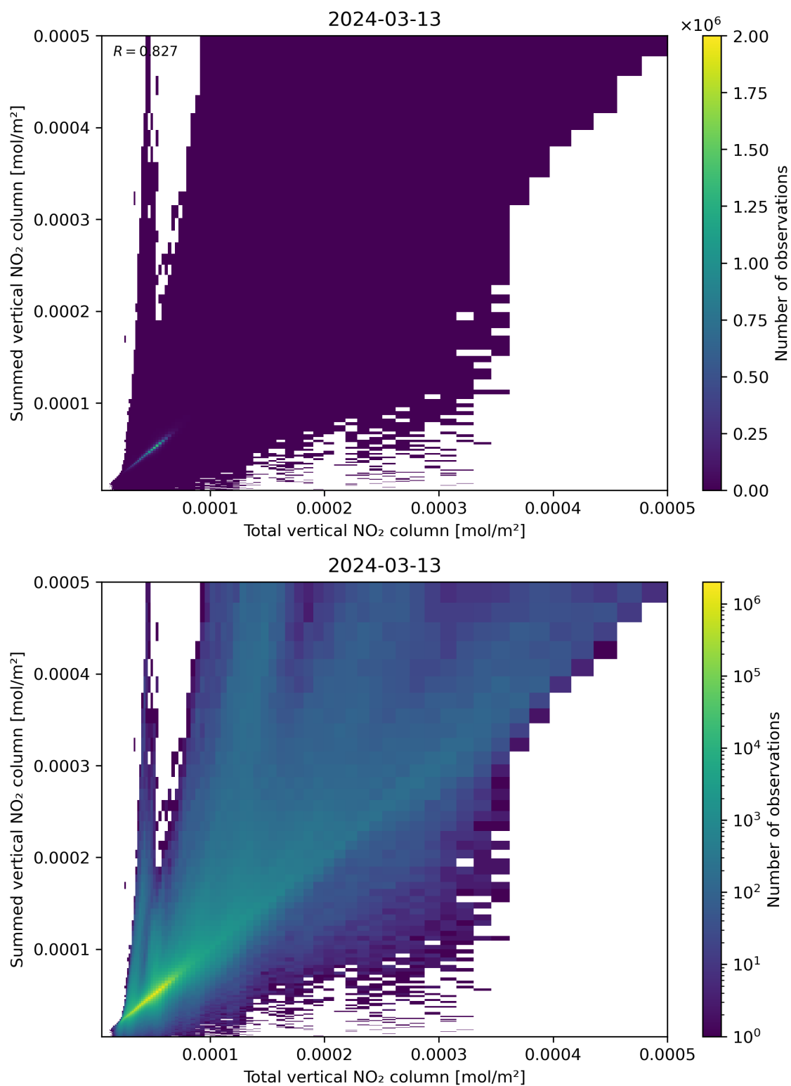
Figure 112: Scatter density plot of “Total vertical NO 2 column” against “Summed vertical NO 2 column” for 2024-03-12 to 2024-03-14.
