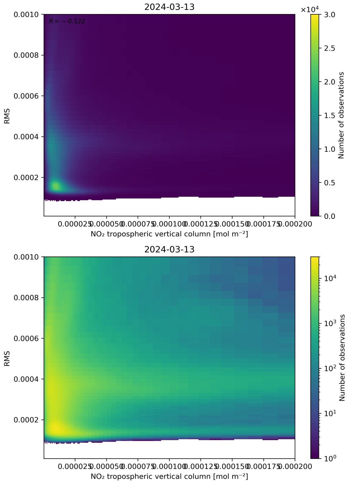
Figure 142: Scatter density plot of “NO 2 tropospheric vertical column” against “RMS” for 2024-03-12 to 2024-03-14.
