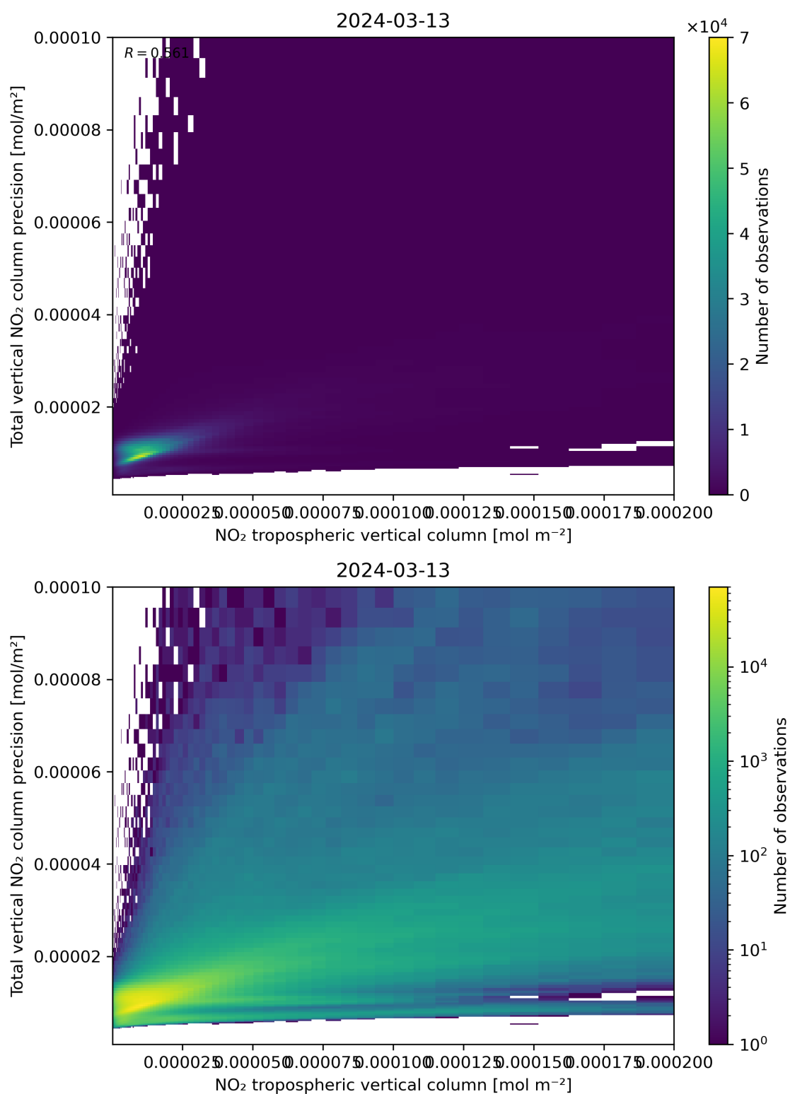
Figure 129: Scatter density plot of “NO 2 tropospheric vertical column” against “Total vertical NO 2 column precision” for 2024-03-12 to 2024-03-14.
