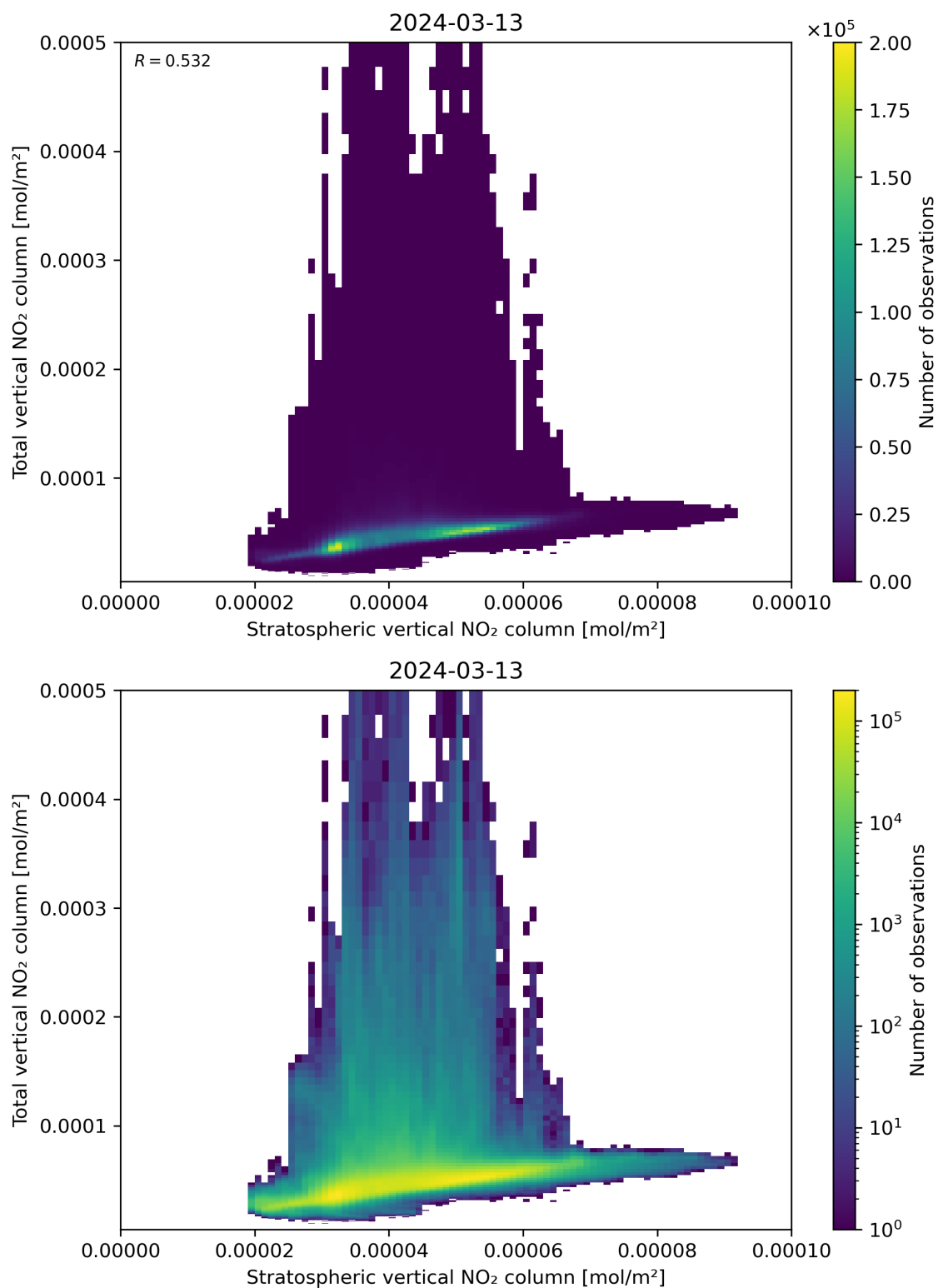
Figure 100: Scatter density plot of “Stratospheric vertical NO 2 column” against “Total vertical NO 2 column” for 2024-03-12 to 2024-03-14.
