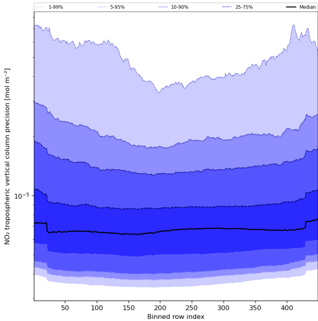
Figure 47: Along track statistics of “NO 2 tropospheric vertical column precision” for 2024-03-12 to 2024-03-14
