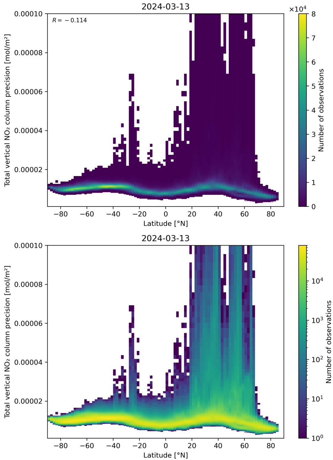
Figure 91: Scatter density plot of “Latitude” against “Total vertical NO 2 column precision” for 2024-03-12 to 2024-03-14.
