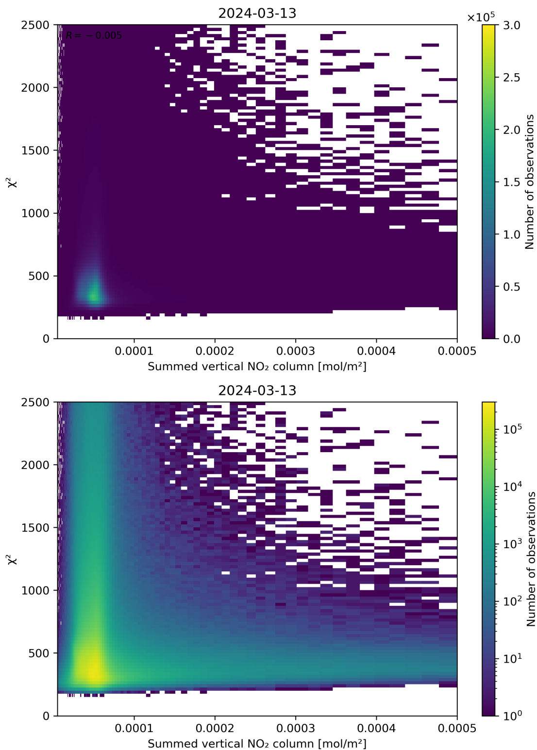
Figure 104: Scatter density plot of “Summed vertical NO 2 column” against “ \chi^2 ” for 2024-03-12 to 2024-03-14.
