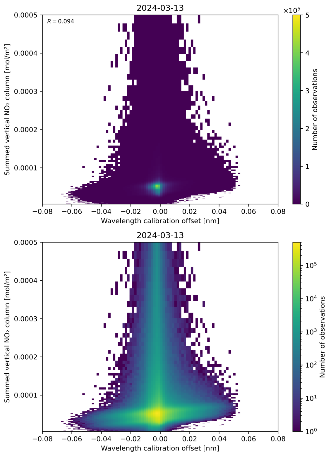
Figure 177: Scatter density plot of “Wavelength calibration offset” against “Summed vertical NO 2 column” for 2024-03-12 to 2024-03-14.
