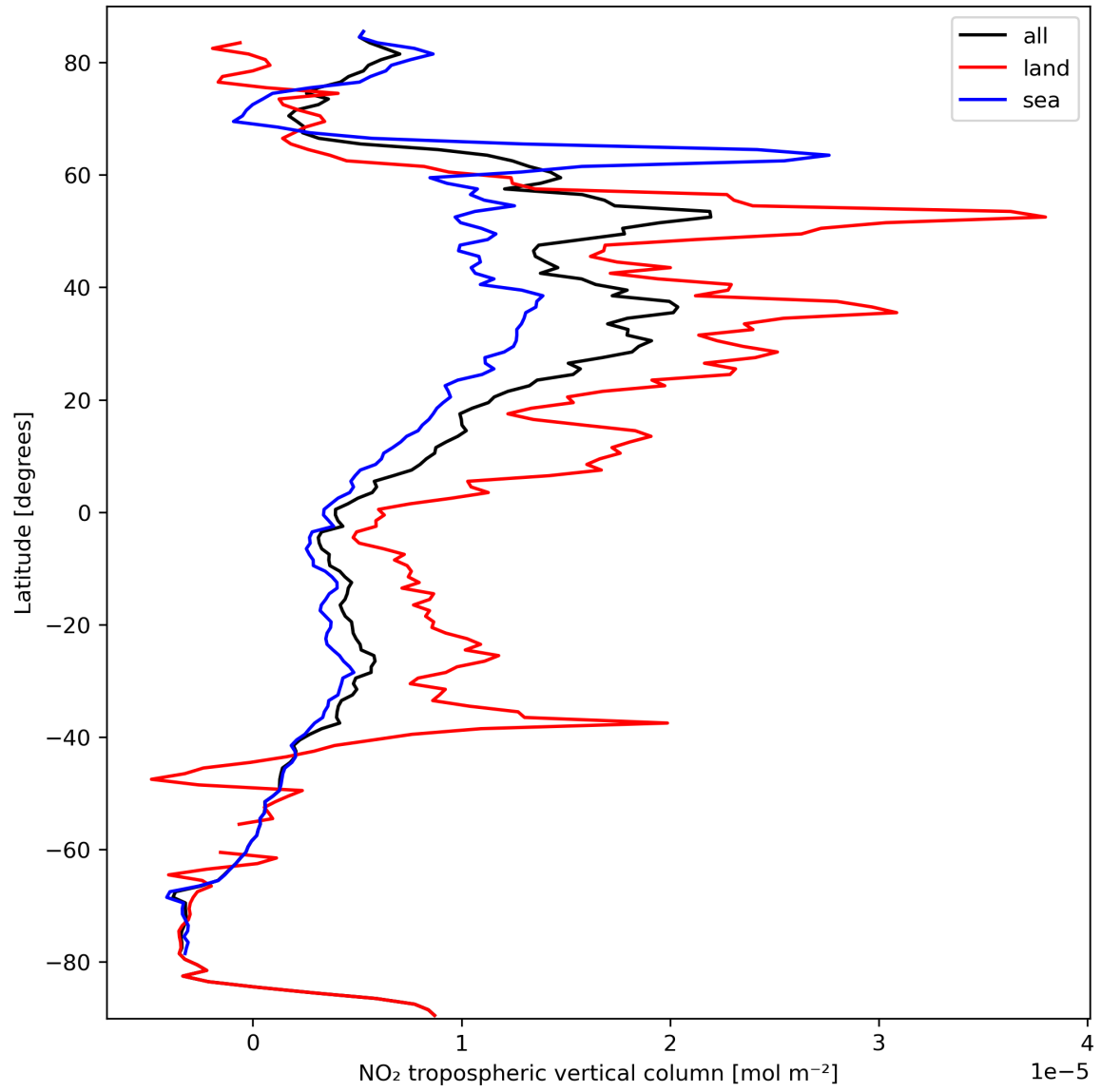
Figure 12: Zonal average of “NO 2 tropospheric vertical column” for 2024-03-12 to 2024-03-14.
