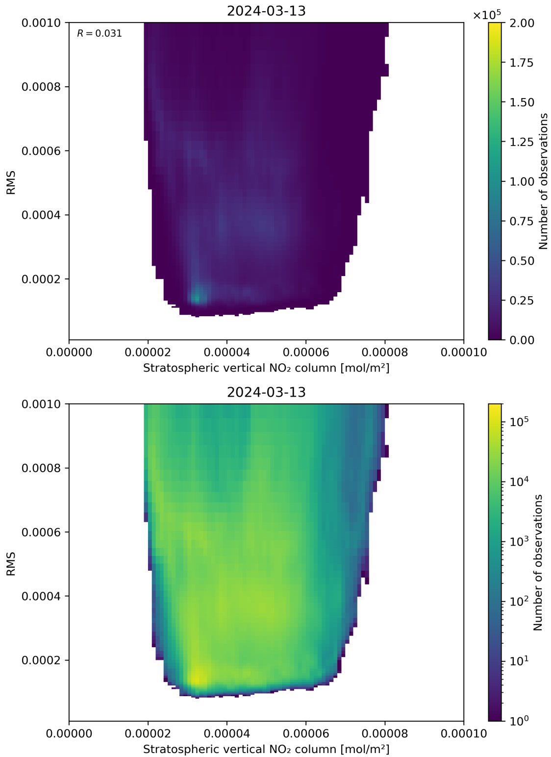
Figure 102: Scatter density plot of “Stratospheric vertical NO 2 column” against “RMS” for 2024-03-12 to 2024-03-14.
