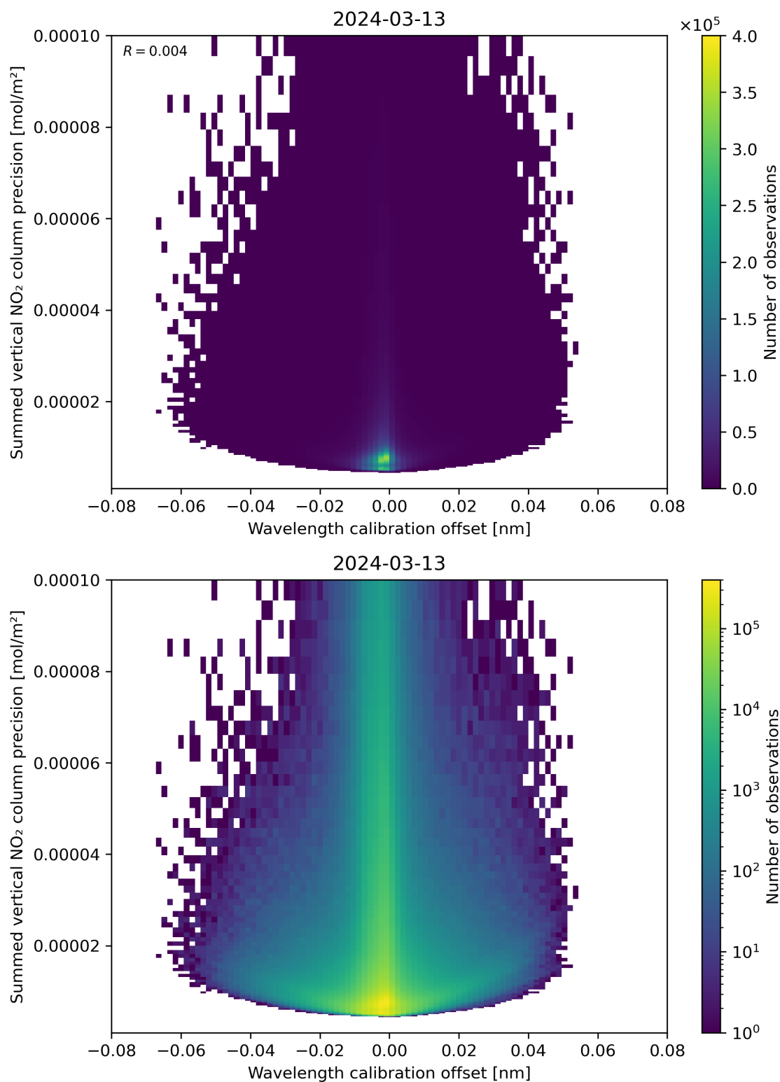
Figure 178: Scatter density plot of “Wavelength calibration offset” against “Summed vertical NO 2 column precision” for 2024-03-12 to 2024-03-14.
