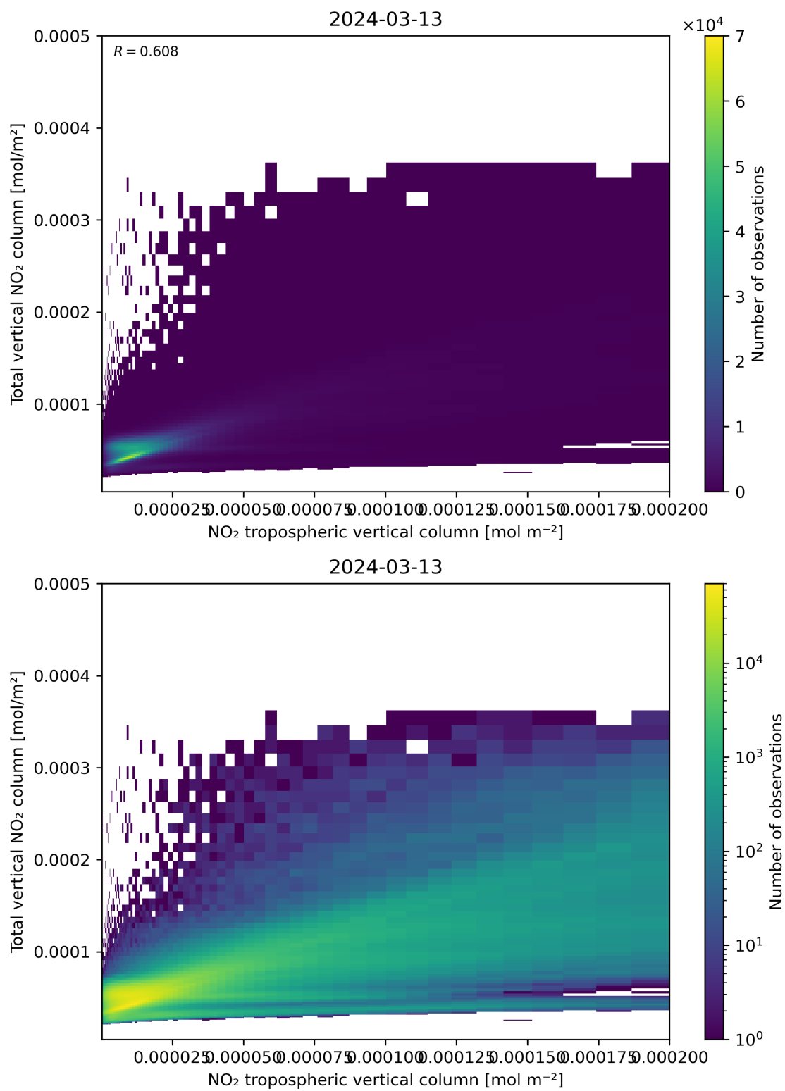
Figure 128: Scatter density plot of “NO 2 tropospheric vertical column” against “Total vertical NO 2 column” for 2024-03-12 to 2024-03-14.
