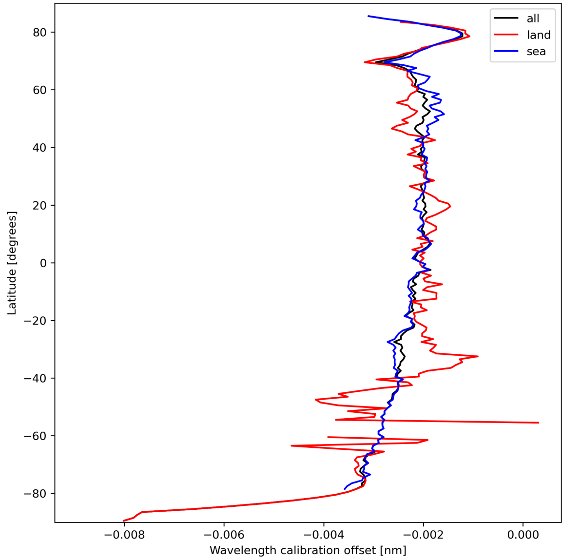
Figure 18: Zonal average of “Wavelength calibration offset” for 2024-03-12 to 2024-03-14.
