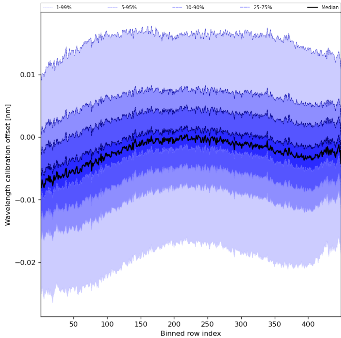
Figure 52: Along track statistics of “Wavelength calibration offset” for 2024-03-12 to 2024-03-14
