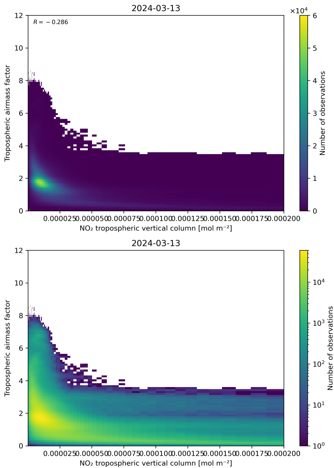
Figure 123: Scatter density plot of “NO 2 tropospheric vertical column” against “Tropospheric air mass factor” for 2024-03-12 to 2024-03-14.
