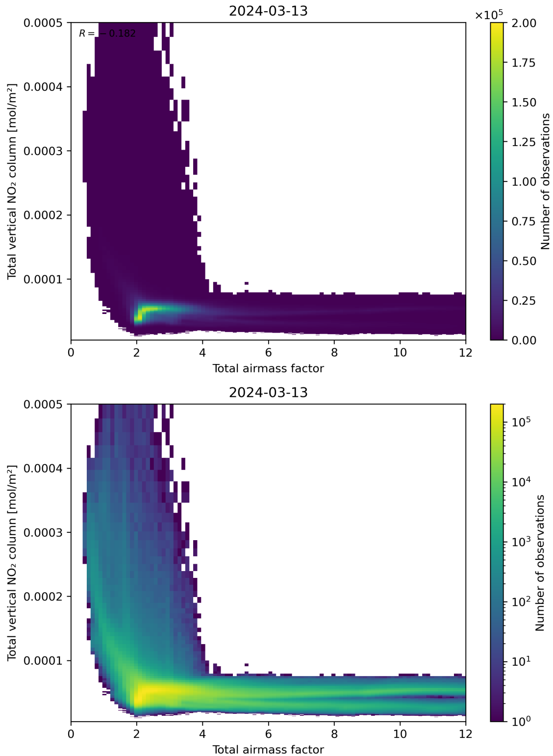
Figure 67: Scatter density plot of “Total airmass factor” against “Total vertical NO 2 column” for 2024-03-12 to 2024-03-14.
