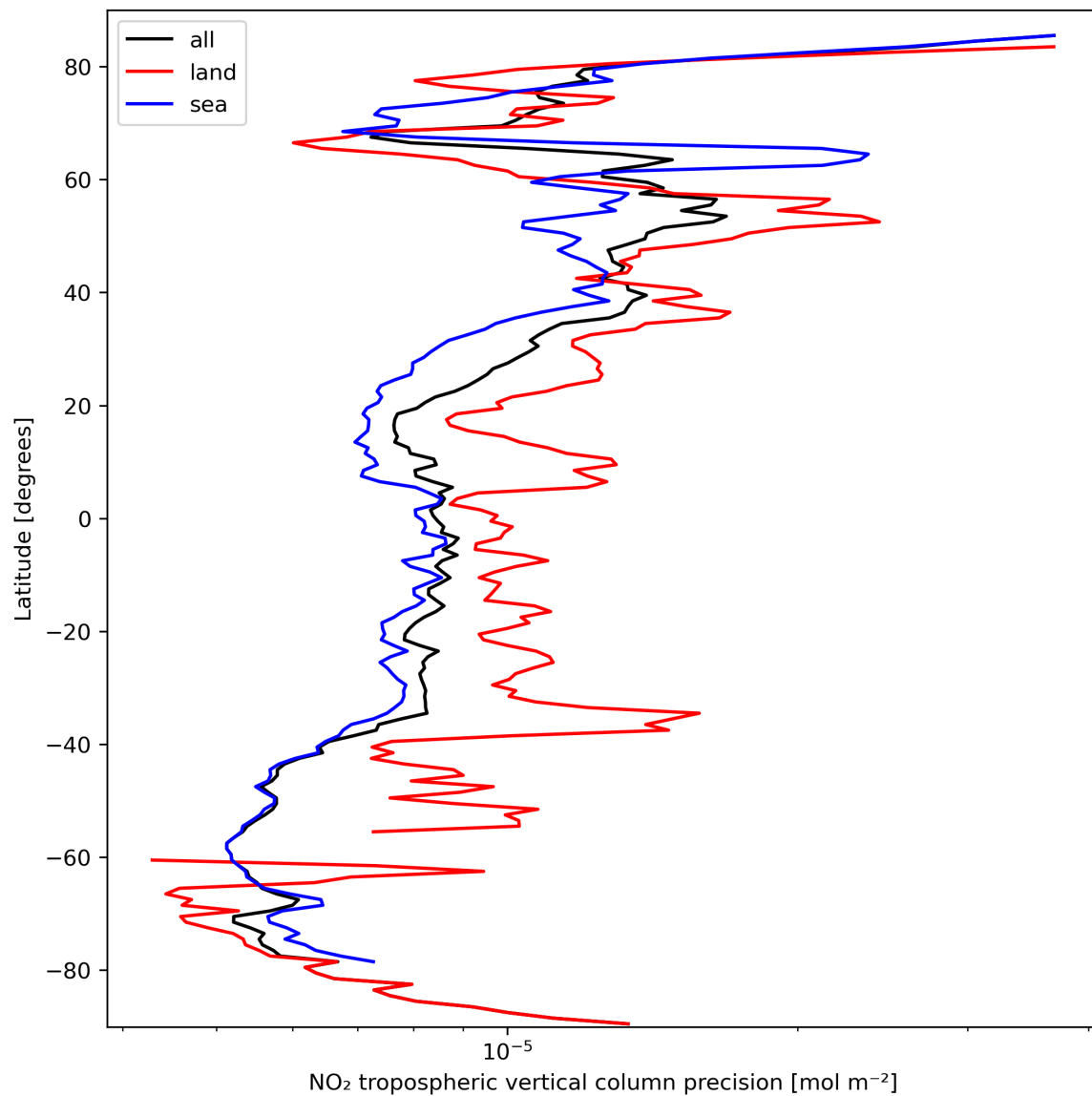
Figure 13: Zonal average of “NO 2 tropospheric vertical column precision” for 2024-03-12 to 2024-03-14.
