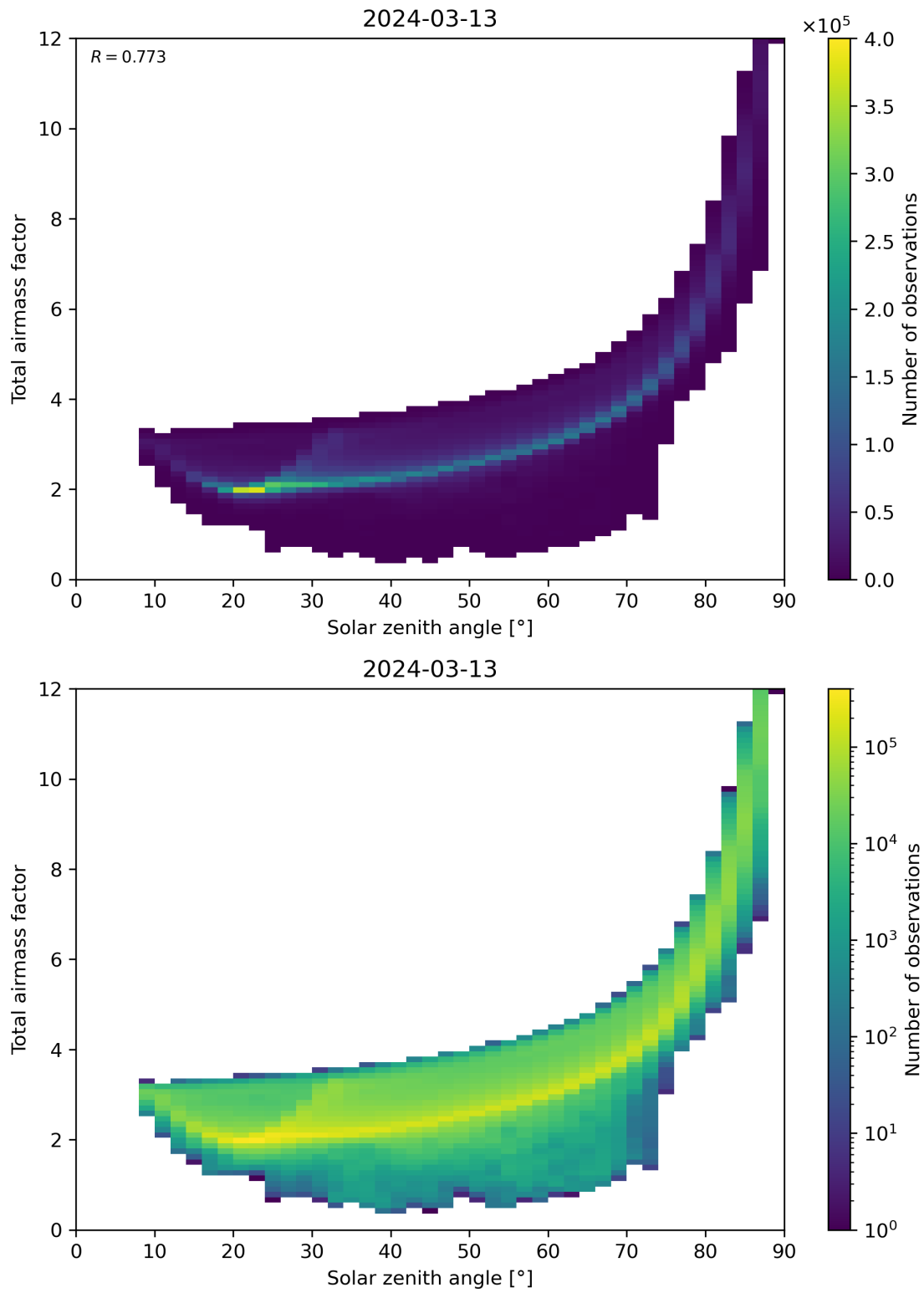
Figure 146: Scatter density plot of “Solar zenith angle” against “Total air mass factor” for 2024-03-12 to 2024-03-14.
