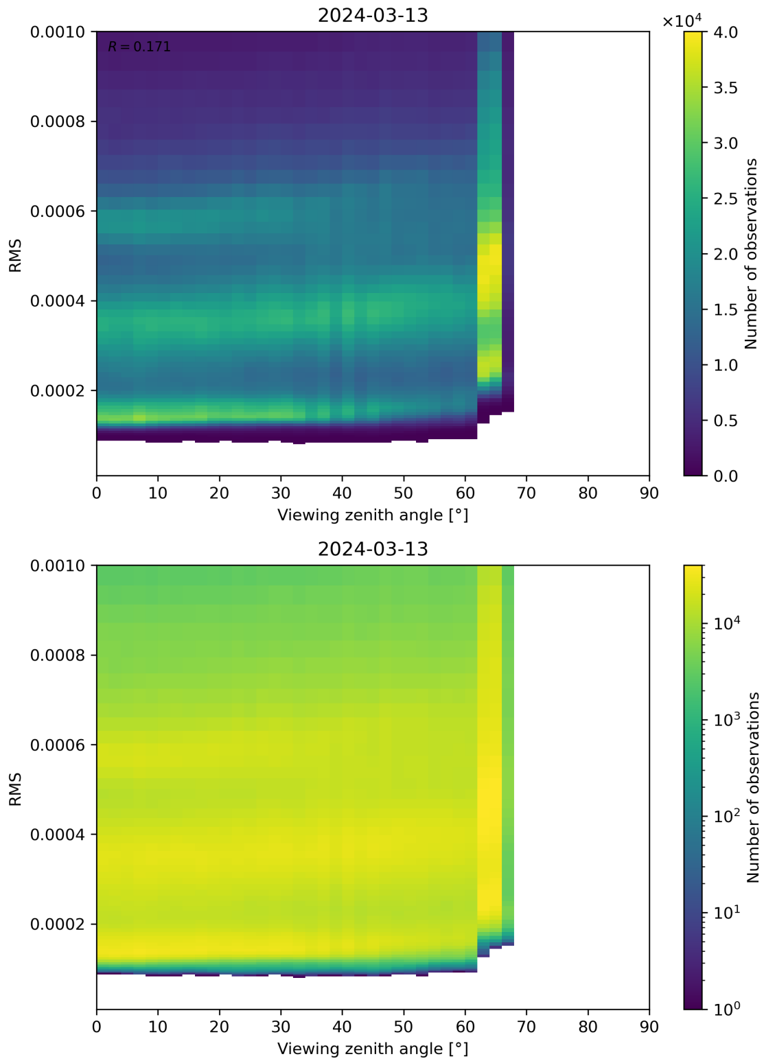
Figure 171: Scatter density plot of “Viewing zenith angle” against “RMS” for 2024-03-12 to 2024-03-14.
