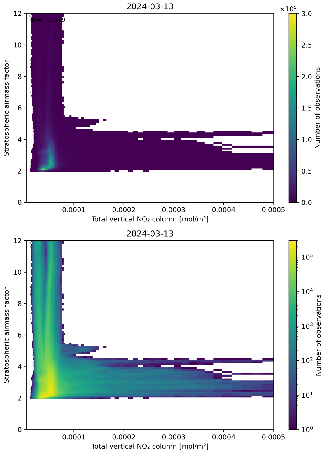
Figure 110: Scatter density plot of “Total vertical NO 2 column” against “Stratospheric airmass factor” for 2024-03-12 to 2024-03-14.
