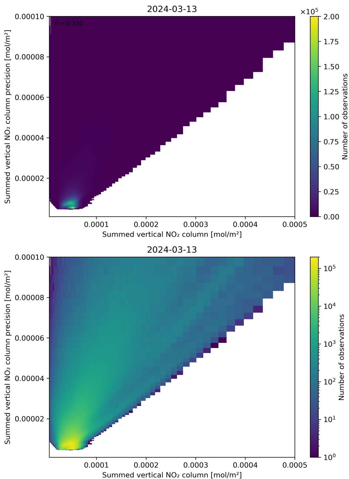
Figure 105: Scatter density plot of “Summed vertical NO 2 column” against “Summed vertical NO 2 column precision” for 2024-03-12 to 2024-03-14.
