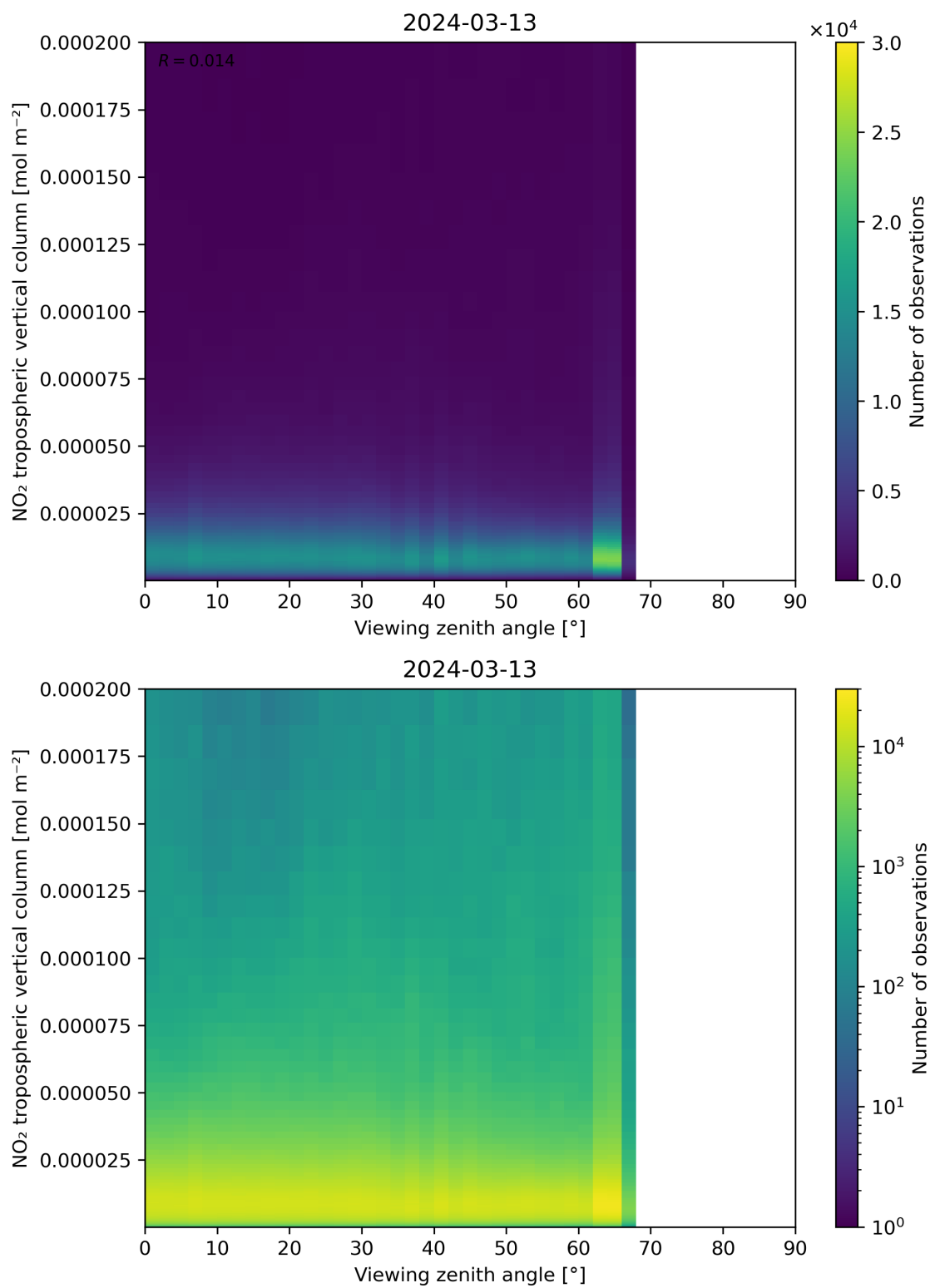
Figure 169: Scatter density plot of “Viewing zenith angle” against “NO 2 tropospheric vertical column” for 2024-03-12 to 2024-03-14.
