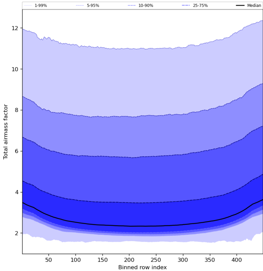
Figure 49: Along track statistics of “Total airmass factor” for 2024-03-12 to 2024-03-14
