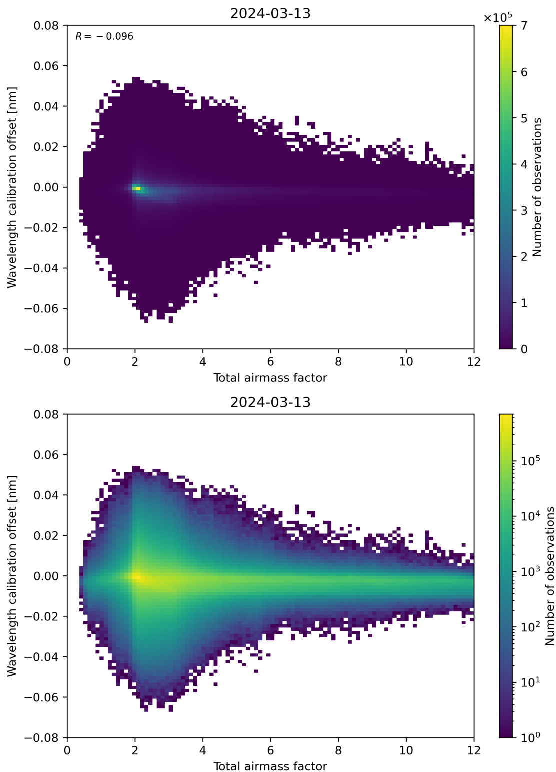
Figure 70: Scatter density plot of “Total airmass factor” against “Wavelength calibration offset” for 2024-03-12 to 2024-03-14.
