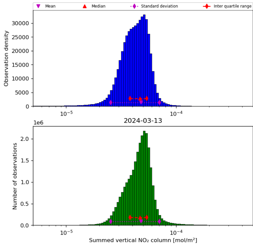
Figure 40: Histogram of “Summed vertical NO 2 column” for 2024-03-12 to 2024-03-14
