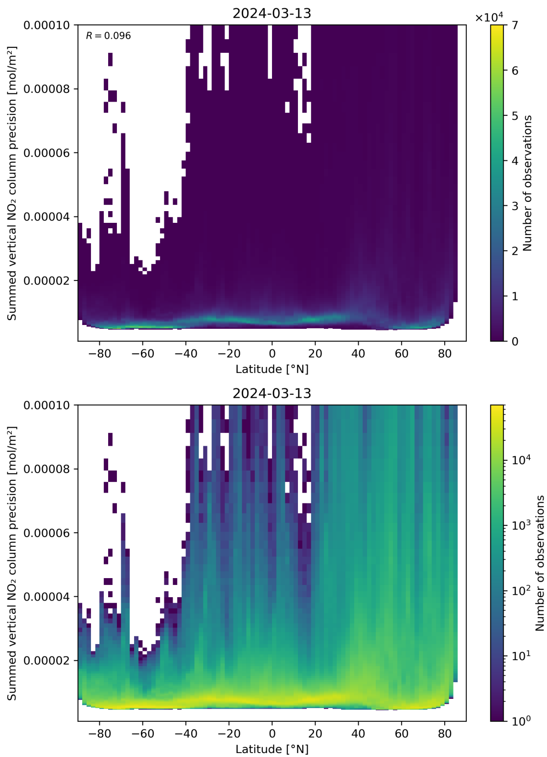
Figure 89: Scatter density plot of “Latitude” against “Summed vertical NO 2 column precision” for 2024-03-12 to 2024-03-14.
