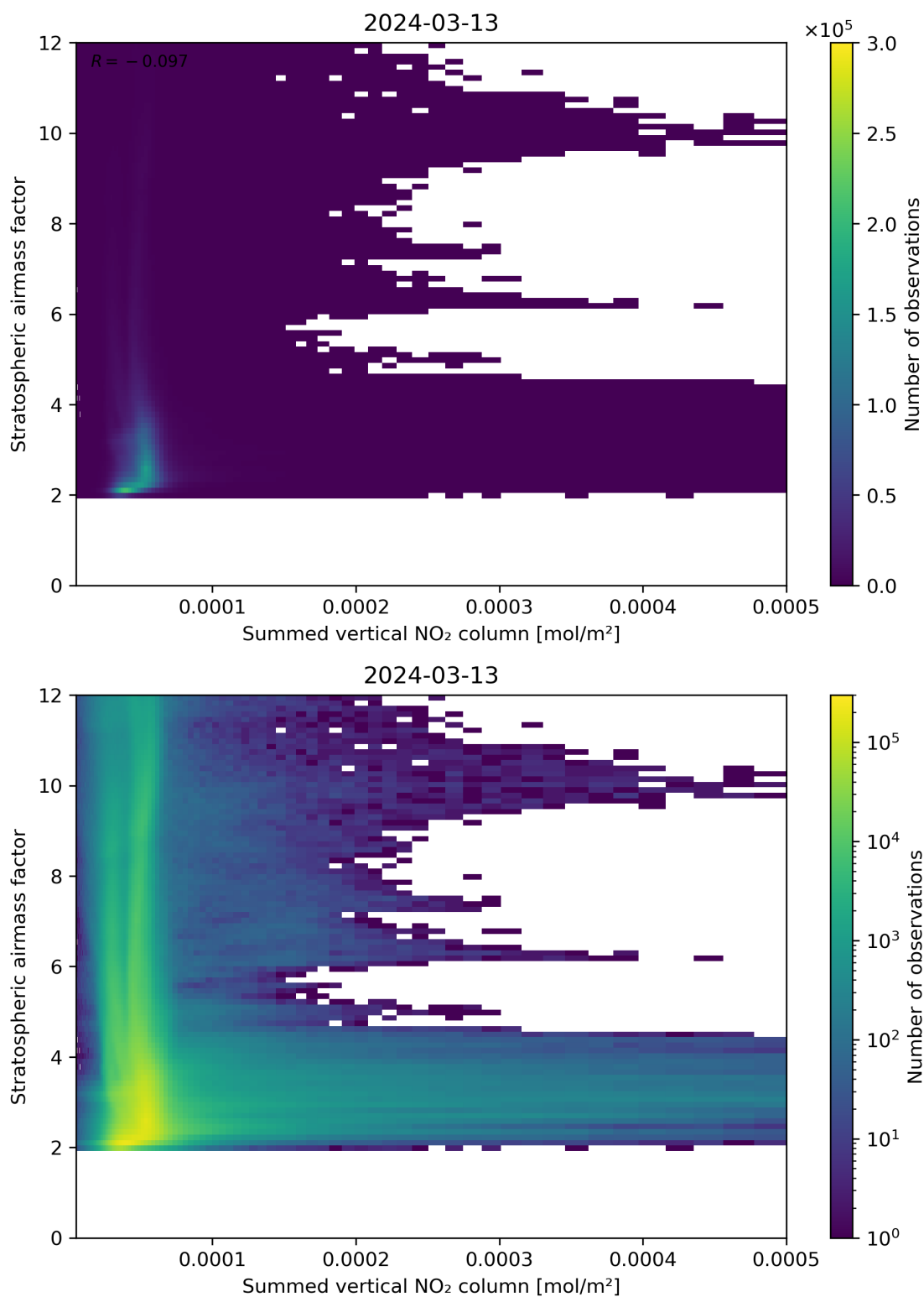
Figure 103: Scatter density plot of “Summed vertical NO 2 column” against “Stratospheric air mass factor” for 2024-03-12 to 2024-03-14.
