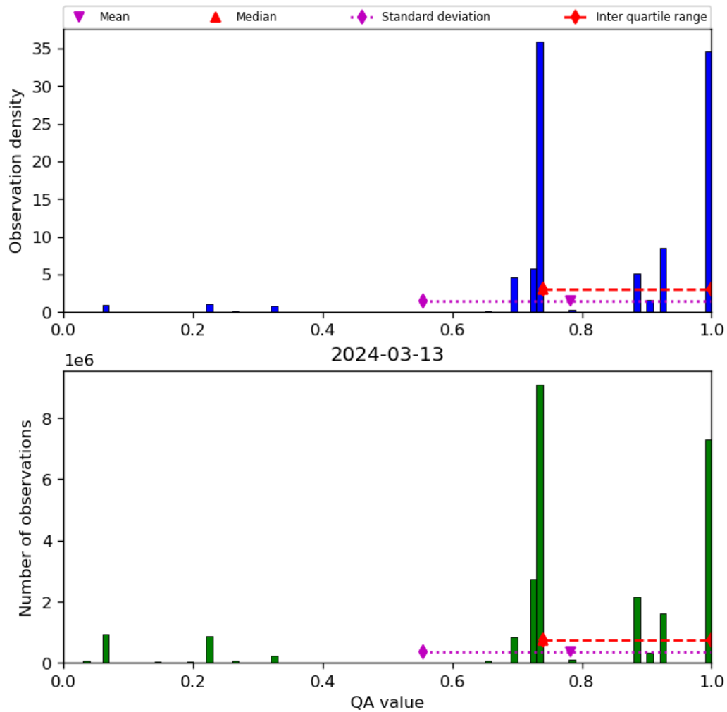
Figure 28: Histogram of “QA value” for 2024-03-12 to 2024-03-14
