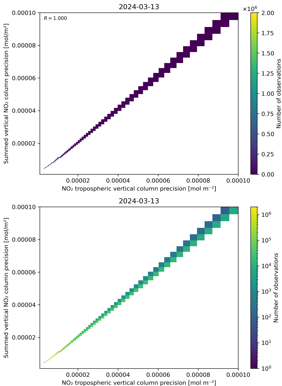
Figure 137: Scatter density plot of “NO 2 tropospheric vertical column precision” against “Summed vertical NO 2 column precision” for 2024-03-12 to 2024-03-14.
