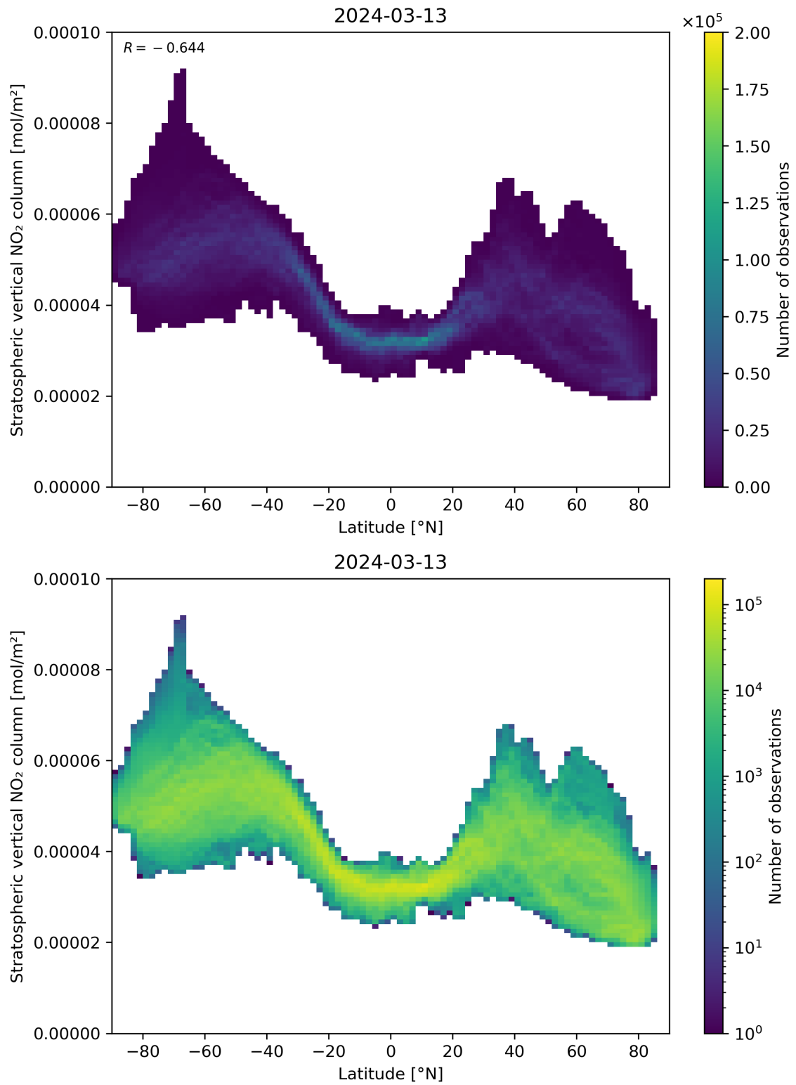
Figure 87: Scatter density plot of “Latitude” against “Stratospheric vertical NO 2 column” for 2024-03-12 to 2024-03-14.
