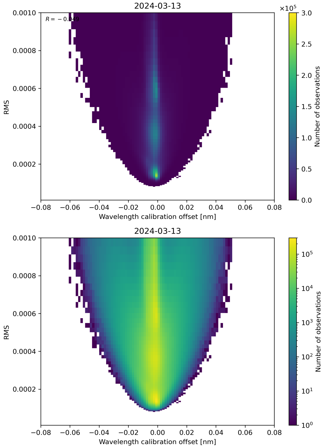
Figure 181: Scatter density plot of “Wavelength calibration offset” against “RMS” for 2024-03-12 to 2024-03-14.
