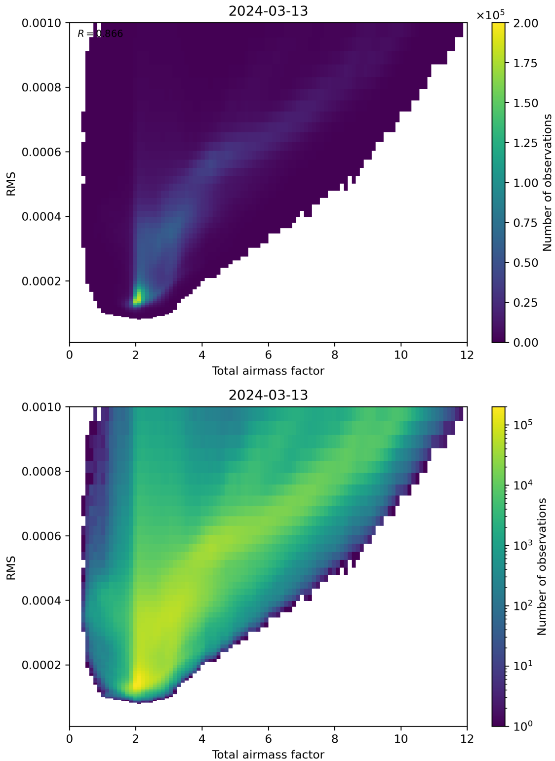
Figure 69: Scatter density plot of “Total airmass factor” against “RMS” for 2024-03-12 to 2024-03-14.
