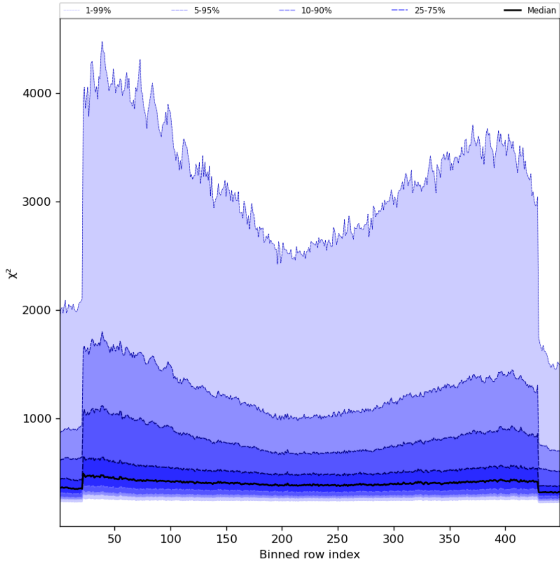
Figure 59: Along track statistics of “ \chi^2 ” for 2024-03-12 to 2024-03-14
