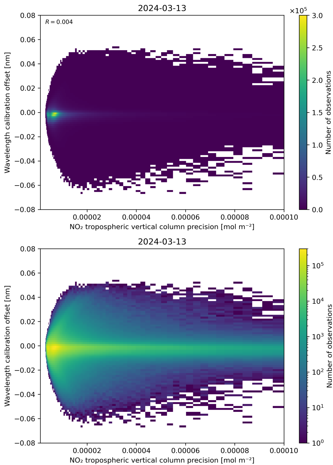
Figure 141: Scatter density plot of “NO 2 tropospheric vertical column precision” against “Wavelength calibration offset” for 2024-03-12 to 2024-03-14.
