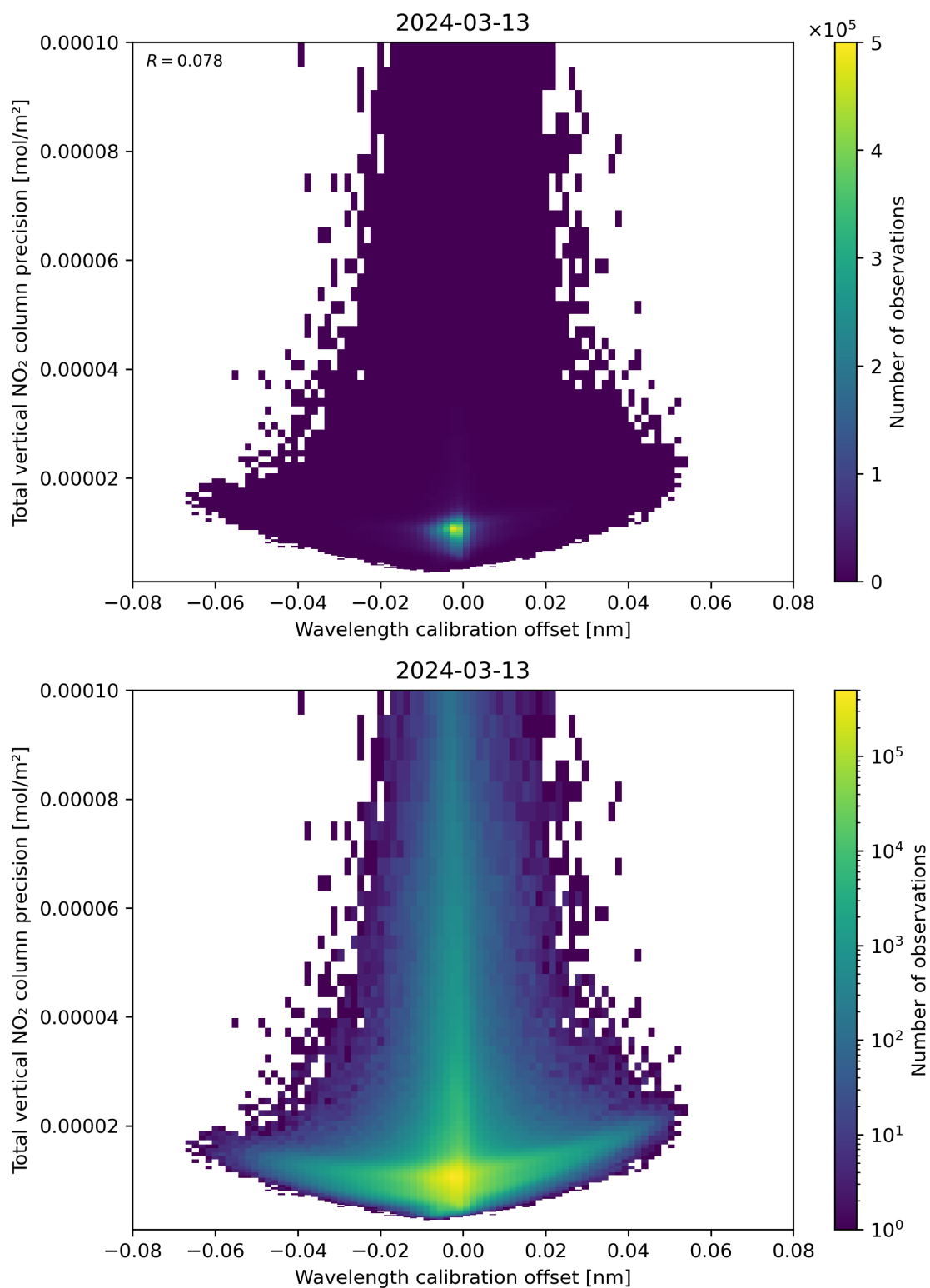
Figure 180: Scatter density plot of “Wavelength calibration offset” against “Total vertical NO 2 column precision” for 2024-03-12 to 2024-03-14.
