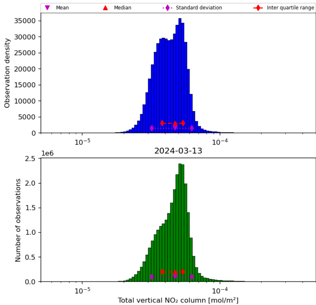
Figure 38: Histogram of “Total vertical NO 2 column” for 2024-03-12 to 2024-03-14
