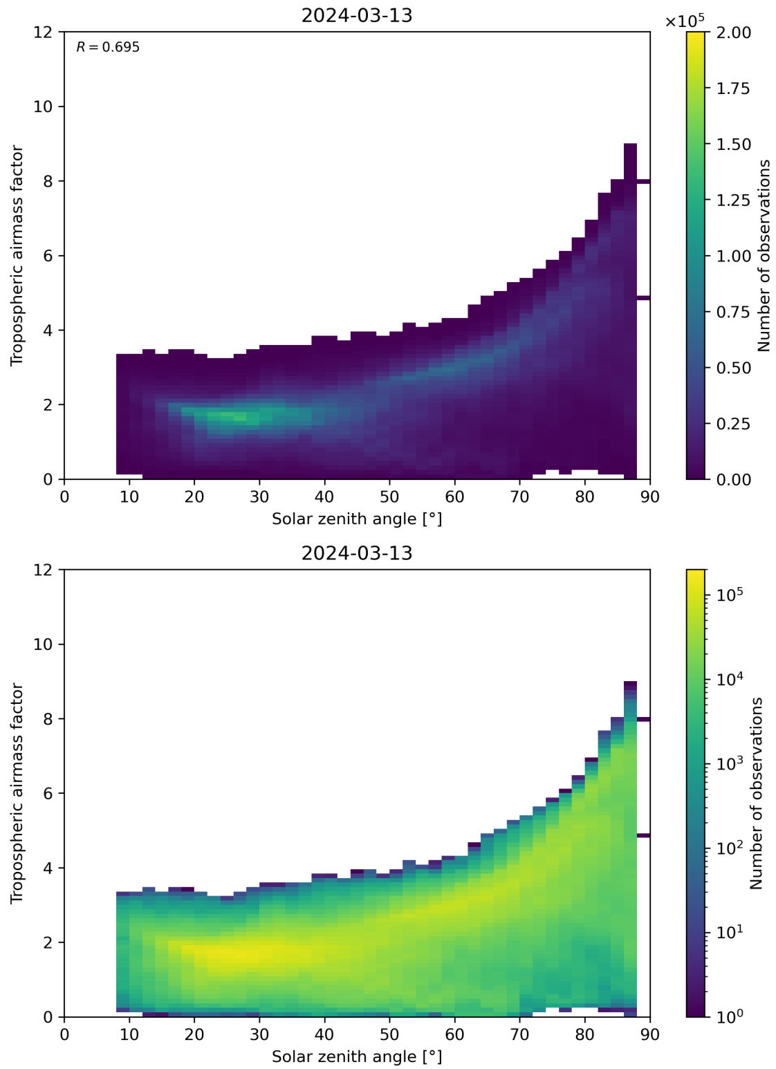
Figure 147: Scatter density plot of “Solar zenith angle” against “Tropospheric airmass factor” for 2024-03-12 to 2024-03-14.
