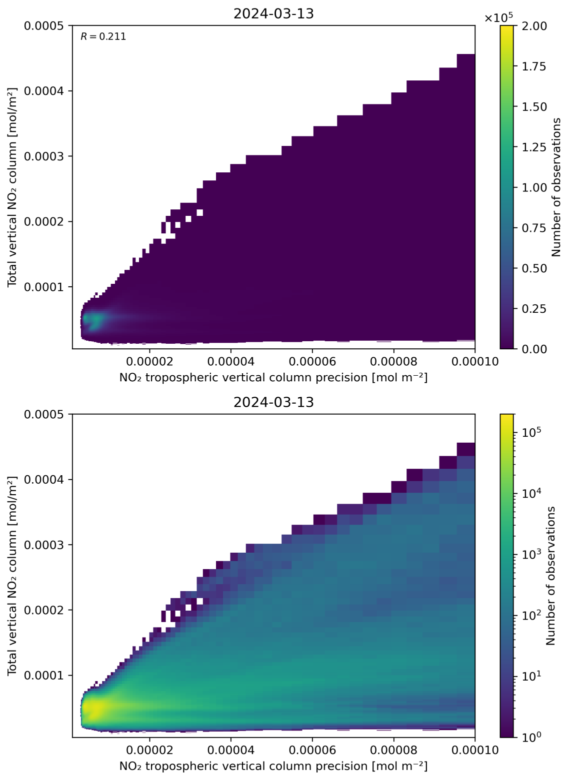
Figure 138: Scatter density plot of “NO 2 tropospheric vertical column precision” against “Total vertical NO 2 column” for 2024-03-12 to 2024-03-14.
