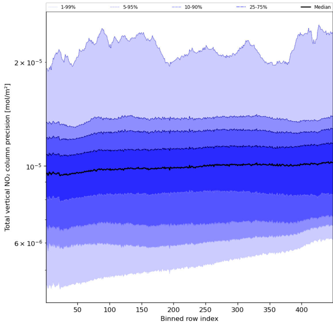
Figure 56: Along track statistics of “Total vertical NO 2 column precision” for 2024-03-12 to 2024-03-14
