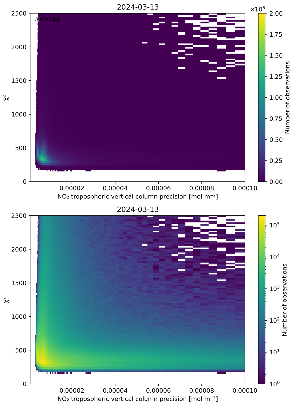
Figure 134: Scatter density plot of “NO 2 tropospheric vertical column precision” against “ \chi^2 ” for 2024-03-12 to 2024-03-14.
