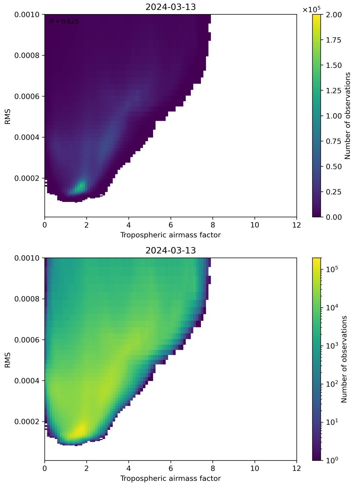
Figure 79: Scatter density plot of “Tropospheric airmass factor” against “RMS” for 2024-03-12 to 2024-03-14.
