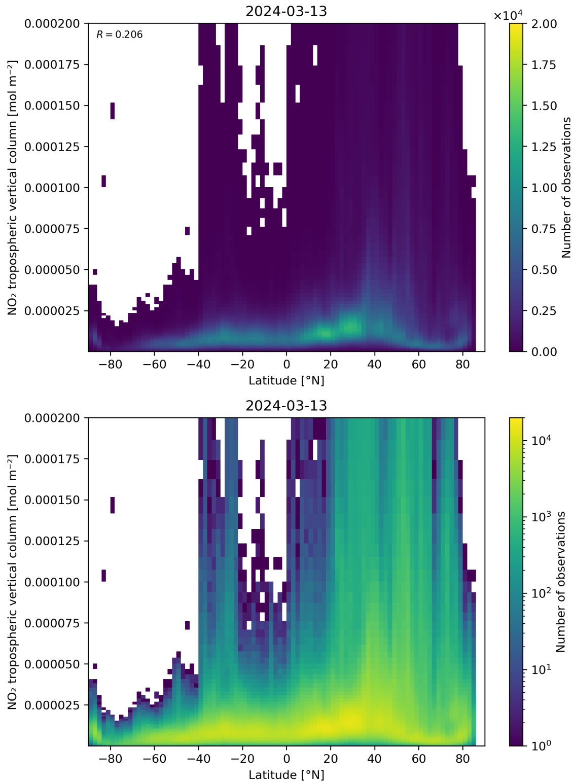
Figure 92: Scatter density plot of “Latitude” against “NO 2 tropospheric vertical column” for 2024-03-12 to 2024-03-14.
