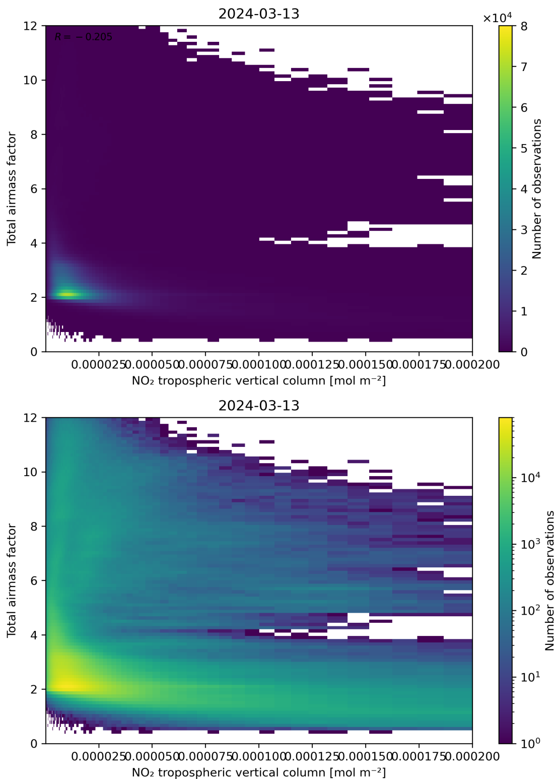
Figure 122: Scatter density plot of “NO 2 tropospheric vertical column” against “Total air mass factor” for 2024-03-12 to 2024-03-14.
