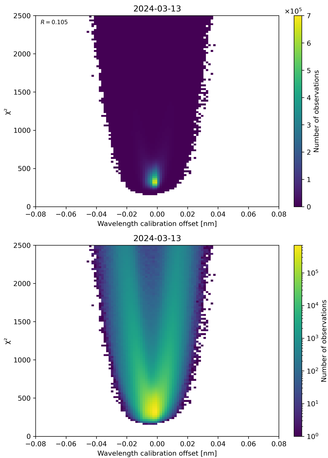
Figure 175: Scatter density plot of “Wavelength calibration offset” against “ \chi^2 ” for 2024-03-12 to 2024-03-14.
