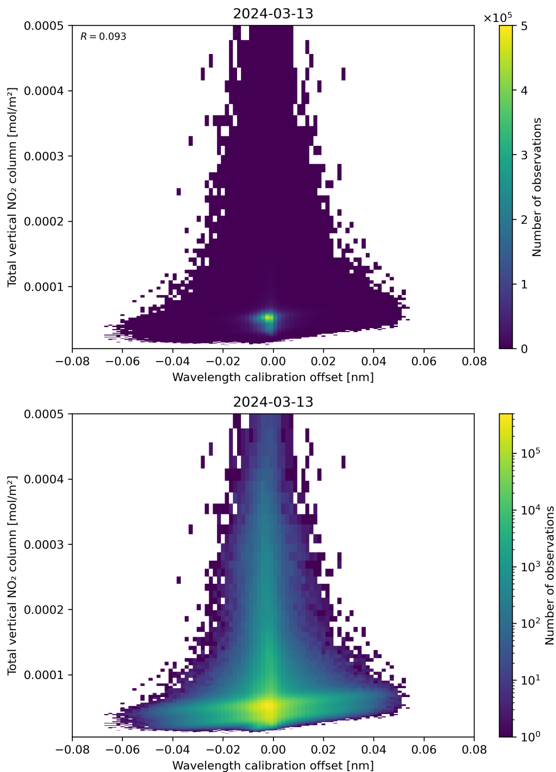
Figure 179: Scatter density plot of “Wavelength calibration offset” against “Total vertical NO 2 column” for 2024-03-12 to 2024-03-14.
