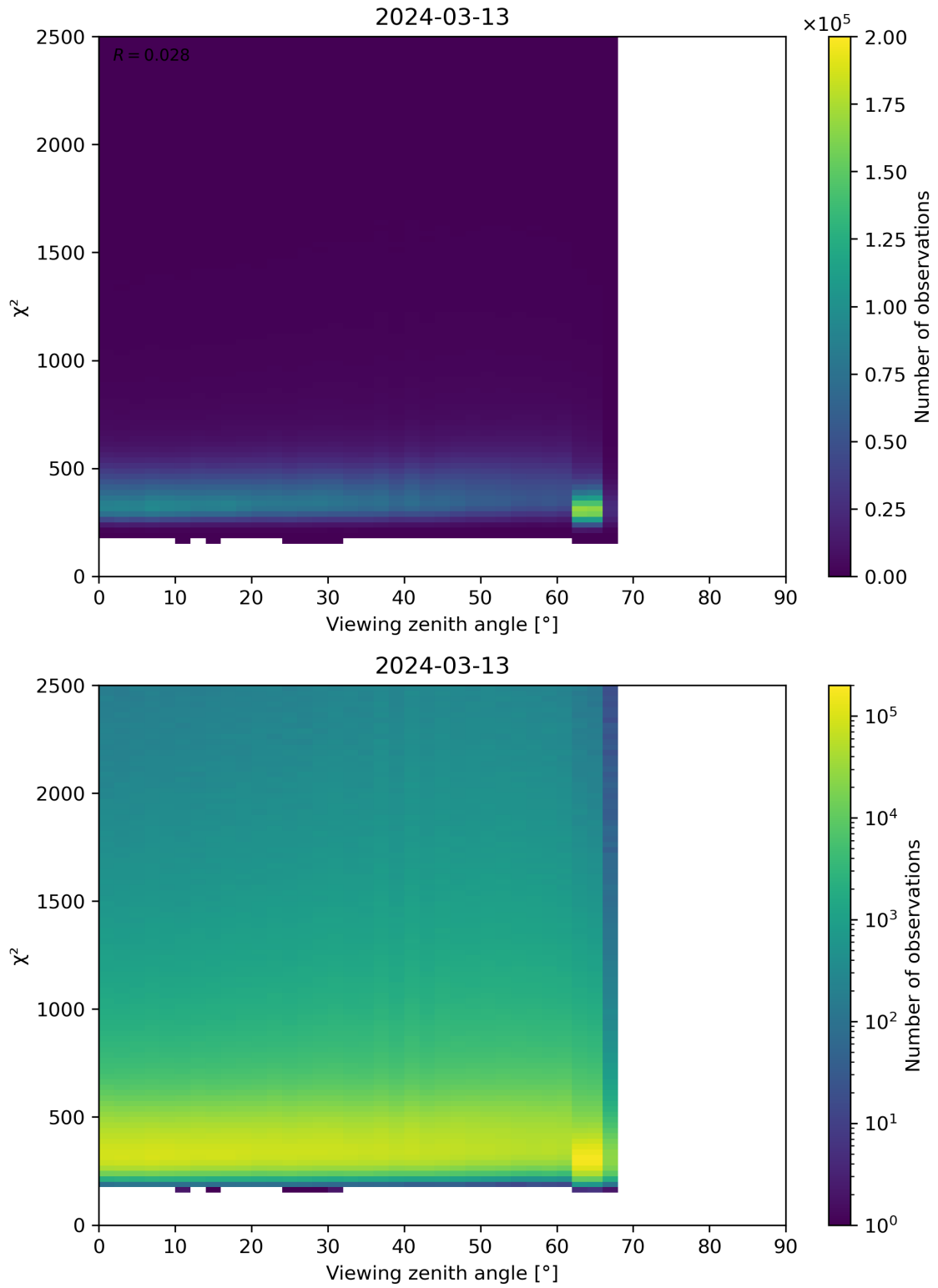
Figure 162: Scatter density plot of “Viewing zenith angle” against “ \chi^2 ” for 2024-03-12 to 2024-03-14.
