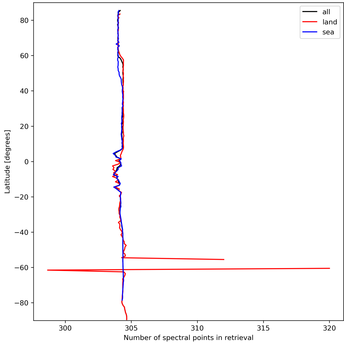
Figure 16: Zonal average of “Number of spectral points in retrieval” for 2024-03-12 to 2024-03-14.
