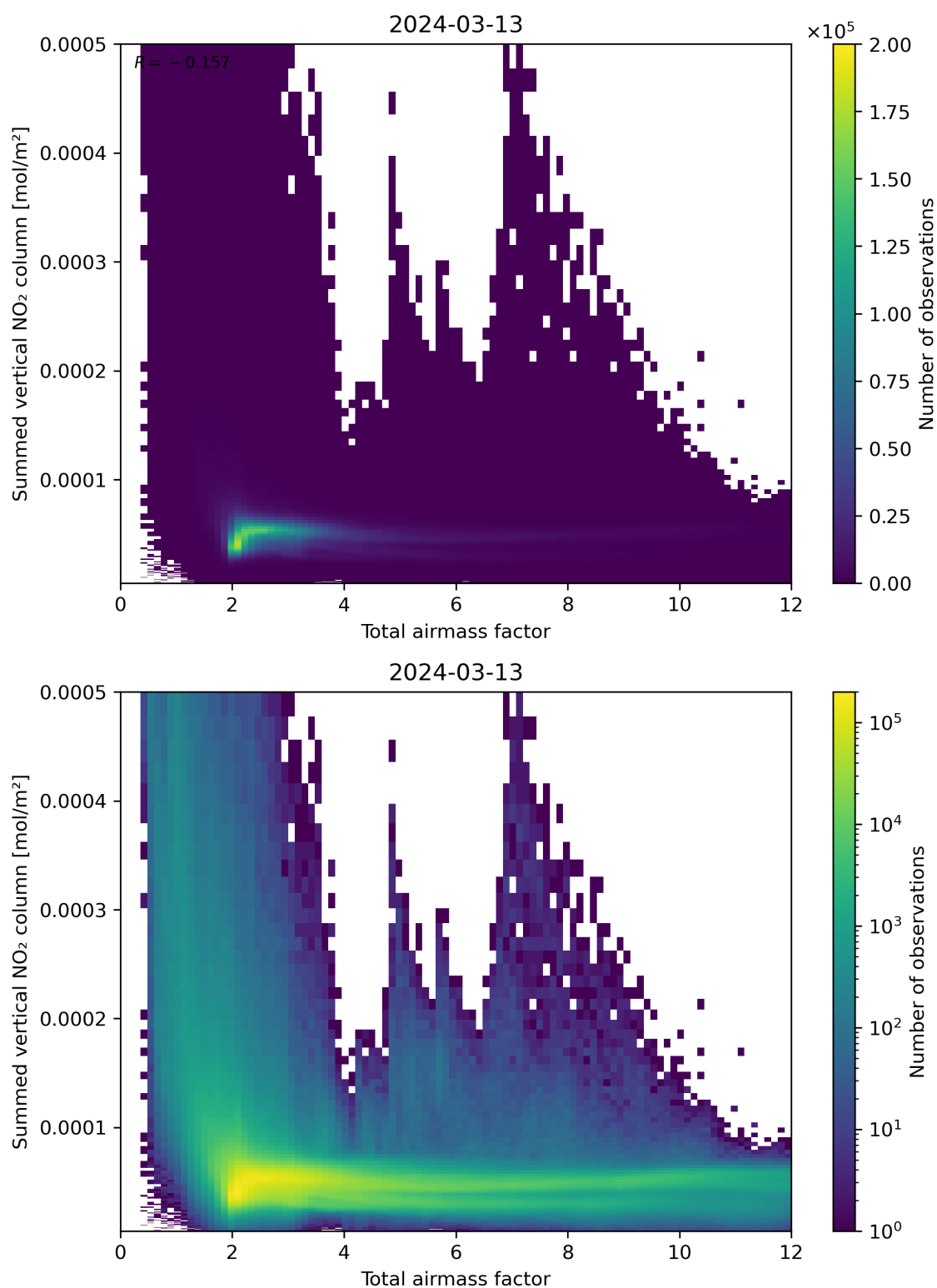
Figure 65: Scatter density plot of “Total airmass factor” against “Summed vertical NO 2 column” for 2024-03-12 to 2024-03-14.
