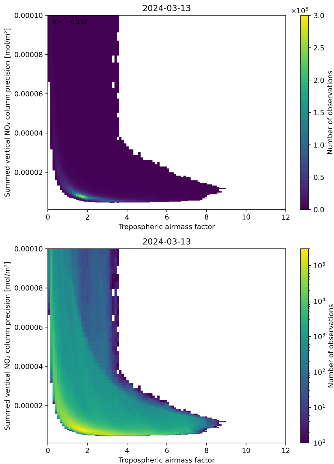
Figure 76: Scatter density plot of “Tropospheric air mass factor” against “Summed vertical NO 2 column precision” for 2024-03-12 to 2024-03-14.
