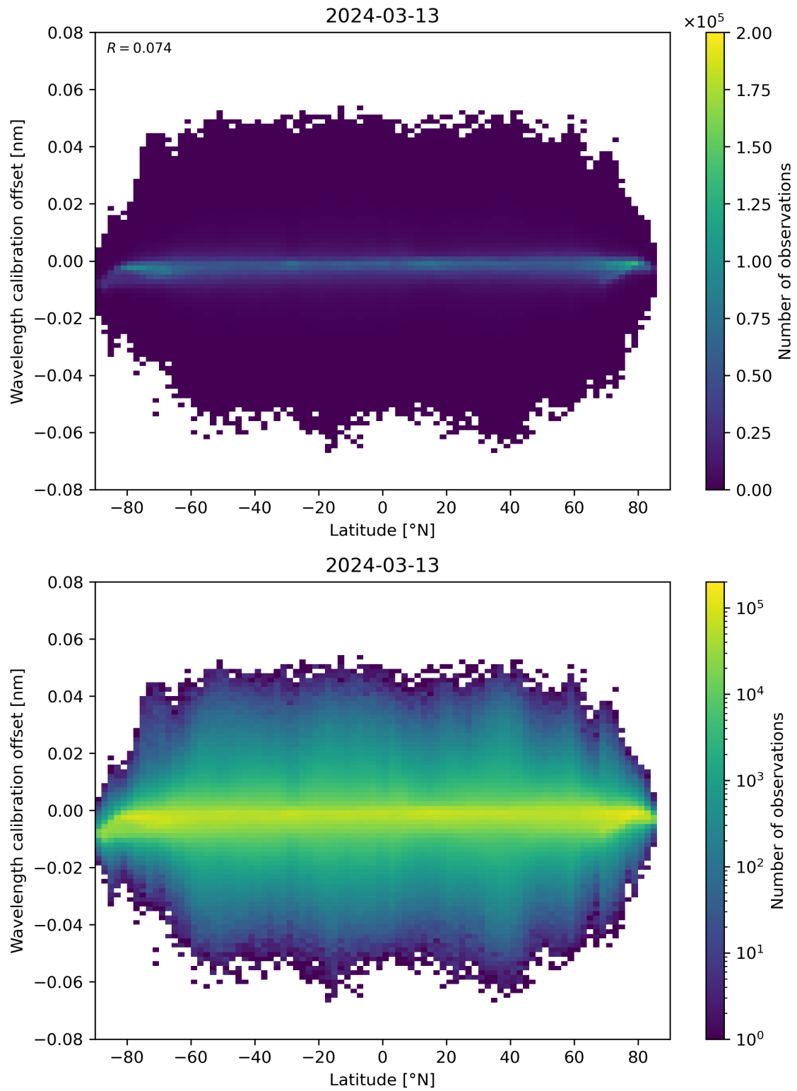
Figure 95: Scatter density plot of “Latitude” against “Wavelength calibration offset” for 2024-03-12 to 2024-03-14.
