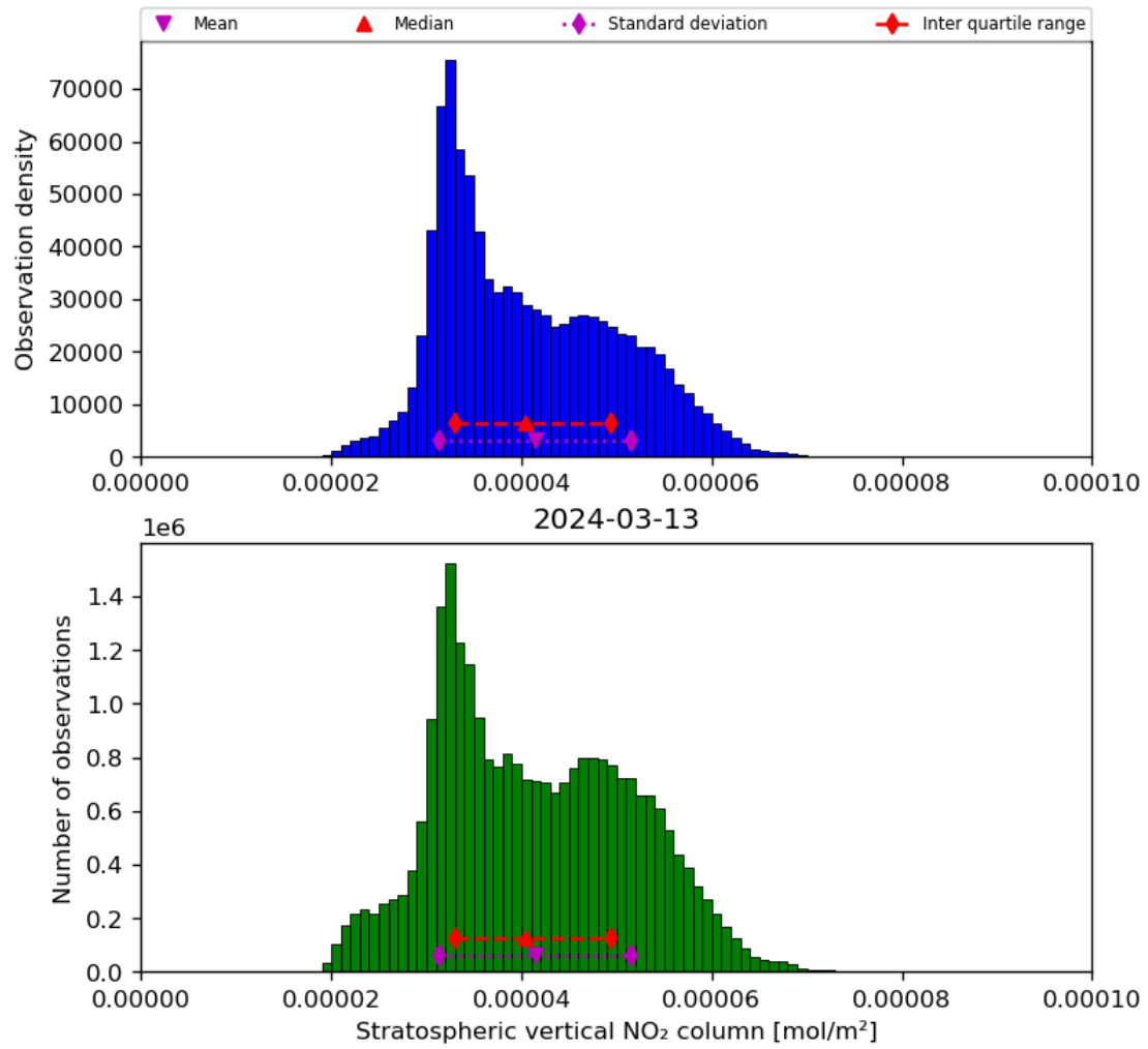
Figure 36: Histogram of “Stratospheric vertical NO 2 column” for 2024-03-12 to 2024-03-14
