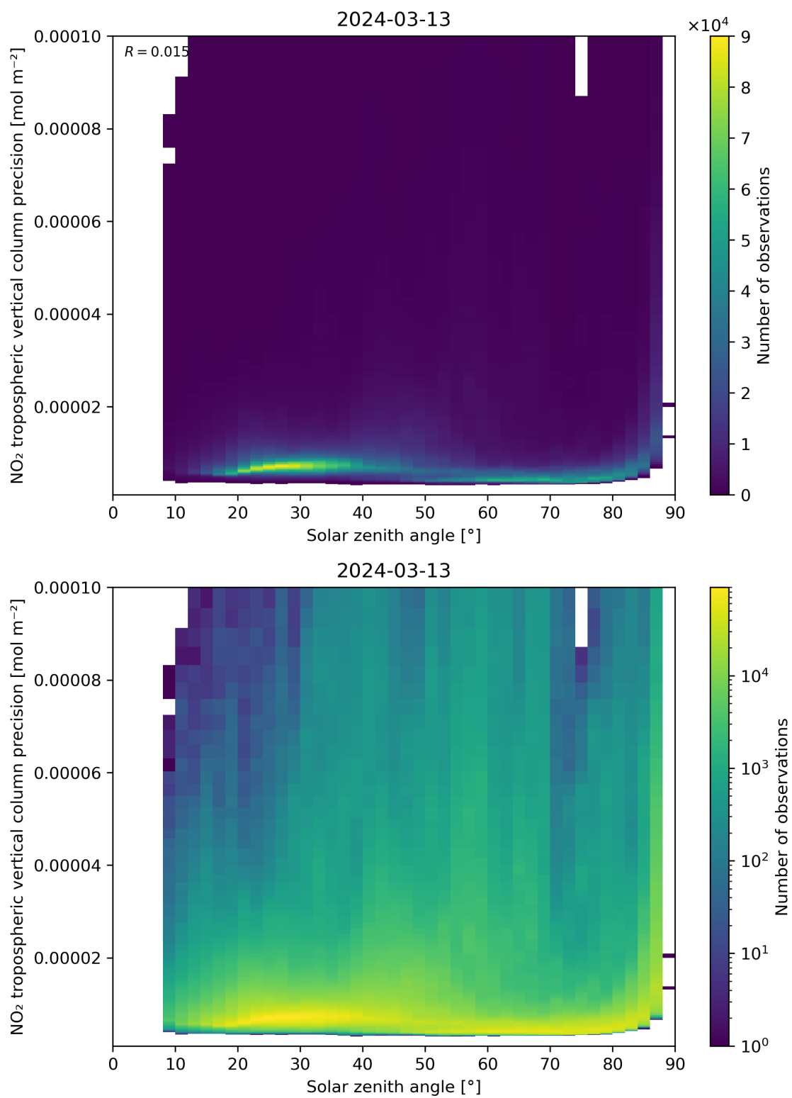
Figure 156: Scatter density plot of “Solar zenith angle” against “NO 2 tropospheric vertical column precision” for 2024-03-12 to 2024-03-14.
