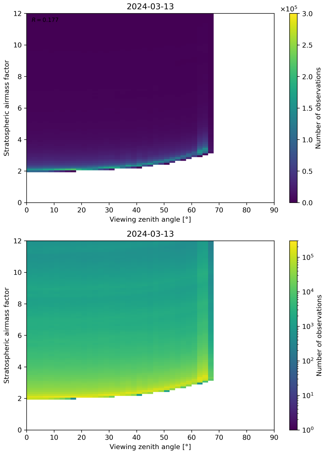
Figure 159: Scatter density plot of “Viewing zenith angle” against “Stratospheric airmass factor” for 2024-03-12 to 2024-03-14.
