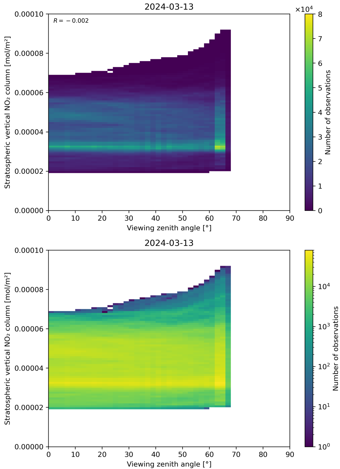
Figure 164: Scatter density plot of “Viewing zenith angle” against “Stratospheric vertical NO 2 column” for 2024-03-12 to 2024-03-14.
