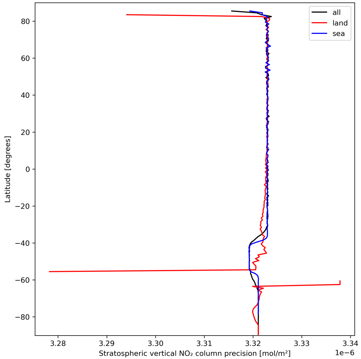
Figure 20: Zonal average of “Stratospheric vertical NO 2 column precision” for 2024-03-12 to 2024-03-14.
