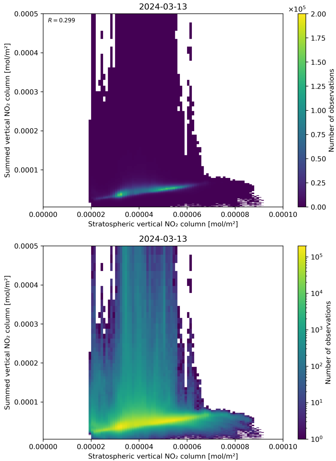
Figure 98: Scatter density plot of “Stratospheric vertical NO 2 column” against “Summed vertical NO 2 column” for 2024-03-12 to 2024-03-14.
