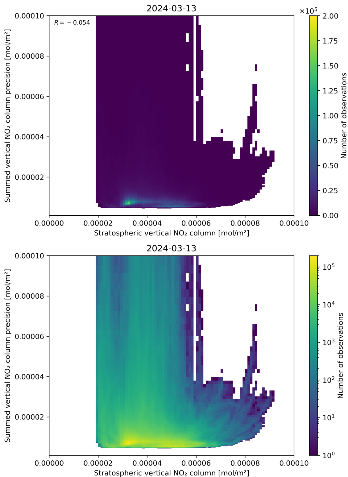
Figure 99: Scatter density plot of “Stratospheric vertical NO 2 column” against “Summed vertical NO 2 column precision” for 2024-03-12 to 2024-03-14.
