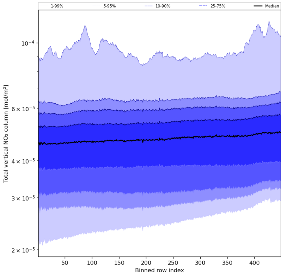
Figure 55: Along track statistics of “Total vertical NO 2 column” for 2024-03-12 to 2024-03-14
