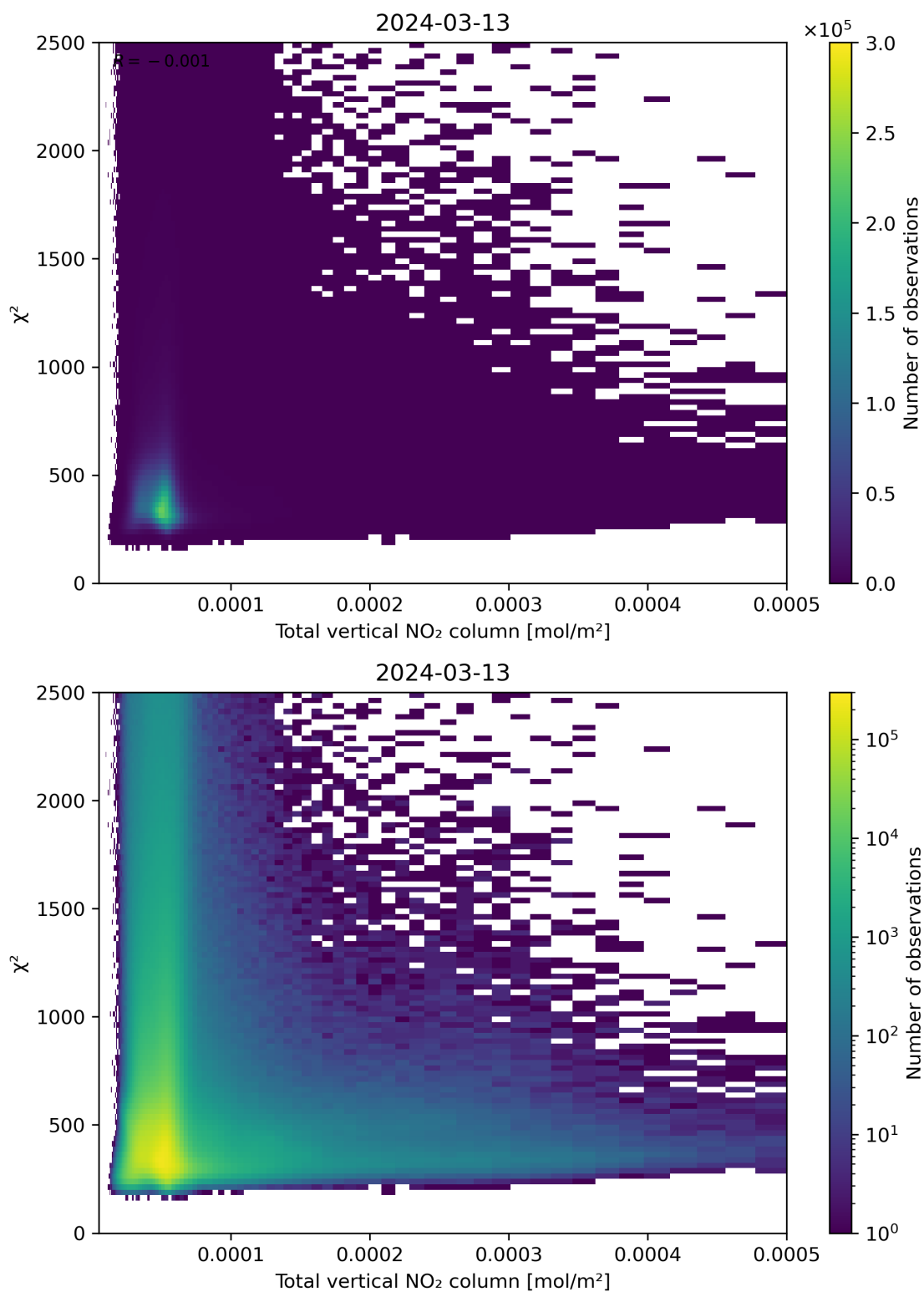
Figure 111: Scatter density plot of “Total vertical NO 2 column” against “ \chi^2 ” for 2024-03-12 to 2024-03-14.
