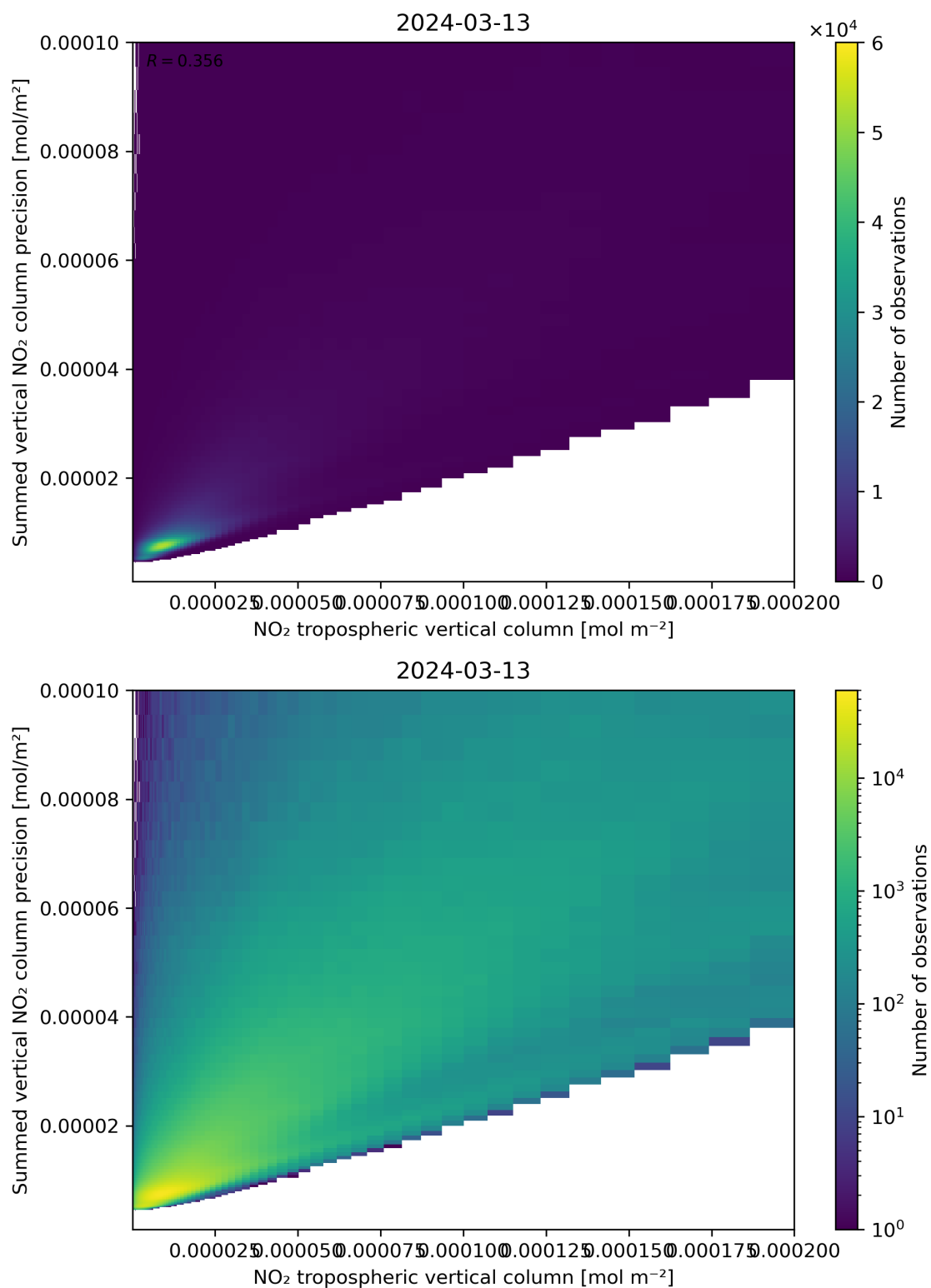
Figure 127: Scatter density plot of “NO 2 tropospheric vertical column” against “Summed vertical NO 2 column precision” for 2024-03-12 to 2024-03-14.
