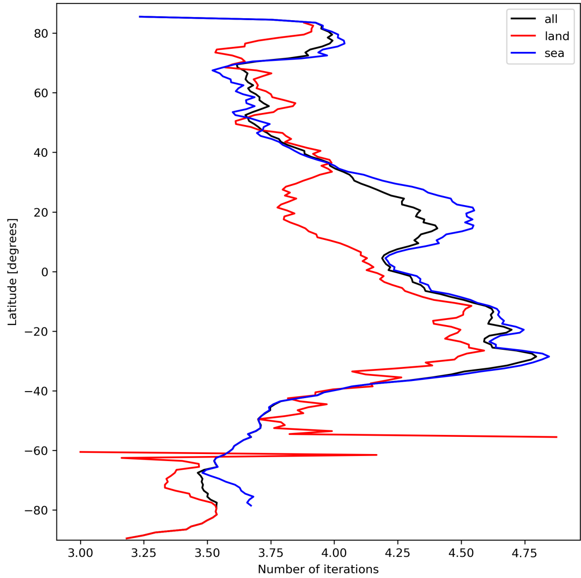
Figure 17: Zonal average of “Number of iterations” for 2024-03-12 to 2024-03-14.
