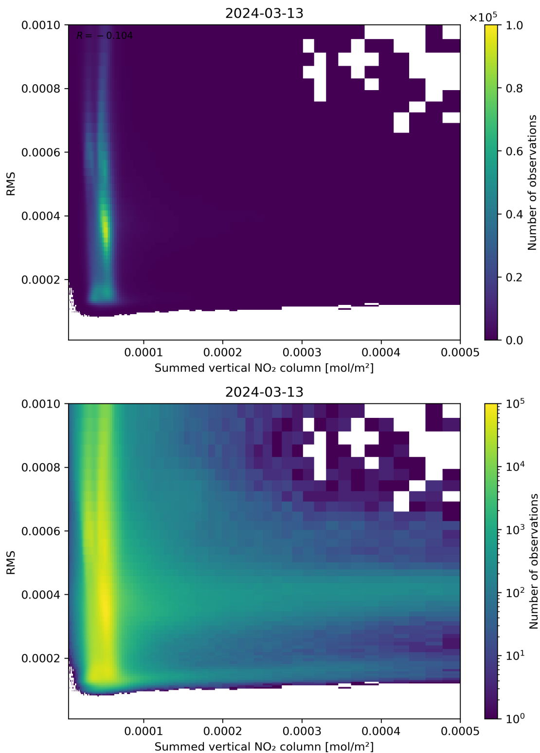
Figure 109: Scatter density plot of “Summed vertical NO 2 column” against “RMS” for 2024-03-12 to 2024-03-14.
