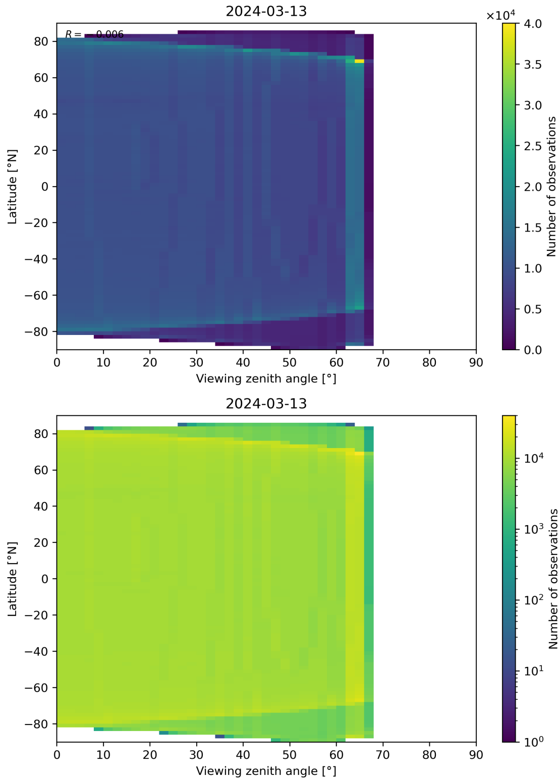
Figure 163: Scatter density plot of “Viewing zenith angle” against “Latitude” for 2024-03-12 to 2024-03-14.
