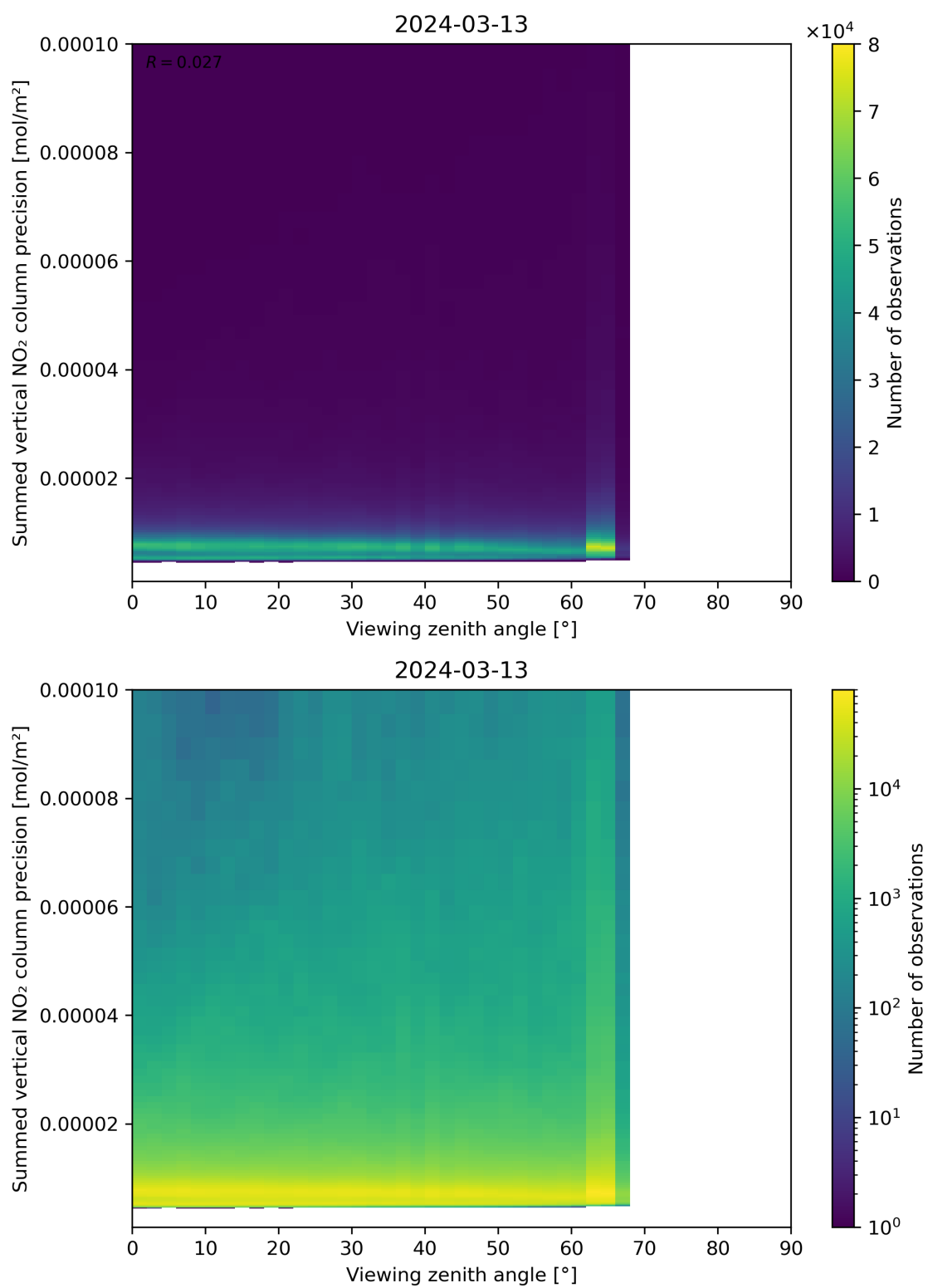
Figure 166: Scatter density plot of “Viewing zenith angle” against “Summed vertical NO 2 column precision” for 2024-03-12 to 2024-03-14.
