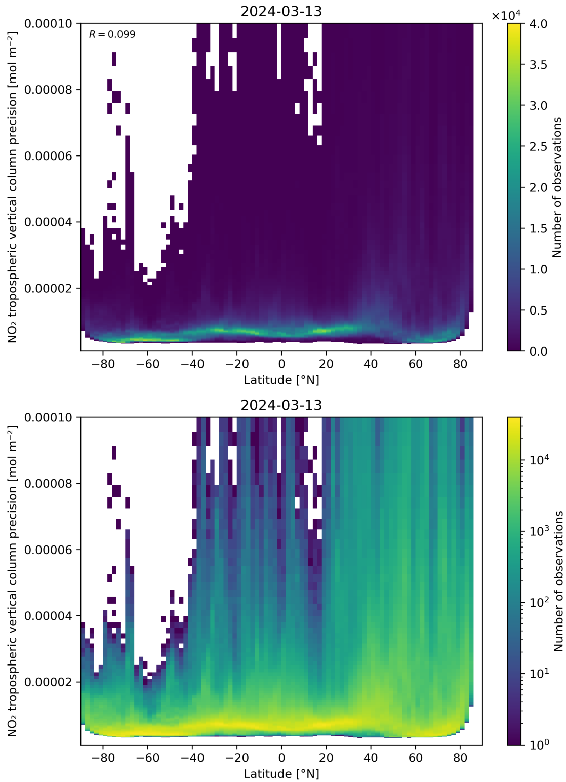
Figure 93: Scatter density plot of “Latitude” against “NO 2 tropospheric vertical column precision” for 2024-03-12 to 2024-03-14.
