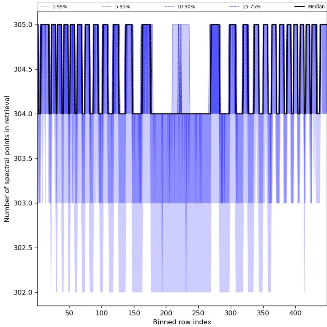
Figure 50: Along track statistics of “Number of spectral points in retrieval” for 2024-03-12 to 2024-03-14
