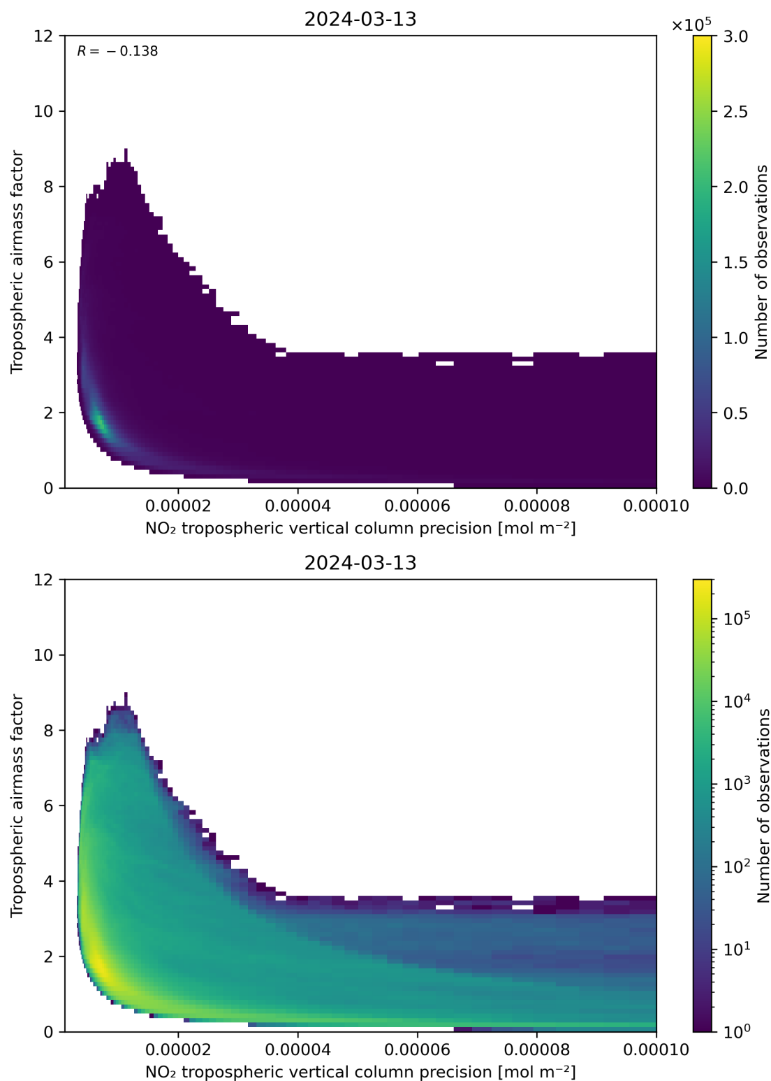
Figure 133: Scatter density plot of “NO 2 tropospheric vertical column precision” against “Tropospheric airmass factor” for 2024-03-12 to 2024-03-14.
