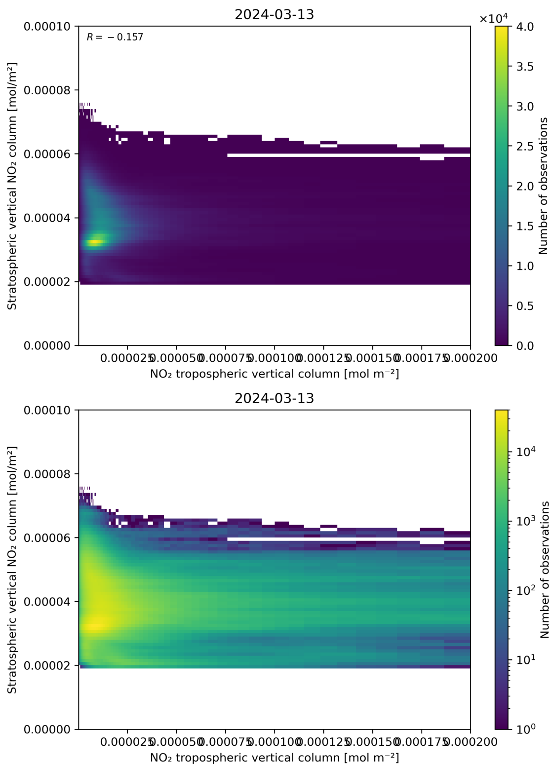
Figure 125: Scatter density plot of “NO 2 tropospheric vertical column” against “Stratospheric vertical NO 2 column” for 2024-03-12 to 2024-03-14.
