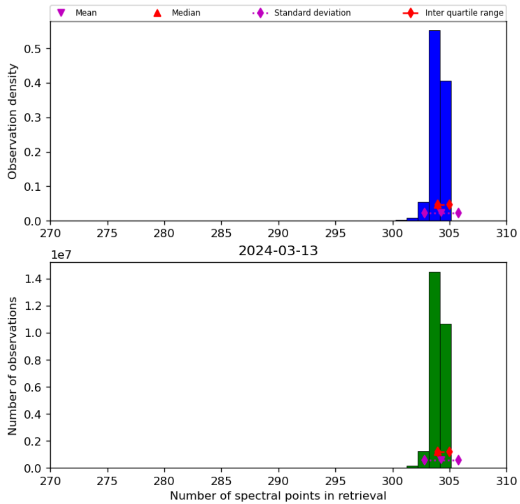
Figure 33: Histogram of “Number of spectral points in retrieval” for 2024-03-12 to 2024-03-14
