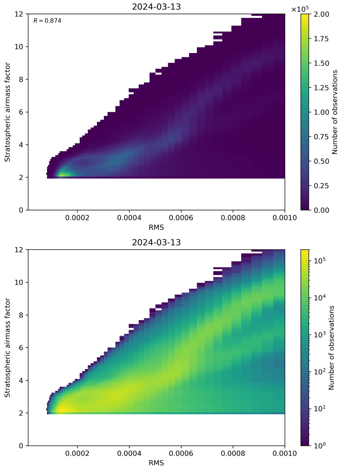
Figure 144: Scatter density plot of “RMS” against “Stratospheric airmass factor” for 2024-03-12 to 2024-03-14.
