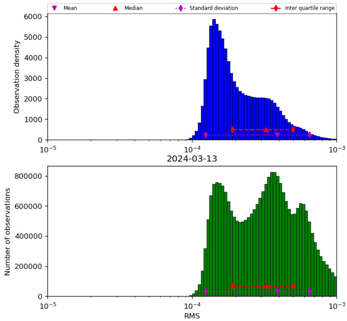
Figure 43: Histogram of “RMS” for 2024-03-12 to 2024-03-14
