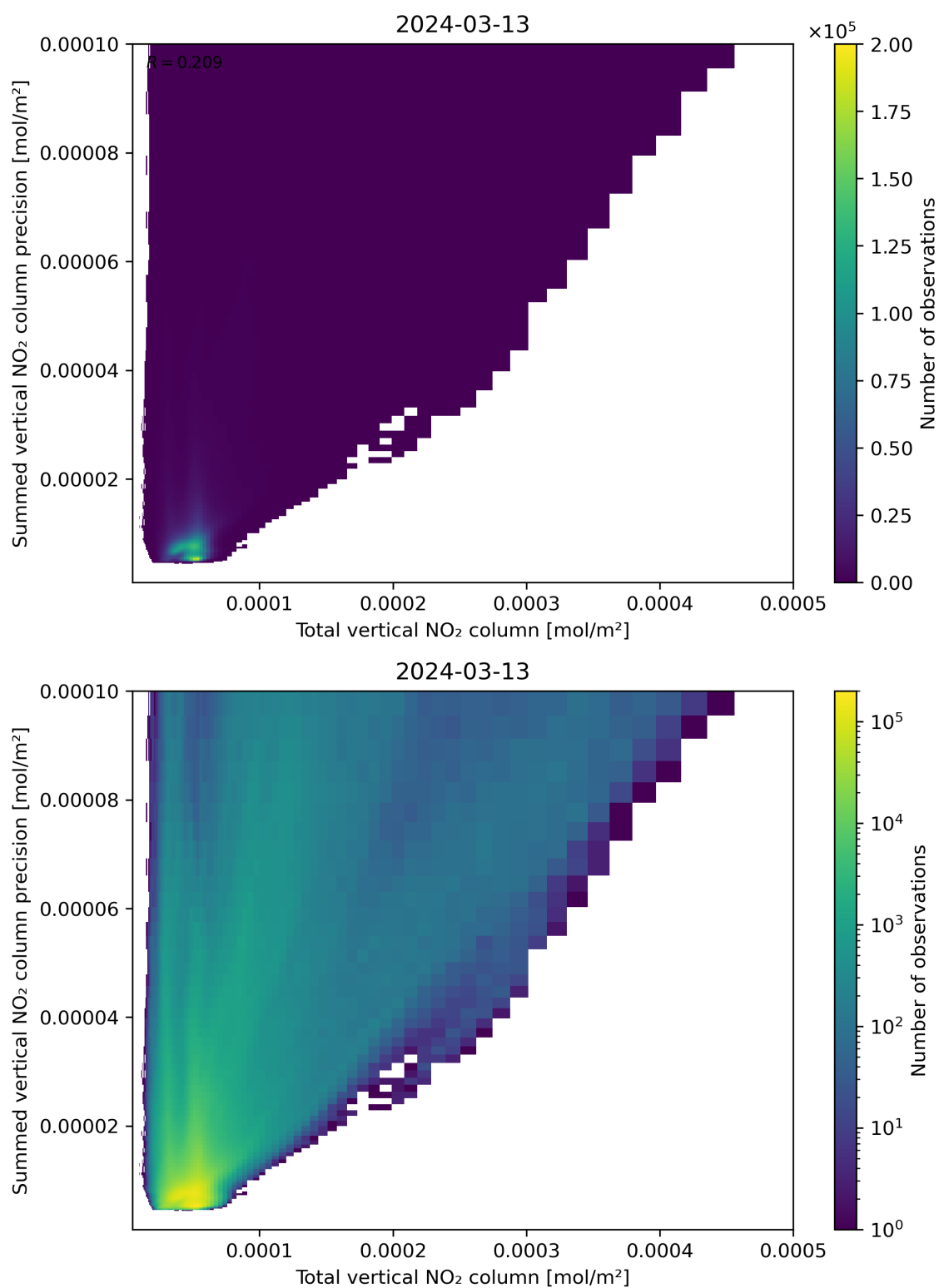
Figure 113: Scatter density plot of “Total vertical NO 2 column” against “Summed vertical NO 2 column precision” for 2024-03-12 to 2024-03-14.
