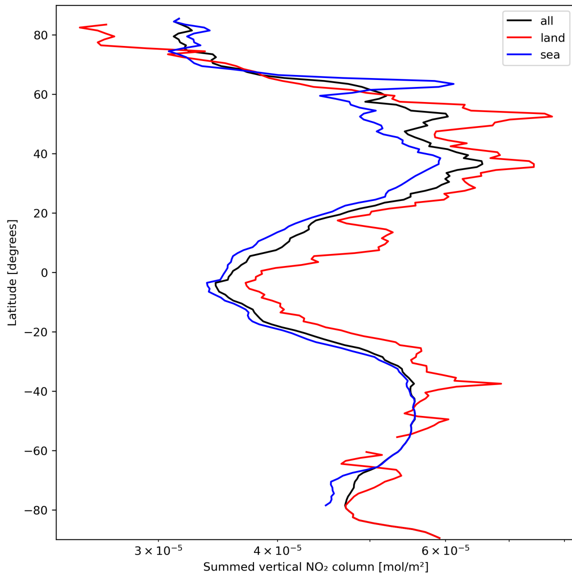
Figure 23: Zonal average of “Summed vertical NO 2 column” for 2024-03-12 to 2024-03-14.
