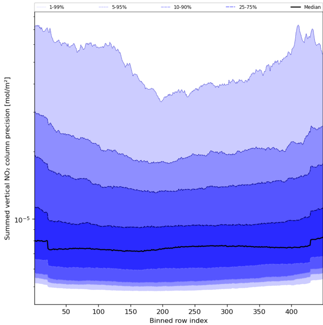
Figure 58: Along track statistics of “Summed vertical NO 2 column precision” for 2024-03-12 to 2024-03-14
