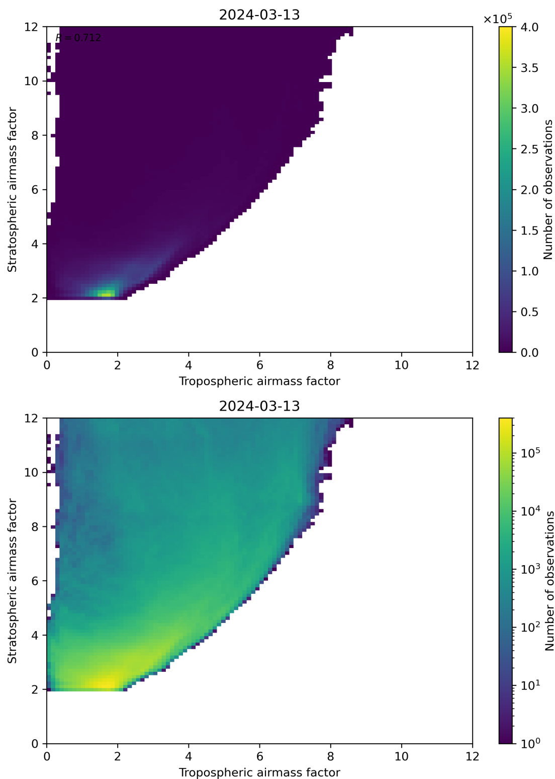
Figure 71: Scatter density plot of “Tropospheric airmass factor” against “Stratospheric airmass factor” for 2024-03-12 to 2024-03-14.
