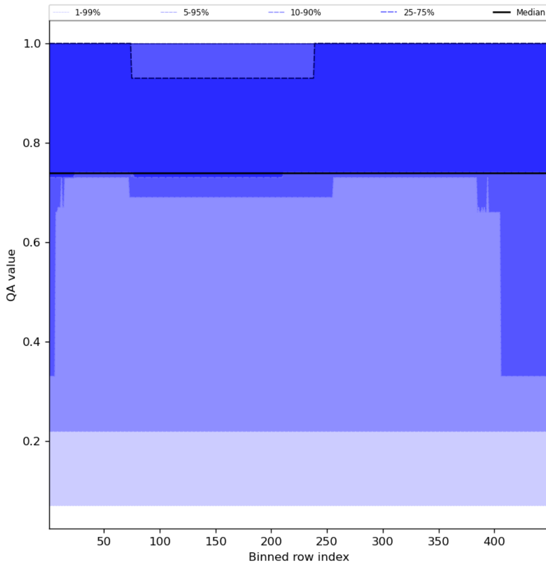
Figure 45: Along track statistics of “QA value” for 2024-03-12 to 2024-03-14
