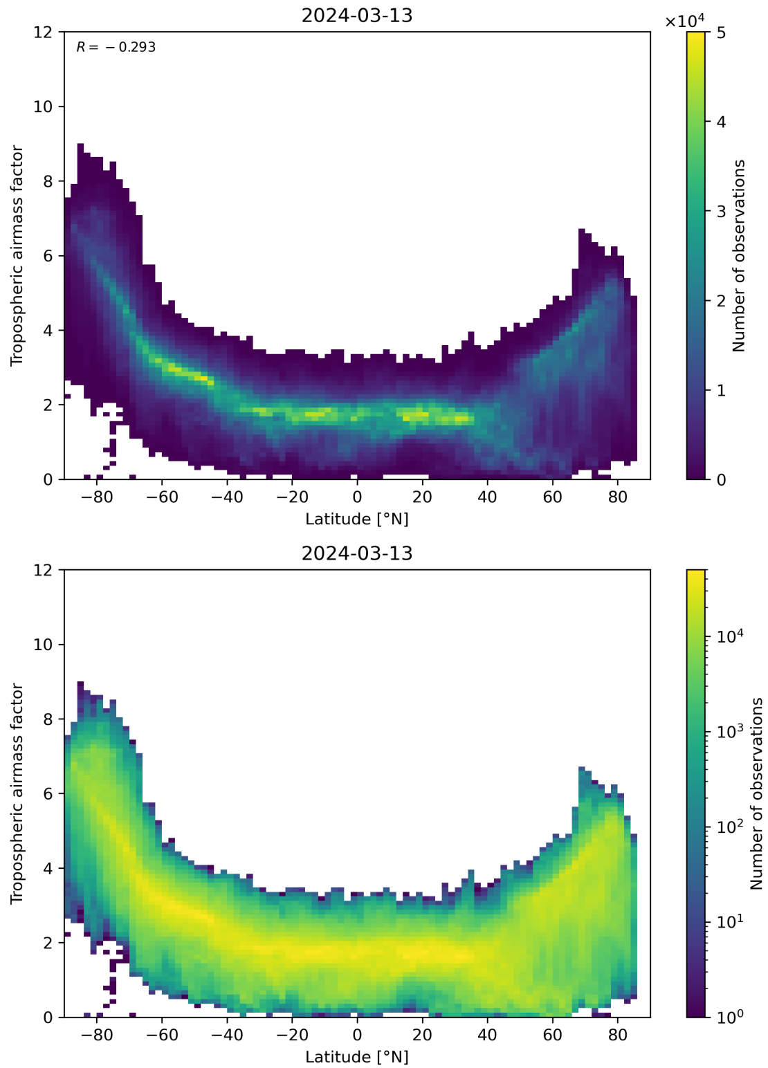
Figure 85: Scatter density plot of “Latitude” against “Tropospheric airmass factor” for 2024-03-12 to 2024-03-14.
