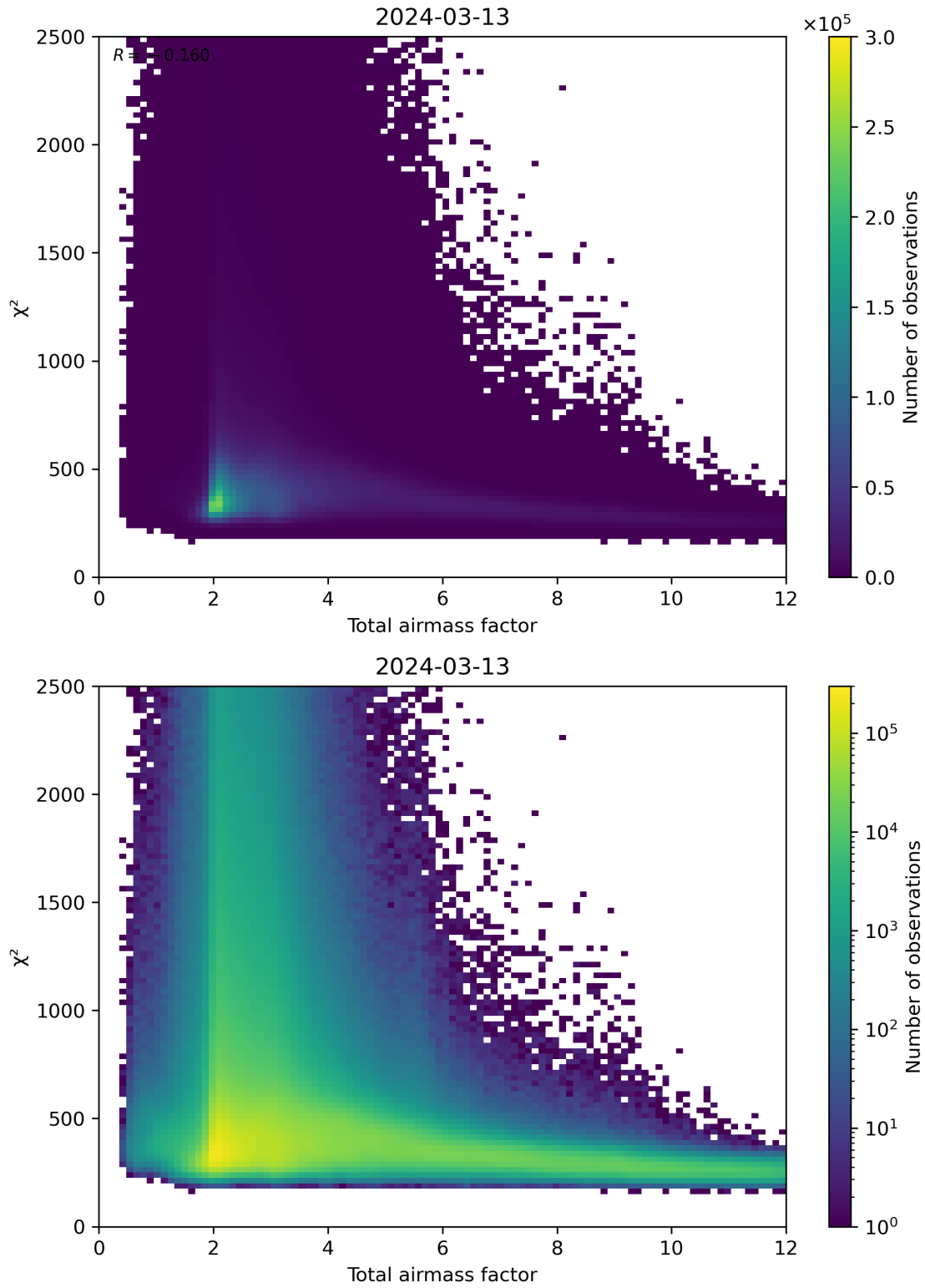
Figure 63: Scatter density plot of “Total airmass factor” against “ \chi^2 ” for 2024-03-12 to 2024-03-14.
