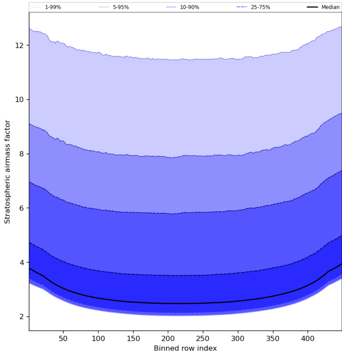
Figure 61: Along track statistics of “Stratospheric airmass factor” for 2024-03-12 to 2024-03-14
