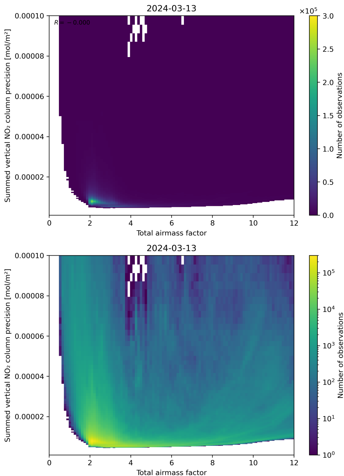
Figure 66: Scatter density plot of “Total airmass factor” against “Summed vertical NO 2 column precision” for 2024-03-12 to 2024-03-14.
