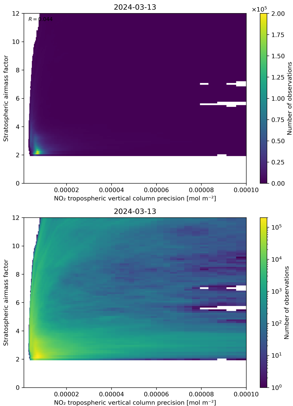
Figure 131: Scatter density plot of “NO 2 tropospheric vertical column precision” against “Stratospheric airmass factor” for 2024-03-12 to 2024-03-14.
