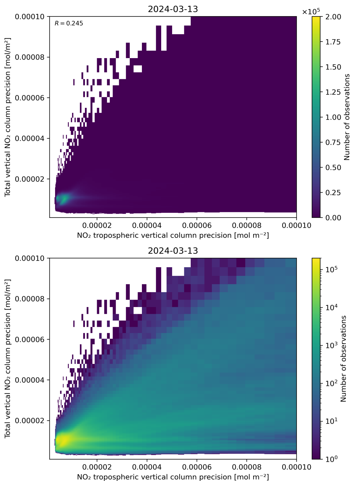
Figure 139: Scatter density plot of “NO 2 tropospheric vertical column precision” against “Total vertical NO 2 column precision” for 2024-03-12 to 2024-03-14.
