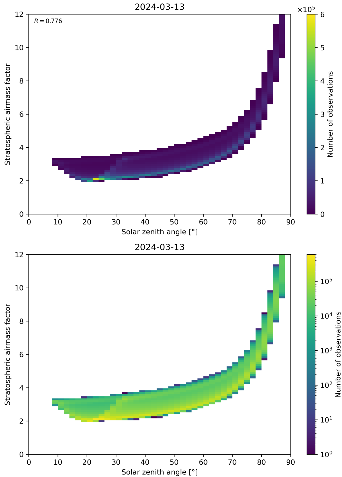
Figure 145: Scatter density plot of “Solar zenith angle” against “Stratospheric airmass factor” for 2024-03-12 to 2024-03-14.
