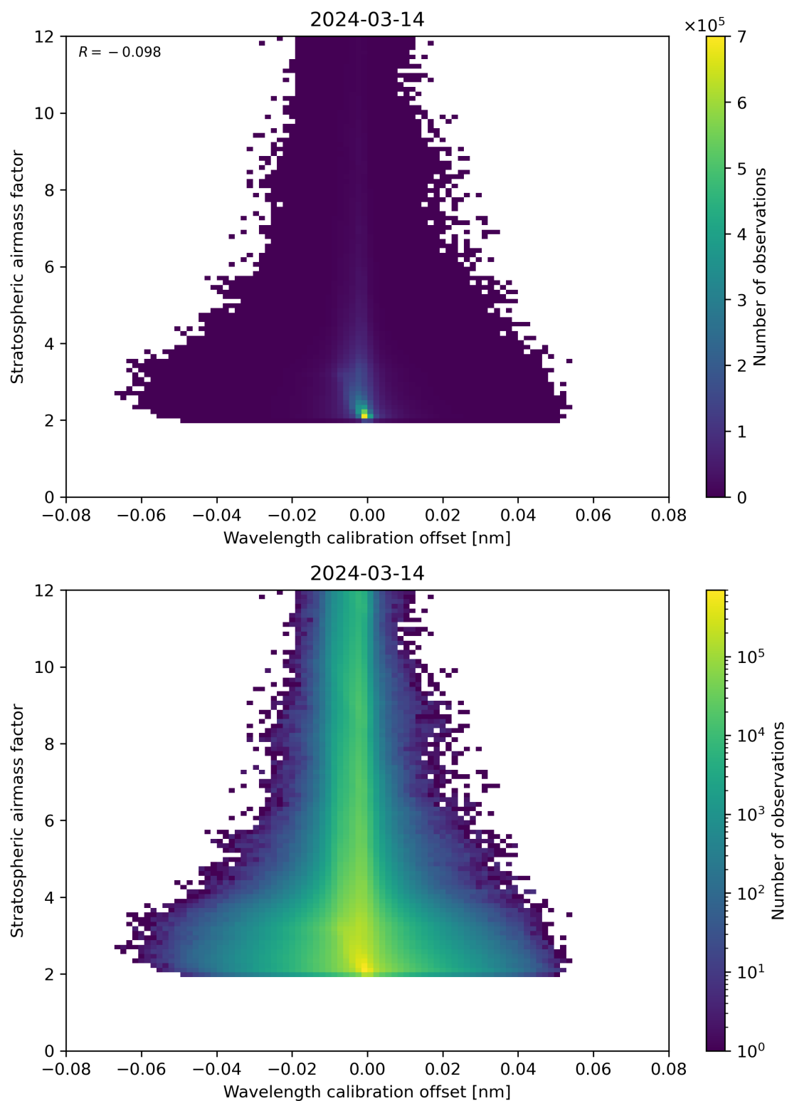
Figure 174: Scatter density plot of “Wavelength calibration offset” against “Stratospheric air mass factor” for 2024-03-14 to 2024-03-15.
