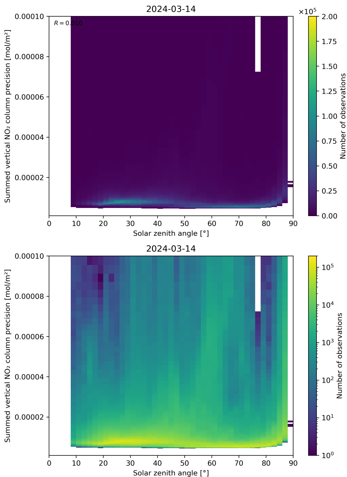
Figure 152: Scatter density plot of “Solar zenith angle” against “Summed vertical NO 2 column precision” for 2024-03-14 to 2024-03-15.
