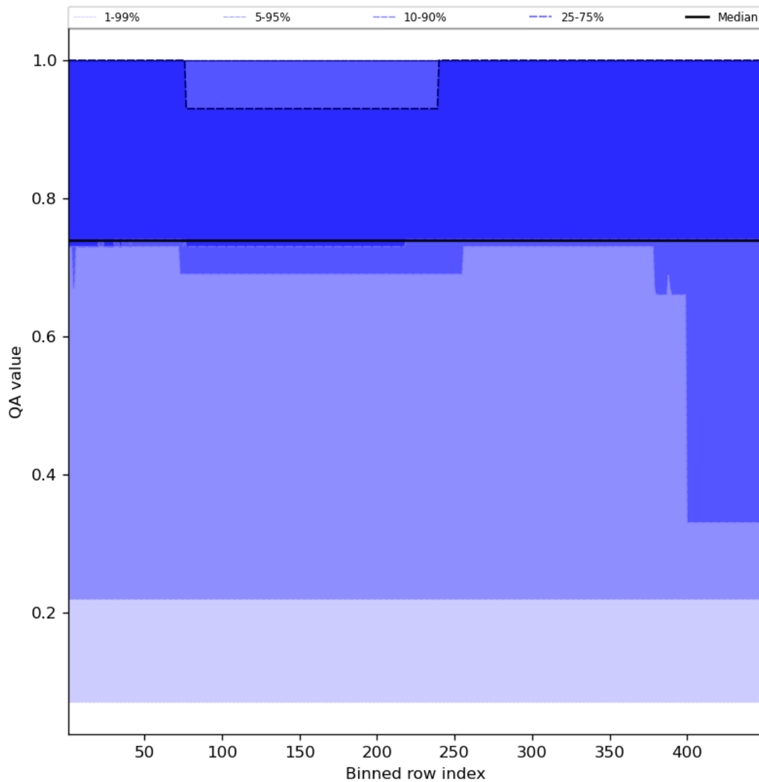
Figure 45: Along track statistics of “QA value” for 2024-03-14 to 2024-03-15
