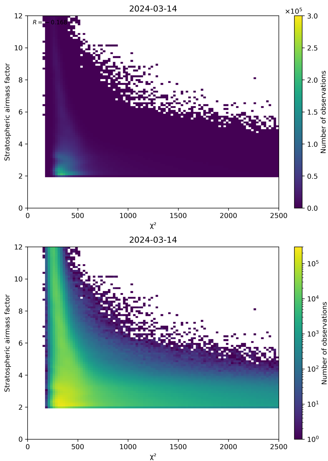
Figure 81: Scatter density plot of “ \chi^2 ” against “Stratospheric airmass factor” for 2024-03-14 to 2024-03-15.
