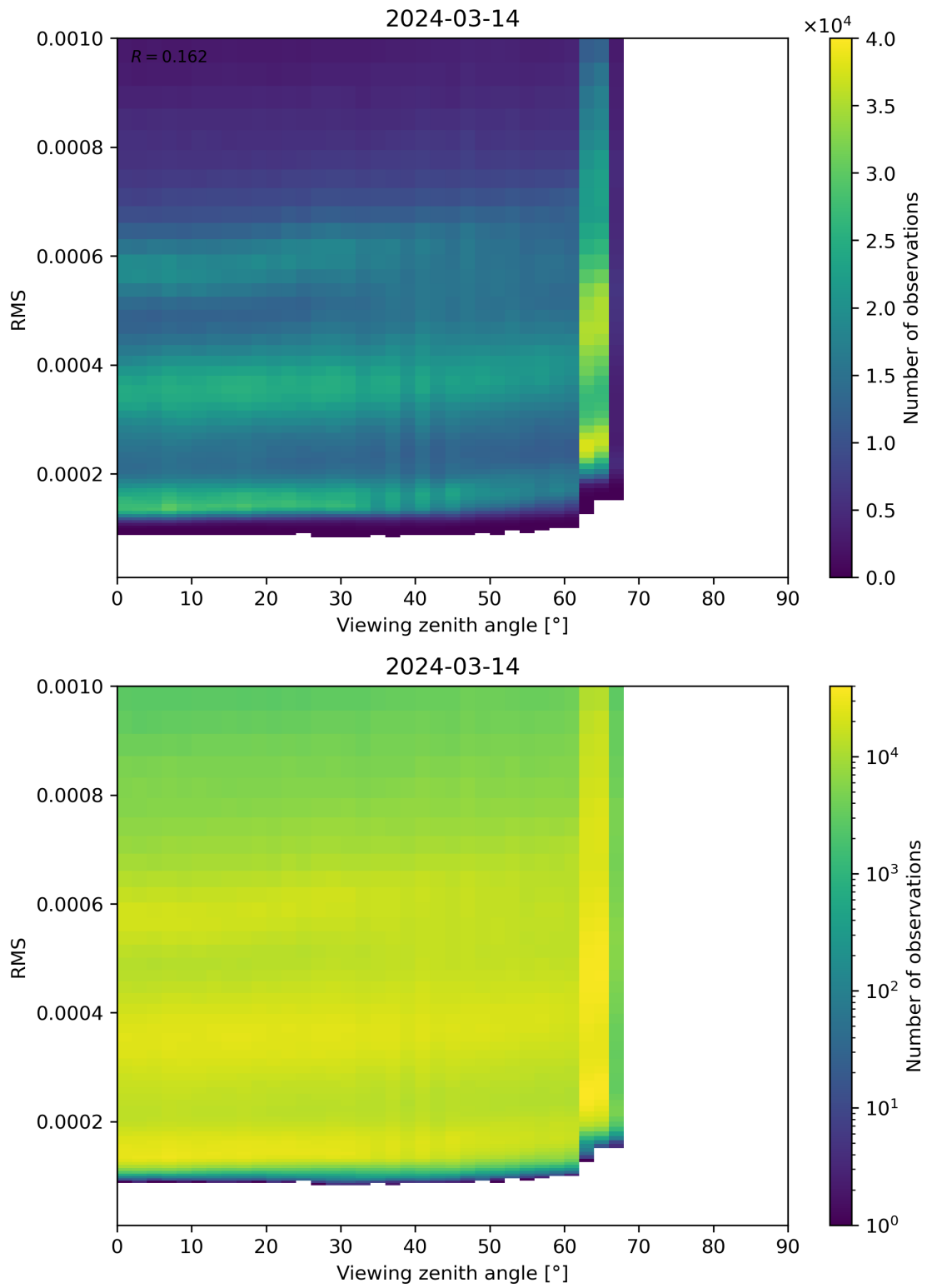
Figure 171: Scatter density plot of “Viewing zenith angle” against “RMS” for 2024-03-14 to 2024-03-15.
