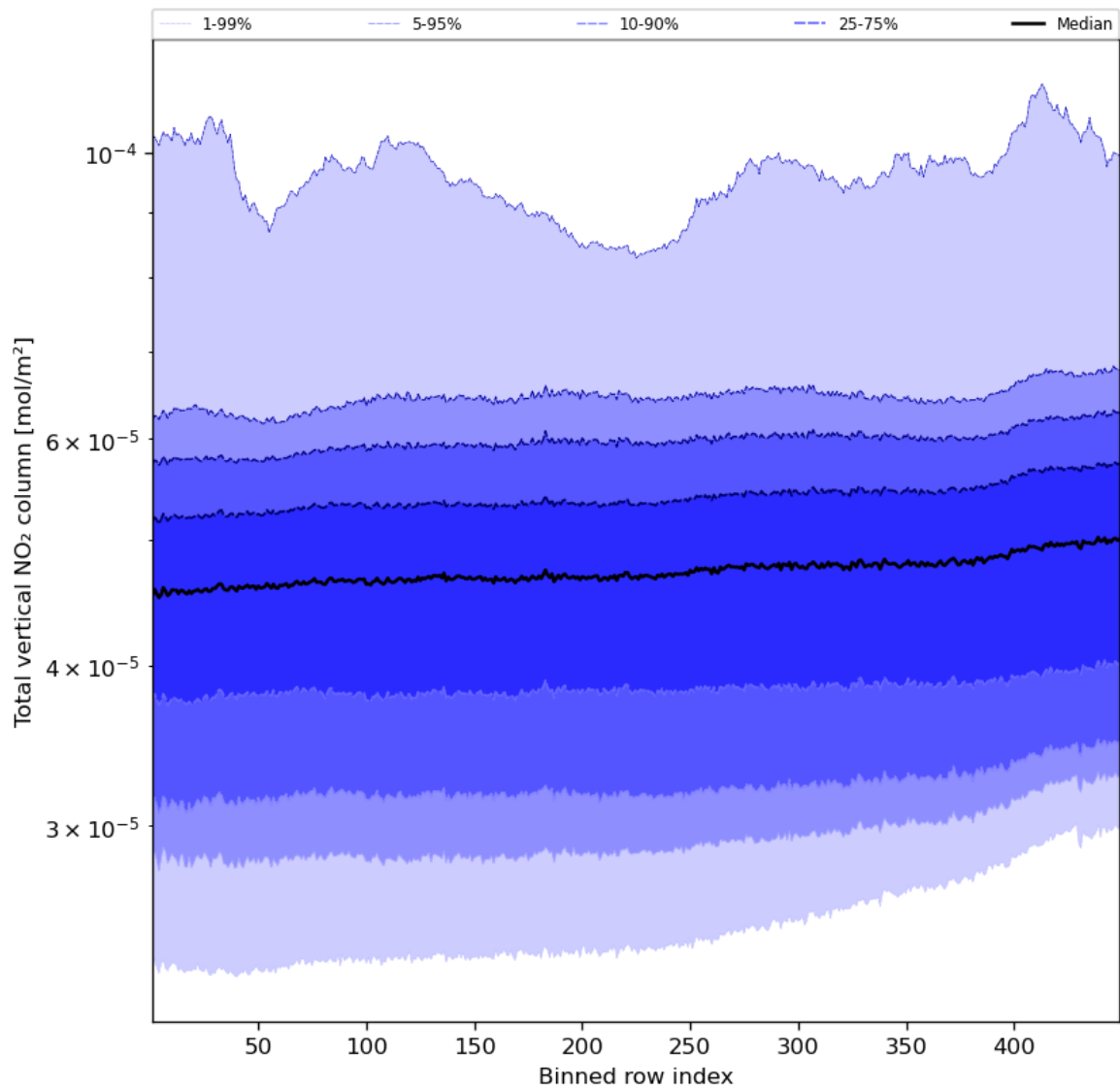
Figure 55: Along track statistics of “Total vertical NO 2 column” for 2024-03-14 to 2024-03-15
