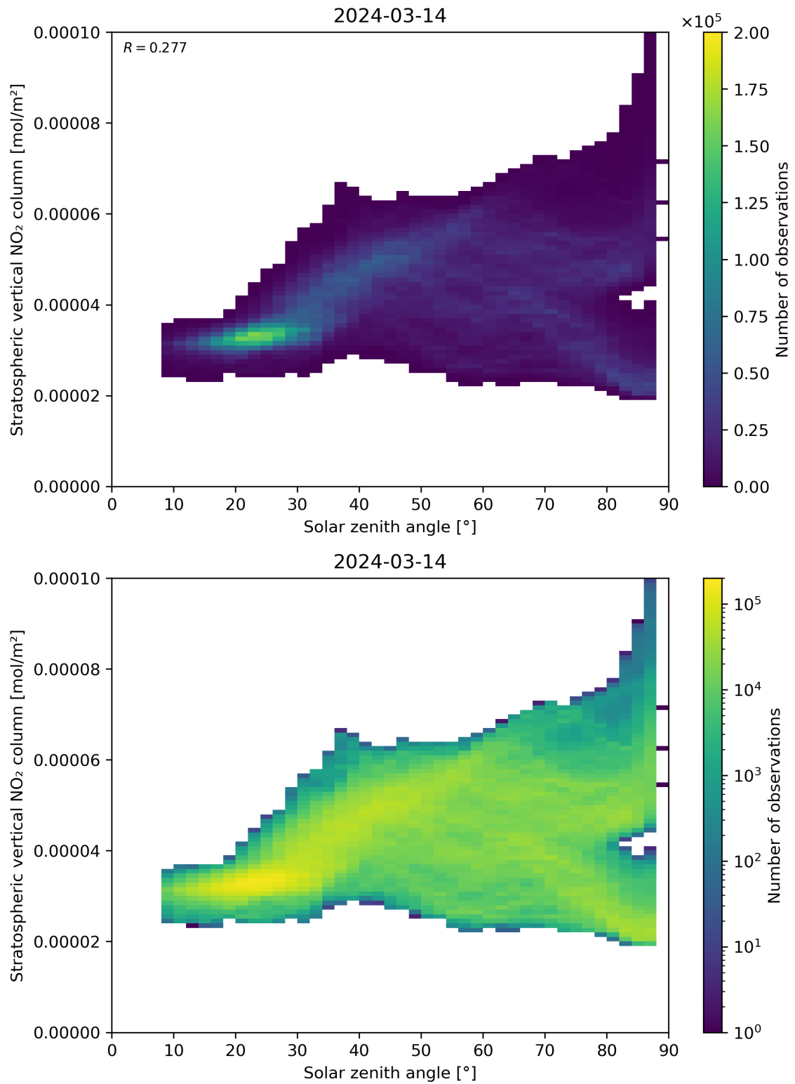
Figure 150: Scatter density plot of “Solar zenith angle” against “Stratospheric vertical \text{NO}_2 column” for 2024-03-14 to 2024-03-15.
