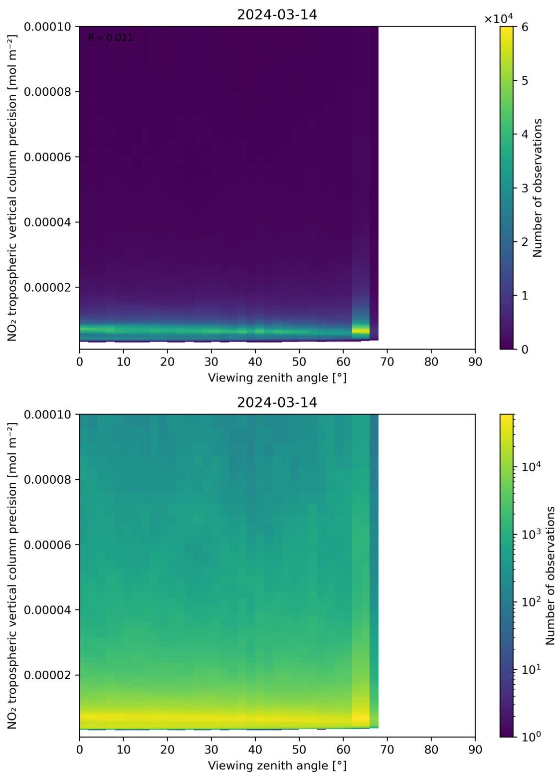
Figure 170: Scatter density plot of “Viewing zenith angle” against “NO 2 tropospheric vertical column precision” for 2024-03-14 to 2024-03-15.
