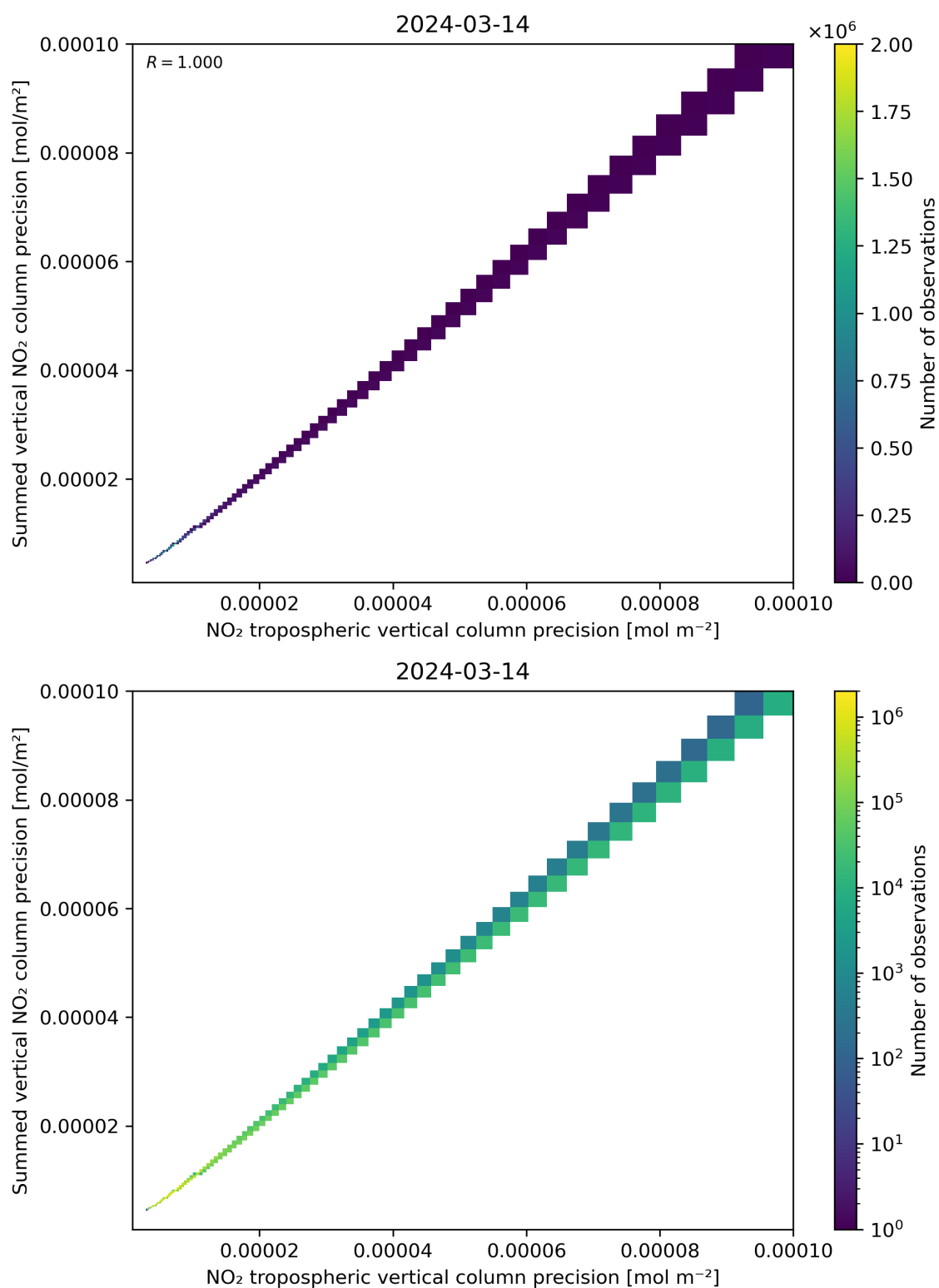
Figure 137: Scatter density plot of “NO 2 tropospheric vertical column precision” against “Summed vertical NO 2 column precision” for 2024-03-14 to 2024-03-15.
