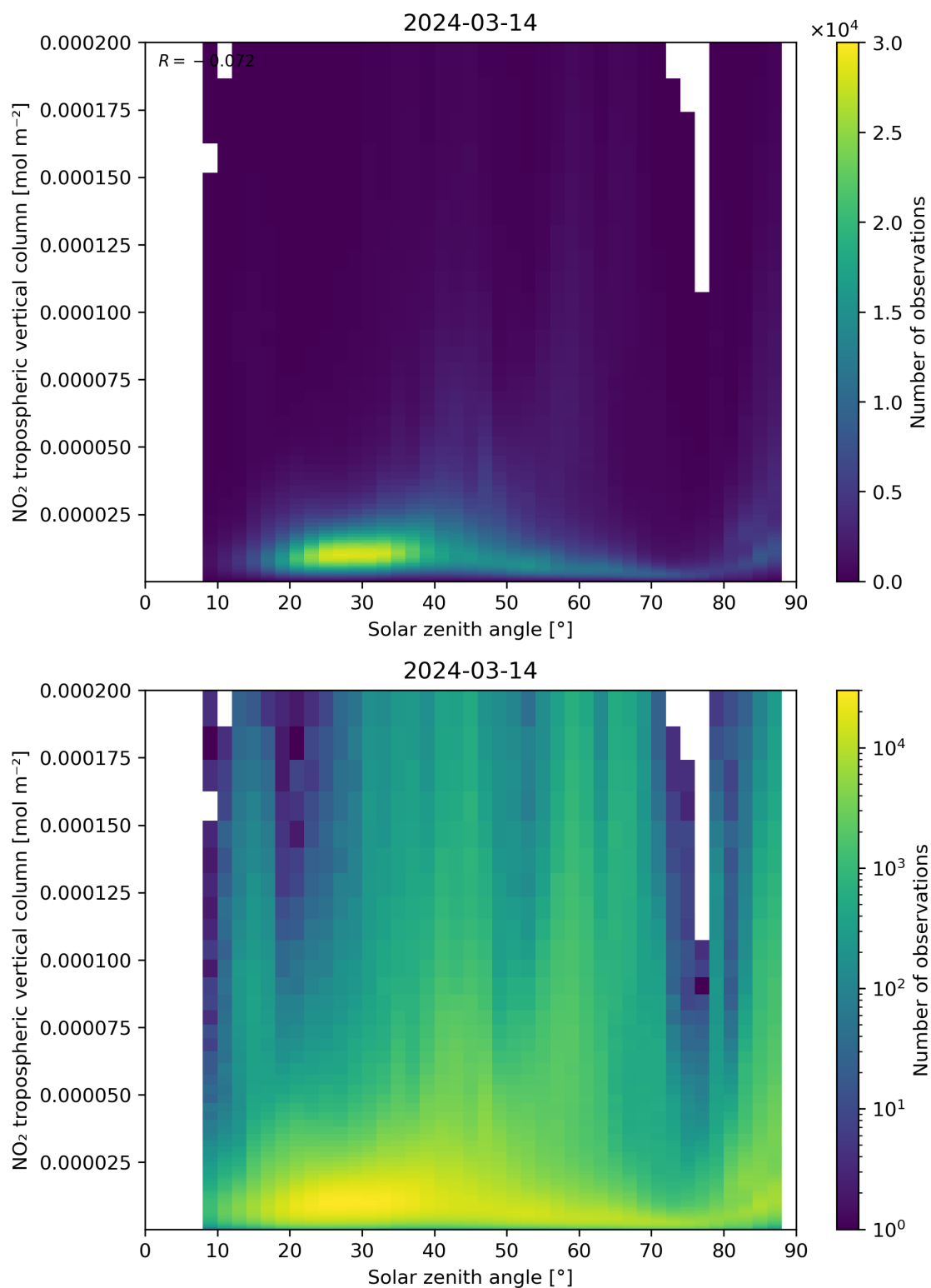
Figure 155: Scatter density plot of “Solar zenith angle” against “NO 2 tropospheric vertical column” for 2024-03-14 to 2024-03-15.
