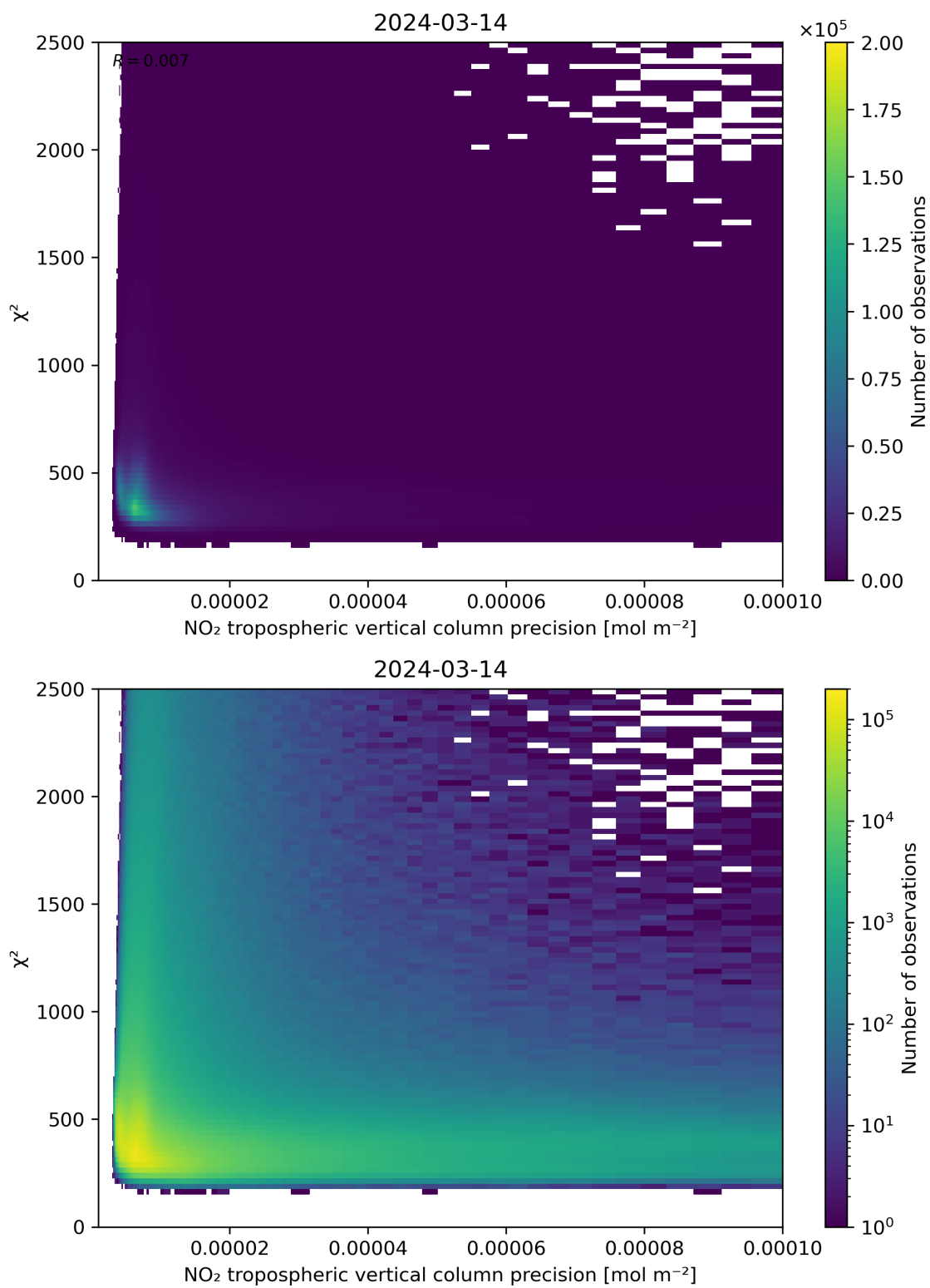
Figure 134: Scatter density plot of “NO 2 tropospheric vertical column precision” against “ \chi^2 ” for 2024-03-14 to 2024-03-15.
