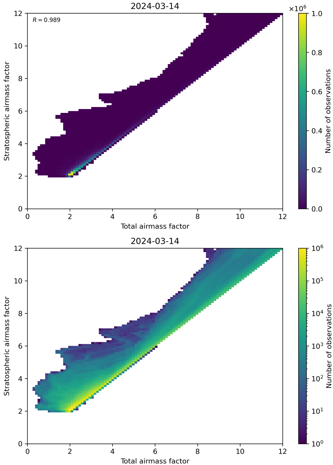
Figure 62: Scatter density plot of “Total airmass factor” against “Stratospheric airmass factor” for 2024-03-14 to 2024-03-15.
