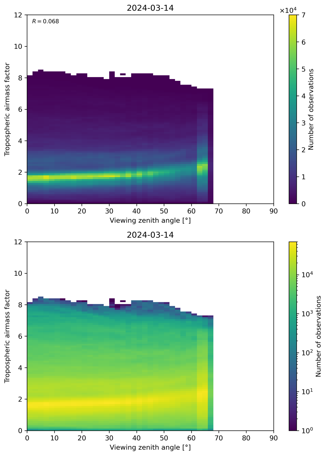
Figure 161: Scatter density plot of “Viewing zenith angle” against “Tropospheric airmass factor” for 2024-03-14 to 2024-03-15.
