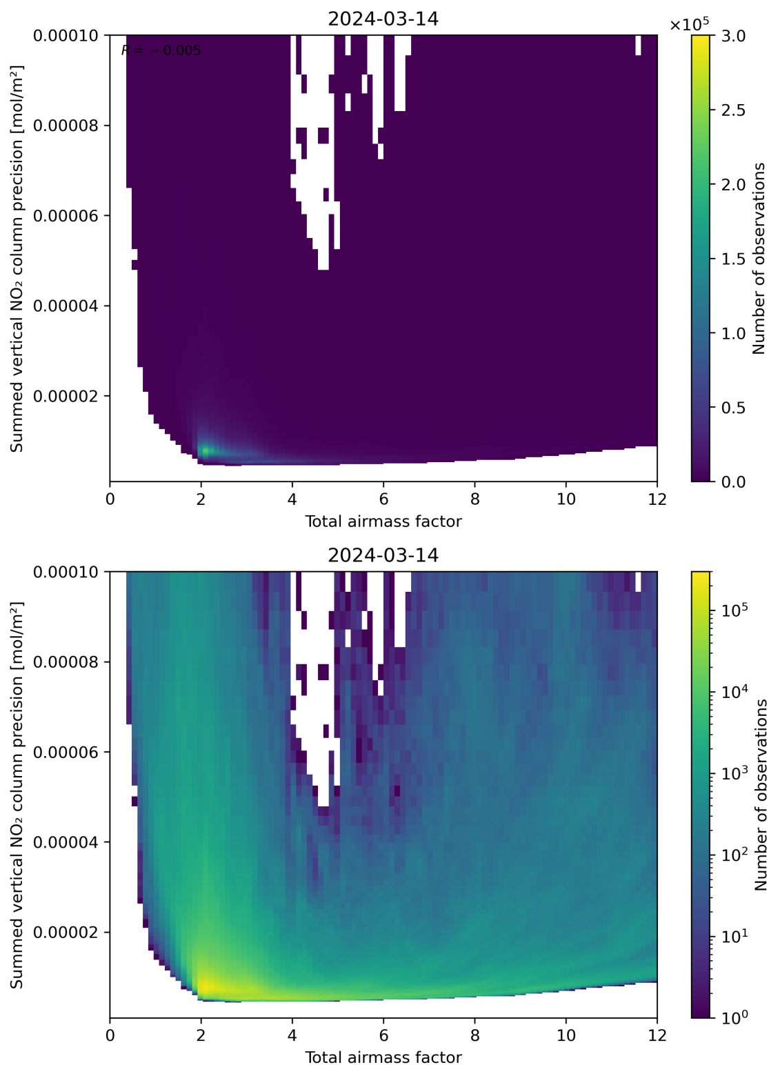
Figure 66: Scatter density plot of “Total airmass factor” against “Summed vertical NO 2 column precision” for 2024-03-14 to 2024-03-15.
