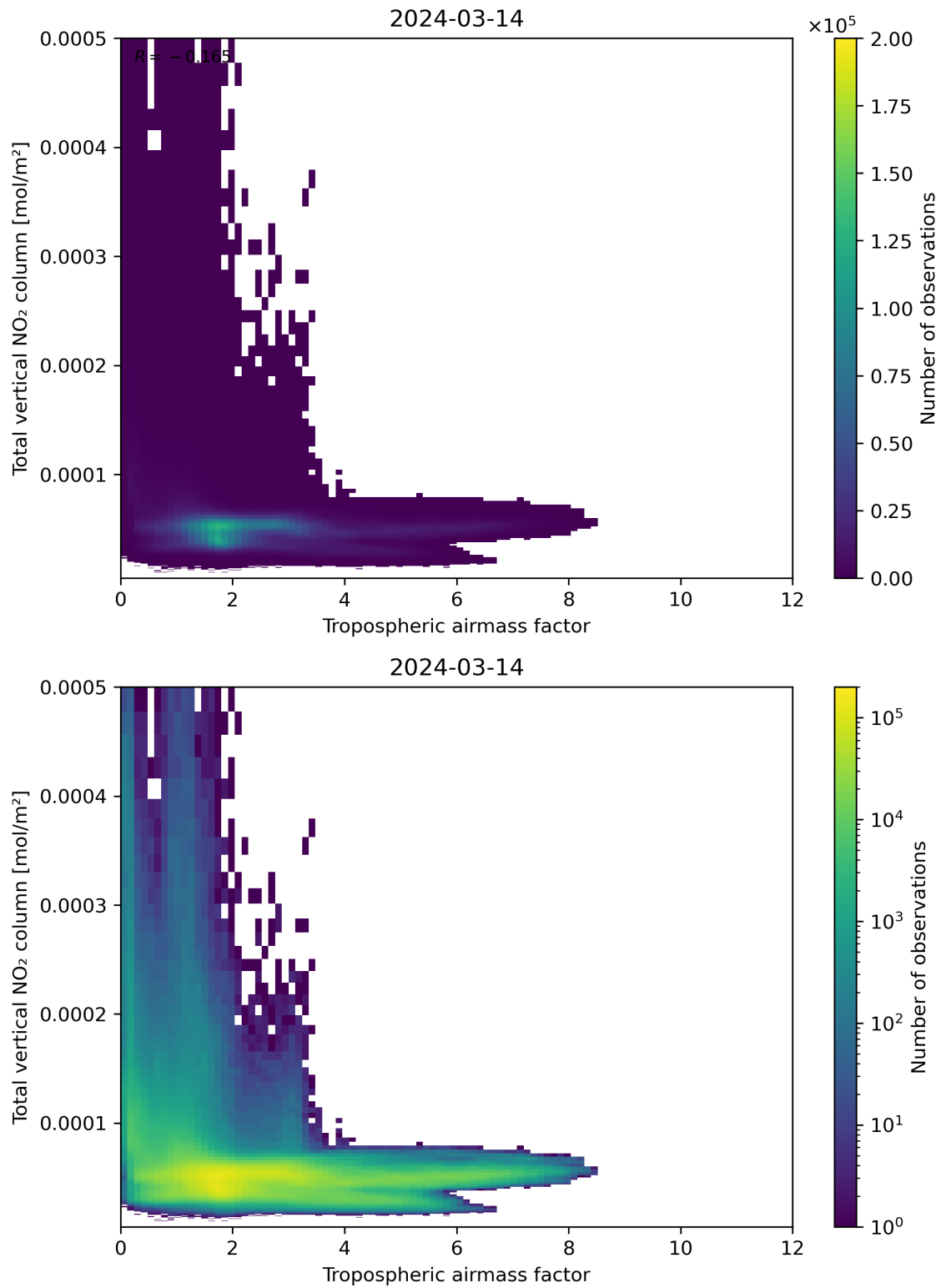
Figure 77: Scatter density plot of “Tropospheric airmass factor” against “Total vertical NO 2 column” for 2024-03-14 to 2024-03-15.
