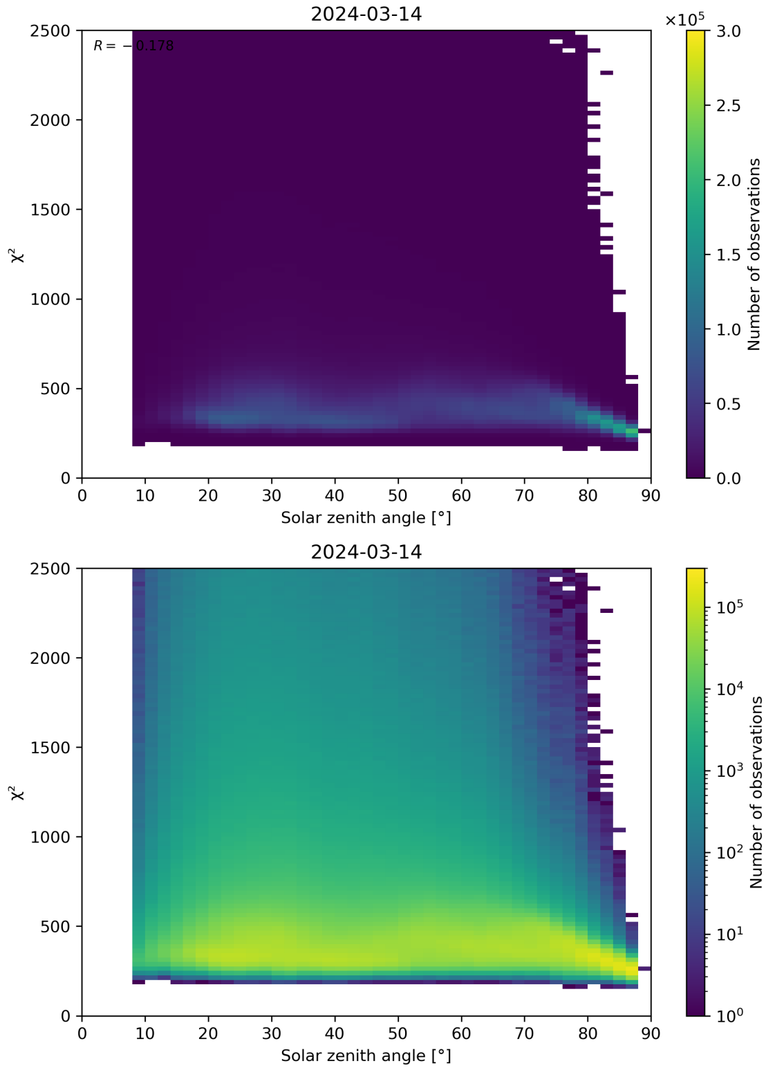
Figure 148: Scatter density plot of “Solar zenith angle” against “ \chi^2 ” for 2024-03-14 to 2024-03-15.
