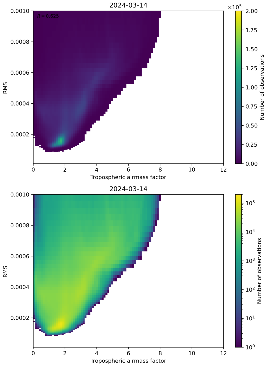
Figure 79: Scatter density plot of “Tropospheric airmass factor” against “RMS” for 2024-03-14 to 2024-03-15.
