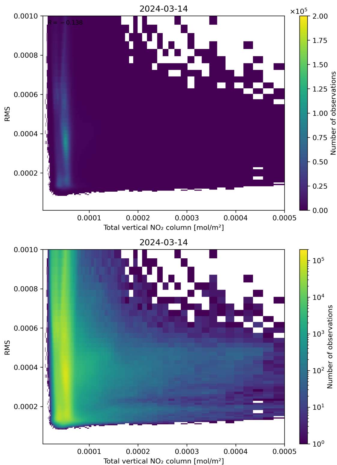
Figure 120: Scatter density plot of “Total vertical NO 2 column” against “RMS” for 2024-03-14 to 2024-03-15.
