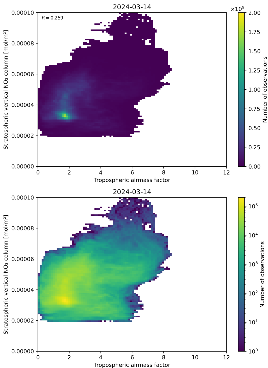
Figure 74: Scatter density plot of “Tropospheric air mass factor” against “Stratospheric vertical NO 2 column” for 2024-03-14 to 2024-03-15.
