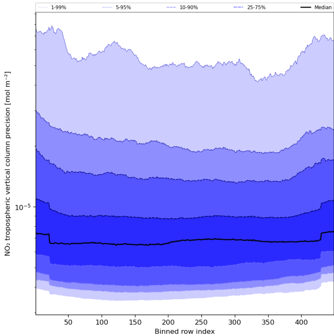
Figure 47: Along track statistics of “NO 2 tropospheric vertical column precision” for 2024-03-14 to 2024-03-15
