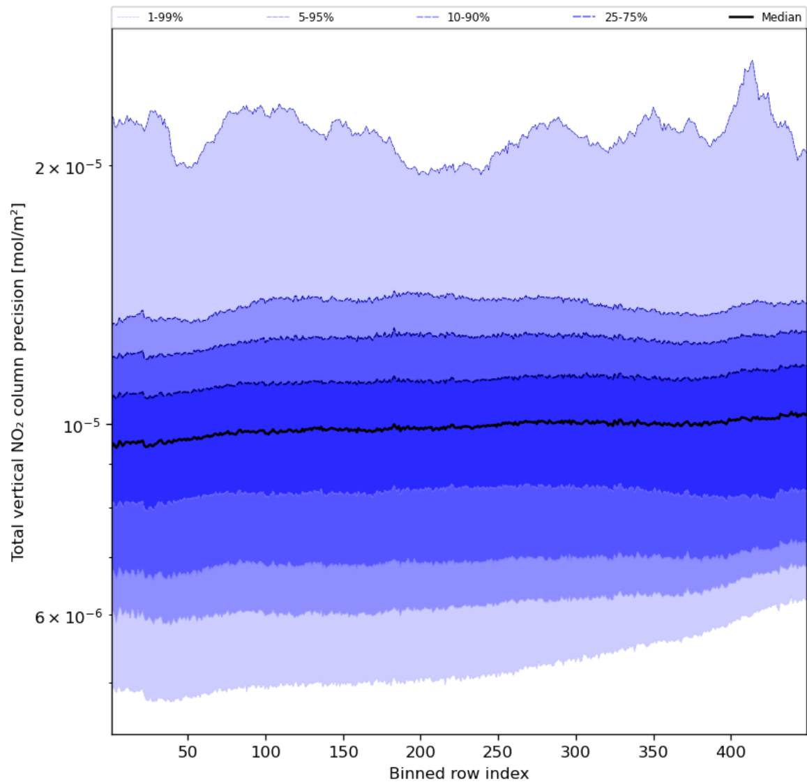
Figure 56: Along track statistics of “Total vertical NO 2 column precision” for 2024-03-14 to 2024-03-15
