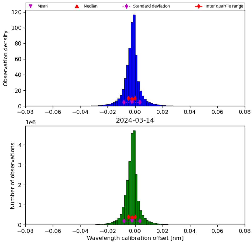
Figure 35: Histogram of “Wavelength calibration offset” for 2024-03-14 to 2024-03-15
