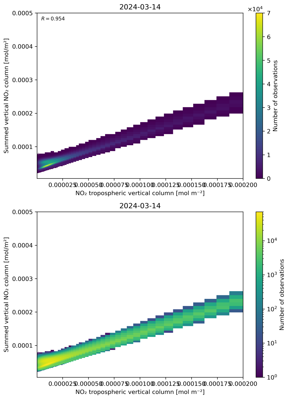
Figure 126: Scatter density plot of “NO 2 tropospheric vertical column” against “Summed vertical NO 2 column” for 2024-03-14 to 2024-03-15.
