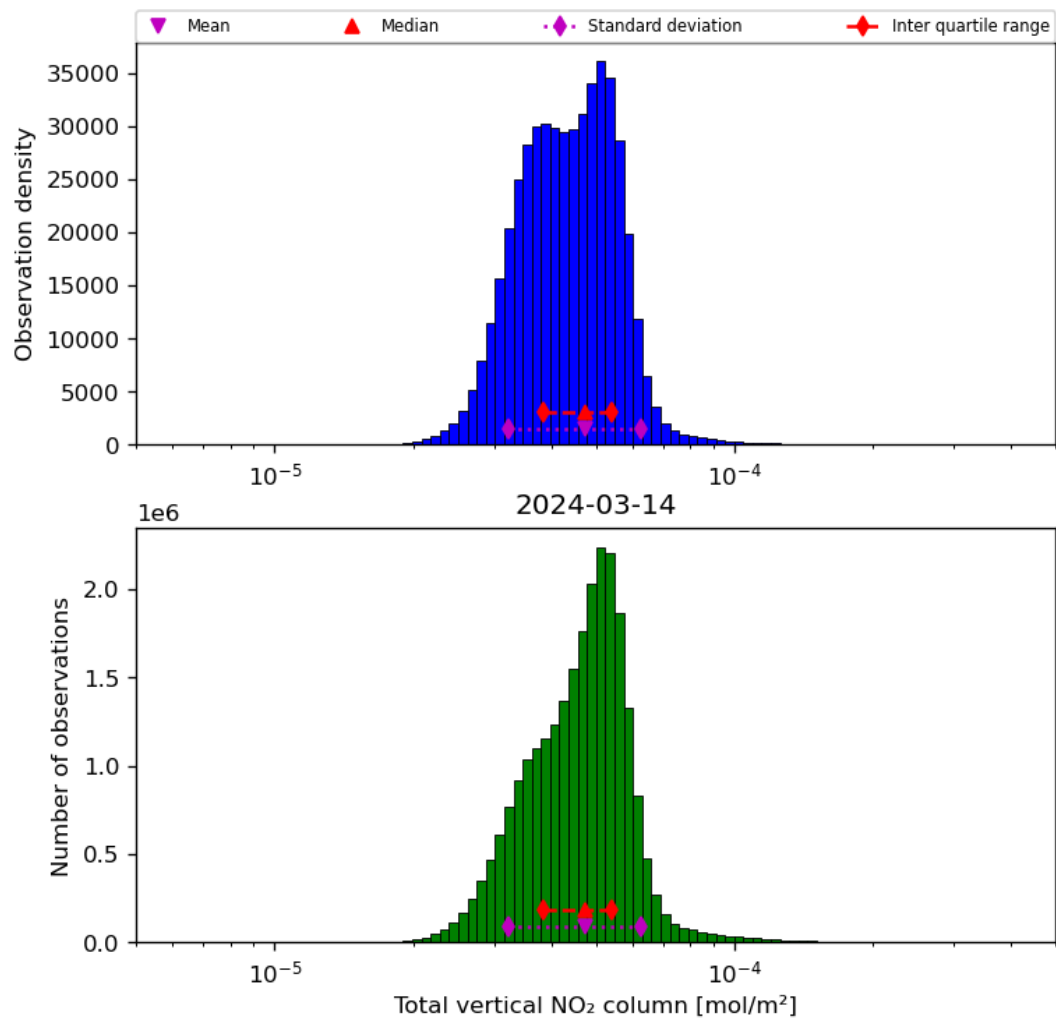
Figure 38: Histogram of “Total vertical NO 2 column” for 2024-03-14 to 2024-03-15
