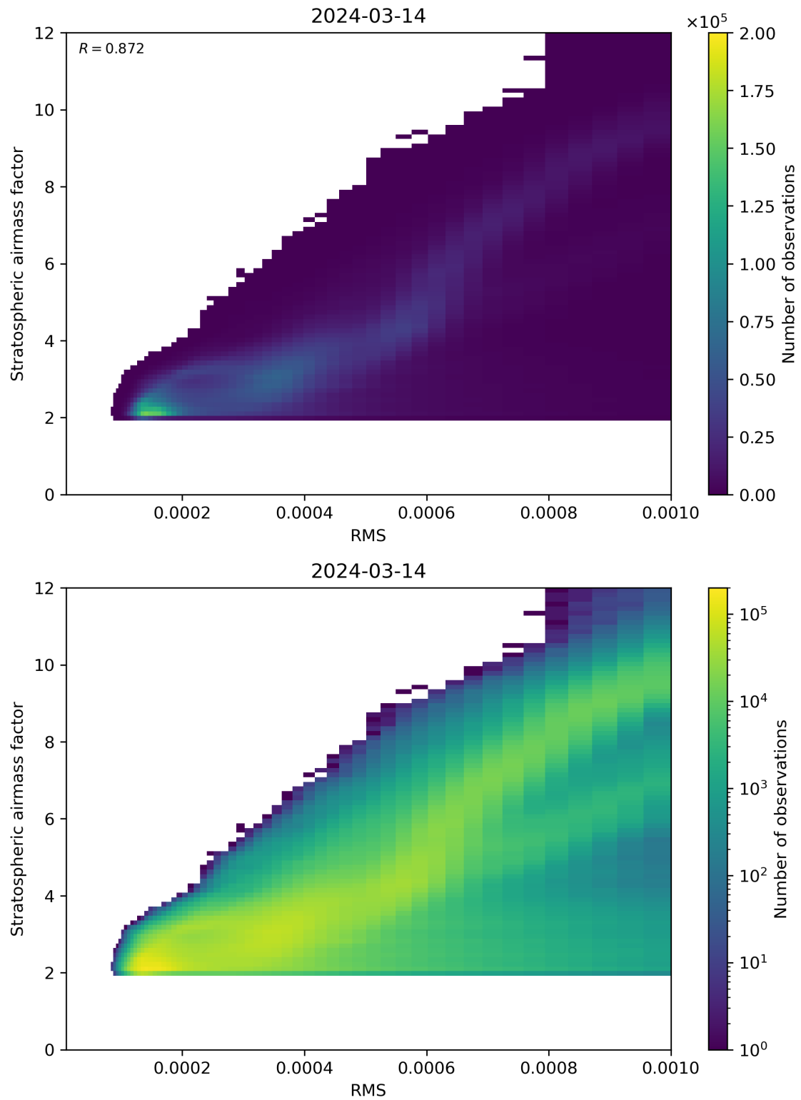
Figure 144: Scatter density plot of “RMS” against “Stratospheric airmass factor” for 2024-03-14 to 2024-03-15.
