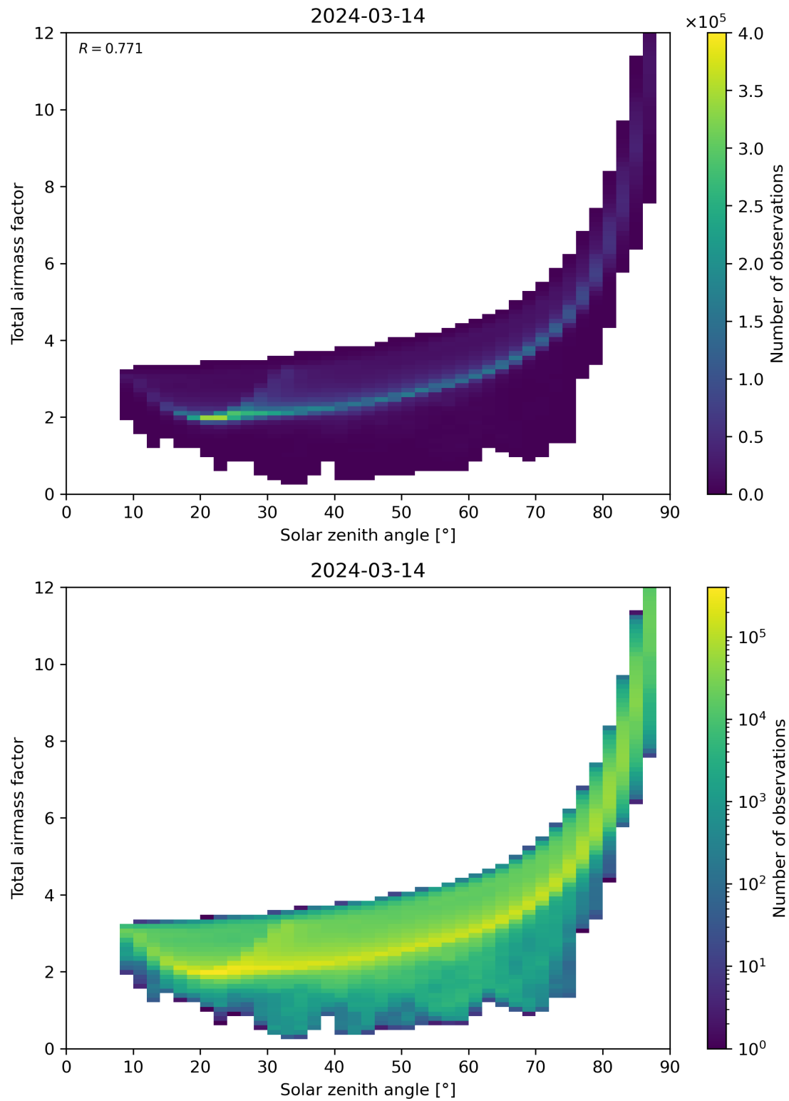
Figure 146: Scatter density plot of “Solar zenith angle” against “Total air mass factor” for 2024-03-14 to 2024-03-15.
