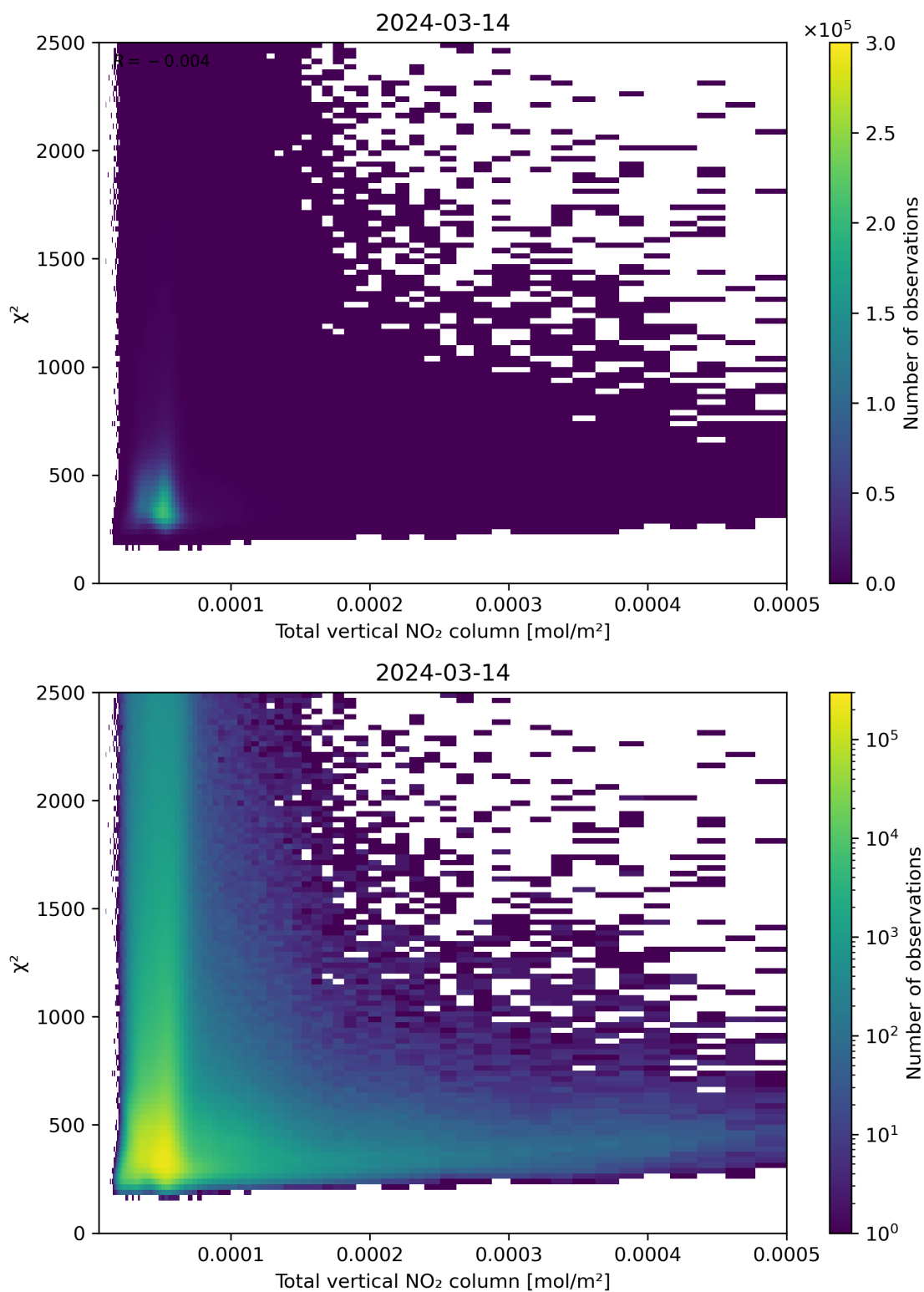
Figure 111: Scatter density plot of “Total vertical NO 2 column” against “ \chi^2 ” for 2024-03-14 to 2024-03-15.
