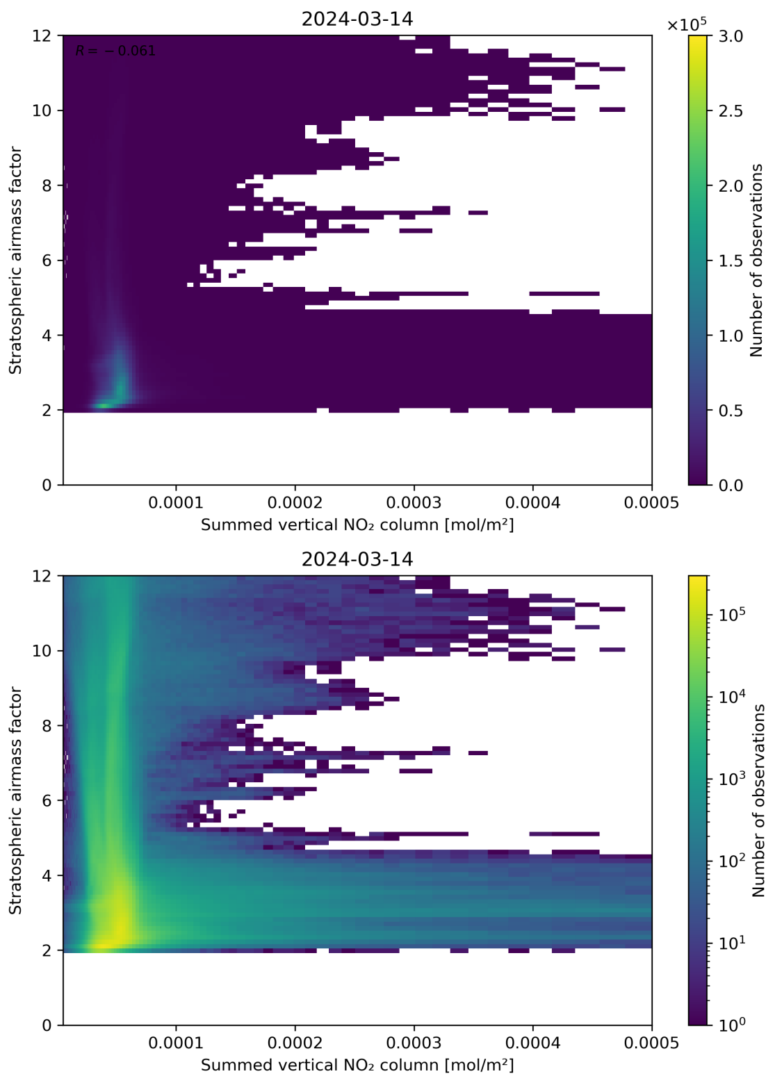
Figure 103: Scatter density plot of “Summed vertical NO 2 column” against “Stratospheric airmass factor” for 2024-03-14 to 2024-03-15.
