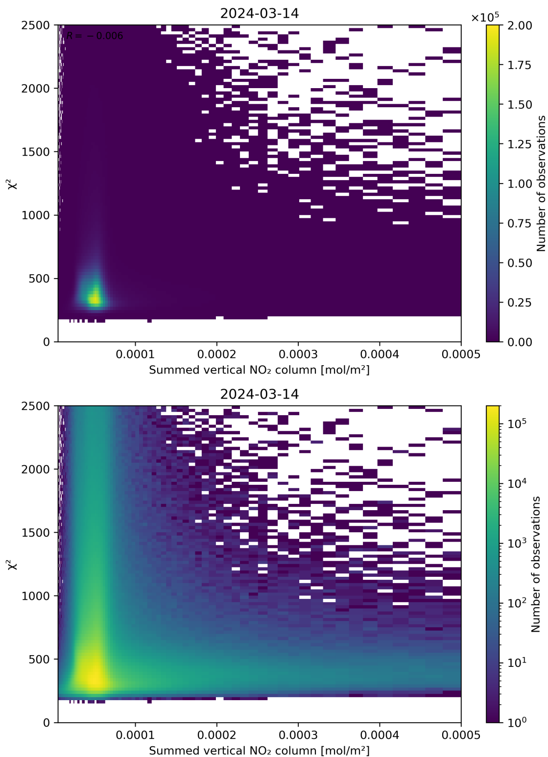
Figure 104: Scatter density plot of “Summed vertical NO 2 column” against “ \chi^2 ” for 2024-03-14 to 2024-03-15.
