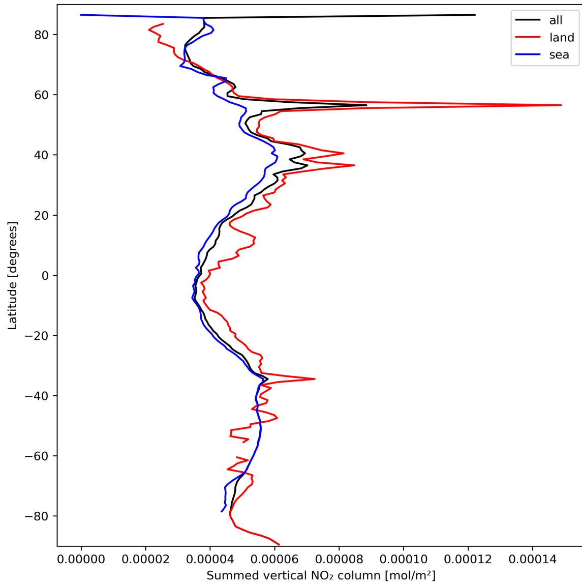
Figure 23: Zonal average of “Summed vertical NO 2 column” for 2024-03-14 to 2024-03-15.
