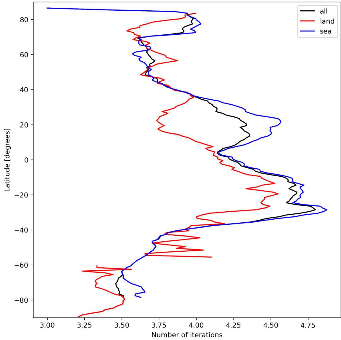
Figure 17: Zonal average of “Number of iterations” for 2024-03-14 to 2024-03-15.
