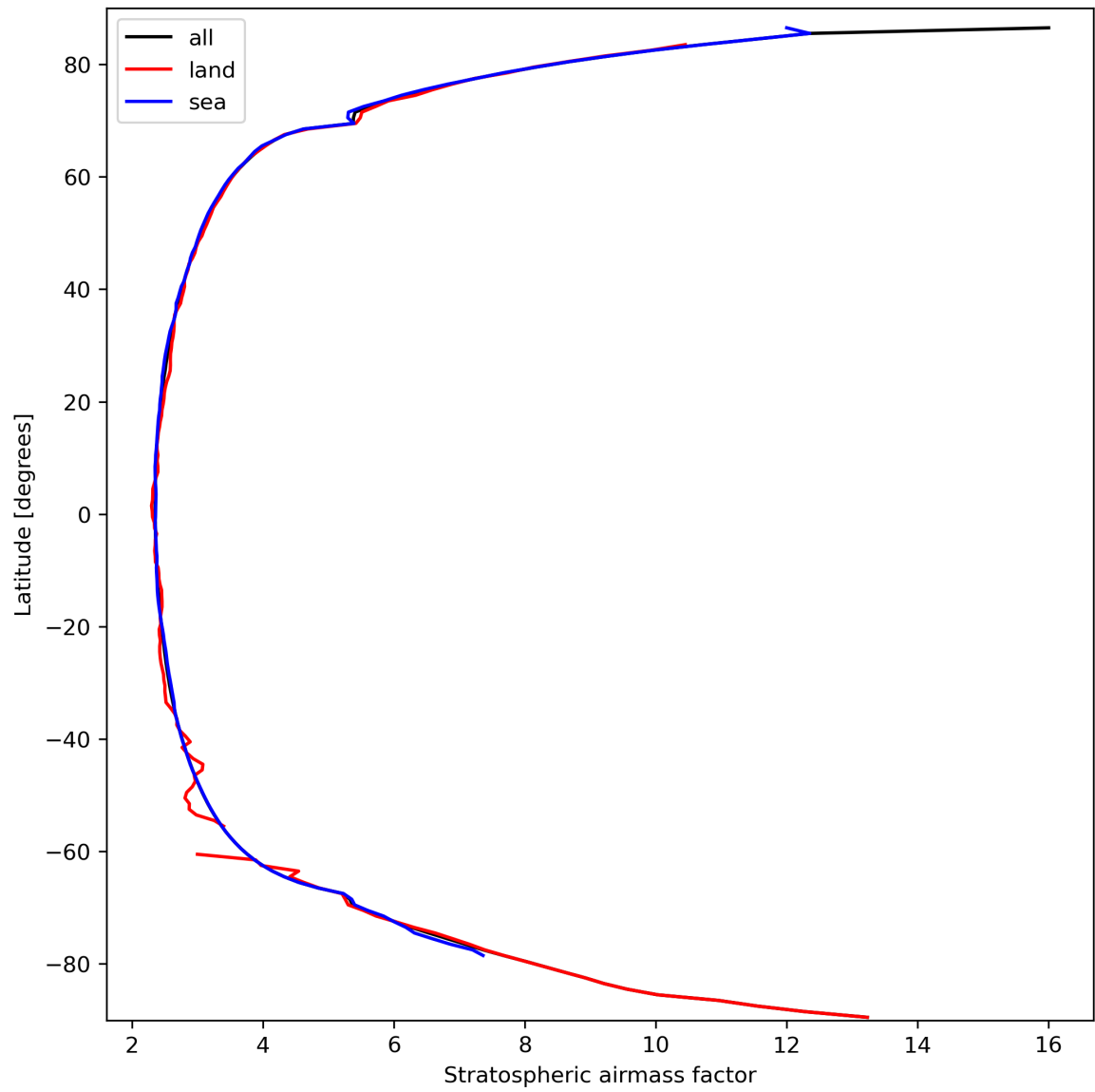
Figure 27: Zonal average of “Stratospheric air mass factor” for 2024-03-14 to 2024-03-15.
