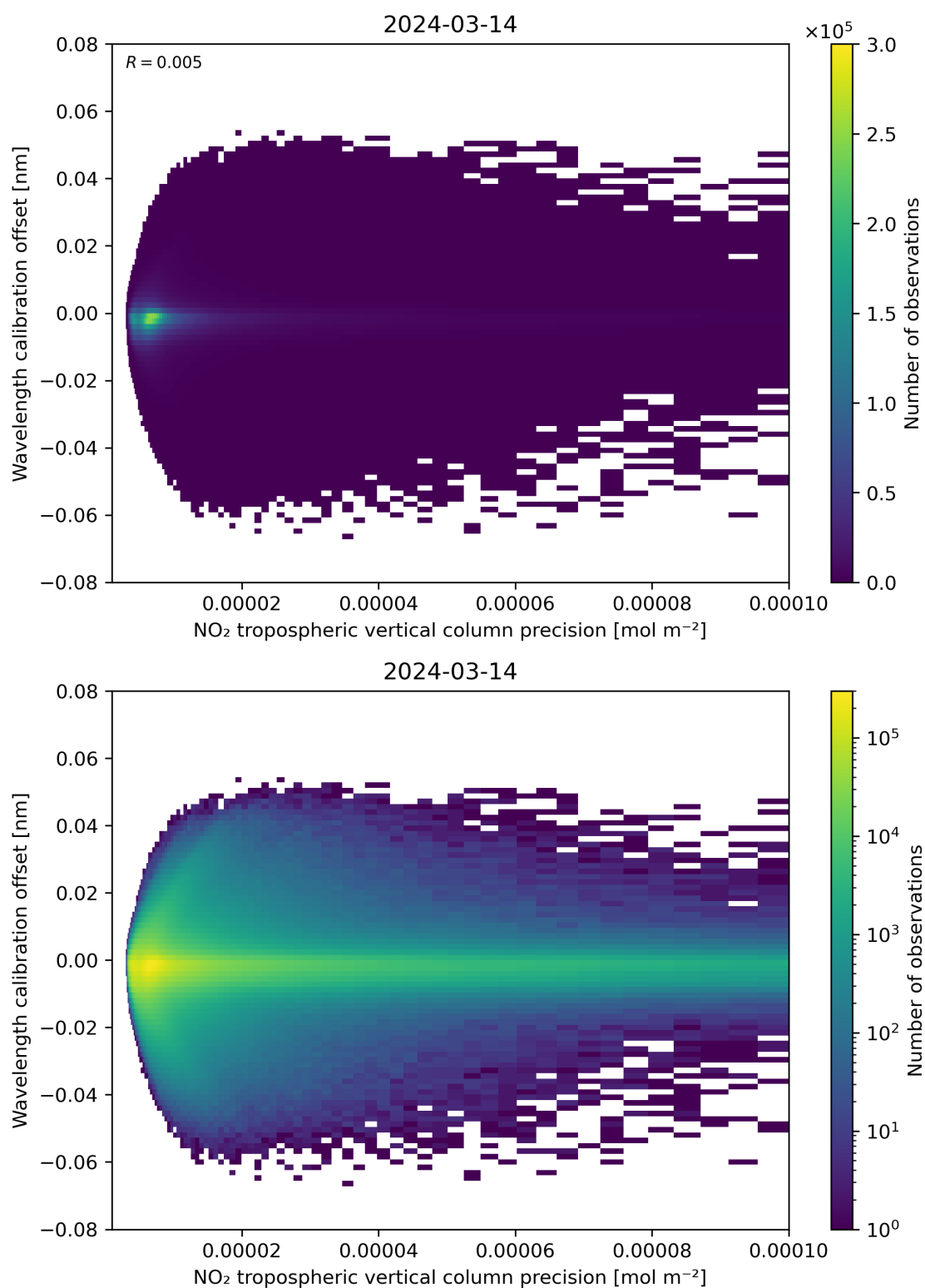
Figure 141: Scatter density plot of “NO 2 tropospheric vertical column precision” against “Wavelength calibration offset” for 2024-03-14 to 2024-03-15.
