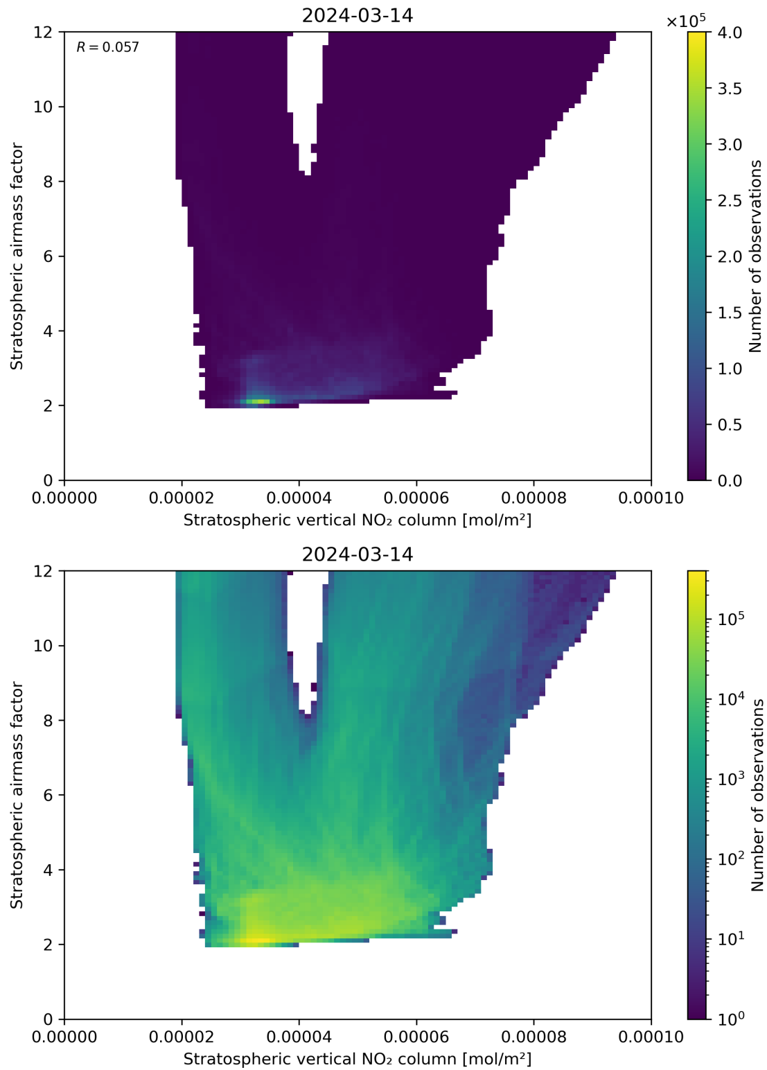
Figure 96: Scatter density plot of “Stratospheric vertical NO 2 column” against “Stratospheric airmass factor” for 2024-03-14 to 2024-03-15.
