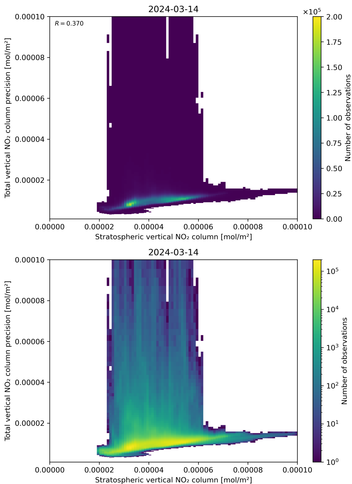
Figure 101: Scatter density plot of “Stratospheric vertical NO 2 column” against “Total vertical NO 2 column precision” for 2024-03-14 to 2024-03-15.
