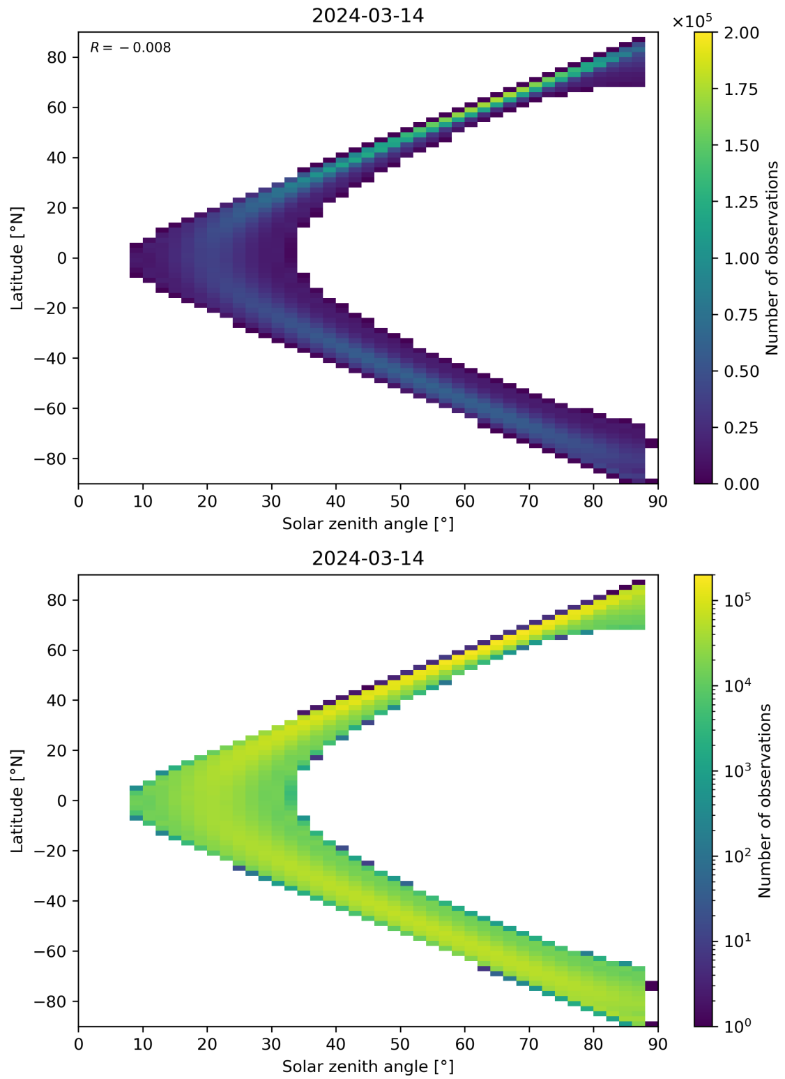
Figure 149: Scatter density plot of “Solar zenith angle” against “Latitude” for 2024-03-14 to 2024-03-15.
