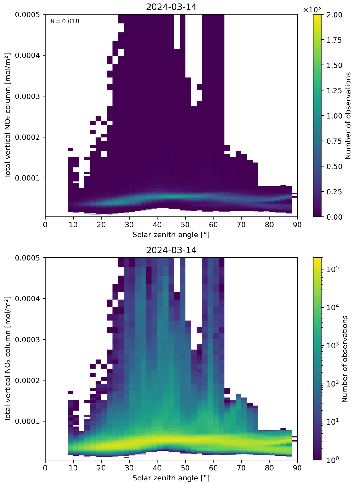
Figure 153: Scatter density plot of “Solar zenith angle” against “Total vertical NO 2 column” for 2024-03-14 to 2024-03-15.
