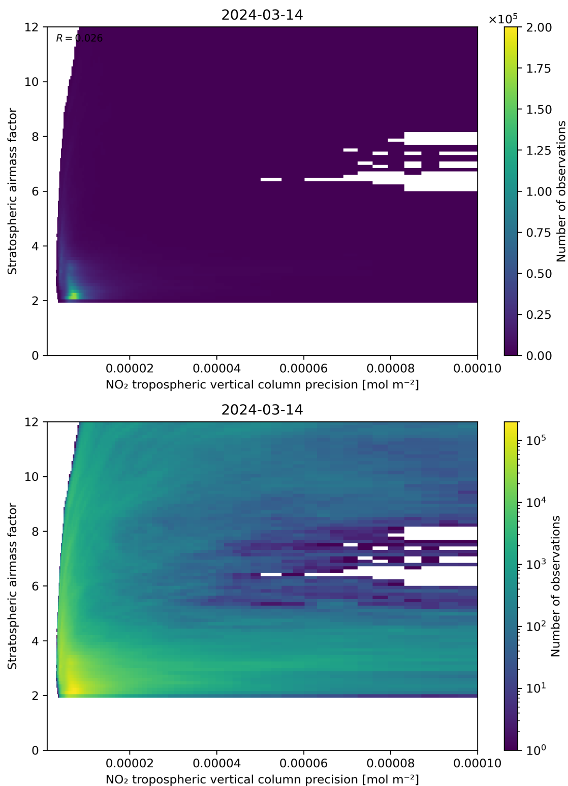
Figure 131: Scatter density plot of “NO 2 tropospheric vertical column precision” against “Stratospheric airmass factor” for 2024-03-14 to 2024-03-15.
