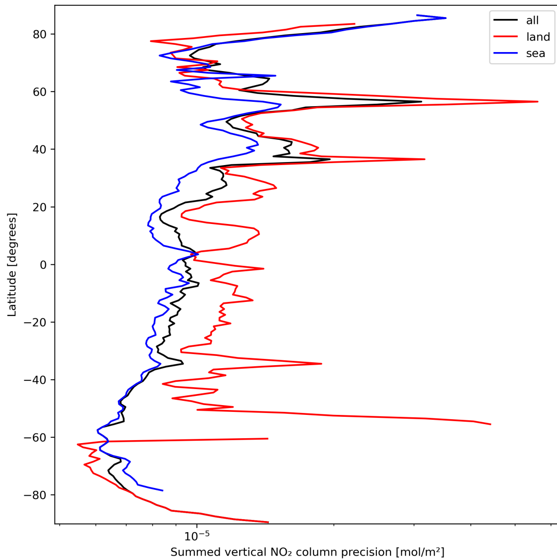
Figure 24: Zonal average of “Summed vertical NO 2 column precision” for 2024-03-14 to 2024-03-15.
