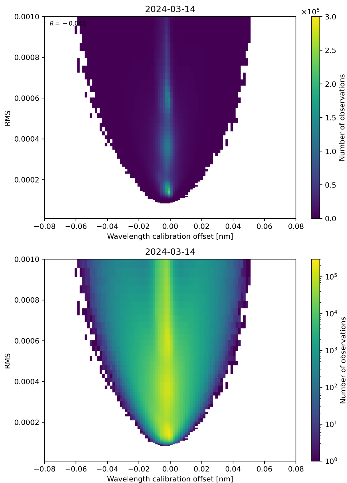
Figure 181: Scatter density plot of “Wavelength calibration offset” against “RMS” for 2024-03-14 to 2024-03-15.
