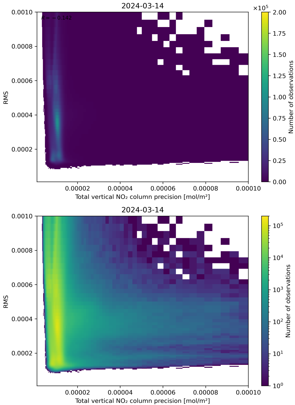
Figure 119: Scatter density plot of “Total vertical NO 2 column precision” against “RMS” for 2024-03-14 to 2024-03-15.
