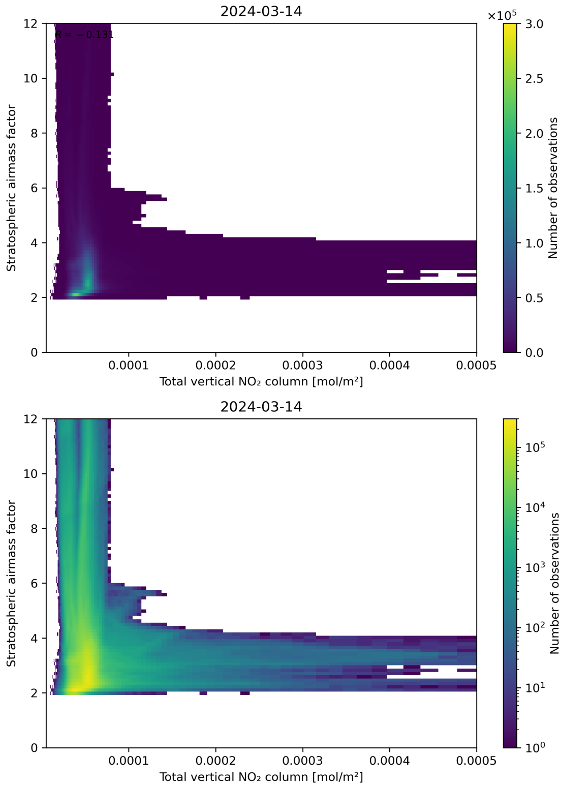
Figure 110: Scatter density plot of “Total vertical NO 2 column” against “Stratospheric airmass factor” for 2024-03-14 to 2024-03-15.
