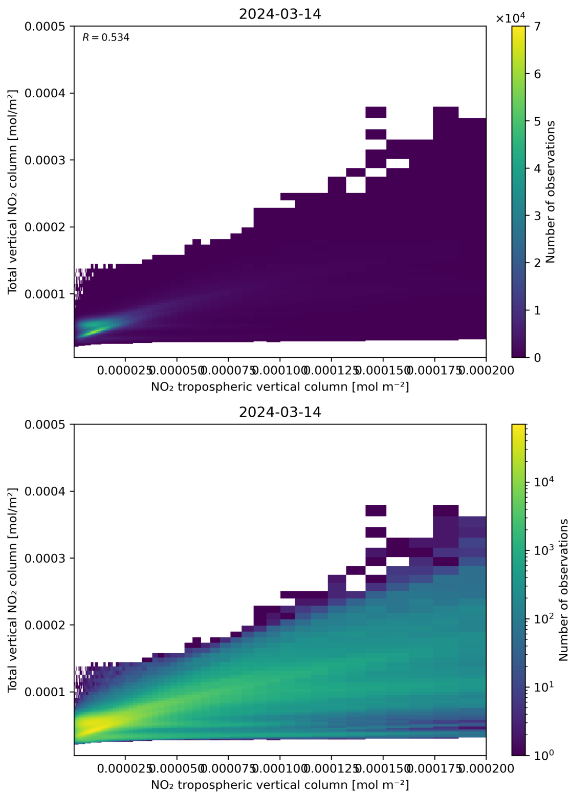
Figure 128: Scatter density plot of “NO 2 tropospheric vertical column” against “Total vertical NO 2 column” for 2024-03-14 to 2024-03-15.
