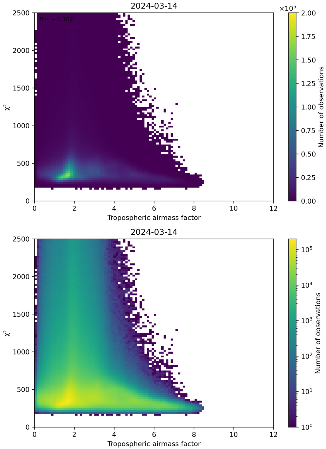
Figure 73: Scatter density plot of “Tropospheric airmass factor” against “ \chi^2 ” for 2024-03-14 to 2024-03-15.
