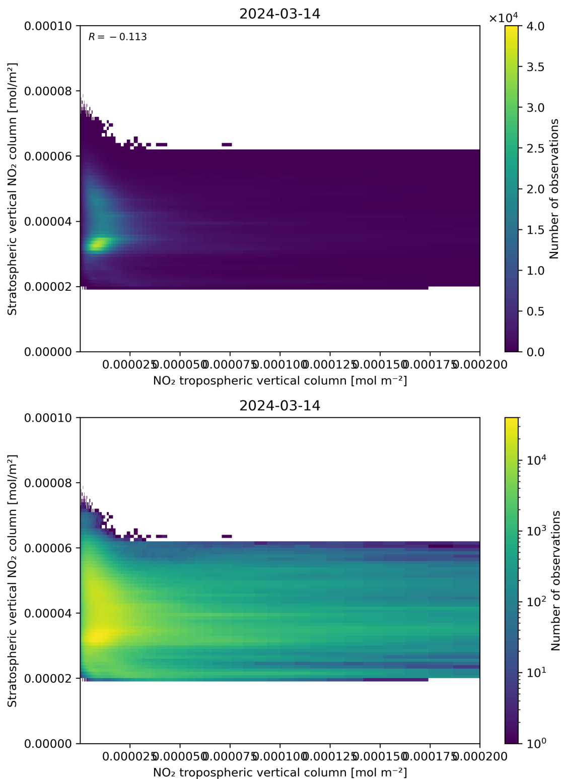
Figure 125: Scatter density plot of “NO 2 tropospheric vertical column” against “Stratospheric vertical NO 2 column” for 2024-03-14 to 2024-03-15.
