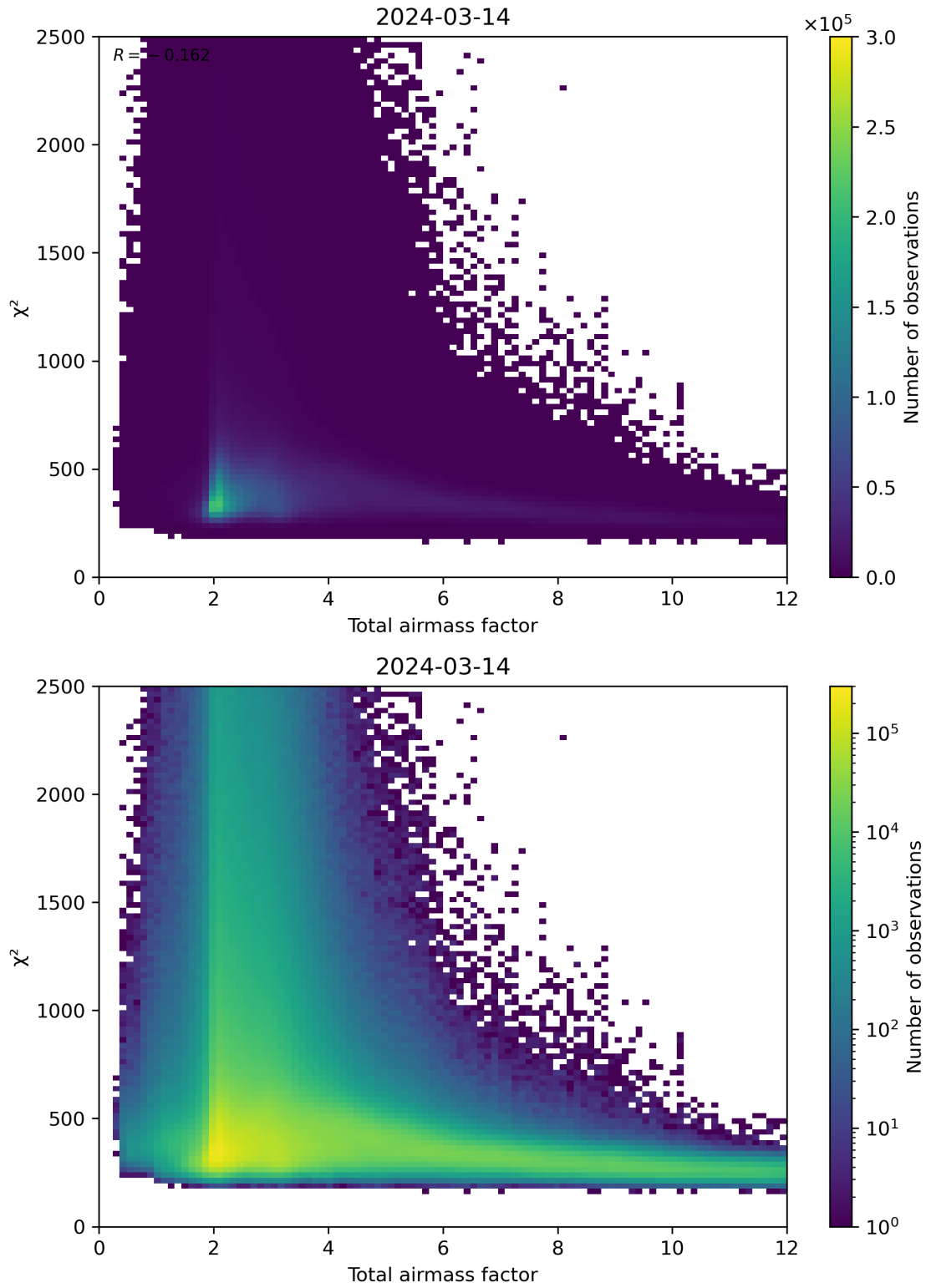
Figure 63: Scatter density plot of “Total airmass factor” against “ \chi^2 ” for 2024-03-14 to 2024-03-15.
