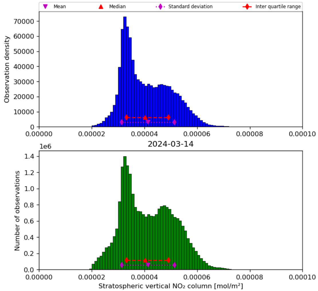
Figure 36: Histogram of “Stratospheric vertical NO 2 column” for 2024-03-14 to 2024-03-15
