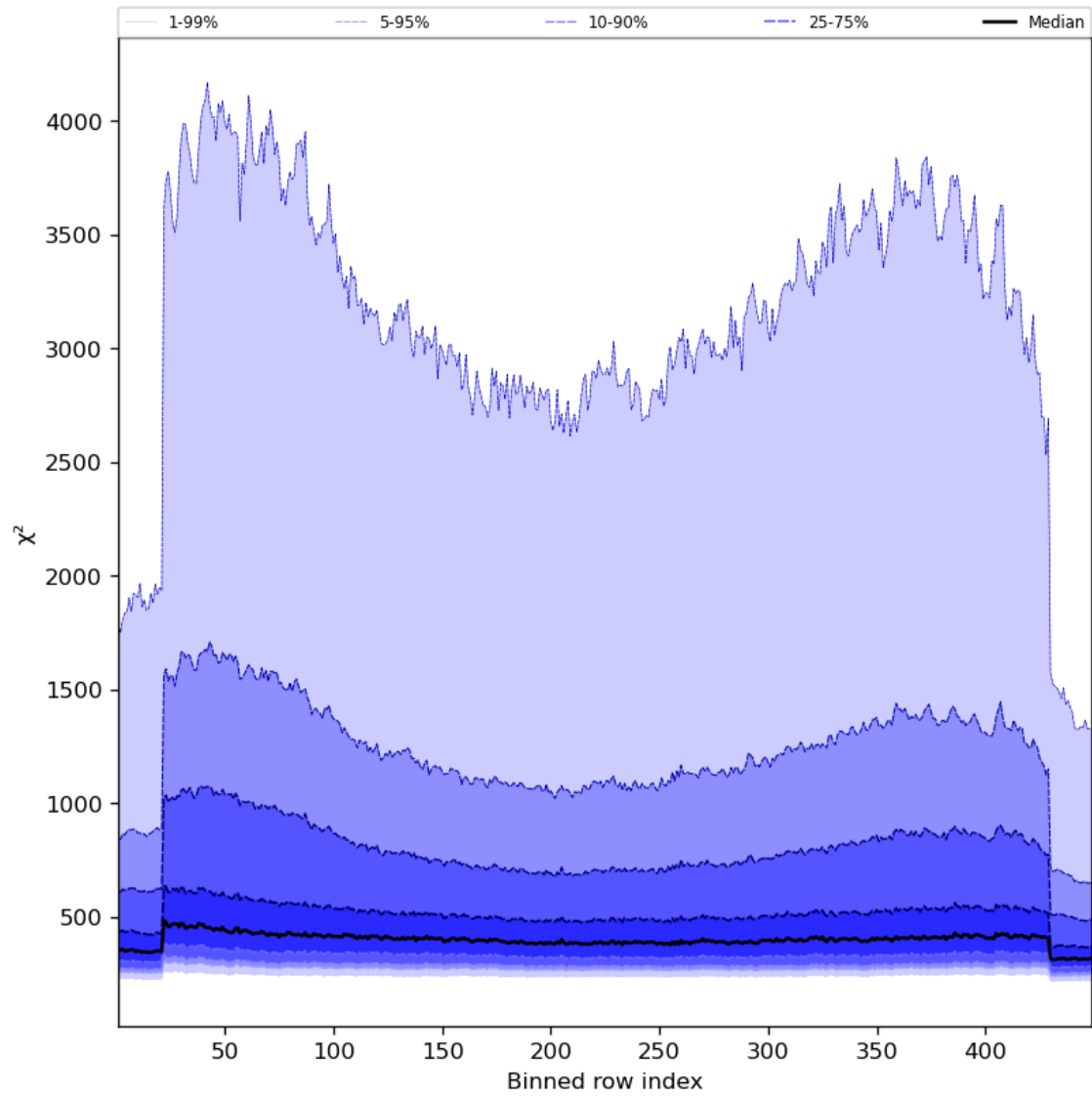
Figure 59: Along track statistics of “ \chi^2 ” for 2024-03-14 to 2024-03-15
