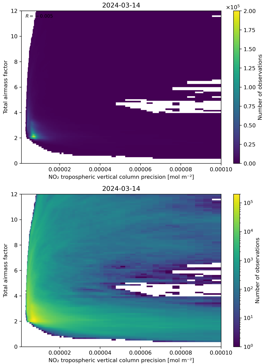
Figure 132: Scatter density plot of “NO 2 tropospheric vertical column precision” against “Total air mass factor” for 2024-03-14 to 2024-03-15.
