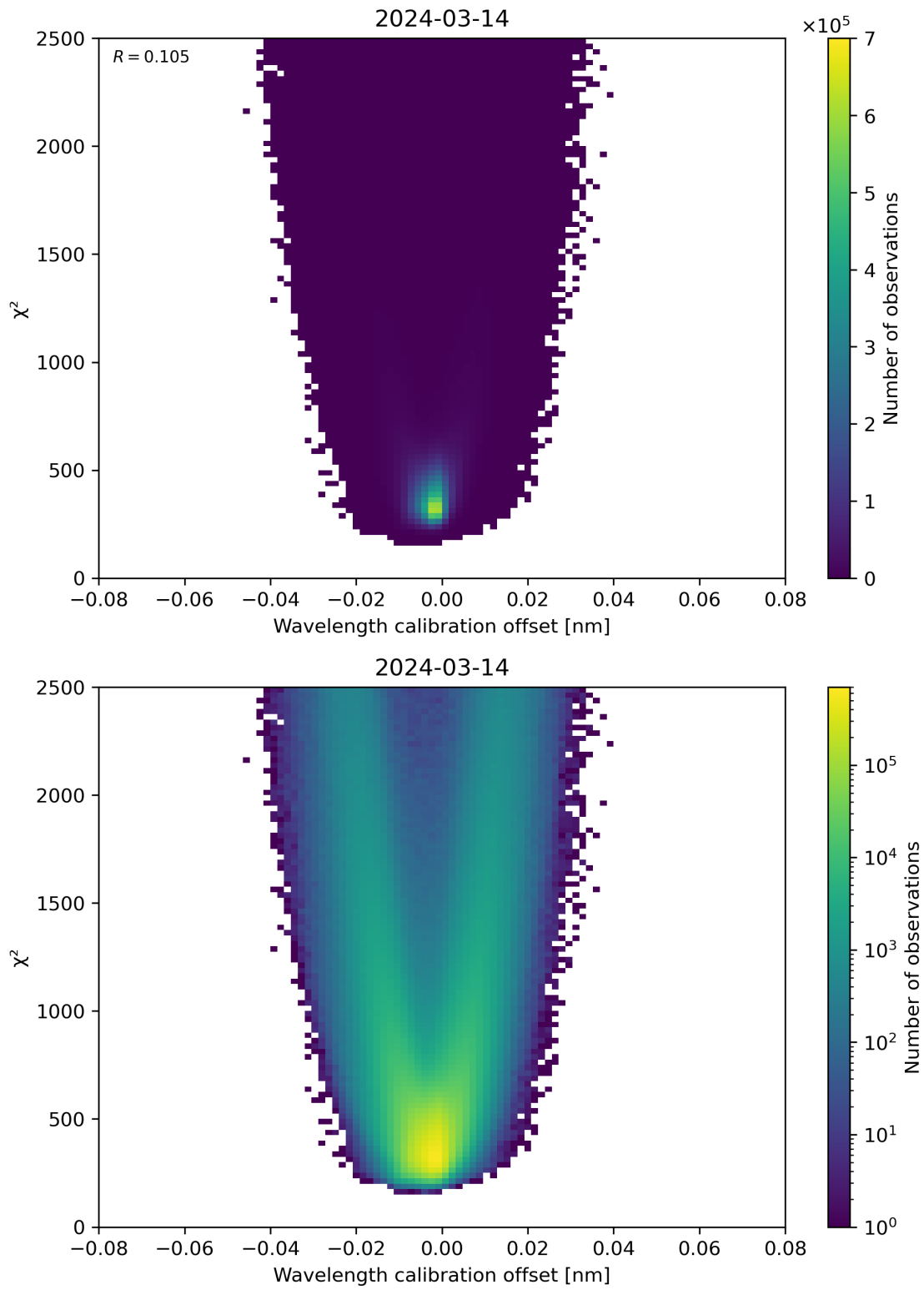
Figure 175: Scatter density plot of “Wavelength calibration offset” against “ \chi^2 ” for 2024-03-14 to 2024-03-15.
