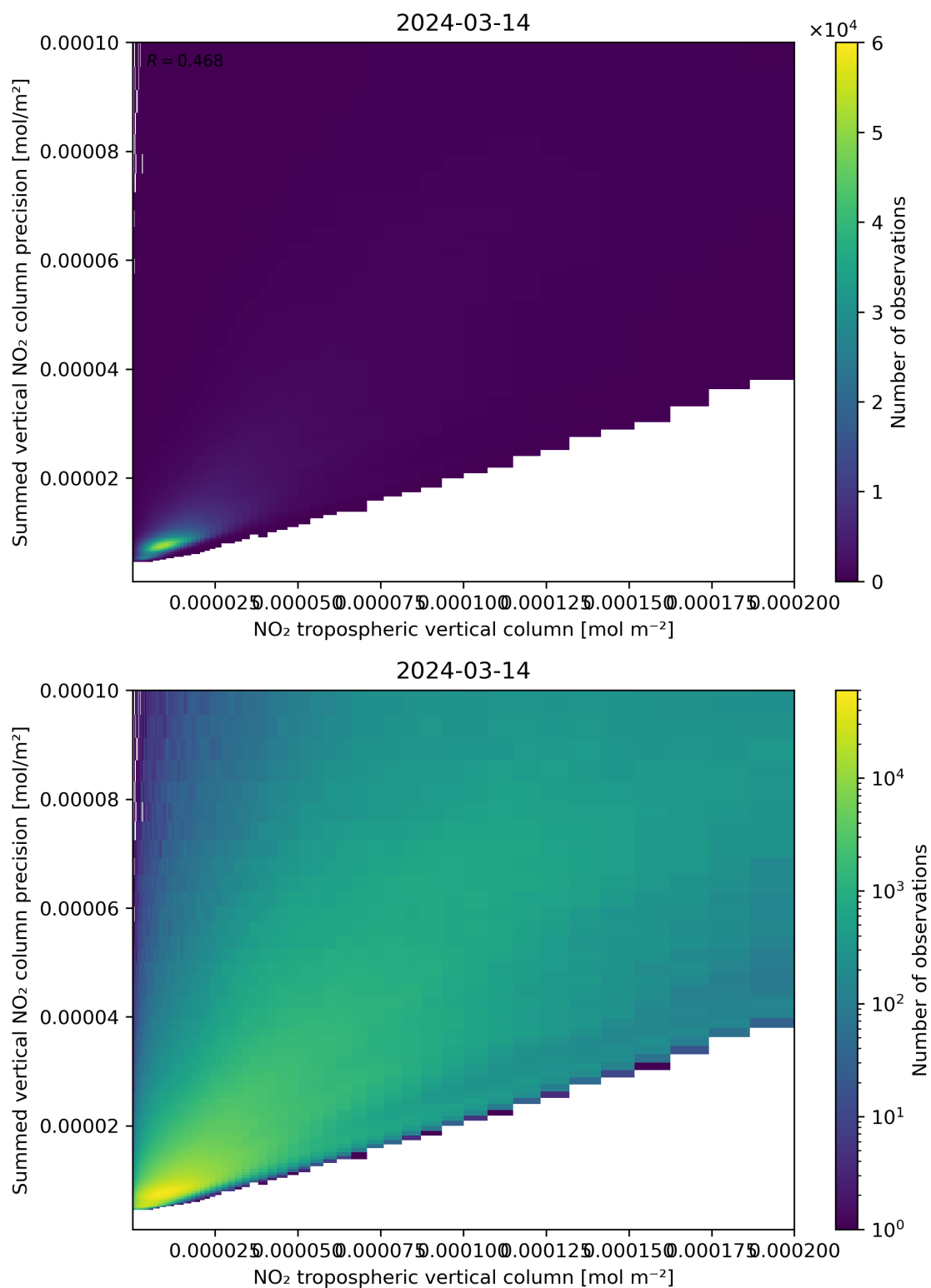
Figure 127: Scatter density plot of “NO 2 tropospheric vertical column” against “Summed vertical NO 2 column precision” for 2024-03-14 to 2024-03-15.
