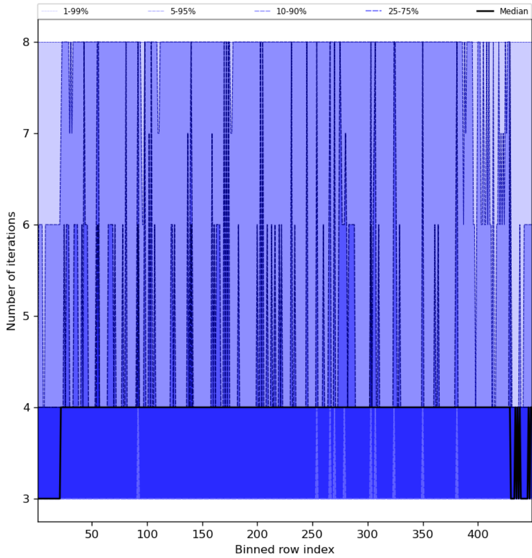
Figure 51: Along track statistics of “Number of iterations” for 2024-03-14 to 2024-03-15
