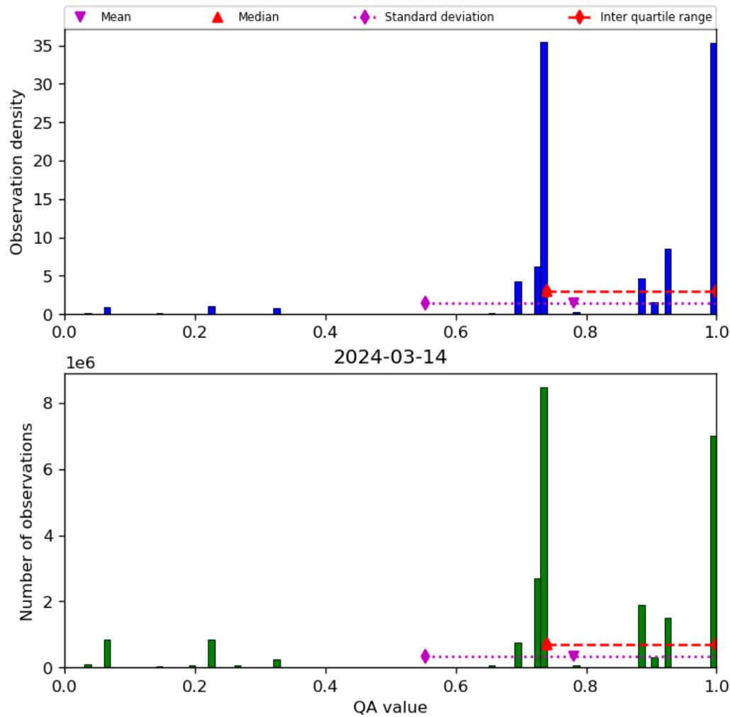
Figure 28: Histogram of “QA value” for 2024-03-14 to 2024-03-15
