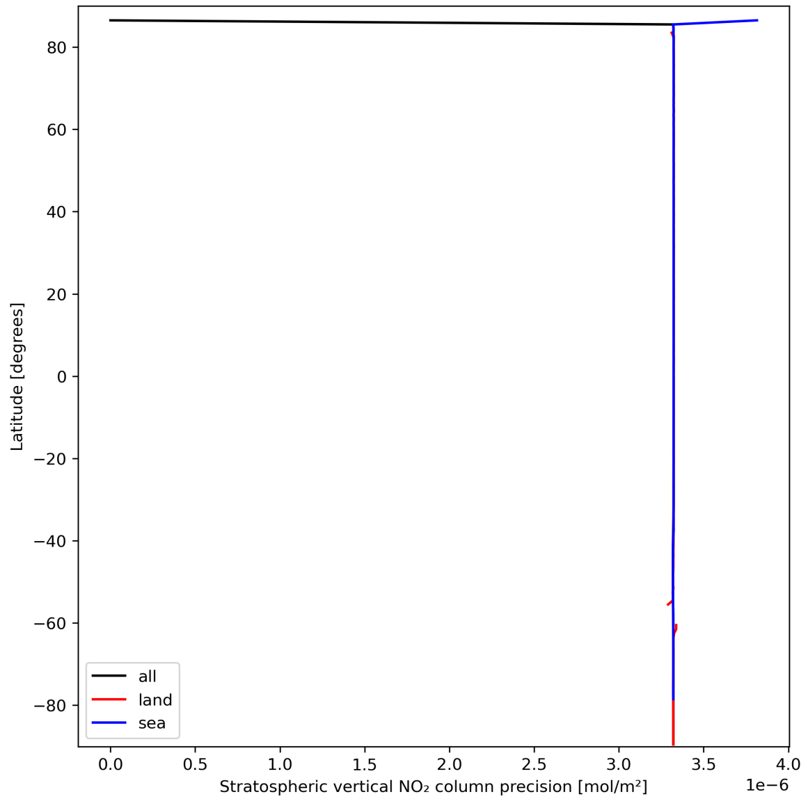
Figure 20: Zonal average of “Stratospheric vertical NO 2 column precision” for 2024-03-14 to 2024-03-15.
