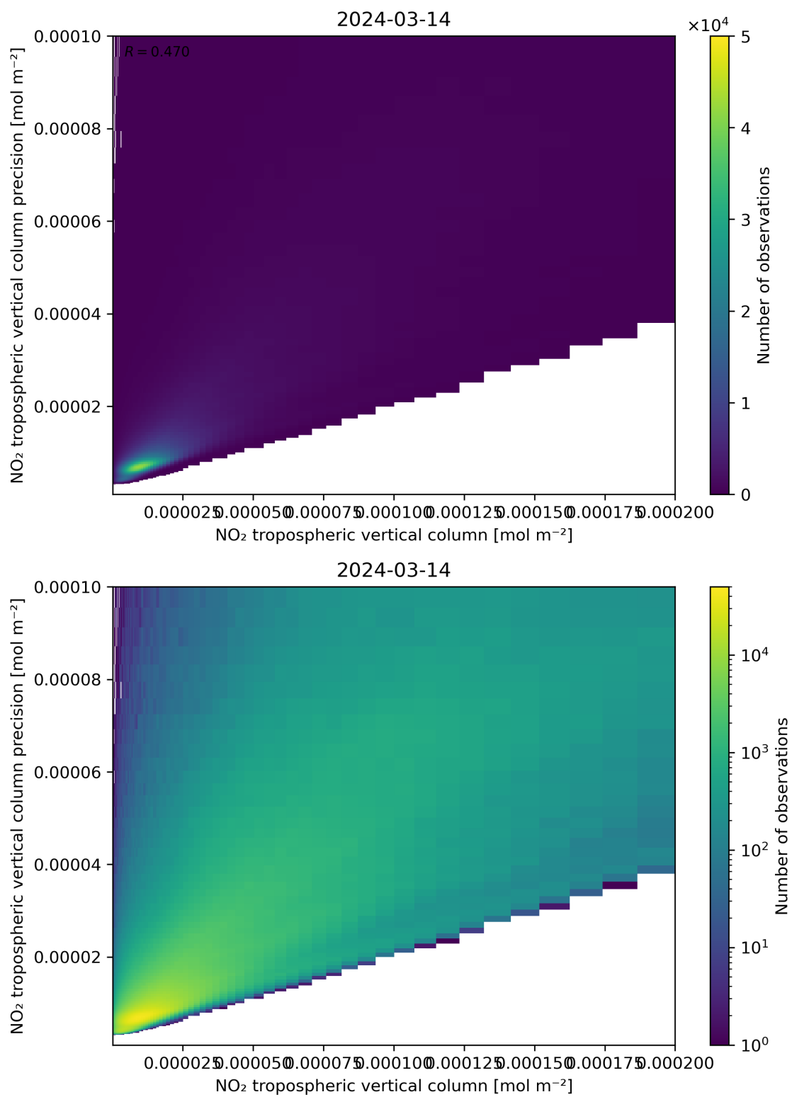
Figure 130: Scatter density plot of “NO 2 tropospheric vertical column” against “NO 2 tropospheric vertical column precision” for 2024-03-14 to 2024-03-15.
