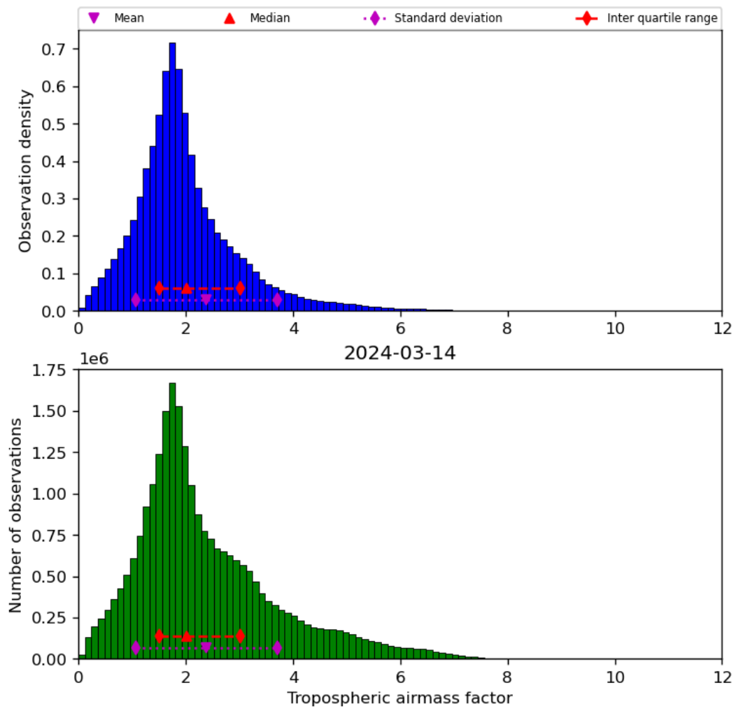
Figure 31: Histogram of “Tropospheric airmass factor” for 2024-03-14 to 2024-03-15
