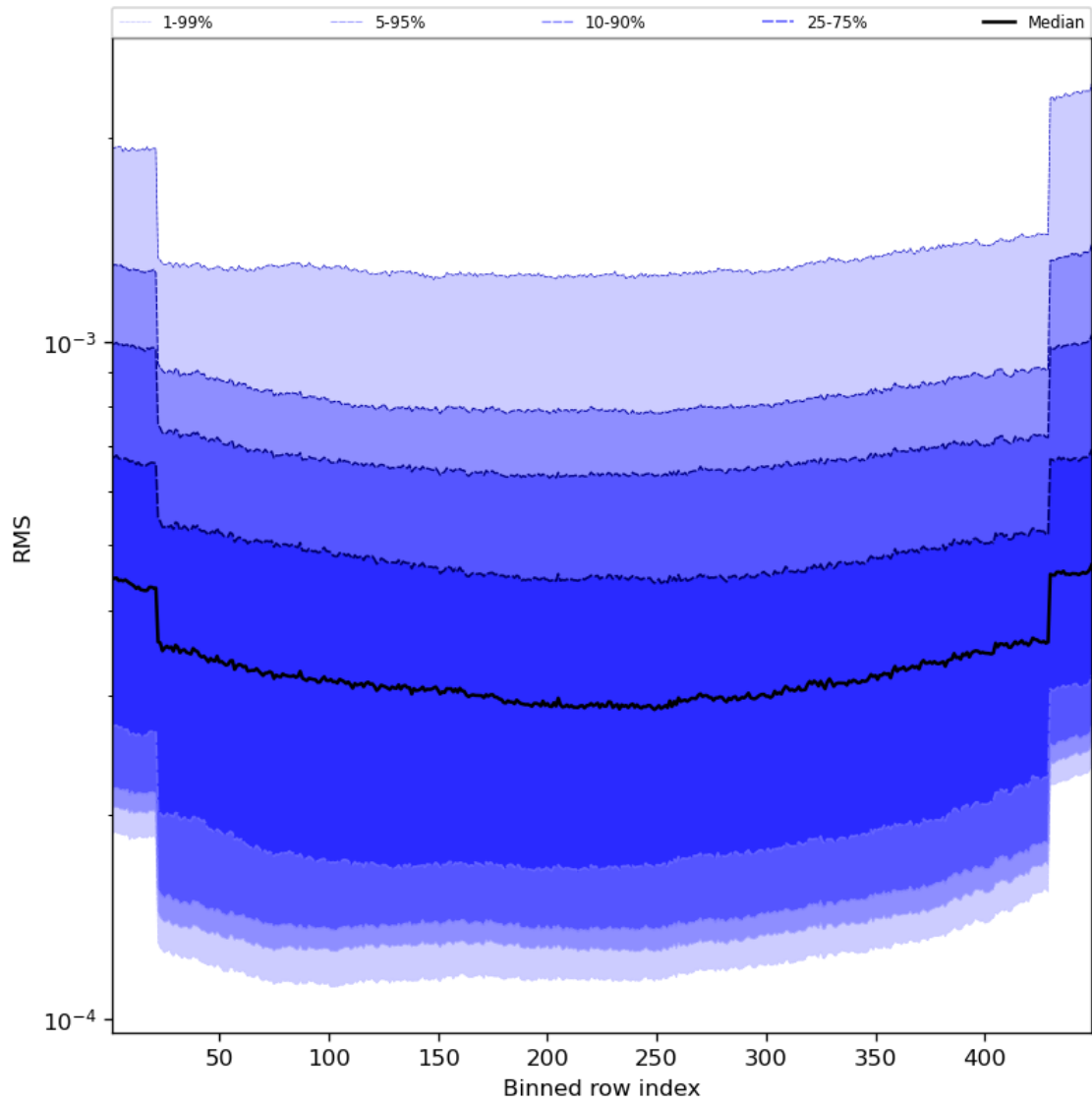
Figure 60: Along track statistics of “RMS” for 2024-03-14 to 2024-03-15
