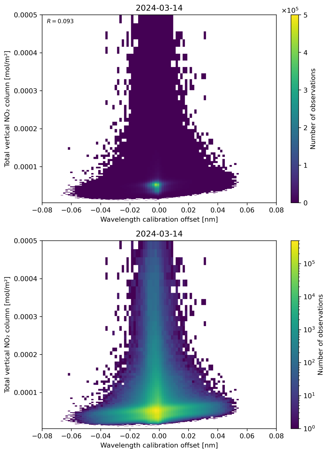
Figure 179: Scatter density plot of “Wavelength calibration offset” against “Total vertical NO 2 column” for 2024-03-14 to 2024-03-15.
