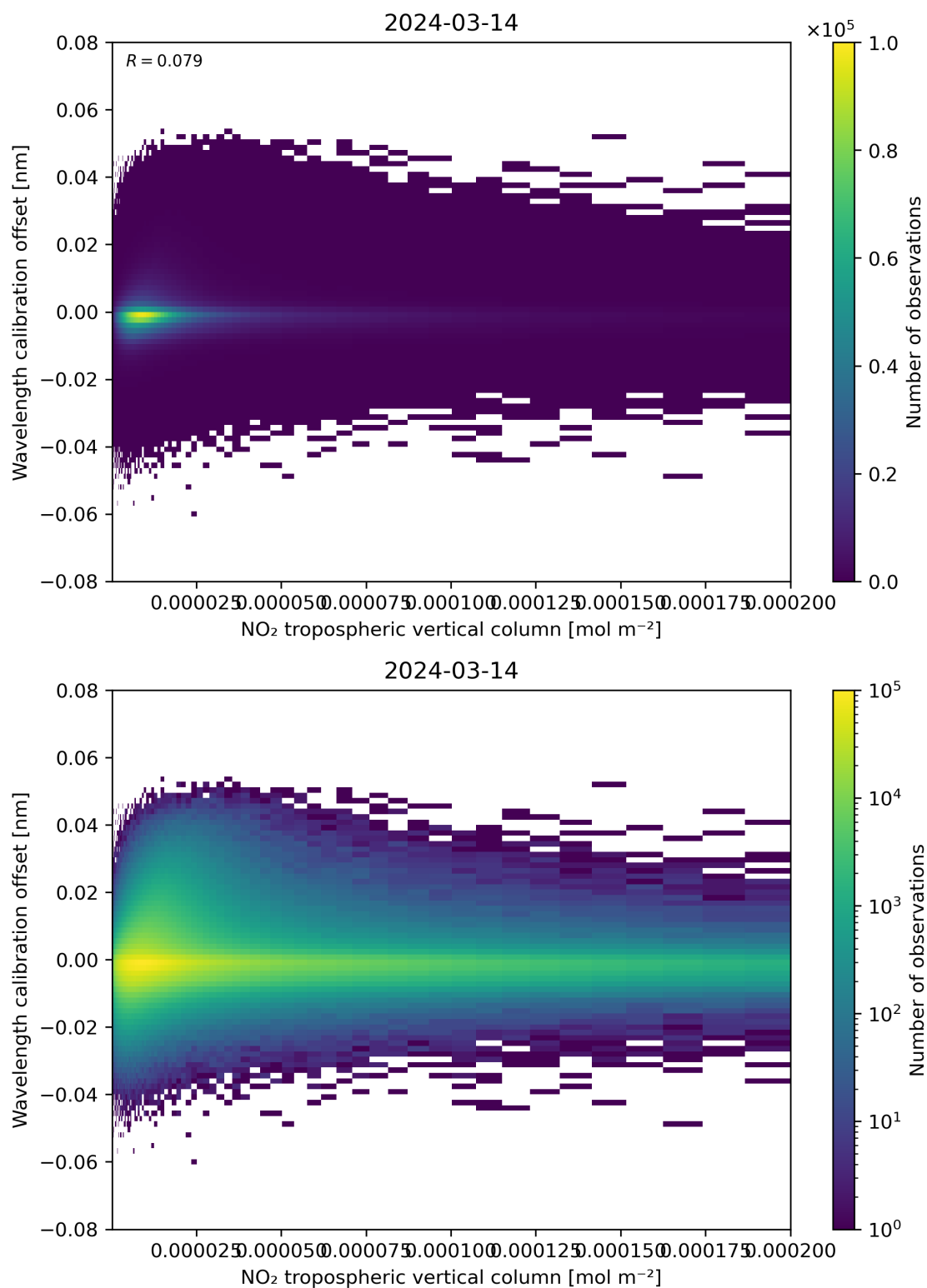
Figure 143: Scatter density plot of “NO 2 tropospheric vertical column” against “Wavelength calibration offset” for 2024-03-14 to 2024-03-15.
