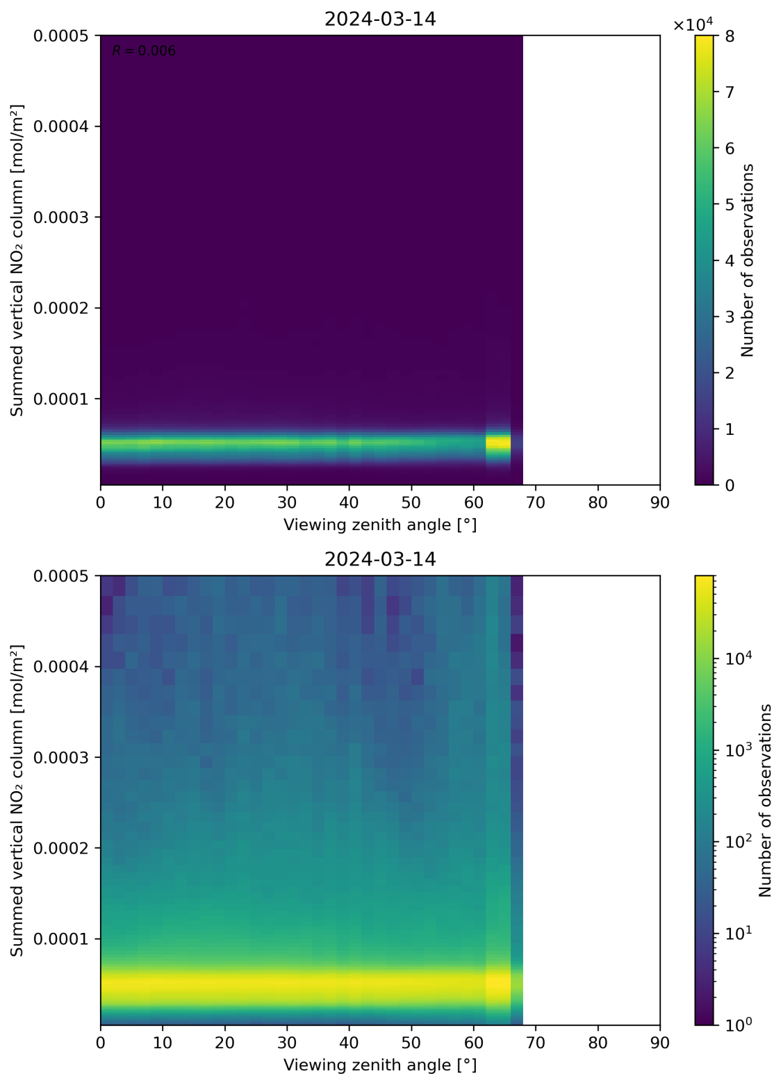
Figure 165: Scatter density plot of “Viewing zenith angle” against “Summed vertical NO 2 column” for 2024-03-14 to 2024-03-15.
