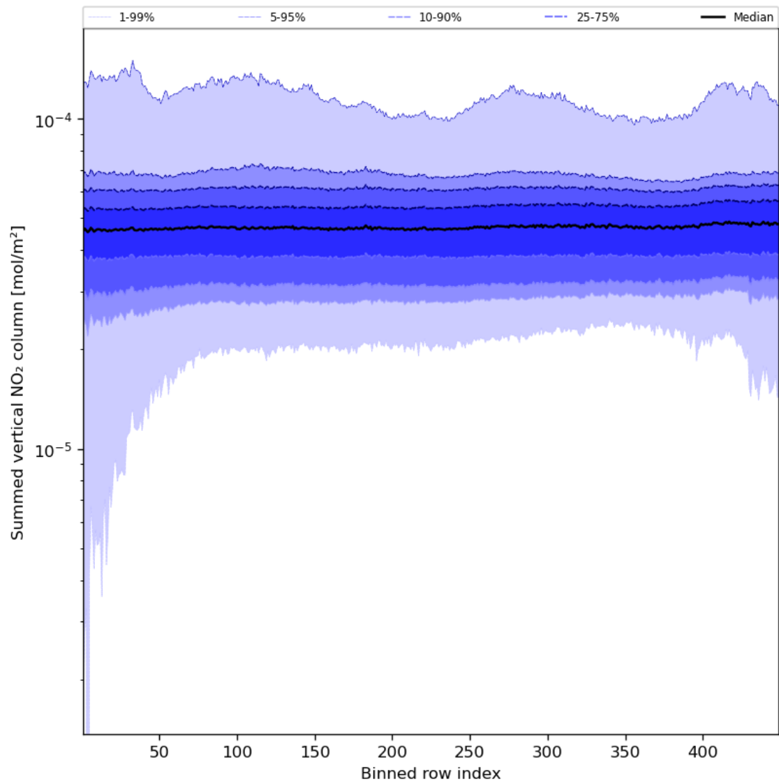
Figure 57: Along track statistics of “Summed vertical NO 2 column” for 2024-03-14 to 2024-03-15
