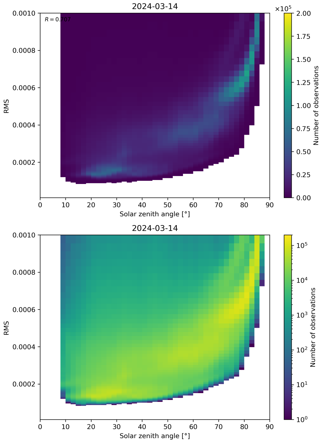
Figure 157: Scatter density plot of “Solar zenith angle” against “RMS” for 2024-03-14 to 2024-03-15.
