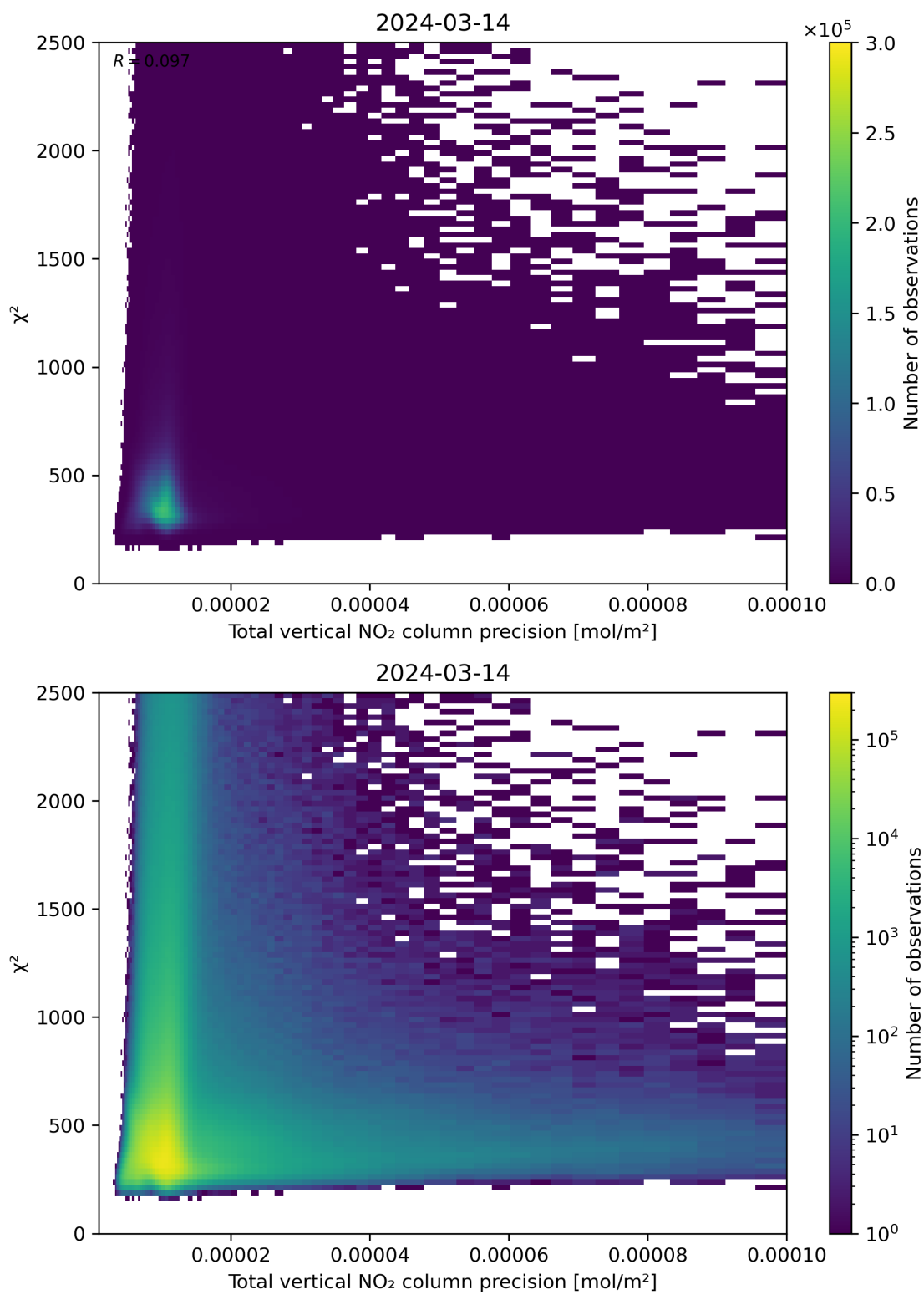
Figure 116: Scatter density plot of “Total vertical NO 2 column precision” against “ \chi^2 ” for 2024-03-14 to 2024-03-15.
