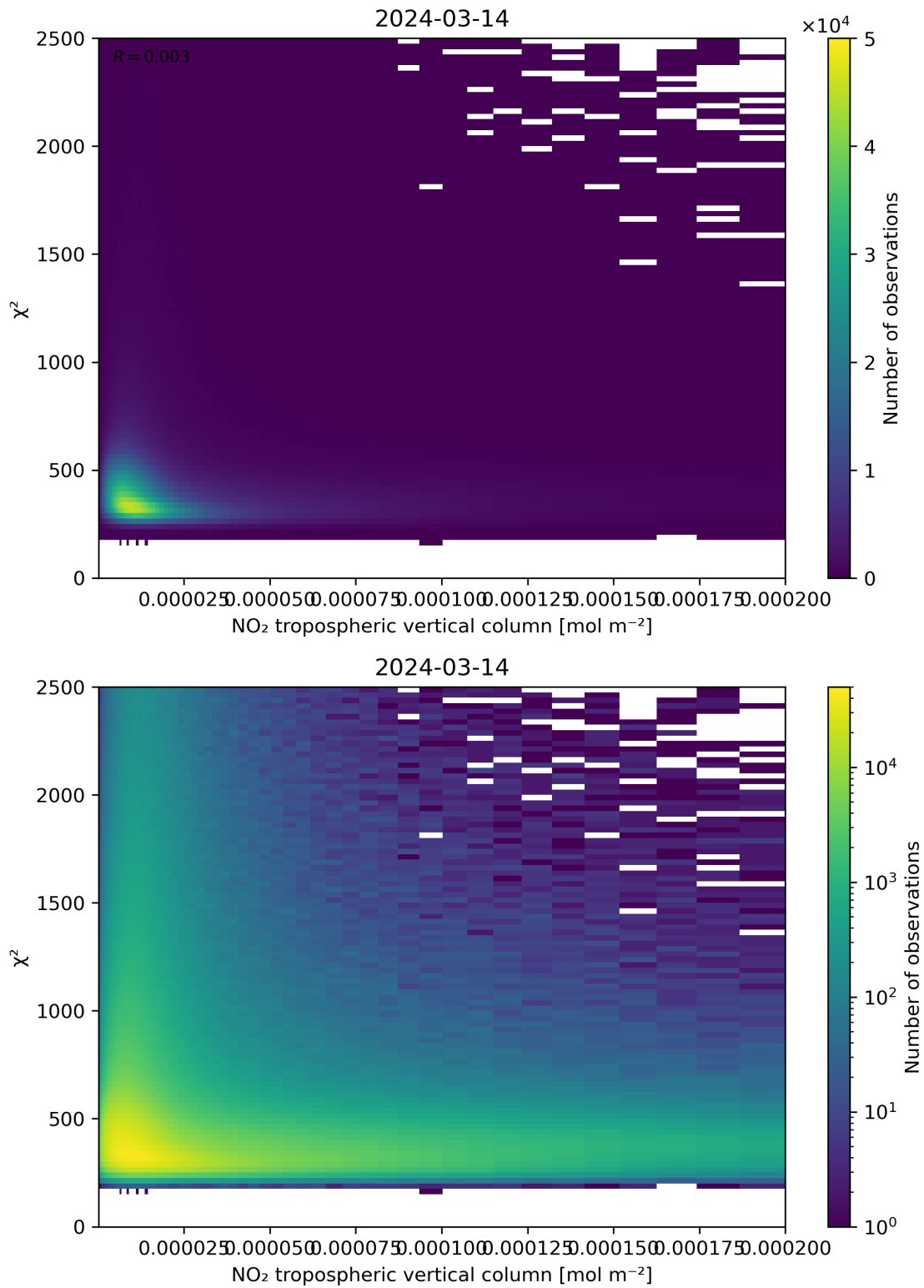
Figure 124: Scatter density plot of “NO 2 tropospheric vertical column” against “ \chi^2 ” for 2024-03-14 to 2024-03-15.
