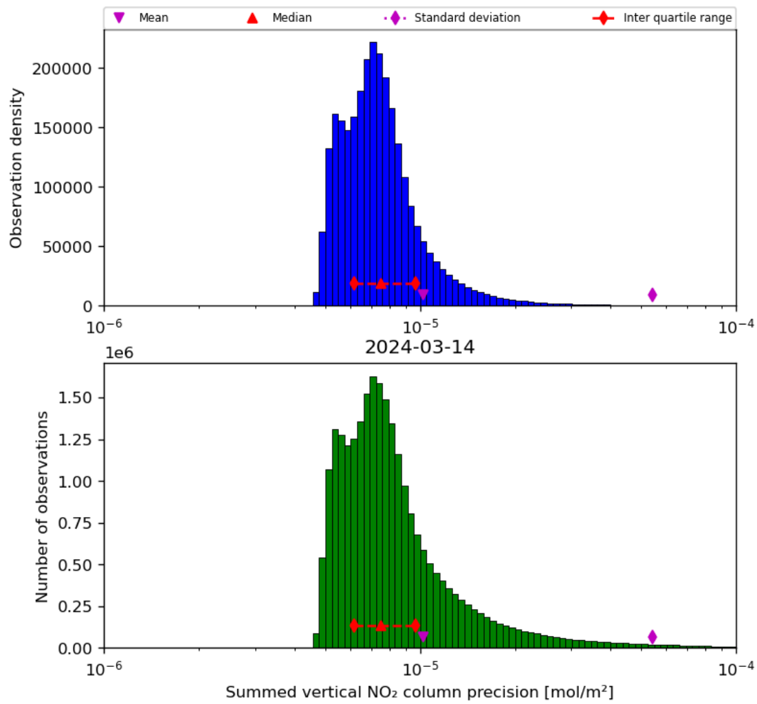
Figure 41: Histogram of “Summed vertical NO 2 column precision” for 2024-03-14 to 2024-03-15
