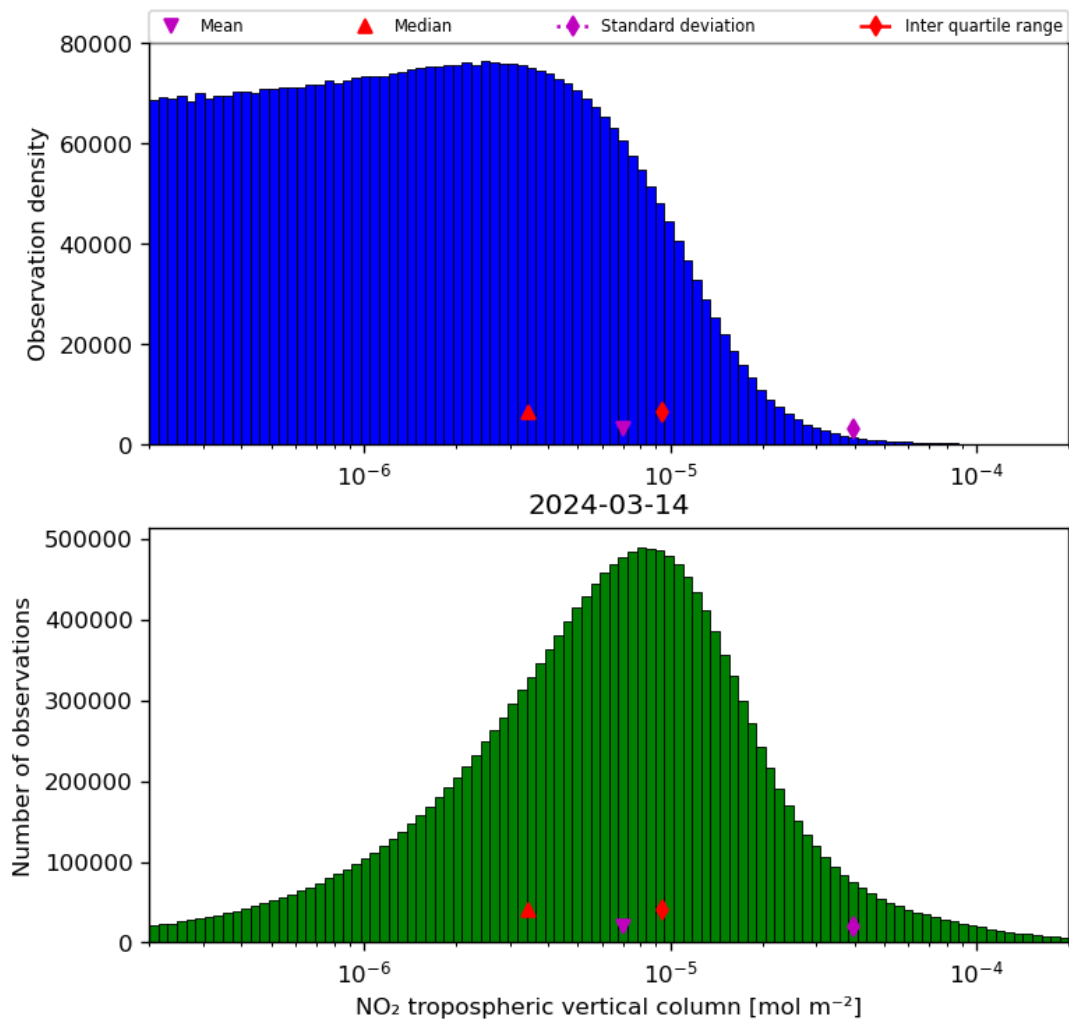
Figure 29: Histogram of “NO 2 tropospheric vertical column” for 2024-03-14 to 2024-03-15
