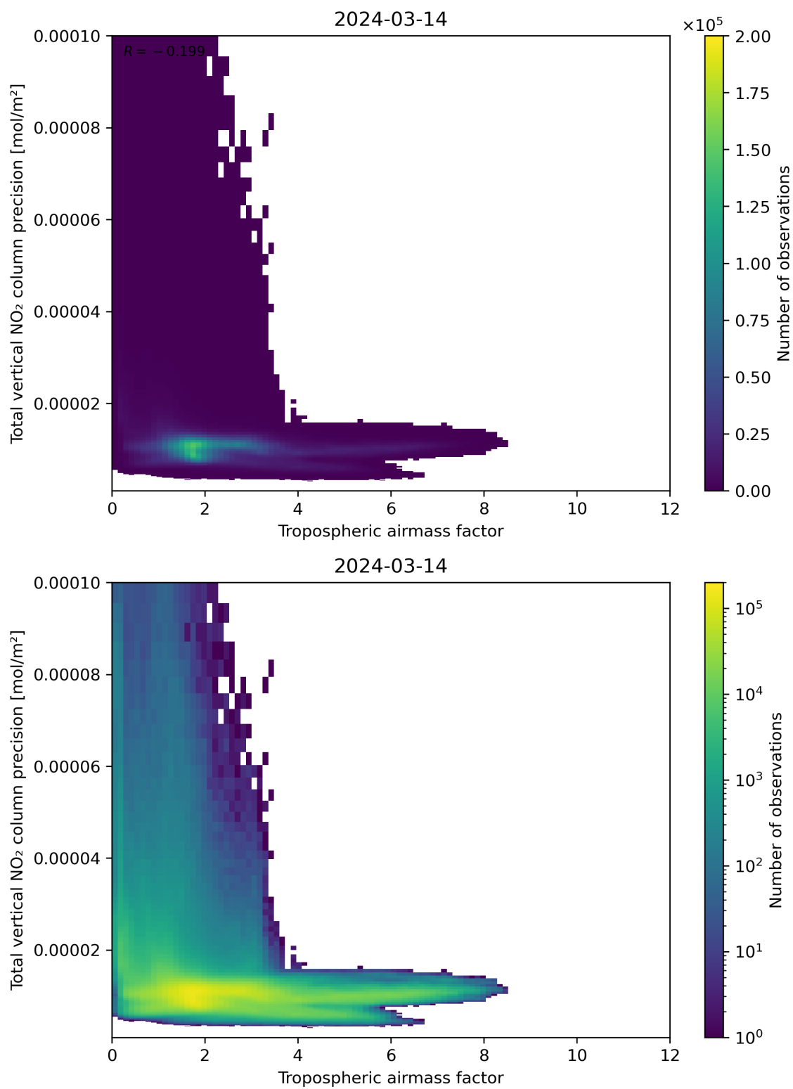
Figure 78: Scatter density plot of “Tropospheric air mass factor” against “Total vertical NO 2 column precision” for 2024-03-14 to 2024-03-15.
