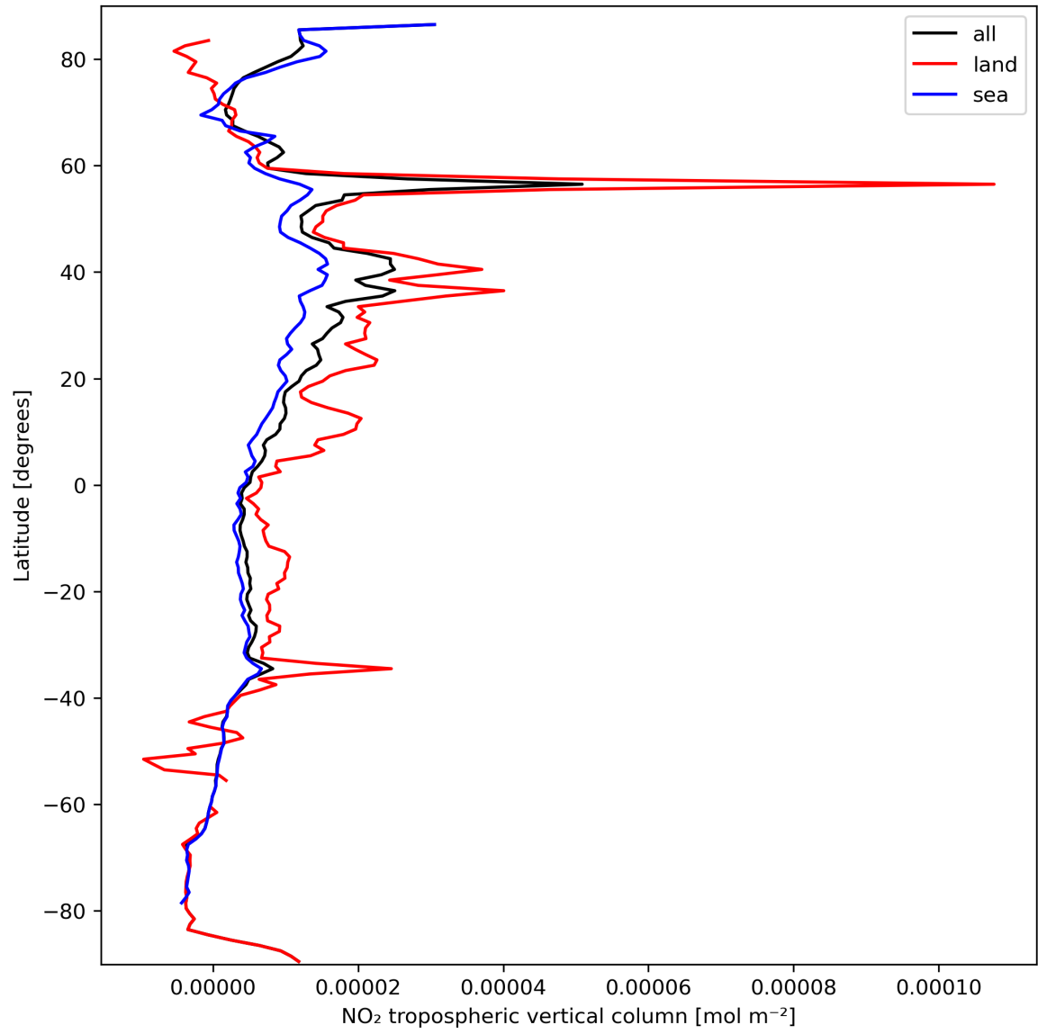
Figure 12: Zonal average of “NO 2 tropospheric vertical column” for 2024-03-14 to 2024-03-15.
