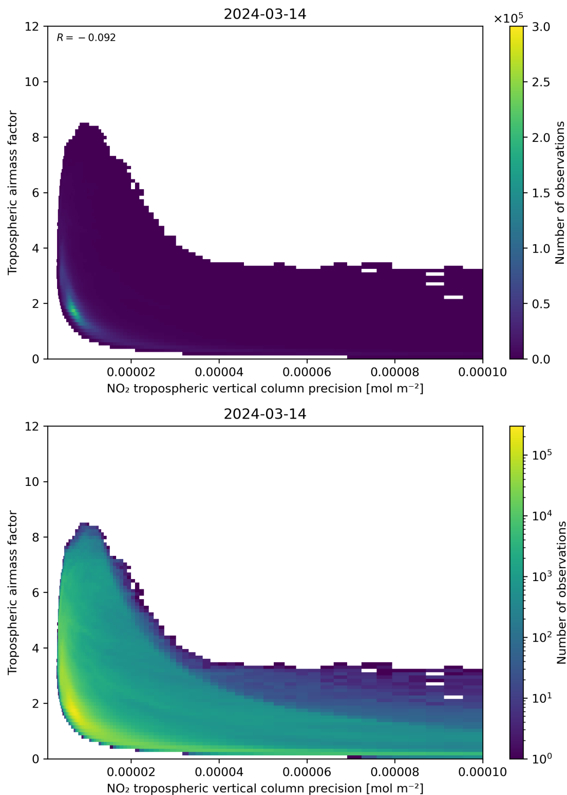
Figure 133: Scatter density plot of “NO 2 tropospheric vertical column precision” against “Tropospheric airmass factor” for 2024-03-14 to 2024-03-15.
