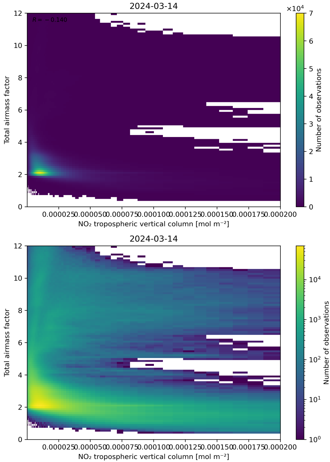
Figure 122: Scatter density plot of “NO 2 tropospheric vertical column” against “Total air mass factor” for 2024-03-14 to 2024-03-15.
