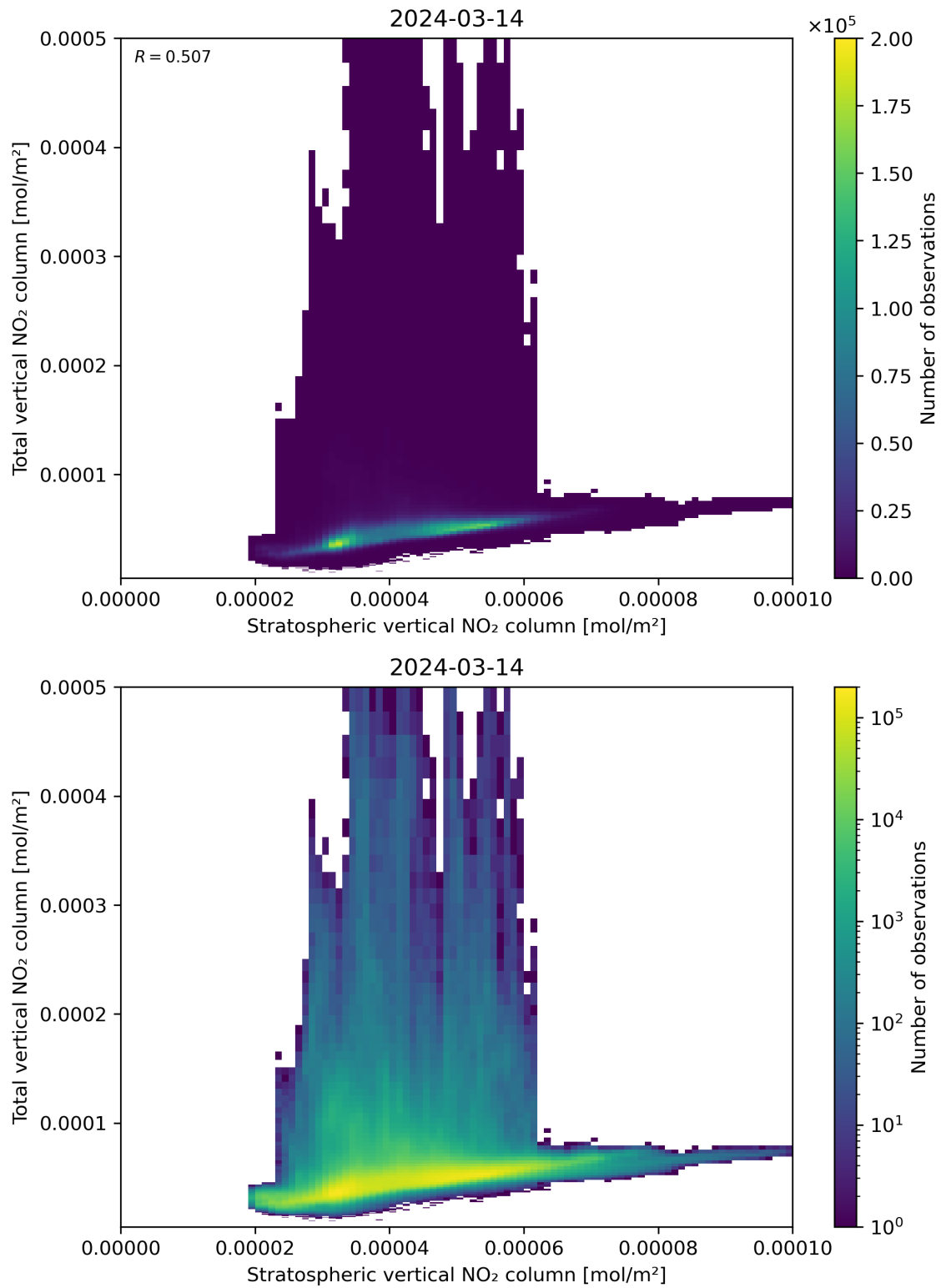
Figure 100: Scatter density plot of “Stratospheric vertical NO 2 column” against “Total vertical NO 2 column” for 2024-03-14 to 2024-03-15.
