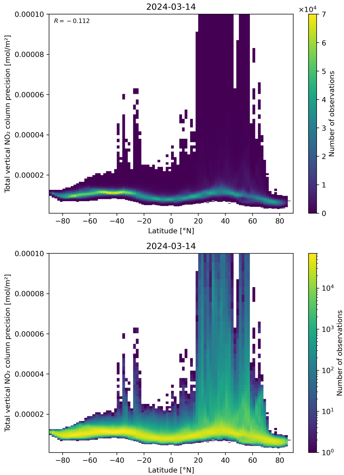
Figure 91: Scatter density plot of “Latitude” against “Total vertical NO 2 column precision” for 2024-03-14 to 2024-03-15.
