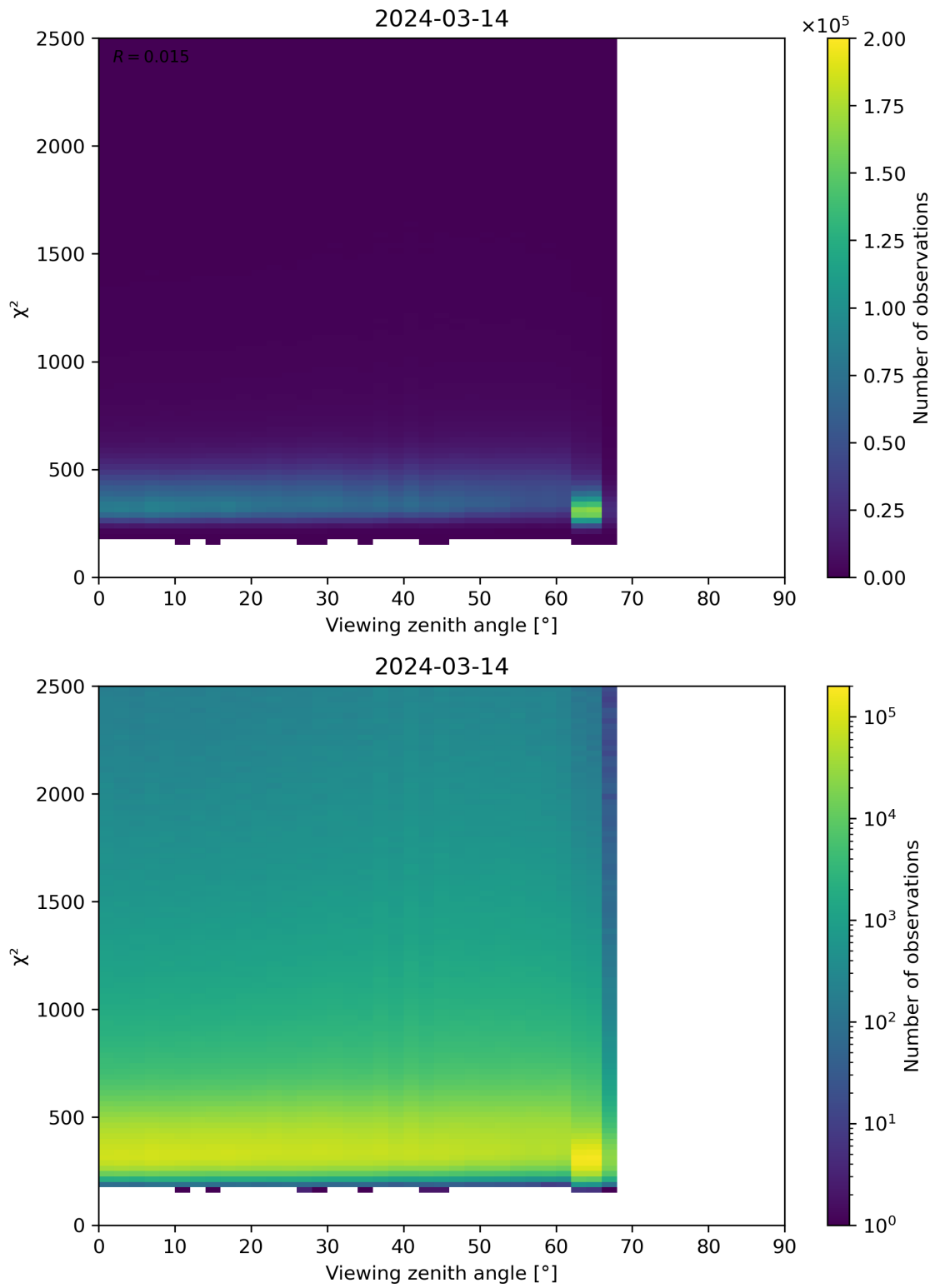
Figure 162: Scatter density plot of “Viewing zenith angle” against “ \chi^2 ” for 2024-03-14 to 2024-03-15.
