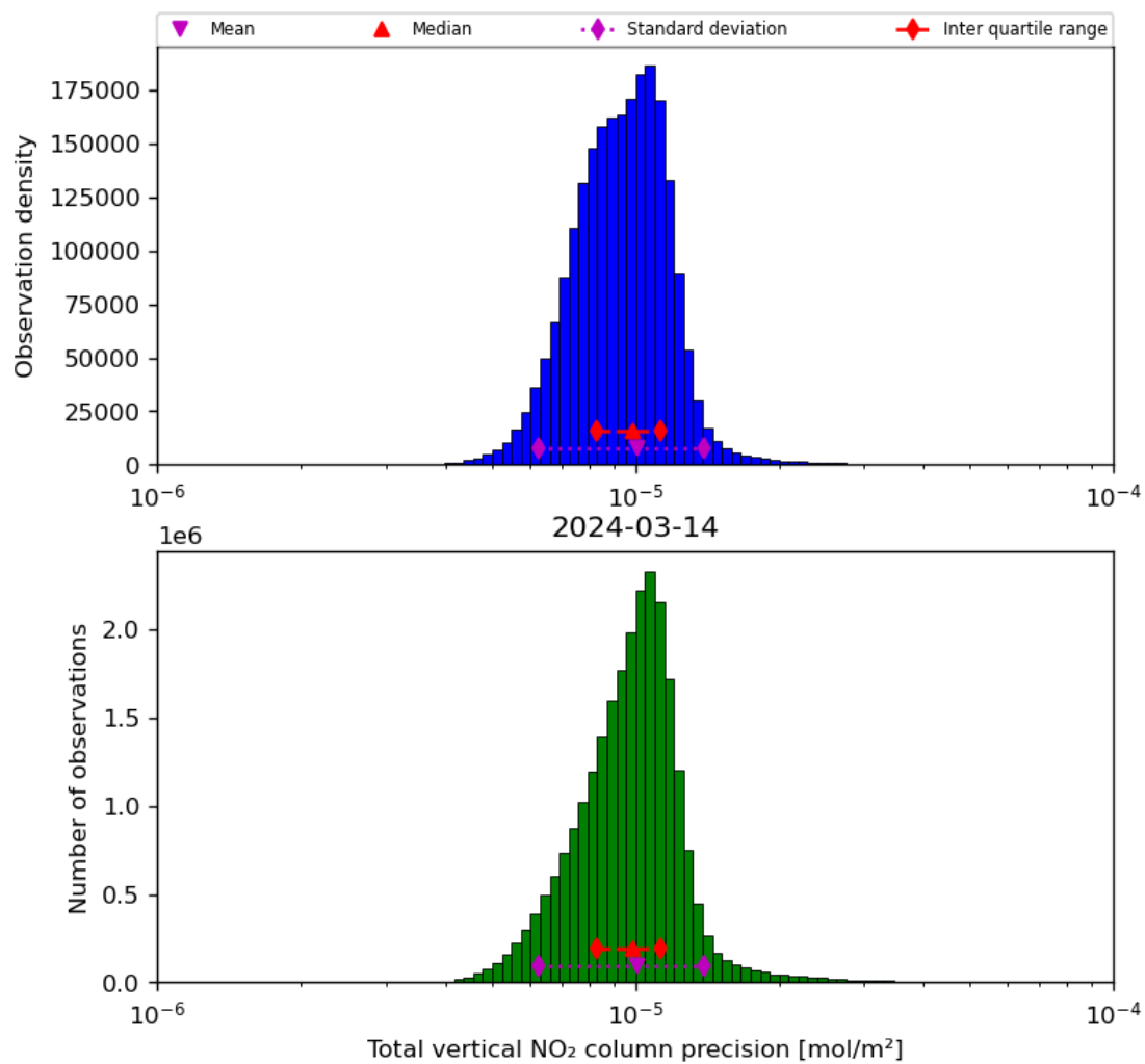
Figure 39: Histogram of “Total vertical NO 2 column precision” for 2024-03-14 to 2024-03-15
