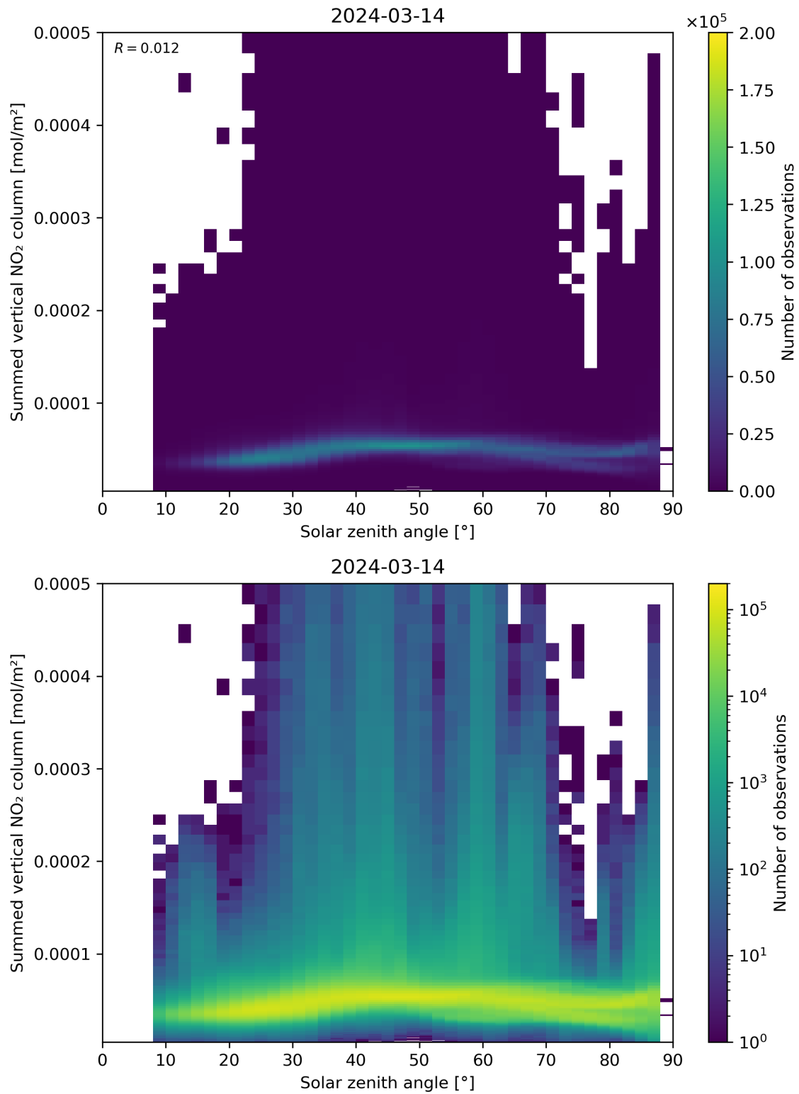
Figure 151: Scatter density plot of “Solar zenith angle” against “Summed vertical NO 2 column” for 2024-03-14 to 2024-03-15.
