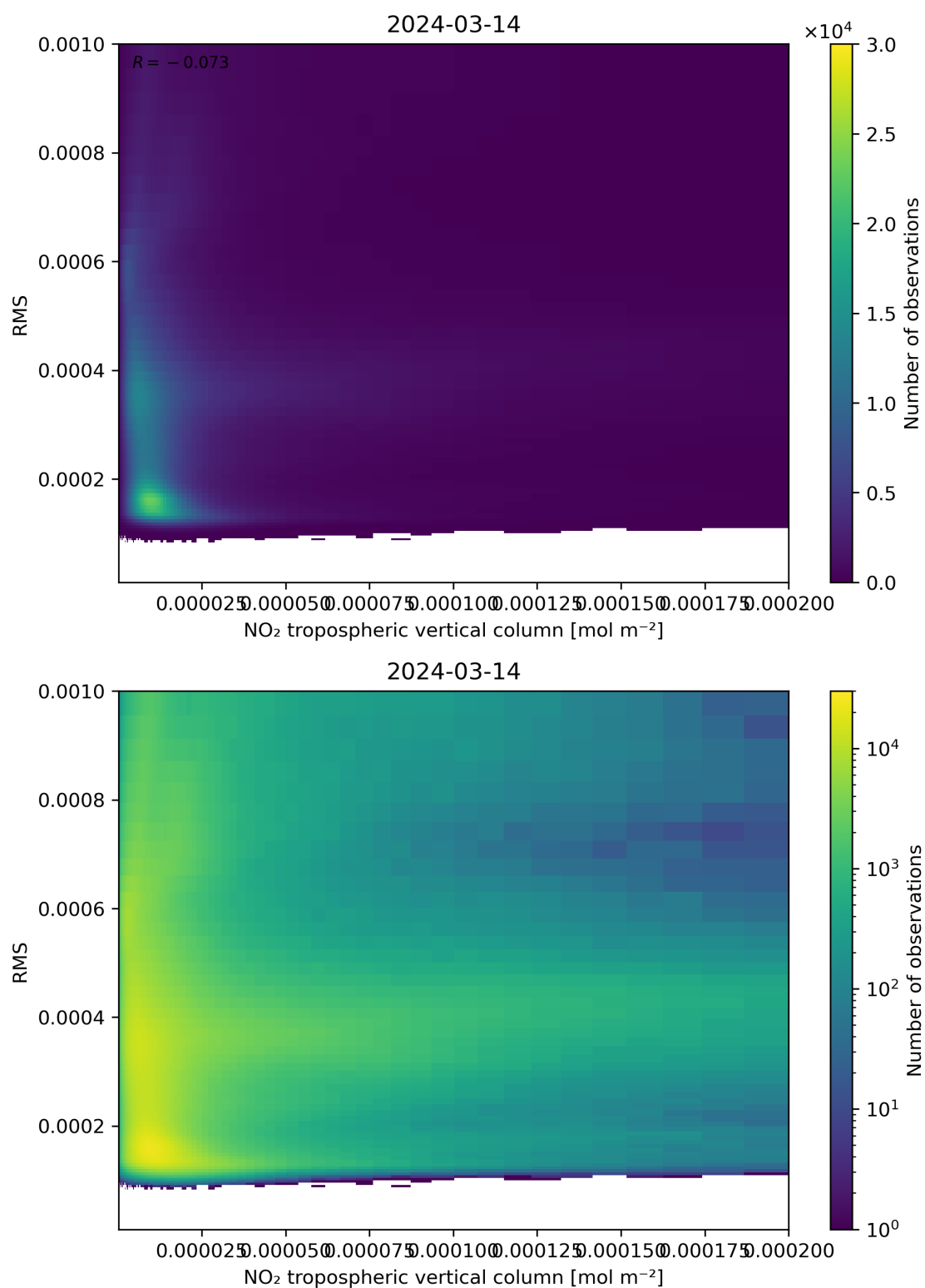
Figure 142: Scatter density plot of “NO 2 tropospheric vertical column” against “RMS” for 2024-03-14 to 2024-03-15.
