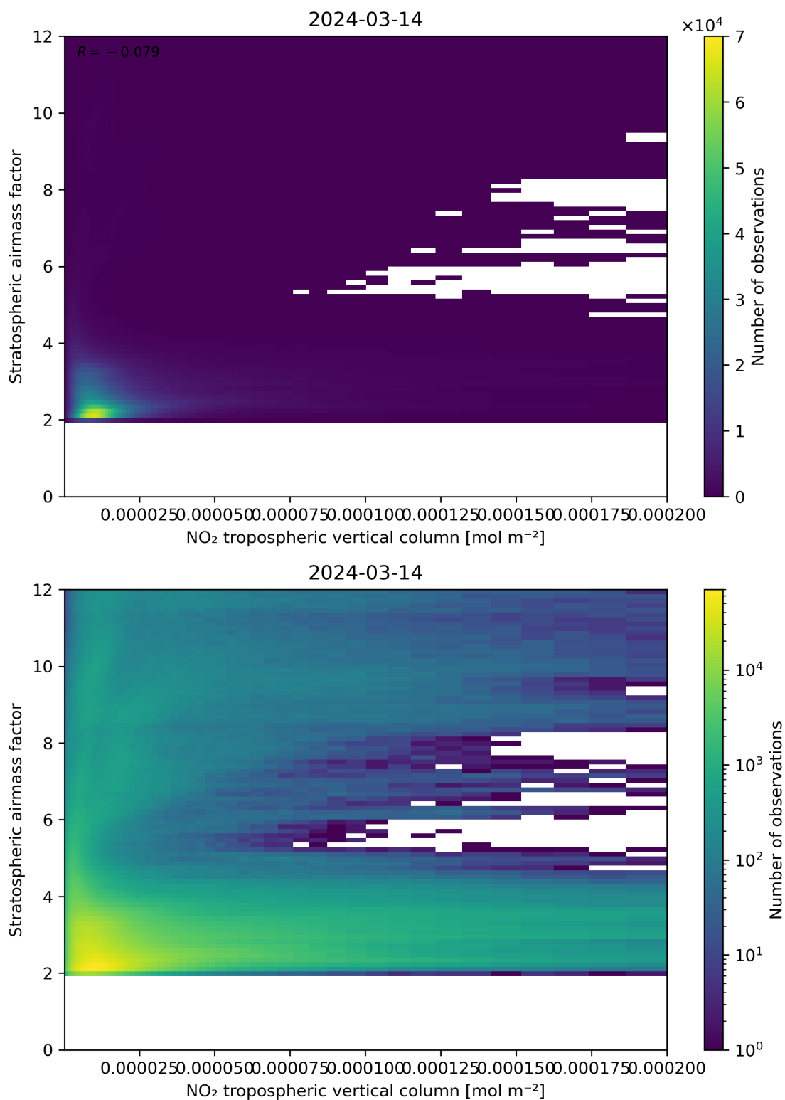
Figure 121: Scatter density plot of “NO 2 tropospheric vertical column” against “Stratospheric air mass factor” for 2024-03-14 to 2024-03-15.
