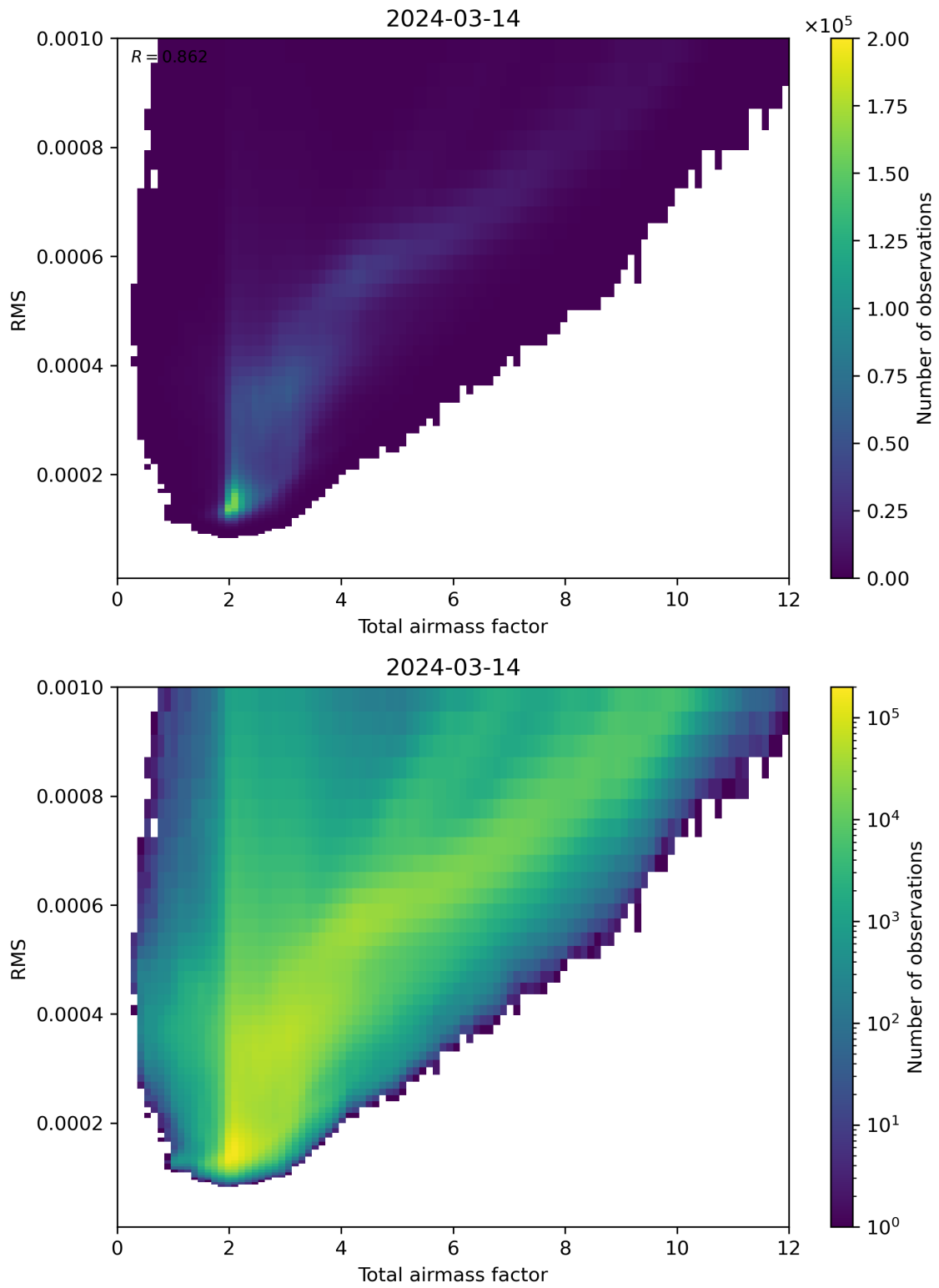
Figure 69: Scatter density plot of “Total airmass factor” against “RMS” for 2024-03-14 to 2024-03-15.
