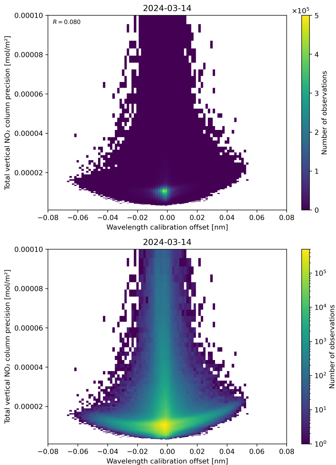
Figure 180: Scatter density plot of “Wavelength calibration offset” against “Total vertical NO 2 column precision” for 2024-03-14 to 2024-03-15.
