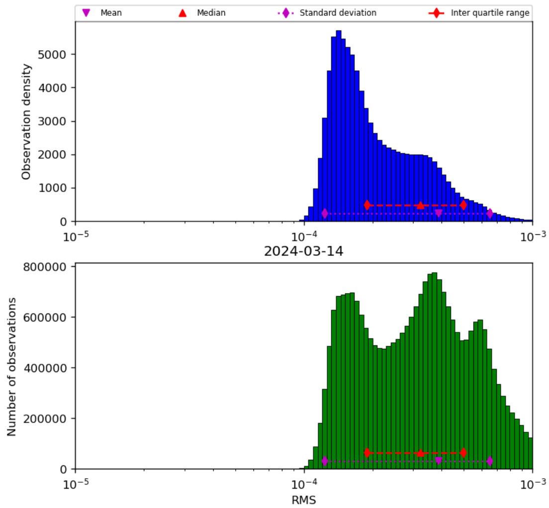
Figure 43: Histogram of “RMS” for 2024-03-14 to 2024-03-15
