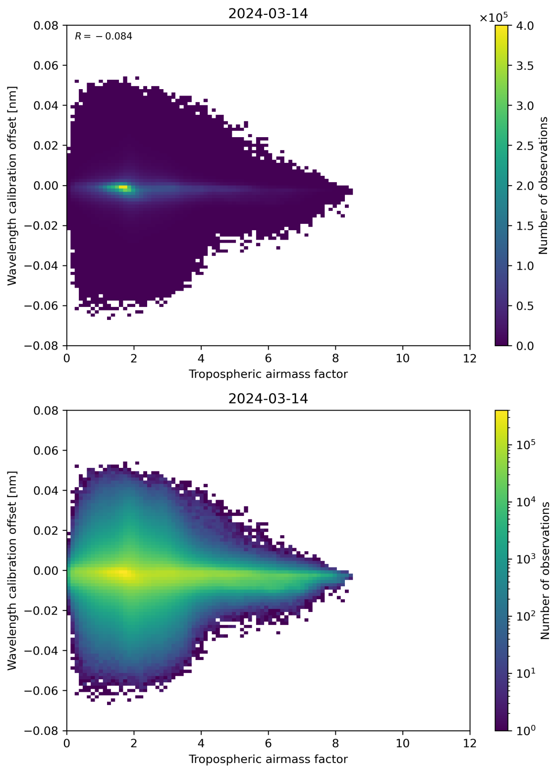
Figure 80: Scatter density plot of “Tropospheric airmass factor” against “Wavelength calibration offset” for 2024-03-14 to 2024-03-15.
