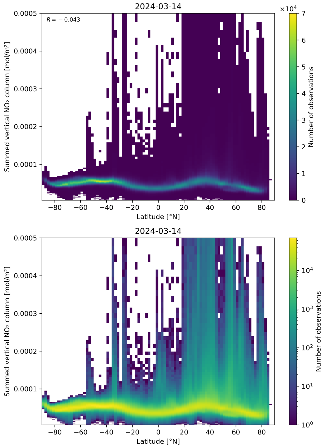
Figure 88: Scatter density plot of “Latitude” against “Summed vertical NO 2 column” for 2024-03-14 to 2024-03-15.
