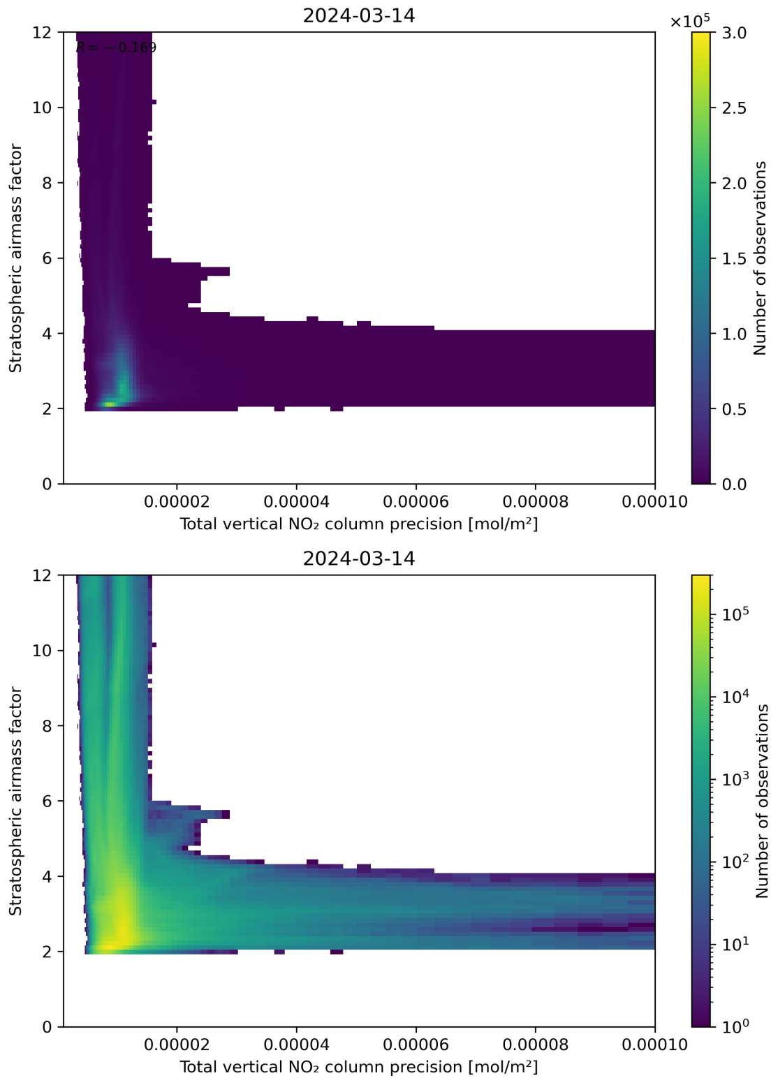
Figure 115: Scatter density plot of “Total vertical NO 2 column precision” against “Stratospheric airmass factor” for 2024-03-14 to 2024-03-15.
