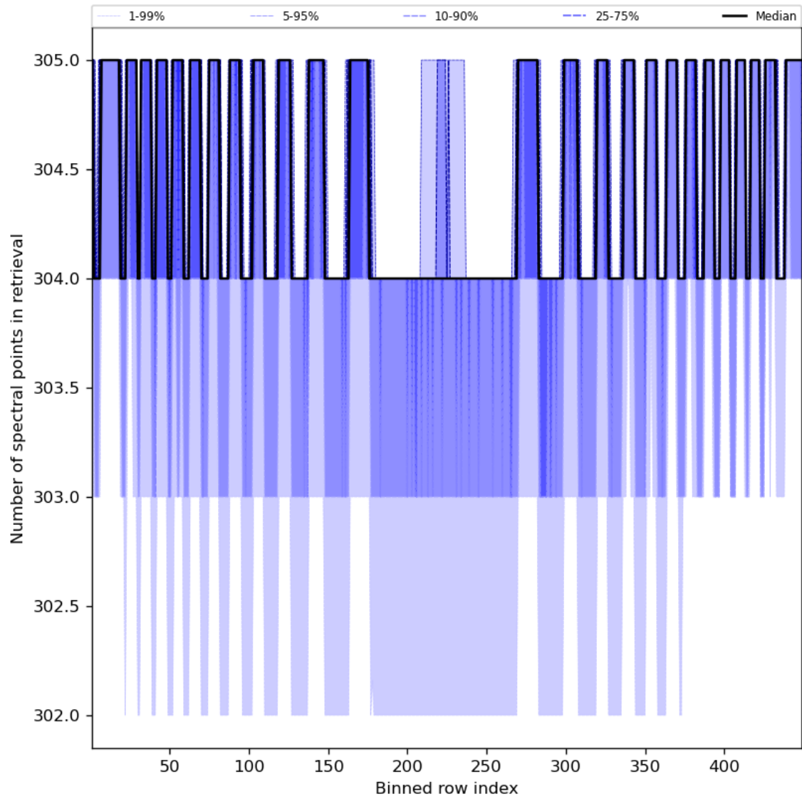
Figure 50: Along track statistics of “Number of spectral points in retrieval” for 2024-03-14 to 2024-03-15
