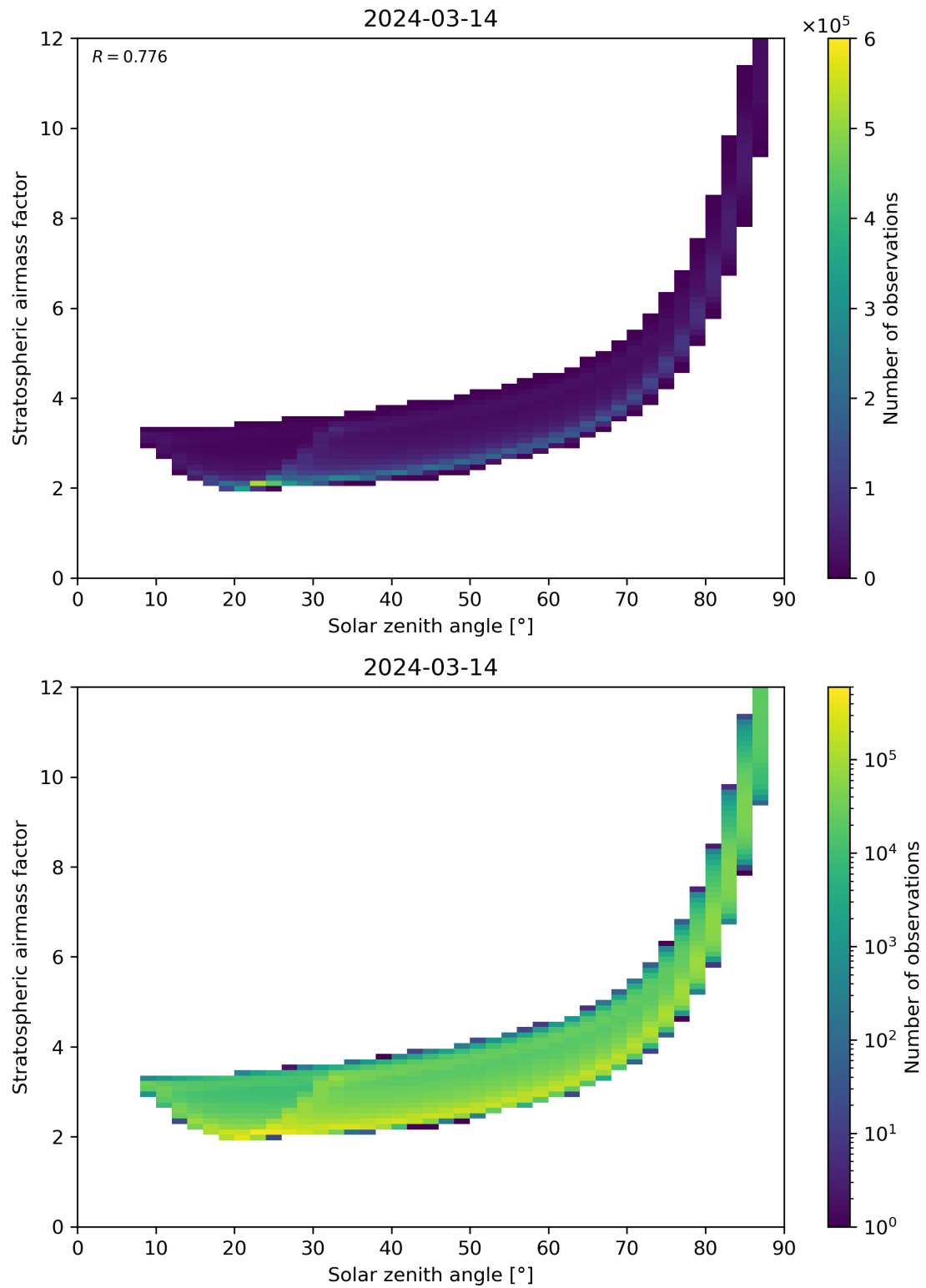
Figure 145: Scatter density plot of “Solar zenith angle” against “Stratospheric airmass factor” for 2024-03-14 to 2024-03-15.
