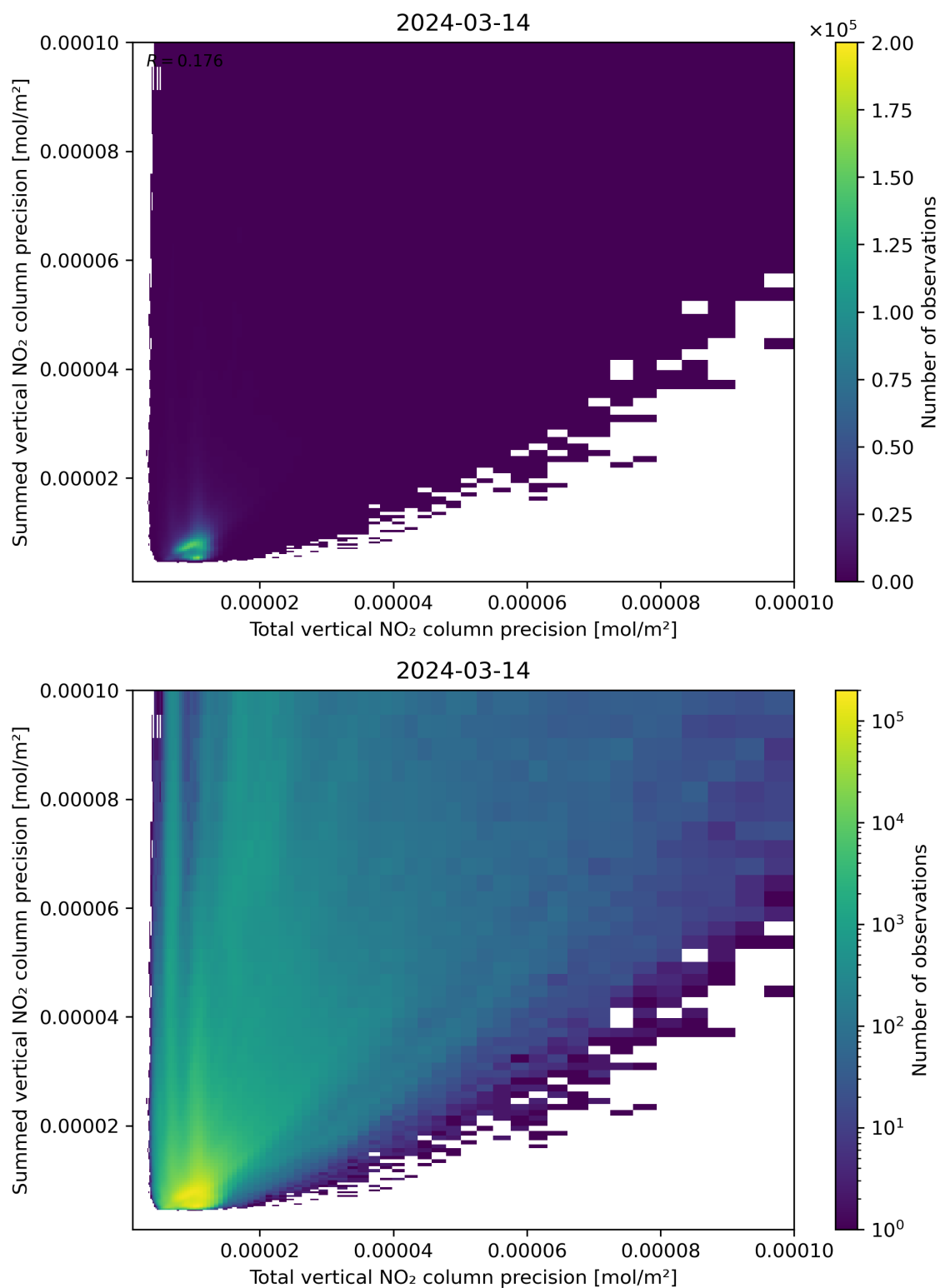
Figure 118: Scatter density plot of “Total vertical NO 2 column precision” against “Summed vertical NO 2 column precision” for 2024-03-14 to 2024-03-15.
