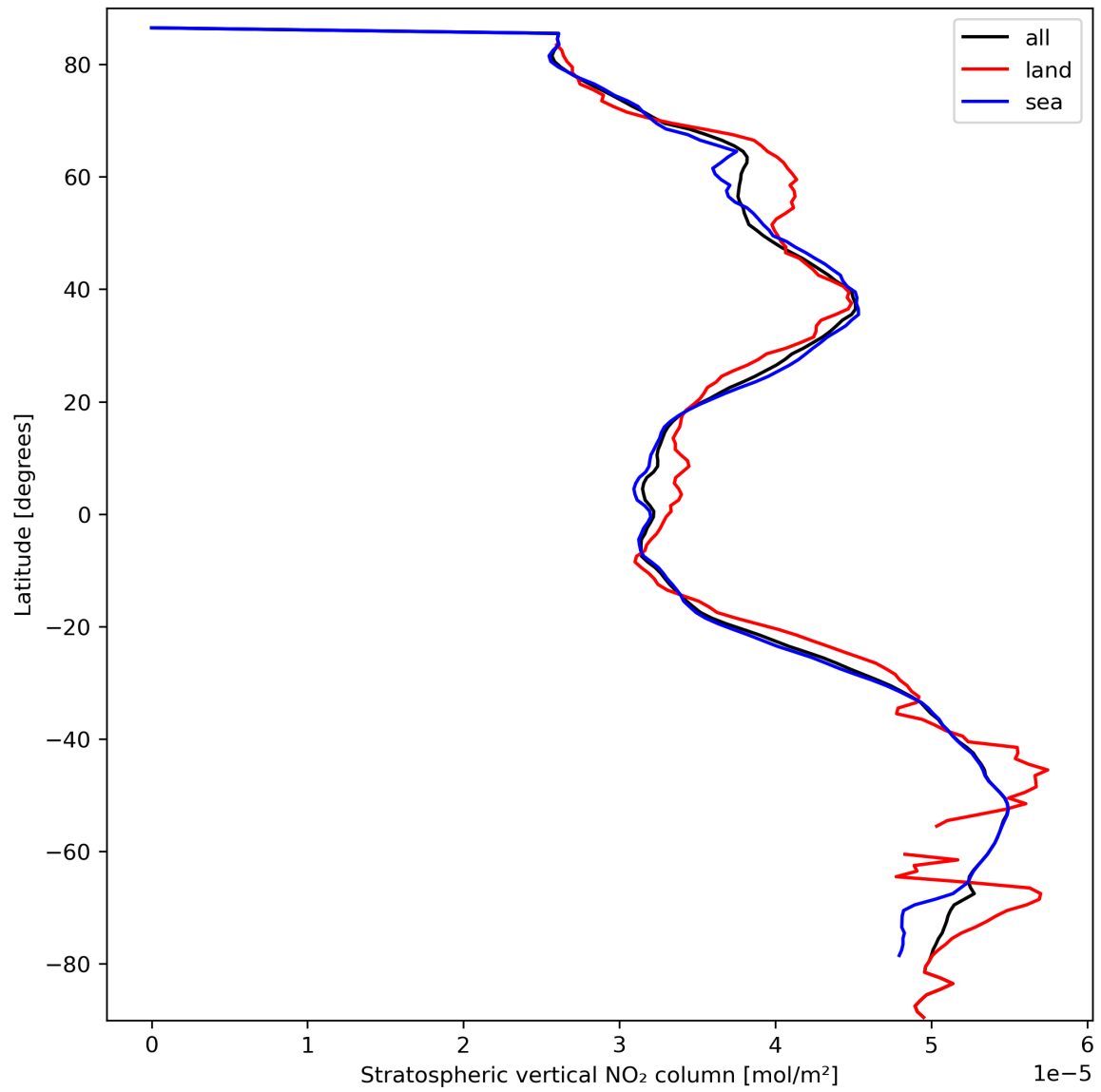
Figure 19: Zonal average of “Stratospheric vertical NO 2 column” for 2024-03-14 to 2024-03-15.
