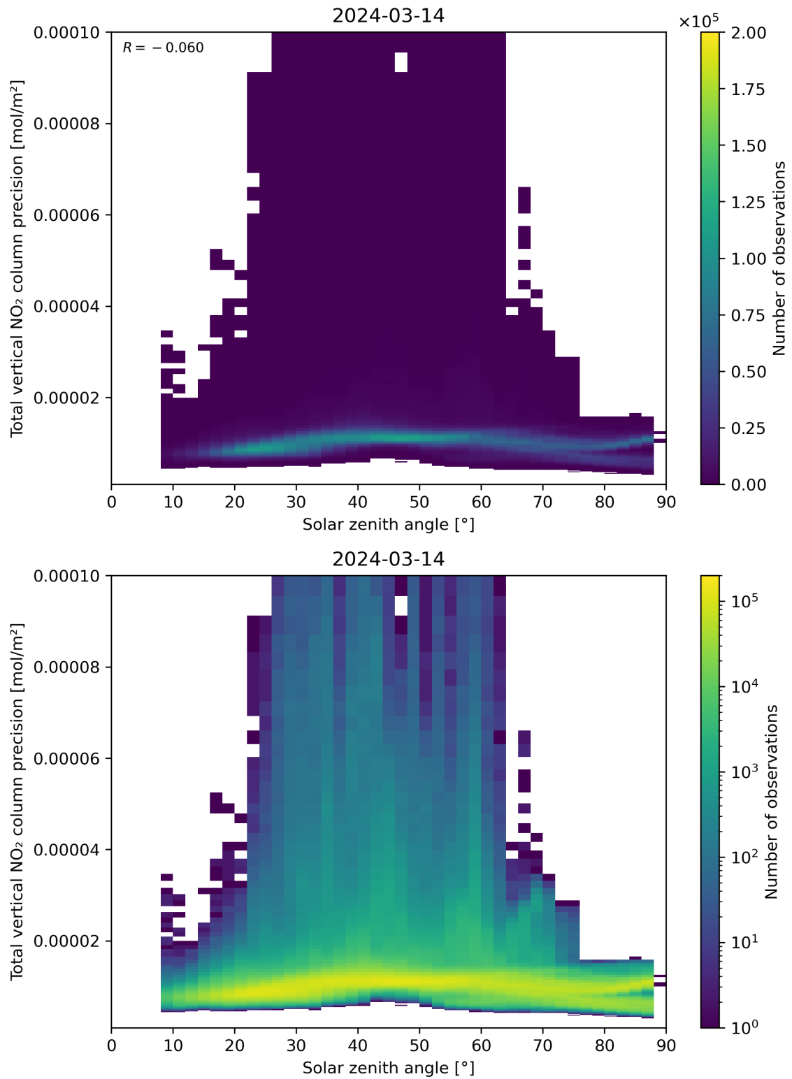
Figure 154: Scatter density plot of “Solar zenith angle” against “Total vertical NO 2 column precision” for 2024-03-14 to 2024-03-15.
