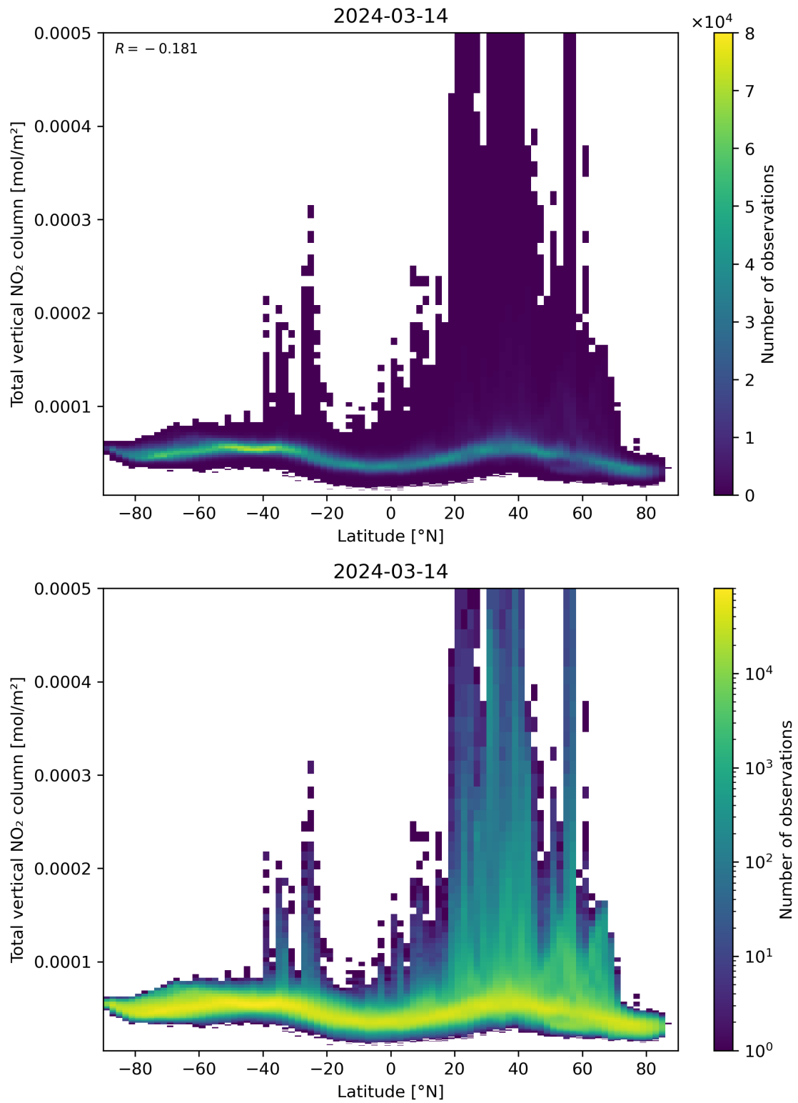
Figure 90: Scatter density plot of “Latitude” against “Total vertical NO 2 column” for 2024-03-14 to 2024-03-15.
