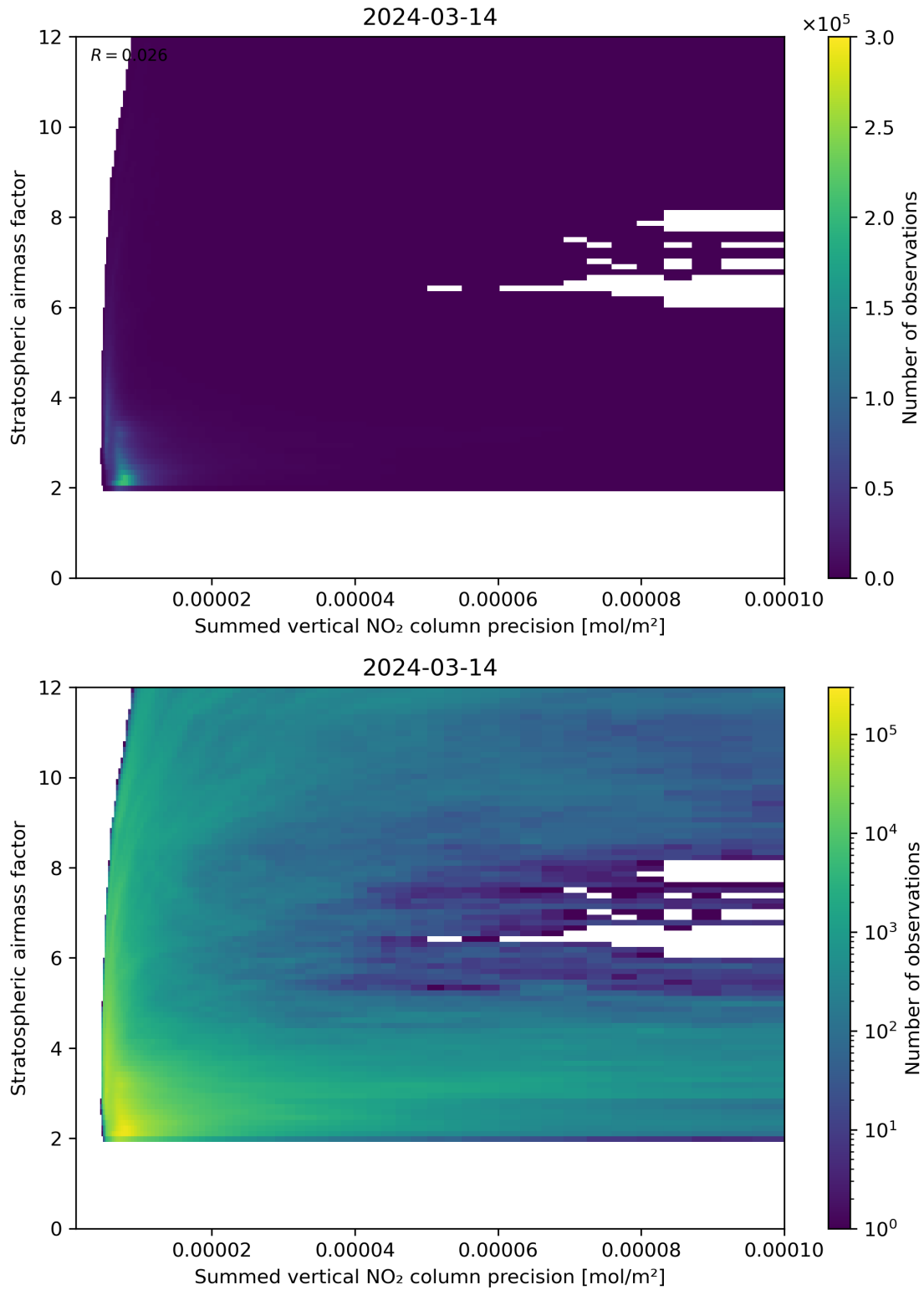
Figure 106: Scatter density plot of “Summed vertical NO 2 column precision” against “Stratospheric airmass factor” for 2024-03-14 to 2024-03-15.
