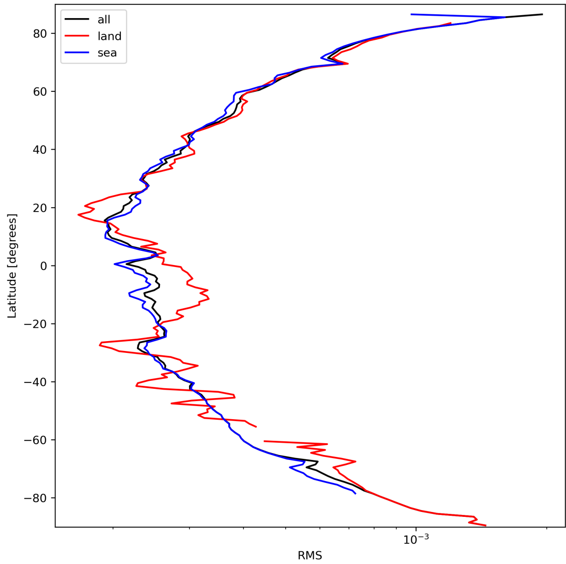
Figure 26: Zonal average of “RMS” for 2024-03-14 to 2024-03-15.
