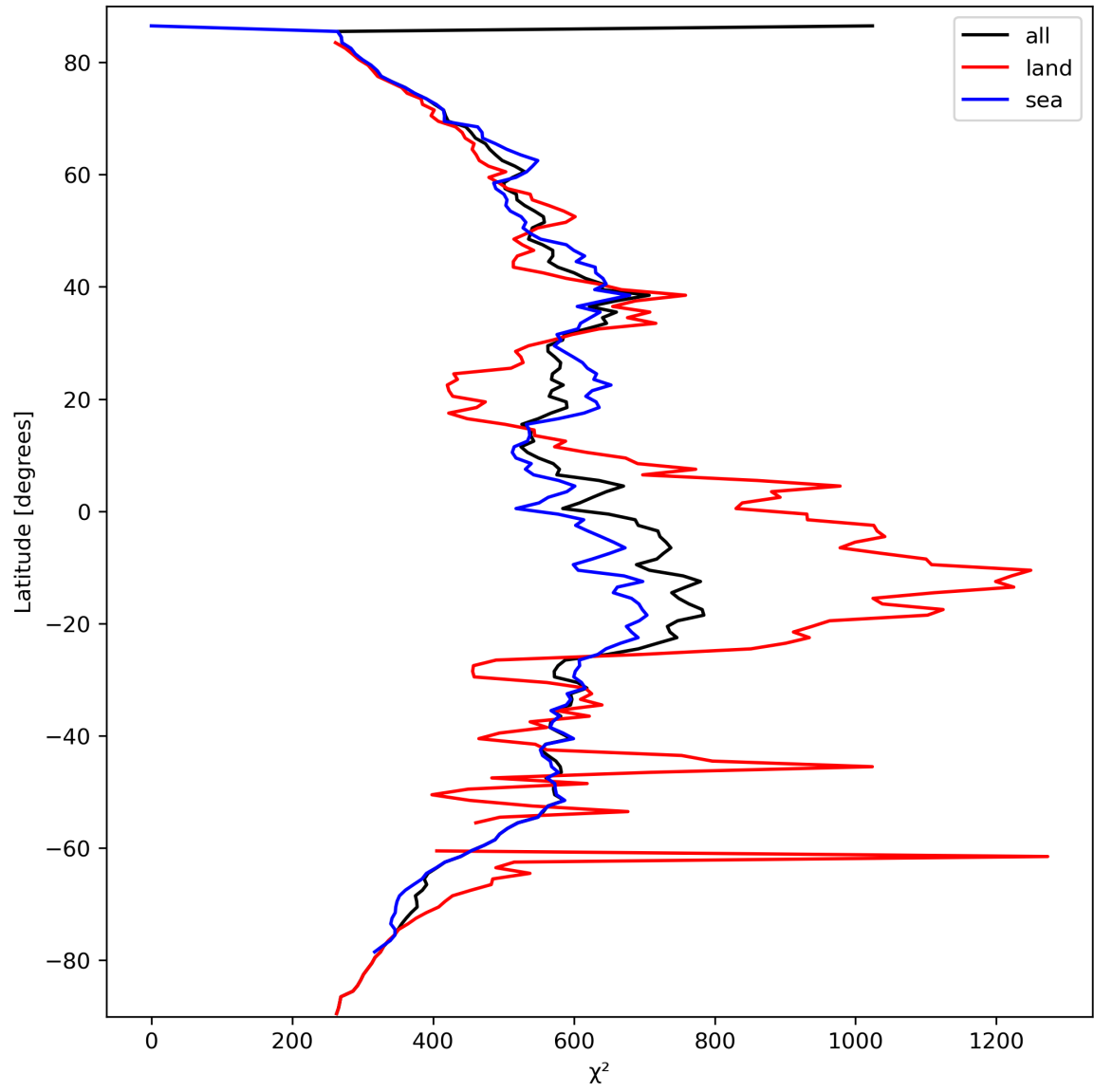
Figure 25: Zonal average of “ \chi^2 ” for 2024-03-14 to 2024-03-15.
