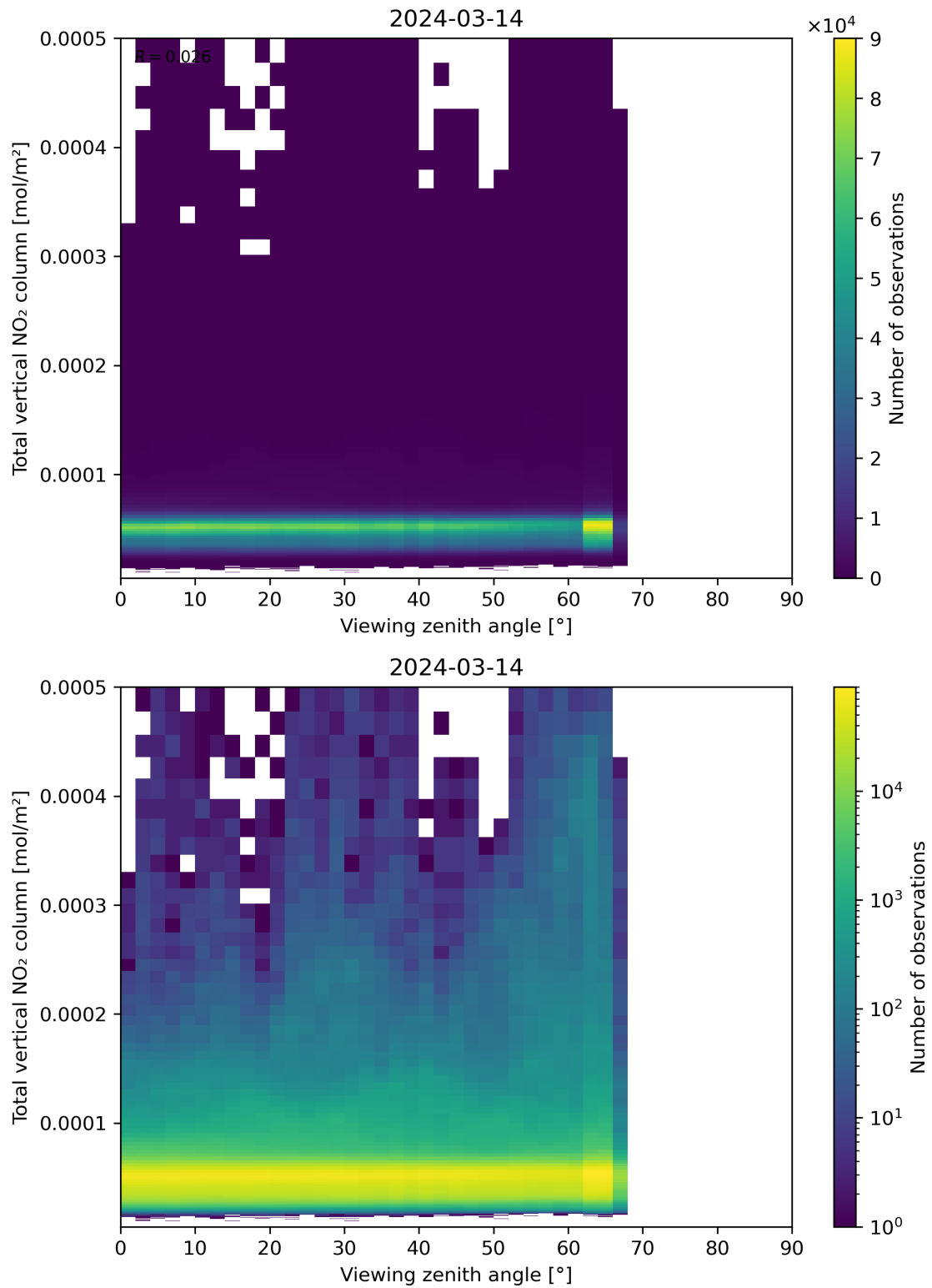
Figure 167: Scatter density plot of “Viewing zenith angle” against “Total vertical NO 2 column” for 2024-03-14 to 2024-03-15.
