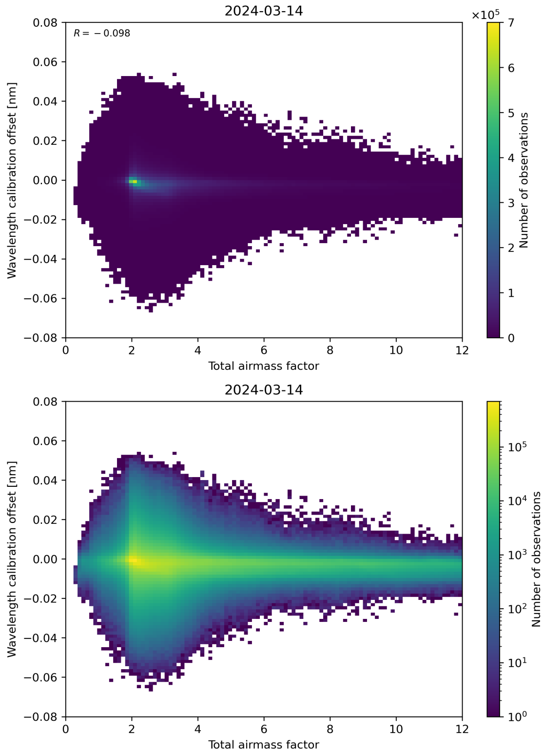
Figure 70: Scatter density plot of “Total airmass factor” against “Wavelength calibration offset” for 2024-03-14 to 2024-03-15.
