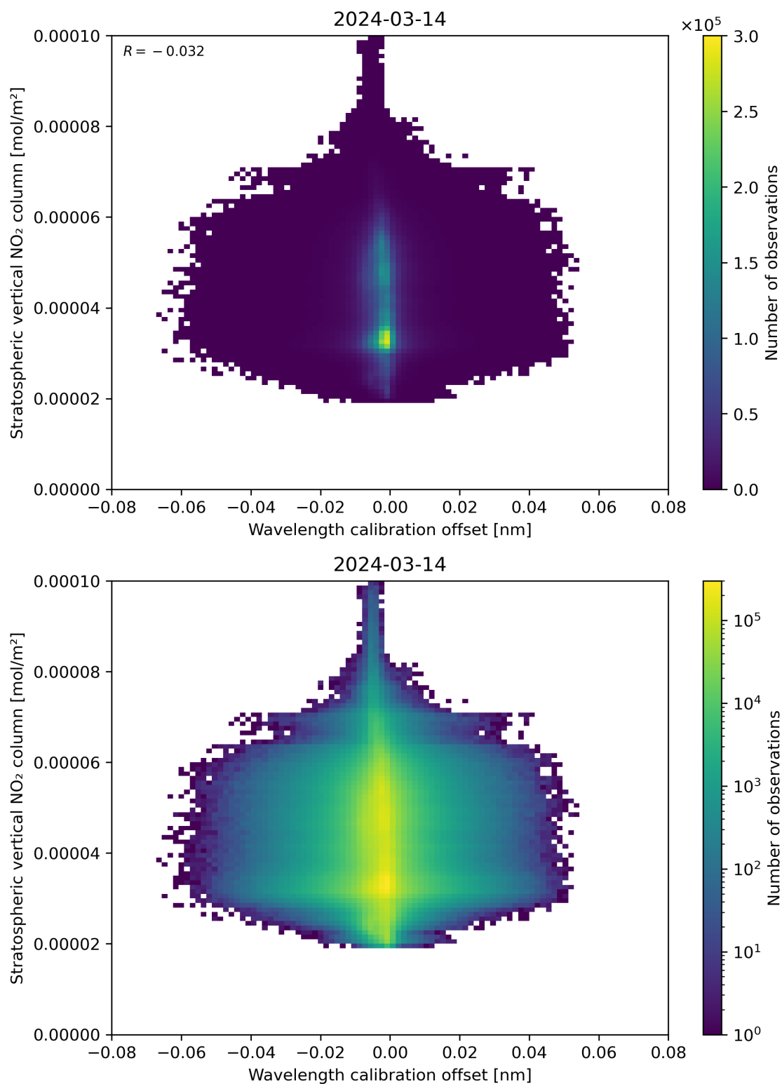
Figure 176: Scatter density plot of “Wavelength calibration offset” against “Stratospheric vertical NO 2 column” for 2024-03-14 to 2024-03-15.
