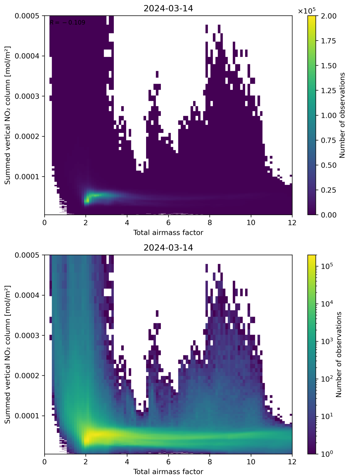
Figure 65: Scatter density plot of “Total airmass factor” against “Summed vertical NO 2 column” for 2024-03-14 to 2024-03-15.
