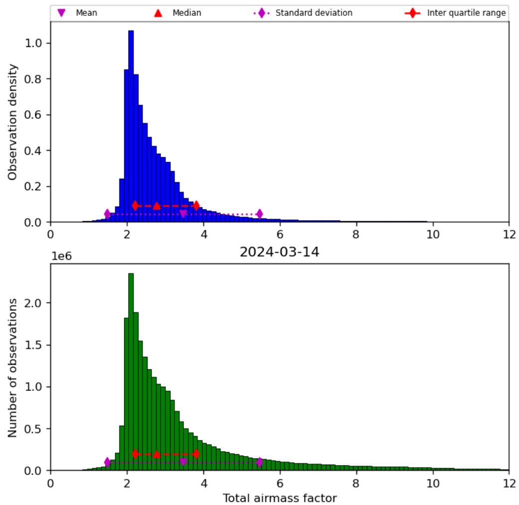
Figure 32: Histogram of “Total airmass factor” for 2024-03-14 to 2024-03-15
