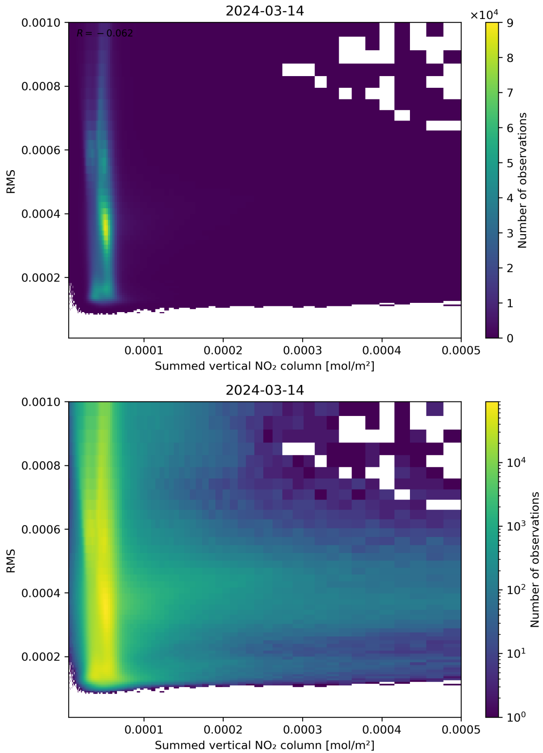
Figure 109: Scatter density plot of “Summed vertical NO 2 column” against “RMS” for 2024-03-14 to 2024-03-15.
