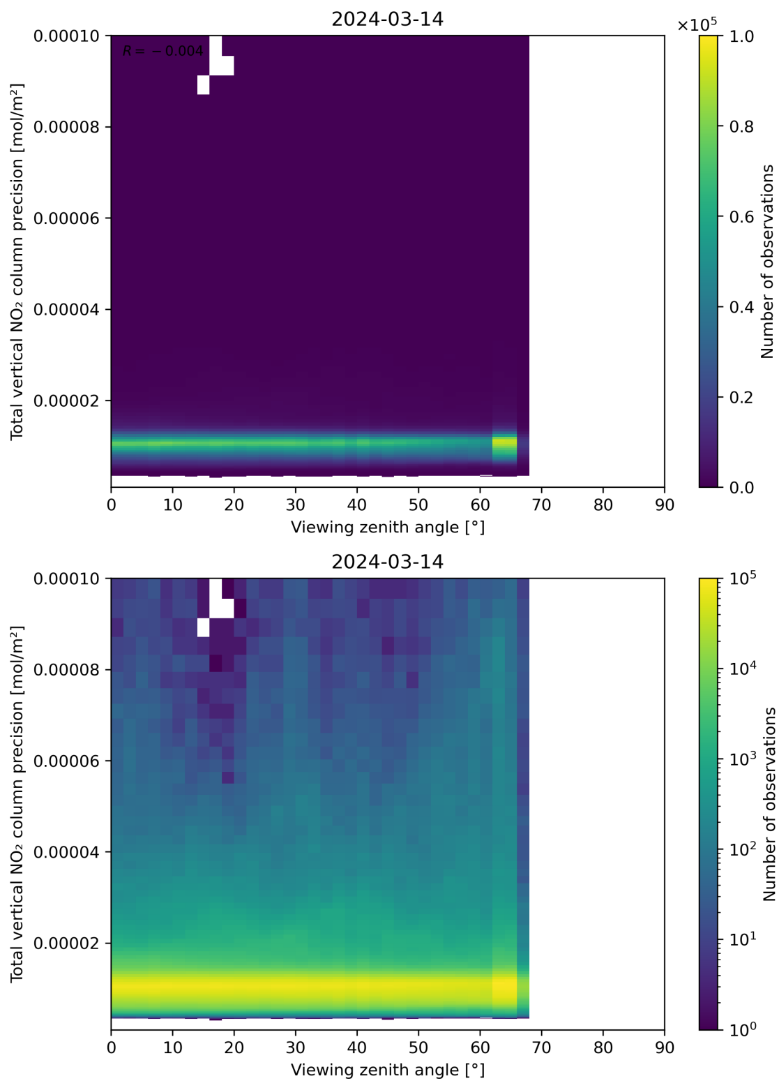
Figure 168: Scatter density plot of “Viewing zenith angle” against “Total vertical NO 2 column precision” for 2024-03-14 to 2024-03-15.
