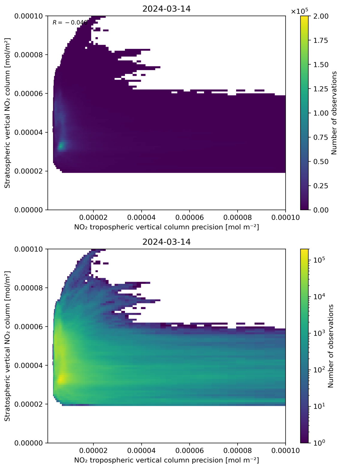
Figure 135: Scatter density plot of “NO 2 tropospheric vertical column precision” against “Stratospheric vertical NO 2 column” for 2024-03-14 to 2024-03-15.
