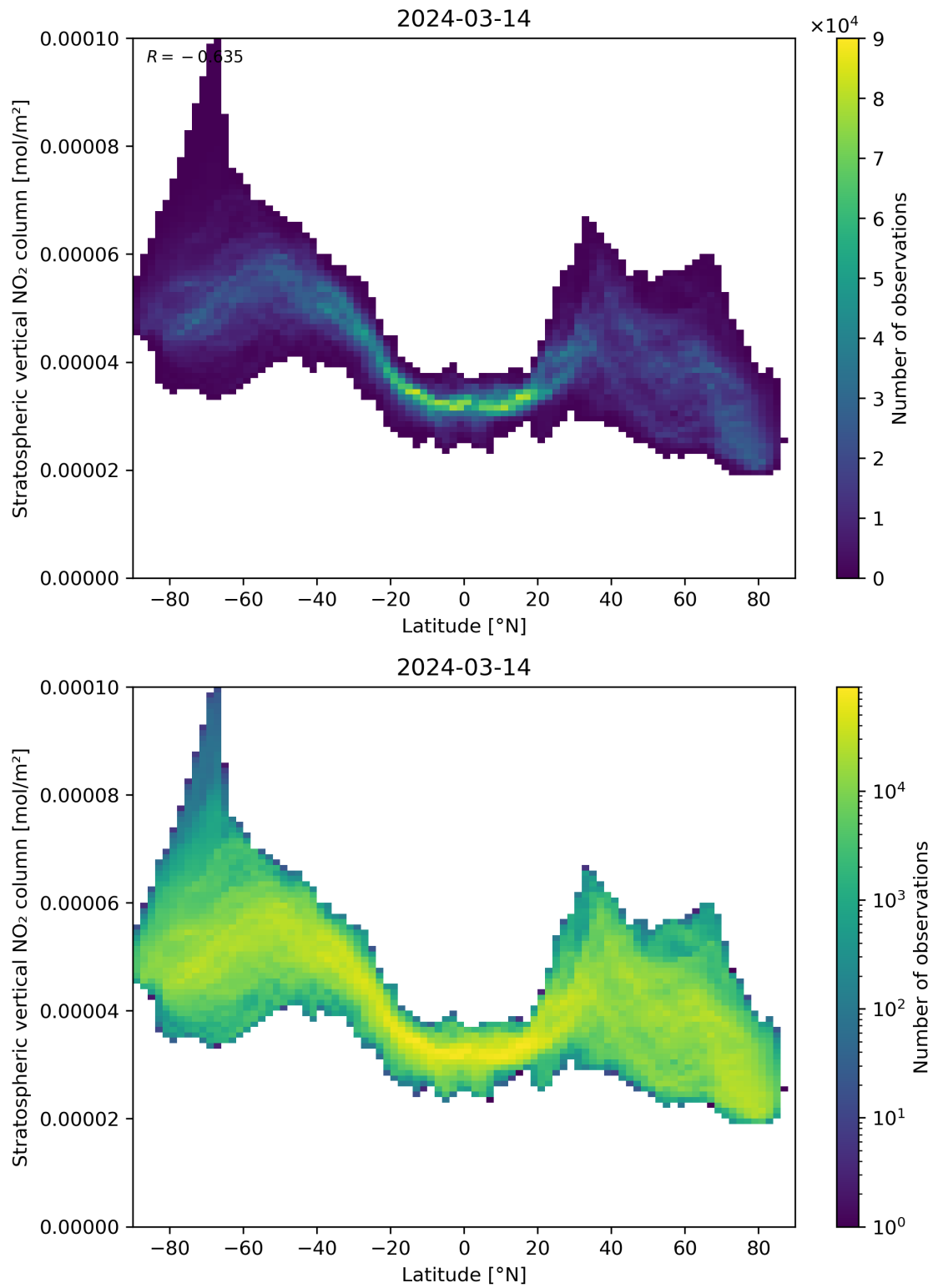
Figure 87: Scatter density plot of “Latitude” against “Stratospheric vertical NO 2 column” for 2024-03-14 to 2024-03-15.
