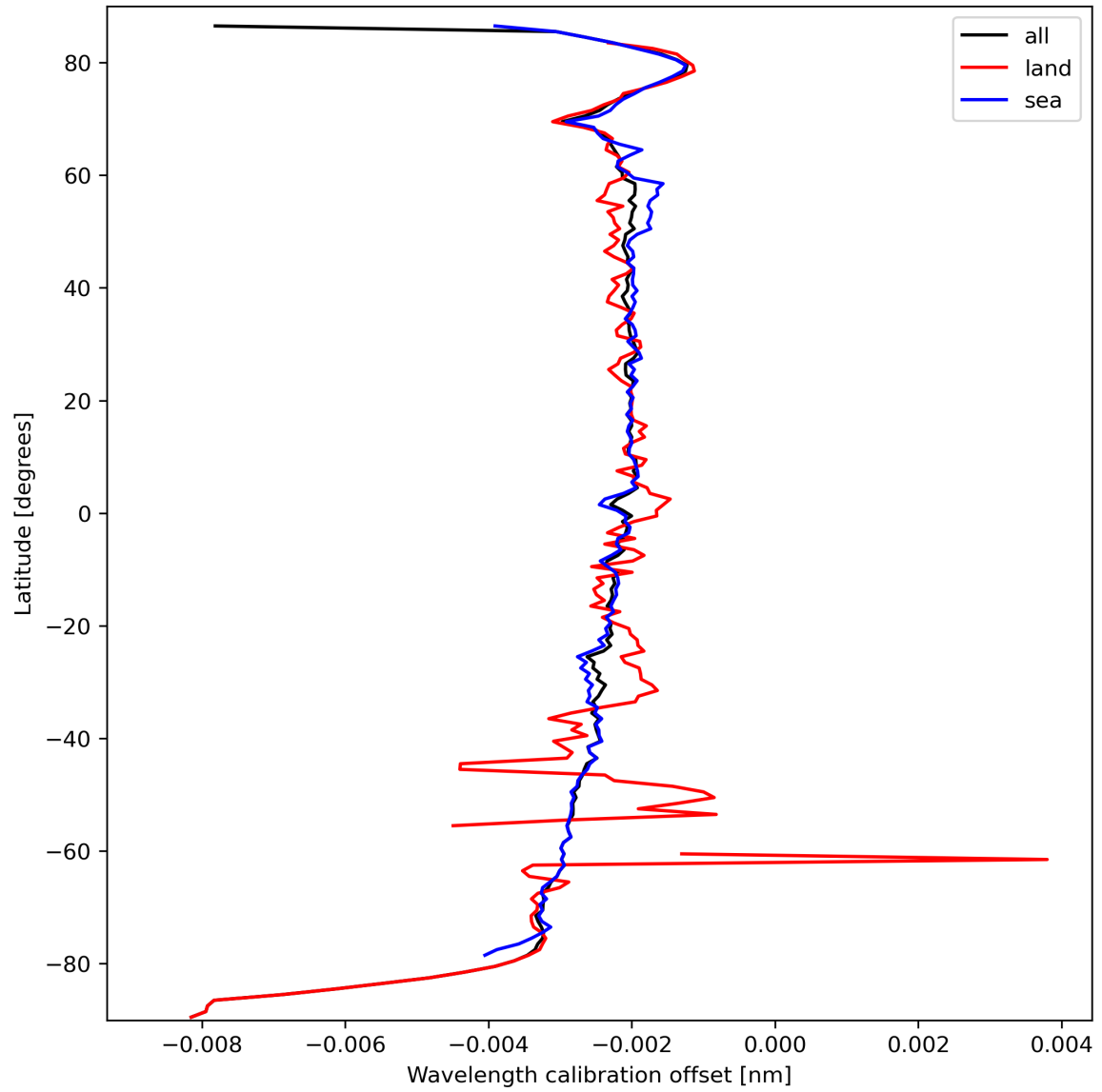
Figure 18: Zonal average of “Wavelength calibration offset” for 2024-03-14 to 2024-03-15.
