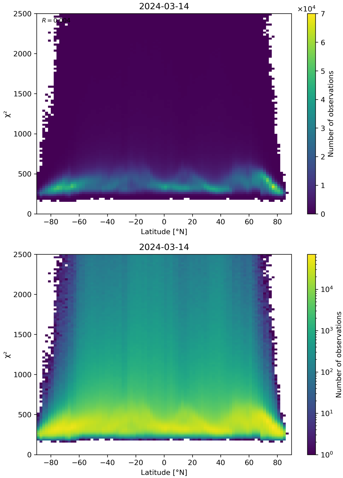
Figure 86: Scatter density plot of “Latitude” against “ \chi^2 ” for 2024-03-14 to 2024-03-15.
