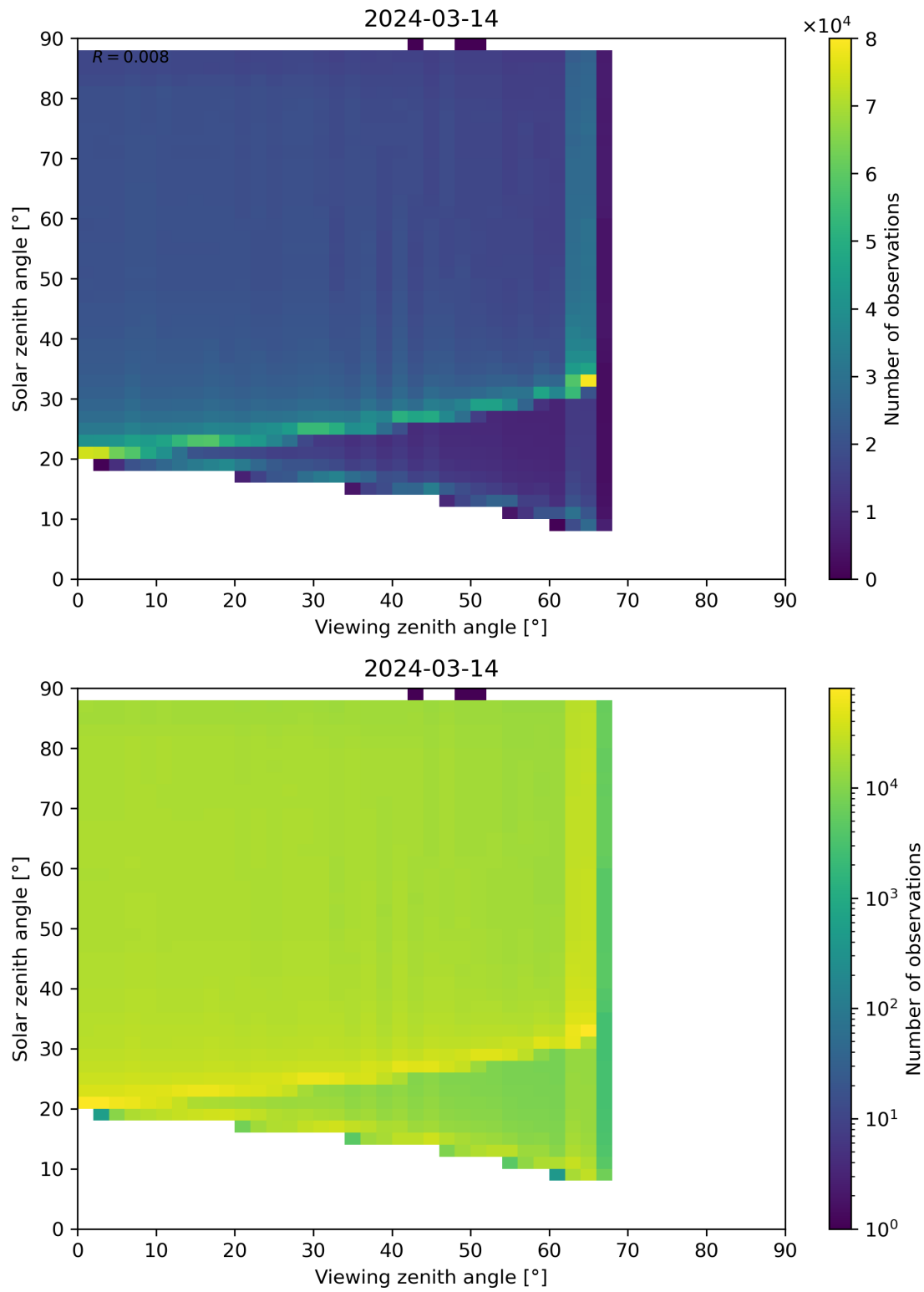
Figure 172: Scatter density plot of “Viewing zenith angle” against “Solar zenith angle” for 2024-03-14 to 2024-03-15.
