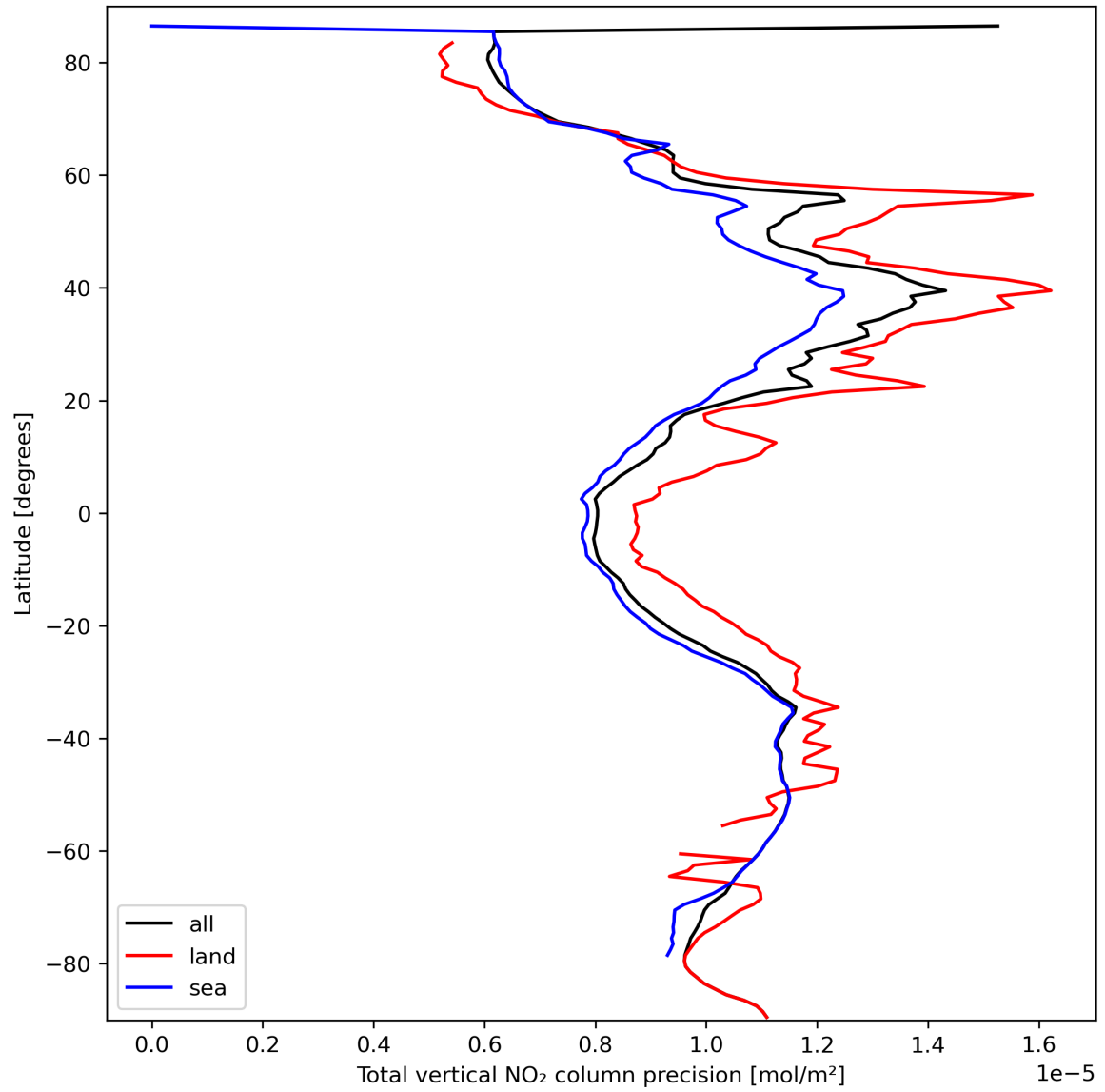
Figure 22: Zonal average of “Total vertical NO 2 column precision” for 2024-03-14 to 2024-03-15.
