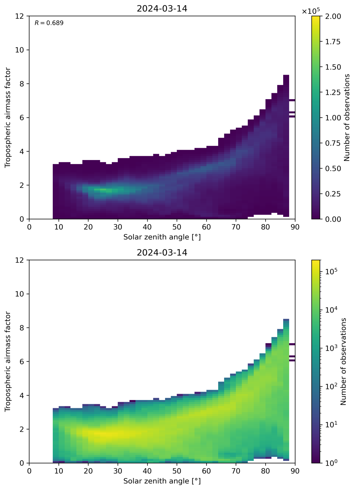
Figure 147: Scatter density plot of “Solar zenith angle” against “Tropospheric airmass factor” for 2024-03-14 to 2024-03-15.
