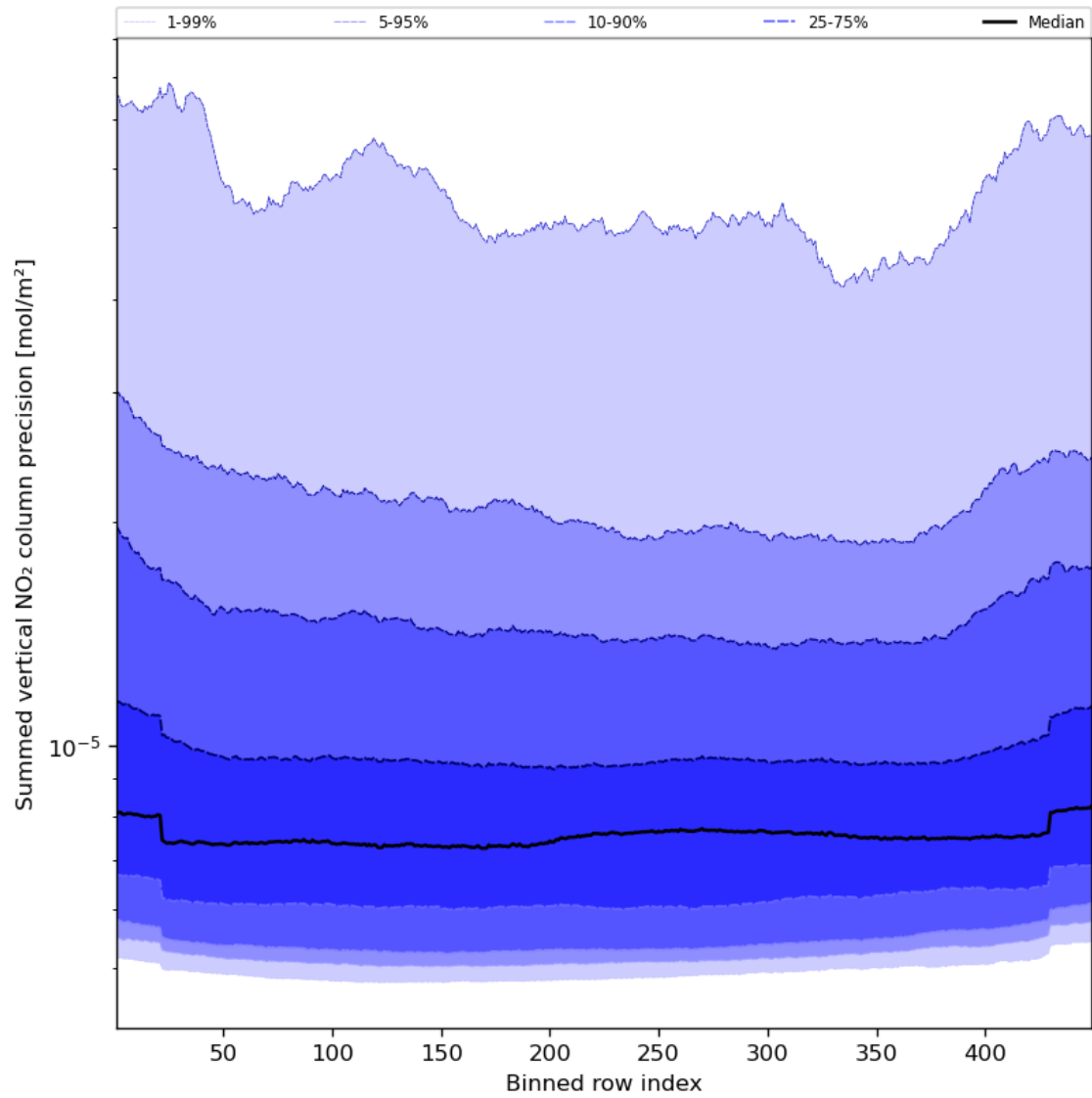
Figure 58: Along track statistics of “Summed vertical NO 2 column precision” for 2024-03-14 to 2024-03-15
