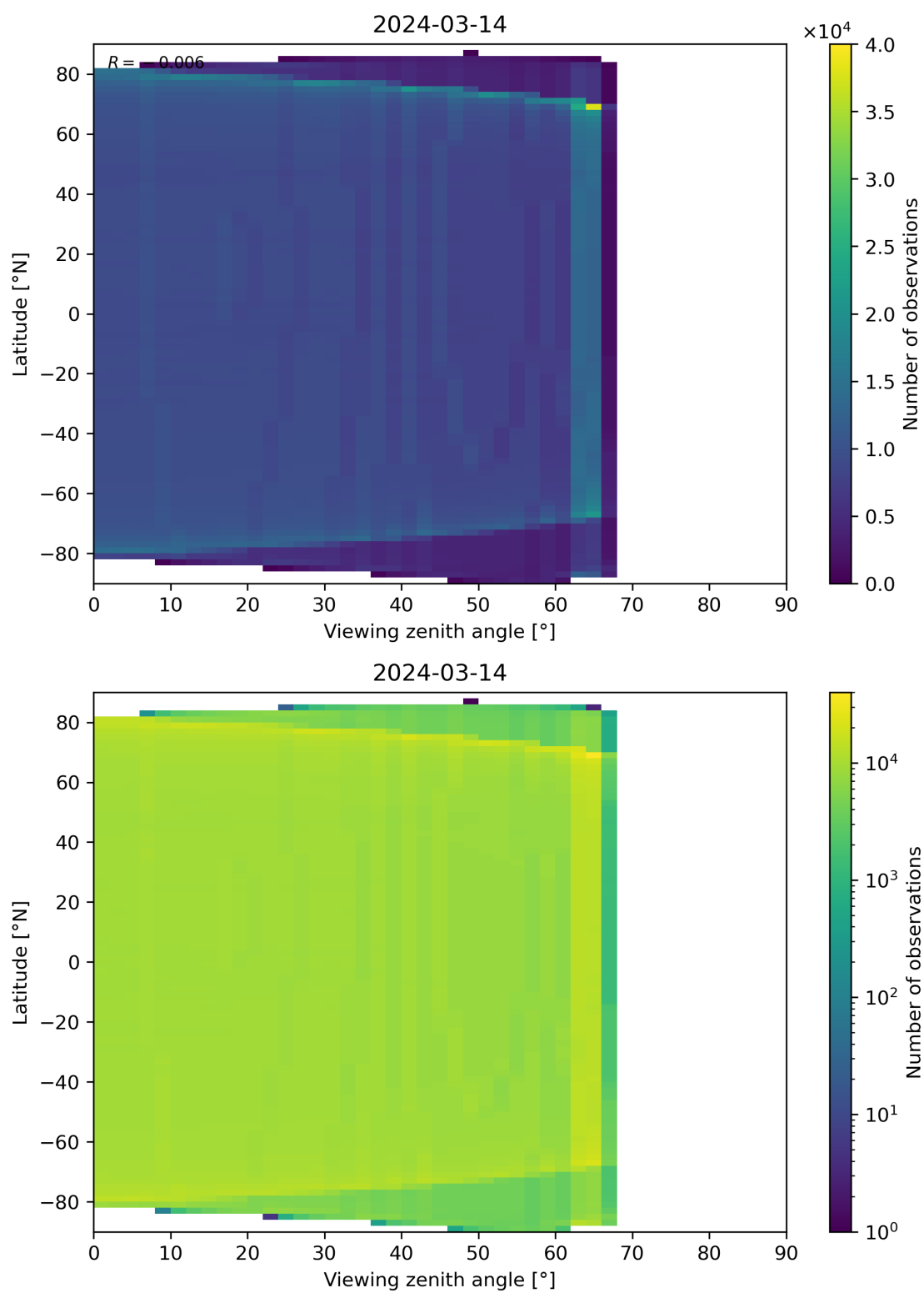
Figure 163: Scatter density plot of “Viewing zenith angle” against “Latitude” for 2024-03-14 to 2024-03-15.
