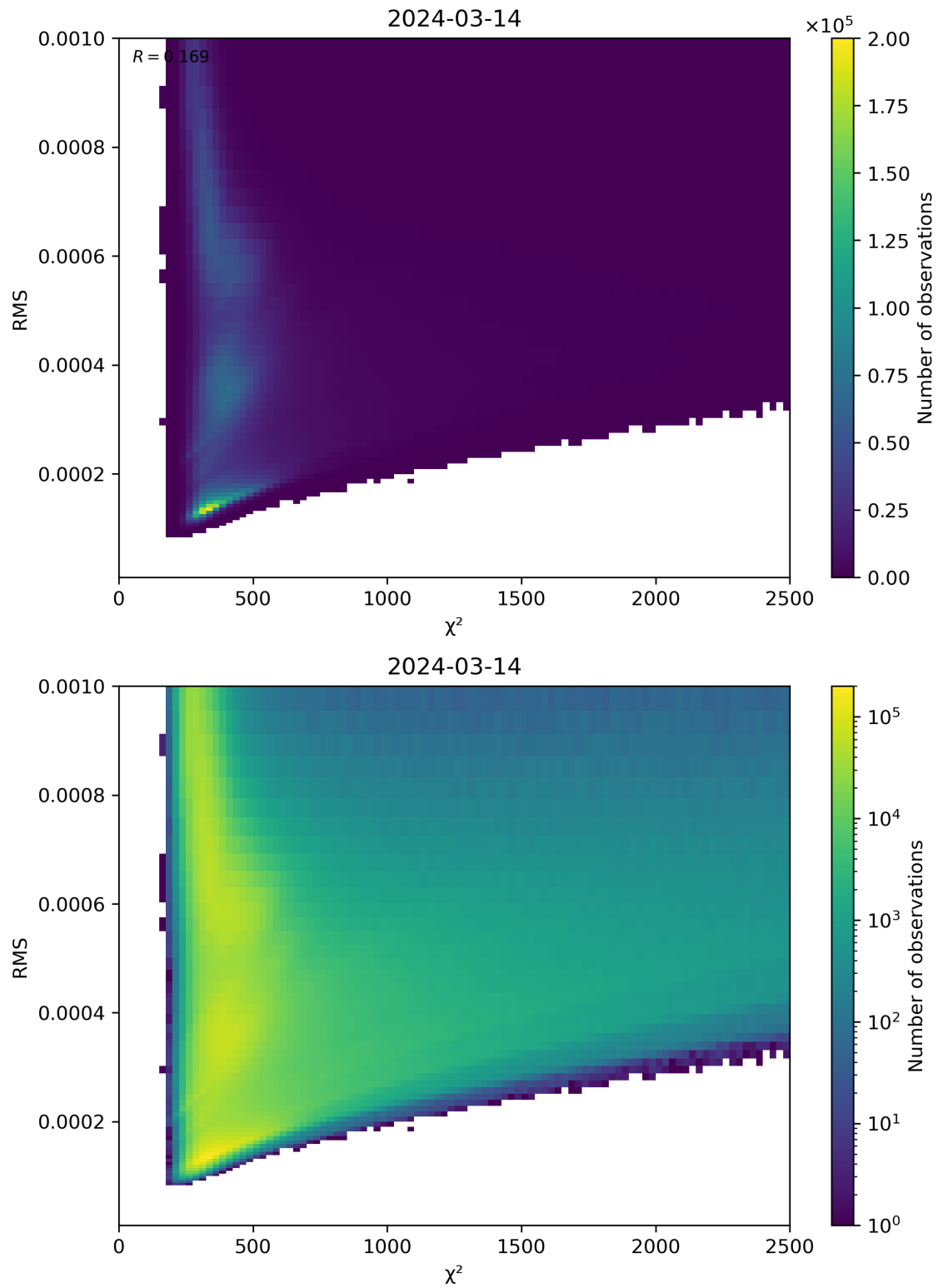
Figure 82: Scatter density plot of “ \chi^2 ” against “RMS” for 2024-03-14 to 2024-03-15.
