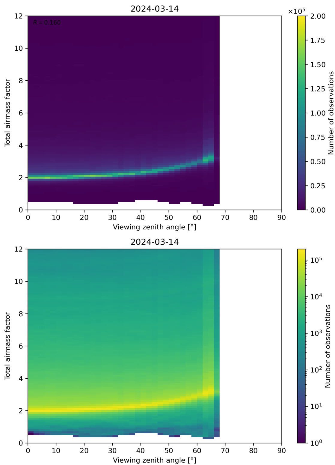
Figure 160: Scatter density plot of “Viewing zenith angle” against “Total airmass factor” for 2024-03-14 to 2024-03-15.
