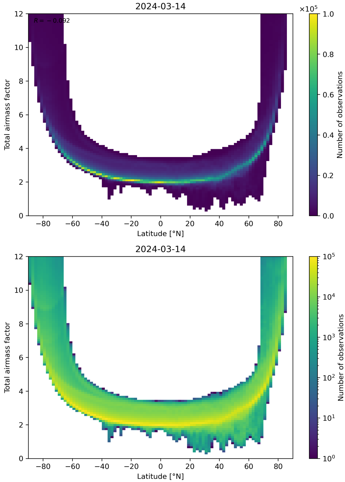
Figure 84: Scatter density plot of “Latitude” against “Total airmass factor” for 2024-03-14 to 2024-03-15.
