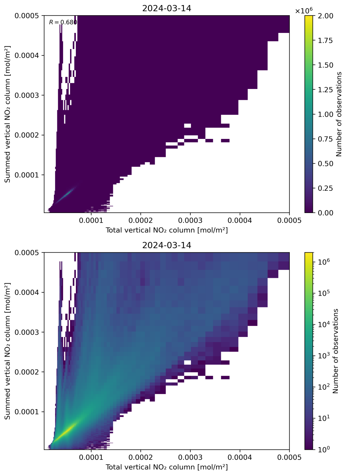
Figure 112: Scatter density plot of “Total vertical NO 2 column” against “Summed vertical NO 2 column” for 2024-03-14 to 2024-03-15.
