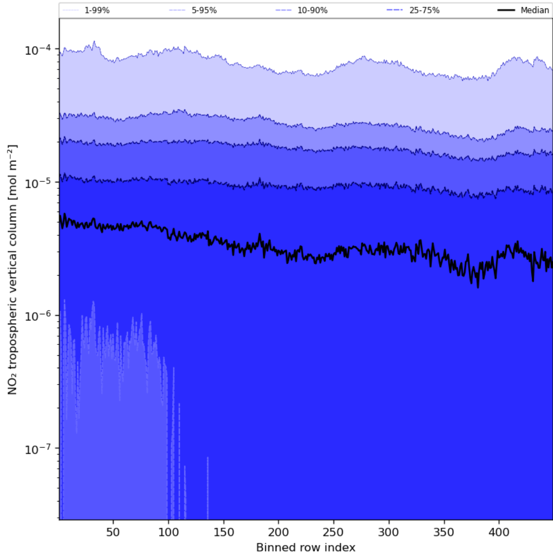
Figure 46: Along track statistics of “NO 2 tropospheric vertical column” for 2024-03-14 to 2024-03-15
