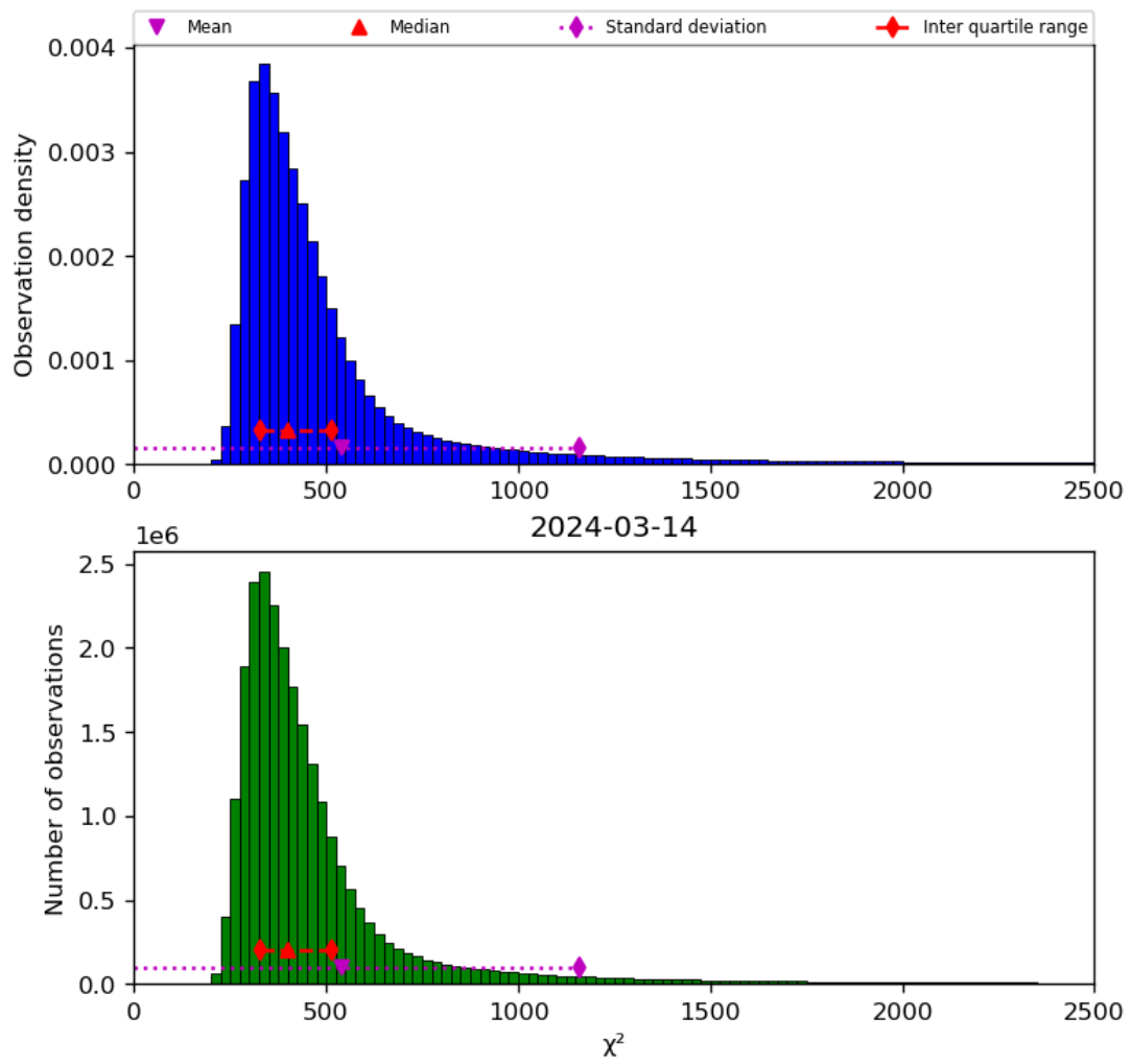
Figure 42: Histogram of “ \chi^2 ” for 2024-03-14 to 2024-03-15
