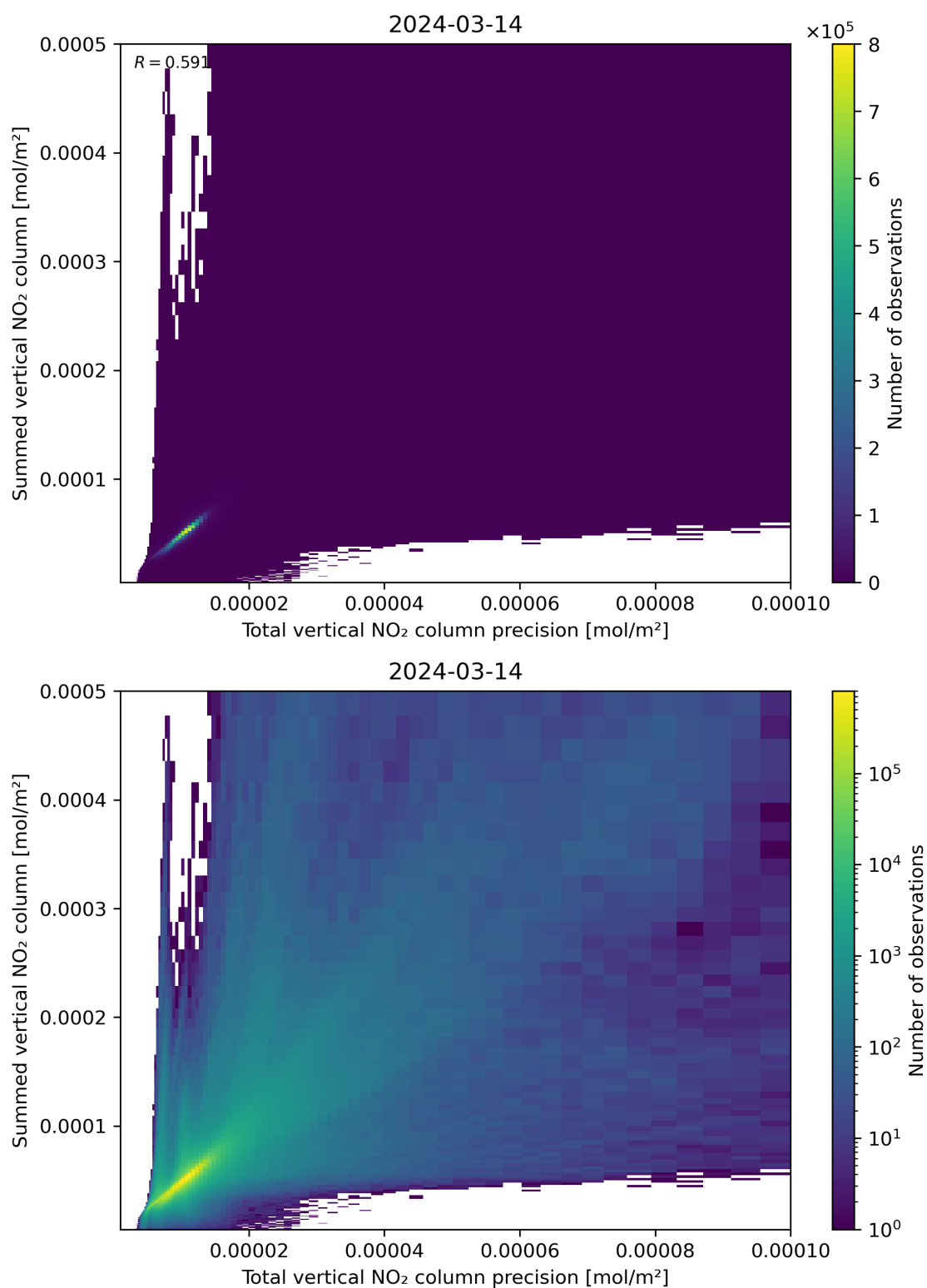
Figure 117: Scatter density plot of “Total vertical NO 2 column precision” against “Summed vertical NO 2 column” for 2024-03-14 to 2024-03-15.
