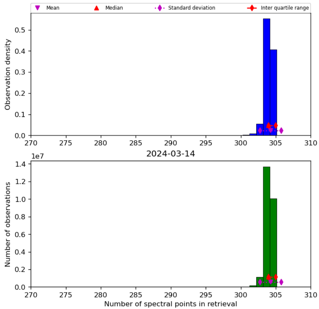
Figure 33: Histogram of “Number of spectral points in retrieval” for 2024-03-14 to 2024-03-15
