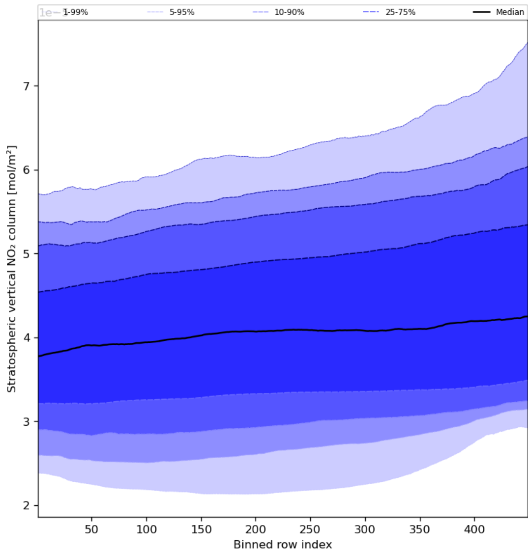
Figure 53: Along track statistics of “Stratospheric vertical NO 2 column” for 2024-03-14 to 2024-03-15
