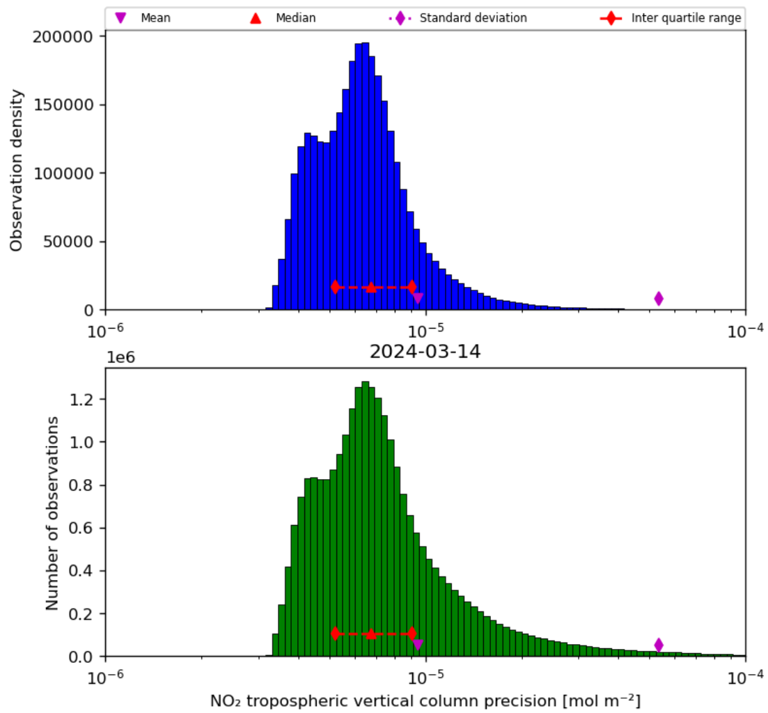
Figure 30: Histogram of “NO 2 tropospheric vertical column precision” for 2024-03-14 to 2024-03-15
