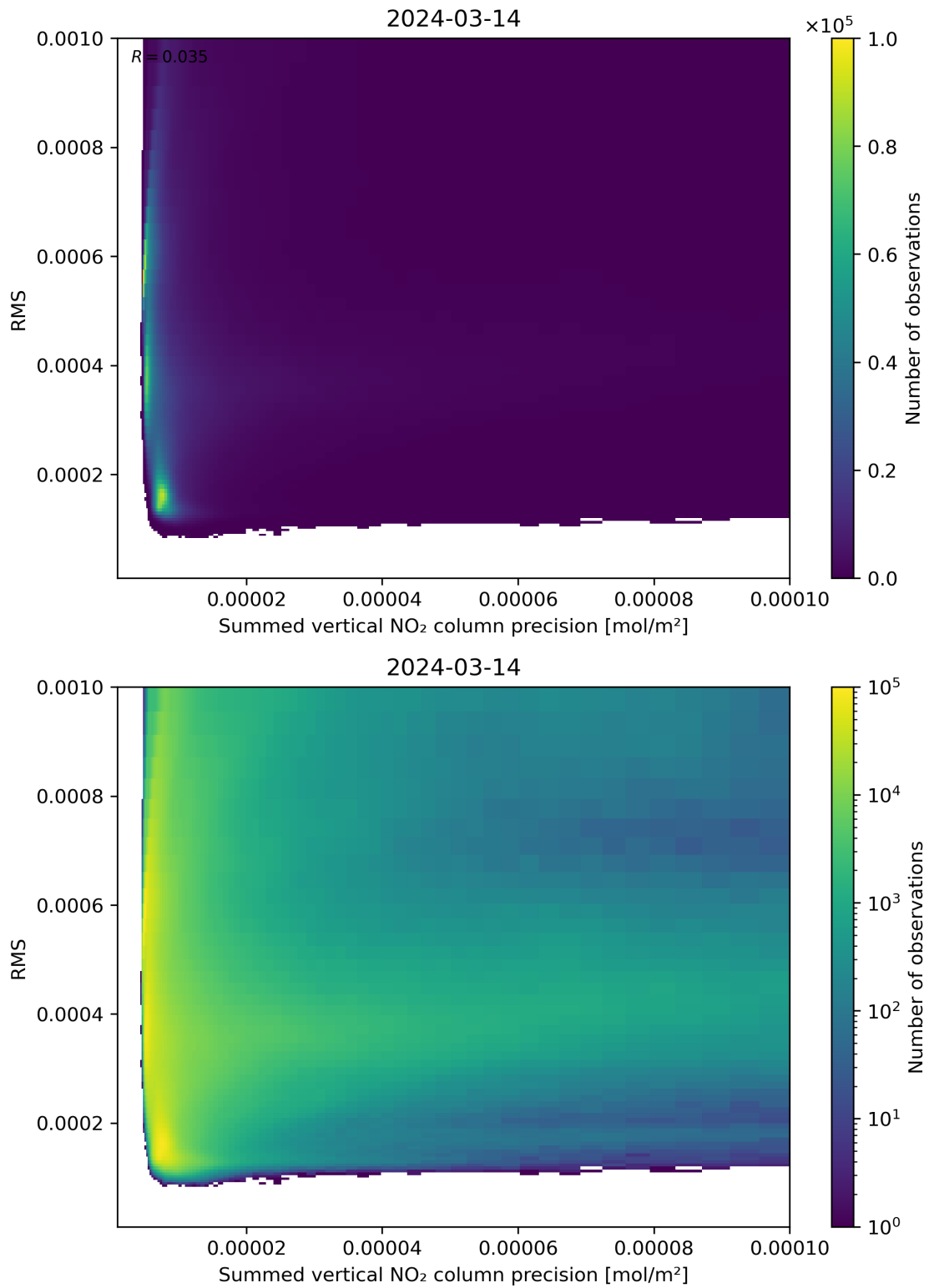
Figure 108: Scatter density plot of “Summed vertical NO 2 column precision” against “RMS” for 2024-03-14 to 2024-03-15.
