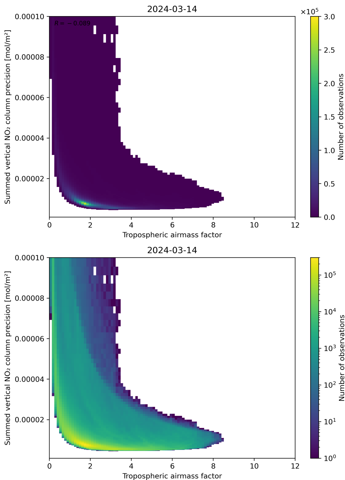
Figure 76: Scatter density plot of “Tropospheric air mass factor” against “Summed vertical NO 2 column precision” for 2024-03-14 to 2024-03-15.
