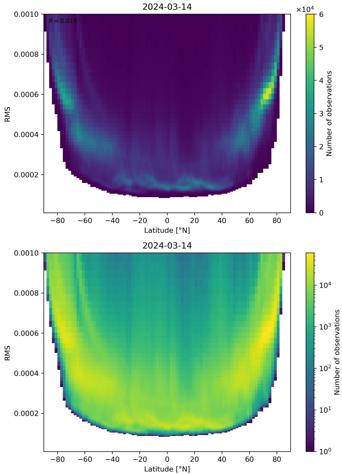
Figure 94: Scatter density plot of “Latitude” against “RMS” for 2024-03-14 to 2024-03-15.
