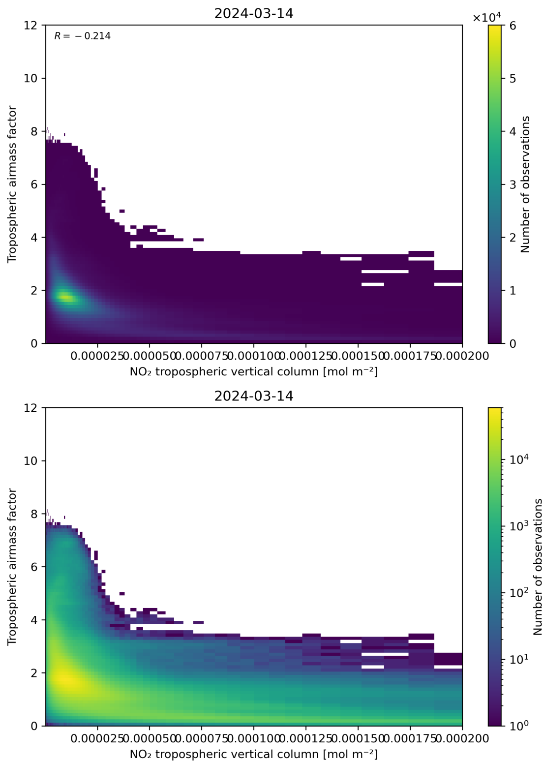
Figure 123: Scatter density plot of “NO 2 tropospheric vertical column” against “Tropospheric air mass factor” for 2024-03-14 to 2024-03-15.
