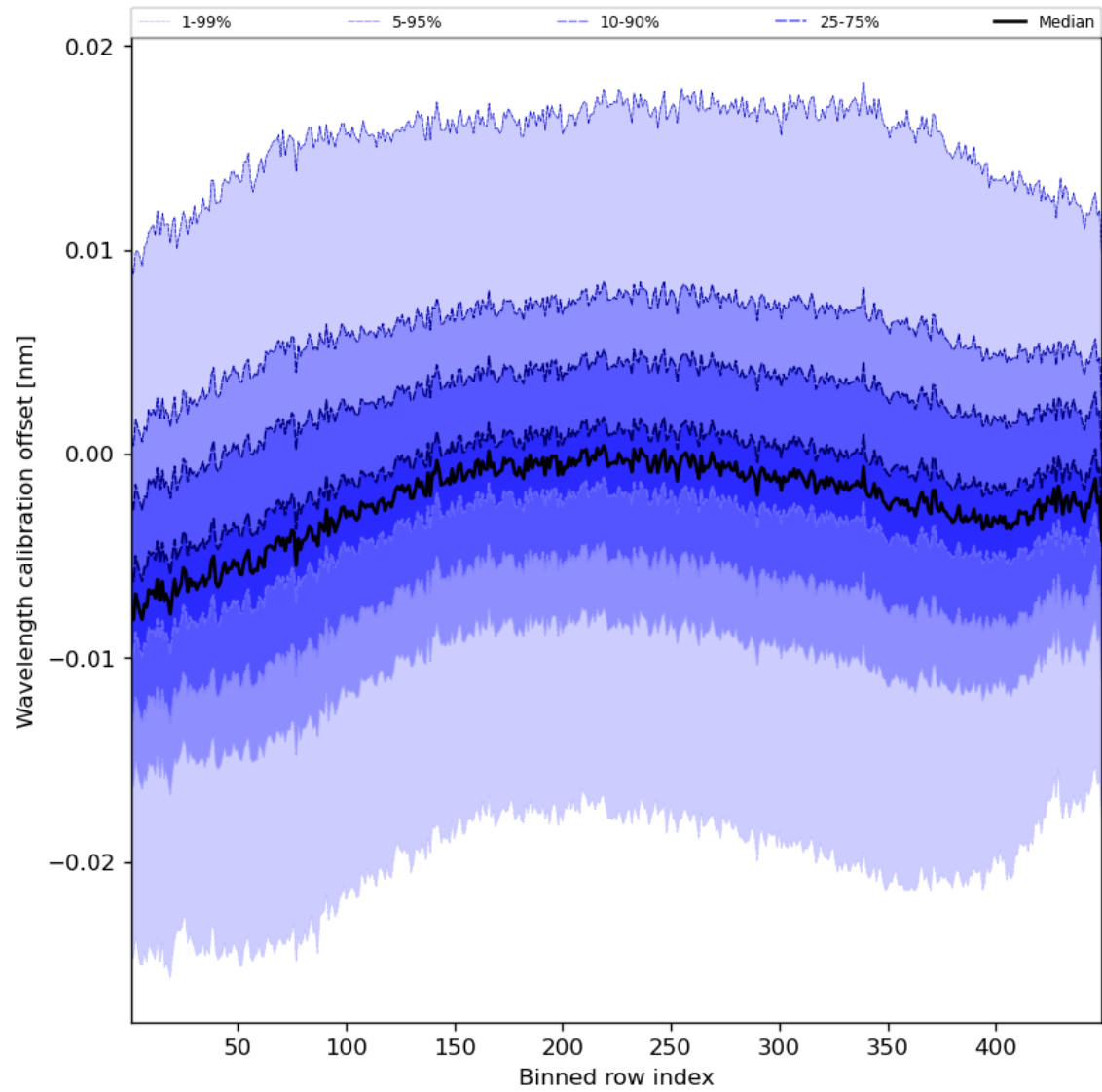
Figure 52: Along track statistics of “Wavelength calibration offset” for 2024-03-14 to 2024-03-15
