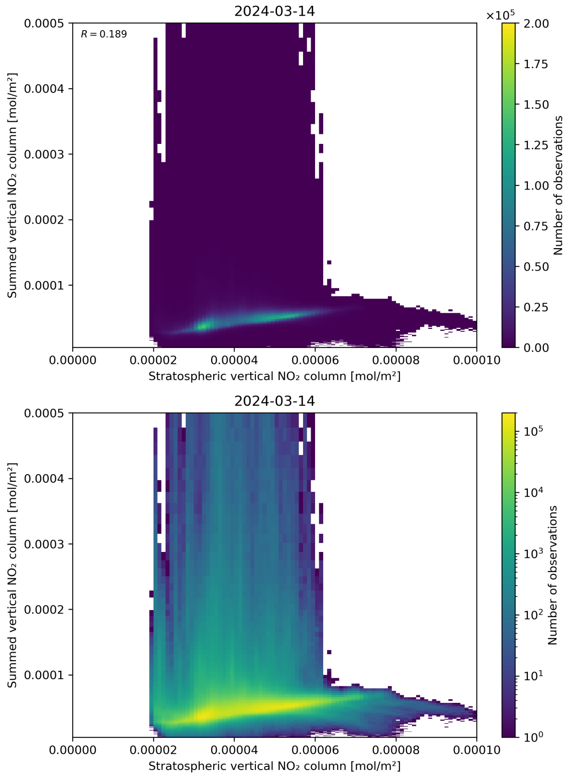
Figure 98: Scatter density plot of “Stratospheric vertical NO 2 column” against “Summed vertical NO 2 column” for 2024-03-14 to 2024-03-15.
