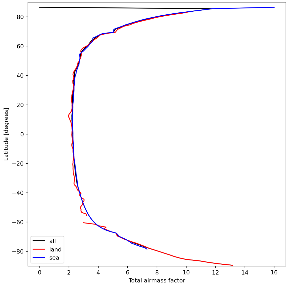
Figure 15: Zonal average of “Total airmass factor” for 2024-03-14 to 2024-03-15.
