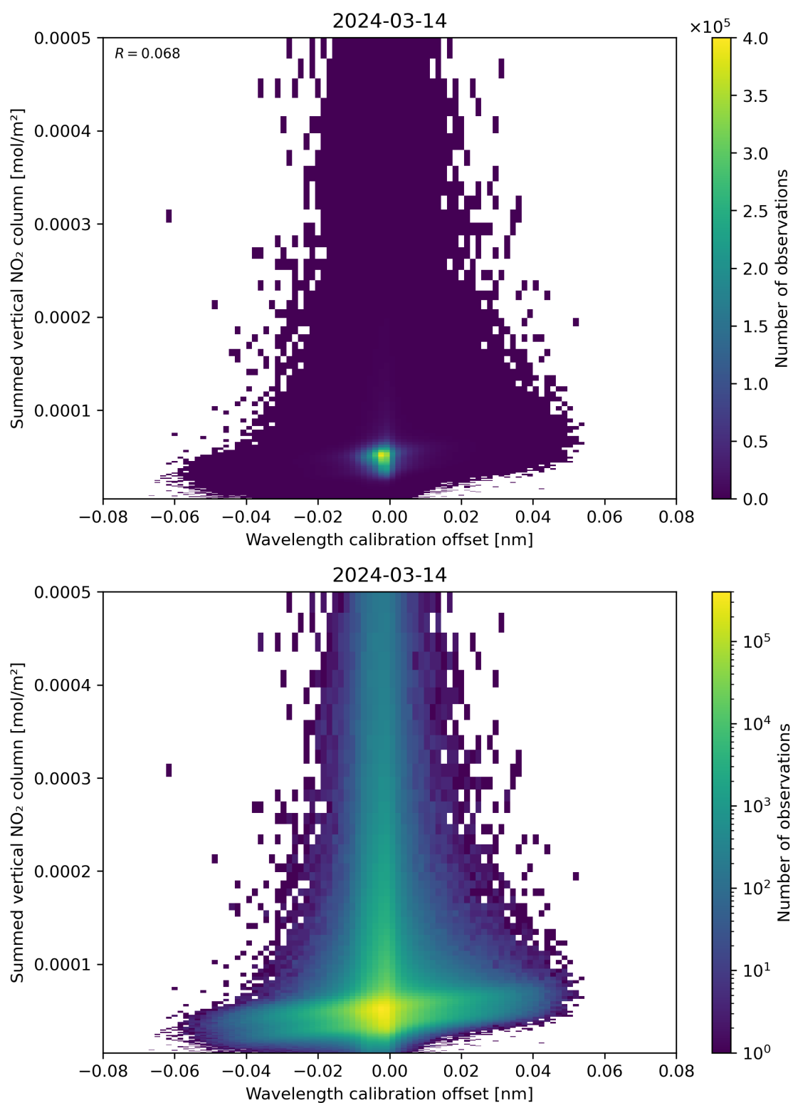
Figure 177: Scatter density plot of “Wavelength calibration offset” against “Summed vertical NO 2 column” for 2024-03-14 to 2024-03-15.
