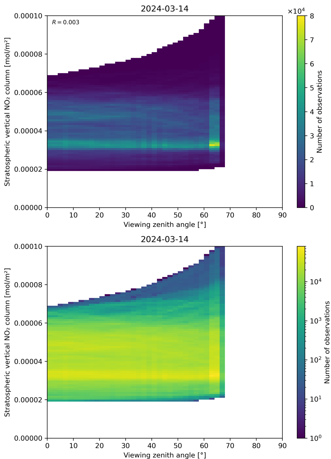
Figure 164: Scatter density plot of “Viewing zenith angle” against “Stratospheric vertical NO 2 column” for 2024-03-14 to 2024-03-15.
