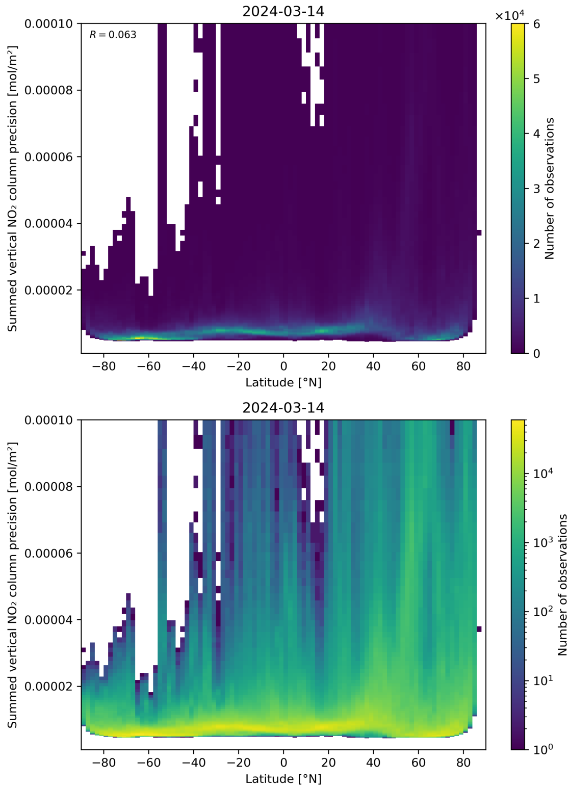
Figure 89: Scatter density plot of “Latitude” against “Summed vertical NO 2 column precision” for 2024-03-14 to 2024-03-15.
