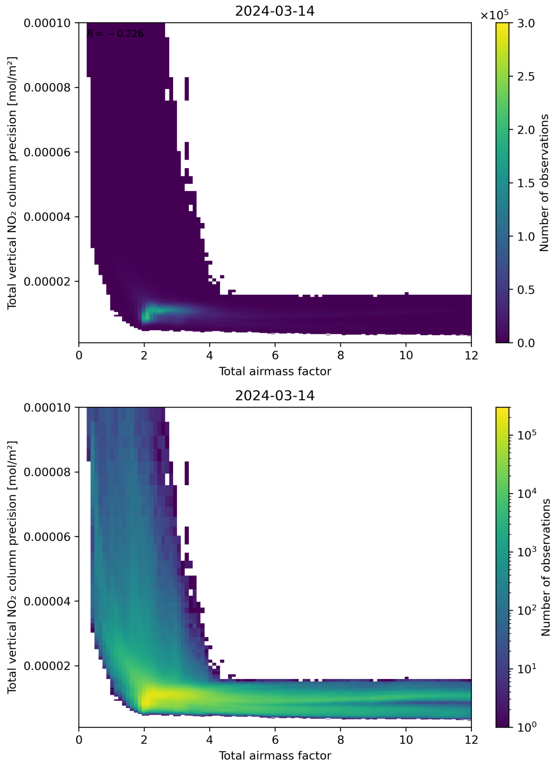
Figure 68: Scatter density plot of “Total airmass factor” against “Total vertical NO 2 column precision” for 2024-03-14 to 2024-03-15.
