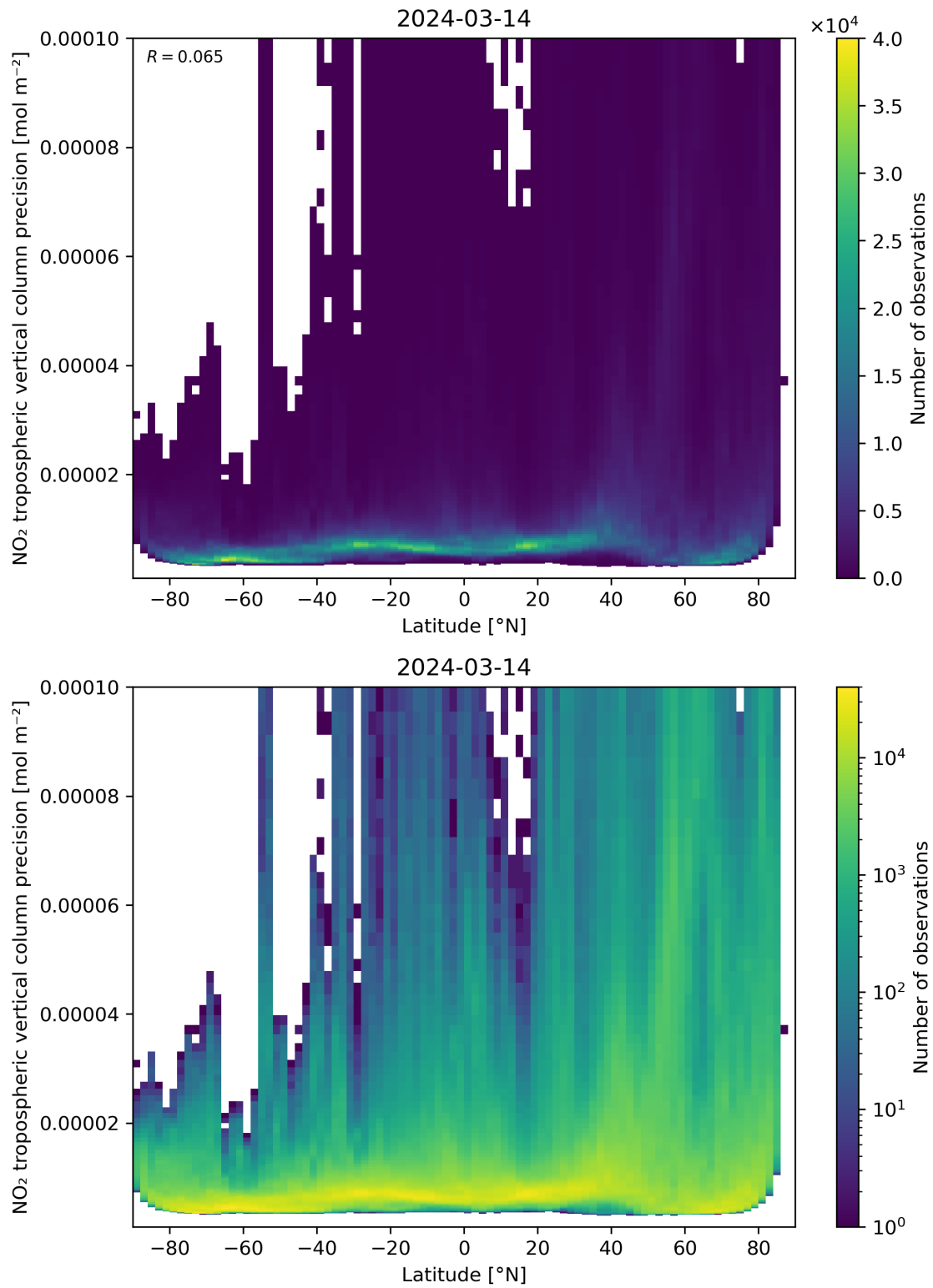
Figure 93: Scatter density plot of “Latitude” against “NO 2 tropospheric vertical column precision” for 2024-03-14 to 2024-03-15.
