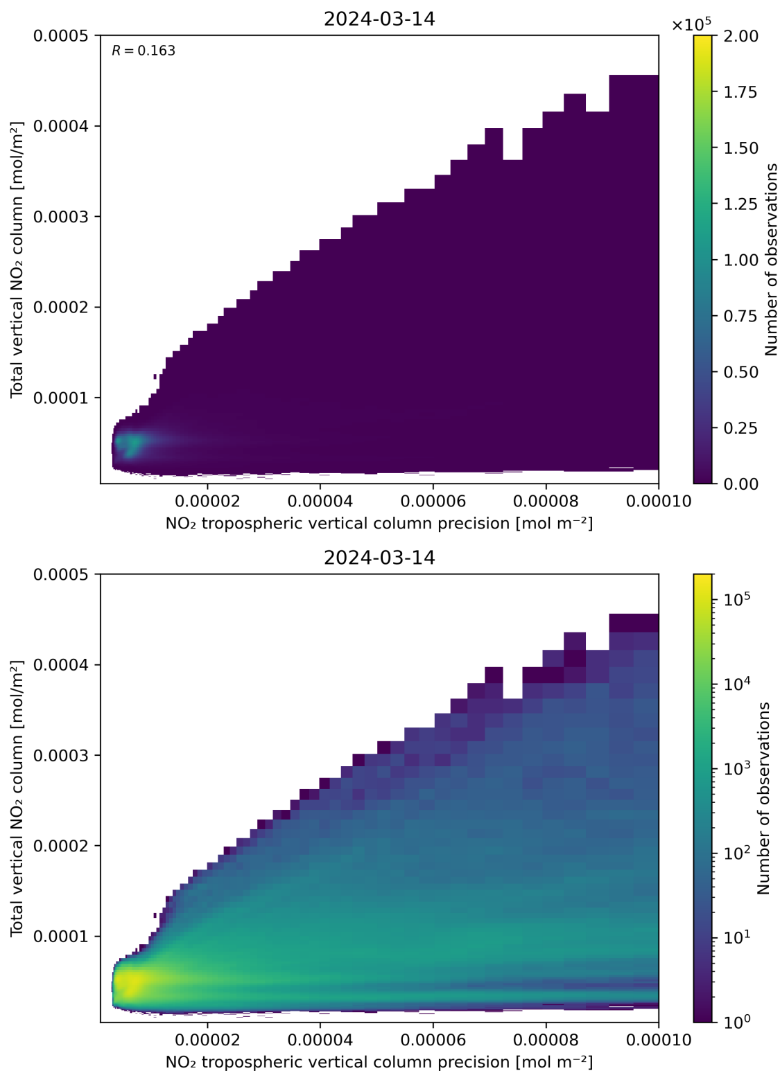
Figure 138: Scatter density plot of “NO 2 tropospheric vertical column precision” against “Total vertical NO 2 column” for 2024-03-14 to 2024-03-15.
