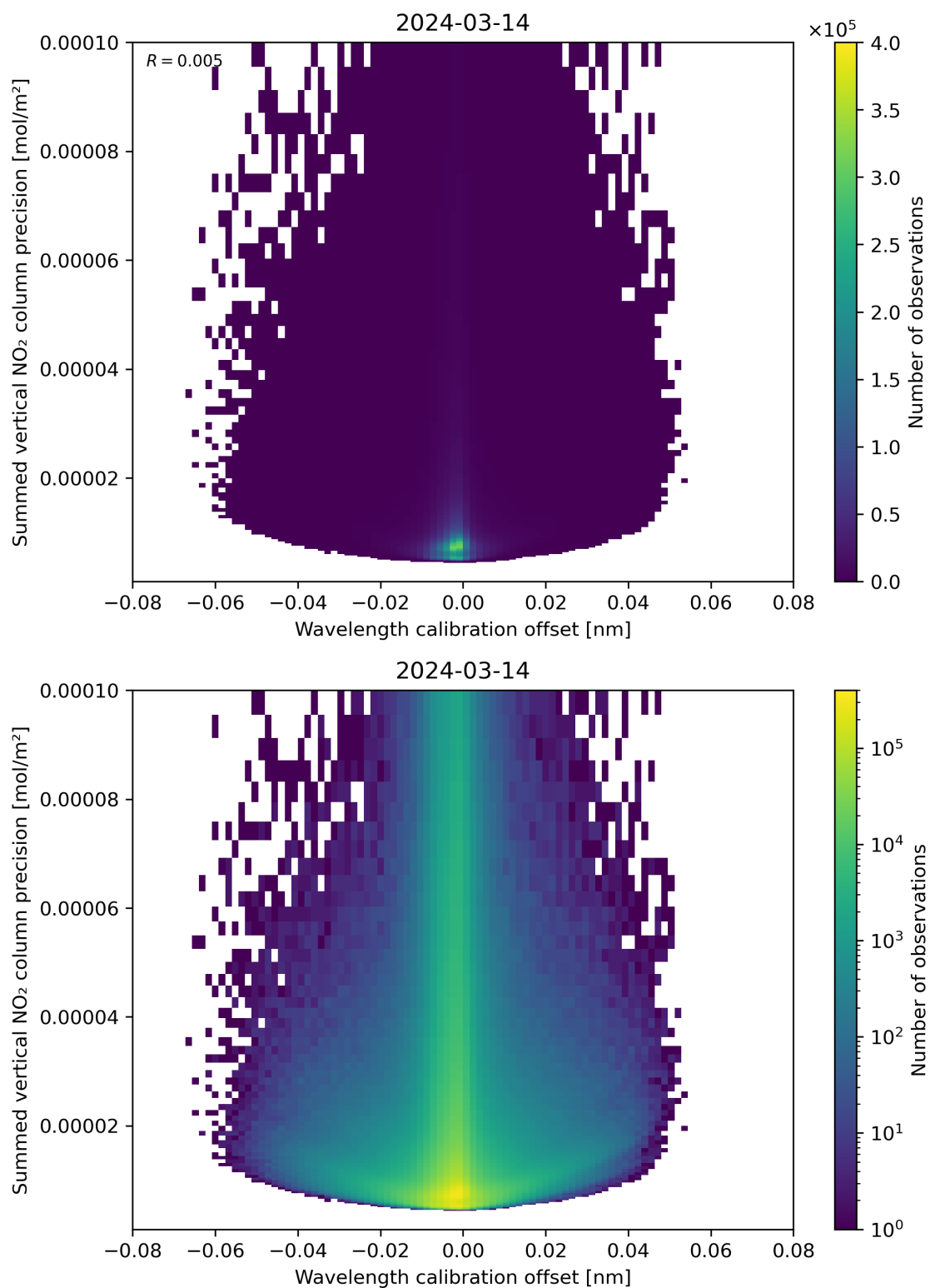
Figure 178: Scatter density plot of “Wavelength calibration offset” against “Summed vertical NO 2 column precision” for 2024-03-14 to 2024-03-15.
