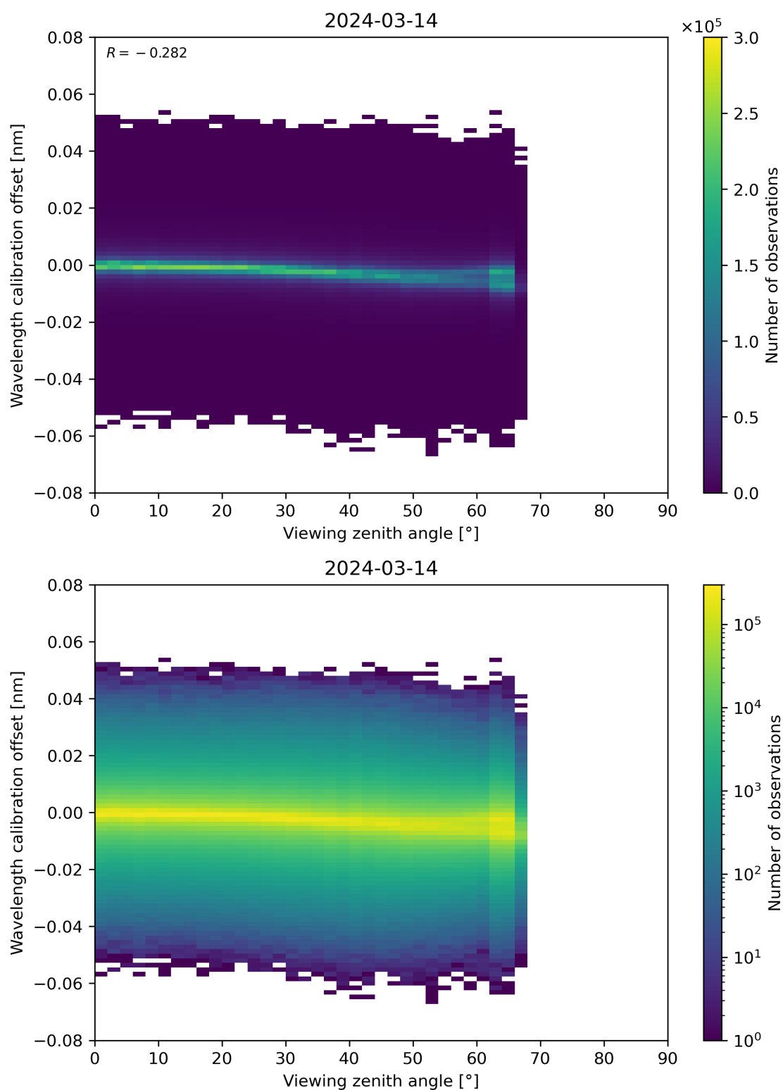
Figure 173: Scatter density plot of “Viewing zenith angle” against “Wavelength calibration offset” for 2024-03-14 to 2024-03-15.
