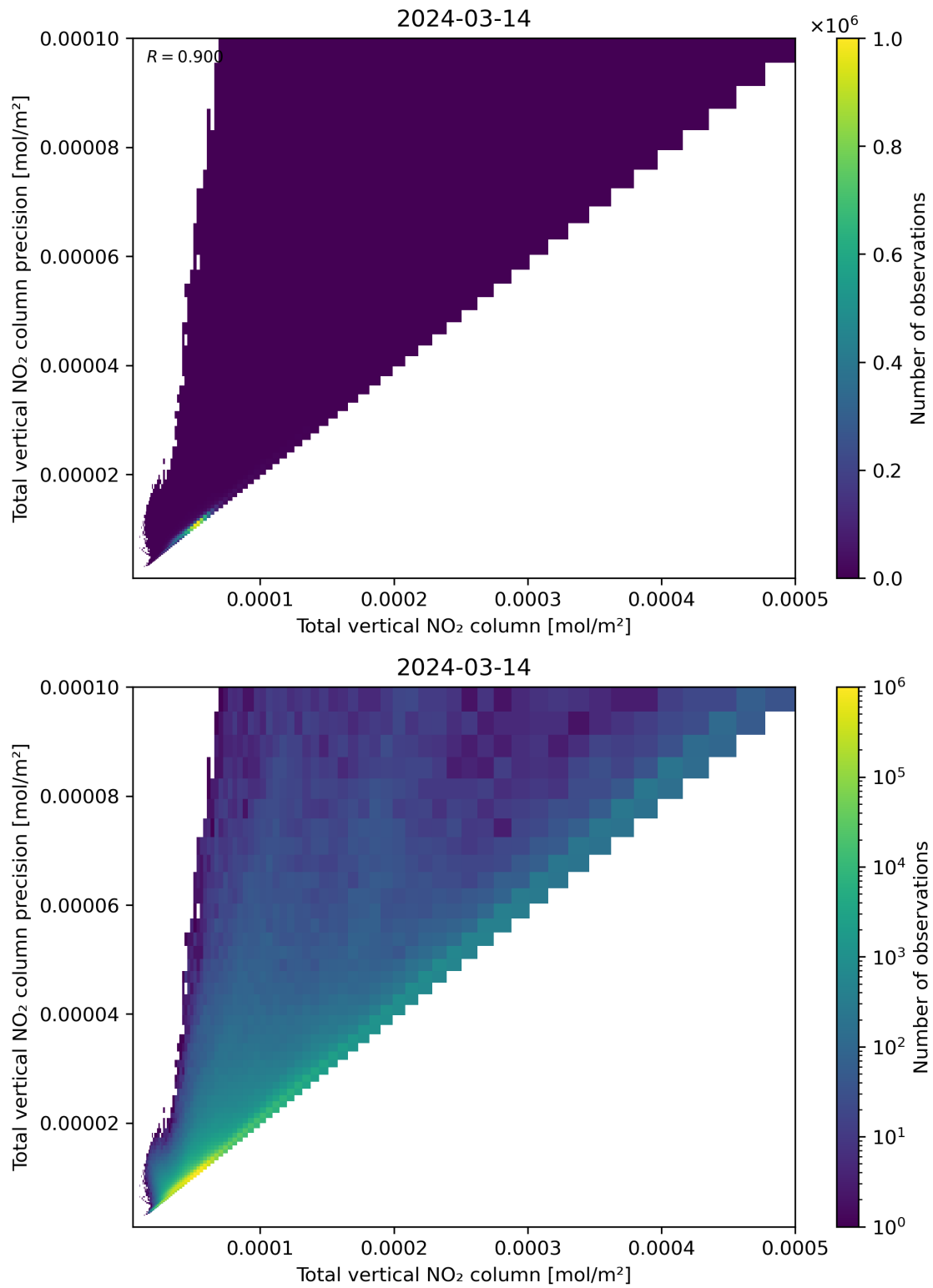
Figure 114: Scatter density plot of “Total vertical NO 2 column” against “Total vertical NO 2 column precision” for 2024-03-14 to 2024-03-15.
