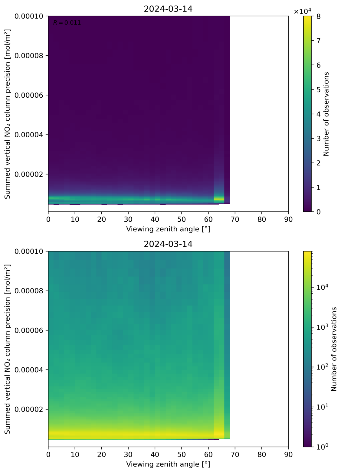
Figure 166: Scatter density plot of “Viewing zenith angle” against “Summed vertical NO 2 column precision” for 2024-03-14 to 2024-03-15.
