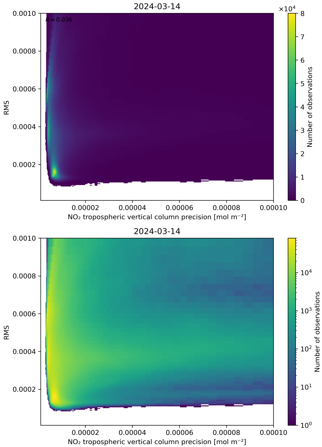
Figure 140: Scatter density plot of “NO 2 tropospheric vertical column precision” against “RMS” for 2024-03-14 to 2024-03-15.
