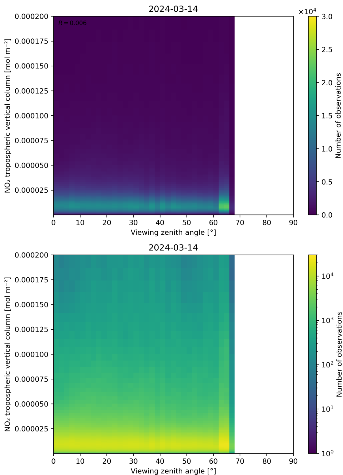
Figure 169: Scatter density plot of “Viewing zenith angle” against “NO 2 tropospheric vertical column” for 2024-03-14 to 2024-03-15.
