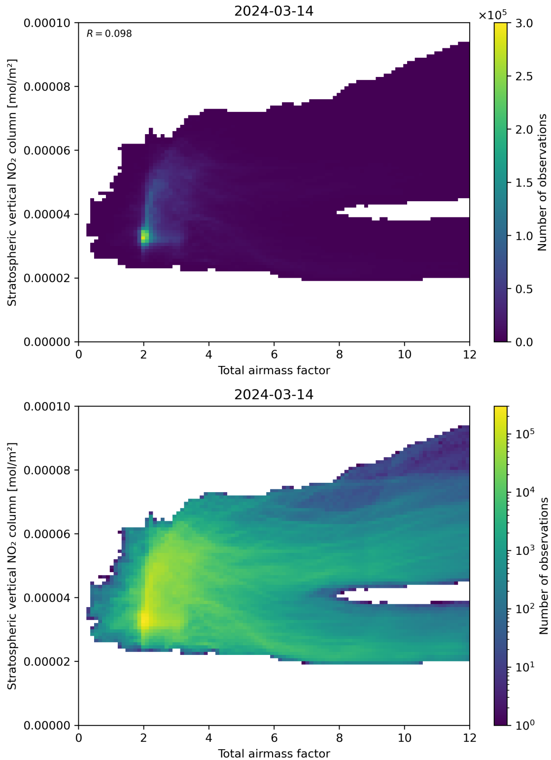
Figure 64: Scatter density plot of “Total airmass factor” against “Stratospheric vertical NO 2 column” for 2024-03-14 to 2024-03-15.
