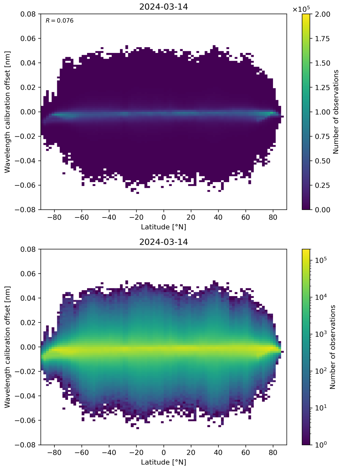
Figure 95: Scatter density plot of “Latitude” against “Wavelength calibration offset” for 2024-03-14 to 2024-03-15.
