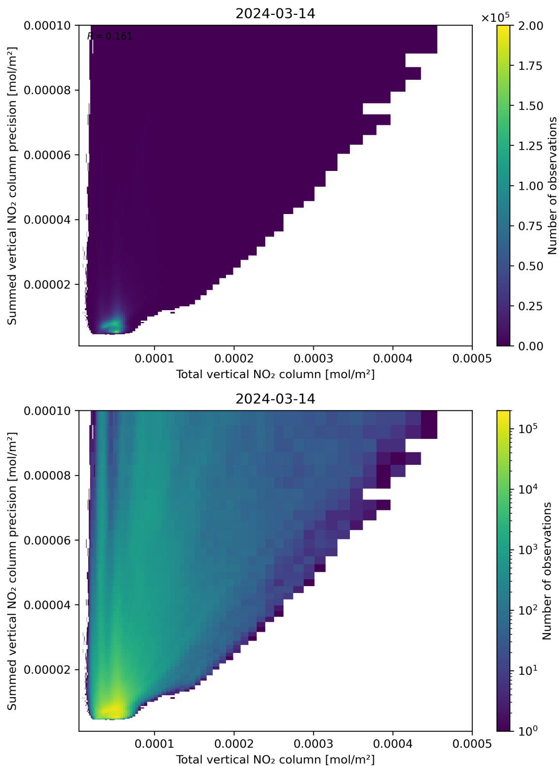
Figure 113: Scatter density plot of “Total vertical NO 2 column” against “Summed vertical NO 2 column precision” for 2024-03-14 to 2024-03-15.
