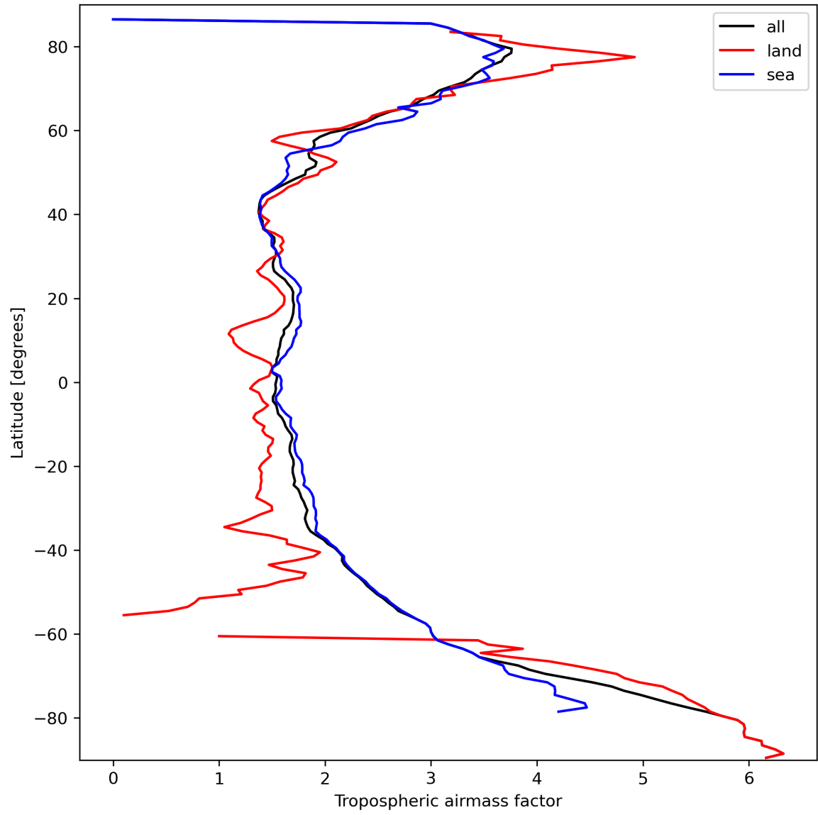
Figure 14: Zonal average of “Tropospheric airmass factor” for 2024-03-14 to 2024-03-15.
