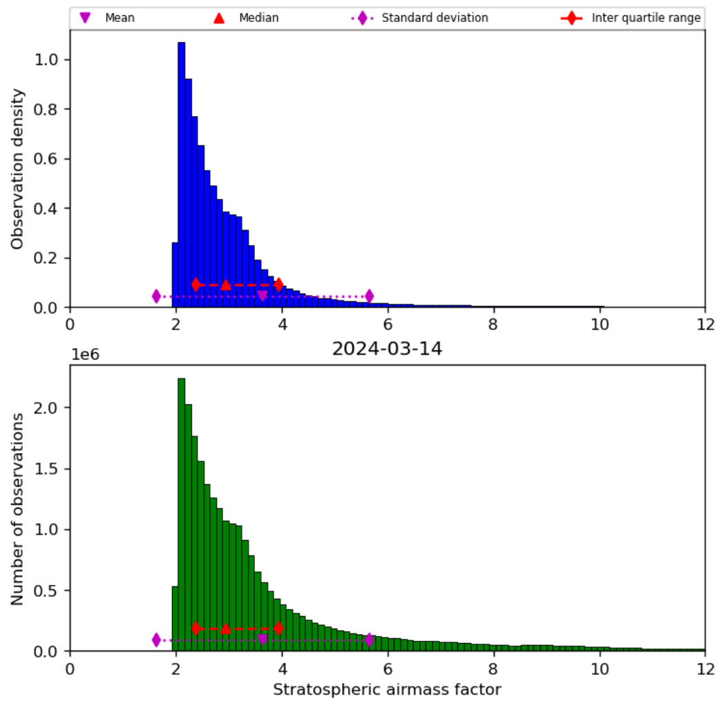
Figure 44: Histogram of “Stratospheric airmass factor” for 2024-03-14 to 2024-03-15
