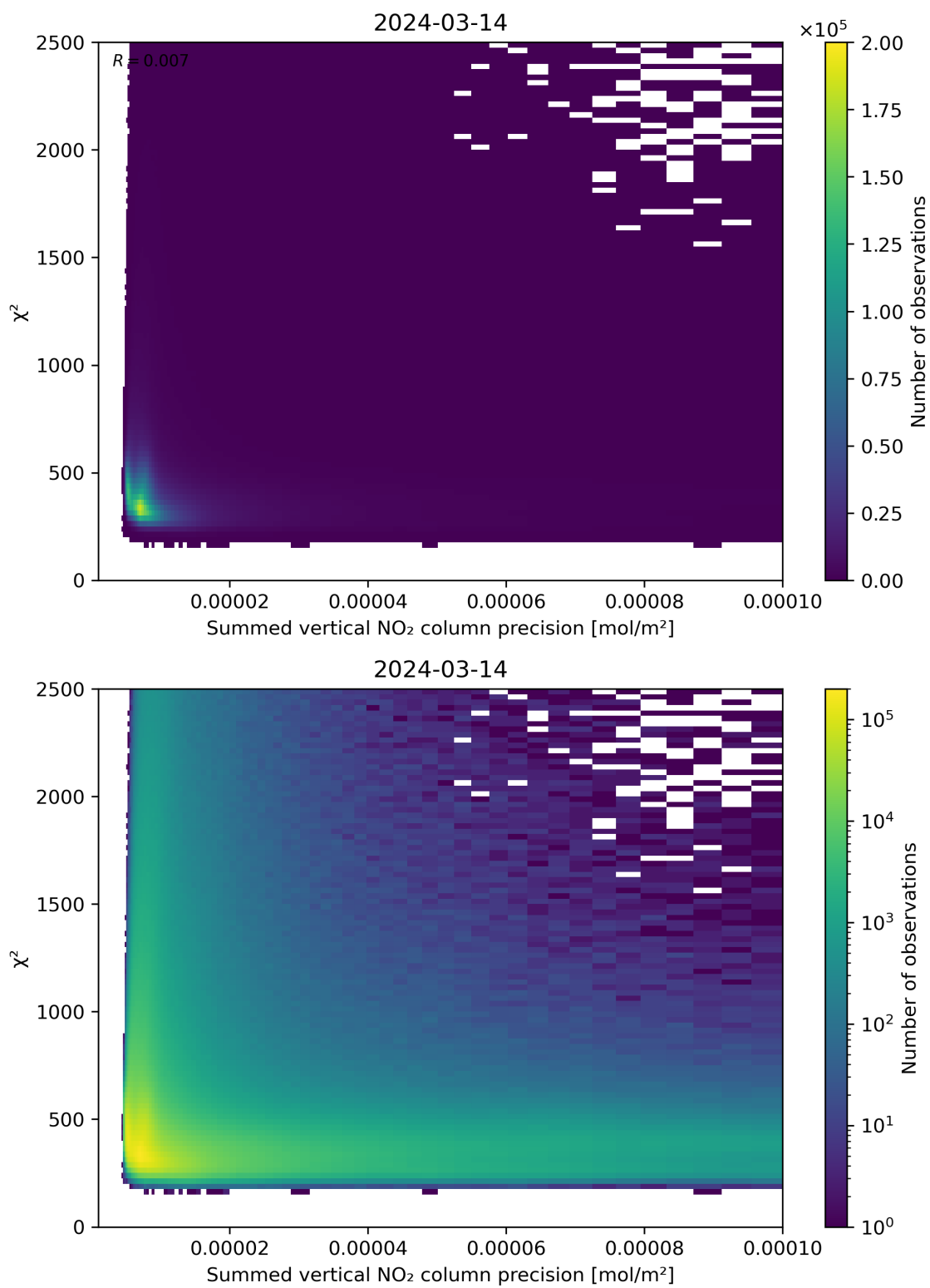
Figure 107: Scatter density plot of “Summed vertical NO 2 column precision” against “ \chi^2 ” for 2024-03-14 to 2024-03-15.
