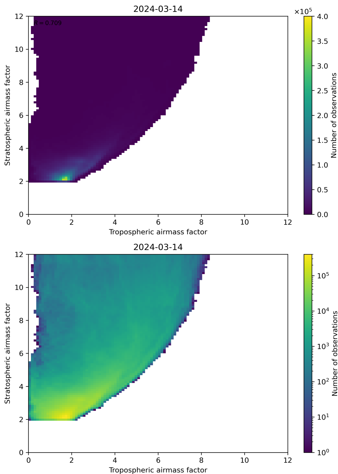
Figure 71: Scatter density plot of “Tropospheric airmass factor” against “Stratospheric airmass factor” for 2024-03-14 to 2024-03-15.
