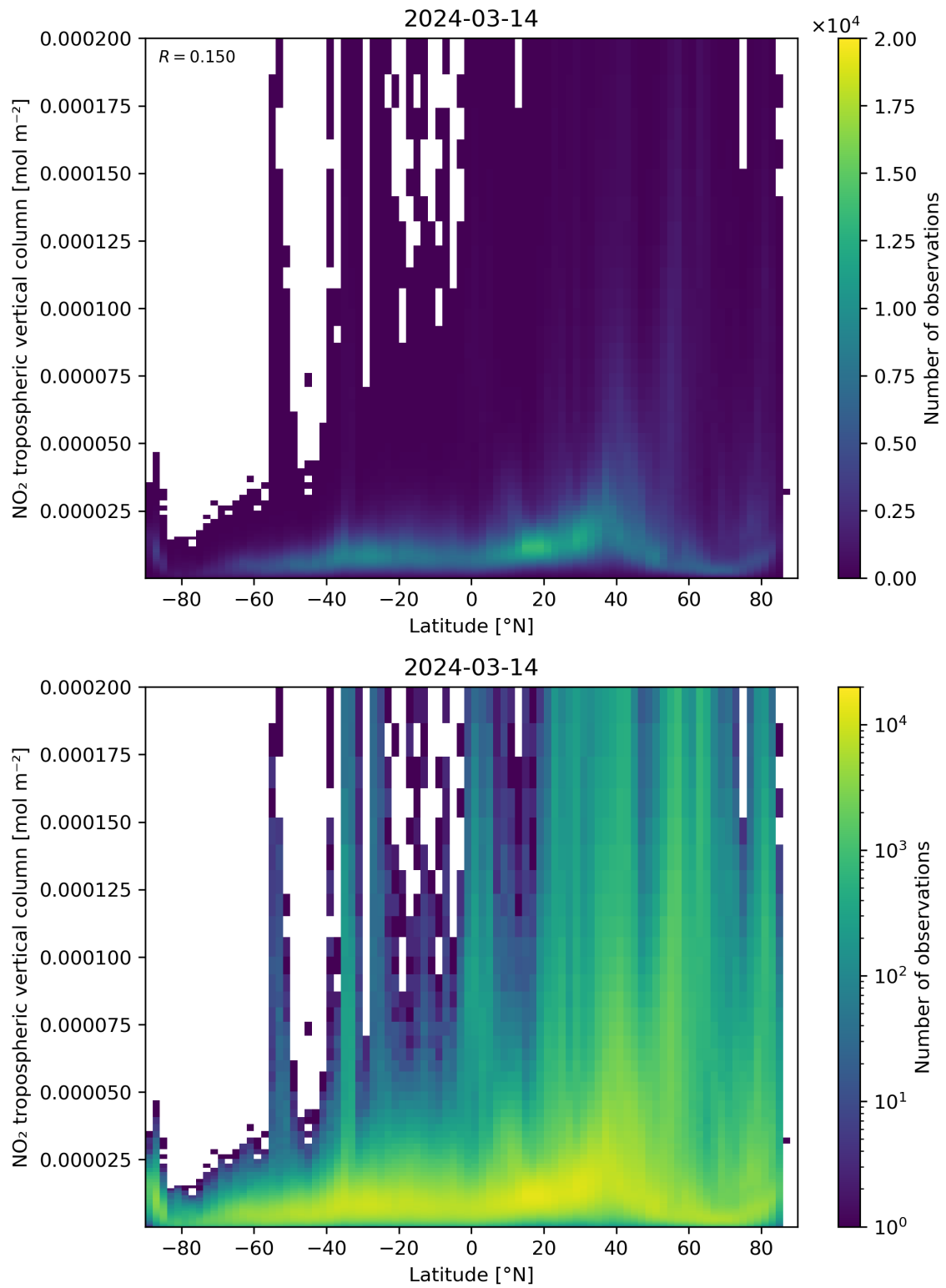
Figure 92: Scatter density plot of “Latitude” against “NO 2 tropospheric vertical column” for 2024-03-14 to 2024-03-15.
