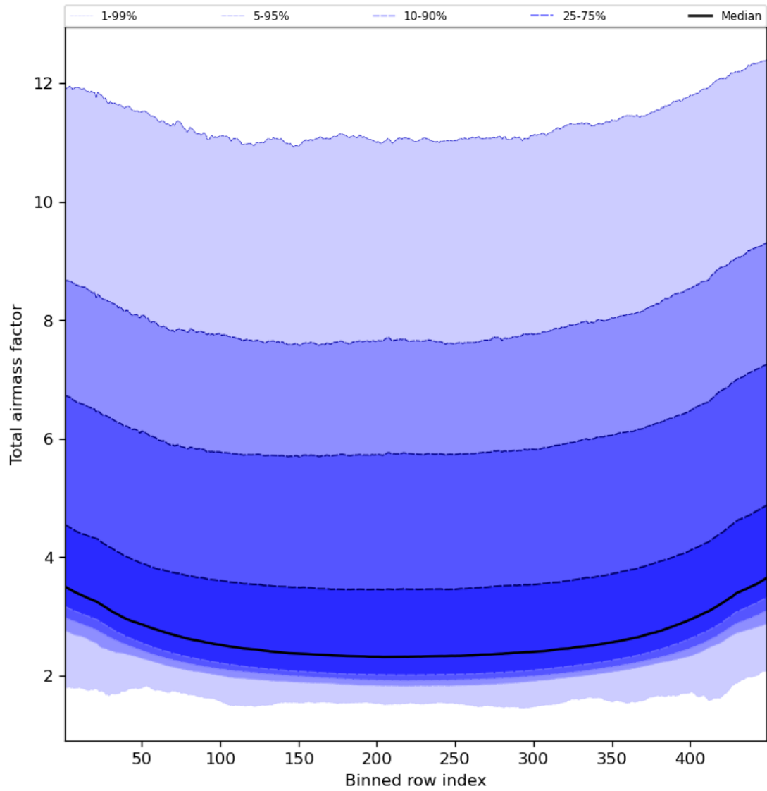
Figure 49: Along track statistics of “Total airmass factor” for 2024-03-14 to 2024-03-15
