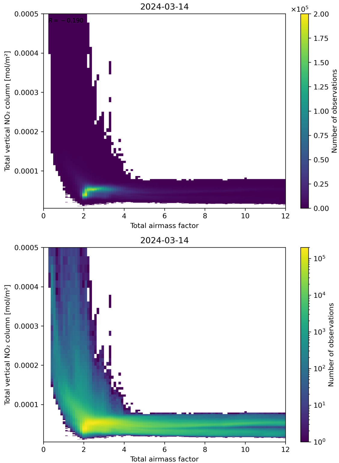
Figure 67: Scatter density plot of “Total airmass factor” against “Total vertical NO 2 column” for 2024-03-14 to 2024-03-15.
