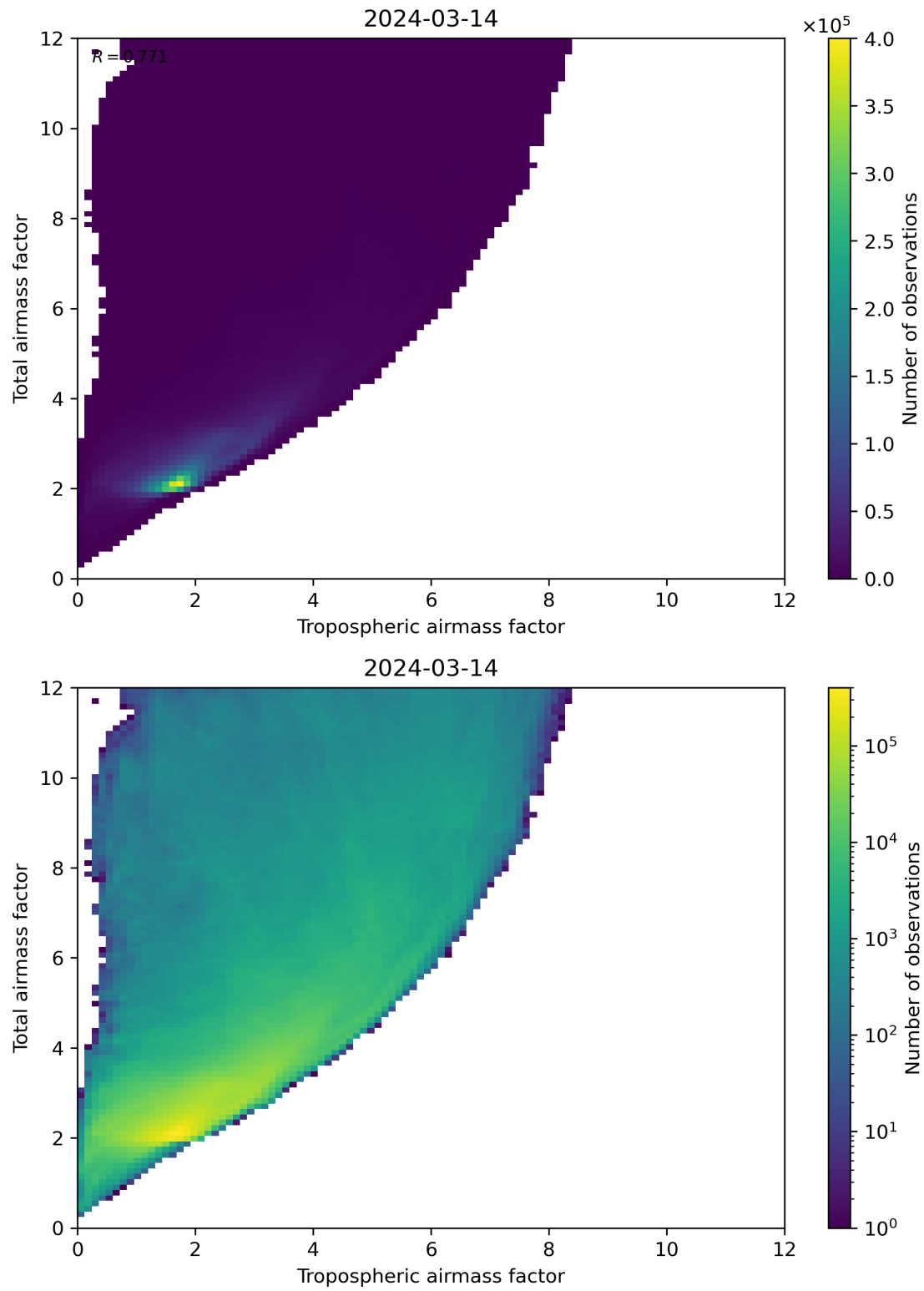
Figure 72: Scatter density plot of “Tropospheric airmass factor” against “Total airmass factor” for 2024-03-14 to 2024-03-15.
