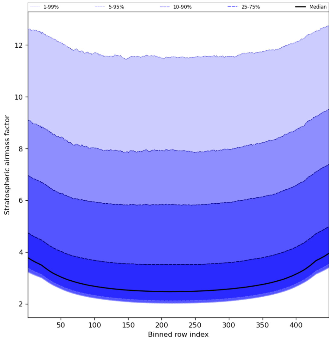
Figure 61: Along track statistics of “Stratospheric airmass factor” for 2024-03-14 to 2024-03-15
