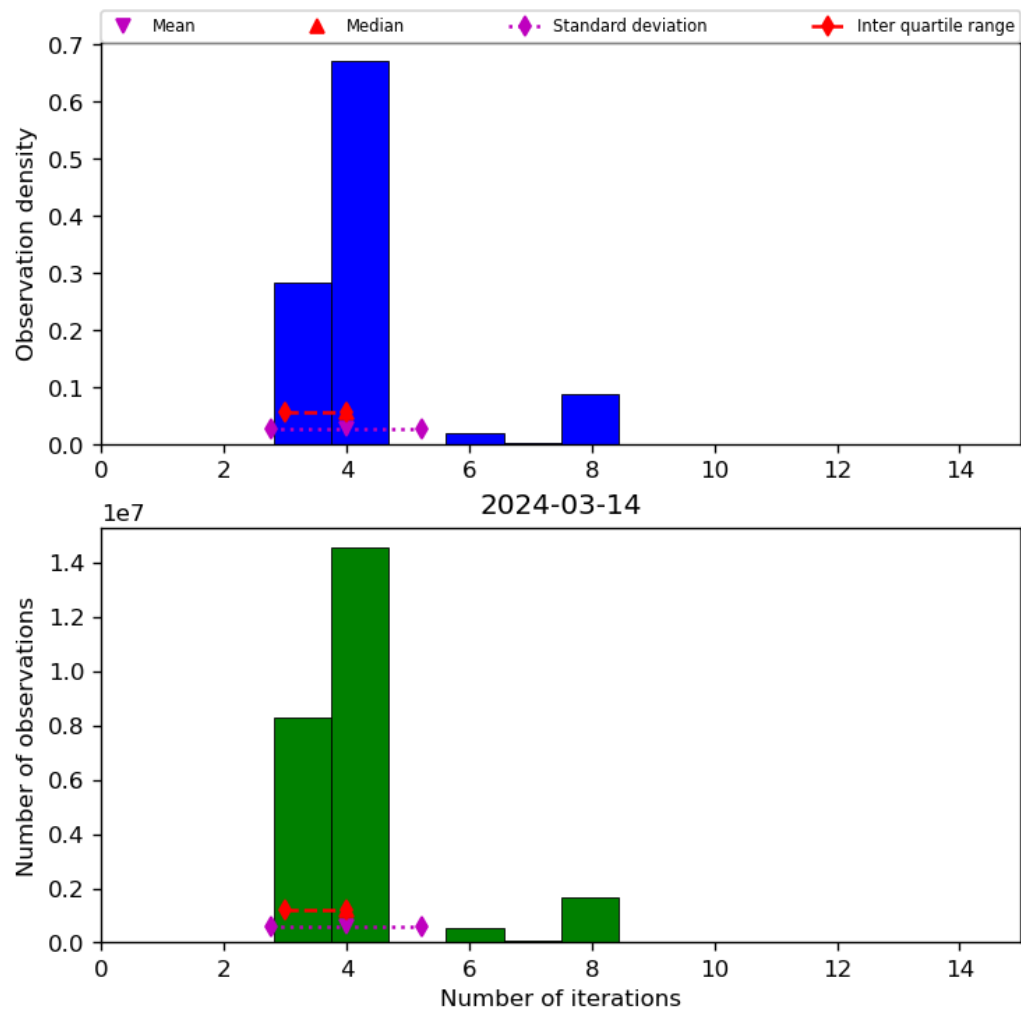
Figure 34: Histogram of “Number of iterations” for 2024-03-14 to 2024-03-15
