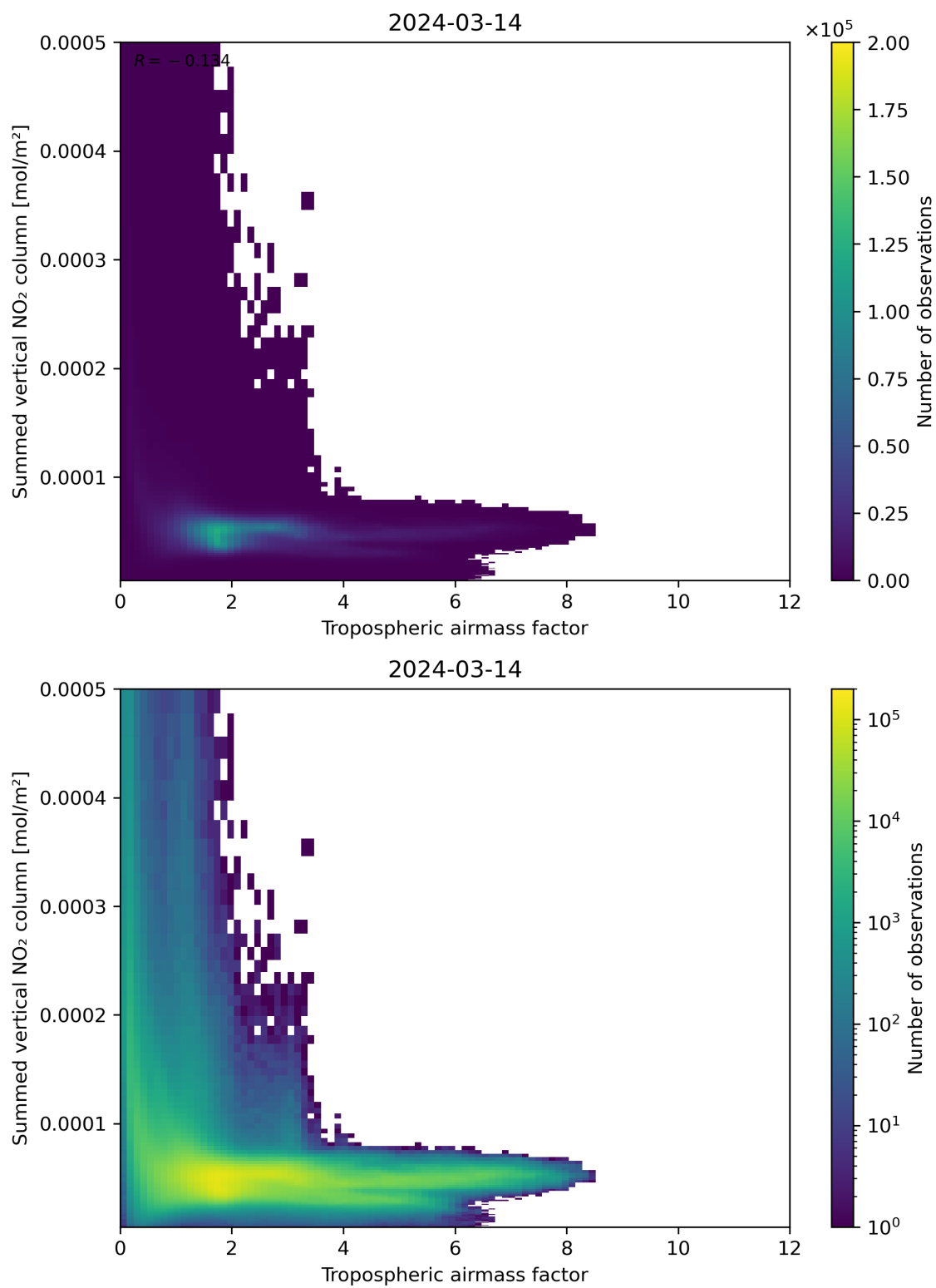
Figure 75: Scatter density plot of “Tropospheric air mass factor” against “Summed vertical NO 2 column” for 2024-03-14 to 2024-03-15.
