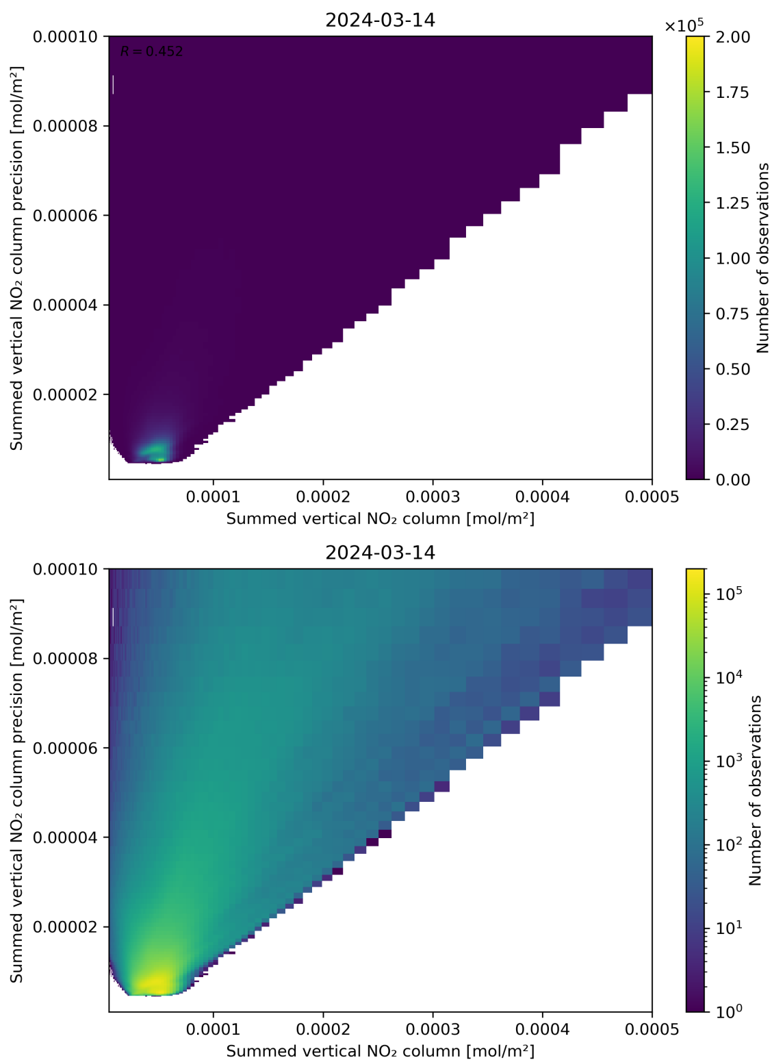
Figure 105: Scatter density plot of “Summed vertical NO 2 column” against “Summed vertical NO 2 column precision” for 2024-03-14 to 2024-03-15.
