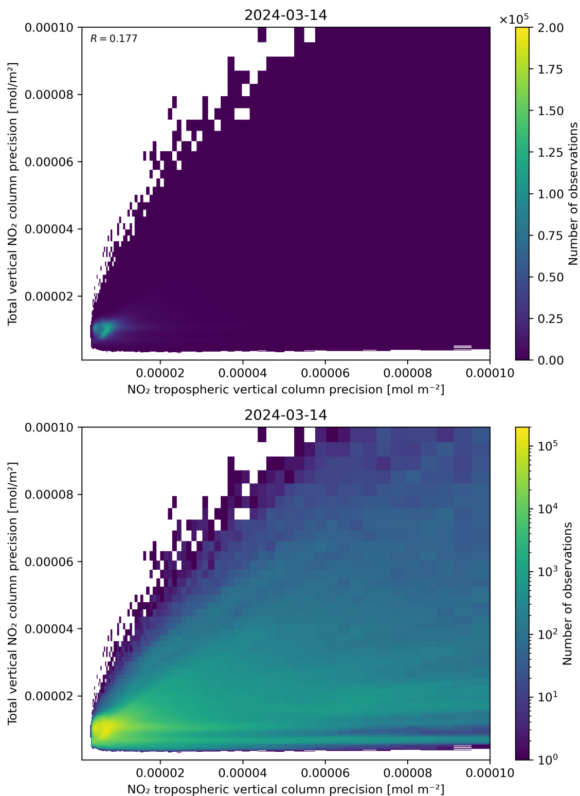
Figure 139: Scatter density plot of “NO 2 tropospheric vertical column precision” against “Total vertical NO 2 column precision” for 2024-03-14 to 2024-03-15.
