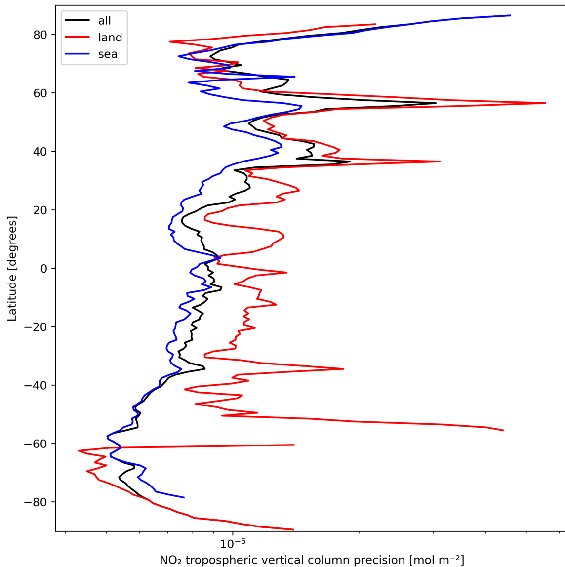
Figure 13: Zonal average of “NO 2 tropospheric vertical column precision” for 2024-03-14 to 2024-03-15.
