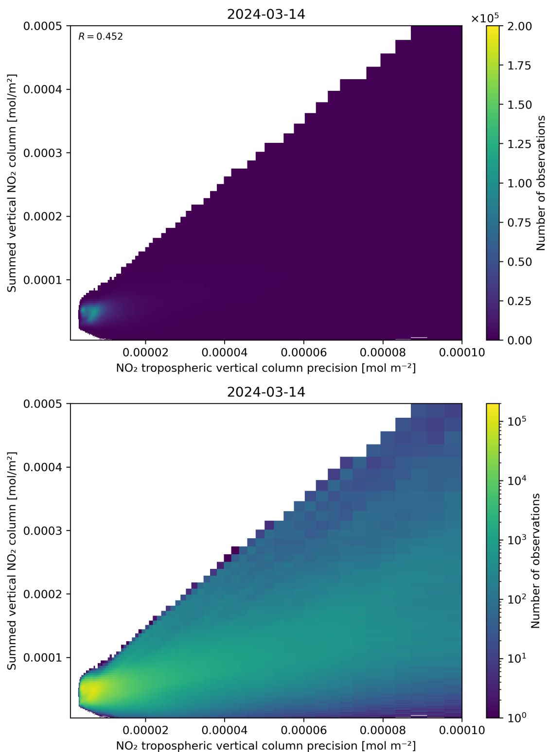
Figure 136: Scatter density plot of “NO 2 tropospheric vertical column precision” against “Summed vertical NO 2 column” for 2024-03-14 to 2024-03-15.
