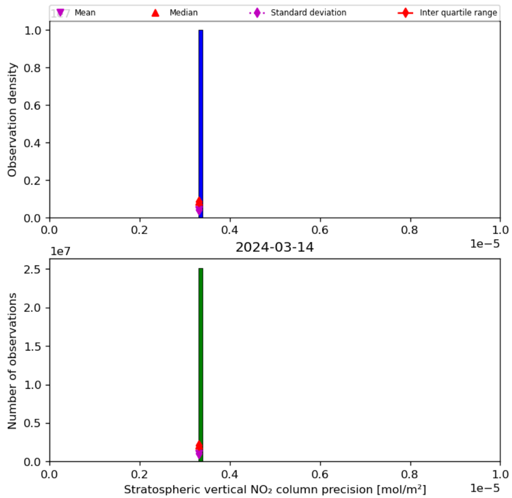
Figure 37: Histogram of “Stratospheric vertical NO 2 column precision” for 2024-03-14 to 2024-03-15
