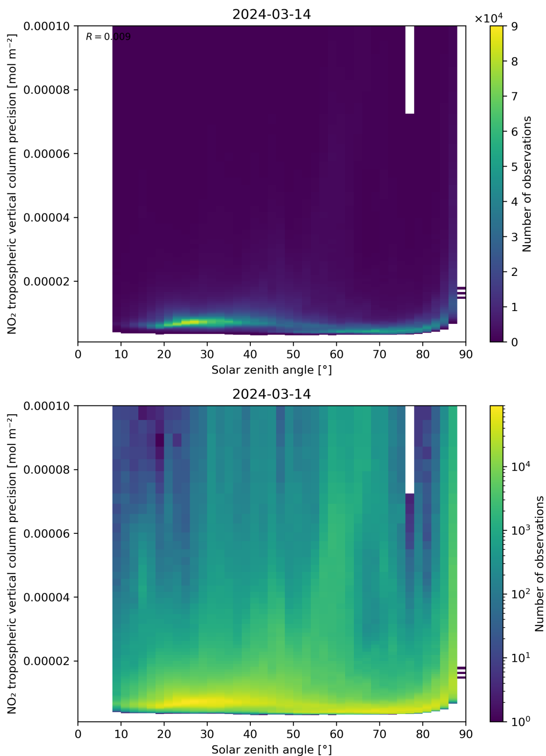
Figure 156: Scatter density plot of “Solar zenith angle” against “NO 2 tropospheric vertical column precision” for 2024-03-14 to 2024-03-15.
