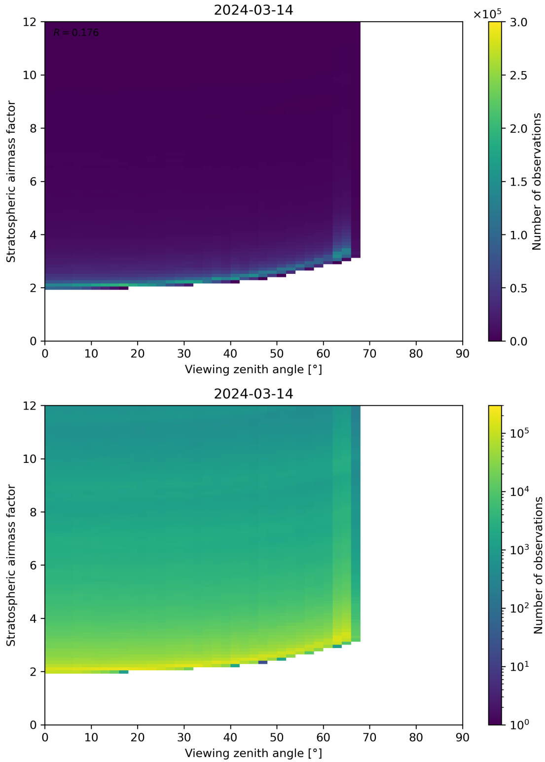
Figure 159: Scatter density plot of “Viewing zenith angle” against “Stratospheric airmass factor” for 2024-03-14 to 2024-03-15.
