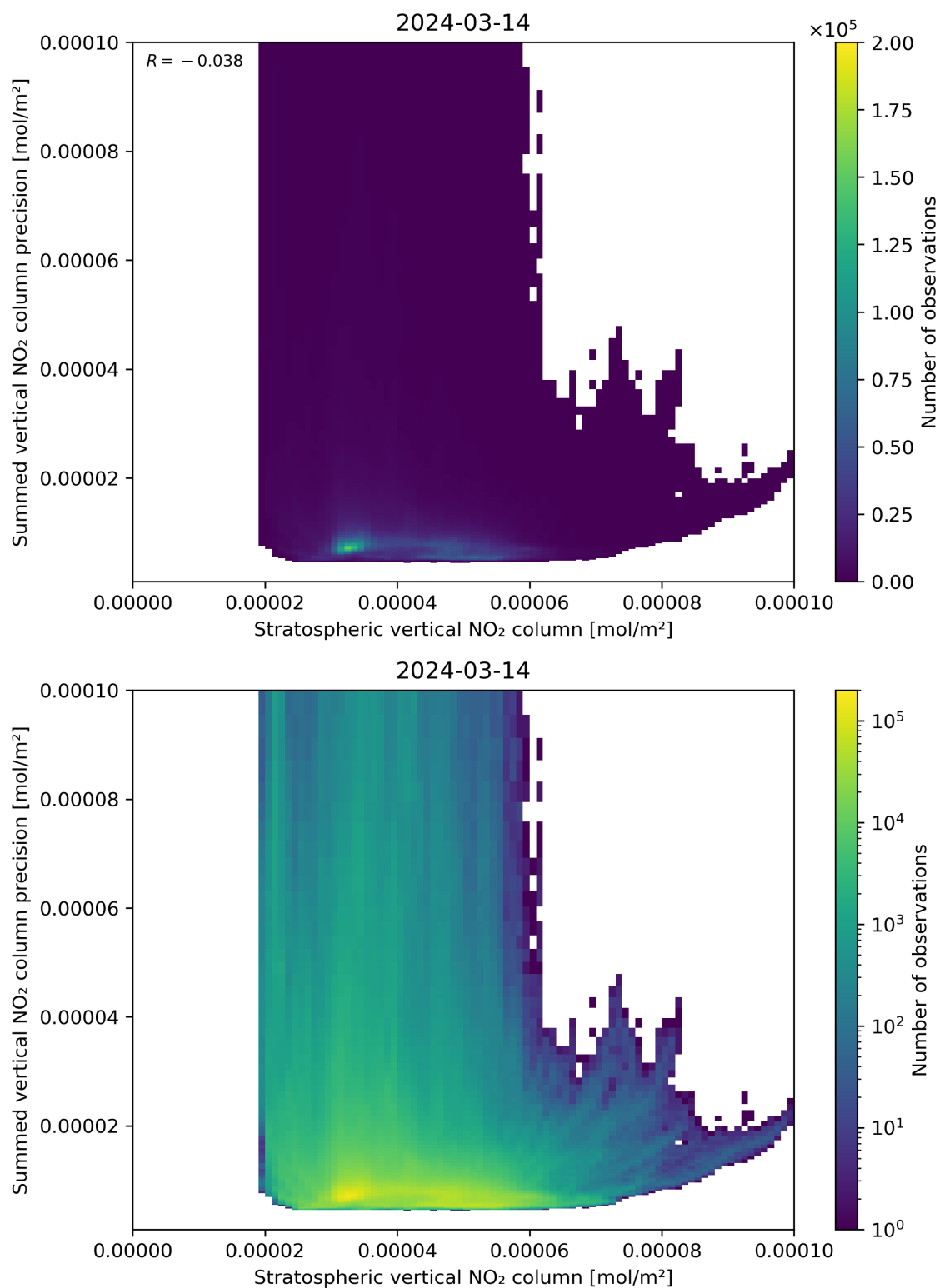
Figure 99: Scatter density plot of “Stratospheric vertical NO 2 column” against “Summed vertical NO 2 column precision” for 2024-03-14 to 2024-03-15.
