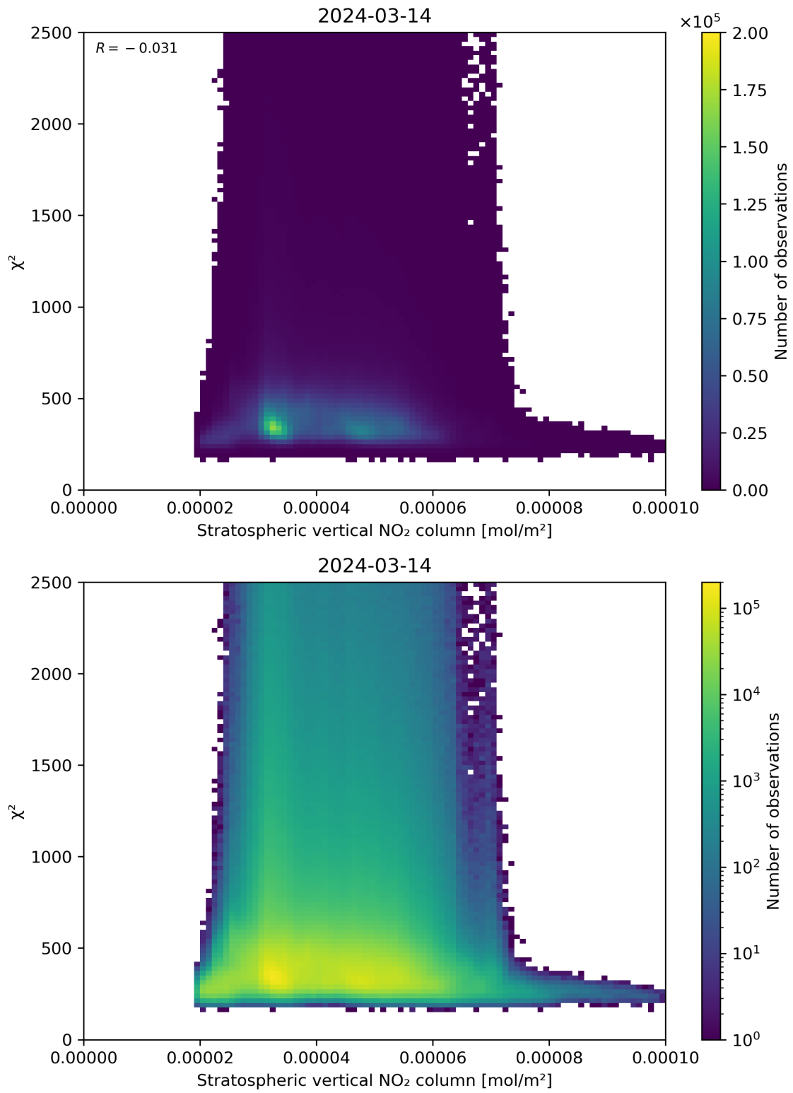
Figure 97: Scatter density plot of “Stratospheric vertical NO 2 column” against “ \chi^2 ” for 2024-03-14 to 2024-03-15.
