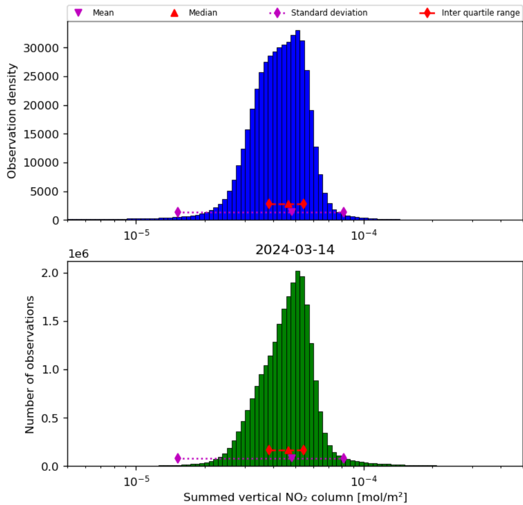
Figure 40: Histogram of “Summed vertical NO 2 column” for 2024-03-14 to 2024-03-15
