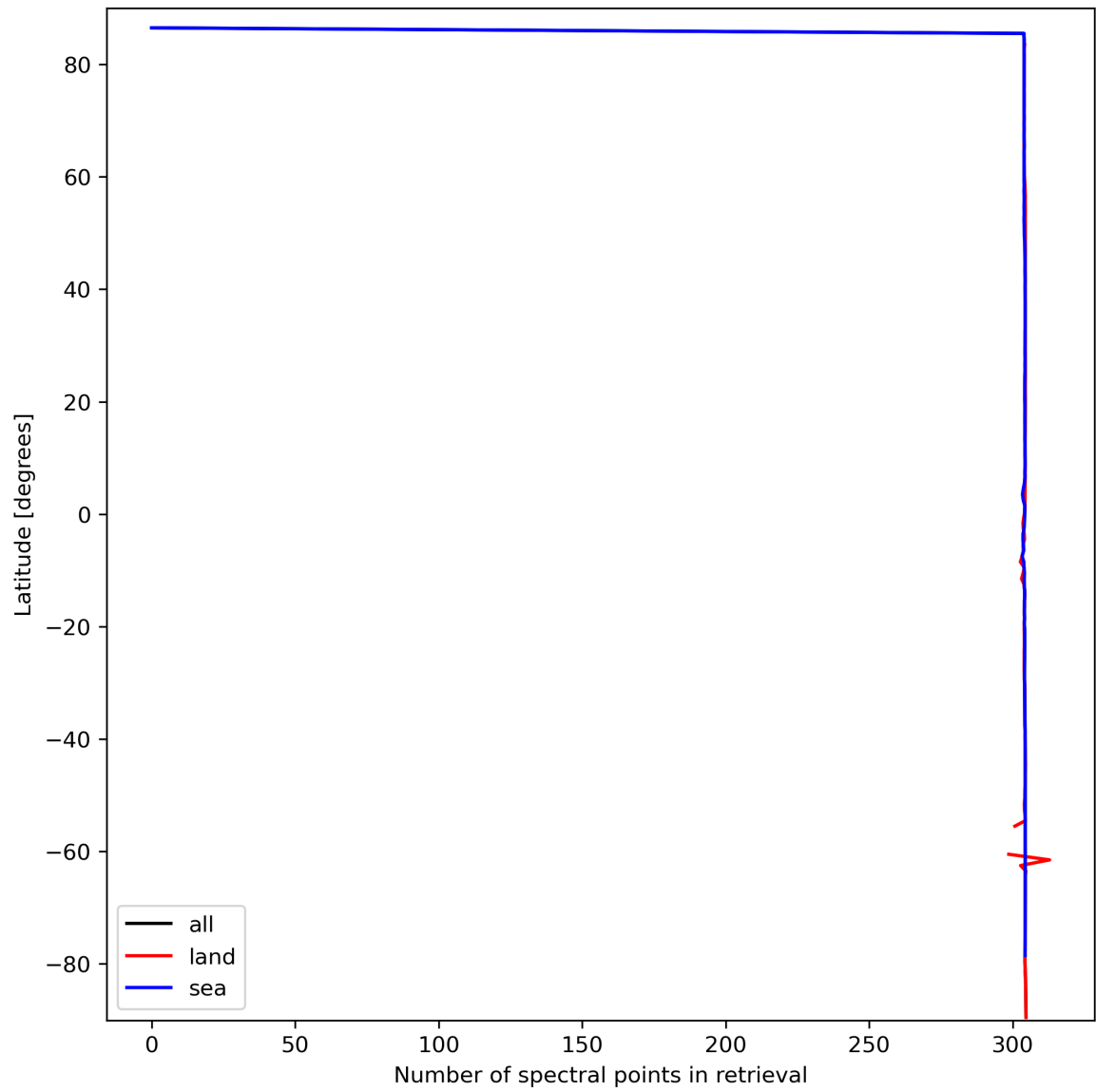
Figure 16: Zonal average of “Number of spectral points in retrieval” for 2024-03-14 to 2024-03-15.
