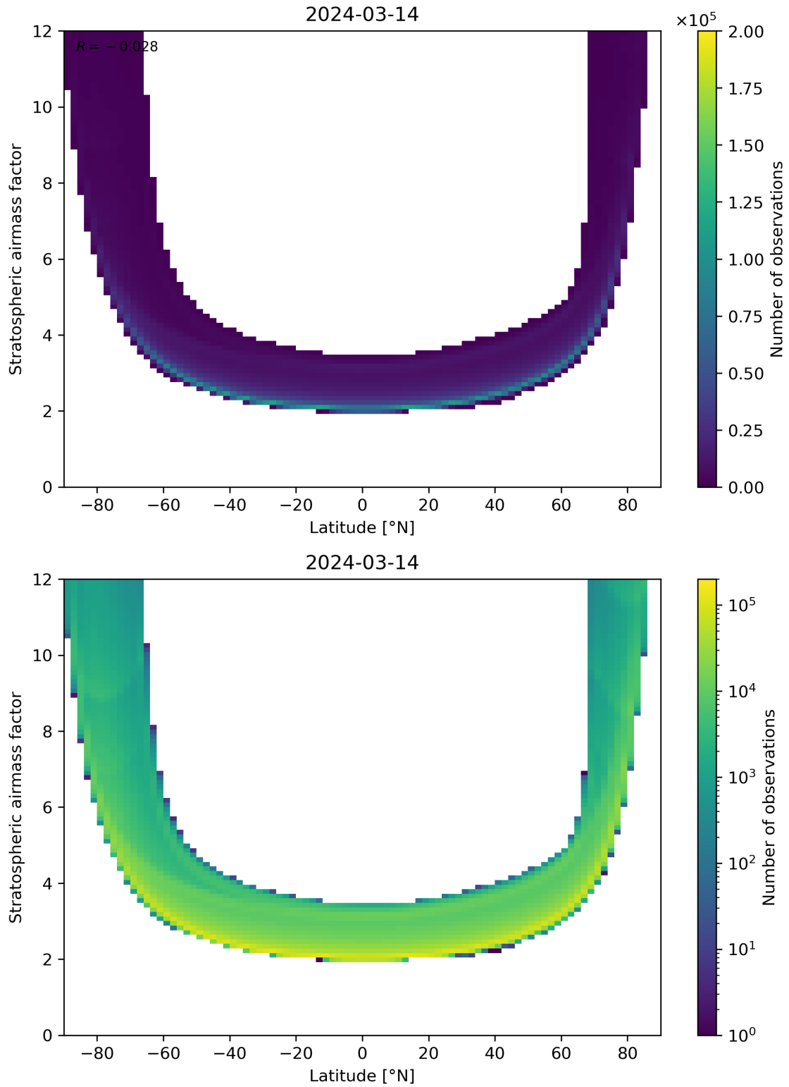
Figure 83: Scatter density plot of “Latitude” against “Stratospheric airmass factor” for 2024-03-14 to 2024-03-15.
