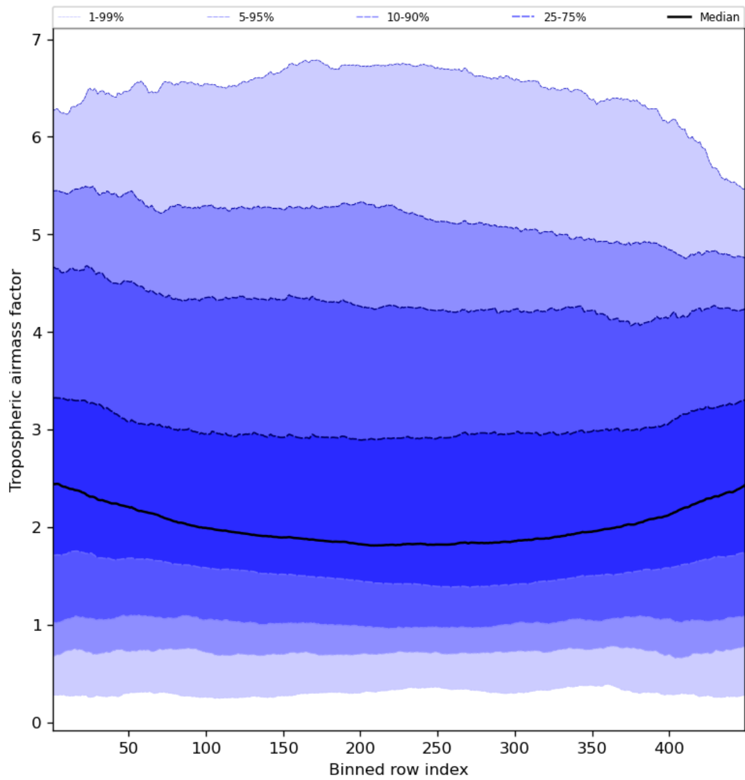
Figure 48: Along track statistics of “Tropospheric air mass factor” for 2024-03-14 to 2024-03-15
