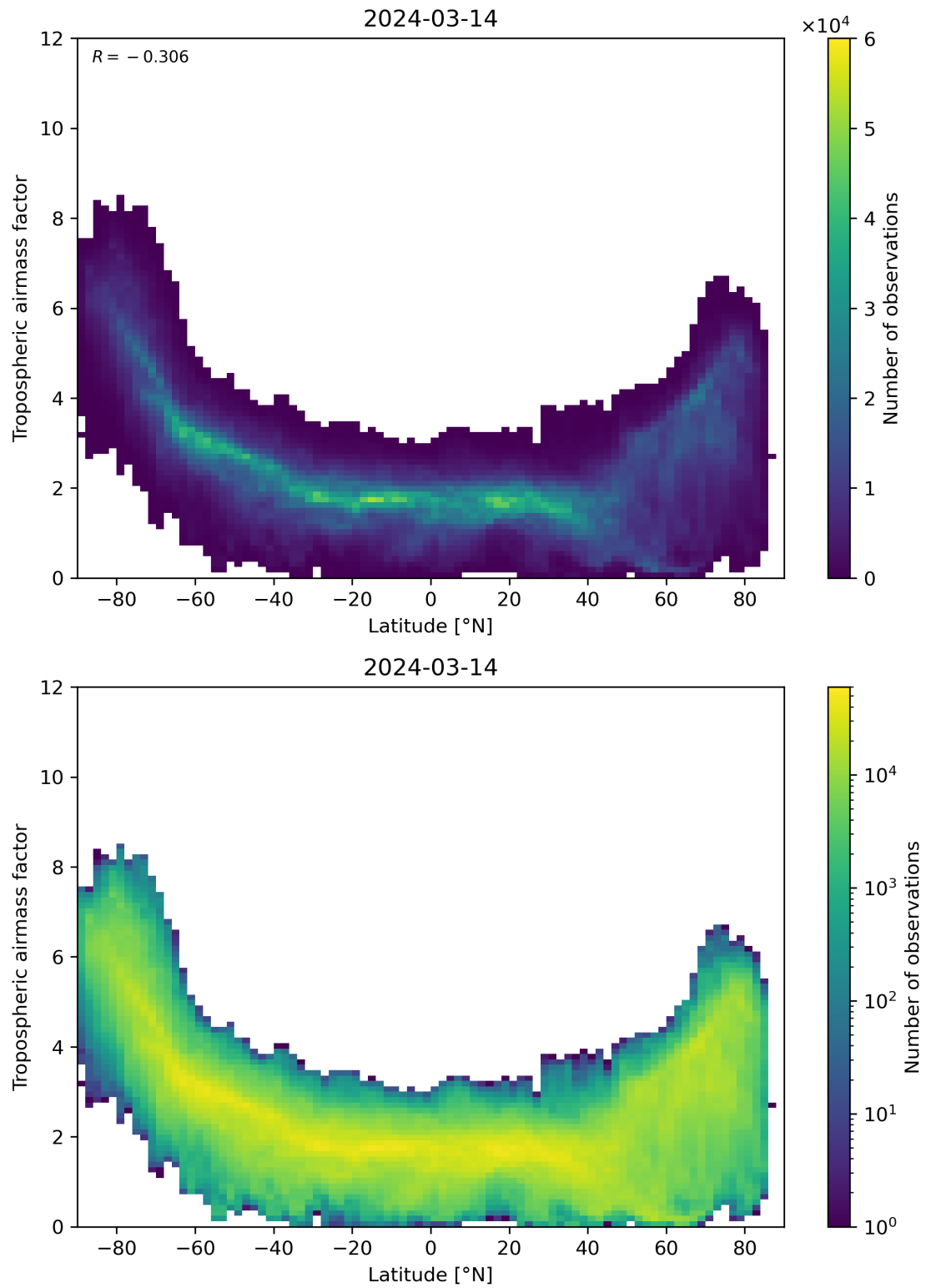
Figure 85: Scatter density plot of “Latitude” against “Tropospheric airmass factor” for 2024-03-14 to 2024-03-15.
