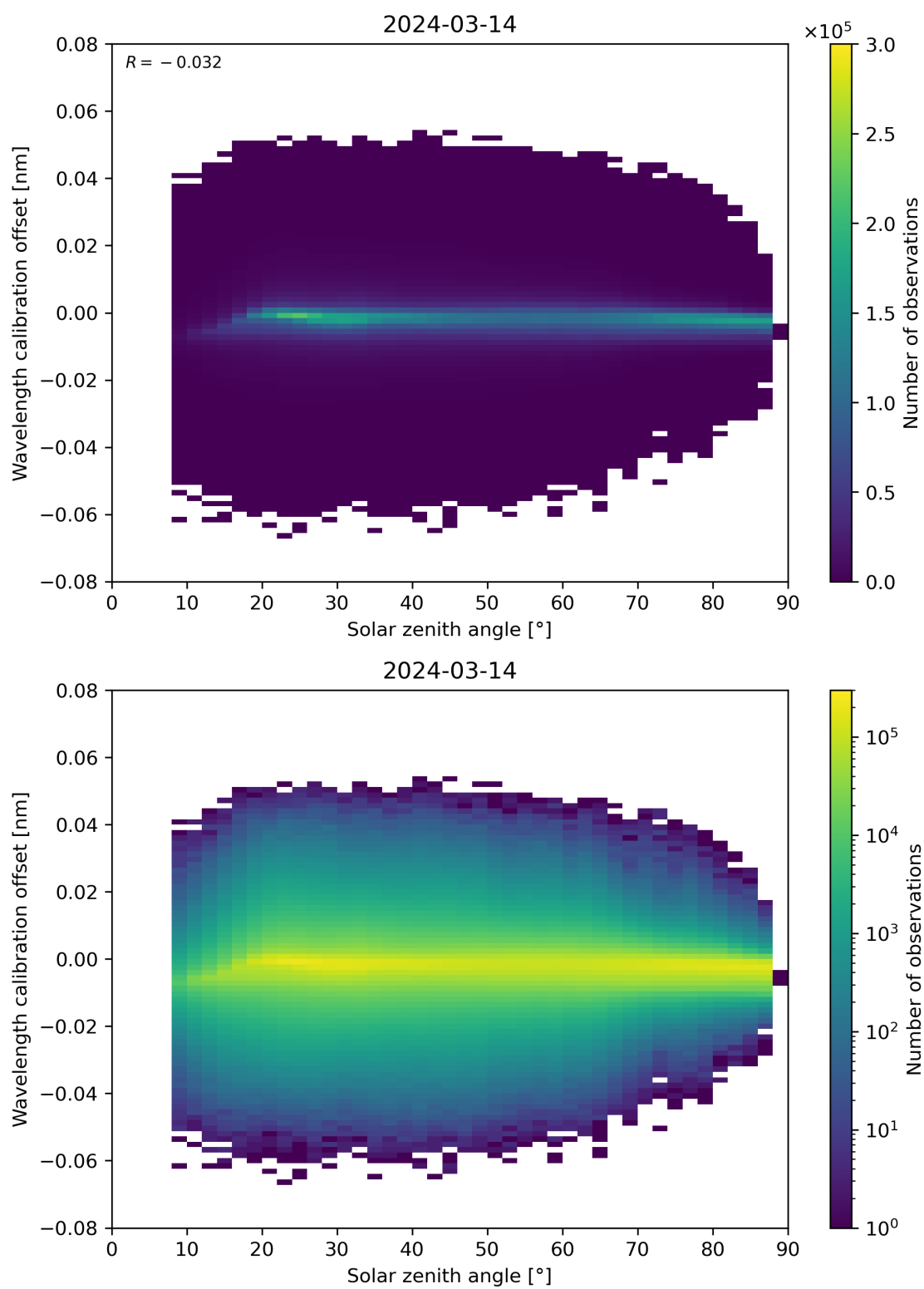
Figure 158: Scatter density plot of “Solar zenith angle” against “Wavelength calibration offset” for 2024-03-14 to 2024-03-15.
