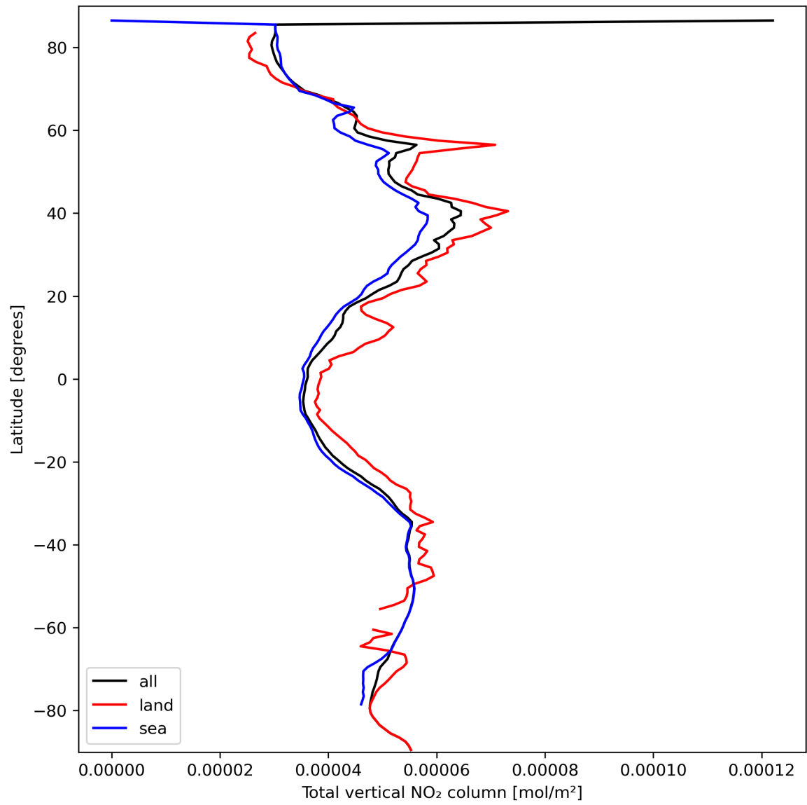
Figure 21: Zonal average of “Total vertical NO 2 column” for 2024-03-14 to 2024-03-15.
