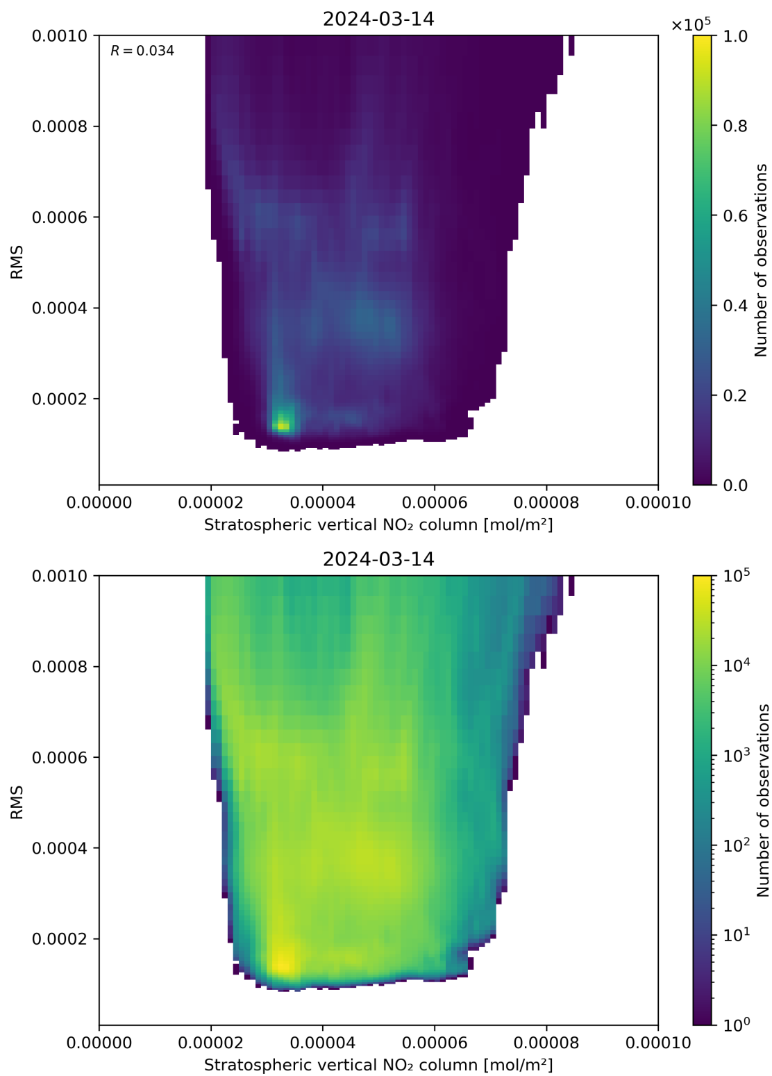
Figure 102: Scatter density plot of “Stratospheric vertical NO 2 column” against “RMS” for 2024-03-14 to 2024-03-15.
