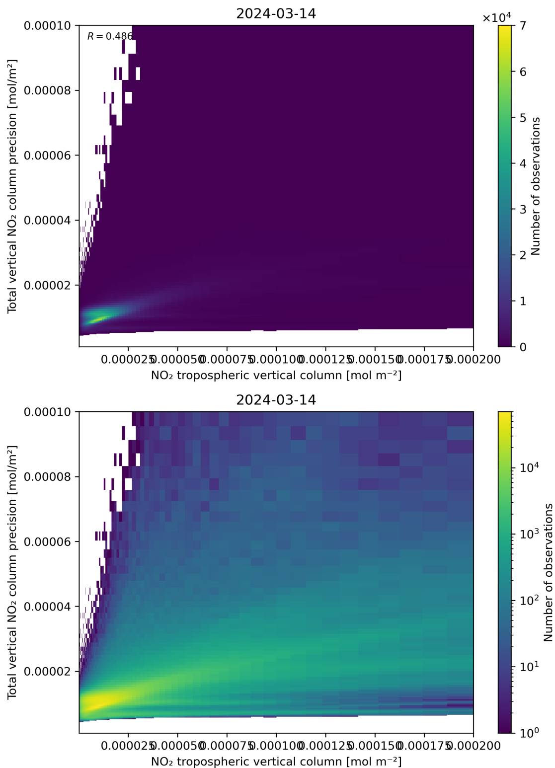
Figure 129: Scatter density plot of “NO 2 tropospheric vertical column” against “Total vertical NO 2 column precision” for 2024-03-14 to 2024-03-15.
