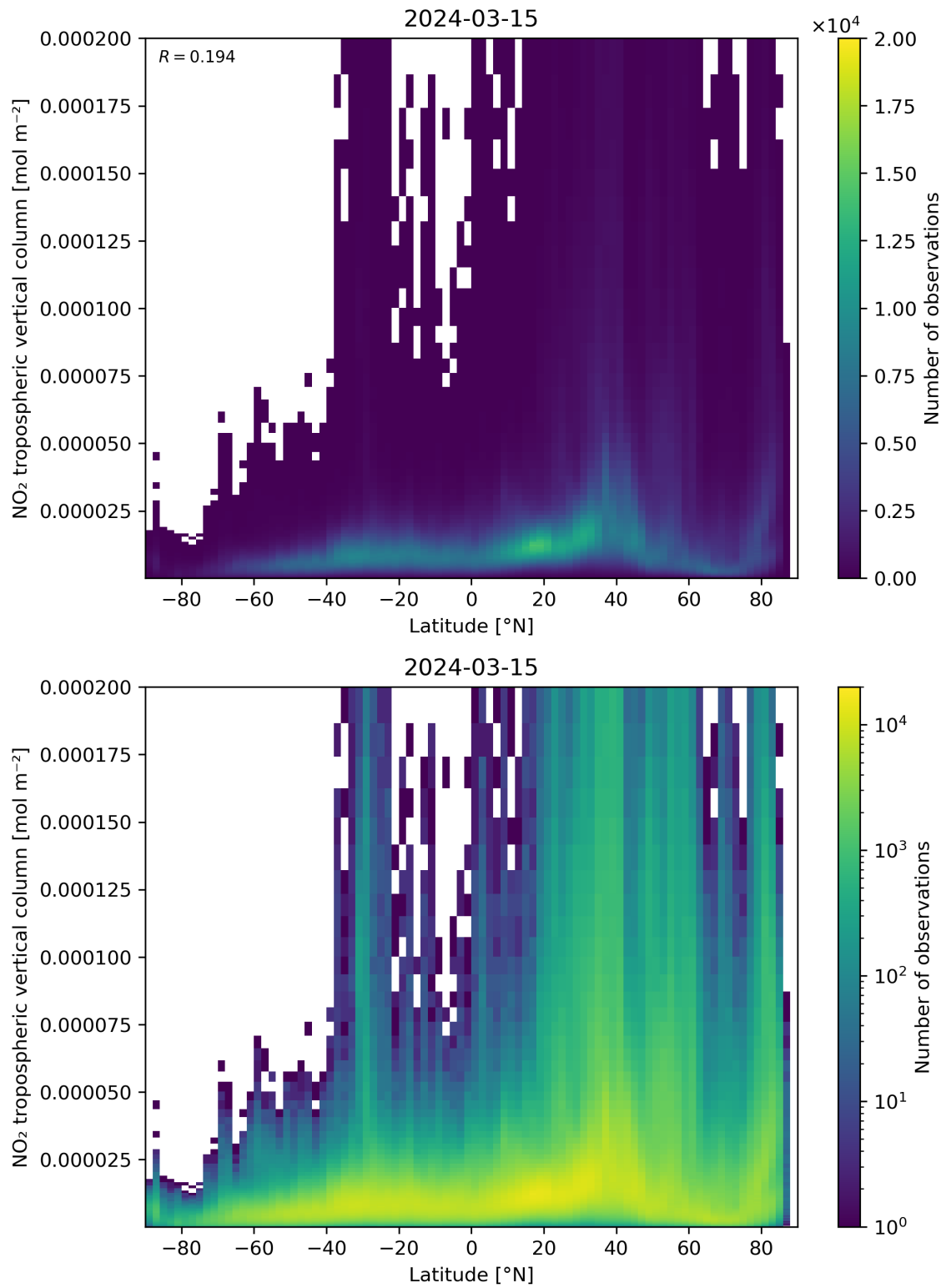
Figure 92: Scatter density plot of “Latitude” against “NO 2 tropospheric vertical column” for 2024-03-14 to 2024-03-16.
