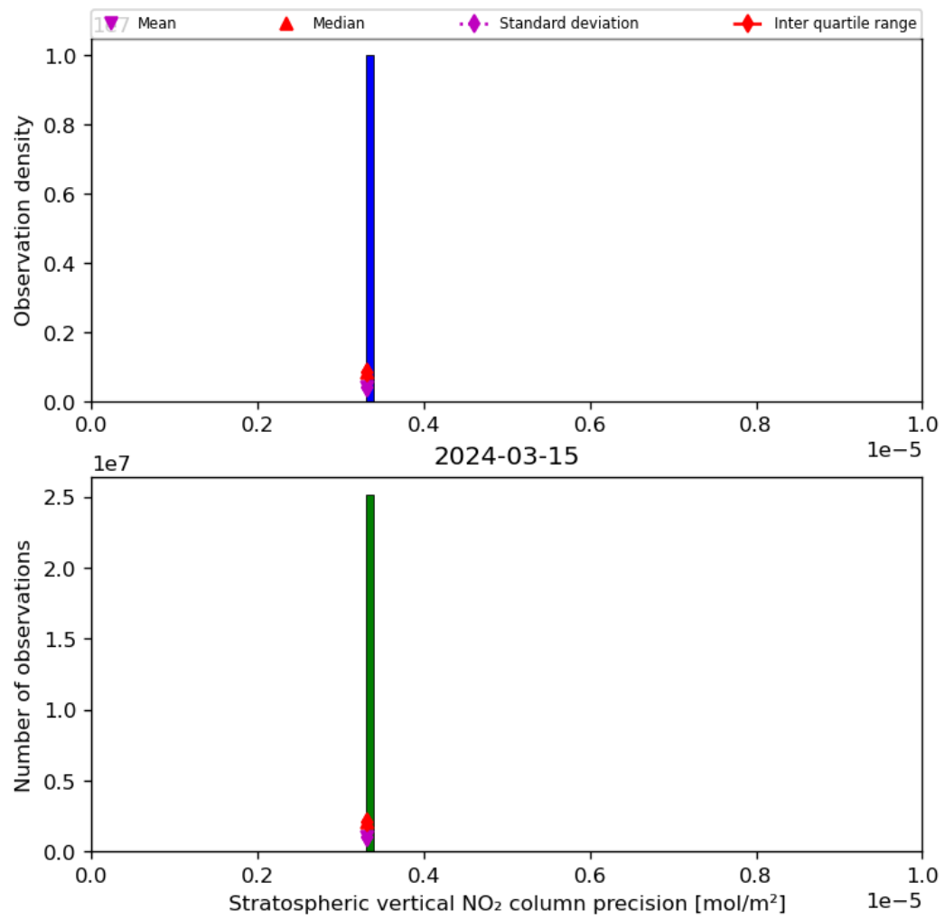
Figure 37: Histogram of “Stratospheric vertical NO 2 column precision” for 2024-03-14 to 2024-03-16
