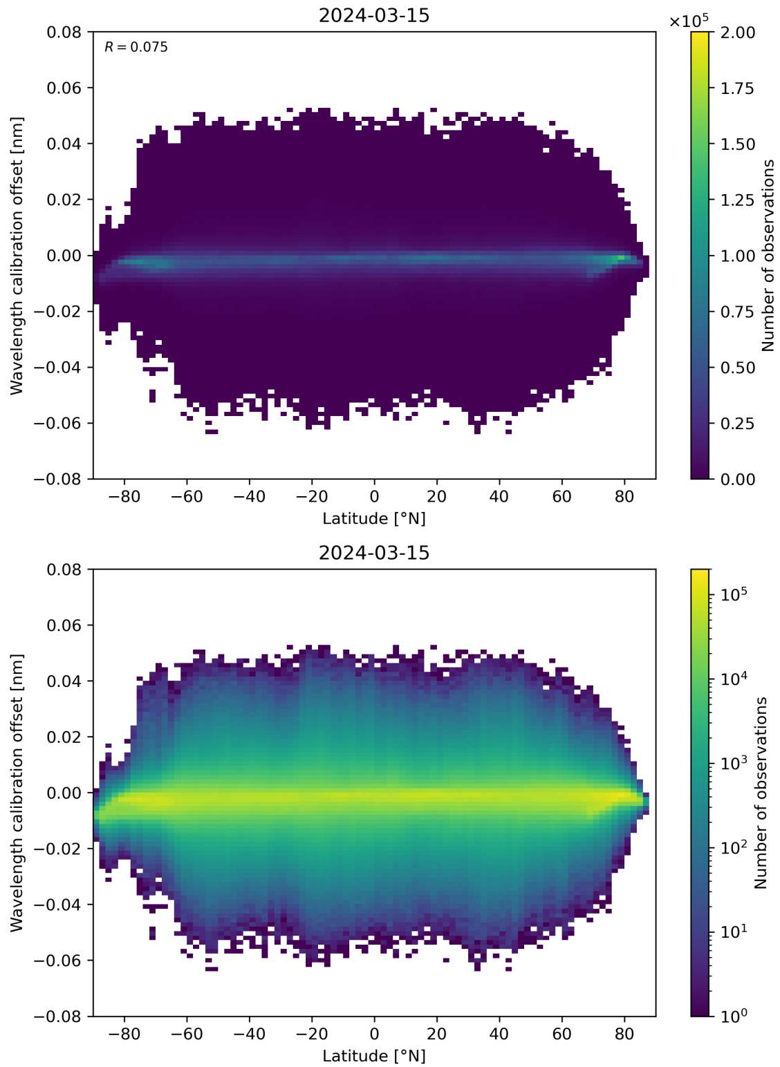
Figure 95: Scatter density plot of “Latitude” against “Wavelength calibration offset” for 2024-03-14 to 2024-03-16.
