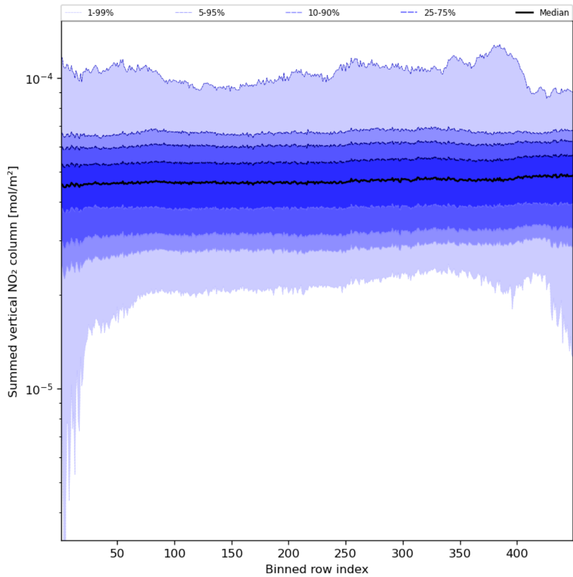
Figure 57: Along track statistics of “Summed vertical NO 2 column” for 2024-03-14 to 2024-03-16
