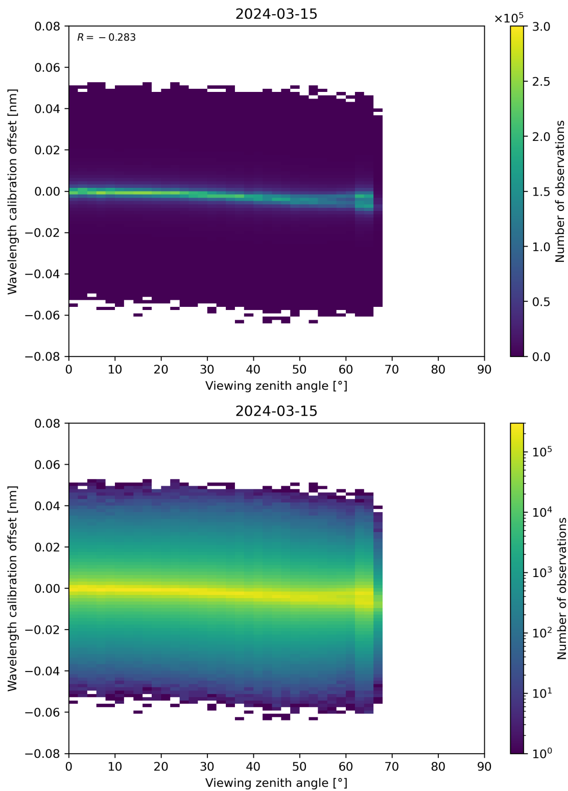
Figure 173: Scatter density plot of “Viewing zenith angle” against “Wavelength calibration offset” for 2024-03-14 to 2024-03-16.
