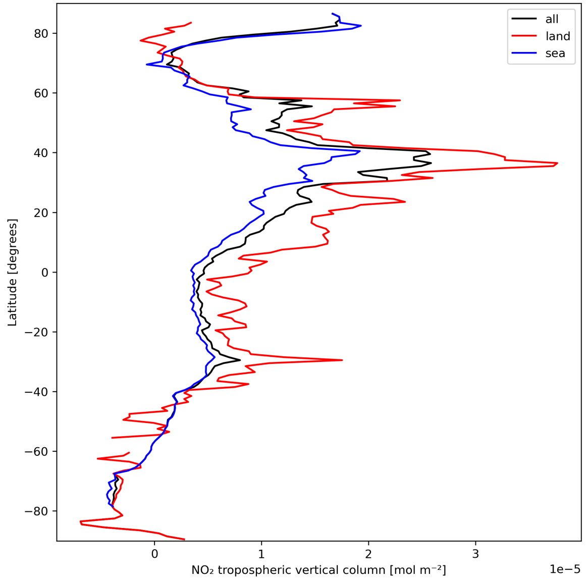
Figure 12: Zonal average of “NO 2 tropospheric vertical column” for 2024-03-14 to 2024-03-16.
