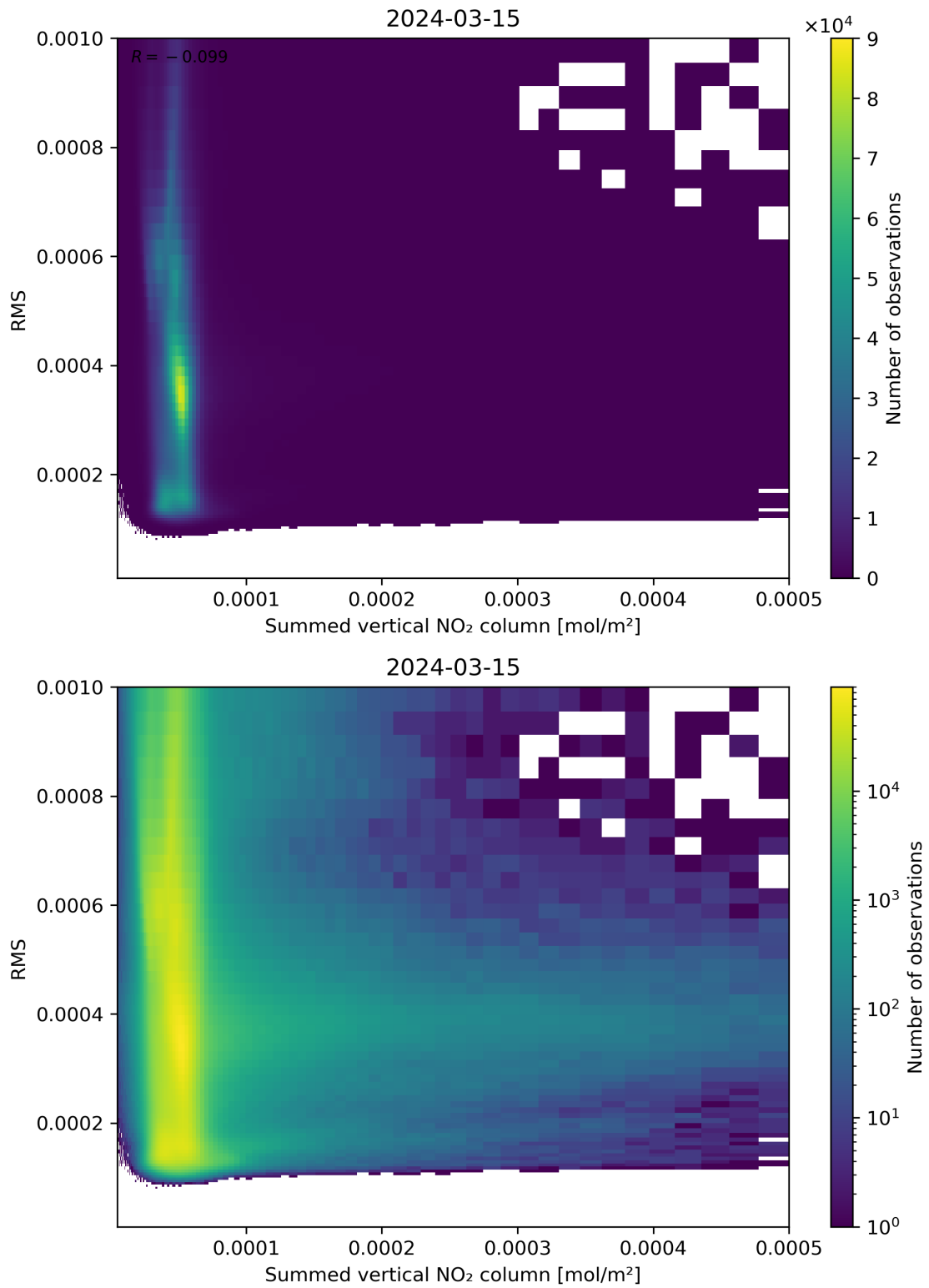
Figure 109: Scatter density plot of “Summed vertical NO 2 column” against “RMS” for 2024-03-14 to 2024-03-16.
