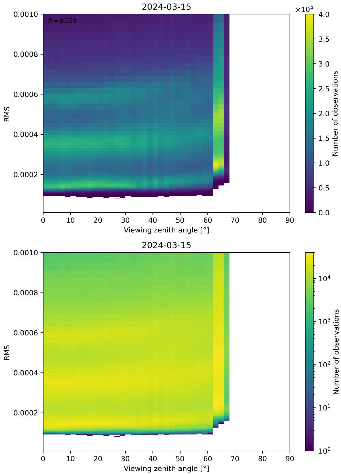
Figure 171: Scatter density plot of “Viewing zenith angle” against “RMS” for 2024-03-14 to 2024-03-16.
