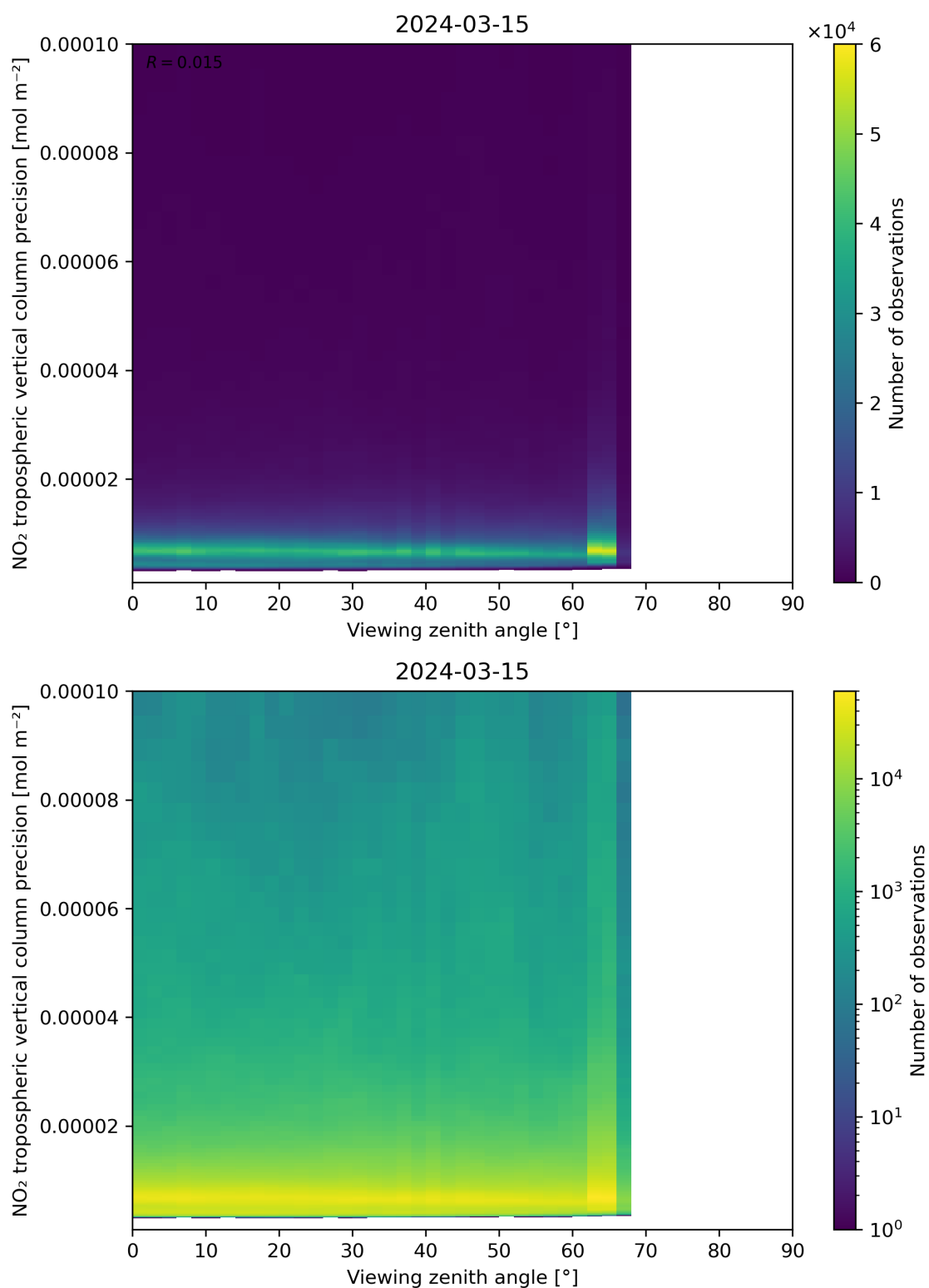
Figure 170: Scatter density plot of “Viewing zenith angle” against “NO 2 tropospheric vertical column precision” for 2024-03-14 to 2024-03-16.
