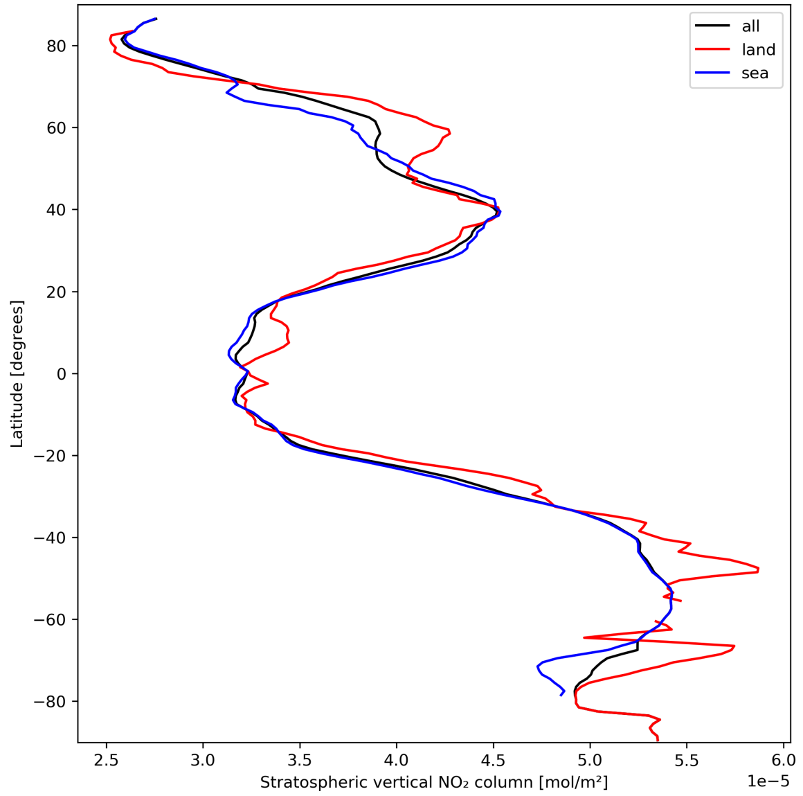
Figure 19: Zonal average of “Stratospheric vertical NO 2 column” for 2024-03-14 to 2024-03-16.
