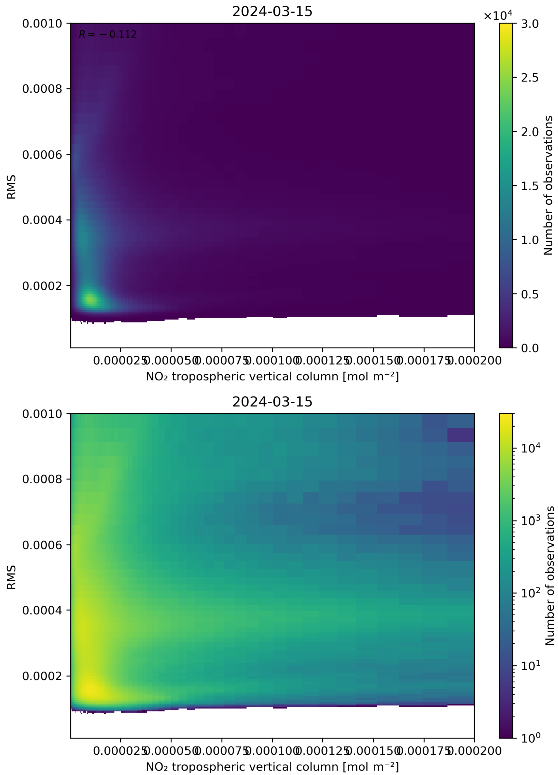
Figure 142: Scatter density plot of “NO 2 tropospheric vertical column” against “RMS” for 2024-03-14 to 2024-03-16.
