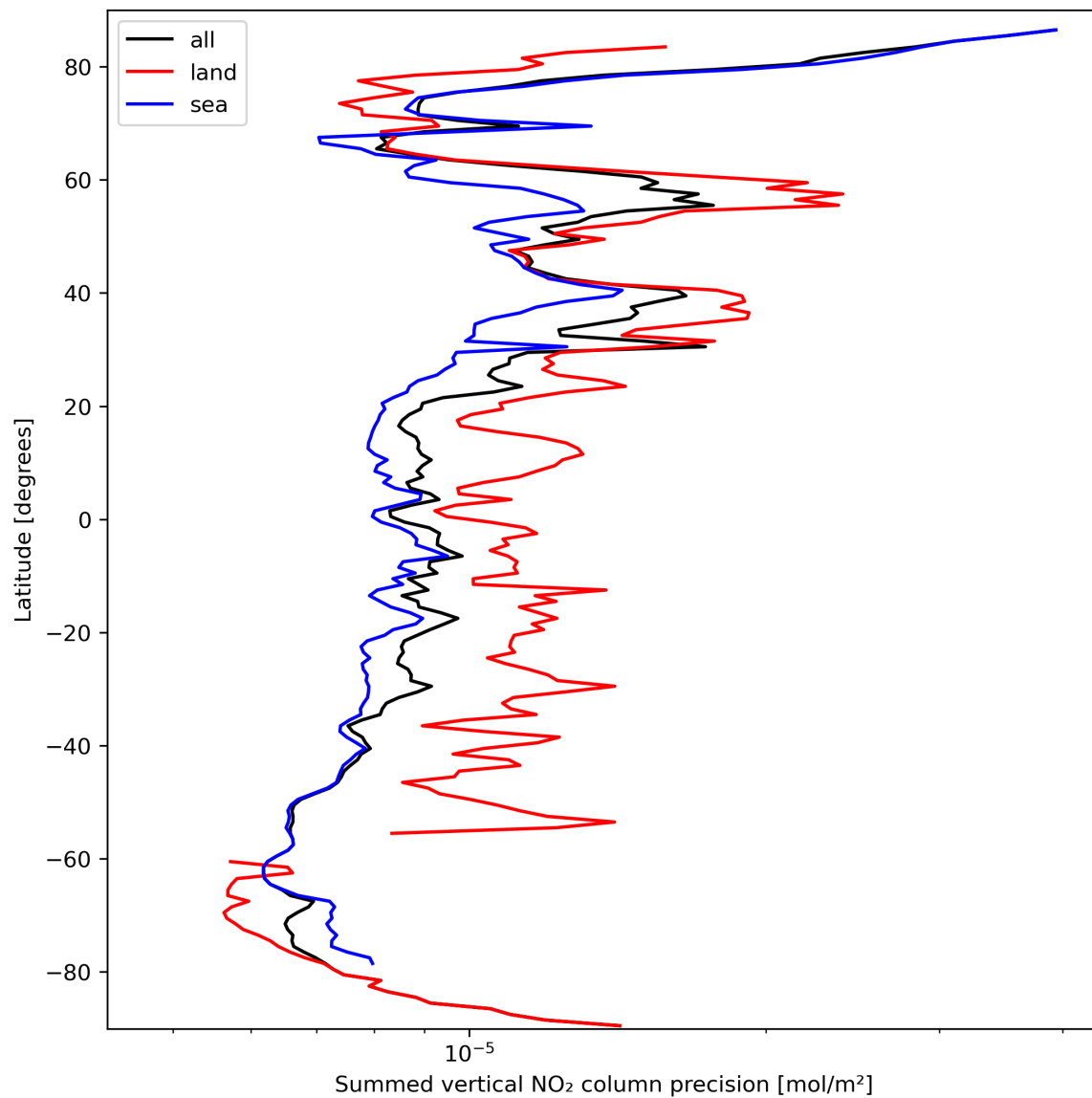
Figure 24: Zonal average of “Summed vertical NO 2 column precision” for 2024-03-14 to 2024-03-16.
