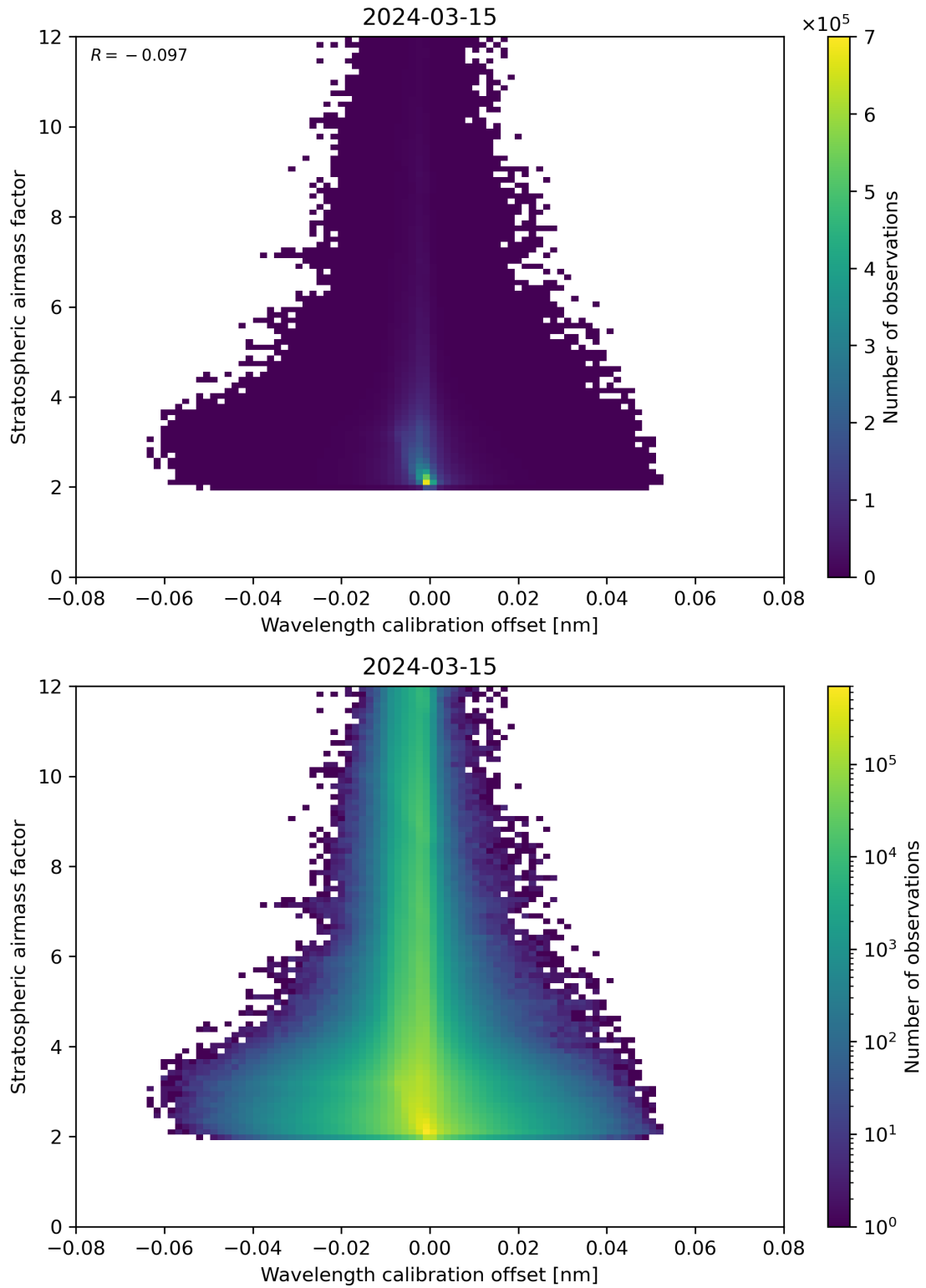
Figure 174: Scatter density plot of “Wavelength calibration offset” against “Stratospheric air mass factor” for 2024-03-14 to 2024-03-16.
