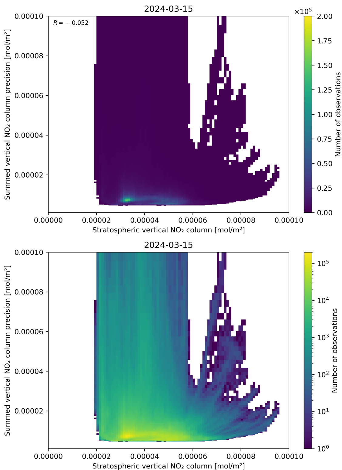
Figure 99: Scatter density plot of “Stratospheric vertical NO 2 column” against “Summed vertical NO 2 column precision” for 2024-03-14 to 2024-03-16.
