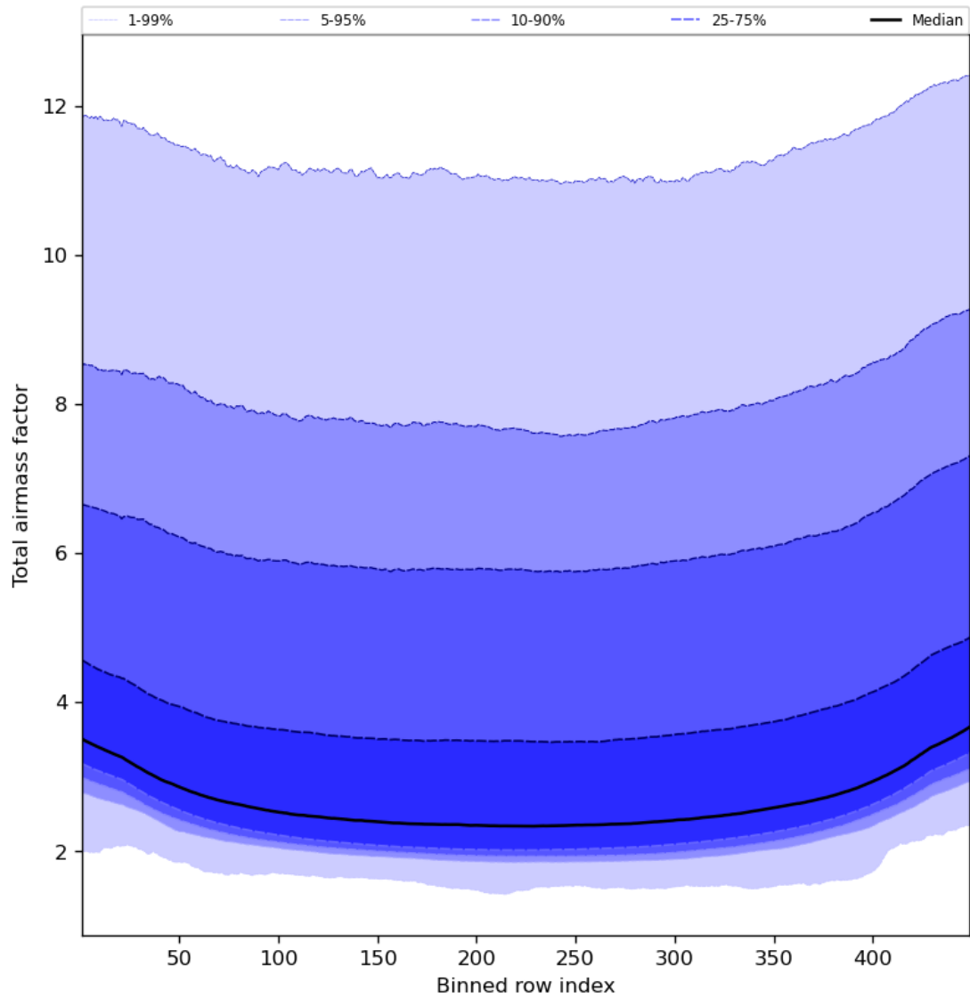
Figure 49: Along track statistics of “Total airmass factor” for 2024-03-14 to 2024-03-16
