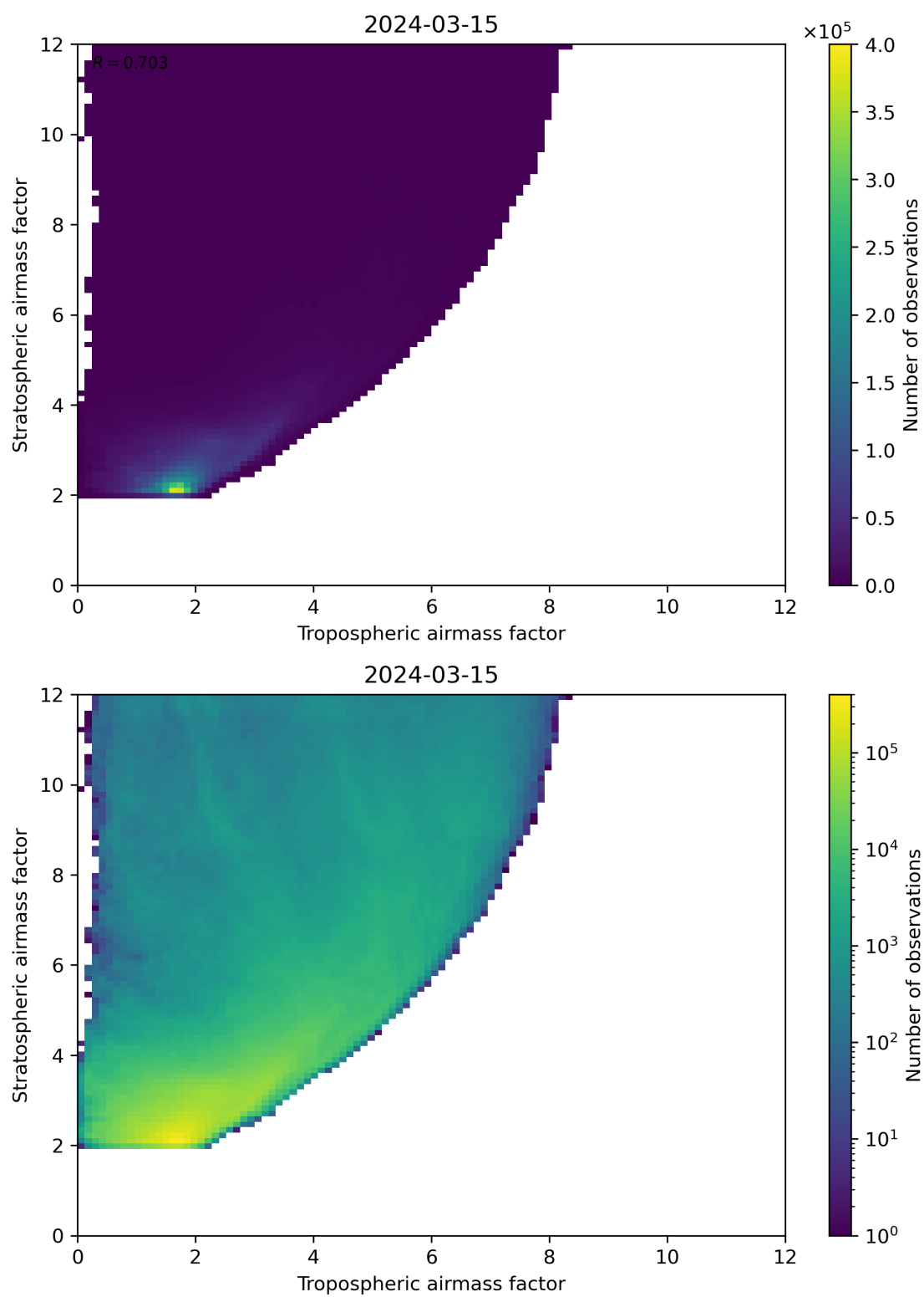
Figure 71: Scatter density plot of “Tropospheric airmass factor” against “Stratospheric airmass factor” for 2024-03-14 to 2024-03-16.
