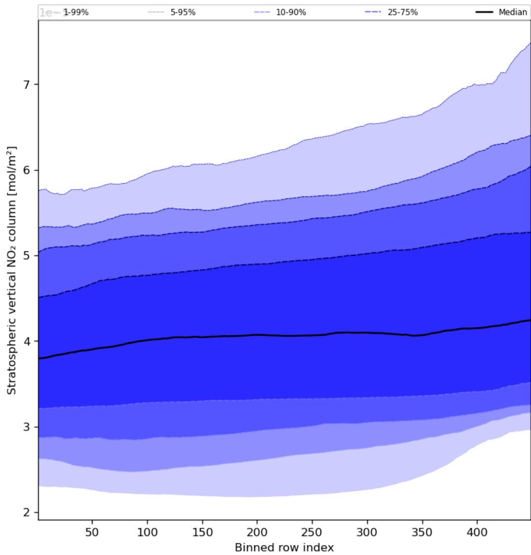
Figure 53: Along track statistics of “Stratospheric vertical NO 2 column” for 2024-03-14 to 2024-03-16
