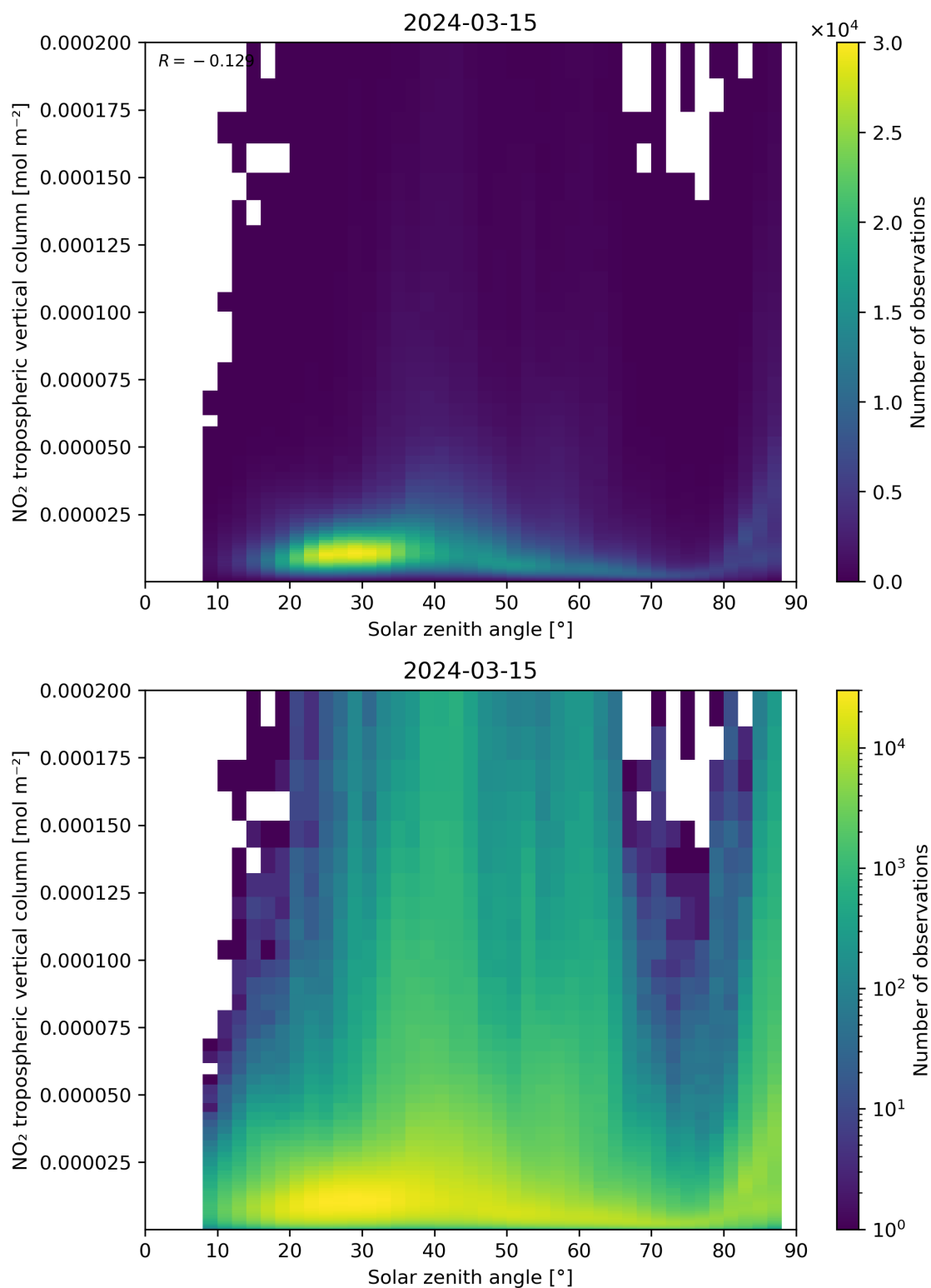
Figure 155: Scatter density plot of “Solar zenith angle” against “NO 2 tropospheric vertical column” for 2024-03-14 to 2024-03-16.
