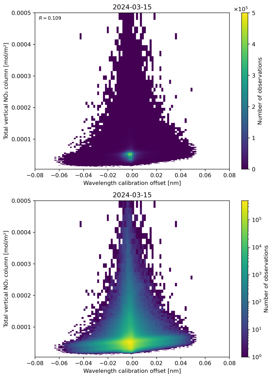
Figure 179: Scatter density plot of “Wavelength calibration offset” against “Total vertical NO 2 column” for 2024-03-14 to 2024-03-16.
