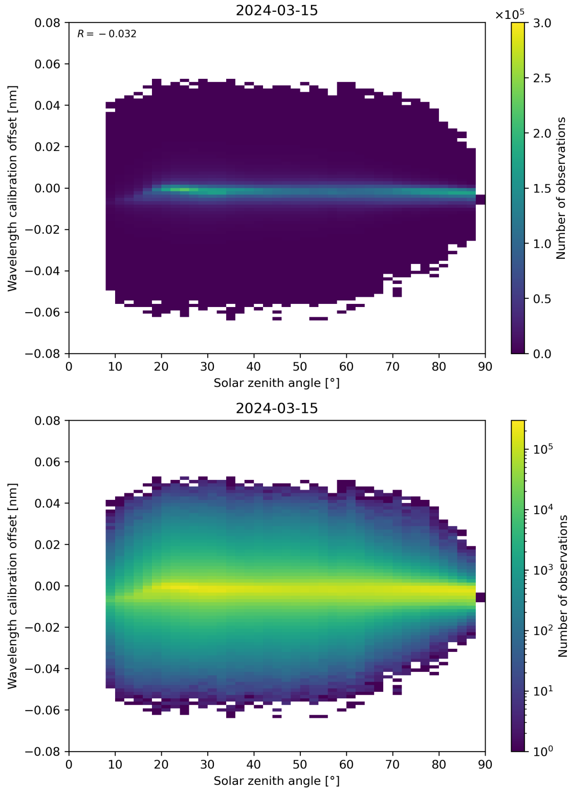
Figure 158: Scatter density plot of “Solar zenith angle” against “Wavelength calibration offset” for 2024-03-14 to 2024-03-16.
