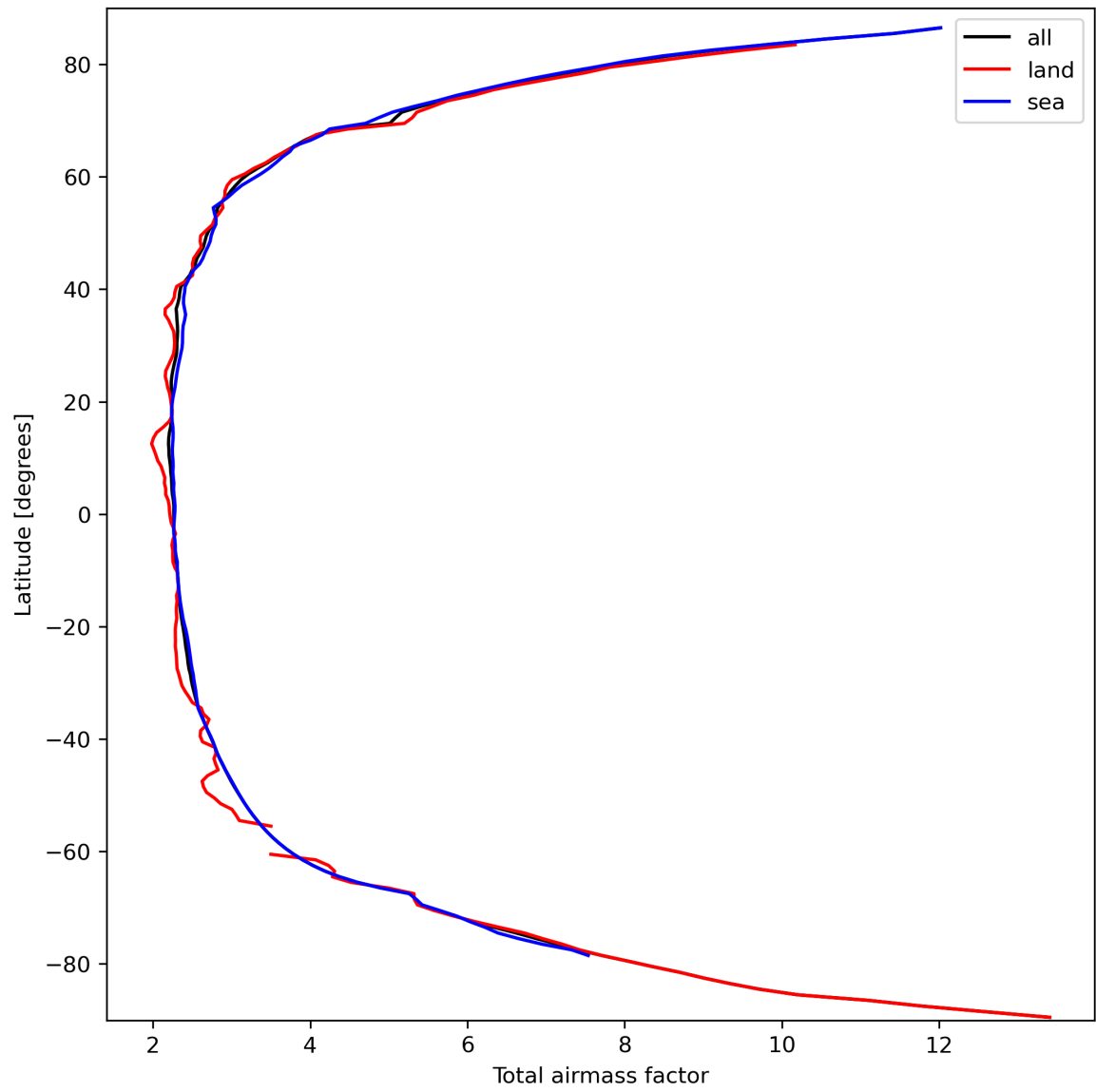
Figure 15: Zonal average of “Total airmass factor” for 2024-03-14 to 2024-03-16.
