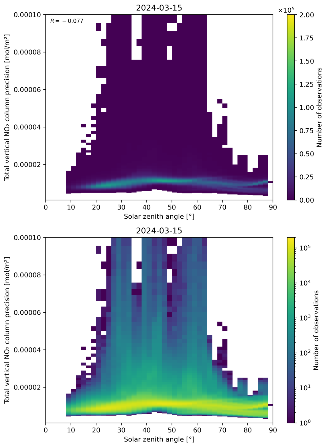
Figure 154: Scatter density plot of “Solar zenith angle” against “Total vertical NO 2 column precision” for 2024-03-14 to 2024-03-16.
