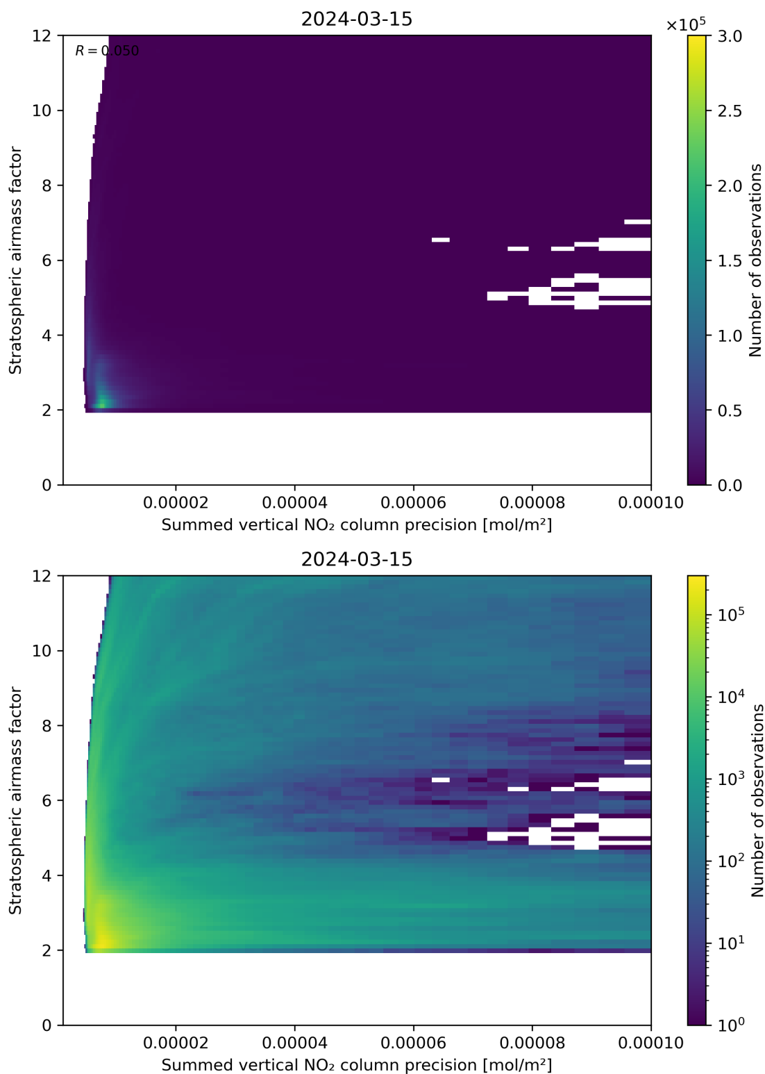
Figure 106: Scatter density plot of “Summed vertical NO 2 column precision” against “Stratospheric airmass factor” for 2024-03-14 to 2024-03-16.
