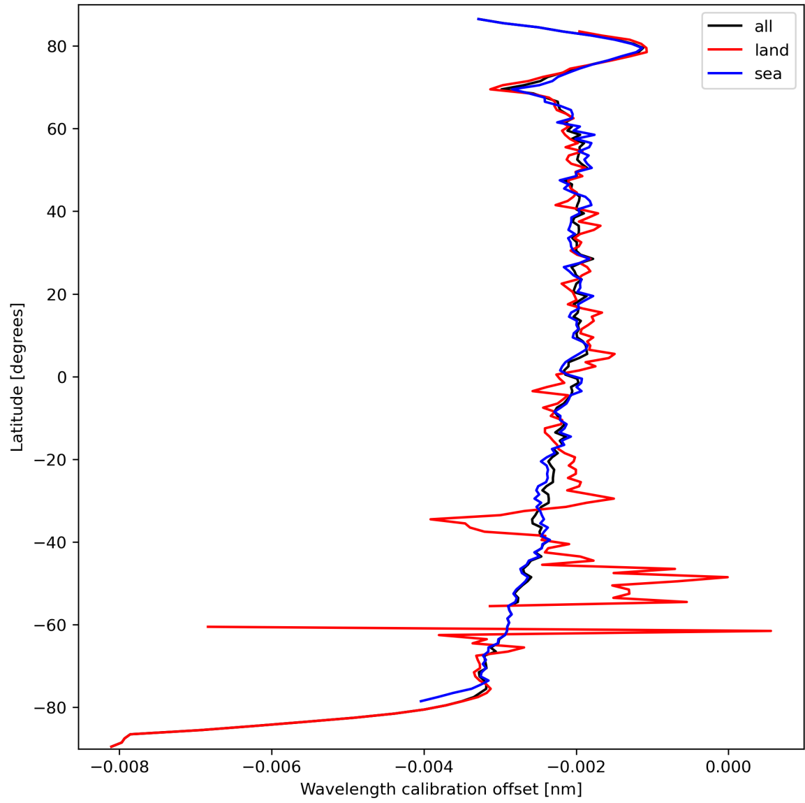
Figure 18: Zonal average of “Wavelength calibration offset” for 2024-03-14 to 2024-03-16.
