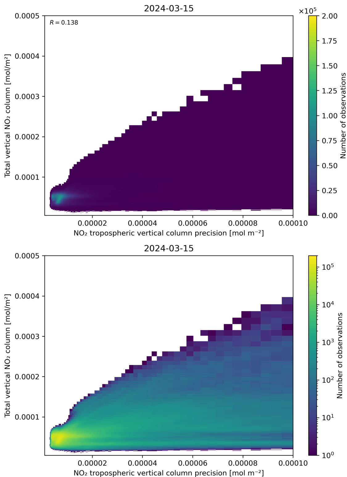
Figure 138: Scatter density plot of “NO 2 tropospheric vertical column precision” against “Total vertical NO 2 column” for 2024-03-14 to 2024-03-16.
