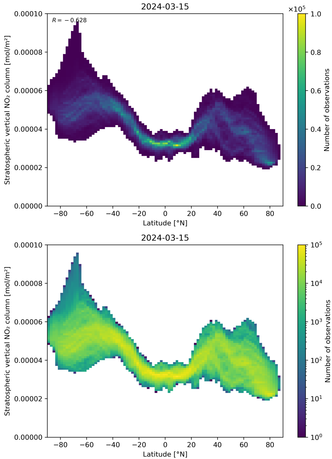
Figure 87: Scatter density plot of “Latitude” against “Stratospheric vertical NO 2 column” for 2024-03-14 to 2024-03-16.
