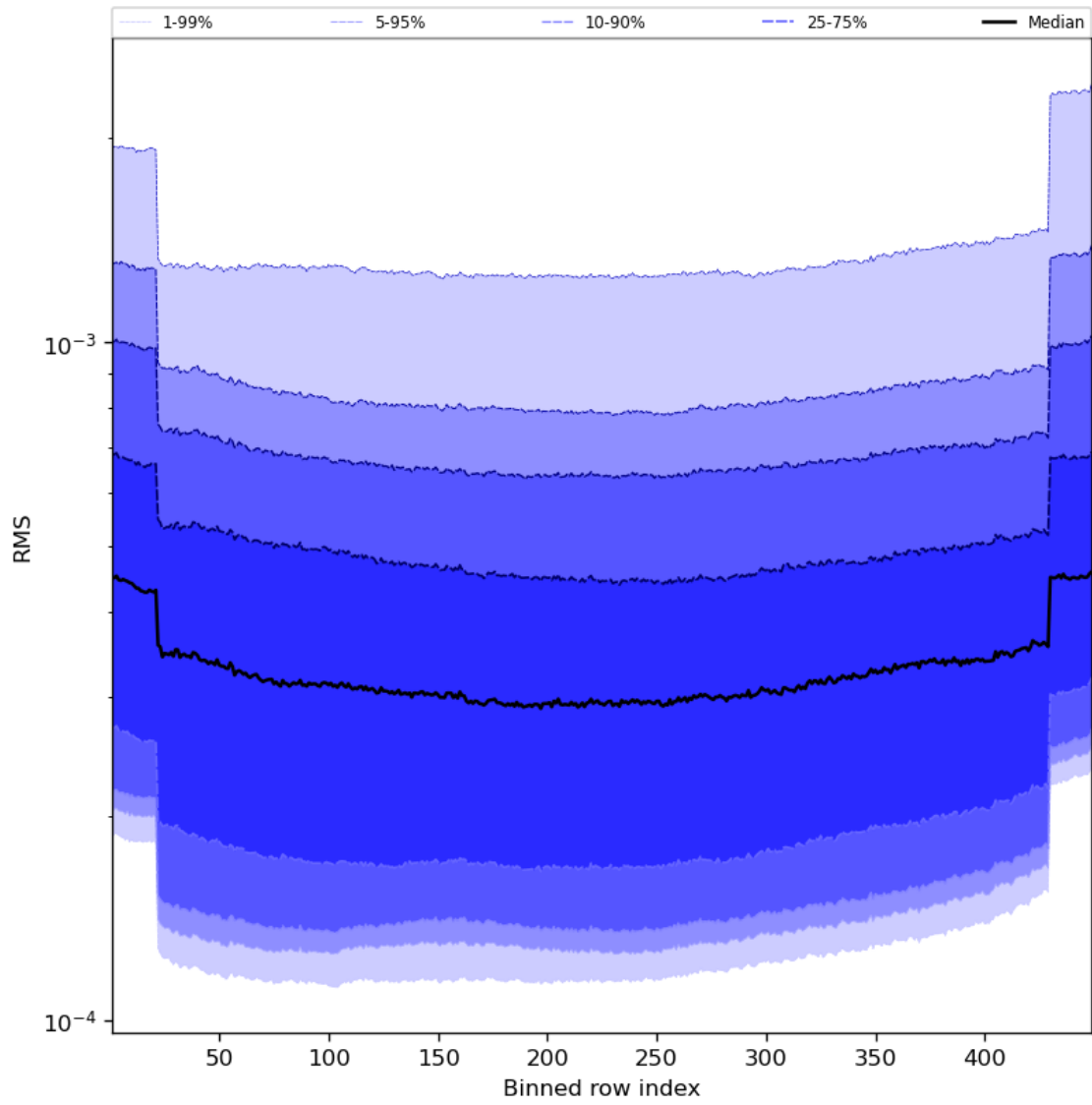
Figure 60: Along track statistics of “RMS” for 2024-03-14 to 2024-03-16
