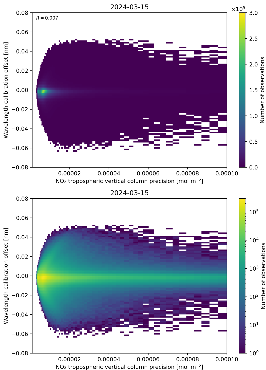
Figure 141: Scatter density plot of “NO 2 tropospheric vertical column precision” against “Wavelength calibration offset” for 2024-03-14 to 2024-03-16.
