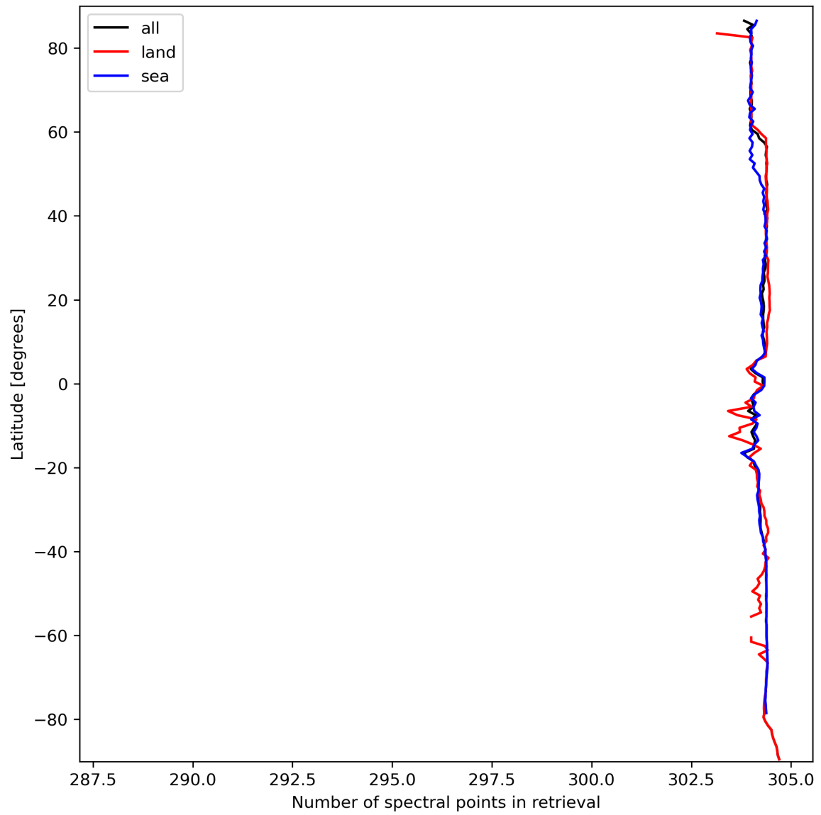
Figure 16: Zonal average of “Number of spectral points in retrieval” for 2024-03-14 to 2024-03-16.
