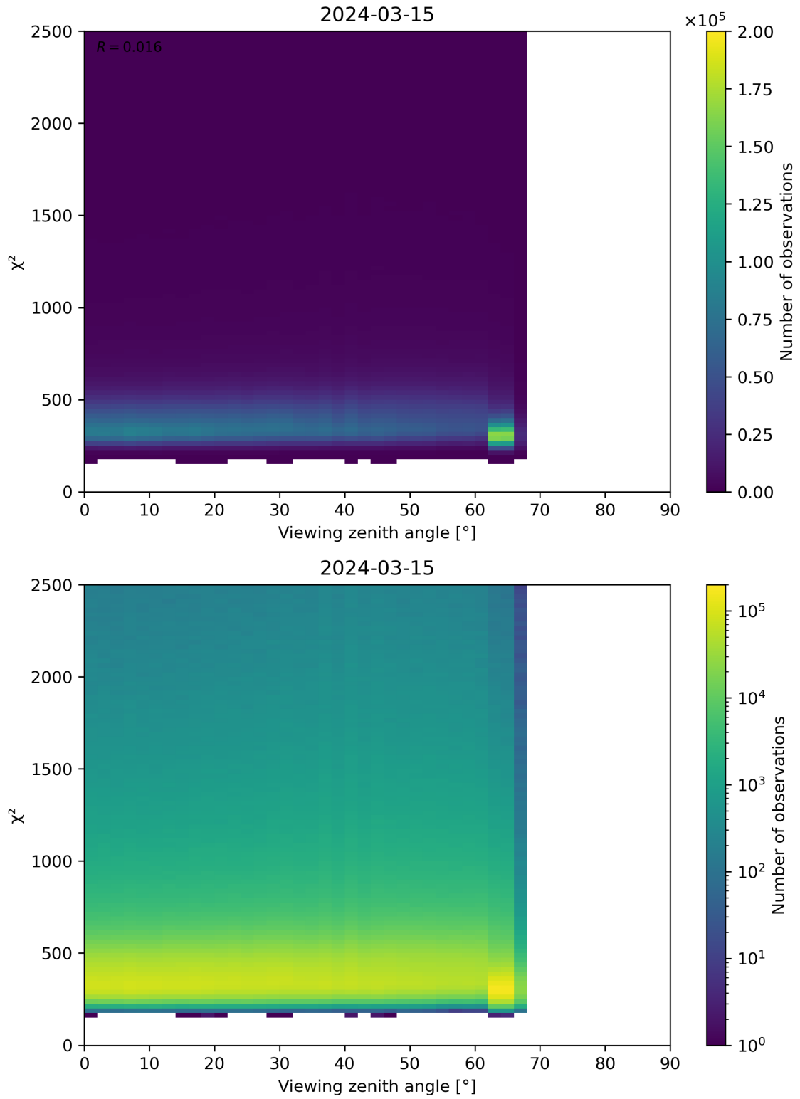
Figure 162: Scatter density plot of “Viewing zenith angle” against “ \chi^2 ” for 2024-03-14 to 2024-03-16.
