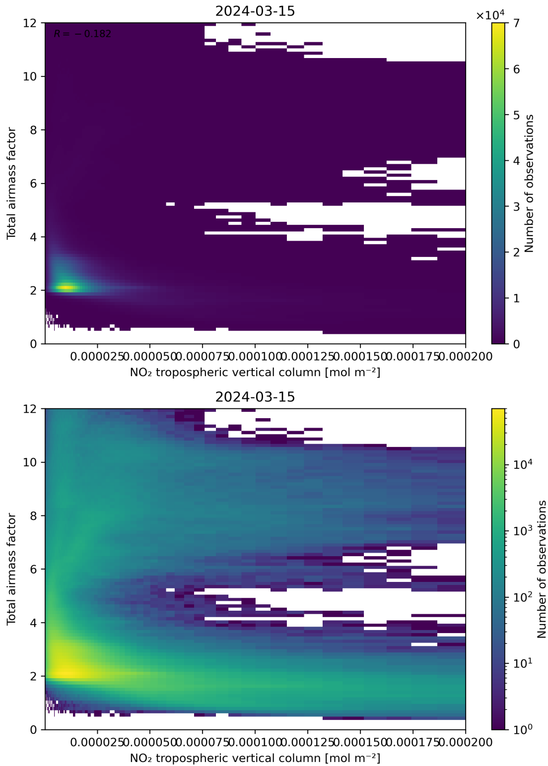
Figure 122: Scatter density plot of “NO 2 tropospheric vertical column” against “Total air mass factor” for 2024-03-14 to 2024-03-16.
