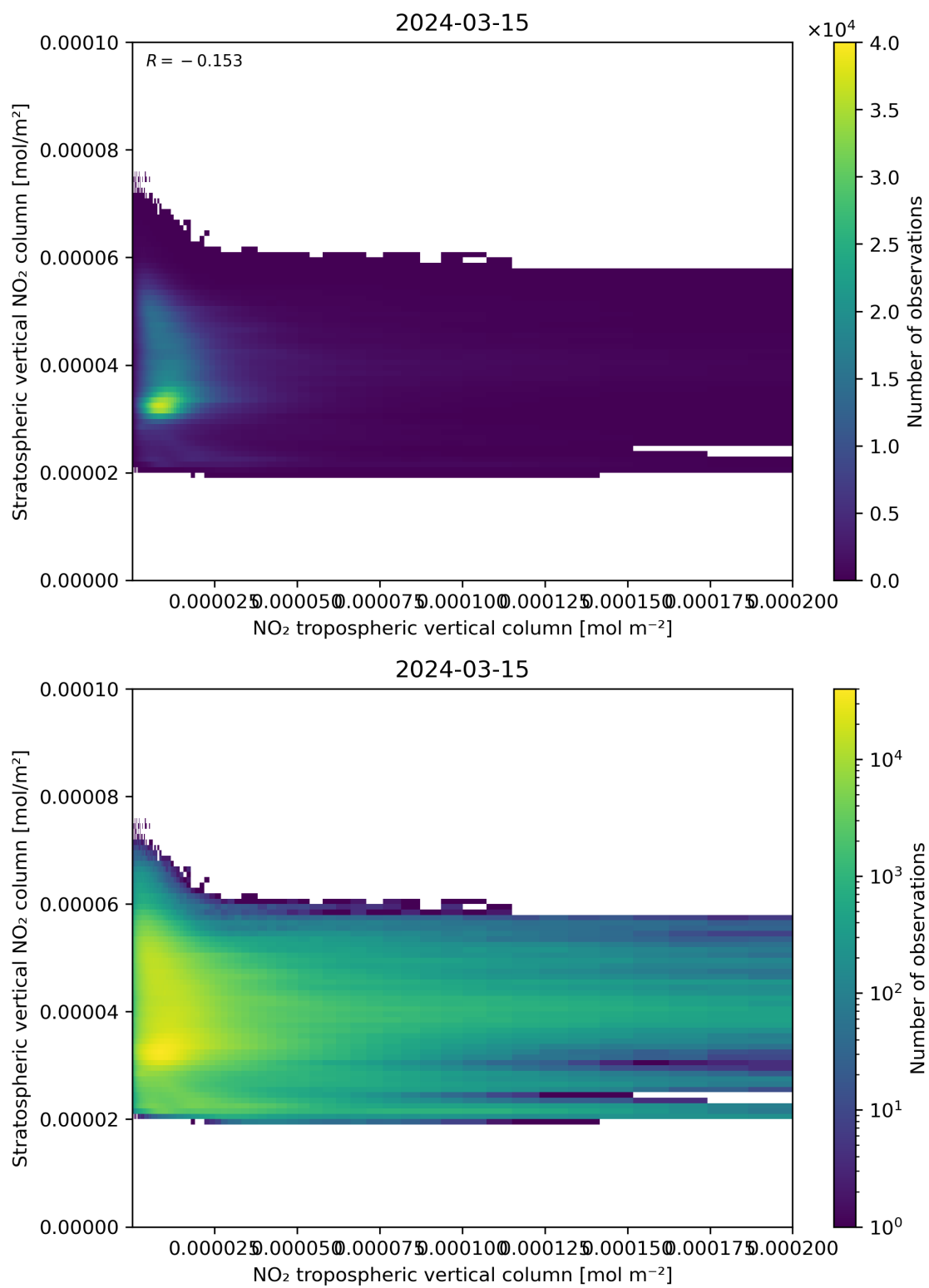
Figure 125: Scatter density plot of “NO 2 tropospheric vertical column” against “Stratospheric vertical NO 2 column” for 2024-03-14 to 2024-03-16.
