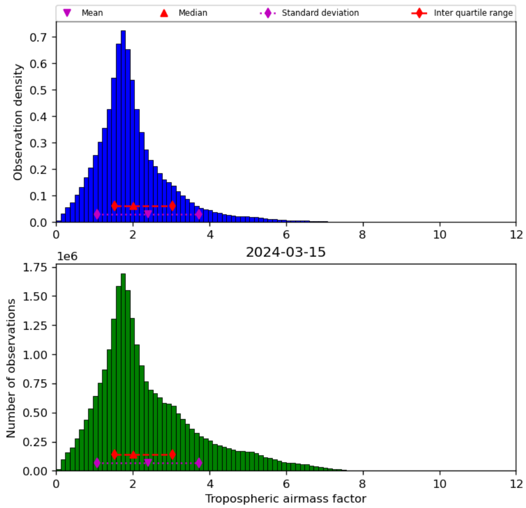
Figure 31: Histogram of “Tropospheric airmass factor” for 2024-03-14 to 2024-03-16
