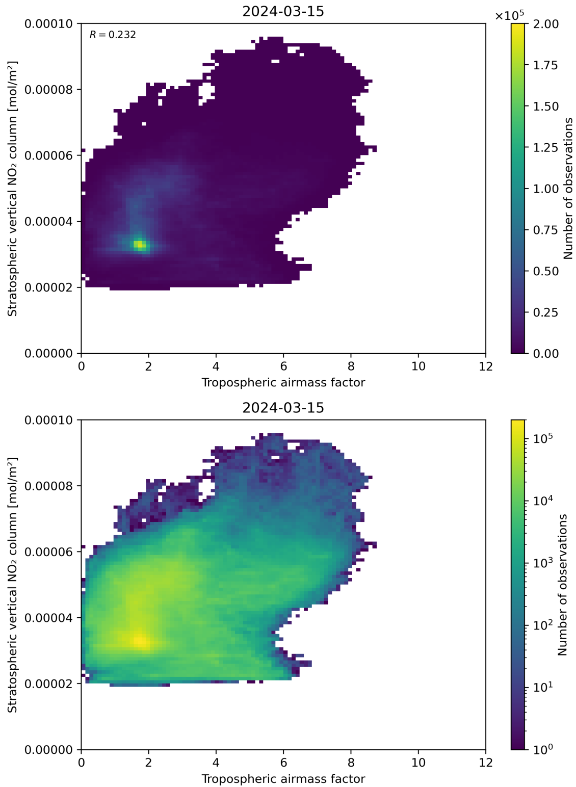
Figure 74: Scatter density plot of “Tropospheric air mass factor” against “Stratospheric vertical NO 2 column” for 2024-03-14 to 2024-03-16.
