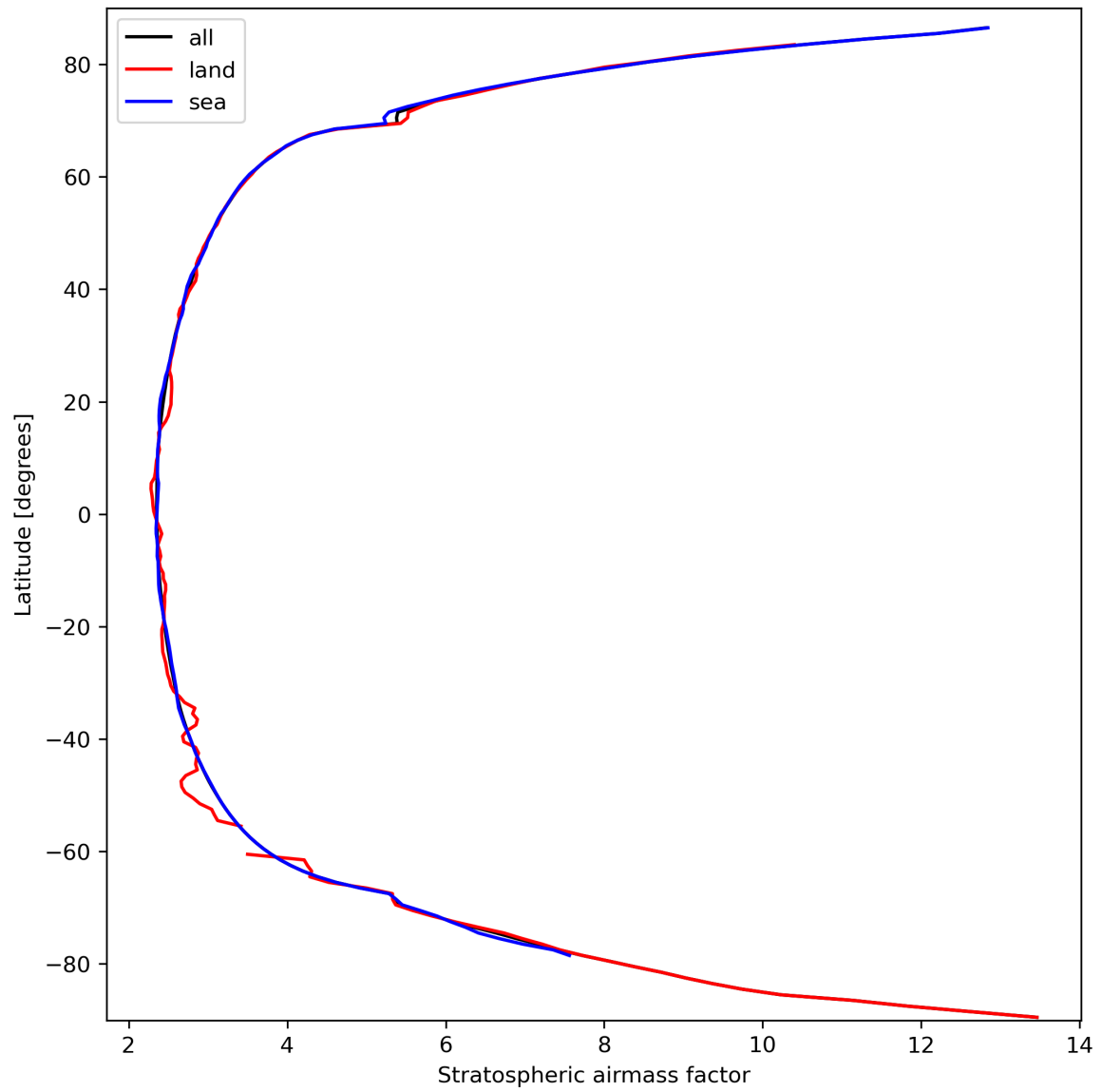
Figure 27: Zonal average of “Stratospheric airmass factor” for 2024-03-14 to 2024-03-16.
