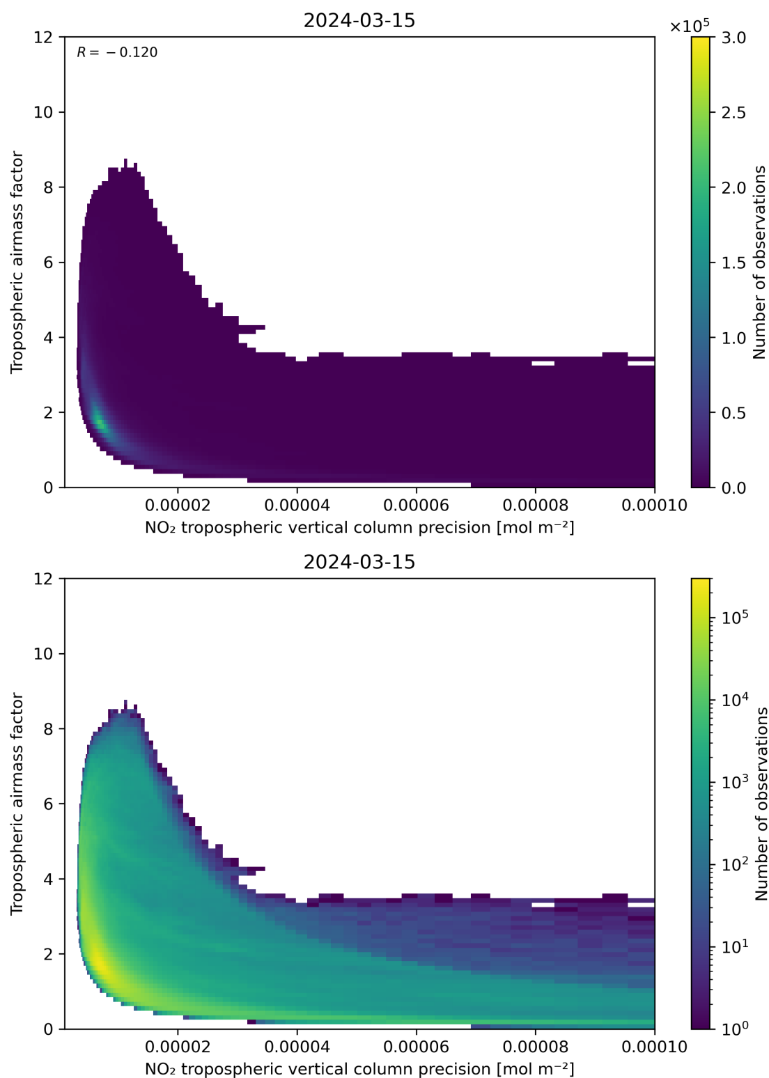
Figure 133: Scatter density plot of “NO 2 tropospheric vertical column precision” against “Tropospheric airmass factor” for 2024-03-14 to 2024-03-16.
