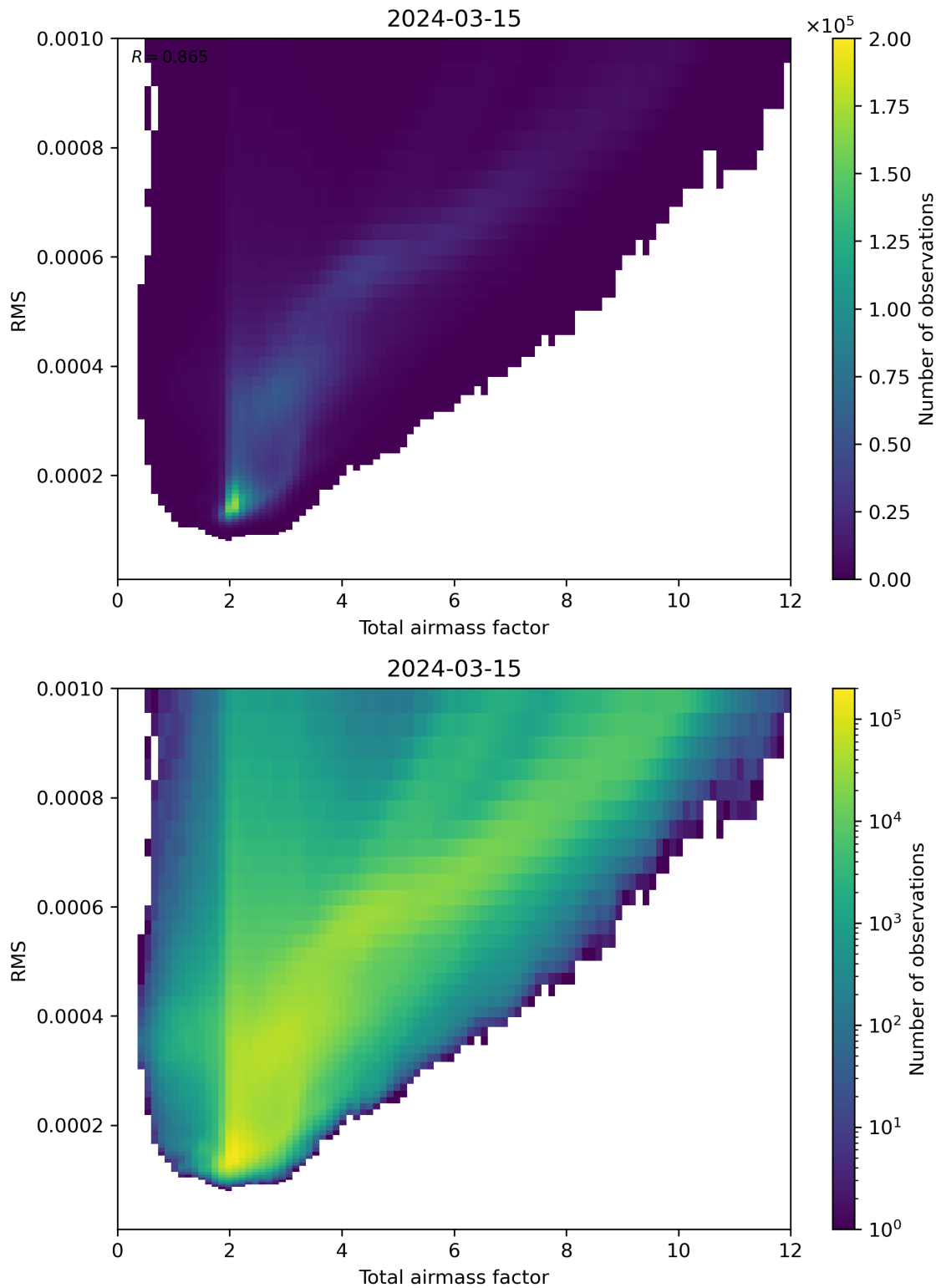
Figure 69: Scatter density plot of “Total airmass factor” against “RMS” for 2024-03-14 to 2024-03-16.
