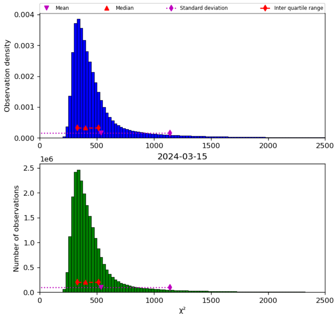
Figure 42: Histogram of “ \chi^2 ” for 2024-03-14 to 2024-03-16
