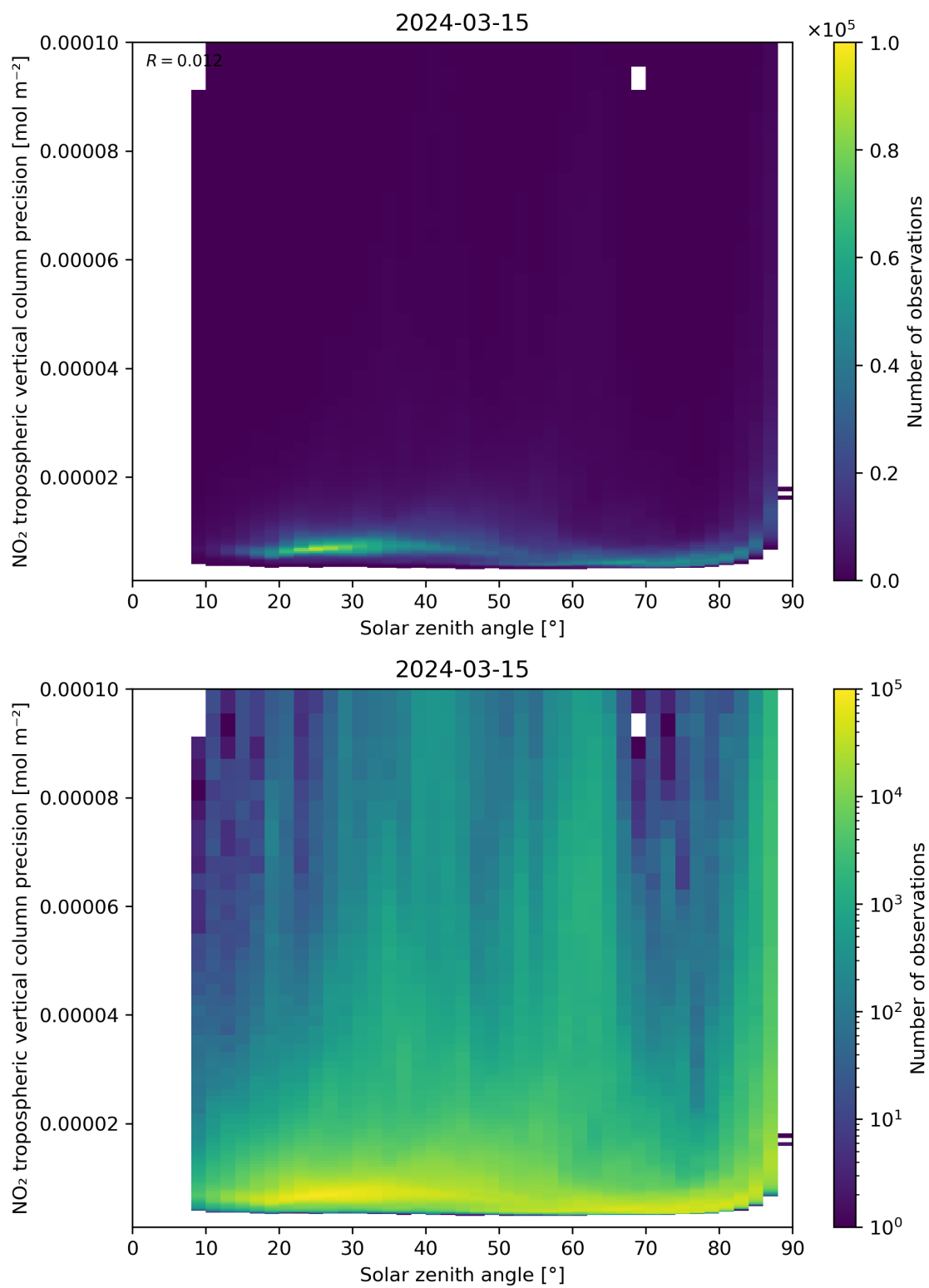
Figure 156: Scatter density plot of “Solar zenith angle” against “NO 2 tropospheric vertical column precision” for 2024-03-14 to 2024-03-16.
