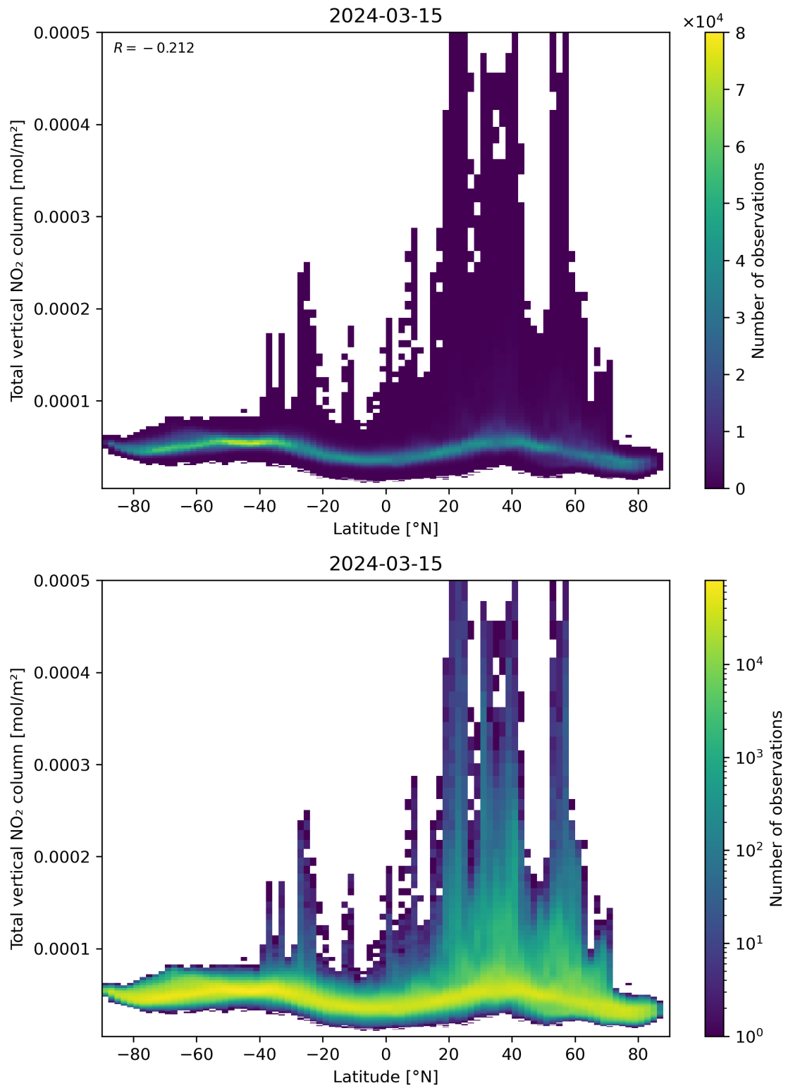
Figure 90: Scatter density plot of “Latitude” against “Total vertical NO 2 column” for 2024-03-14 to 2024-03-16.
