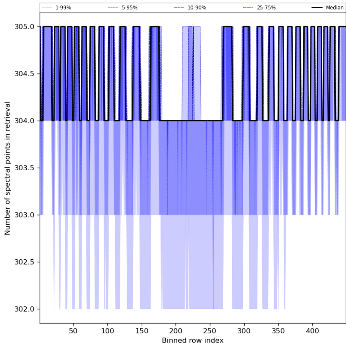
Figure 50: Along track statistics of “Number of spectral points in retrieval” for 2024-03-14 to 2024-03-16
