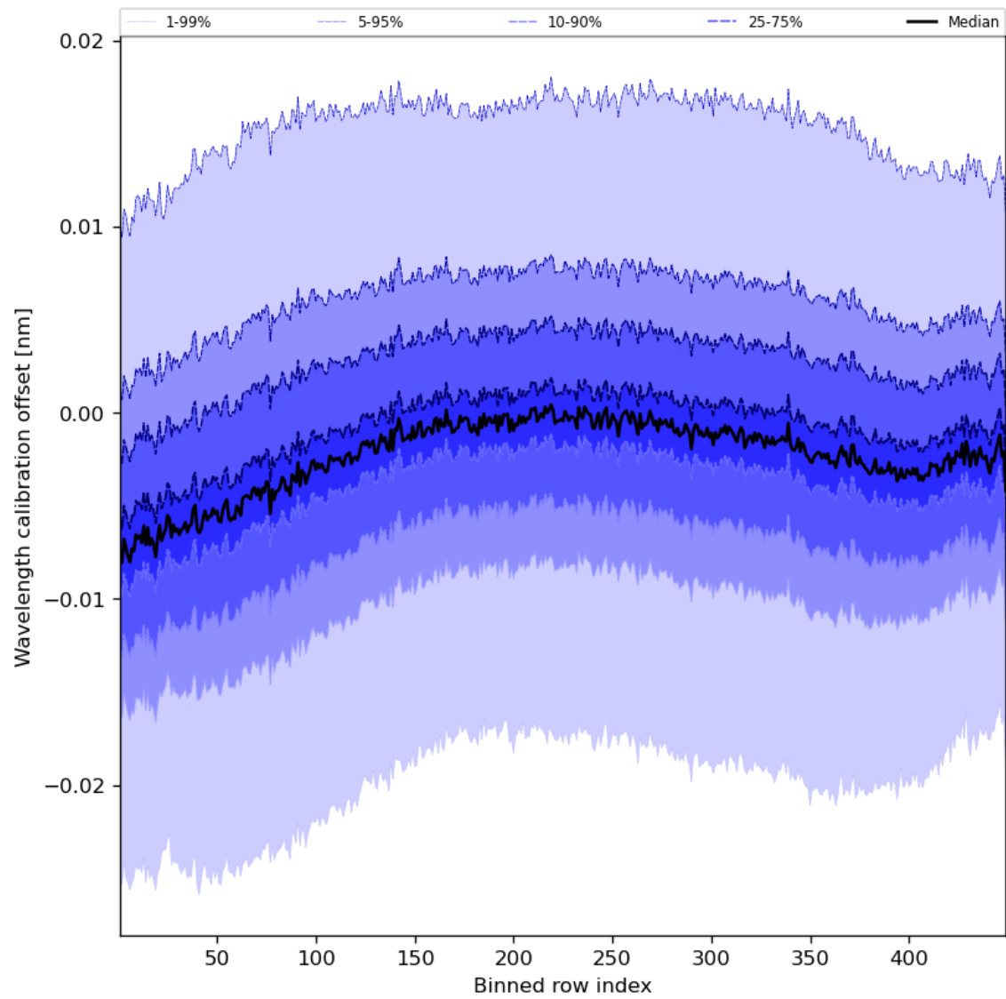
Figure 52: Along track statistics of “Wavelength calibration offset” for 2024-03-14 to 2024-03-16
