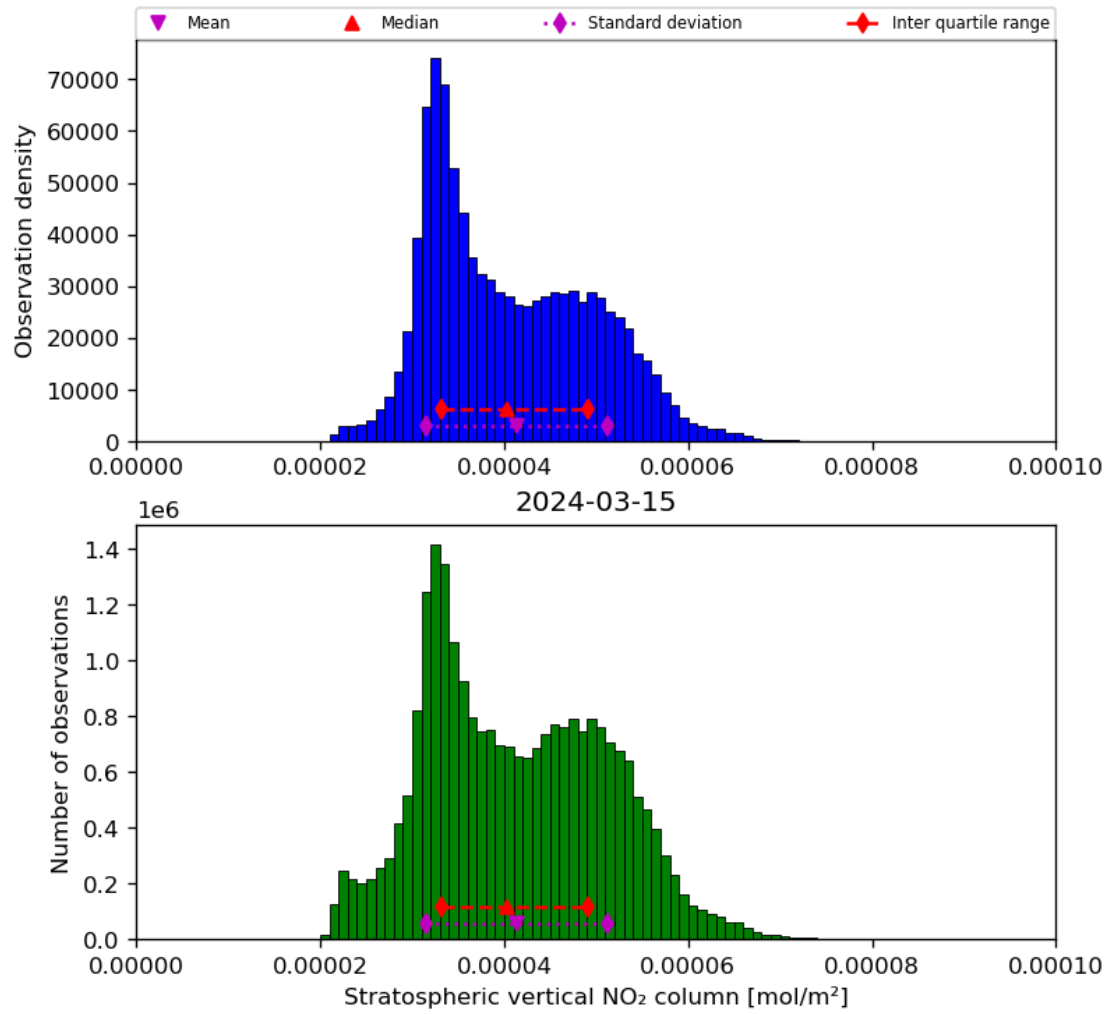
Figure 36: Histogram of “Stratospheric vertical NO 2 column” for 2024-03-14 to 2024-03-16
