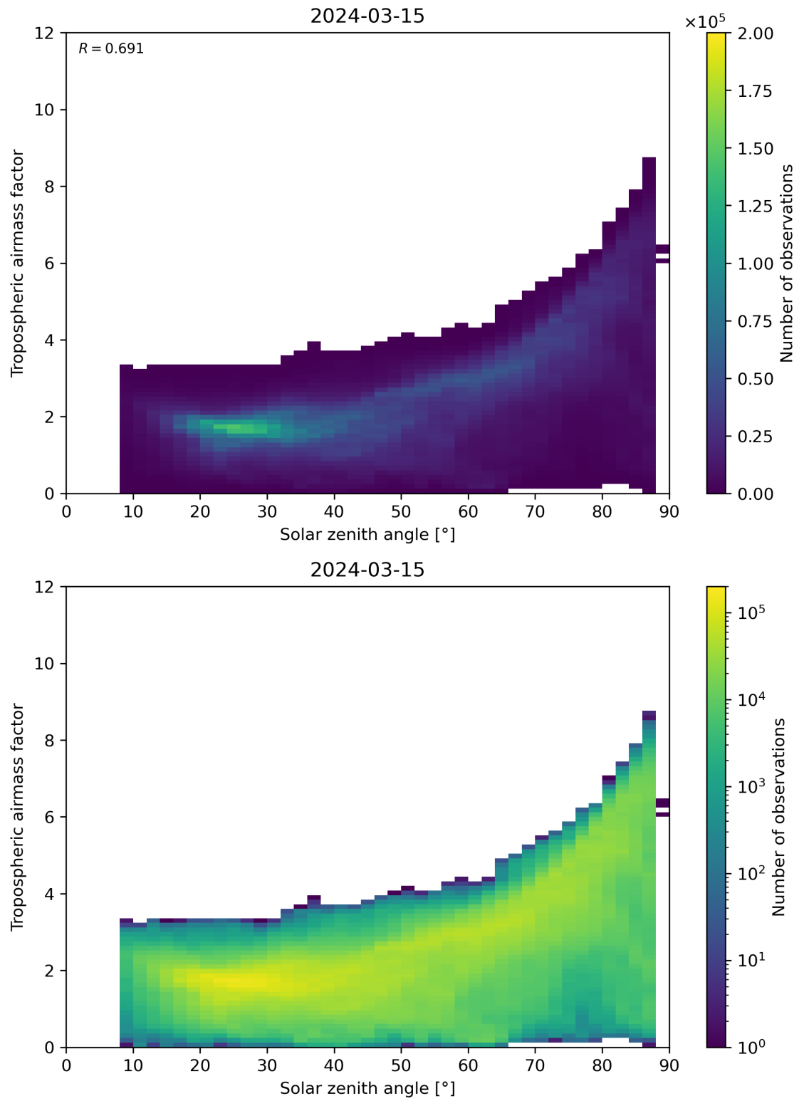
Figure 147: Scatter density plot of “Solar zenith angle” against “Tropospheric airmass factor” for 2024-03-14 to 2024-03-16.
