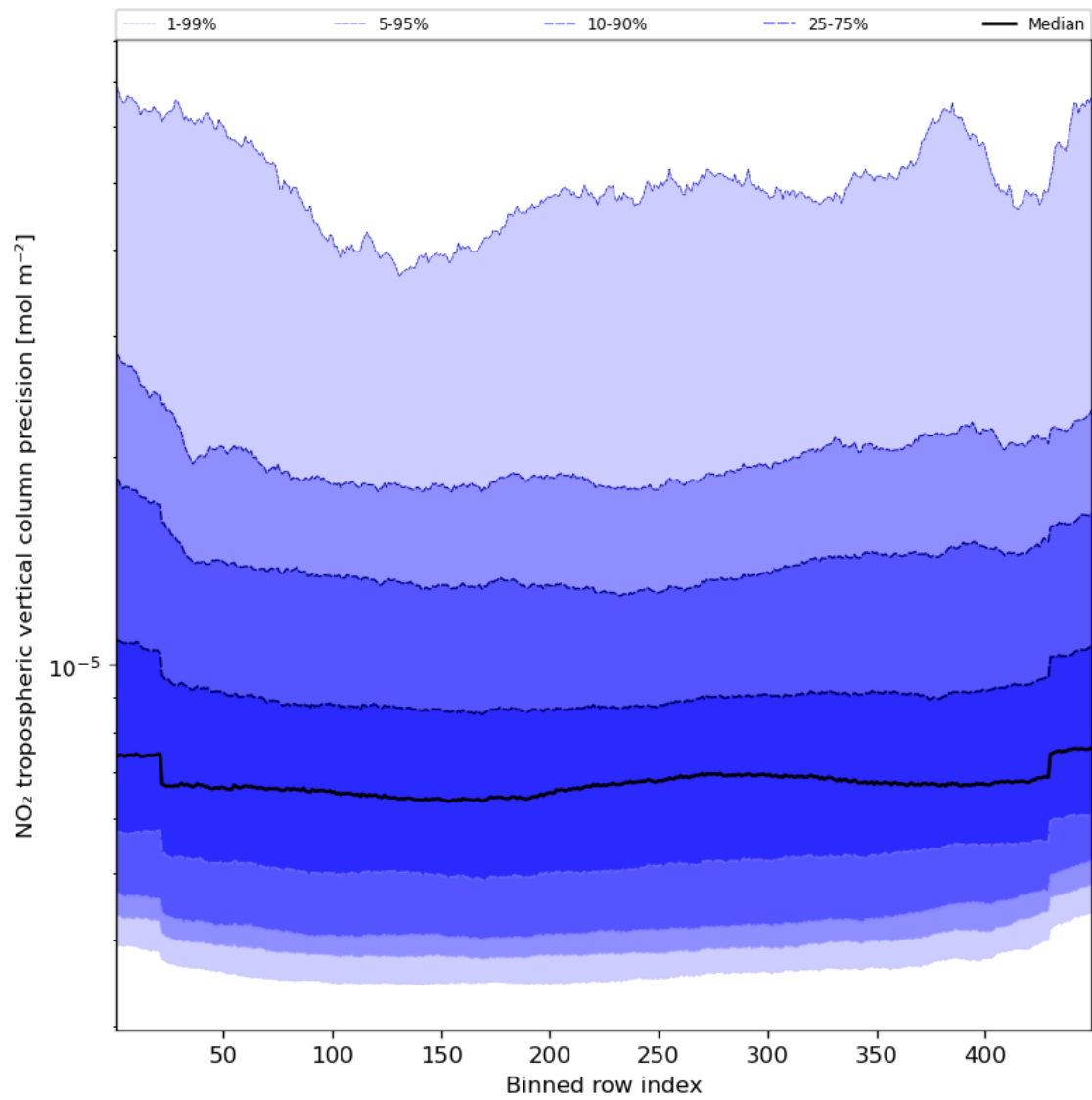
Figure 47: Along track statistics of “NO 2 tropospheric vertical column precision” for 2024-03-14 to 2024-03-16
