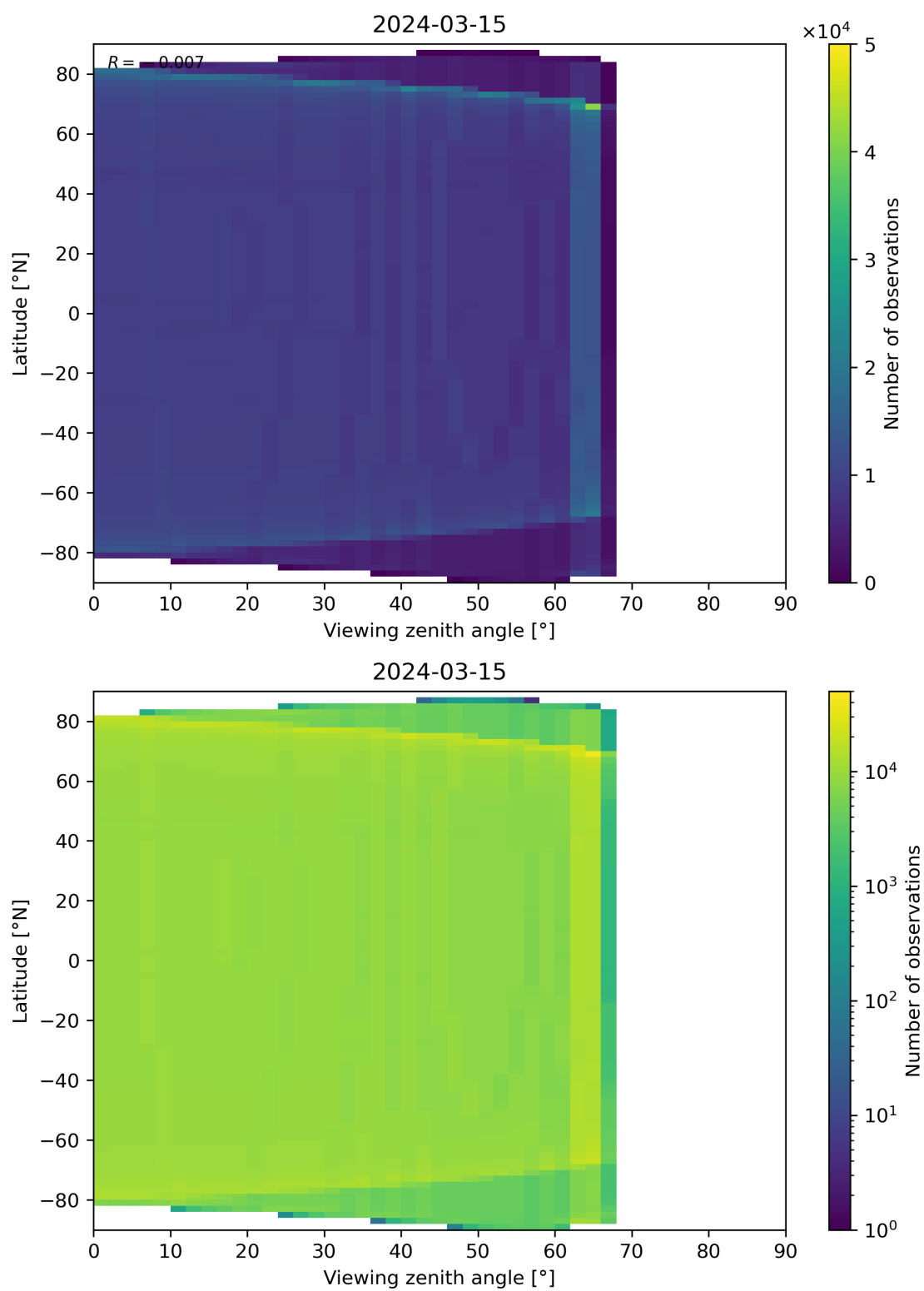
Figure 163: Scatter density plot of “Viewing zenith angle” against “Latitude” for 2024-03-14 to 2024-03-16.
