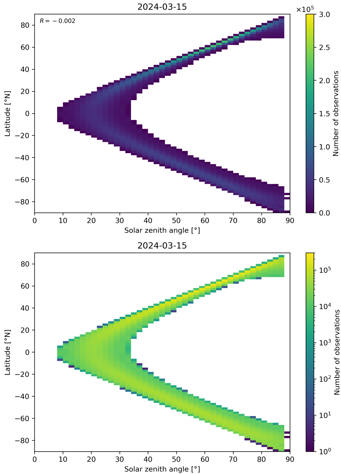
Figure 149: Scatter density plot of “Solar zenith angle” against “Latitude” for 2024-03-14 to 2024-03-16.
