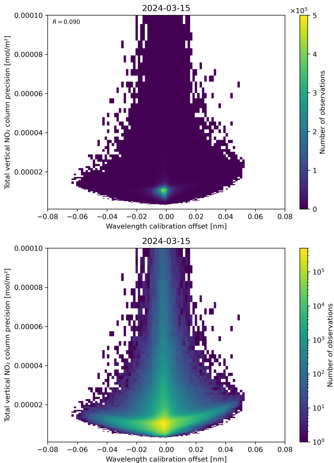
Figure 180: Scatter density plot of “Wavelength calibration offset” against “Total vertical NO 2 column precision” for 2024-03-14 to 2024-03-16.
