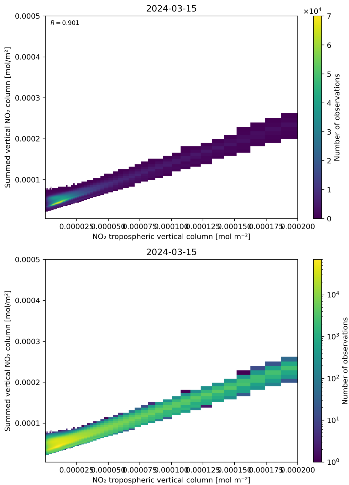
Figure 126: Scatter density plot of “NO 2 tropospheric vertical column” against “Summed vertical NO 2 column” for 2024-03-14 to 2024-03-16.
