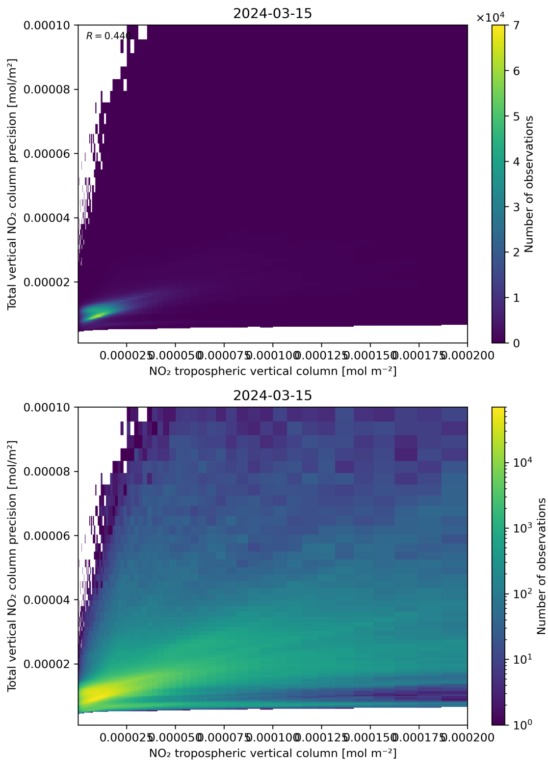
Figure 129: Scatter density plot of “NO 2 tropospheric vertical column” against “Total vertical NO 2 column precision” for 2024-03-14 to 2024-03-16.
