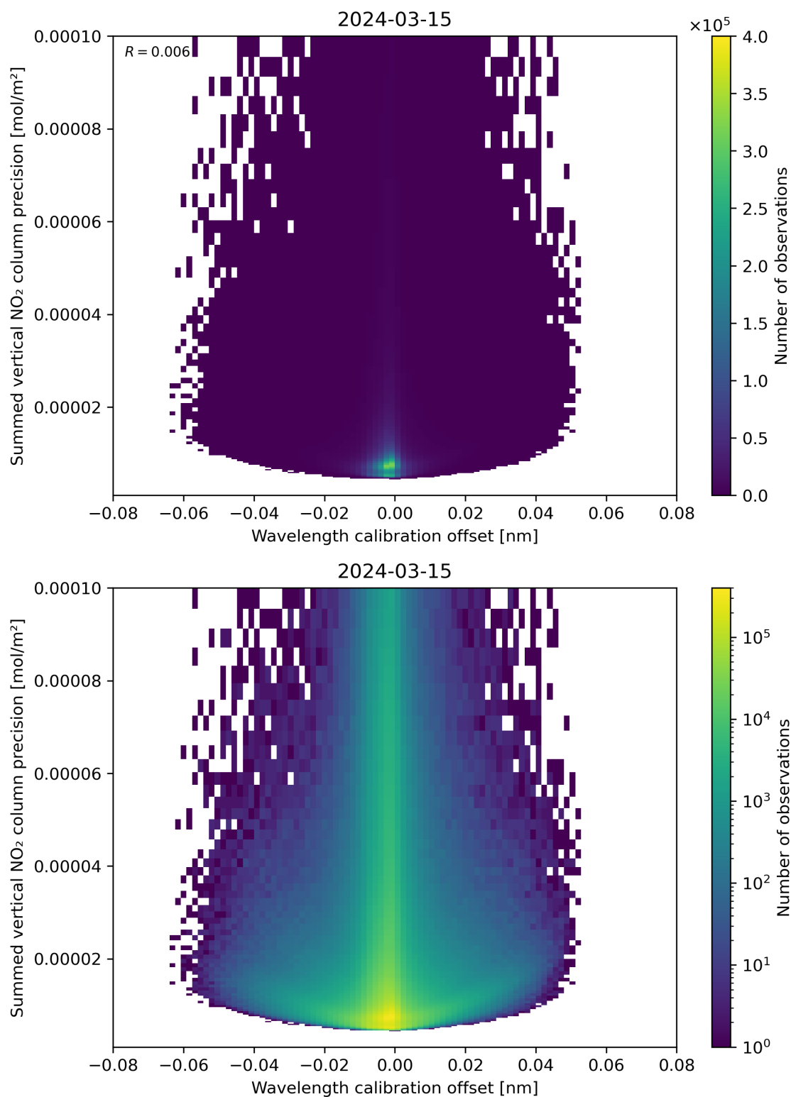
Figure 178: Scatter density plot of “Wavelength calibration offset” against “Summed vertical NO 2 column precision” for 2024-03-14 to 2024-03-16.
