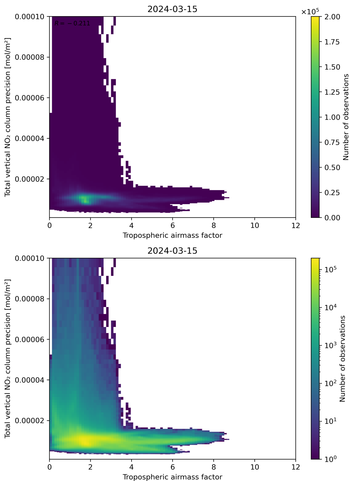
Figure 78: Scatter density plot of “Tropospheric air mass factor” against “Total vertical NO 2 column precision” for 2024-03-14 to 2024-03-16.
