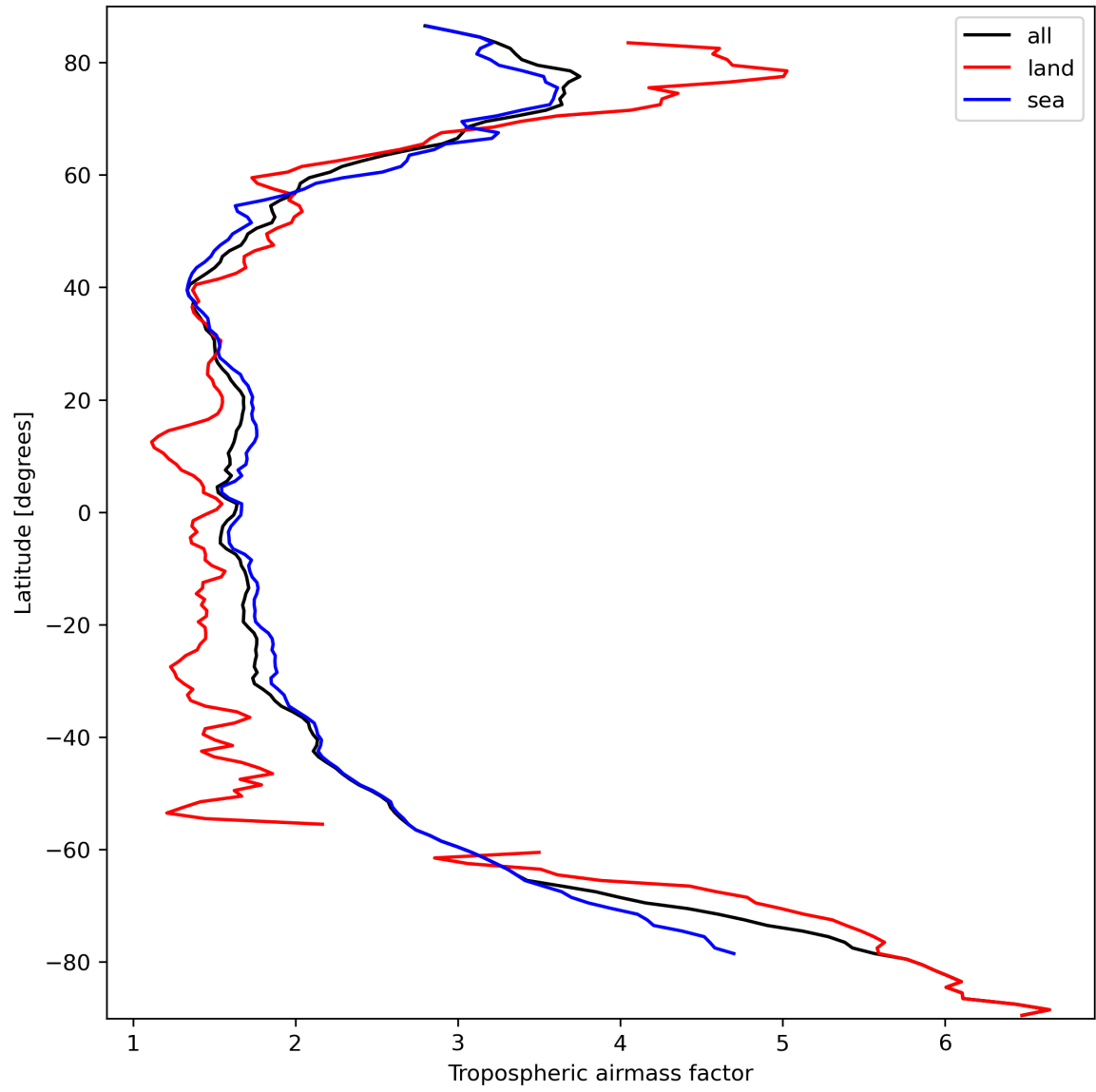
Figure 14: Zonal average of “Tropospheric airmass factor” for 2024-03-14 to 2024-03-16.
