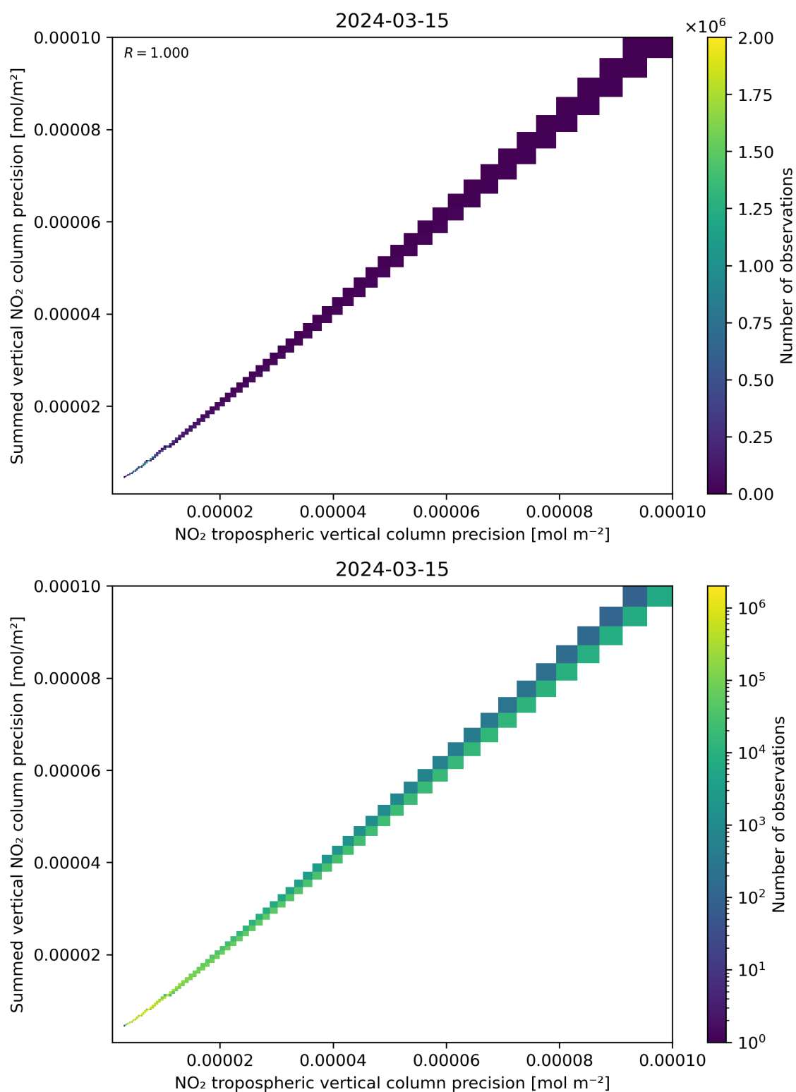
Figure 137: Scatter density plot of “NO 2 tropospheric vertical column precision” against “Summed vertical NO 2 column precision” for 2024-03-14 to 2024-03-16.
