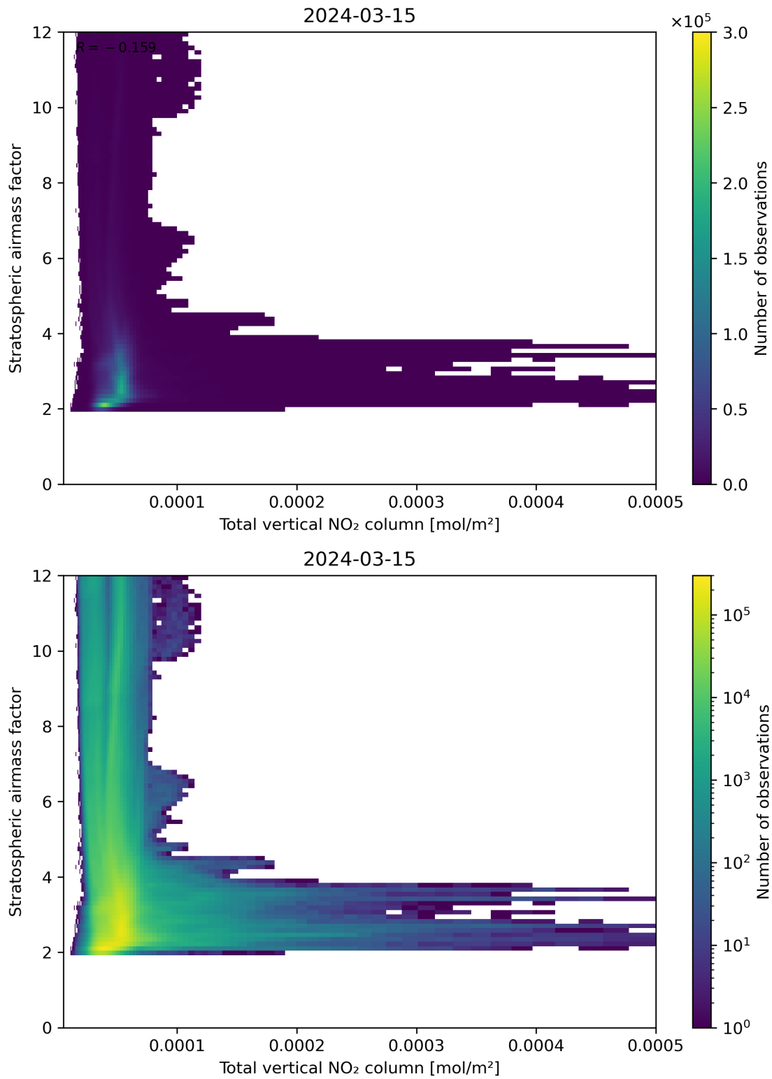
Figure 110: Scatter density plot of “Total vertical NO 2 column” against “Stratospheric airmass factor” for 2024-03-14 to 2024-03-16.
