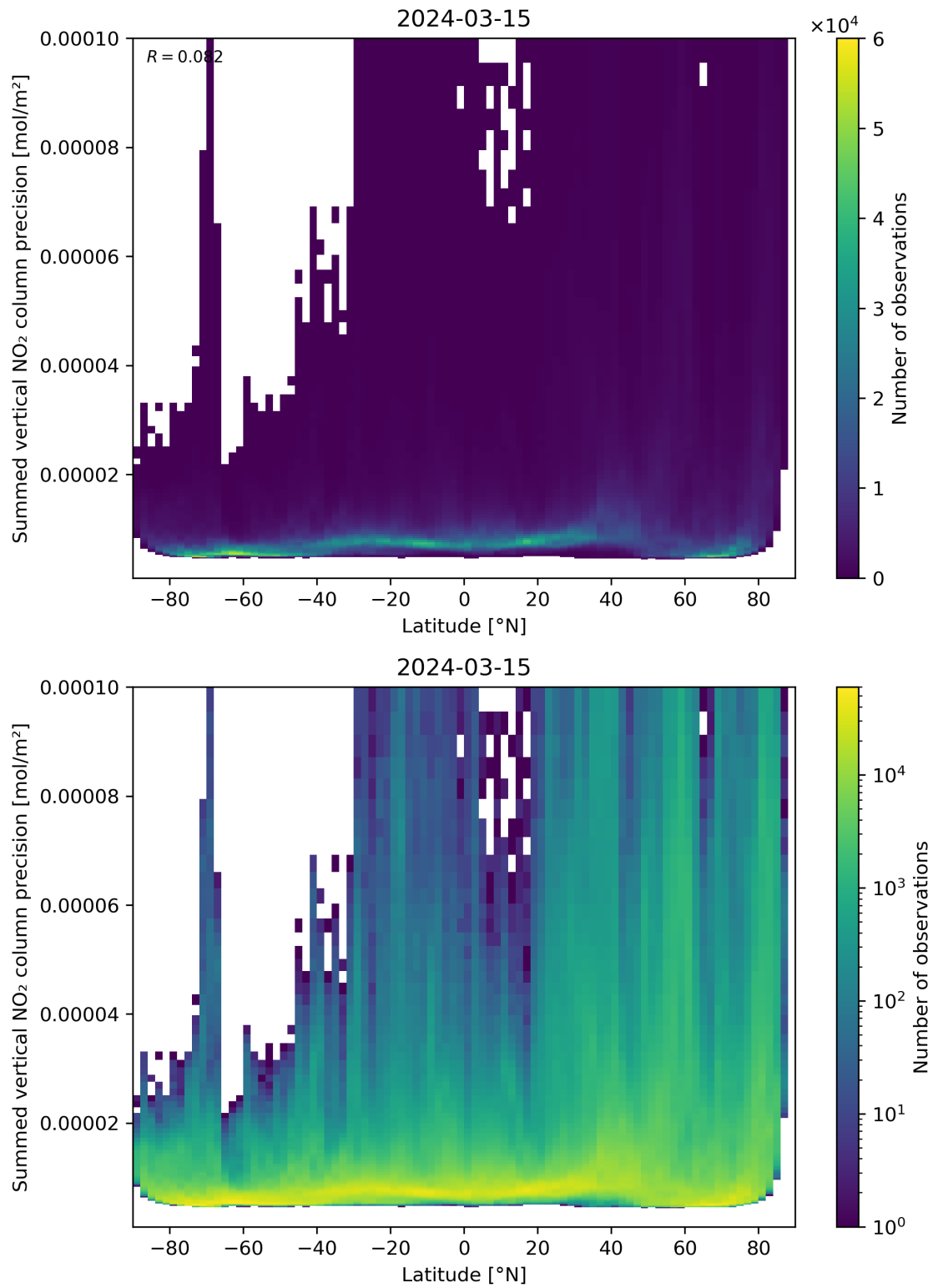
Figure 89: Scatter density plot of “Latitude” against “Summed vertical NO 2 column precision” for 2024-03-14 to 2024-03-16.
