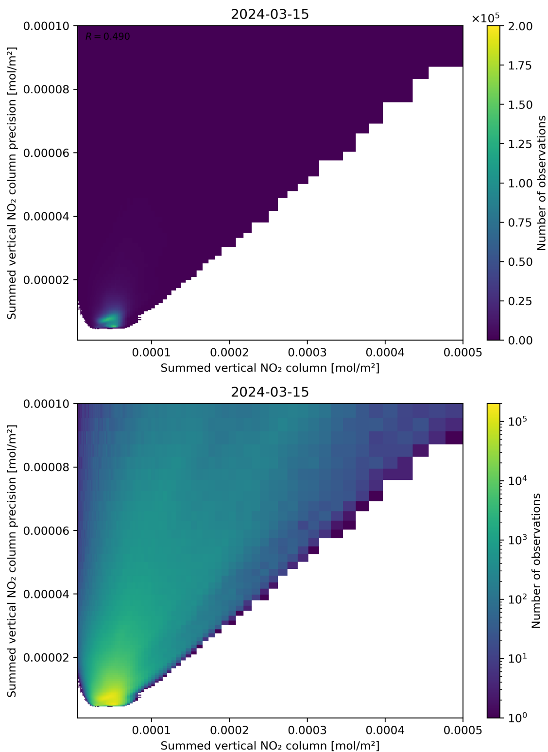
Figure 105: Scatter density plot of “Summed vertical NO 2 column” against “Summed vertical NO 2 column precision” for 2024-03-14 to 2024-03-16.
