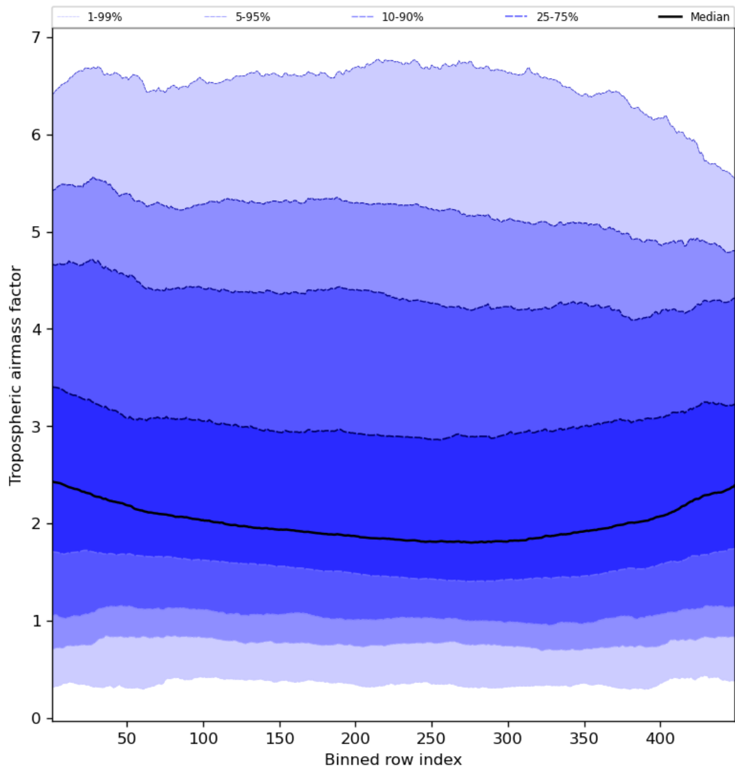
Figure 48: Along track statistics of “Tropospheric air mass factor” for 2024-03-14 to 2024-03-16
