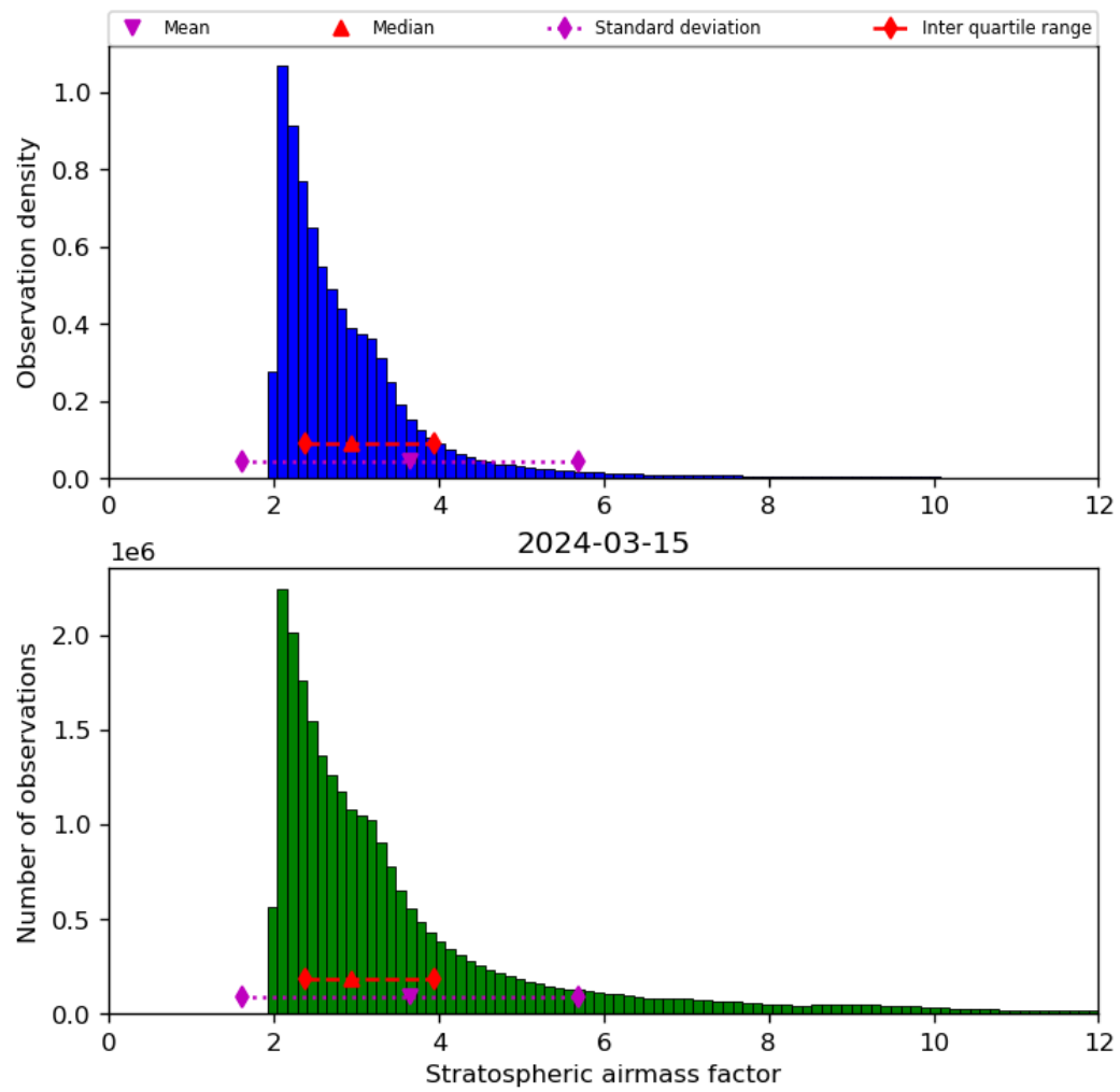
Figure 44: Histogram of “Stratospheric airmass factor” for 2024-03-14 to 2024-03-16
