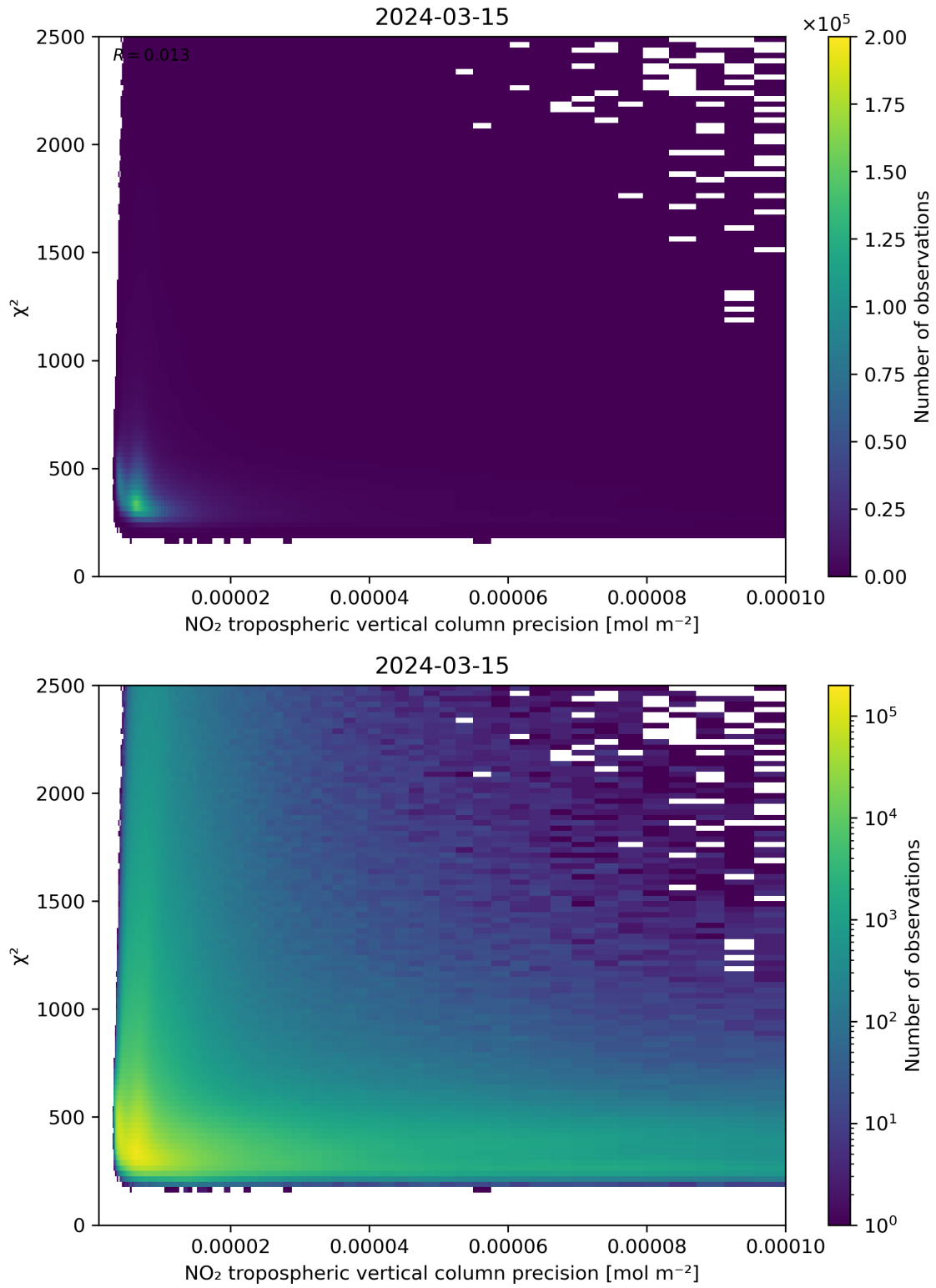
Figure 134: Scatter density plot of “NO 2 tropospheric vertical column precision” against “ \chi^2 ” for 2024-03-14 to 2024-03-16.
