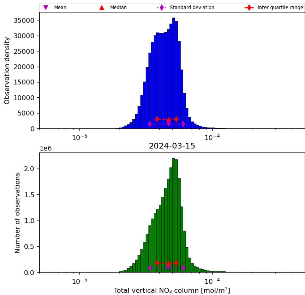
Figure 38: Histogram of “Total vertical NO 2 column” for 2024-03-14 to 2024-03-16
