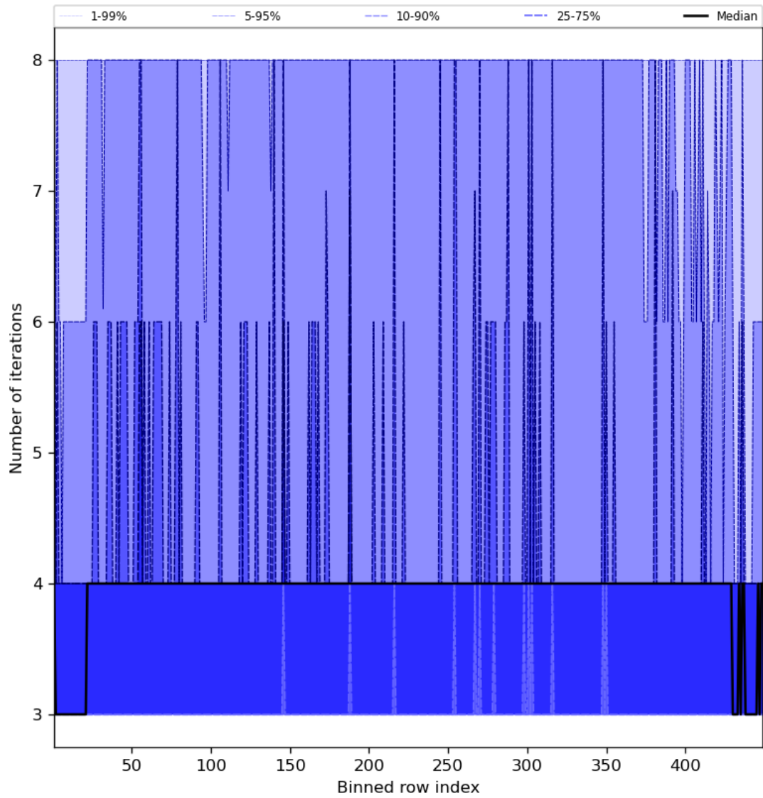
Figure 51: Along track statistics of “Number of iterations” for 2024-03-14 to 2024-03-16
