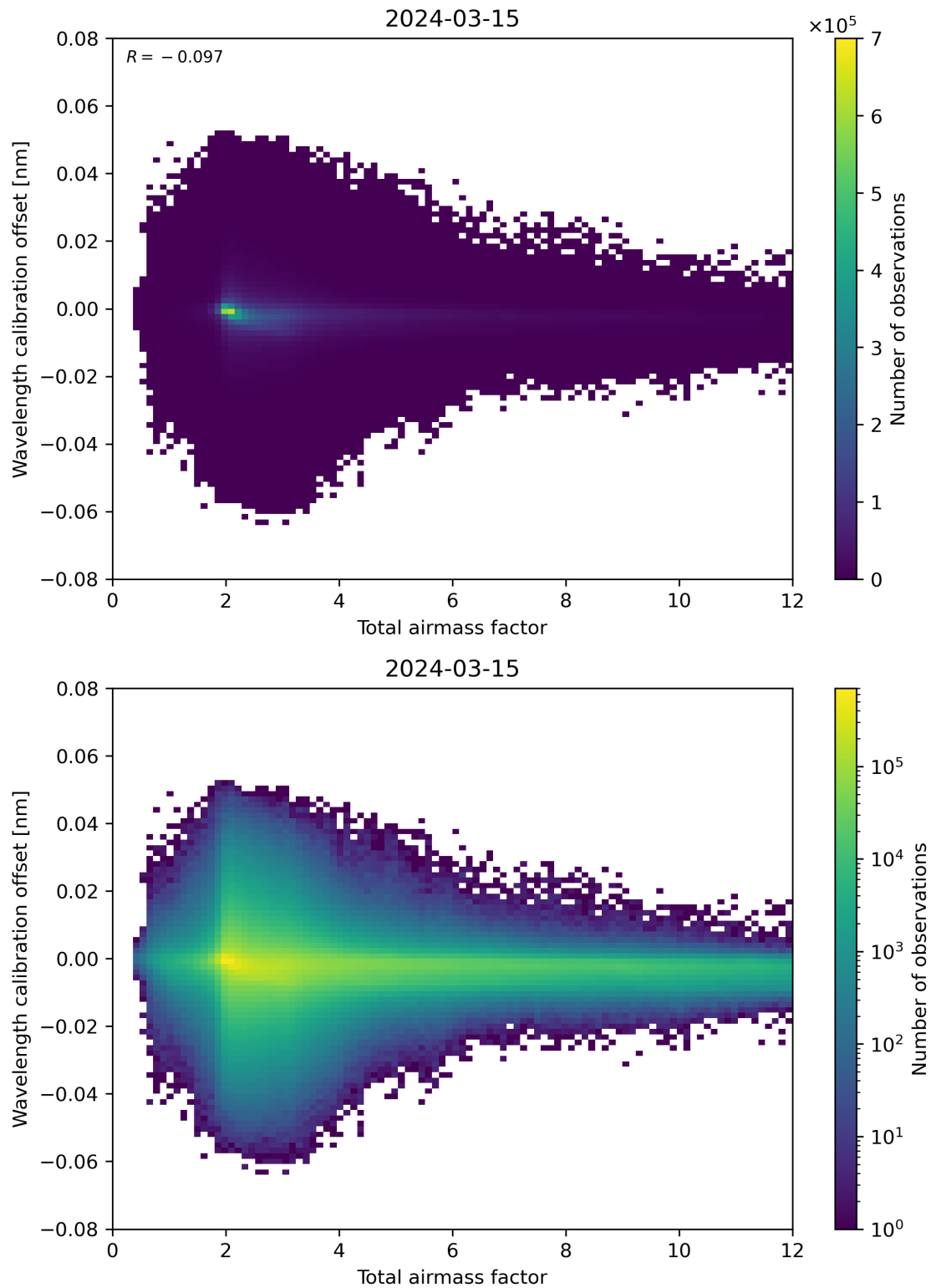
Figure 70: Scatter density plot of “Total airmass factor” against “Wavelength calibration offset” for 2024-03-14 to 2024-03-16.
