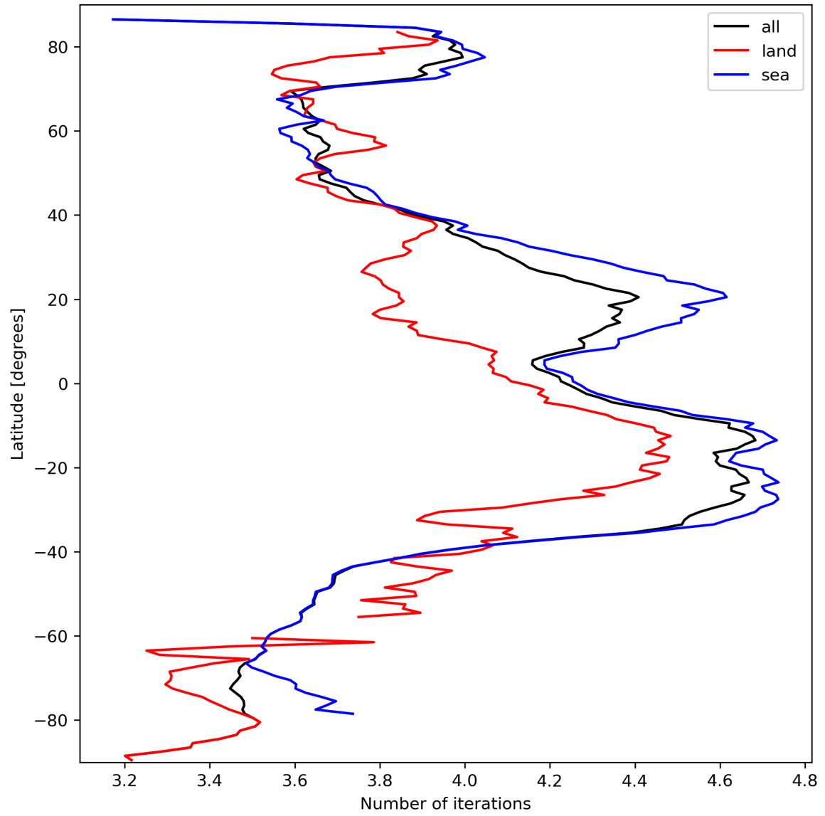
Figure 17: Zonal average of “Number of iterations” for 2024-03-14 to 2024-03-16.
