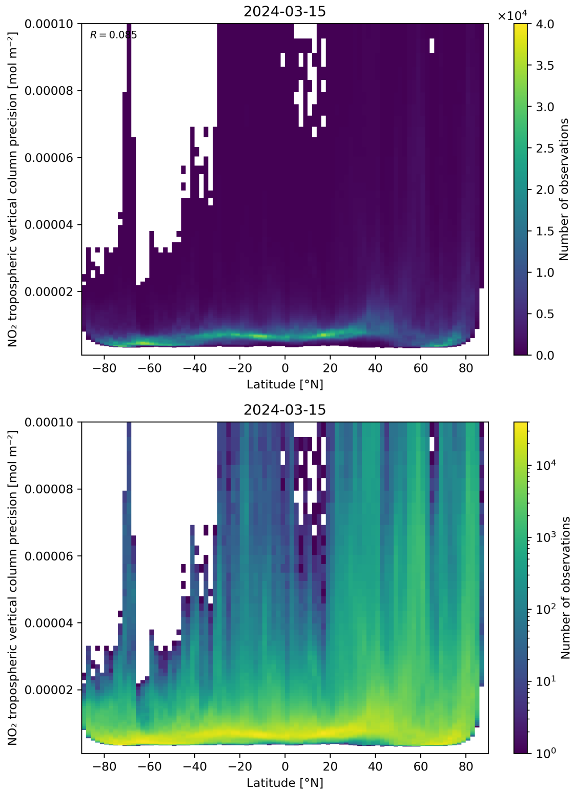
Figure 93: Scatter density plot of “Latitude” against “NO 2 tropospheric vertical column precision” for 2024-03-14 to 2024-03-16.
