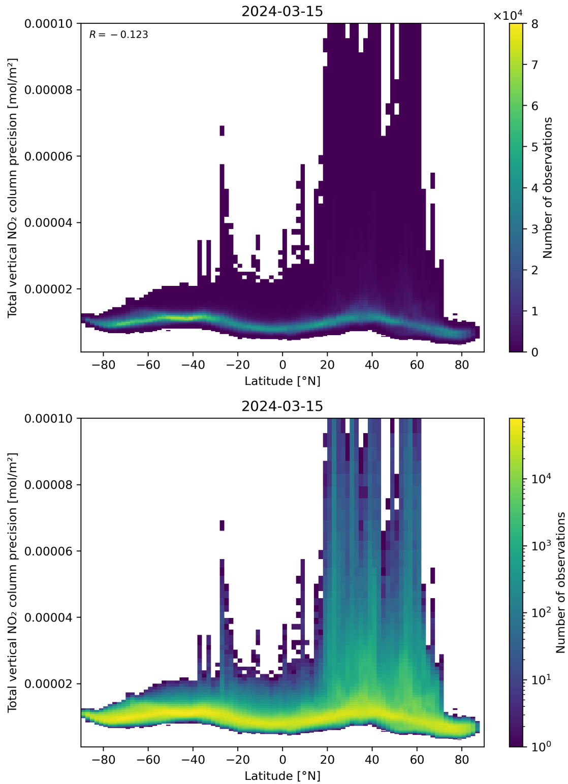
Figure 91: Scatter density plot of “Latitude” against “Total vertical NO 2 column precision” for 2024-03-14 to 2024-03-16.
