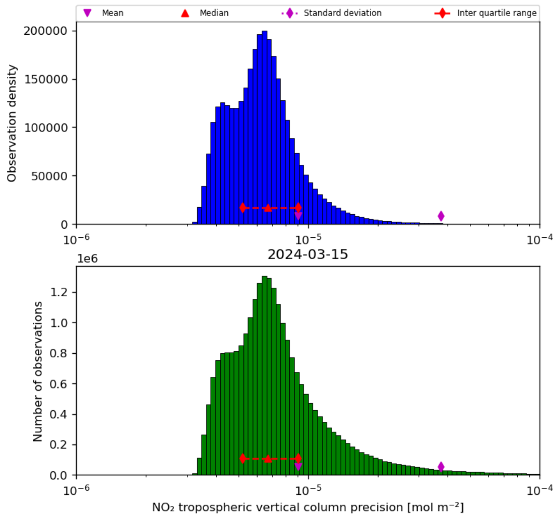
Figure 30: Histogram of “NO 2 tropospheric vertical column precision” for 2024-03-14 to 2024-03-16
