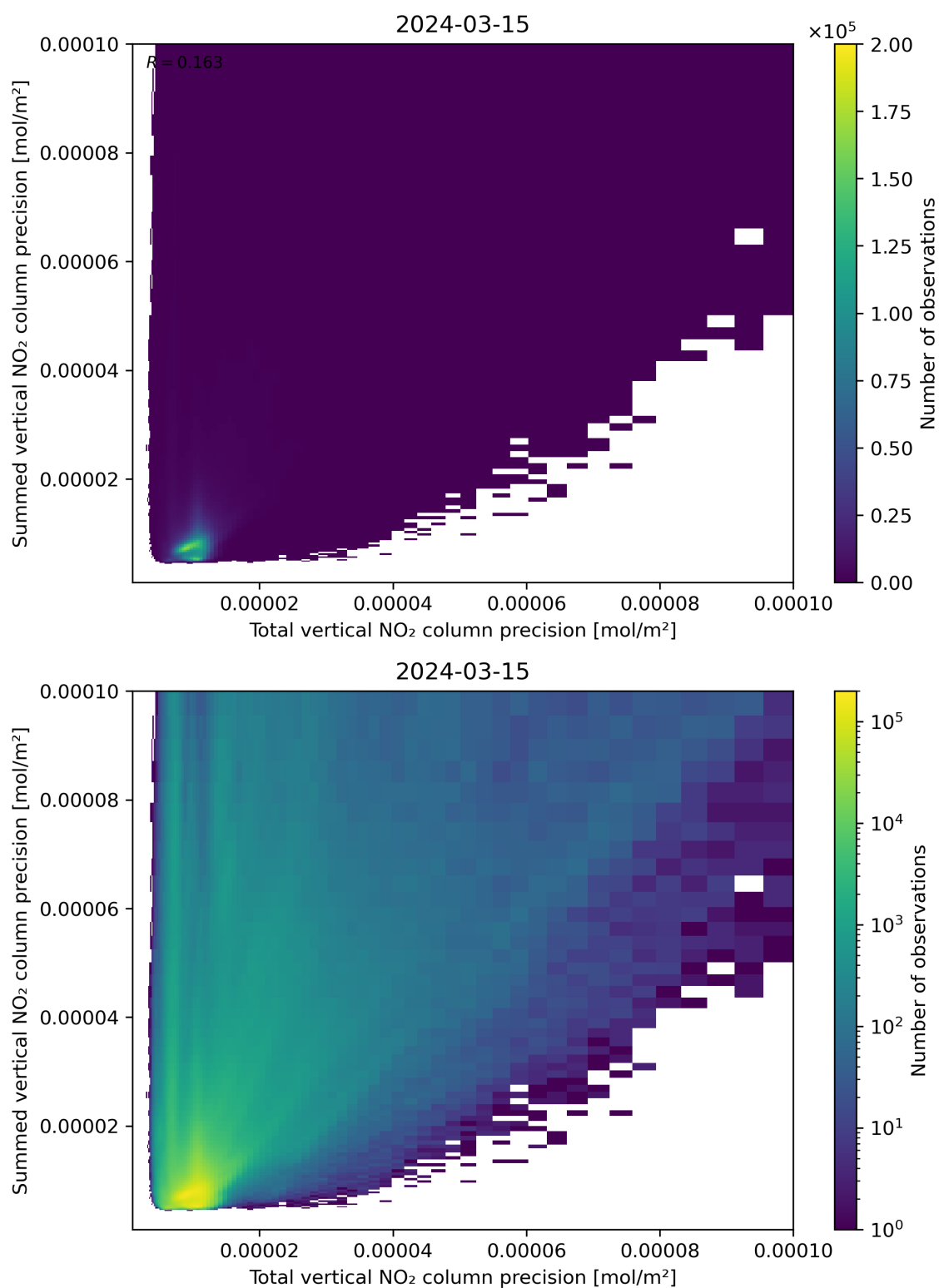
Figure 118: Scatter density plot of “Total vertical NO 2 column precision” against “Summed vertical NO 2 column precision” for 2024-03-14 to 2024-03-16.
