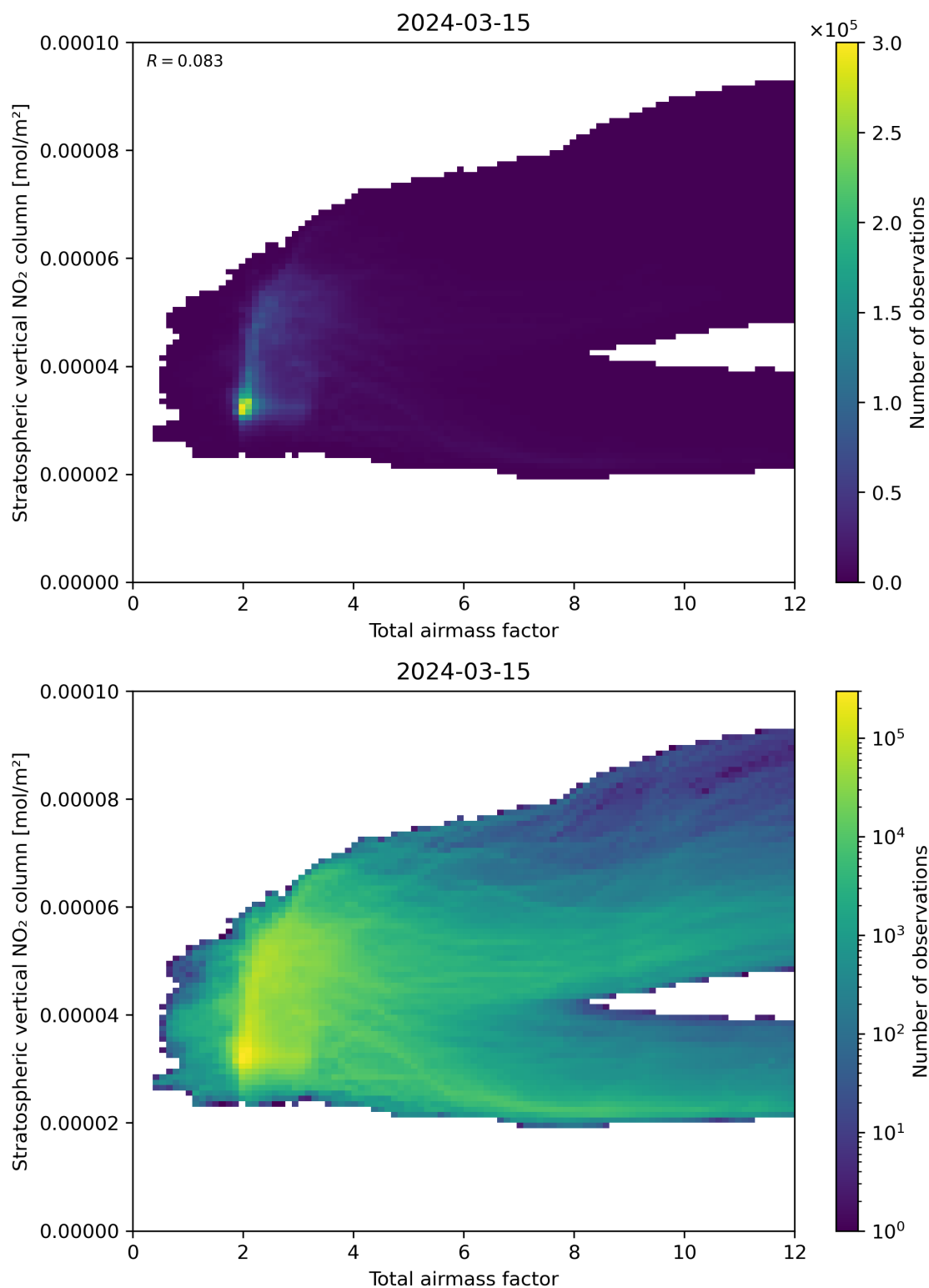
Figure 64: Scatter density plot of “Total airmass factor” against “Stratospheric vertical \text{NO}_2 column” for 2024-03-14 to 2024-03-16.
