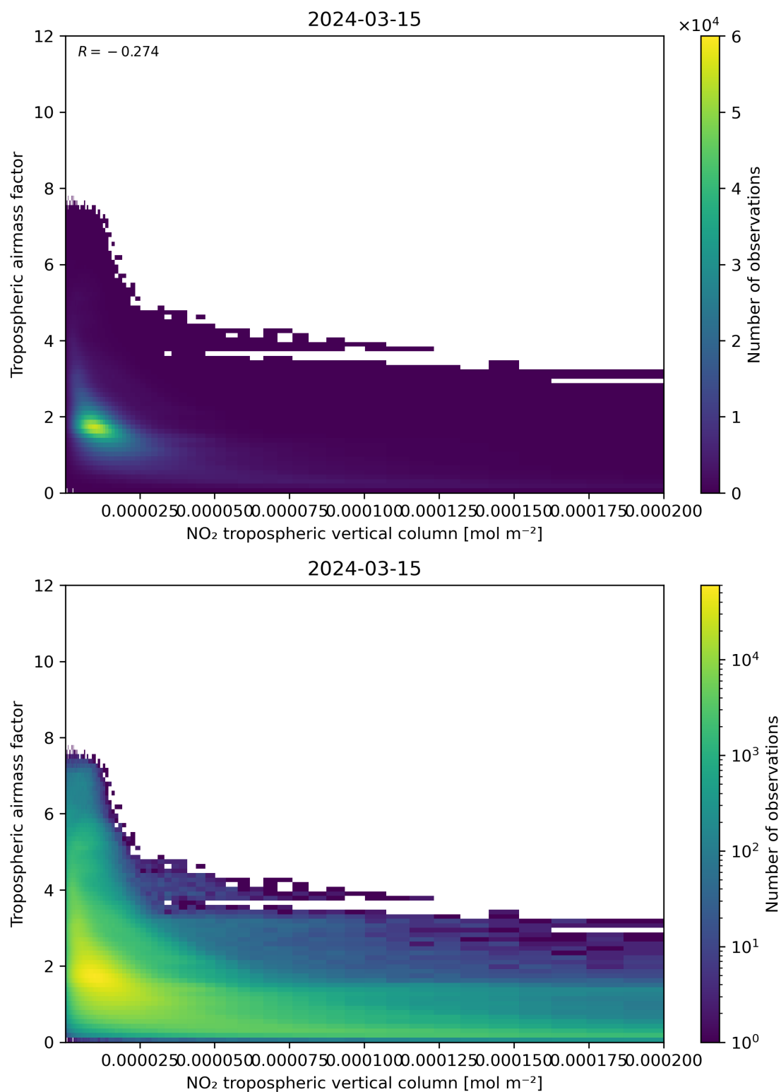
Figure 123: Scatter density plot of “NO 2 tropospheric vertical column” against “Tropospheric air mass factor” for 2024-03-14 to 2024-03-16.
