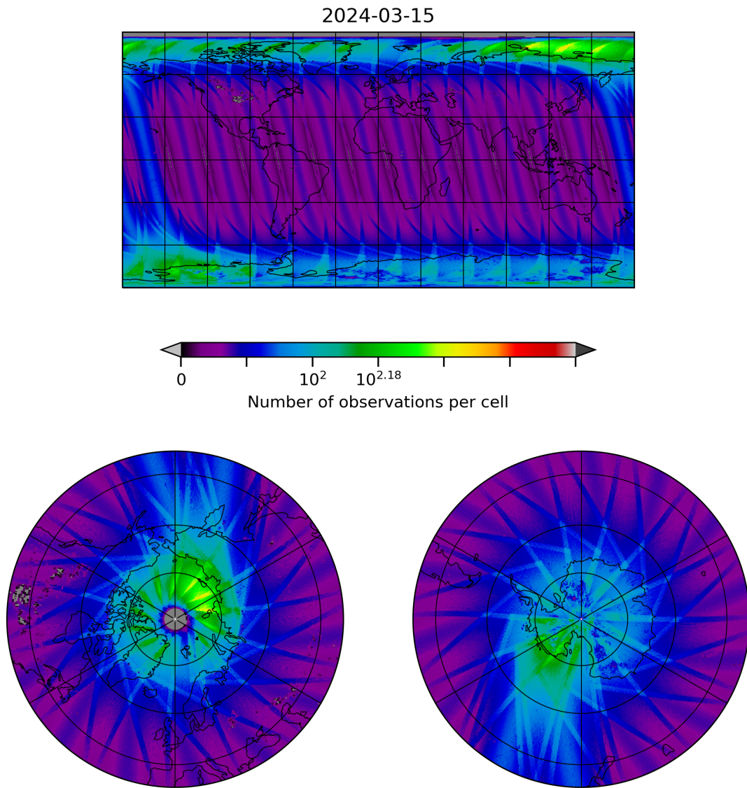
Figure 10: Map of the number of observations for 2024-03-14 to 2024-03-16
