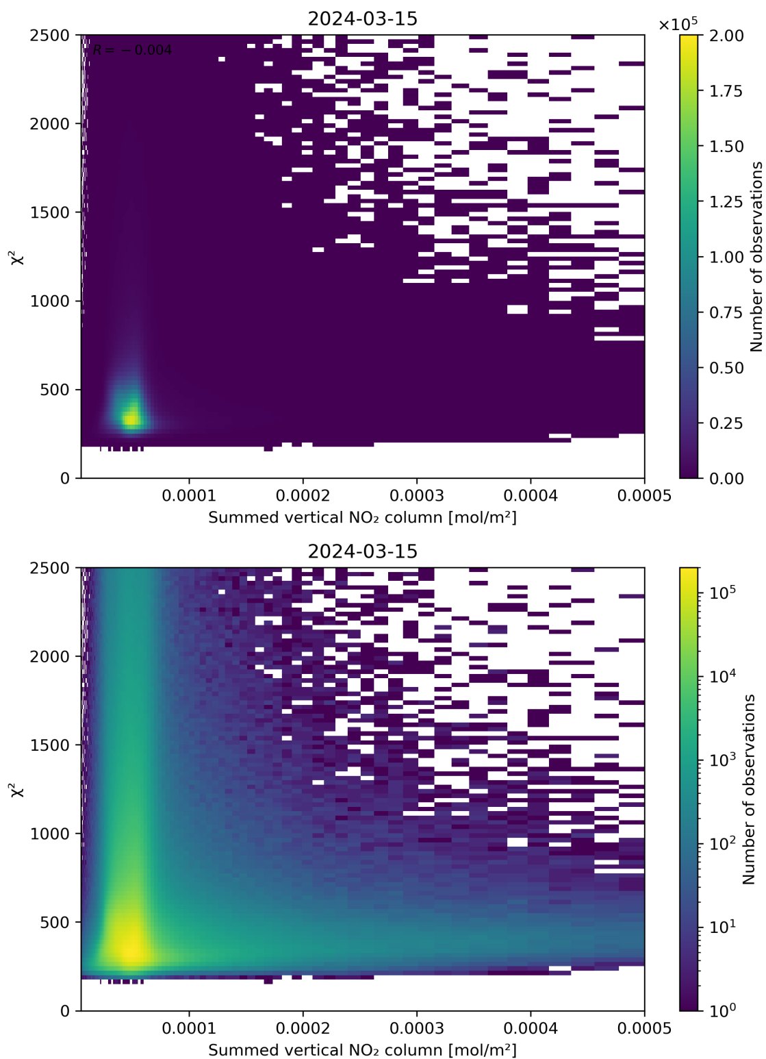
Figure 104: Scatter density plot of “Summed vertical NO 2 column” against “ \chi^2 ” for 2024-03-14 to 2024-03-16.
