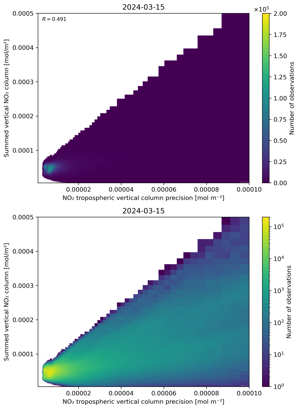
Figure 136: Scatter density plot of “NO 2 tropospheric vertical column precision” against “Summed vertical NO 2 column” for 2024-03-14 to 2024-03-16.
