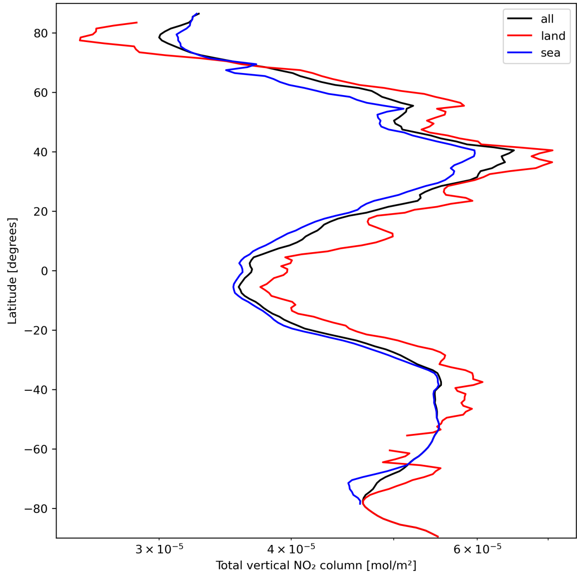
Figure 21: Zonal average of “Total vertical NO 2 column” for 2024-03-14 to 2024-03-16.
