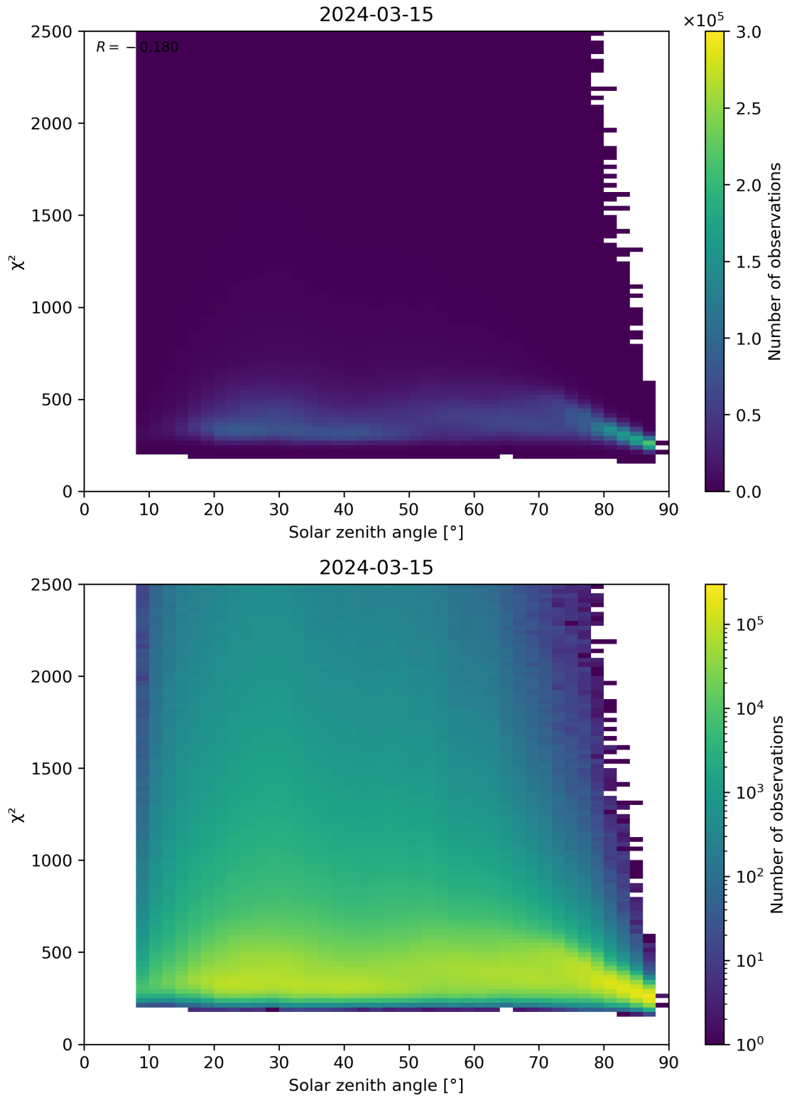
Figure 148: Scatter density plot of “Solar zenith angle” against “ \chi^2 ” for 2024-03-14 to 2024-03-16.
