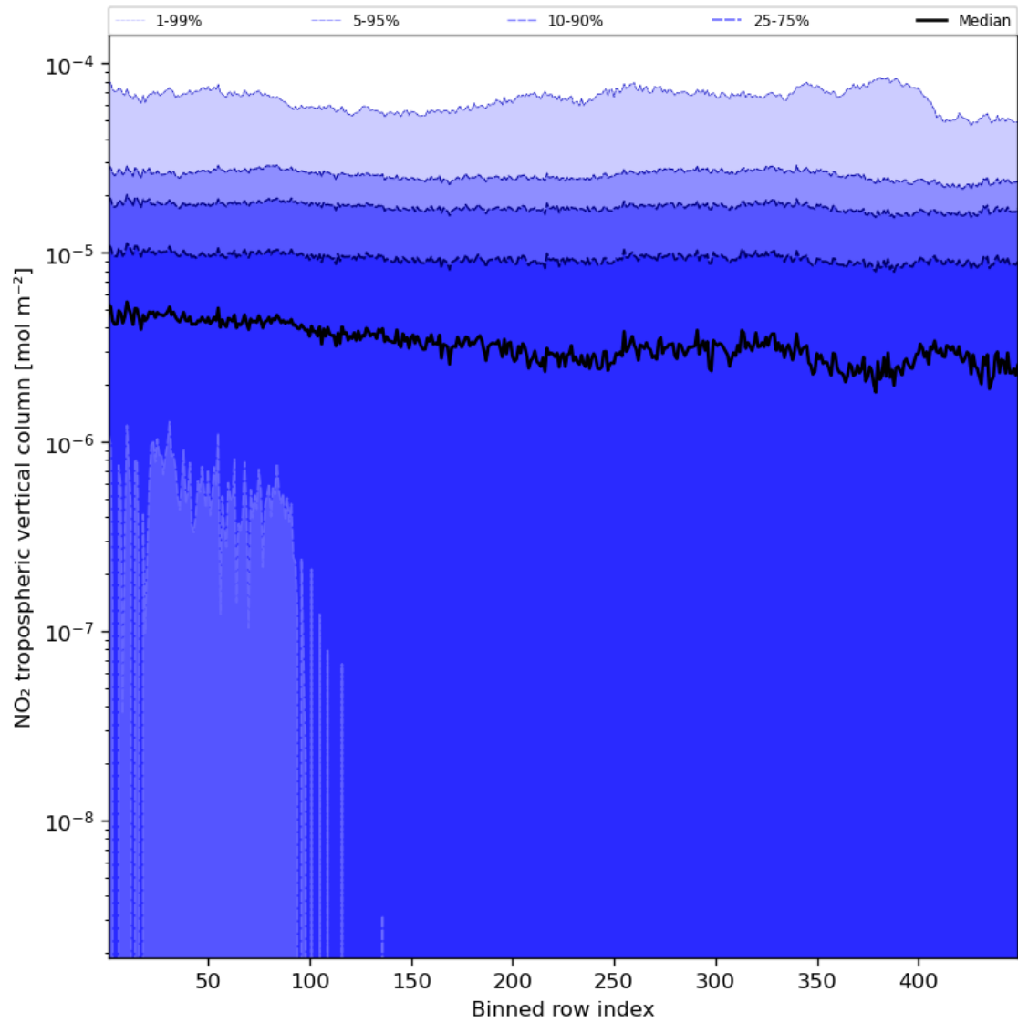
Figure 46: Along track statistics of “NO 2 tropospheric vertical column” for 2024-03-14 to 2024-03-16
