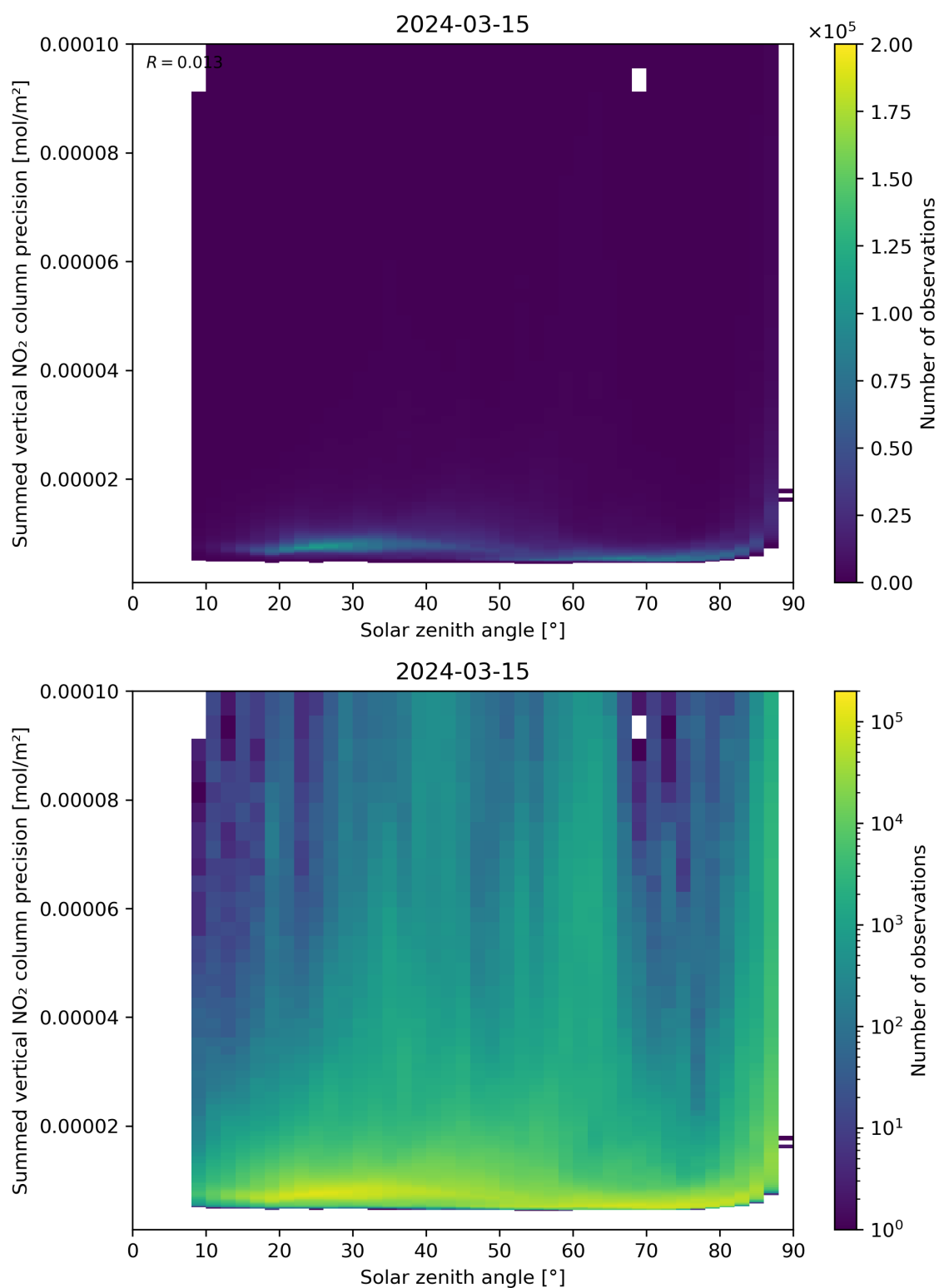
Figure 152: Scatter density plot of “Solar zenith angle” against “Summed vertical NO 2 column precision” for 2024-03-14 to 2024-03-16.
