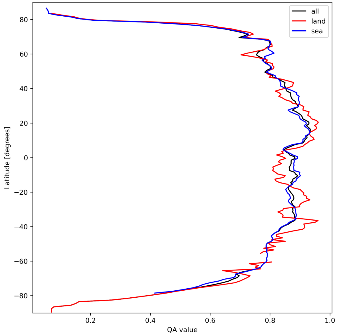
Figure 11: Zonal average of “QA value” for 2024-03-14 to 2024-03-16.
