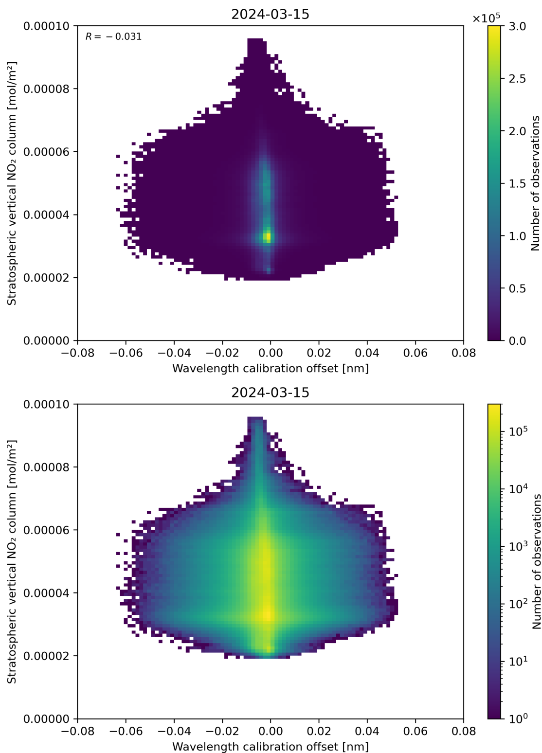
Figure 176: Scatter density plot of “Wavelength calibration offset” against “Stratospheric vertical NO 2 column” for 2024-03-14 to 2024-03-16.
