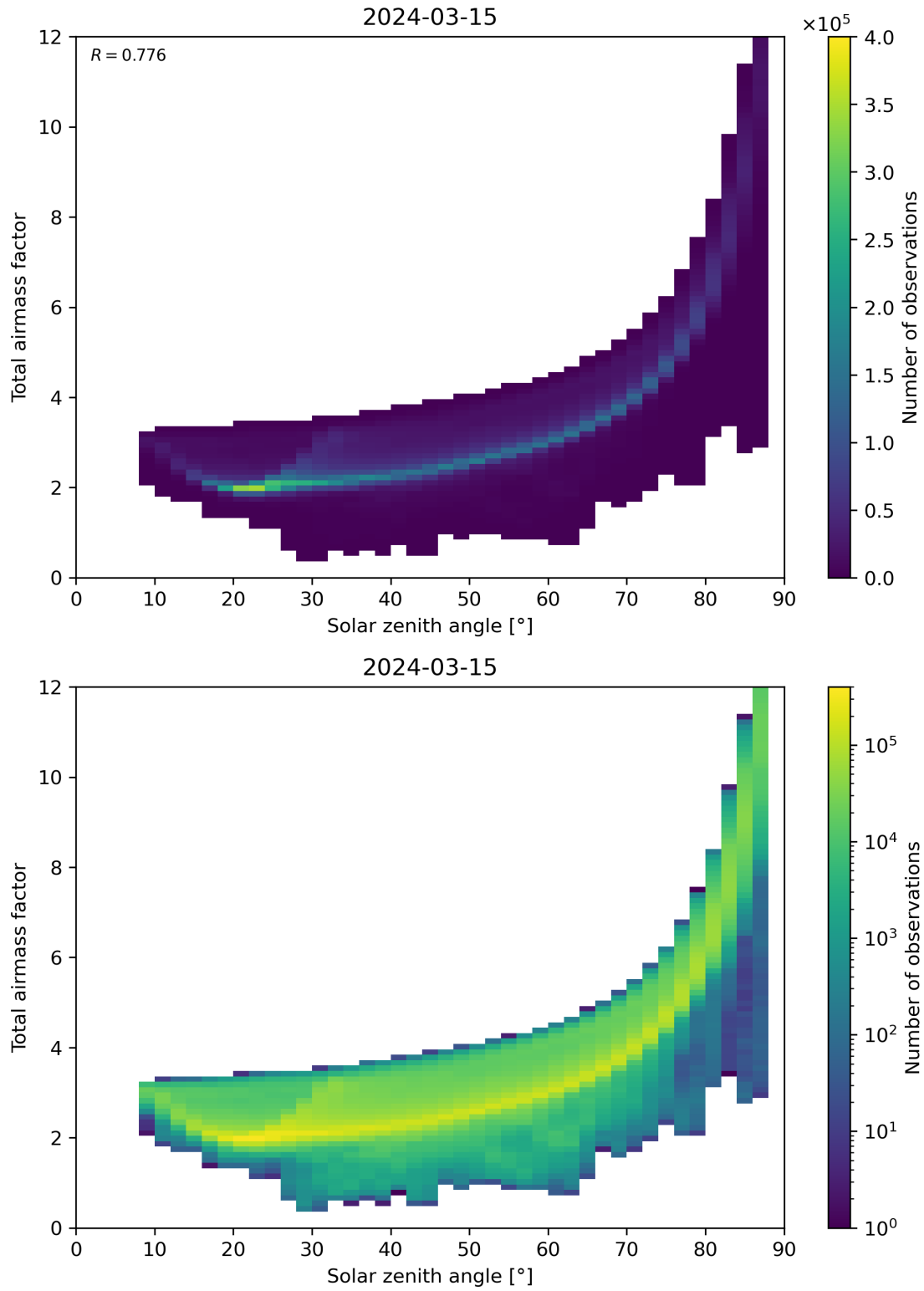
Figure 146: Scatter density plot of “Solar zenith angle” against “Total air mass factor” for 2024-03-14 to 2024-03-16.
