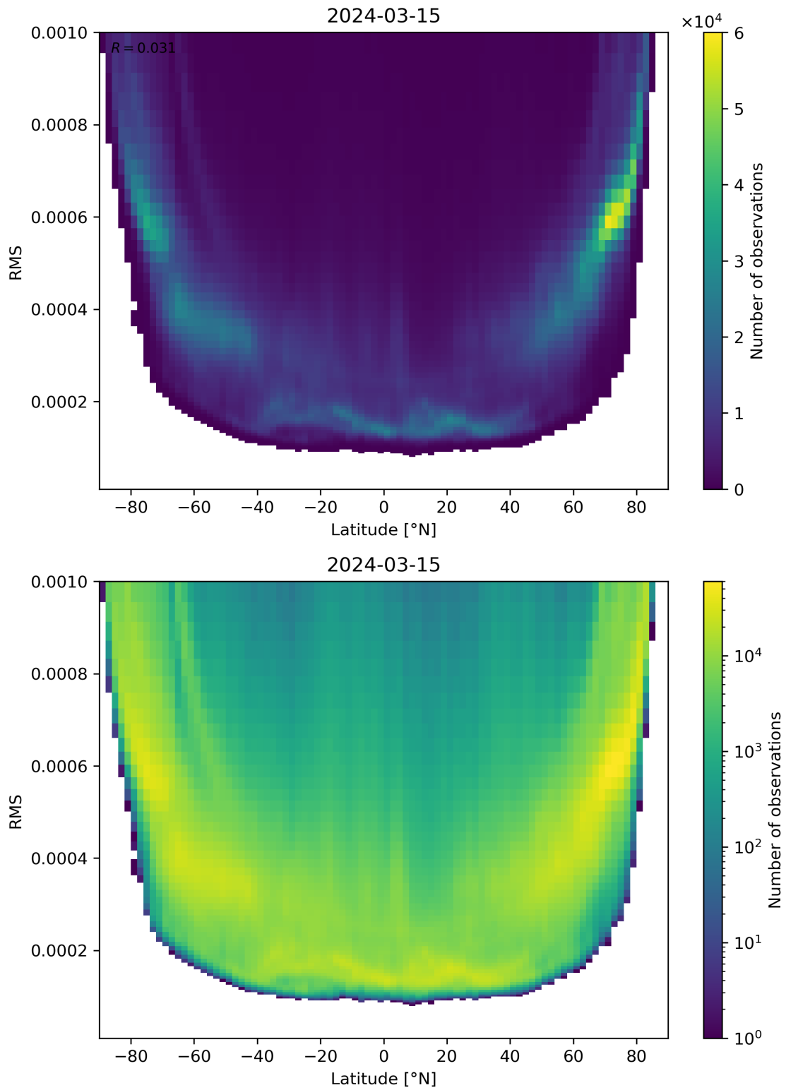
Figure 94: Scatter density plot of “Latitude” against “RMS” for 2024-03-14 to 2024-03-16.
