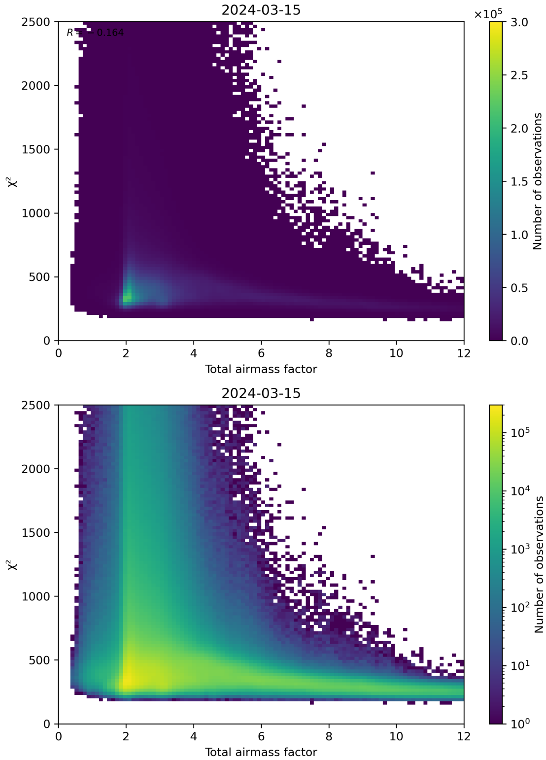
Figure 63: Scatter density plot of “Total airmass factor” against “ \chi^2 ” for 2024-03-14 to 2024-03-16.
