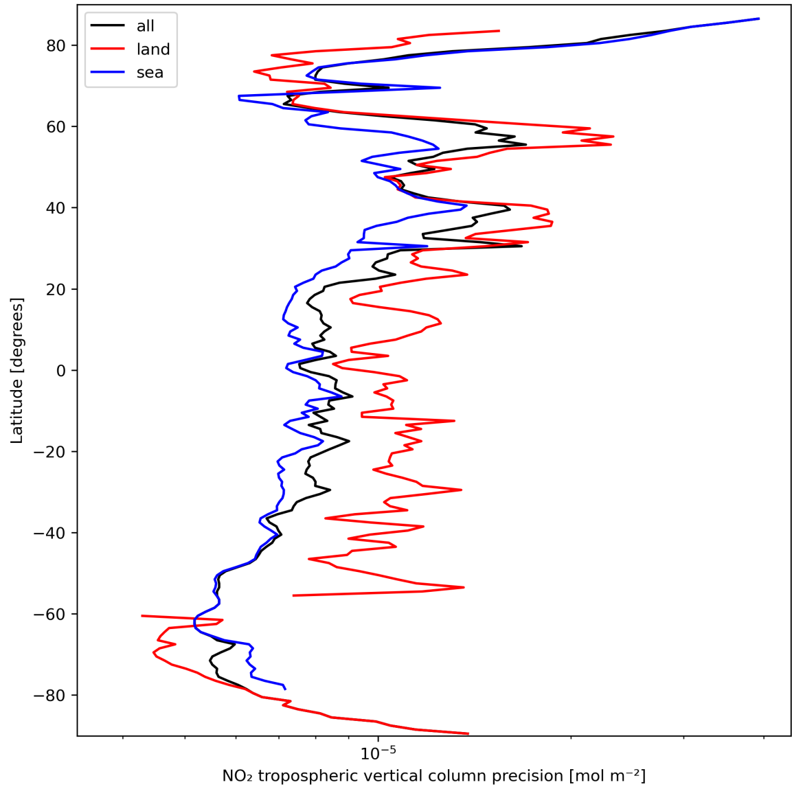
Figure 13: Zonal average of “NO 2 tropospheric vertical column precision” for 2024-03-14 to 2024-03-16.
