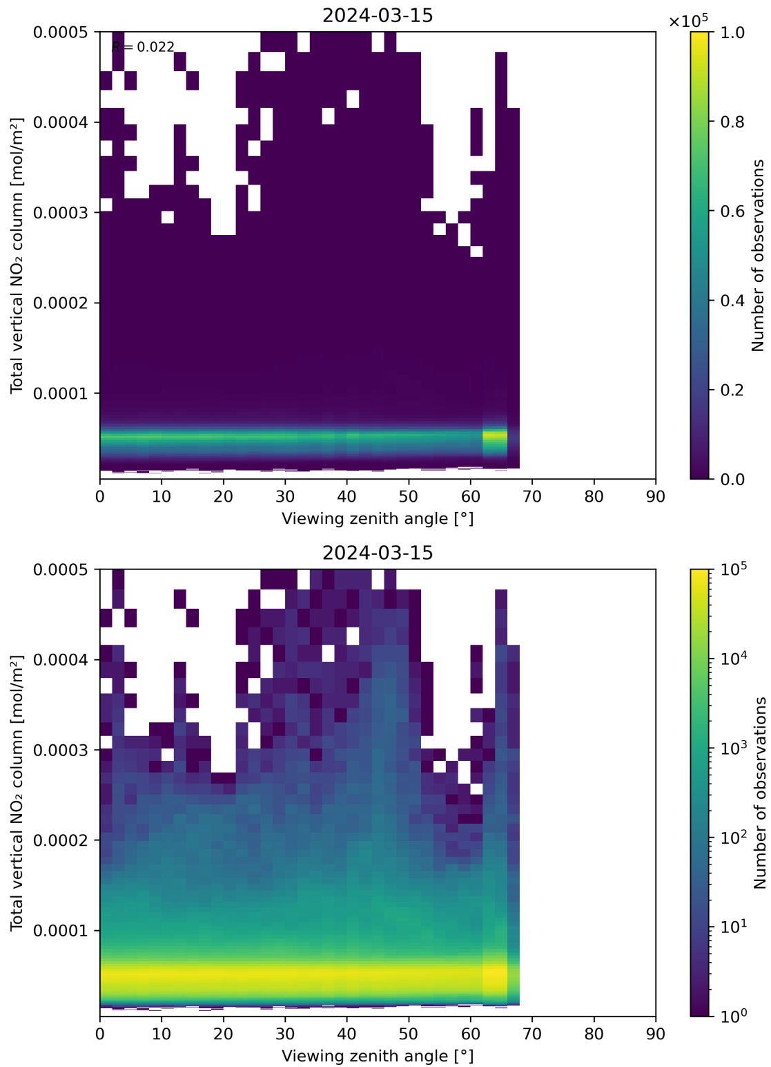
Figure 167: Scatter density plot of “Viewing zenith angle” against “Total vertical NO 2 column” for 2024-03-14 to 2024-03-16.
