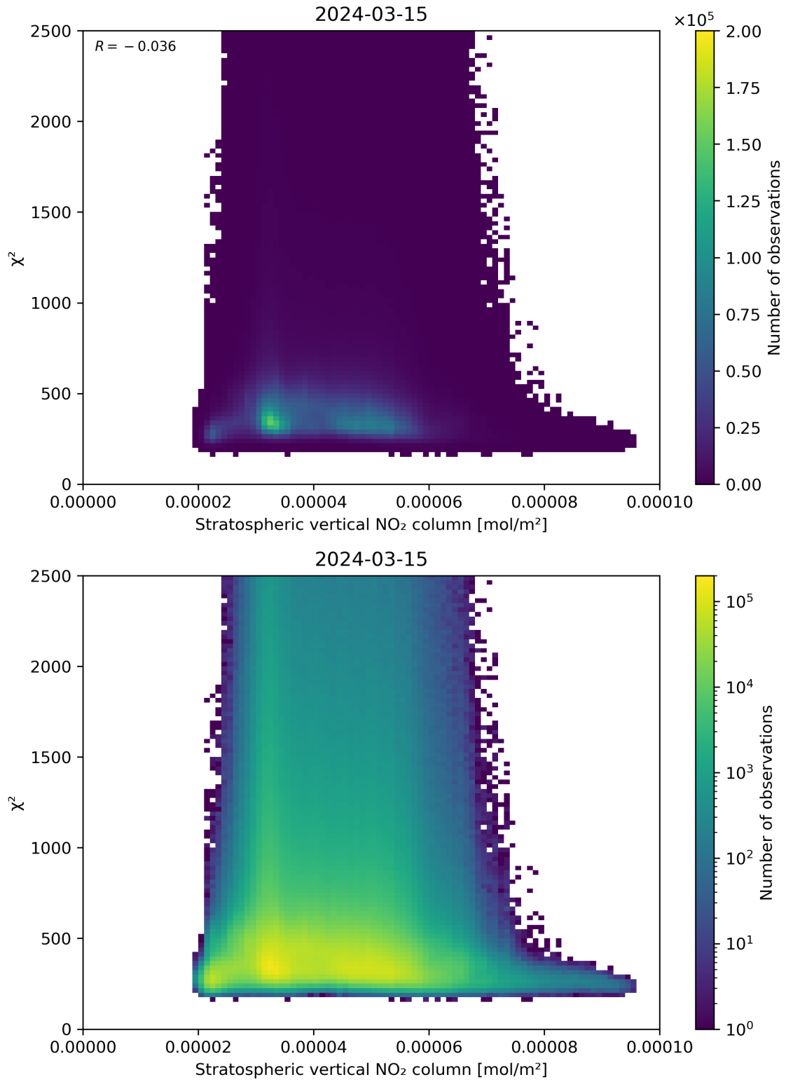
Figure 97: Scatter density plot of “Stratospheric vertical NO 2 column” against “ \chi^2 ” for 2024-03-14 to 2024-03-16.
