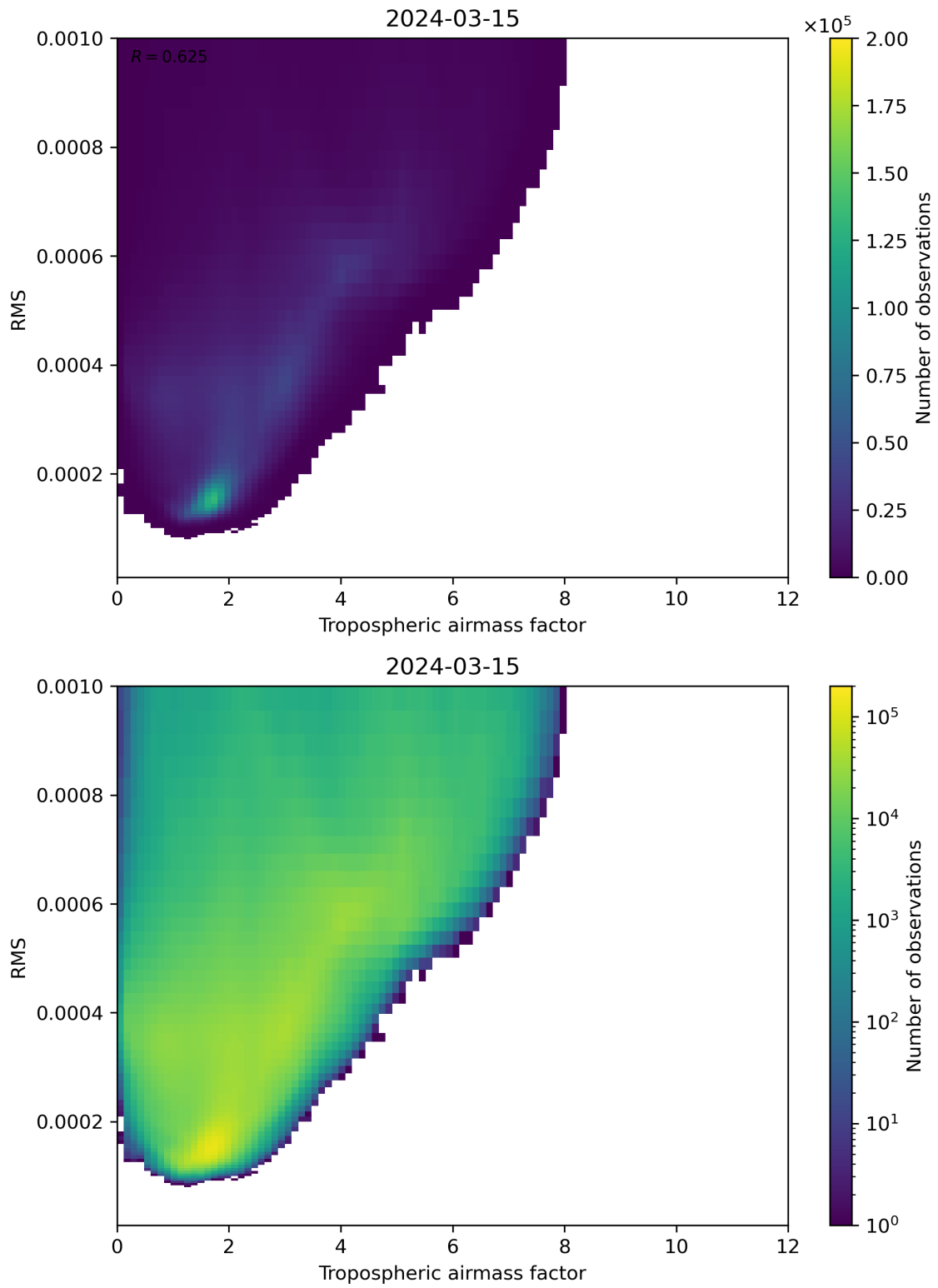
Figure 79: Scatter density plot of “Tropospheric airmass factor” against “RMS” for 2024-03-14 to 2024-03-16.
