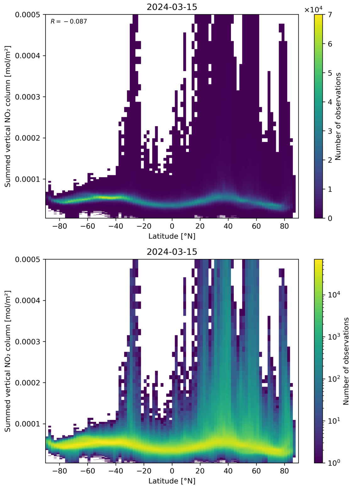
Figure 88: Scatter density plot of “Latitude” against “Summed vertical NO 2 column” for 2024-03-14 to 2024-03-16.
