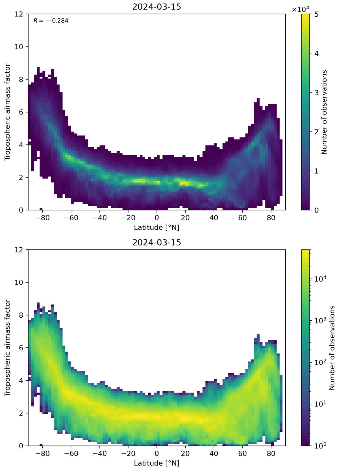
Figure 85: Scatter density plot of “Latitude” against “Tropospheric airmass factor” for 2024-03-14 to 2024-03-16.
