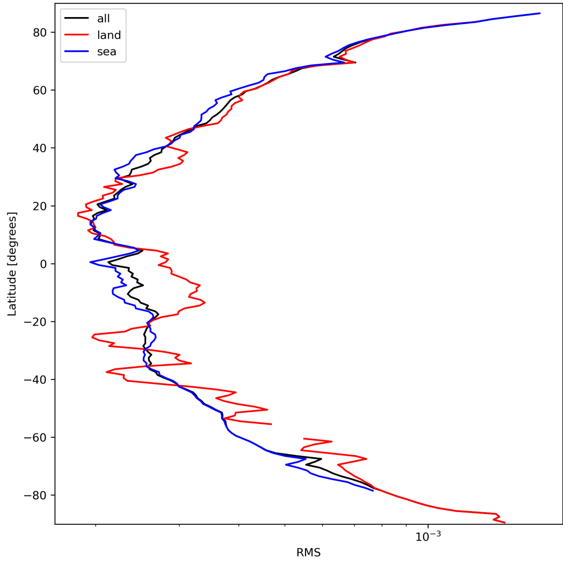
Figure 26: Zonal average of “RMS” for 2024-03-14 to 2024-03-16.
