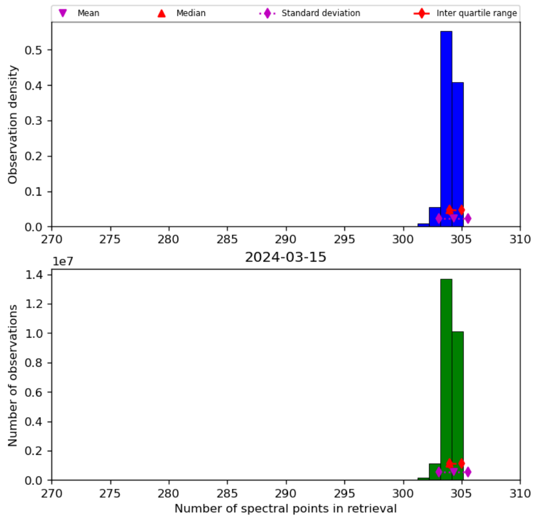
Figure 33: Histogram of “Number of spectral points in retrieval” for 2024-03-14 to 2024-03-16
