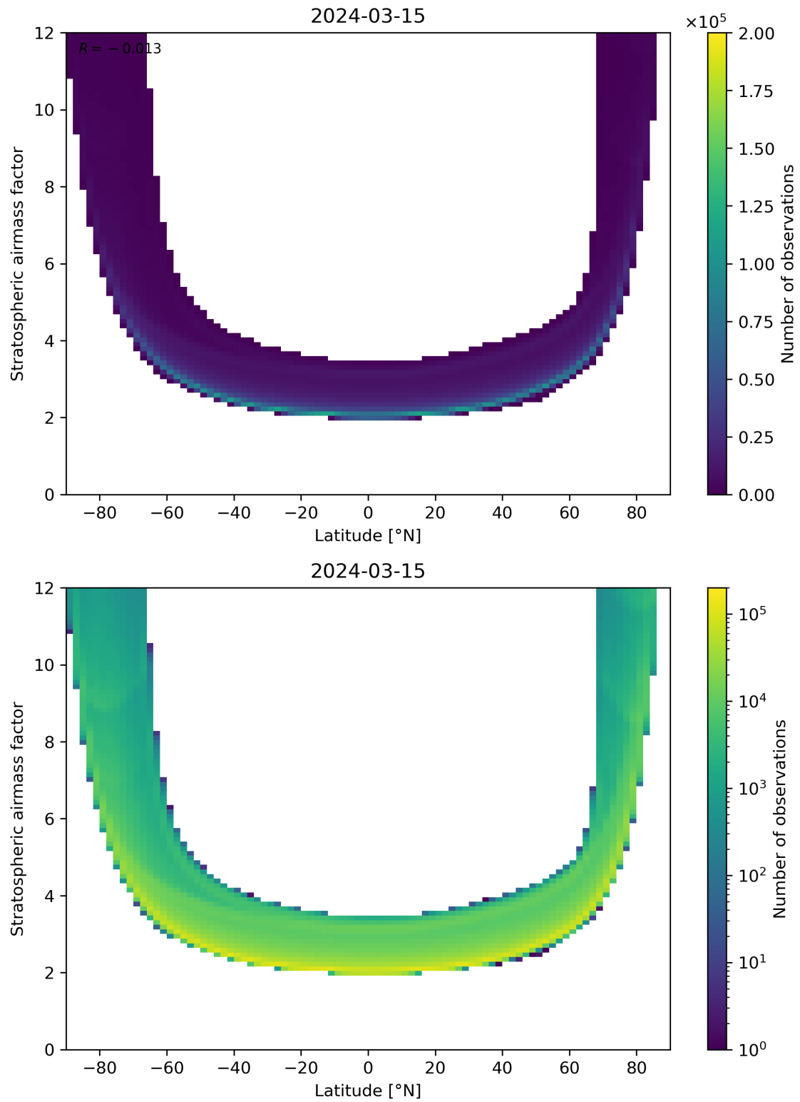
Figure 83: Scatter density plot of “Latitude” against “Stratospheric air mass factor” for 2024-03-14 to 2024-03-16.
