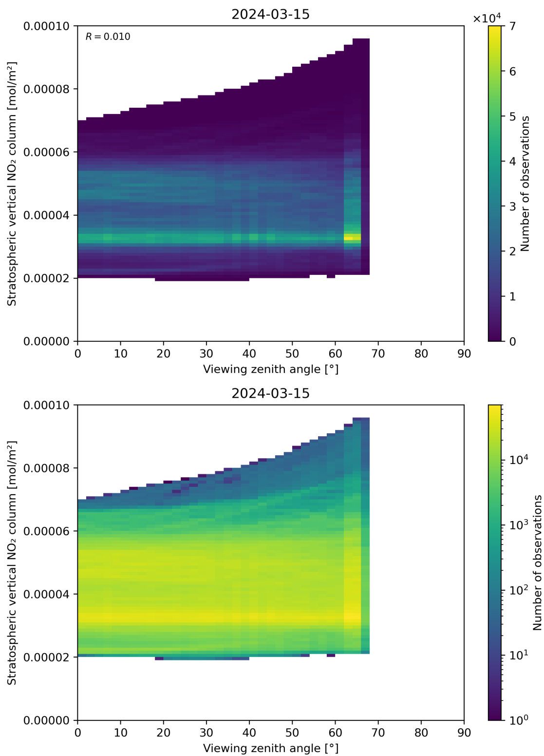
Figure 164: Scatter density plot of “Viewing zenith angle” against “Stratospheric vertical NO 2 column” for 2024-03-14 to 2024-03-16.
