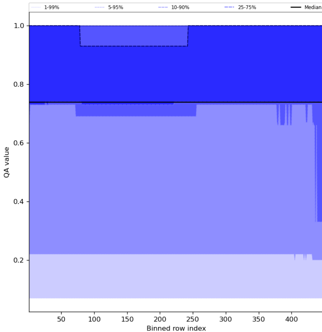
Figure 45: Along track statistics of “QA value” for 2024-03-14 to 2024-03-16
