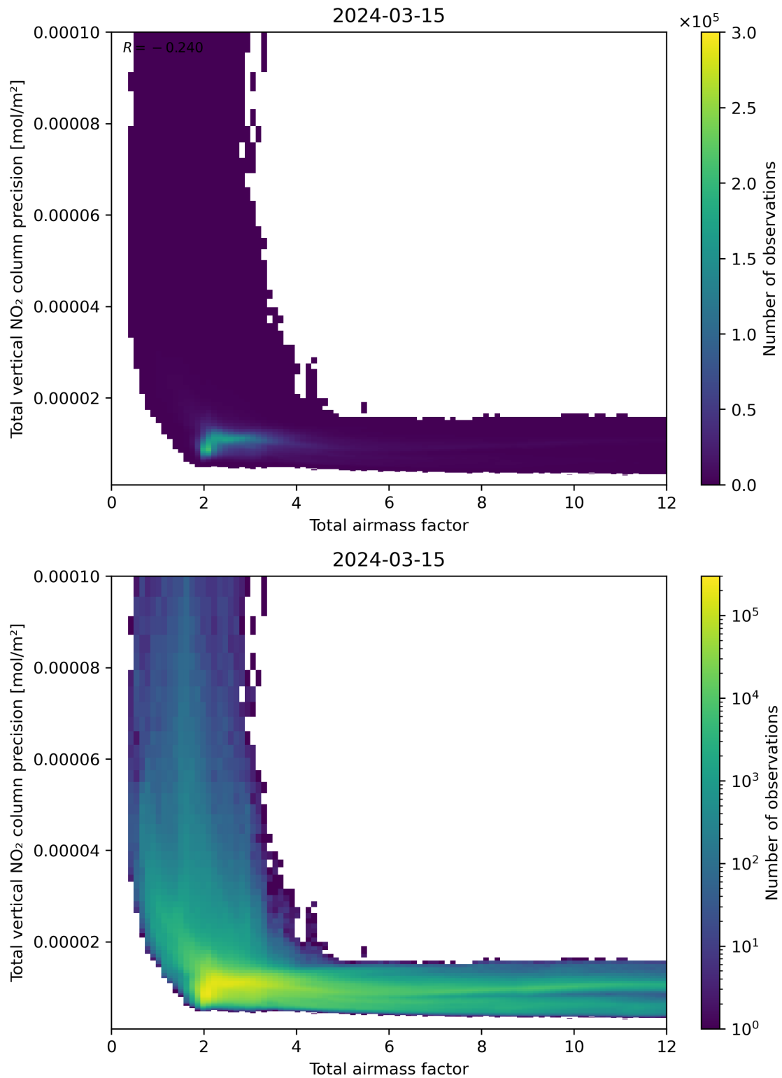
Figure 68: Scatter density plot of “Total airmass factor” against “Total vertical NO 2 column precision” for 2024-03-14 to 2024-03-16.
