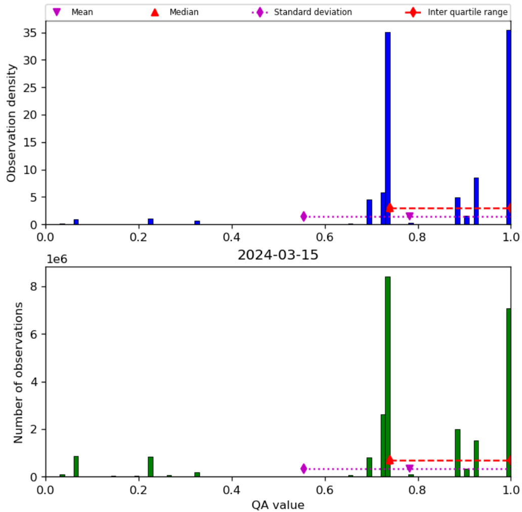
Figure 28: Histogram of “QA value” for 2024-03-14 to 2024-03-16
