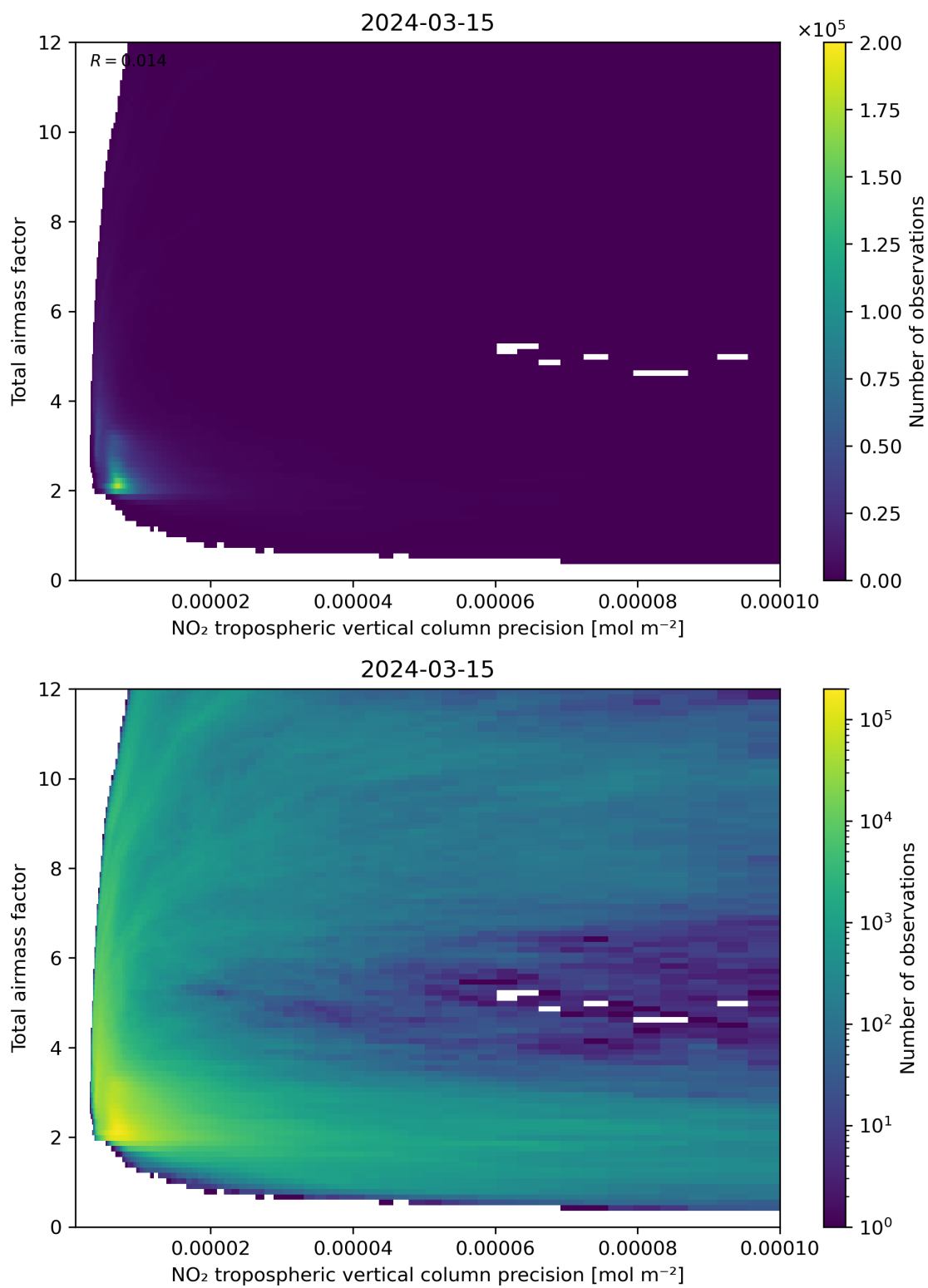
Figure 132: Scatter density plot of “NO 2 tropospheric vertical column precision” against “Total air mass factor” for 2024-03-14 to 2024-03-16.
