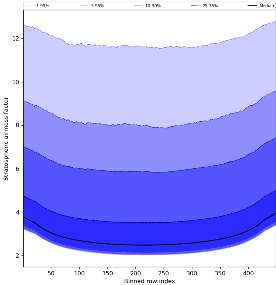
Figure 61: Along track statistics of “Stratospheric airmass factor” for 2024-03-14 to 2024-03-16
