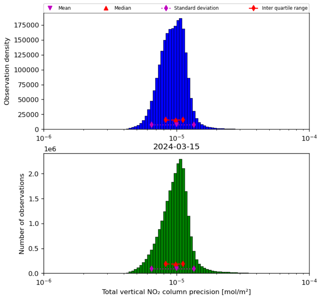
Figure 39: Histogram of “Total vertical NO 2 column precision” for 2024-03-14 to 2024-03-16
