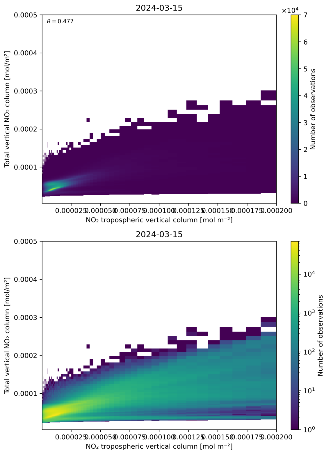
Figure 128: Scatter density plot of “NO 2 tropospheric vertical column” against “Total vertical NO 2 column” for 2024-03-14 to 2024-03-16.
