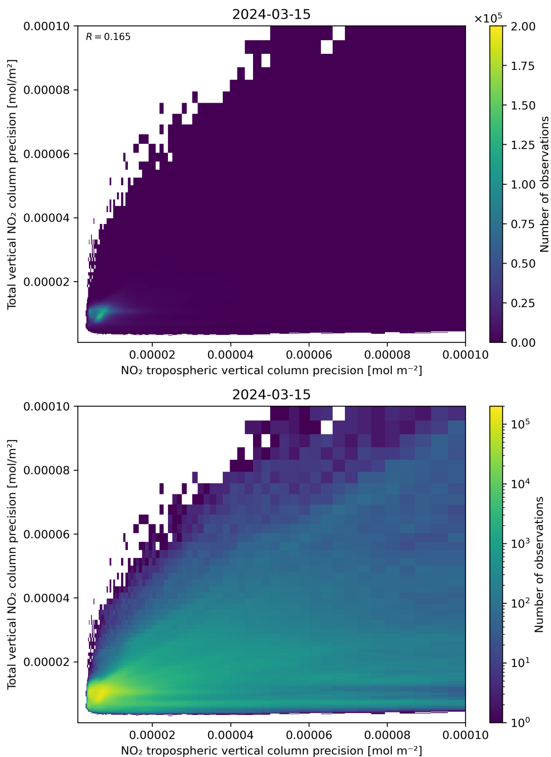
Figure 139: Scatter density plot of “NO 2 tropospheric vertical column precision” against “Total vertical NO 2 column precision” for 2024-03-14 to 2024-03-16.
