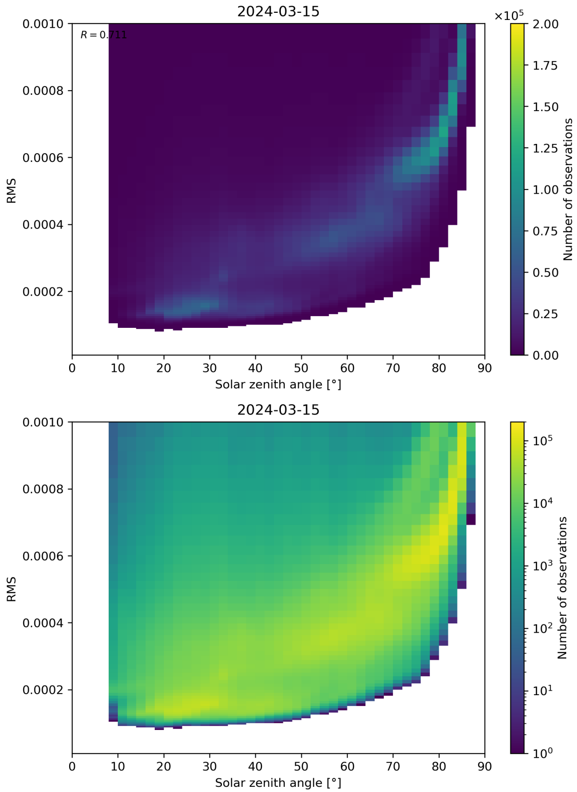
Figure 157: Scatter density plot of “Solar zenith angle” against “RMS” for 2024-03-14 to 2024-03-16.
