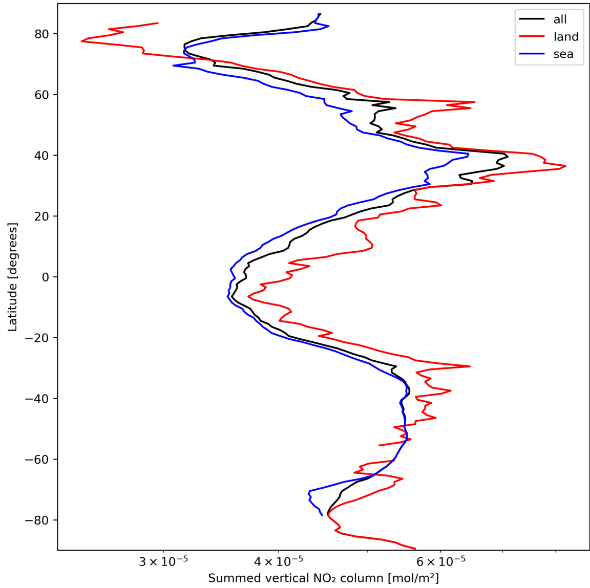
Figure 23: Zonal average of “Summed vertical NO 2 column” for 2024-03-14 to 2024-03-16.
