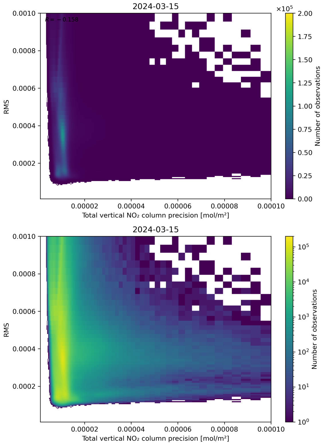
Figure 119: Scatter density plot of “Total vertical NO 2 column precision” against “RMS” for 2024-03-14 to 2024-03-16.
