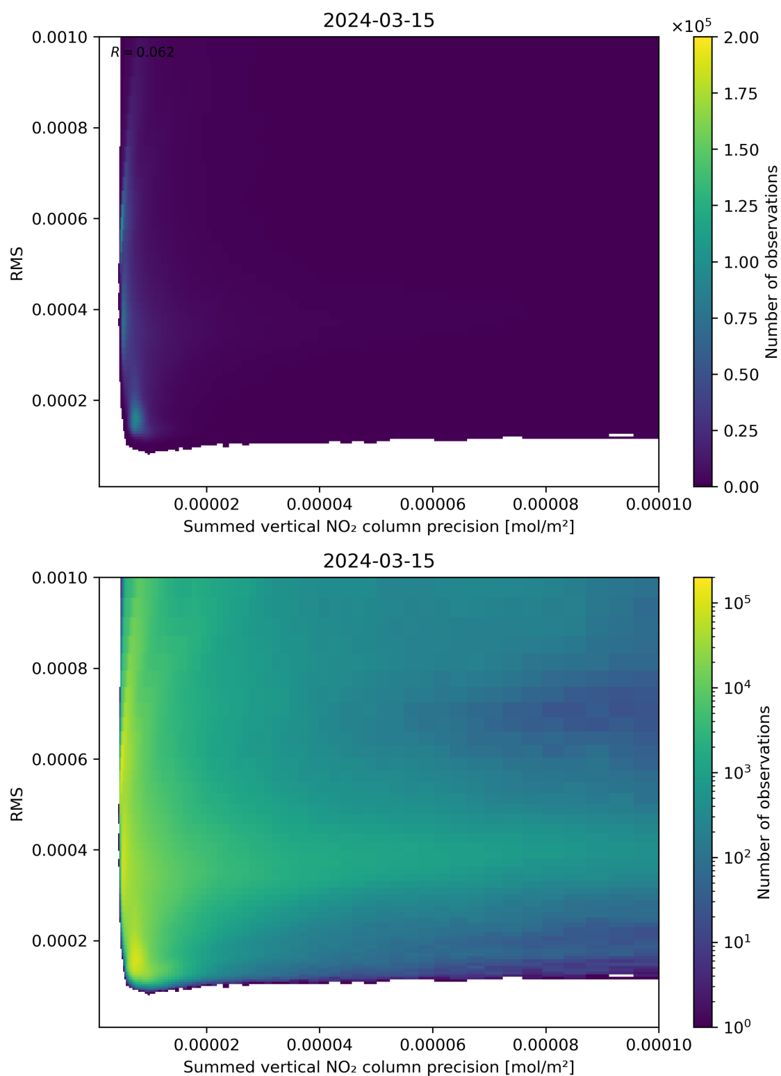
Figure 108: Scatter density plot of “Summed vertical NO 2 column precision” against “RMS” for 2024-03-14 to 2024-03-16.
