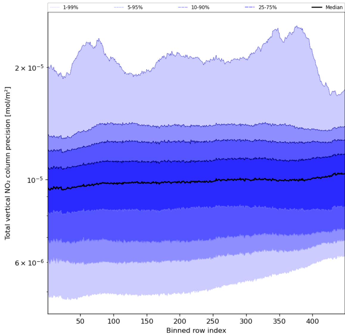
Figure 56: Along track statistics of “Total vertical NO 2 column precision” for 2024-03-14 to 2024-03-16
