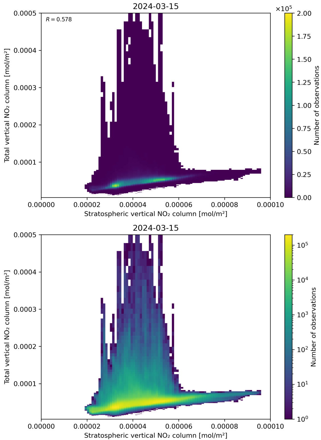
Figure 100: Scatter density plot of “Stratospheric vertical NO 2 column” against “Total vertical NO 2 column” for 2024-03-14 to 2024-03-16.
