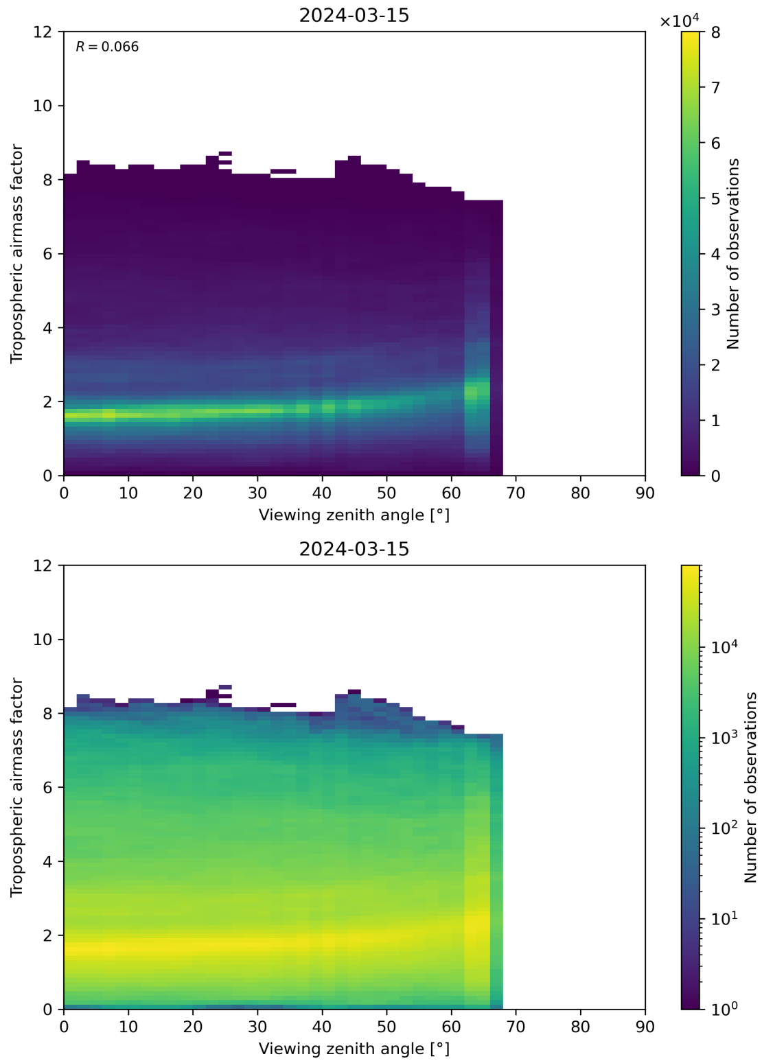
Figure 161: Scatter density plot of “Viewing zenith angle” against “Tropospheric airmass factor” for 2024-03-14 to 2024-03-16.
