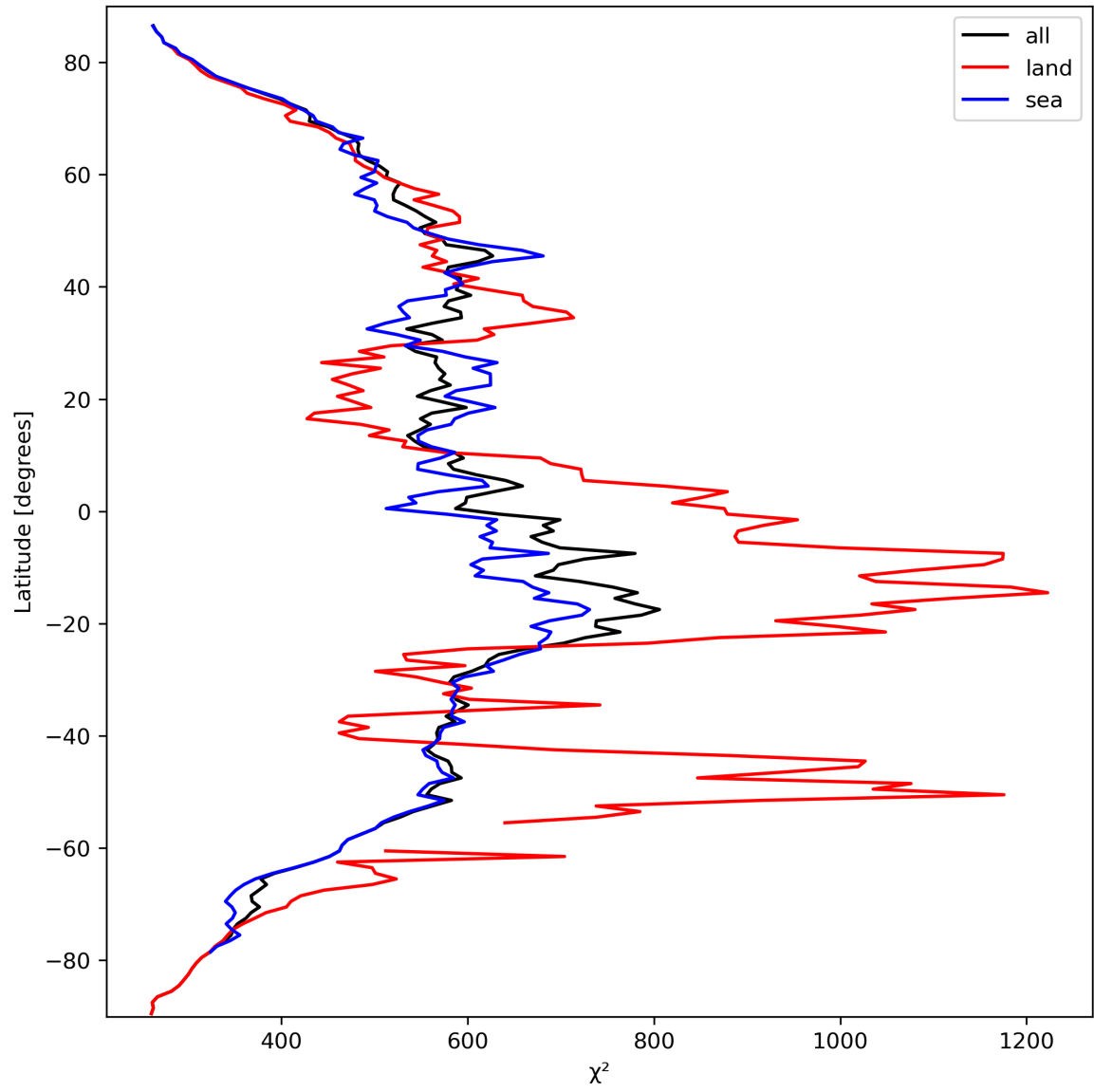
Figure 25: Zonal average of “ \chi^2 ” for 2024-03-14 to 2024-03-16.
