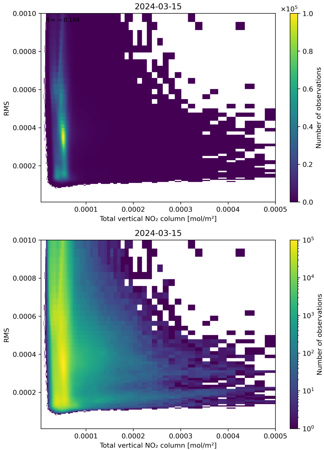
Figure 120: Scatter density plot of “Total vertical NO 2 column” against “RMS” for 2024-03-14 to 2024-03-16.
