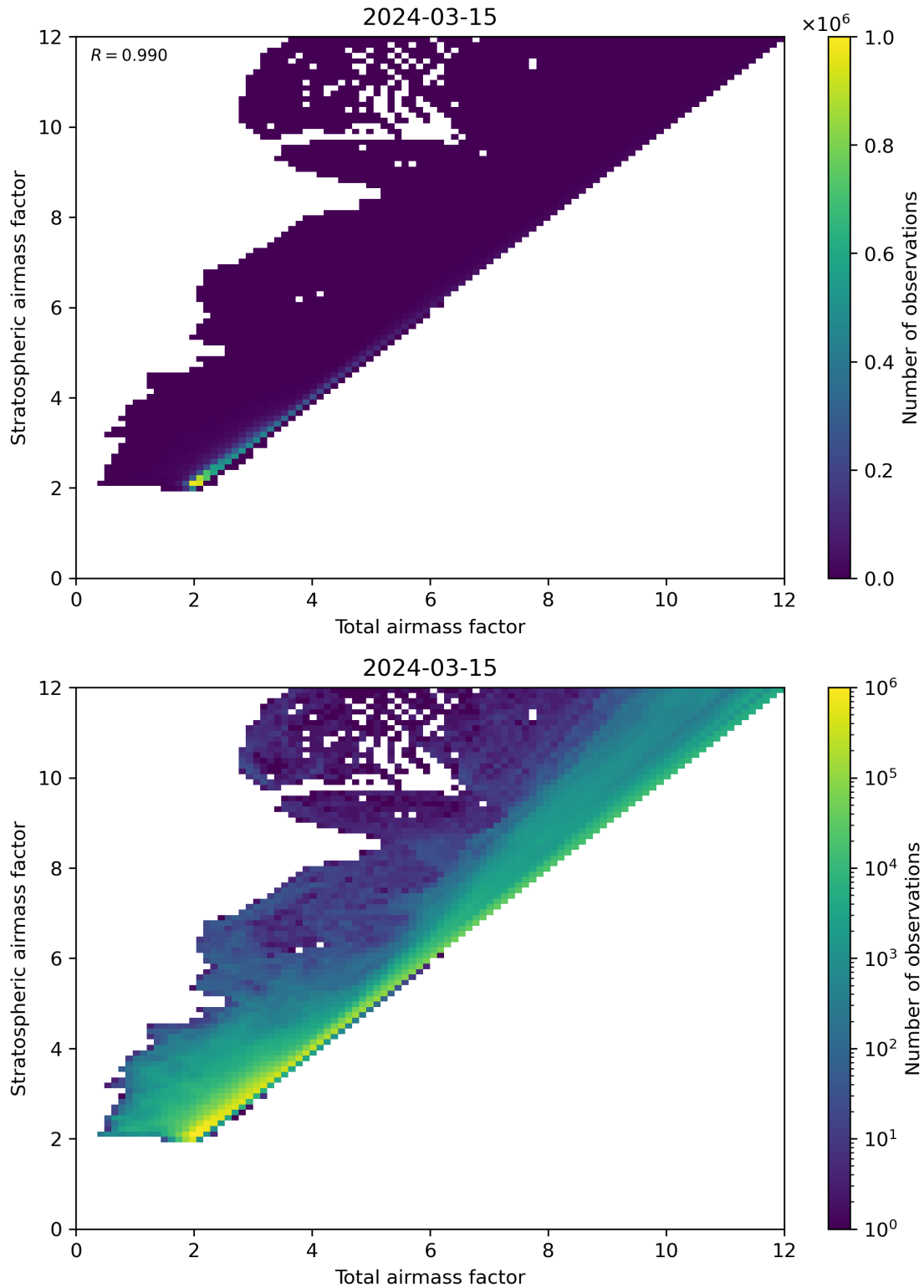
Figure 62: Scatter density plot of “Total airmass factor” against “Stratospheric airmass factor” for 2024-03-14 to 2024-03-16.
