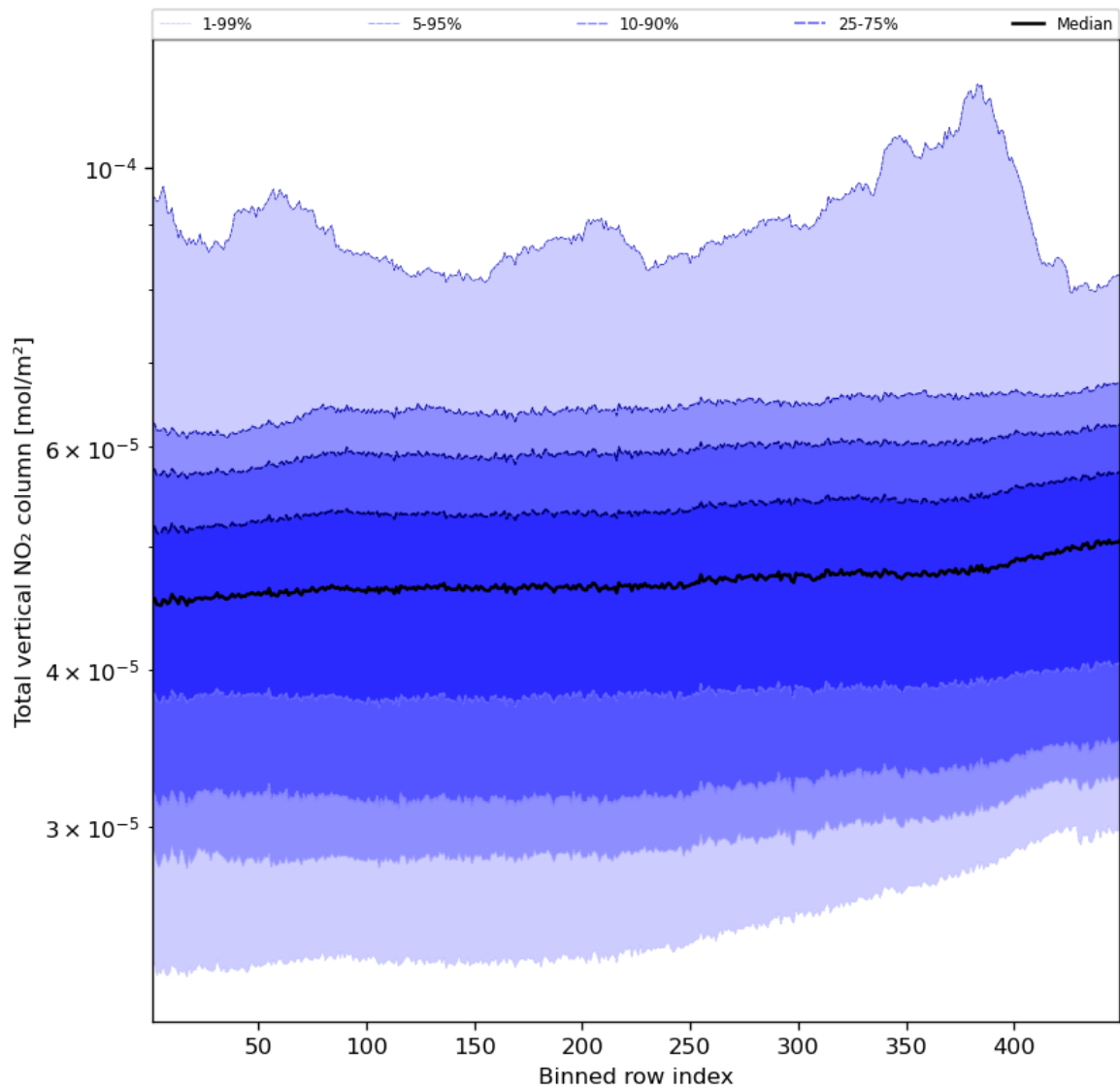
Figure 55: Along track statistics of “Total vertical NO 2 column” for 2024-03-14 to 2024-03-16
