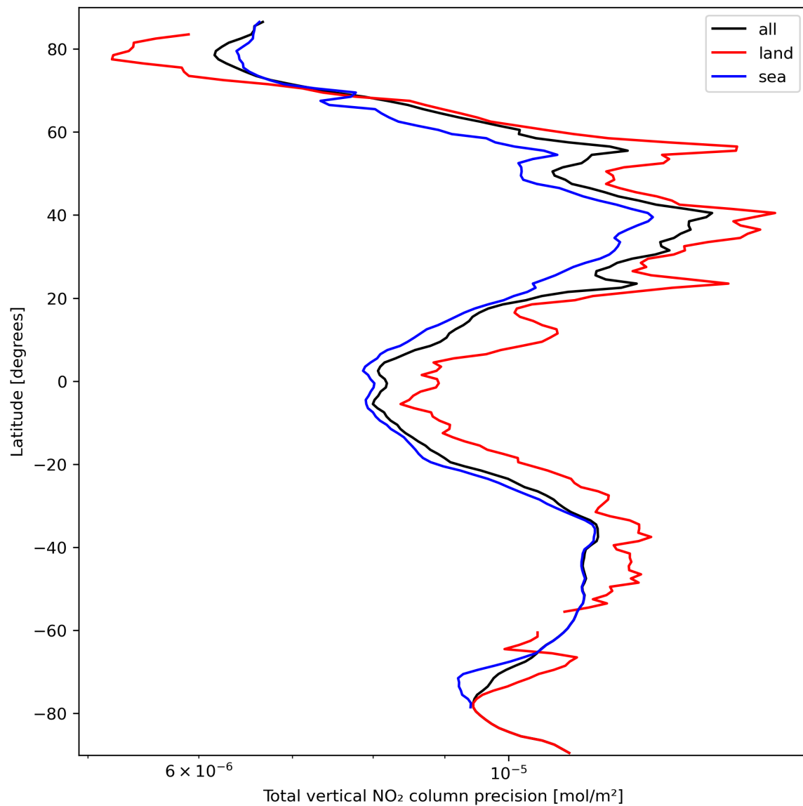
Figure 22: Zonal average of “Total vertical NO 2 column precision” for 2024-03-14 to 2024-03-16.
