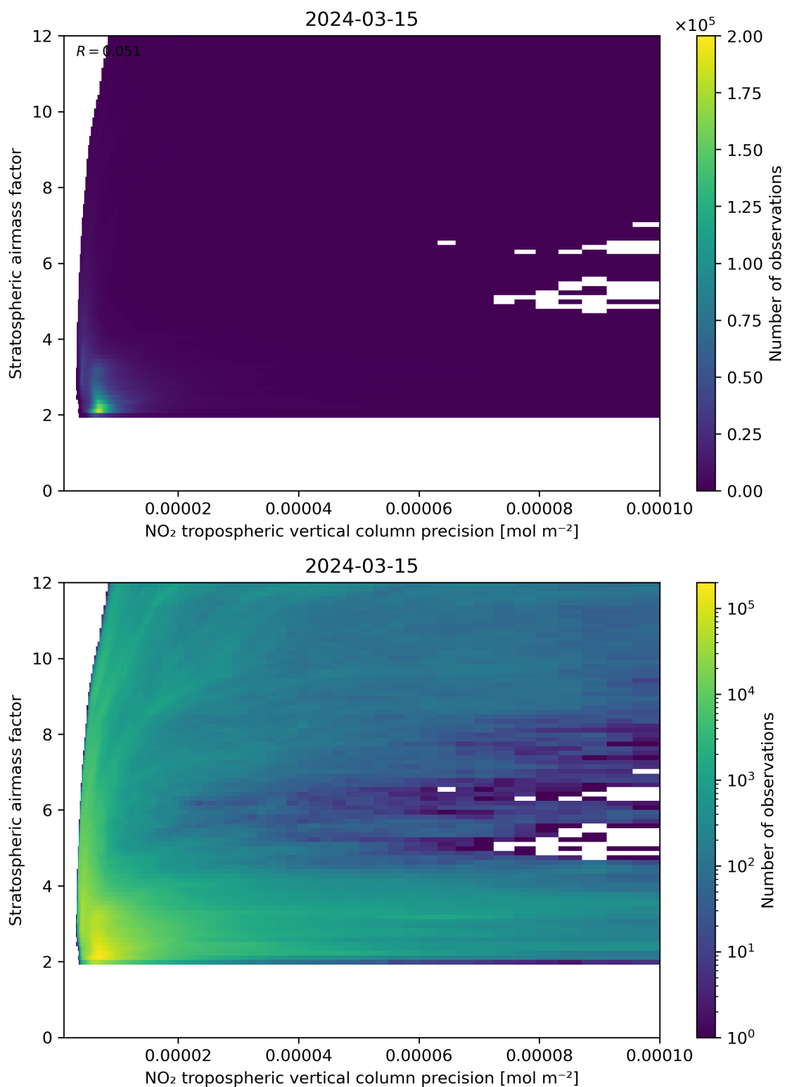
Figure 131: Scatter density plot of “NO 2 tropospheric vertical column precision” against “Stratospheric airmass factor” for 2024-03-14 to 2024-03-16.
