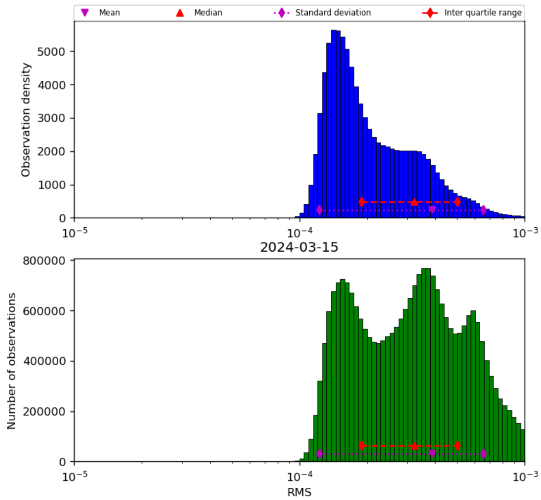
Figure 43: Histogram of “RMS” for 2024-03-14 to 2024-03-16
