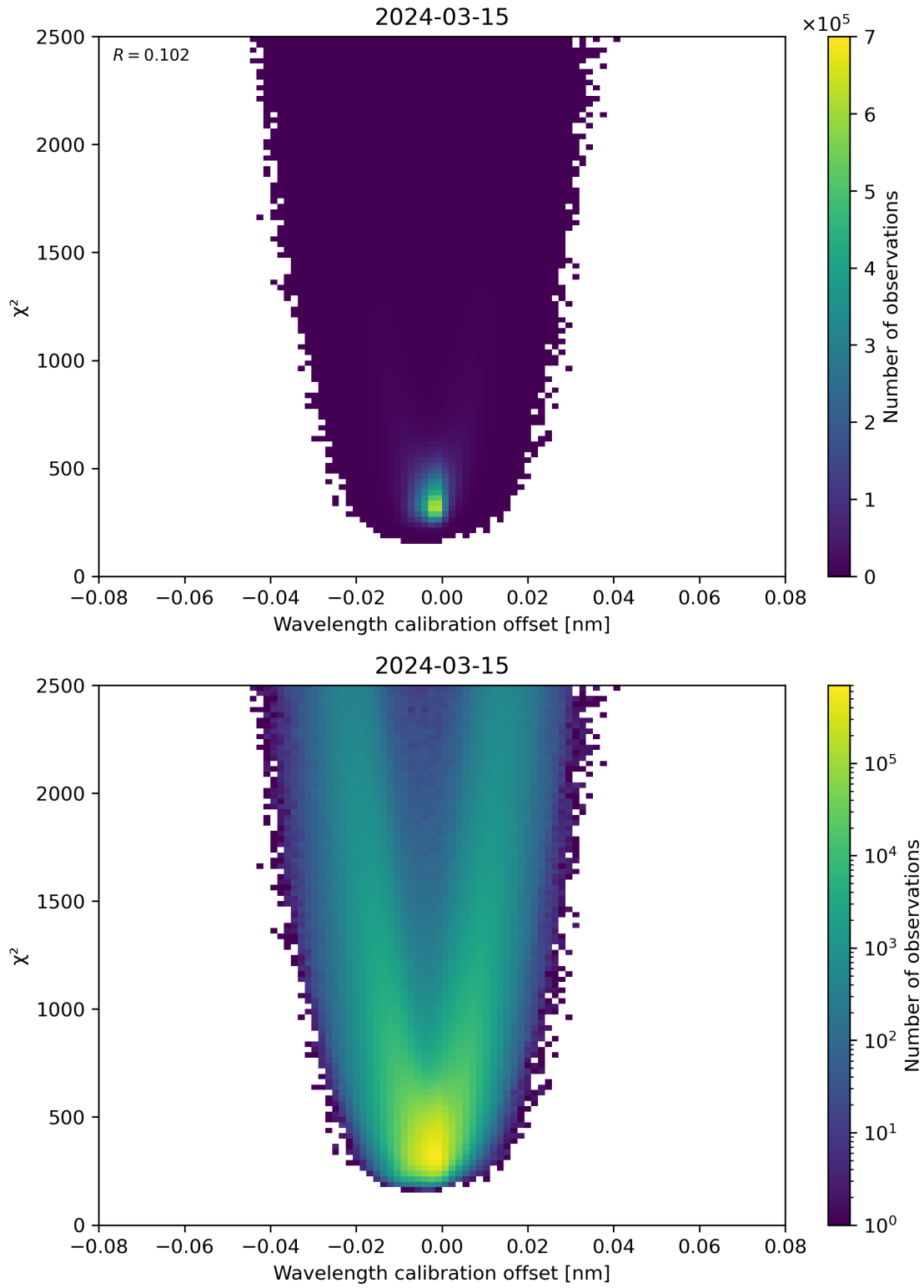
Figure 175: Scatter density plot of “Wavelength calibration offset” against “ \chi^2 ” for 2024-03-14 to 2024-03-16.
