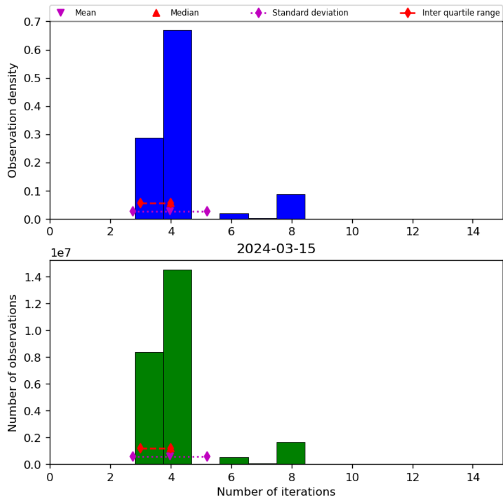
Figure 34: Histogram of “Number of iterations” for 2024-03-14 to 2024-03-16
