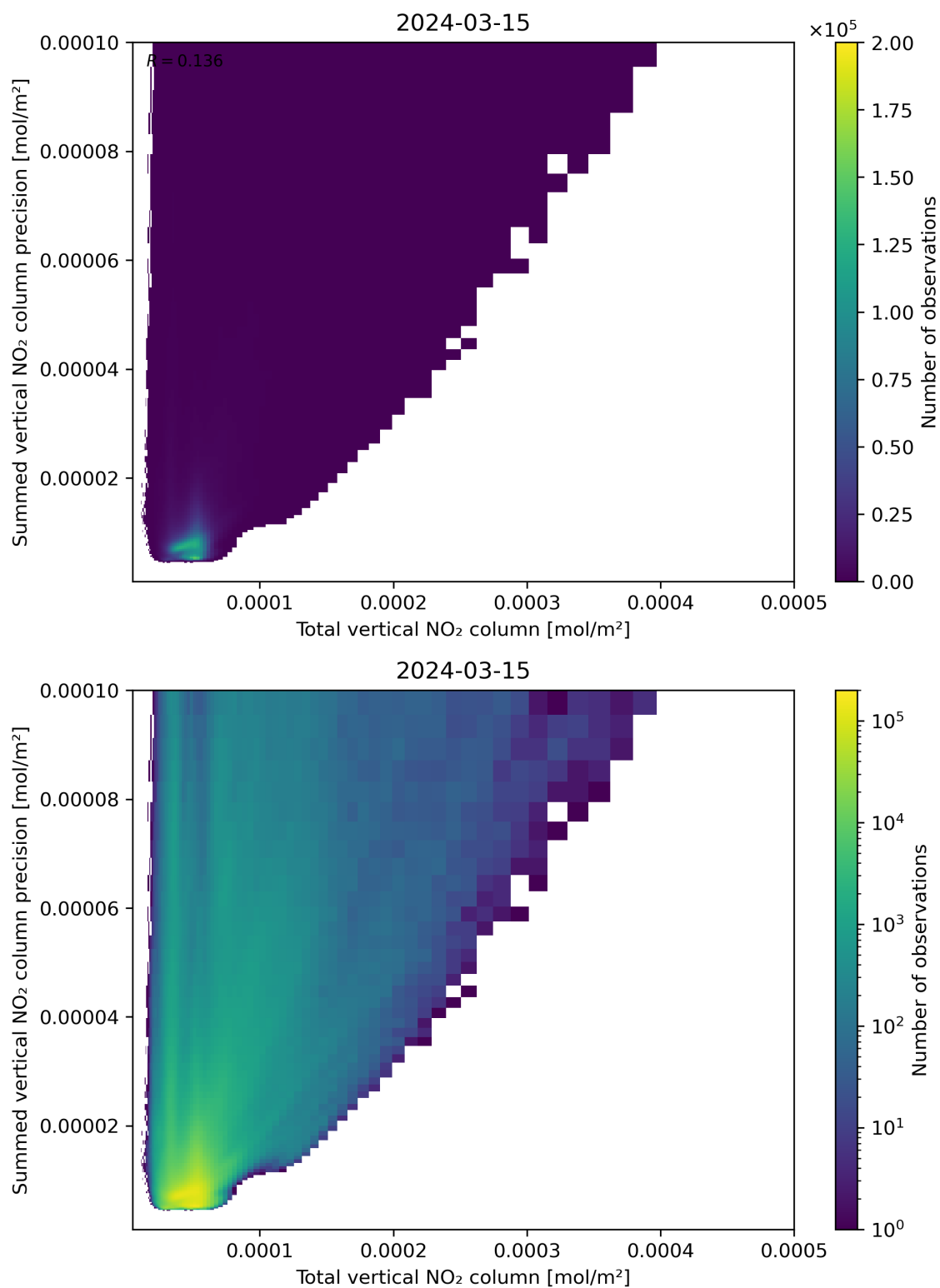
Figure 113: Scatter density plot of “Total vertical NO 2 column” against “Summed vertical NO 2 column precision” for 2024-03-14 to 2024-03-16.
