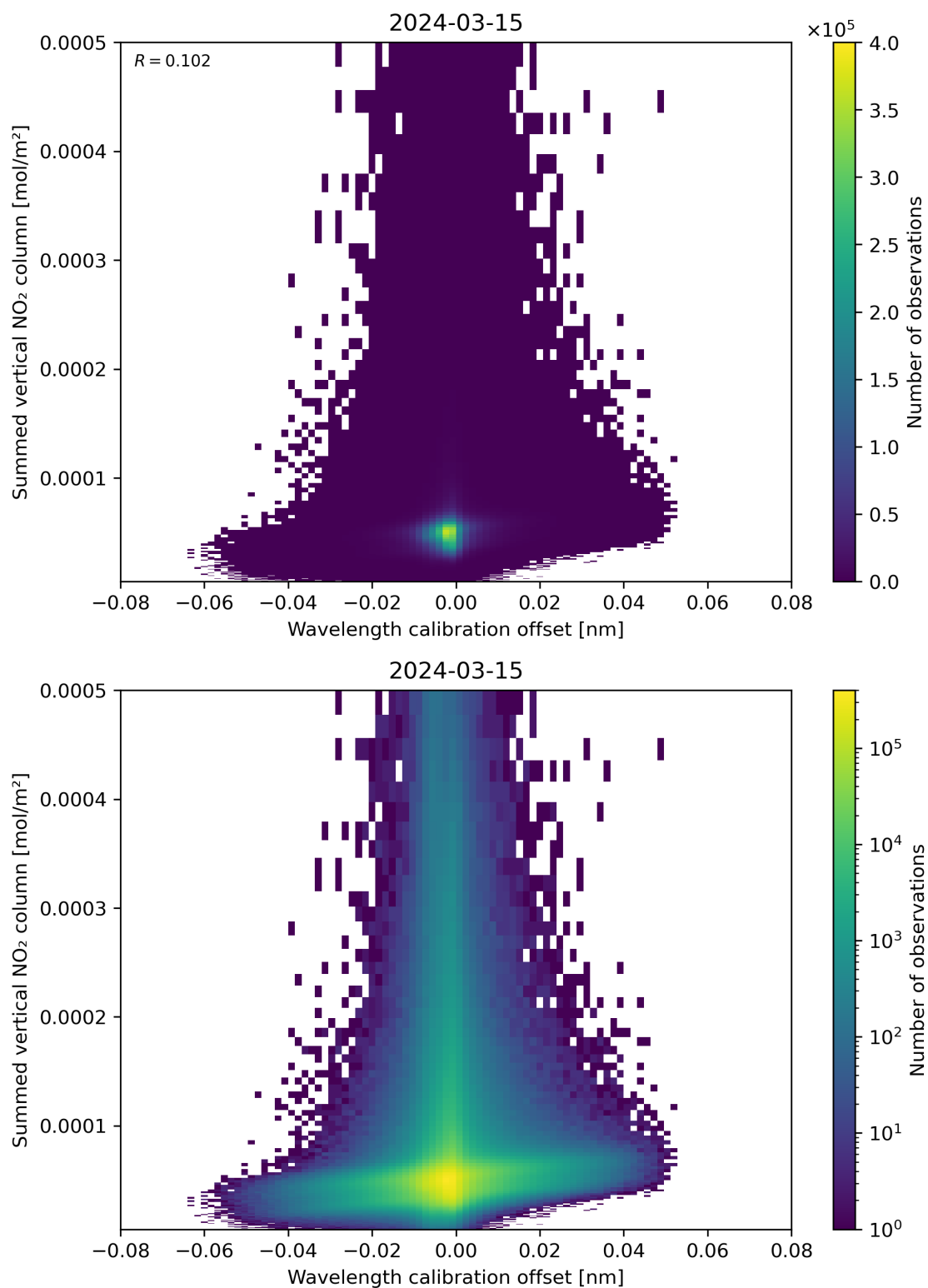
Figure 177: Scatter density plot of “Wavelength calibration offset” against “Summed vertical NO 2 column” for 2024-03-14 to 2024-03-16.
