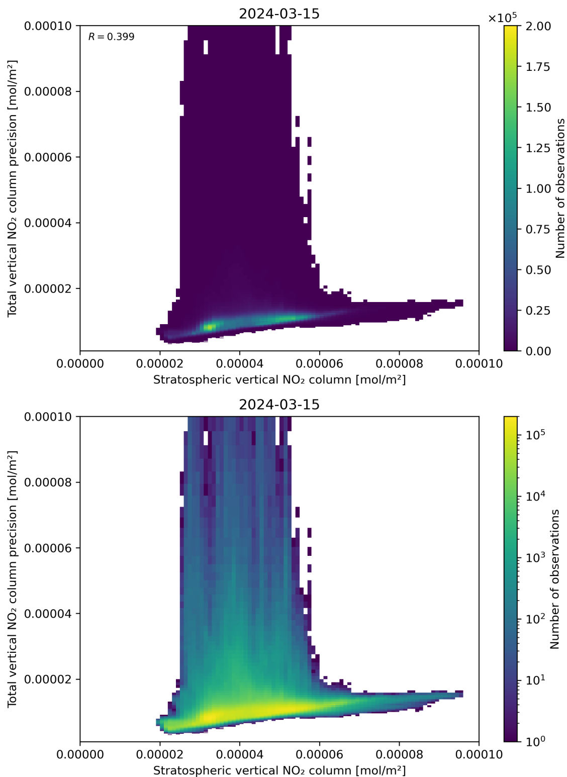
Figure 101: Scatter density plot of “Stratospheric vertical NO 2 column” against “Total vertical NO 2 column precision” for 2024-03-14 to 2024-03-16.
