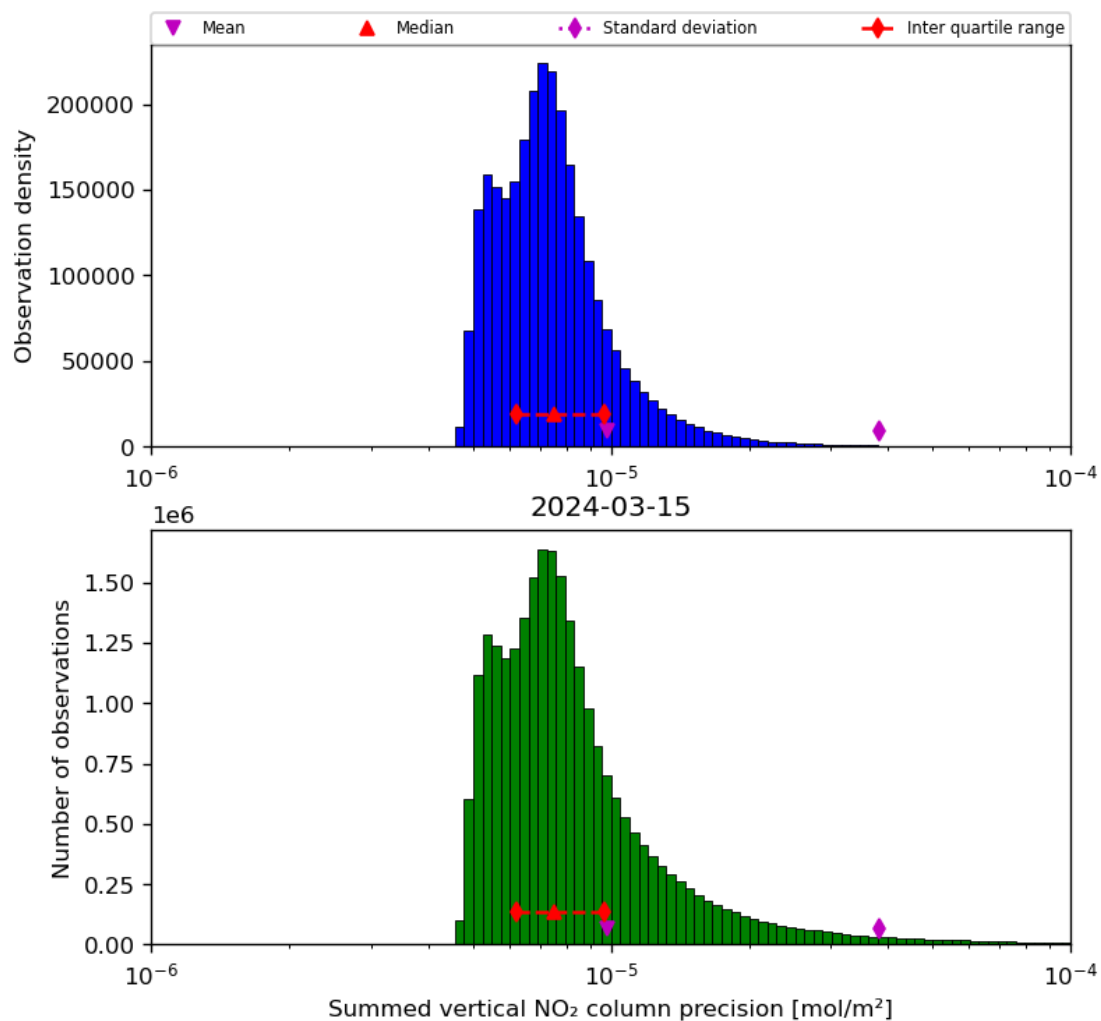
Figure 41: Histogram of "Summed vertical NO 2 column precision" for 2024-03-14 to 2024-03-16
