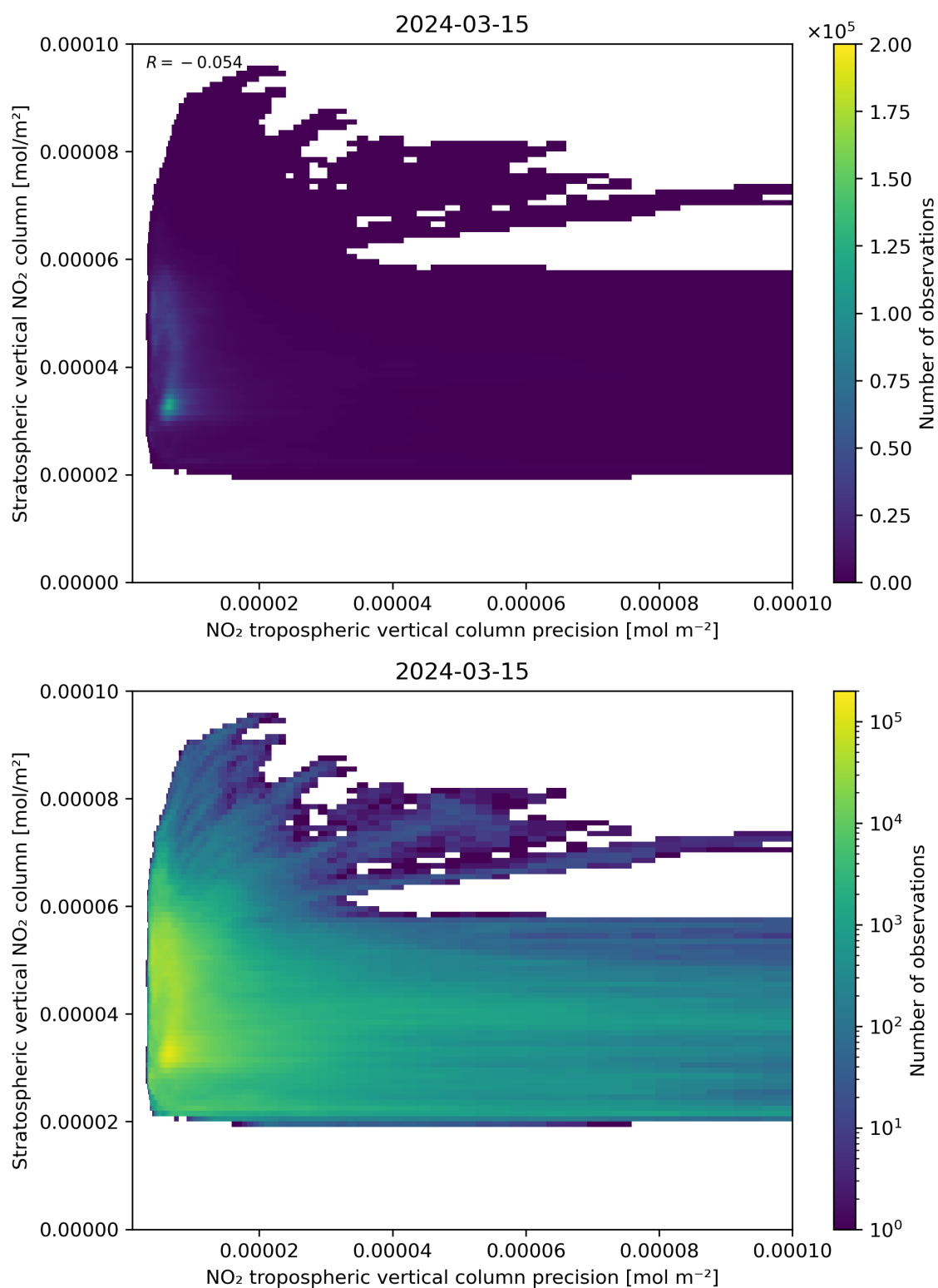
Figure 135: Scatter density plot of “NO 2 tropospheric vertical column precision” against “Stratospheric vertical NO 2 column” for 2024-03-14 to 2024-03-16.
