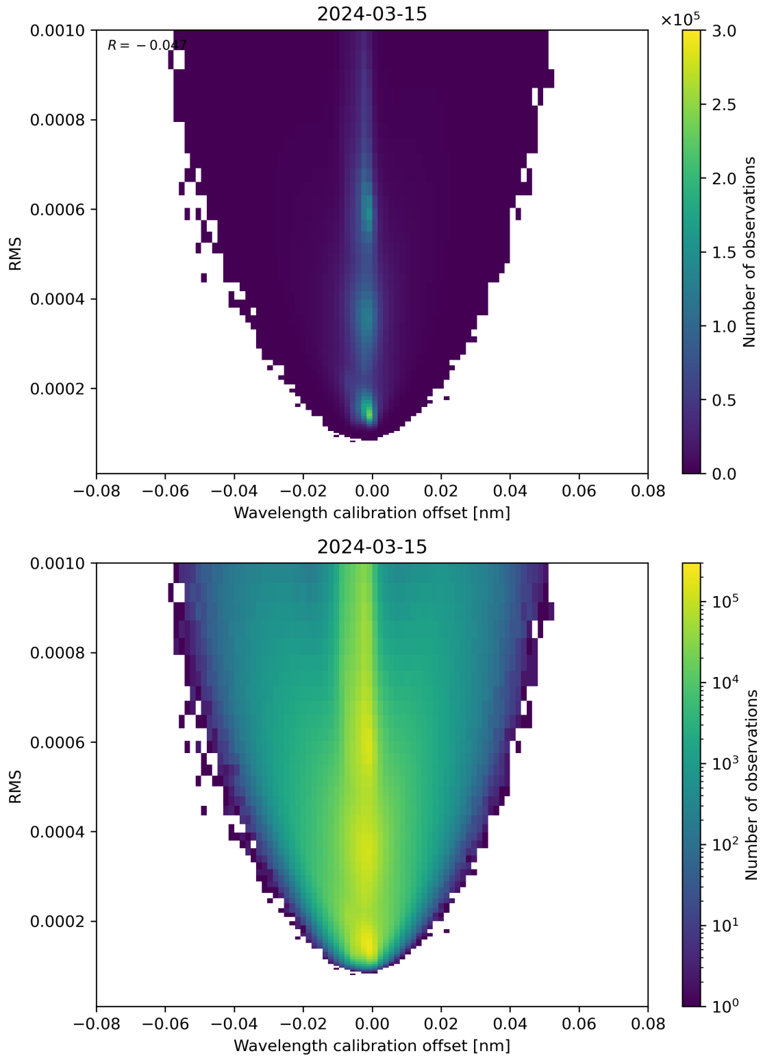
Figure 181: Scatter density plot of “Wavelength calibration offset” against “RMS” for 2024-03-14 to 2024-03-16.
