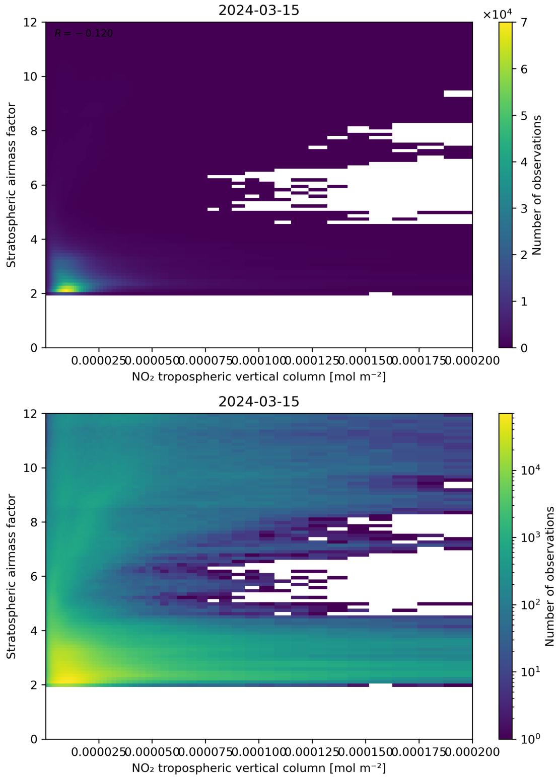
Figure 121: Scatter density plot of “NO 2 tropospheric vertical column” against “Stratospheric air mass factor” for 2024-03-14 to 2024-03-16.
