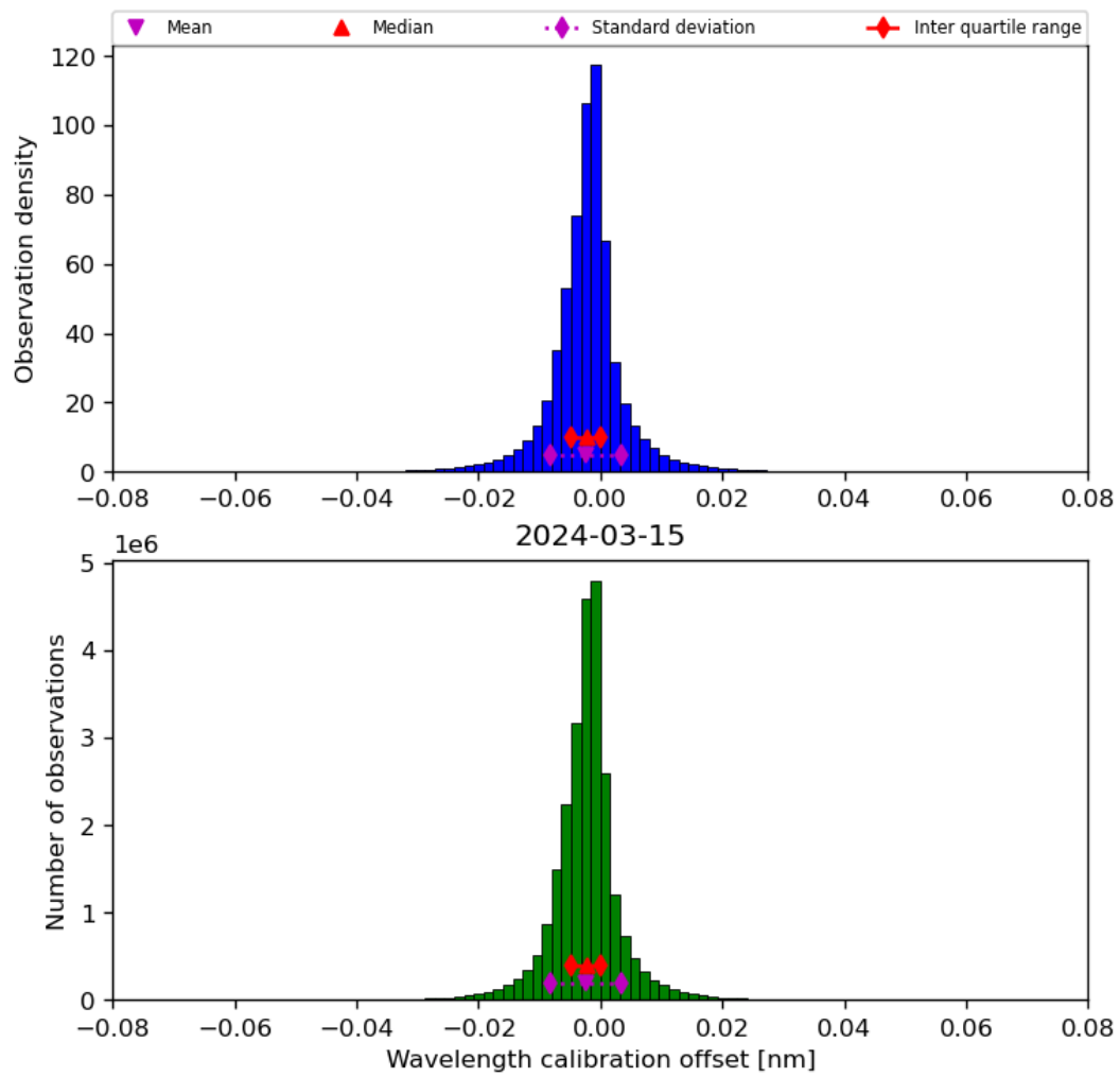
Figure 35: Histogram of “Wavelength calibration offset” for 2024-03-14 to 2024-03-16
