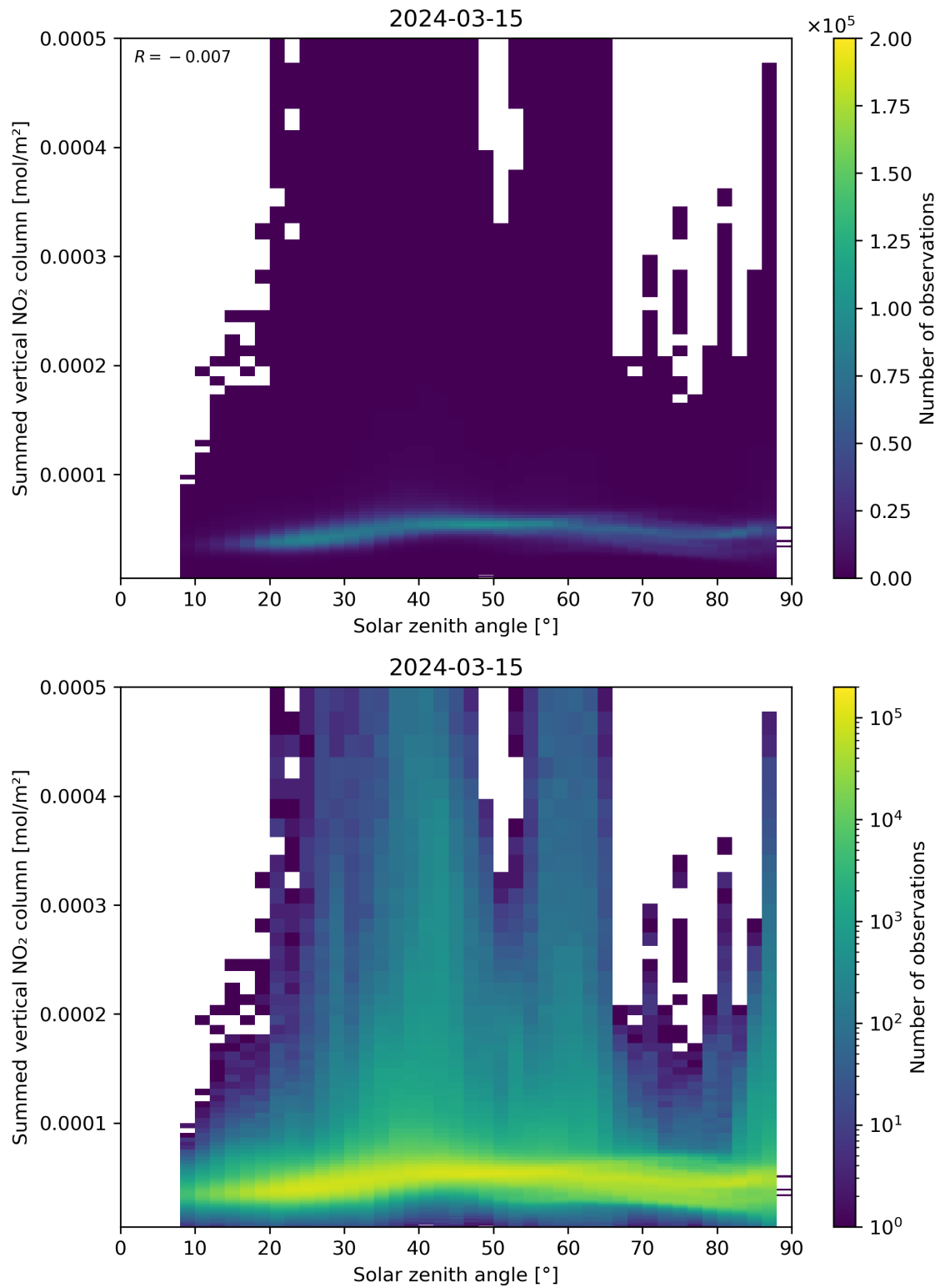
Figure 151: Scatter density plot of “Solar zenith angle” against “Summed vertical NO 2 column” for 2024-03-14 to 2024-03-16.
