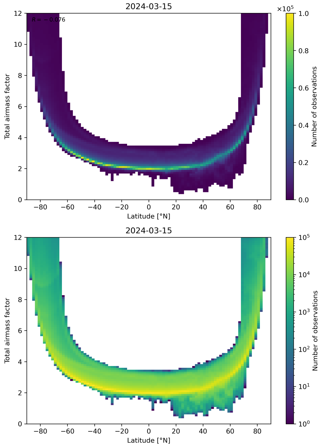
Figure 84: Scatter density plot of “Latitude” against “Total airmass factor” for 2024-03-14 to 2024-03-16.
