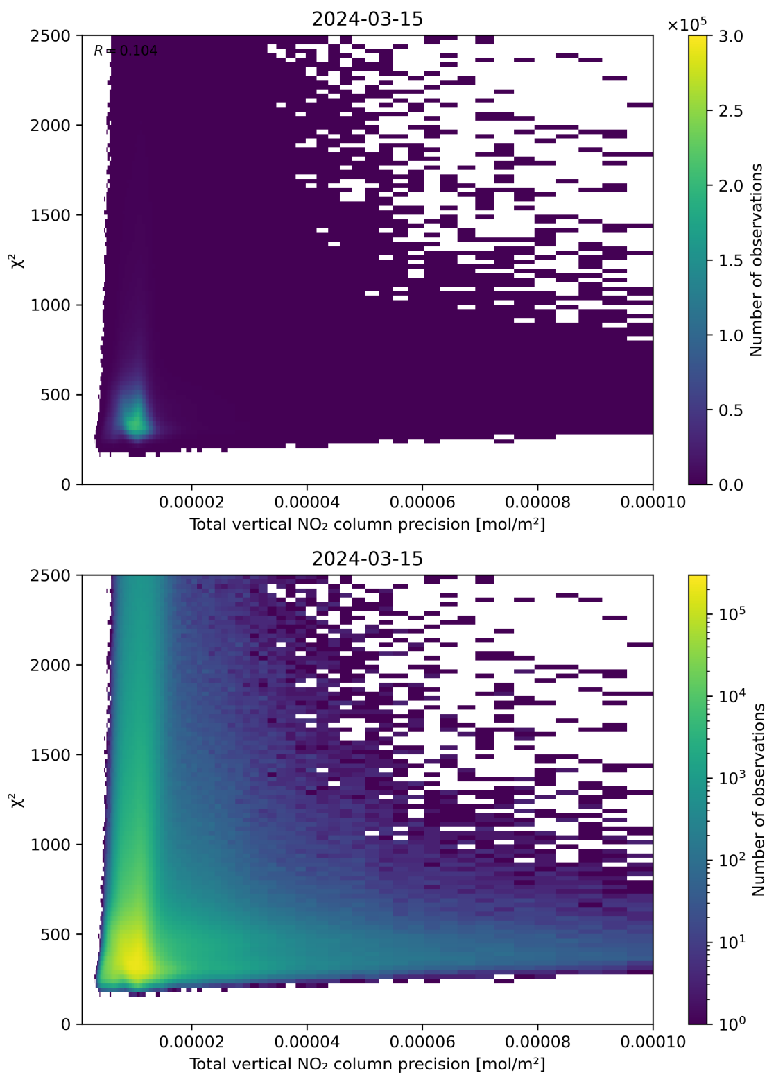
Figure 116: Scatter density plot of “Total vertical NO 2 column precision” against “ \chi^2 ” for 2024-03-14 to 2024-03-16.
