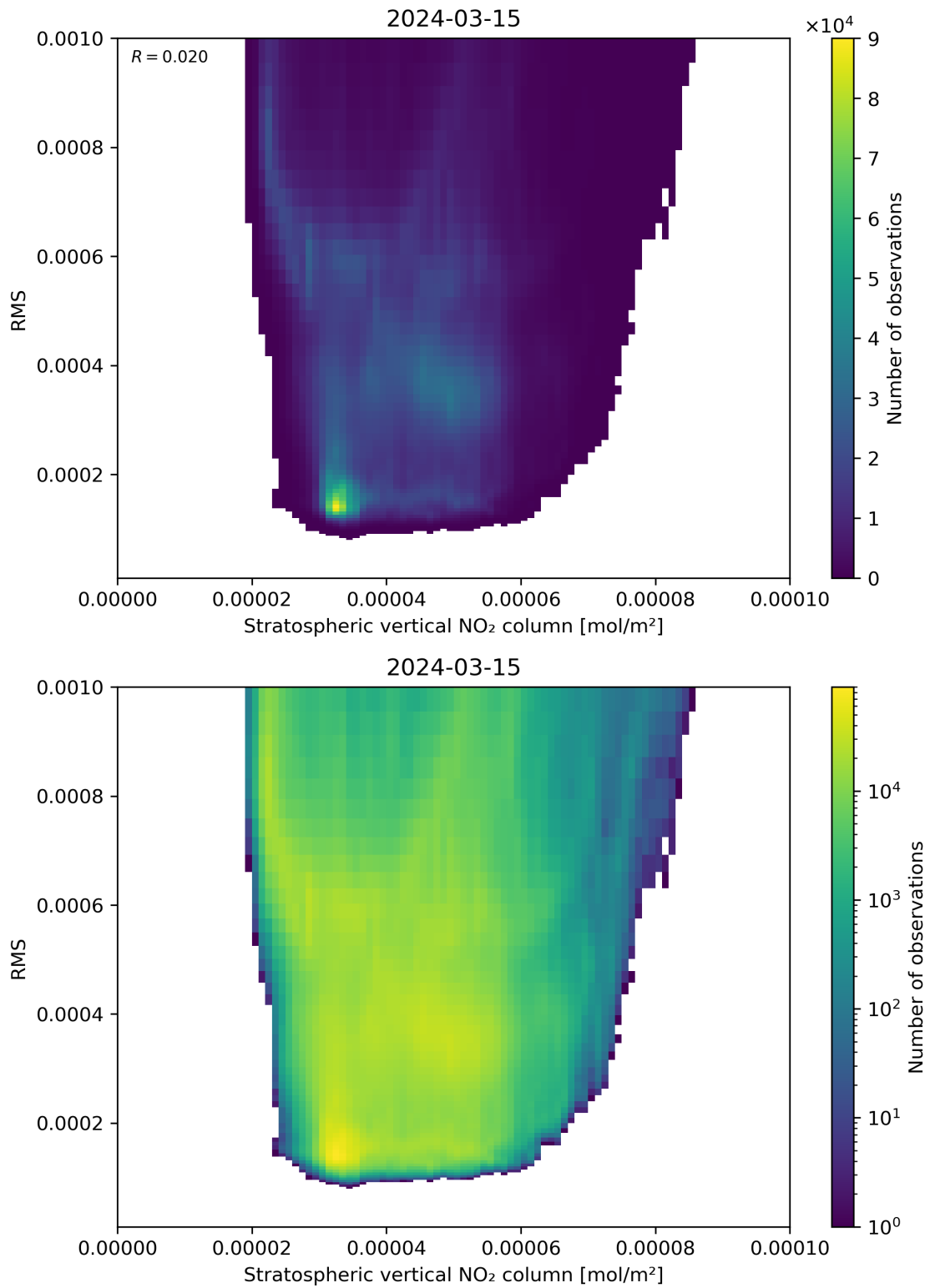
Figure 102: Scatter density plot of “Stratospheric vertical NO 2 column” against “RMS” for 2024-03-14 to 2024-03-16.
