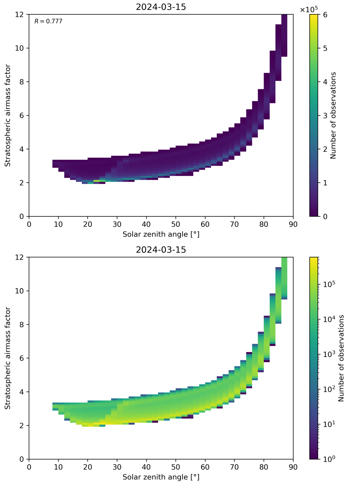
Figure 145: Scatter density plot of “Solar zenith angle” against “Stratospheric airmass factor” for 2024-03-14 to 2024-03-16.
