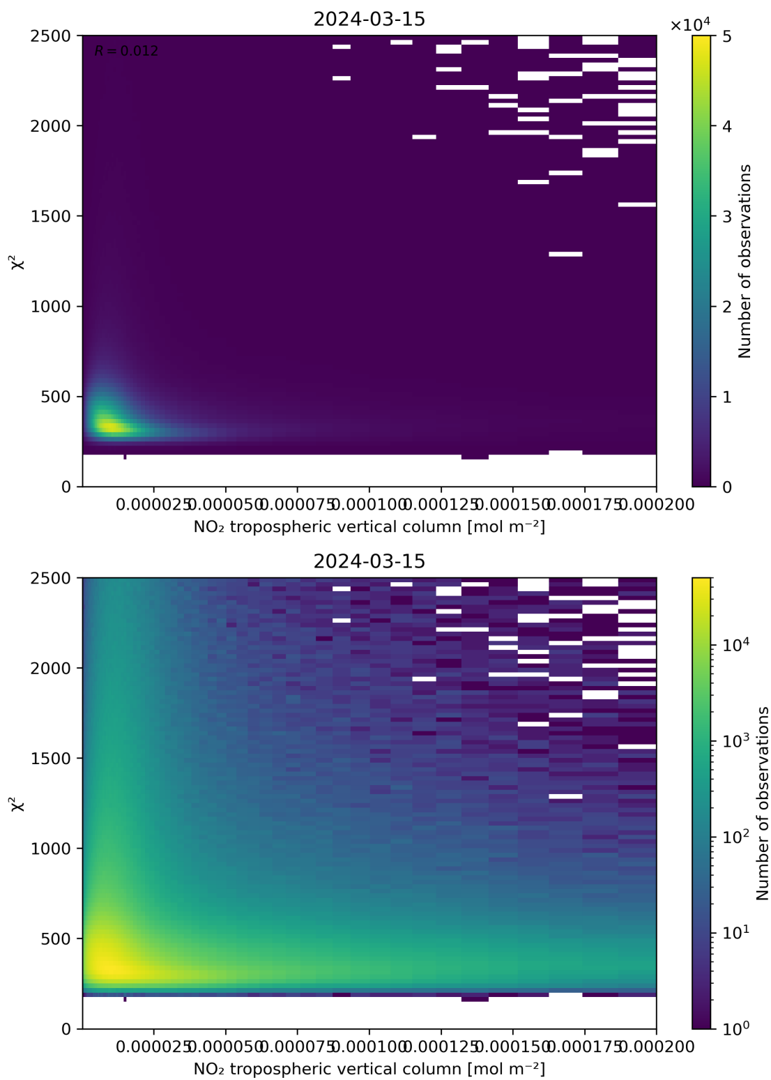
Figure 124: Scatter density plot of “NO 2 tropospheric vertical column” against “ \chi^2 ” for 2024-03-14 to 2024-03-16.
