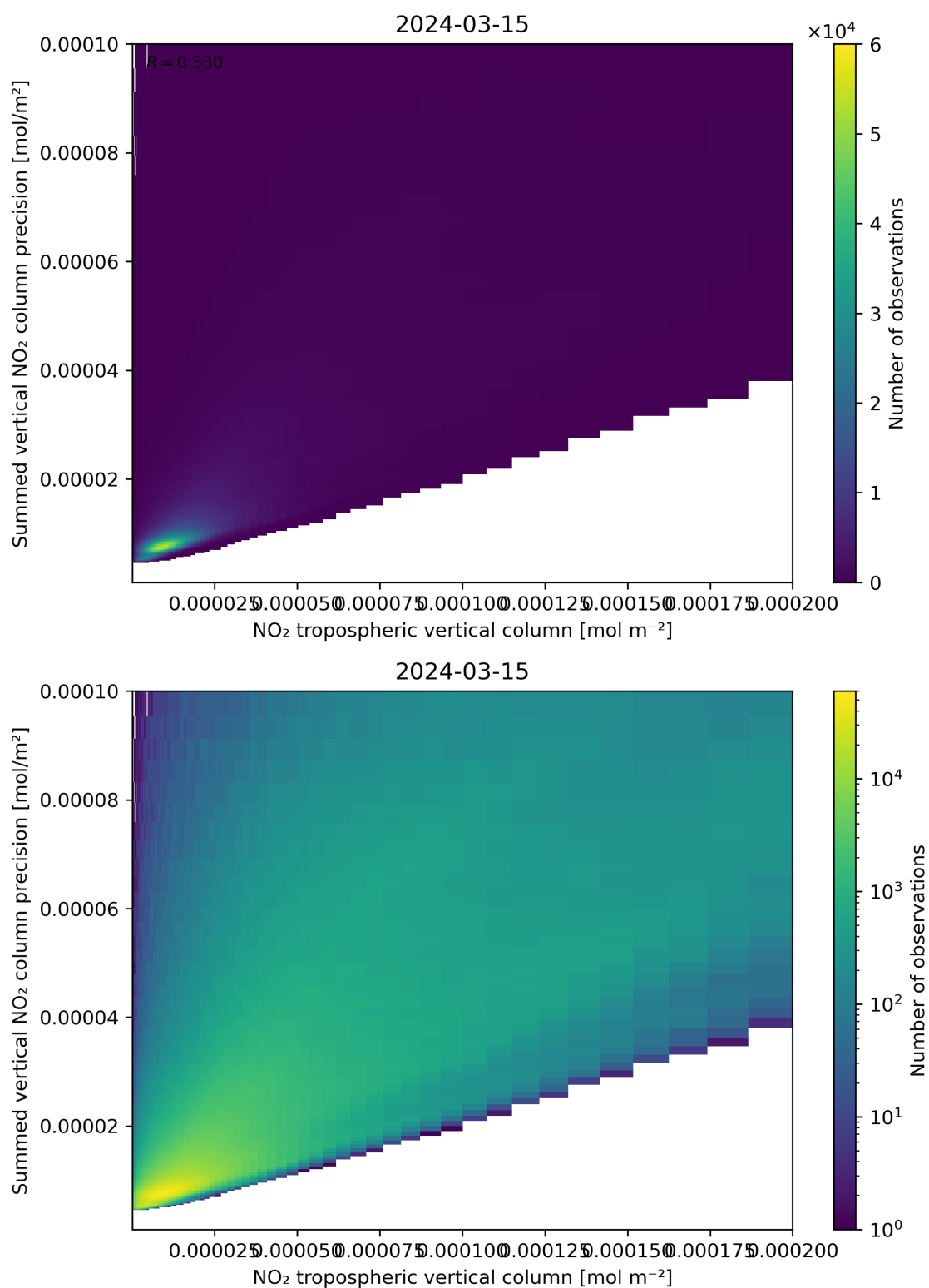
Figure 127: Scatter density plot of “NO 2 tropospheric vertical column” against “Summed vertical NO 2 column precision” for 2024-03-14 to 2024-03-16.
