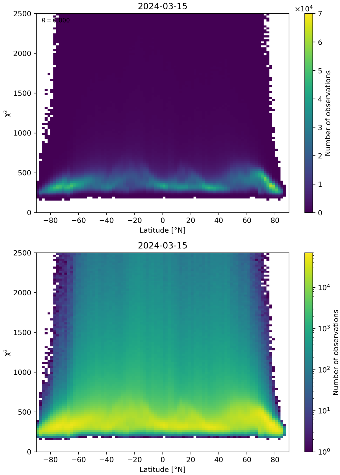
Figure 86: Scatter density plot of “Latitude” against “ \chi^2 ” for 2024-03-14 to 2024-03-16.
