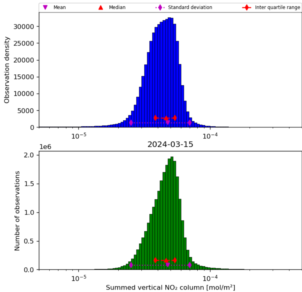
Figure 40: Histogram of “Summed vertical NO 2 column” for 2024-03-14 to 2024-03-16
