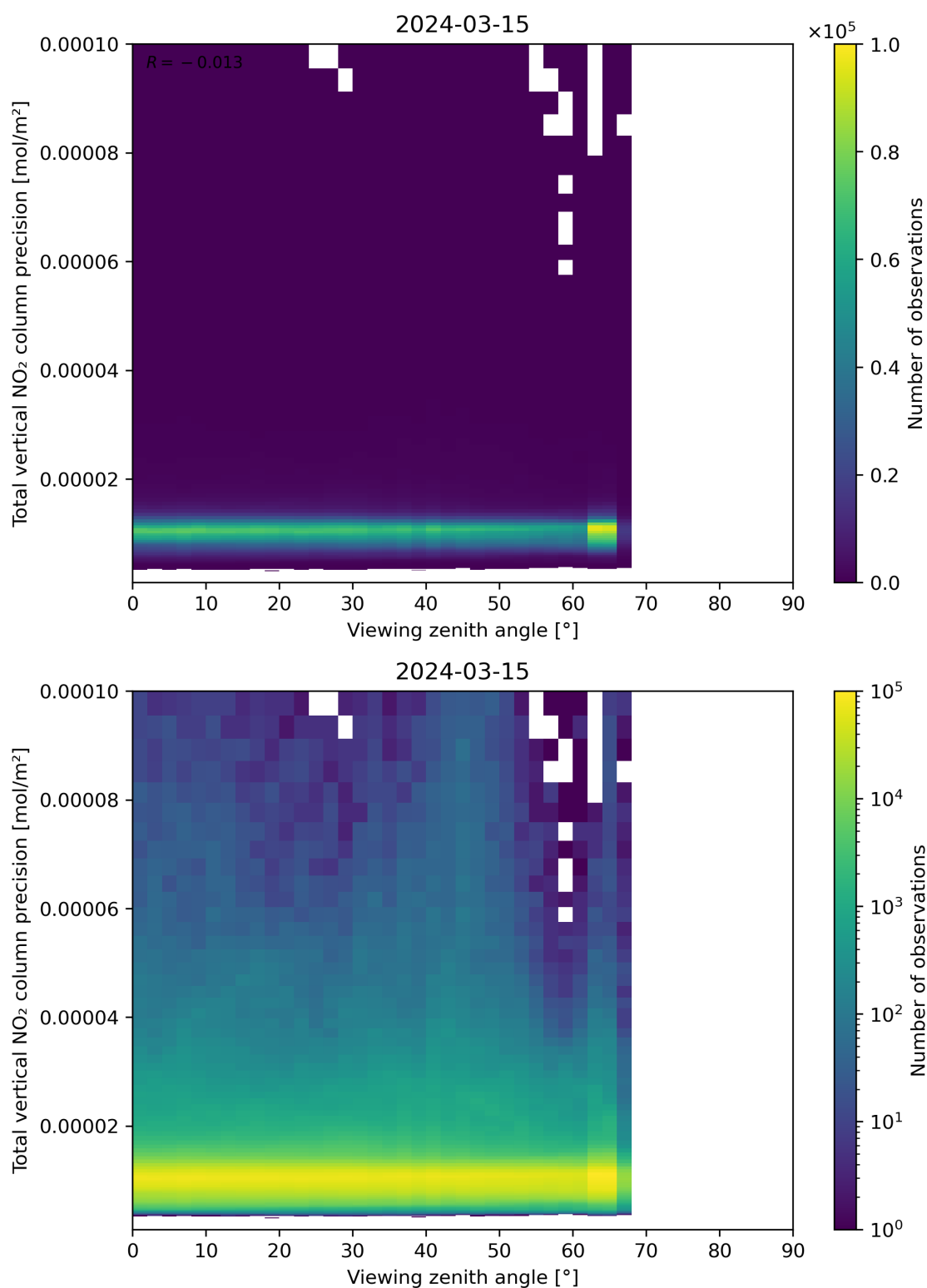
Figure 168: Scatter density plot of “Viewing zenith angle” against “Total vertical NO 2 column precision” for 2024-03-14 to 2024-03-16.
