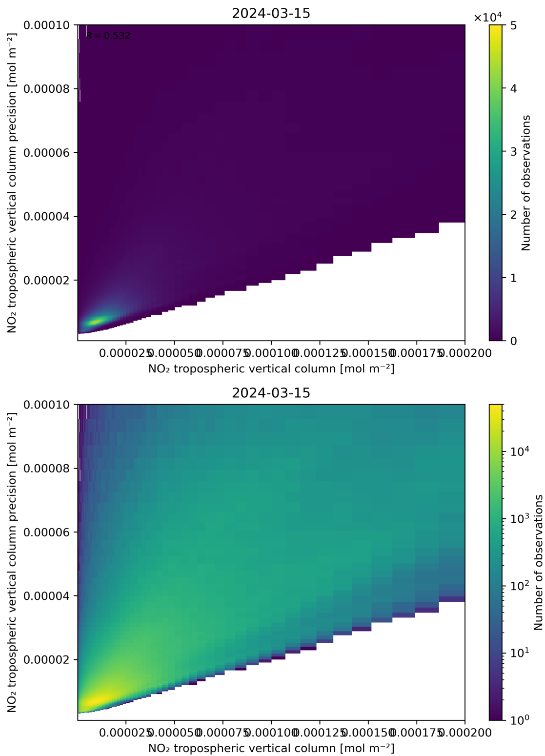
Figure 130: Scatter density plot of “NO 2 tropospheric vertical column” against “NO 2 tropospheric vertical column precision” for 2024-03-14 to 2024-03-16.
