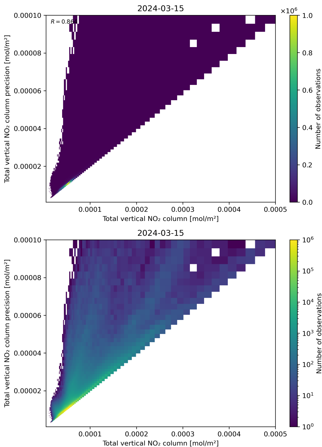
Figure 114: Scatter density plot of “Total vertical NO 2 column” against “Total vertical NO 2 column precision” for 2024-03-14 to 2024-03-16.
