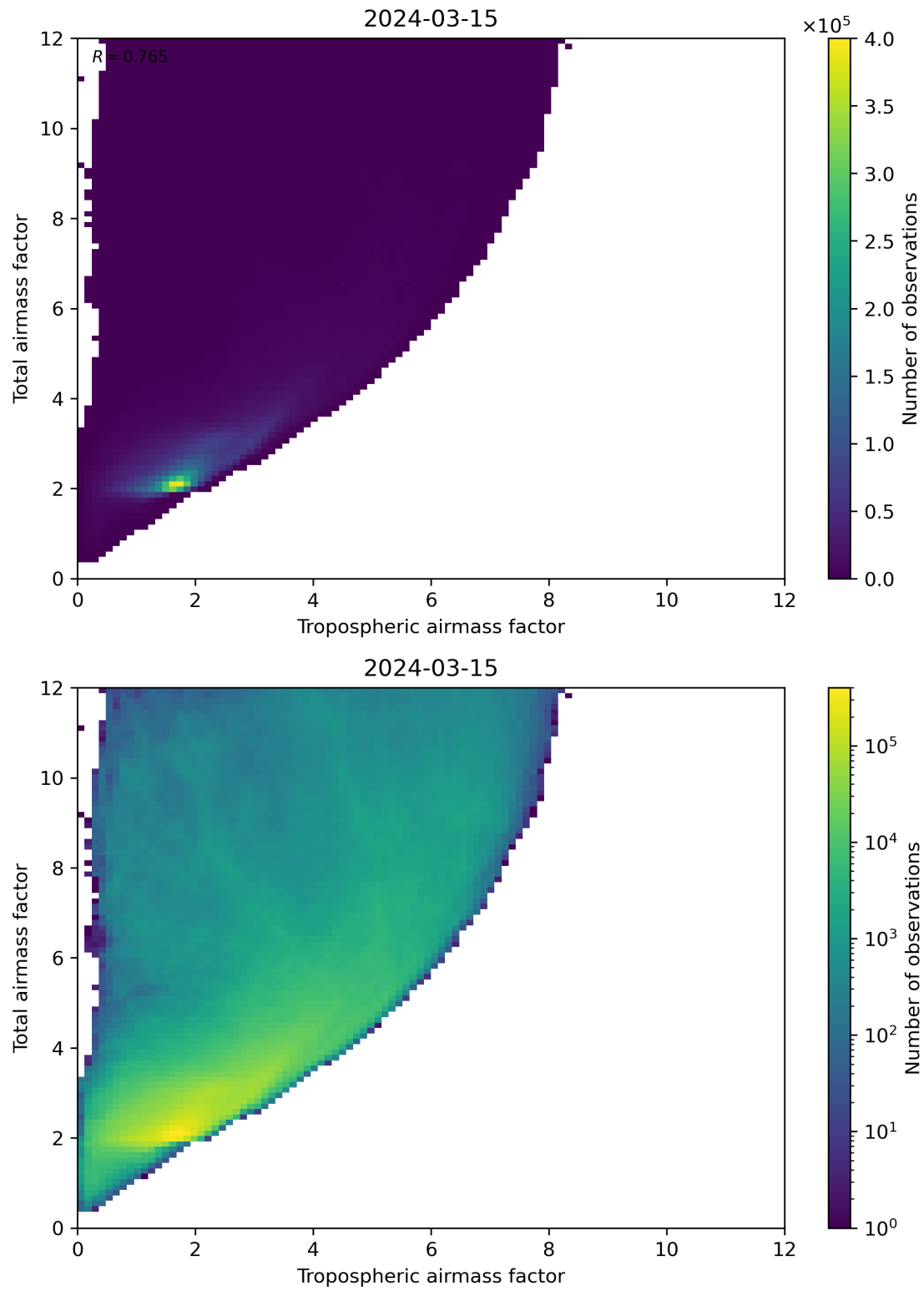
Figure 72: Scatter density plot of “Tropospheric airmass factor” against “Total airmass factor” for 2024-03-14 to 2024-03-16.
