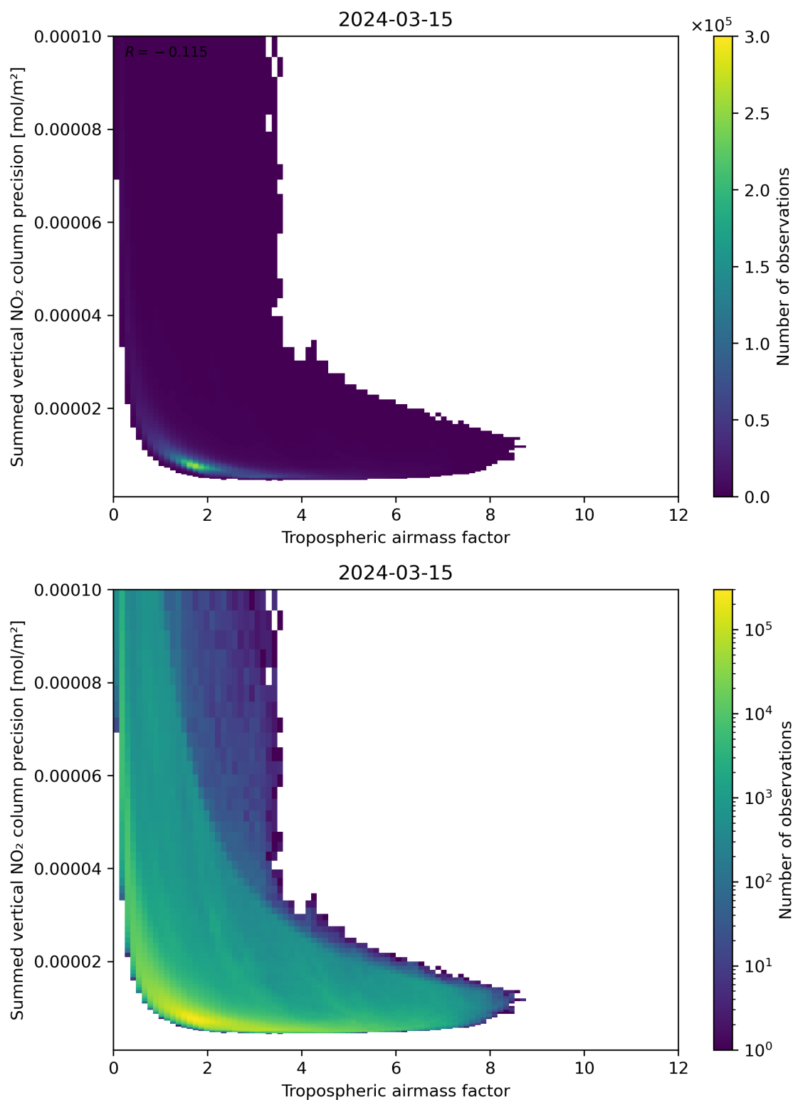
Figure 76: Scatter density plot of “Tropospheric air mass factor” against “Summed vertical NO 2 column precision” for 2024-03-14 to 2024-03-16.
