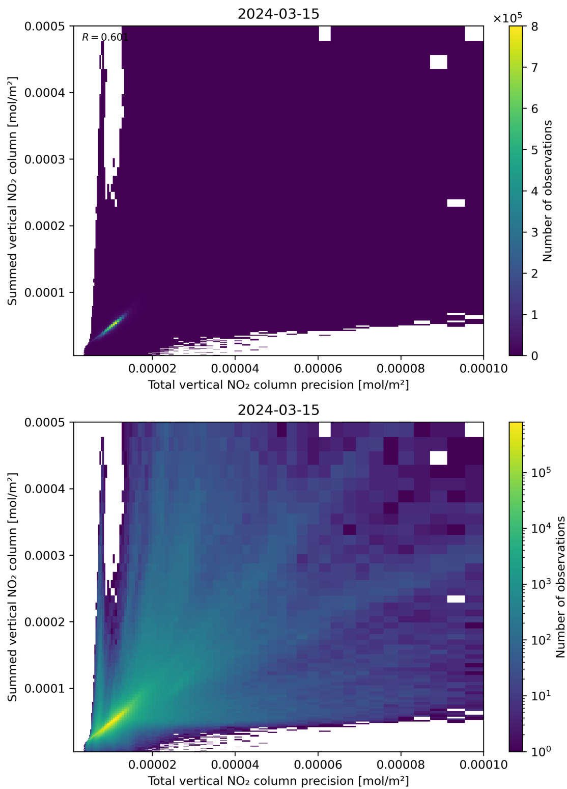
Figure 117: Scatter density plot of “Total vertical NO 2 column precision” against “Summed vertical NO 2 column” for 2024-03-14 to 2024-03-16.
