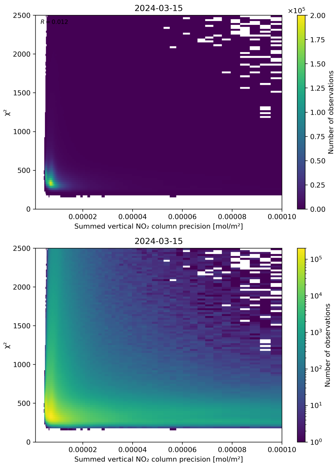
Figure 107: Scatter density plot of “Summed vertical NO 2 column precision” against “ \chi^2 ” for 2024-03-14 to 2024-03-16.
