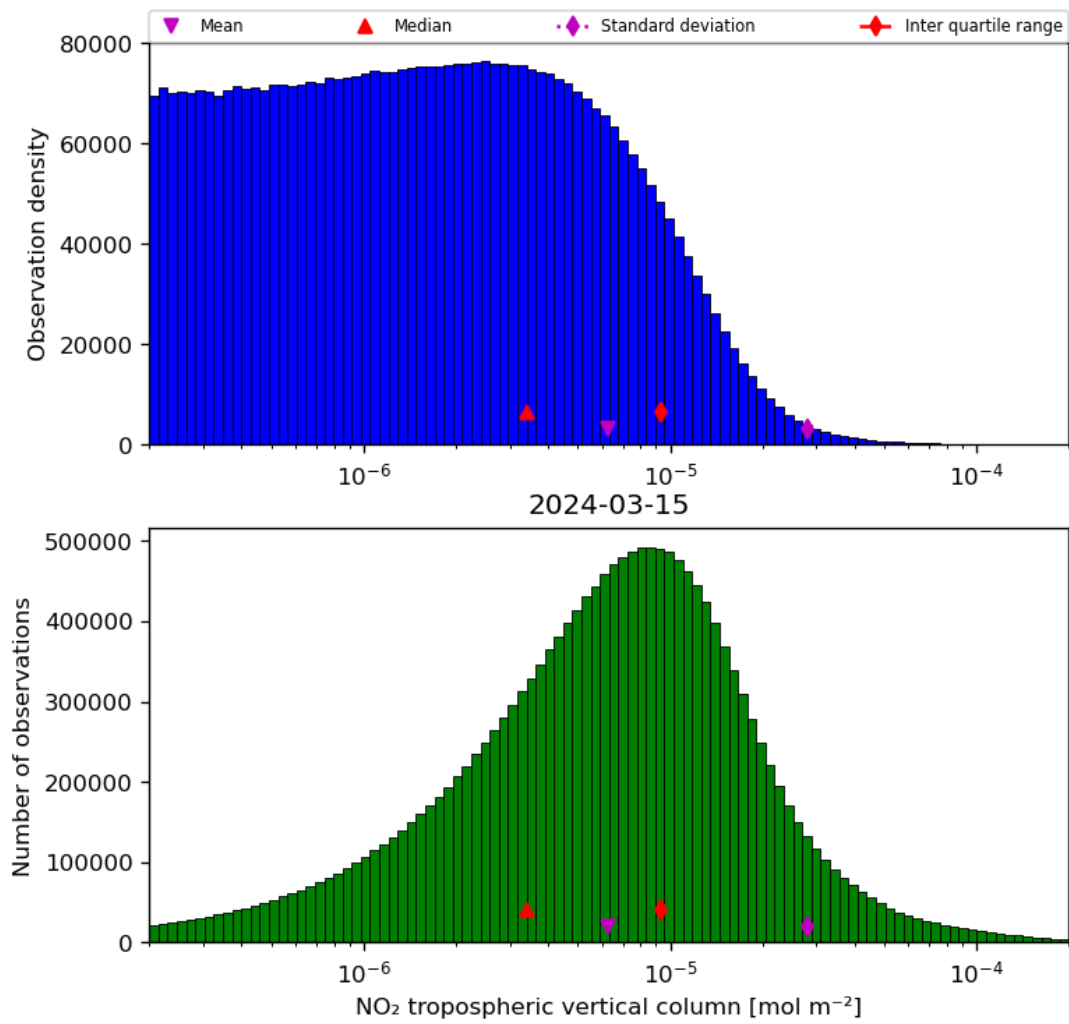
Figure 29: Histogram of “NO 2 tropospheric vertical column” for 2024-03-14 to 2024-03-16
