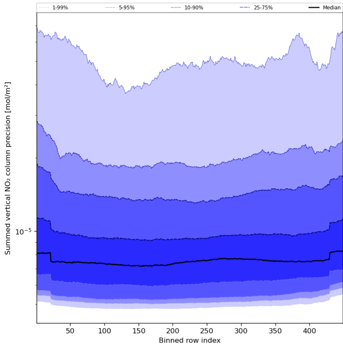
Figure 58: Along track statistics of “Summed vertical NO 2 column precision” for 2024-03-14 to 2024-03-16
