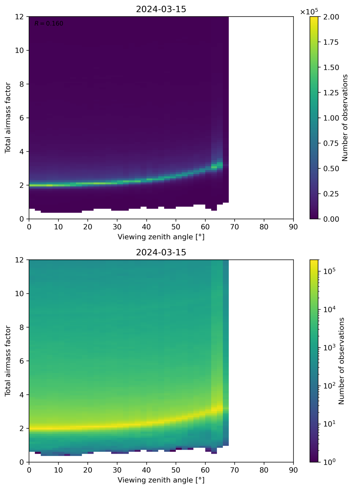
Figure 160: Scatter density plot of “Viewing zenith angle” against “Total airmass factor” for 2024-03-14 to 2024-03-16.
