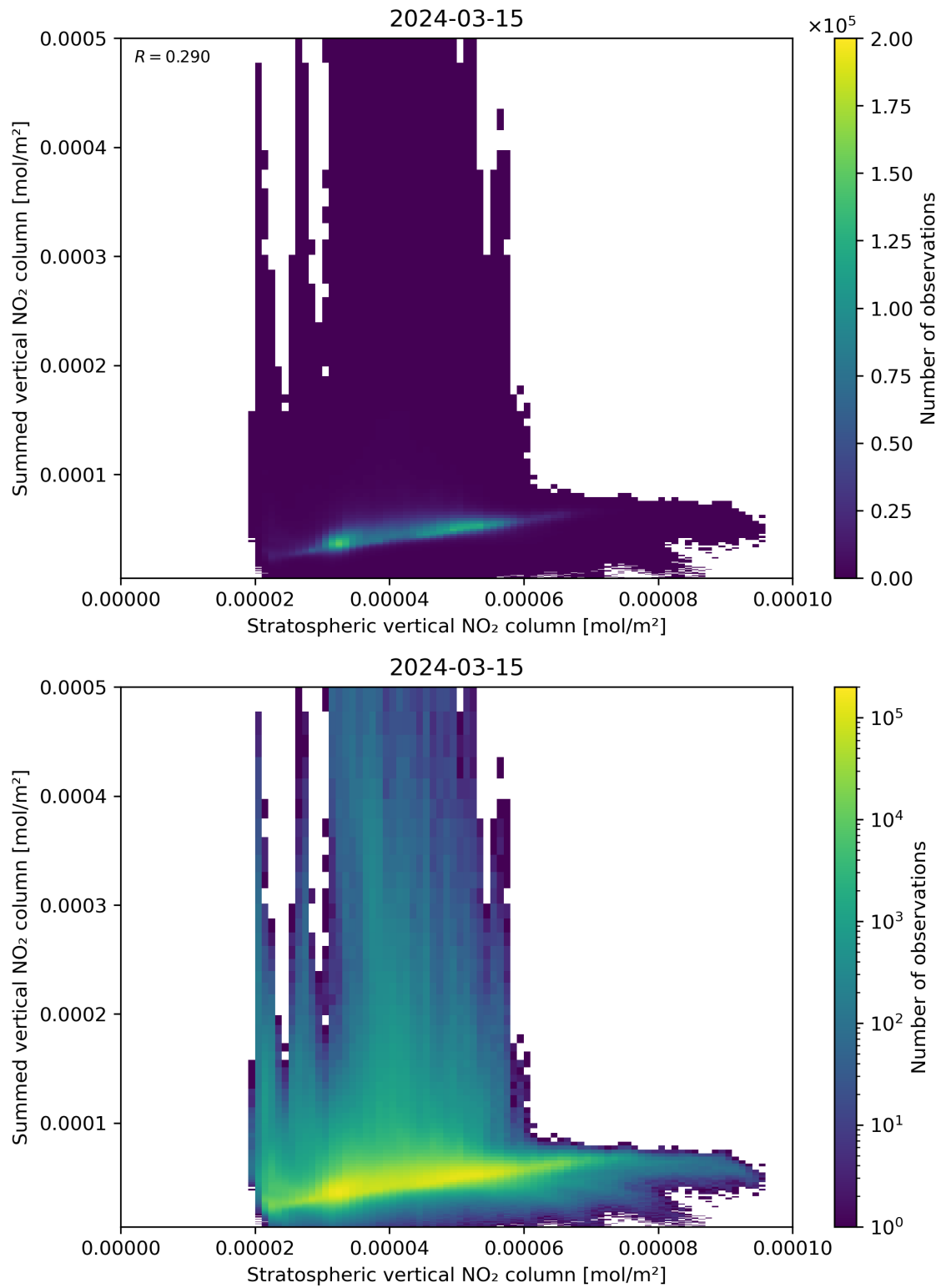
Figure 98: Scatter density plot of “Stratospheric vertical NO 2 column” against “Summed vertical NO 2 column” for 2024-03-14 to 2024-03-16.
