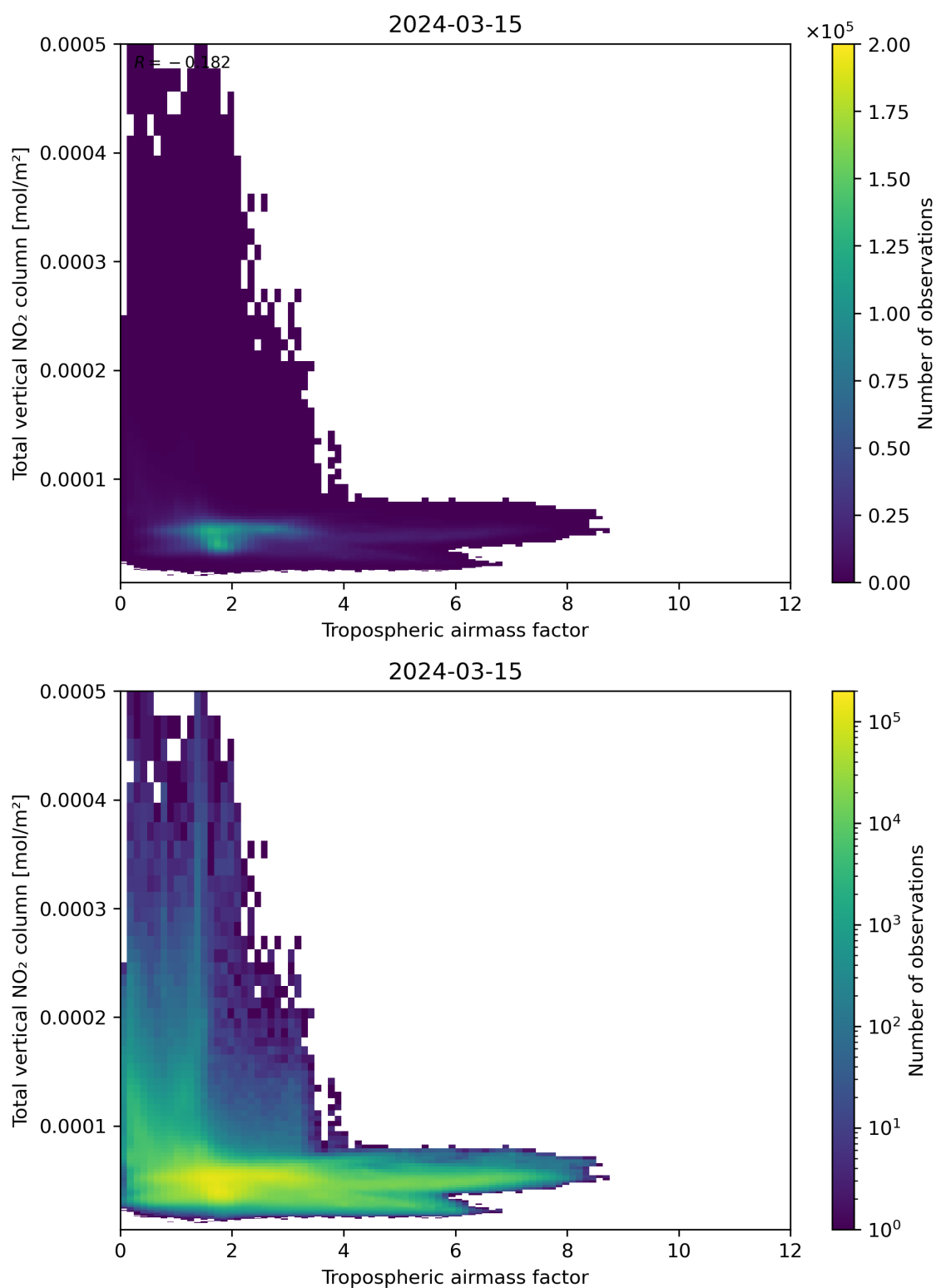
Figure 77: Scatter density plot of “Tropospheric airmass factor” against “Total vertical NO 2 column” for 2024-03-14 to 2024-03-16.
