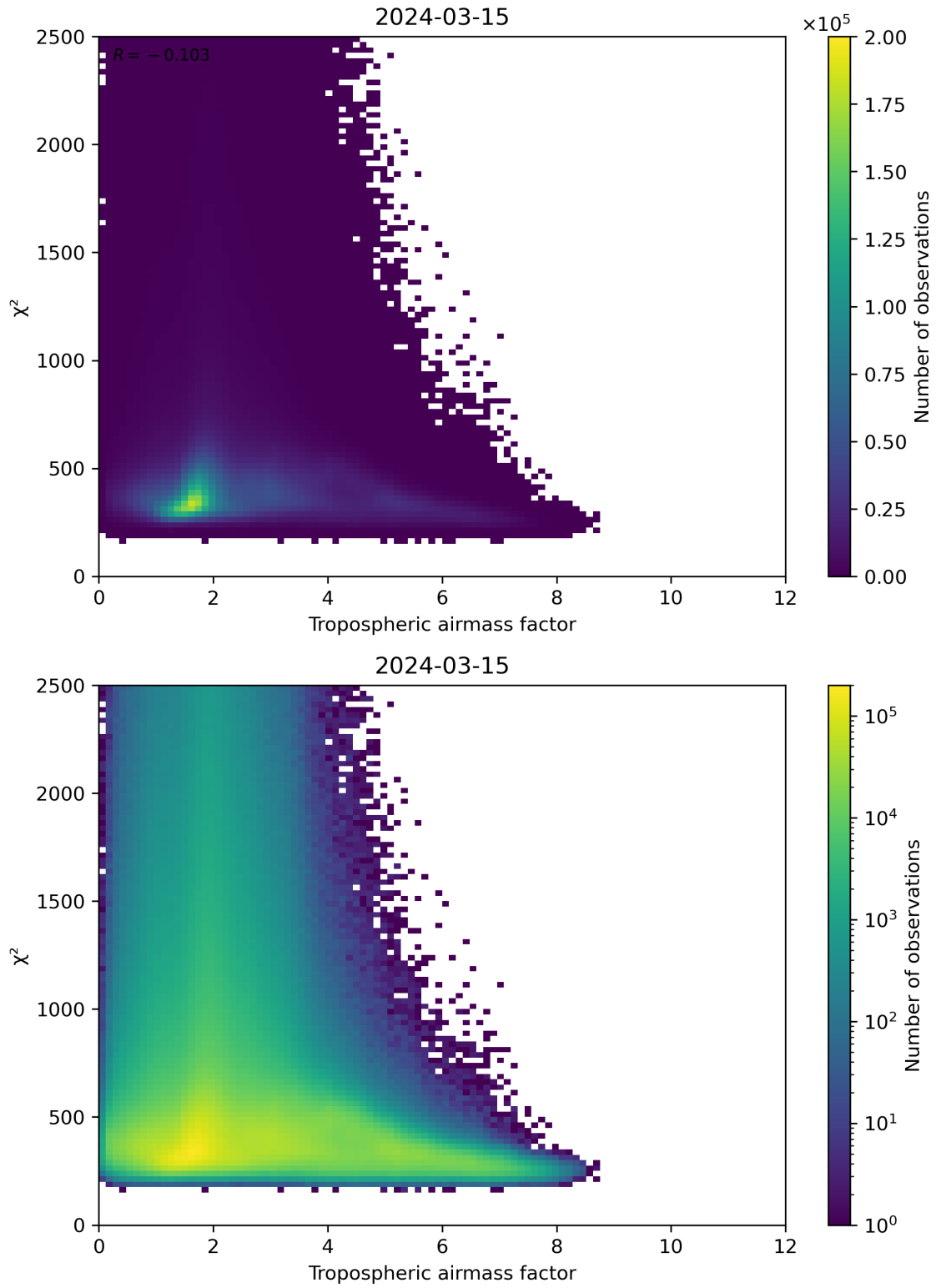
Figure 73: Scatter density plot of “Tropospheric airmass factor” against “ \chi^2 ” for 2024-03-14 to 2024-03-16.
