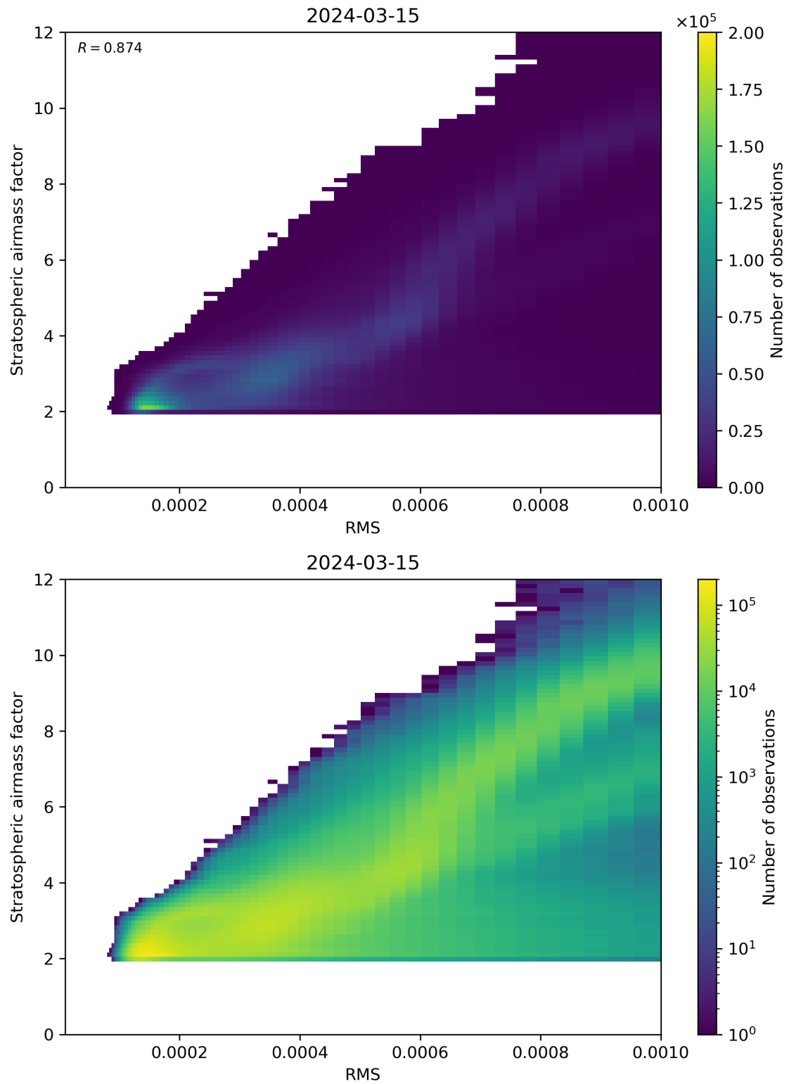
Figure 144: Scatter density plot of “RMS” against “Stratospheric airmass factor” for 2024-03-14 to 2024-03-16.
