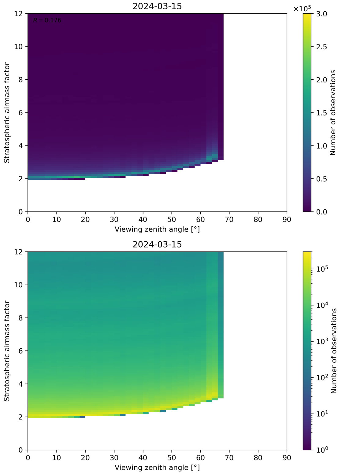
Figure 159: Scatter density plot of “Viewing zenith angle” against “Stratospheric airmass factor” for 2024-03-14 to 2024-03-16.
