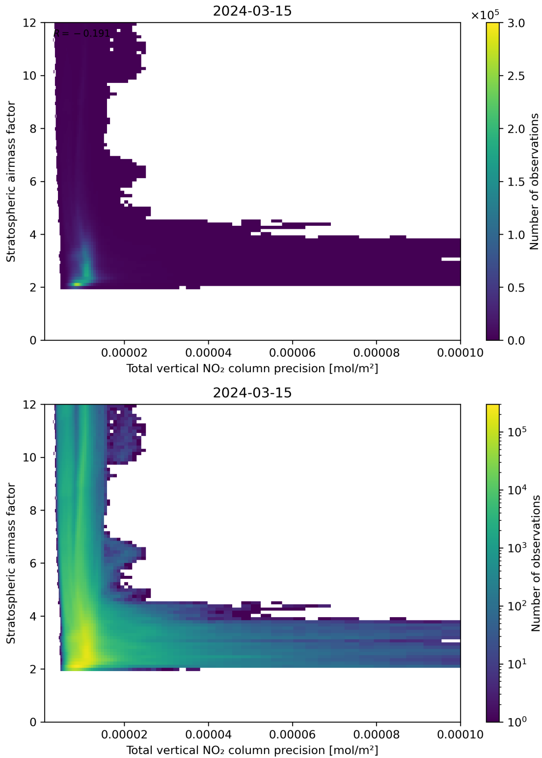
Figure 115: Scatter density plot of “Total vertical NO 2 column precision” against “Stratospheric airmass factor” for 2024-03-14 to 2024-03-16.
