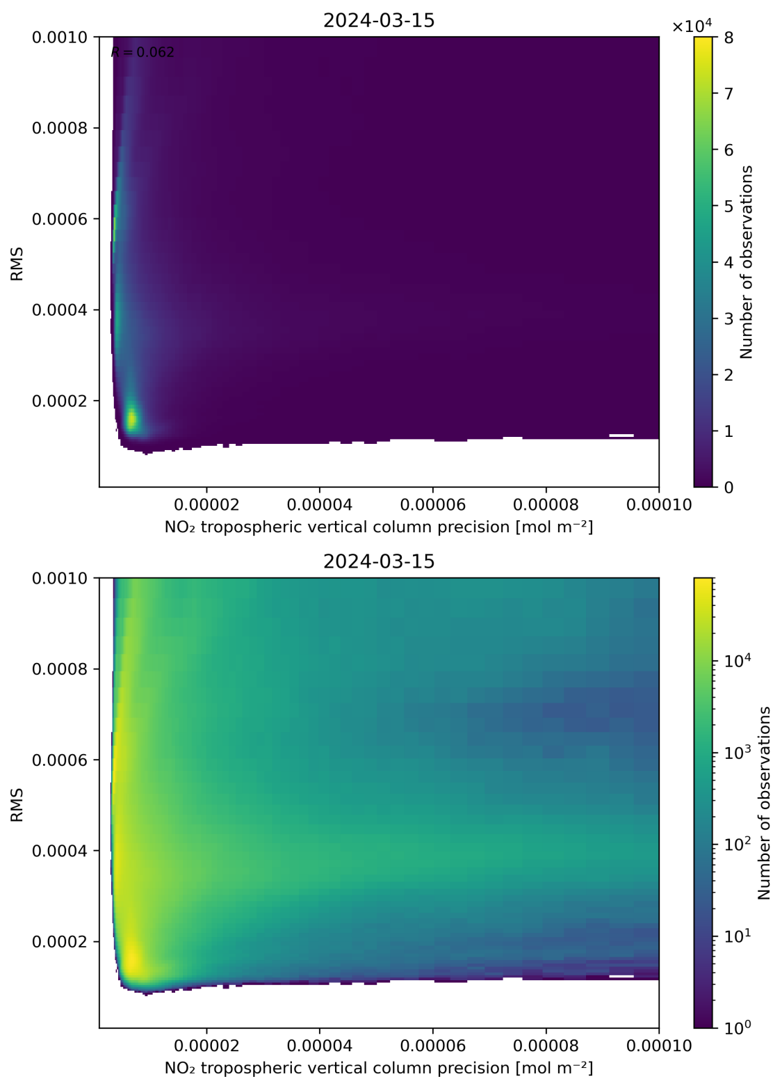
Figure 140: Scatter density plot of “NO 2 tropospheric vertical column precision” against “RMS” for 2024-03-14 to 2024-03-16.
