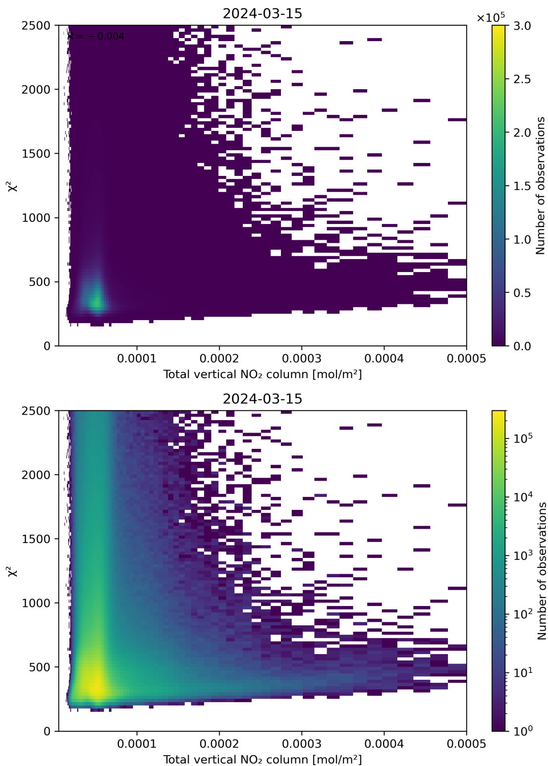
Figure 111: Scatter density plot of “Total vertical NO 2 column” against “ \chi^2 ” for 2024-03-14 to 2024-03-16.
