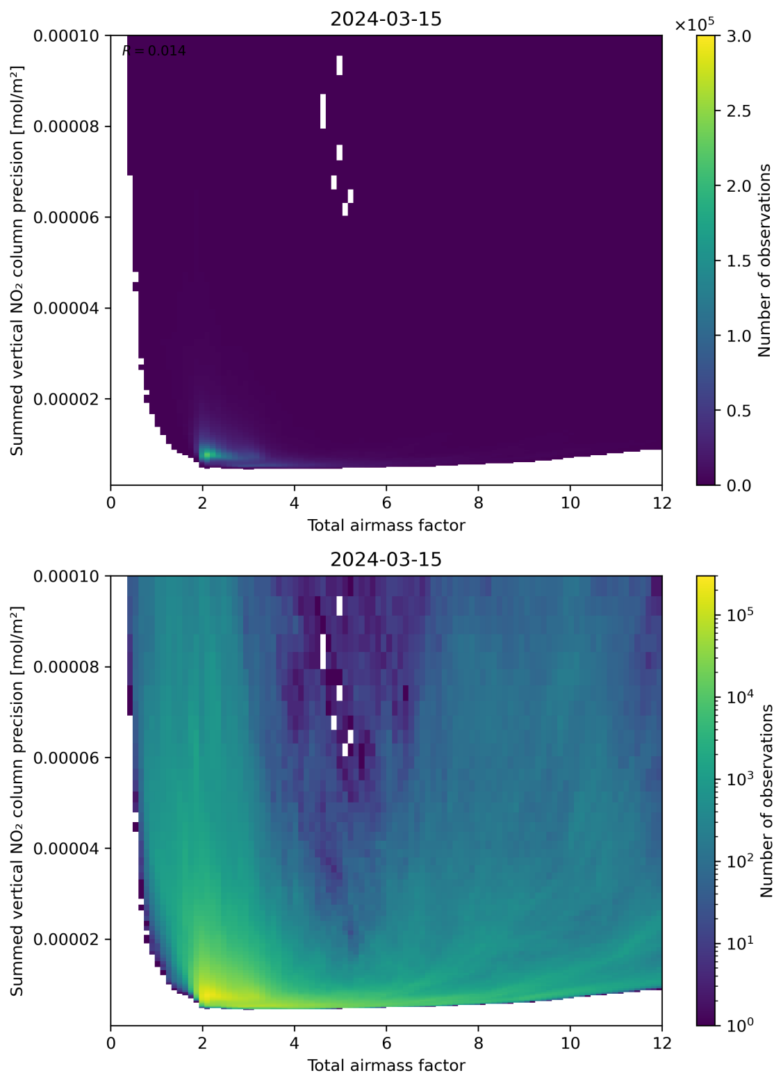
Figure 66: Scatter density plot of “Total airmass factor” against “Summed vertical NO 2 column precision” for 2024-03-14 to 2024-03-16.
