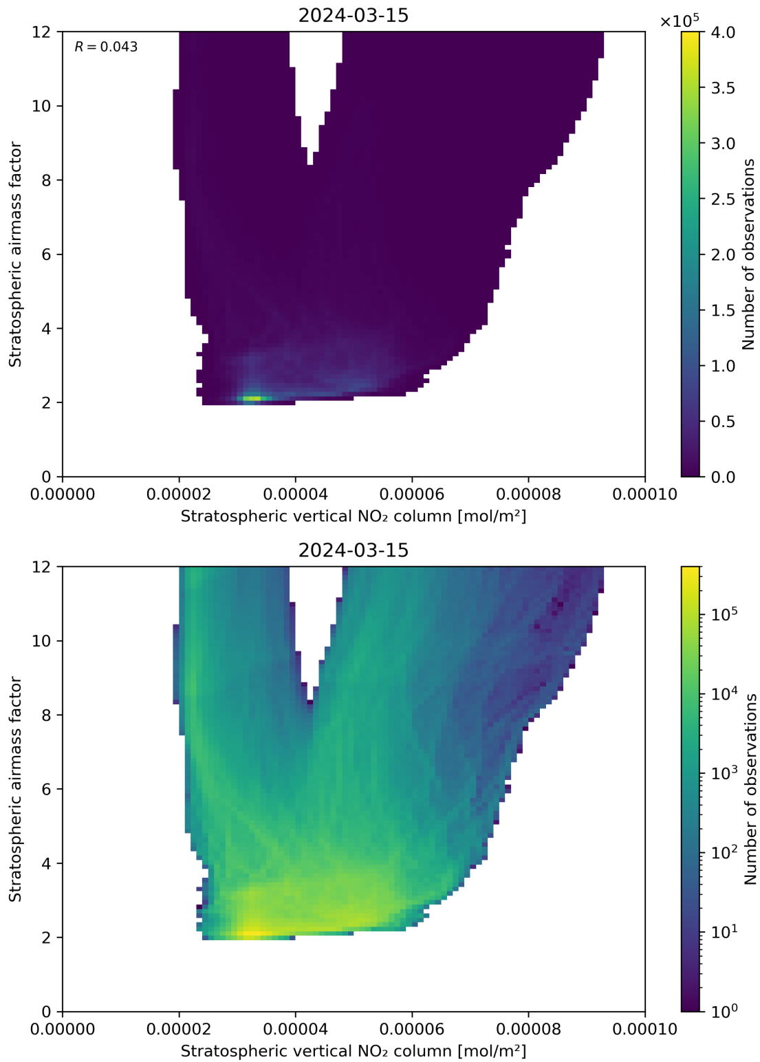
Figure 96: Scatter density plot of “Stratospheric vertical NO 2 column” against “Stratospheric airmass factor” for 2024-03-14 to 2024-03-16.
