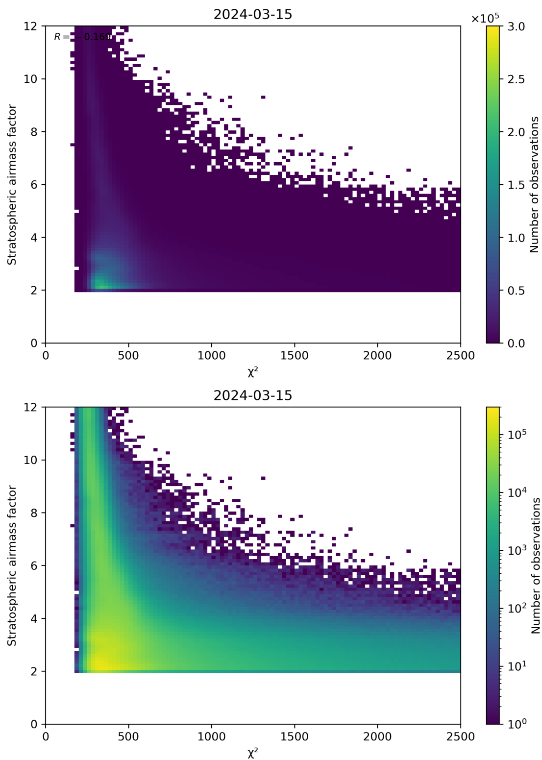
Figure 81: Scatter density plot of “ \chi^2 ” against “Stratospheric airmass factor” for 2024-03-14 to 2024-03-16.
