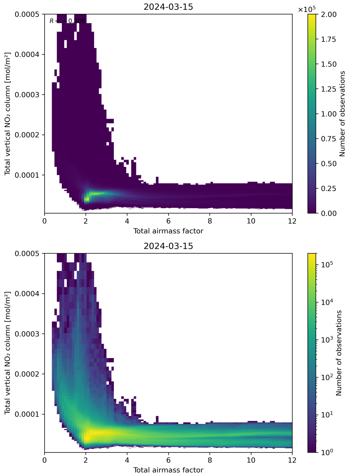
Figure 67: Scatter density plot of “Total airmass factor” against “Total vertical NO 2 column” for 2024-03-14 to 2024-03-16.
