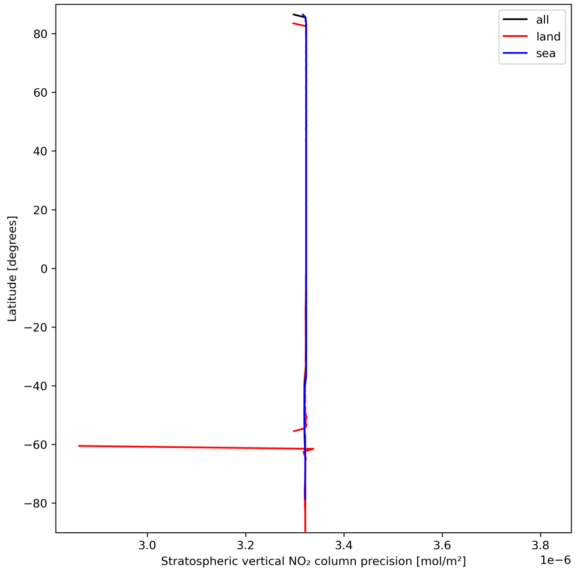
Figure 20: Zonal average of “Stratospheric vertical NO 2 column precision” for 2024-03-14 to 2024-03-16.
