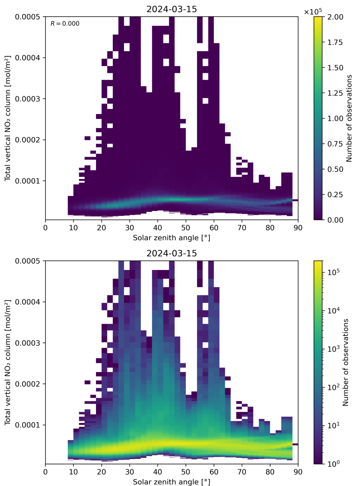
Figure 153: Scatter density plot of “Solar zenith angle” against “Total vertical NO 2 column” for 2024-03-14 to 2024-03-16.
