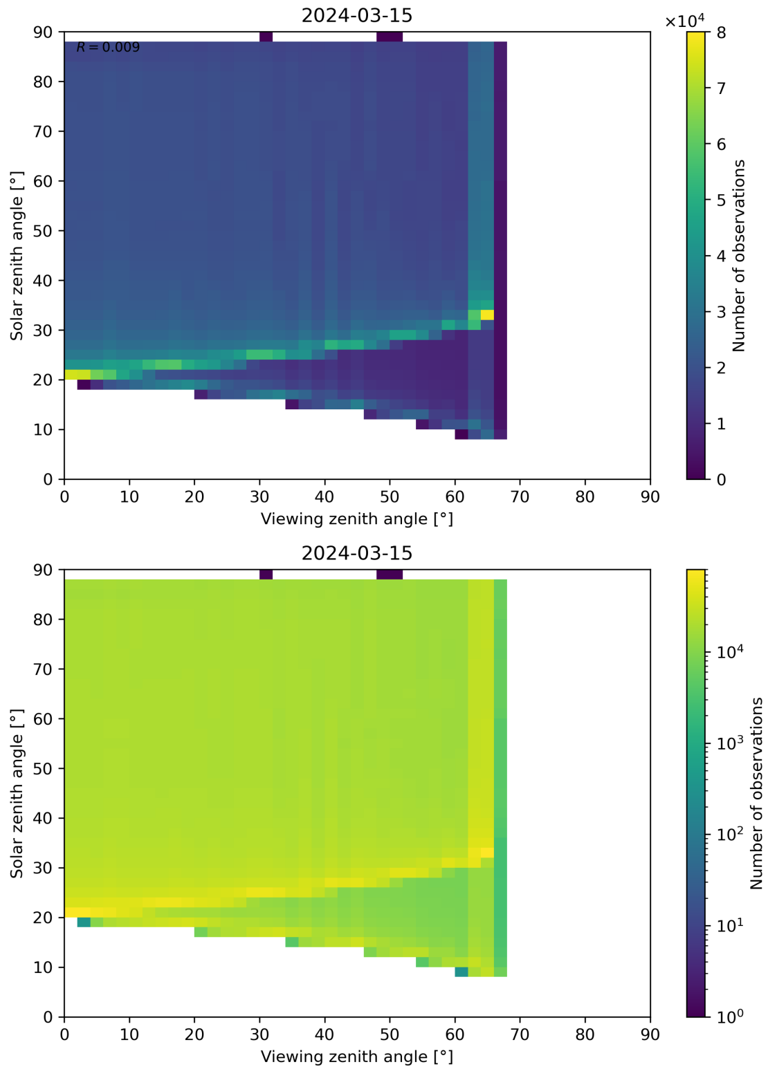
Figure 172: Scatter density plot of “Viewing zenith angle” against “Solar zenith angle” for 2024-03-14 to 2024-03-16.
