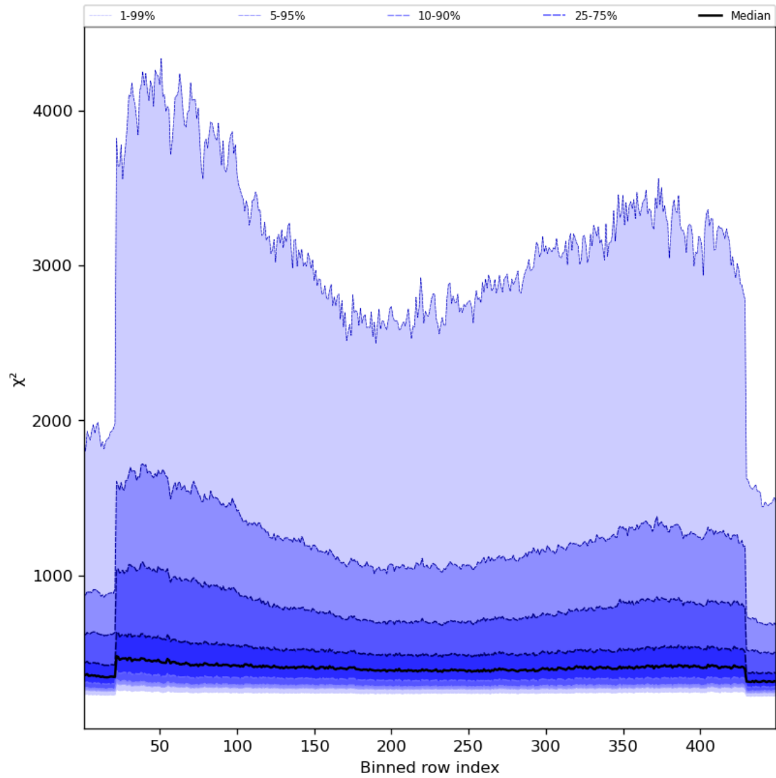
Figure 59: Along track statistics of “ \chi^2 ” for 2024-03-14 to 2024-03-16
