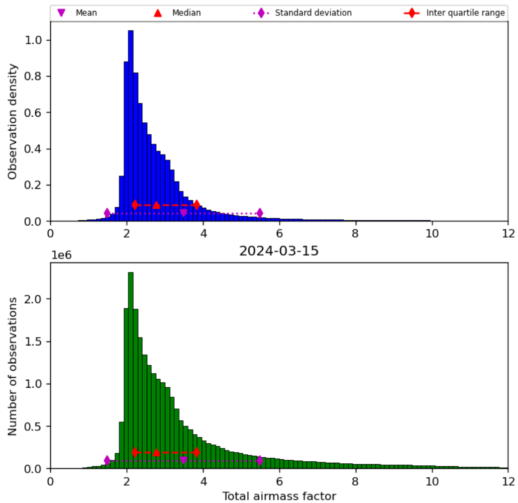
Figure 32: Histogram of “Total airmass factor” for 2024-03-14 to 2024-03-16
