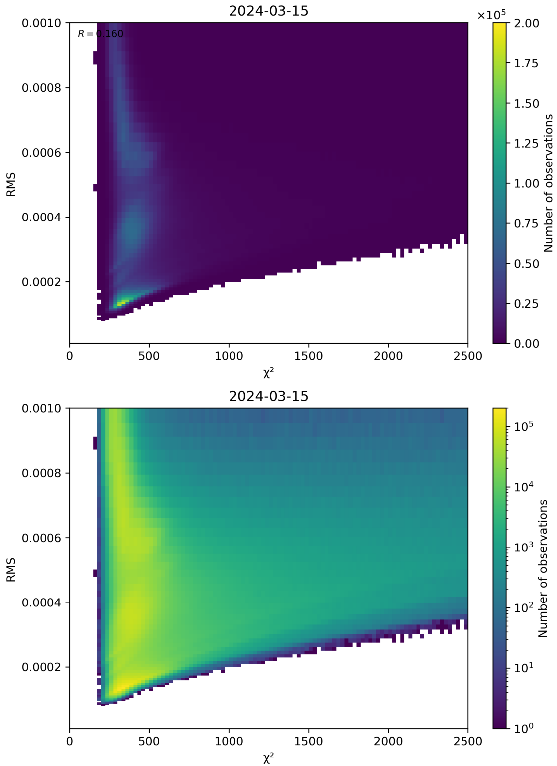
Figure 82: Scatter density plot of “ \chi^2 ” against “RMS” for 2024-03-14 to 2024-03-16.
