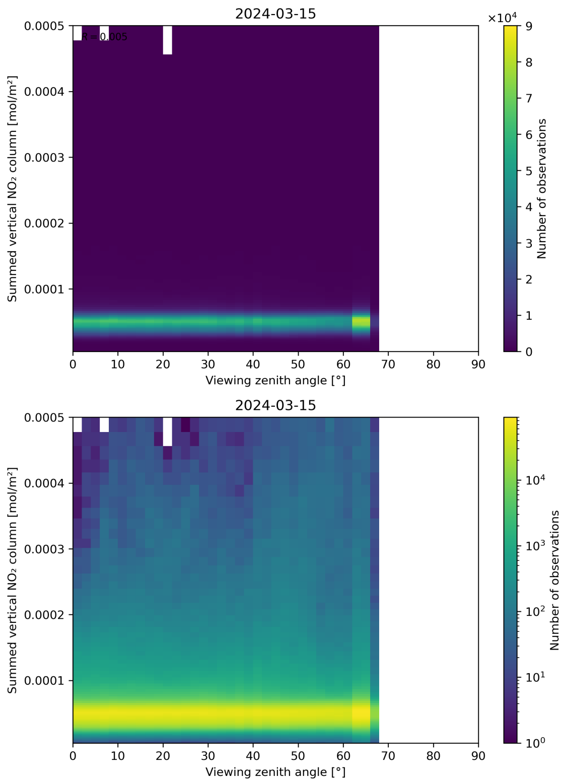
Figure 165: Scatter density plot of “Viewing zenith angle” against “Summed vertical NO 2 column” for 2024-03-14 to 2024-03-16.
