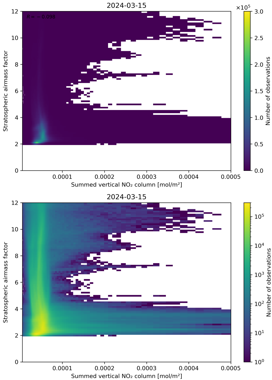
Figure 103: Scatter density plot of “Summed vertical NO 2 column” against “Stratospheric airmass factor” for 2024-03-14 to 2024-03-16.
