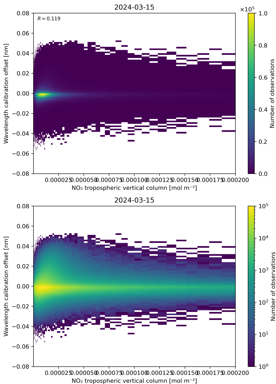
Figure 143: Scatter density plot of “NO 2 tropospheric vertical column” against “Wavelength calibration offset” for 2024-03-14 to 2024-03-16.
