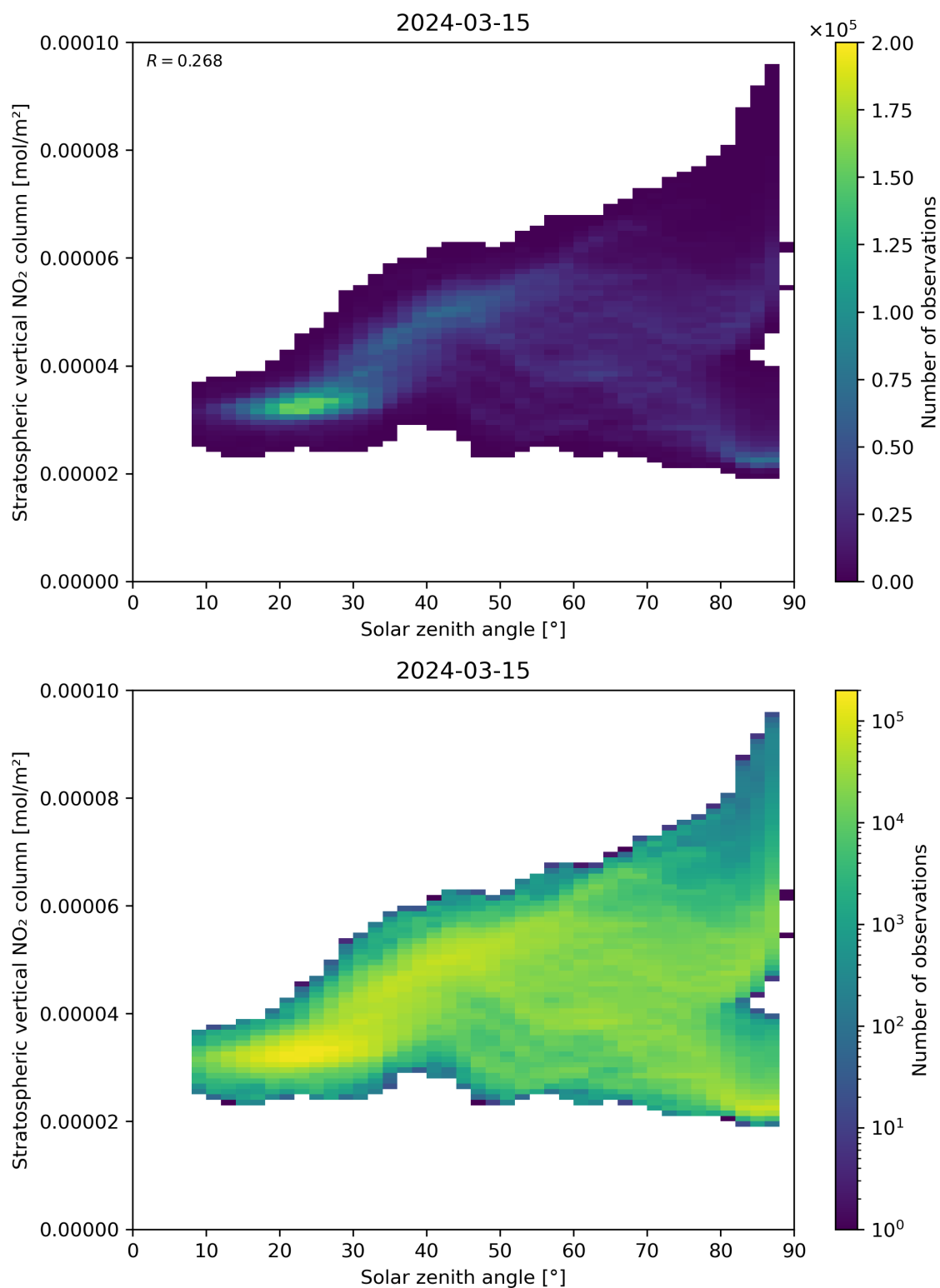
Figure 150: Scatter density plot of “Solar zenith angle” against “Stratospheric vertical \text{NO}_2 column” for 2024-03-14 to 2024-03-16.
