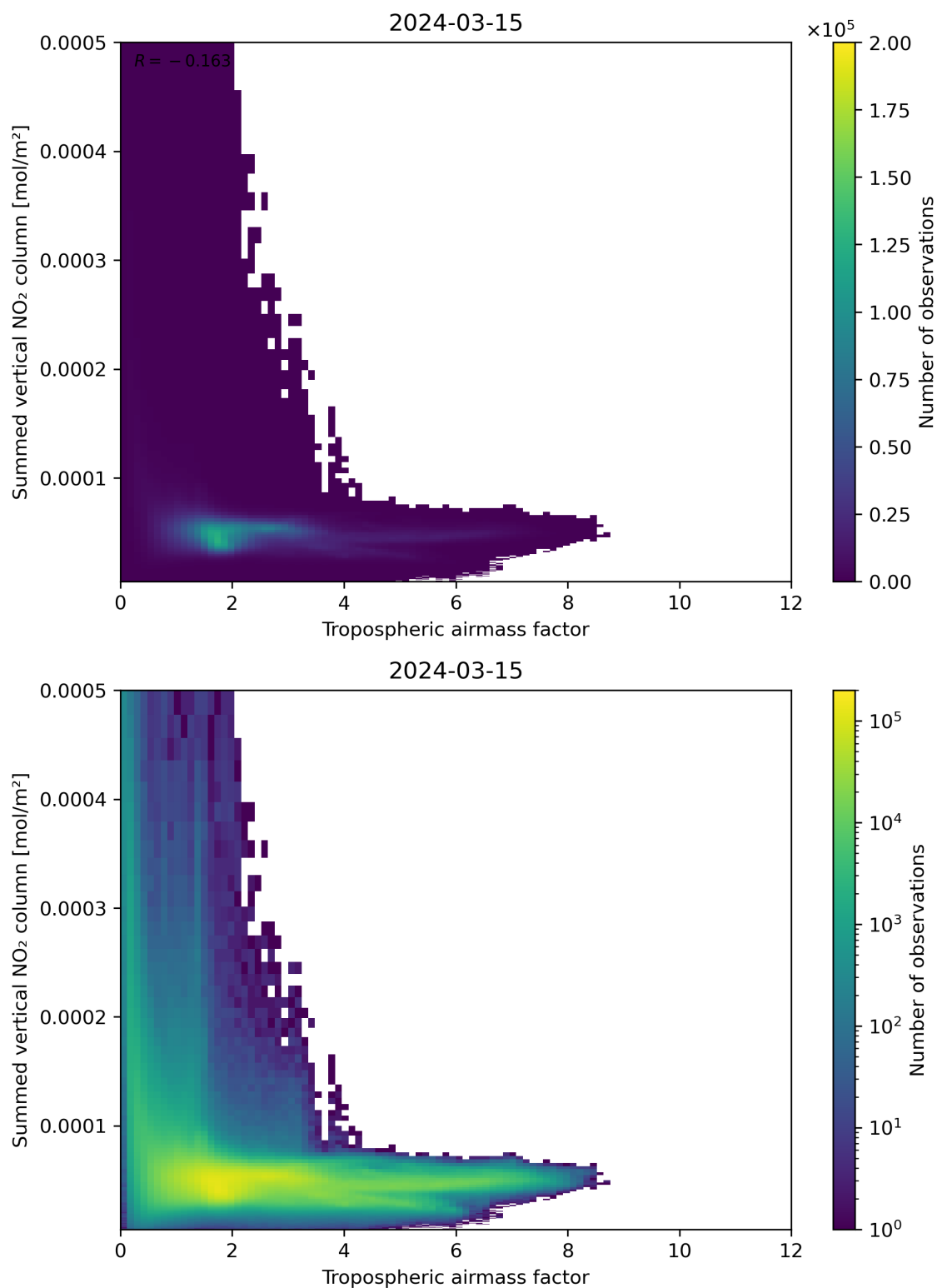
Figure 75: Scatter density plot of “Tropospheric airmass factor” against “Summed vertical NO 2 column” for 2024-03-14 to 2024-03-16.
