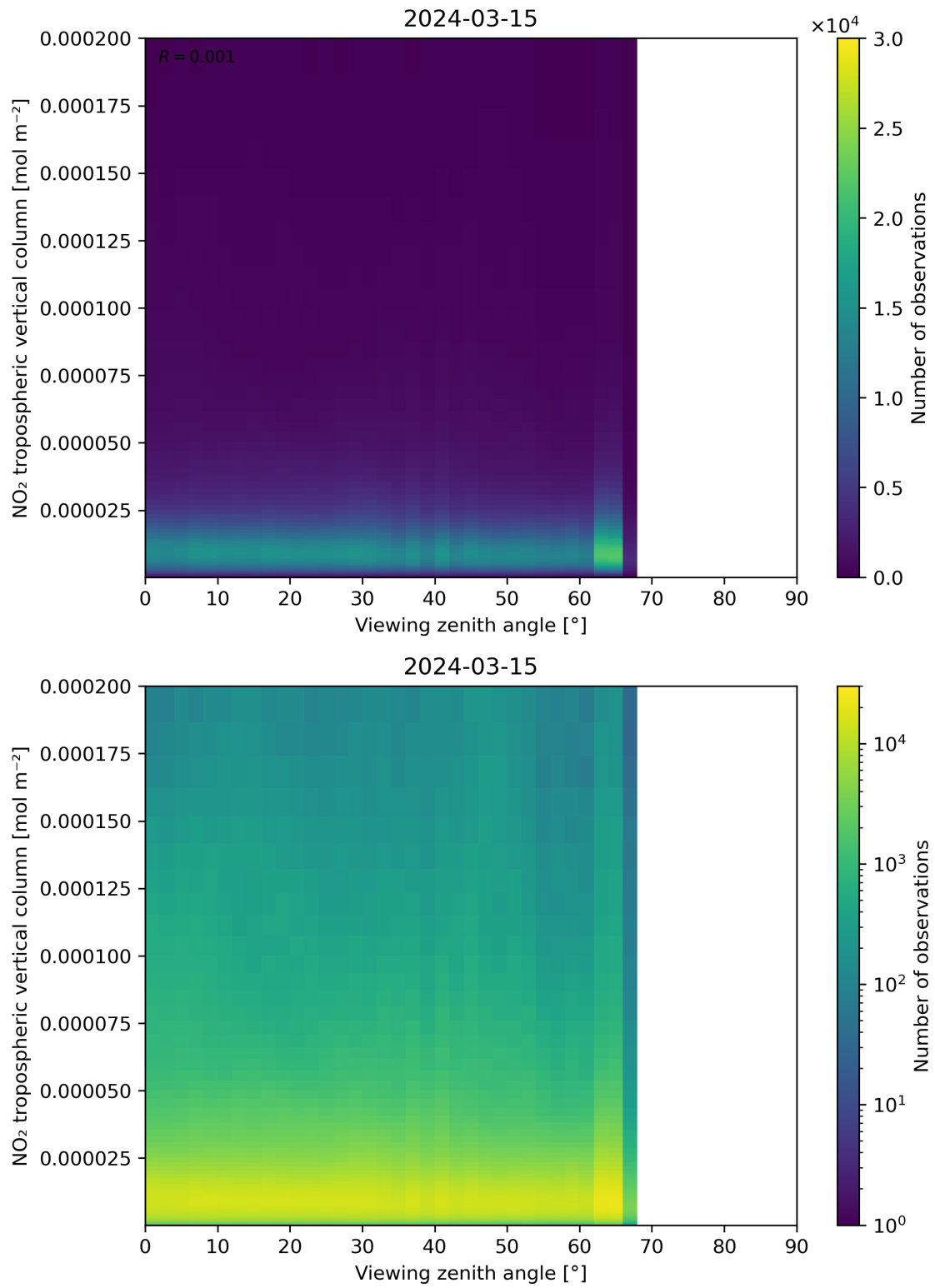
Figure 169: Scatter density plot of “Viewing zenith angle” against “NO 2 tropospheric vertical column” for 2024-03-14 to 2024-03-16.
