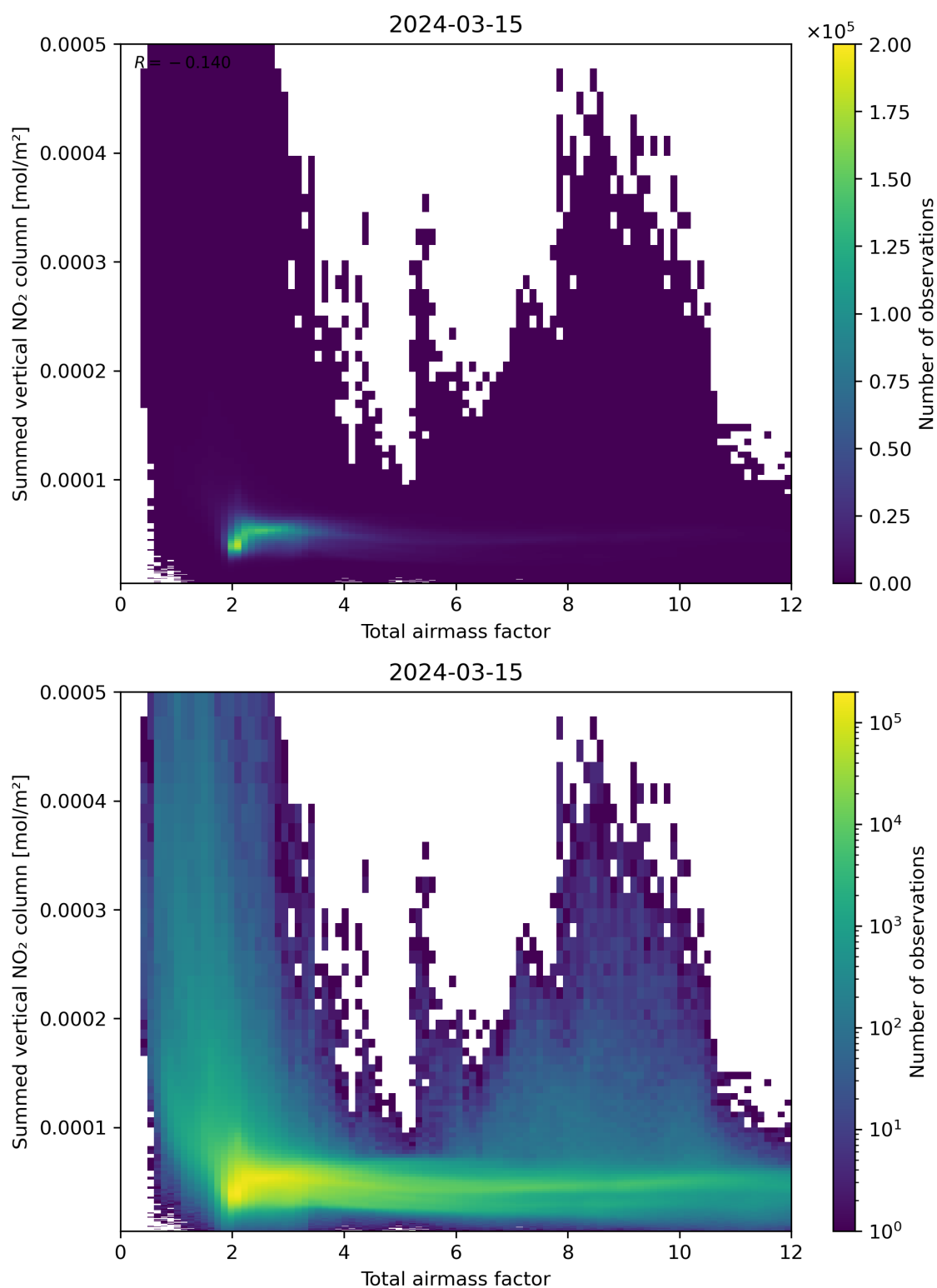
Figure 65: Scatter density plot of “Total airmass factor” against “Summed vertical NO 2 column” for 2024-03-14 to 2024-03-16.
