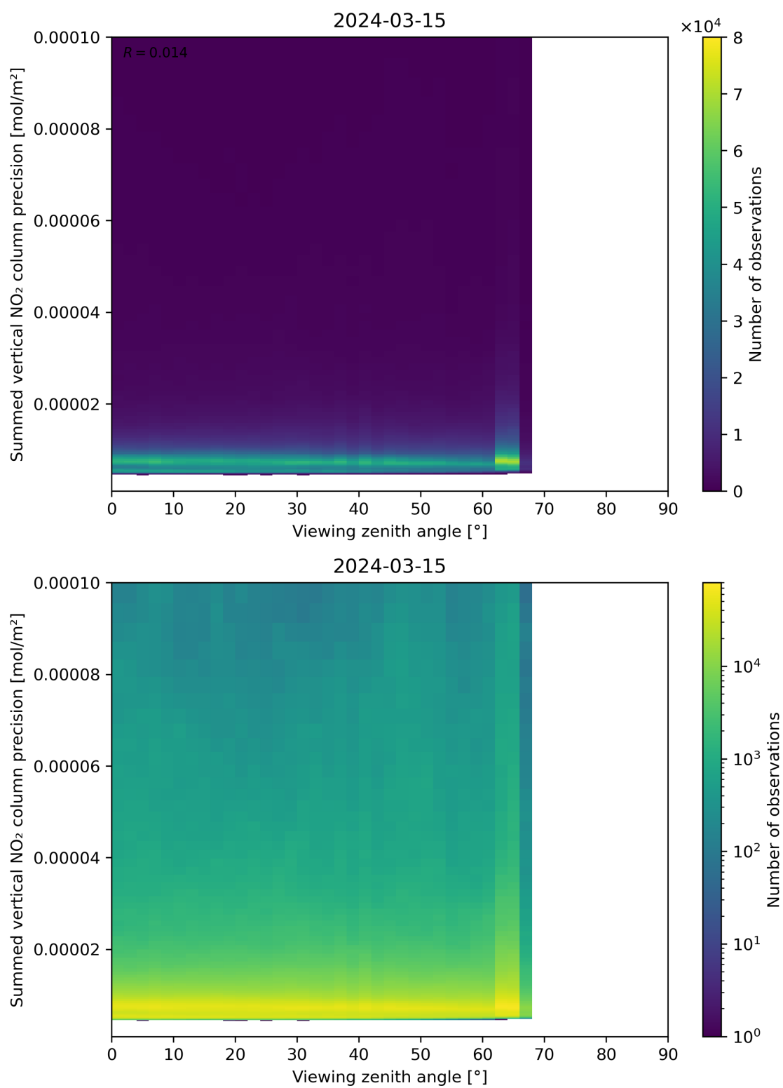
Figure 166: Scatter density plot of “Viewing zenith angle” against “Summed vertical NO 2 column precision” for 2024-03-14 to 2024-03-16.
