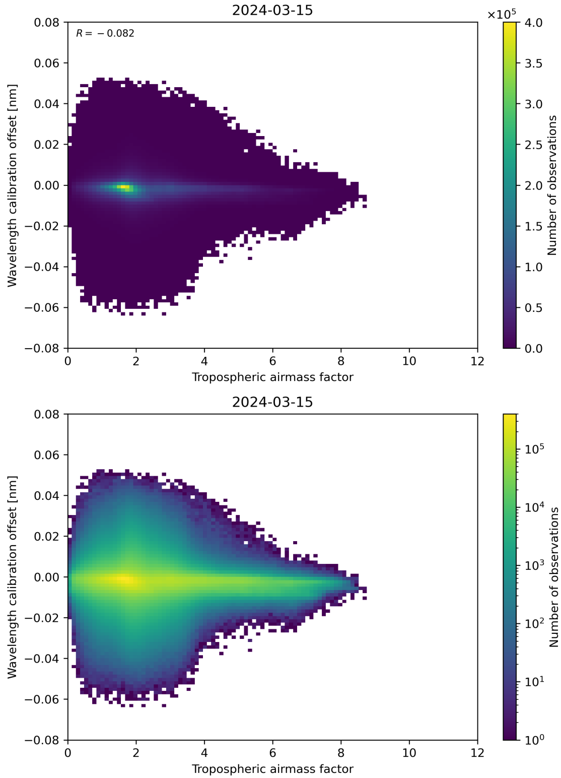
Figure 80: Scatter density plot of “Tropospheric air mass factor” against “Wavelength calibration offset” for 2024-03-14 to 2024-03-16.
