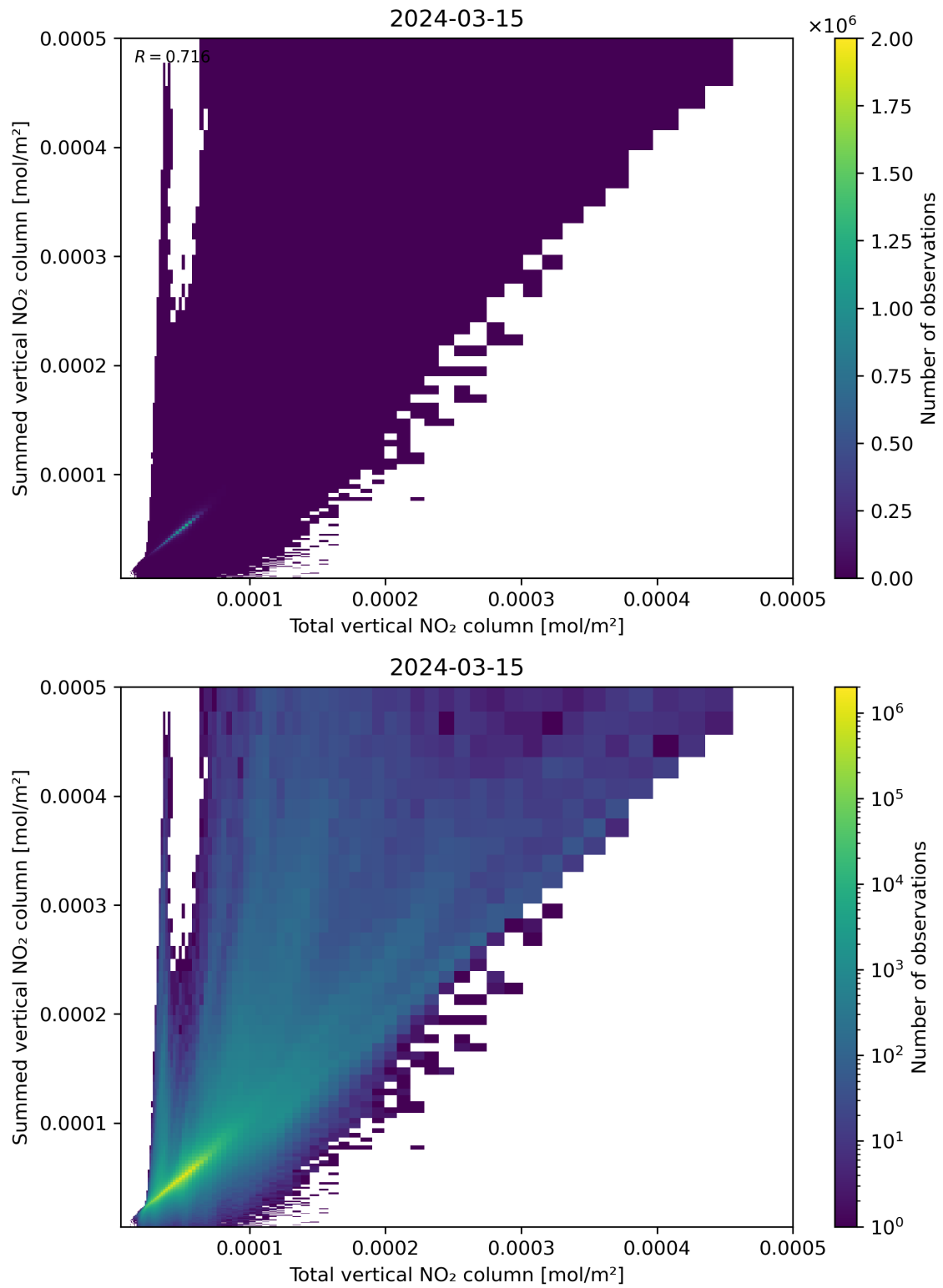
Figure 112: Scatter density plot of “Total vertical NO 2 column” against “Summed vertical NO 2 column” for 2024-03-14 to 2024-03-16.
