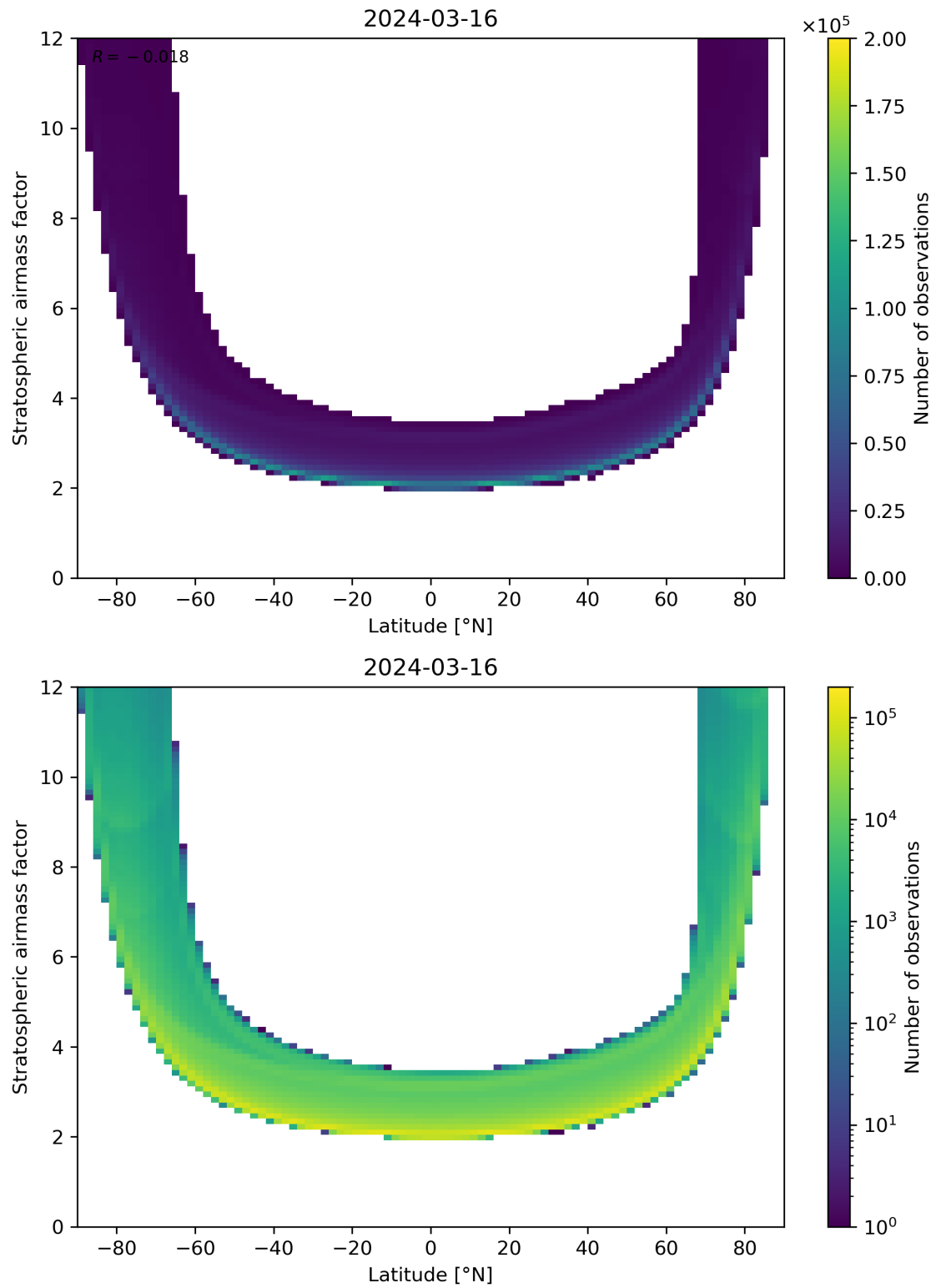
Figure 83: Scatter density plot of “Latitude” against “Stratospheric airmass factor” for 2024-03-15 to 2024-03-17.
