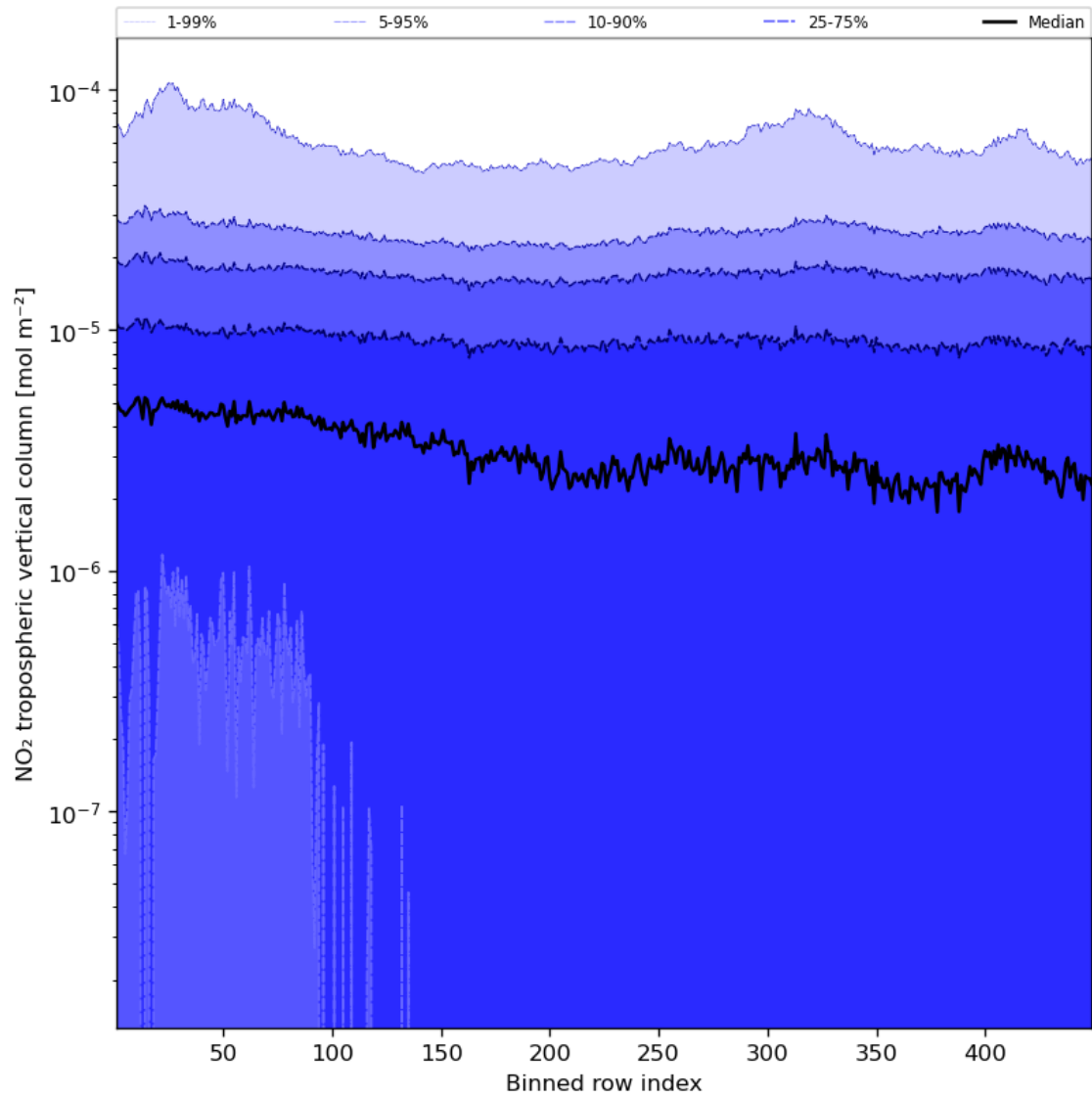
Figure 46: Along track statistics of “NO 2 tropospheric vertical column” for 2024-03-15 to 2024-03-17
