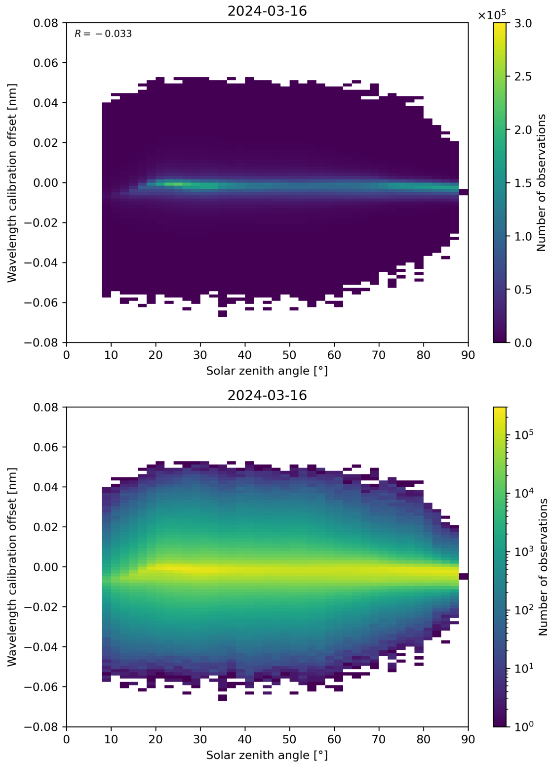
Figure 158: Scatter density plot of “Solar zenith angle” against “Wavelength calibration offset” for 2024-03-15 to 2024-03-17.
