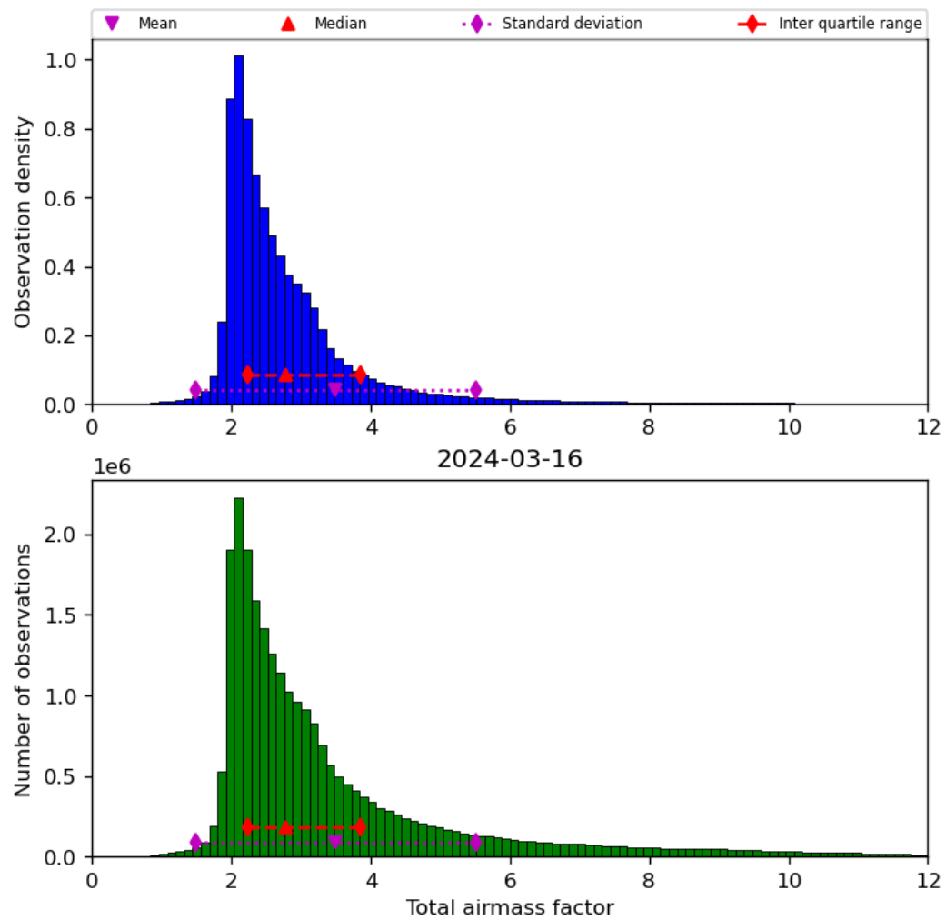
Figure 32: Histogram of “Total airmass factor” for 2024-03-15 to 2024-03-17
