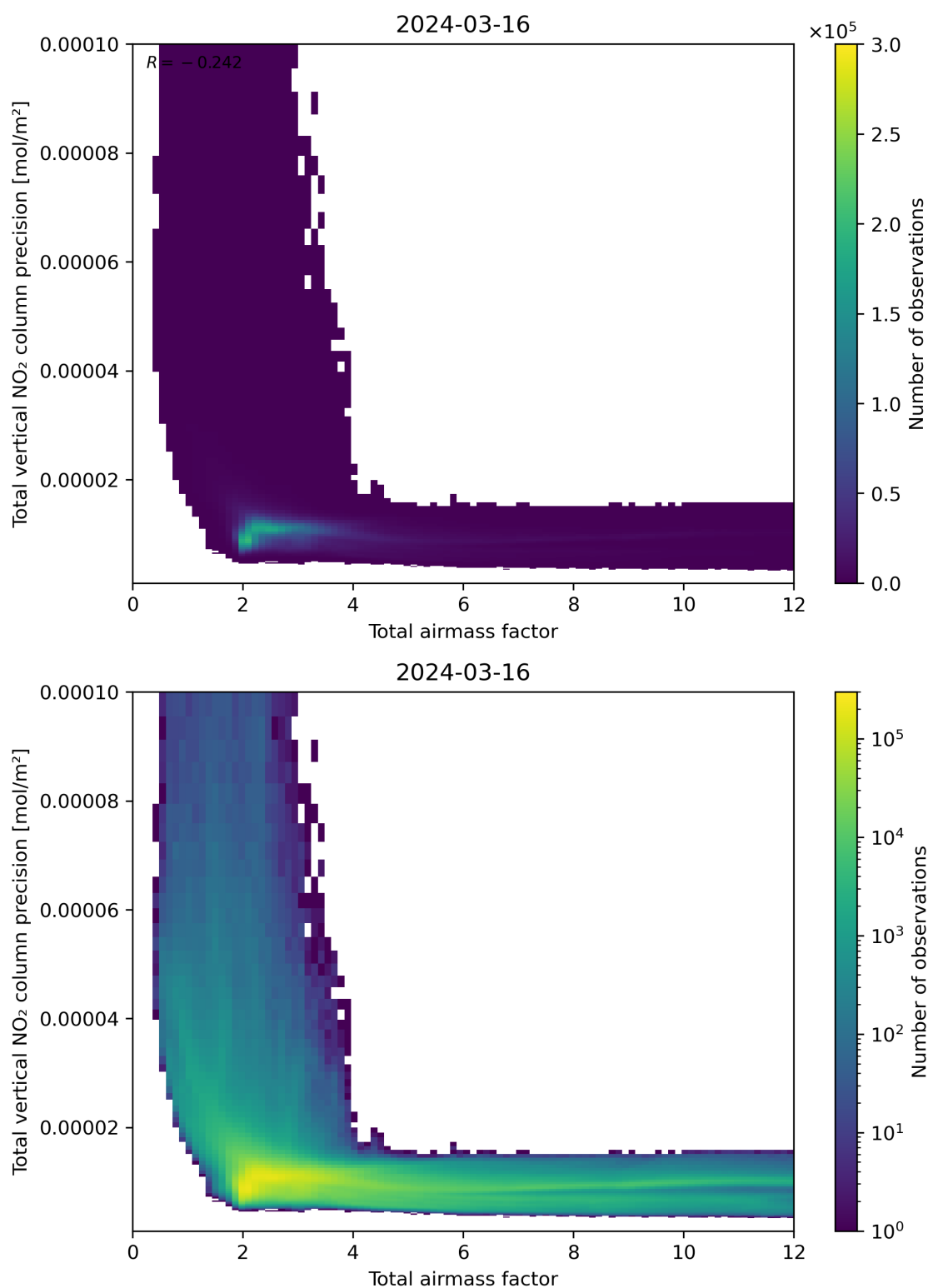
Figure 68: Scatter density plot of “Total airmass factor” against “Total vertical NO 2 column precision” for 2024-03-15 to 2024-03-17.
