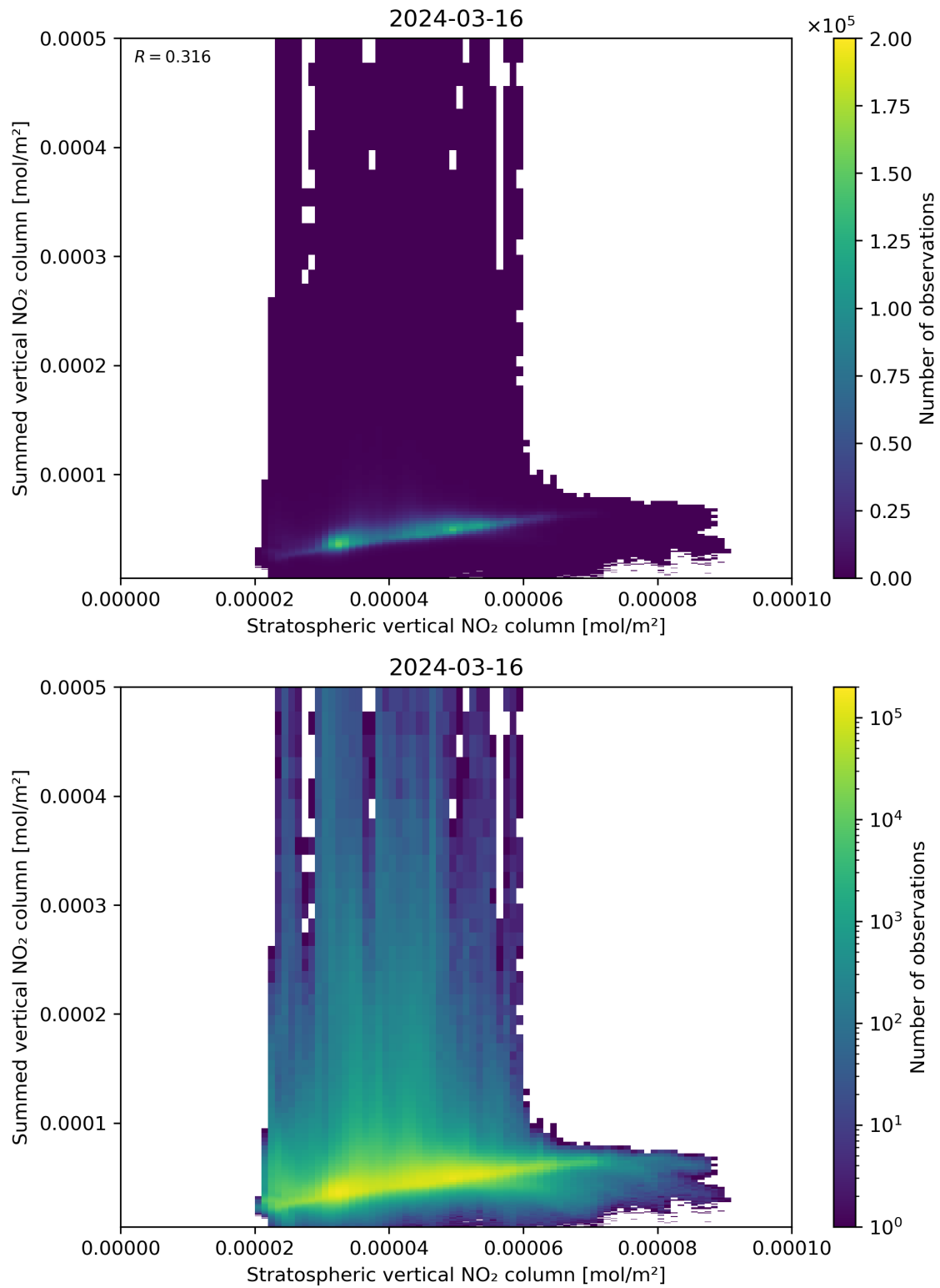
Figure 98: Scatter density plot of “Stratospheric vertical NO 2 column” against “Summed vertical NO 2 column” for 2024-03-15 to 2024-03-17.
