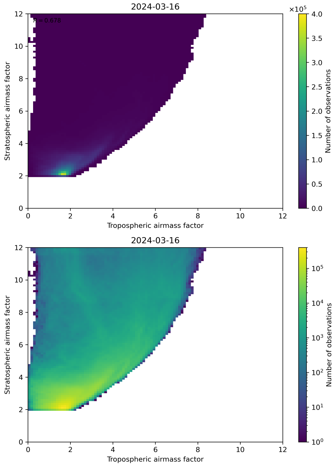
Figure 71: Scatter density plot of “Tropospheric airmass factor” against “Stratospheric airmass factor” for 2024-03-15 to 2024-03-17.
