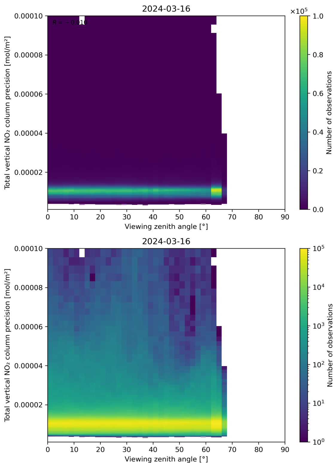
Figure 168: Scatter density plot of “Viewing zenith angle” against “Total vertical NO 2 column precision” for 2024-03-15 to 2024-03-17.
