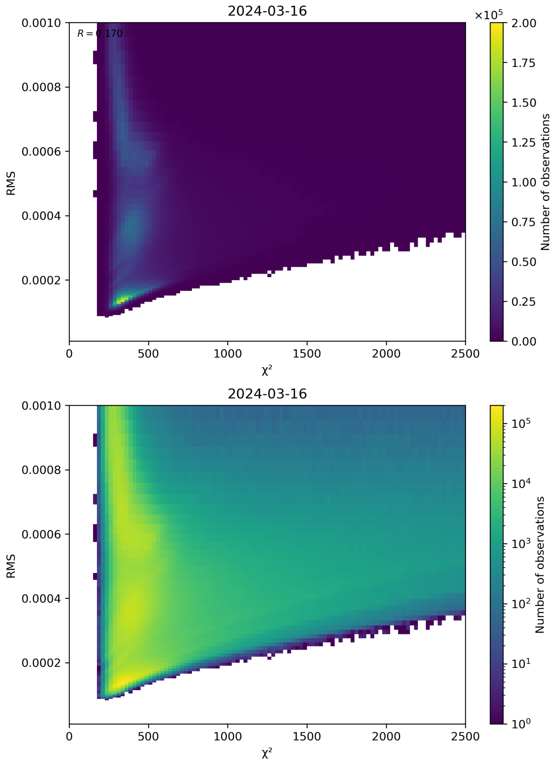
Figure 82: Scatter density plot of “ \chi^2 ” against “RMS” for 2024-03-15 to 2024-03-17.
