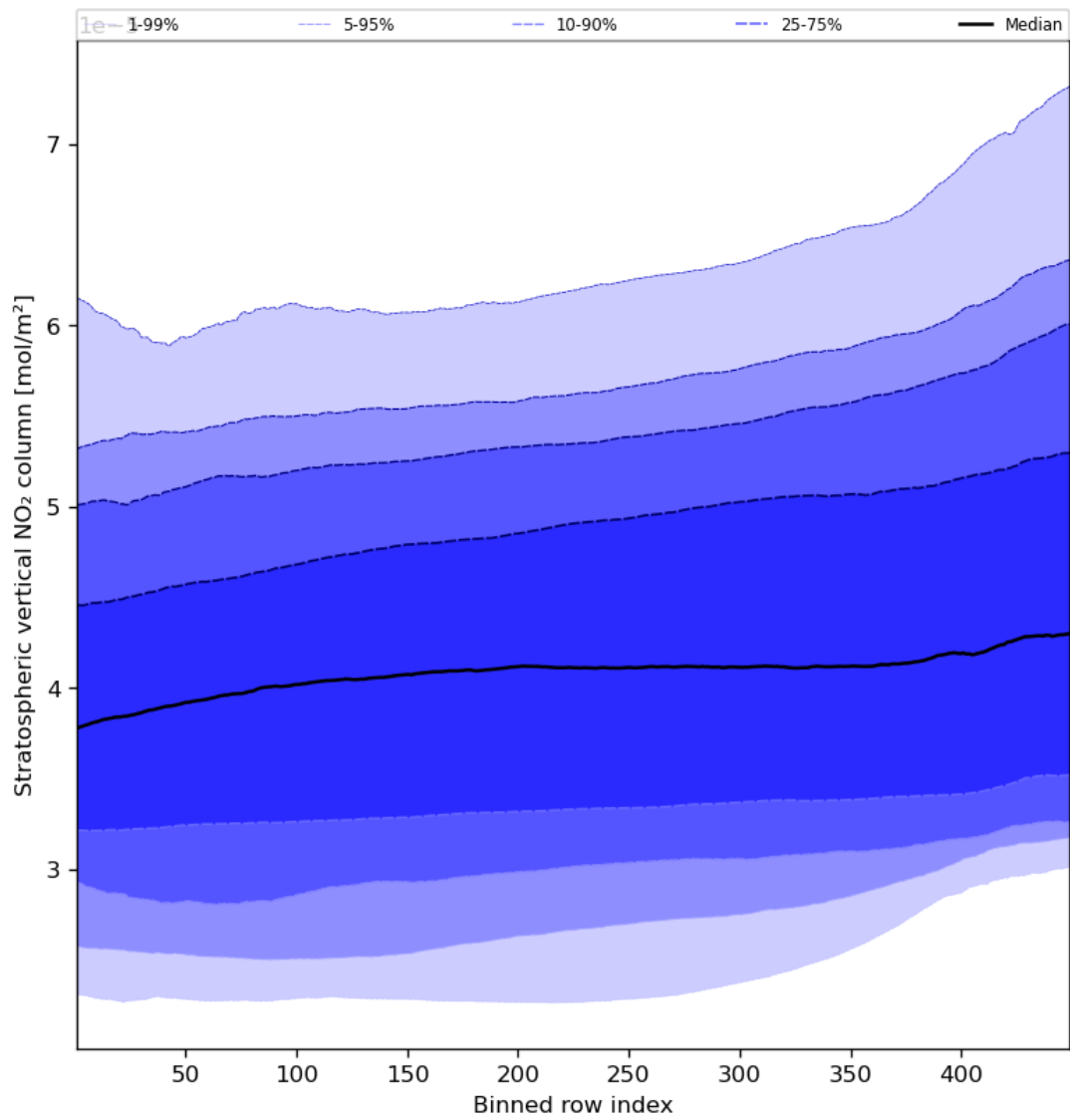
Figure 53: Along track statistics of “Stratospheric vertical NO 2 column” for 2024-03-15 to 2024-03-17
