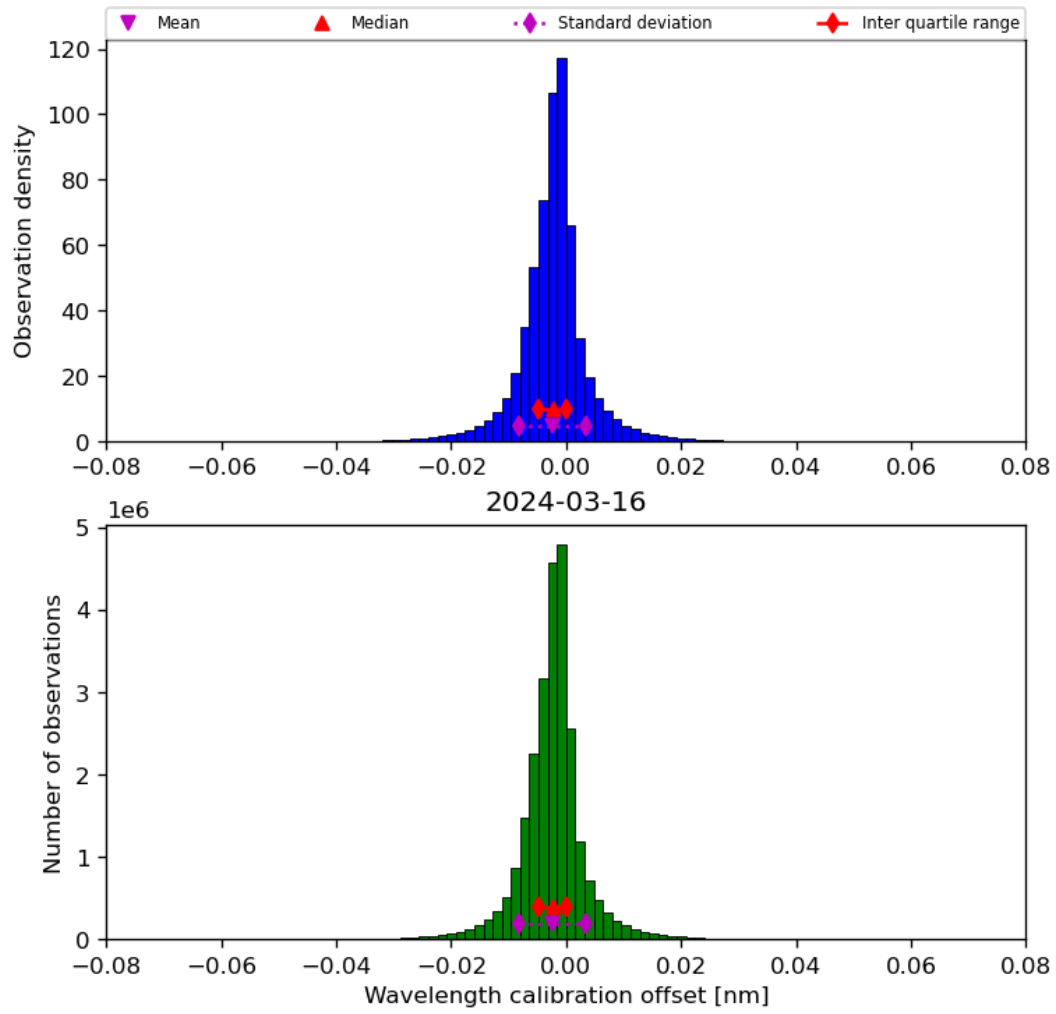
Figure 35: Histogram of “Wavelength calibration offset” for 2024-03-15 to 2024-03-17
