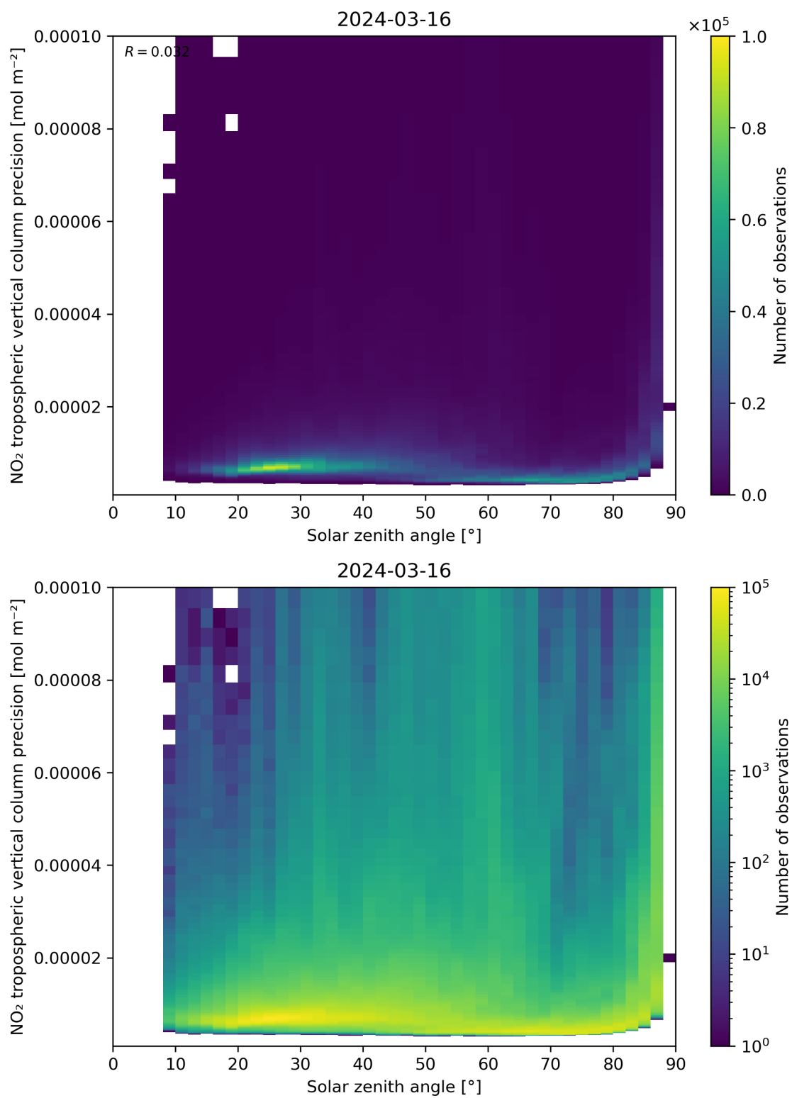
Figure 156: Scatter density plot of “Solar zenith angle” against “NO 2 tropospheric vertical column precision” for 2024-03-15 to 2024-03-17.
