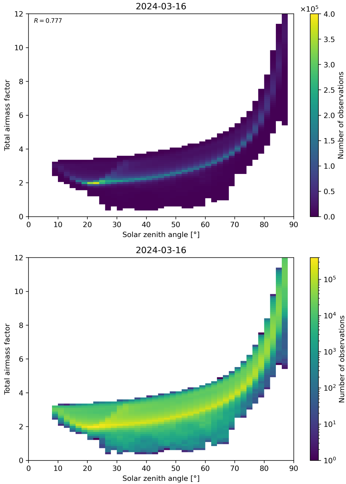
Figure 146: Scatter density plot of “Solar zenith angle” against “Total air mass factor” for 2024-03-15 to 2024-03-17.
