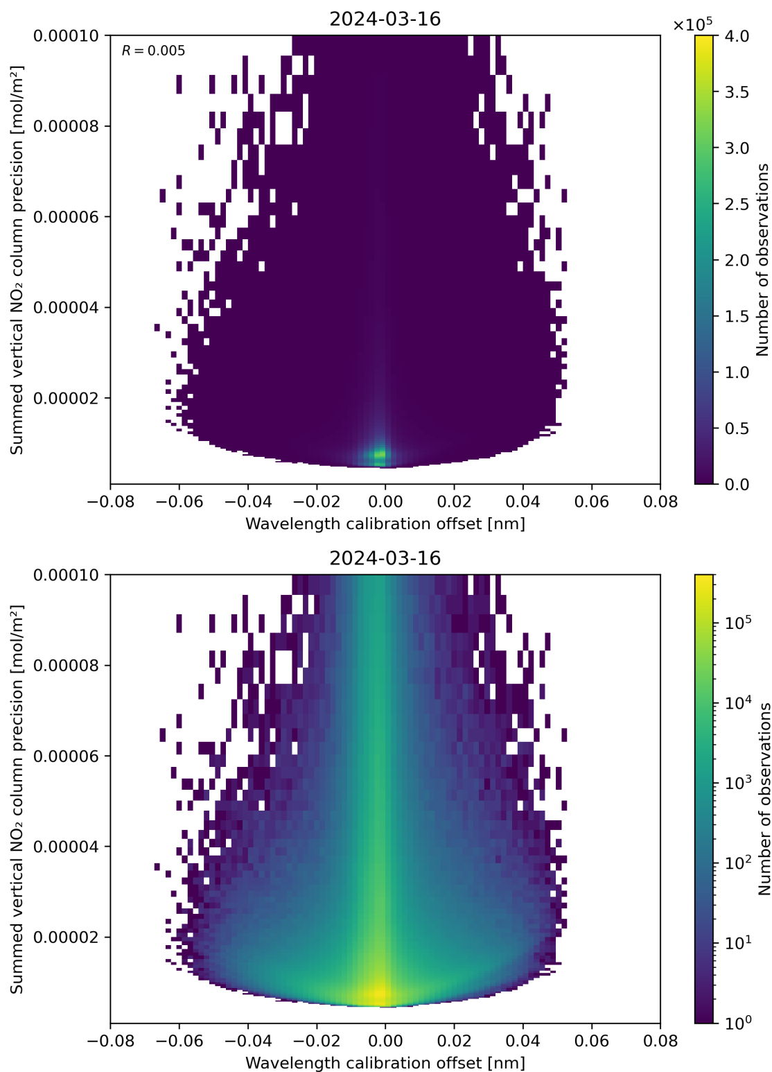
Figure 178: Scatter density plot of “Wavelength calibration offset” against “Summed vertical NO 2 column precision” for 2024-03-15 to 2024-03-17.
