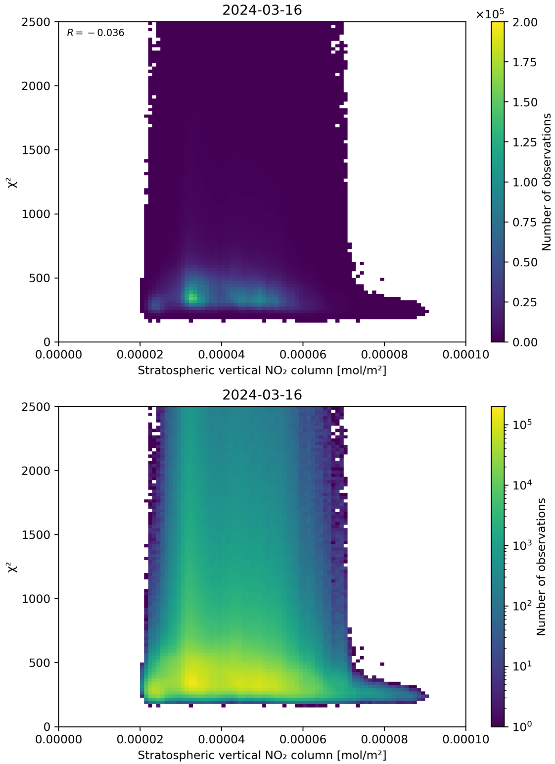
Figure 97: Scatter density plot of “Stratospheric vertical NO 2 column” against “ \chi^2 ” for 2024-03-15 to 2024-03-17.
