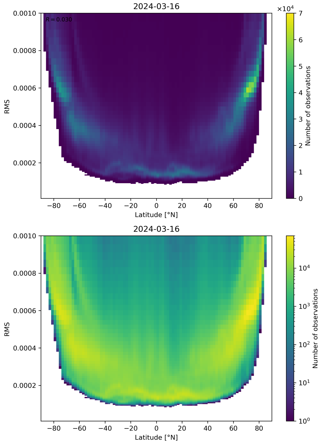
Figure 94: Scatter density plot of “Latitude” against “RMS” for 2024-03-15 to 2024-03-17.
