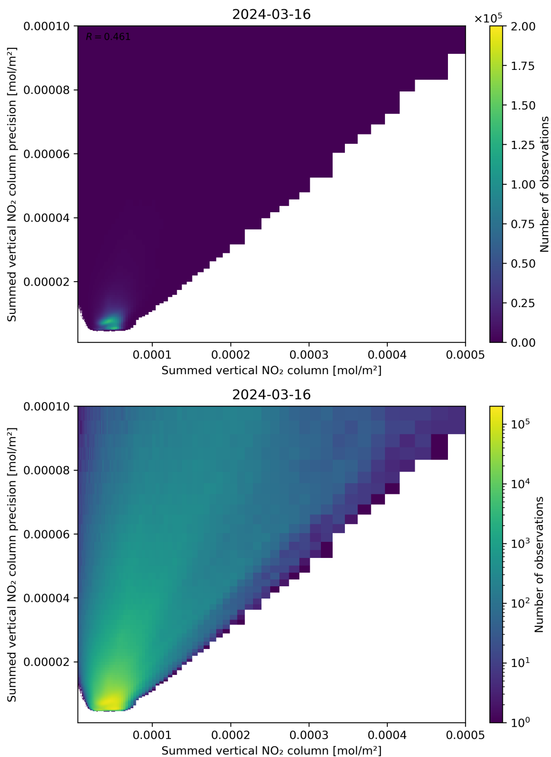
Figure 105: Scatter density plot of “Summed vertical NO 2 column” against “Summed vertical NO 2 column precision” for 2024-03-15 to 2024-03-17.
