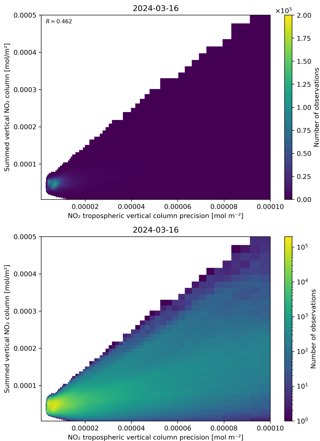
Figure 136: Scatter density plot of “NO 2 tropospheric vertical column precision” against “Summed vertical NO 2 column” for 2024-03-15 to 2024-03-17.
