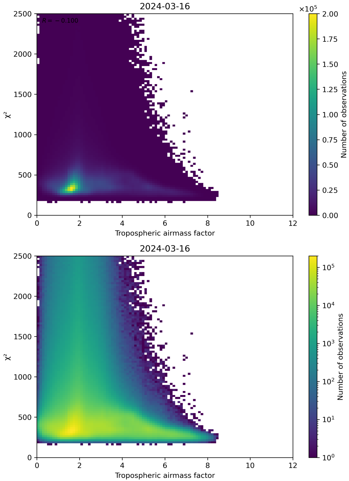
Figure 73: Scatter density plot of “Tropospheric airmass factor” against “ \chi^2 ” for 2024-03-15 to 2024-03-17.
