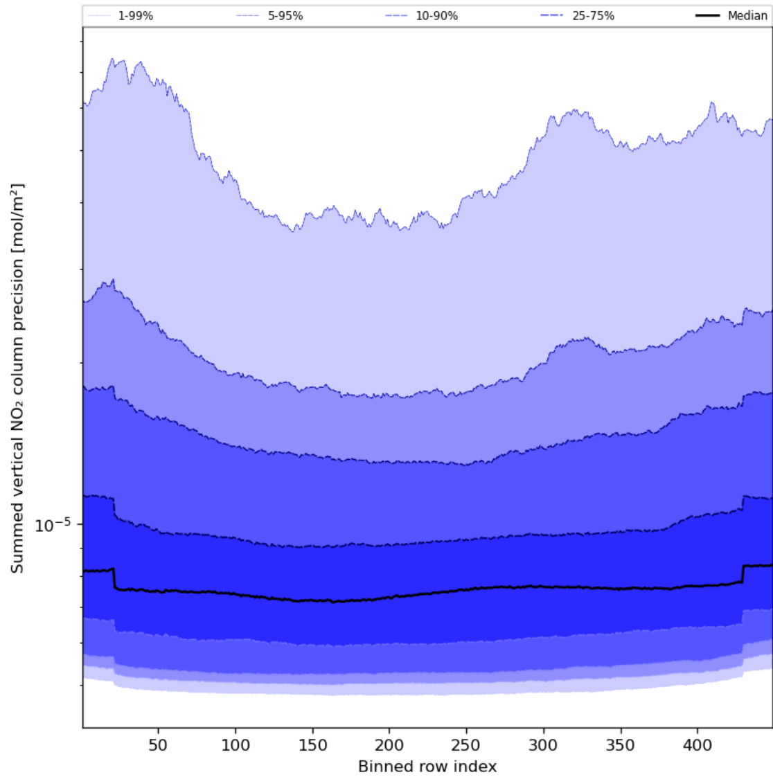
Figure 58: Along track statistics of “Summed vertical NO 2 column precision” for 2024-03-15 to 2024-03-17
