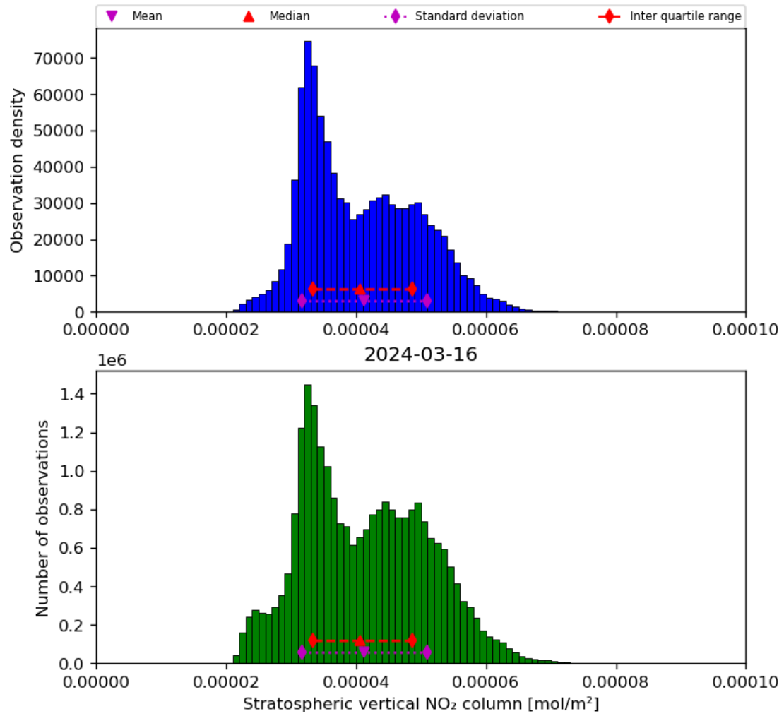
Figure 36: Histogram of “Stratospheric vertical NO 2 column” for 2024-03-15 to 2024-03-17
