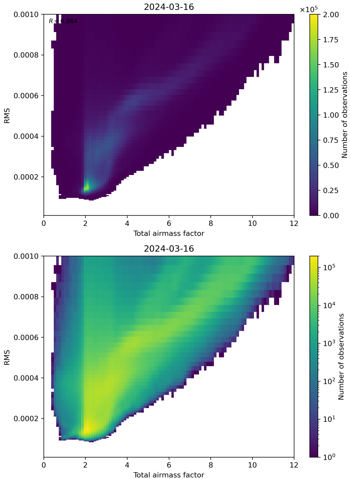
Figure 69: Scatter density plot of “Total airmass factor” against “RMS” for 2024-03-15 to 2024-03-17.
