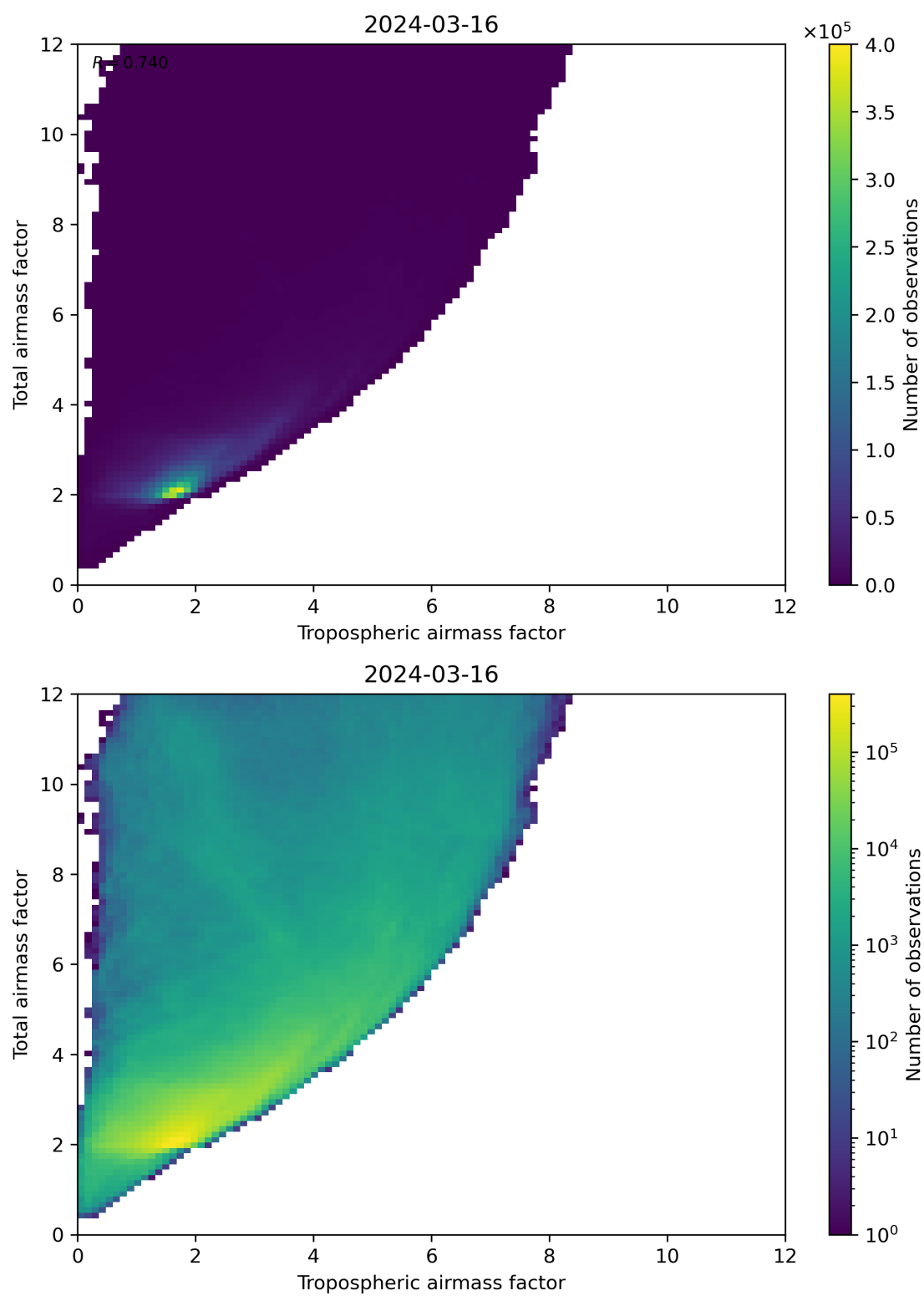
Figure 72: Scatter density plot of “Tropospheric airmass factor” against “Total airmass factor” for 2024-03-15 to 2024-03-17.
