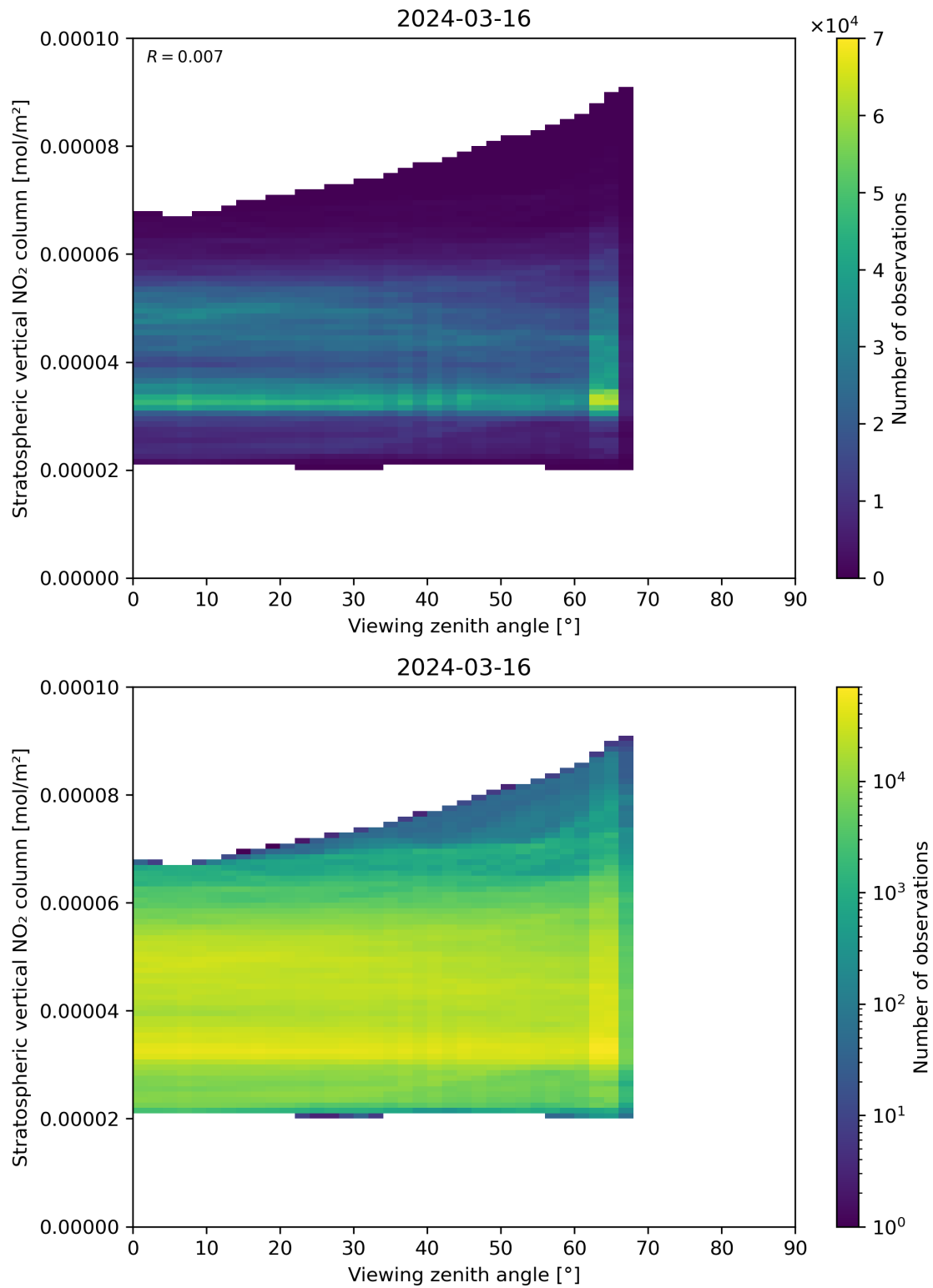
Figure 164: Scatter density plot of “Viewing zenith angle” against “Stratospheric vertical NO 2 column” for 2024-03-15 to 2024-03-17.
