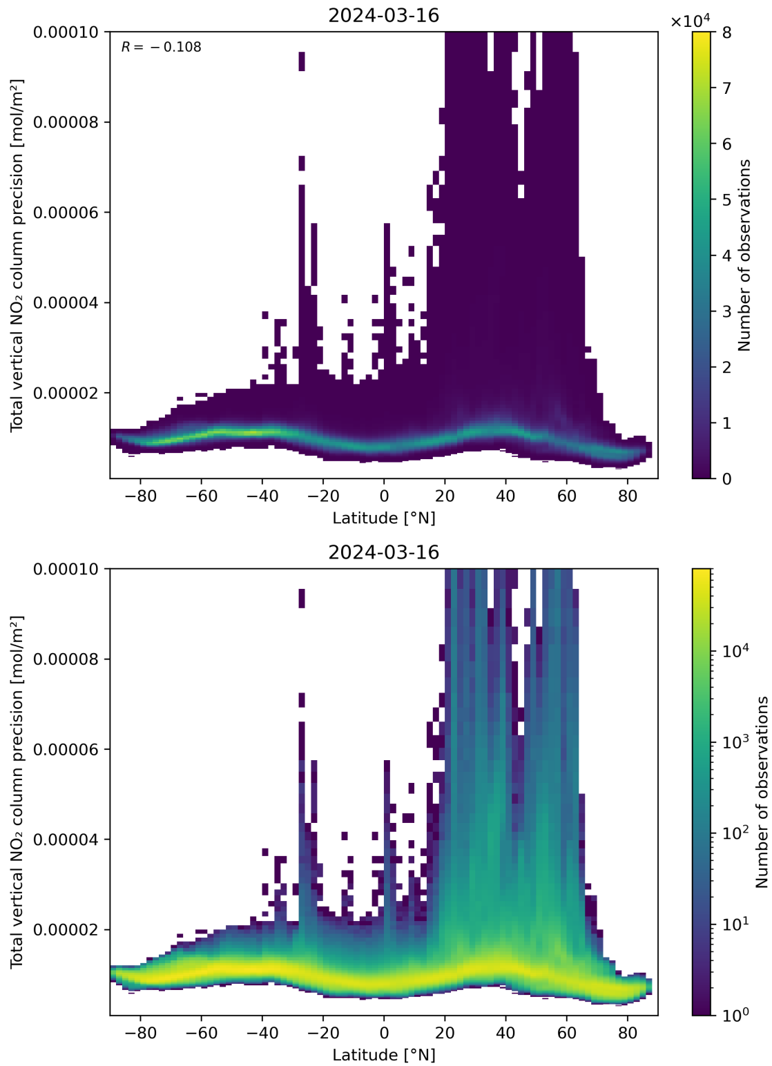
Figure 91: Scatter density plot of “Latitude” against “Total vertical NO 2 column precision” for 2024-03-15 to 2024-03-17.
