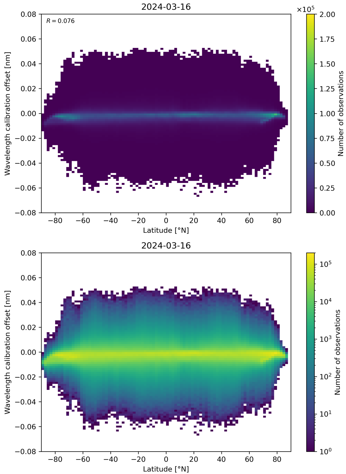
Figure 95: Scatter density plot of “Latitude” against “Wavelength calibration offset” for 2024-03-15 to 2024-03-17.
