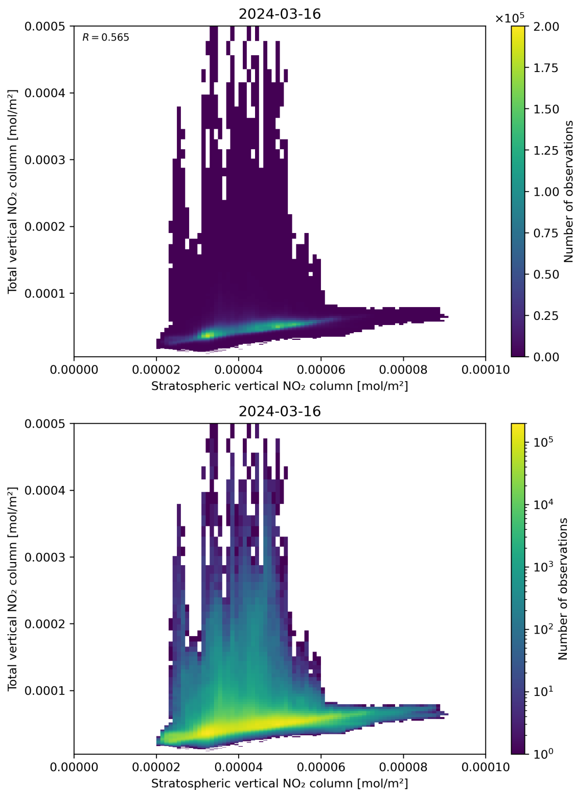
Figure 100: Scatter density plot of “Stratospheric vertical NO 2 column” against “Total vertical NO 2 column” for 2024-03-15 to 2024-03-17.
