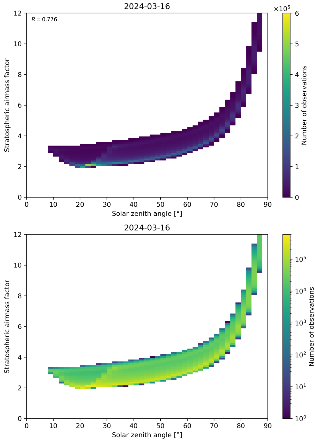
Figure 145: Scatter density plot of “Solar zenith angle” against “Stratospheric airmass factor” for 2024-03-15 to 2024-03-17.
