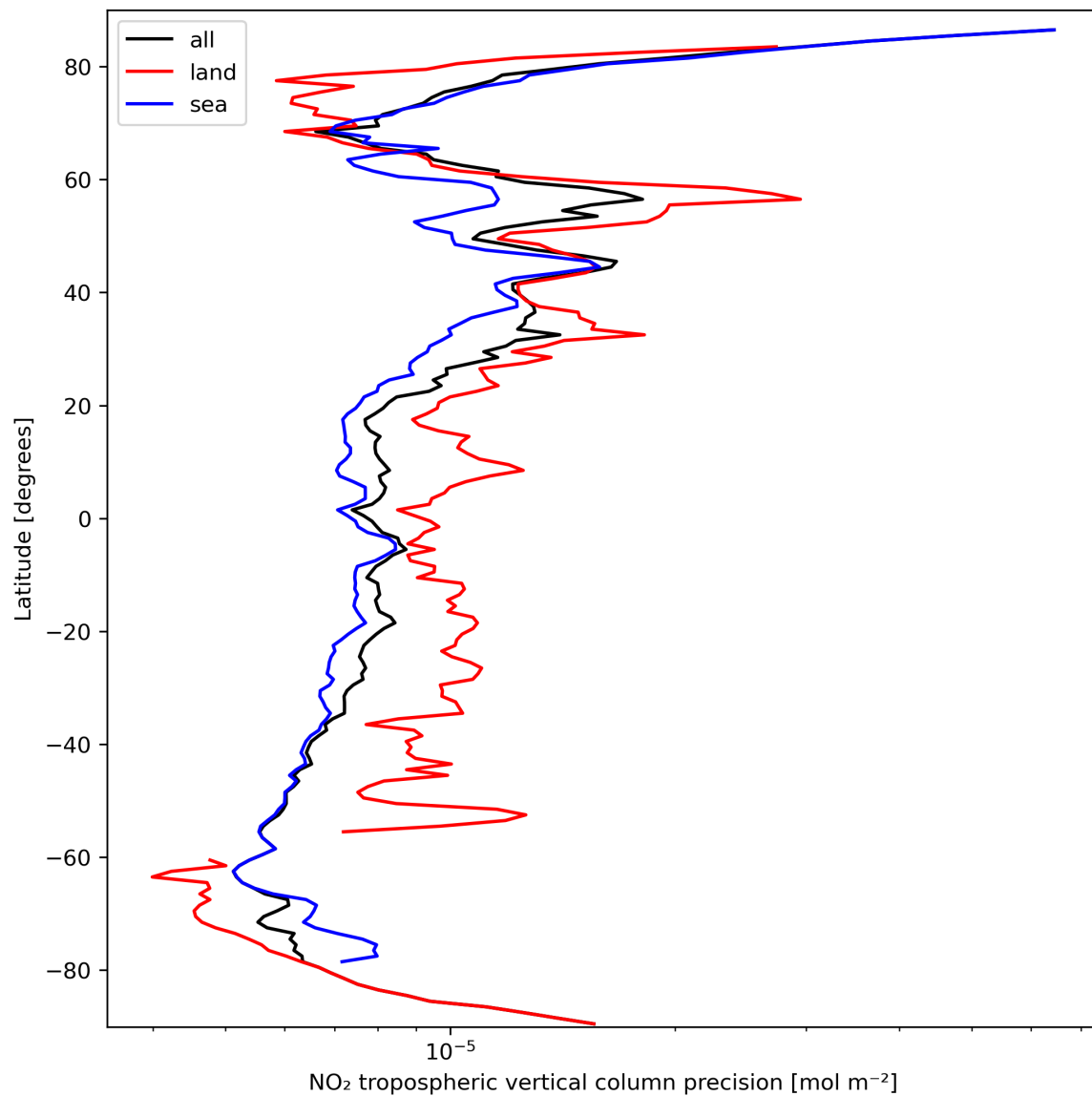
Figure 13: Zonal average of "NO 2 tropospheric vertical column precision" for 2024-03-15 to 2024-03-17.
