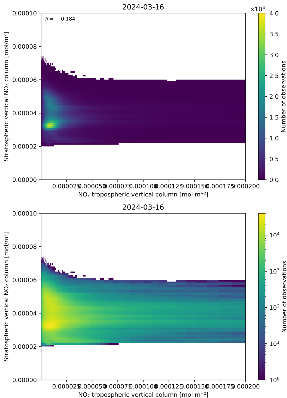
Figure 125: Scatter density plot of “NO 2 tropospheric vertical column” against “Stratospheric vertical NO 2 column” for 2024-03-15 to 2024-03-17.
