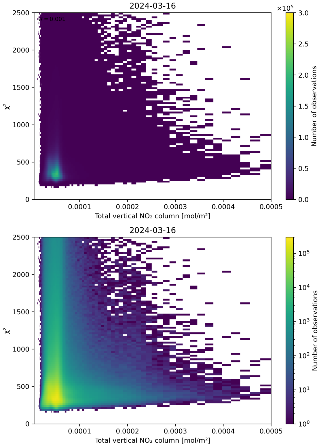
Figure 111: Scatter density plot of “Total vertical NO 2 column” against “ \chi^2 ” for 2024-03-15 to 2024-03-17.
