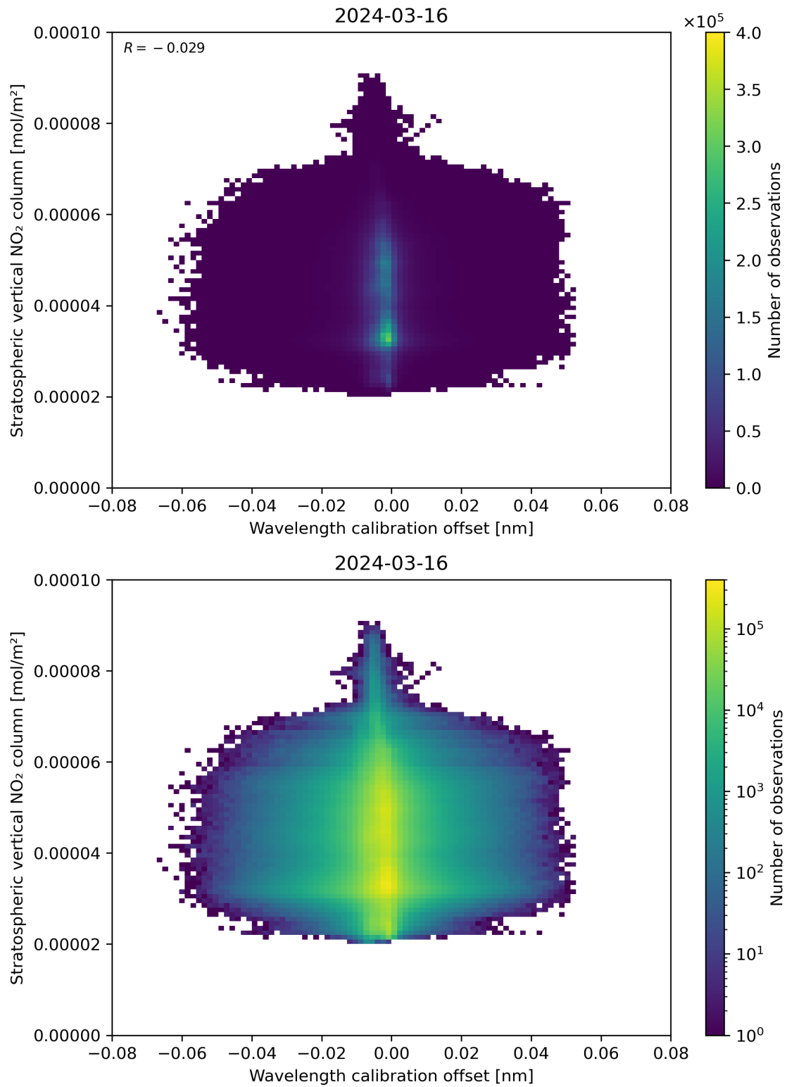
Figure 176: Scatter density plot of “Wavelength calibration offset” against “Stratospheric vertical NO 2 column” for 2024-03-15 to 2024-03-17.
