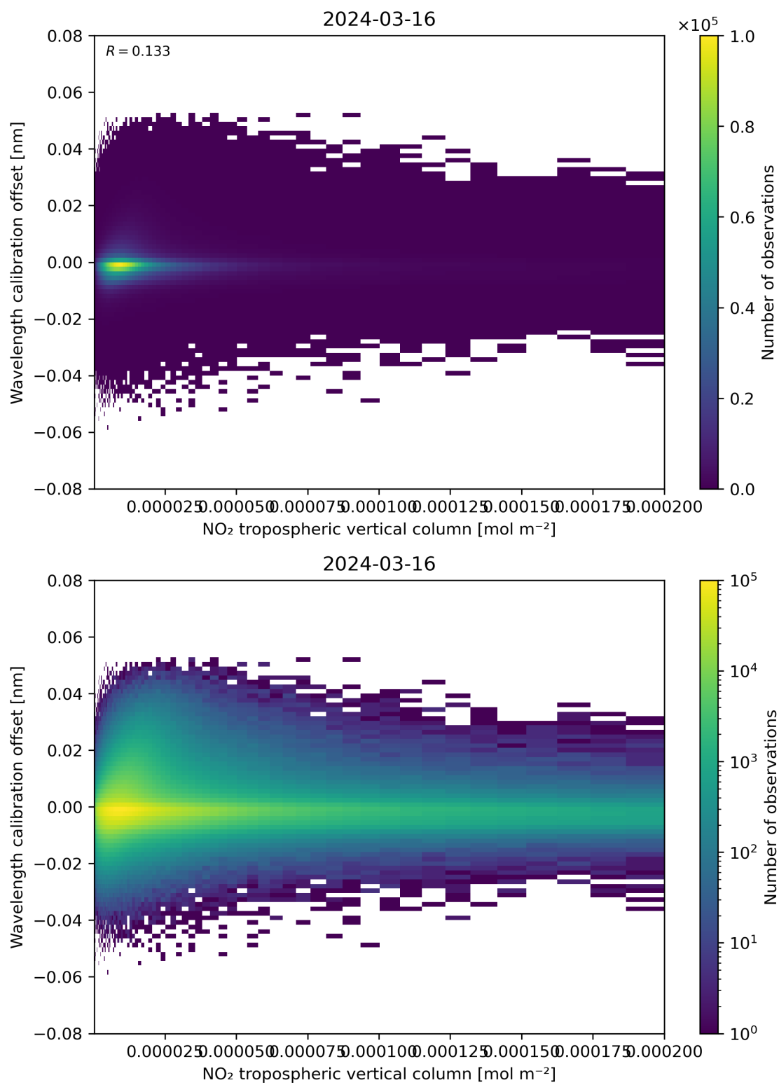
Figure 143: Scatter density plot of “NO 2 tropospheric vertical column” against “Wavelength calibration offset” for 2024-03-15 to 2024-03-17.
