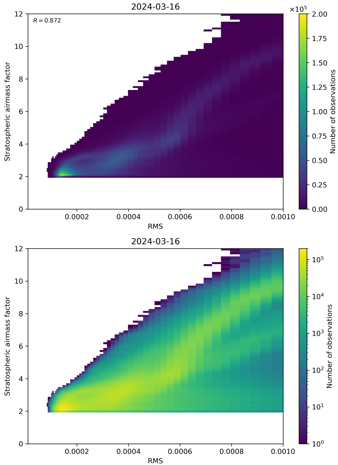
Figure 144: Scatter density plot of “RMS” against “Stratospheric airmass factor” for 2024-03-15 to 2024-03-17.
