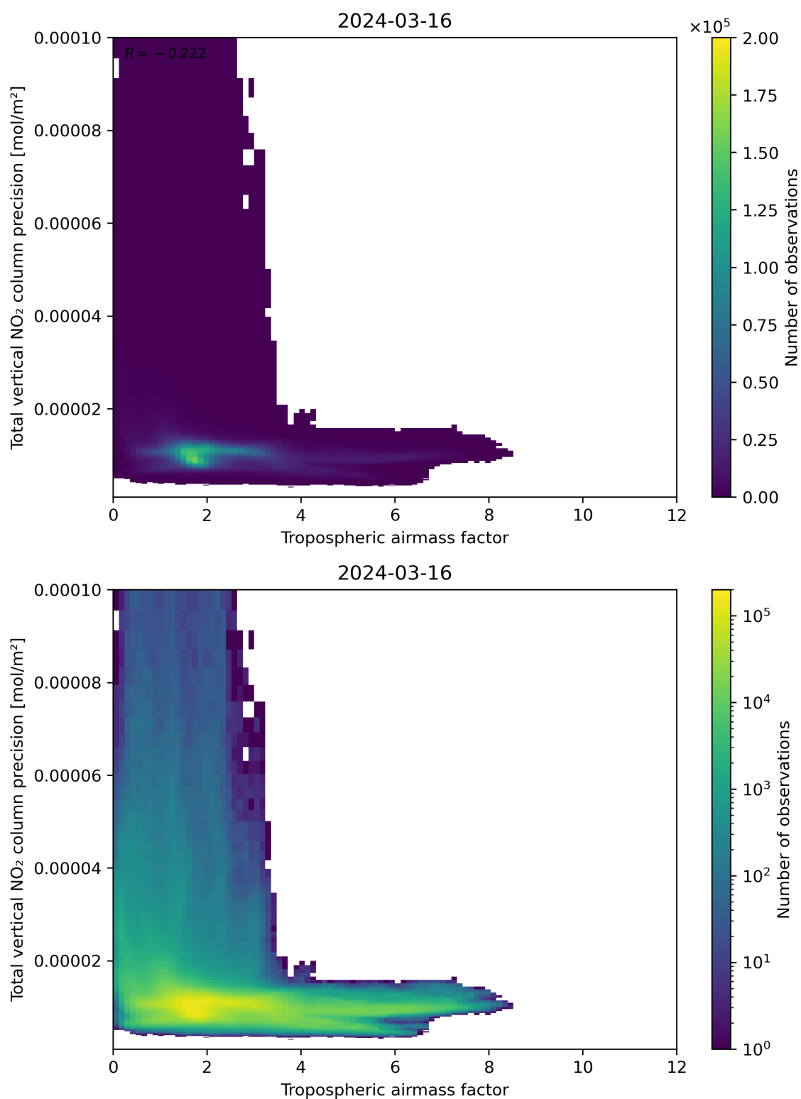
Figure 78: Scatter density plot of “Tropospheric air mass factor” against “Total vertical NO 2 column precision” for 2024-03-15 to 2024-03-17.
