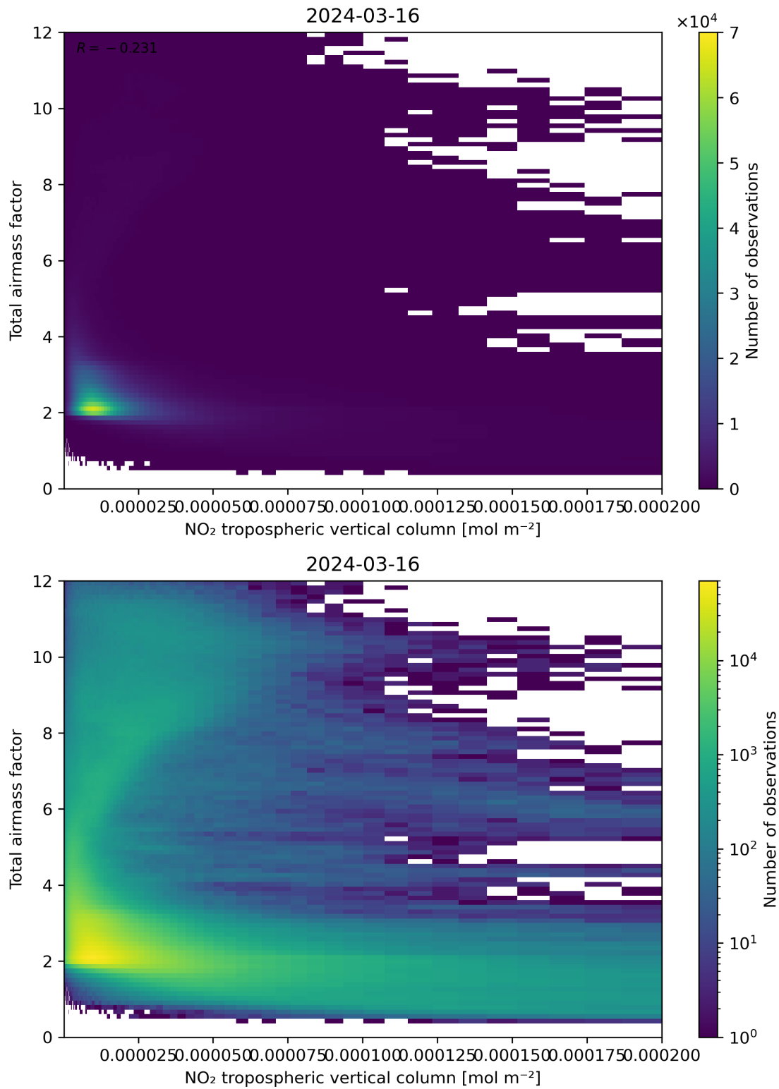
Figure 122: Scatter density plot of “NO 2 tropospheric vertical column” against “Total air mass factor” for 2024-03-15 to 2024-03-17.
