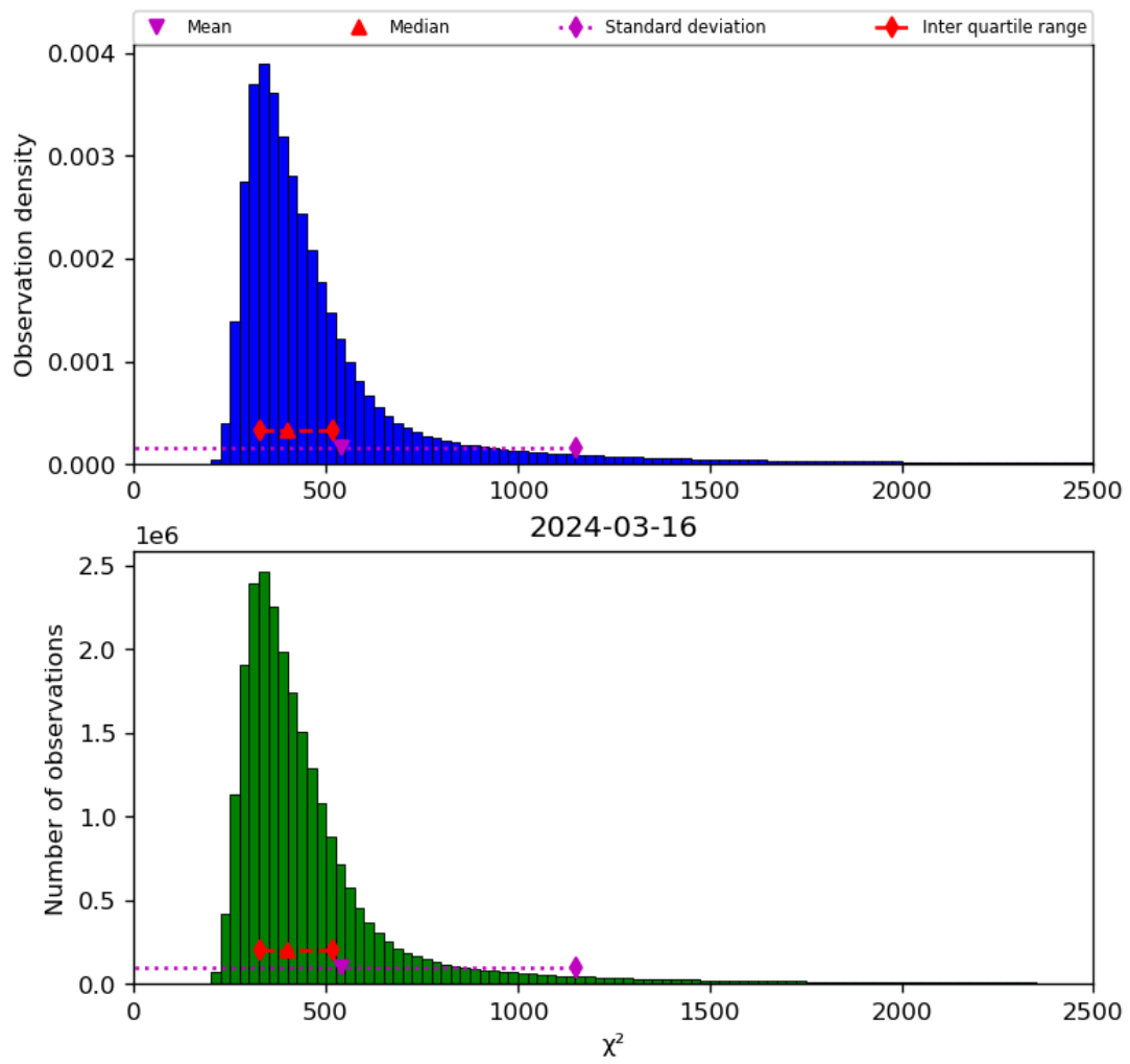
Figure 42: Histogram of “ \chi^2 ” for 2024-03-15 to 2024-03-17
