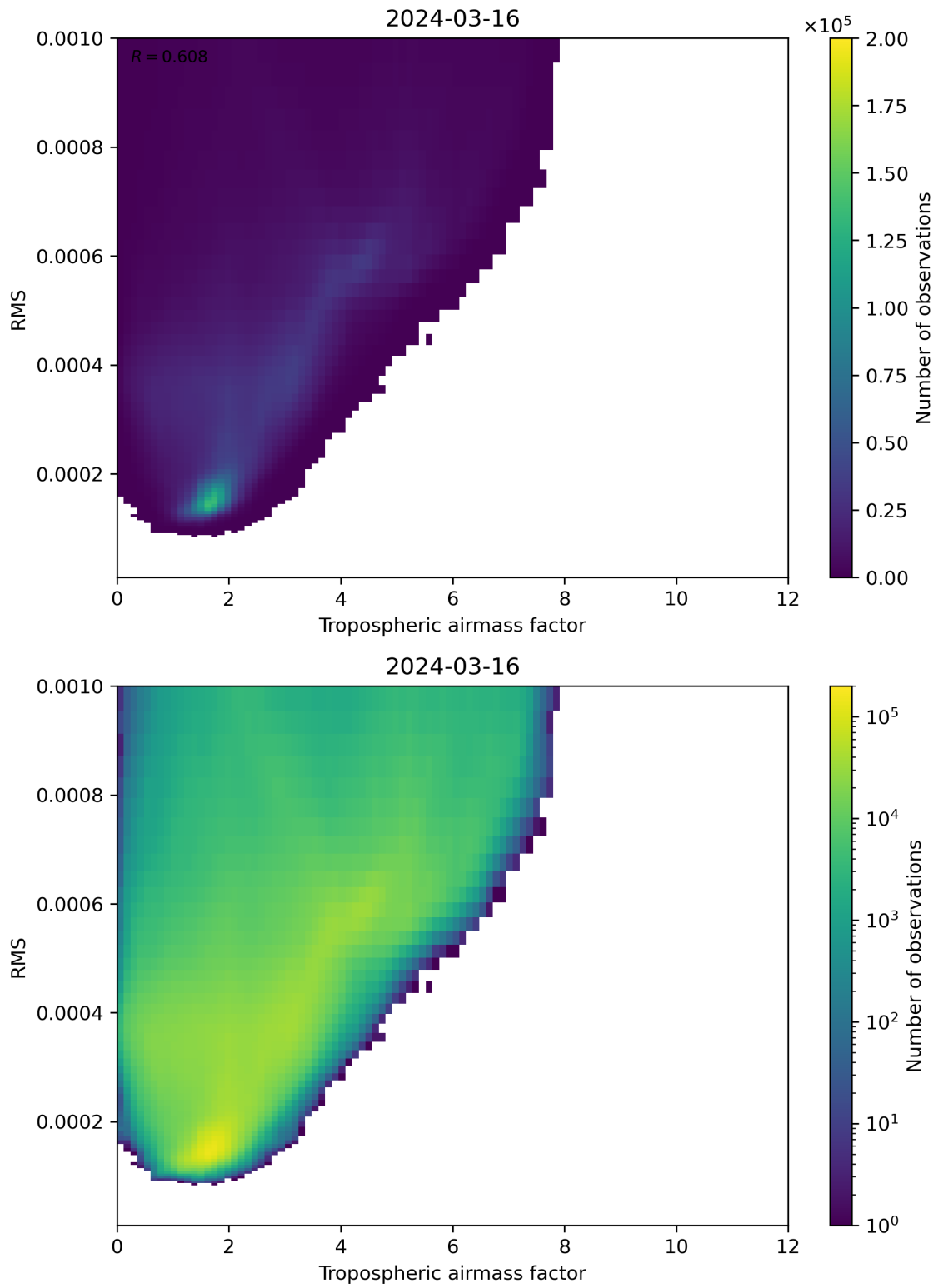
Figure 79: Scatter density plot of “Tropospheric airmass factor” against “RMS” for 2024-03-15 to 2024-03-17.
