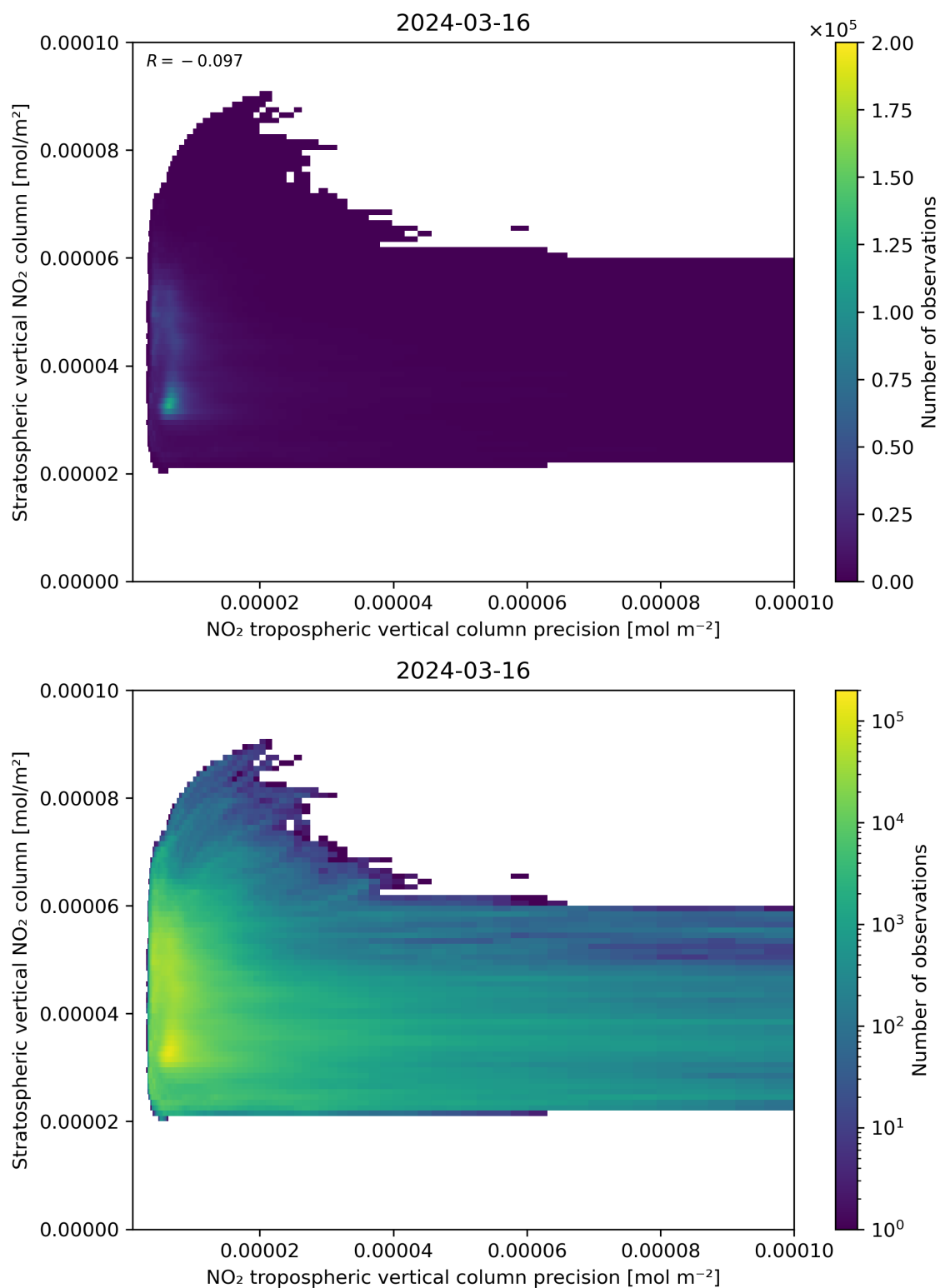
Figure 135: Scatter density plot of “NO 2 tropospheric vertical column precision” against “Stratospheric vertical NO 2 column” for 2024-03-15 to 2024-03-17.
