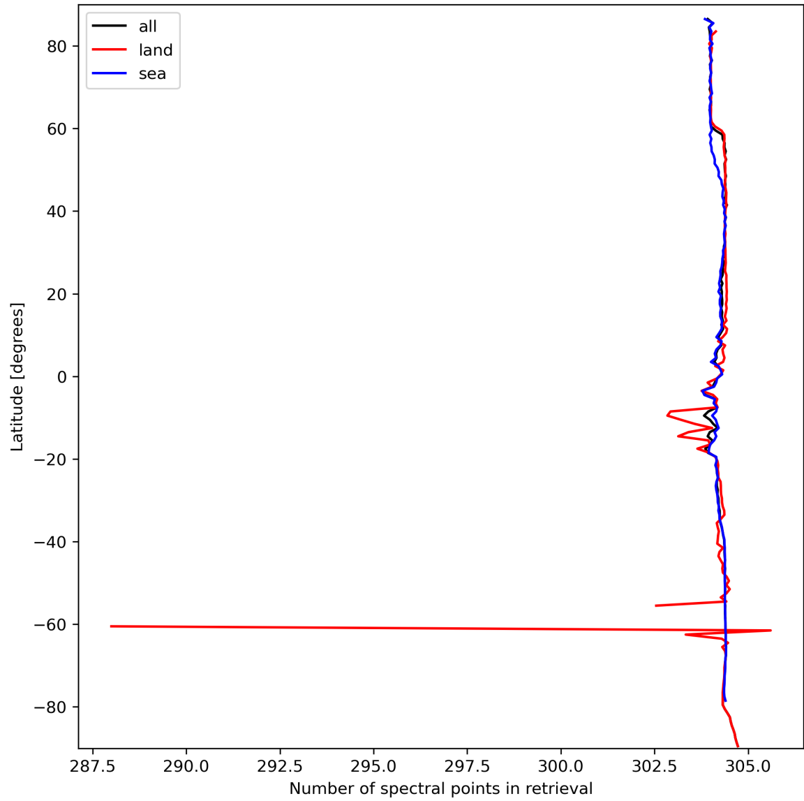
Figure 16: Zonal average of “Number of spectral points in retrieval” for 2024-03-15 to 2024-03-17.
