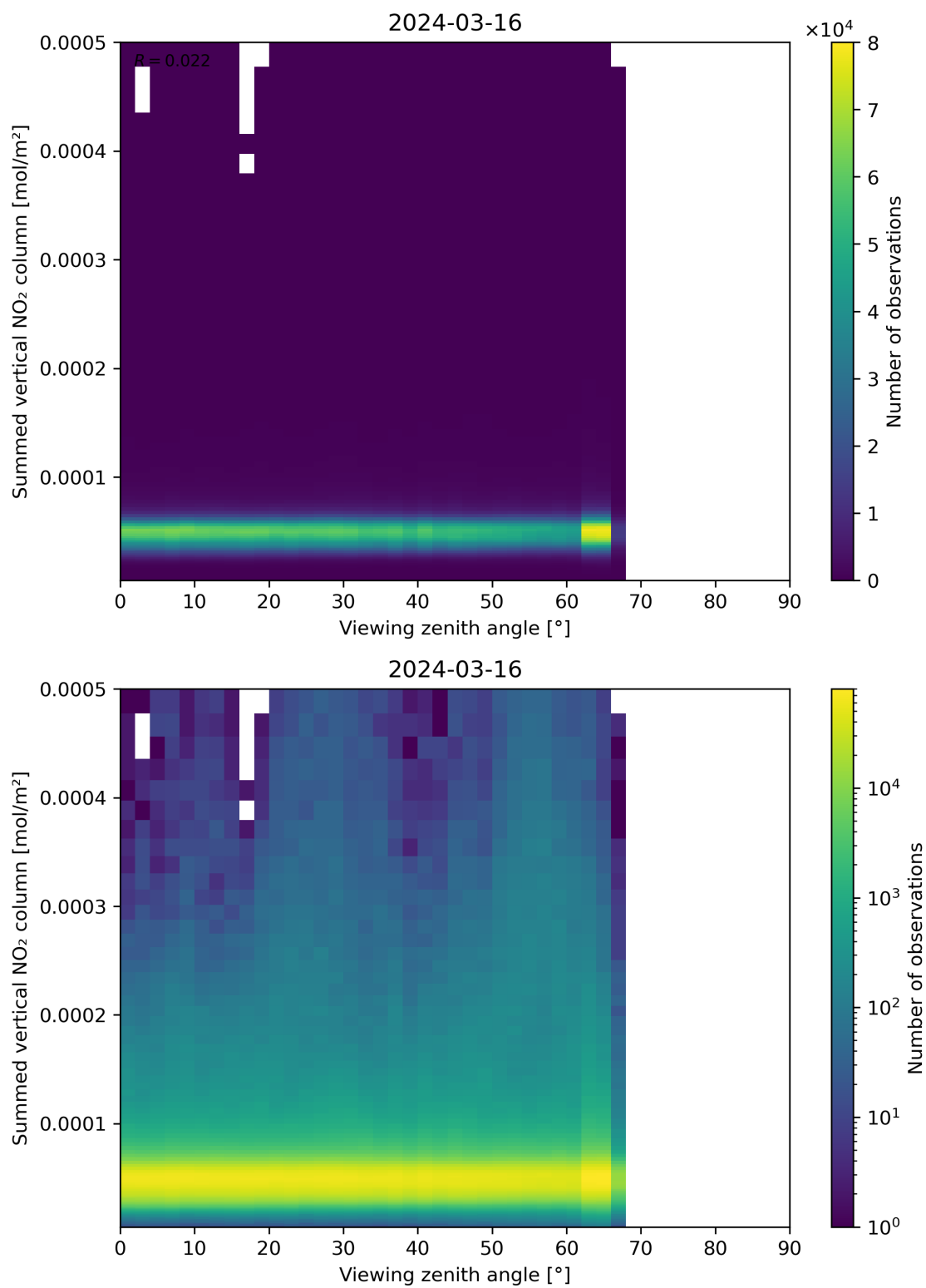
Figure 165: Scatter density plot of “Viewing zenith angle” against “Summed vertical NO 2 column” for 2024-03-15 to 2024-03-17.
