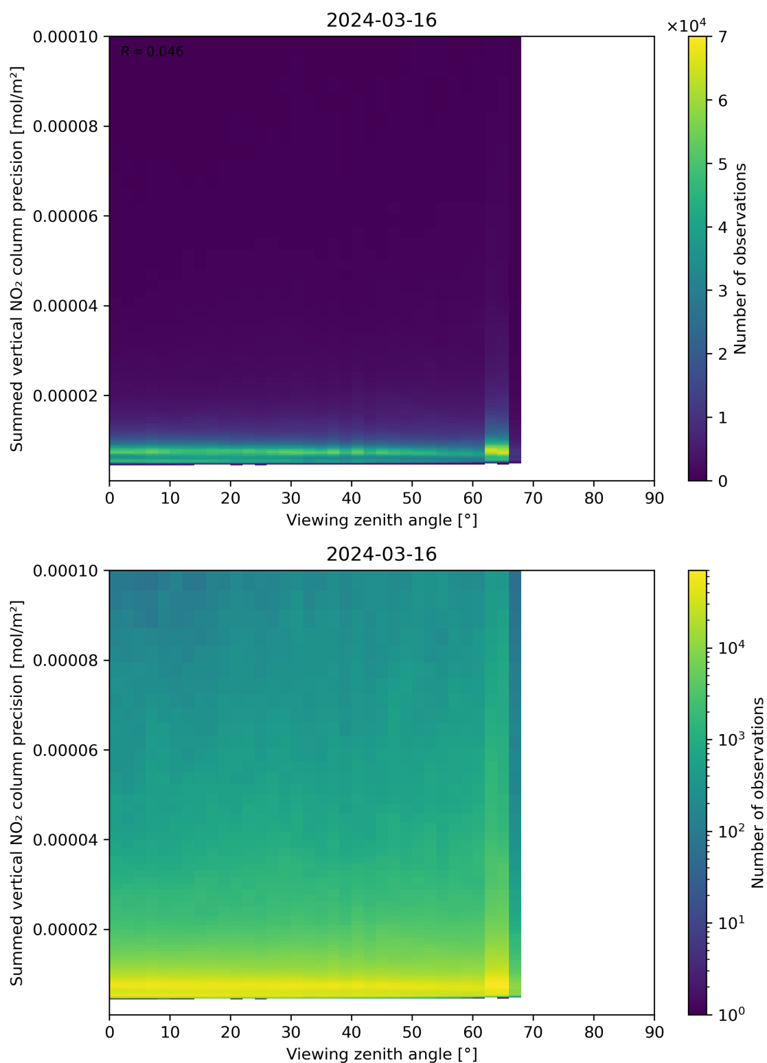
Figure 166: Scatter density plot of “Viewing zenith angle” against “Summed vertical NO 2 column precision” for 2024-03-15 to 2024-03-17.
