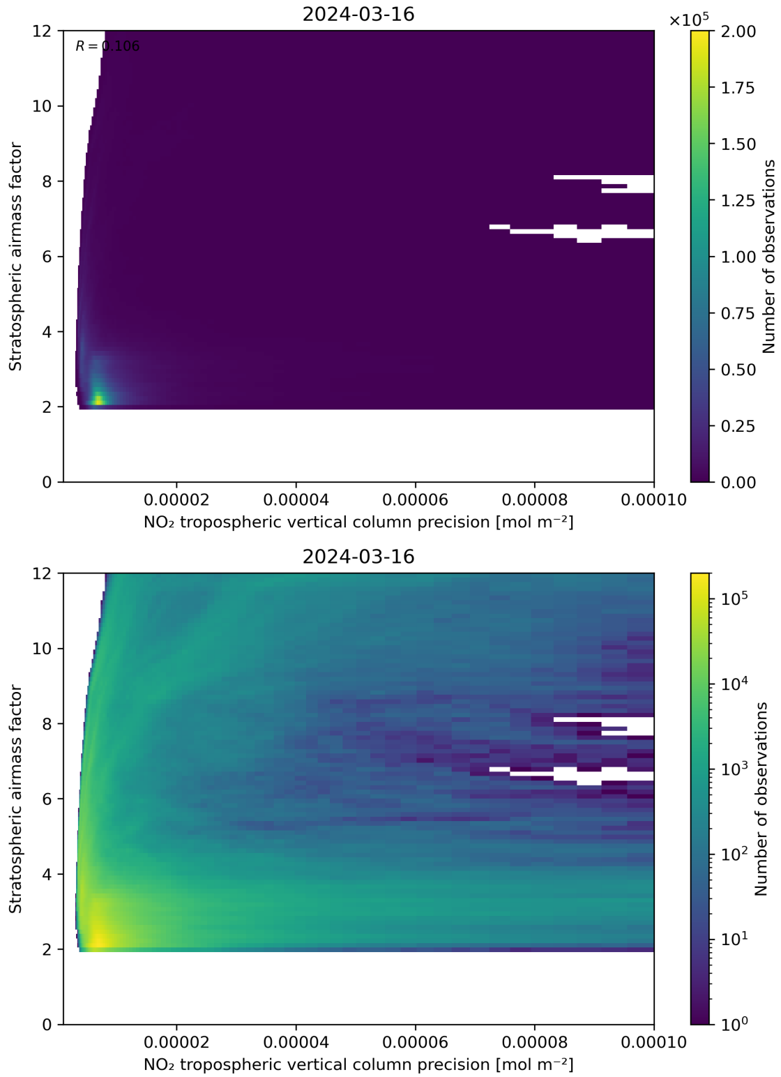
Figure 131: Scatter density plot of “NO 2 tropospheric vertical column precision” against “Stratospheric airmass factor” for 2024-03-15 to 2024-03-17.
