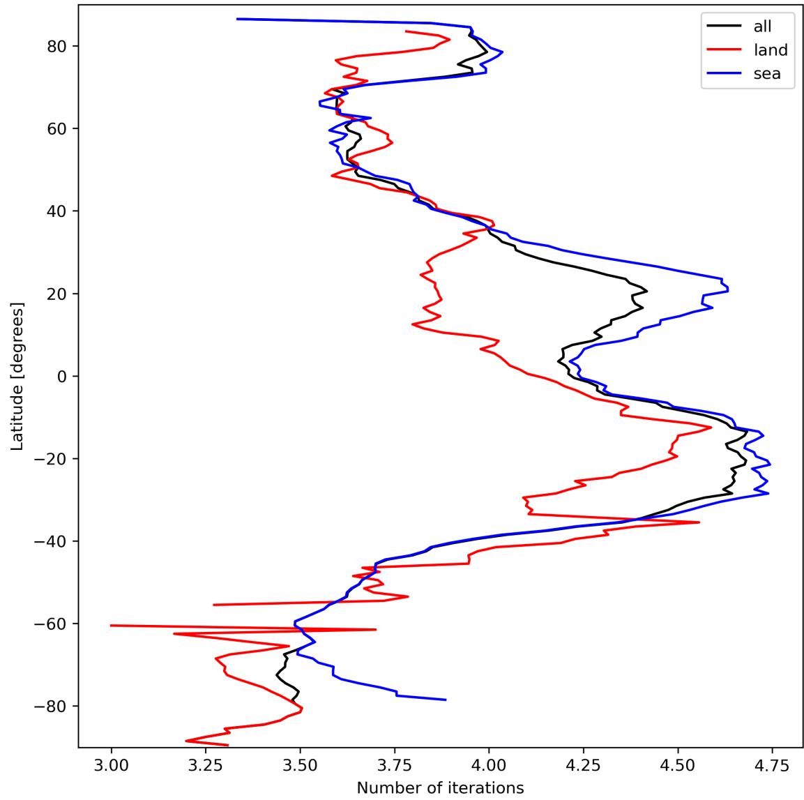
Figure 17: Zonal average of “Number of iterations” for 2024-03-15 to 2024-03-17.
