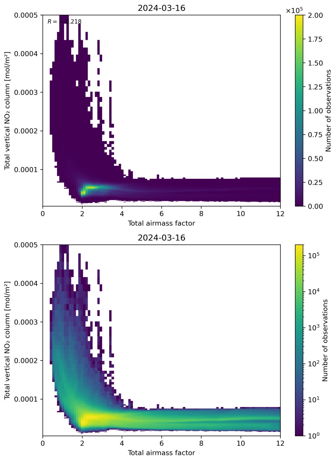
Figure 67: Scatter density plot of “Total air mass factor” against “Total vertical NO 2 column” for 2024-03-15 to 2024-03-17.
