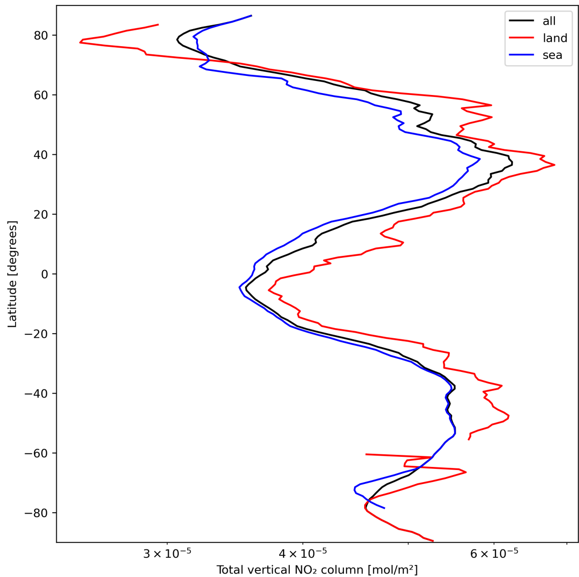
Figure 21: Zonal average of “Total vertical NO 2 column” for 2024-03-15 to 2024-03-17.
