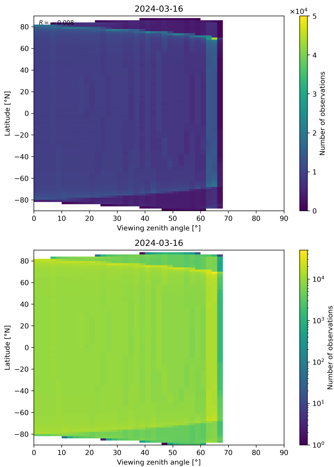
Figure 163: Scatter density plot of “Viewing zenith angle” against “Latitude” for 2024-03-15 to 2024-03-17.
