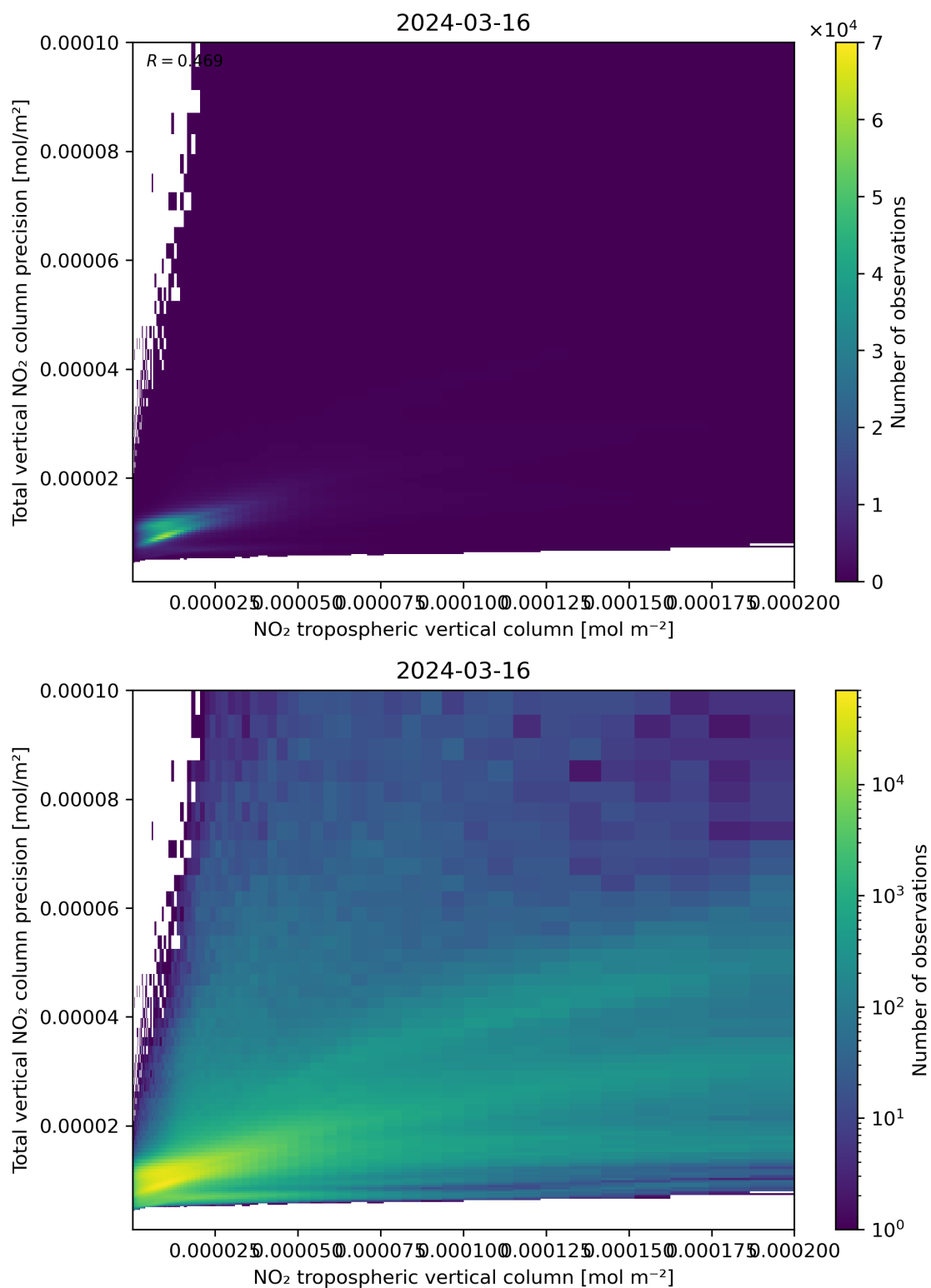
Figure 129: Scatter density plot of “NO 2 tropospheric vertical column” against “Total vertical NO 2 column precision” for 2024-03-15 to 2024-03-17.
