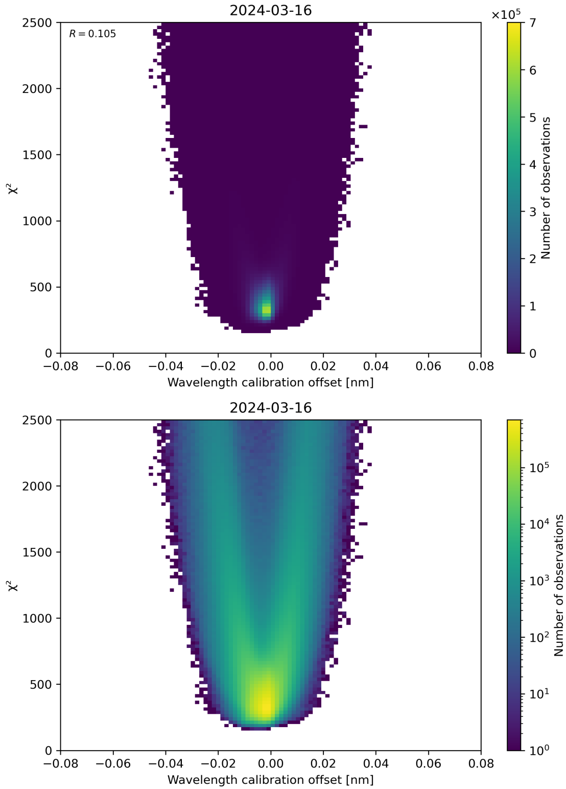
Figure 175: Scatter density plot of “Wavelength calibration offset” against “ \chi^2 ” for 2024-03-15 to 2024-03-17.
