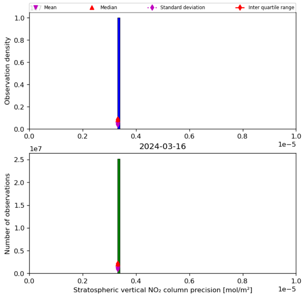
Figure 37: Histogram of “Stratospheric vertical NO 2 column precision” for 2024-03-15 to 2024-03-17
