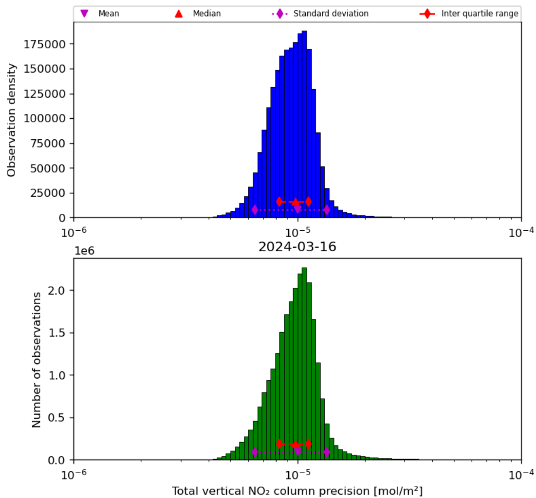
Figure 39: Histogram of "Total vertical NO 2 column precision" for 2024-03-15 to 2024-03-17
