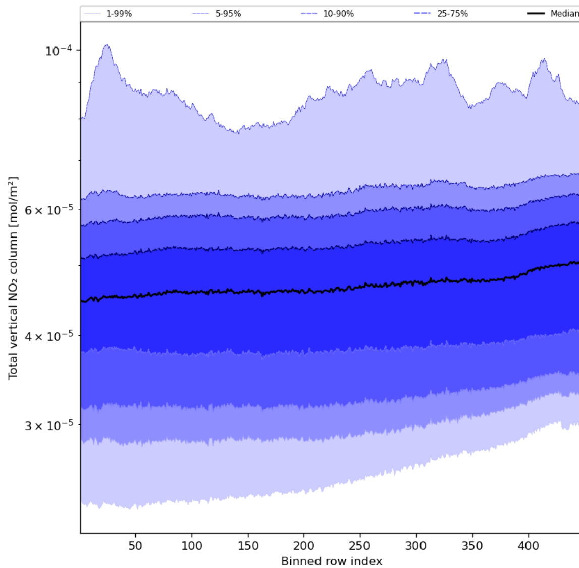
Figure 55: Along track statistics of “Total vertical NO 2 column” for 2024-03-15 to 2024-03-17
