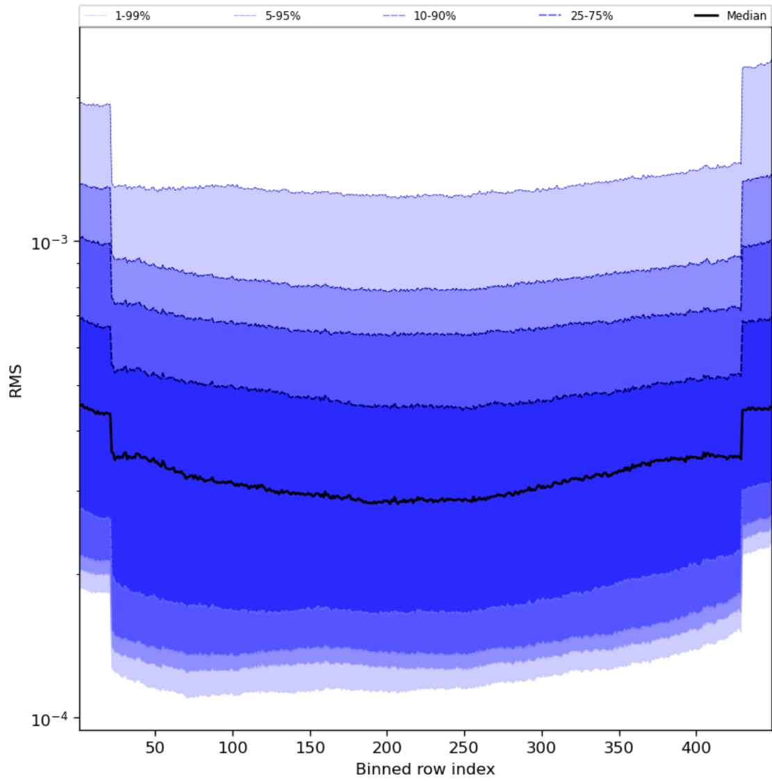
Figure 60: Along track statistics of “RMS” for 2024-03-15 to 2024-03-17
