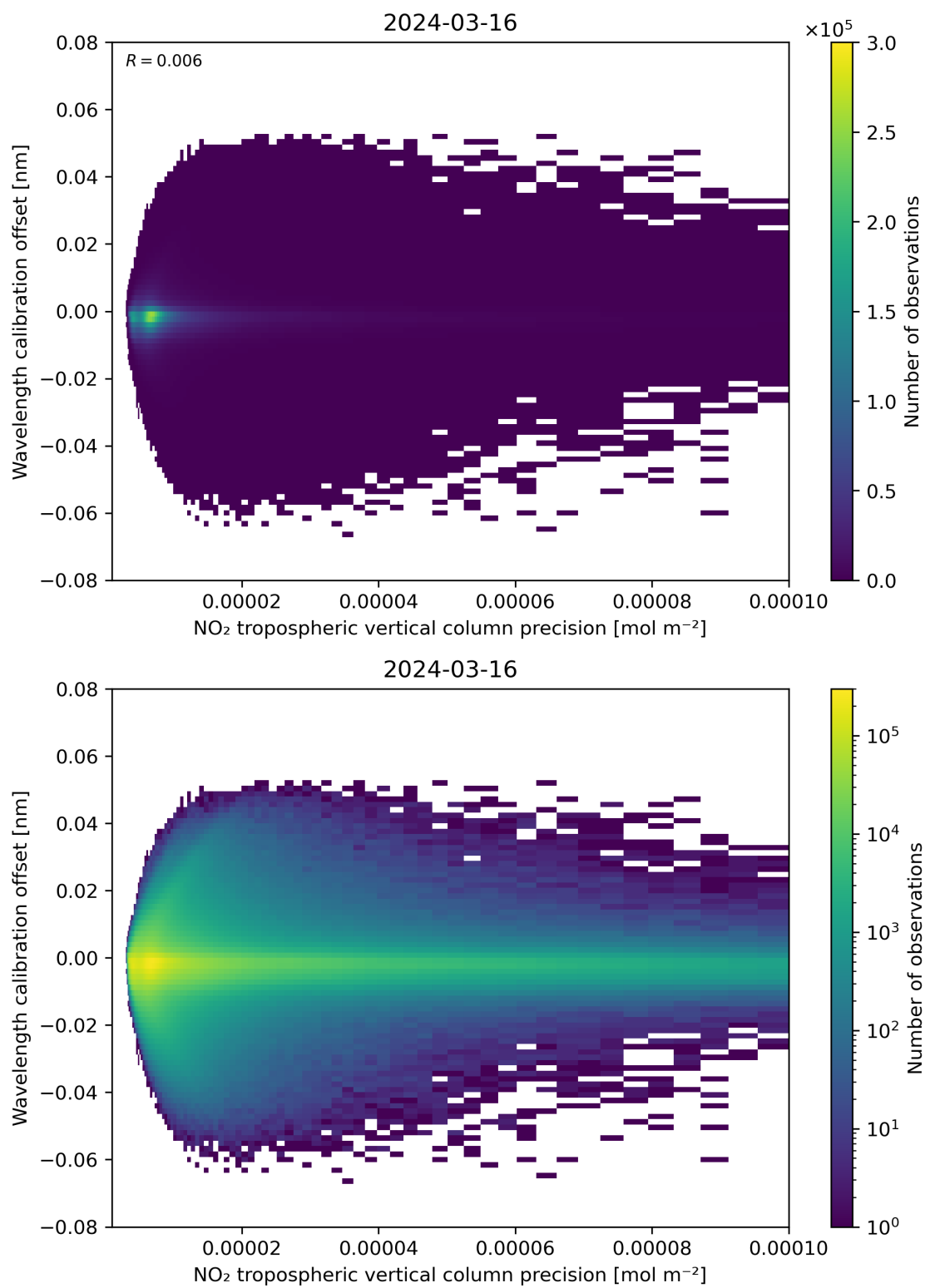
Figure 141: Scatter density plot of “NO 2 tropospheric vertical column precision” against “Wavelength calibration offset” for 2024-03-15 to 2024-03-17.
