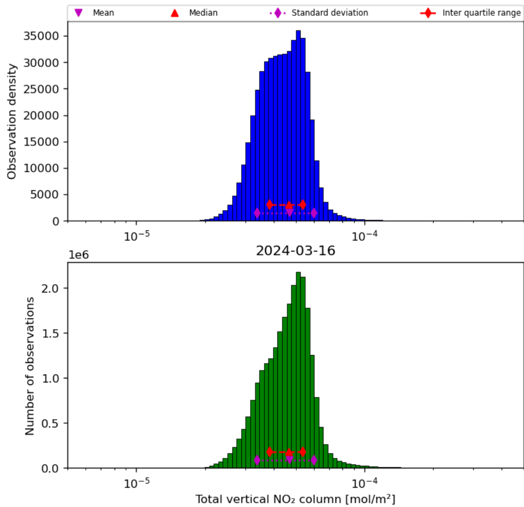
Figure 38: Histogram of “Total vertical NO 2 column” for 2024-03-15 to 2024-03-17
