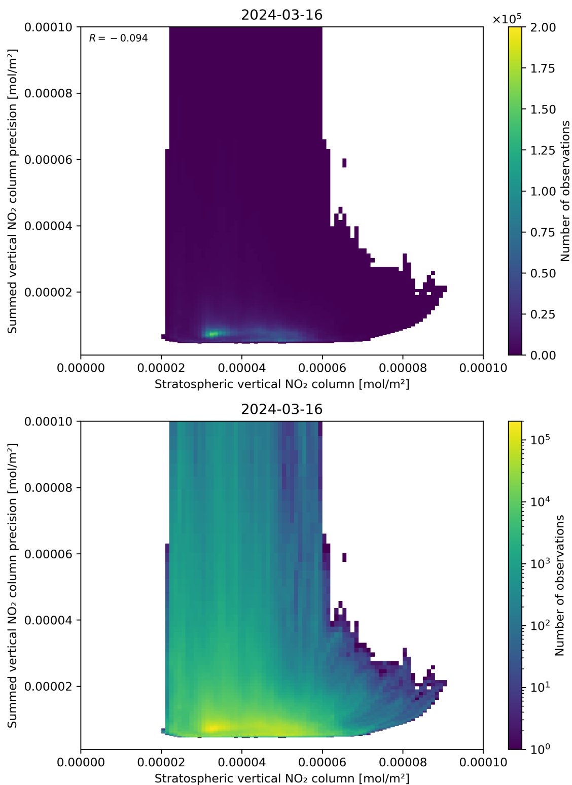
Figure 99: Scatter density plot of “Stratospheric vertical NO 2 column” against “Summed vertical NO 2 column precision” for 2024-03-15 to 2024-03-17.
