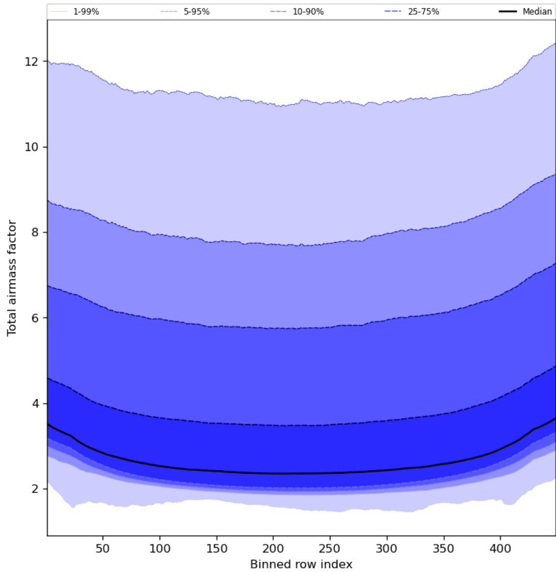
Figure 49: Along track statistics of “Total airmass factor” for 2024-03-15 to 2024-03-17
