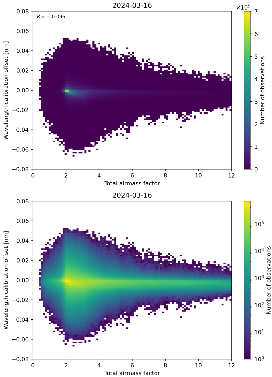
Figure 70: Scatter density plot of “Total airmass factor” against “Wavelength calibration offset” for 2024-03-15 to 2024-03-17.
