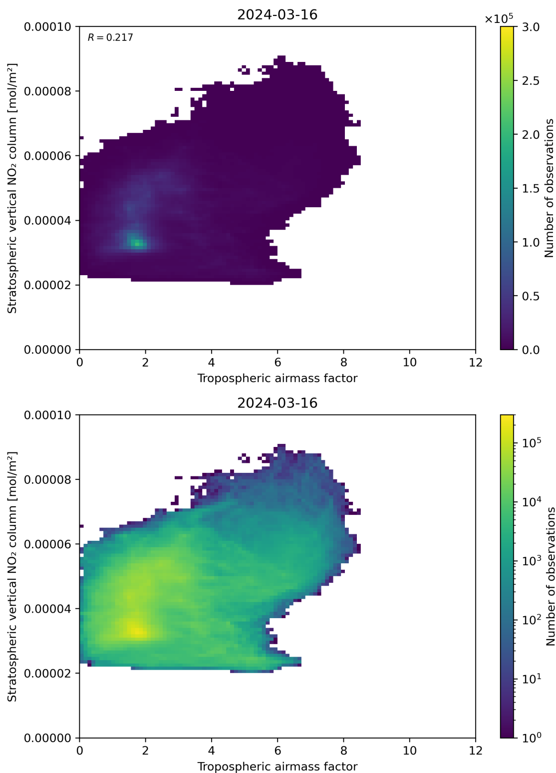
Figure 74: Scatter density plot of “Tropospheric air mass factor” against “Stratospheric vertical NO 2 column” for 2024-03-15 to 2024-03-17.
