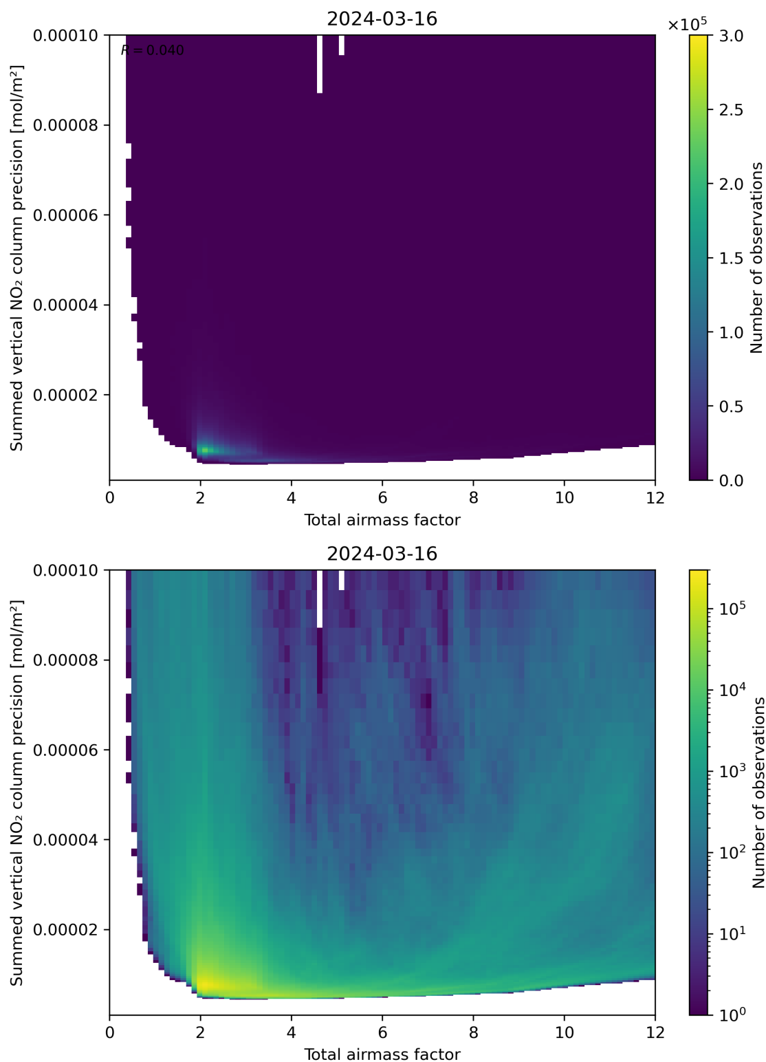
Figure 66: Scatter density plot of “Total airmass factor” against “Summed vertical NO 2 column precision” for 2024-03-15 to 2024-03-17.
