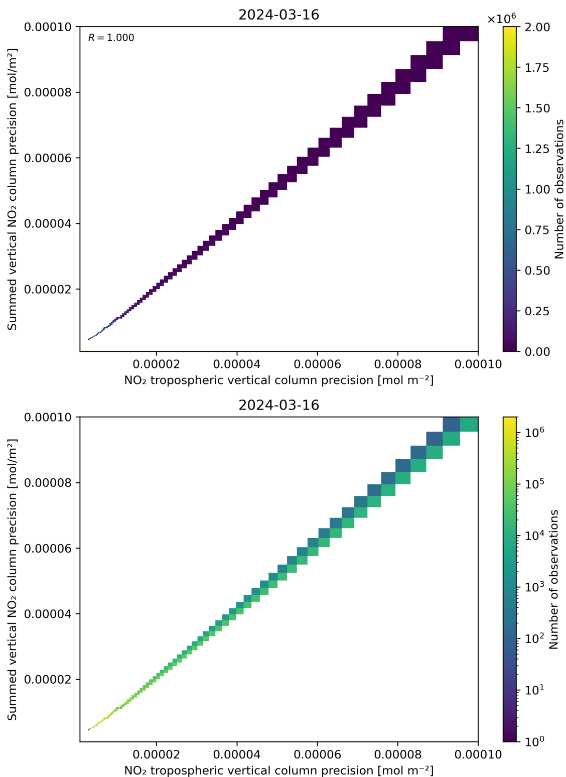
Figure 137: Scatter density plot of “NO 2 tropospheric vertical column precision” against “Summed vertical NO 2 column precision” for 2024-03-15 to 2024-03-17.
