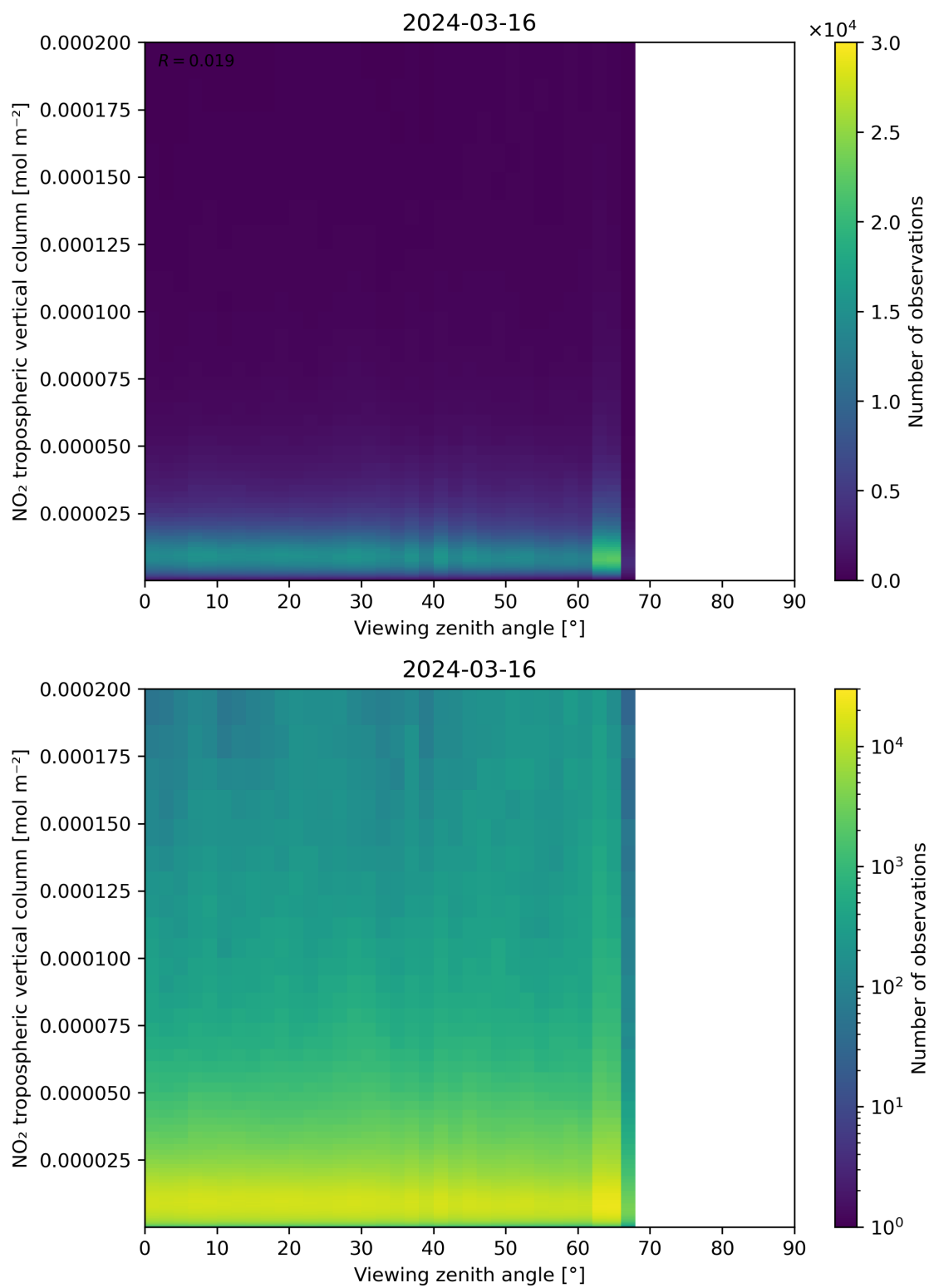
Figure 169: Scatter density plot of “Viewing zenith angle” against “NO 2 tropospheric vertical column” for 2024-03-15 to 2024-03-17.
