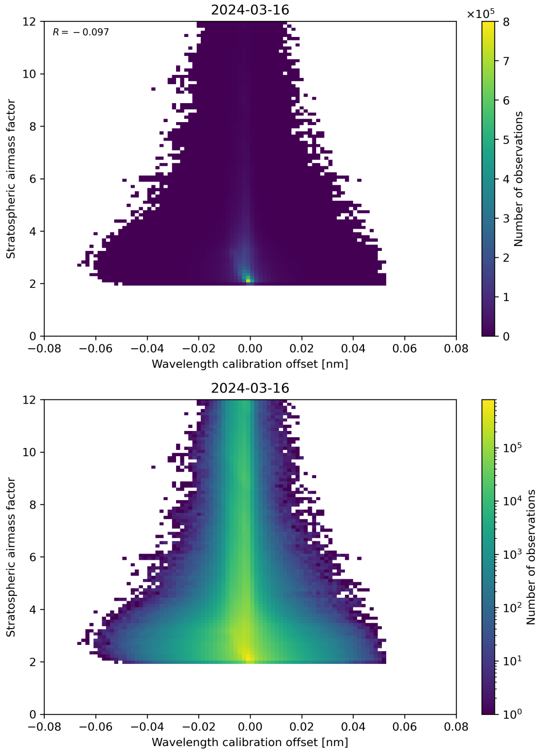
Figure 174: Scatter density plot of “Wavelength calibration offset” against “Stratospheric airmass factor” for 2024-03-15 to 2024-03-17.
