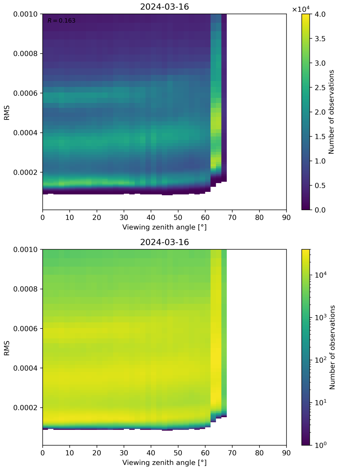
Figure 171: Scatter density plot of “Viewing zenith angle” against “RMS” for 2024-03-15 to 2024-03-17.
