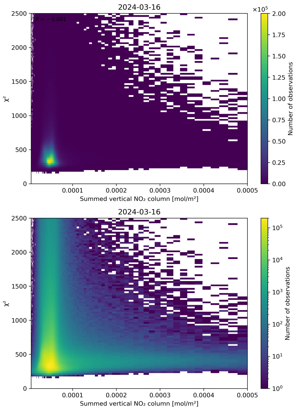
Figure 104: Scatter density plot of “Summed vertical NO 2 column” against “ \chi^2 ” for 2024-03-15 to 2024-03-17.
