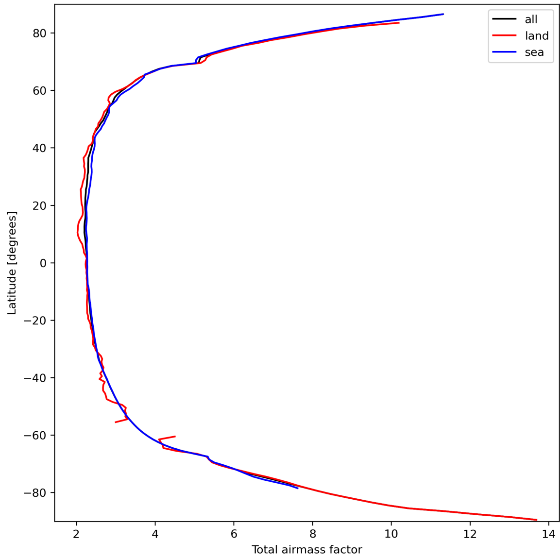
Figure 15: Zonal average of “Total airmass factor” for 2024-03-15 to 2024-03-17.
