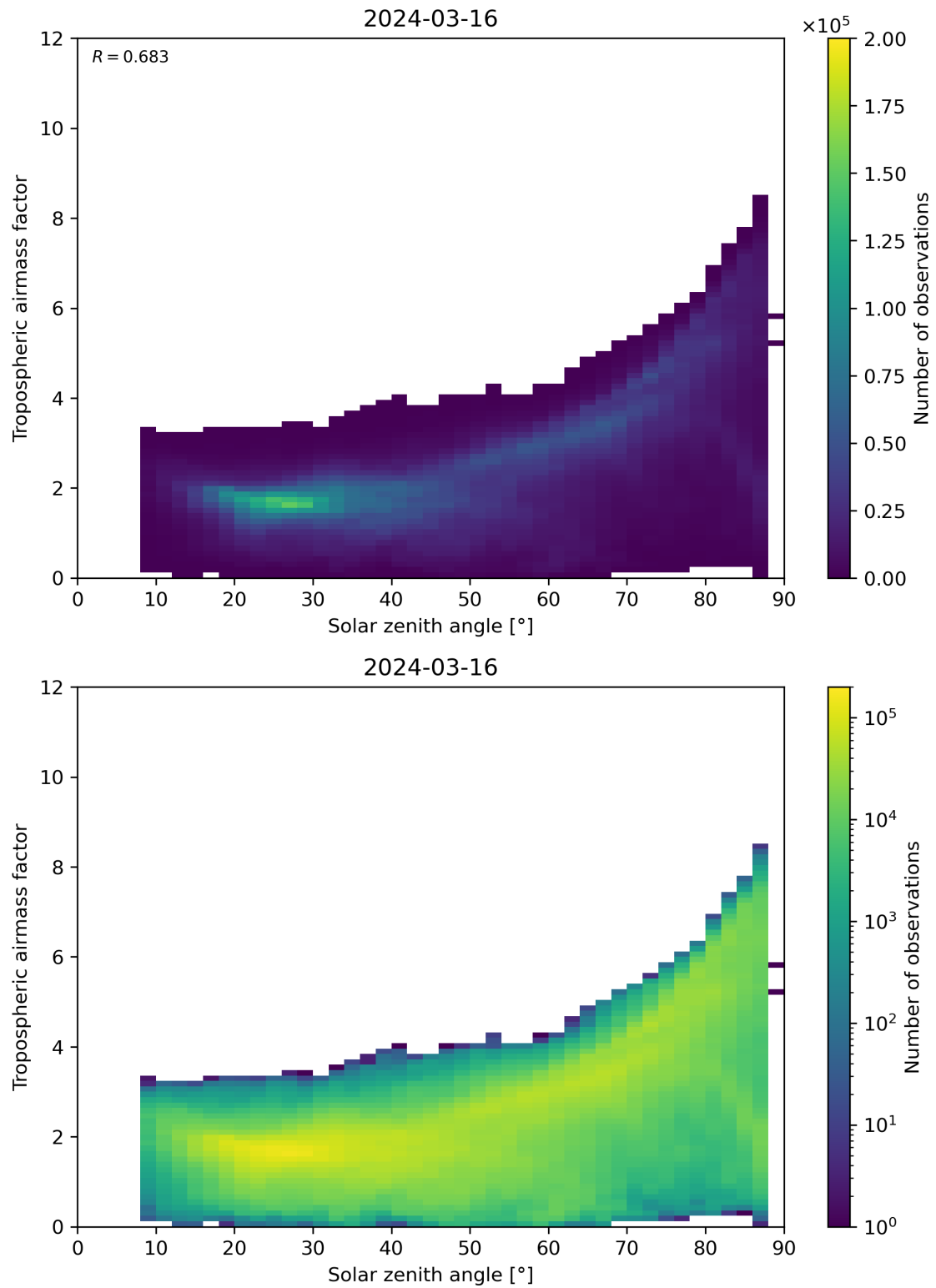
Figure 147: Scatter density plot of “Solar zenith angle” against “Tropospheric airmass factor” for 2024-03-15 to 2024-03-17.
