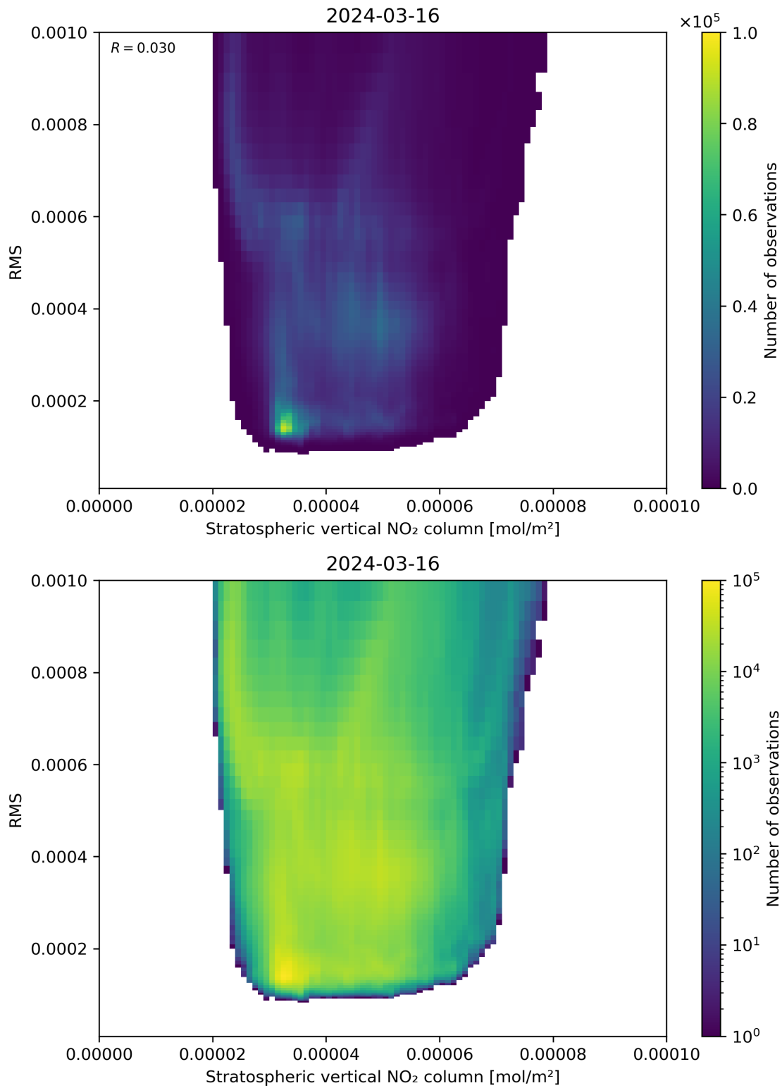
Figure 102: Scatter density plot of “Stratospheric vertical NO 2 column” against “RMS” for 2024-03-15 to 2024-03-17.
