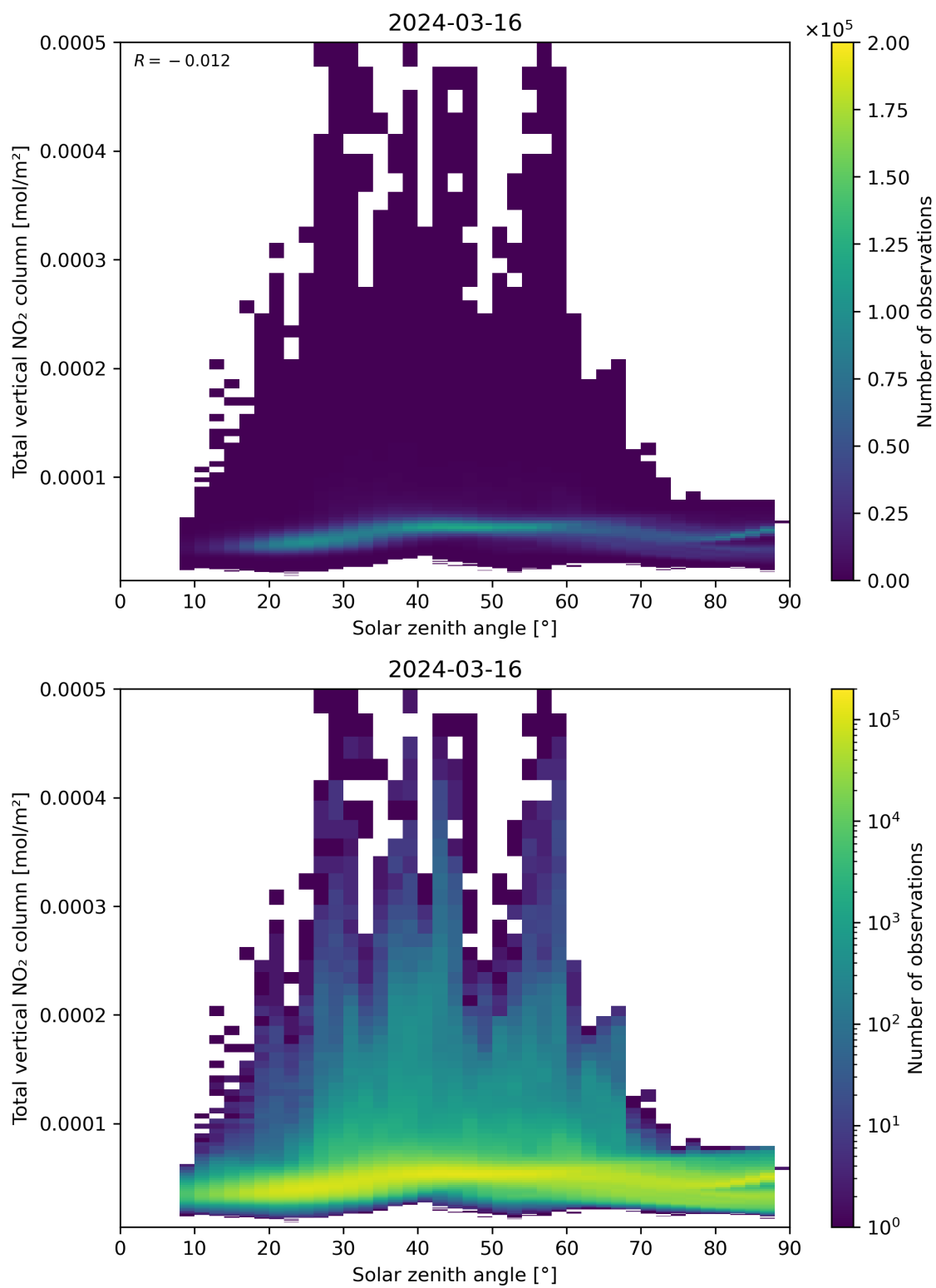
Figure 153: Scatter density plot of “Solar zenith angle” against “Total vertical NO 2 column” for 2024-03-15 to 2024-03-17.
