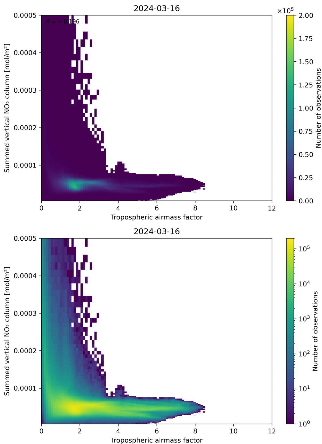
Figure 75: Scatter density plot of “Tropospheric airmass factor” against “Summed vertical NO 2 column” for 2024-03-15 to 2024-03-17.
