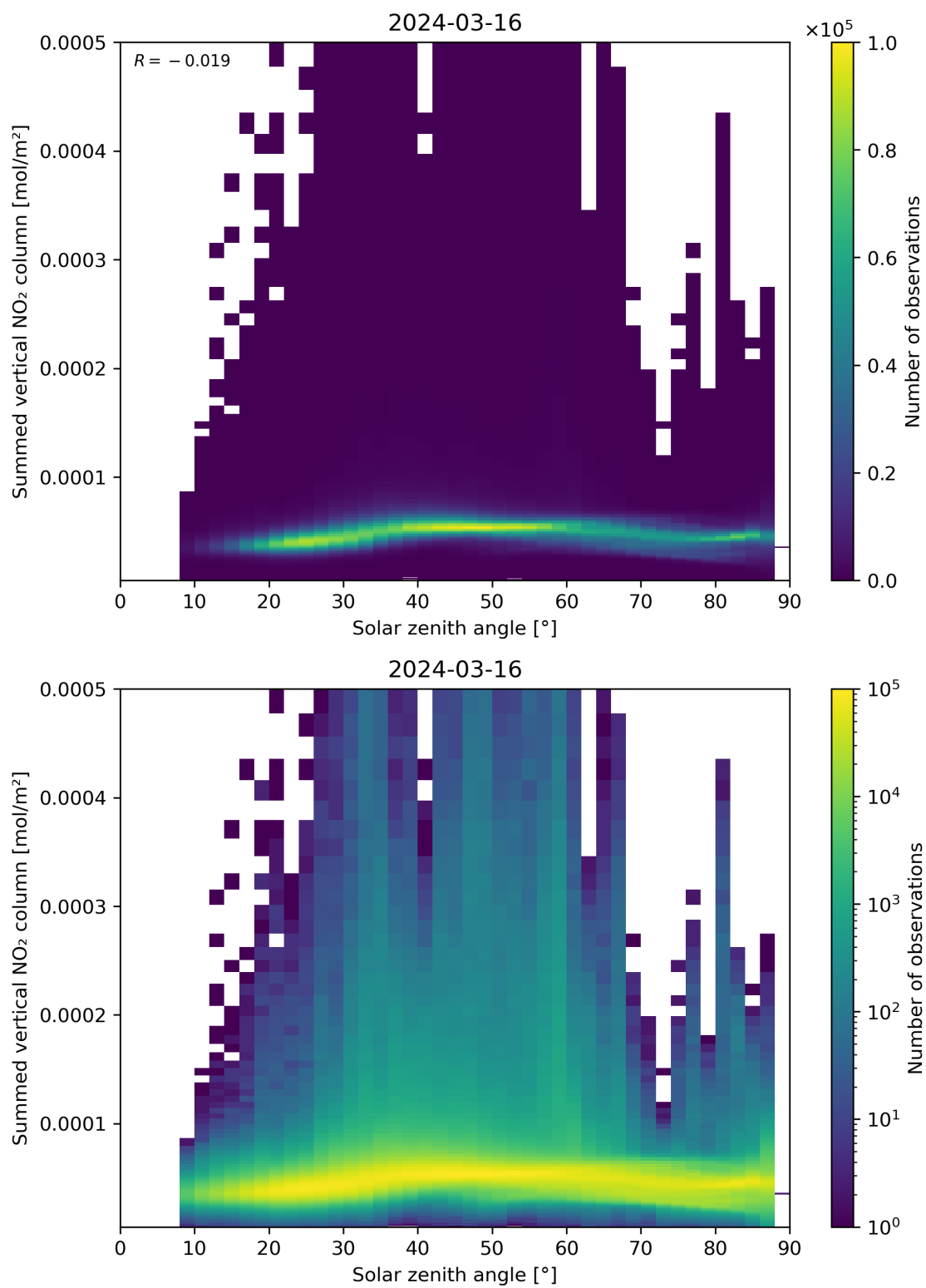
Figure 151: Scatter density plot of “Solar zenith angle” against “Summed vertical NO 2 column” for 2024-03-15 to 2024-03-17.
