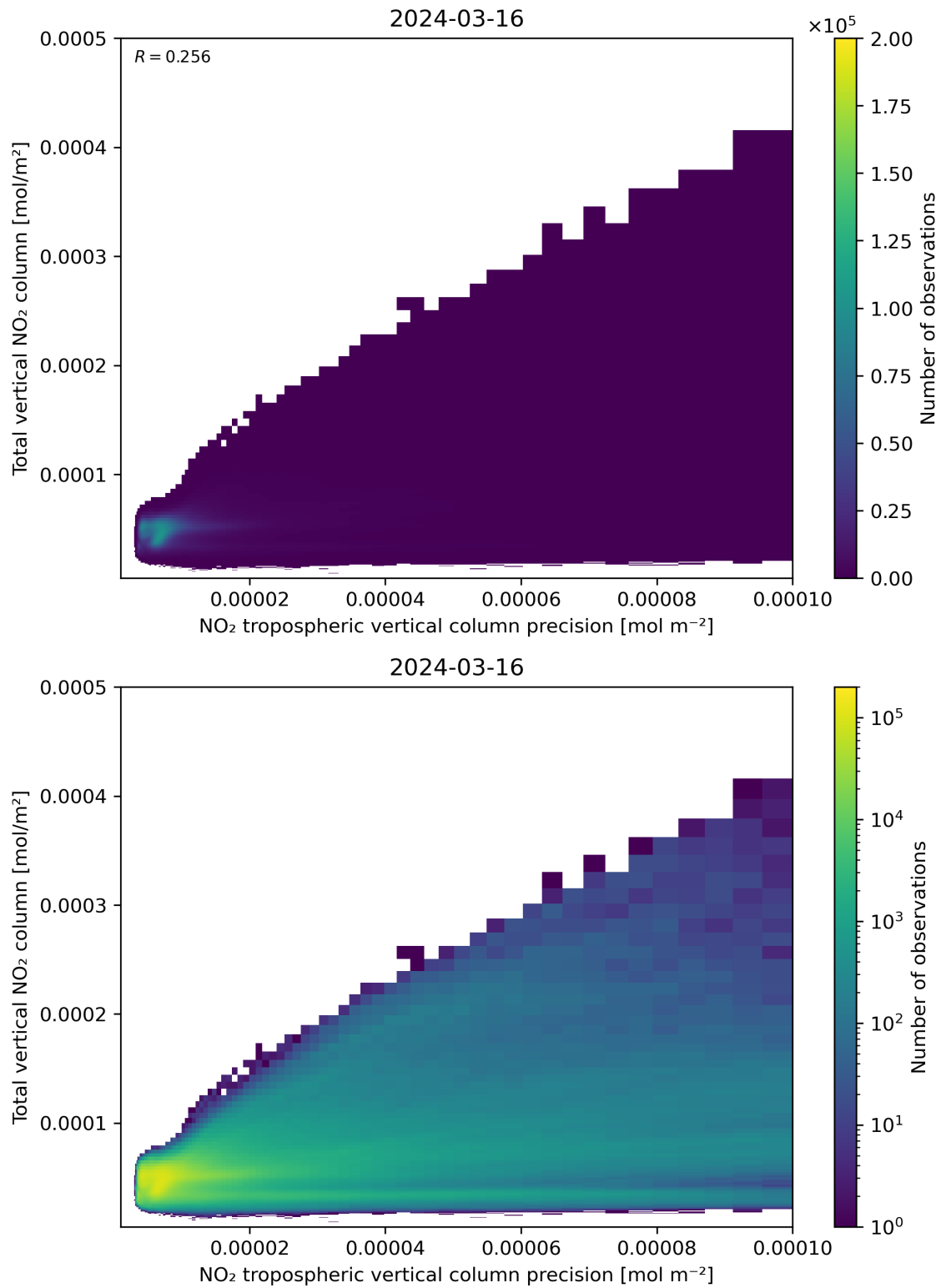
Figure 138: Scatter density plot of “NO 2 tropospheric vertical column precision” against “Total vertical NO 2 column” for 2024-03-15 to 2024-03-17.
