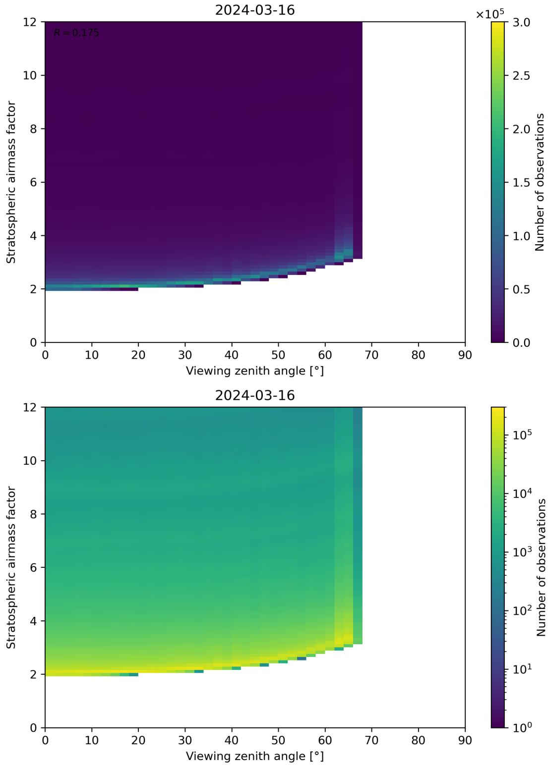
Figure 159: Scatter density plot of “Viewing zenith angle” against “Stratospheric airmass factor” for 2024-03-15 to 2024-03-17.
