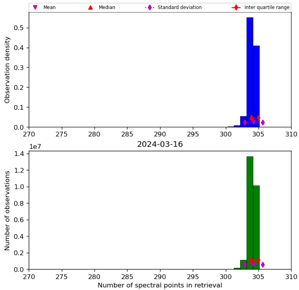
Figure 33: Histogram of “Number of spectral points in retrieval” for 2024-03-15 to 2024-03-17
