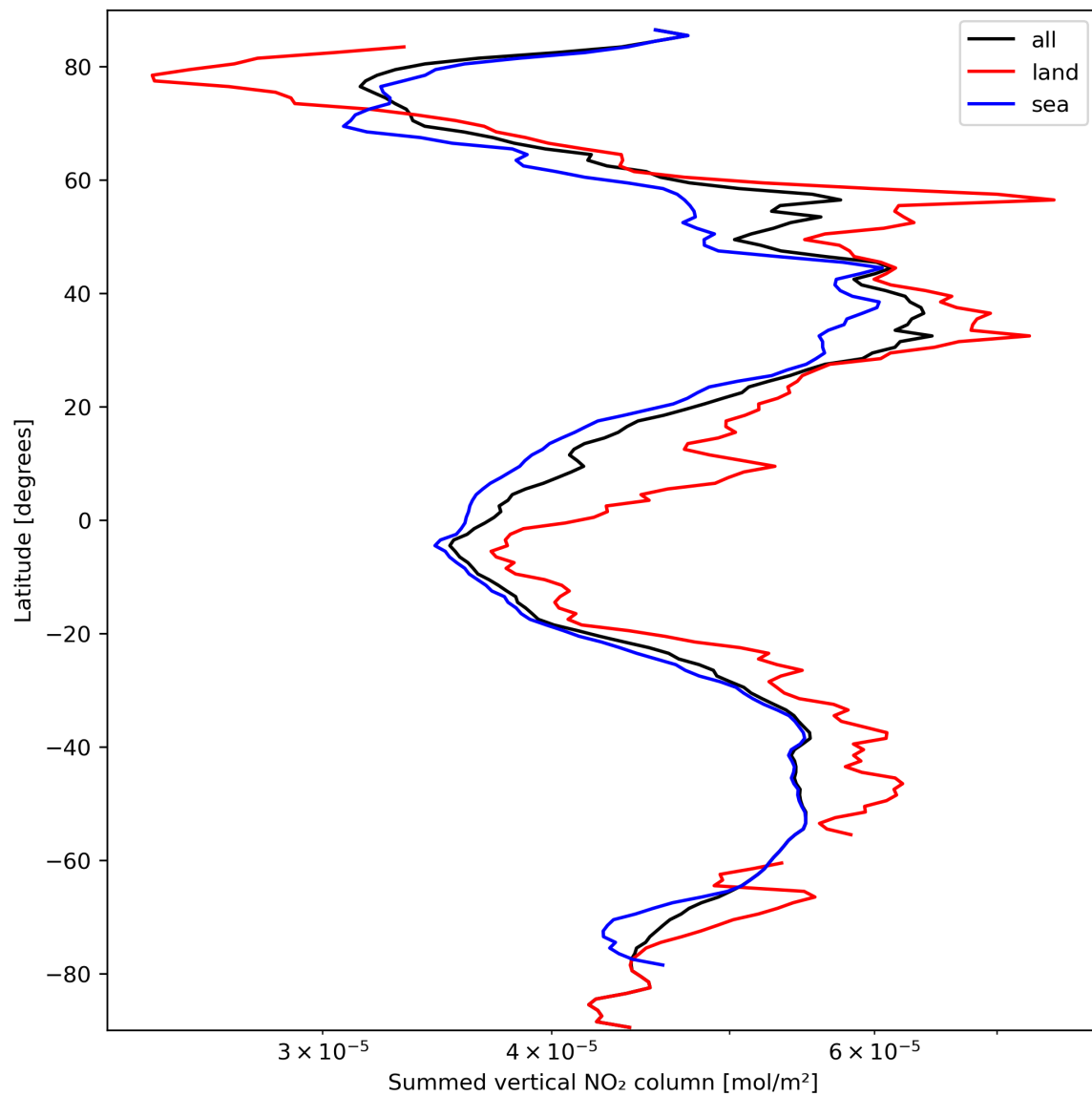
Figure 23: Zonal average of “Summed vertical NO 2 column” for 2024-03-15 to 2024-03-17.
