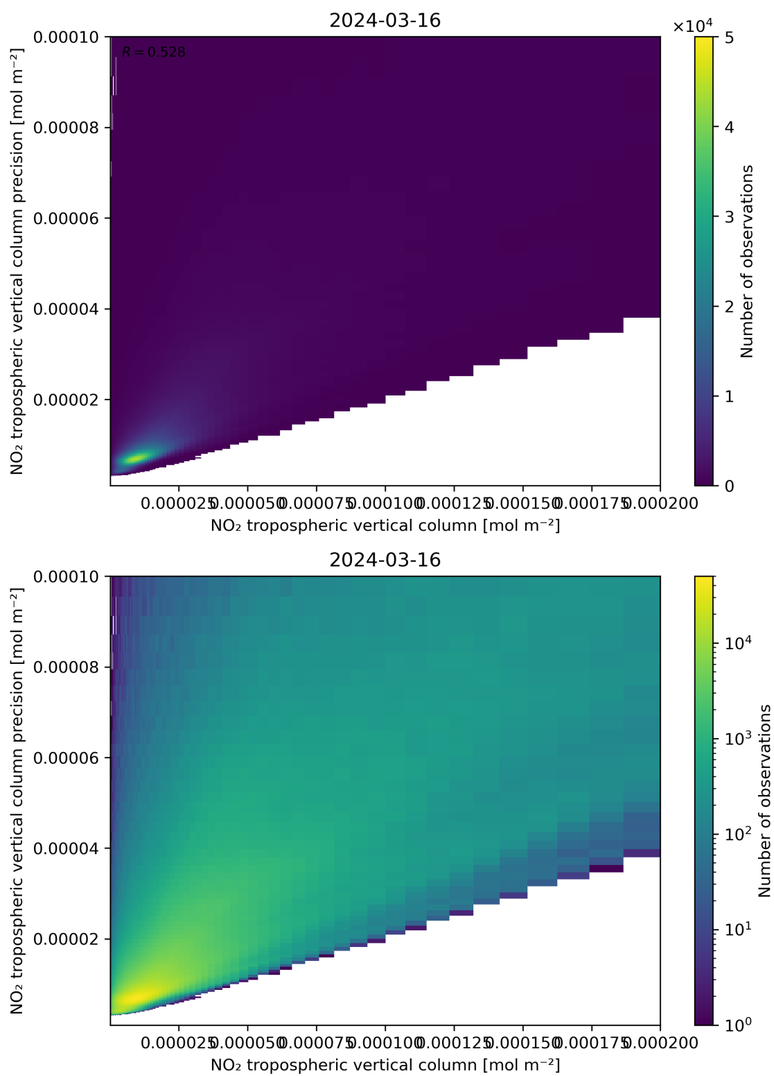
Figure 130: Scatter density plot of “NO 2 tropospheric vertical column” against “NO 2 tropospheric vertical column precision” for 2024-03-15 to 2024-03-17.
