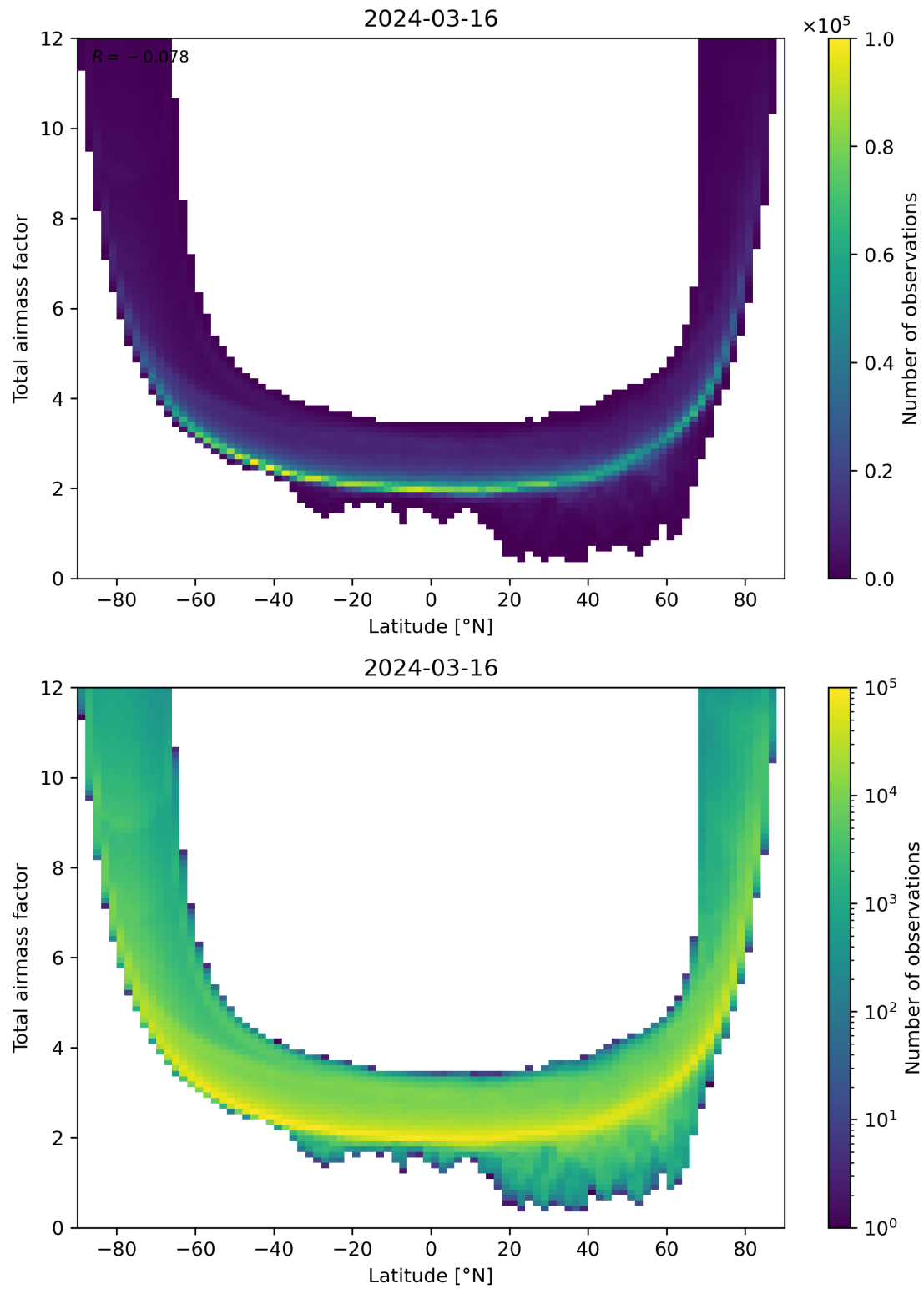
Figure 84: Scatter density plot of “Latitude” against “Total airmass factor” for 2024-03-15 to 2024-03-17.
