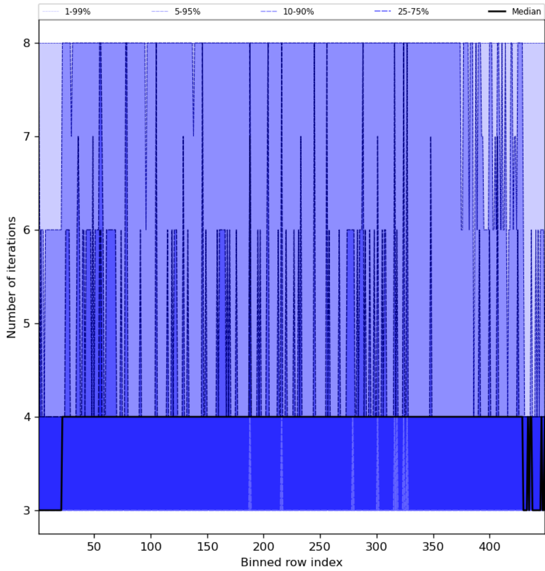
Figure 51: Along track statistics of “Number of iterations” for 2024-03-15 to 2024-03-17
