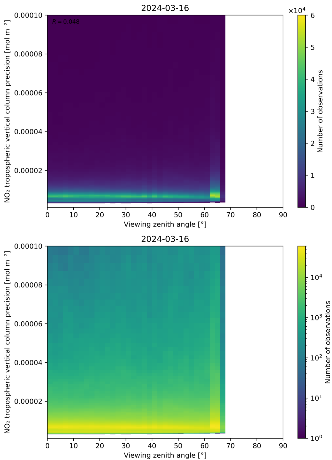
Figure 170: Scatter density plot of “Viewing zenith angle” against “NO 2 tropospheric vertical column precision” for 2024-03-15 to 2024-03-17.
