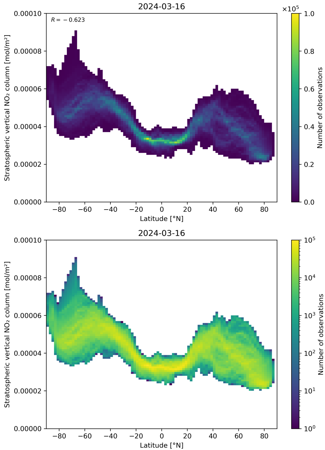
Figure 87: Scatter density plot of “Latitude” against “Stratospheric vertical NO 2 column” for 2024-03-15 to 2024-03-17.
