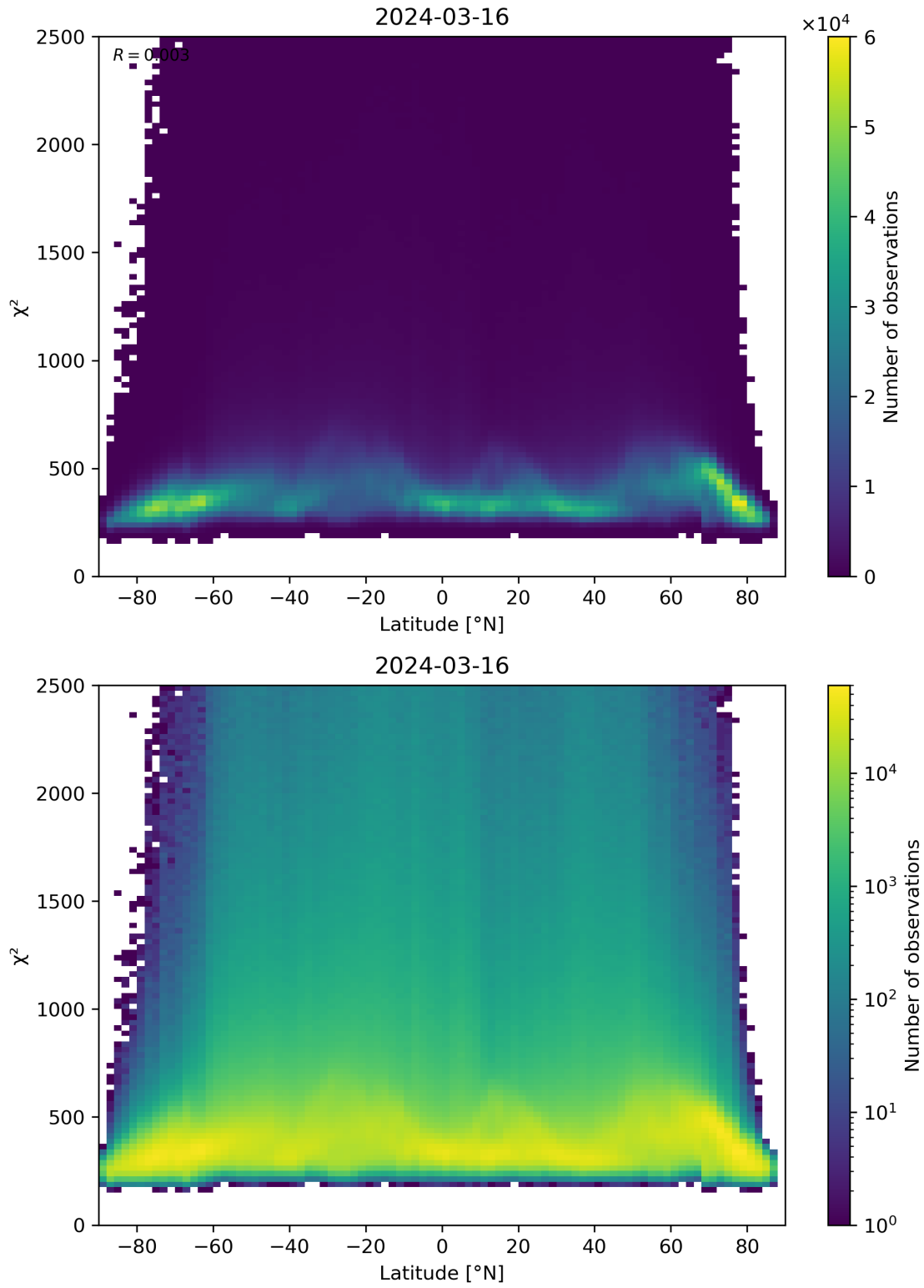
Figure 86: Scatter density plot of “Latitude” against “ \chi^2 ” for 2024-03-15 to 2024-03-17.
