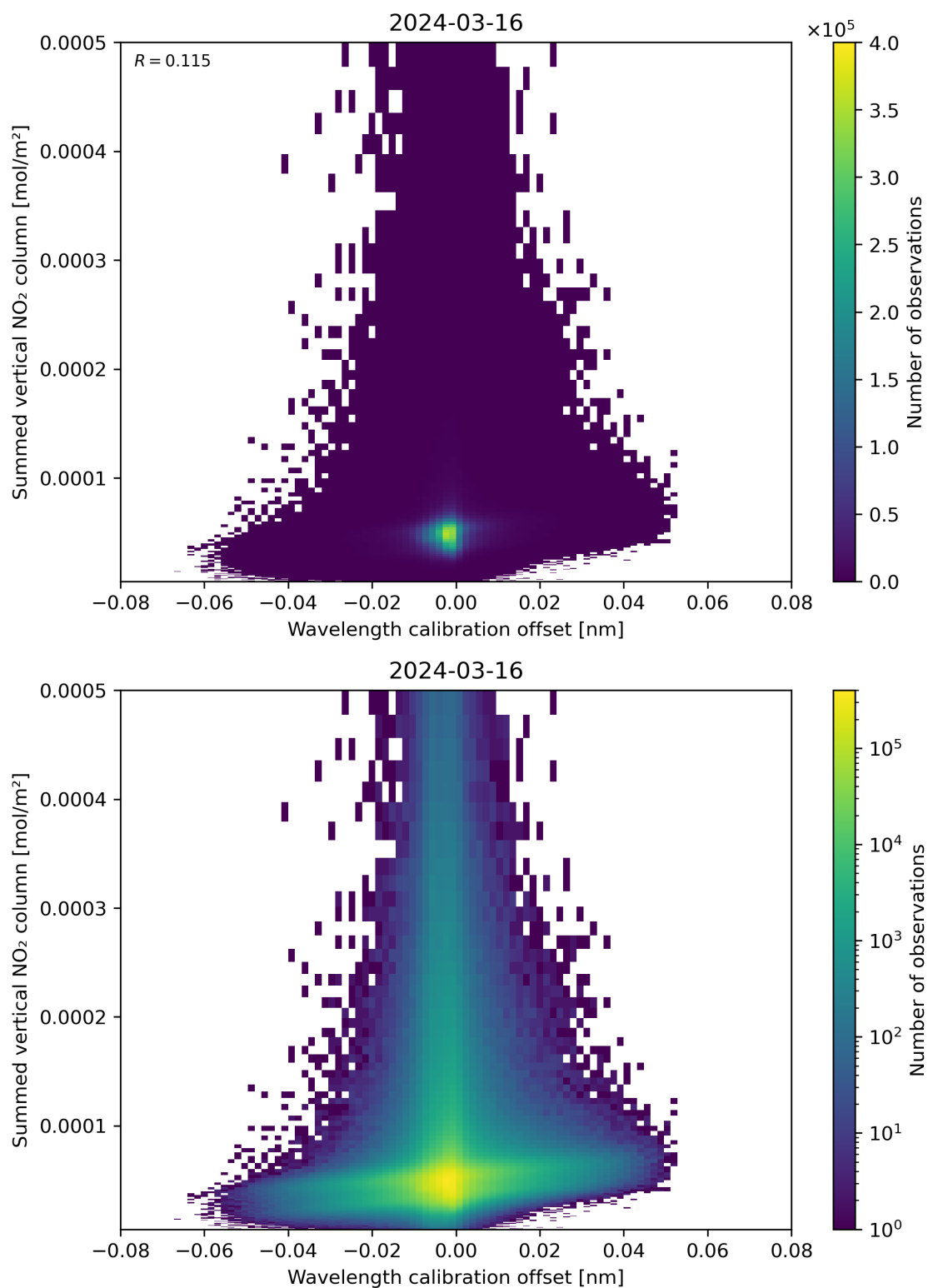
Figure 177: Scatter density plot of “Wavelength calibration offset” against “Summed vertical NO 2 column” for 2024-03-15 to 2024-03-17.
