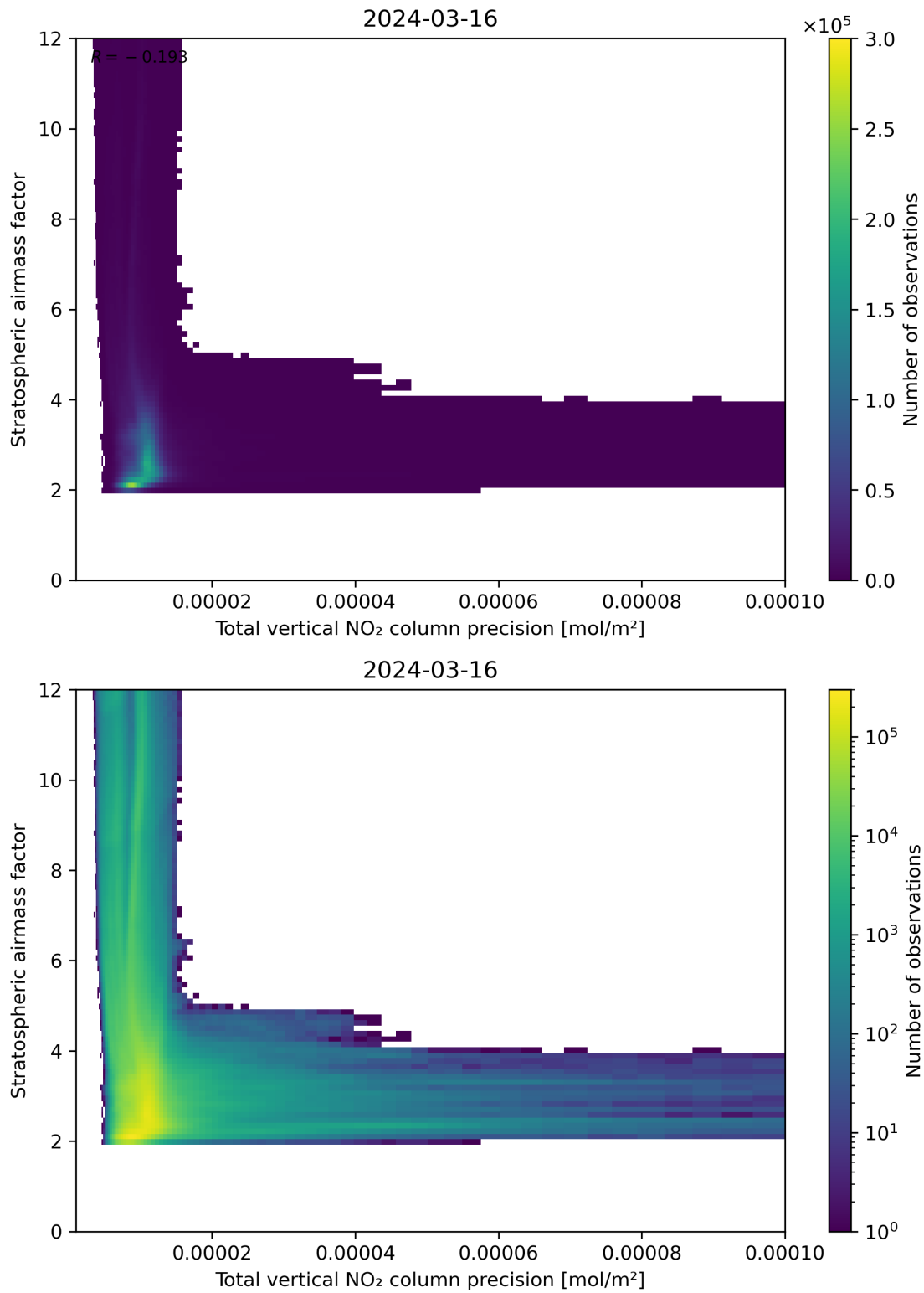
Figure 115: Scatter density plot of “Total vertical NO 2 column precision” against “Stratospheric air mass factor” for 2024-03-15 to 2024-03-17.
