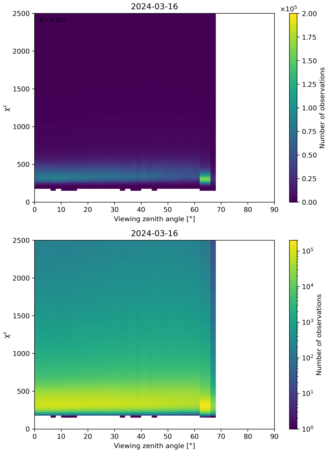
Figure 162: Scatter density plot of “Viewing zenith angle” against “ \chi^2 ” for 2024-03-15 to 2024-03-17.
