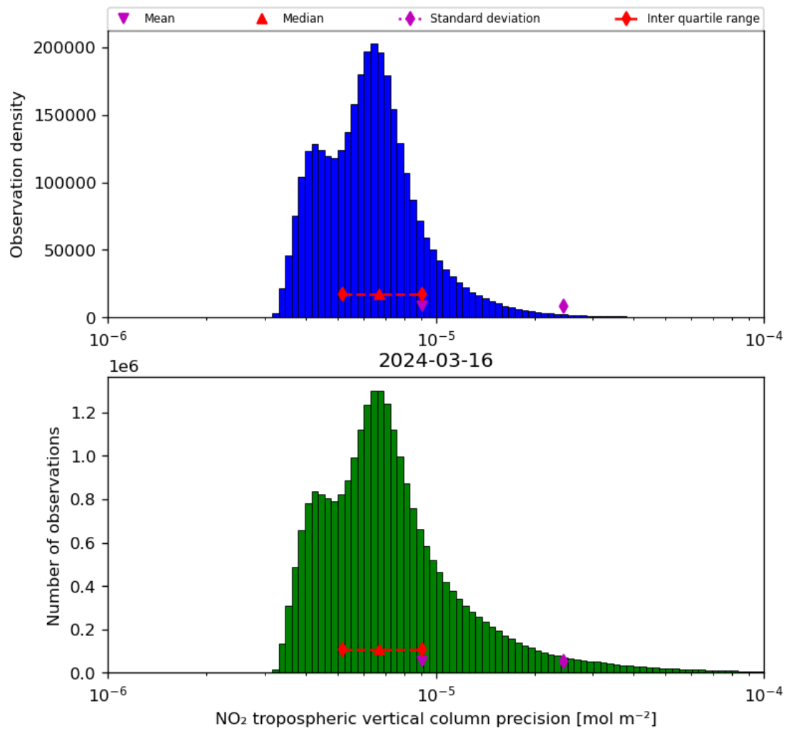
Figure 30: Histogram of “NO 2 tropospheric vertical column precision” for 2024-03-15 to 2024-03-17
