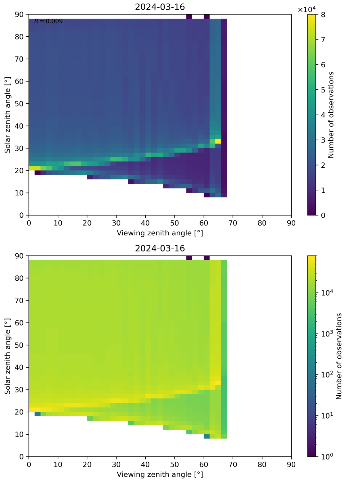
Figure 172: Scatter density plot of “Viewing zenith angle” against “Solar zenith angle” for 2024-03-15 to 2024-03-17.
