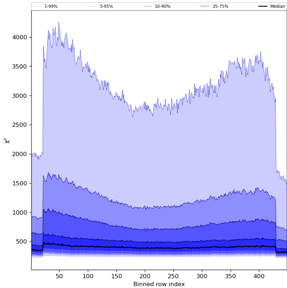
Figure 59: Along track statistics of “ \chi^2 ” for 2024-03-15 to 2024-03-17
