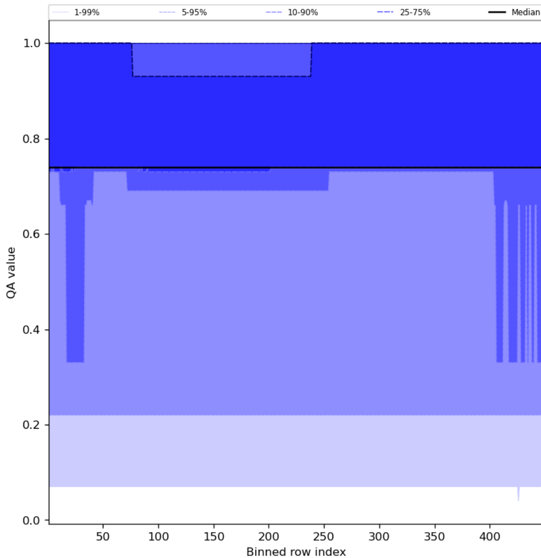
Figure 45: Along track statistics of “QA value” for 2024-03-15 to 2024-03-17
