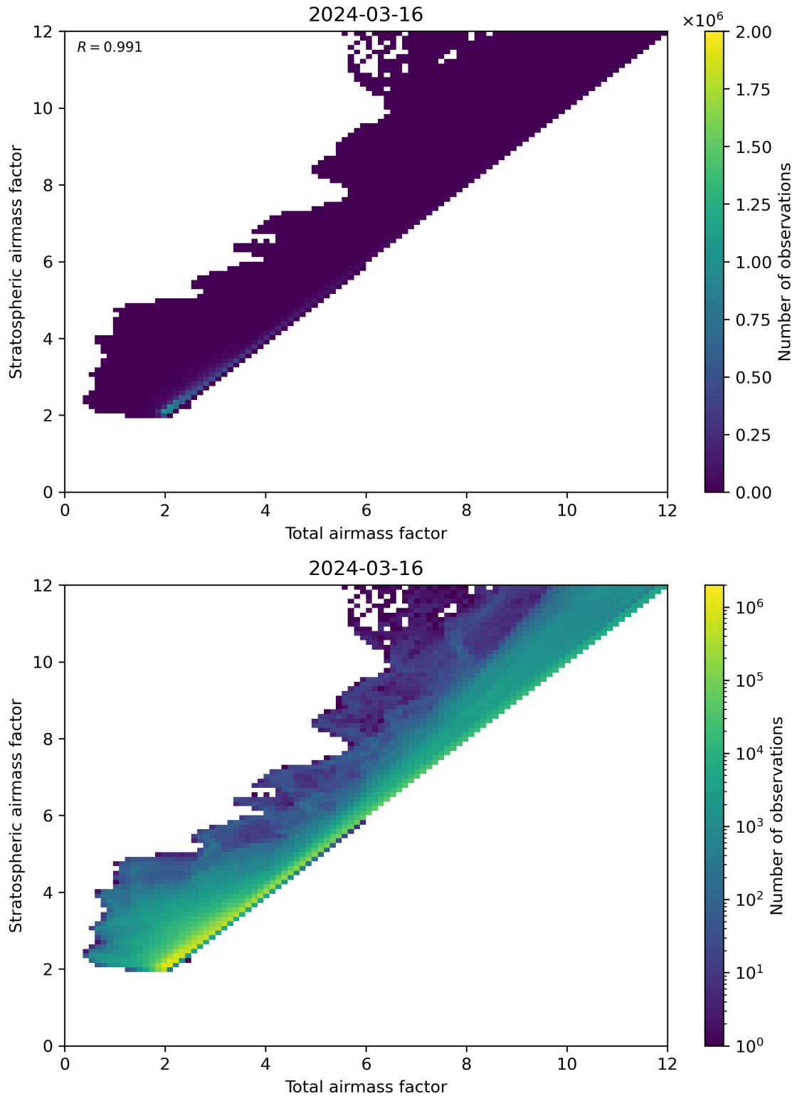
Figure 62: Scatter density plot of “Total airmass factor” against “Stratospheric airmass factor” for 2024-03-15 to 2024-03-17.
