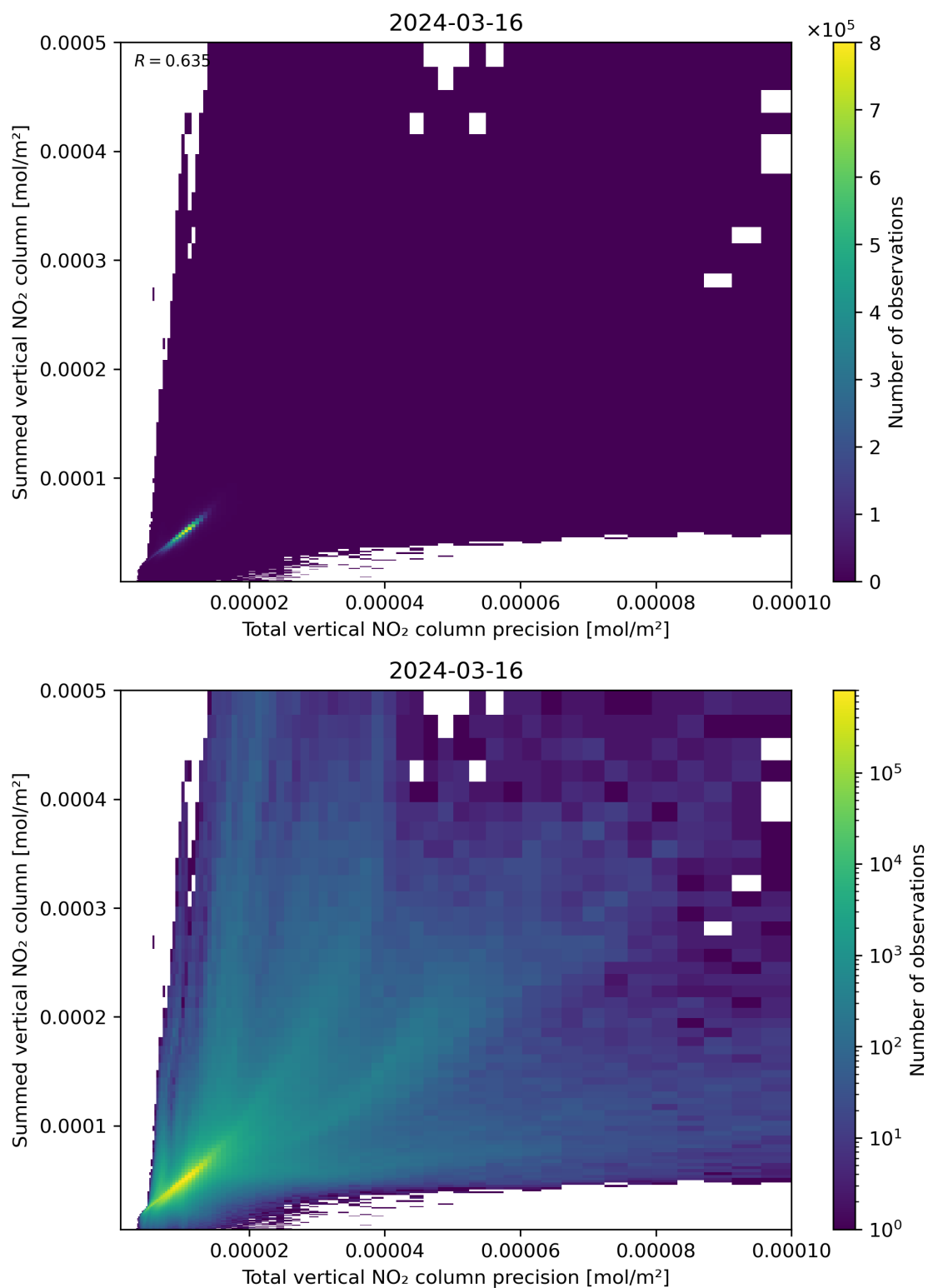
Figure 117: Scatter density plot of “Total vertical NO 2 column precision” against “Summed vertical NO 2 column” for 2024-03-15 to 2024-03-17.
