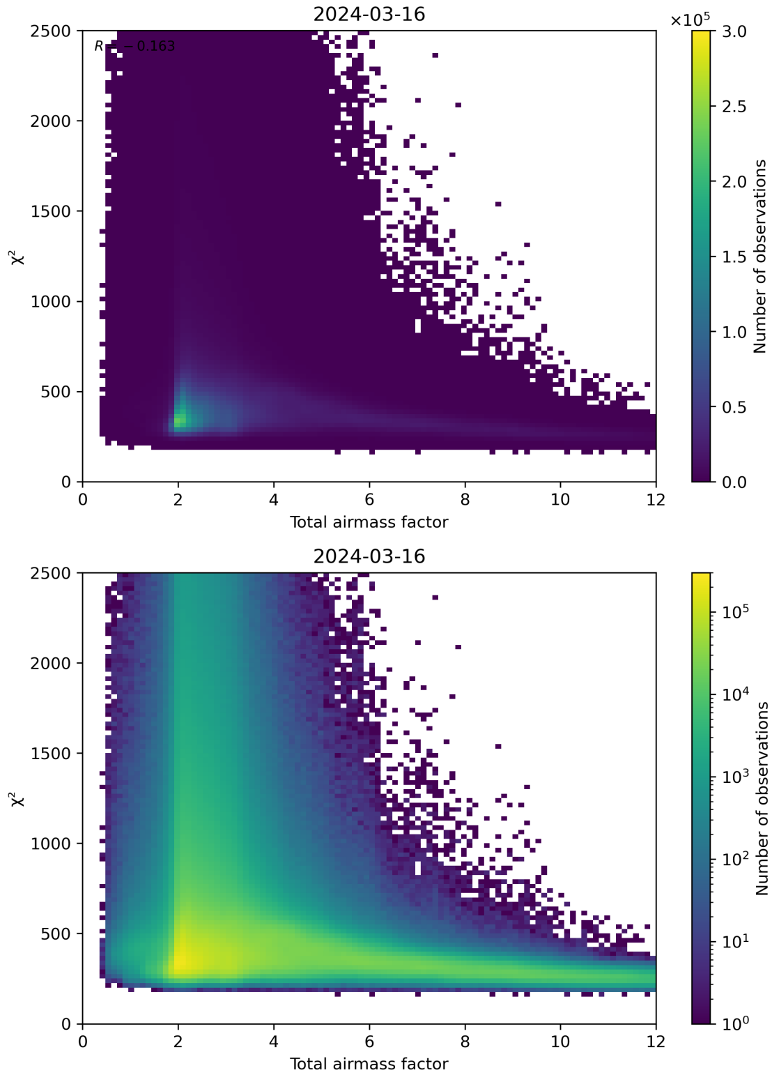
Figure 63: Scatter density plot of “Total airmass factor” against “ \chi^2 ” for 2024-03-15 to 2024-03-17.
