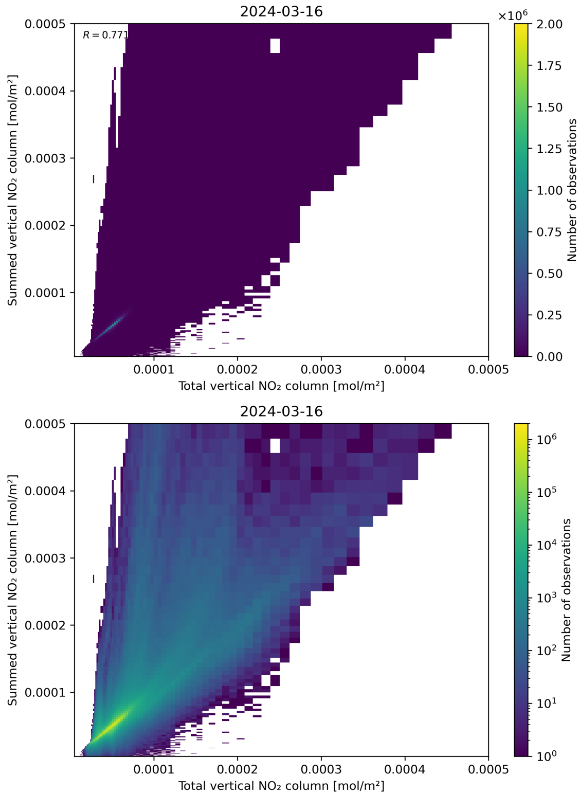
Figure 112: Scatter density plot of “Total vertical NO 2 column” against “Summed vertical NO 2 column” for 2024-03-15 to 2024-03-17.
