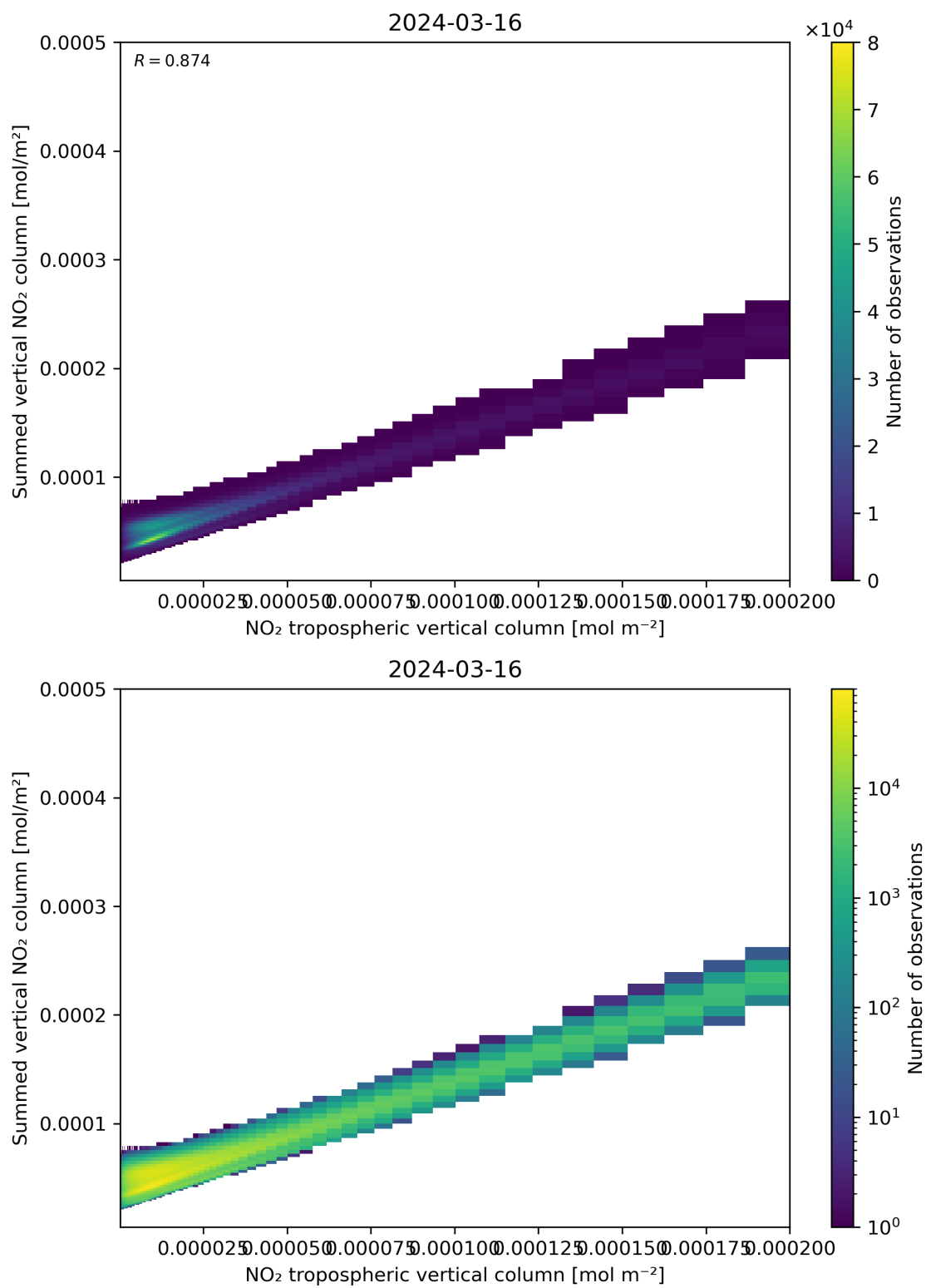
Figure 126: Scatter density plot of “NO 2 tropospheric vertical column” against “Summed vertical NO 2 column” for 2024-03-15 to 2024-03-17.
