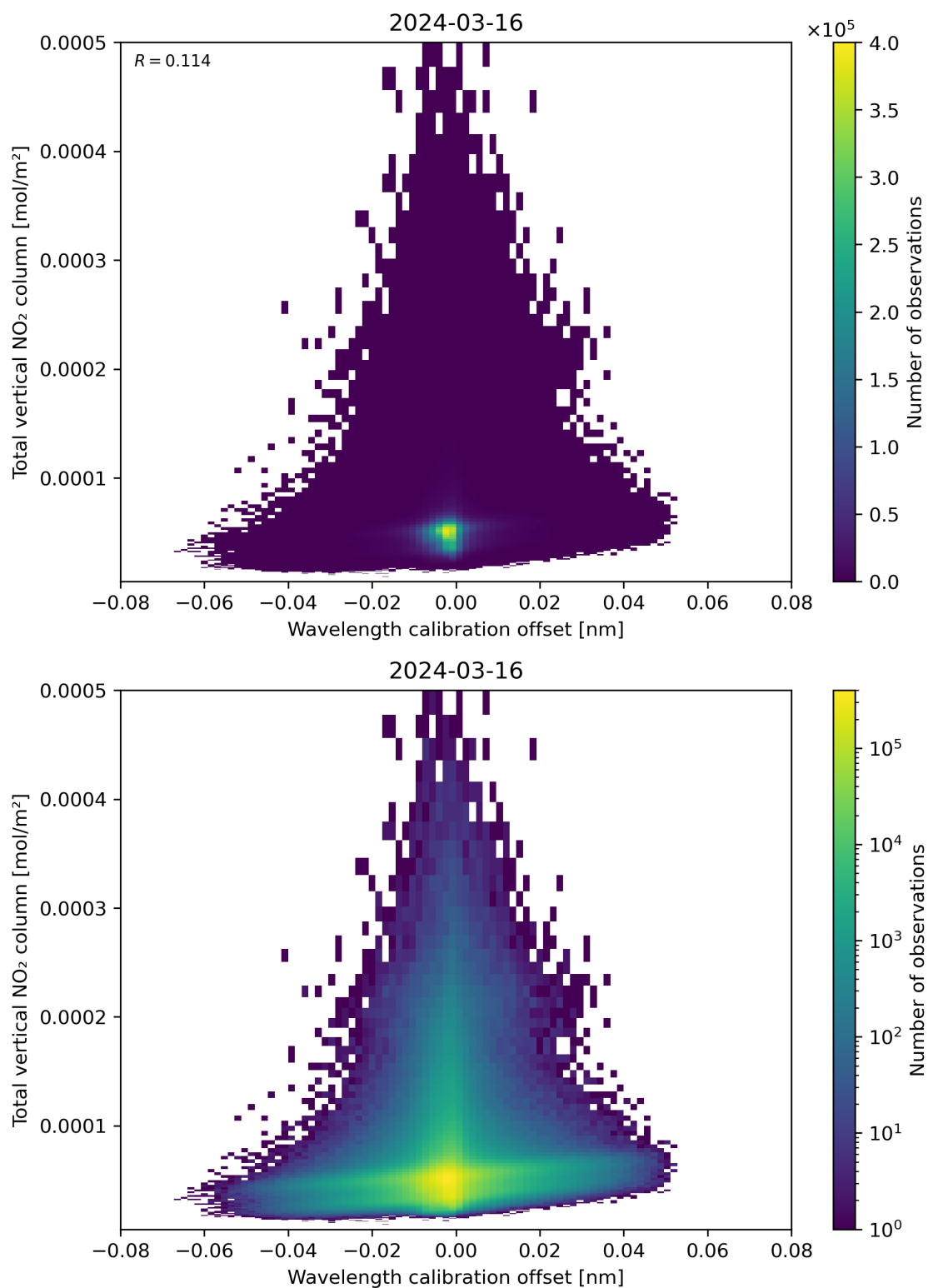
Figure 179: Scatter density plot of “Wavelength calibration offset” against “Total vertical NO 2 column” for 2024-03-15 to 2024-03-17.
