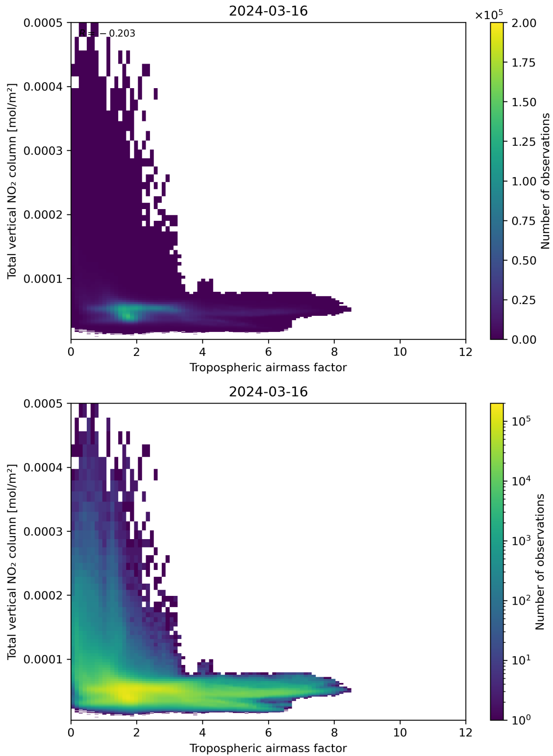
Figure 77: Scatter density plot of “Tropospheric airmass factor” against “Total vertical NO 2 column” for 2024-03-15 to 2024-03-17.
