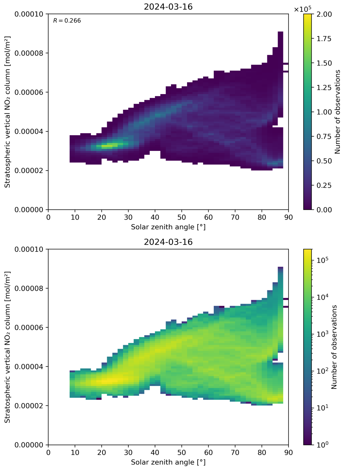
Figure 150: Scatter density plot of “Solar zenith angle” against “Stratospheric vertical NO 2 column” for 2024-03-15 to 2024-03-17.
