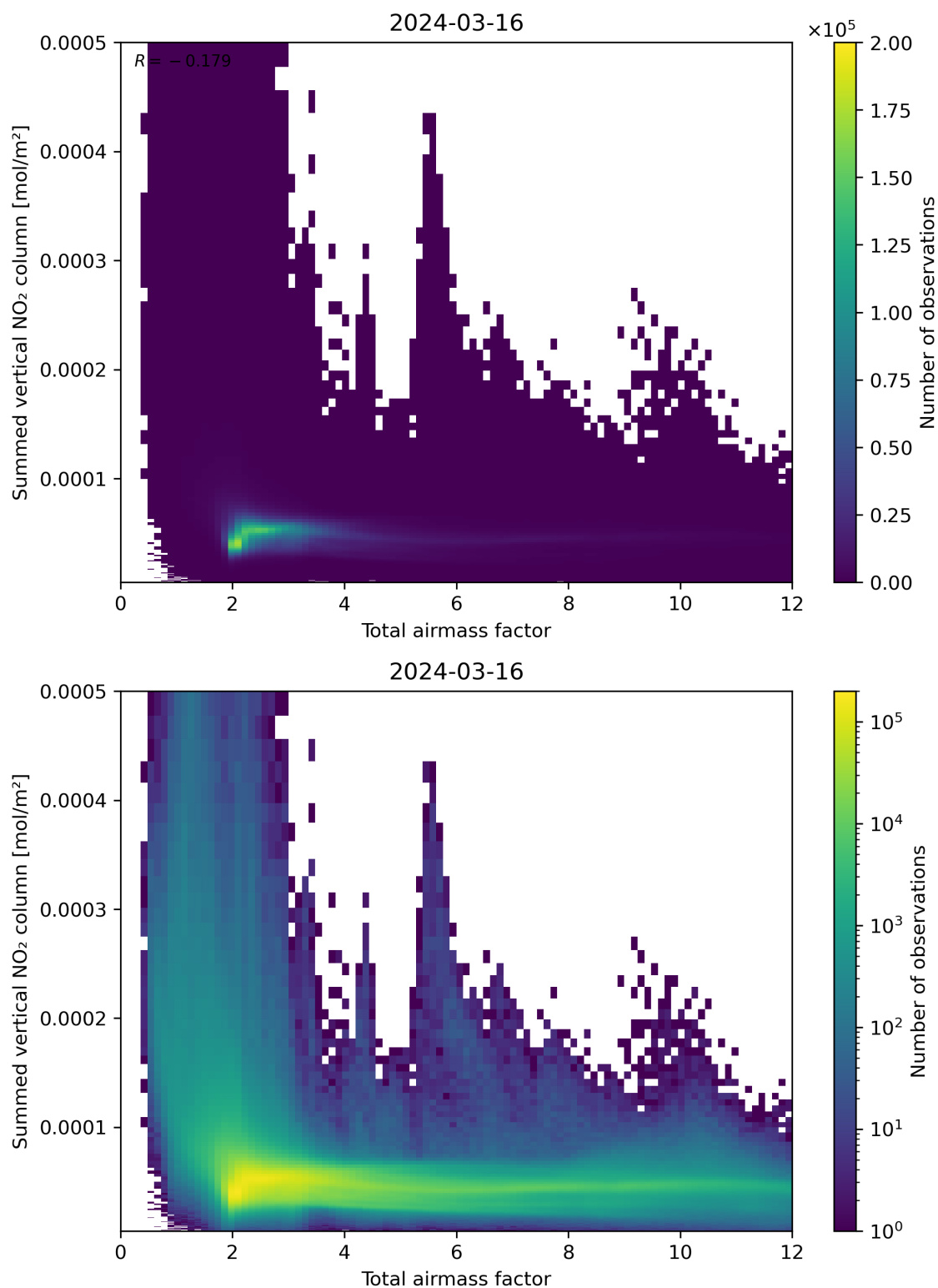
Figure 65: Scatter density plot of “Total airmass factor” against “Summed vertical NO 2 column” for 2024-03-15 to 2024-03-17.
