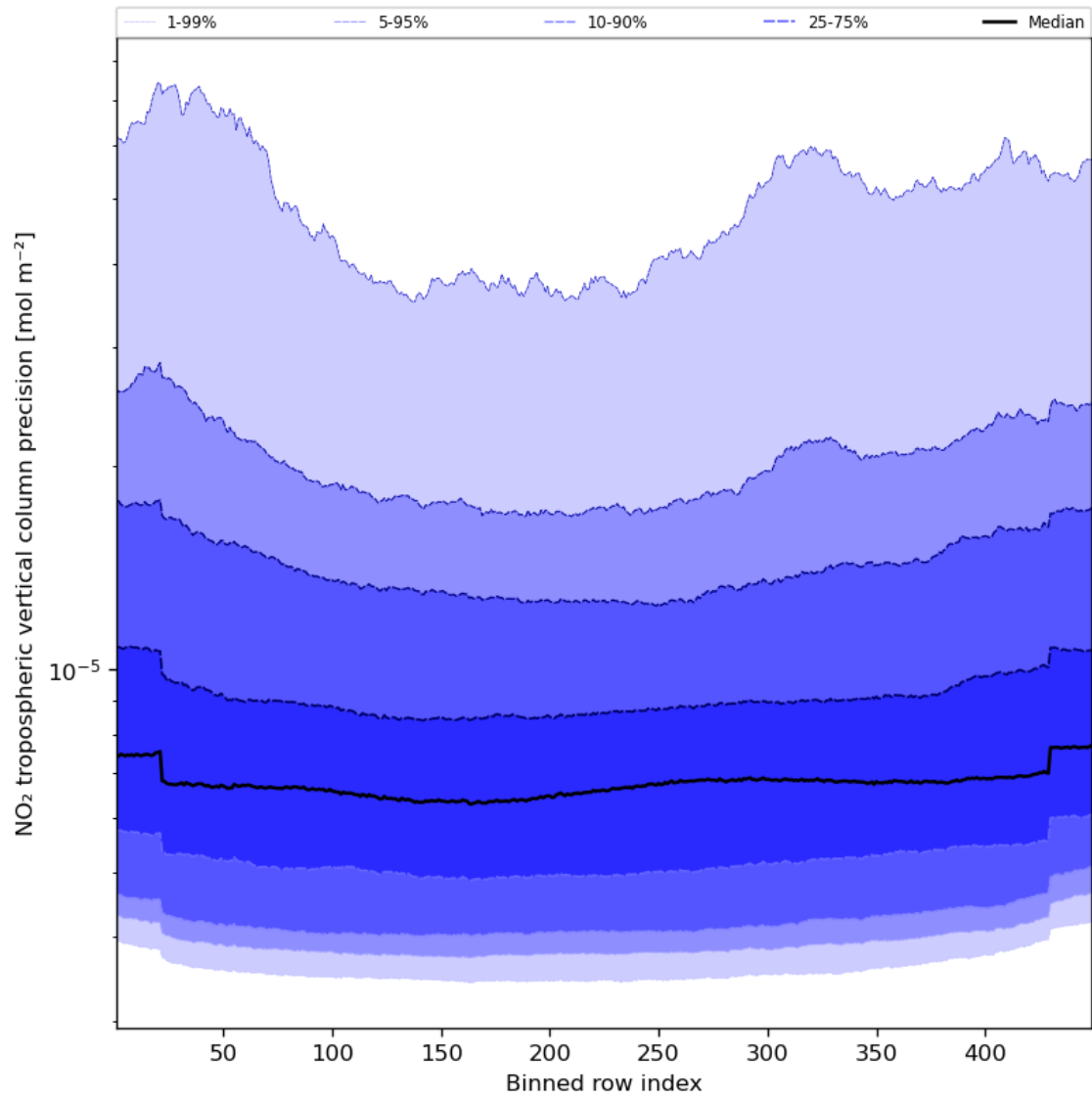
Figure 47: Along track statistics of “NO 2 tropospheric vertical column precision” for 2024-03-15 to 2024-03-17
