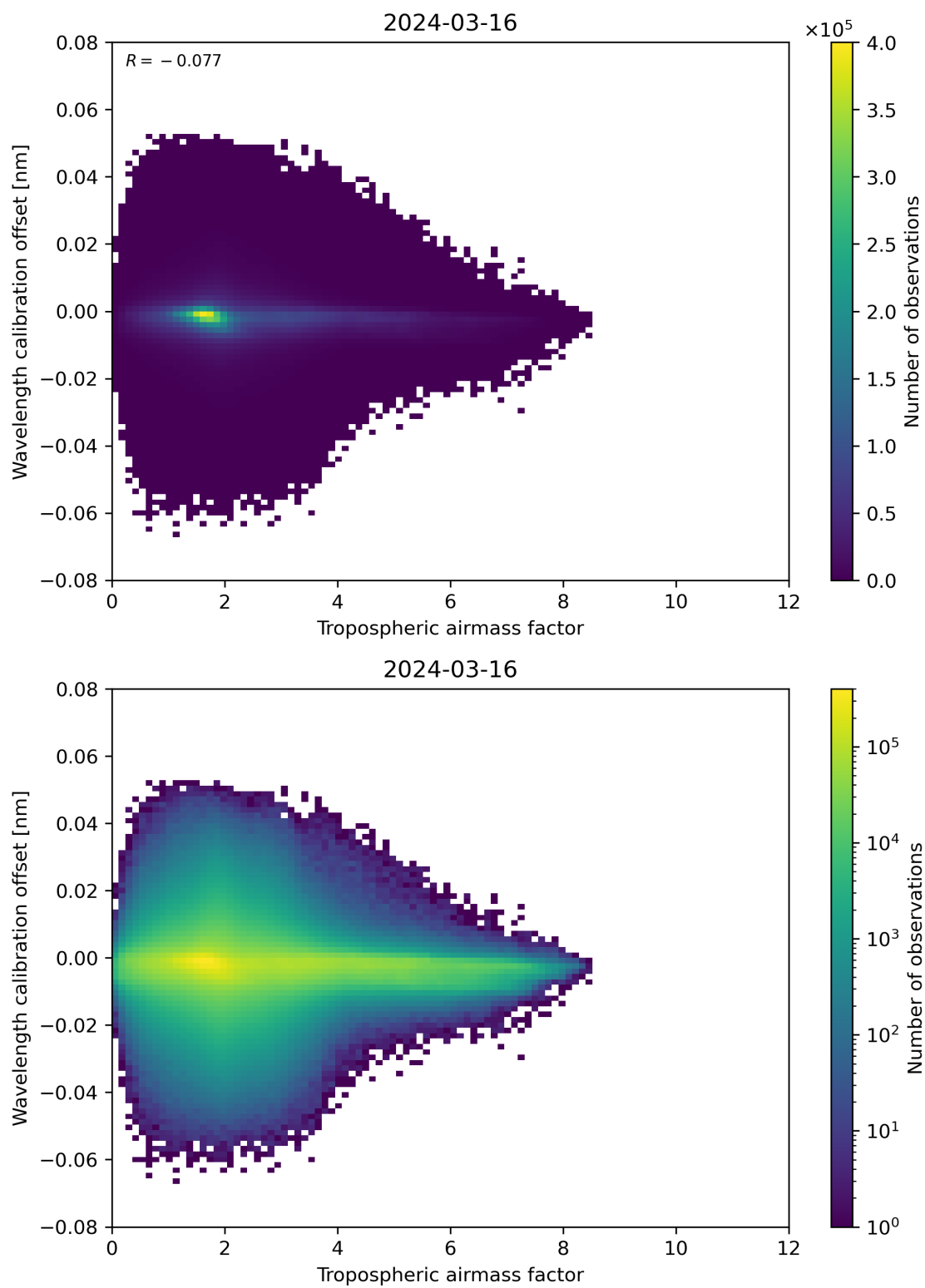
Figure 80: Scatter density plot of “Tropospheric airmass factor” against “Wavelength calibration offset” for 2024-03-15 to 2024-03-17.
