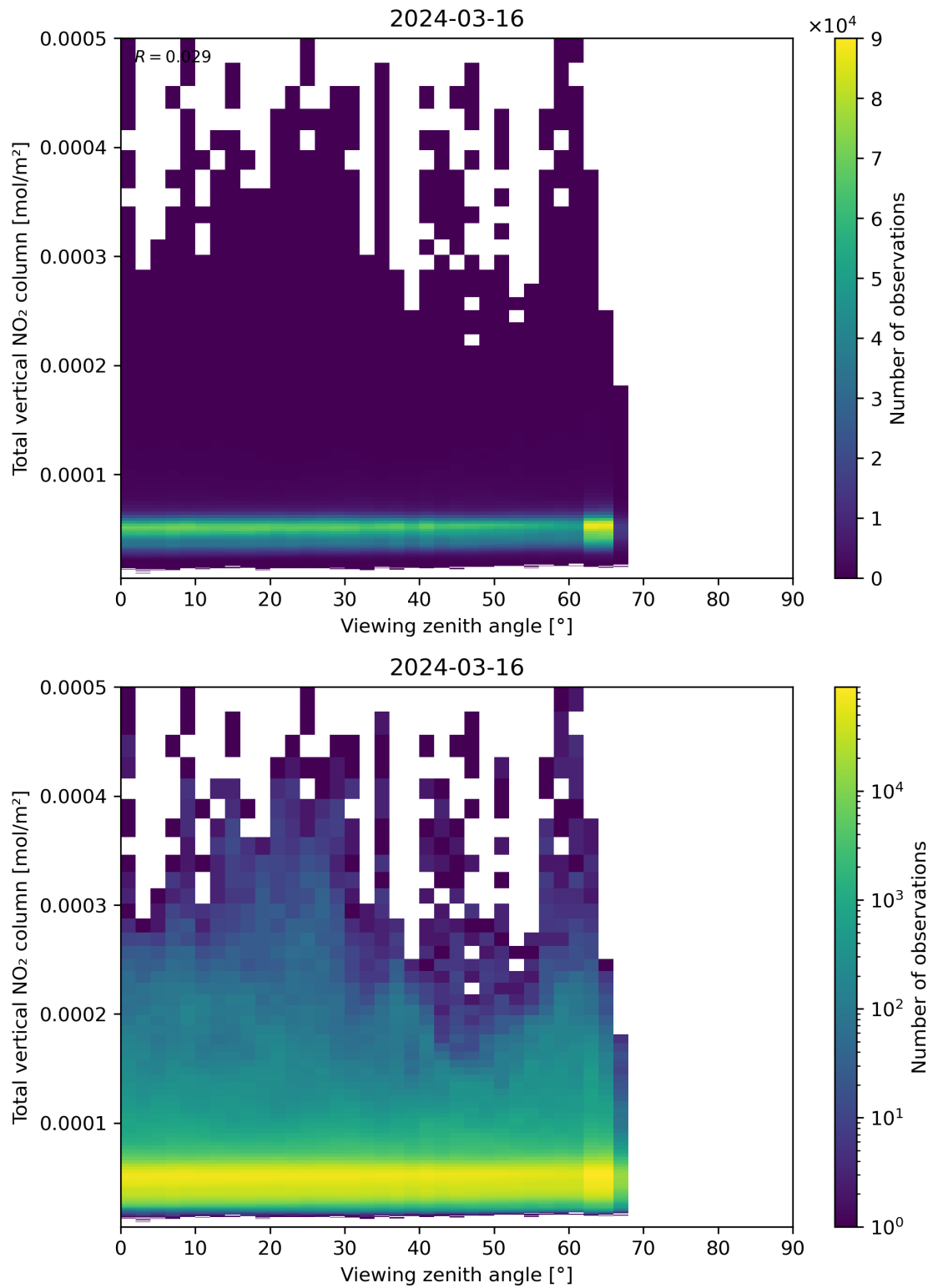
Figure 167: Scatter density plot of “Viewing zenith angle” against “Total vertical NO 2 column” for 2024-03-15 to 2024-03-17.
