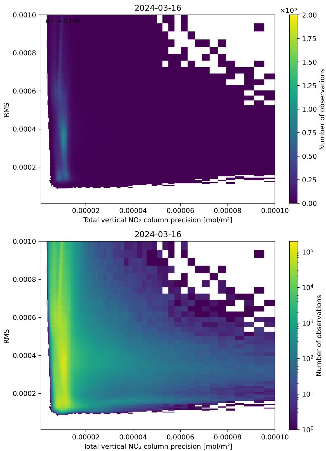
Figure 119: Scatter density plot of “Total vertical NO 2 column precision” against “RMS” for 2024-03-15 to 2024-03-17.
