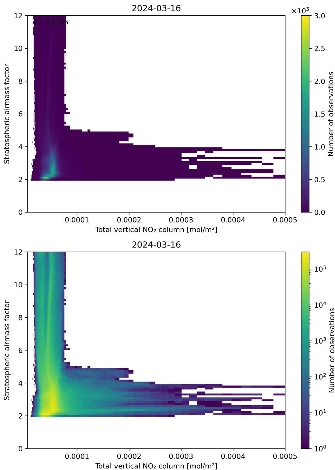
Figure 110: Scatter density plot of “Total vertical NO 2 column” against “Stratospheric air mass factor” for 2024-03-15 to 2024-03-17.
