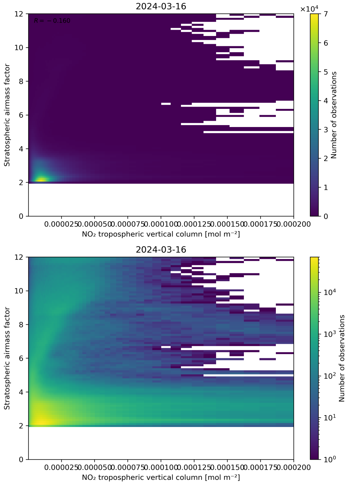
Figure 121: Scatter density plot of “NO 2 tropospheric vertical column” against “Stratospheric air mass factor” for 2024-03-15 to 2024-03-17.
