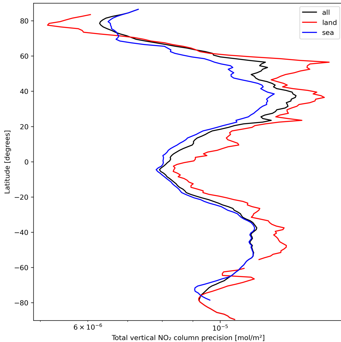
Figure 22: Zonal average of “Total vertical NO 2 column precision” for 2024-03-15 to 2024-03-17.
