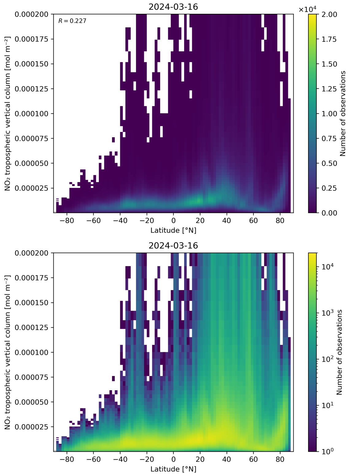
Figure 92: Scatter density plot of “Latitude” against “NO 2 tropospheric vertical column” for 2024-03-15 to 2024-03-17.
