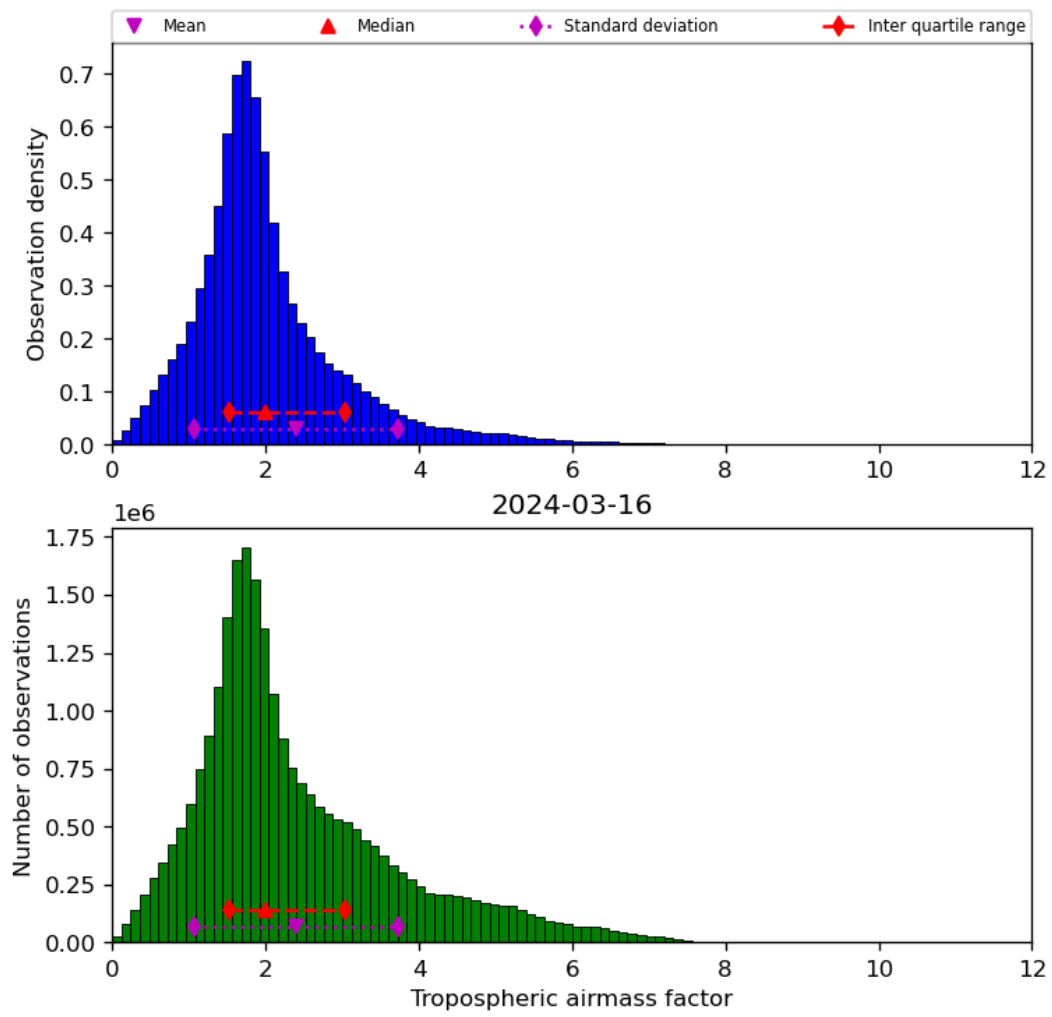
Figure 31: Histogram of “Tropospheric airmass factor” for 2024-03-15 to 2024-03-17
