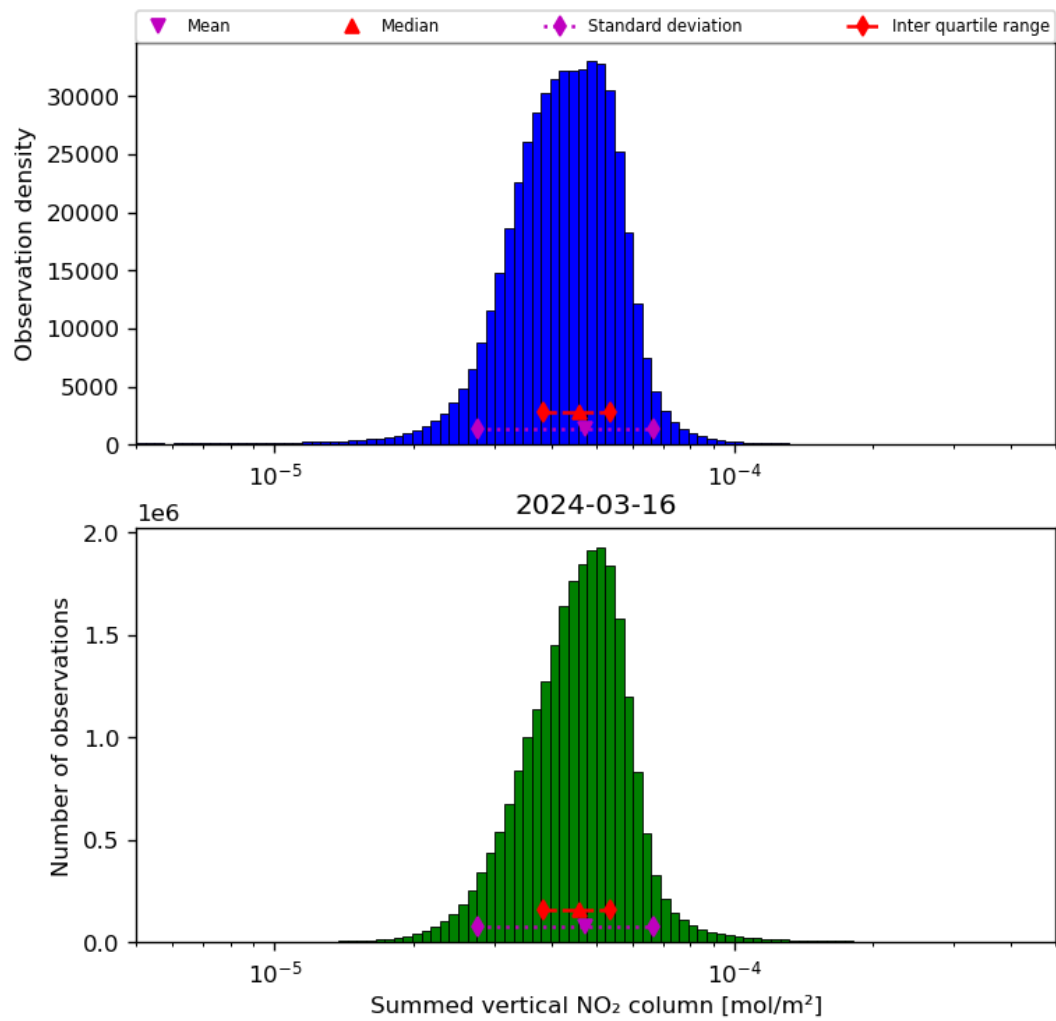
Figure 40: Histogram of “Summed vertical NO 2 column” for 2024-03-15 to 2024-03-17
