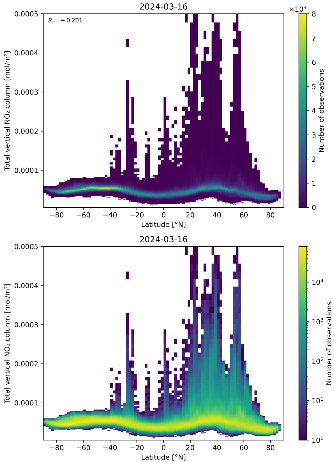
Figure 90: Scatter density plot of “Latitude” against “Total vertical NO 2 column” for 2024-03-15 to 2024-03-17.
