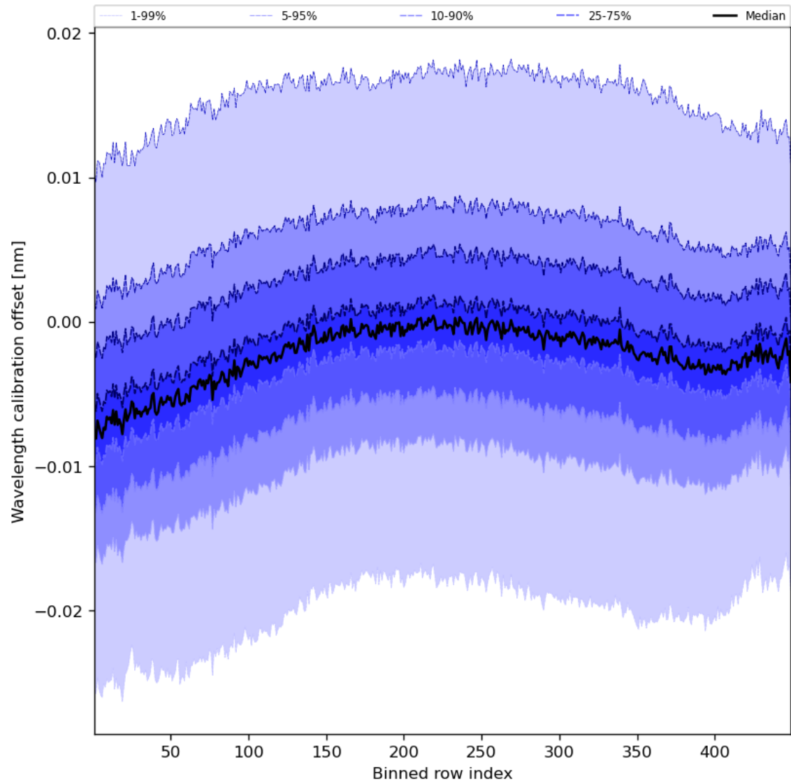
Figure 52: Along track statistics of “Wavelength calibration offset” for 2024-03-15 to 2024-03-17
