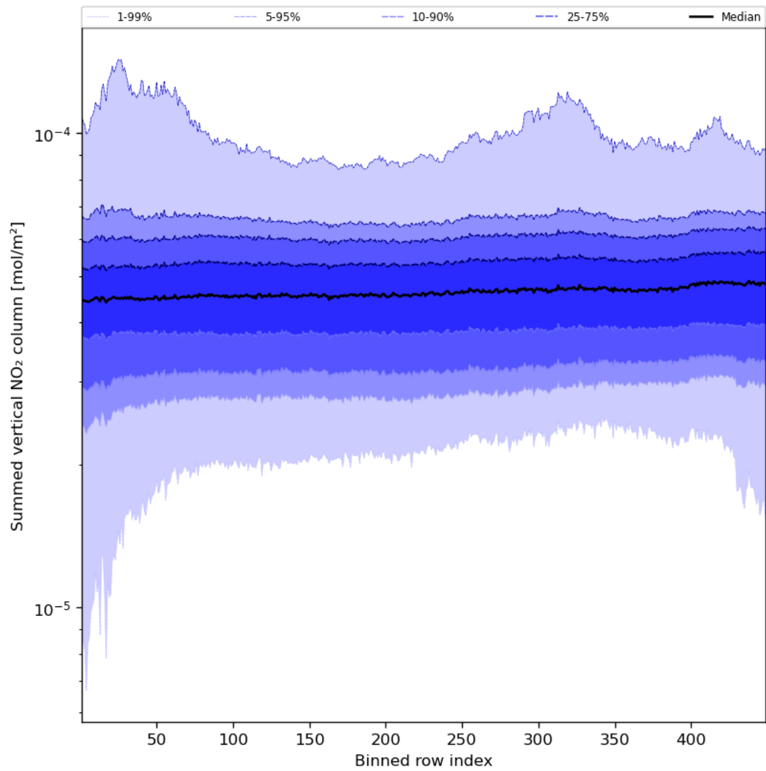
Figure 57: Along track statistics of “Summed vertical NO 2 column” for 2024-03-15 to 2024-03-17
