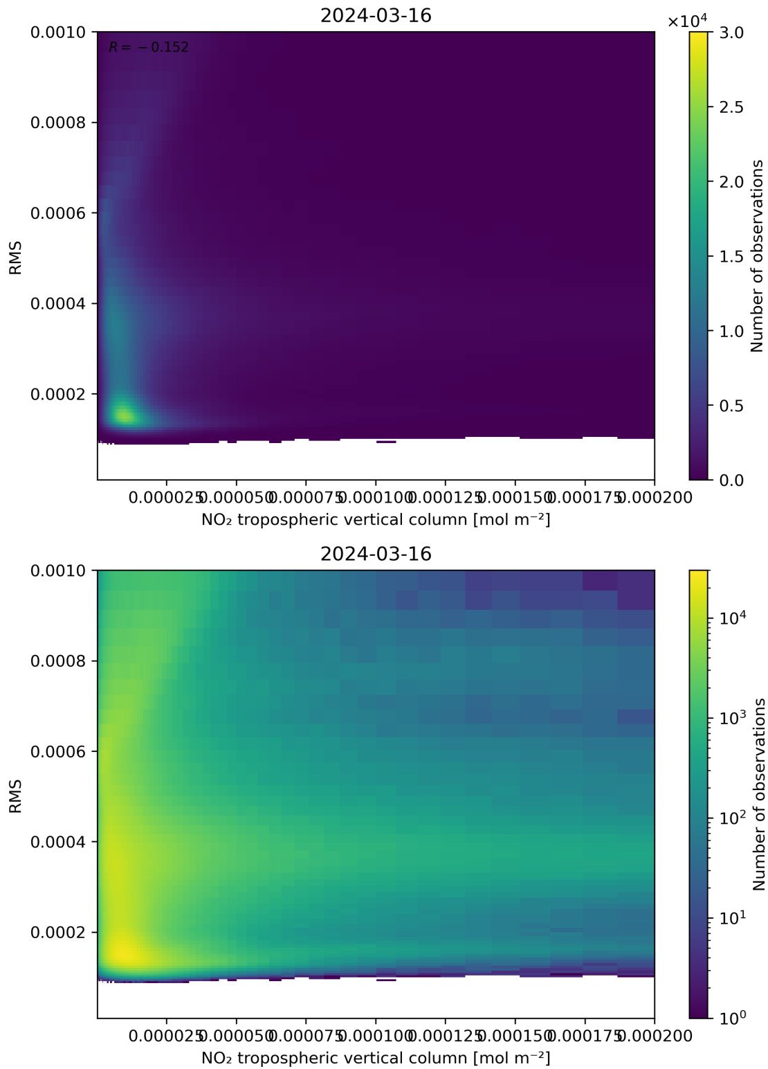
Figure 142: Scatter density plot of “NO 2 tropospheric vertical column” against “RMS” for 2024-03-15 to 2024-03-17.
