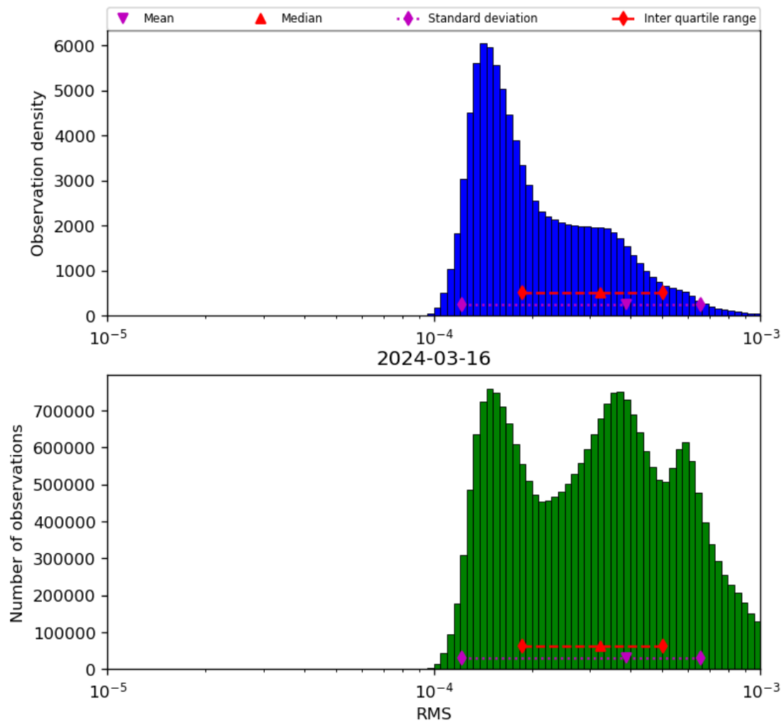
Figure 43: Histogram of “RMS” for 2024-03-15 to 2024-03-17
