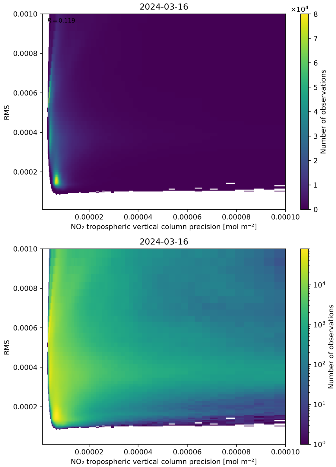
Figure 140: Scatter density plot of “NO 2 tropospheric vertical column precision” against “RMS” for 2024-03-15 to 2024-03-17.
