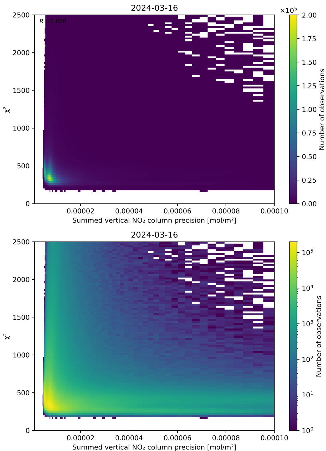
Figure 107: Scatter density plot of “Summed vertical NO 2 column precision” against “ \chi^2 ” for 2024-03-15 to 2024-03-17.
