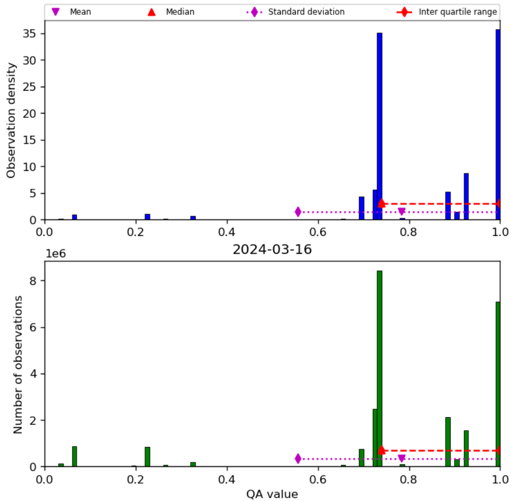
Figure 28: Histogram of “QA value” for 2024-03-15 to 2024-03-17
