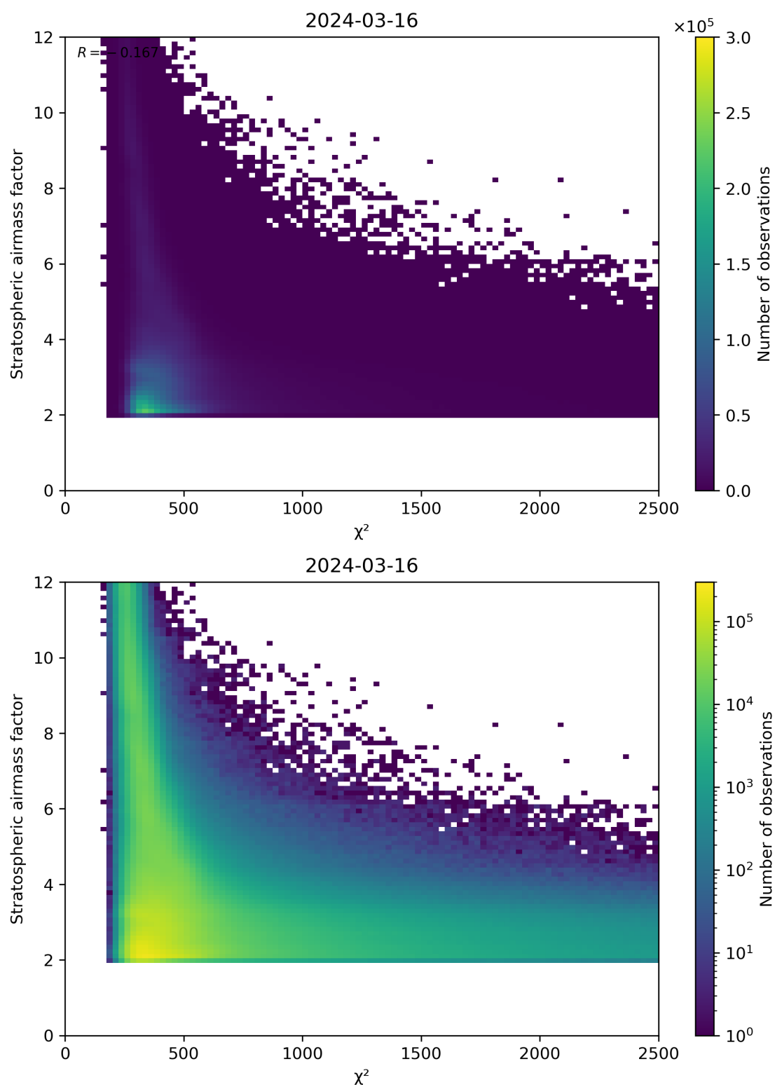
Figure 81: Scatter density plot of “ \chi^2 ” against “Stratospheric airmass factor” for 2024-03-15 to 2024-03-17.
