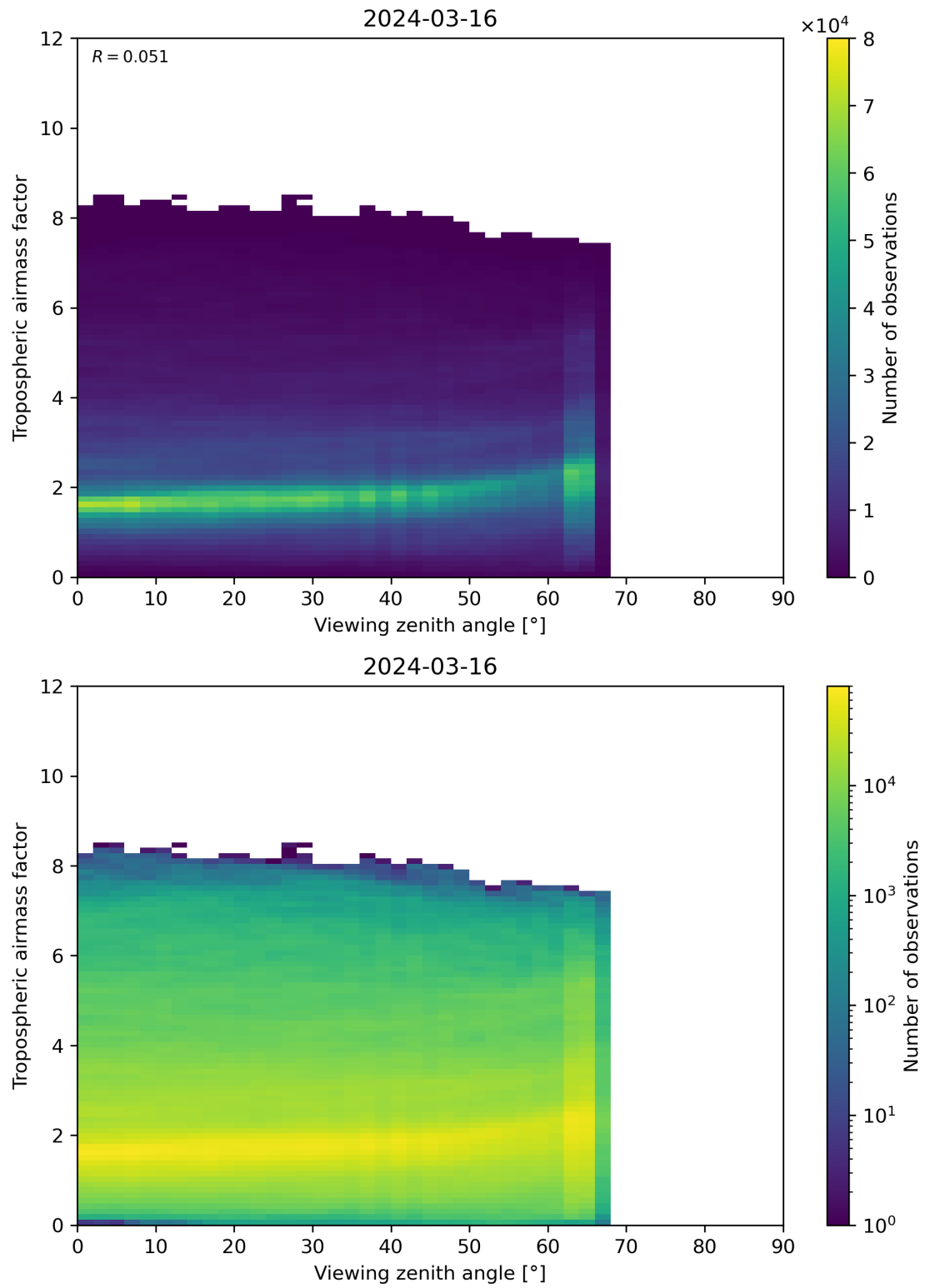
Figure 161: Scatter density plot of “Viewing zenith angle” against “Tropospheric airmass factor” for 2024-03-15 to 2024-03-17.
