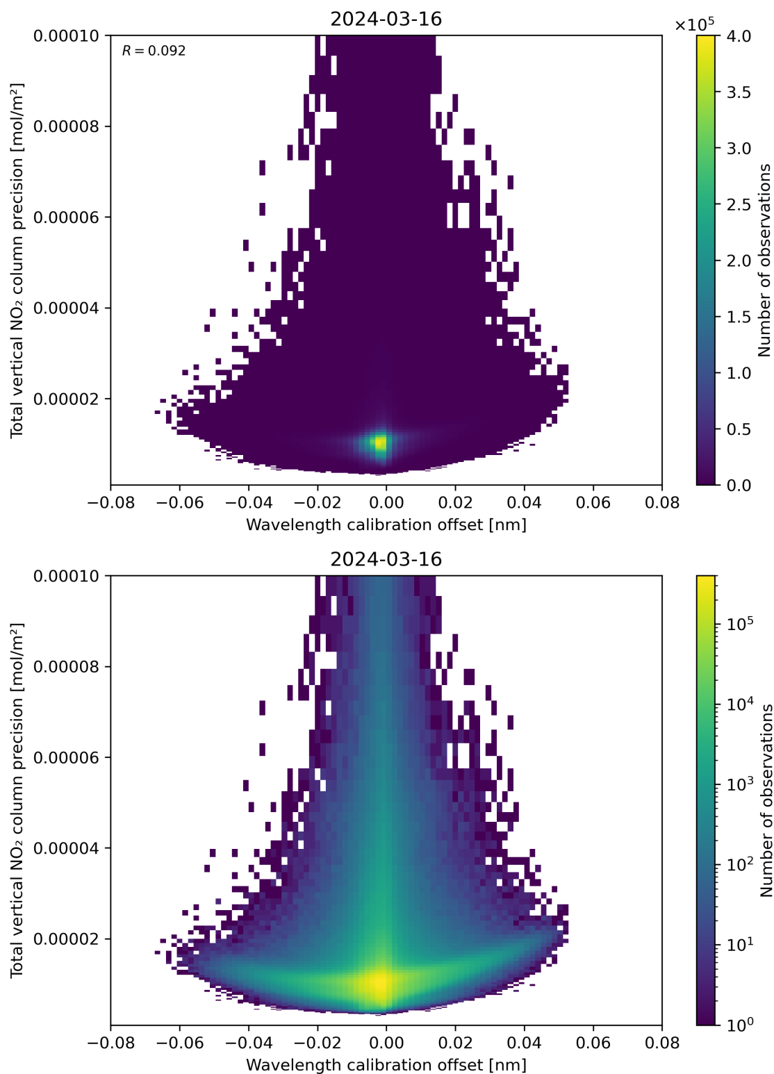
Figure 180: Scatter density plot of “Wavelength calibration offset” against “Total vertical NO 2 column precision” for 2024-03-15 to 2024-03-17.
