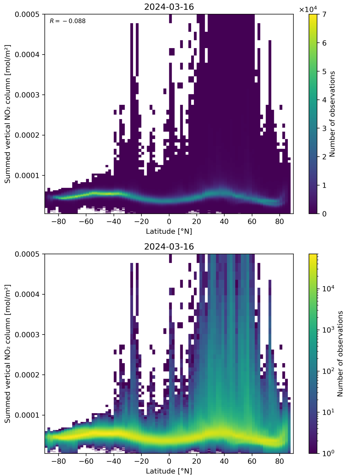
Figure 88: Scatter density plot of “Latitude” against “Summed vertical NO 2 column” for 2024-03-15 to 2024-03-17.
