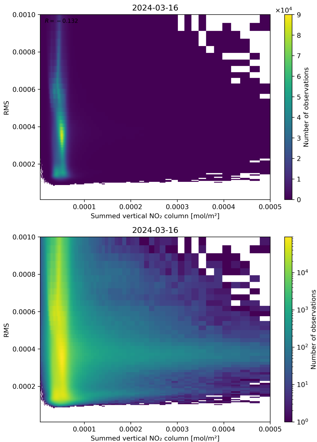
Figure 109: Scatter density plot of “Summed vertical NO 2 column” against “RMS” for 2024-03-15 to 2024-03-17.
