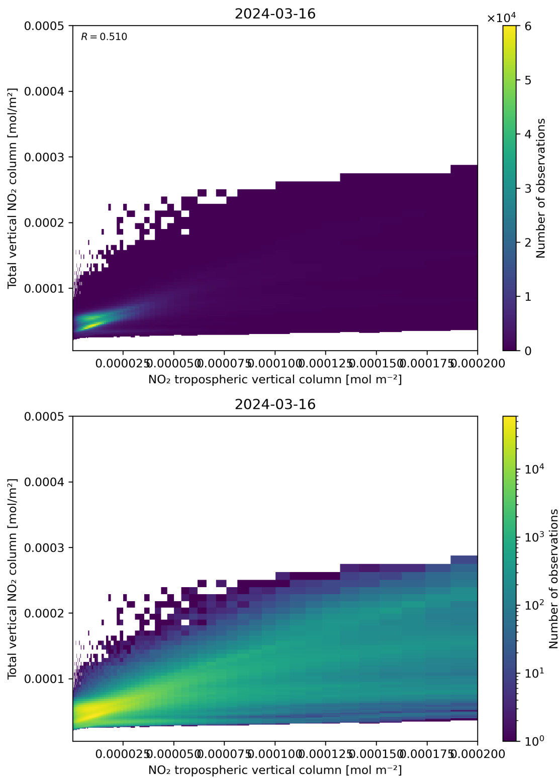
Figure 128: Scatter density plot of “NO 2 tropospheric vertical column” against “Total vertical NO 2 column” for 2024-03-15 to 2024-03-17.
