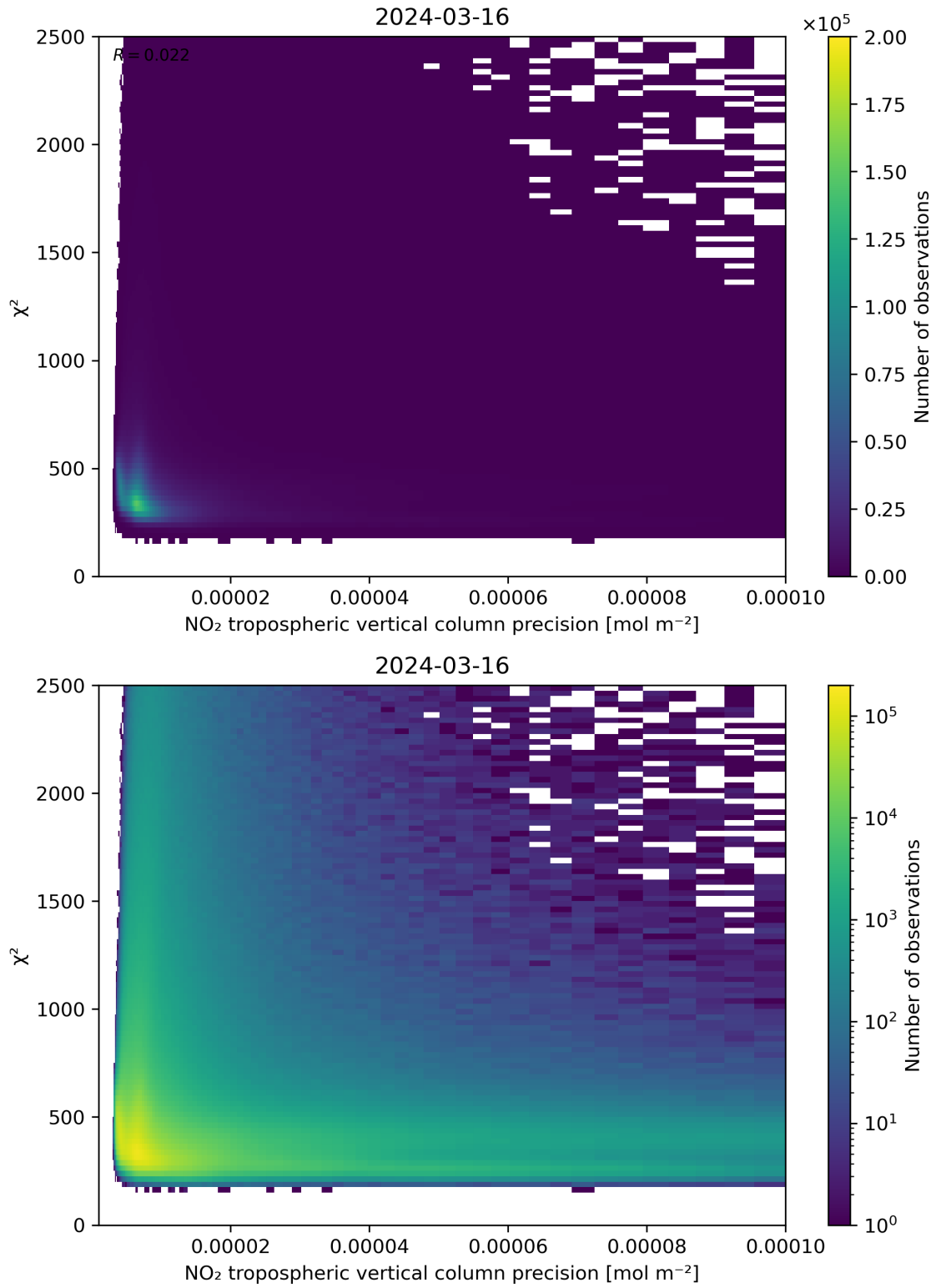
Figure 134: Scatter density plot of “NO 2 tropospheric vertical column precision” against “ \chi^2 ” for 2024-03-15 to 2024-03-17.
