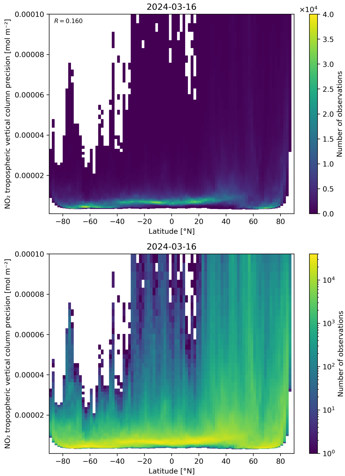
Figure 93: Scatter density plot of “Latitude” against “NO 2 tropospheric vertical column precision” for 2024-03-15 to 2024-03-17.
