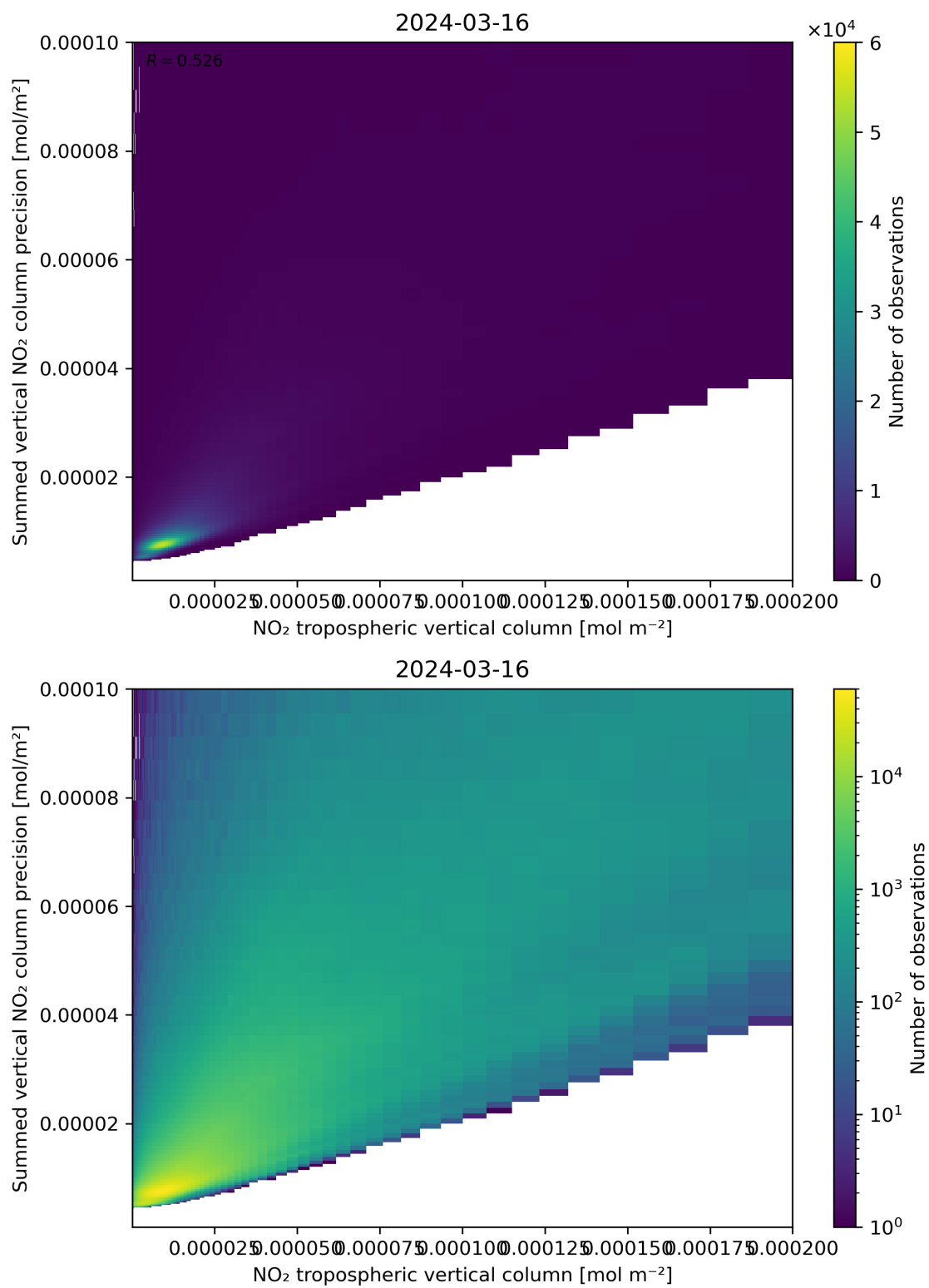
Figure 127: Scatter density plot of “NO 2 tropospheric vertical column” against “Summed vertical NO 2 column precision” for 2024-03-15 to 2024-03-17.
