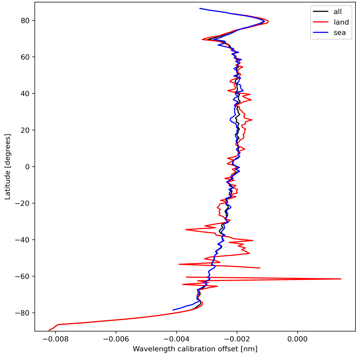
Figure 18: Zonal average of “Wavelength calibration offset” for 2024-03-15 to 2024-03-17.
