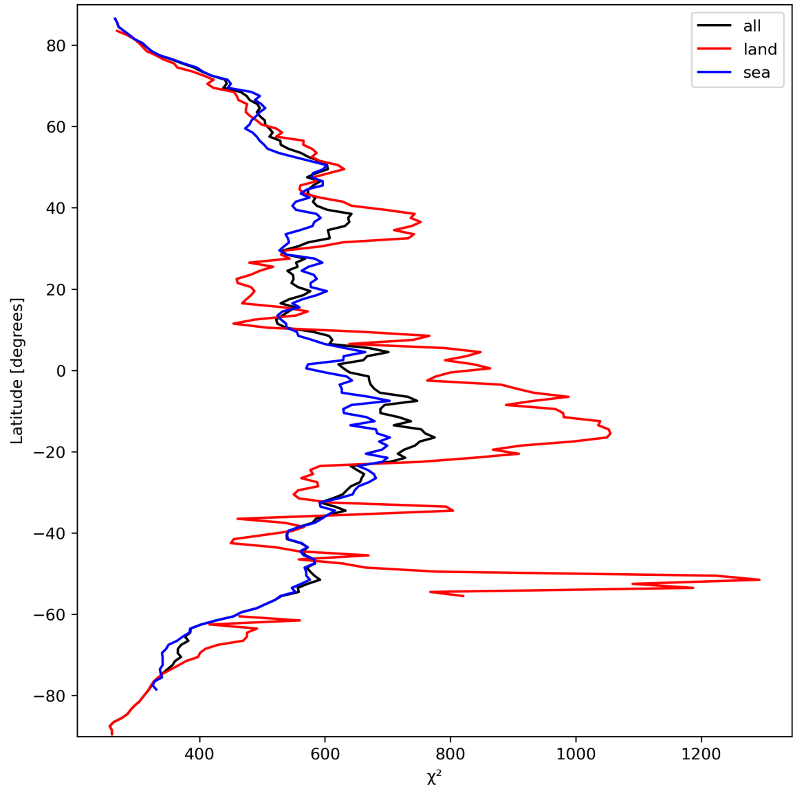
Figure 25: Zonal average of “ \chi^2 ” for 2024-03-15 to 2024-03-17.
