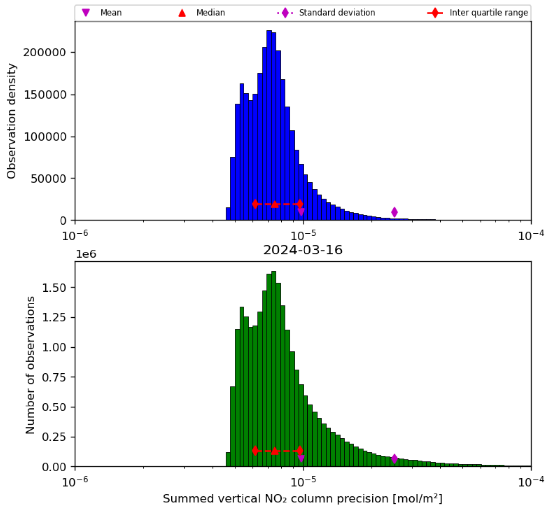
Figure 41: Histogram of "Summed vertical NO 2 column precision" for 2024-03-15 to 2024-03-17
