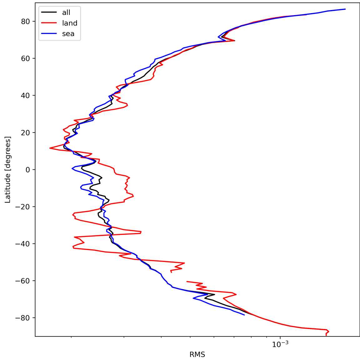
Figure 26: Zonal average of “RMS” for 2024-03-15 to 2024-03-17.
