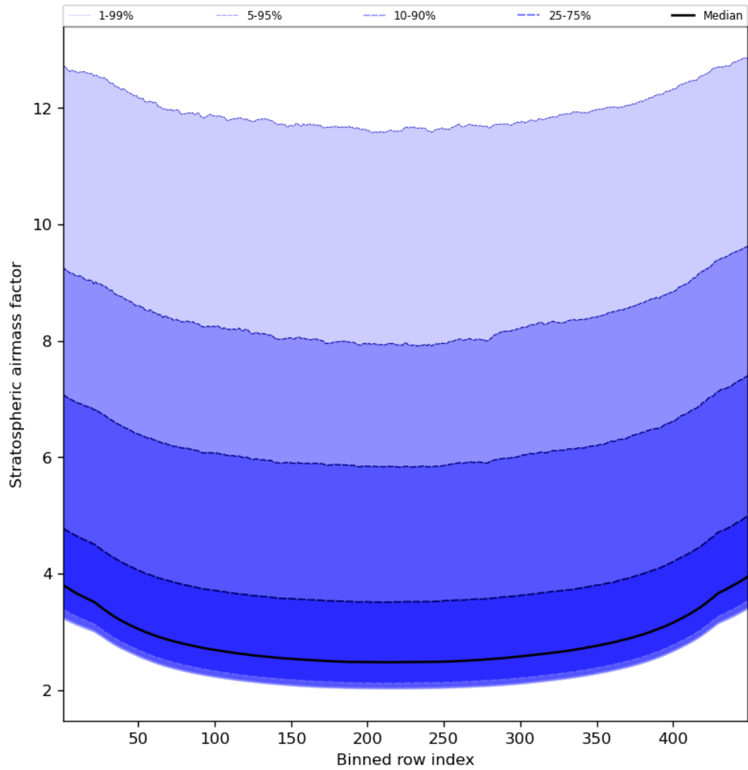
Figure 61: Along track statistics of “Stratospheric airmass factor” for 2024-03-15 to 2024-03-17
