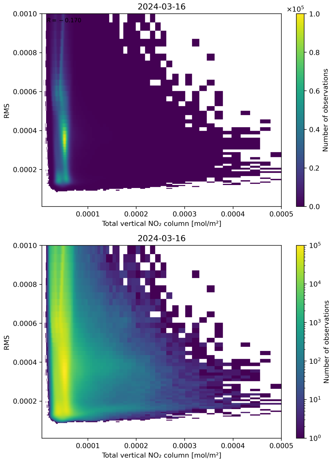
Figure 120: Scatter density plot of “Total vertical NO 2 column” against “RMS” for 2024-03-15 to 2024-03-17.
