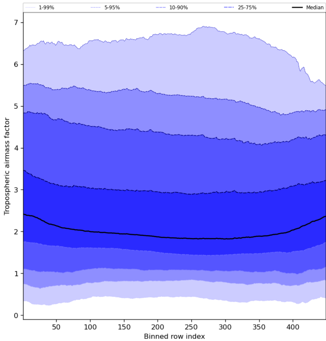
Figure 48: Along track statistics of “Tropospheric air mass factor” for 2024-03-15 to 2024-03-17
