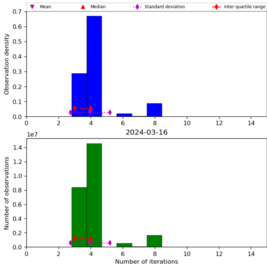
Figure 34: Histogram of “Number of iterations” for 2024-03-15 to 2024-03-17
