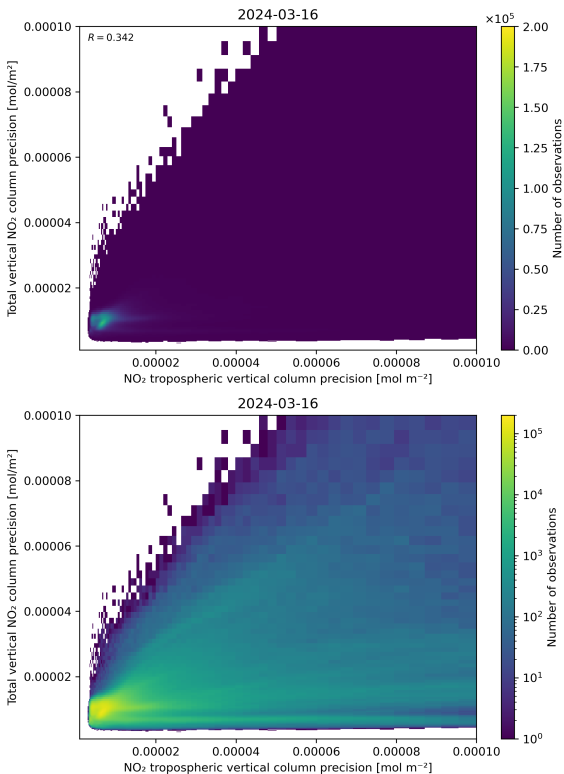
Figure 139: Scatter density plot of “NO 2 tropospheric vertical column precision” against “Total vertical NO 2 column precision” for 2024-03-15 to 2024-03-17.
