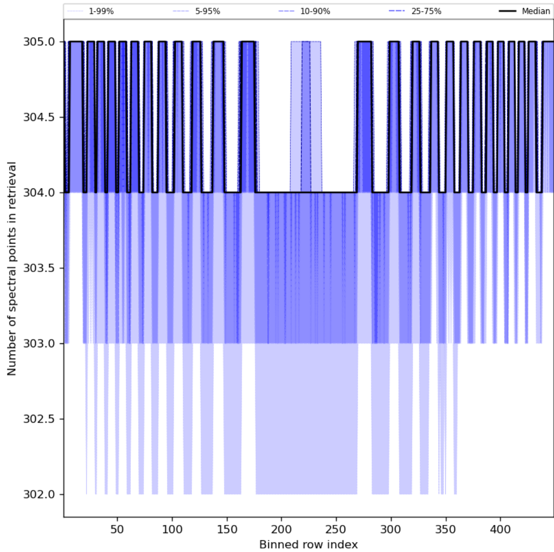
Figure 50: Along track statistics of “Number of spectral points in retrieval” for 2024-03-15 to 2024-03-17
