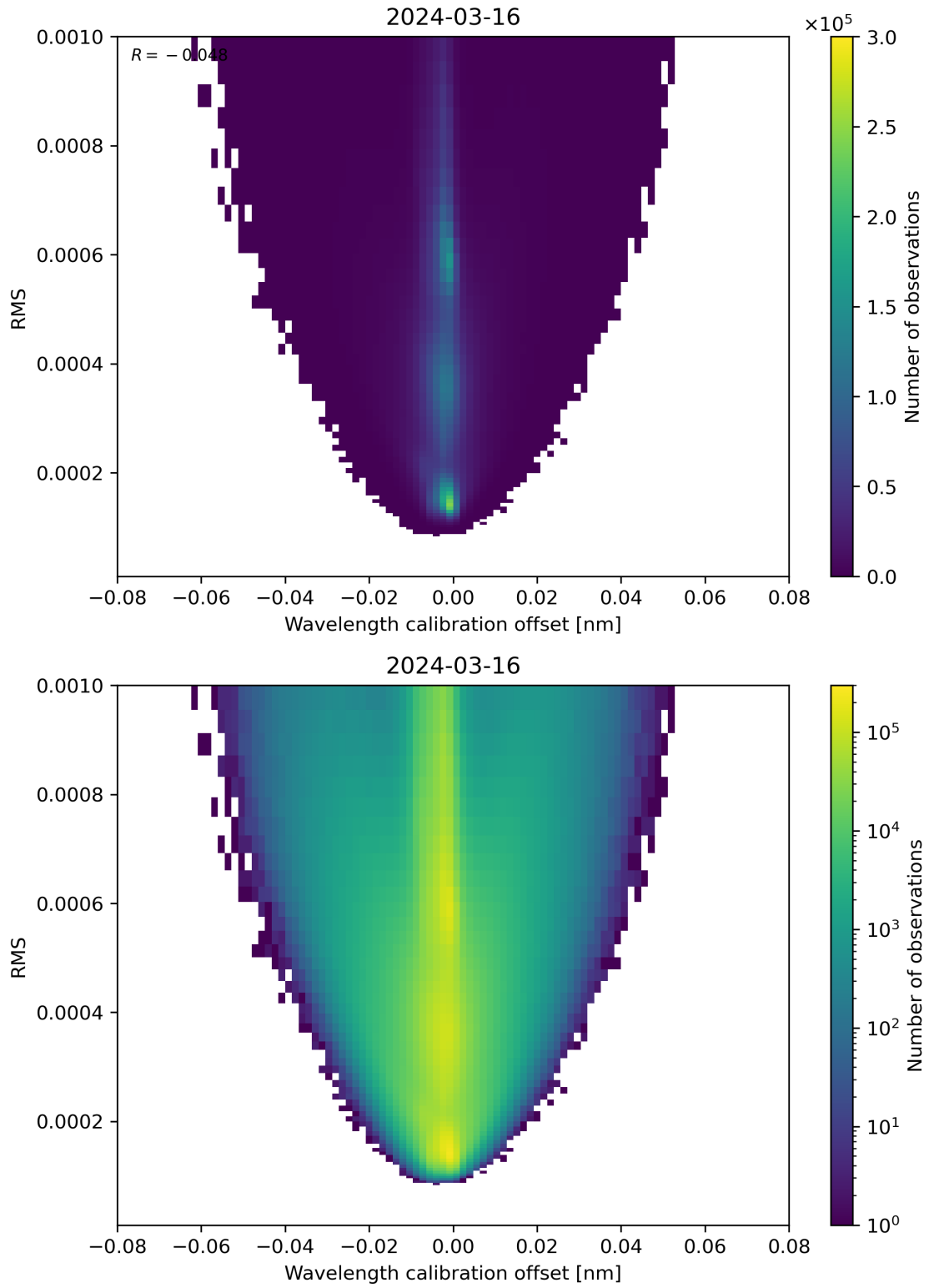
Figure 181: Scatter density plot of “Wavelength calibration offset” against “RMS” for 2024-03-15 to 2024-03-17.
