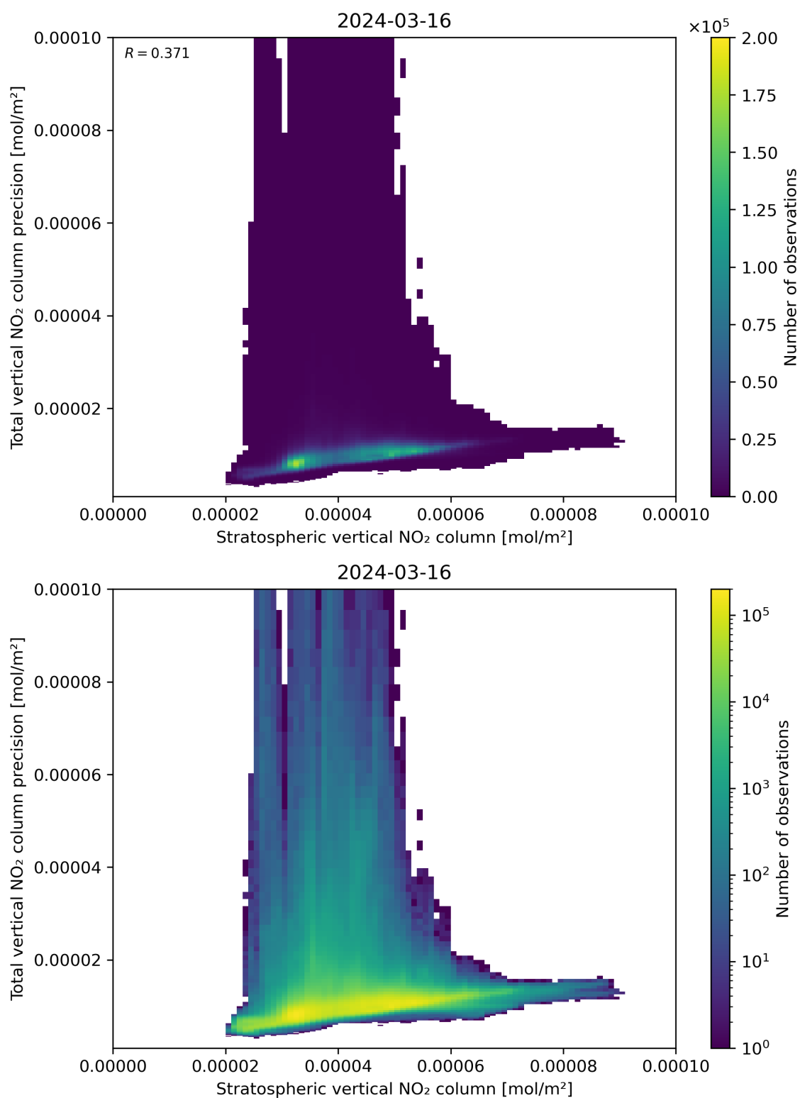
Figure 101: Scatter density plot of “Stratospheric vertical NO 2 column” against “Total vertical NO 2 column precision” for 2024-03-15 to 2024-03-17.
