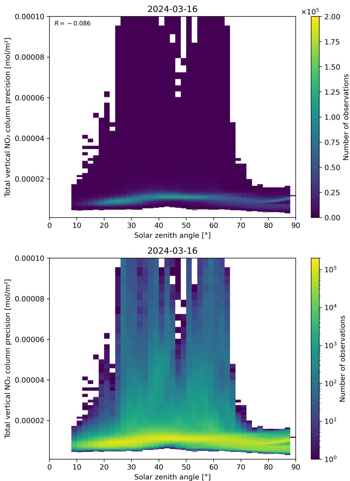
Figure 154: Scatter density plot of “Solar zenith angle” against “Total vertical NO 2 column precision” for 2024-03-15 to 2024-03-17.
