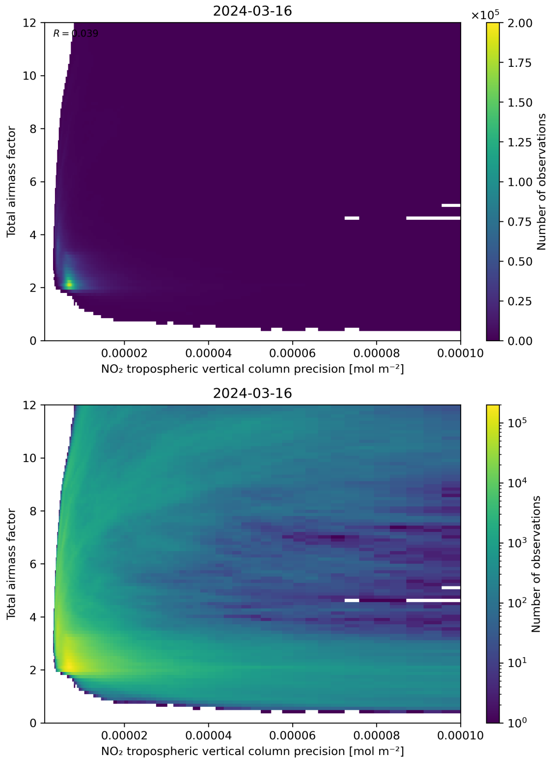
Figure 132: Scatter density plot of “NO 2 tropospheric vertical column precision” against “Total air mass factor” for 2024-03-15 to 2024-03-17.
