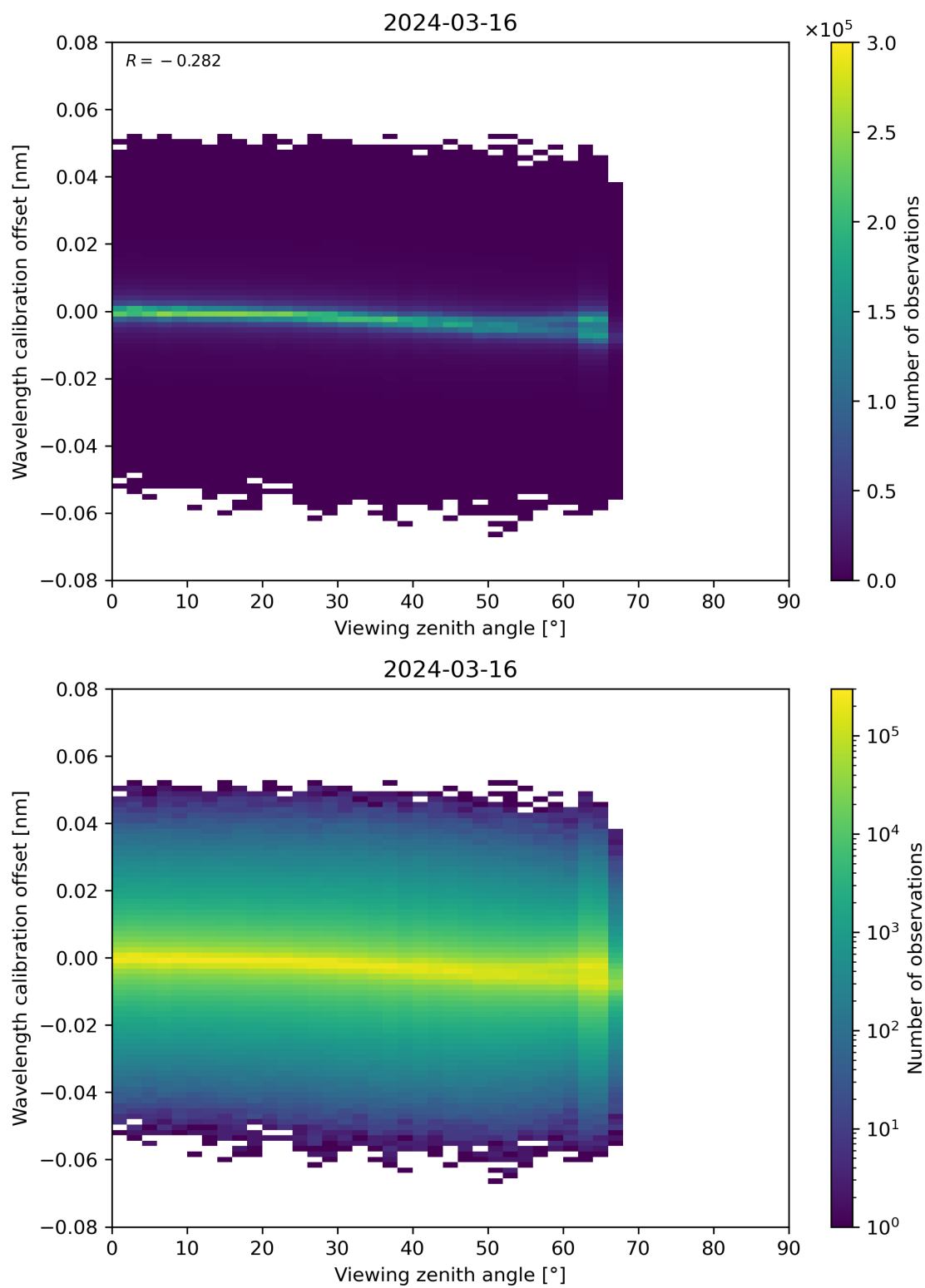
Figure 173: Scatter density plot of “Viewing zenith angle” against “Wavelength calibration offset” for 2024-03-15 to 2024-03-17.
