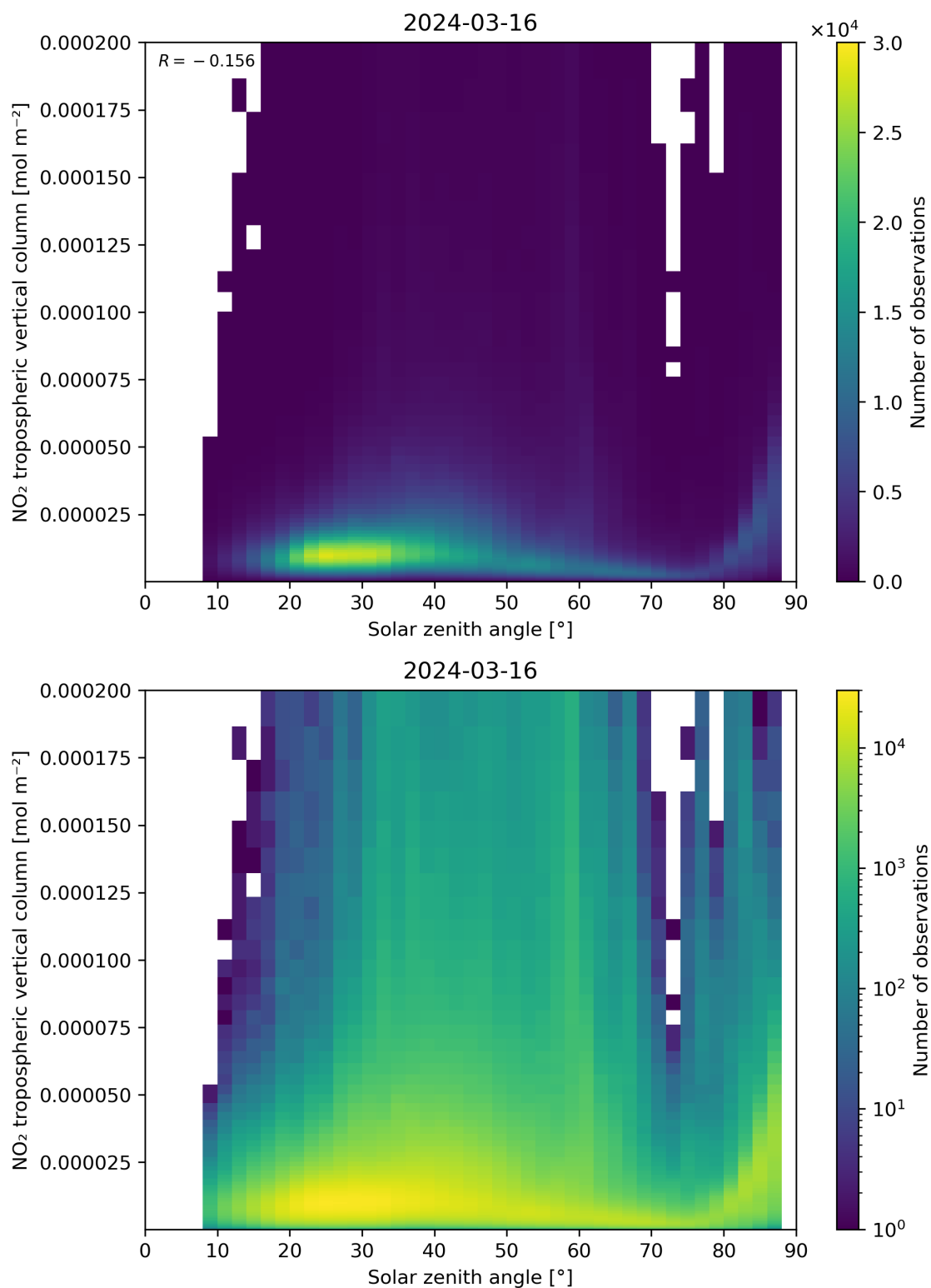
Figure 155: Scatter density plot of “Solar zenith angle” against “NO 2 tropospheric vertical column” for 2024-03-15 to 2024-03-17.
