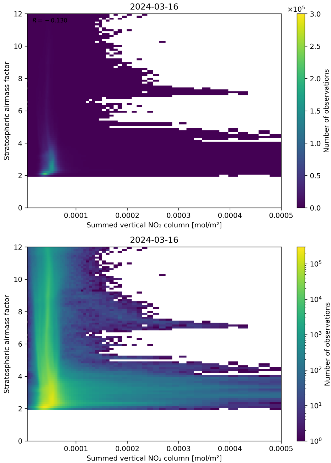
Figure 103: Scatter density plot of “Summed vertical NO 2 column” against “Stratospheric airmass factor” for 2024-03-15 to 2024-03-17.
