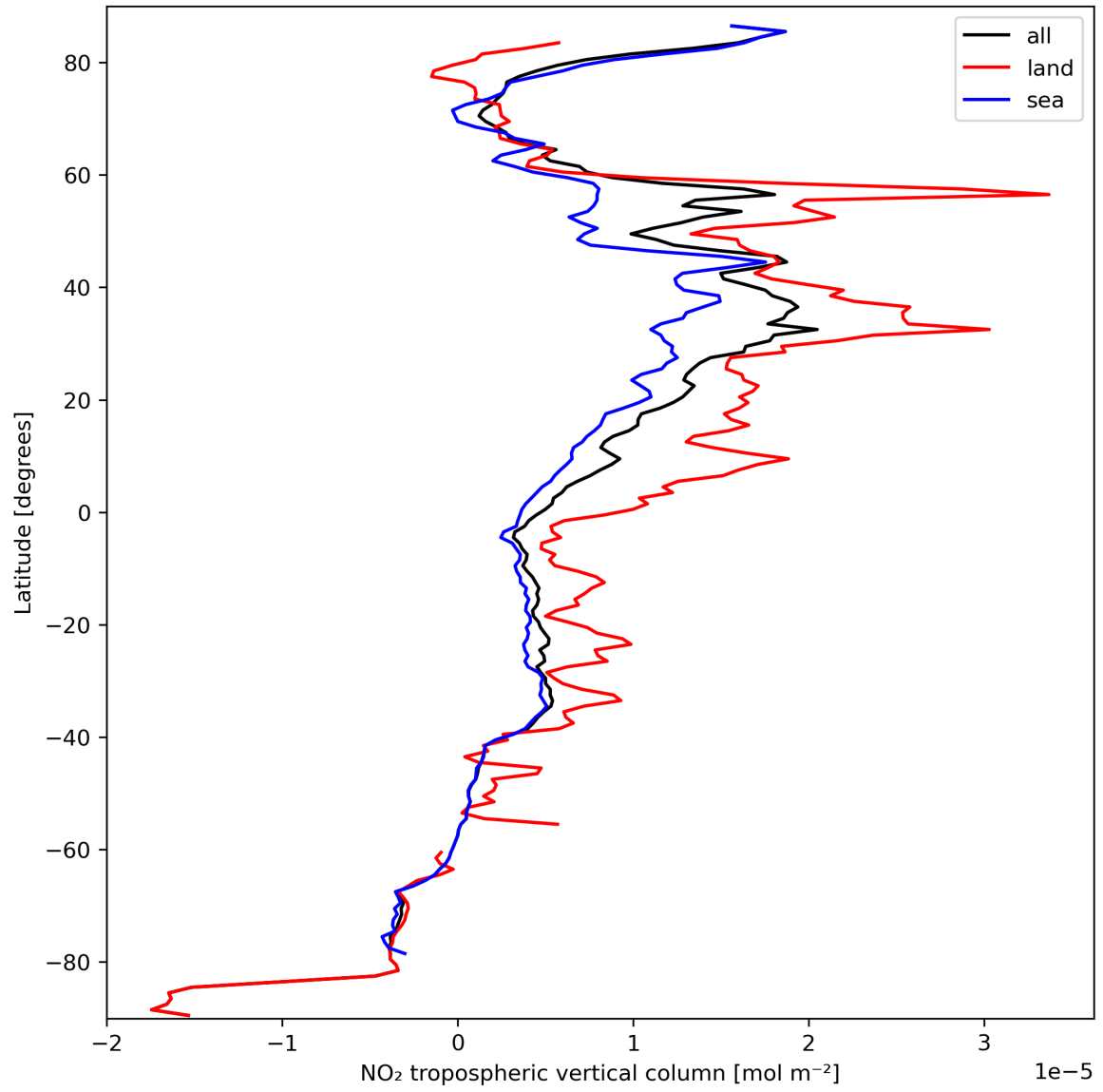
Figure 12: Zonal average of “NO 2 tropospheric vertical column” for 2024-03-15 to 2024-03-17.
