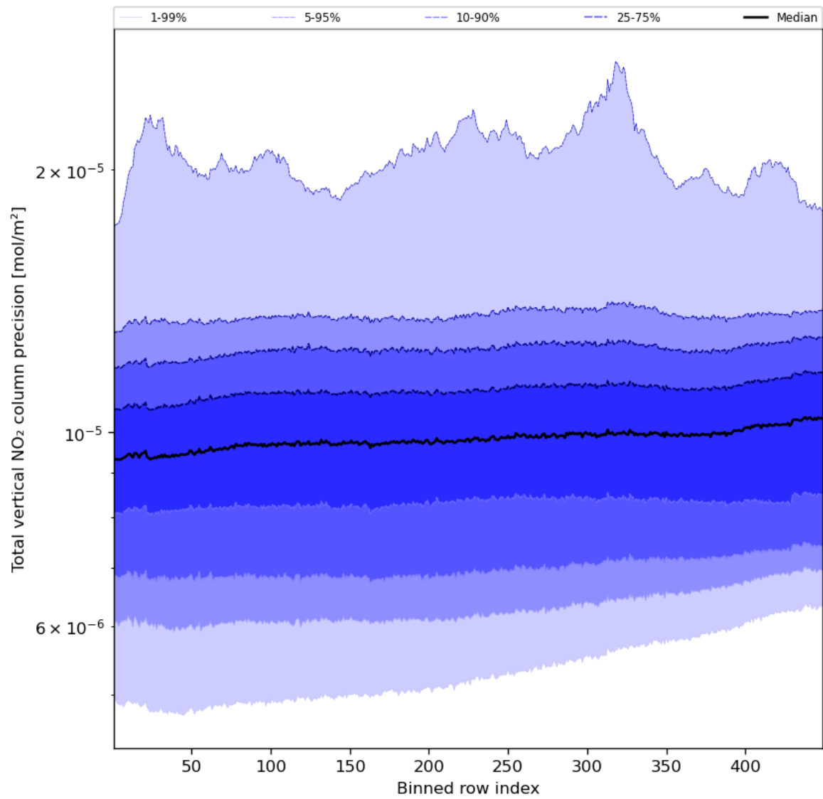
Figure 56: Along track statistics of "Total vertical NO 2 column precision" for 2024-03-15 to 2024-03-17
