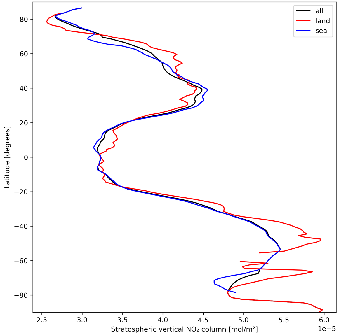
Figure 19: Zonal average of “Stratospheric vertical NO 2 column” for 2024-03-15 to 2024-03-17.
