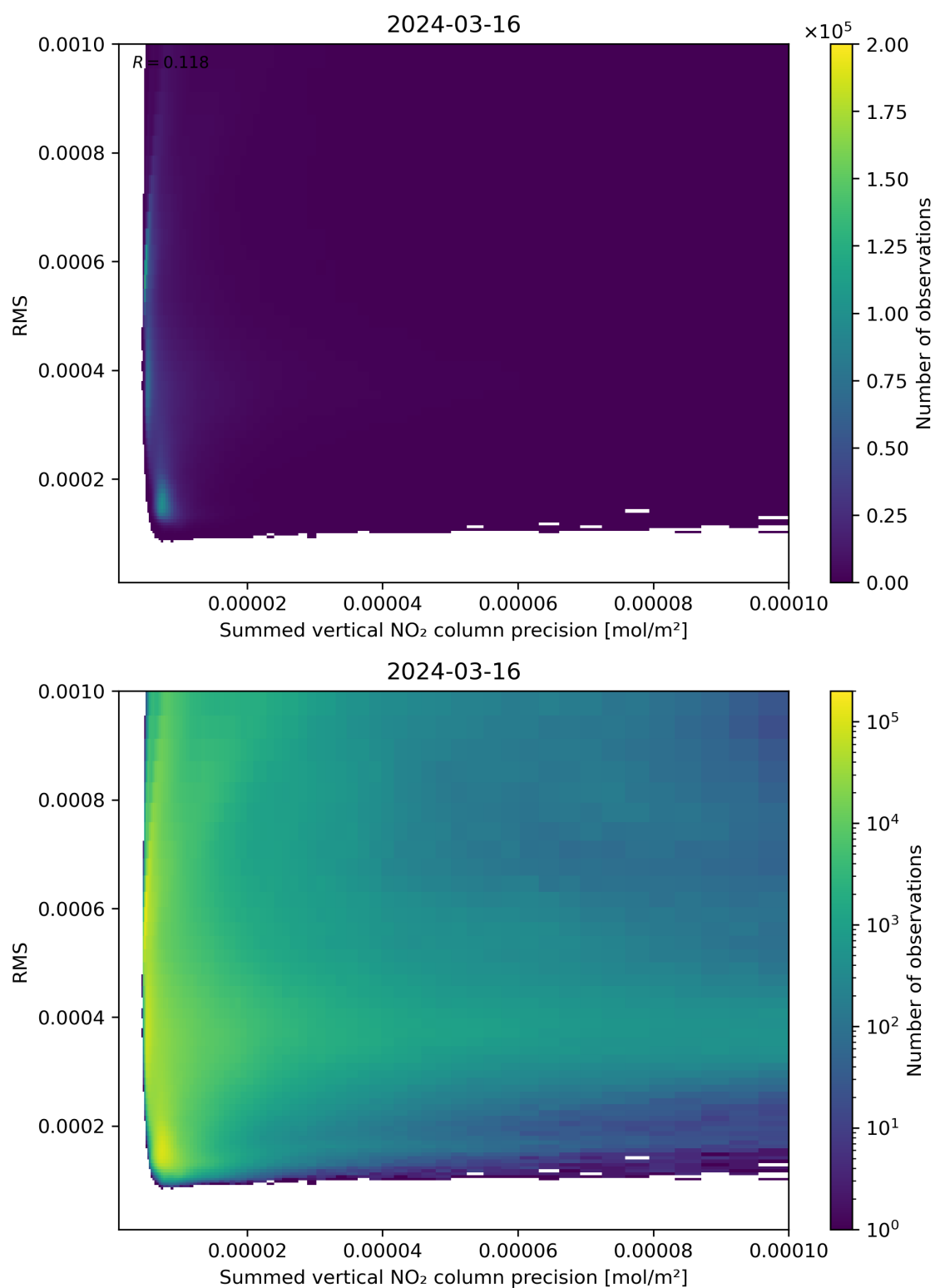
Figure 108: Scatter density plot of “Summed vertical NO 2 column precision” against “RMS” for 2024-03-15 to 2024-03-17.
