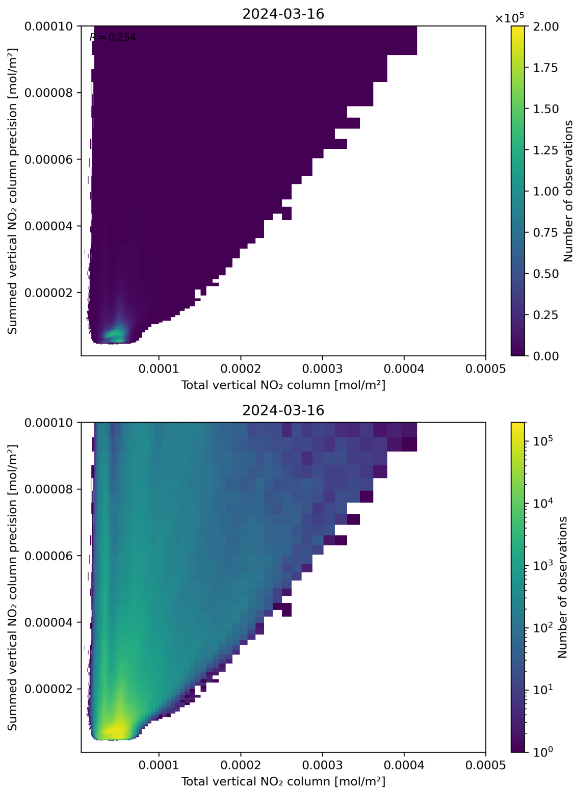
Figure 113: Scatter density plot of “Total vertical NO 2 column” against “Summed vertical NO 2 column precision” for 2024-03-15 to 2024-03-17.
