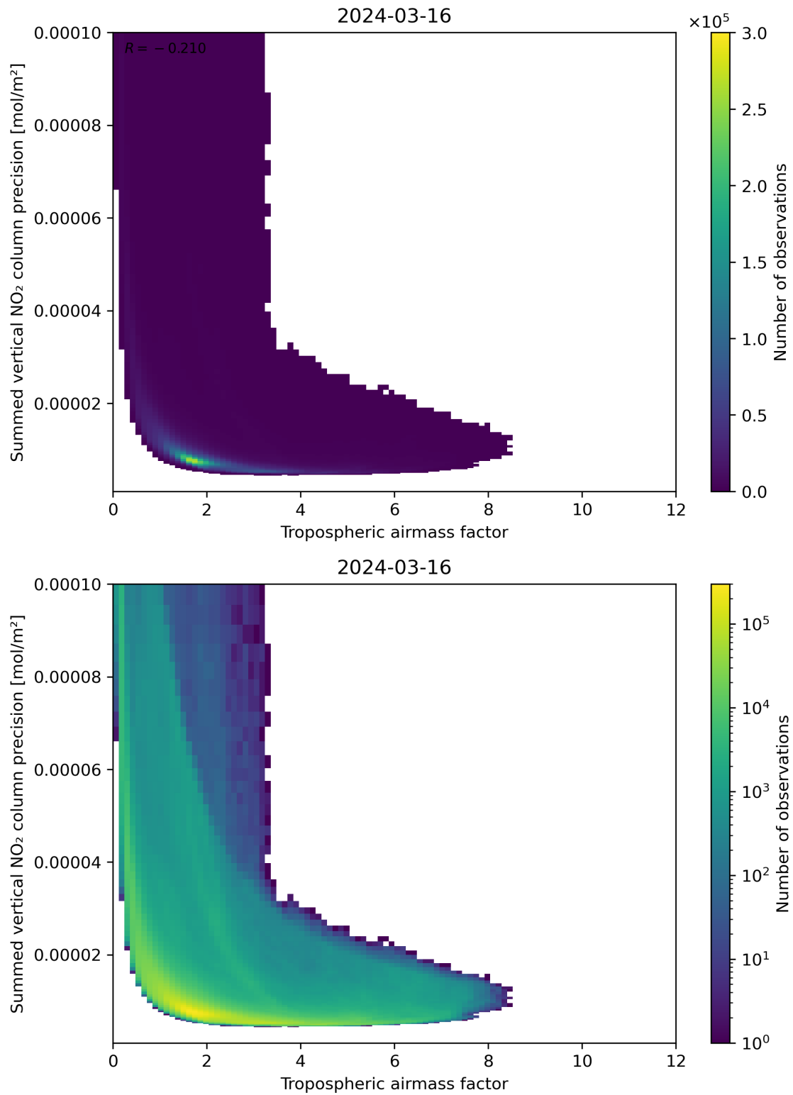
Figure 76: Scatter density plot of “Tropospheric air mass factor” against “Summed vertical NO 2 column precision” for 2024-03-15 to 2024-03-17.
