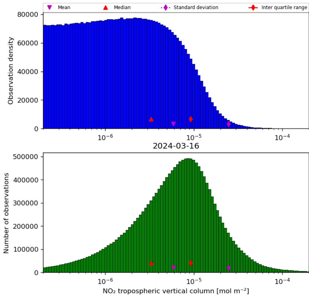
Figure 29: Histogram of “NO 2 tropospheric vertical column” for 2024-03-15 to 2024-03-17
