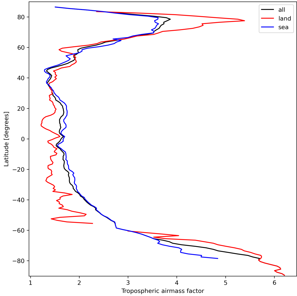
Figure 14: Zonal average of “Tropospheric airmass factor” for 2024-03-15 to 2024-03-17.
