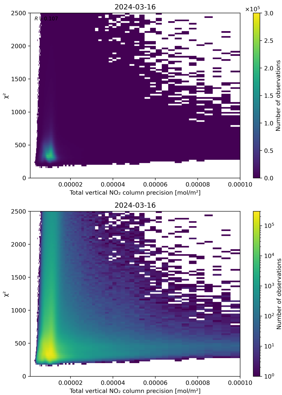
Figure 116: Scatter density plot of “Total vertical NO 2 column precision” against “ \chi^2 ” for 2024-03-15 to 2024-03-17.
