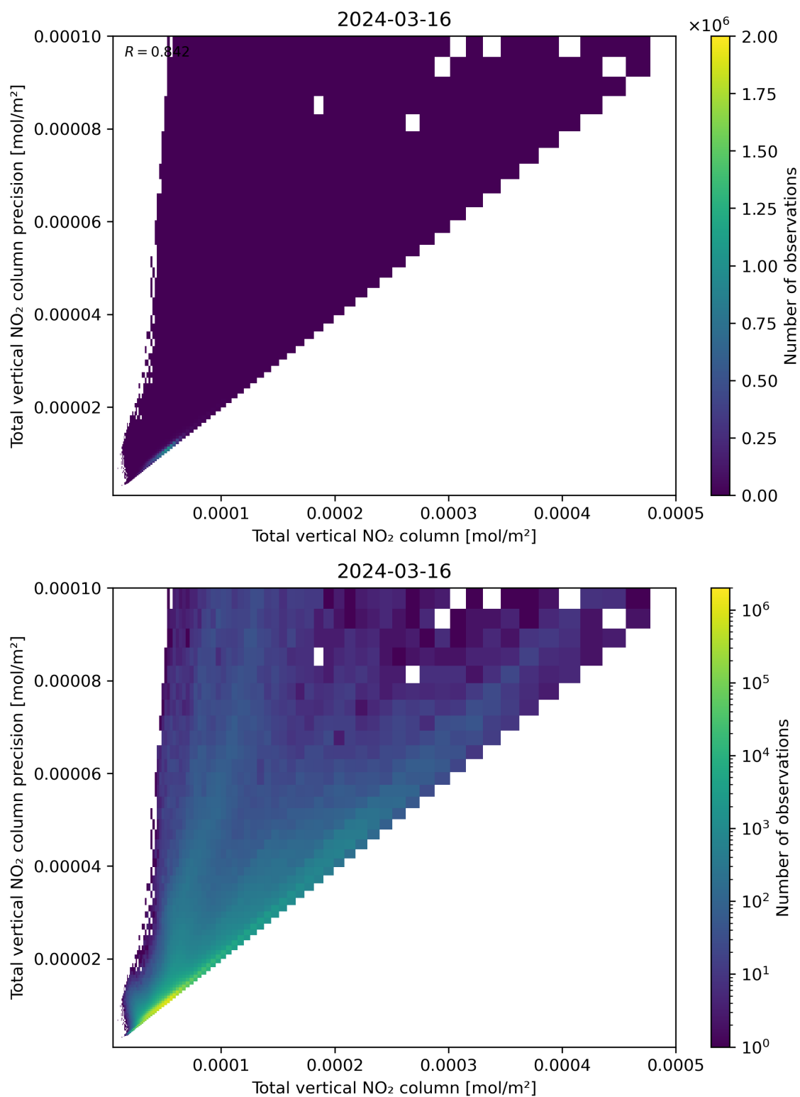
Figure 114: Scatter density plot of “Total vertical NO 2 column” against “Total vertical NO 2 column precision” for 2024-03-15 to 2024-03-17.
