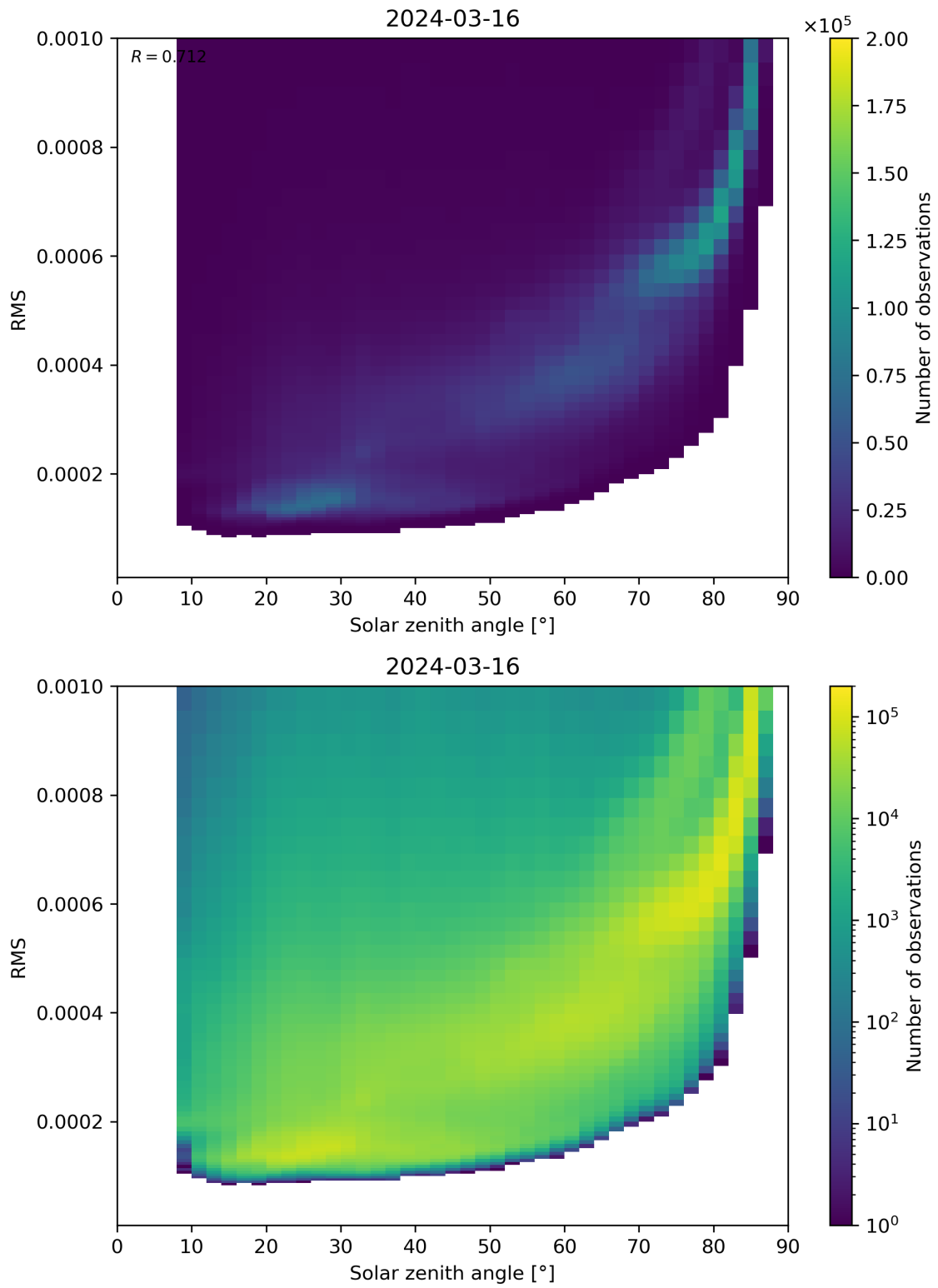
Figure 157: Scatter density plot of “Solar zenith angle” against “RMS” for 2024-03-15 to 2024-03-17.
