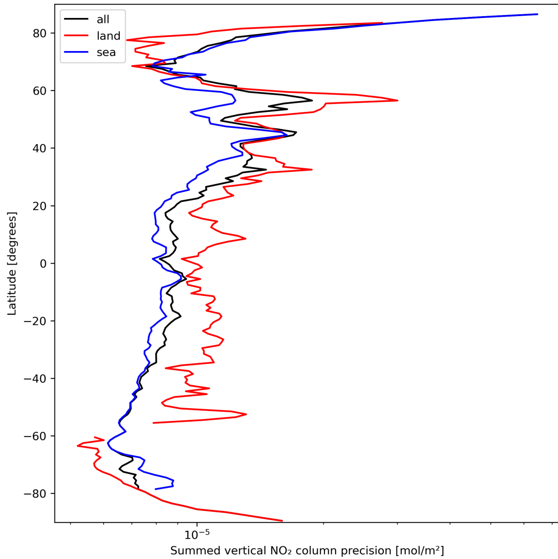
Figure 24: Zonal average of “Summed vertical NO 2 column precision” for 2024-03-15 to 2024-03-17.
