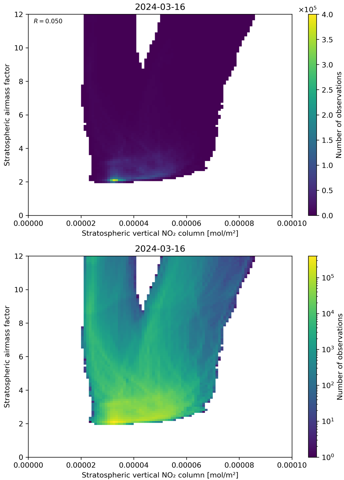
Figure 96: Scatter density plot of “Stratospheric vertical NO 2 column” against “Stratospheric airmass factor” for 2024-03-15 to 2024-03-17.
