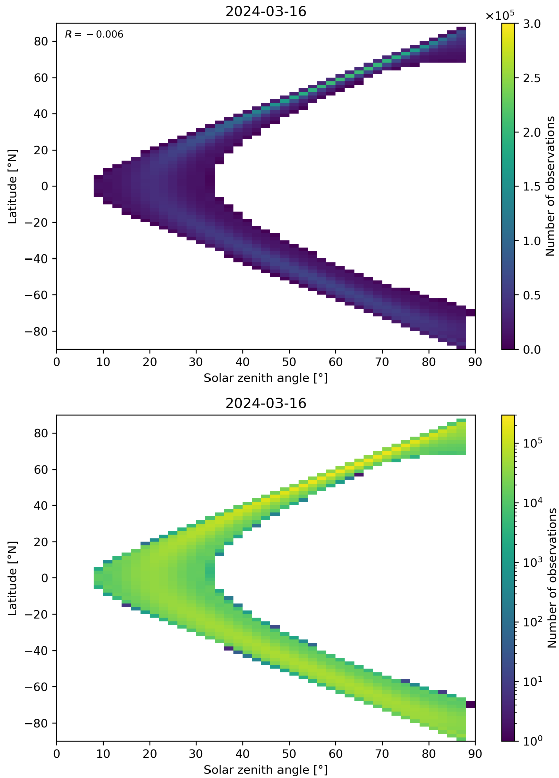
Figure 149: Scatter density plot of “Solar zenith angle” against “Latitude” for 2024-03-15 to 2024-03-17.
