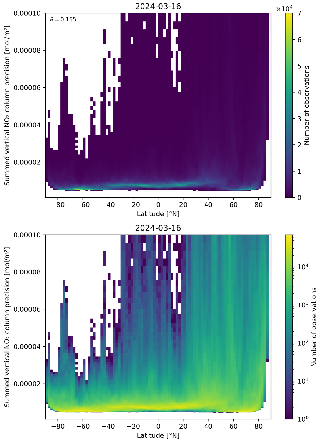
Figure 89: Scatter density plot of “Latitude” against “Summed vertical NO 2 column precision” for 2024-03-15 to 2024-03-17.
