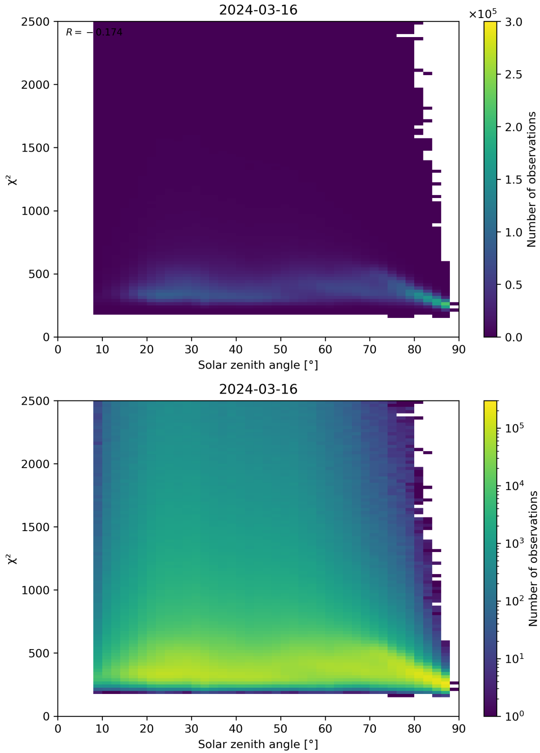
Figure 148: Scatter density plot of “Solar zenith angle” against “ \chi^2 ” for 2024-03-15 to 2024-03-17.
