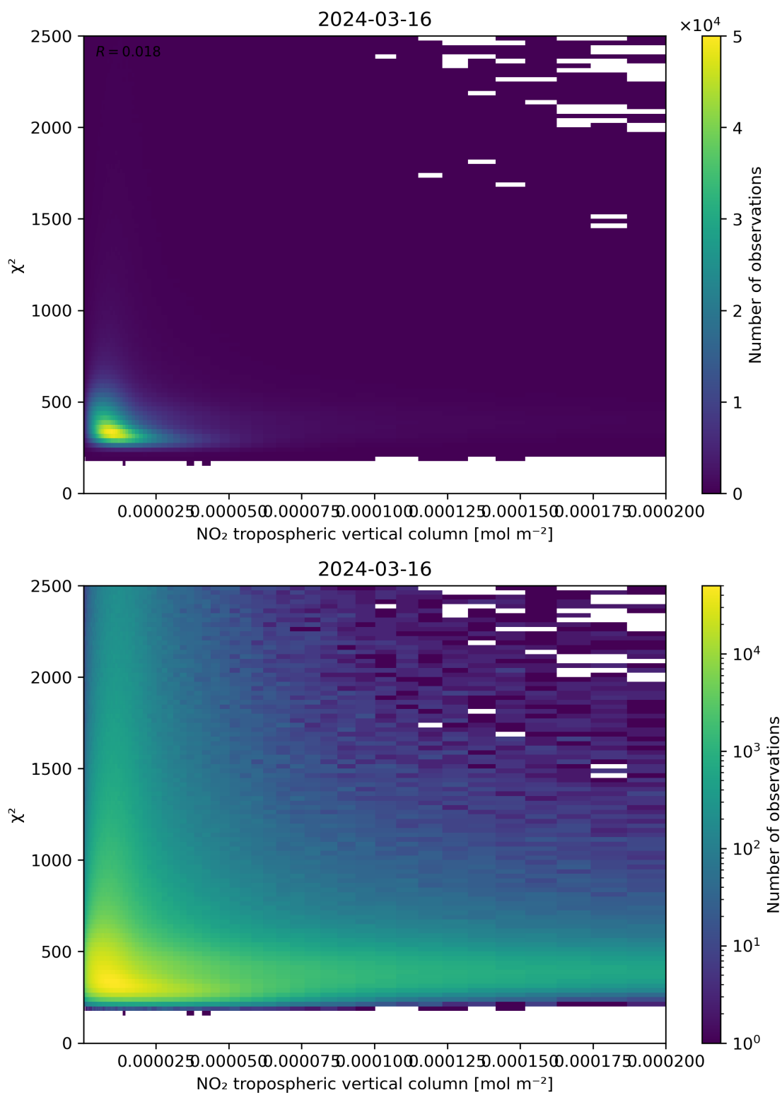
Figure 124: Scatter density plot of “NO 2 tropospheric vertical column” against “ \chi^2 ” for 2024-03-15 to 2024-03-17.
