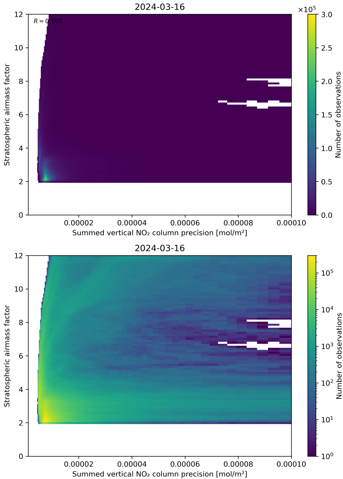
Figure 106: Scatter density plot of “Summed vertical NO 2 column precision” against “Stratospheric airmass factor” for 2024-03-15 to 2024-03-17.
