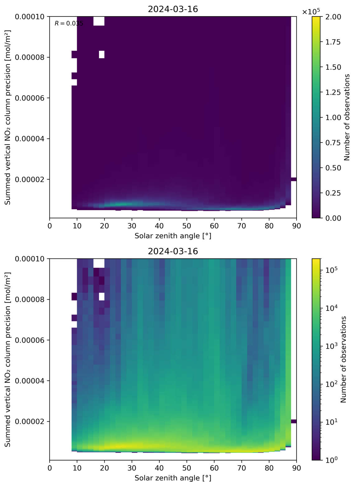
Figure 152: Scatter density plot of “Solar zenith angle” against “Summed vertical NO 2 column precision” for 2024-03-15 to 2024-03-17.
