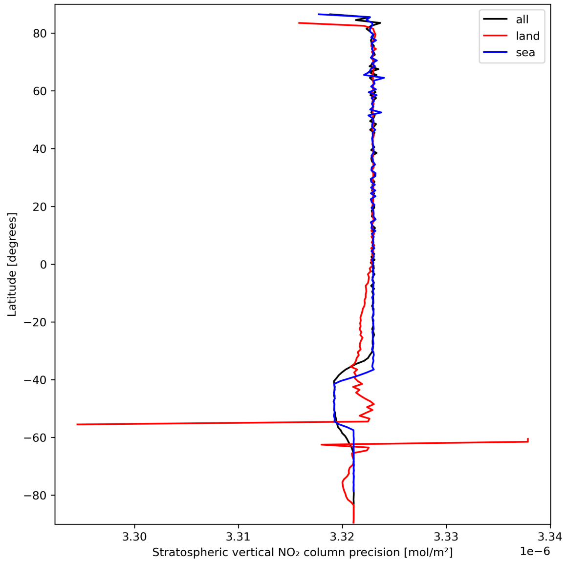
Figure 20: Zonal average of “Stratospheric vertical NO 2 column precision” for 2024-03-15 to 2024-03-17.
