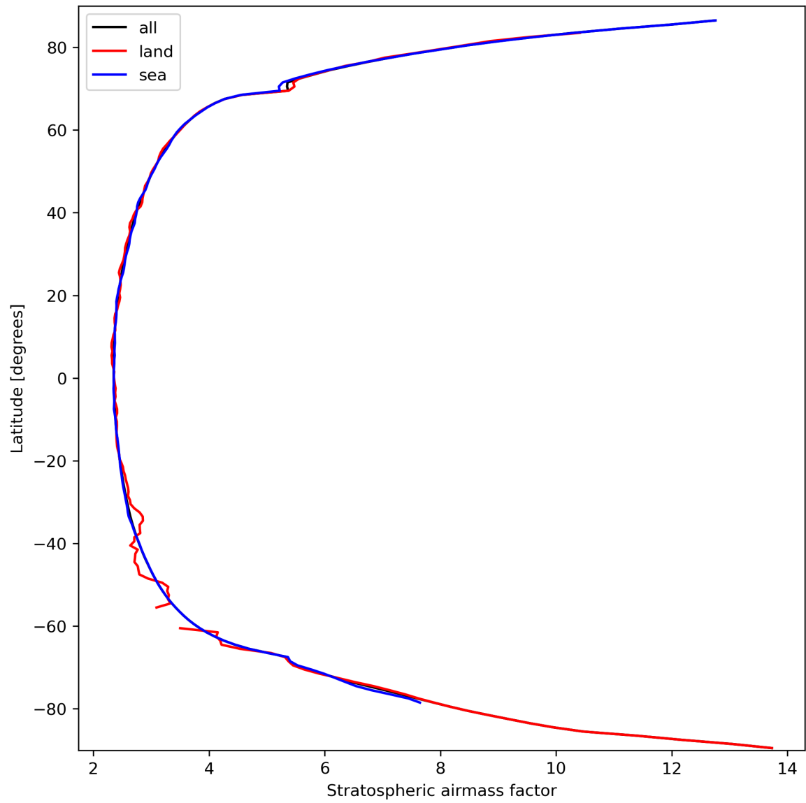
Figure 27: Zonal average of “Stratospheric air mass factor” for 2024-03-15 to 2024-03-17.
