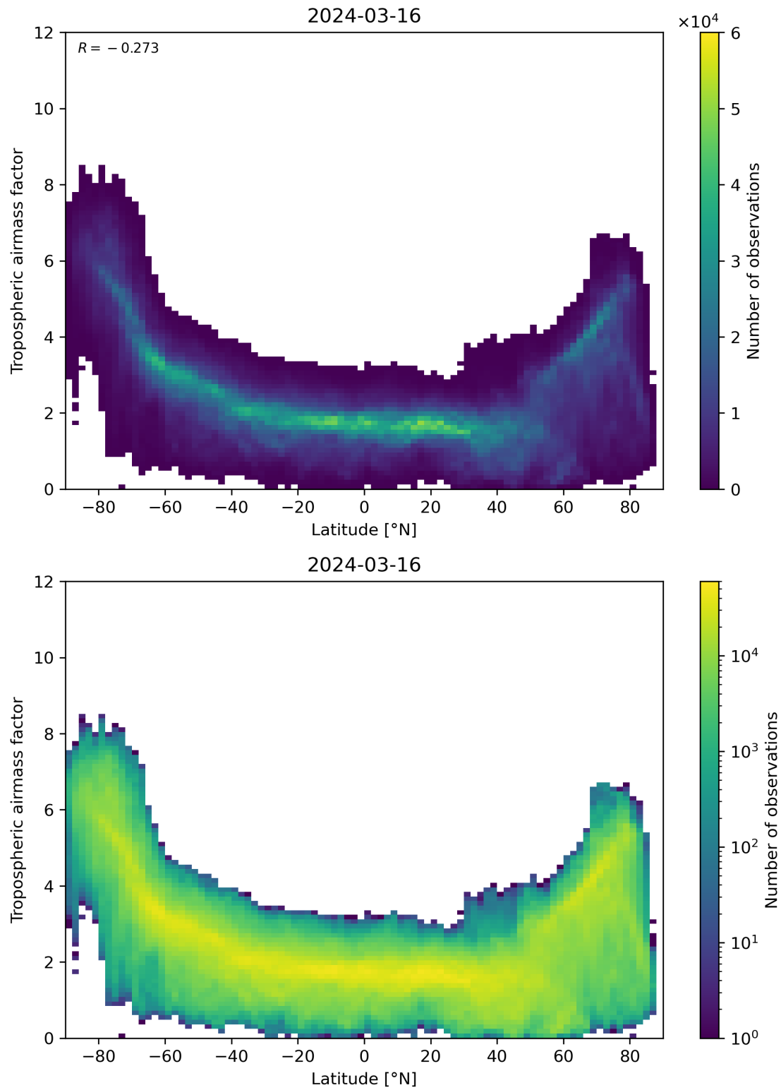
Figure 85: Scatter density plot of “Latitude” against “Tropospheric airmass factor” for 2024-03-15 to 2024-03-17.
