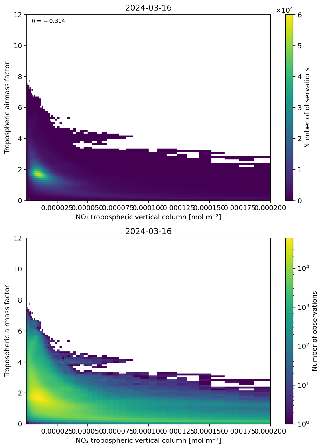
Figure 123: Scatter density plot of “NO 2 tropospheric vertical column” against “Tropospheric air mass factor” for 2024-03-15 to 2024-03-17.
