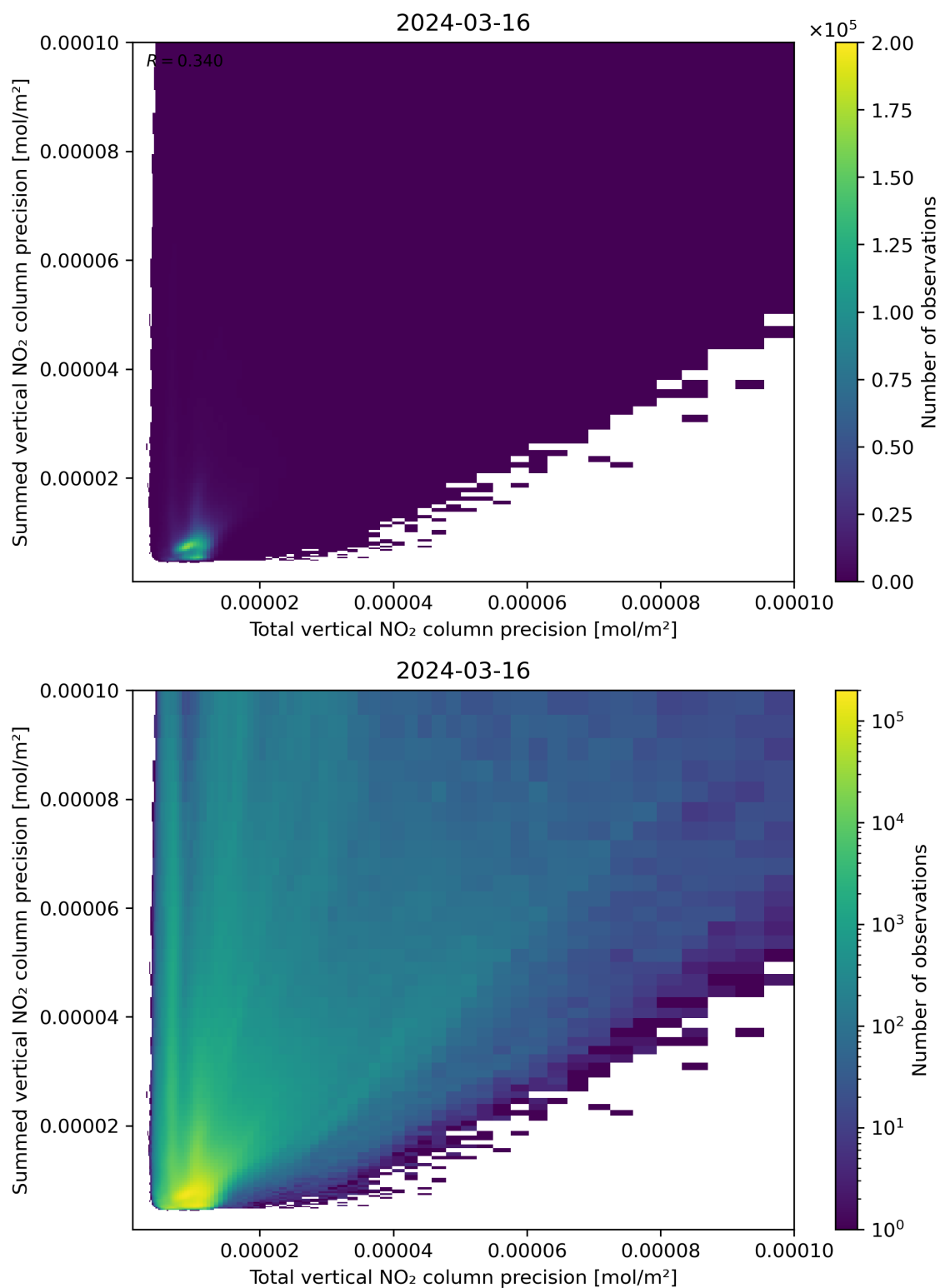
Figure 118: Scatter density plot of “Total vertical NO 2 column precision” against “Summed vertical NO 2 column precision” for 2024-03-15 to 2024-03-17.
