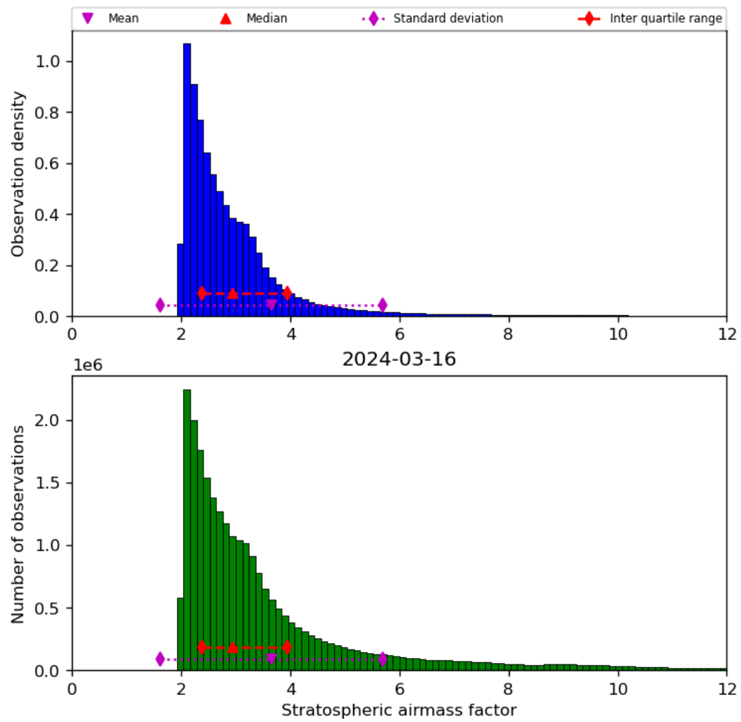
Figure 44: Histogram of “Stratospheric airmass factor” for 2024-03-15 to 2024-03-17
