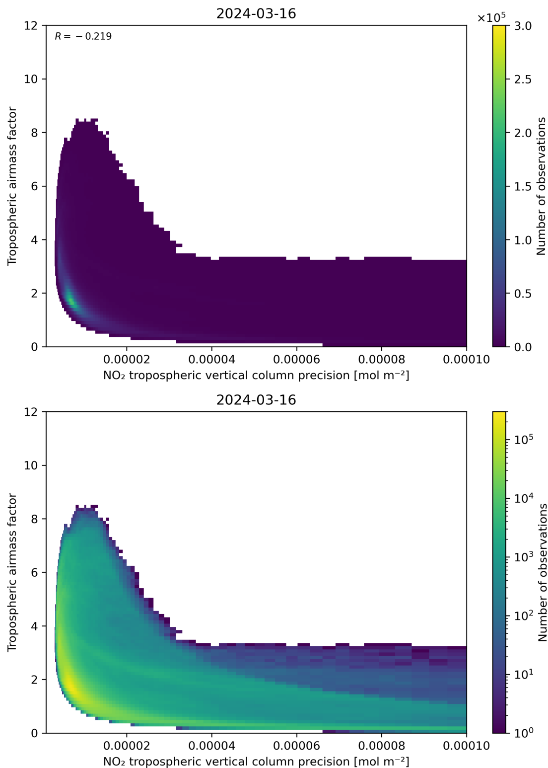
Figure 133: Scatter density plot of “NO 2 tropospheric vertical column precision” against “Tropospheric airmass factor” for 2024-03-15 to 2024-03-17.
