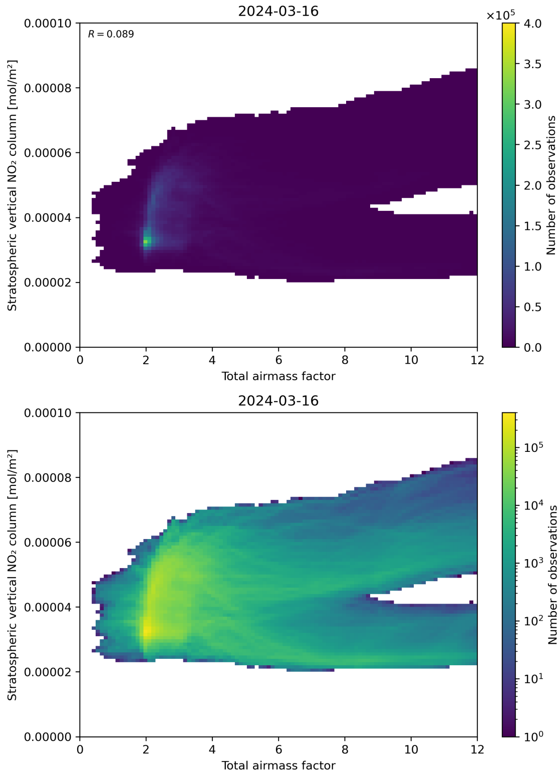
Figure 64: Scatter density plot of “Total airmass factor” against “Stratospheric vertical NO 2 column” for 2024-03-15 to 2024-03-17.
