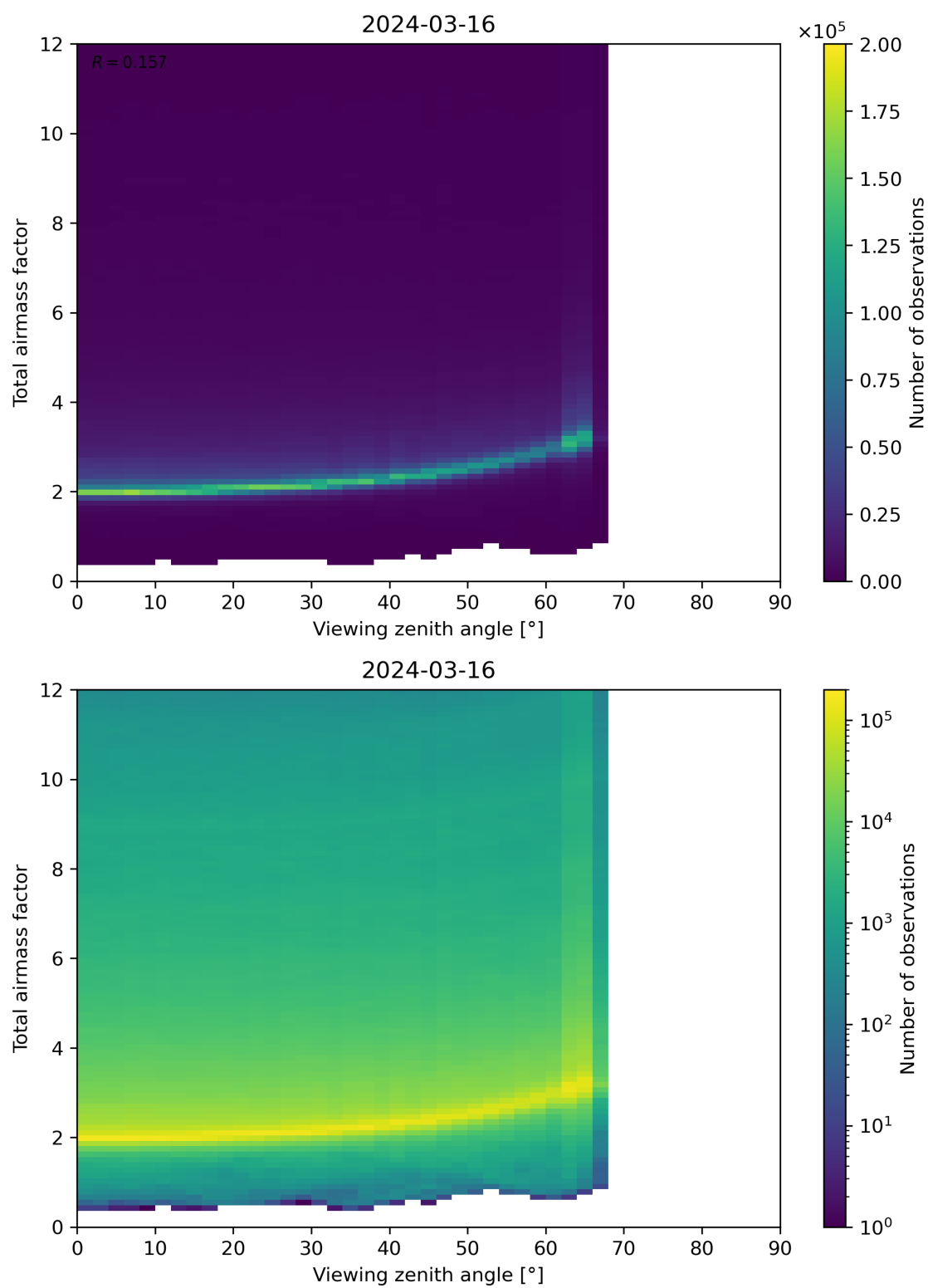
Figure 160: Scatter density plot of “Viewing zenith angle” against “Total airmass factor” for 2024-03-15 to 2024-03-17.
