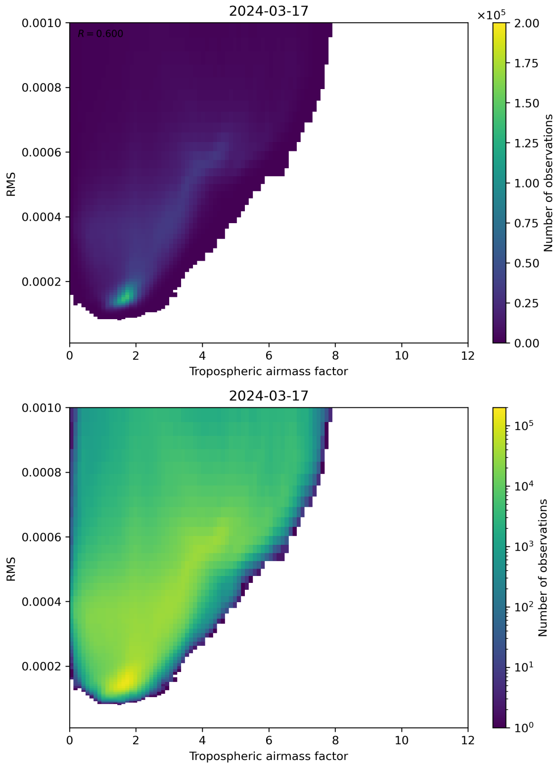
Figure 79: Scatter density plot of “Tropospheric airmass factor” against “RMS” for 2024-03-16 to 2024-03-18.
