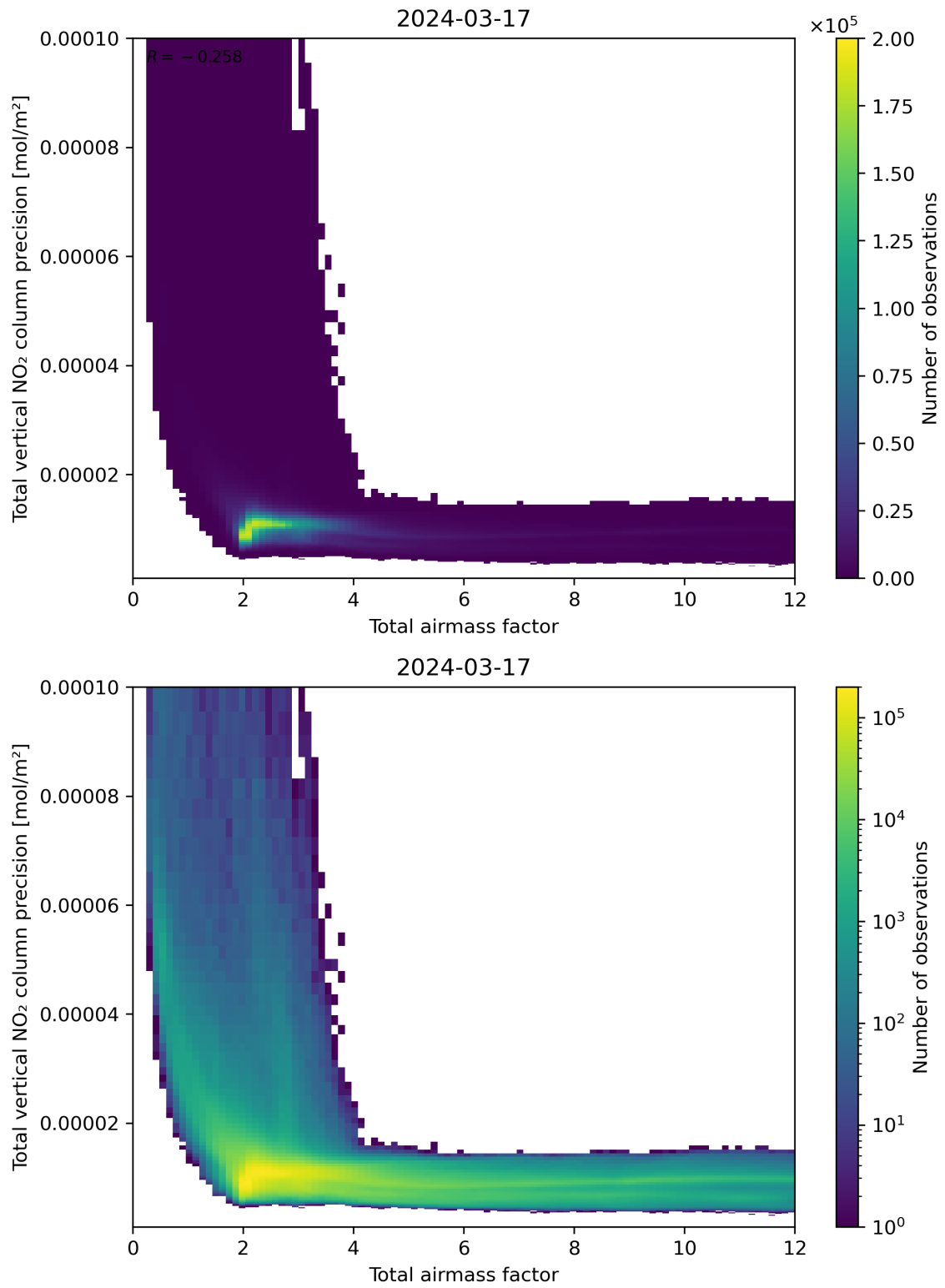
Figure 68: Scatter density plot of “Total airmass factor” against “Total vertical NO 2 column precision” for 2024-03-16 to 2024-03-18.
