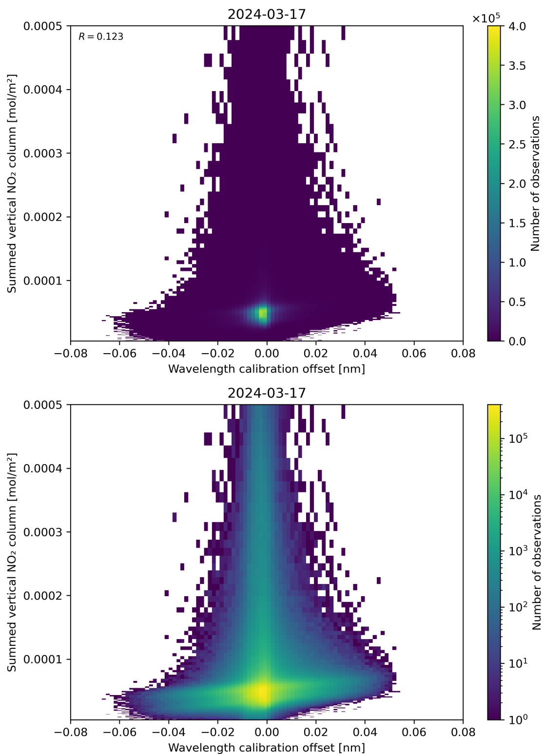
Figure 177: Scatter density plot of “Wavelength calibration offset” against “Summed vertical NO 2 column” for 2024-03-16 to 2024-03-18.
