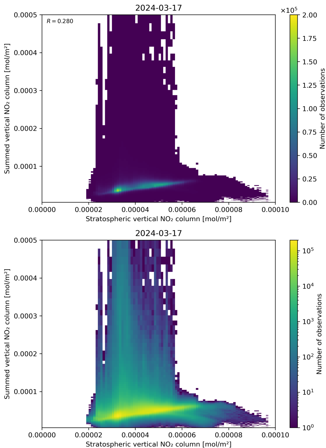
Figure 98: Scatter density plot of “Stratospheric vertical NO 2 column” against “Summed vertical NO 2 column” for 2024-03-16 to 2024-03-18.
