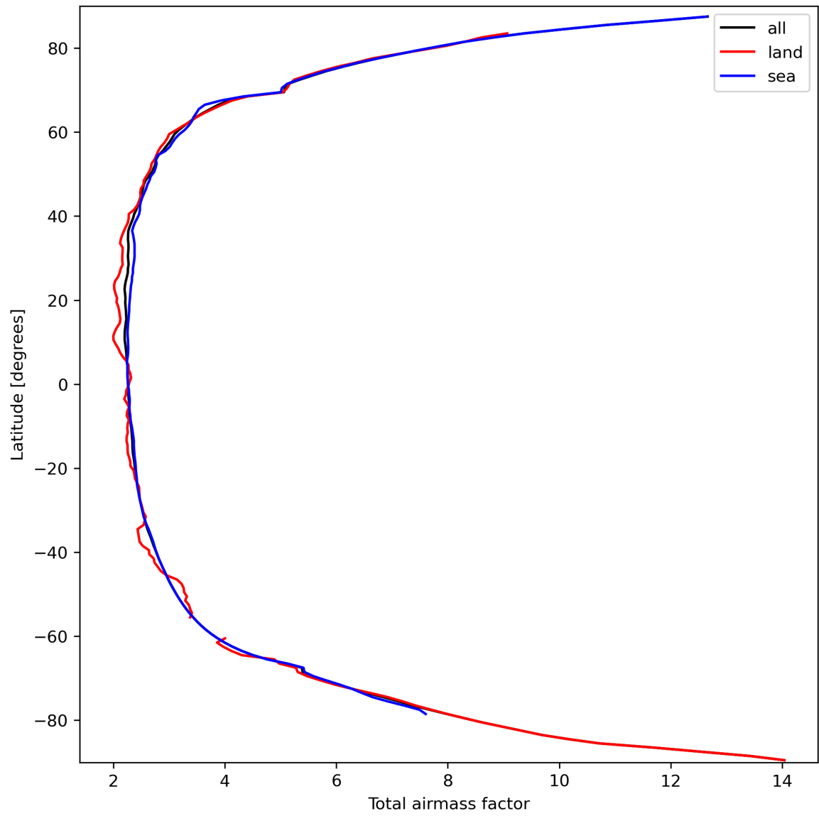
Figure 15: Zonal average of “Total airmass factor” for 2024-03-16 to 2024-03-18.
