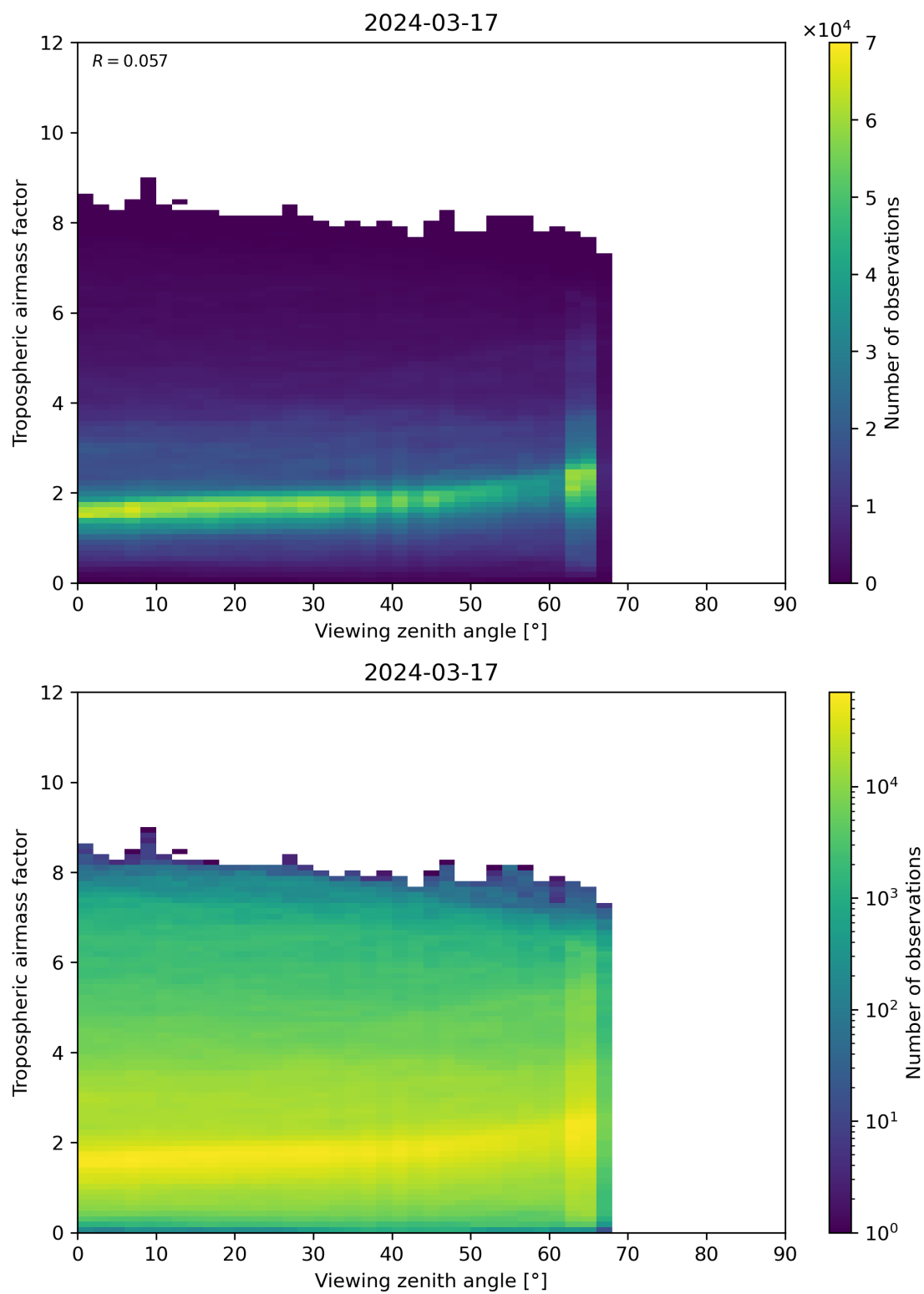
Figure 161: Scatter density plot of “Viewing zenith angle” against “Tropospheric airmass factor” for 2024-03-16 to 2024-03-18.
