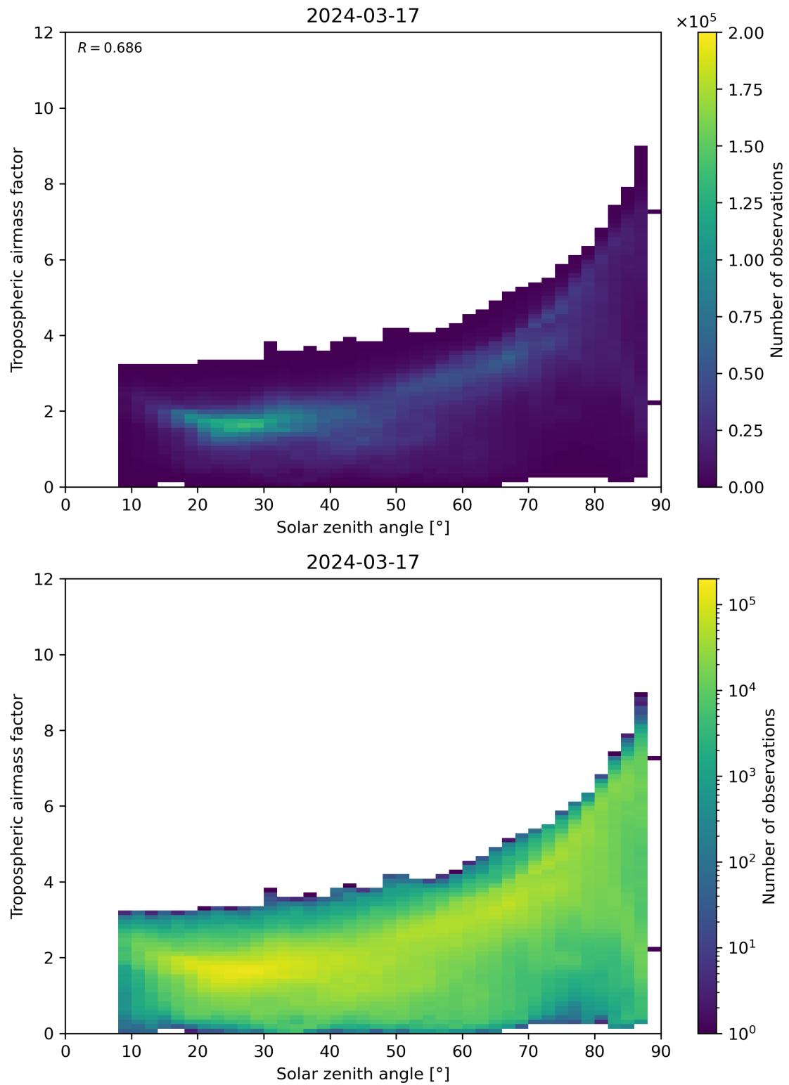
Figure 147: Scatter density plot of “Solar zenith angle” against “Tropospheric airmass factor” for 2024-03-16 to 2024-03-18.
