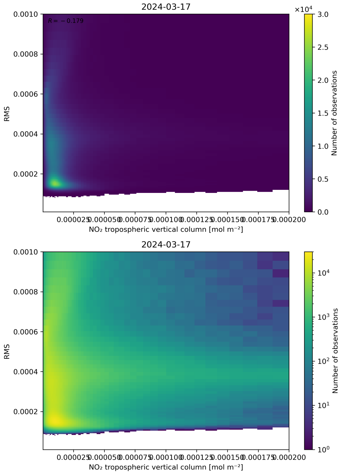
Figure 142: Scatter density plot of “NO 2 tropospheric vertical column” against “RMS” for 2024-03-16 to 2024-03-18.
