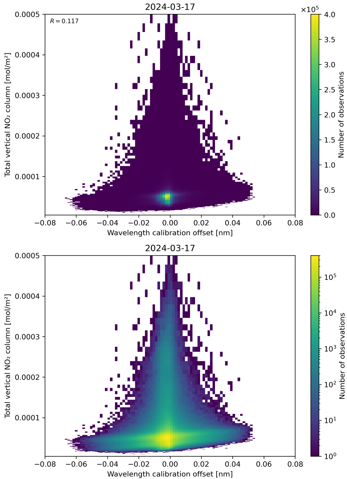
Figure 179: Scatter density plot of “Wavelength calibration offset” against “Total vertical NO 2 column” for 2024-03-16 to 2024-03-18.
