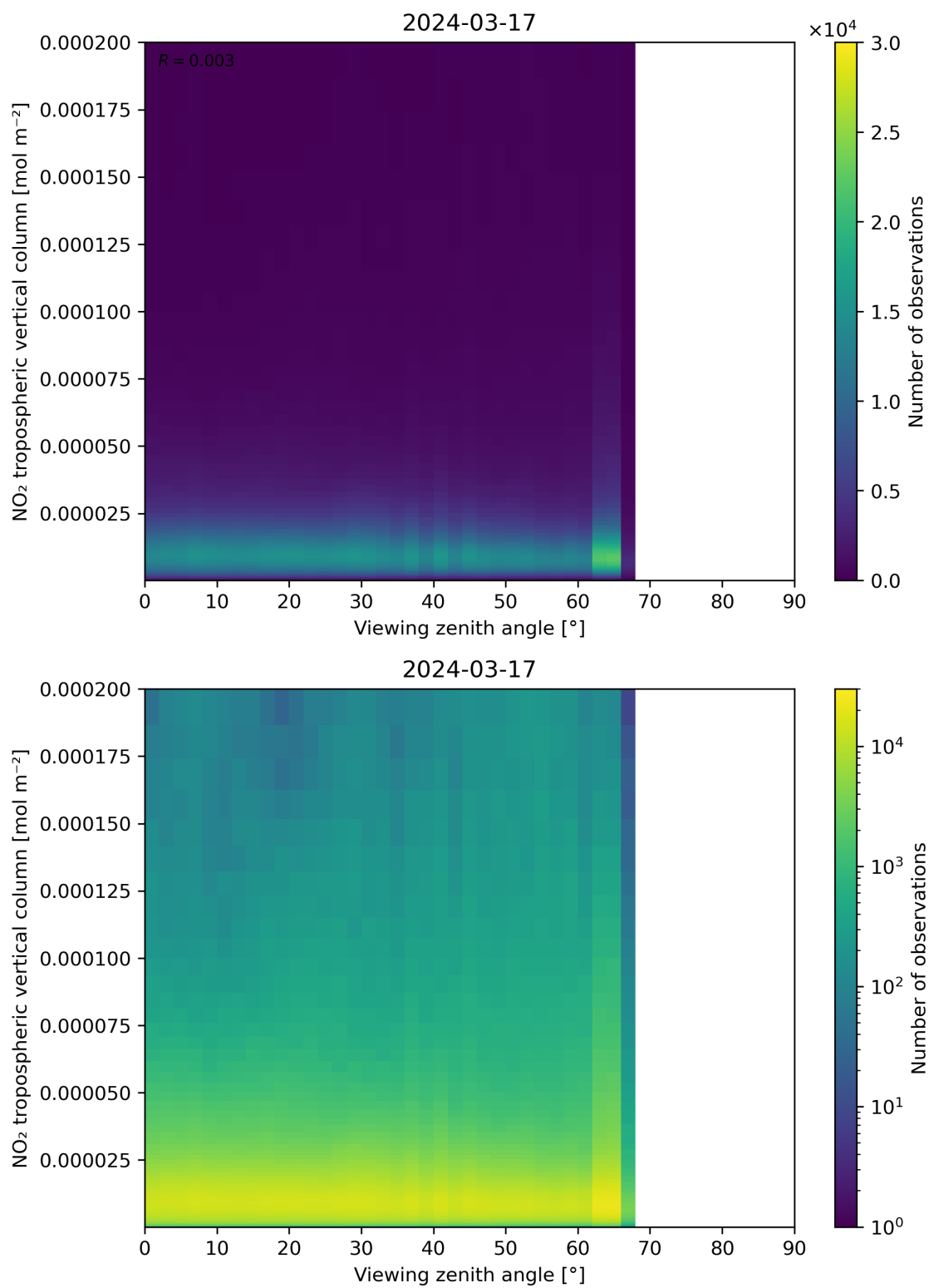
Figure 169: Scatter density plot of “Viewing zenith angle” against “NO 2 tropospheric vertical column” for 2024-03-16 to 2024-03-18.
