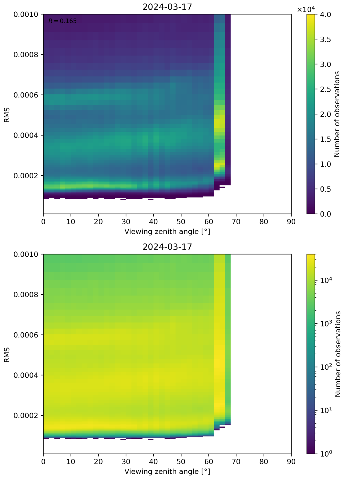
Figure 171: Scatter density plot of “Viewing zenith angle” against “RMS” for 2024-03-16 to 2024-03-18.
