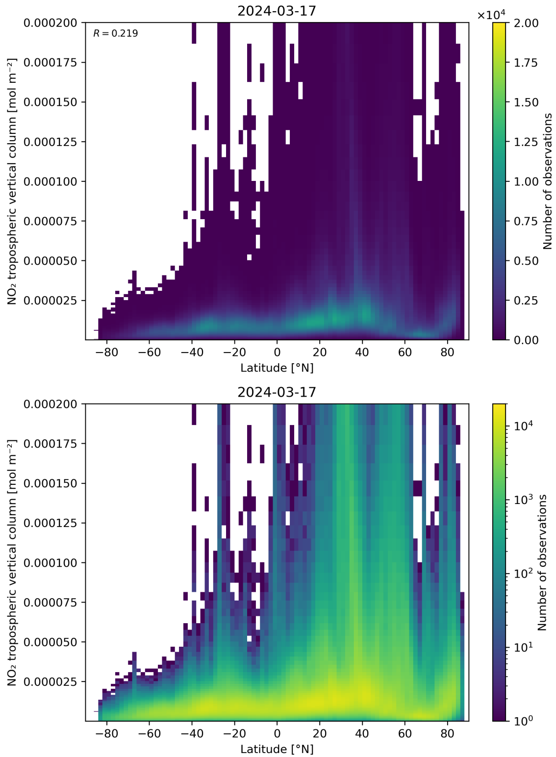
Figure 92: Scatter density plot of “Latitude” against “NO 2 tropospheric vertical column” for 2024-03-16 to 2024-03-18.
