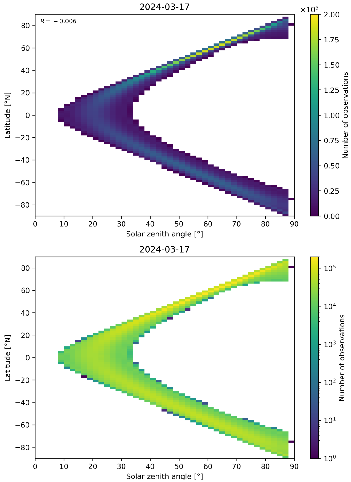
Figure 149: Scatter density plot of “Solar zenith angle” against “Latitude” for 2024-03-16 to 2024-03-18.
