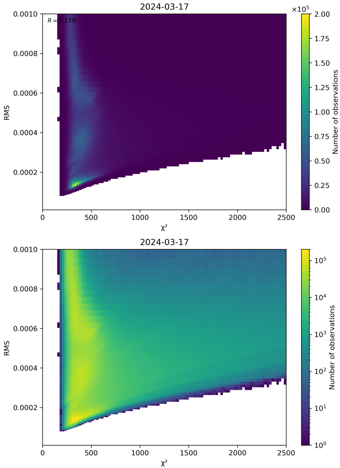
Figure 82: Scatter density plot of “ \chi^2 ” against “RMS” for 2024-03-16 to 2024-03-18.
