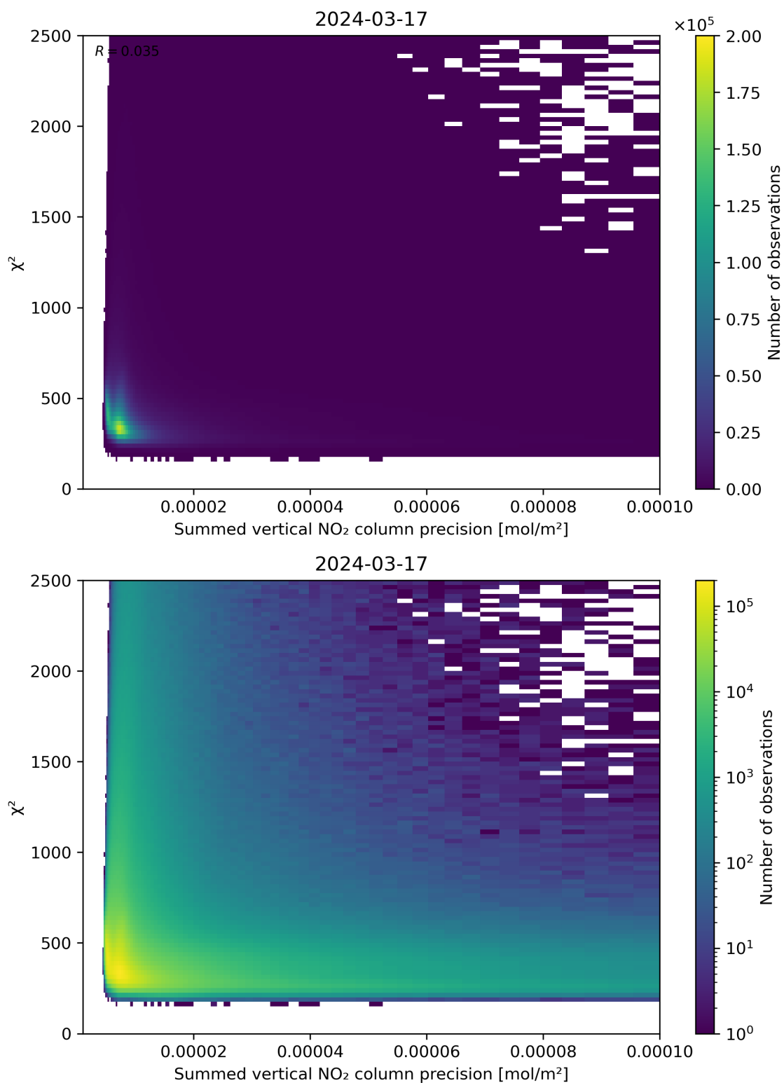
Figure 107: Scatter density plot of “Summed vertical NO 2 column precision” against “ \chi^2 ” for 2024-03-16 to 2024-03-18.
