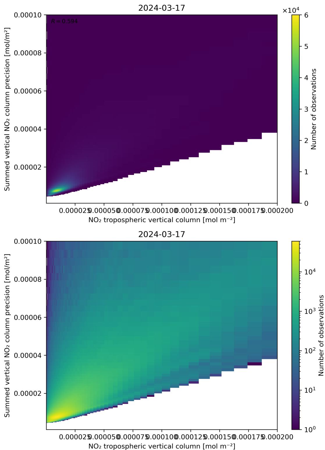
Figure 127: Scatter density plot of “NO 2 tropospheric vertical column” against “Summed vertical NO 2 column precision” for 2024-03-16 to 2024-03-18.
