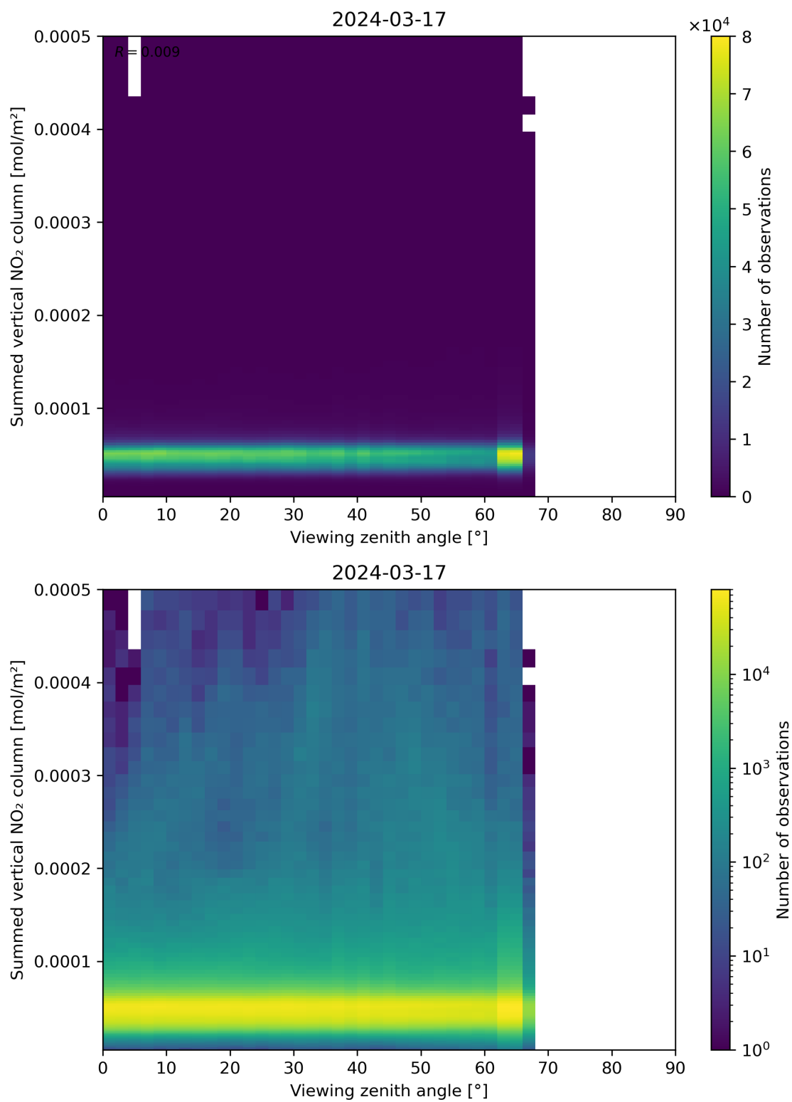
Figure 165: Scatter density plot of “Viewing zenith angle” against “Summed vertical NO 2 column” for 2024-03-16 to 2024-03-18.
