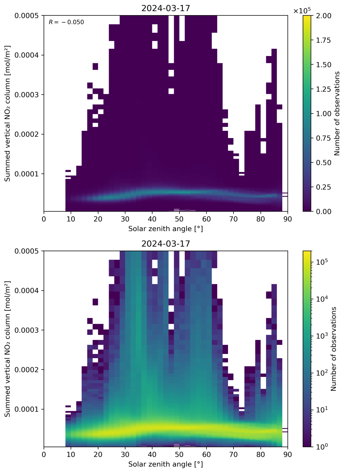
Figure 151: Scatter density plot of “Solar zenith angle” against “Summed vertical NO 2 column” for 2024-03-16 to 2024-03-18.
