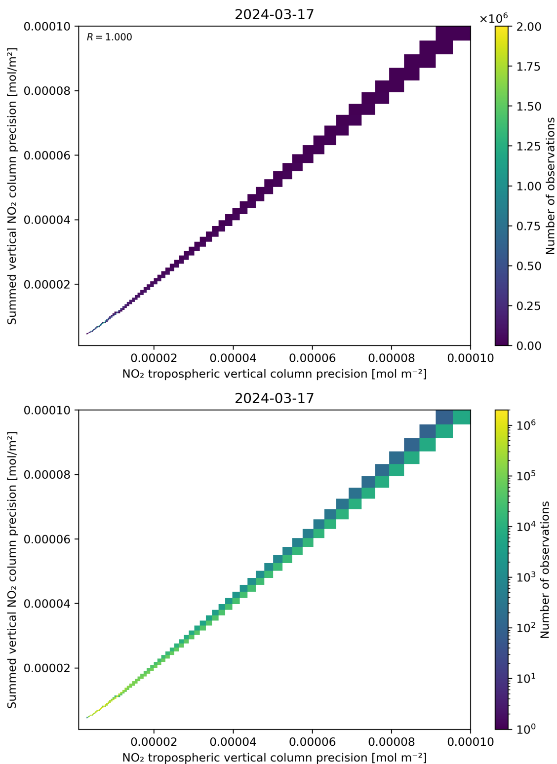
Figure 137: Scatter density plot of “NO 2 tropospheric vertical column precision” against “Summed vertical NO 2 column precision” for 2024-03-16 to 2024-03-18.
