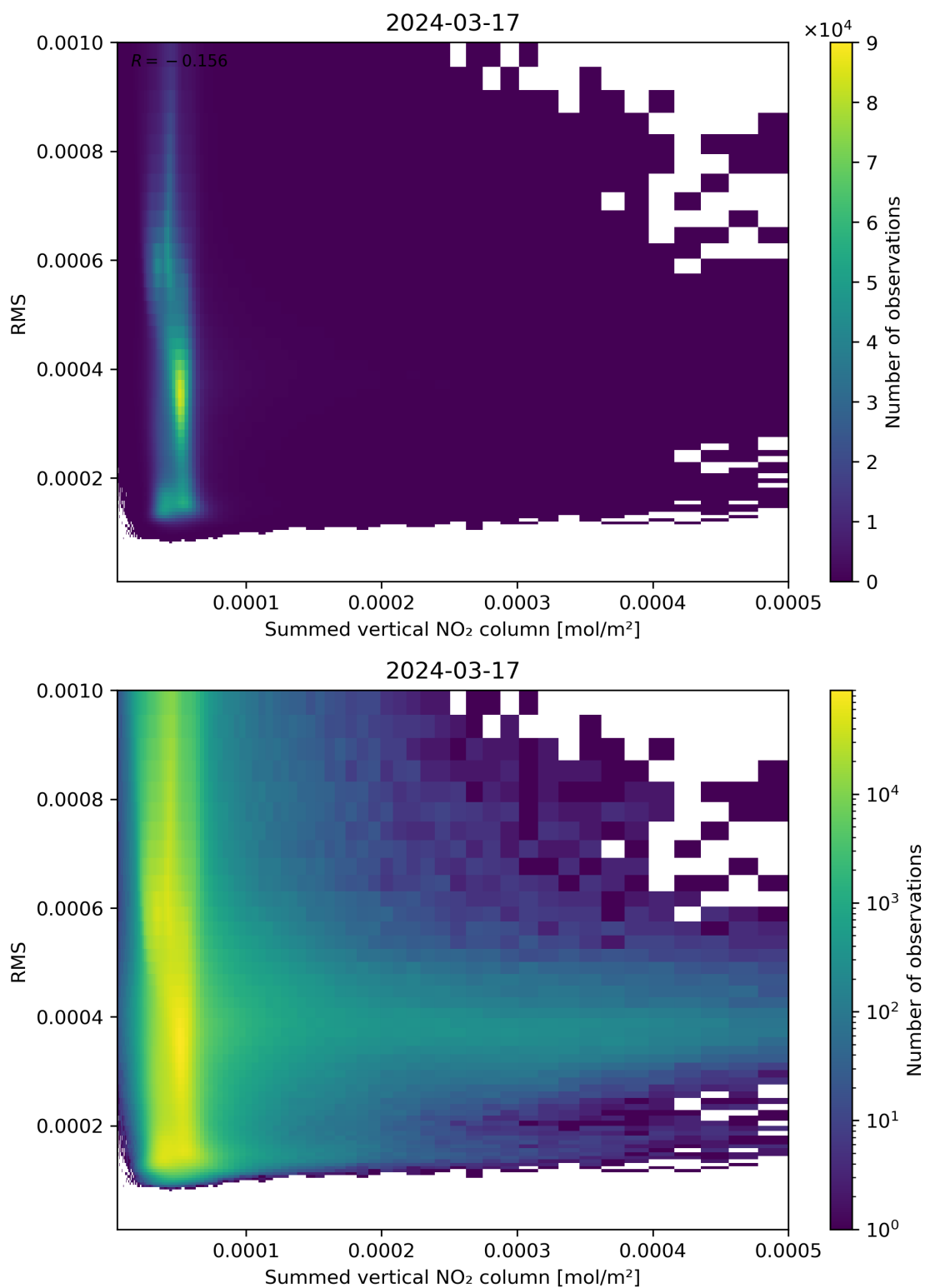
Figure 109: Scatter density plot of “Summed vertical NO 2 column” against “RMS” for 2024-03-16 to 2024-03-18.
