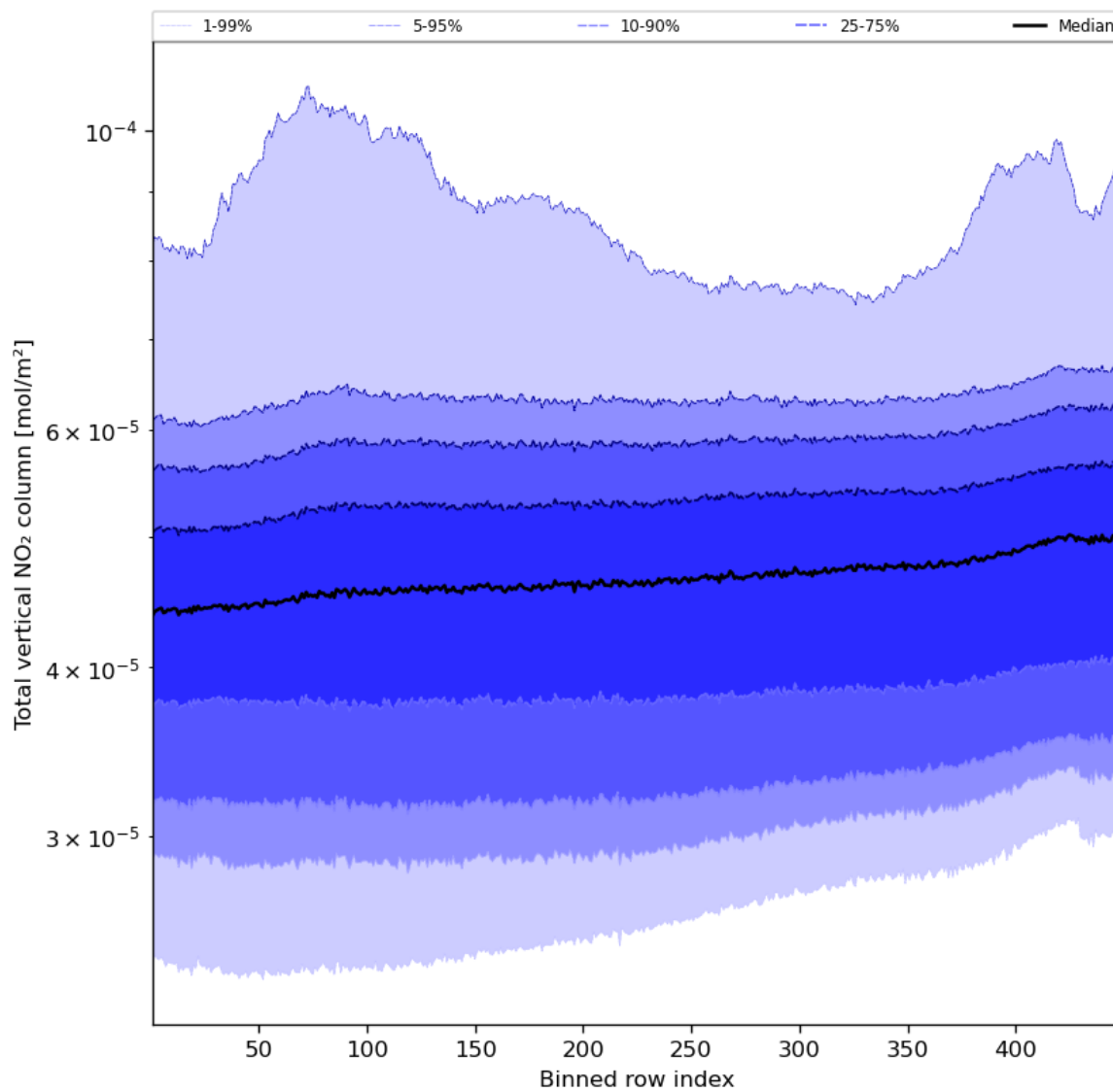
Figure 55: Along track statistics of “Total vertical NO 2 column” for 2024-03-16 to 2024-03-18
