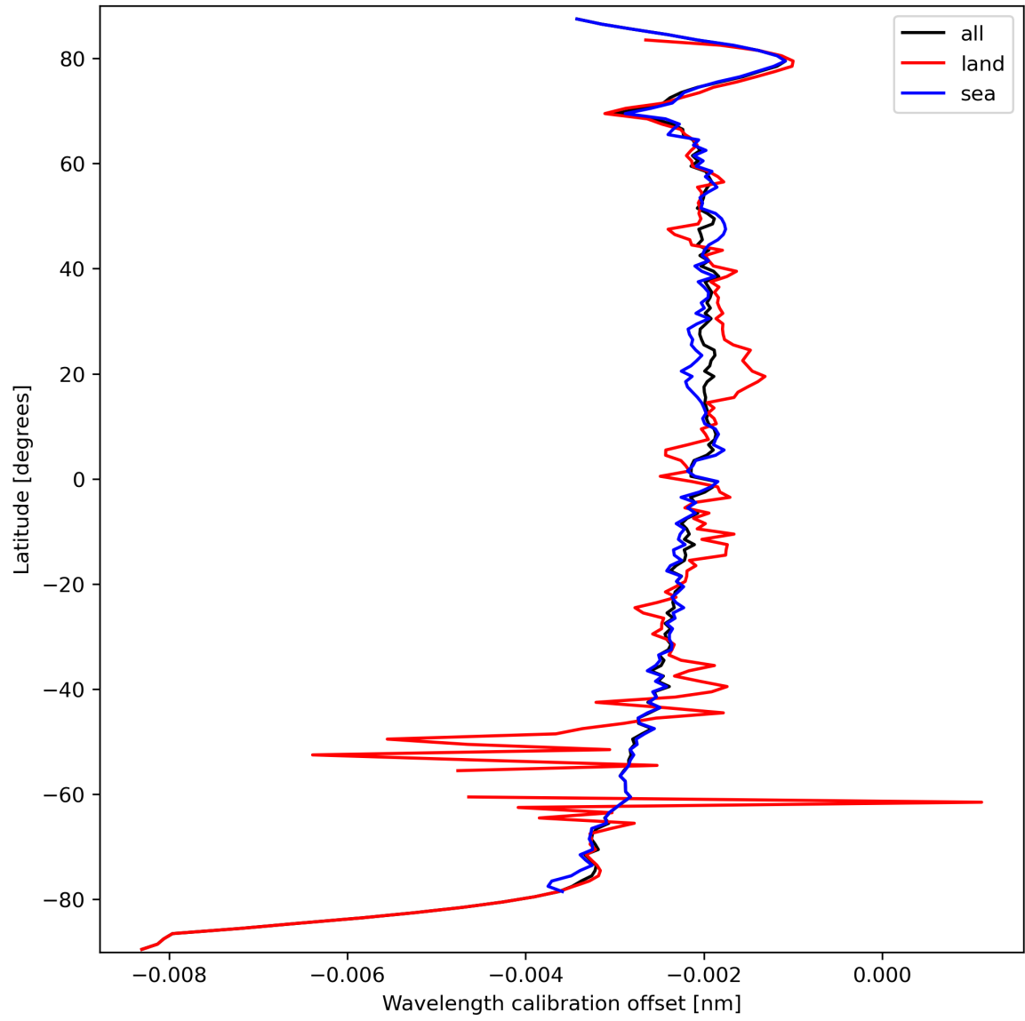
Figure 18: Zonal average of “Wavelength calibration offset” for 2024-03-16 to 2024-03-18.
