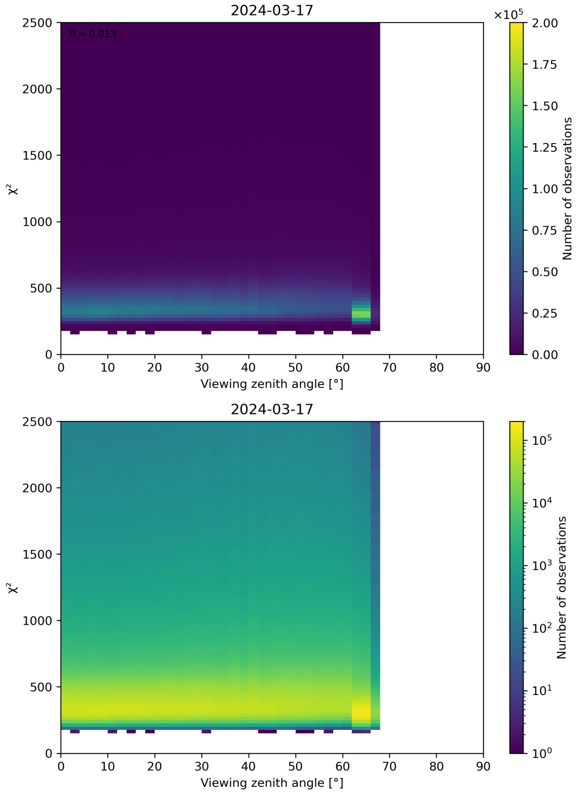
Figure 162: Scatter density plot of “Viewing zenith angle” against “ \chi^2 ” for 2024-03-16 to 2024-03-18.
