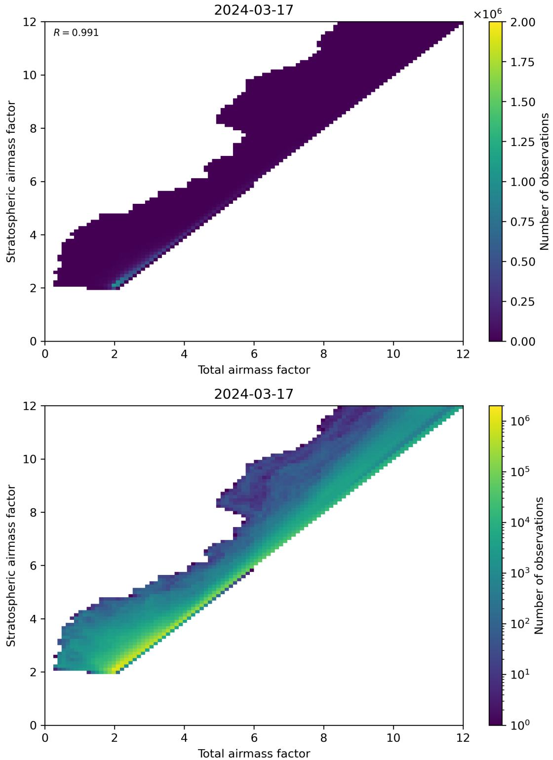
Figure 62: Scatter density plot of “Total airmass factor” against “Stratospheric airmass factor” for 2024-03-16 to 2024-03-18.
