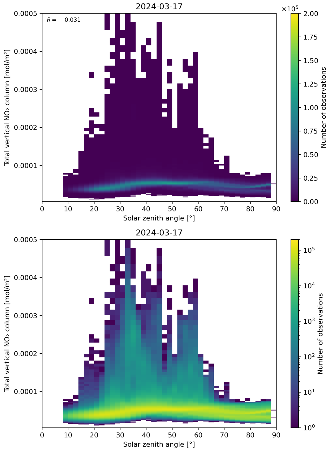
Figure 153: Scatter density plot of “Solar zenith angle” against “Total vertical NO 2 column” for 2024-03-16 to 2024-03-18.
