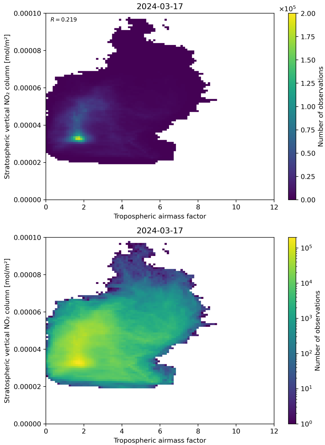
Figure 74: Scatter density plot of “Tropospheric air mass factor” against “Stratospheric vertical NO 2 column” for 2024-03-16 to 2024-03-18.
