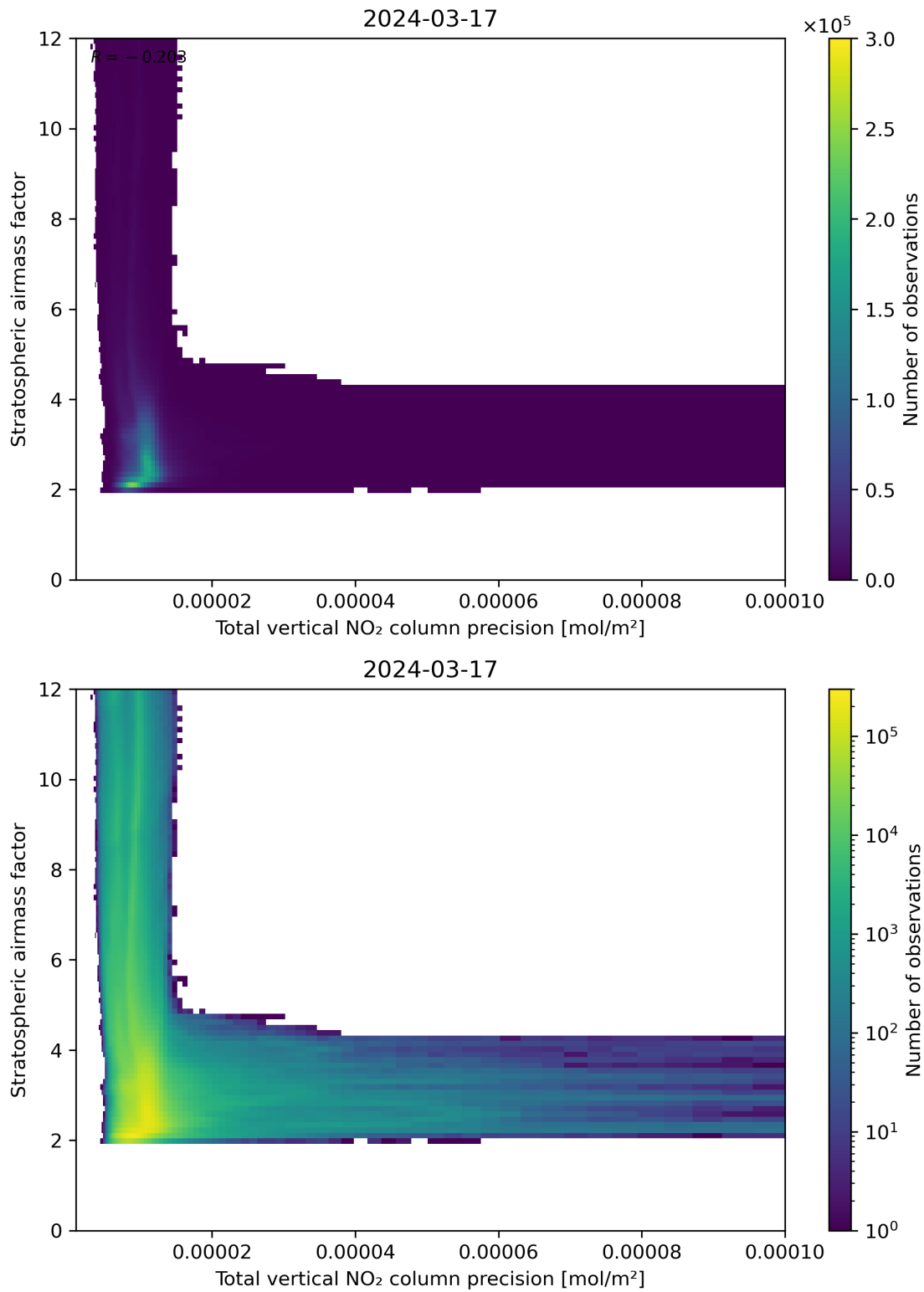
Figure 115: Scatter density plot of “Total vertical NO 2 column precision” against “Stratospheric air mass factor” for 2024-03-16 to 2024-03-18.
