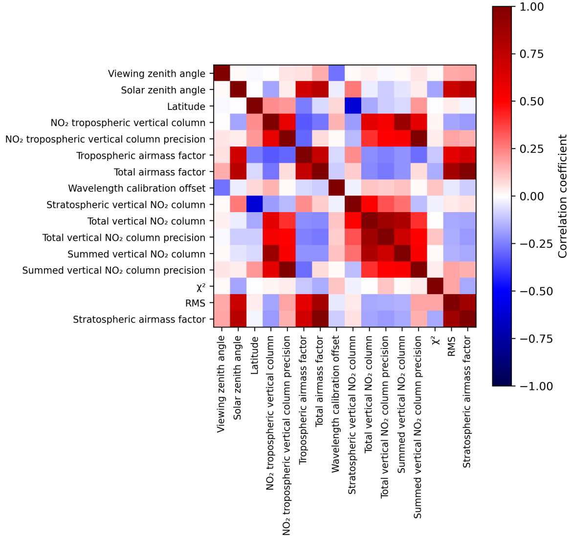
Figure 2: Map of correlation matrix for 2024-03-16 to 2024-03-18.
