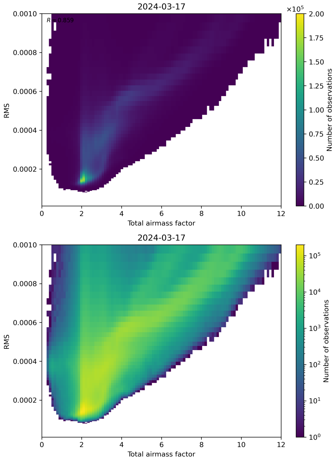
Figure 69: Scatter density plot of “Total airmass factor” against “RMS” for 2024-03-16 to 2024-03-18.
