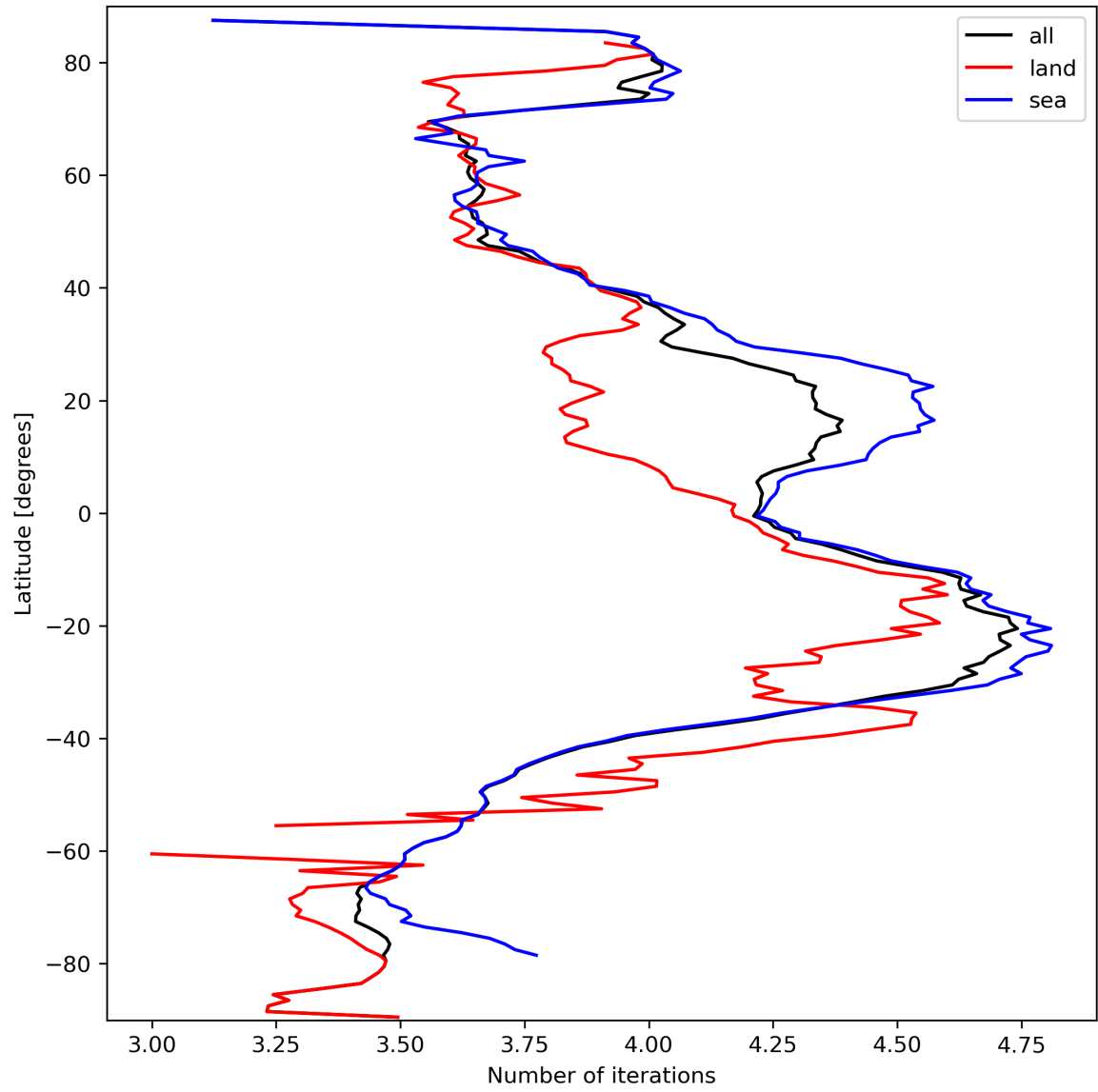
Figure 17: Zonal average of “Number of iterations” for 2024-03-16 to 2024-03-18.
