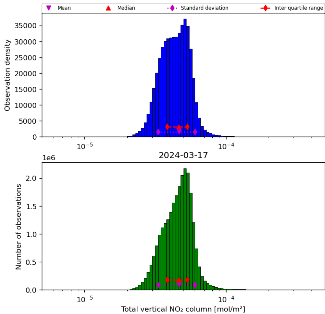
Figure 38: Histogram of “Total vertical NO 2 column” for 2024-03-16 to 2024-03-18
