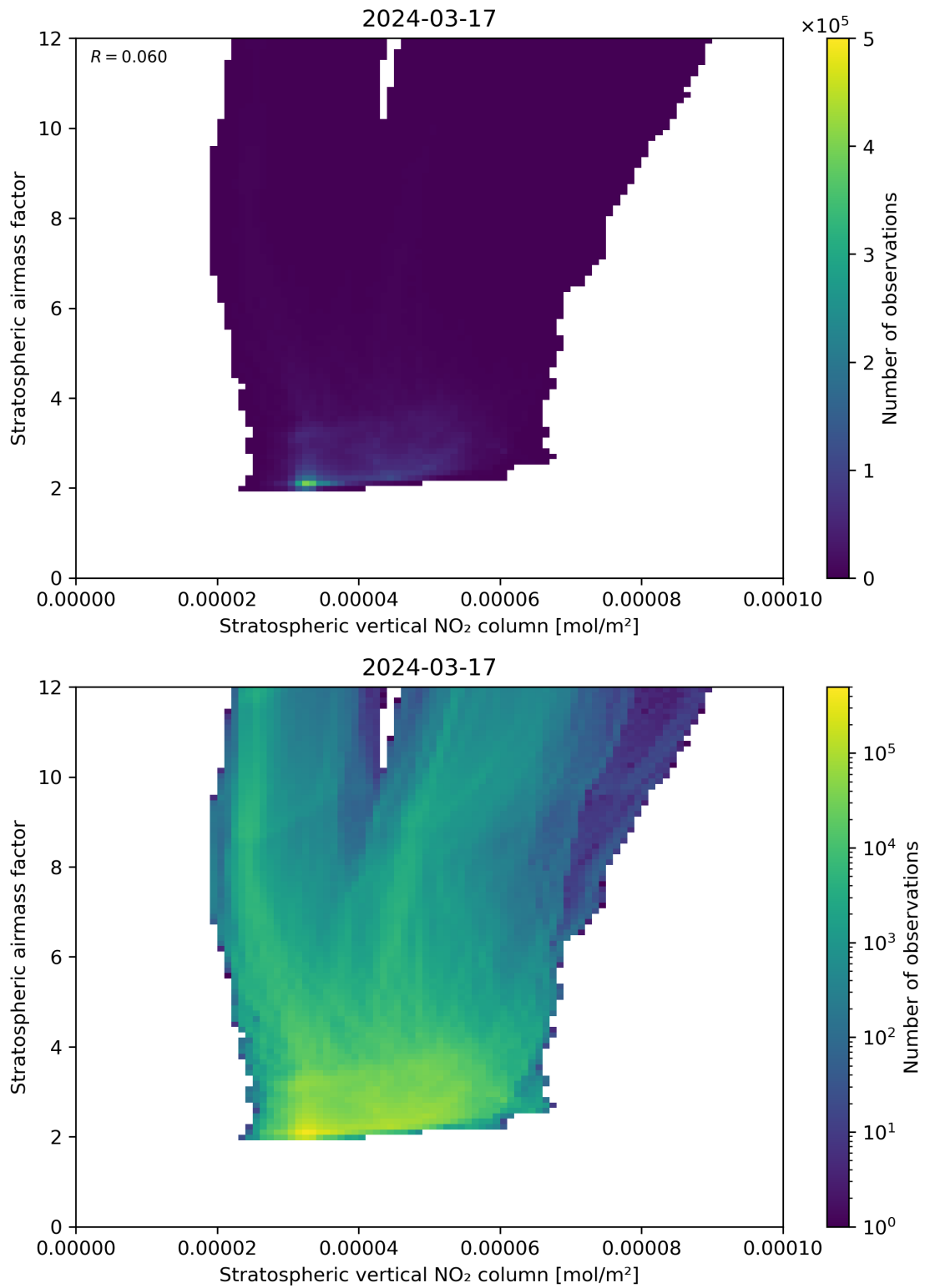
Figure 96: Scatter density plot of “Stratospheric vertical NO 2 column” against “Stratospheric airmass factor” for 2024-03-16 to 2024-03-18.
