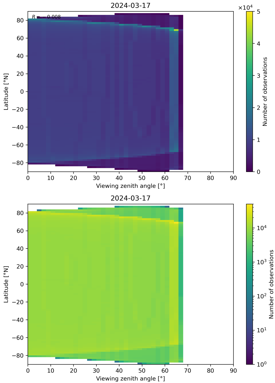
Figure 163: Scatter density plot of “Viewing zenith angle” against “Latitude” for 2024-03-16 to 2024-03-18.
