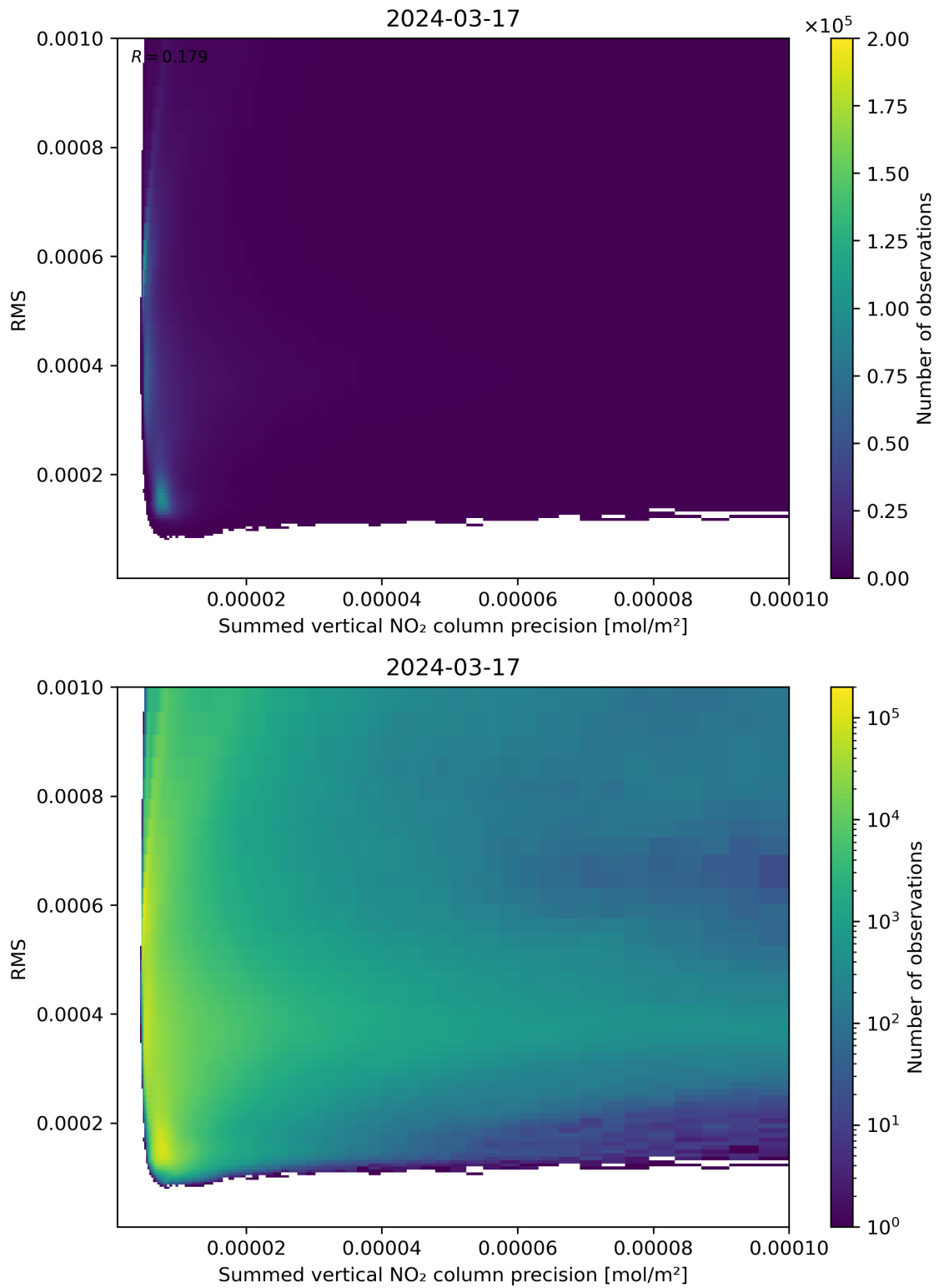
Figure 108: Scatter density plot of “Summed vertical NO 2 column precision” against “RMS” for 2024-03-16 to 2024-03-18.
