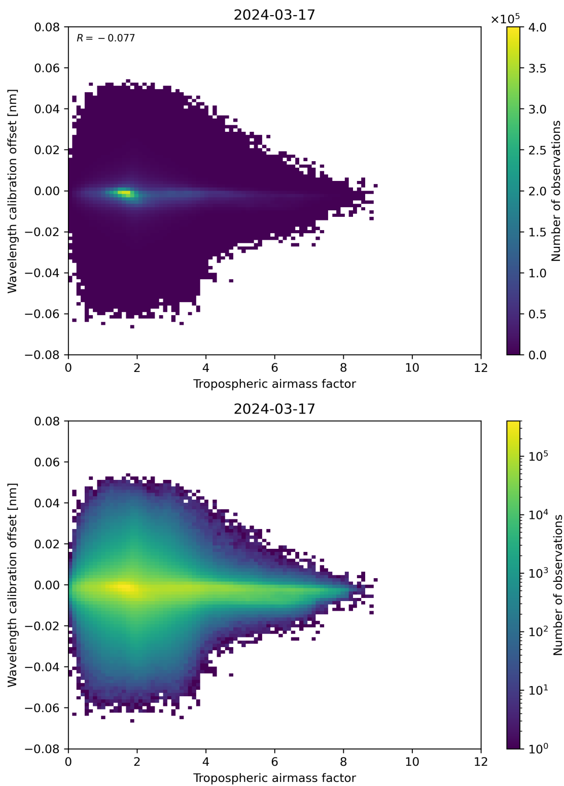
Figure 80: Scatter density plot of “Tropospheric air mass factor” against “Wavelength calibration offset” for 2024-03-16 to 2024-03-18.
