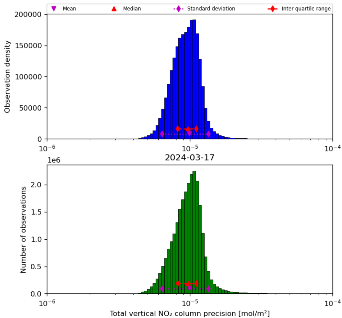
Figure 39: Histogram of “Total vertical NO 2 column precision” for 2024-03-16 to 2024-03-18
