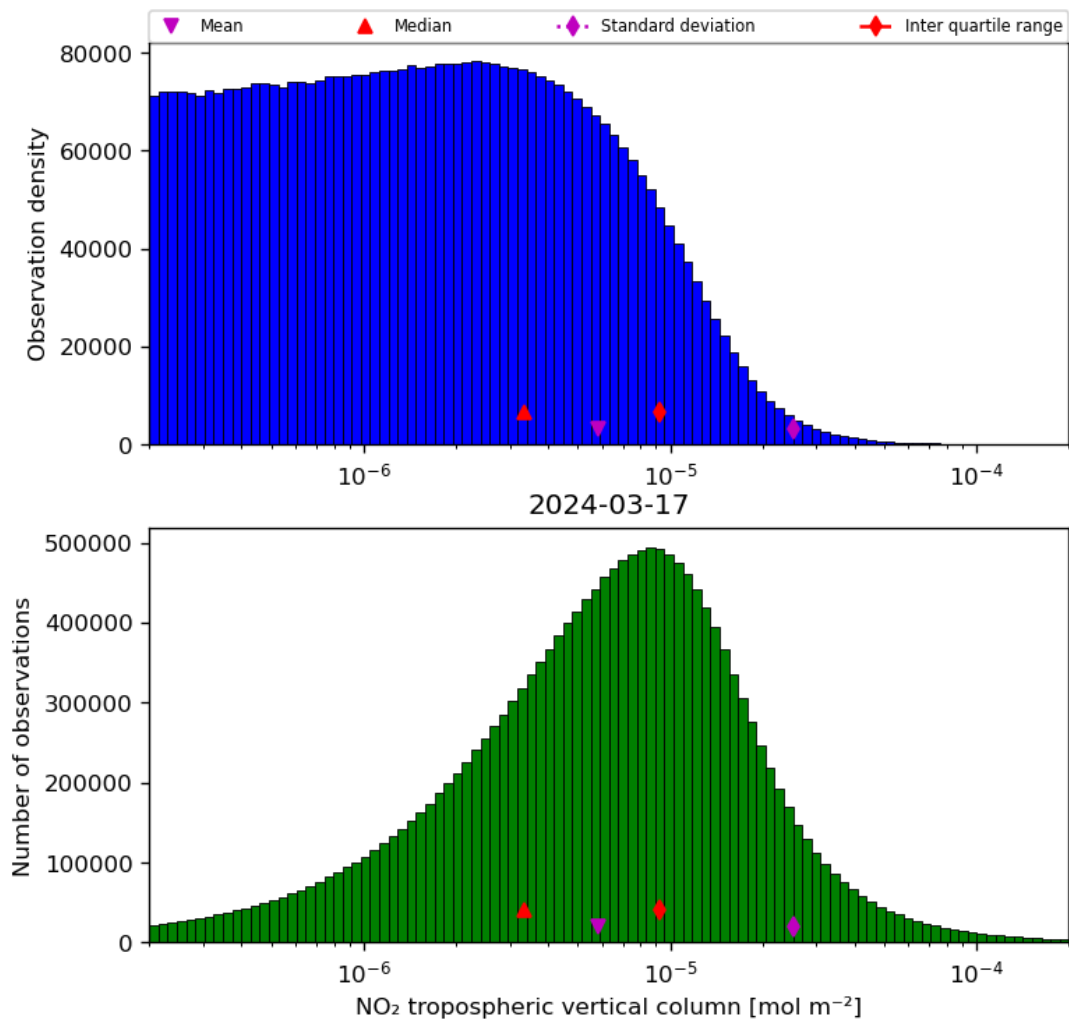
Figure 29: Histogram of “NO 2 tropospheric vertical column” for 2024-03-16 to 2024-03-18
