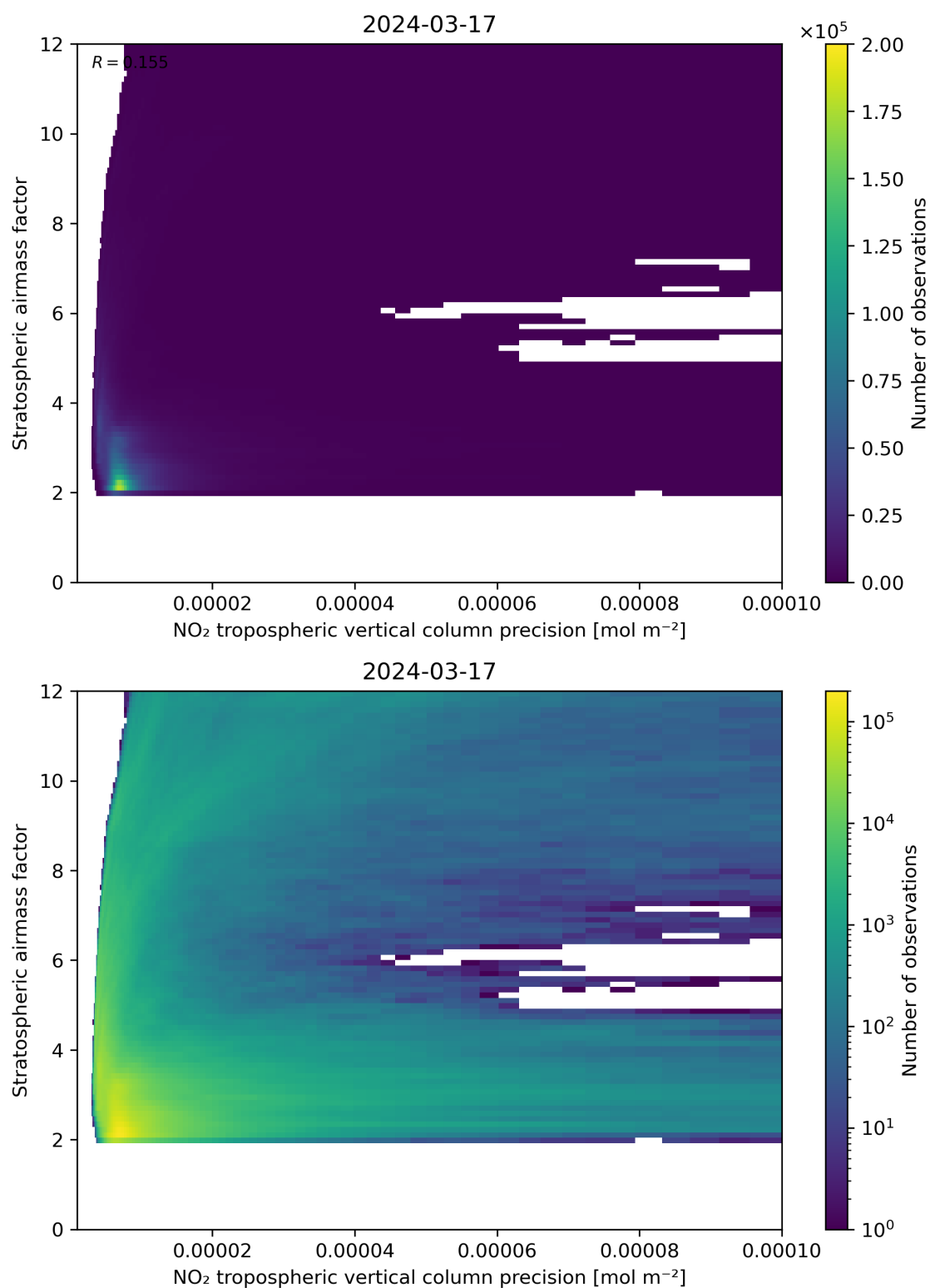
Figure 131: Scatter density plot of “NO 2 tropospheric vertical column precision” against “Stratospheric airmass factor” for 2024-03-16 to 2024-03-18.
