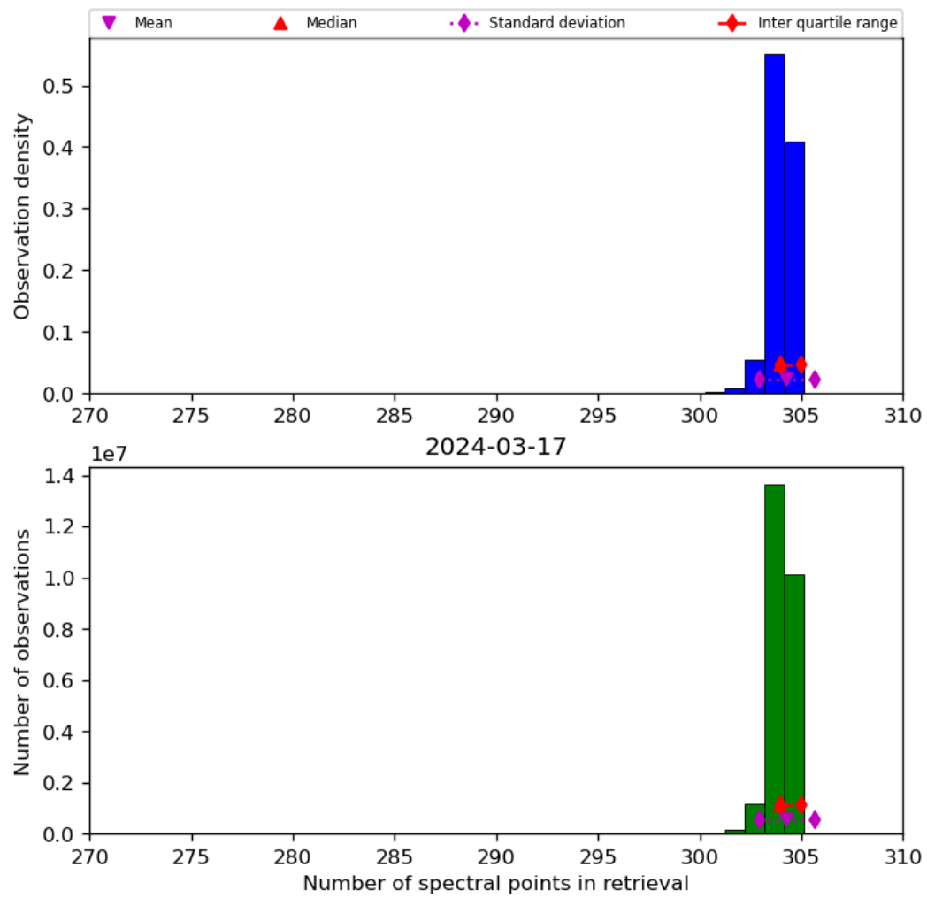
Figure 33: Histogram of “Number of spectral points in retrieval” for 2024-03-16 to 2024-03-18
