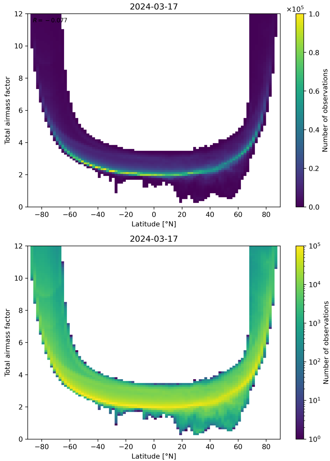
Figure 84: Scatter density plot of “Latitude” against “Total airmass factor” for 2024-03-16 to 2024-03-18.
