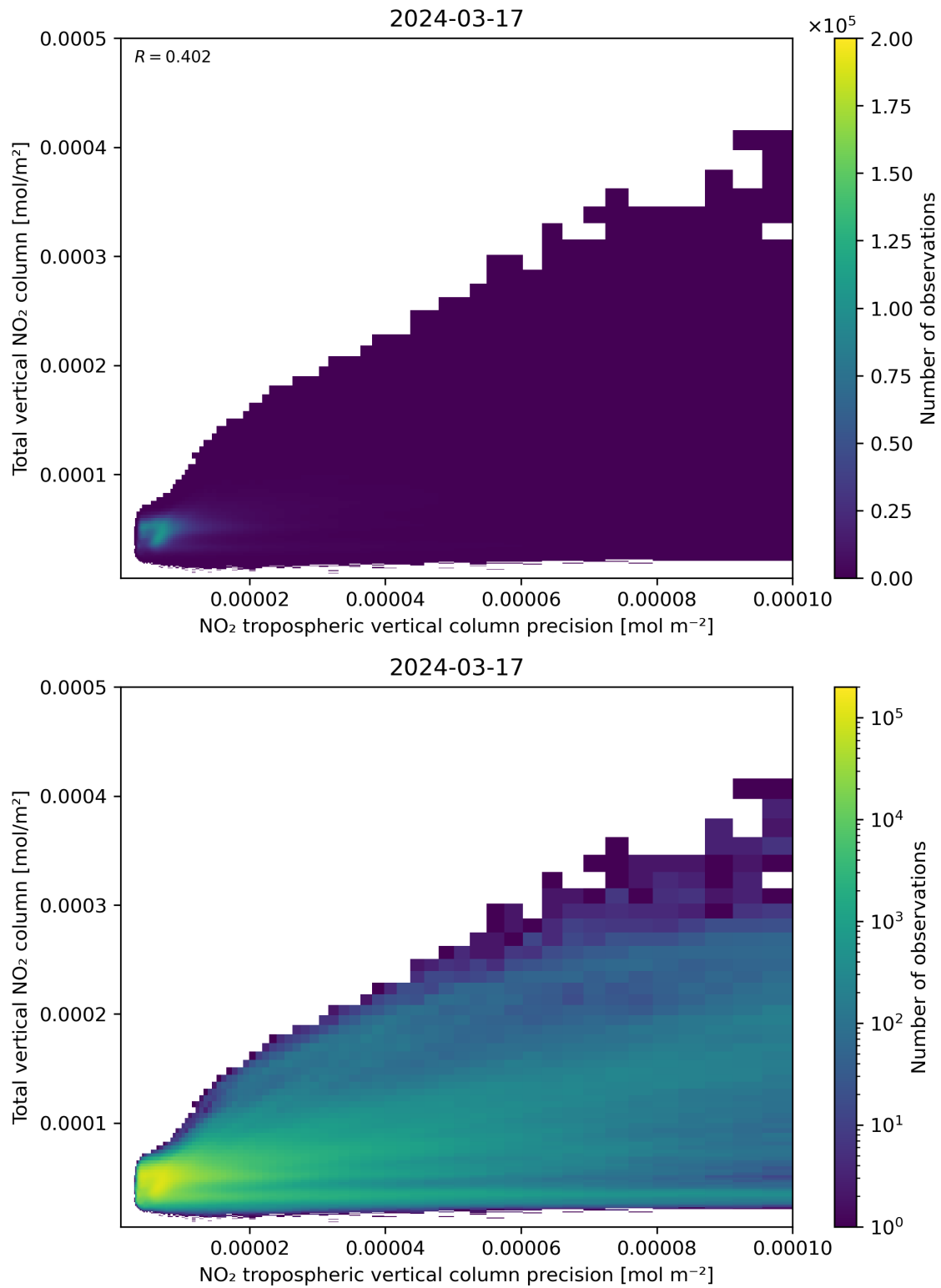
Figure 138: Scatter density plot of “NO 2 tropospheric vertical column precision” against “Total vertical NO 2 column” for 2024-03-16 to 2024-03-18.
