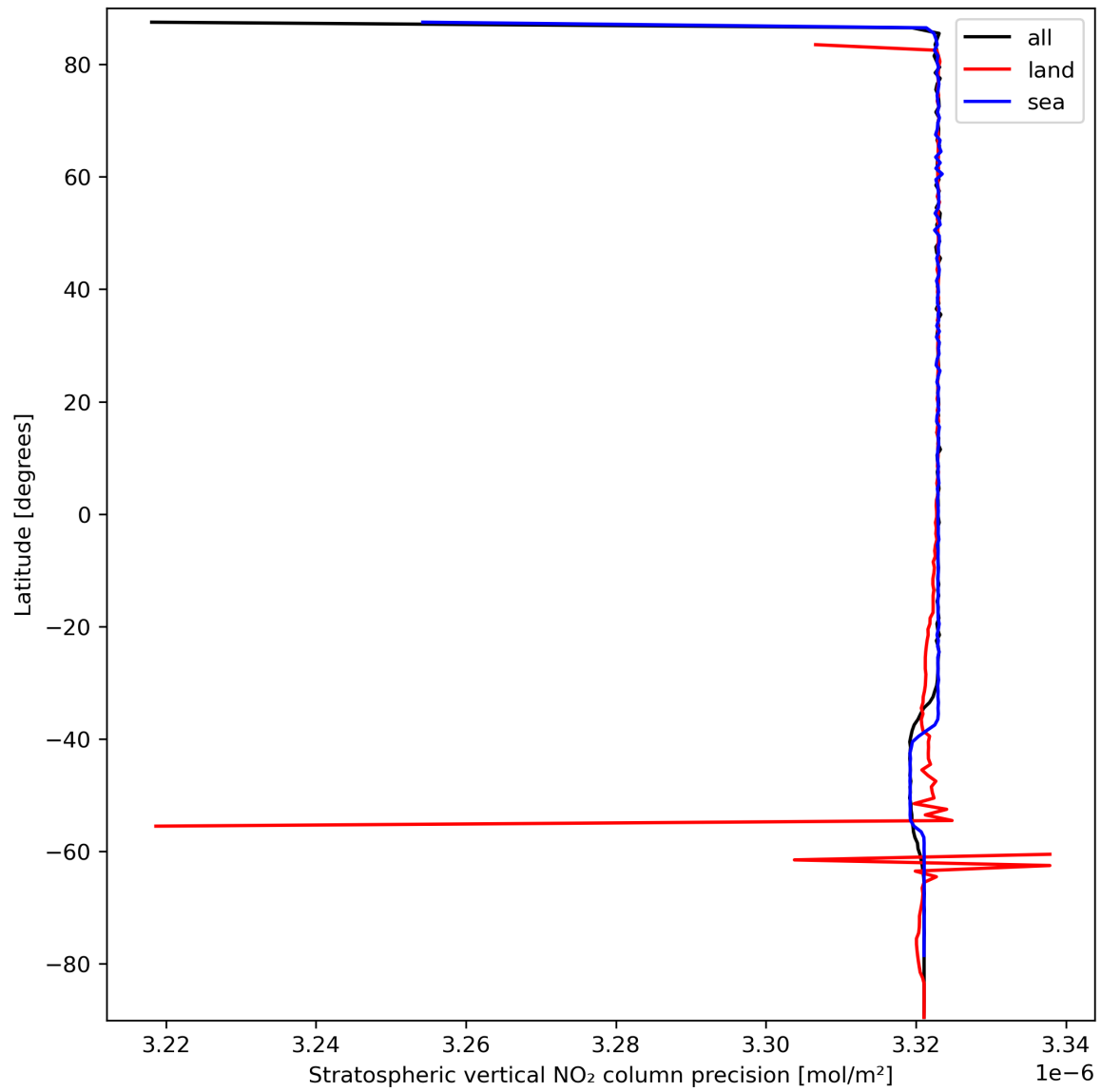
Figure 20: Zonal average of “Stratospheric vertical NO 2 column precision” for 2024-03-16 to 2024-03-18.
