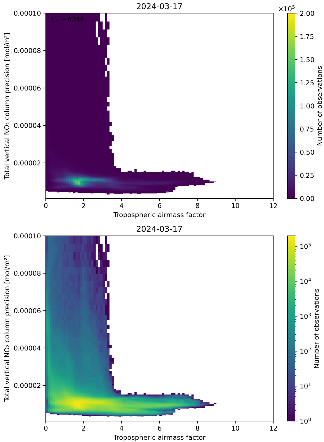
Figure 78: Scatter density plot of “Tropospheric air mass factor” against “Total vertical NO 2 column precision” for 2024-03-16 to 2024-03-18.
