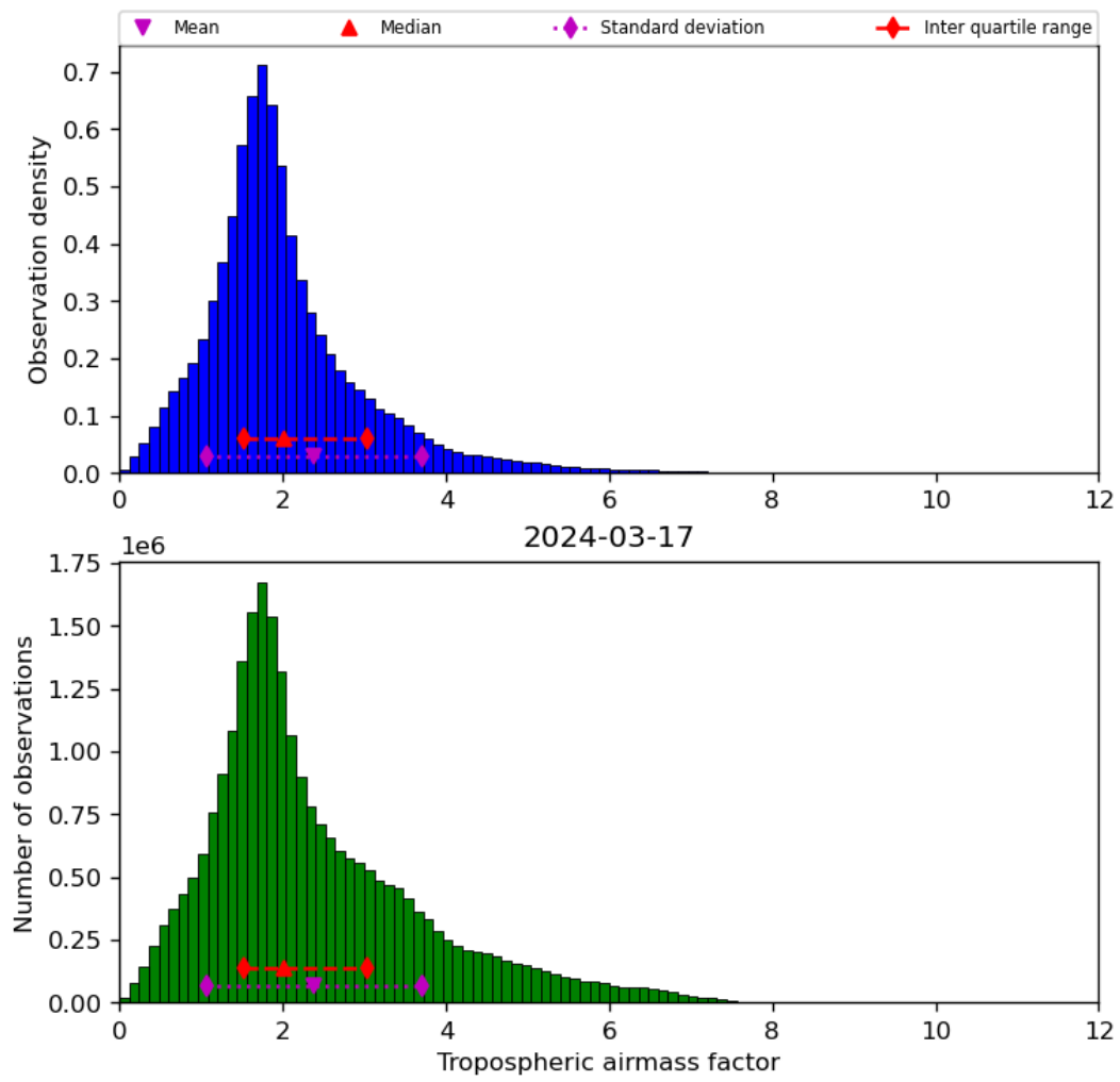
Figure 31: Histogram of “Tropospheric airmass factor” for 2024-03-16 to 2024-03-18
