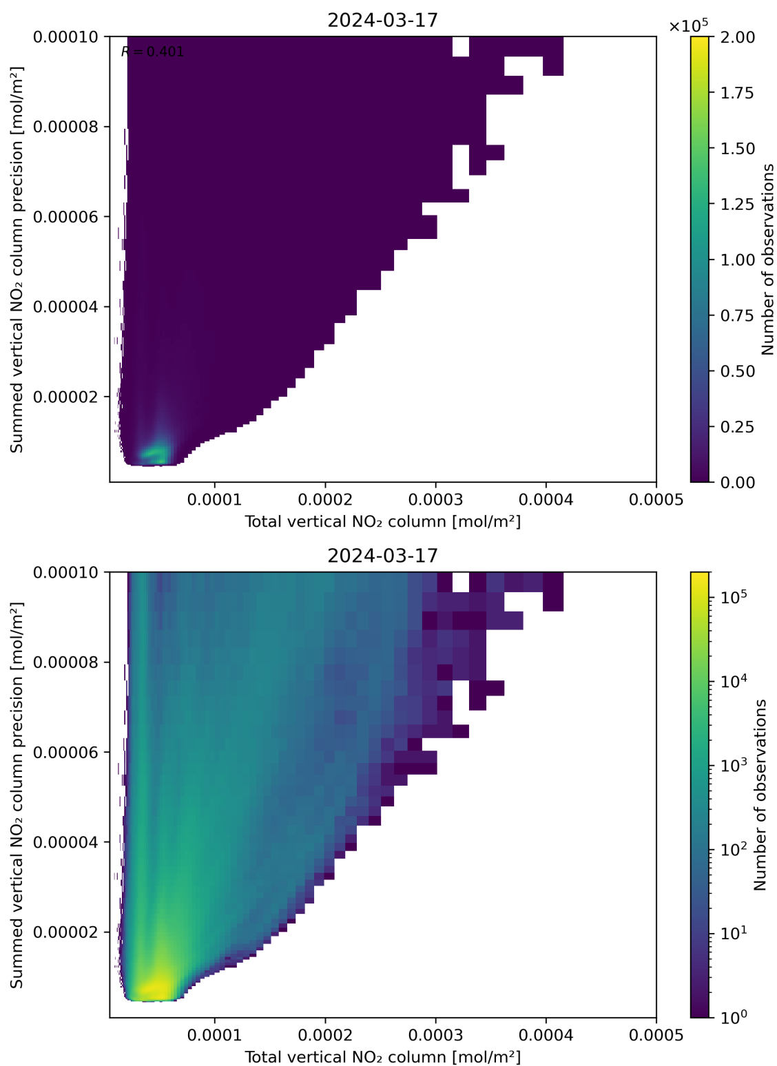
Figure 113: Scatter density plot of “Total vertical NO 2 column” against “Summed vertical NO 2 column precision” for 2024-03-16 to 2024-03-18.
