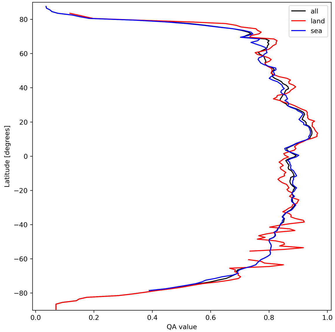
Figure 11: Zonal average of “QA value” for 2024-03-16 to 2024-03-18.
