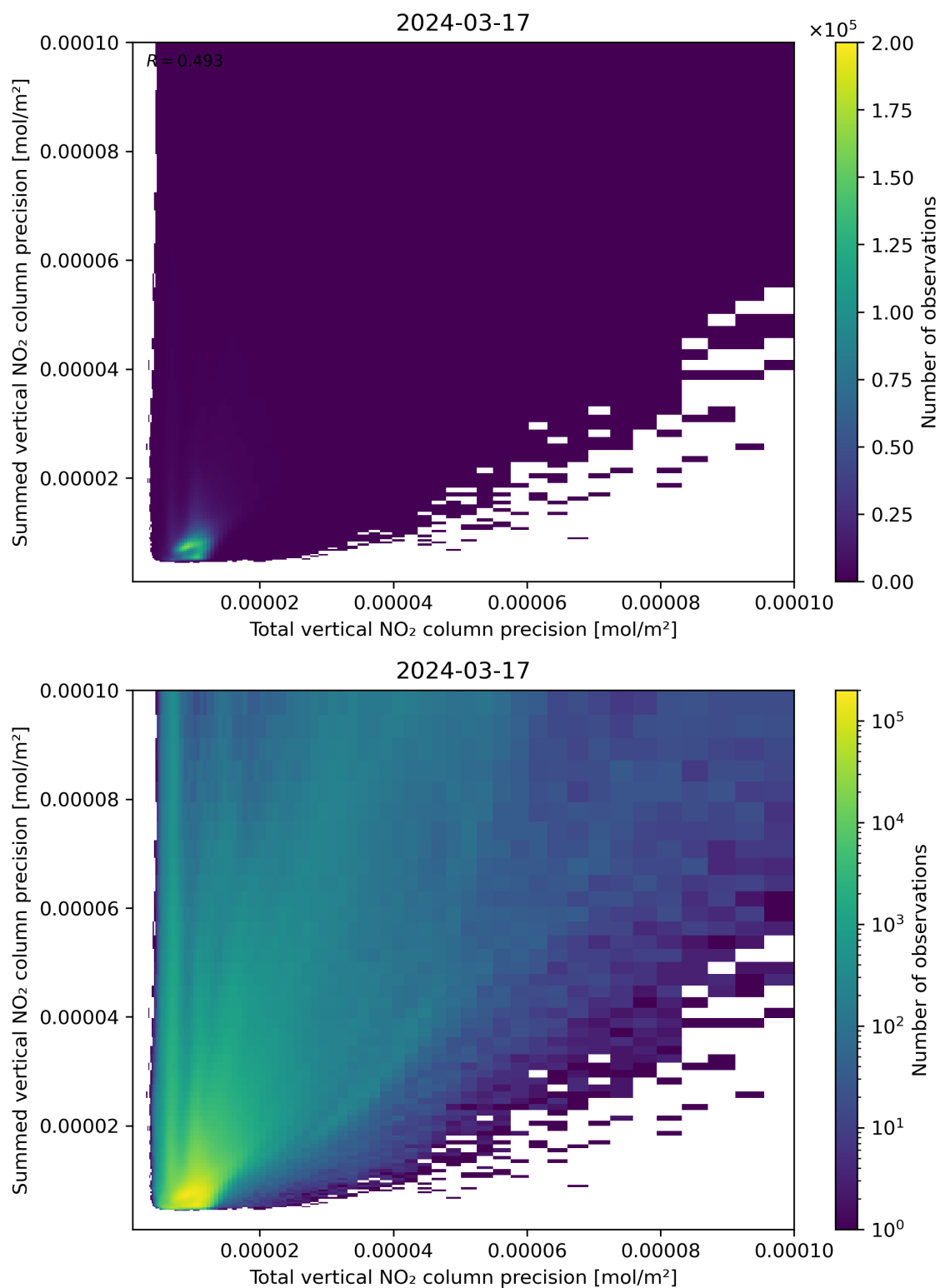
Figure 118: Scatter density plot of “Total vertical NO 2 column precision” against “Summed vertical NO 2 column precision” for 2024-03-16 to 2024-03-18.
