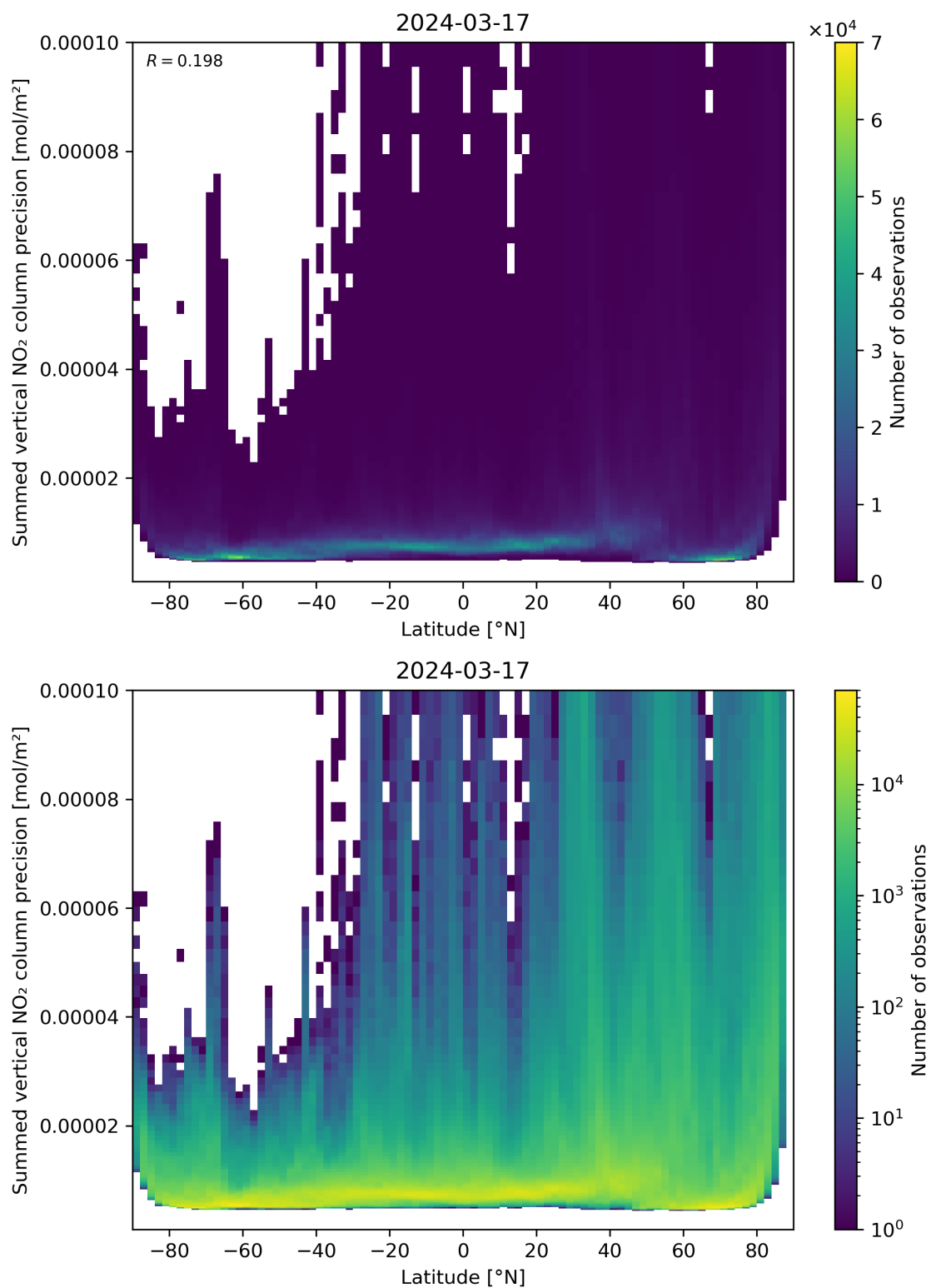
Figure 89: Scatter density plot of “Latitude” against “Summed vertical NO 2 column precision” for 2024-03-16 to 2024-03-18.
