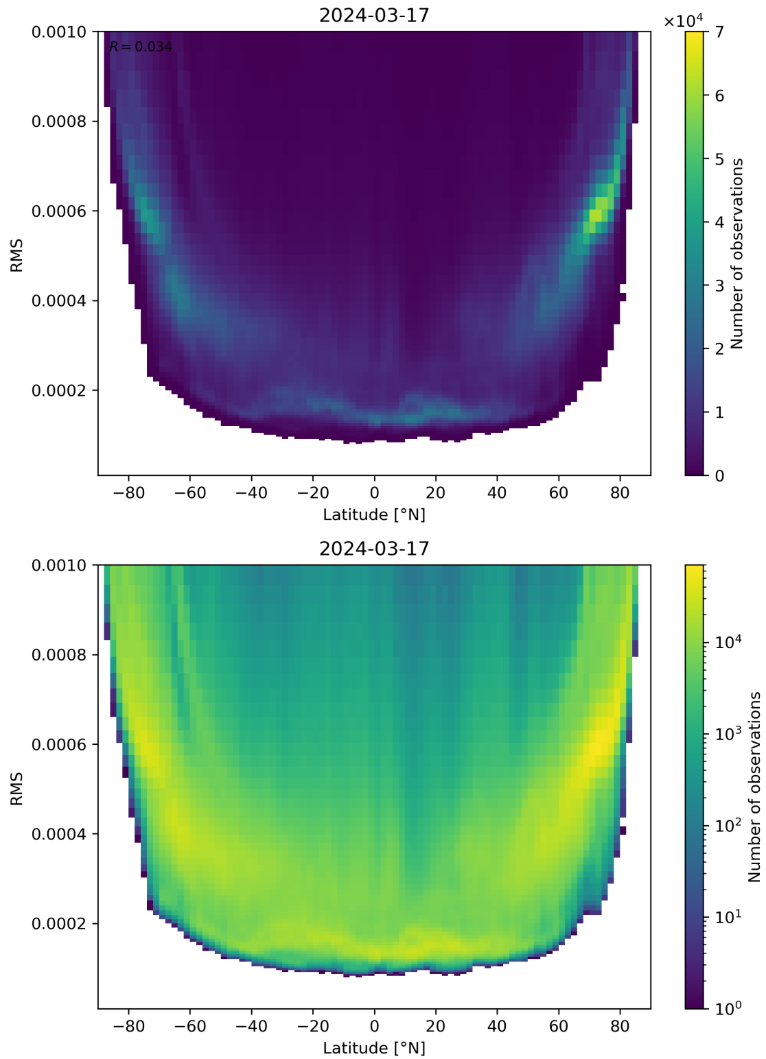
Figure 94: Scatter density plot of “Latitude” against “RMS” for 2024-03-16 to 2024-03-18.
