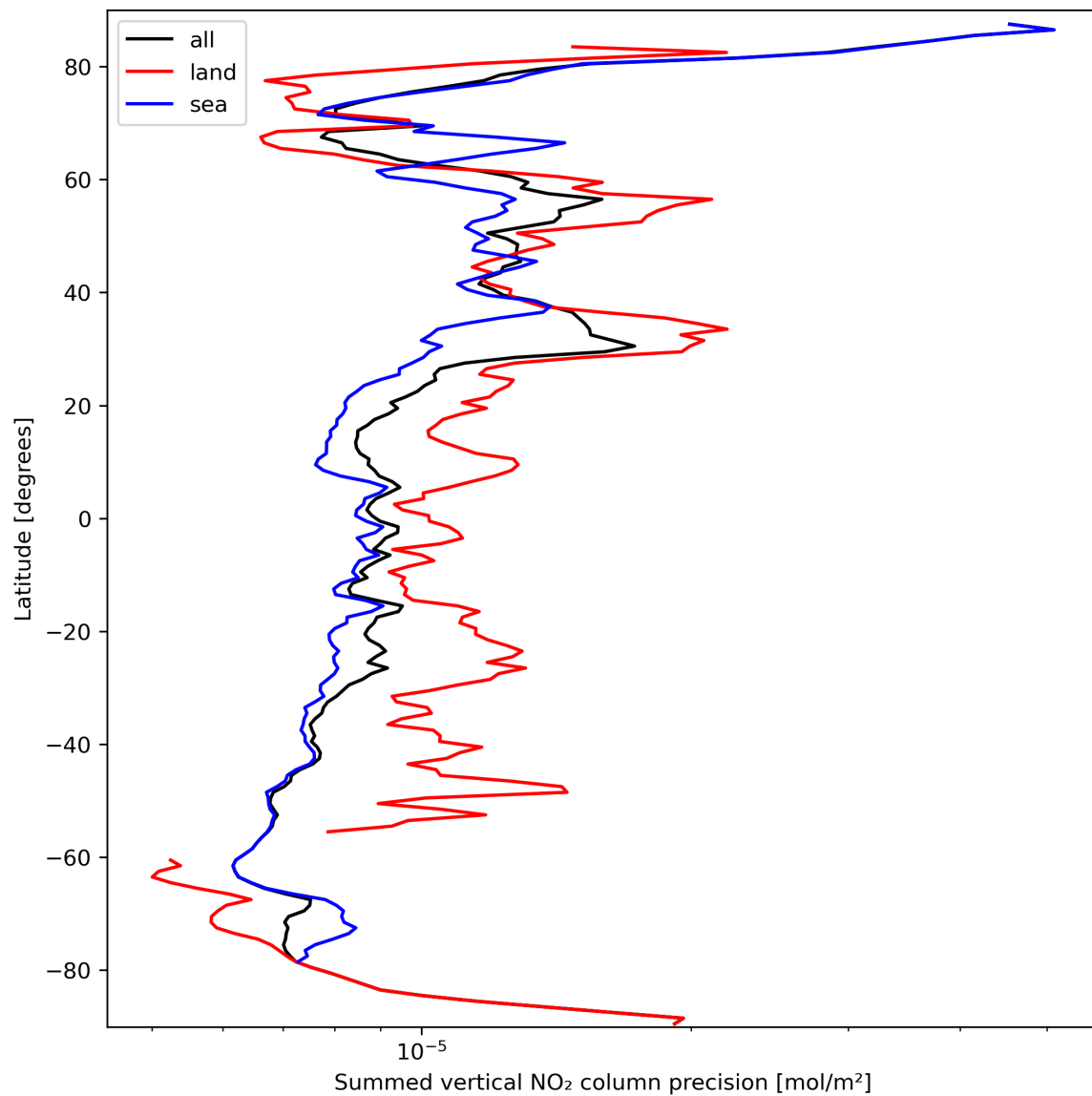
Figure 24: Zonal average of “Summed vertical NO 2 column precision” for 2024-03-16 to 2024-03-18.
