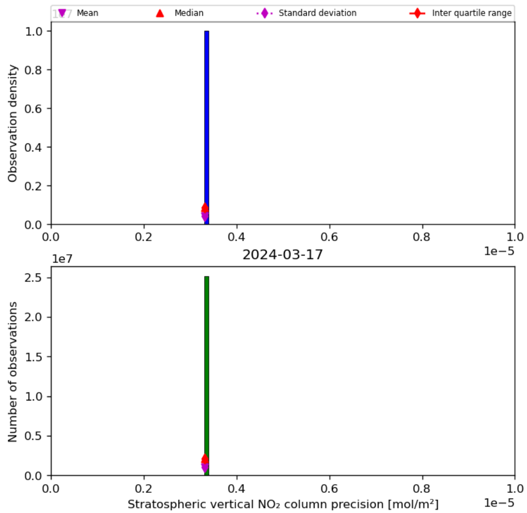
Figure 37: Histogram of “Stratospheric vertical NO 2 column precision” for 2024-03-16 to 2024-03-18
