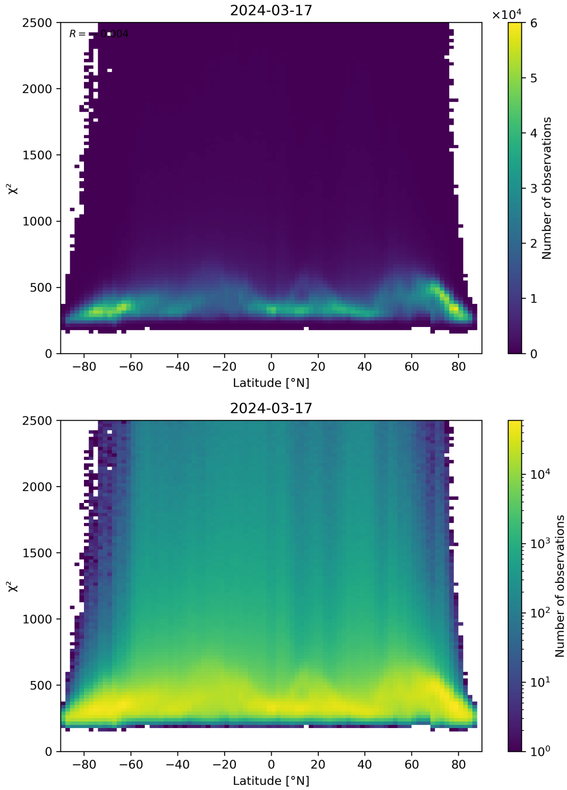
Figure 86: Scatter density plot of “Latitude” against “ \chi^2 ” for 2024-03-16 to 2024-03-18.
