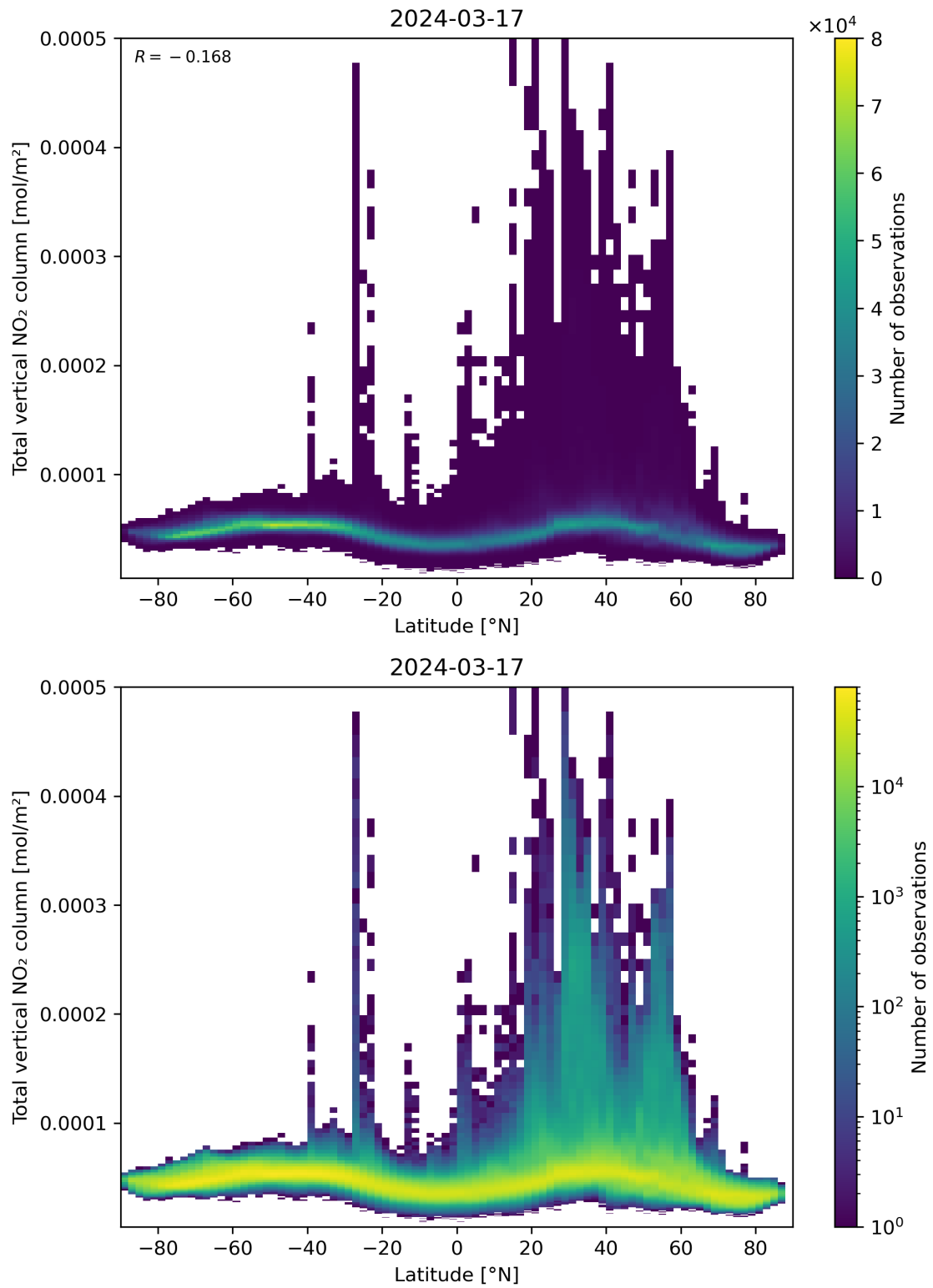
Figure 90: Scatter density plot of “Latitude” against “Total vertical NO 2 column” for 2024-03-16 to 2024-03-18.
