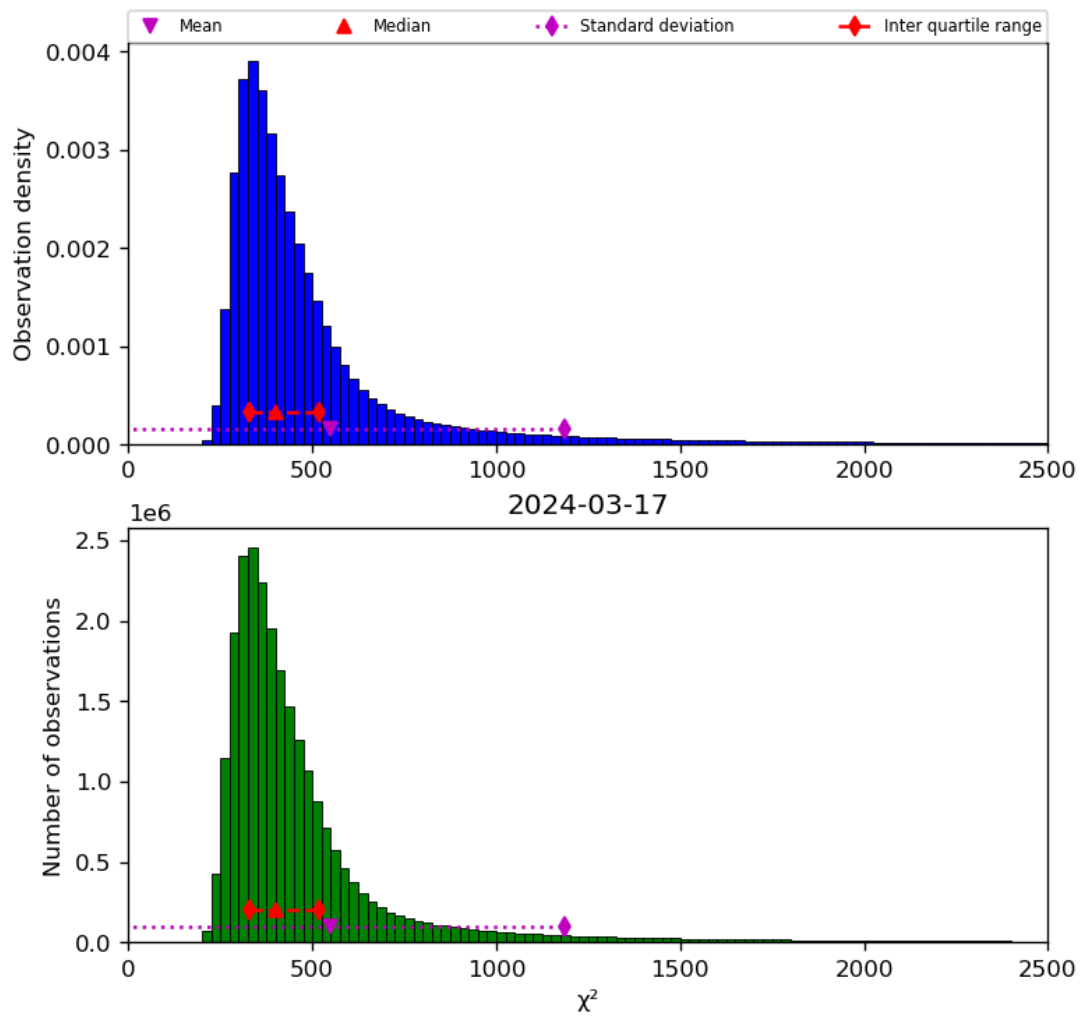
Figure 42: Histogram of “ \chi^2 ” for 2024-03-16 to 2024-03-18
