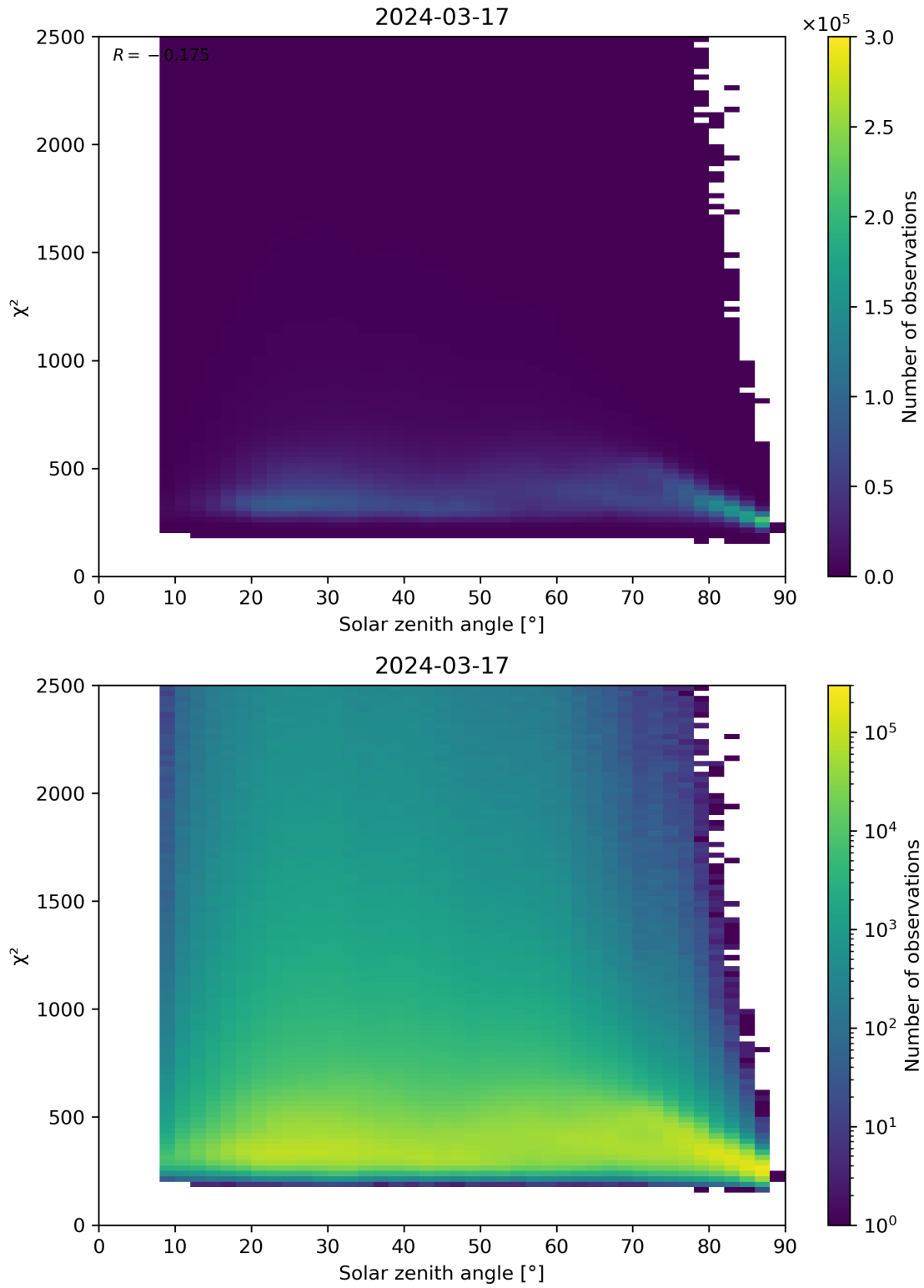
Figure 148: Scatter density plot of “Solar zenith angle” against “ \chi^2 ” for 2024-03-16 to 2024-03-18.
