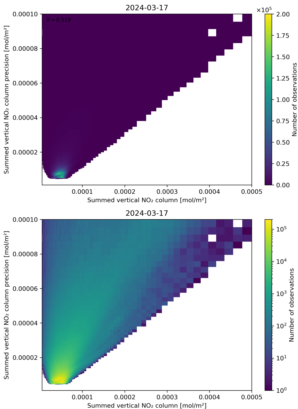
Figure 105: Scatter density plot of “Summed vertical NO 2 column” against “Summed vertical NO 2 column precision” for 2024-03-16 to 2024-03-18.
