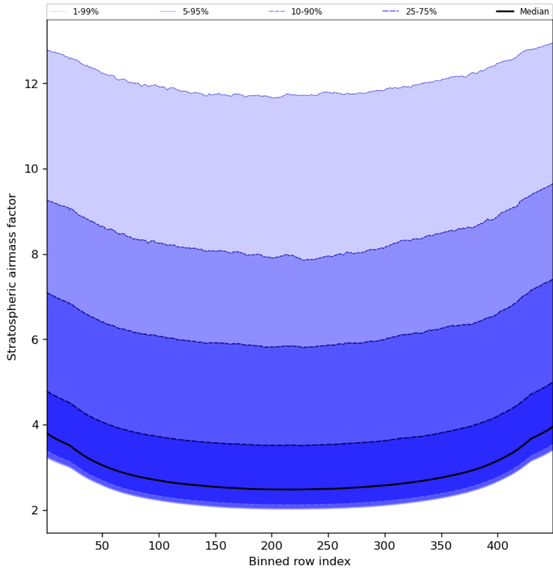
Figure 61: Along track statistics of “Stratospheric airmass factor” for 2024-03-16 to 2024-03-18
