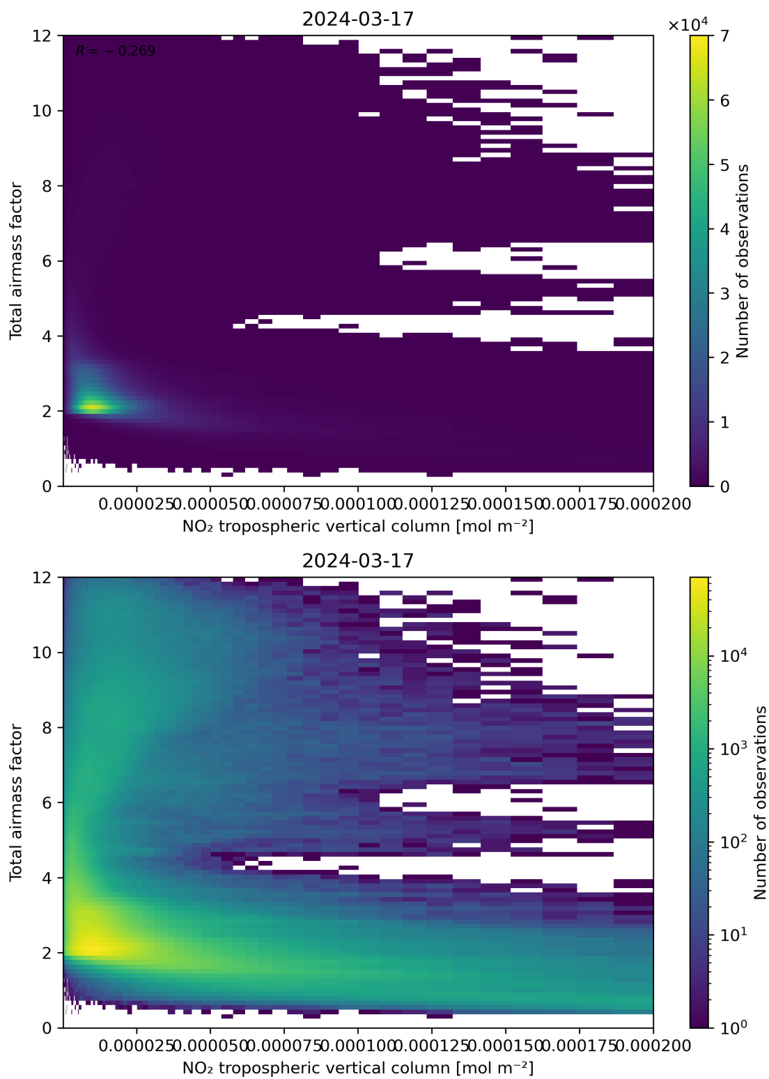
Figure 122: Scatter density plot of “NO 2 tropospheric vertical column” against “Total air mass factor” for 2024-03-16 to 2024-03-18.
