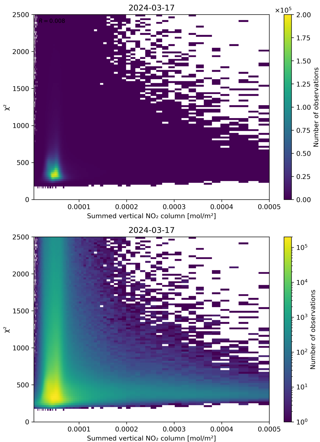
Figure 104: Scatter density plot of “Summed vertical NO 2 column” against “ \chi^2 ” for 2024-03-16 to 2024-03-18.
