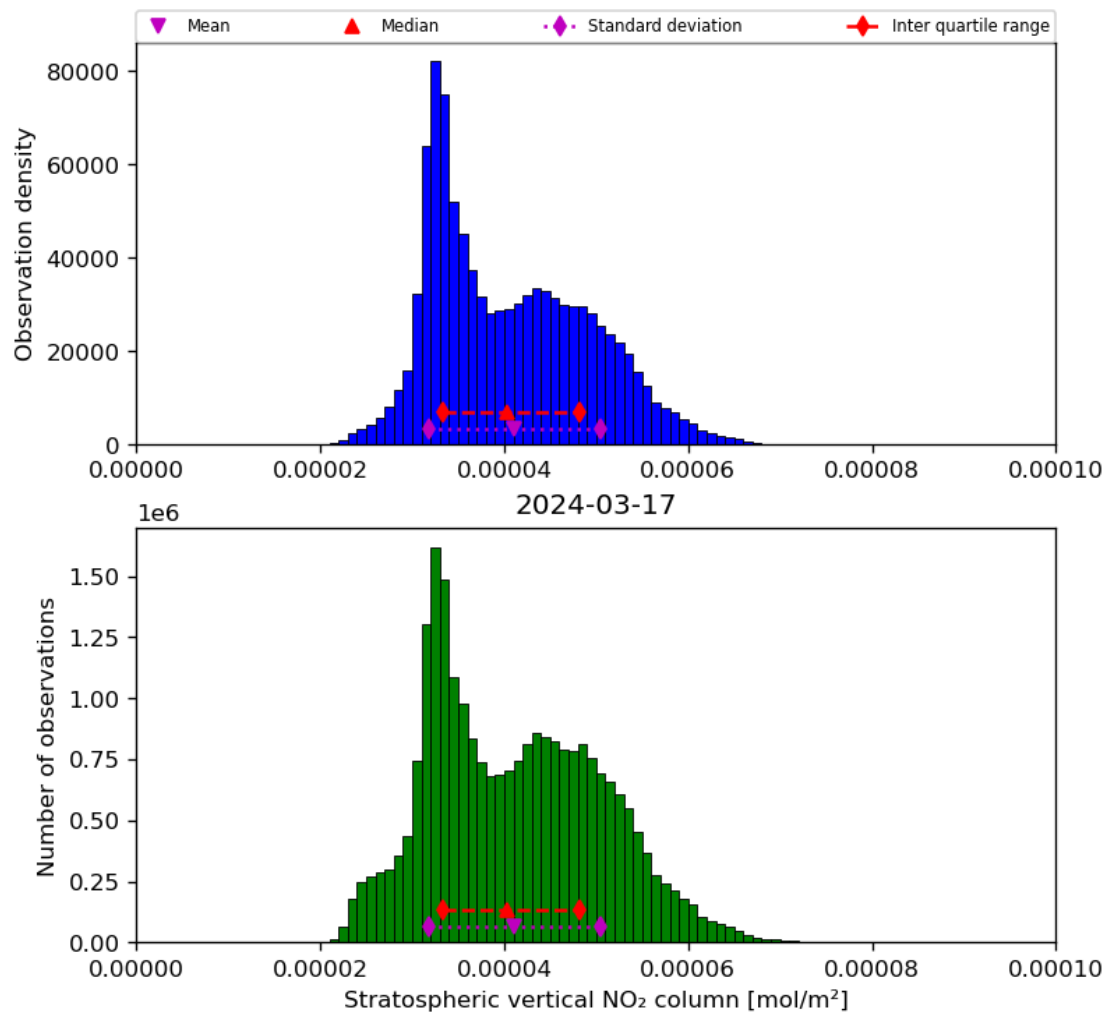
Figure 36: Histogram of “Stratospheric vertical NO 2 column” for 2024-03-16 to 2024-03-18
