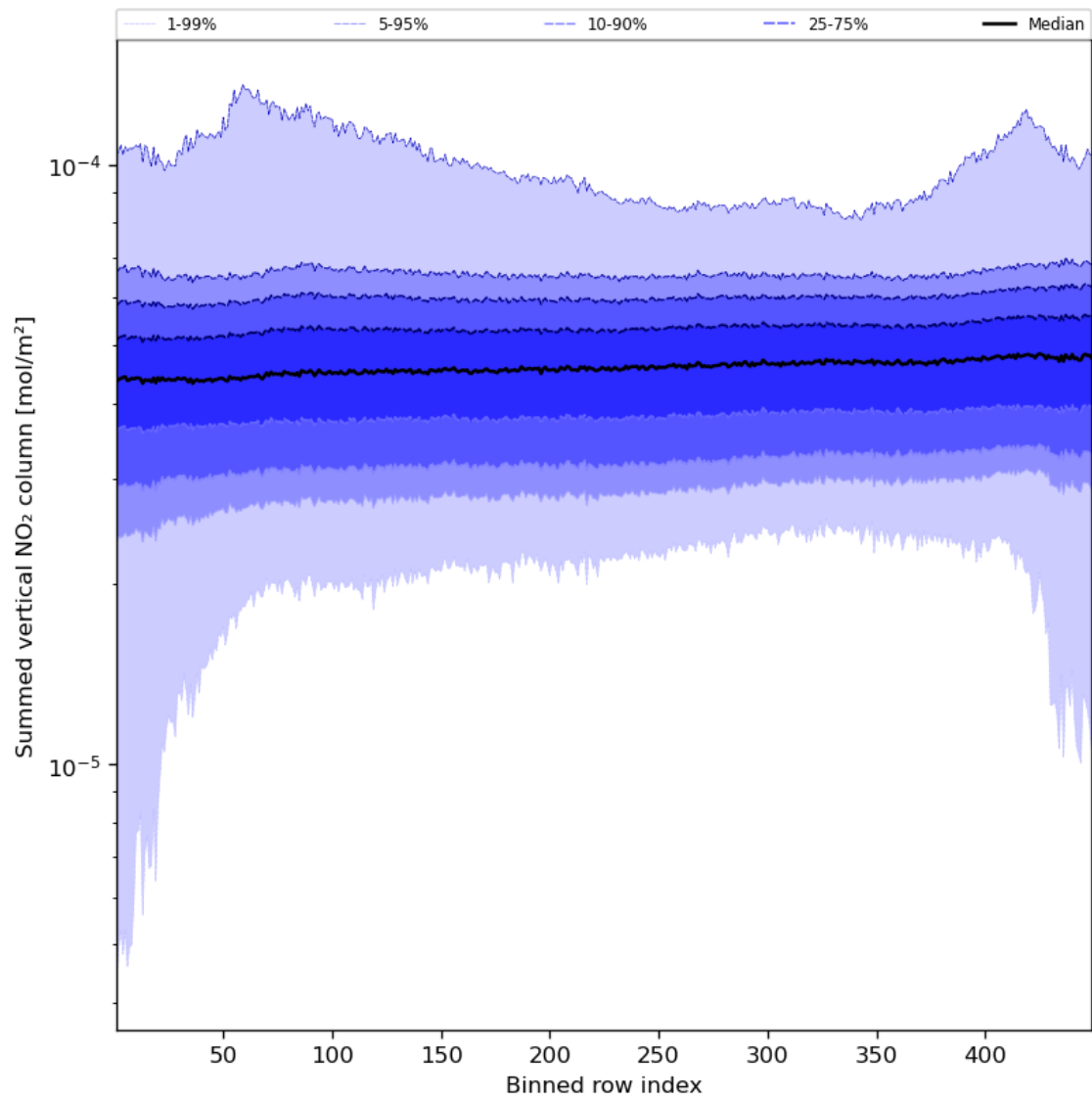
Figure 57: Along track statistics of “Summed vertical NO 2 column” for 2024-03-16 to 2024-03-18
