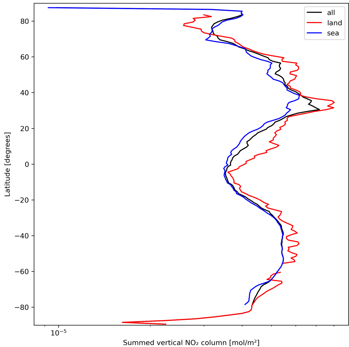
Figure 23: Zonal average of “Summed vertical NO 2 column” for 2024-03-16 to 2024-03-18.
