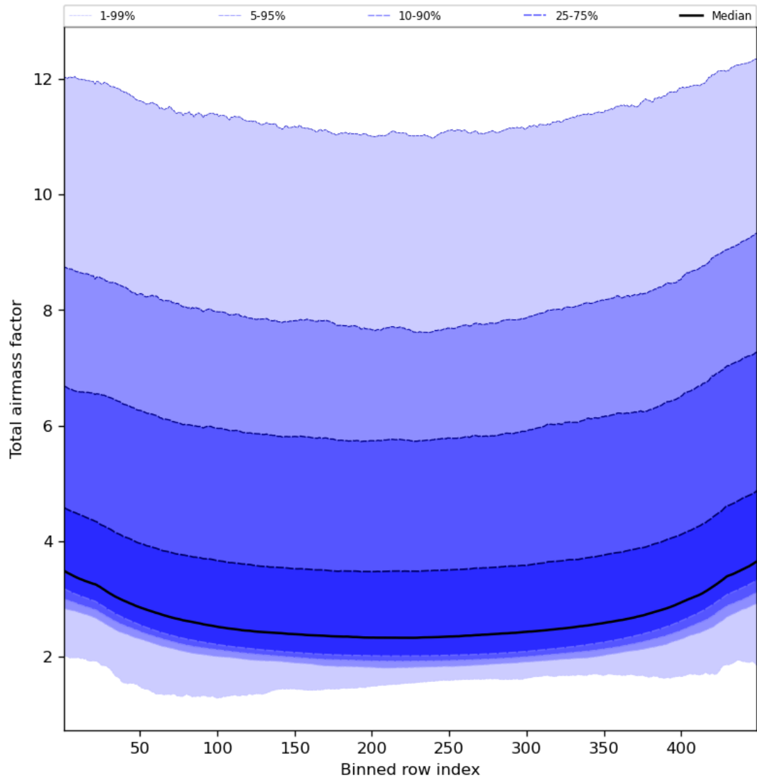
Figure 49: Along track statistics of “Total airmass factor” for 2024-03-16 to 2024-03-18
