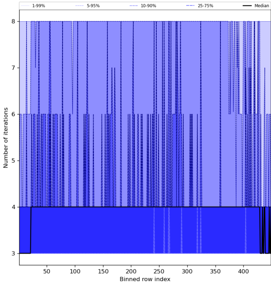
Figure 51: Along track statistics of “Number of iterations” for 2024-03-16 to 2024-03-18
