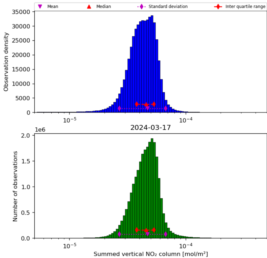
Figure 40: Histogram of “Summed vertical NO 2 column” for 2024-03-16 to 2024-03-18
