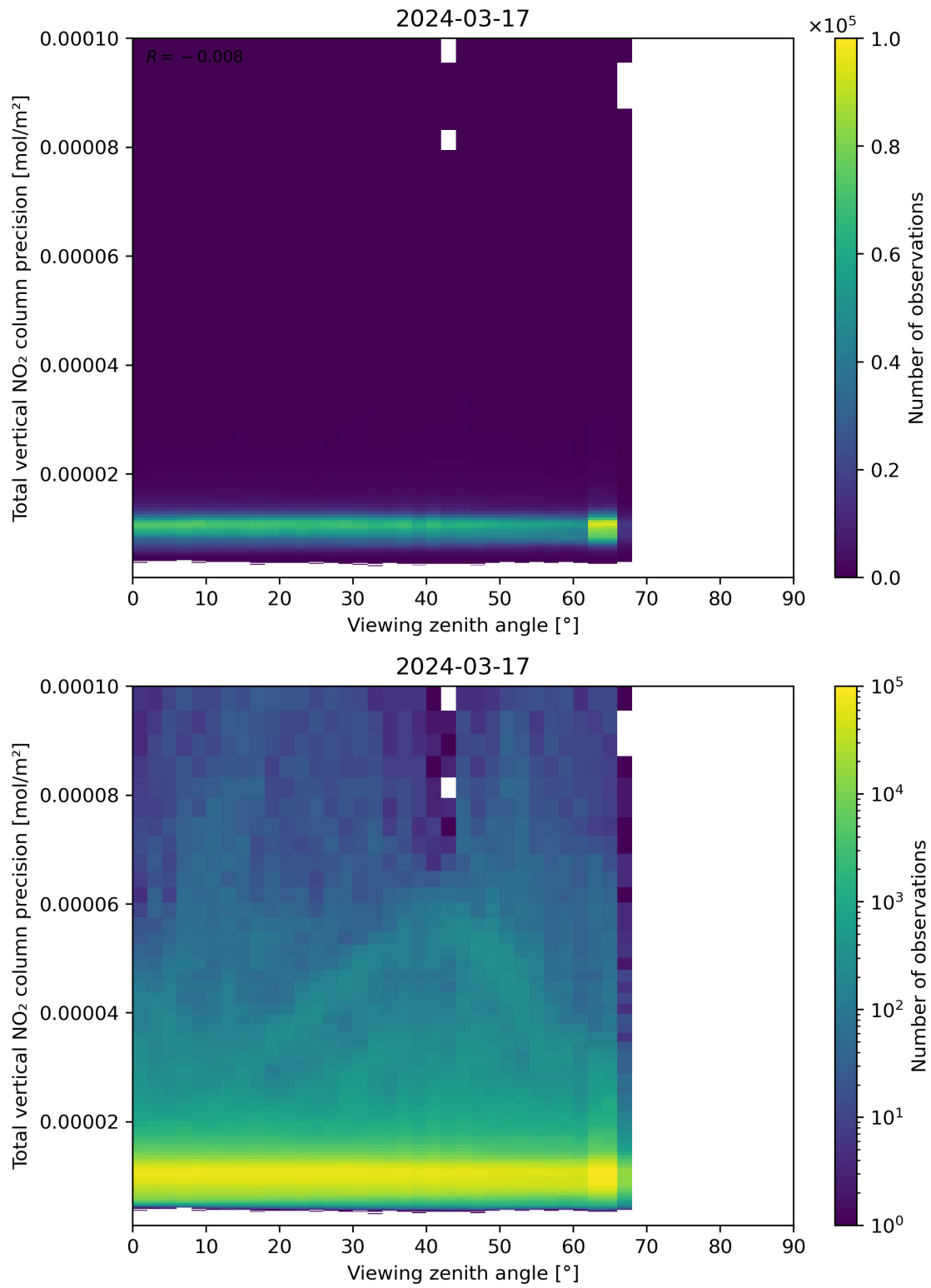
Figure 168: Scatter density plot of “Viewing zenith angle” against “Total vertical NO 2 column precision” for 2024-03-16 to 2024-03-18.
