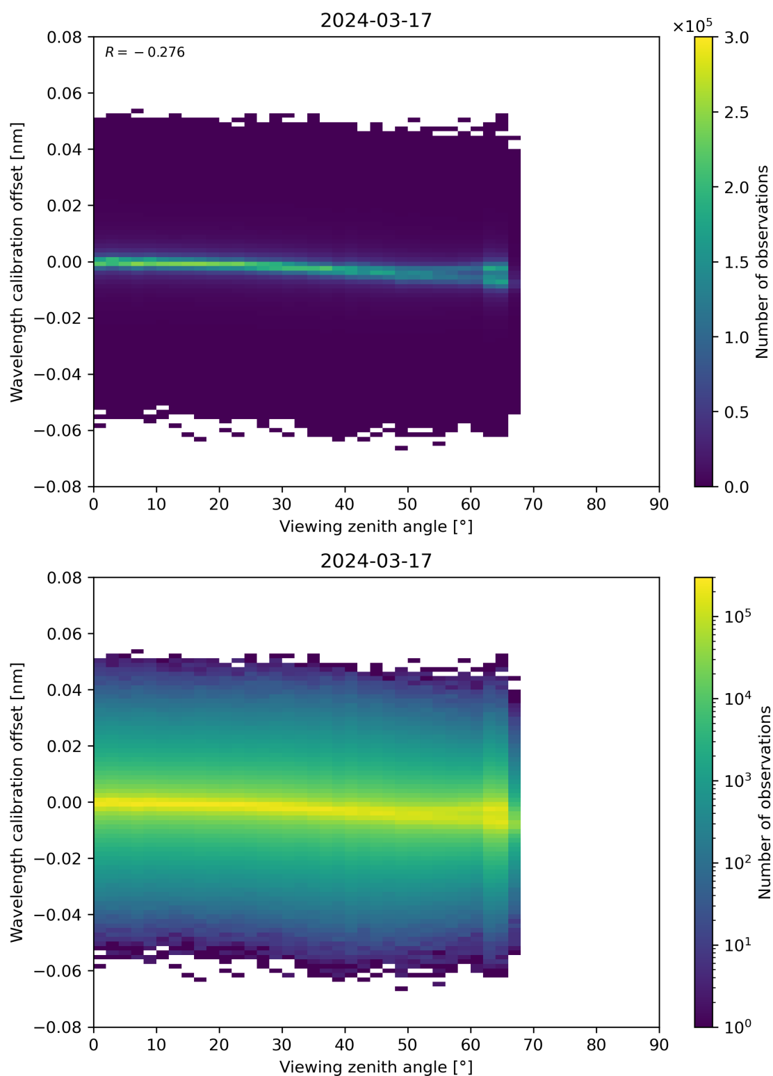
Figure 173: Scatter density plot of “Viewing zenith angle” against “Wavelength calibration offset” for 2024-03-16 to 2024-03-18.
