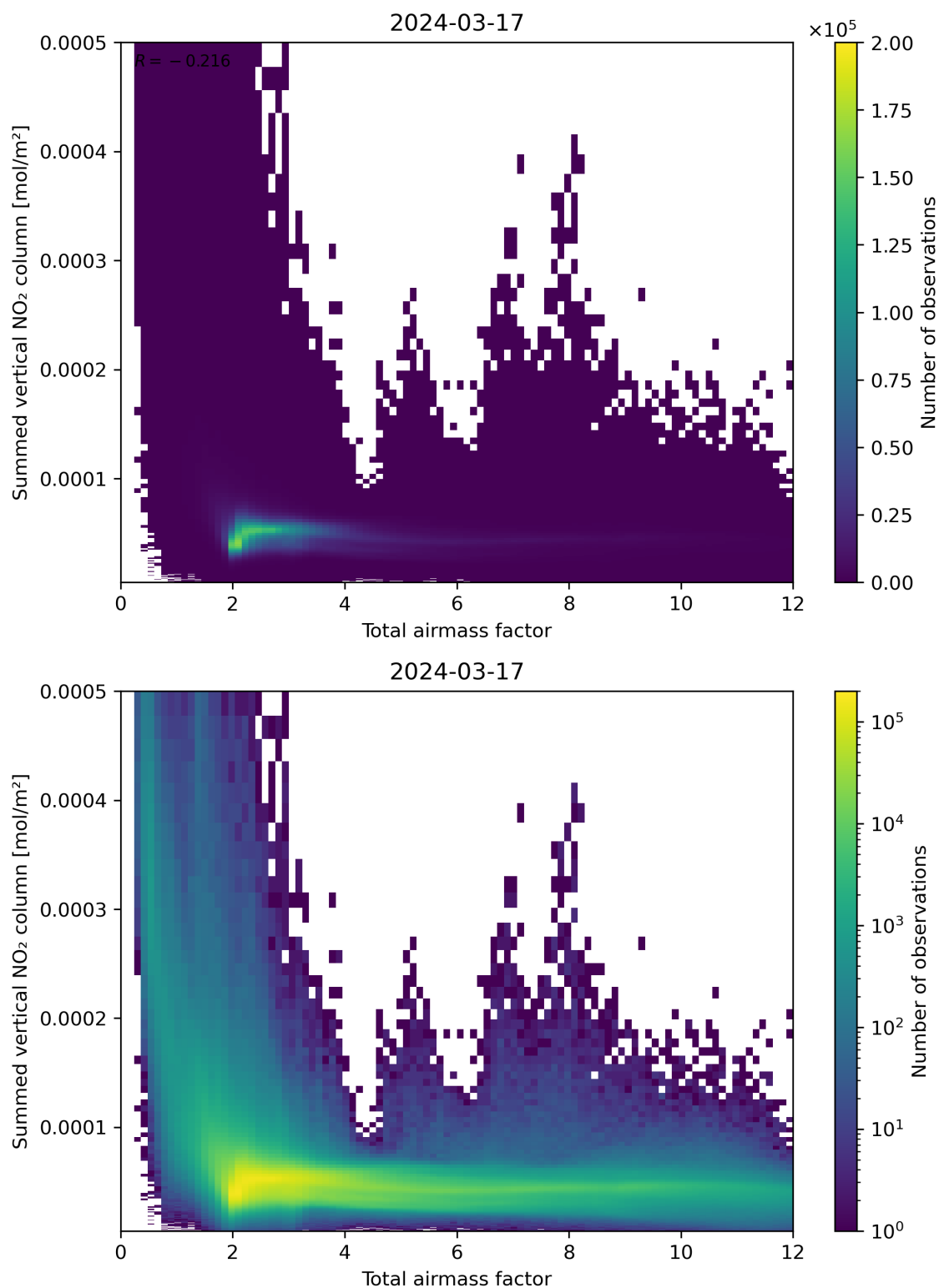
Figure 65: Scatter density plot of “Total airmass factor” against “Summed vertical NO 2 column” for 2024-03-16 to 2024-03-18.
