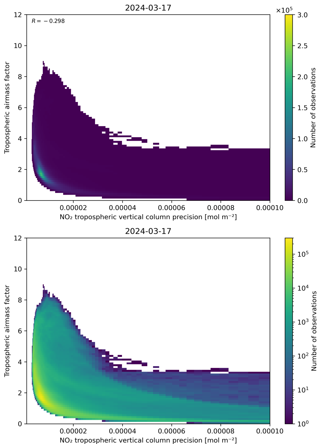
Figure 133: Scatter density plot of “NO 2 tropospheric vertical column precision” against “Tropospheric airmass factor” for 2024-03-16 to 2024-03-18.
