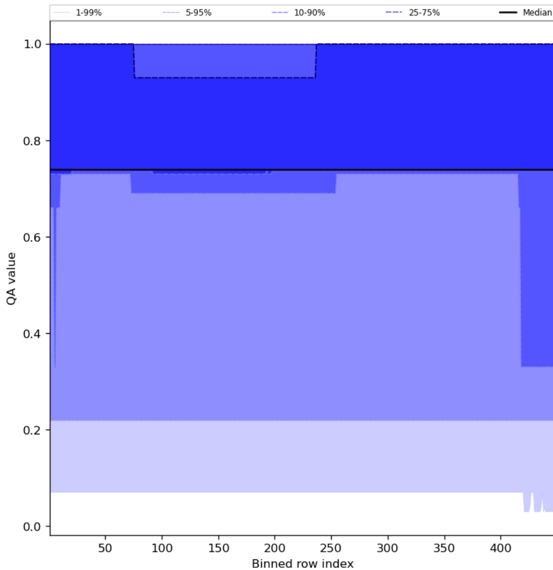
Figure 45: Along track statistics of “QA value” for 2024-03-16 to 2024-03-18
