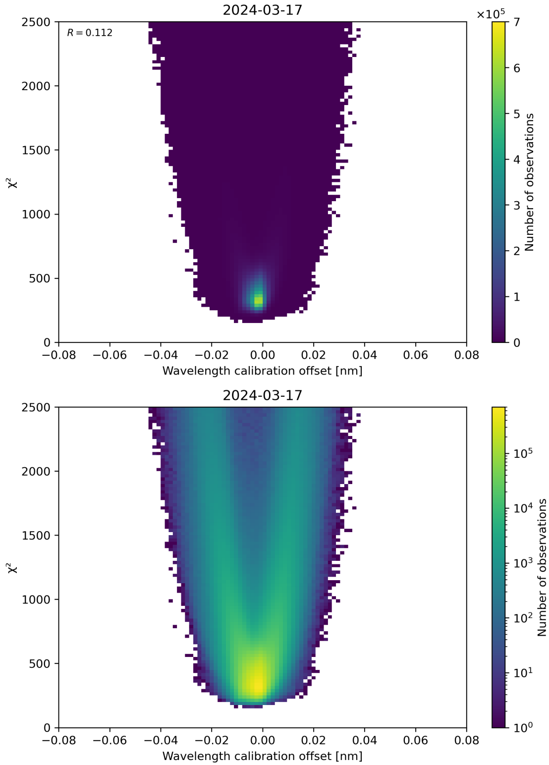
Figure 175: Scatter density plot of “Wavelength calibration offset” against “ \chi^2 ” for 2024-03-16 to 2024-03-18.
