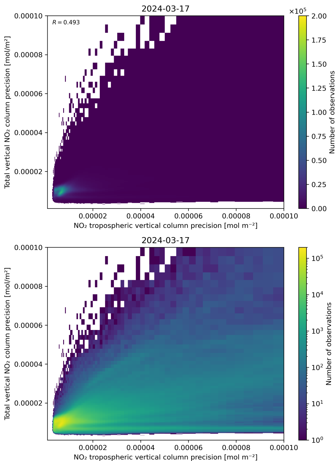
Figure 139: Scatter density plot of “NO 2 tropospheric vertical column precision” against “Total vertical NO 2 column precision” for 2024-03-16 to 2024-03-18.
