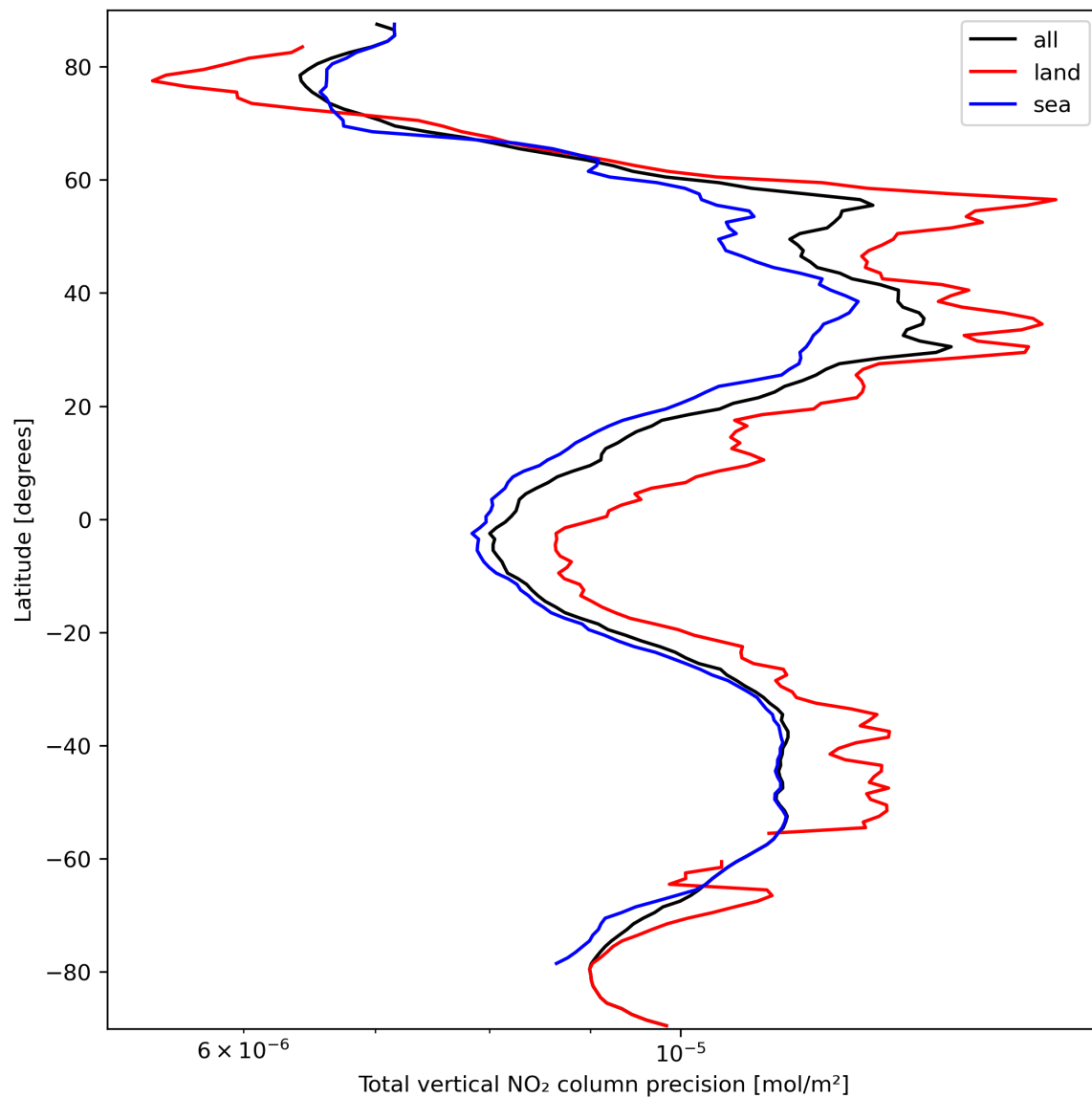
Figure 22: Zonal average of “Total vertical NO 2 column precision” for 2024-03-16 to 2024-03-18.
