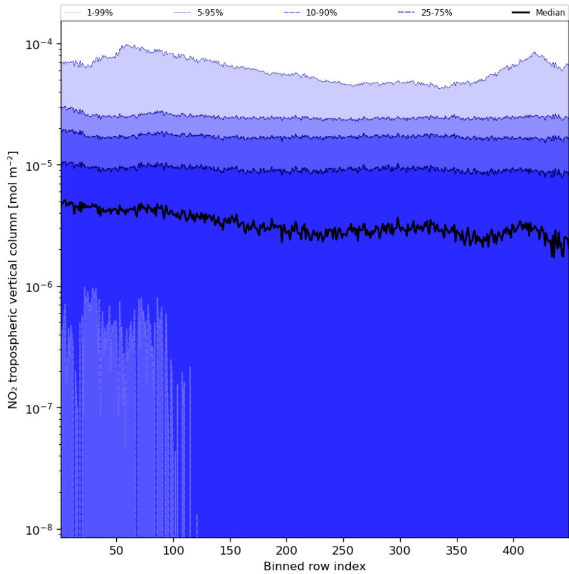
Figure 46: Along track statistics of “NO 2 tropospheric vertical column” for 2024-03-16 to 2024-03-18
