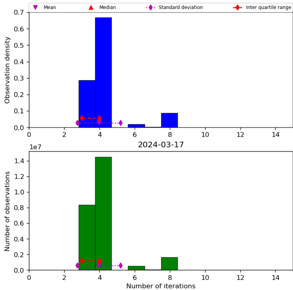
Figure 34: Histogram of “Number of iterations” for 2024-03-16 to 2024-03-18
