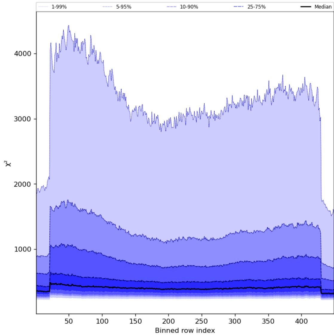
Figure 59: Along track statistics of “ \chi^2 ” for 2024-03-16 to 2024-03-18
