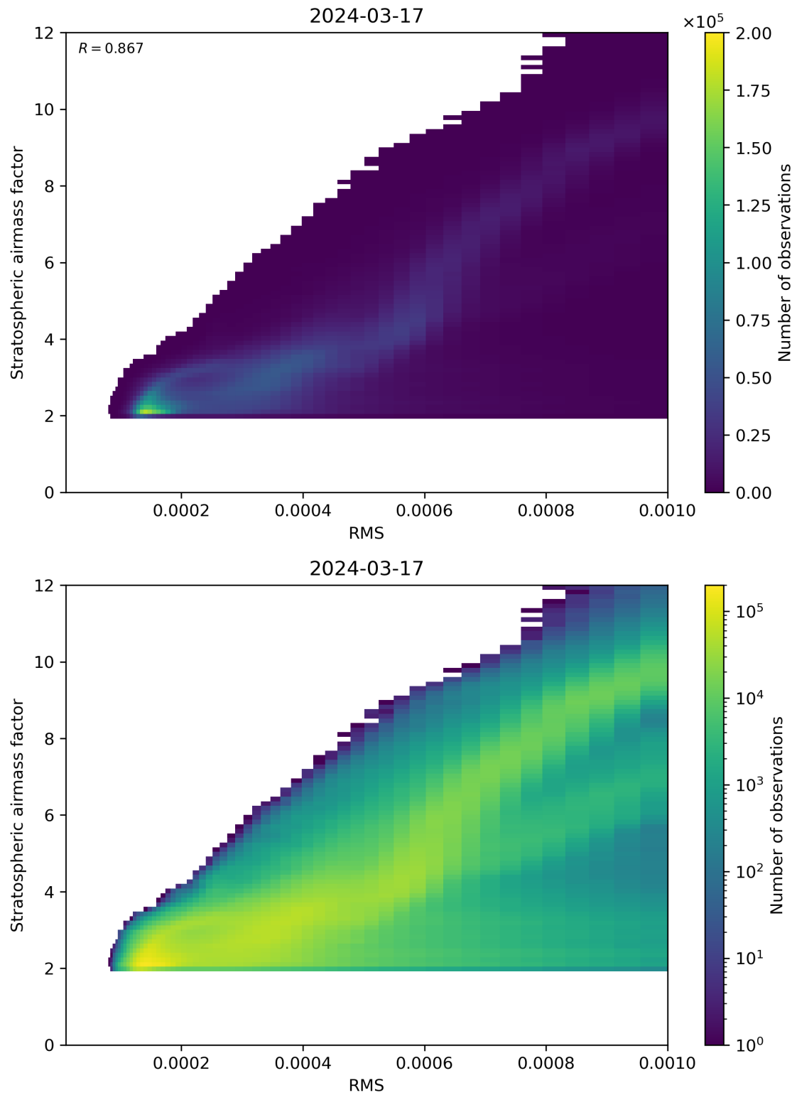
Figure 144: Scatter density plot of “RMS” against “Stratospheric airmass factor” for 2024-03-16 to 2024-03-18.
