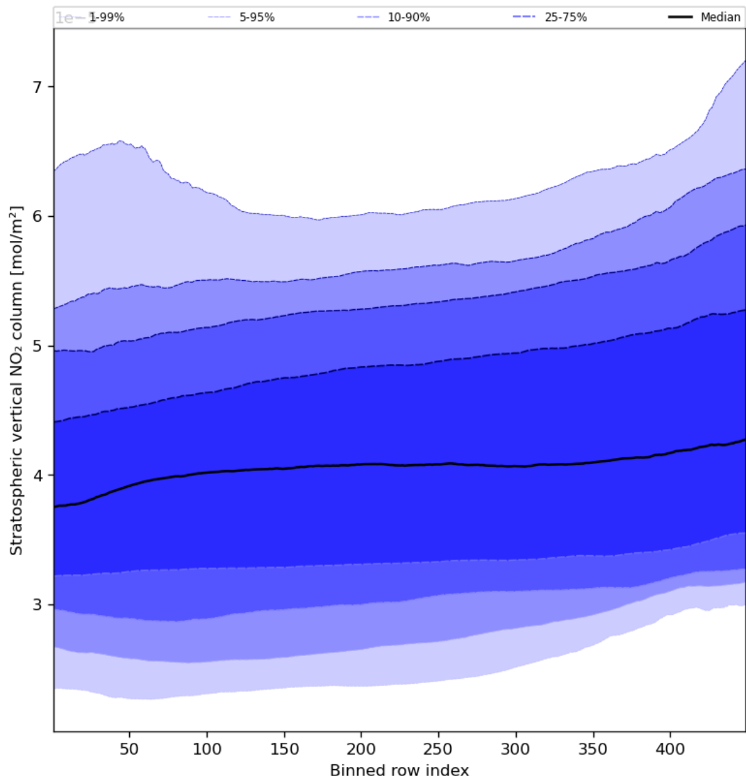
Figure 53: Along track statistics of “Stratospheric vertical NO 2 column” for 2024-03-16 to 2024-03-18
