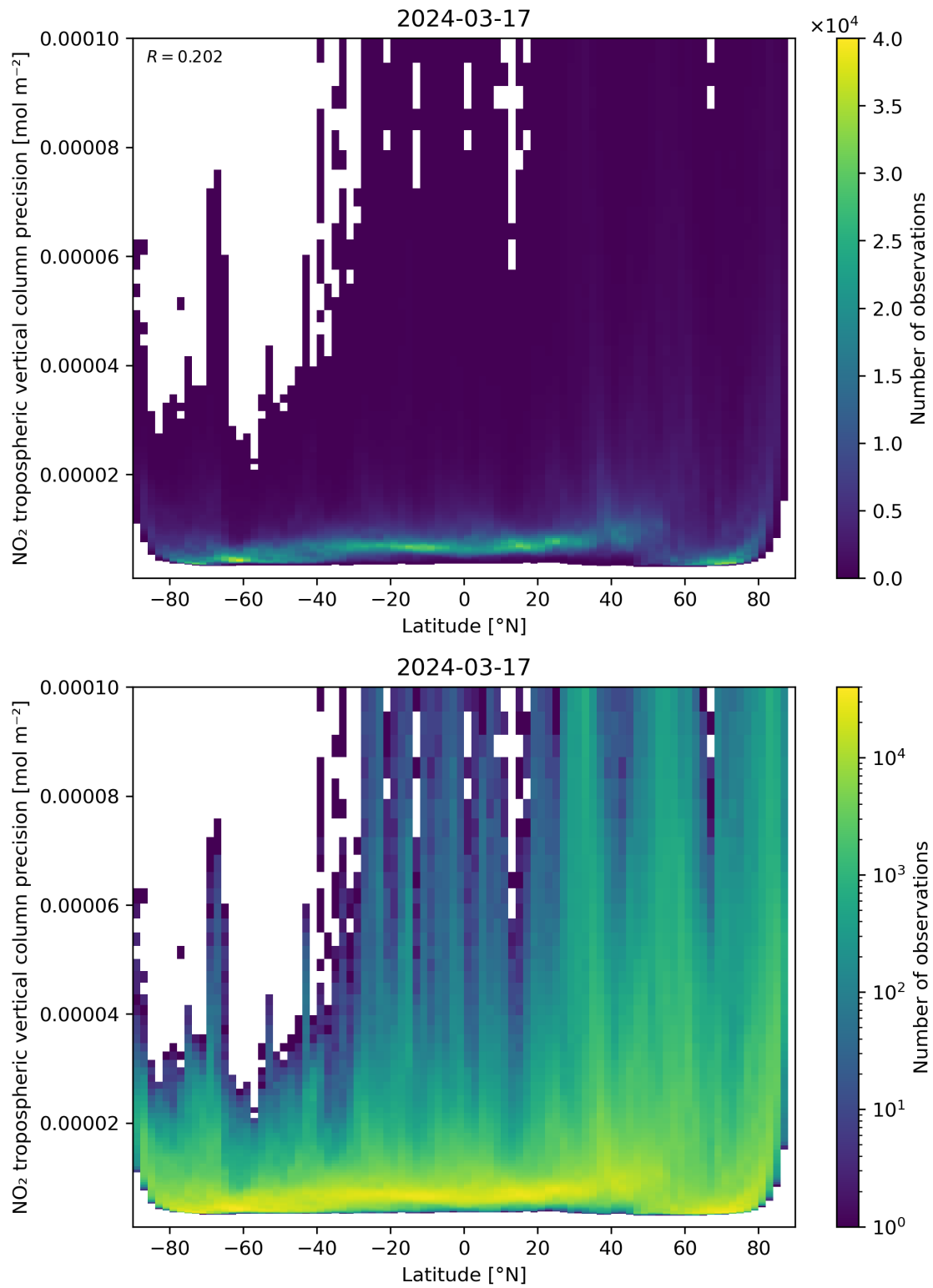
Figure 93: Scatter density plot of “Latitude” against “NO 2 tropospheric vertical column precision” for 2024-03-16 to 2024-03-18.
