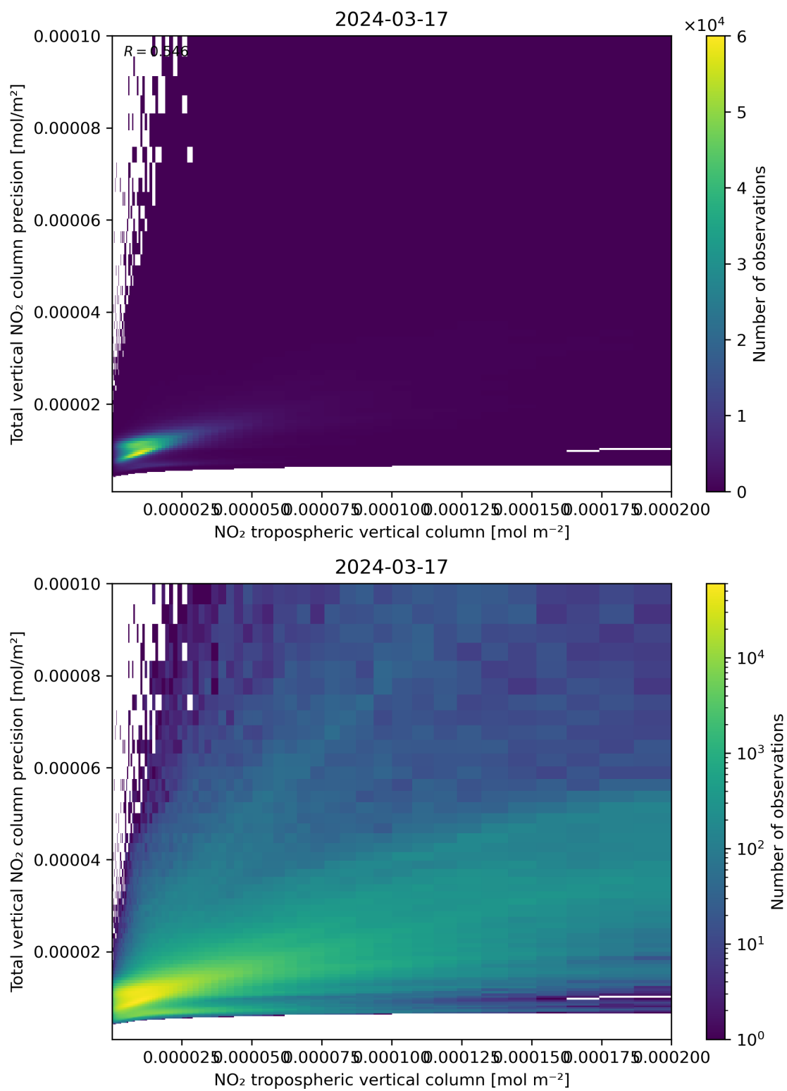
Figure 129: Scatter density plot of “NO 2 tropospheric vertical column” against “Total vertical NO 2 column precision” for 2024-03-16 to 2024-03-18.
