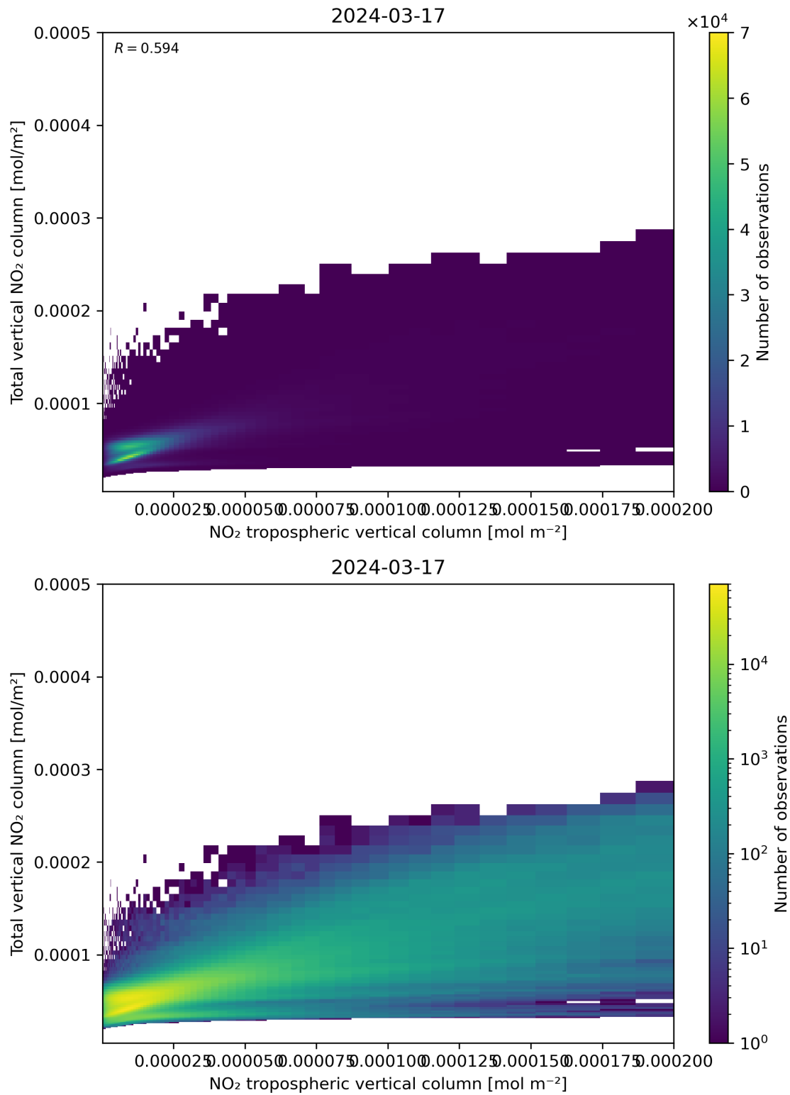
Figure 128: Scatter density plot of “NO 2 tropospheric vertical column” against “Total vertical NO 2 column” for 2024-03-16 to 2024-03-18.
