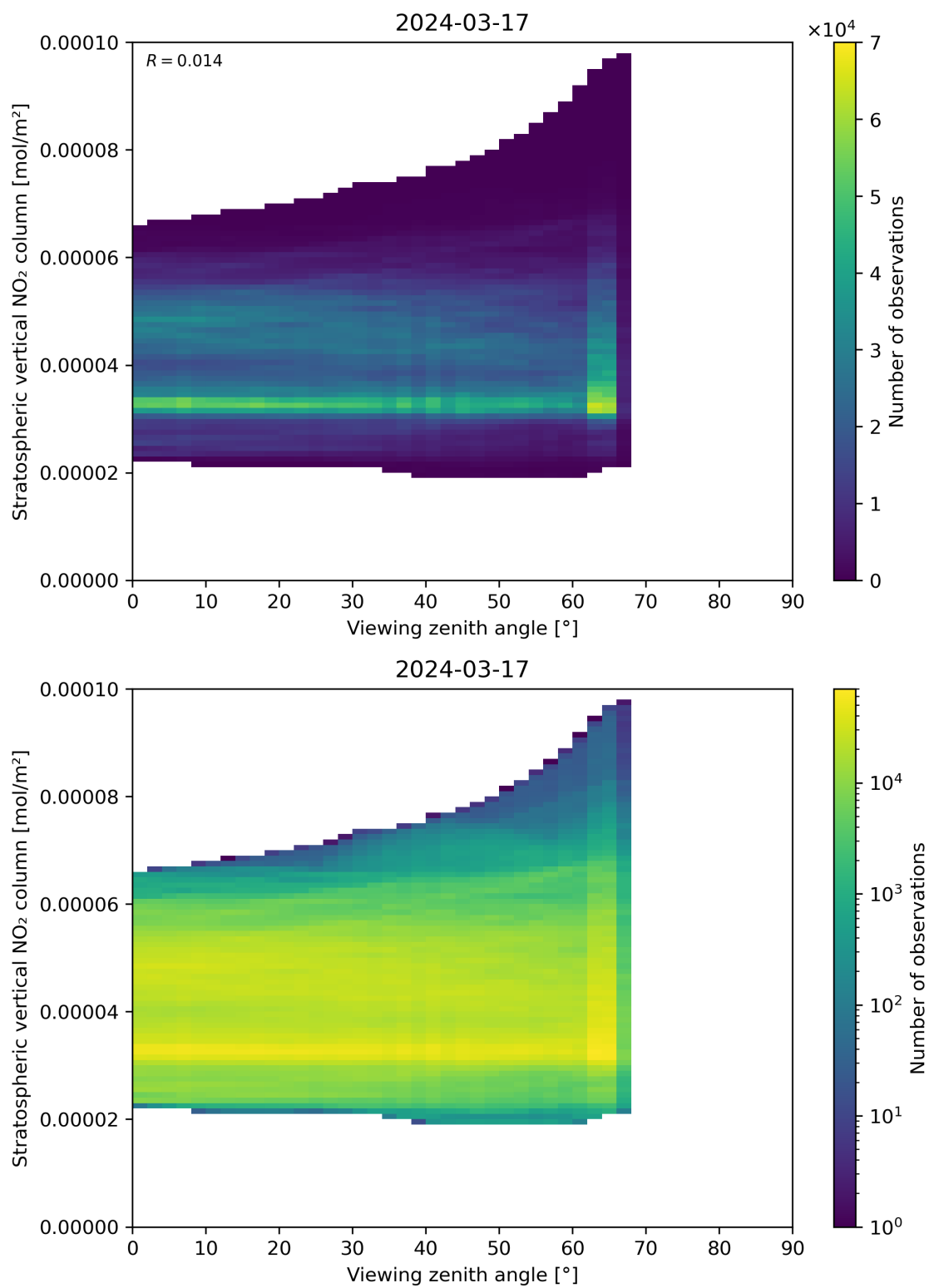
Figure 164: Scatter density plot of “Viewing zenith angle” against “Stratospheric vertical NO 2 column” for 2024-03-16 to 2024-03-18.
