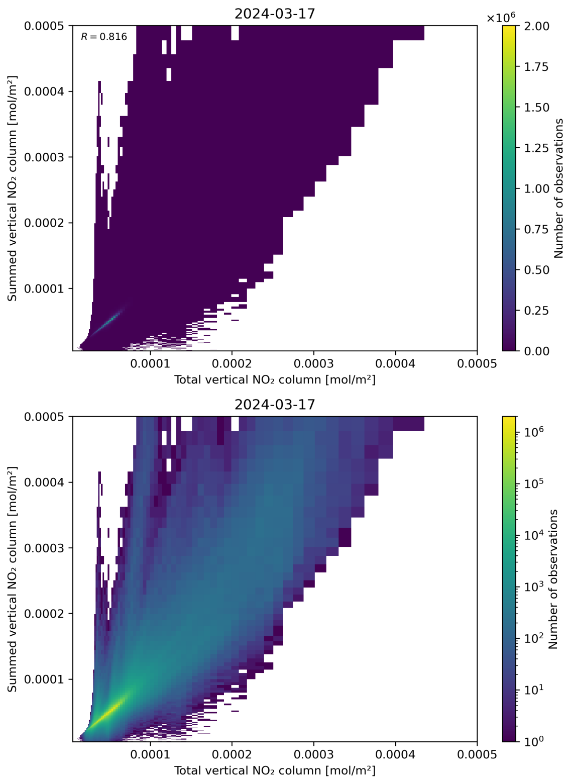
Figure 112: Scatter density plot of “Total vertical NO 2 column” against “Summed vertical NO 2 column” for 2024-03-16 to 2024-03-18.
