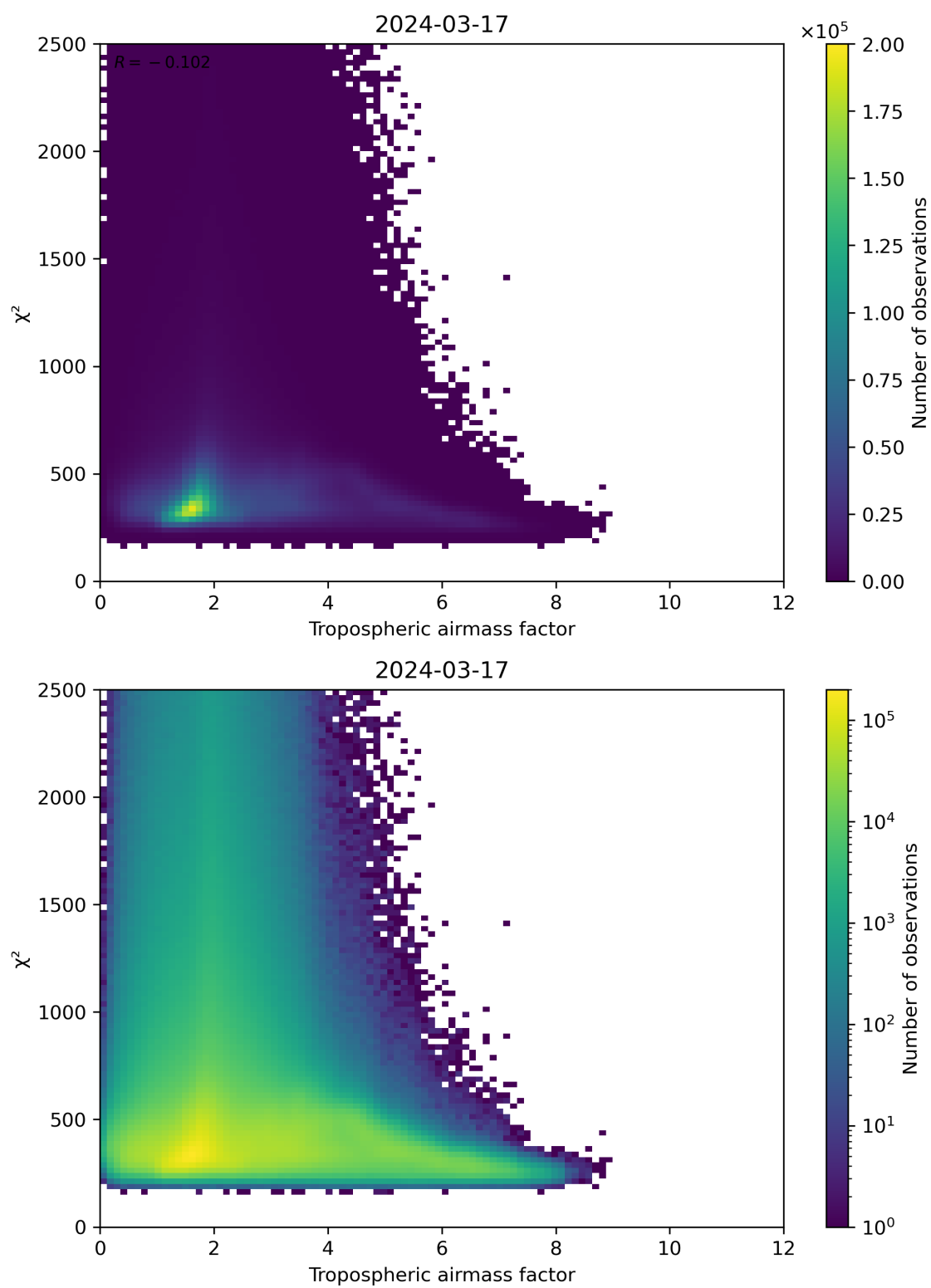
Figure 73: Scatter density plot of “Tropospheric airmass factor” against “ \chi^2 ” for 2024-03-16 to 2024-03-18.
