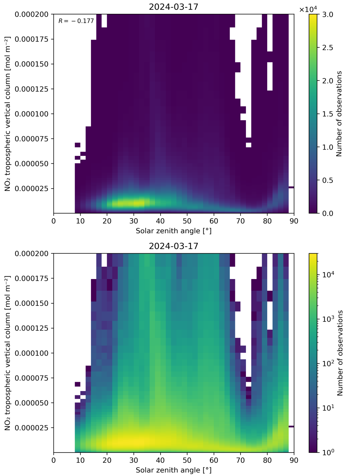
Figure 155: Scatter density plot of “Solar zenith angle” against “NO 2 tropospheric vertical column” for 2024-03-16 to 2024-03-18.
