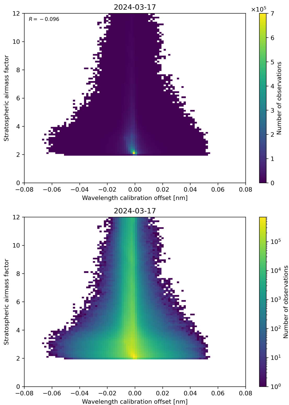
Figure 174: Scatter density plot of “Wavelength calibration offset” against “Stratospheric air mass factor” for 2024-03-16 to 2024-03-18.
