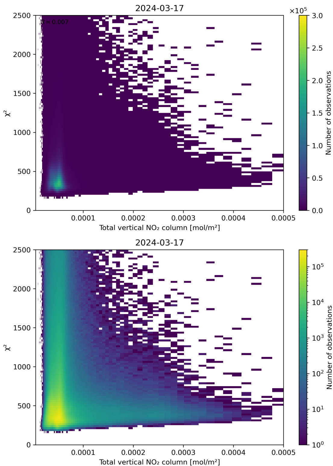
Figure 111: Scatter density plot of “Total vertical NO 2 column” against “ \chi^2 ” for 2024-03-16 to 2024-03-18.
