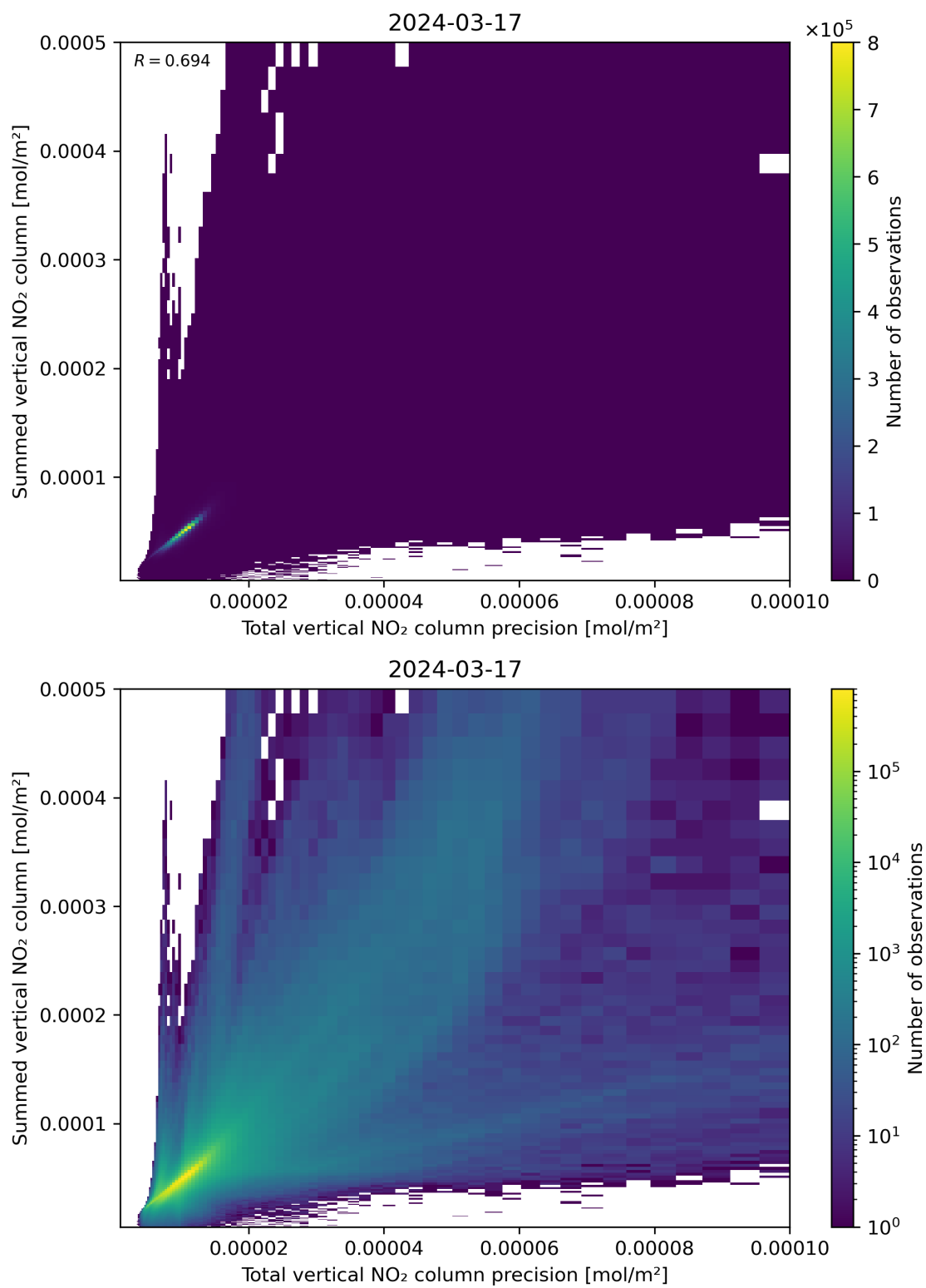
Figure 117: Scatter density plot of “Total vertical NO 2 column precision” against “Summed vertical NO 2 column” for 2024-03-16 to 2024-03-18.
