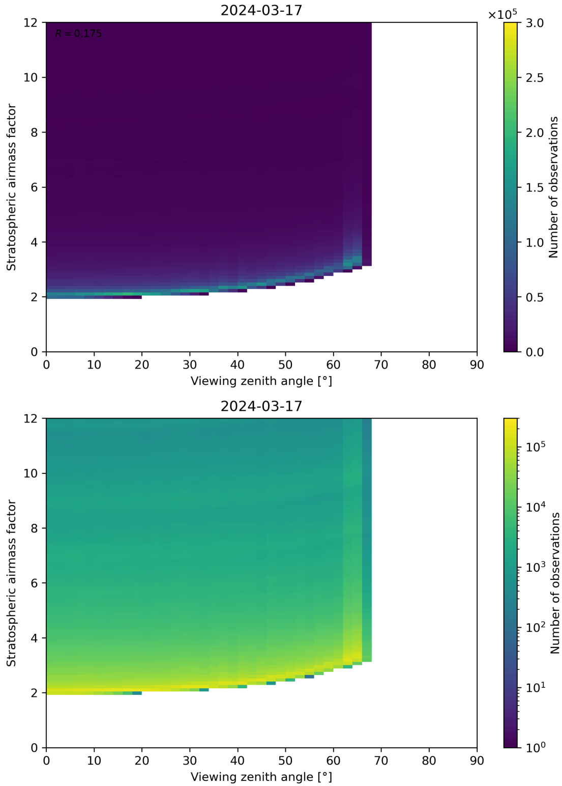
Figure 159: Scatter density plot of “Viewing zenith angle” against “Stratospheric airmass factor” for 2024-03-16 to 2024-03-18.
