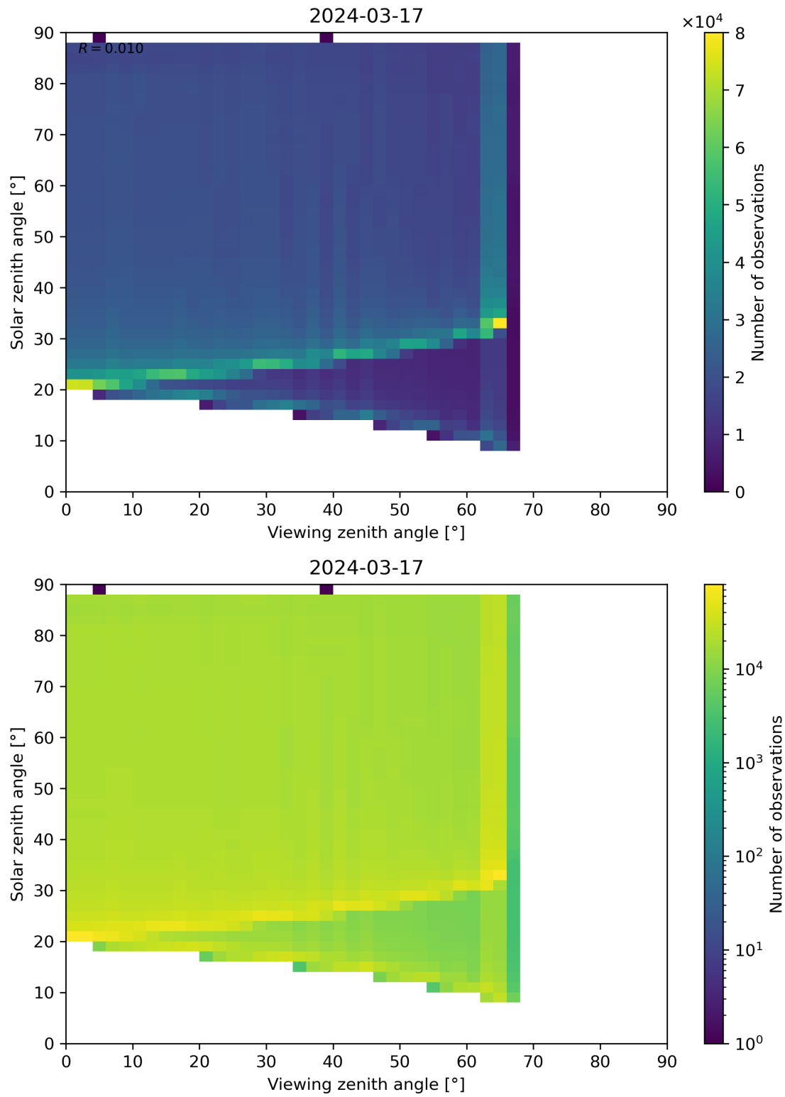
Figure 172: Scatter density plot of “Viewing zenith angle” against “Solar zenith angle” for 2024-03-16 to 2024-03-18.
