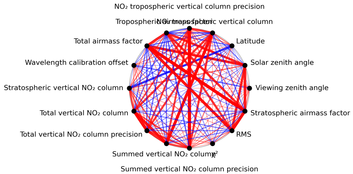
Figure 1: Map of correlation graph for 2024-03-16 to 2024-03-18.
