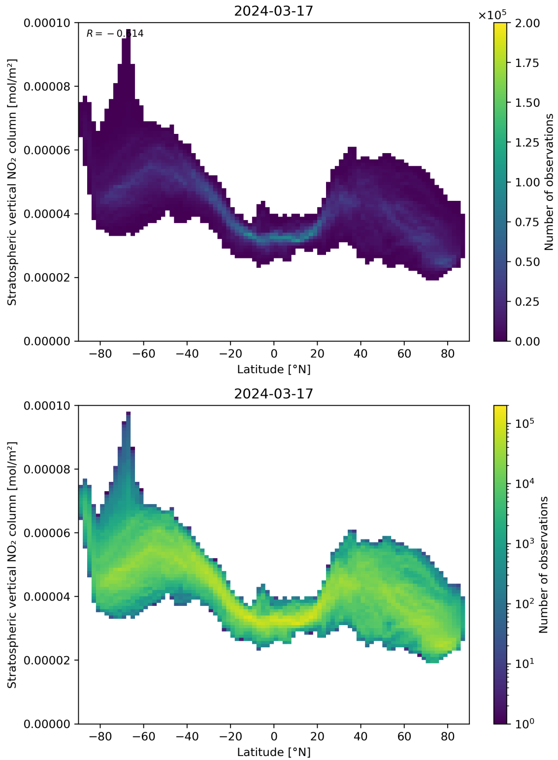
Figure 87: Scatter density plot of “Latitude” against “Stratospheric vertical NO 2 column” for 2024-03-16 to 2024-03-18.
