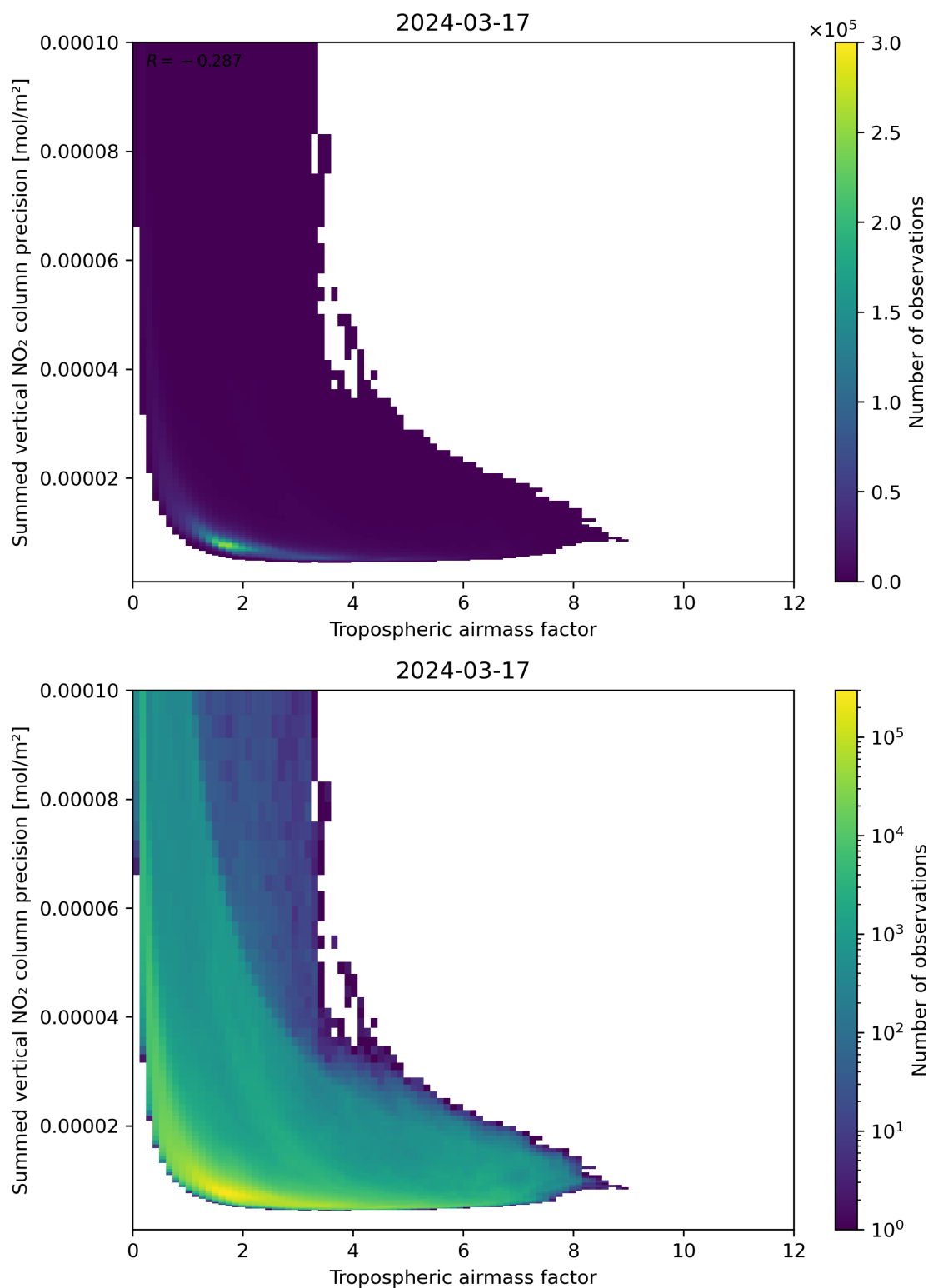
Figure 76: Scatter density plot of “Tropospheric air mass factor” against “Summed vertical NO 2 column precision” for 2024-03-16 to 2024-03-18.
