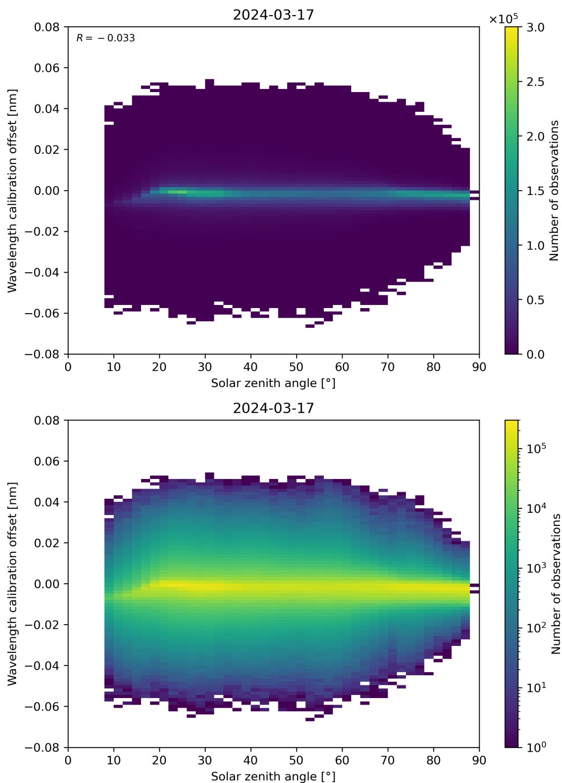
Figure 158: Scatter density plot of “Solar zenith angle” against “Wavelength calibration offset” for 2024-03-16 to 2024-03-18.
