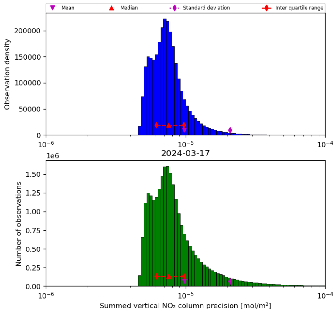
Figure 41: Histogram of "Summed vertical NO 2 column precision" for 2024-03-16 to 2024-03-18
