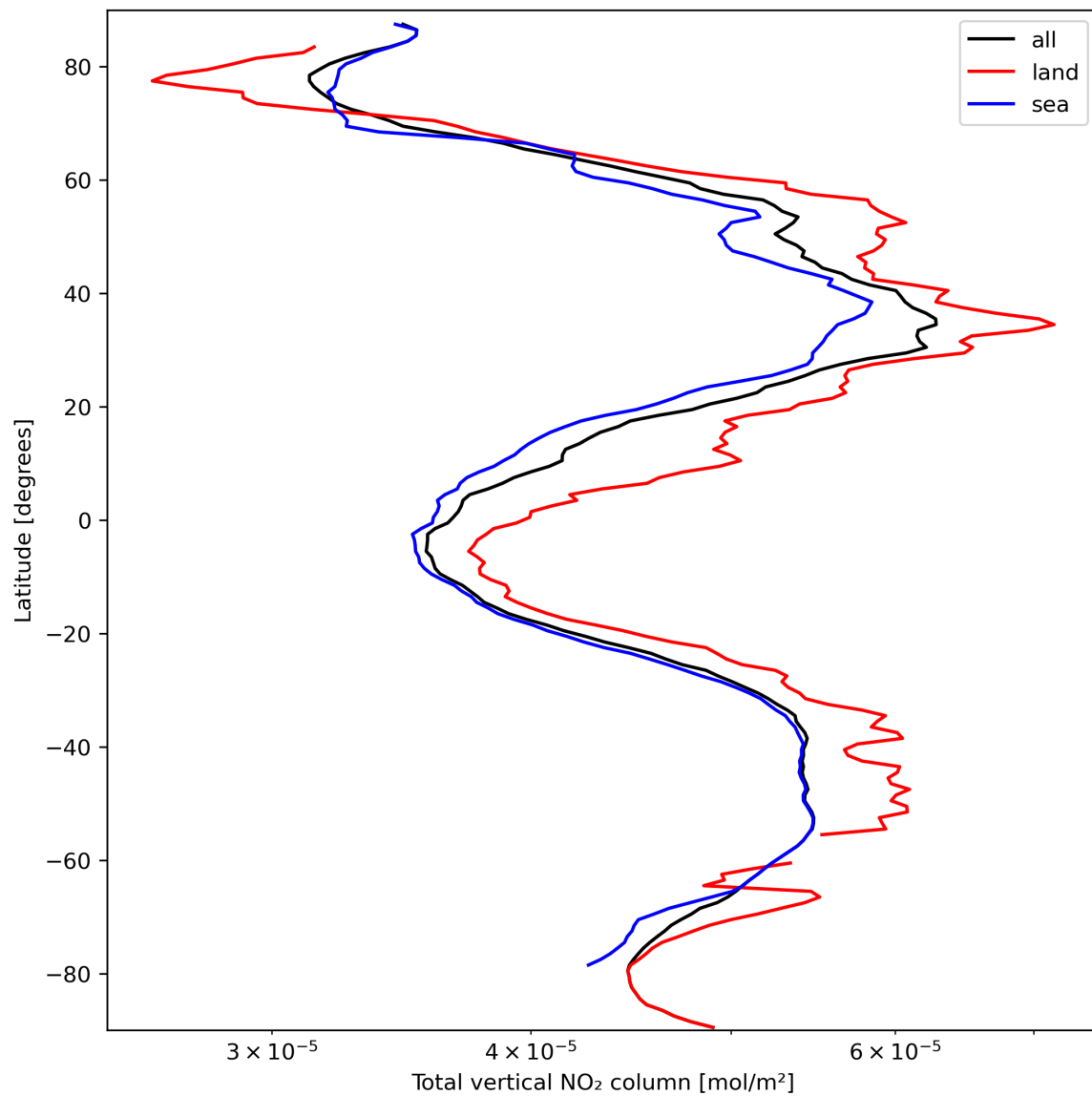
Figure 21: Zonal average of “Total vertical NO 2 column” for 2024-03-16 to 2024-03-18.
