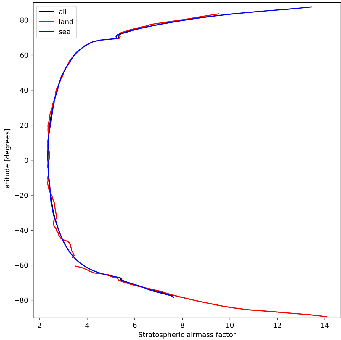
Figure 27: Zonal average of “Stratospheric airmass factor” for 2024-03-16 to 2024-03-18.
