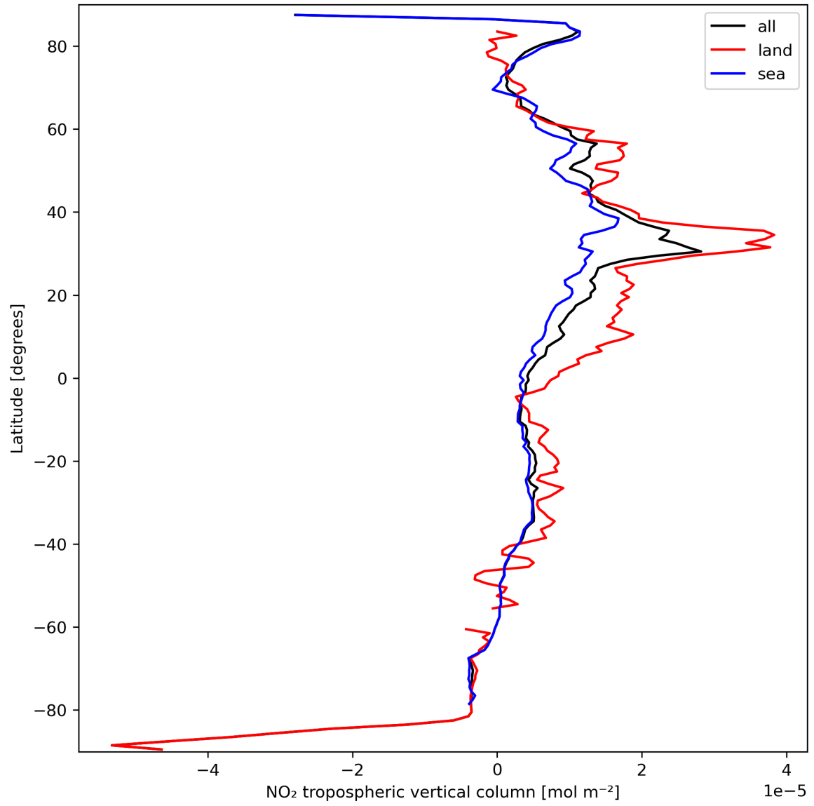
Figure 12: Zonal average of “NO 2 tropospheric vertical column” for 2024-03-16 to 2024-03-18.
