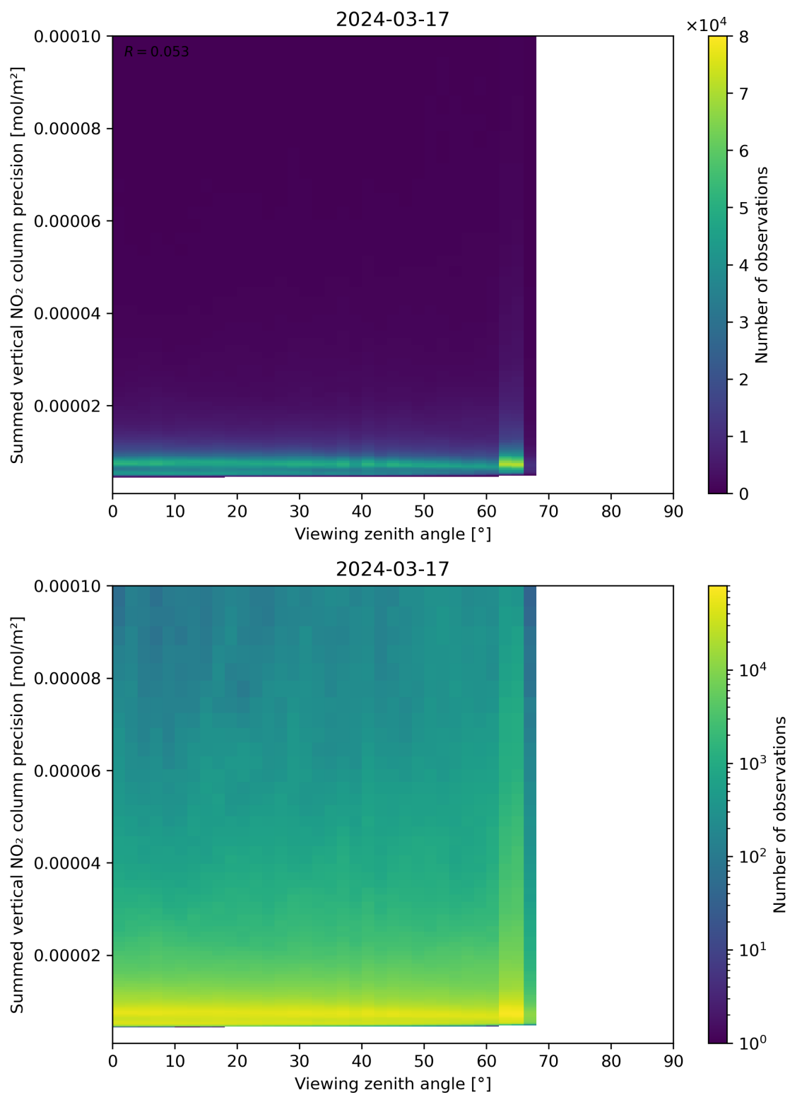
Figure 166: Scatter density plot of “Viewing zenith angle” against “Summed vertical NO 2 column precision” for 2024-03-16 to 2024-03-18.
