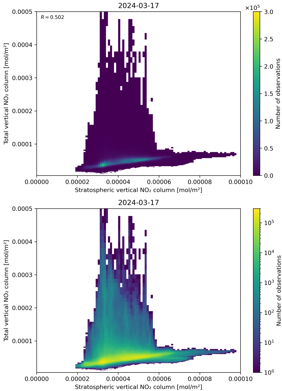
Figure 100: Scatter density plot of “Stratospheric vertical NO 2 column” against “Total vertical NO 2 column” for 2024-03-16 to 2024-03-18.
