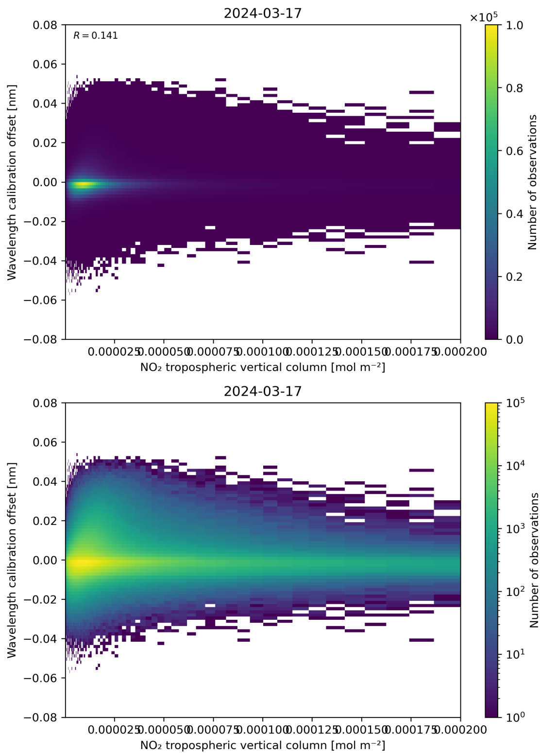
Figure 143: Scatter density plot of “NO 2 tropospheric vertical column” against “Wavelength calibration offset” for 2024-03-16 to 2024-03-18.
