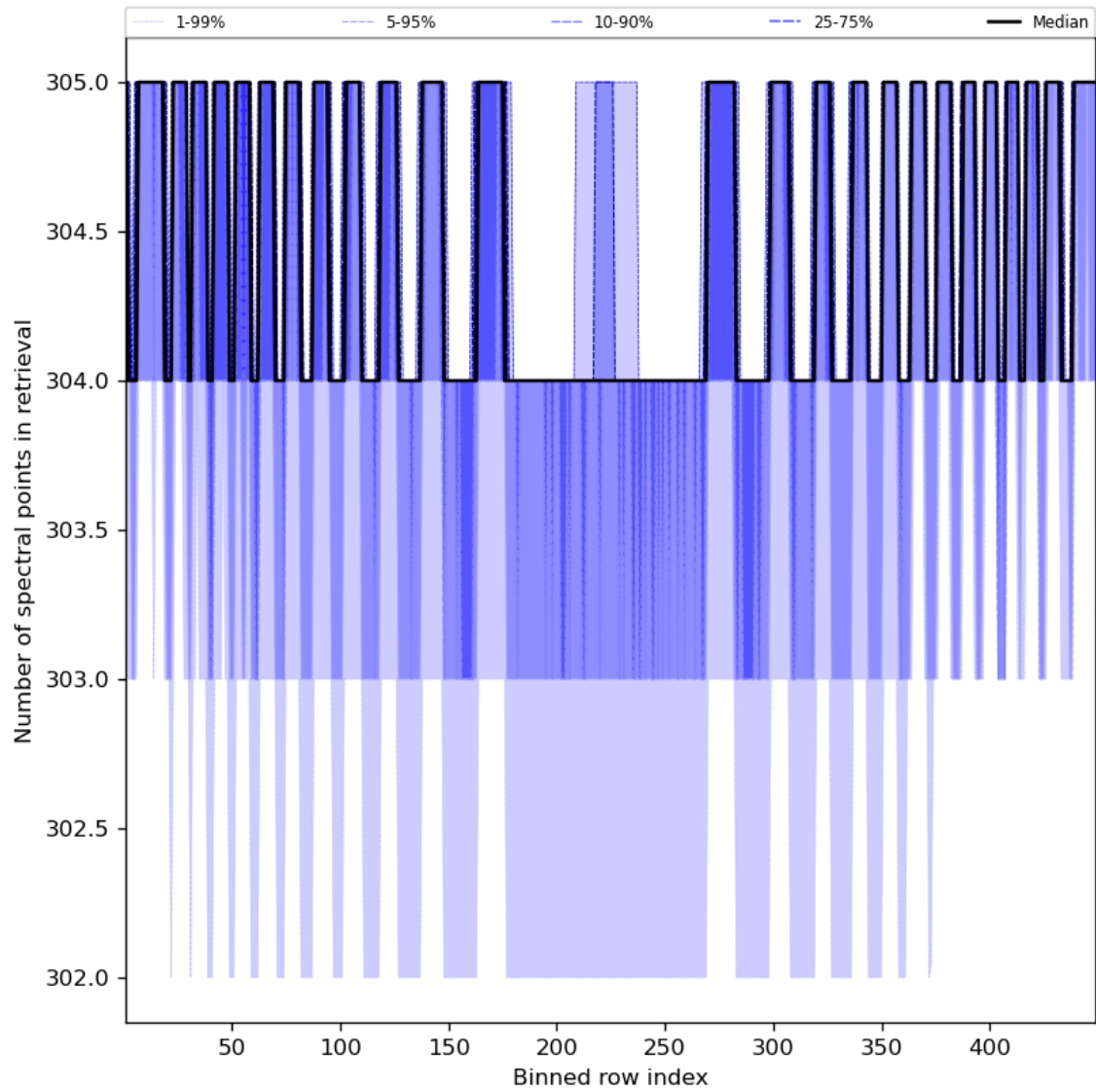
Figure 50: Along track statistics of “Number of spectral points in retrieval” for 2024-03-16 to 2024-03-18
