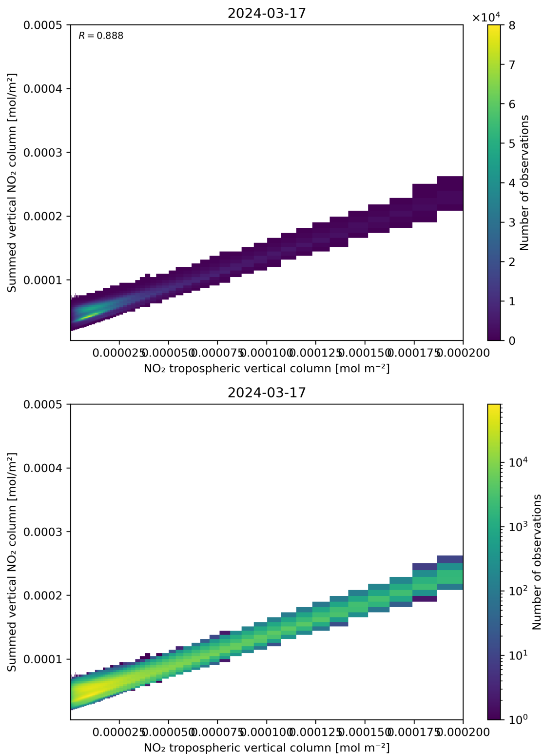
Figure 126: Scatter density plot of “NO 2 tropospheric vertical column” against “Summed vertical NO 2 column” for 2024-03-16 to 2024-03-18.
