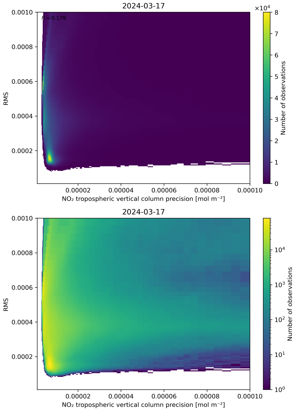
Figure 140: Scatter density plot of “NO 2 tropospheric vertical column precision” against “RMS” for 2024-03-16 to 2024-03-18.
