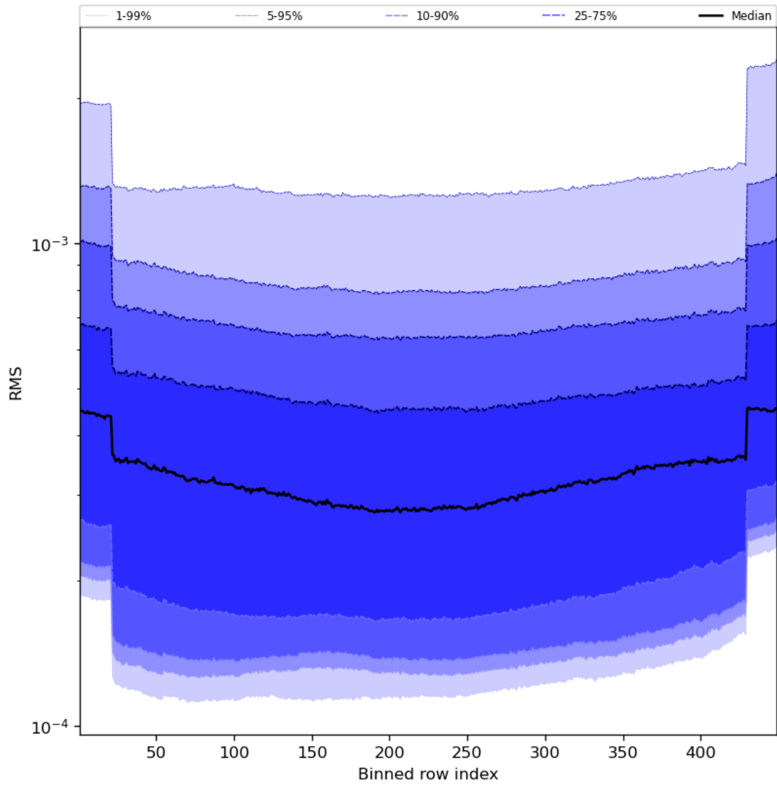
Figure 60: Along track statistics of “RMS” for 2024-03-16 to 2024-03-18
