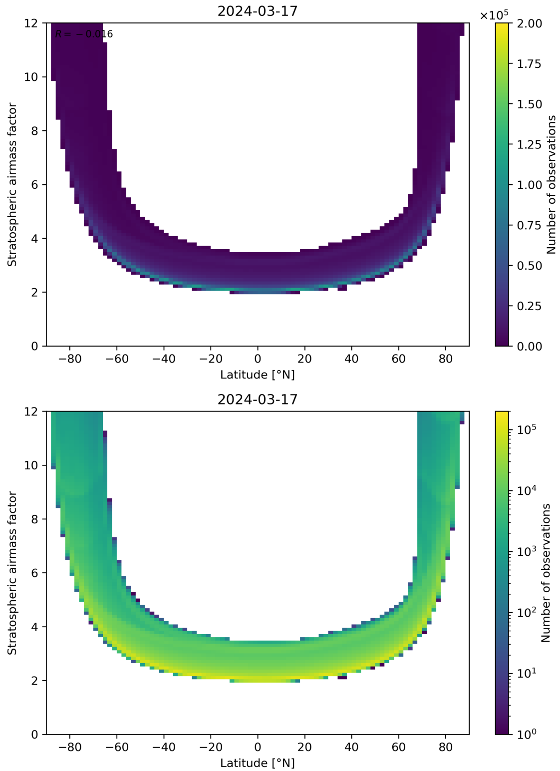
Figure 83: Scatter density plot of “Latitude” against “Stratospheric airmass factor” for 2024-03-16 to 2024-03-18.
