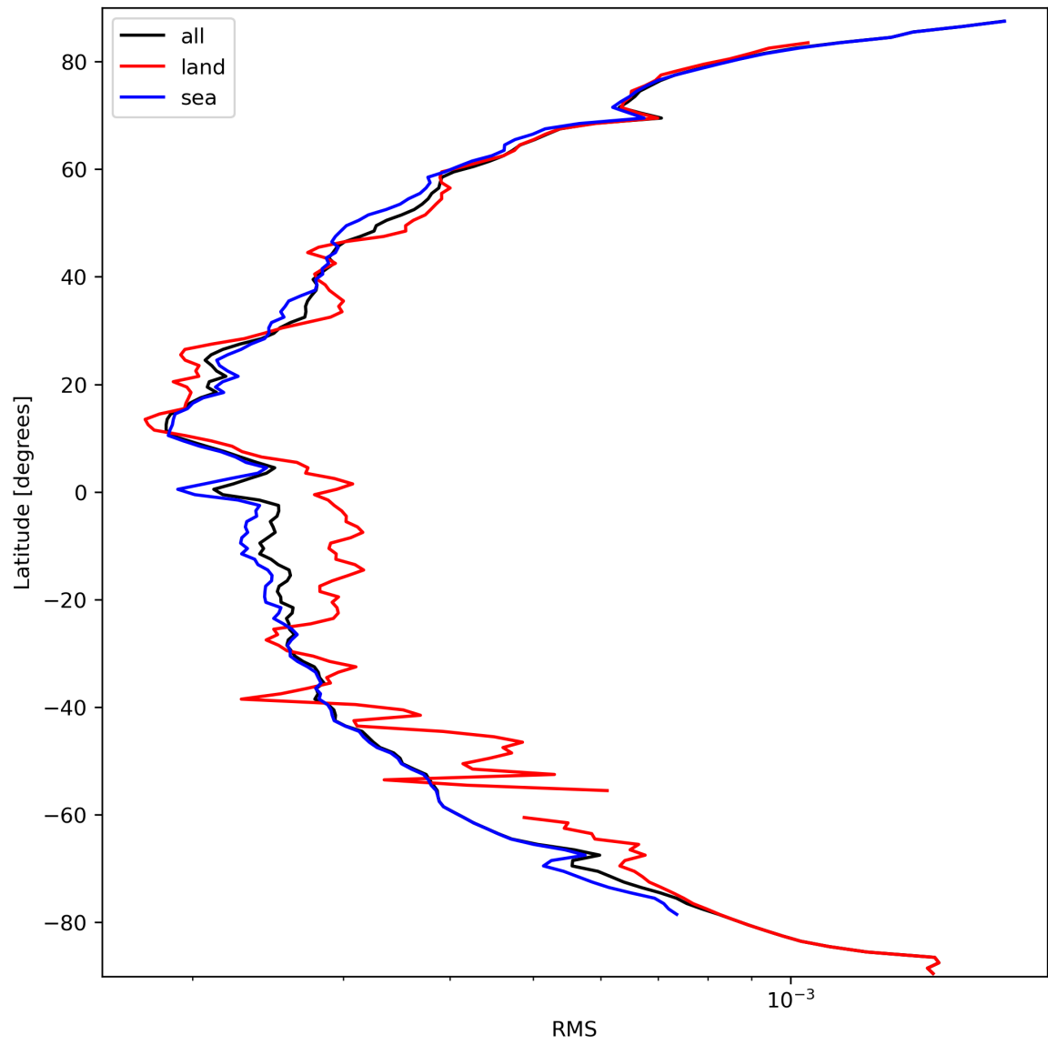
Figure 26: Zonal average of “RMS” for 2024-03-16 to 2024-03-18.
