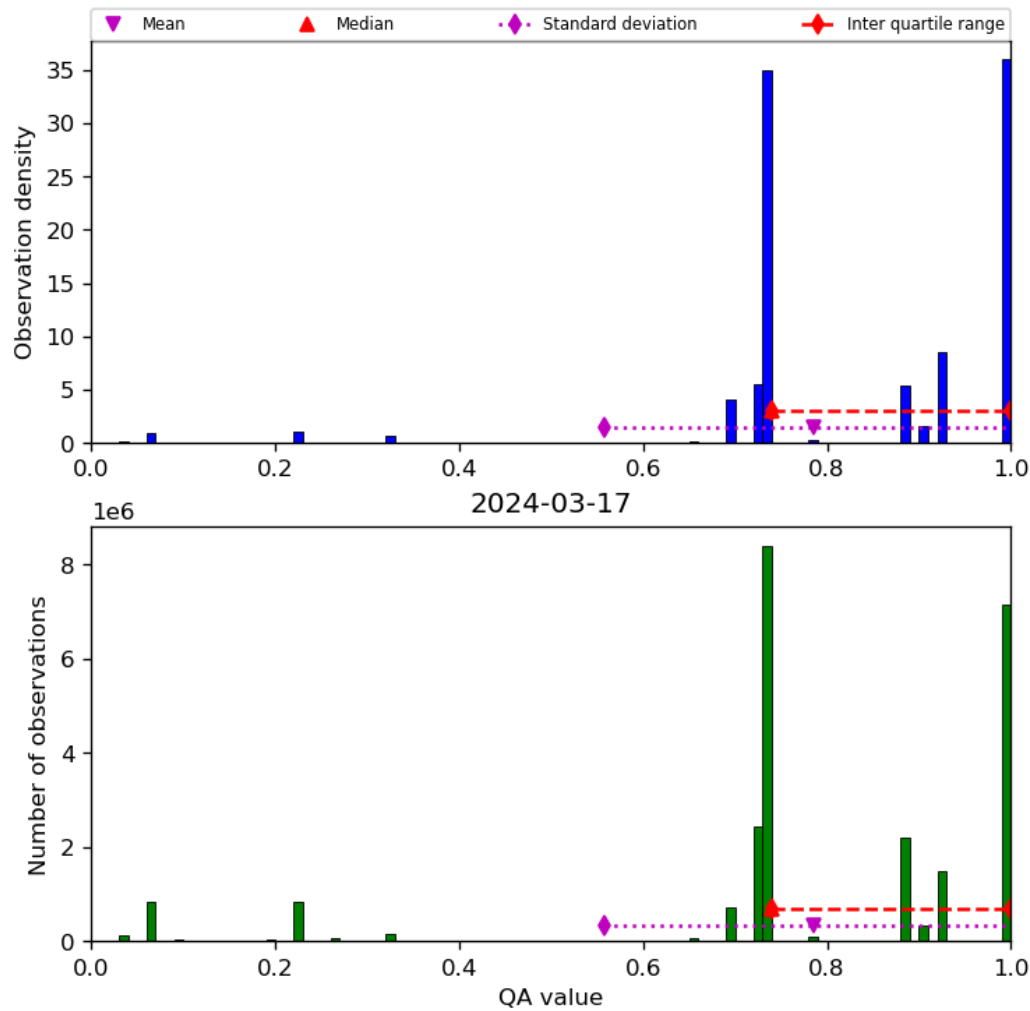
Figure 28: Histogram of “QA value” for 2024-03-16 to 2024-03-18
