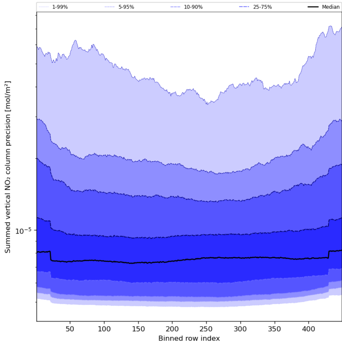
Figure 58: Along track statistics of “Summed vertical NO 2 column precision” for 2024-03-16 to 2024-03-18
