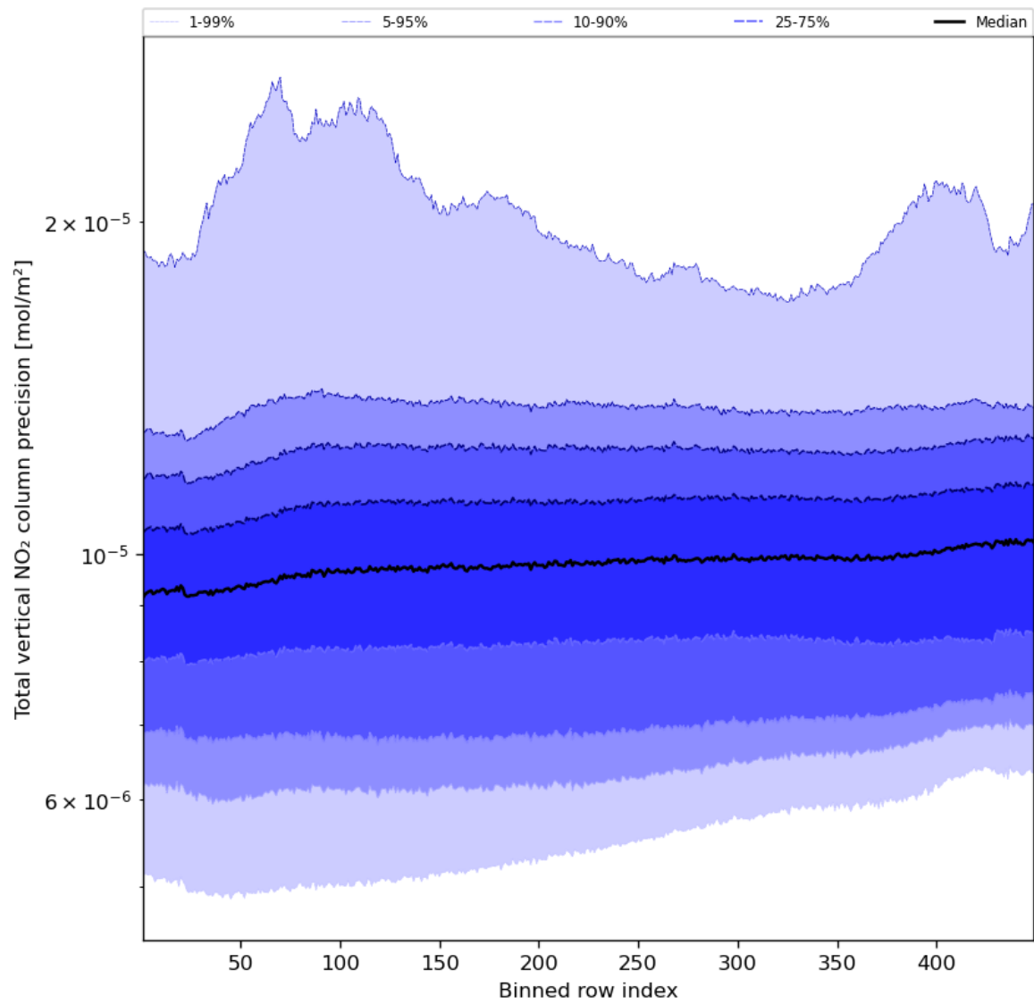
Figure 56: Along track statistics of “Total vertical NO 2 column precision” for 2024-03-16 to 2024-03-18
