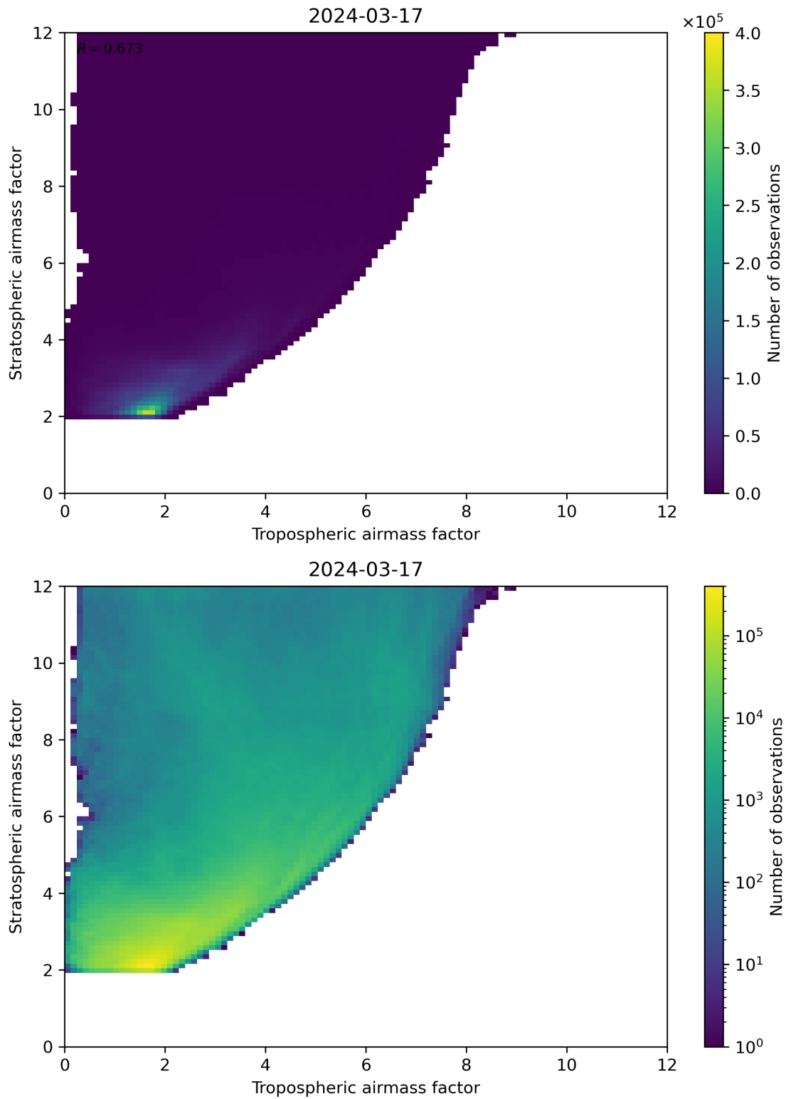
Figure 71: Scatter density plot of “Tropospheric airmass factor” against “Stratospheric airmass factor” for 2024-03-16 to 2024-03-18.
