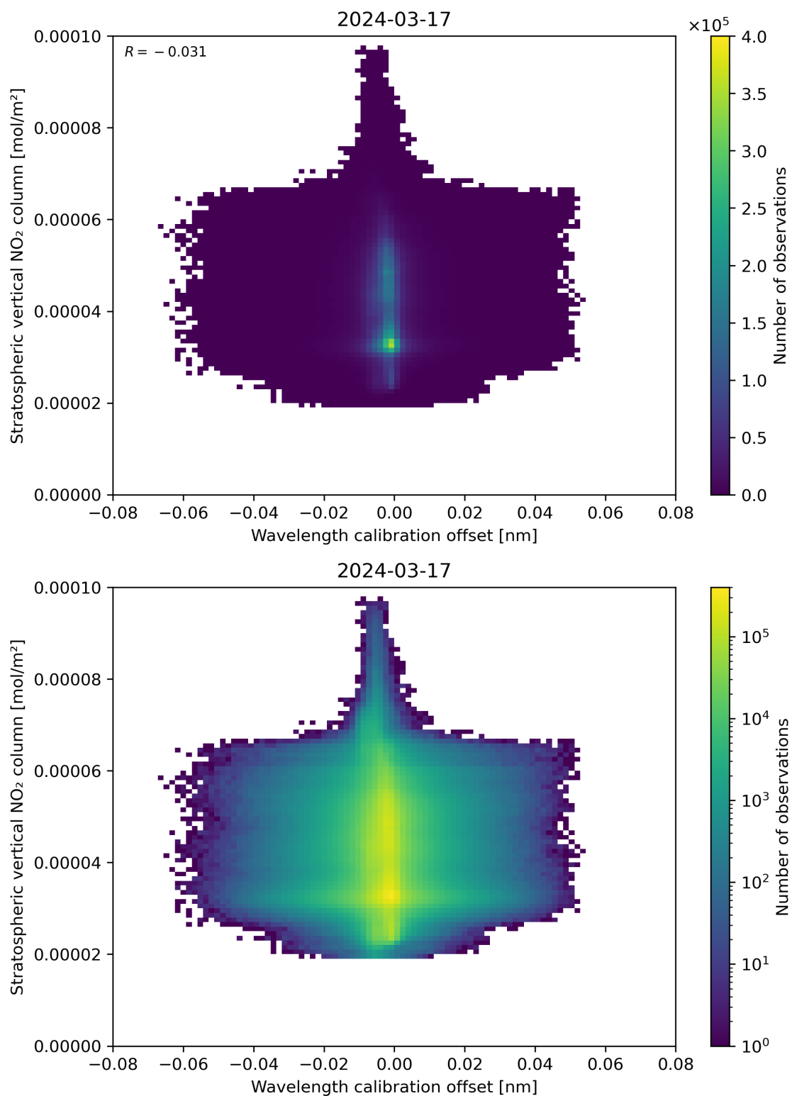
Figure 176: Scatter density plot of “Wavelength calibration offset” against “Stratospheric vertical NO 2 column” for 2024-03-16 to 2024-03-18.
