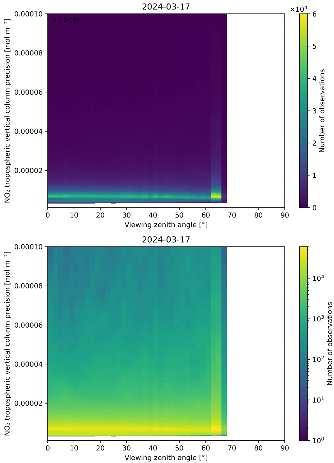
Figure 170: Scatter density plot of “Viewing zenith angle” against “NO 2 tropospheric vertical column precision” for 2024-03-16 to 2024-03-18.
