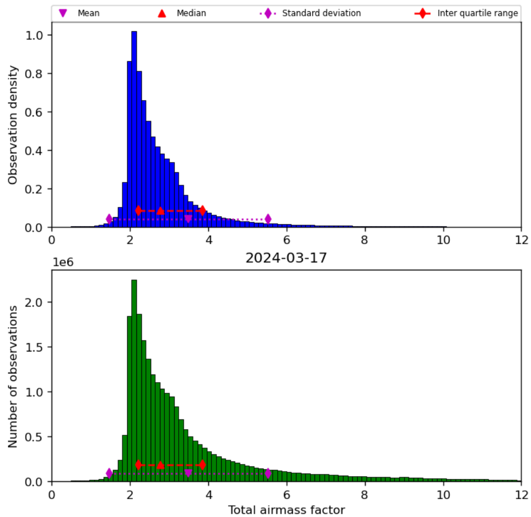
Figure 32: Histogram of “Total airmass factor” for 2024-03-16 to 2024-03-18
