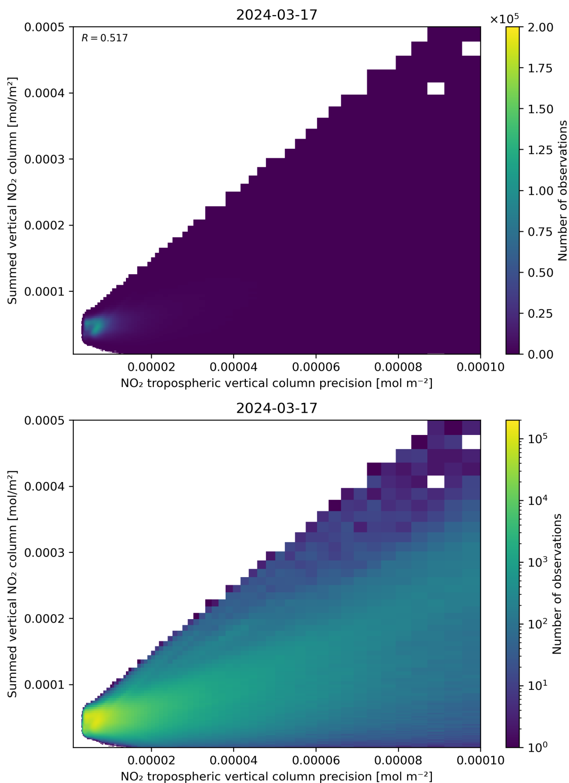
Figure 136: Scatter density plot of “NO 2 tropospheric vertical column precision” against “Summed vertical NO 2 column” for 2024-03-16 to 2024-03-18.
