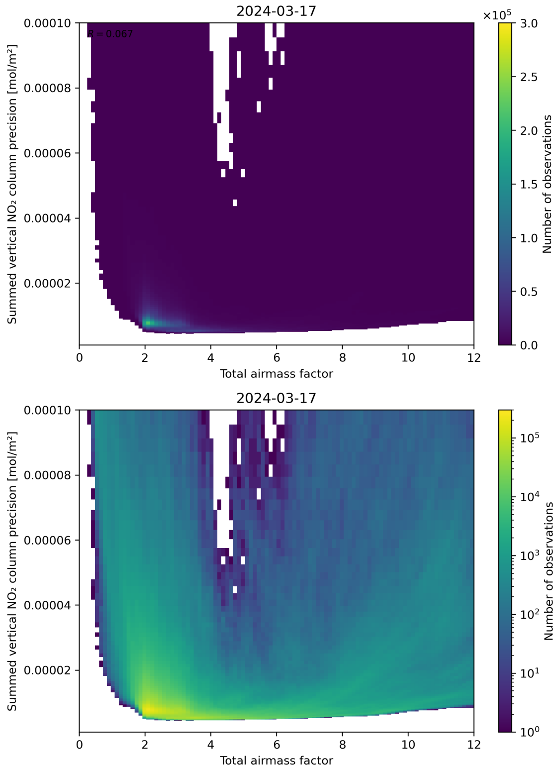
Figure 66: Scatter density plot of “Total airmass factor” against “Summed vertical NO 2 column precision” for 2024-03-16 to 2024-03-18.
