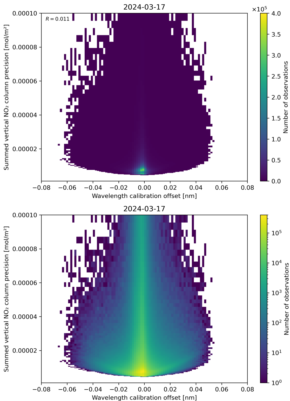
Figure 178: Scatter density plot of “Wavelength calibration offset” against “Summed vertical NO 2 column precision” for 2024-03-16 to 2024-03-18.
