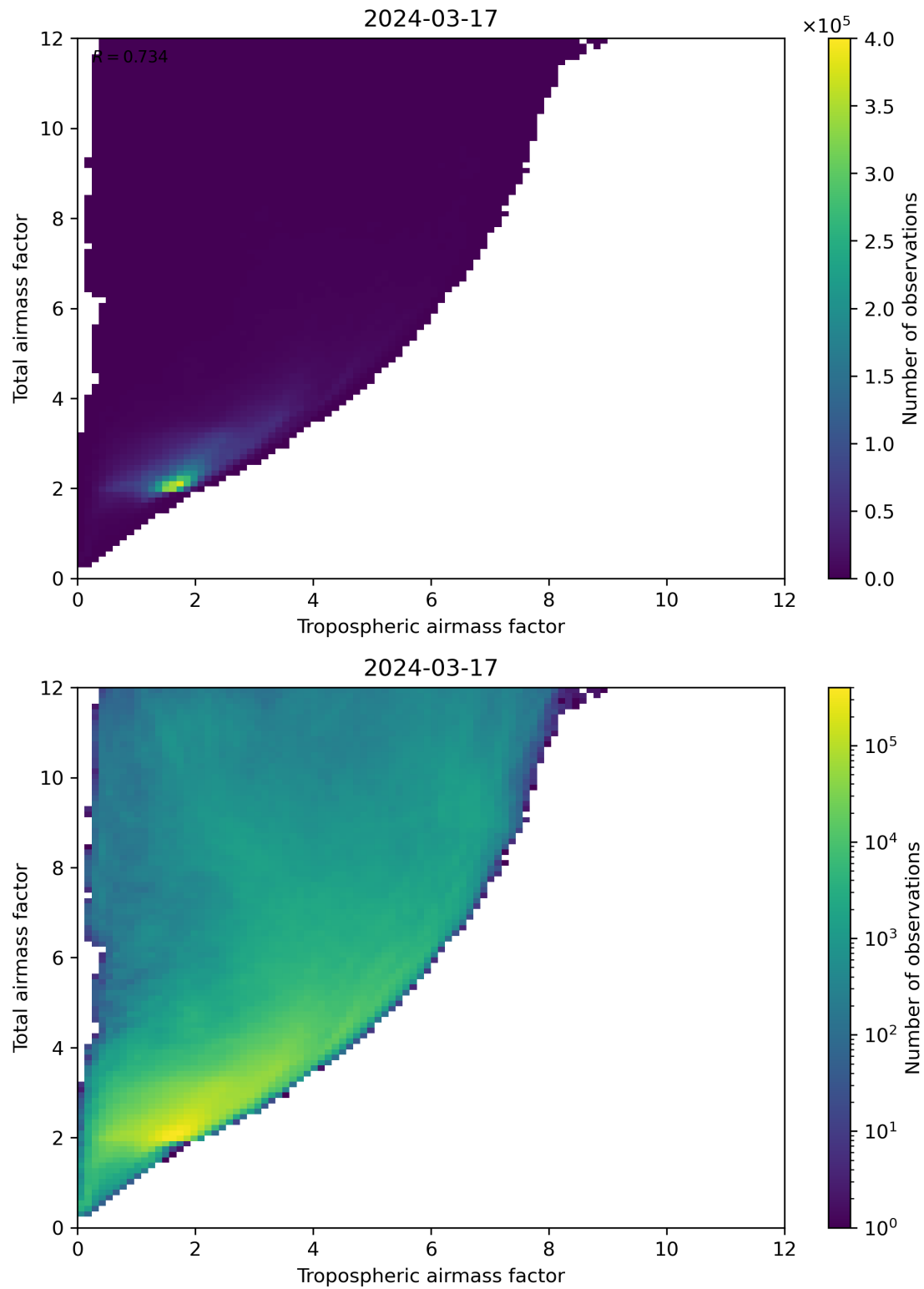
Figure 72: Scatter density plot of “Tropospheric airmass factor” against “Total airmass factor” for 2024-03-16 to 2024-03-18.
