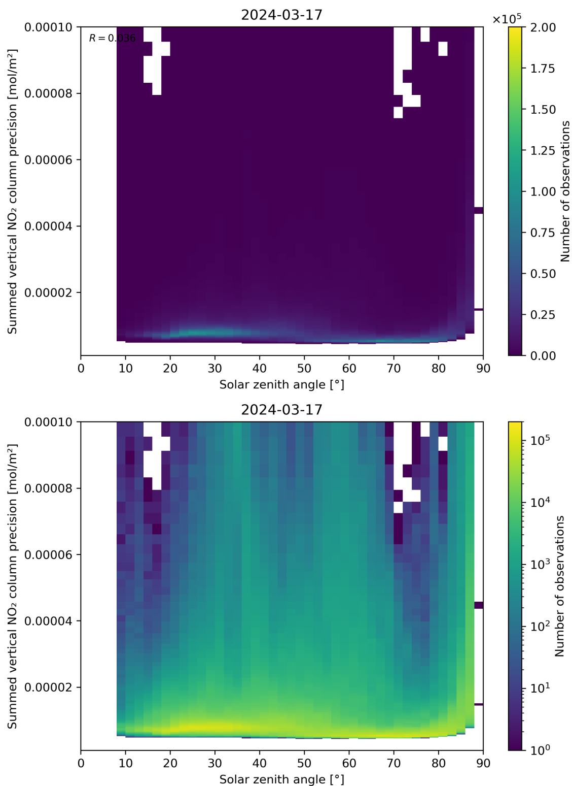
Figure 152: Scatter density plot of “Solar zenith angle” against “Summed vertical NO 2 column precision” for 2024-03-16 to 2024-03-18.
