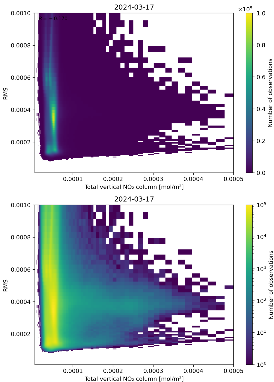
Figure 120: Scatter density plot of “Total vertical NO 2 column” against “RMS” for 2024-03-16 to 2024-03-18.
