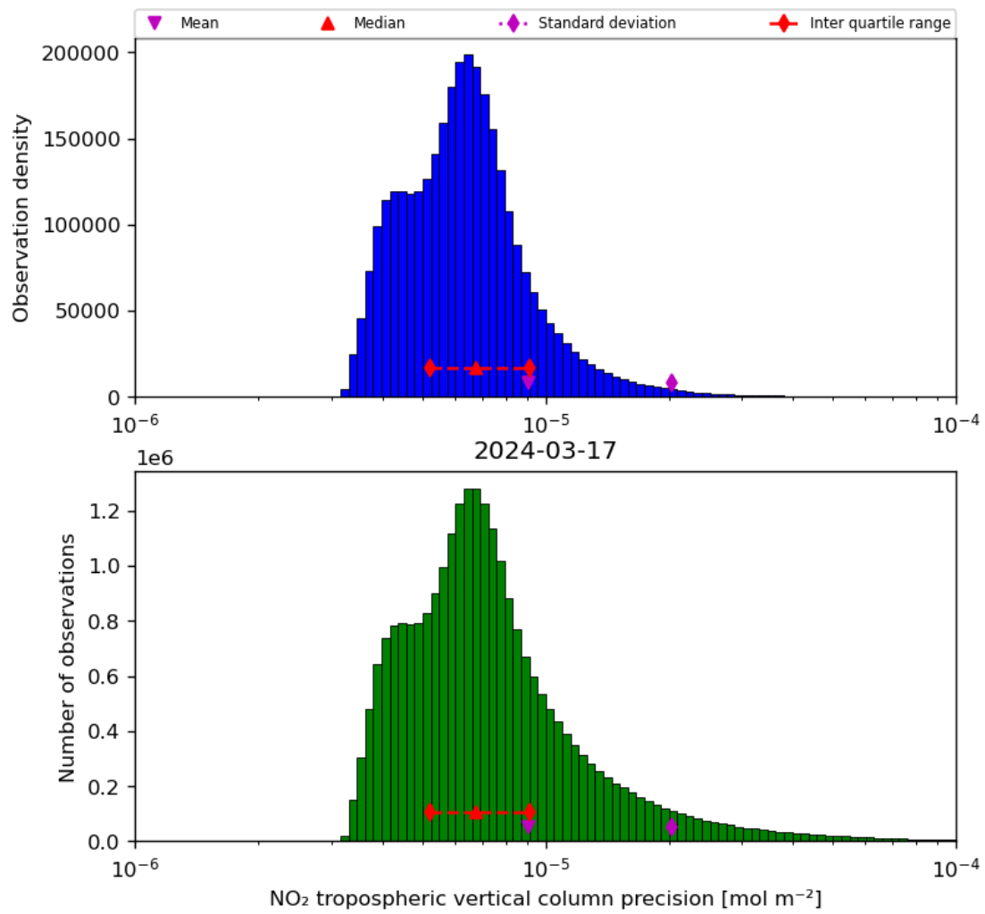
Figure 30: Histogram of “NO 2 tropospheric vertical column precision” for 2024-03-16 to 2024-03-18
