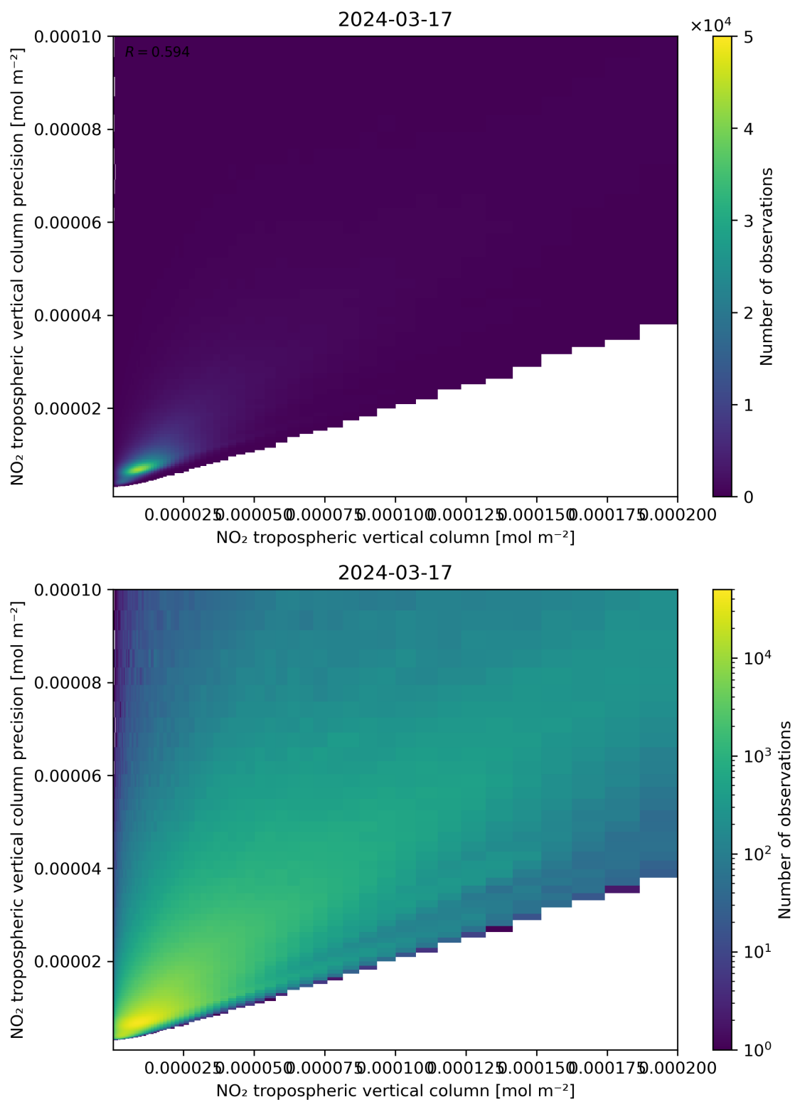
Figure 130: Scatter density plot of “NO 2 tropospheric vertical column” against “NO 2 tropospheric vertical column precision” for 2024-03-16 to 2024-03-18.
