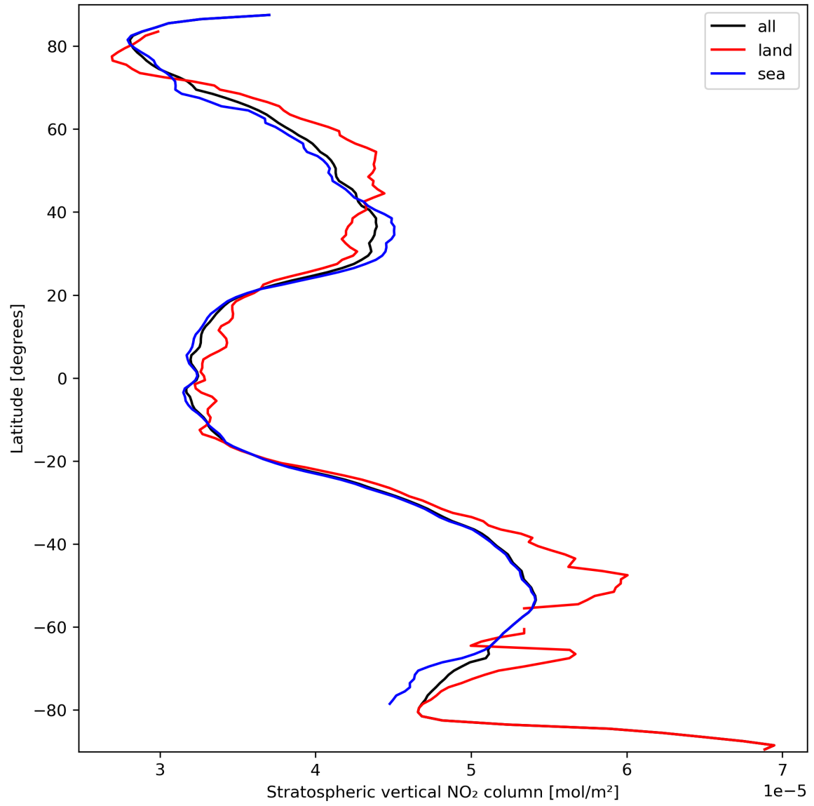
Figure 19: Zonal average of “Stratospheric vertical NO 2 column” for 2024-03-16 to 2024-03-18.
