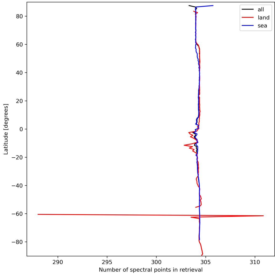
Figure 16: Zonal average of “Number of spectral points in retrieval” for 2024-03-16 to 2024-03-18.
