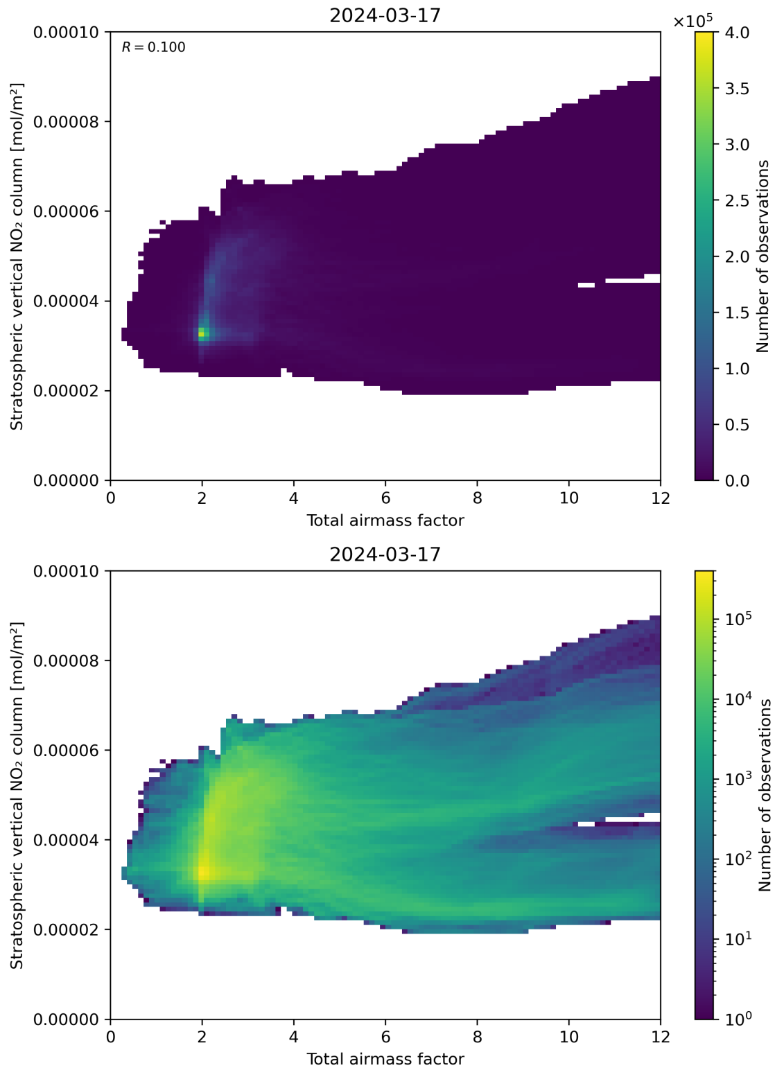
Figure 64: Scatter density plot of “Total airmass factor” against “Stratospheric vertical \text{NO}_2 column” for 2024-03-16 to 2024-03-18.
