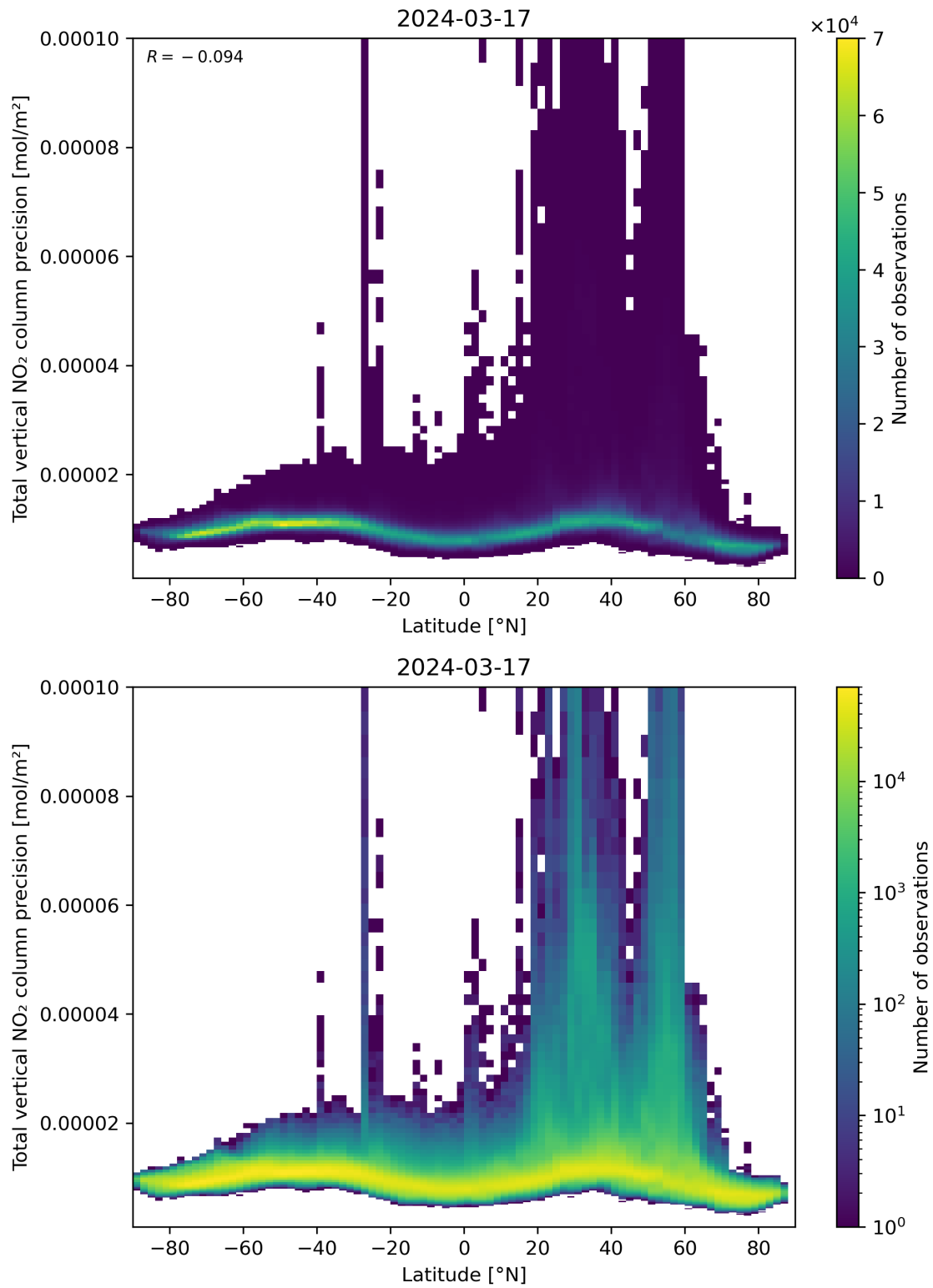
Figure 91: Scatter density plot of “Latitude” against “Total vertical NO 2 column precision” for 2024-03-16 to 2024-03-18.
