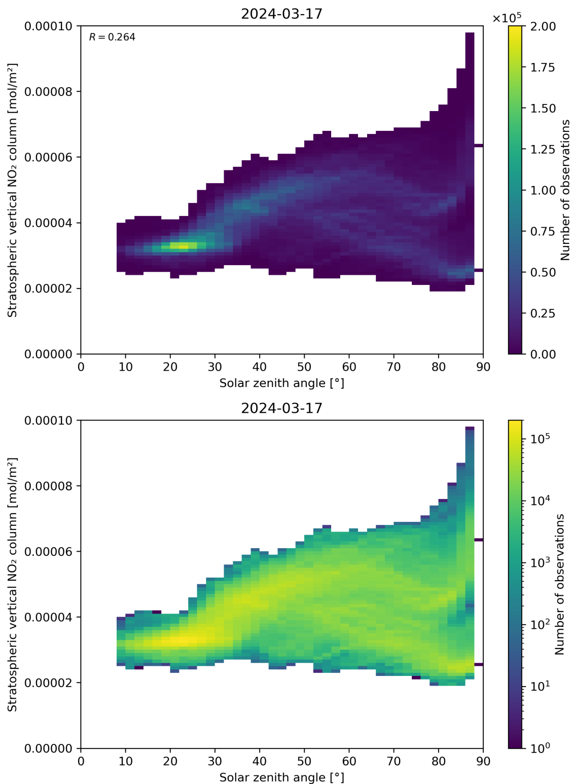
Figure 150: Scatter density plot of “Solar zenith angle” against “Stratospheric vertical \text{NO}_2 column” for 2024-03-16 to 2024-03-18.
