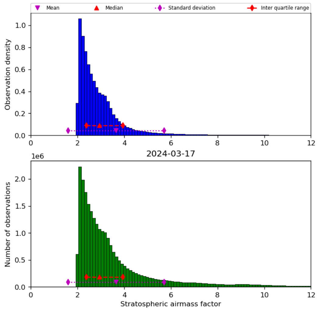
Figure 44: Histogram of “Stratospheric airmass factor” for 2024-03-16 to 2024-03-18
