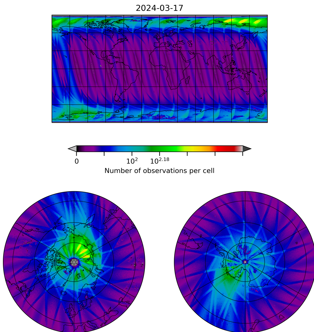
Figure 10: Map of the number of observations for 2024-03-16 to 2024-03-18
