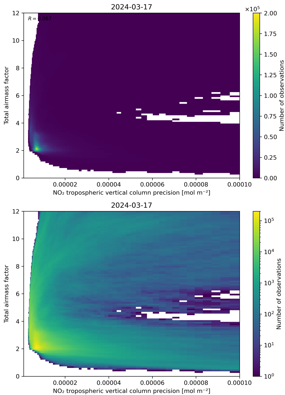
Figure 132: Scatter density plot of “NO 2 tropospheric vertical column precision” against “Total air mass factor” for 2024-03-16 to 2024-03-18.
