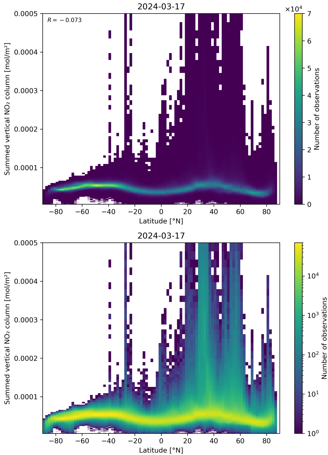
Figure 88: Scatter density plot of “Latitude” against “Summed vertical NO 2 column” for 2024-03-16 to 2024-03-18.
