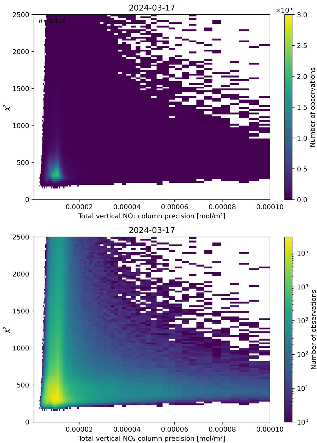
Figure 116: Scatter density plot of “Total vertical NO 2 column precision” against “ \chi^2 ” for 2024-03-16 to 2024-03-18.
