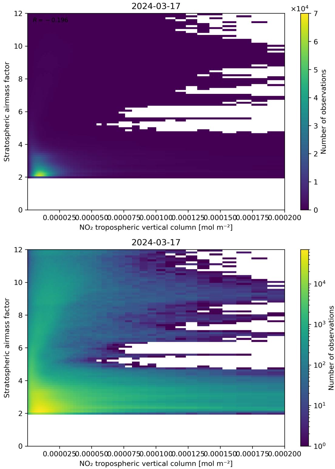
Figure 121: Scatter density plot of “NO 2 tropospheric vertical column” against “Stratospheric air mass factor” for 2024-03-16 to 2024-03-18.
