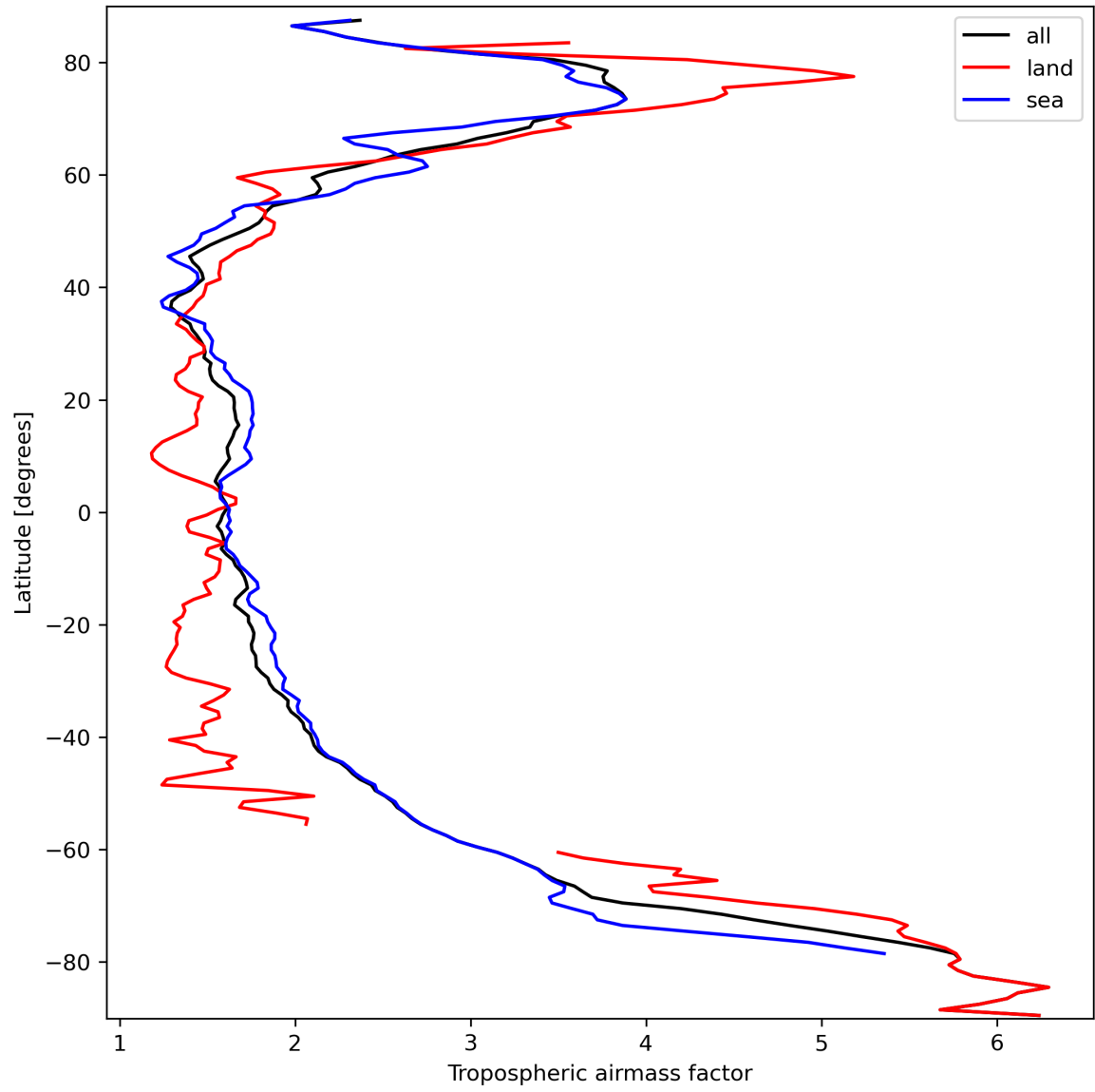
Figure 14: Zonal average of “Tropospheric airmass factor” for 2024-03-16 to 2024-03-18.
