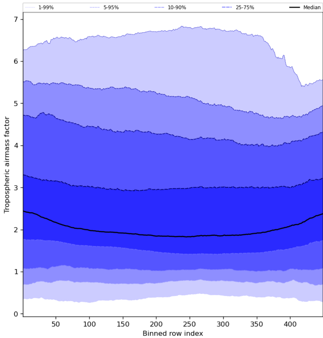
Figure 48: Along track statistics of “Tropospheric airmass factor” for 2024-03-16 to 2024-03-18
