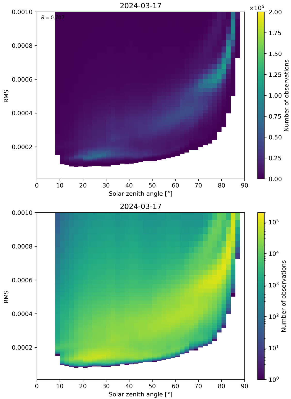
Figure 157: Scatter density plot of “Solar zenith angle” against “RMS” for 2024-03-16 to 2024-03-18.
