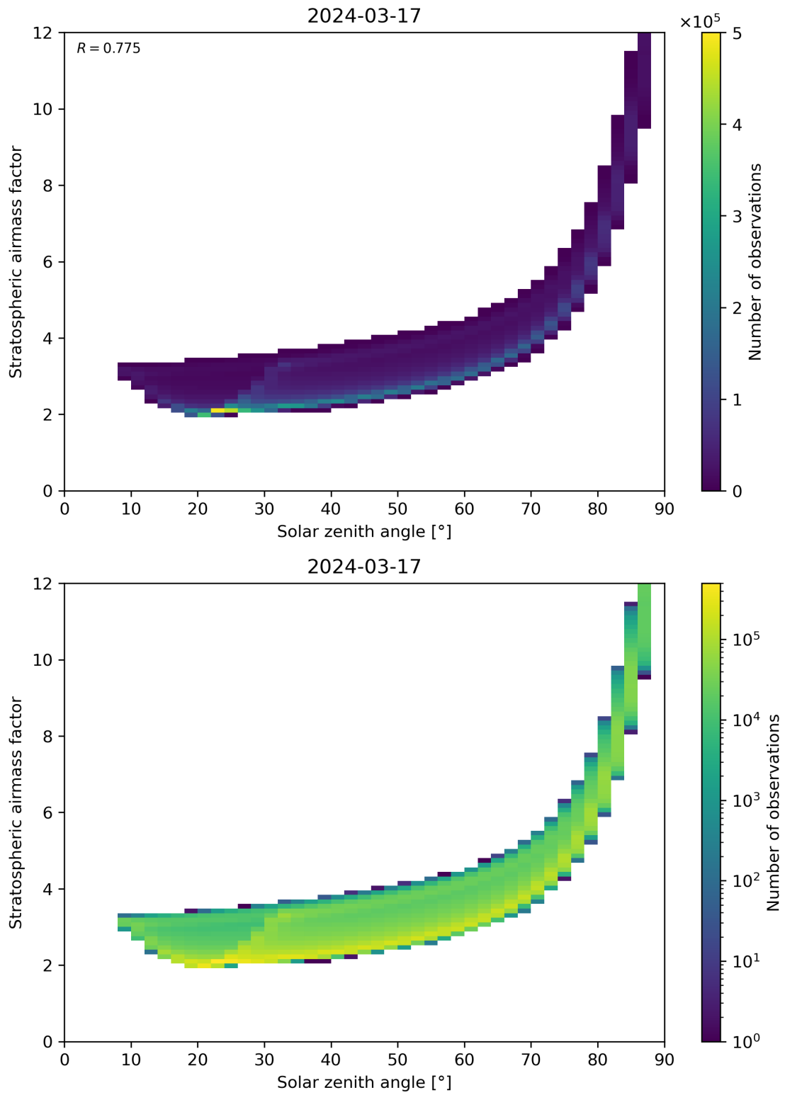
Figure 145: Scatter density plot of “Solar zenith angle” against “Stratospheric airmass factor” for 2024-03-16 to 2024-03-18.
