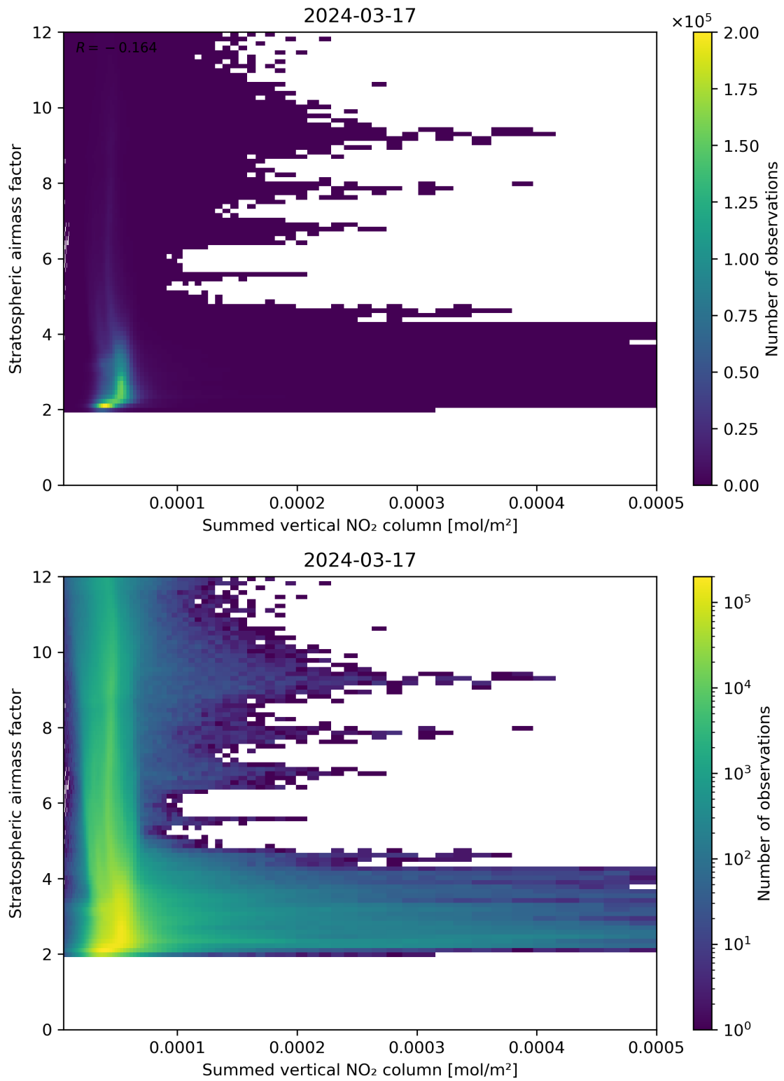
Figure 103: Scatter density plot of “Summed vertical NO 2 column” against “Stratospheric air mass factor” for 2024-03-16 to 2024-03-18.
