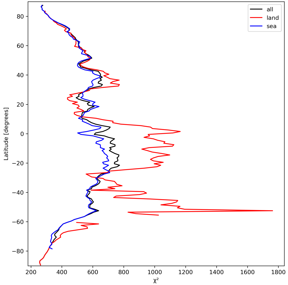
Figure 25: Zonal average of “ \chi^2 ” for 2024-03-16 to 2024-03-18.
