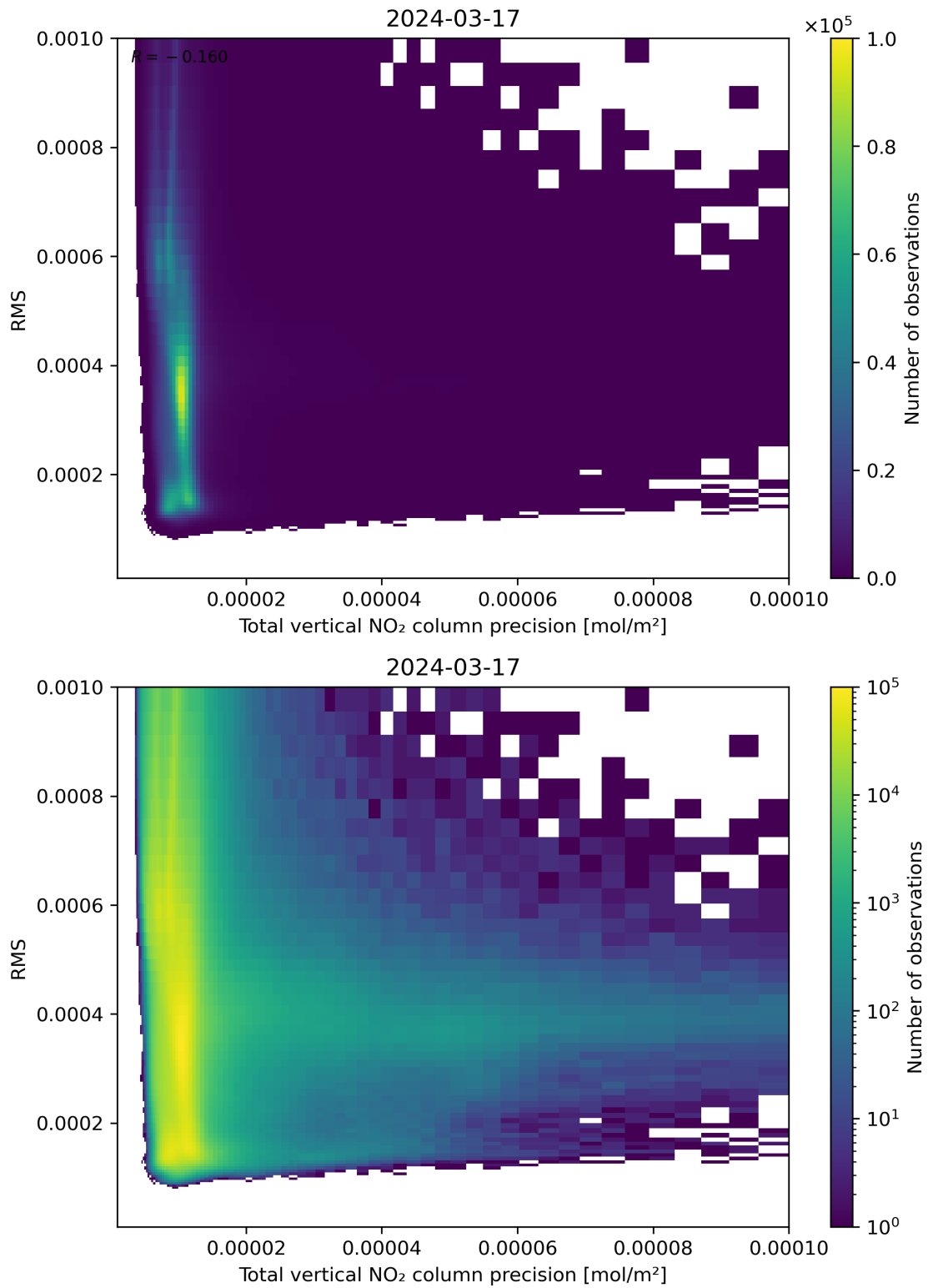
Figure 119: Scatter density plot of “Total vertical NO 2 column precision” against “RMS” for 2024-03-16 to 2024-03-18.
