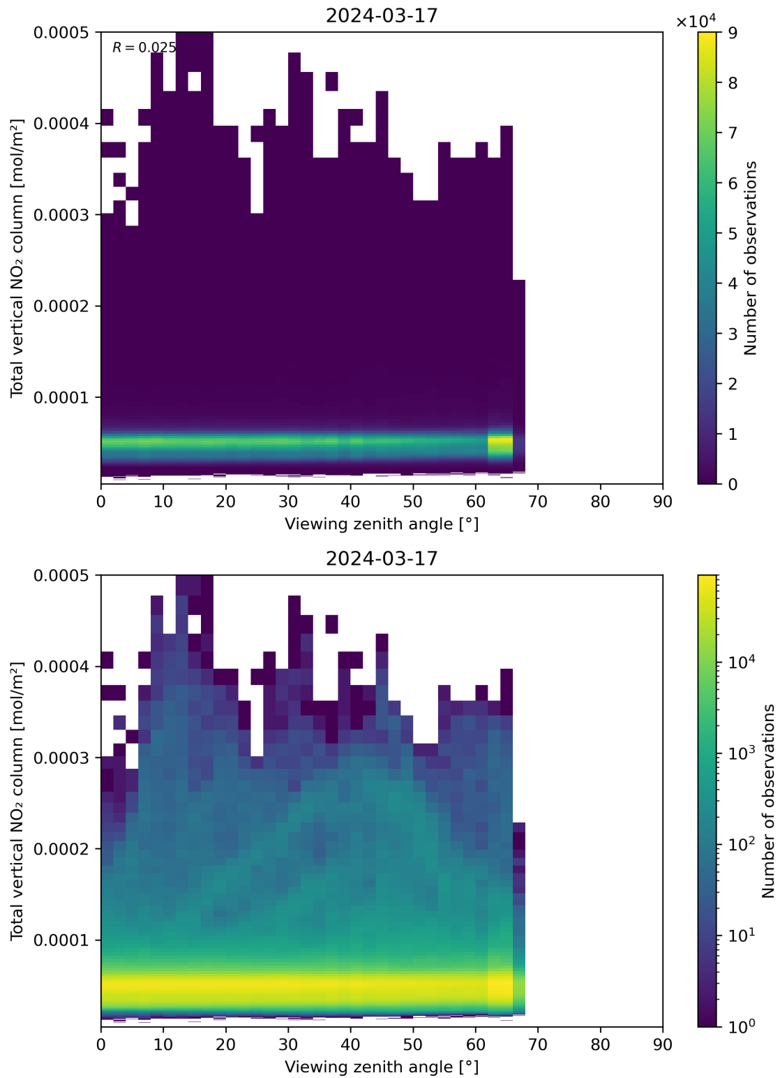
Figure 167: Scatter density plot of “Viewing zenith angle” against “Total vertical NO 2 column” for 2024-03-16 to 2024-03-18.
