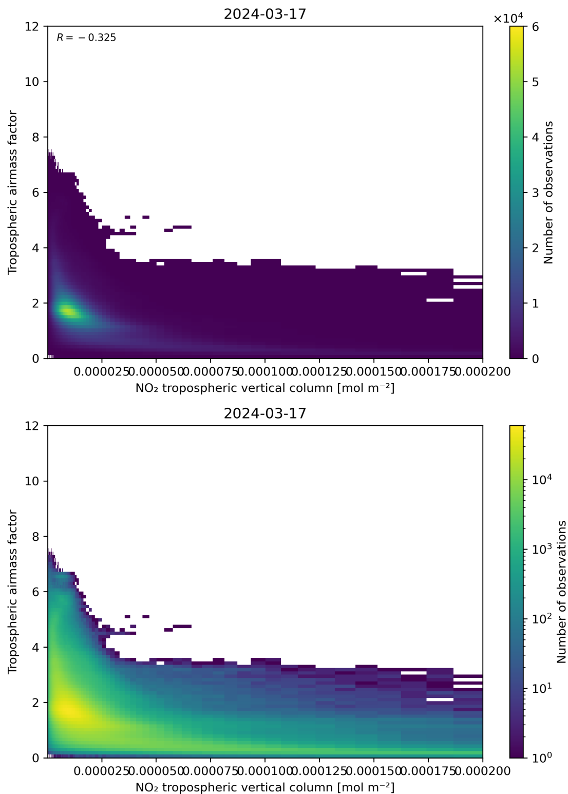
Figure 123: Scatter density plot of “NO 2 tropospheric vertical column” against “Tropospheric airmass factor” for 2024-03-16 to 2024-03-18.
