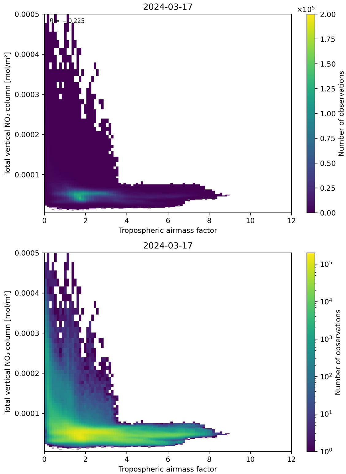
Figure 77: Scatter density plot of “Tropospheric airmass factor” against “Total vertical NO 2 column” for 2024-03-16 to 2024-03-18.
