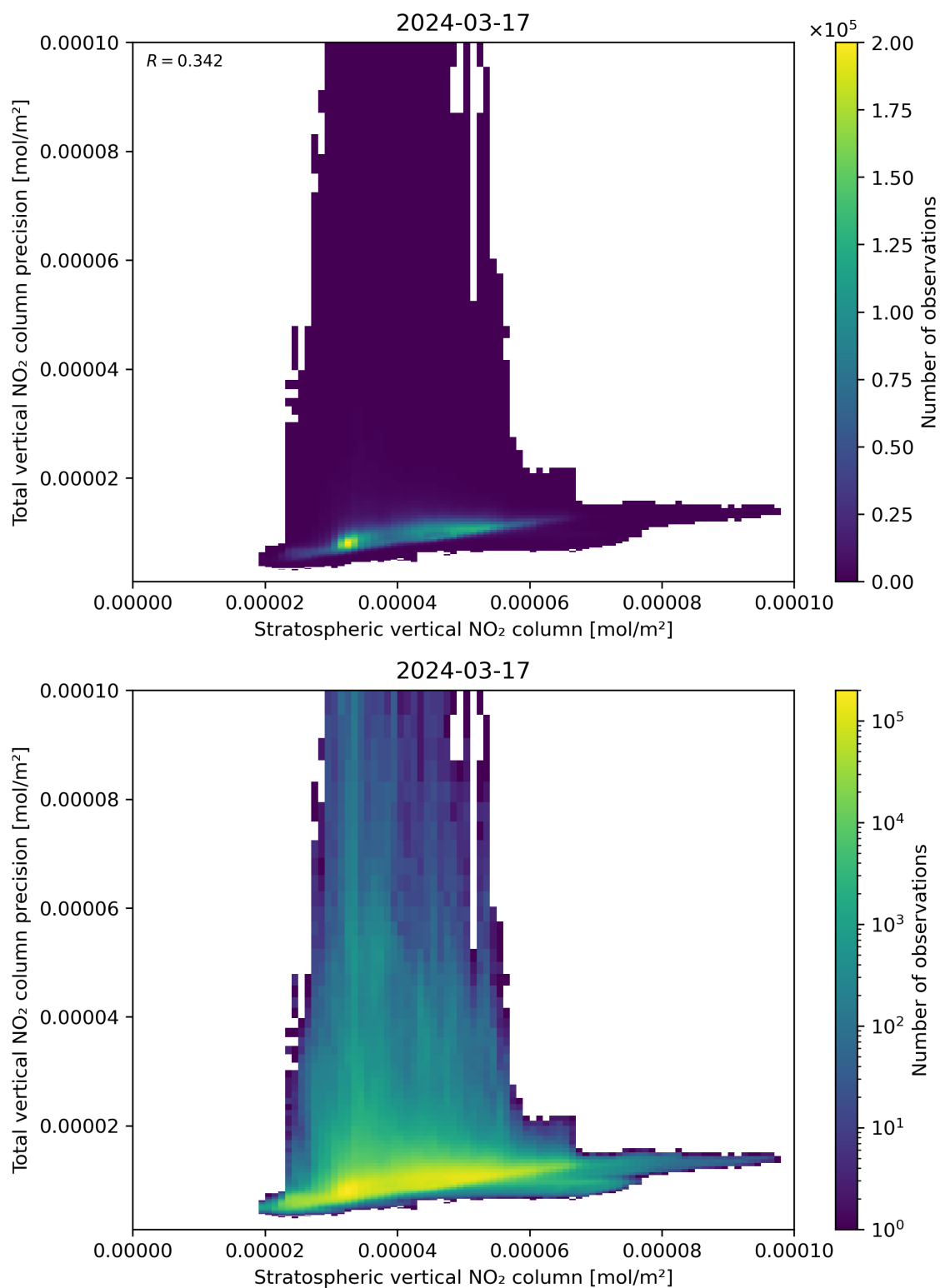
Figure 101: Scatter density plot of “Stratospheric vertical NO 2 column” against “Total vertical NO 2 column precision” for 2024-03-16 to 2024-03-18.
