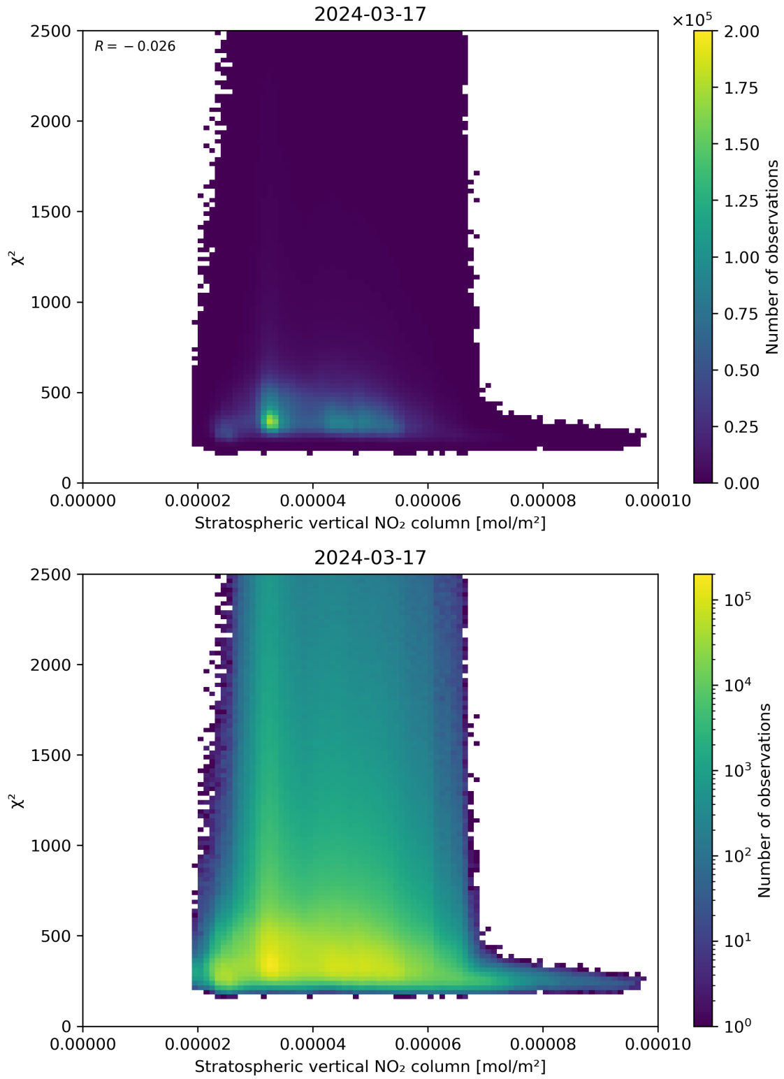
Figure 97: Scatter density plot of “Stratospheric vertical NO 2 column” against “ \chi^2 ” for 2024-03-16 to 2024-03-18.
