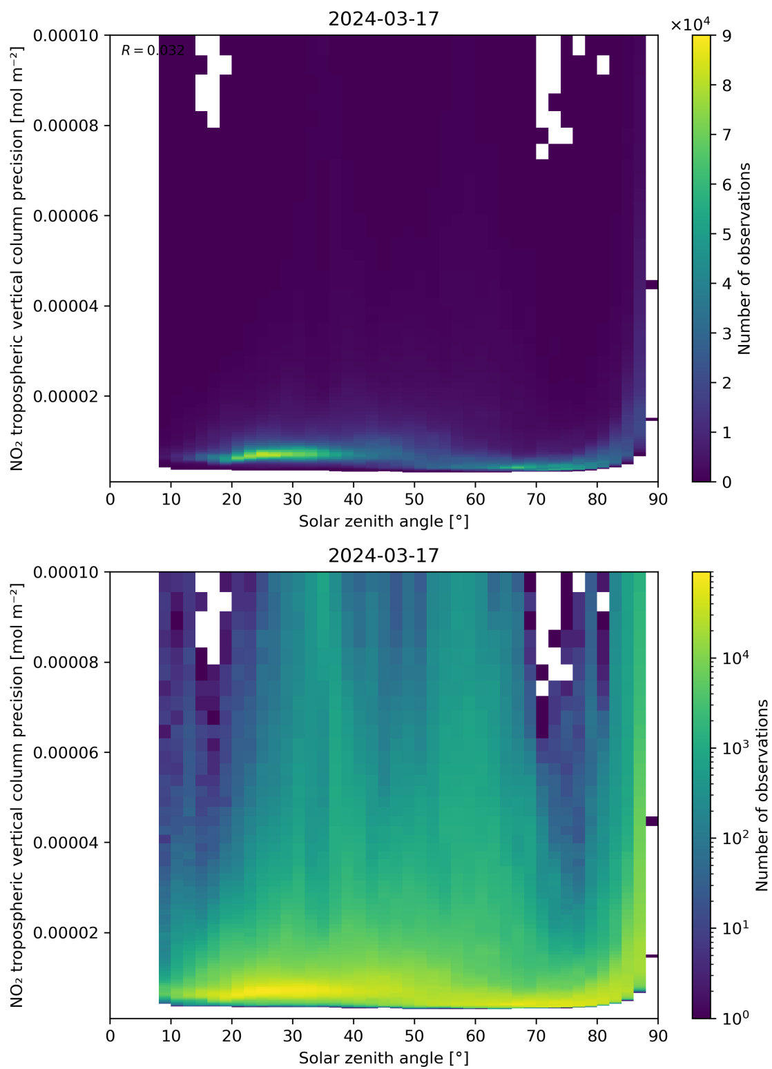
Figure 156: Scatter density plot of “Solar zenith angle” against “NO 2 tropospheric vertical column precision” for 2024-03-16 to 2024-03-18.
