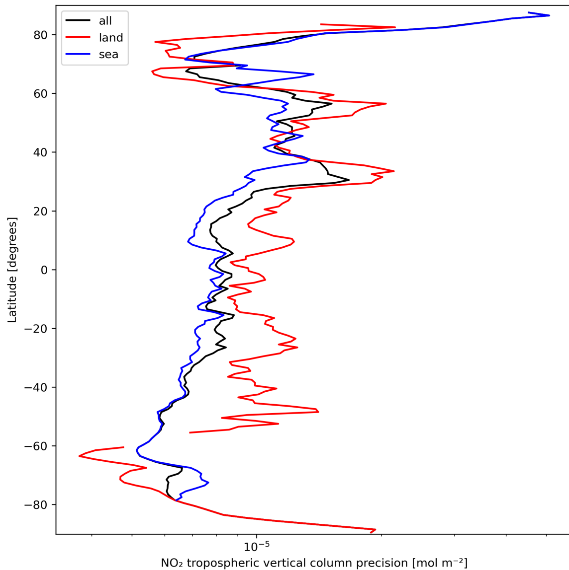
Figure 13: Zonal average of “NO 2 tropospheric vertical column precision” for 2024-03-16 to 2024-03-18.
