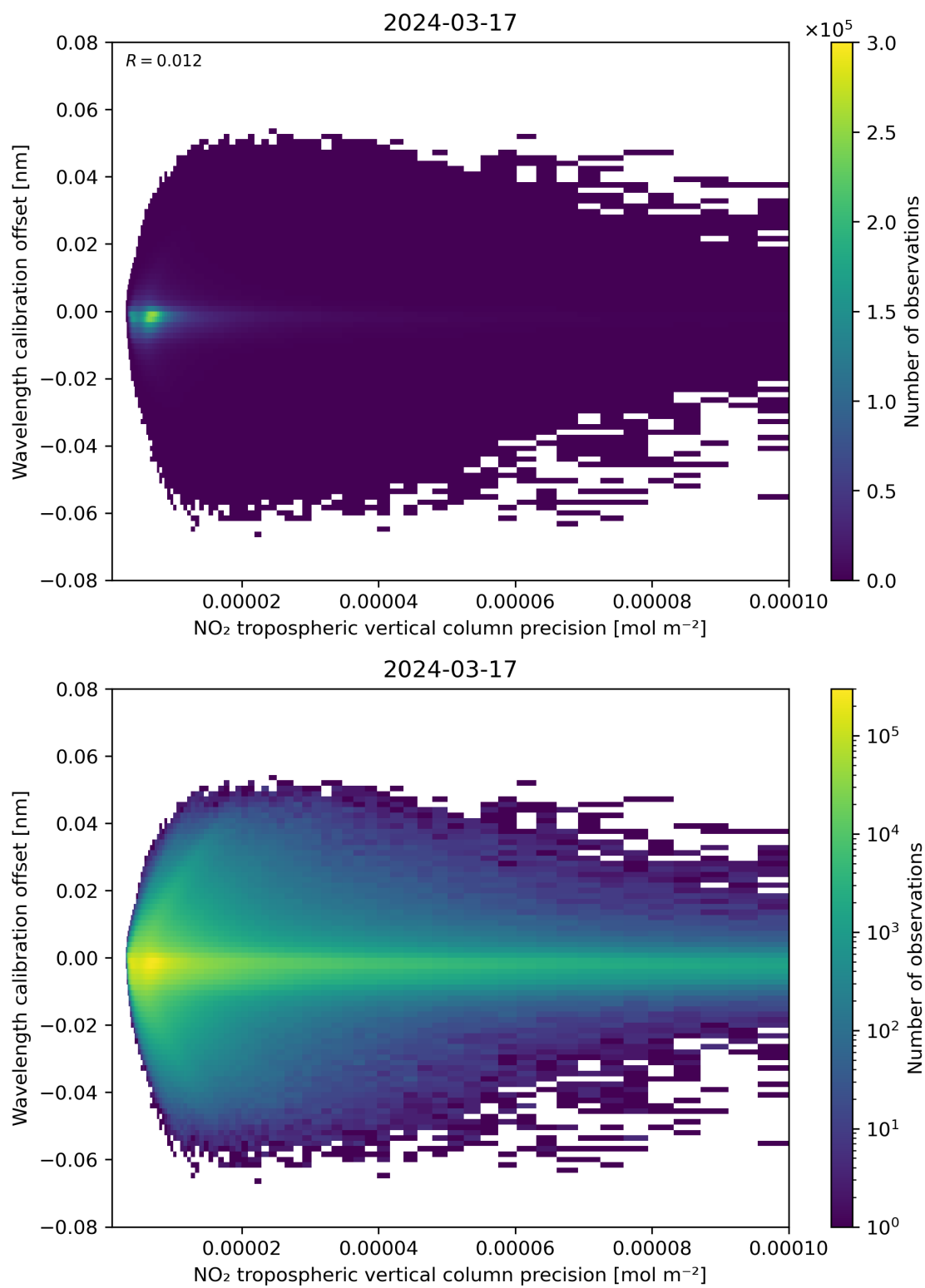
Figure 141: Scatter density plot of “NO 2 tropospheric vertical column precision” against “Wavelength calibration offset” for 2024-03-16 to 2024-03-18.
