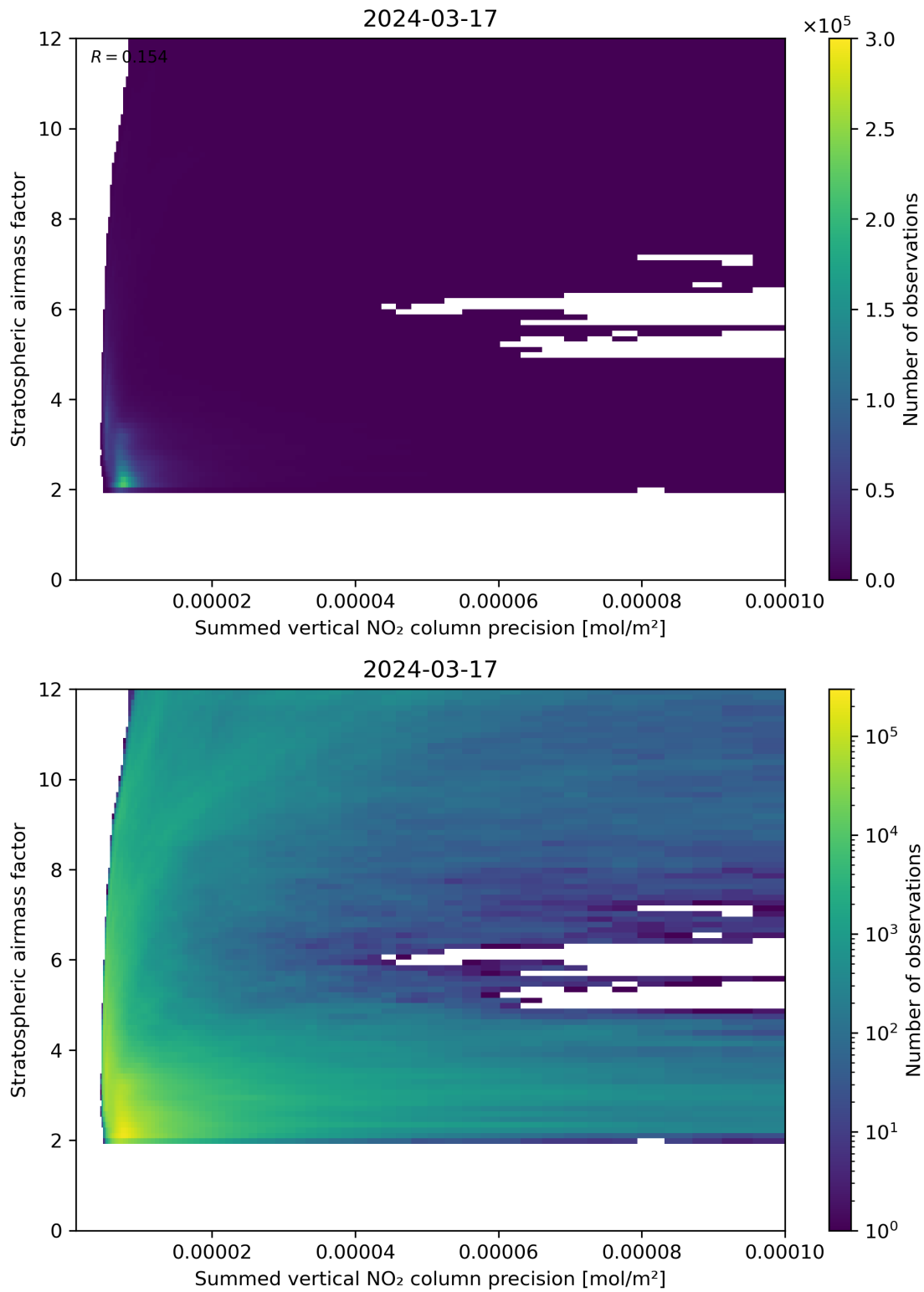
Figure 106: Scatter density plot of “Summed vertical NO 2 column precision” against “Stratospheric airmass factor” for 2024-03-16 to 2024-03-18.
