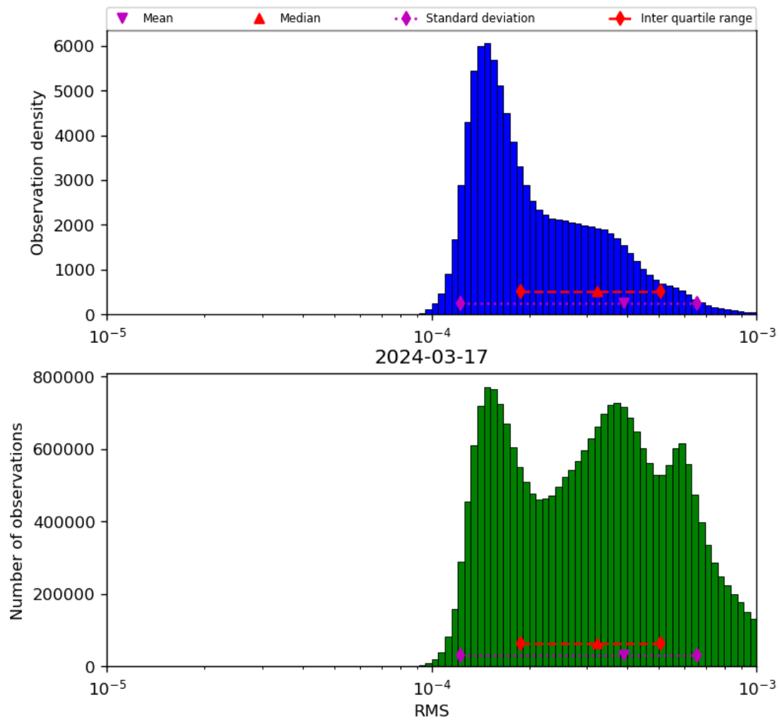
Figure 43: Histogram of “RMS” for 2024-03-16 to 2024-03-18
