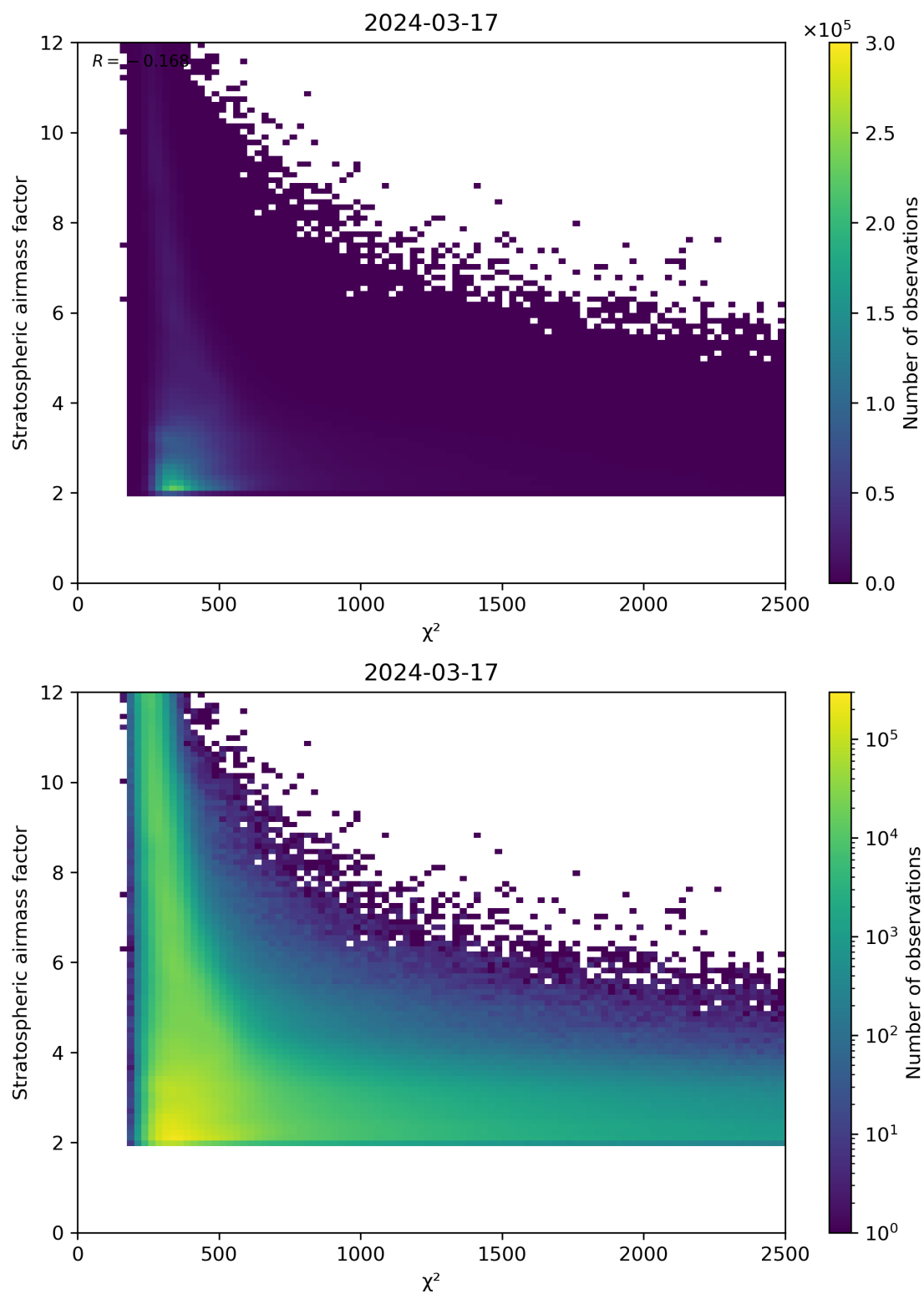
Figure 81: Scatter density plot of “ \chi^2 ” against “Stratospheric airmass factor” for 2024-03-16 to 2024-03-18.
