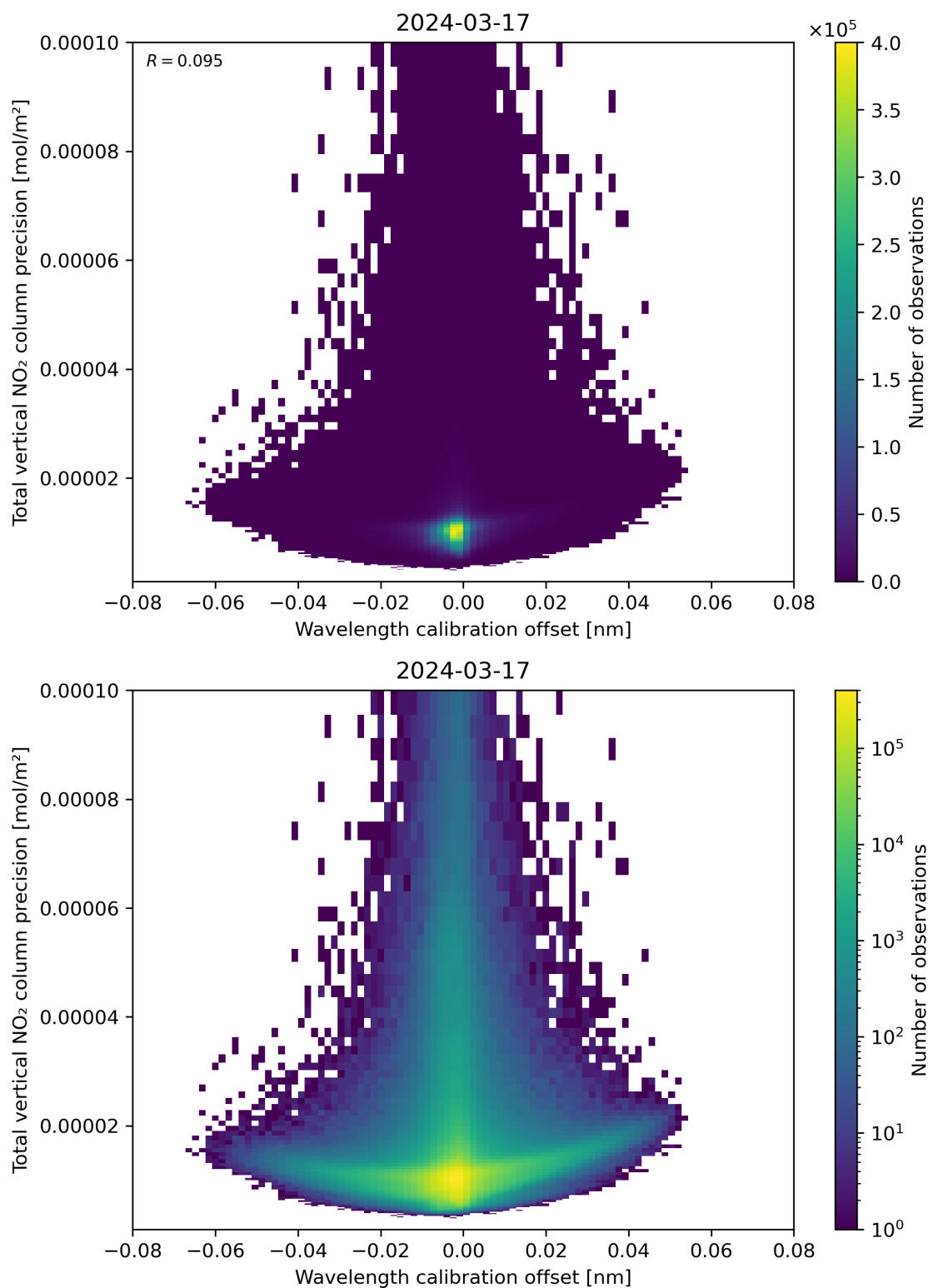
Figure 180: Scatter density plot of “Wavelength calibration offset” against “Total vertical NO 2 column precision” for 2024-03-16 to 2024-03-18.
