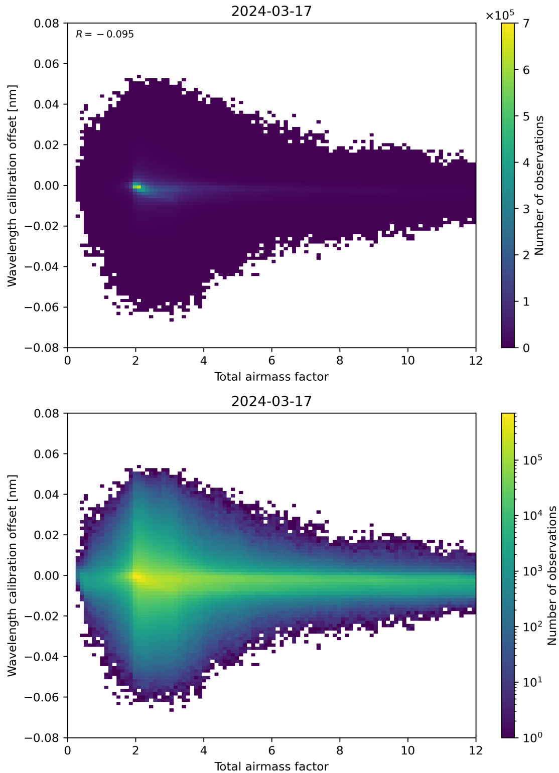
Figure 70: Scatter density plot of “Total airmass factor” against “Wavelength calibration offset” for 2024-03-16 to 2024-03-18.
