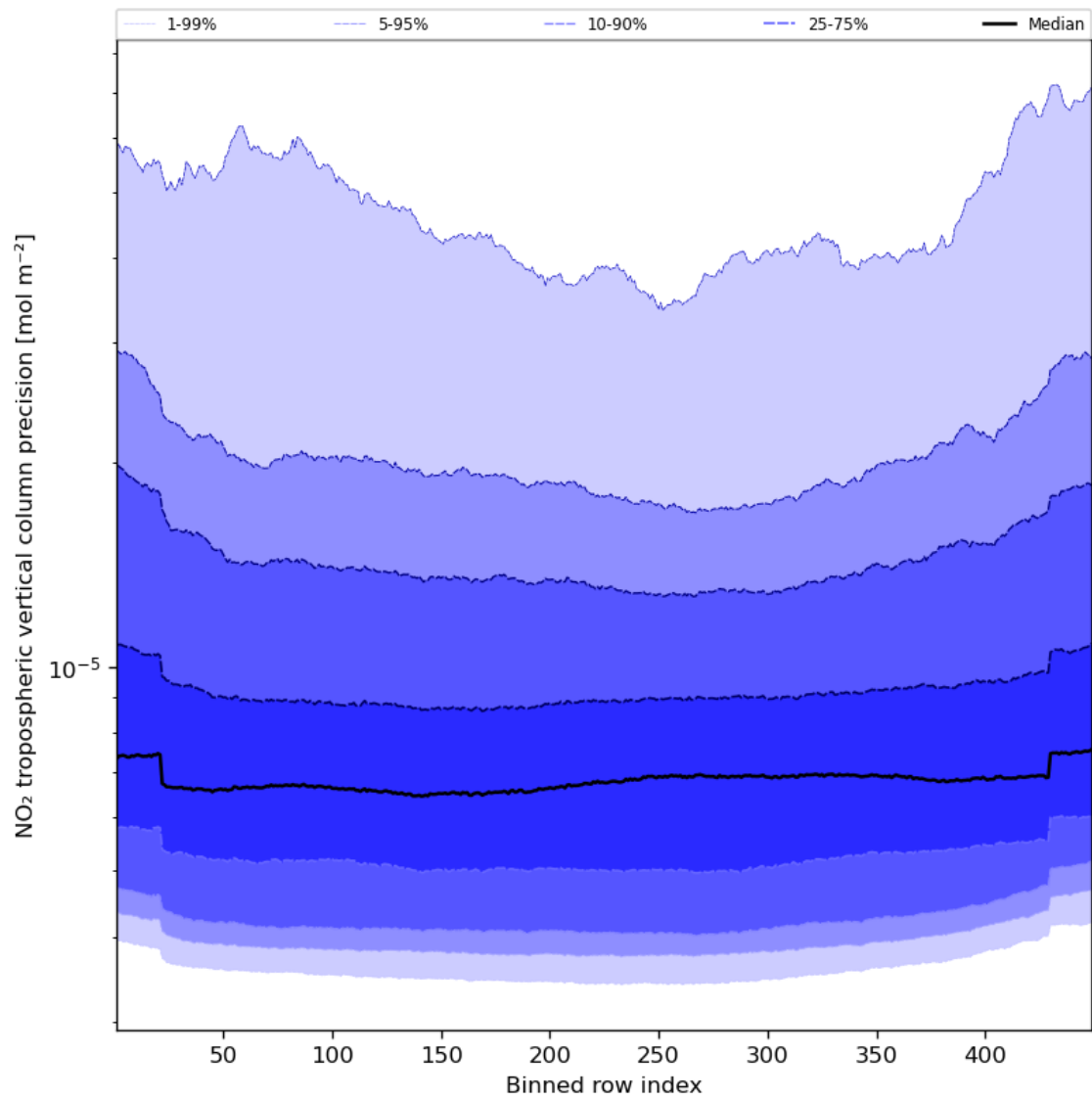
Figure 47: Along track statistics of “NO 2 tropospheric vertical column precision” for 2024-03-16 to 2024-03-18
