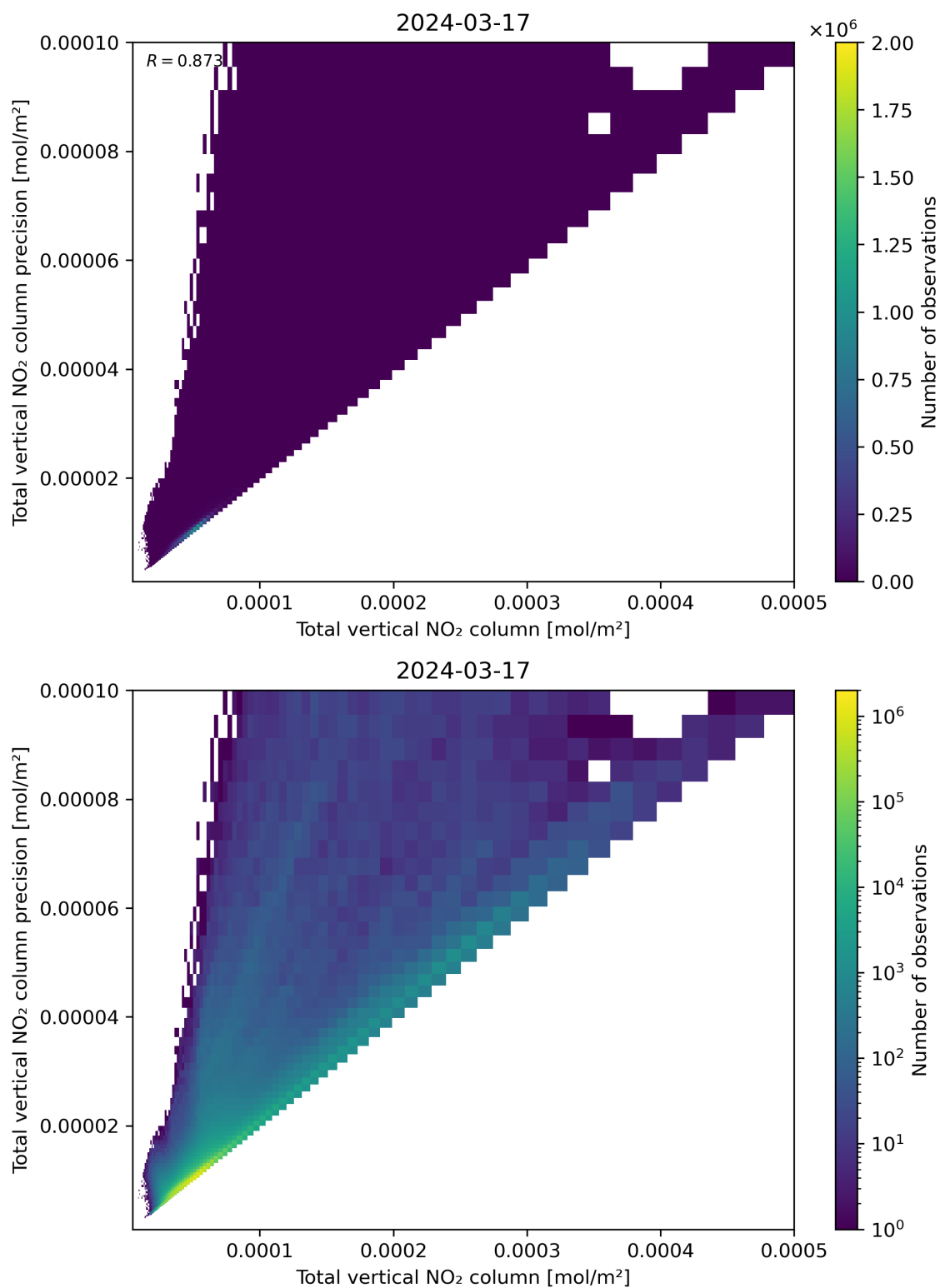
Figure 114: Scatter density plot of “Total vertical NO 2 column” against “Total vertical NO 2 column precision” for 2024-03-16 to 2024-03-18.
