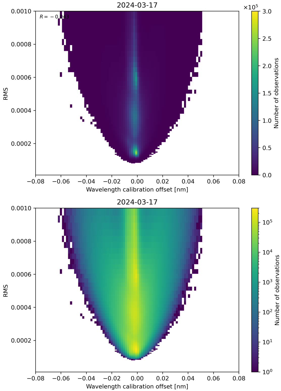
Figure 181: Scatter density plot of “Wavelength calibration offset” against “RMS” for 2024-03-16 to 2024-03-18.
