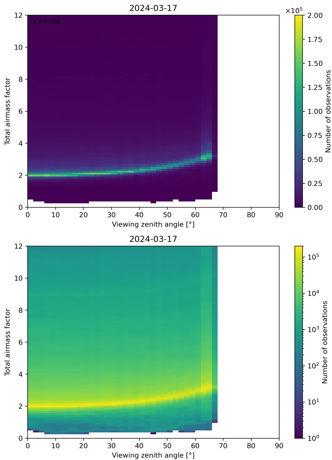
Figure 160: Scatter density plot of “Viewing zenith angle” against “Total airmass factor” for 2024-03-16 to 2024-03-18.
