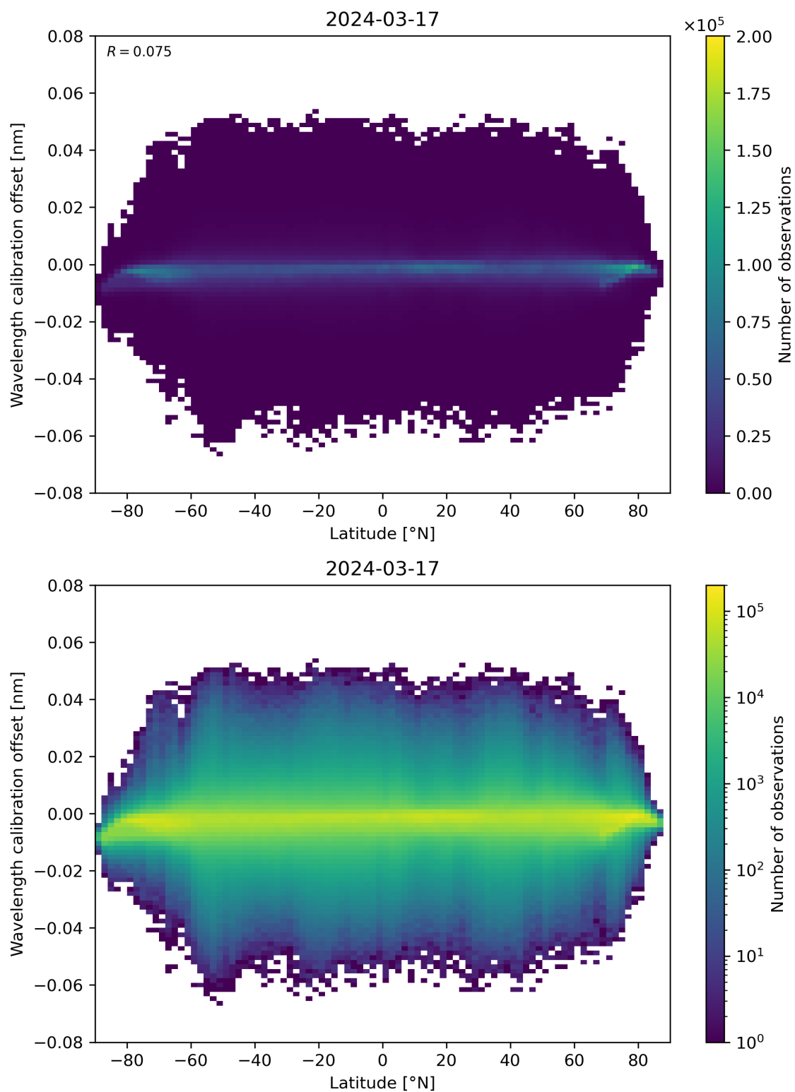
Figure 95: Scatter density plot of “Latitude” against “Wavelength calibration offset” for 2024-03-16 to 2024-03-18.
