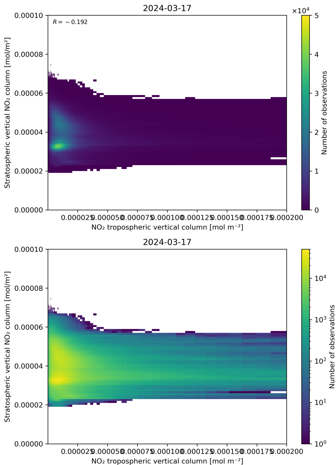
Figure 125: Scatter density plot of “NO 2 tropospheric vertical column” against “Stratospheric vertical NO 2 column” for 2024-03-16 to 2024-03-18.
