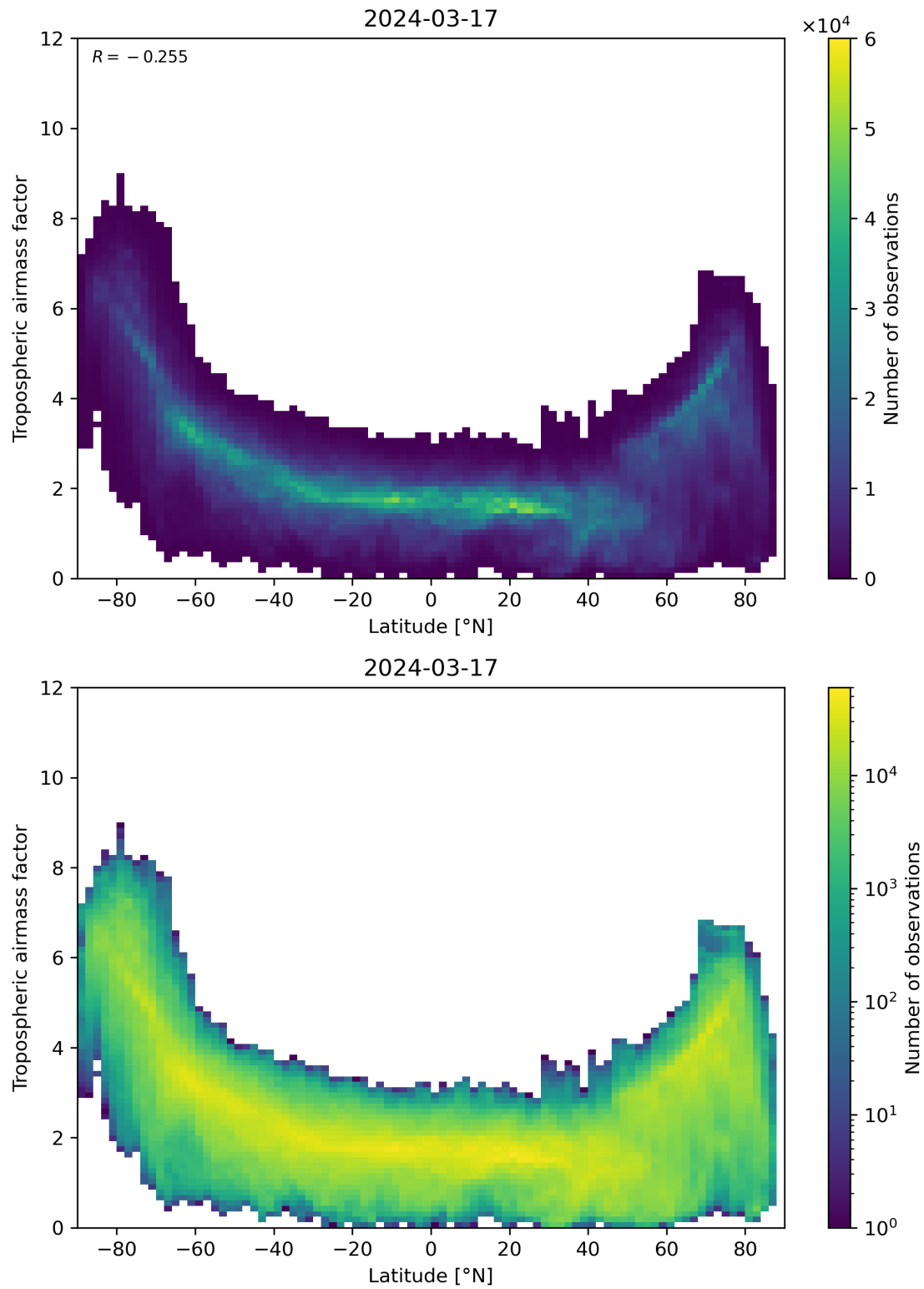
Figure 85: Scatter density plot of “Latitude” against “Tropospheric airmass factor” for 2024-03-16 to 2024-03-18.
