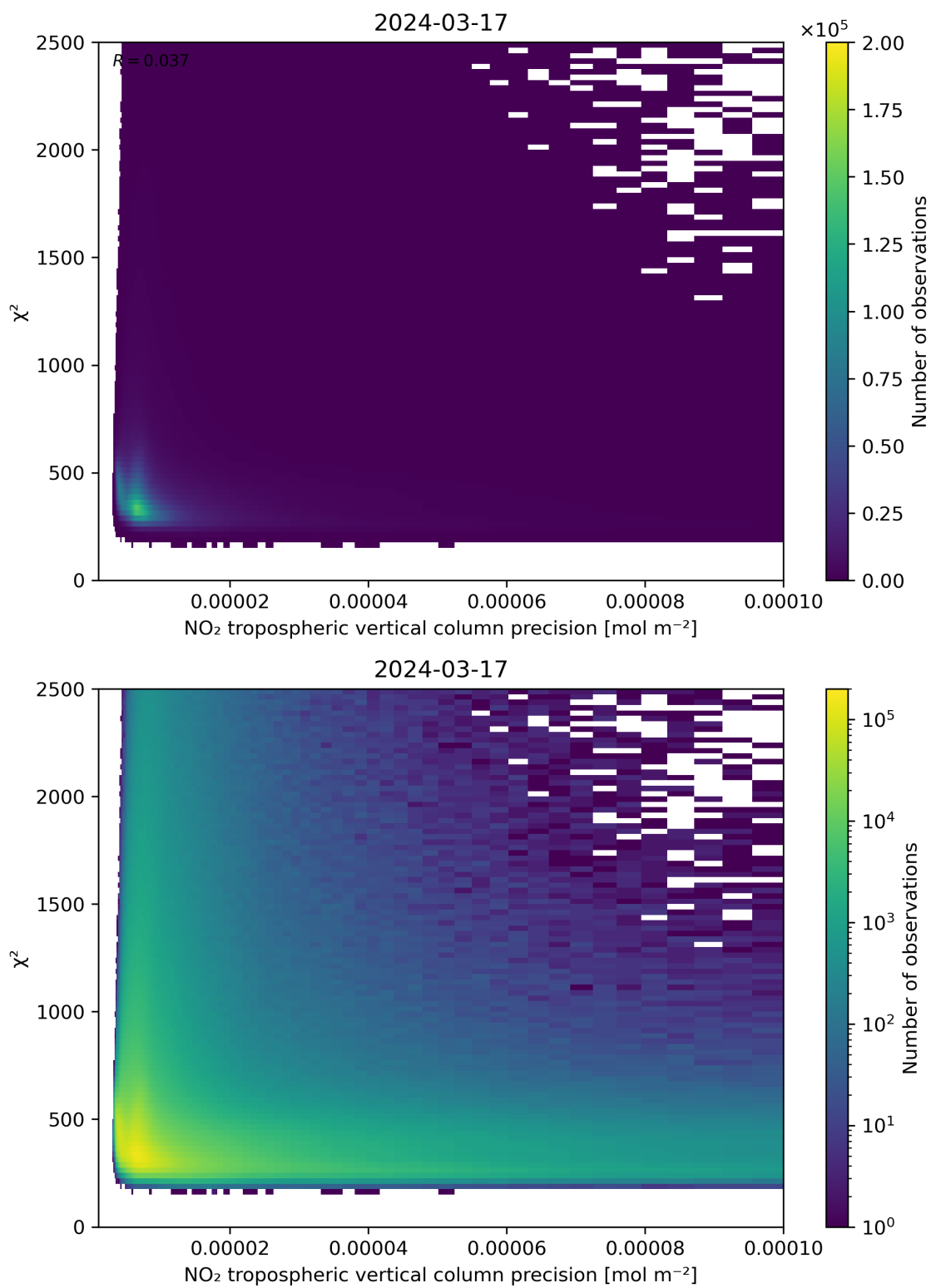
Figure 134: Scatter density plot of “NO 2 tropospheric vertical column precision” against “ \chi^2 ” for 2024-03-16 to 2024-03-18.
