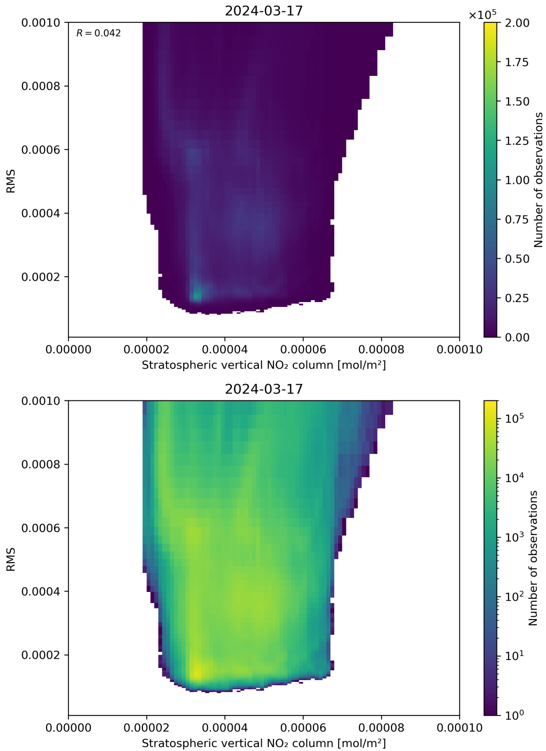
Figure 102: Scatter density plot of “Stratospheric vertical NO 2 column” against “RMS” for 2024-03-16 to 2024-03-18.
