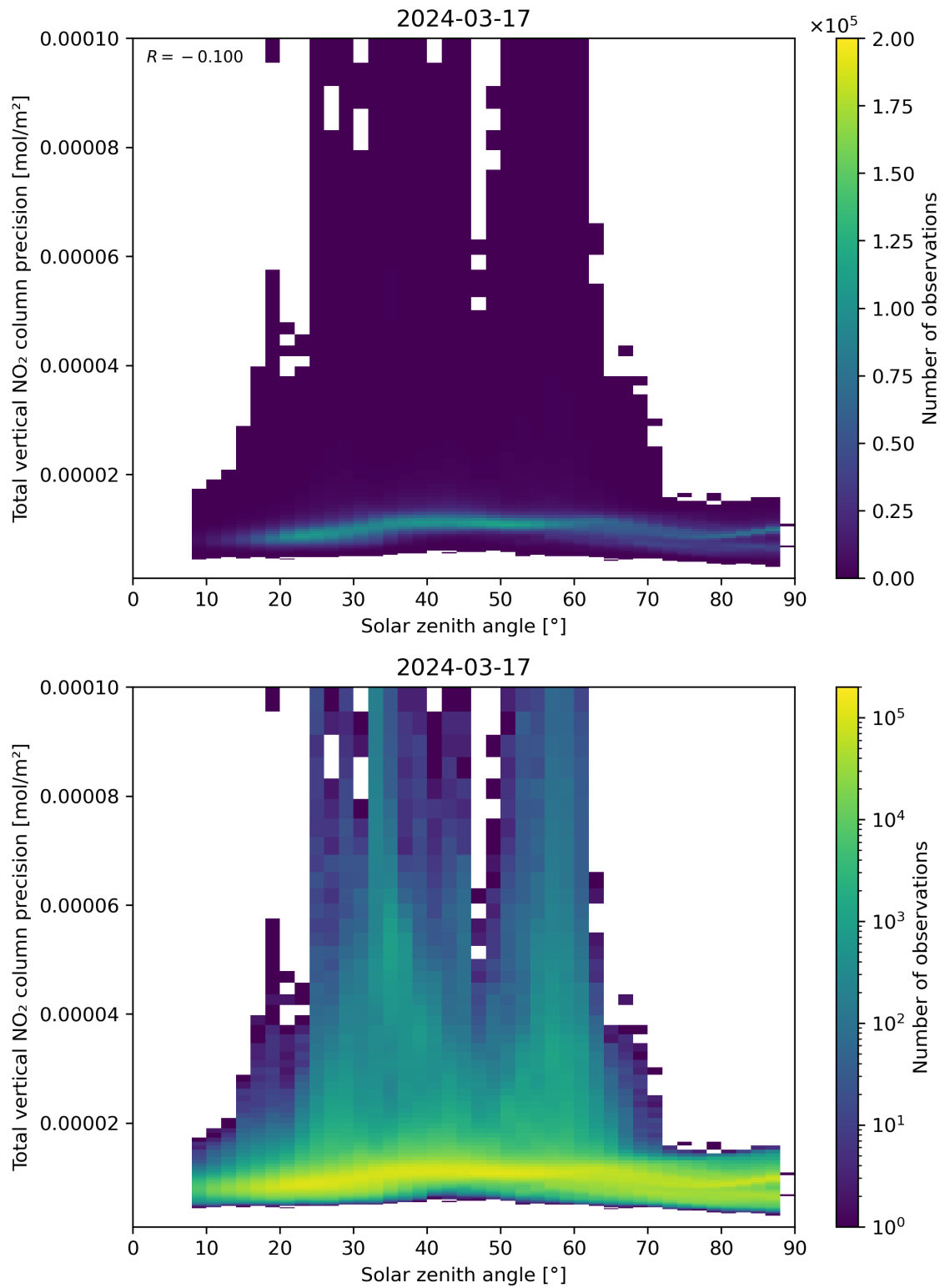
Figure 154: Scatter density plot of “Solar zenith angle” against “Total vertical NO 2 column precision” for 2024-03-16 to 2024-03-18.
