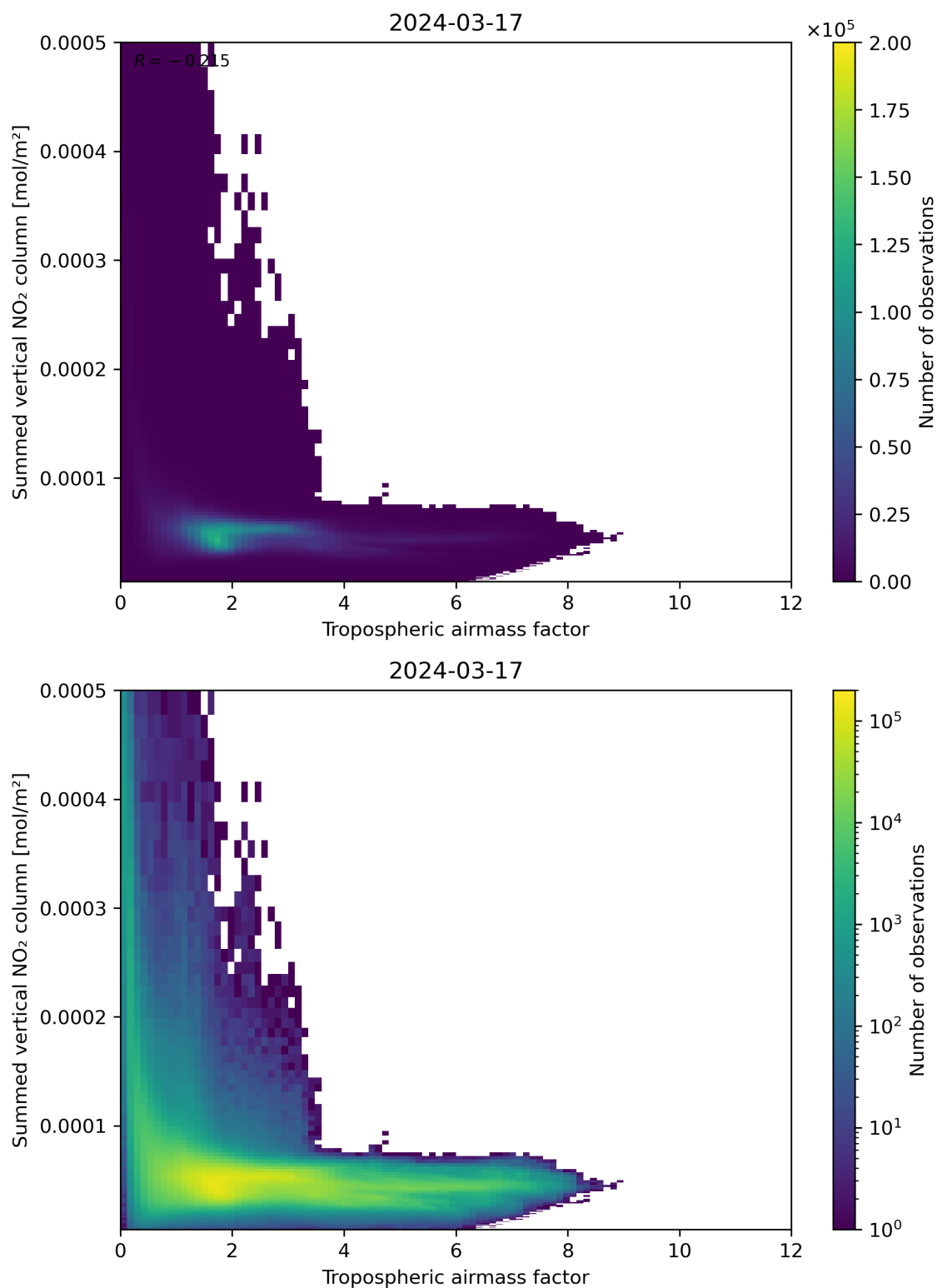
Figure 75: Scatter density plot of “Tropospheric airmass factor” against “Summed vertical NO 2 column” for 2024-03-16 to 2024-03-18.
