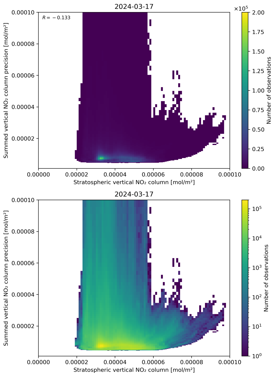
Figure 99: Scatter density plot of “Stratospheric vertical NO 2 column” against “Summed vertical NO 2 column precision” for 2024-03-16 to 2024-03-18.
