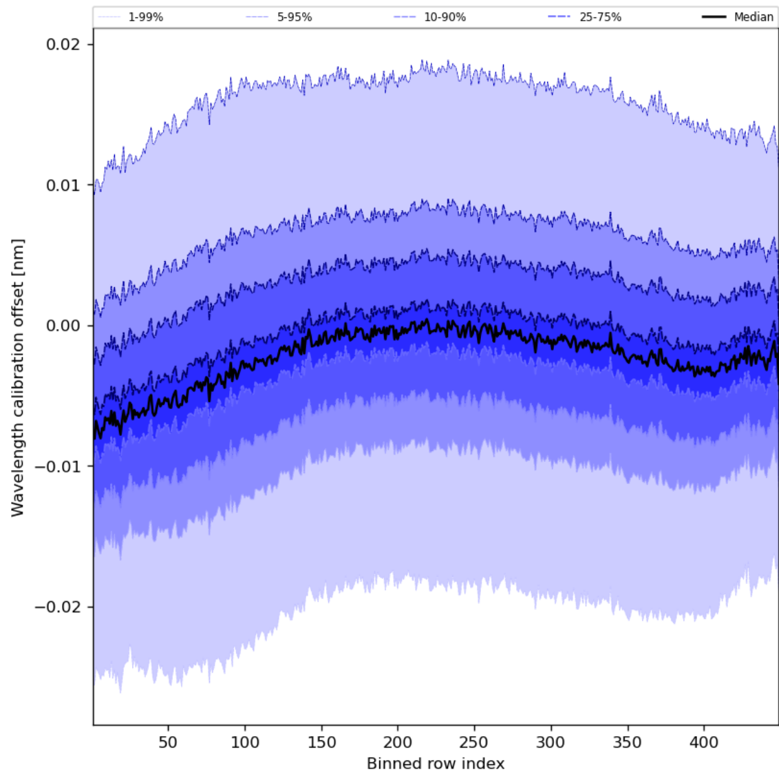
Figure 52: Along track statistics of “Wavelength calibration offset” for 2024-03-16 to 2024-03-18
