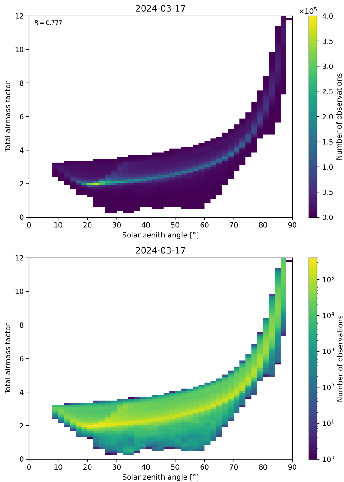
Figure 146: Scatter density plot of “Solar zenith angle” against “Total air mass factor” for 2024-03-16 to 2024-03-18.
