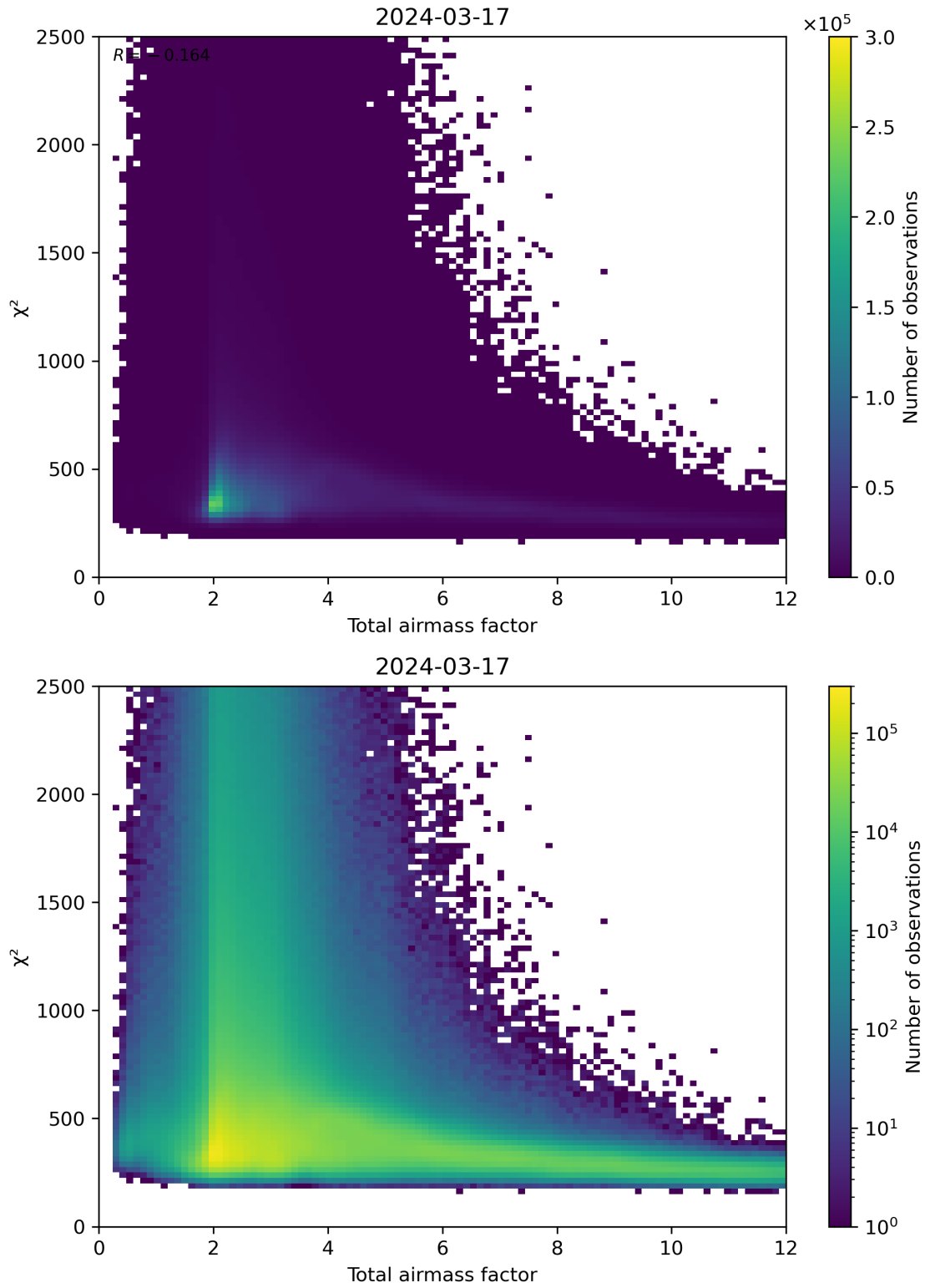
Figure 63: Scatter density plot of “Total airmass factor” against “ \chi^2 ” for 2024-03-16 to 2024-03-18.
