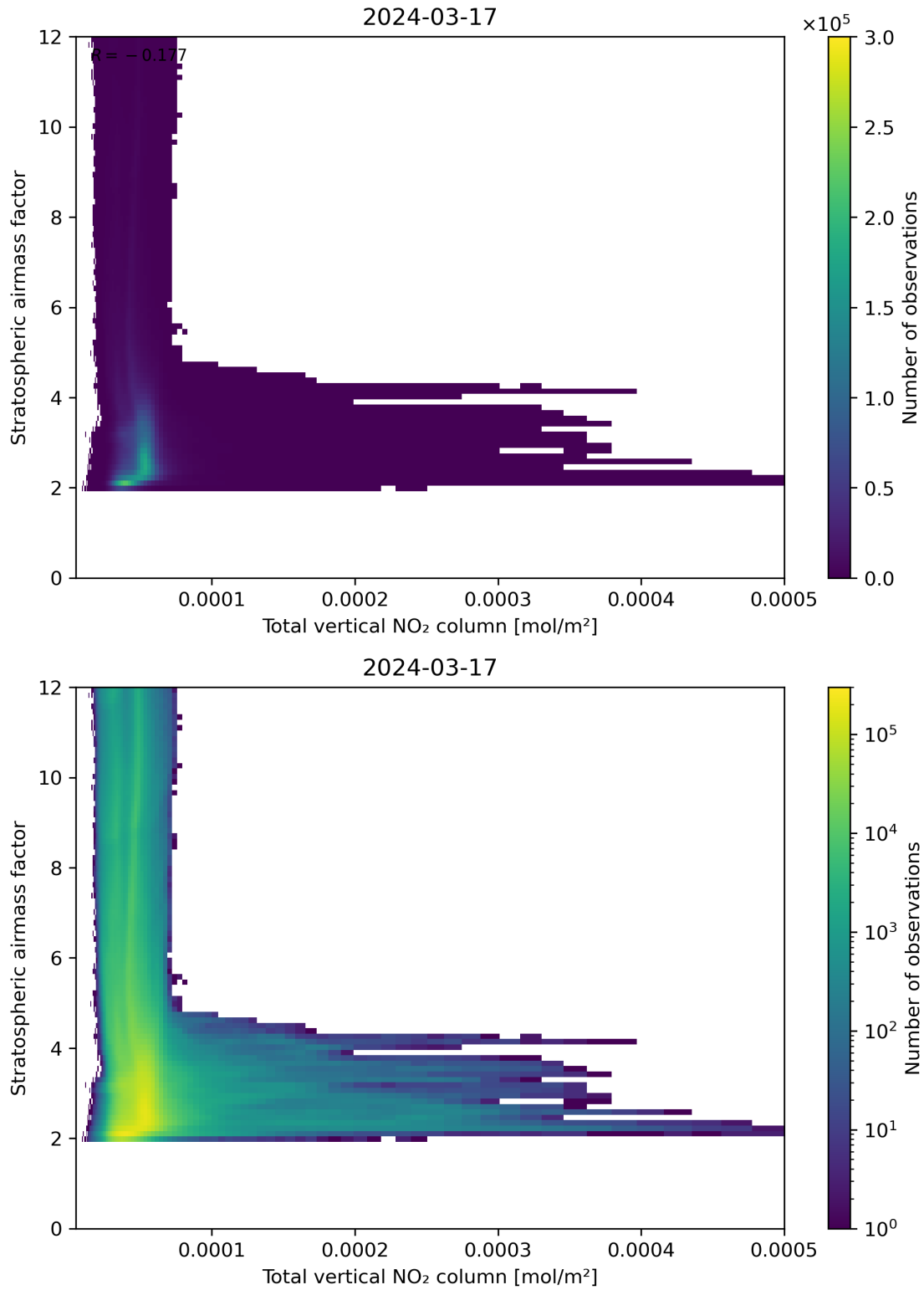
Figure 110: Scatter density plot of “Total vertical NO 2 column” against “Stratospheric airmass factor” for 2024-03-16 to 2024-03-18.
