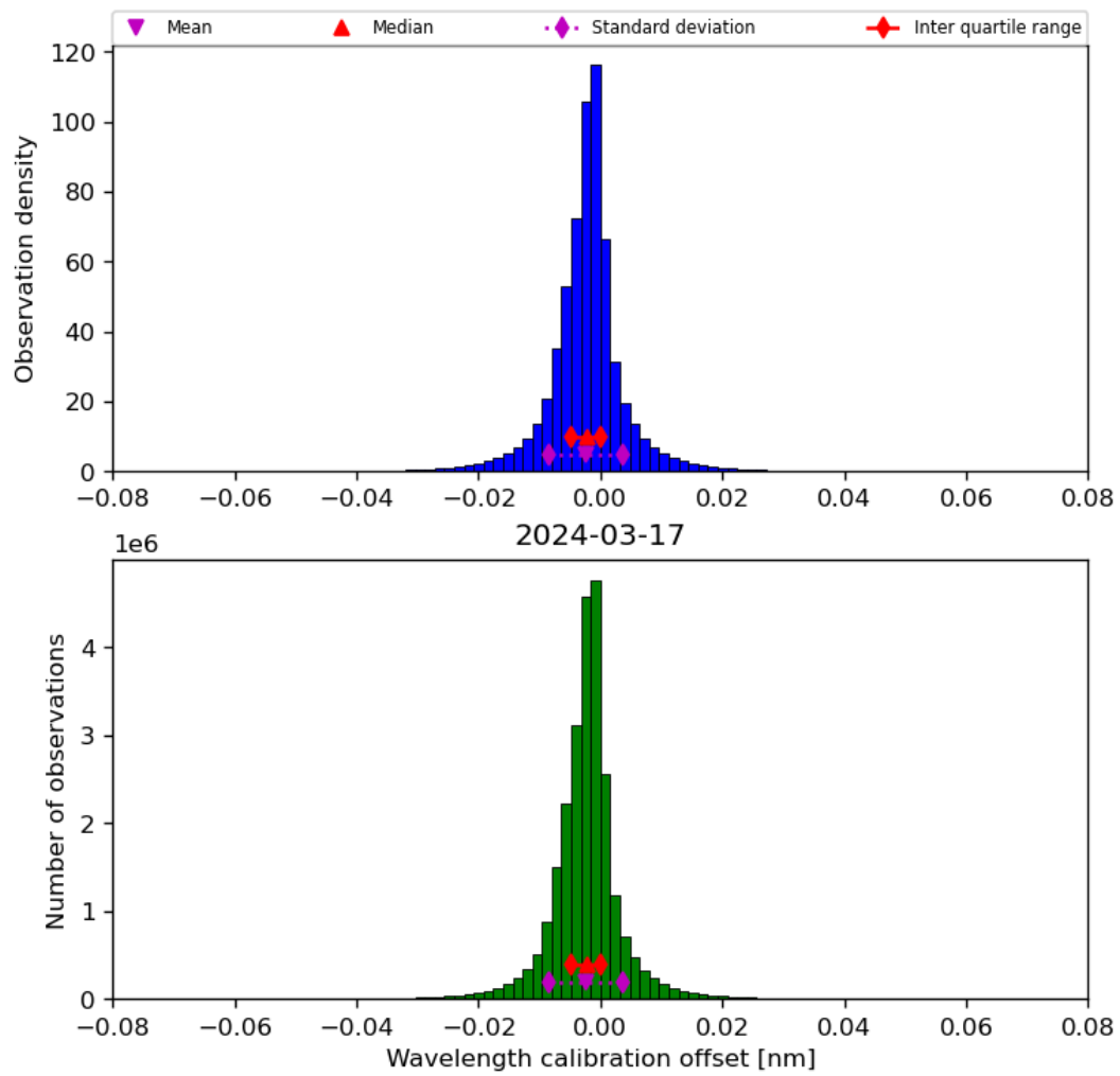
Figure 35: Histogram of “Wavelength calibration offset” for 2024-03-16 to 2024-03-18
