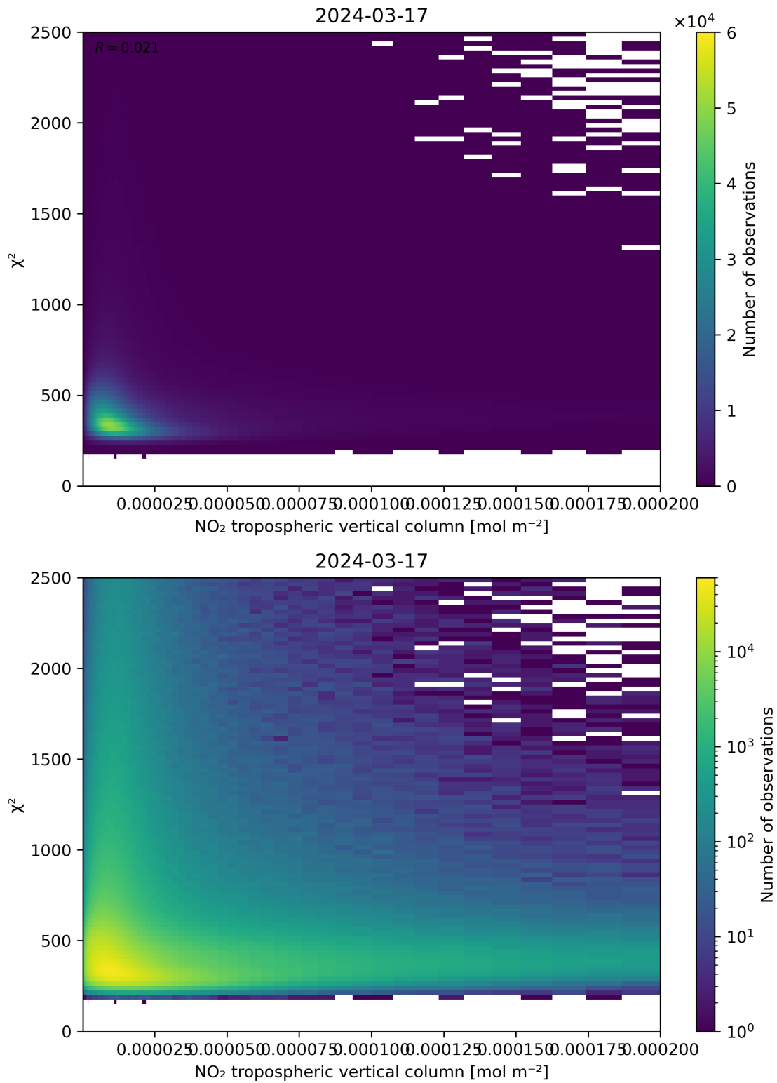
Figure 124: Scatter density plot of “NO 2 tropospheric vertical column” against “ \chi^2 ” for 2024-03-16 to 2024-03-18.
