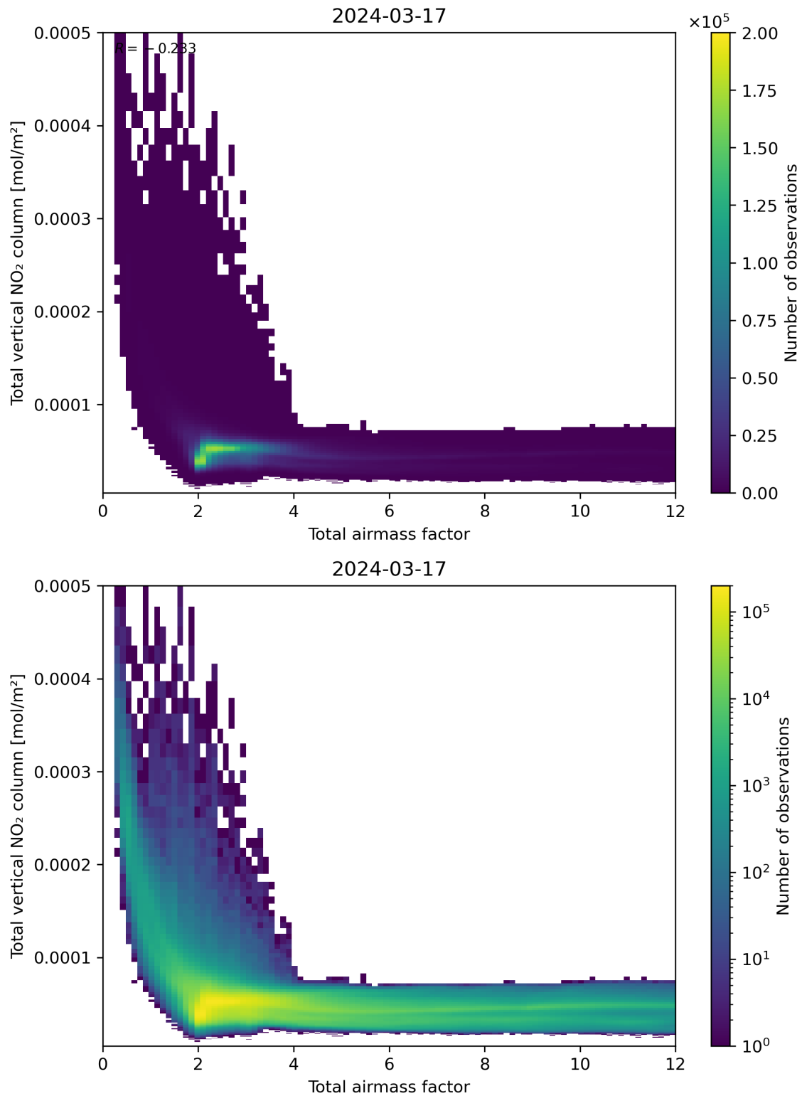
Figure 67: Scatter density plot of “Total airmass factor” against “Total vertical NO 2 column” for 2024-03-16 to 2024-03-18.
