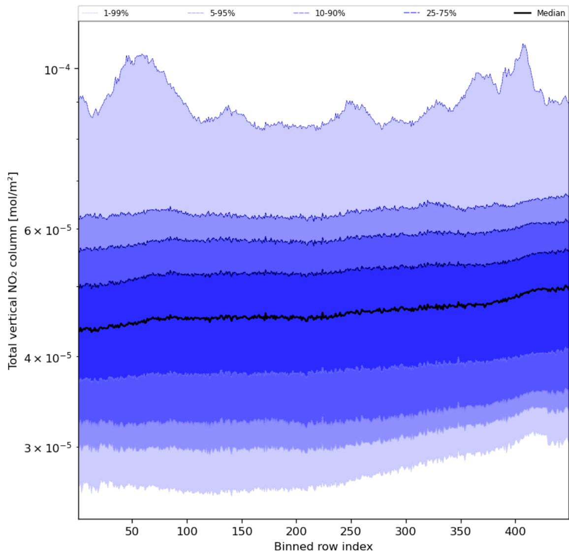
Figure 55: Along track statistics of “Total vertical NO 2 column” for 2024-03-18 to 2024-03-20
