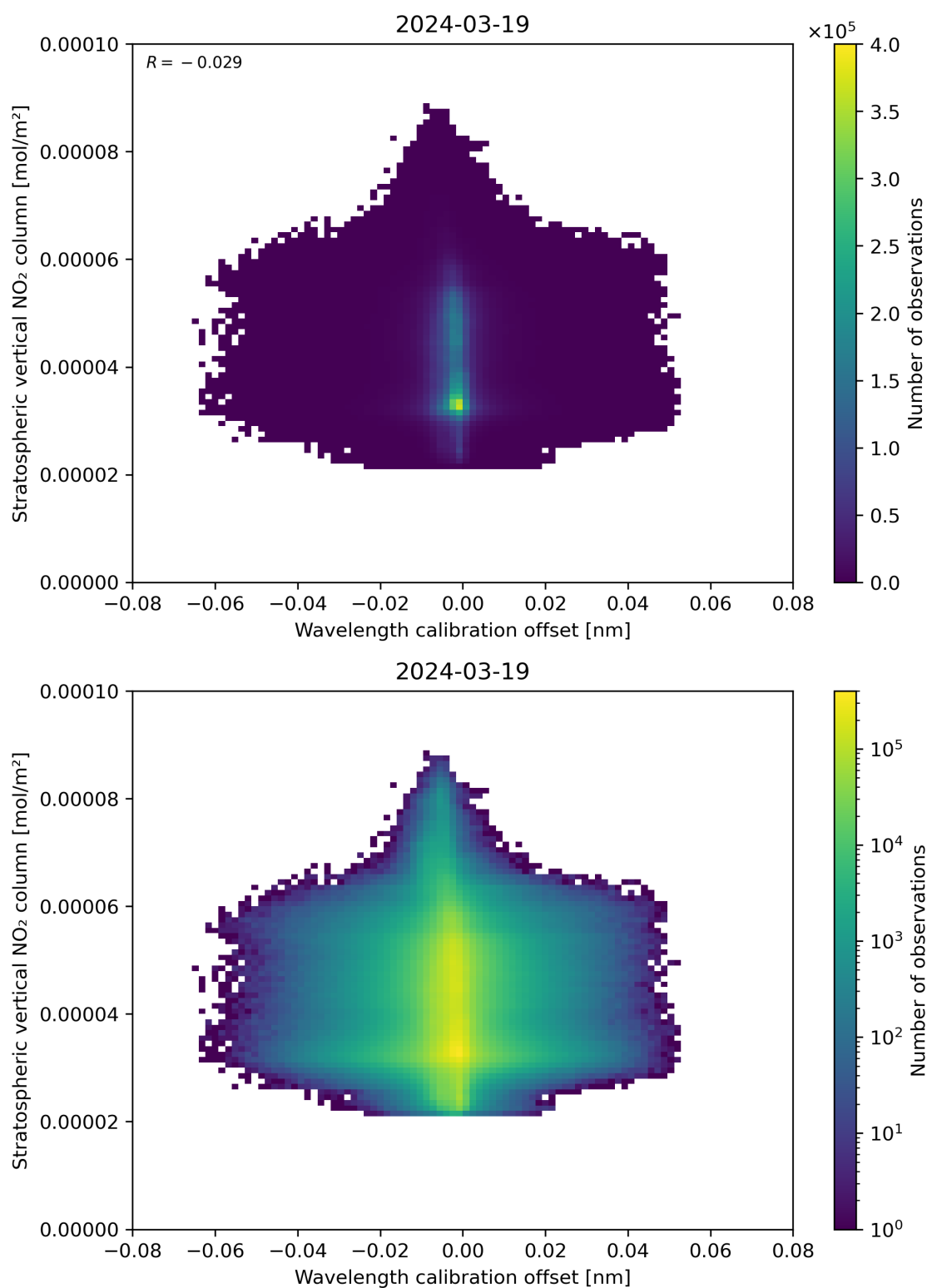
Figure 176: Scatter density plot of “Wavelength calibration offset” against “Stratospheric vertical NO 2 column” for 2024-03-18 to 2024-03-20.
