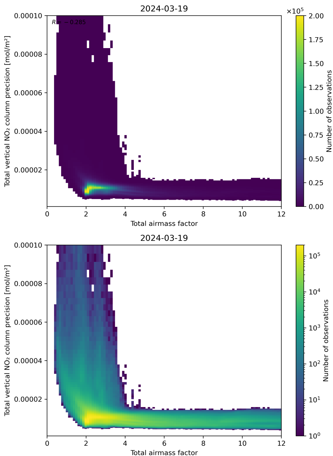
Figure 68: Scatter density plot of “Total airmass factor” against “Total vertical NO 2 column precision” for 2024-03-18 to 2024-03-20.
