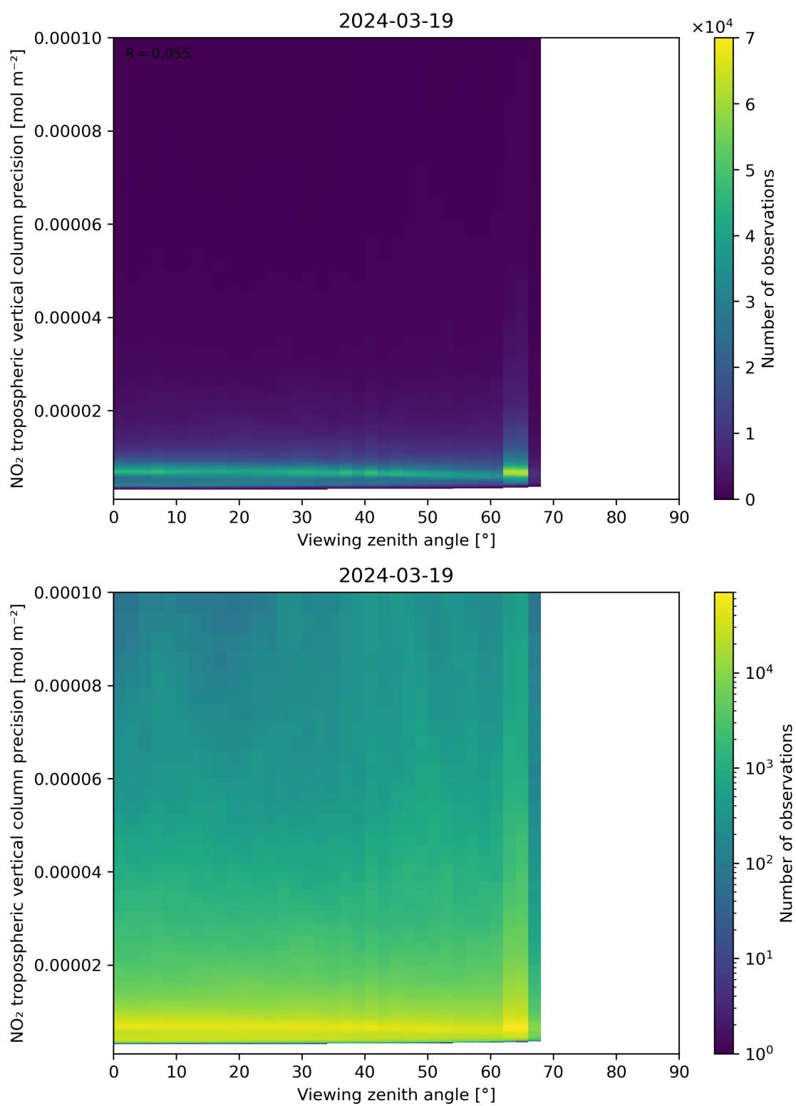
Figure 170: Scatter density plot of “Viewing zenith angle” against “NO 2 tropospheric vertical column precision” for 2024-03-18 to 2024-03-20.
