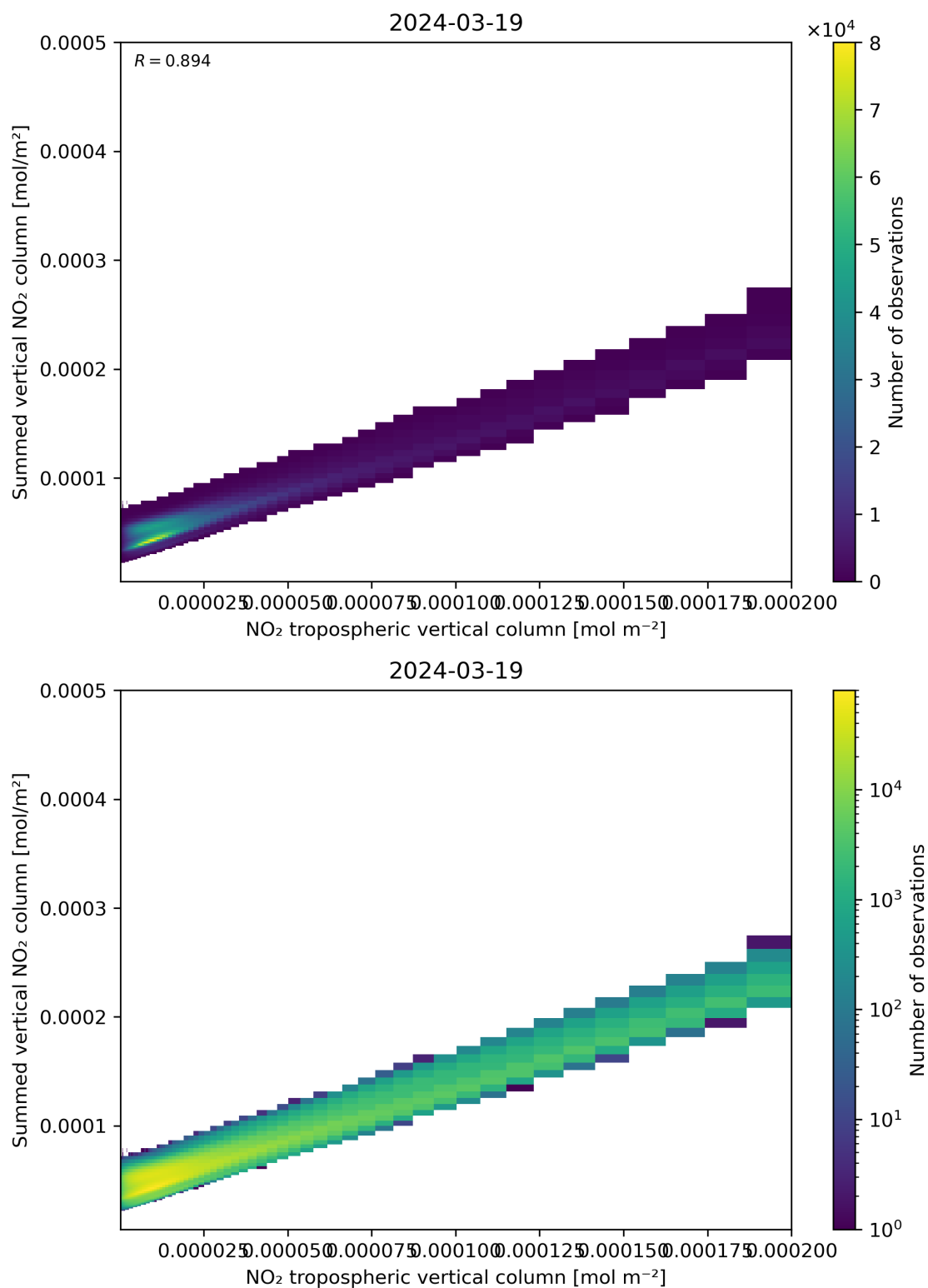
Figure 126: Scatter density plot of “NO 2 tropospheric vertical column” against “Summed vertical NO 2 column” for 2024-03-18 to 2024-03-20.
