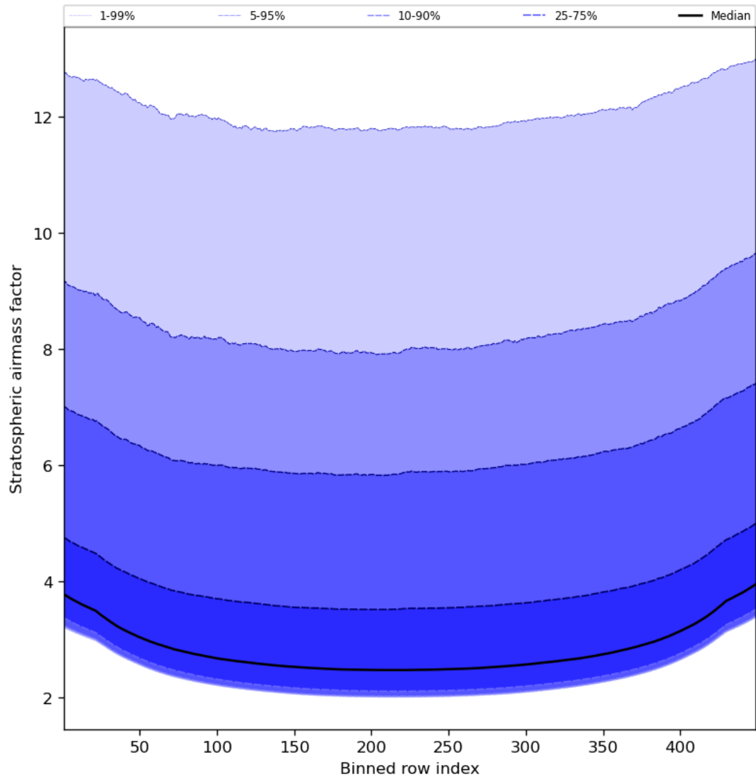
Figure 61: Along track statistics of “Stratospheric airmass factor” for 2024-03-18 to 2024-03-20
