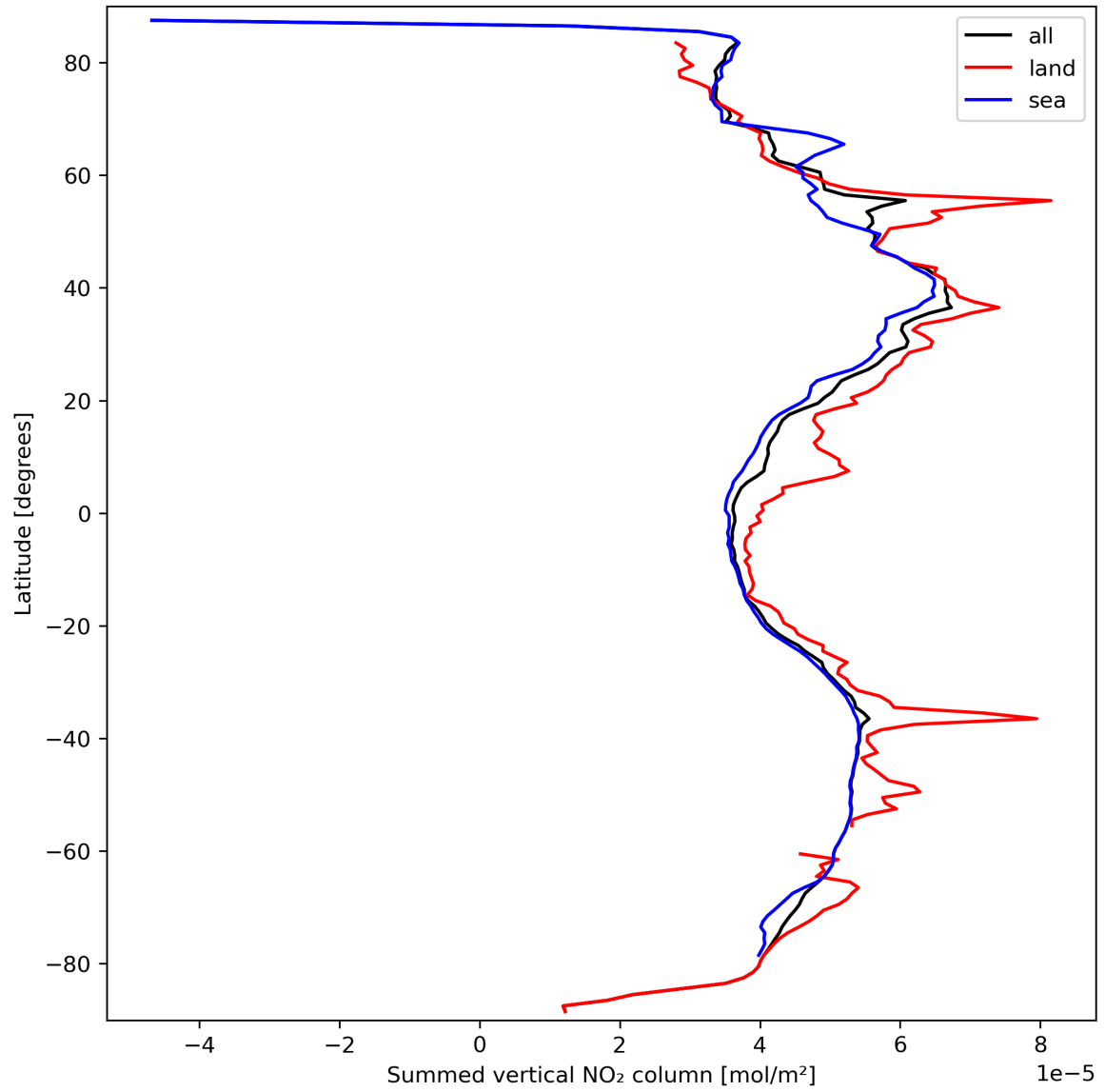
Figure 23: Zonal average of “Summed vertical NO 2 column” for 2024-03-18 to 2024-03-20.
