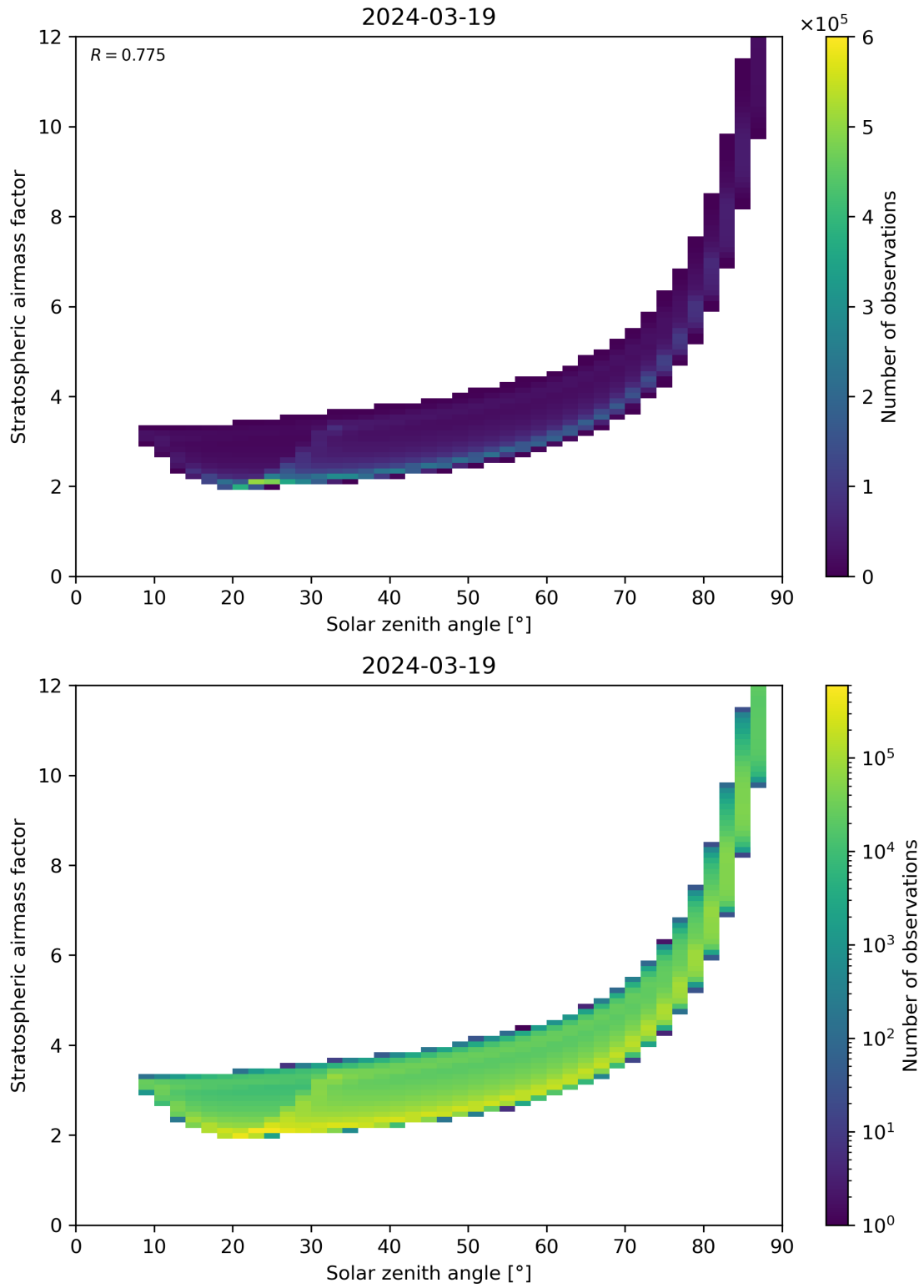
Figure 145: Scatter density plot of “Solar zenith angle” against “Stratospheric airmass factor” for 2024-03-18 to 2024-03-20.
