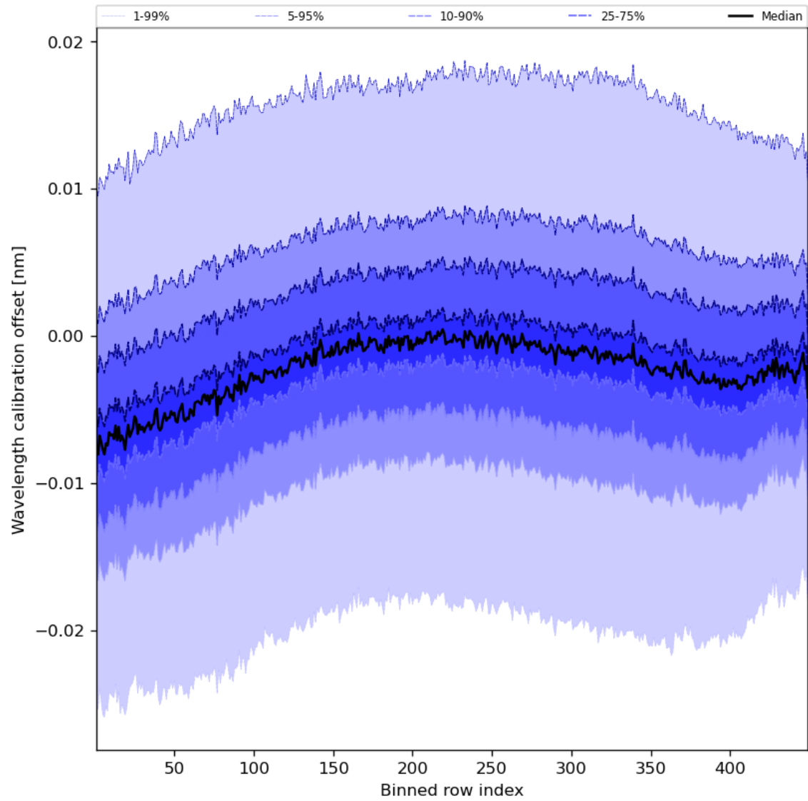
Figure 52: Along track statistics of “Wavelength calibration offset” for 2024-03-18 to 2024-03-20
