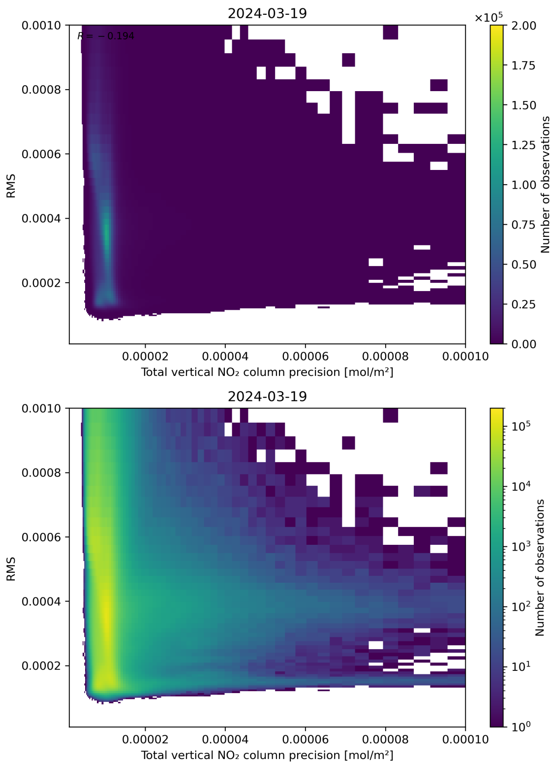
Figure 119: Scatter density plot of “Total vertical NO 2 column precision” against “RMS” for 2024-03-18 to 2024-03-20.
