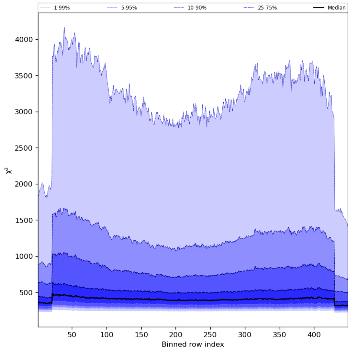
Figure 59: Along track statistics of “ \chi^2 ” for 2024-03-18 to 2024-03-20
