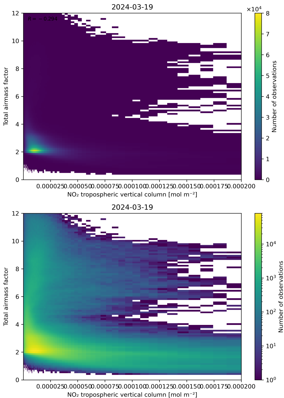
Figure 122: Scatter density plot of “NO 2 tropospheric vertical column” against “Total air mass factor” for 2024-03-18 to 2024-03-20.
