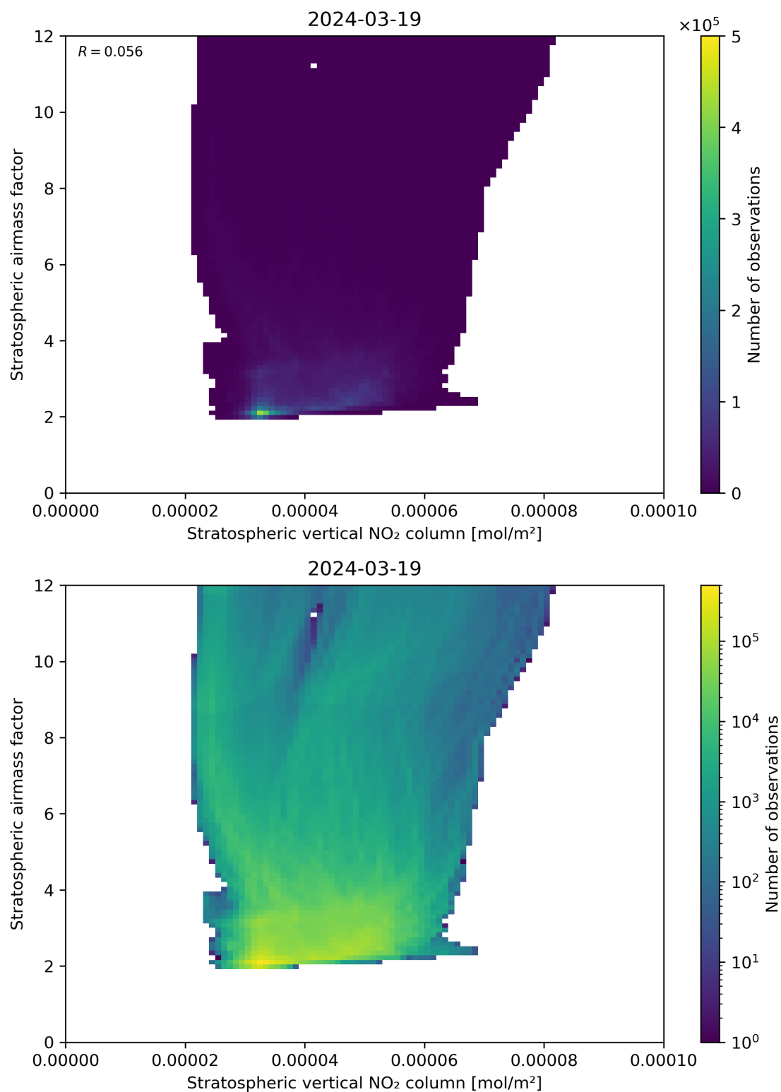
Figure 96: Scatter density plot of “Stratospheric vertical NO 2 column” against “Stratospheric airmass factor” for 2024-03-18 to 2024-03-20.
