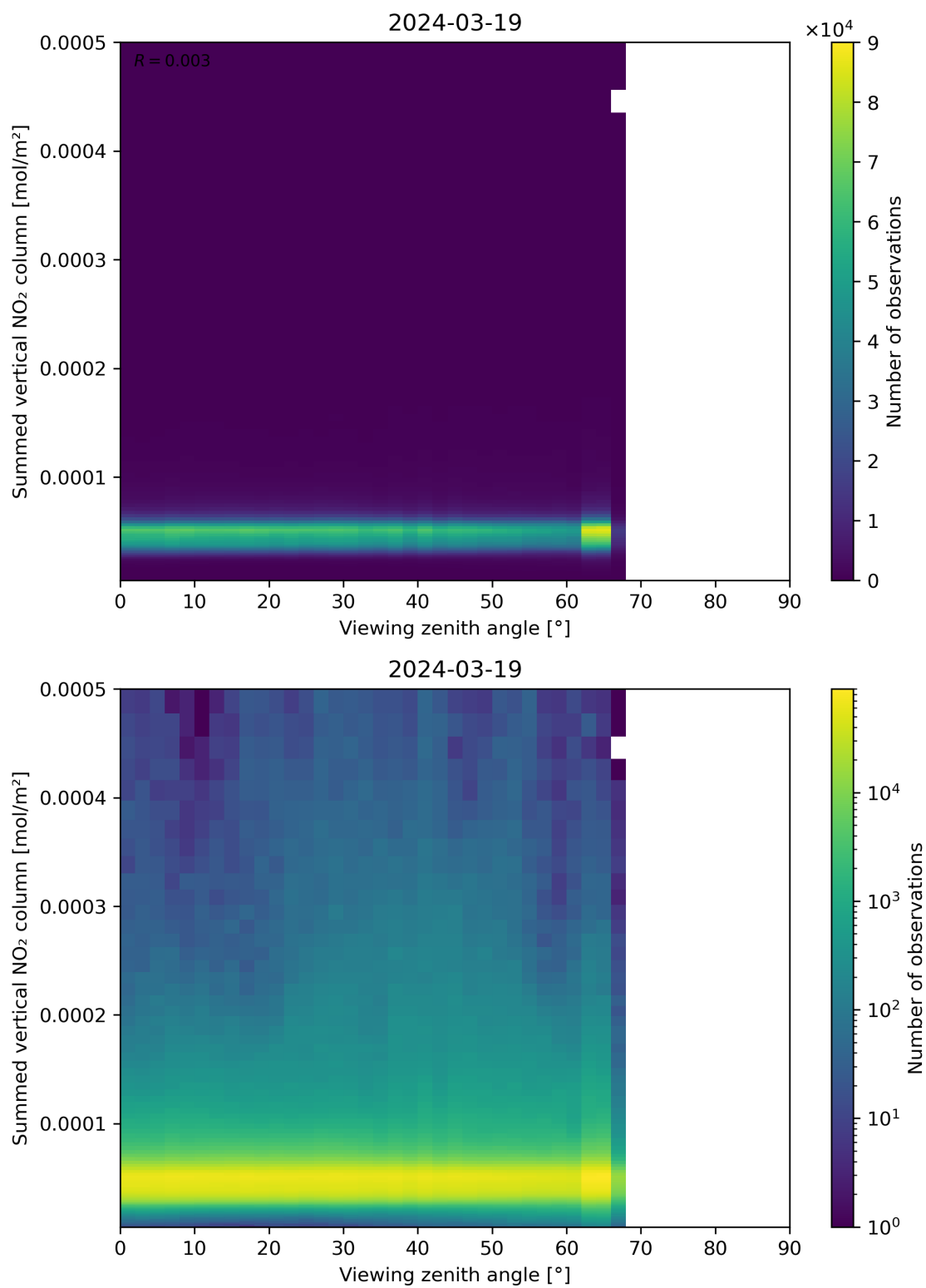
Figure 165: Scatter density plot of “Viewing zenith angle” against “Summed vertical NO 2 column” for 2024-03-18 to 2024-03-20.
