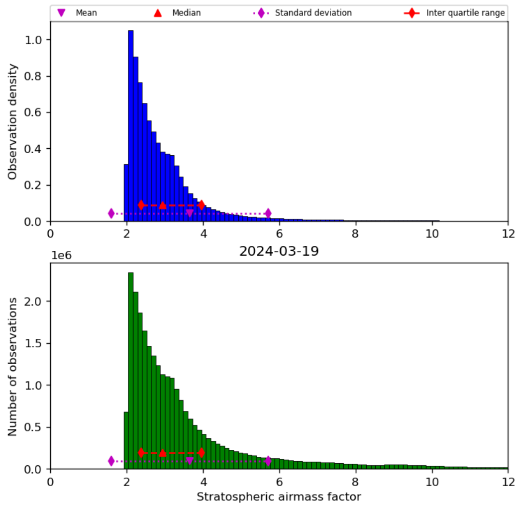
Figure 44: Histogram of “Stratospheric airmass factor” for 2024-03-18 to 2024-03-20
