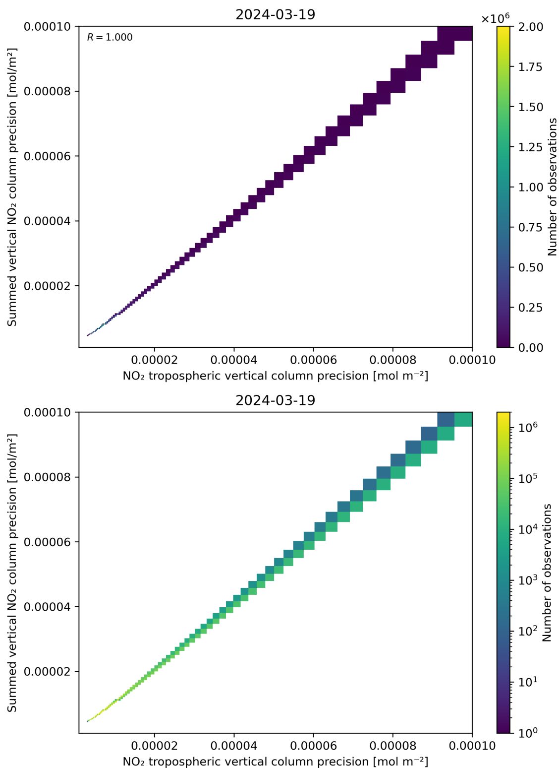
Figure 137: Scatter density plot of “NO 2 tropospheric vertical column precision” against “Summed vertical NO 2 column precision” for 2024-03-18 to 2024-03-20.
