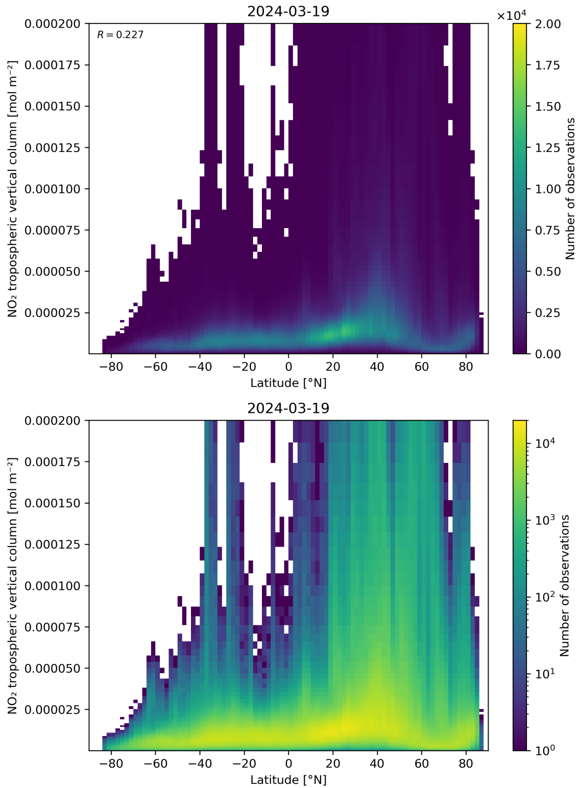
Figure 92: Scatter density plot of “Latitude” against “NO 2 tropospheric vertical column” for 2024-03-18 to 2024-03-20.
