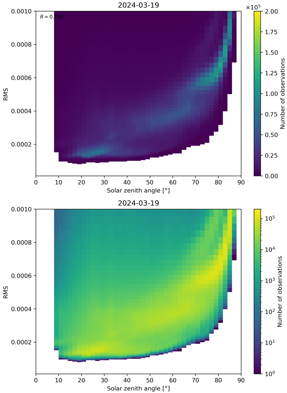
Figure 157: Scatter density plot of “Solar zenith angle” against “RMS” for 2024-03-18 to 2024-03-20.
