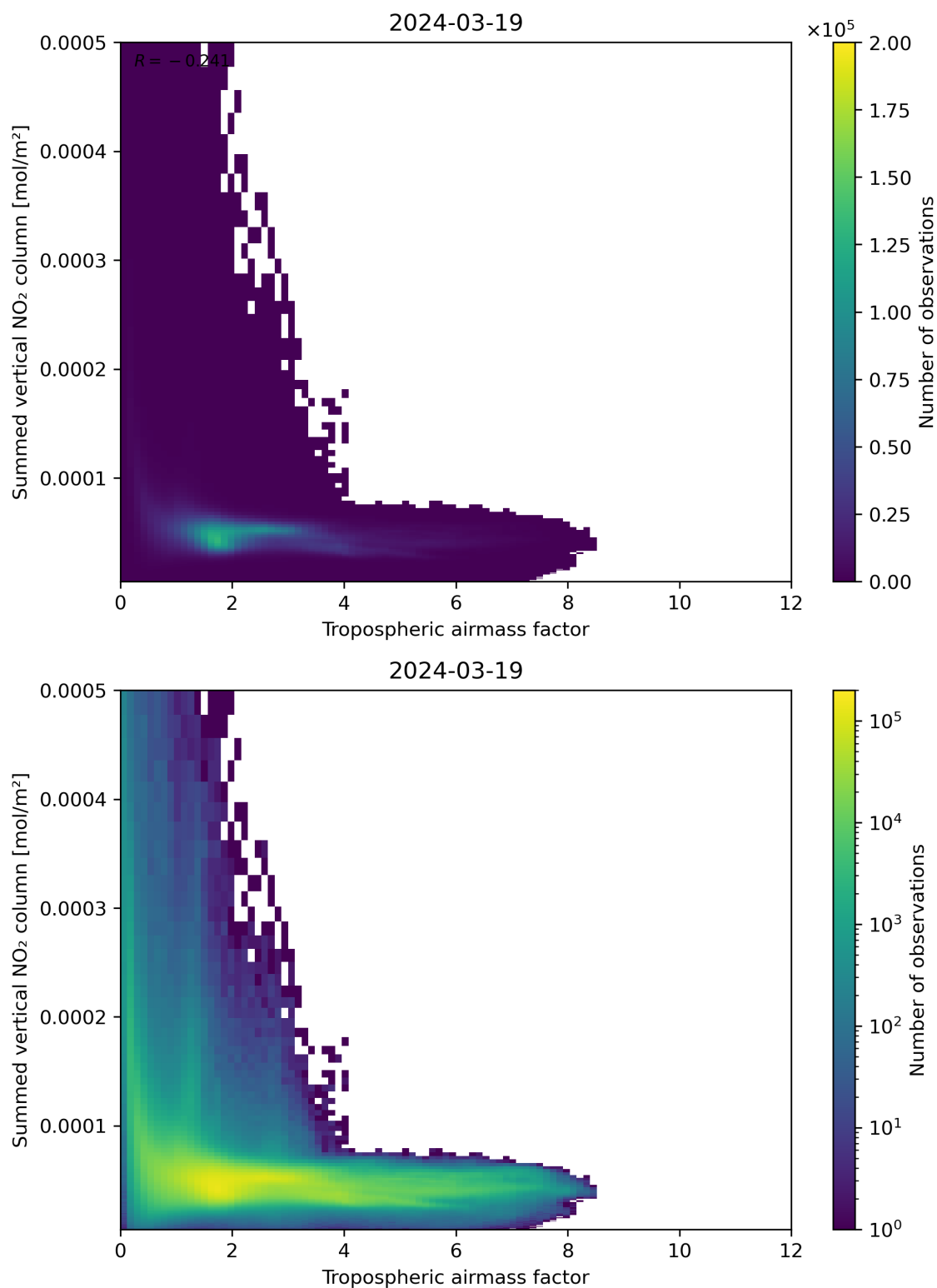
Figure 75: Scatter density plot of “Tropospheric air mass factor” against “Summed vertical NO 2 column” for 2024-03-18 to 2024-03-20.
