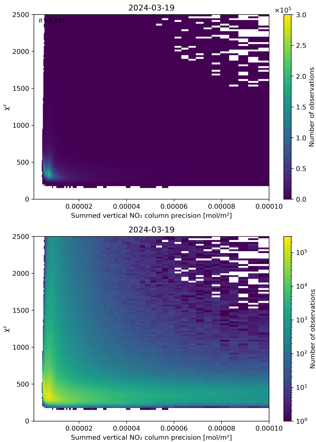
Figure 107: Scatter density plot of “Summed vertical NO 2 column precision” against “ \chi^2 ” for 2024-03-18 to 2024-03-20.
