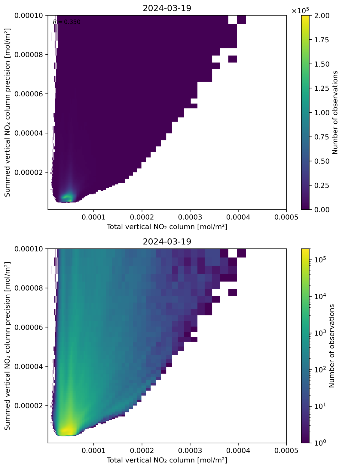
Figure 113: Scatter density plot of “Total vertical NO 2 column” against “Summed vertical NO 2 column precision” for 2024-03-18 to 2024-03-20.
