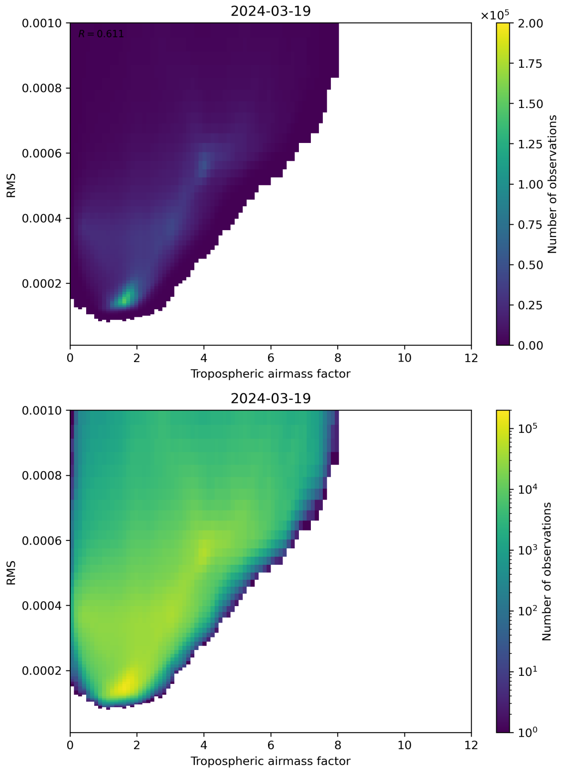
Figure 79: Scatter density plot of “Tropospheric airmass factor” against “RMS” for 2024-03-18 to 2024-03-20.
