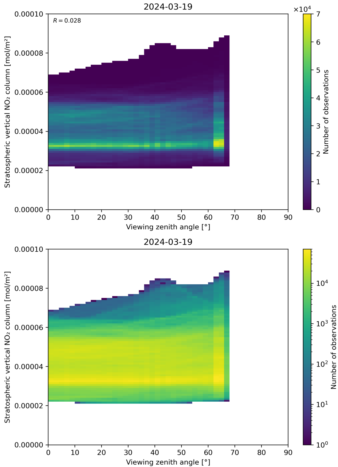
Figure 164: Scatter density plot of “Viewing zenith angle” against “Stratospheric vertical NO 2 column” for 2024-03-18 to 2024-03-20.
