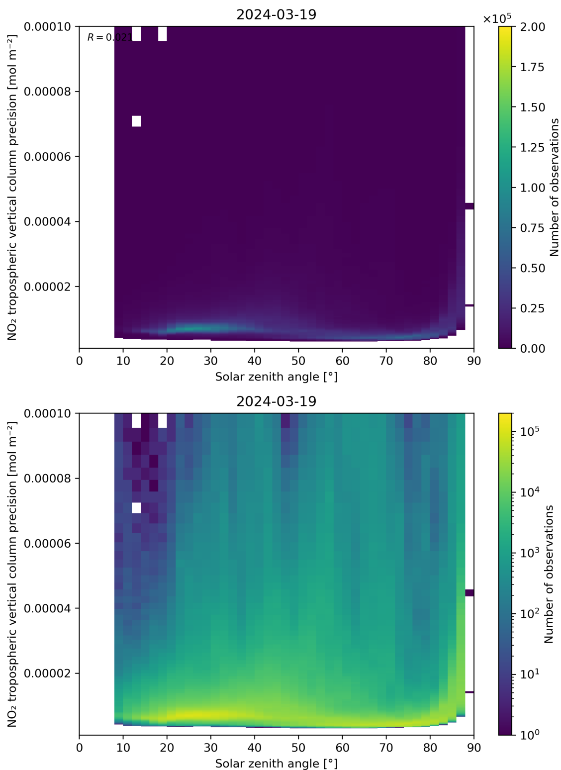
Figure 156: Scatter density plot of “Solar zenith angle” against “NO 2 tropospheric vertical column precision” for 2024-03-18 to 2024-03-20.
