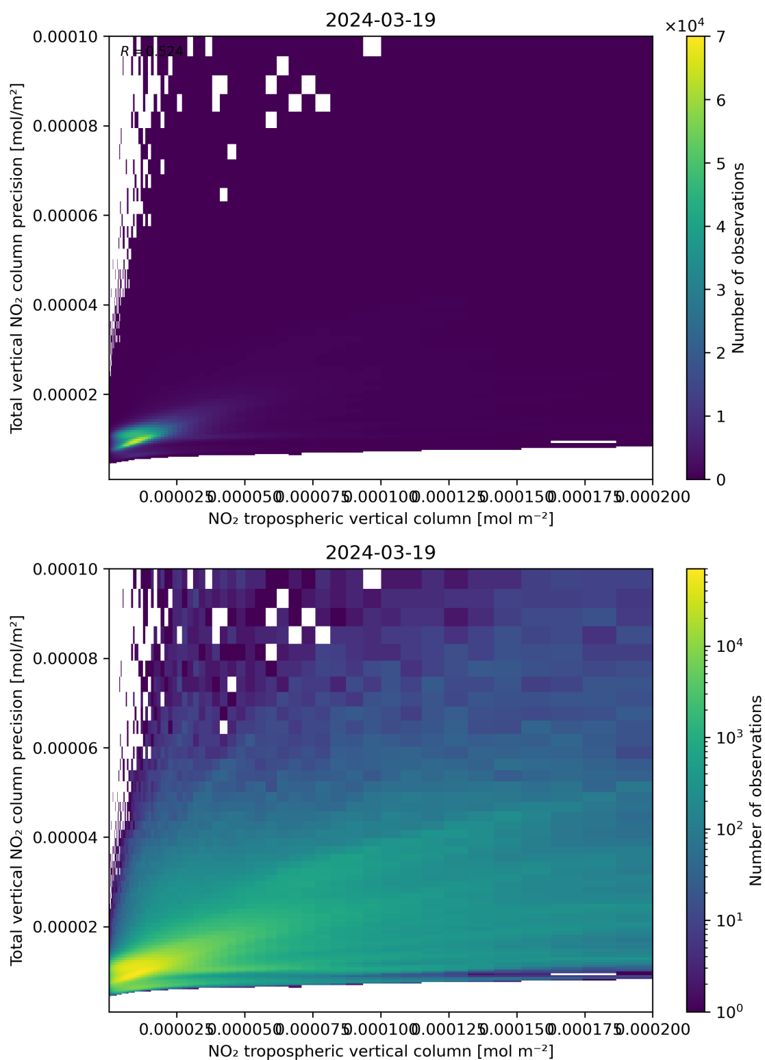
Figure 129: Scatter density plot of “NO 2 tropospheric vertical column” against “Total vertical NO 2 column precision” for 2024-03-18 to 2024-03-20.
