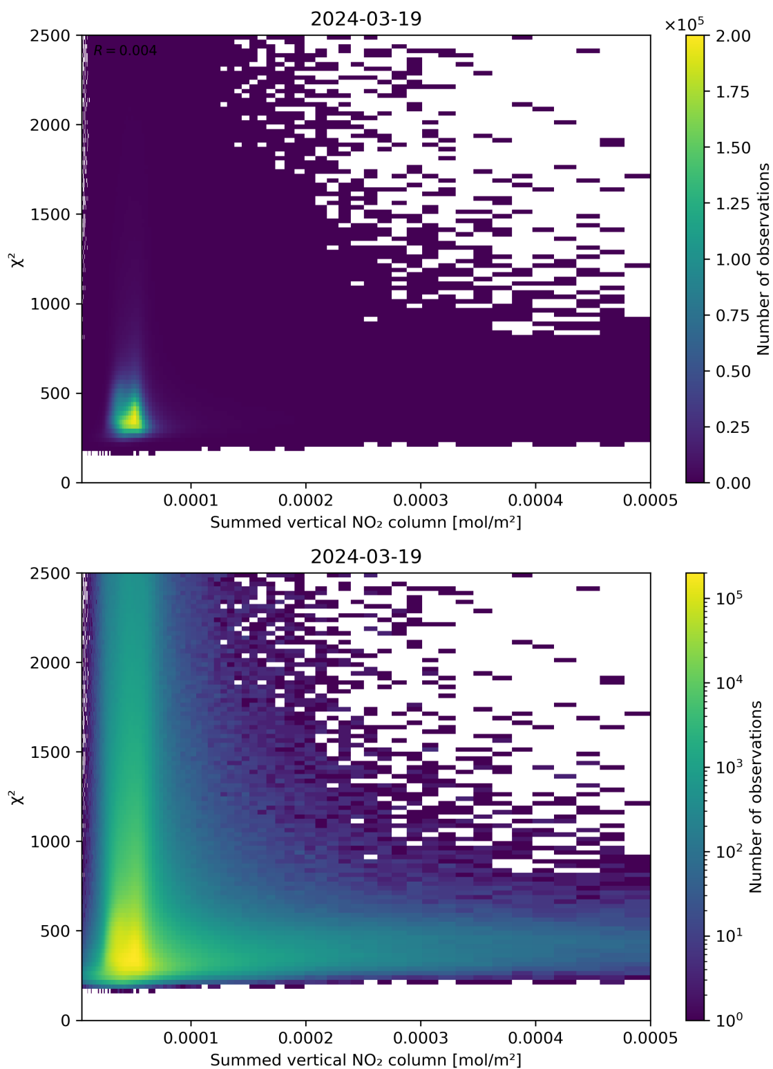
Figure 104: Scatter density plot of “Summed vertical NO 2 column” against “ \chi^2 ” for 2024-03-18 to 2024-03-20.
