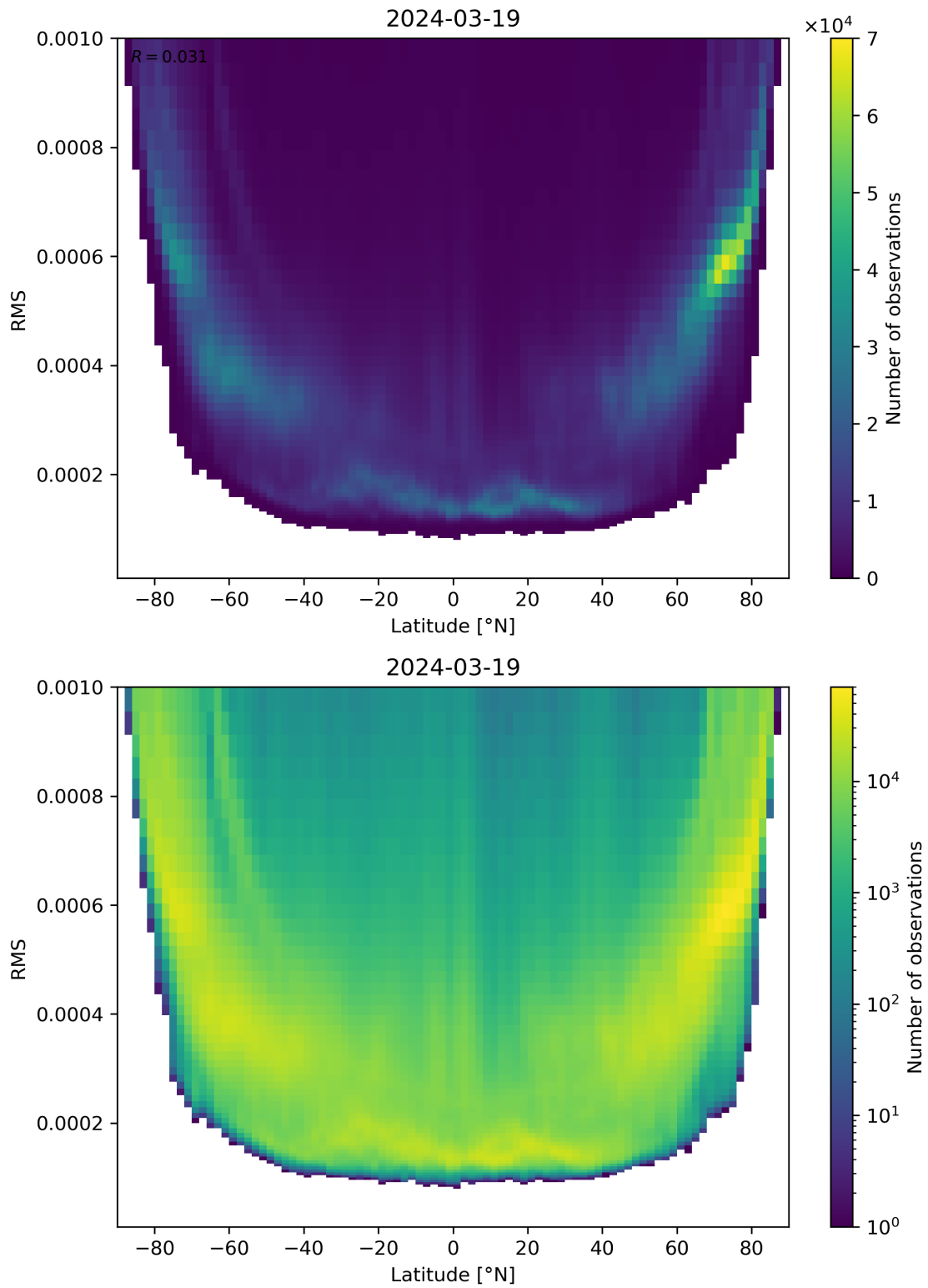
Figure 94: Scatter density plot of “Latitude” against “RMS” for 2024-03-18 to 2024-03-20.
