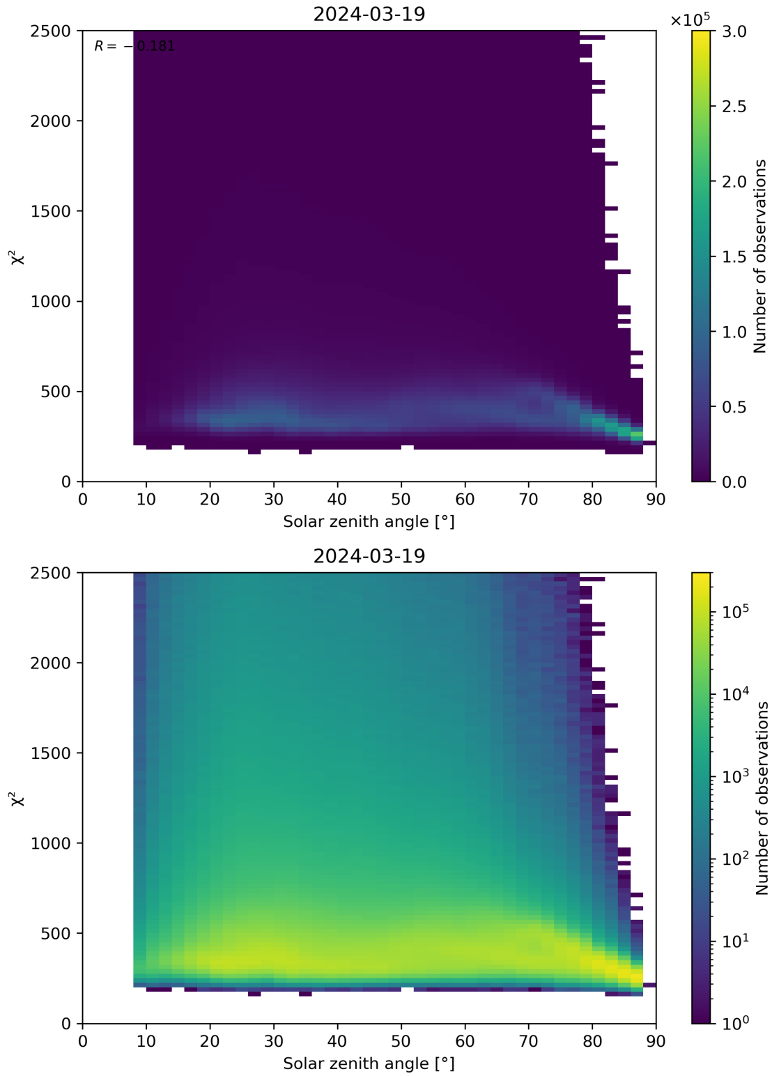
Figure 148: Scatter density plot of “Solar zenith angle” against “ \chi^2 ” for 2024-03-18 to 2024-03-20.
