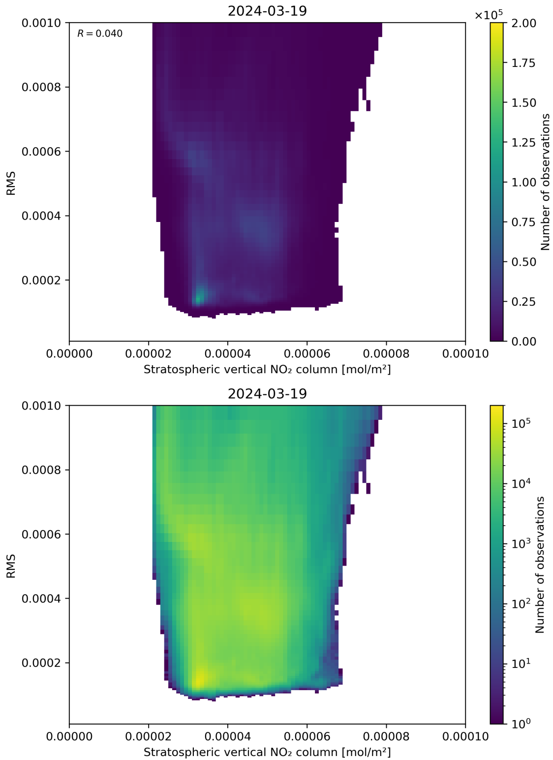
Figure 102: Scatter density plot of “Stratospheric vertical NO 2 column” against “RMS” for 2024-03-18 to 2024-03-20.
