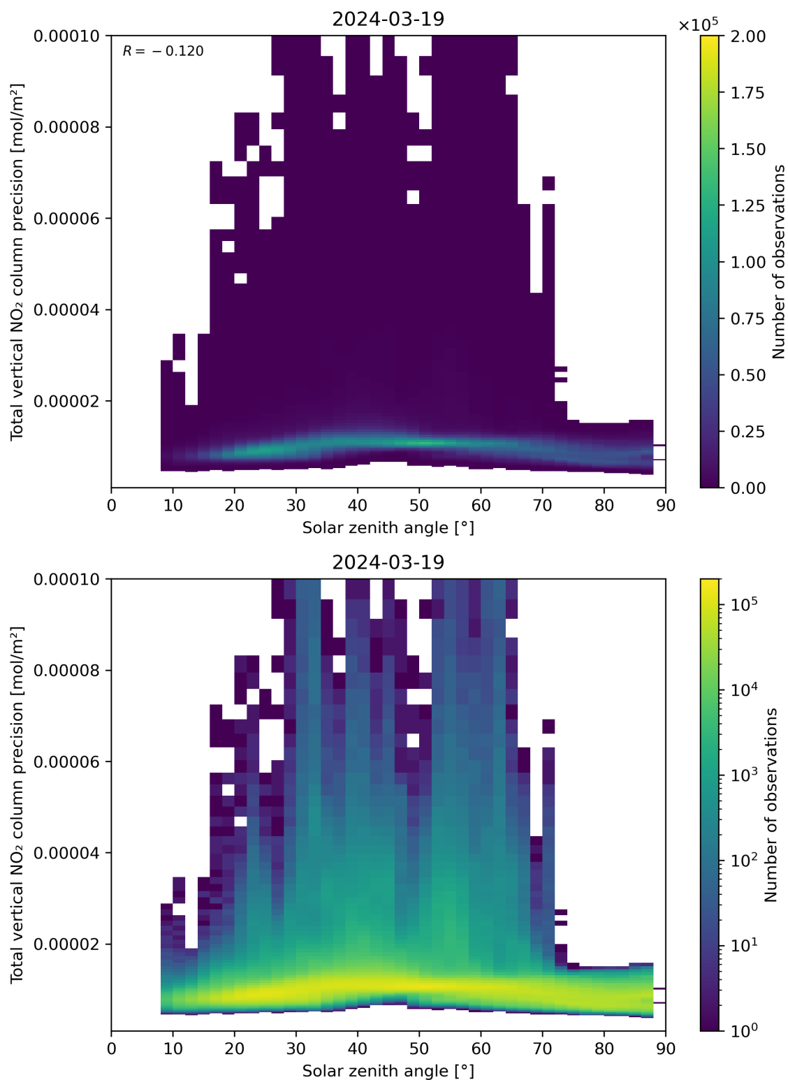
Figure 154: Scatter density plot of “Solar zenith angle” against “Total vertical NO 2 column precision” for 2024-03-18 to 2024-03-20.
