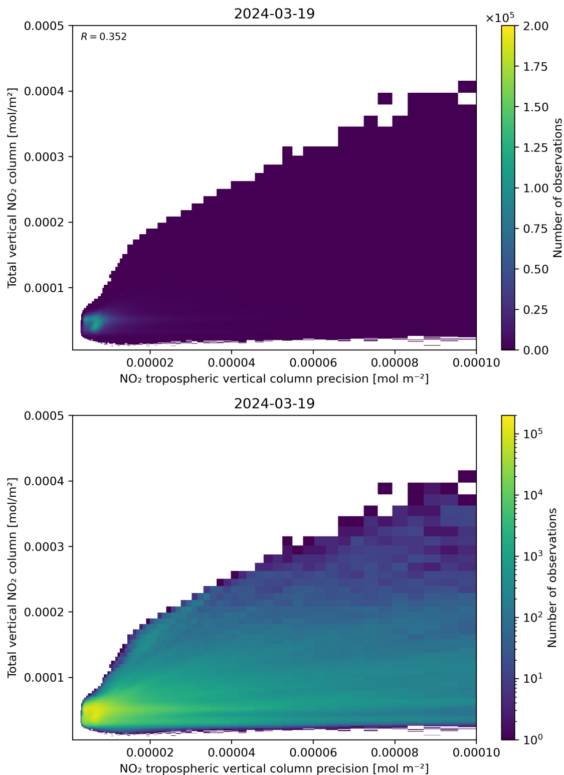
Figure 138: Scatter density plot of “NO 2 tropospheric vertical column precision” against “Total vertical NO 2 column” for 2024-03-18 to 2024-03-20.
