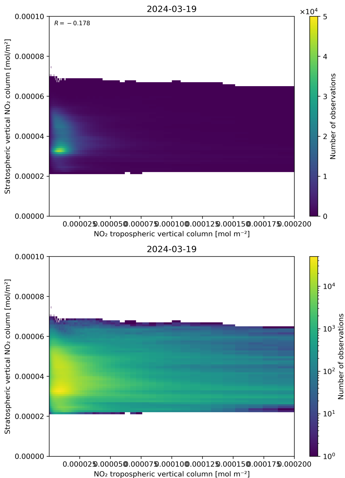
Figure 125: Scatter density plot of “NO 2 tropospheric vertical column” against “Stratospheric vertical NO 2 column” for 2024-03-18 to 2024-03-20.
