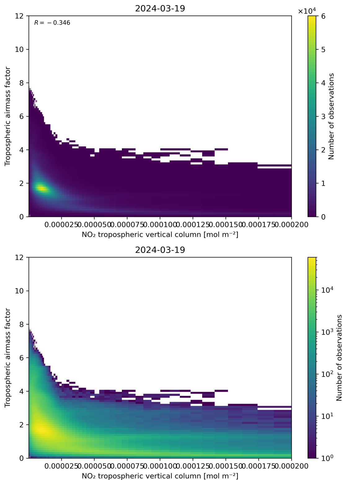
Figure 123: Scatter density plot of “NO 2 tropospheric vertical column” against “Tropospheric airmass factor” for 2024-03-18 to 2024-03-20.
