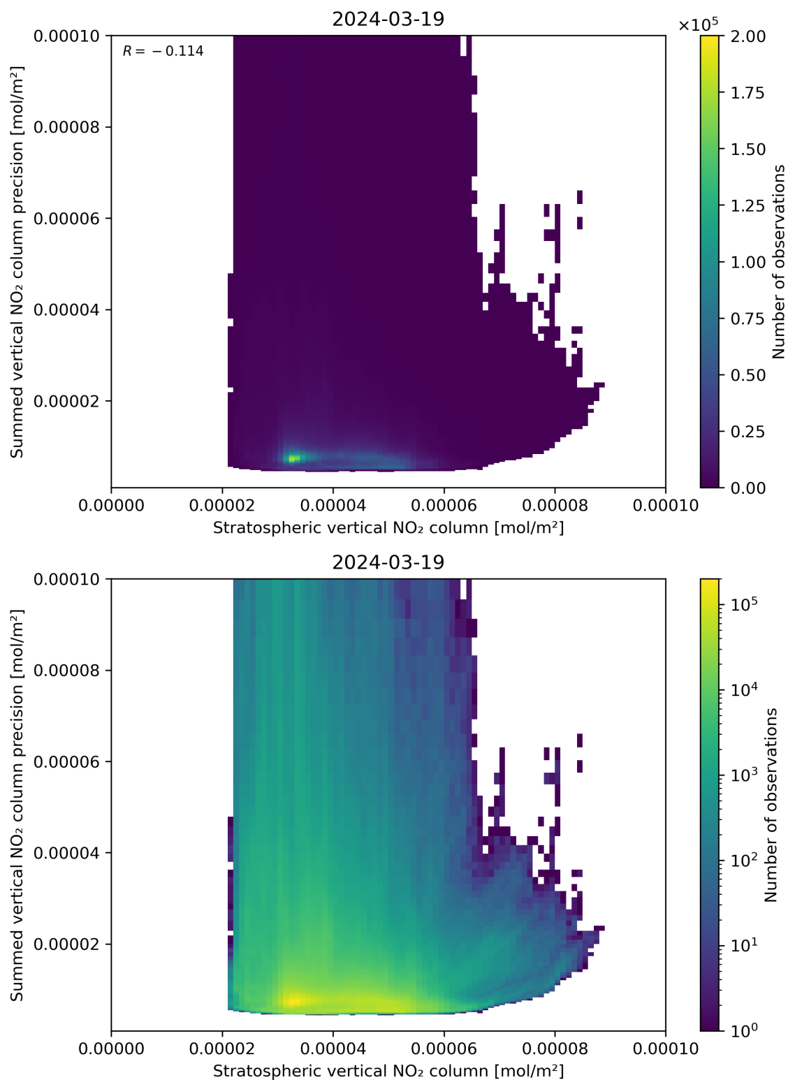
Figure 99: Scatter density plot of “Stratospheric vertical NO 2 column” against “Summed vertical NO 2 column precision” for 2024-03-18 to 2024-03-20.
