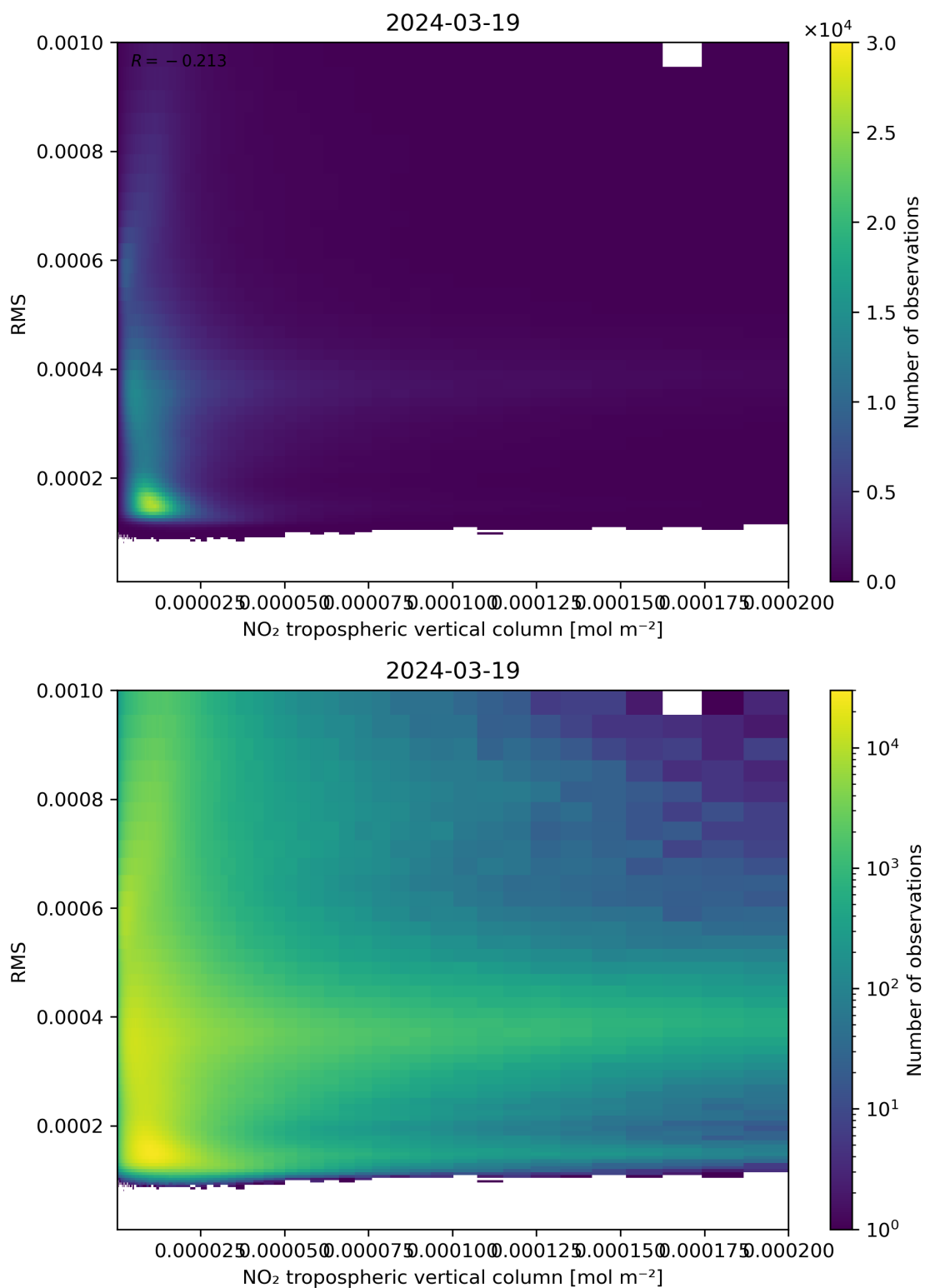
Figure 142: Scatter density plot of “NO 2 tropospheric vertical column” against “RMS” for 2024-03-18 to 2024-03-20.
