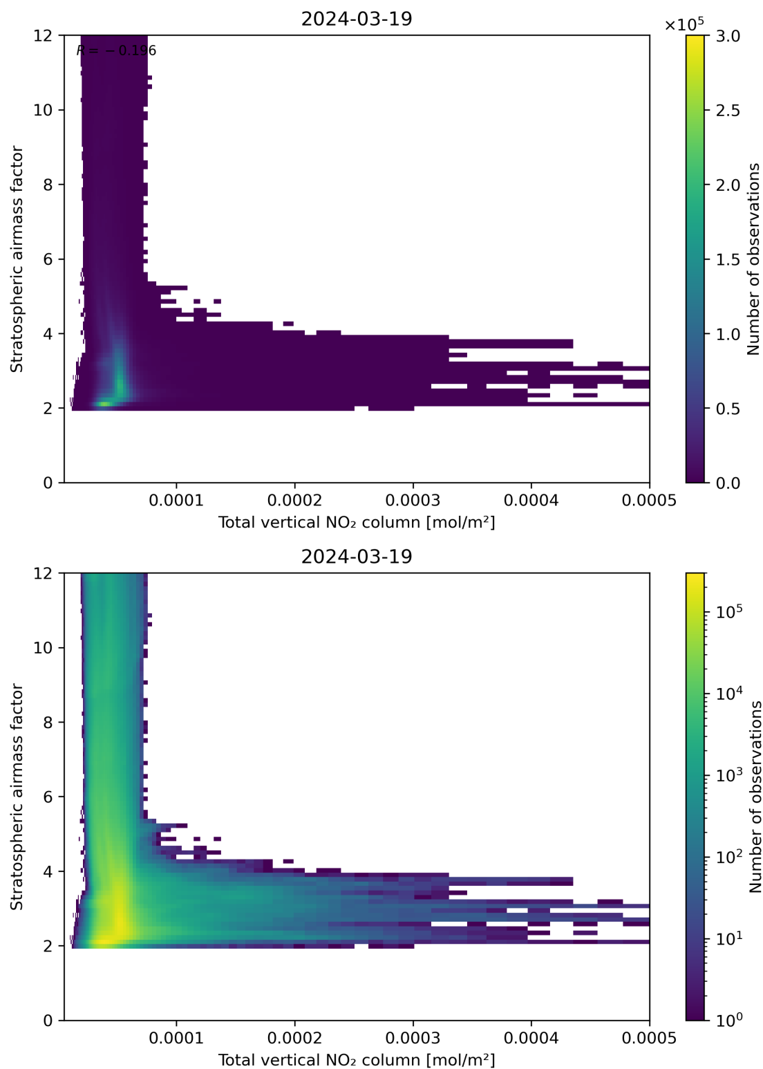
Figure 110: Scatter density plot of “Total vertical NO 2 column” against “Stratospheric airmass factor” for 2024-03-18 to 2024-03-20.
