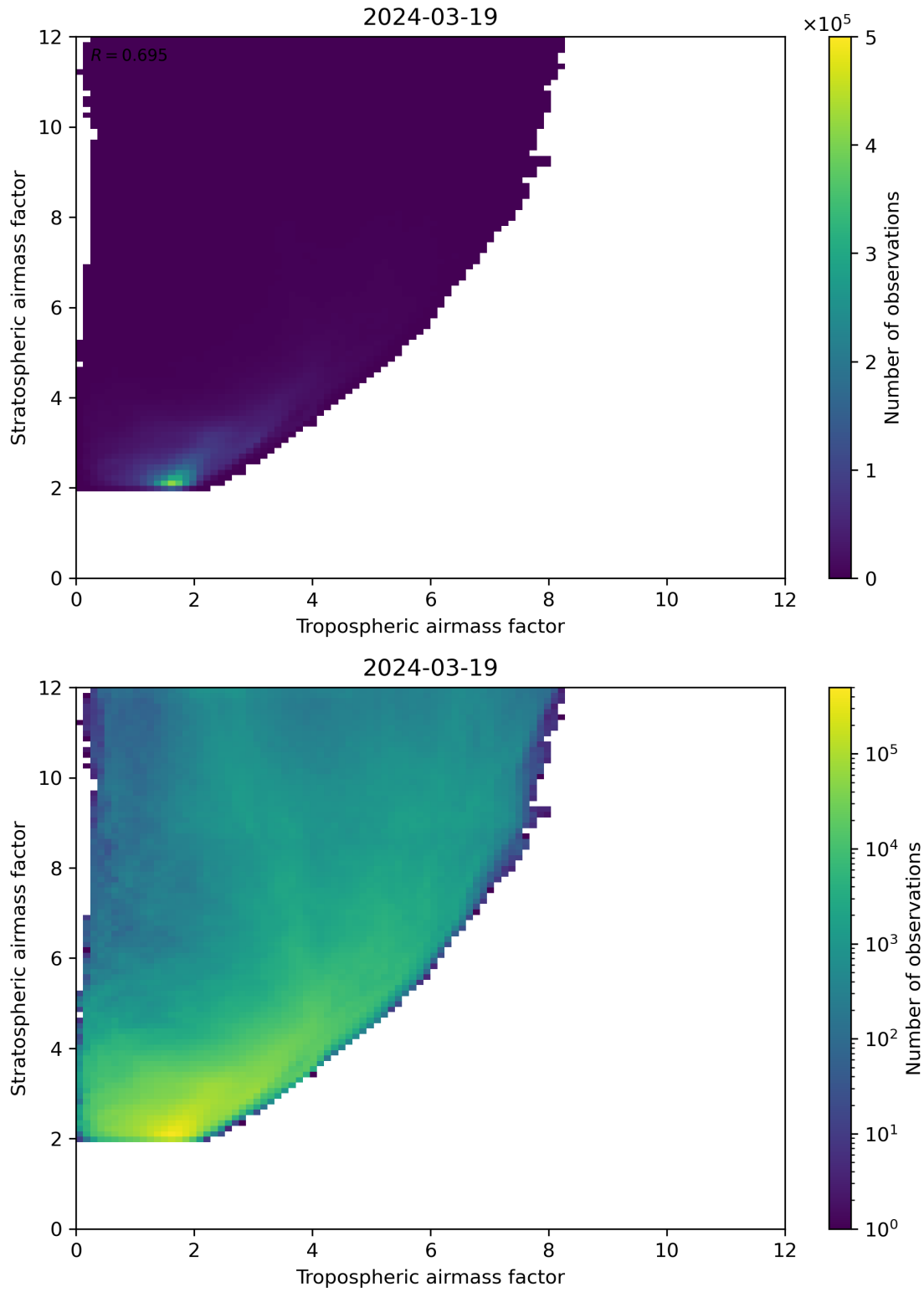
Figure 71: Scatter density plot of “Tropospheric airmass factor” against “Stratospheric airmass factor” for 2024-03-18 to 2024-03-20.
