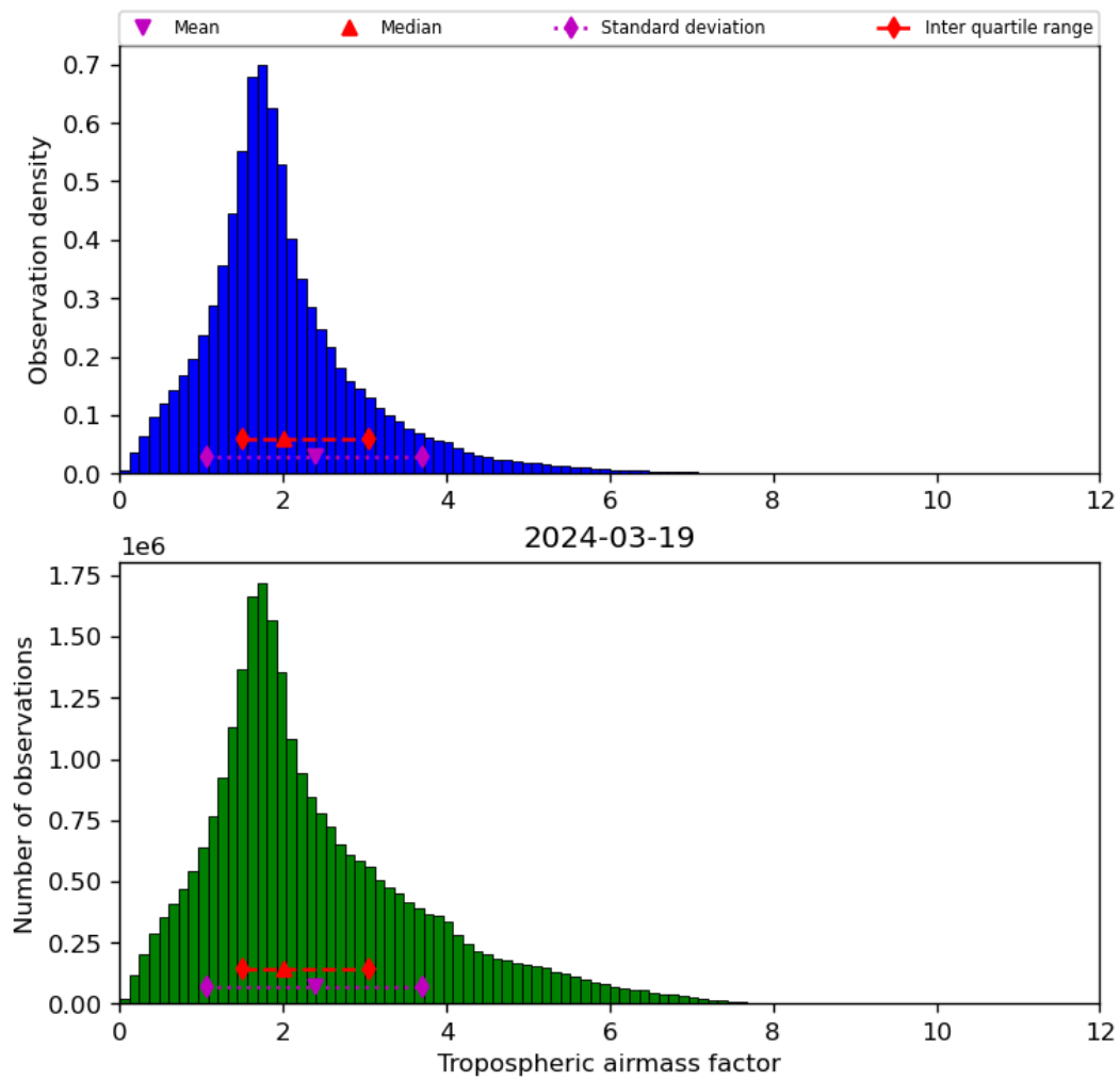
Figure 31: Histogram of “Tropospheric airmass factor” for 2024-03-18 to 2024-03-20
