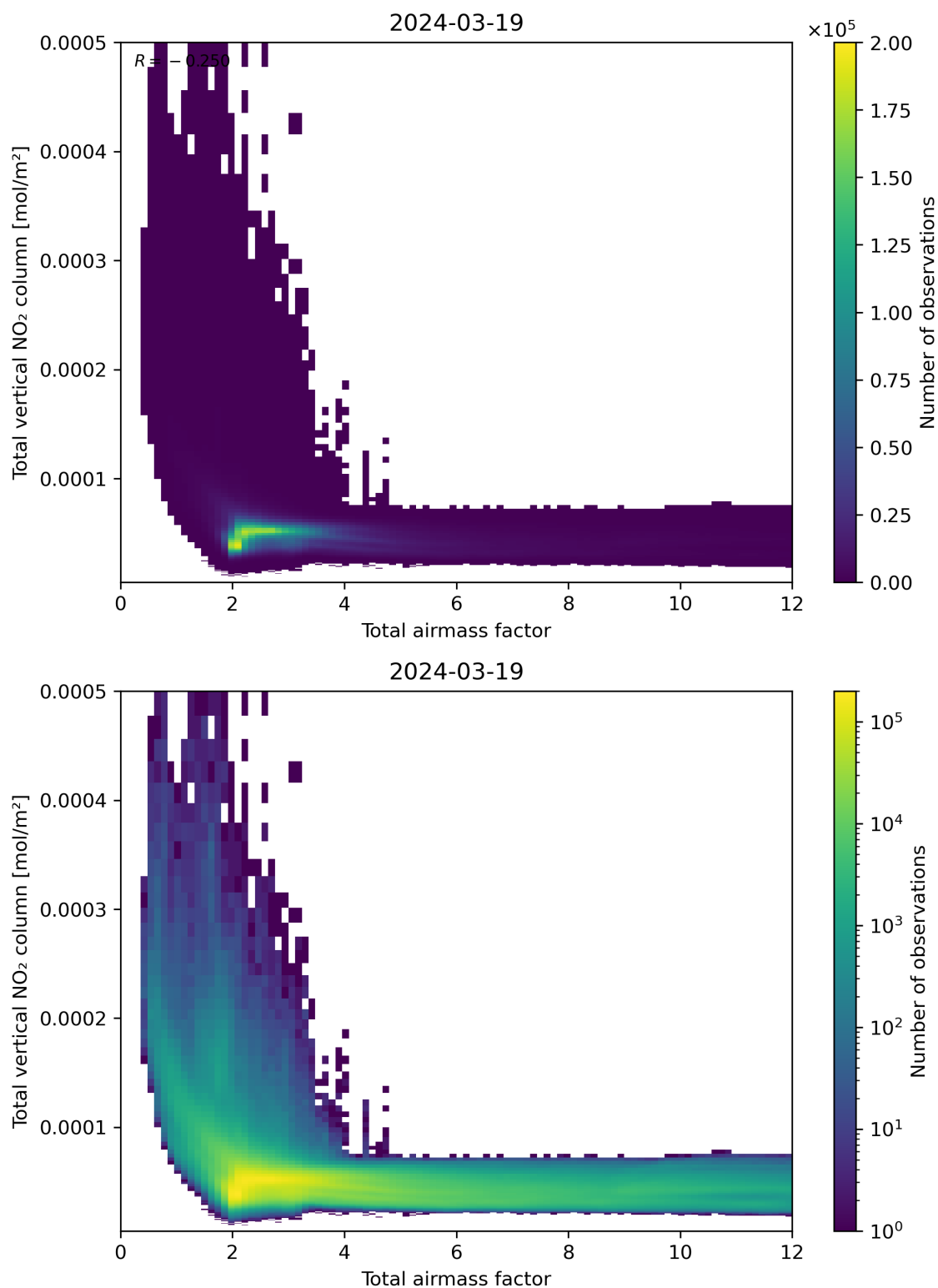
Figure 67: Scatter density plot of “Total airmass factor” against “Total vertical NO 2 column” for 2024-03-18 to 2024-03-20.
