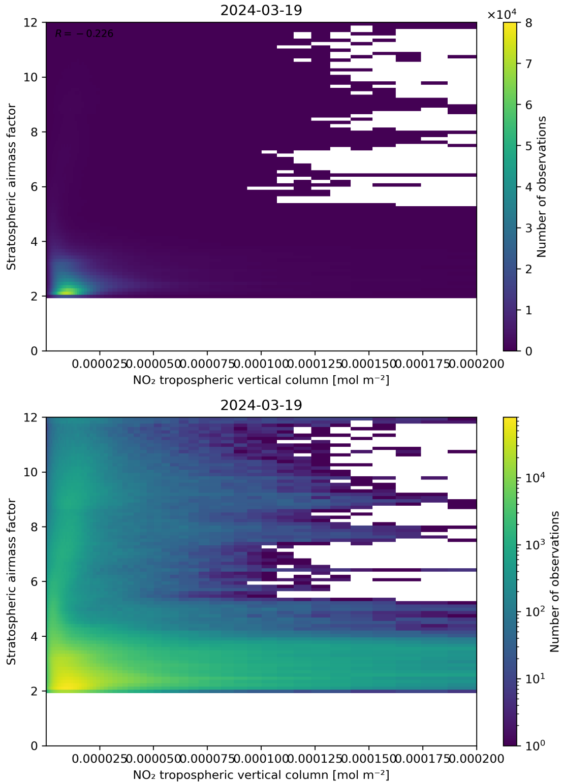
Figure 121: Scatter density plot of “NO 2 tropospheric vertical column” against “Stratospheric air mass factor” for 2024-03-18 to 2024-03-20.
