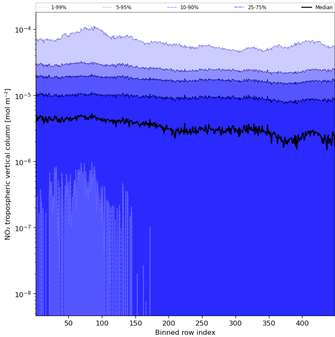
Figure 46: Along track statistics of “NO 2 tropospheric vertical column” for 2024-03-18 to 2024-03-20
