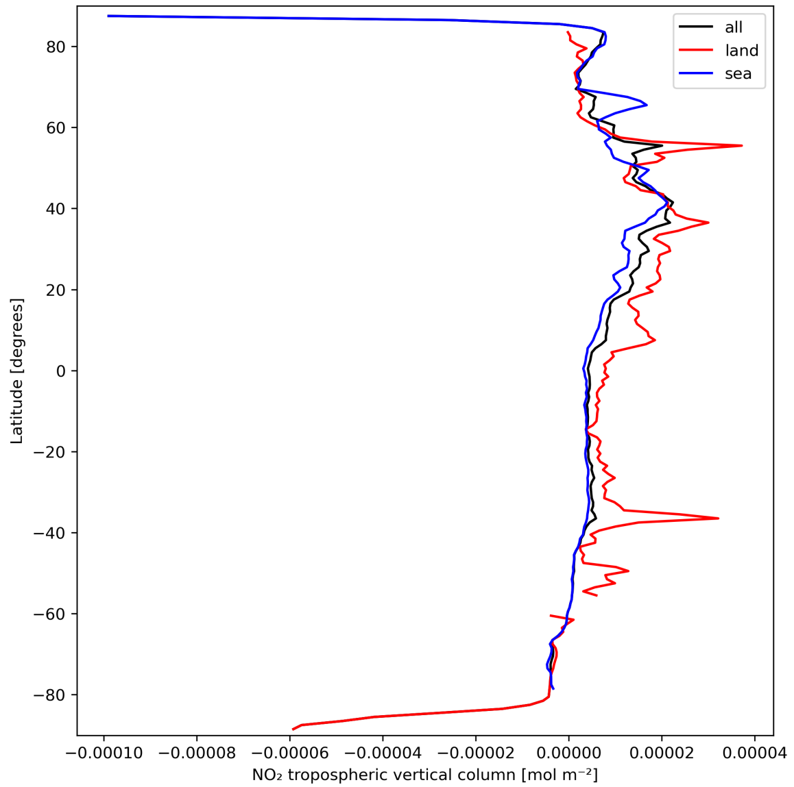
Figure 12: Zonal average of “NO 2 tropospheric vertical column” for 2024-03-18 to 2024-03-20.
