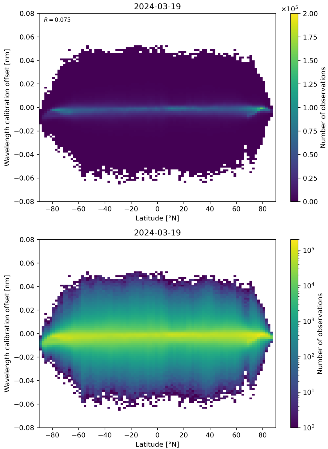
Figure 95: Scatter density plot of “Latitude” against “Wavelength calibration offset” for 2024-03-18 to 2024-03-20.
