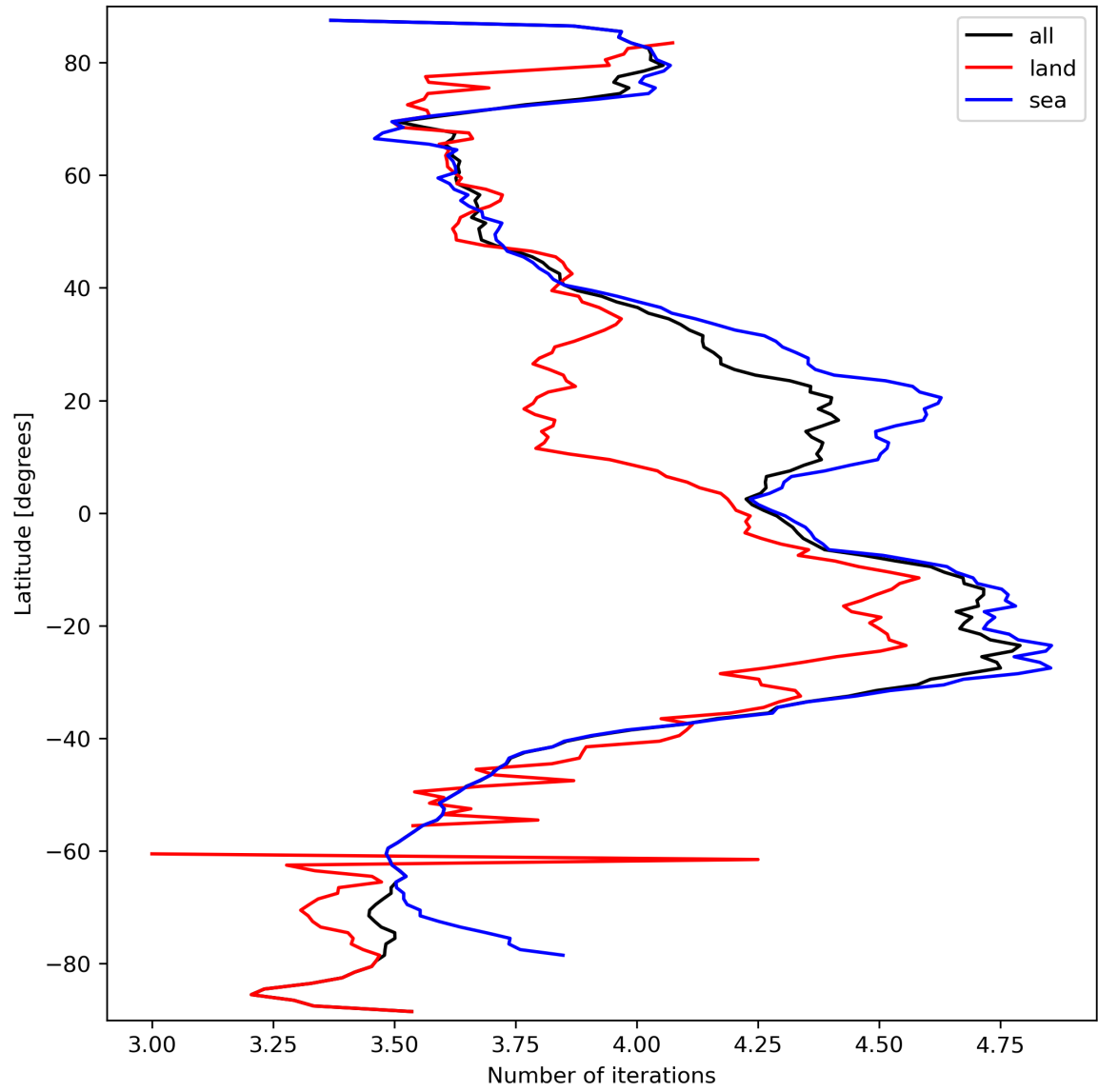
Figure 17: Zonal average of “Number of iterations” for 2024-03-18 to 2024-03-20.
