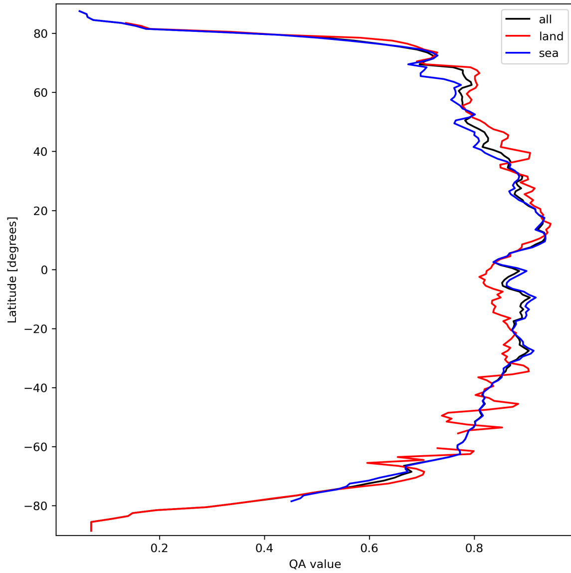
Figure 11: Zonal average of “QA value” for 2024-03-18 to 2024-03-20.
