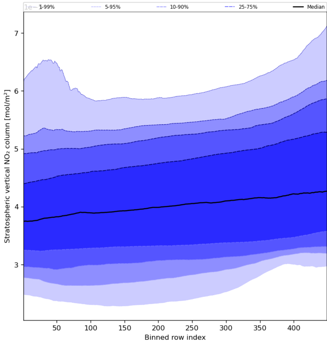
Figure 53: Along track statistics of “Stratospheric vertical NO 2 column” for 2024-03-18 to 2024-03-20
