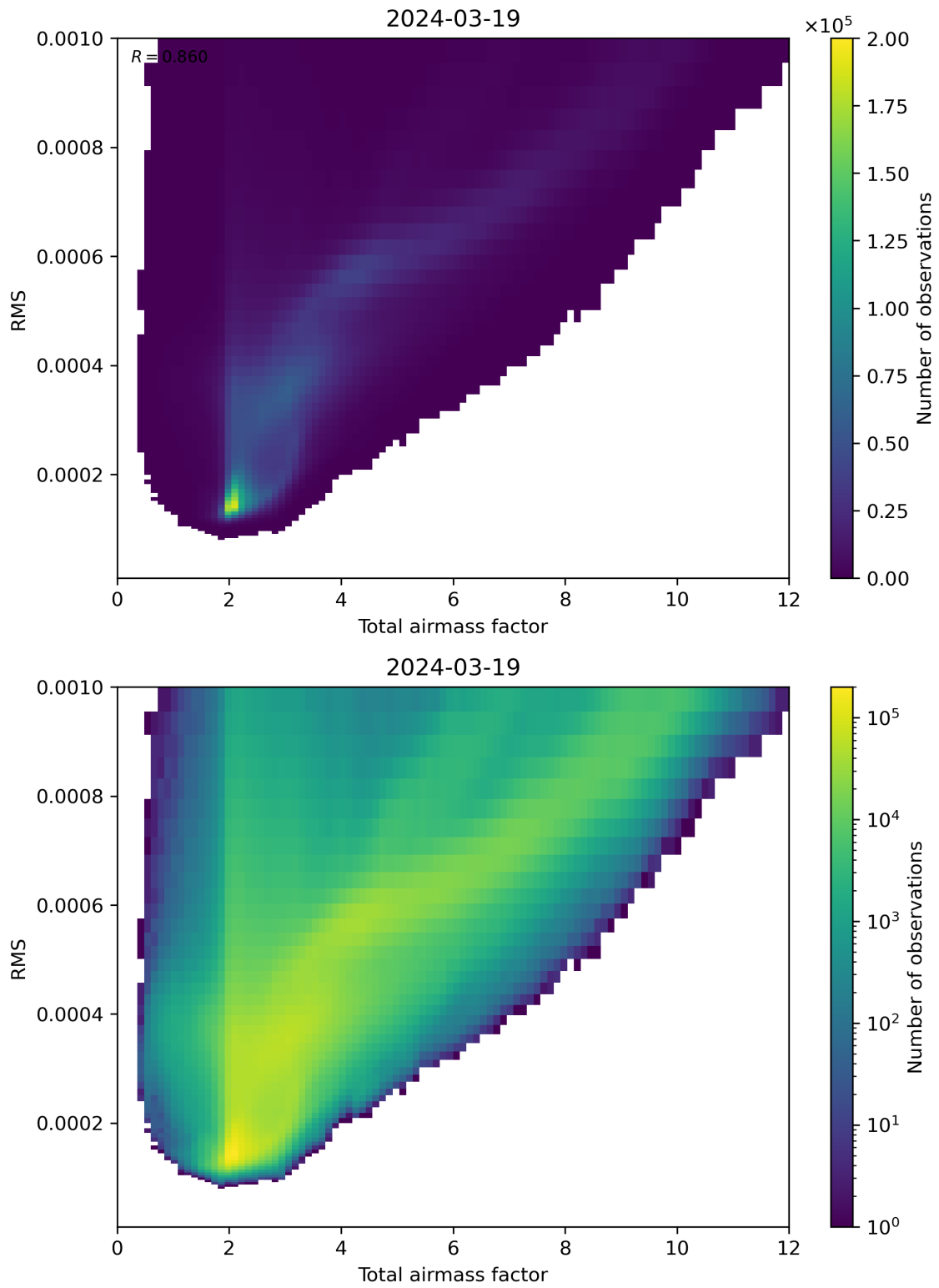
Figure 69: Scatter density plot of “Total airmass factor” against “RMS” for 2024-03-18 to 2024-03-20.
