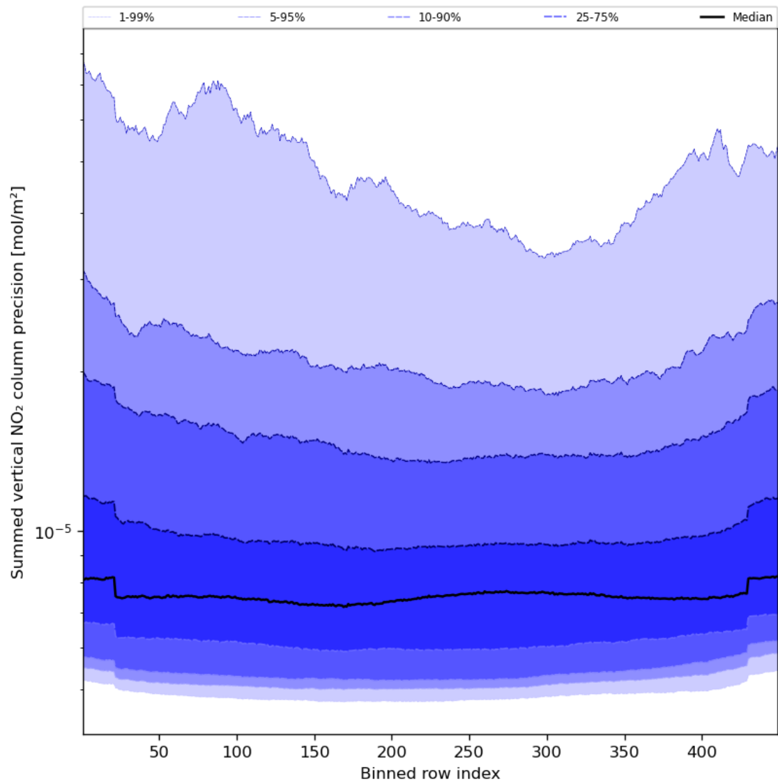
Figure 58: Along track statistics of “Summed vertical NO 2 column precision” for 2024-03-18 to 2024-03-20
