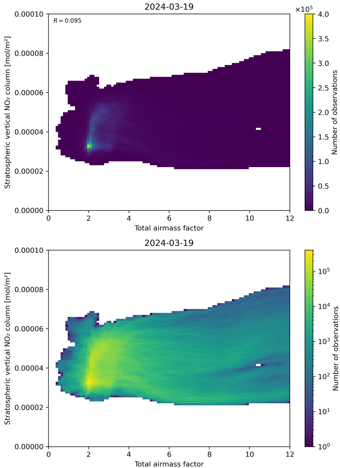
Figure 64: Scatter density plot of “Total airmass factor” against “Stratospheric vertical \text{NO}_2 column” for 2024-03-18 to 2024-03-20.
