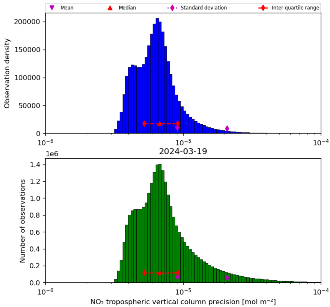
Figure 30: Histogram of “NO 2 tropospheric vertical column precision” for 2024-03-18 to 2024-03-20
