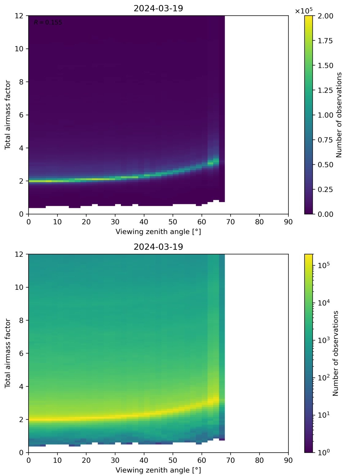
Figure 160: Scatter density plot of “Viewing zenith angle” against “Total airmass factor” for 2024-03-18 to 2024-03-20.
