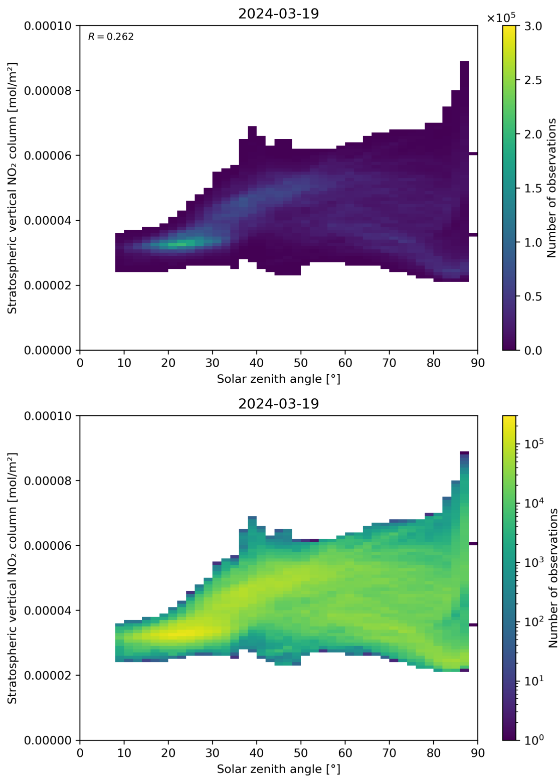
Figure 150: Scatter density plot of “Solar zenith angle” against “Stratospheric vertical \text{NO}_2 column” for 2024-03-18 to 2024-03-20.
