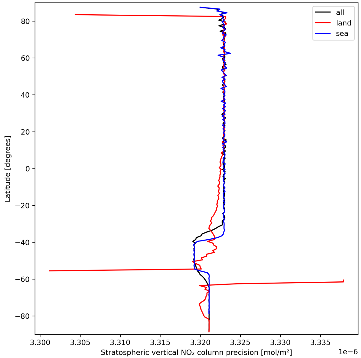
Figure 20: Zonal average of “Stratospheric vertical NO 2 column precision” for 2024-03-18 to 2024-03-20.
