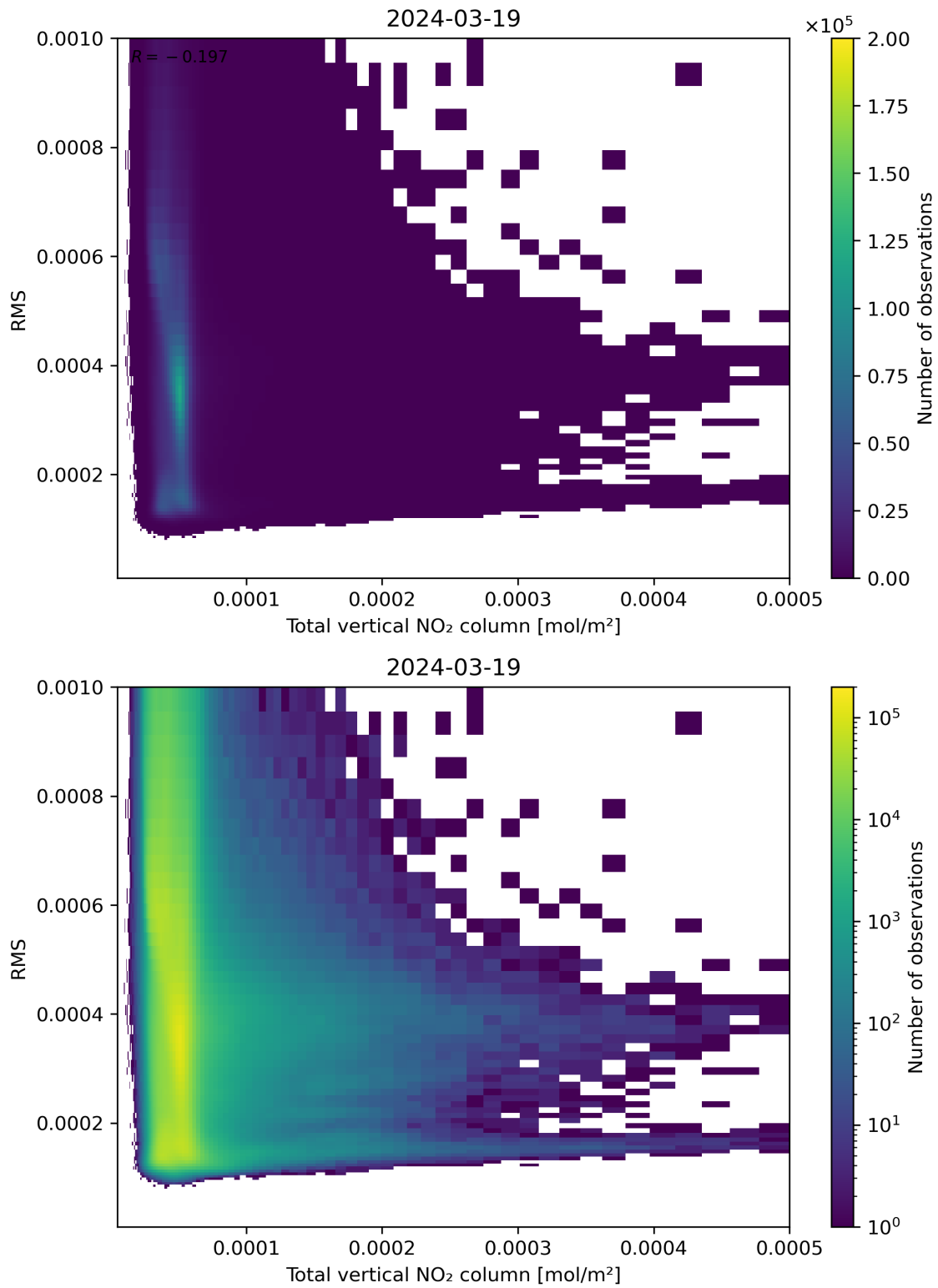
Figure 120: Scatter density plot of “Total vertical NO 2 column” against “RMS” for 2024-03-18 to 2024-03-20.
