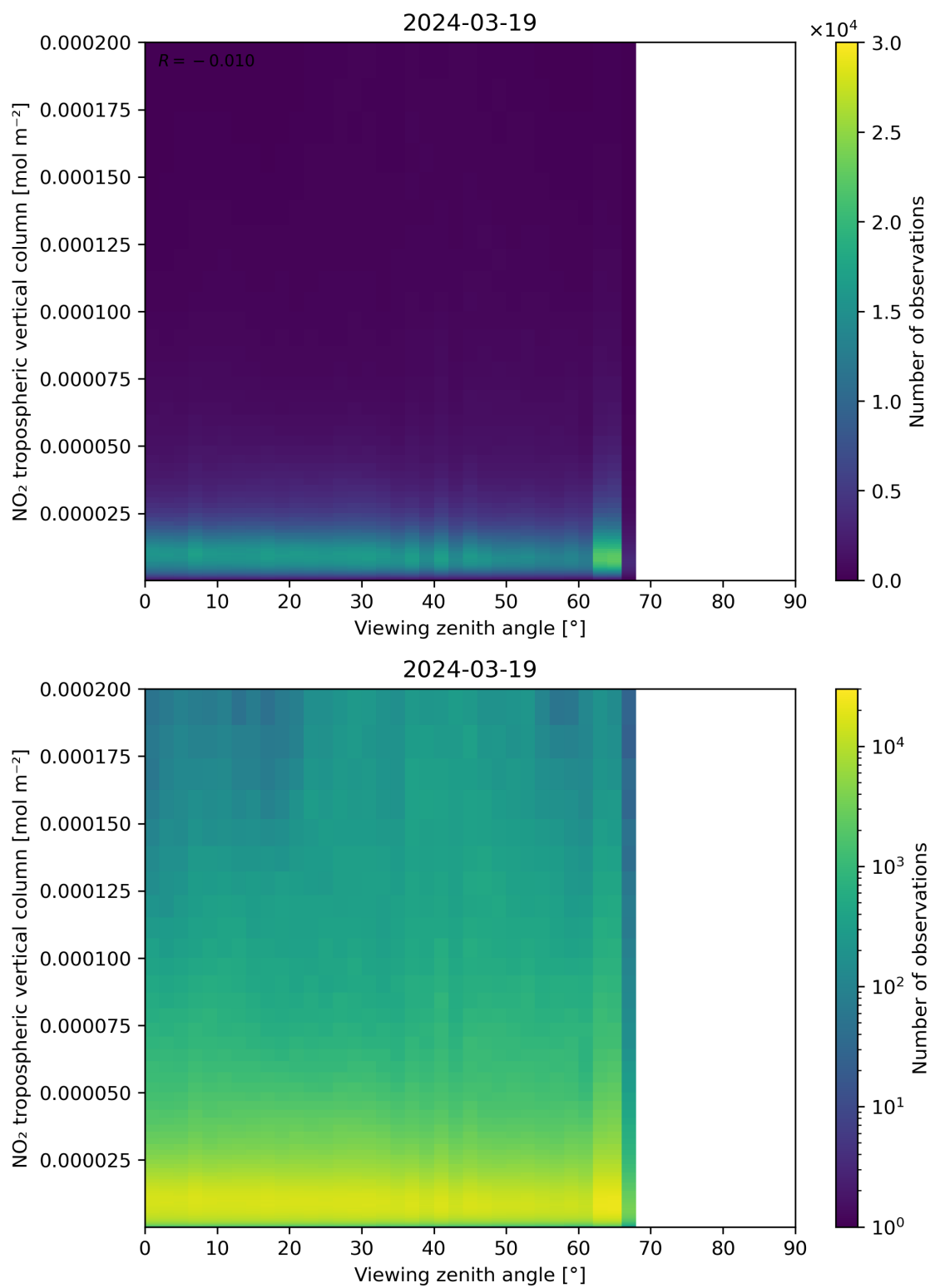
Figure 169: Scatter density plot of “Viewing zenith angle” against “NO 2 tropospheric vertical column” for 2024-03-18 to 2024-03-20.
