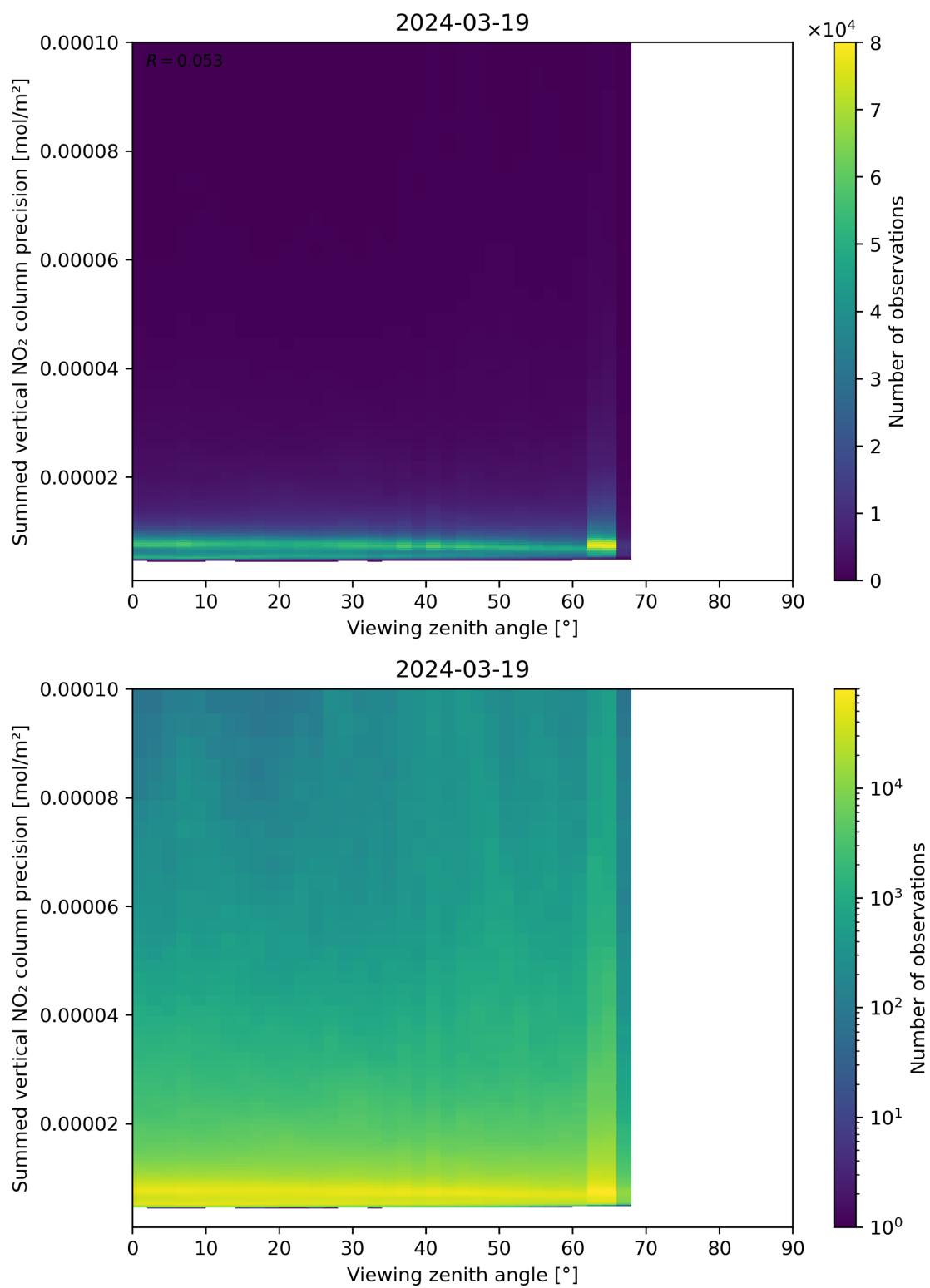
Figure 166: Scatter density plot of “Viewing zenith angle” against “Summed vertical NO 2 column precision” for 2024-03-18 to 2024-03-20.
