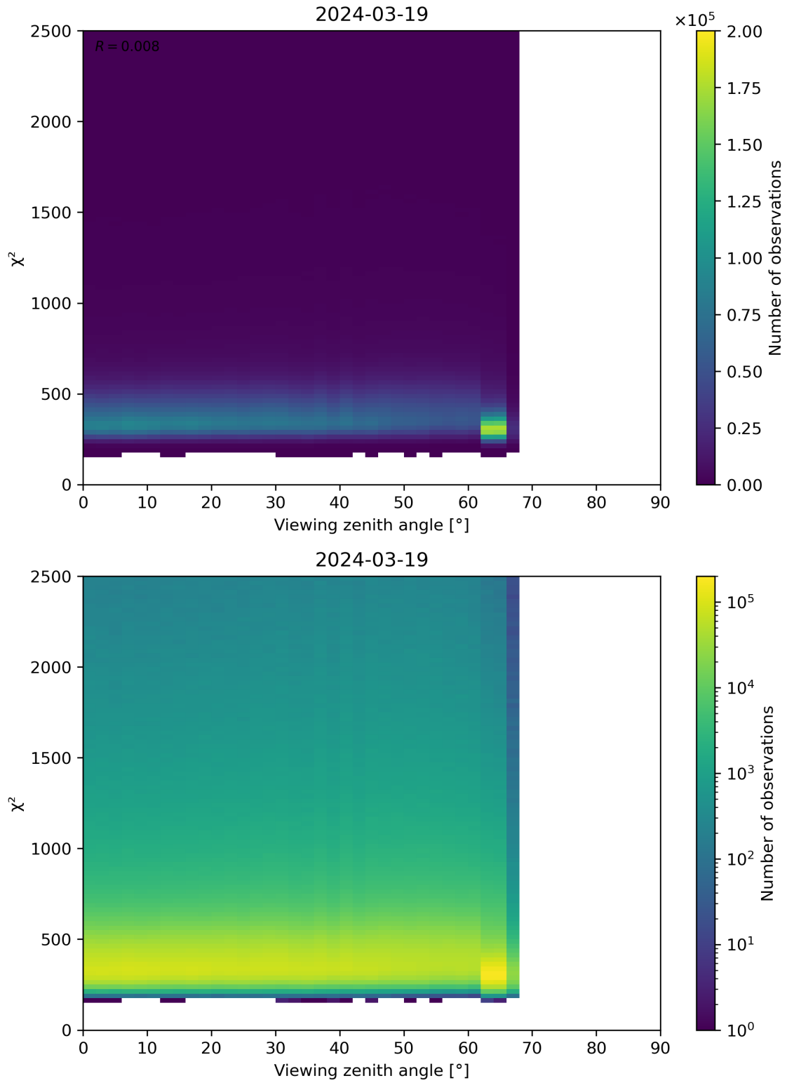
Figure 162: Scatter density plot of “Viewing zenith angle” against “ \chi^2 ” for 2024-03-18 to 2024-03-20.
