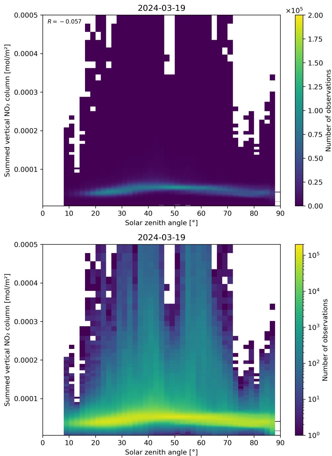
Figure 151: Scatter density plot of “Solar zenith angle” against “Summed vertical NO 2 column” for 2024-03-18 to 2024-03-20.
