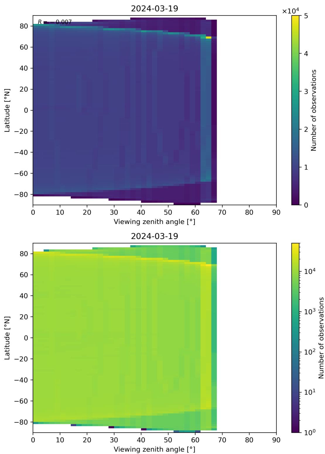
Figure 163: Scatter density plot of “Viewing zenith angle” against “Latitude” for 2024-03-18 to 2024-03-20.
