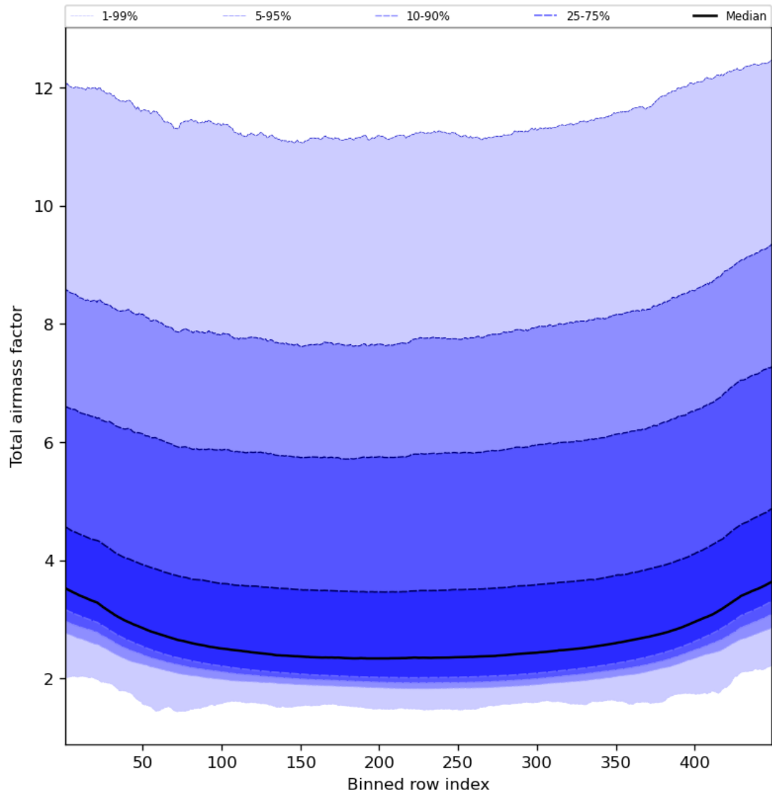
Figure 49: Along track statistics of “Total airmass factor” for 2024-03-18 to 2024-03-20
