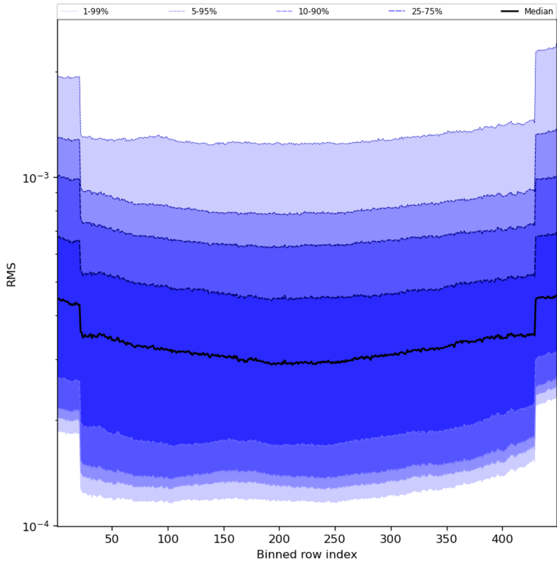
Figure 60: Along track statistics of “RMS” for 2024-03-18 to 2024-03-20
