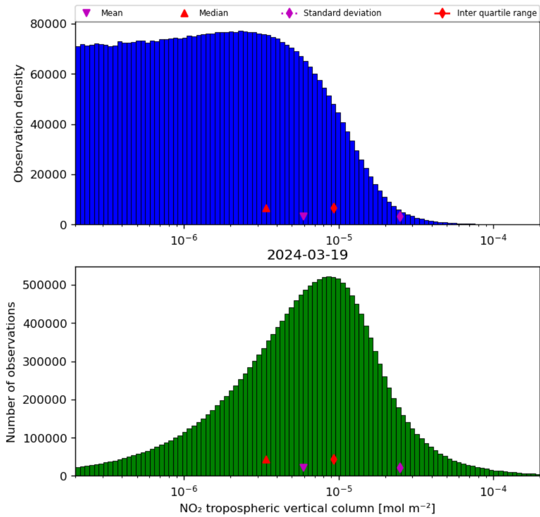
Figure 29: Histogram of “NO 2 tropospheric vertical column” for 2024-03-18 to 2024-03-20
