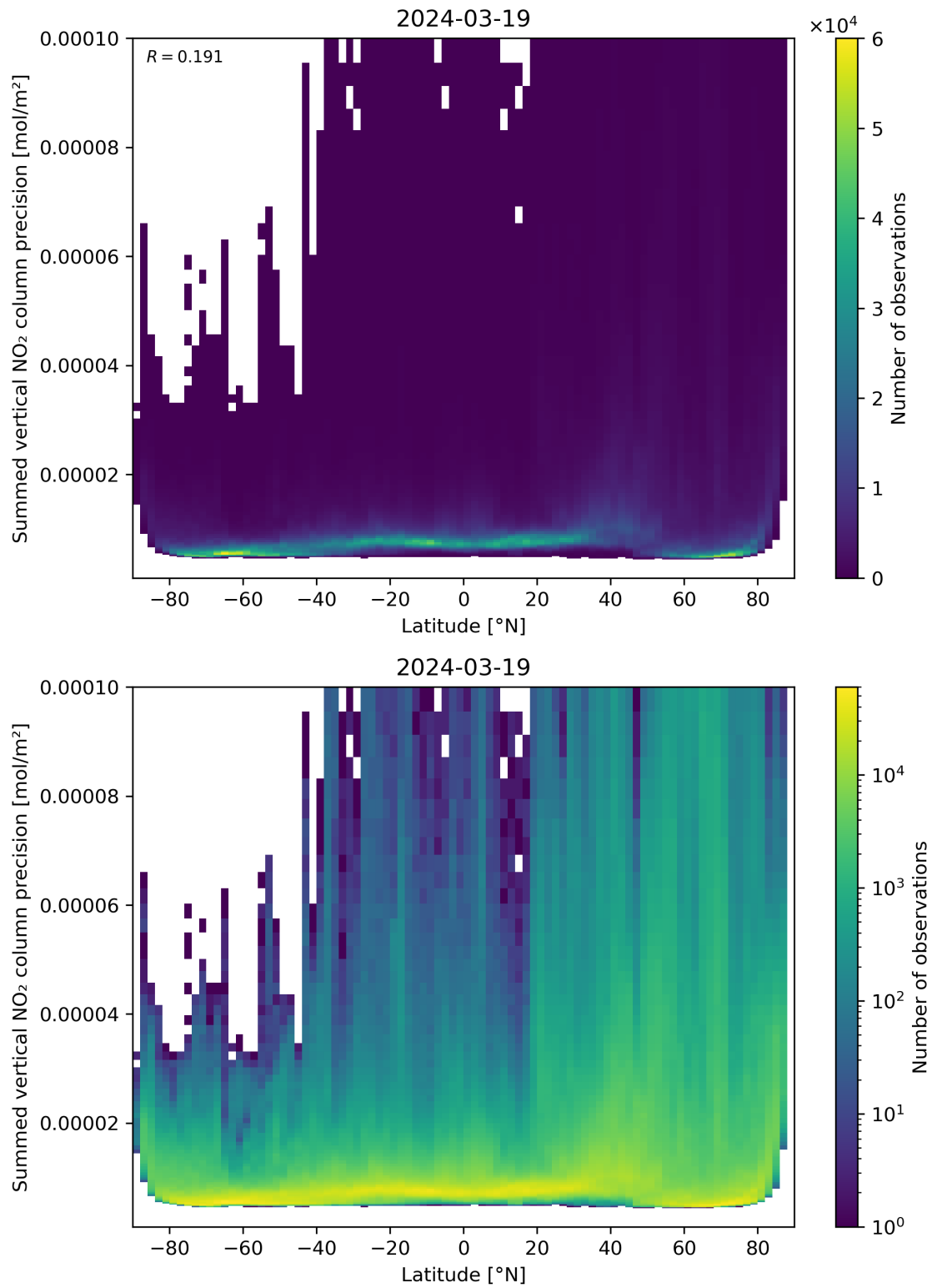
Figure 89: Scatter density plot of “Latitude” against “Summed vertical NO 2 column precision” for 2024-03-18 to 2024-03-20.
