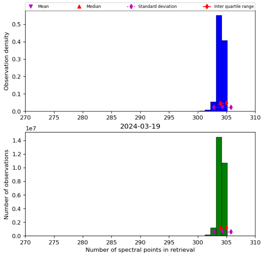
Figure 33: Histogram of “Number of spectral points in retrieval” for 2024-03-18 to 2024-03-20
