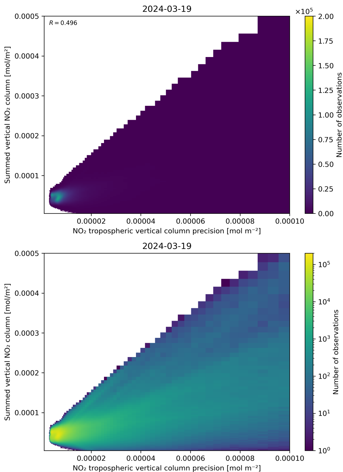
Figure 136: Scatter density plot of “NO 2 tropospheric vertical column precision” against “Summed vertical NO 2 column” for 2024-03-18 to 2024-03-20.
