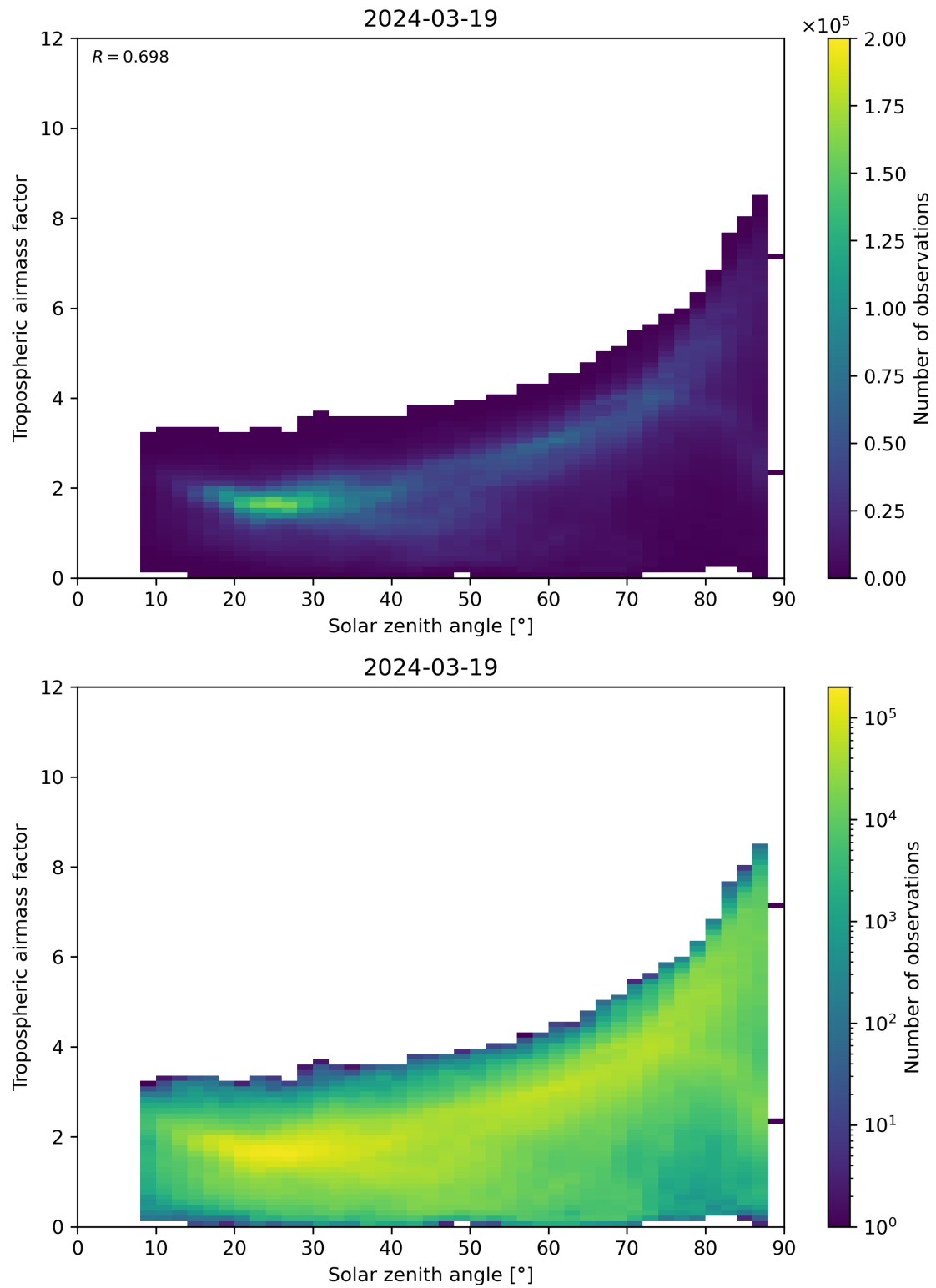
Figure 147: Scatter density plot of “Solar zenith angle” against “Tropospheric airmass factor” for 2024-03-18 to 2024-03-20.
