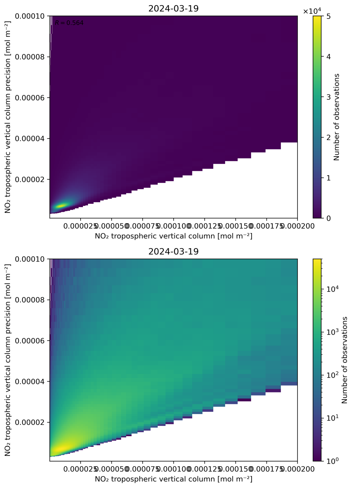
Figure 130: Scatter density plot of “NO 2 tropospheric vertical column” against “NO 2 tropospheric vertical column precision” for 2024-03-18 to 2024-03-20.
