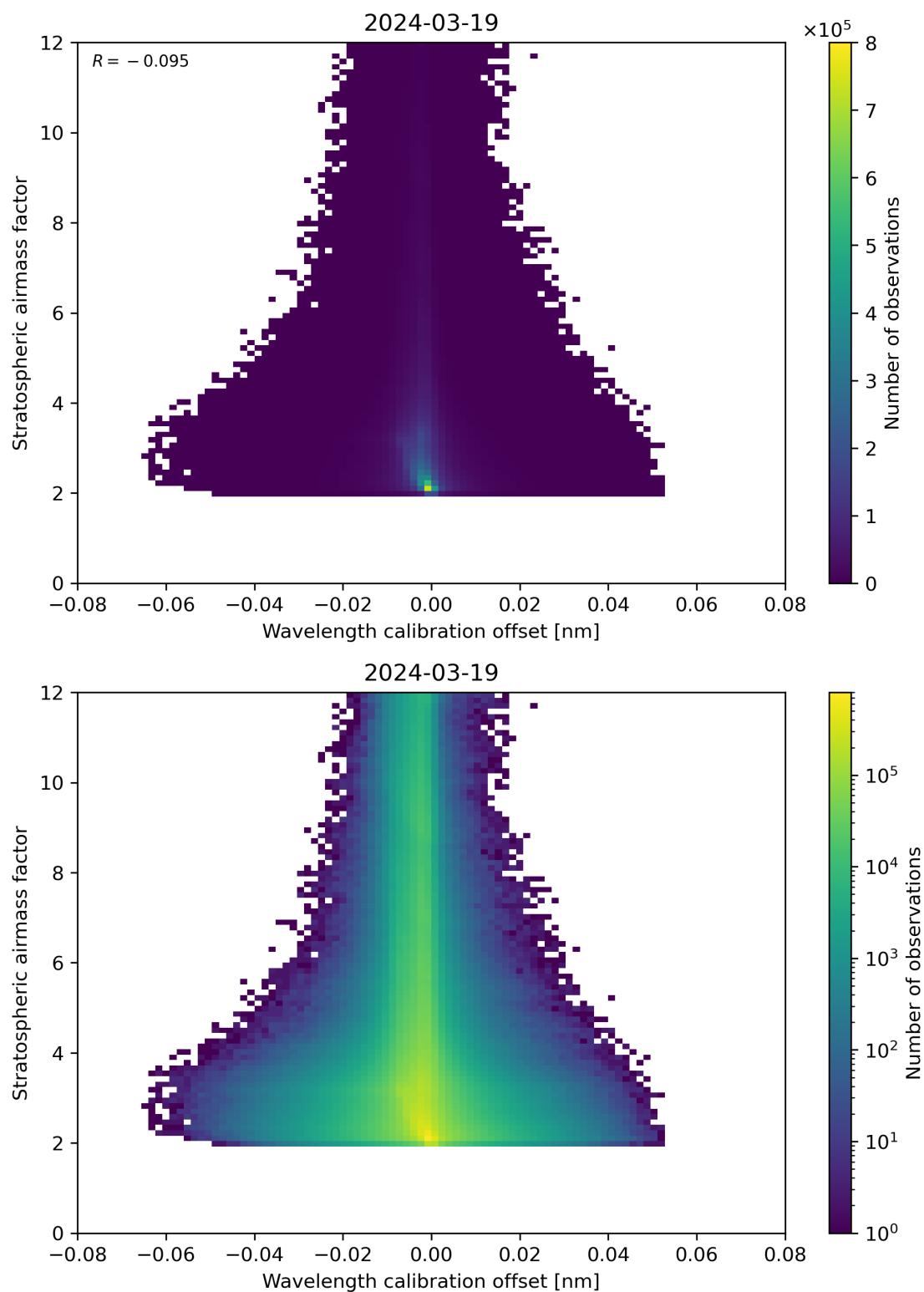
Figure 174: Scatter density plot of “Wavelength calibration offset” against “Stratospheric air mass factor” for 2024-03-18 to 2024-03-20.
