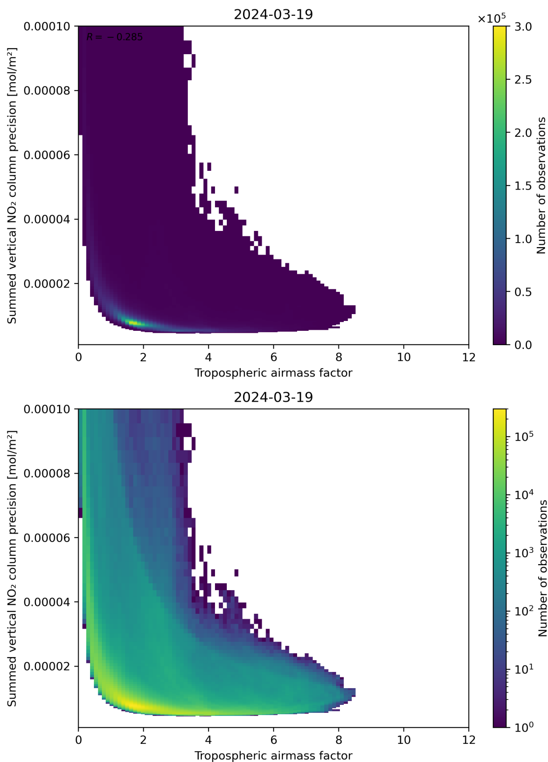
Figure 76: Scatter density plot of “Tropospheric air mass factor” against “Summed vertical NO 2 column precision” for 2024-03-18 to 2024-03-20.
