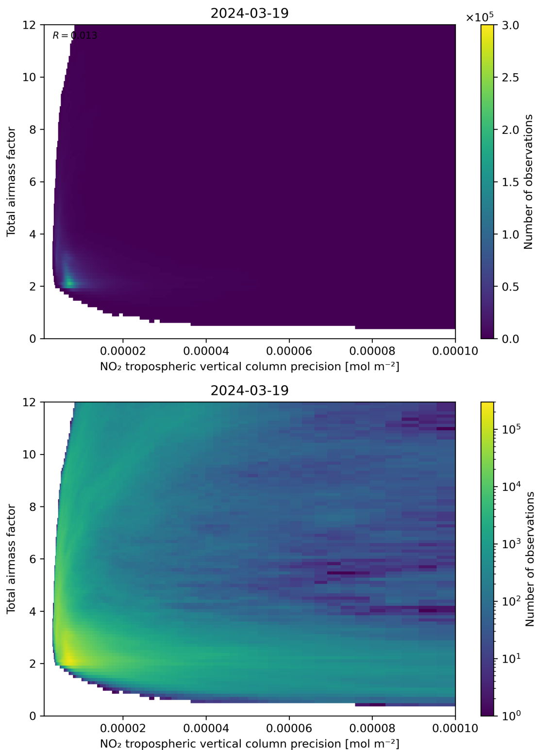
Figure 132: Scatter density plot of “NO 2 tropospheric vertical column precision” against “Total airmass factor” for 2024-03-18 to 2024-03-20.
