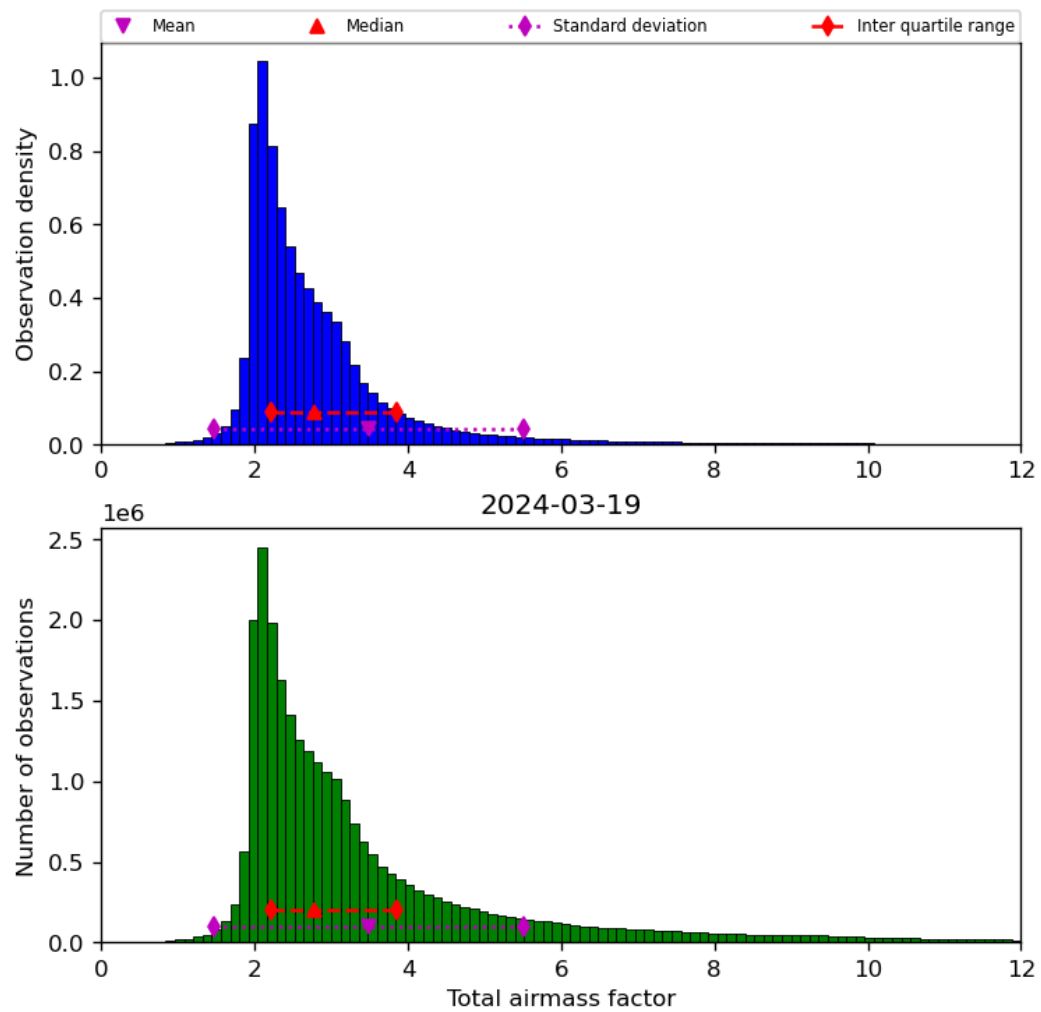
Figure 32: Histogram of “Total airmass factor” for 2024-03-18 to 2024-03-20
