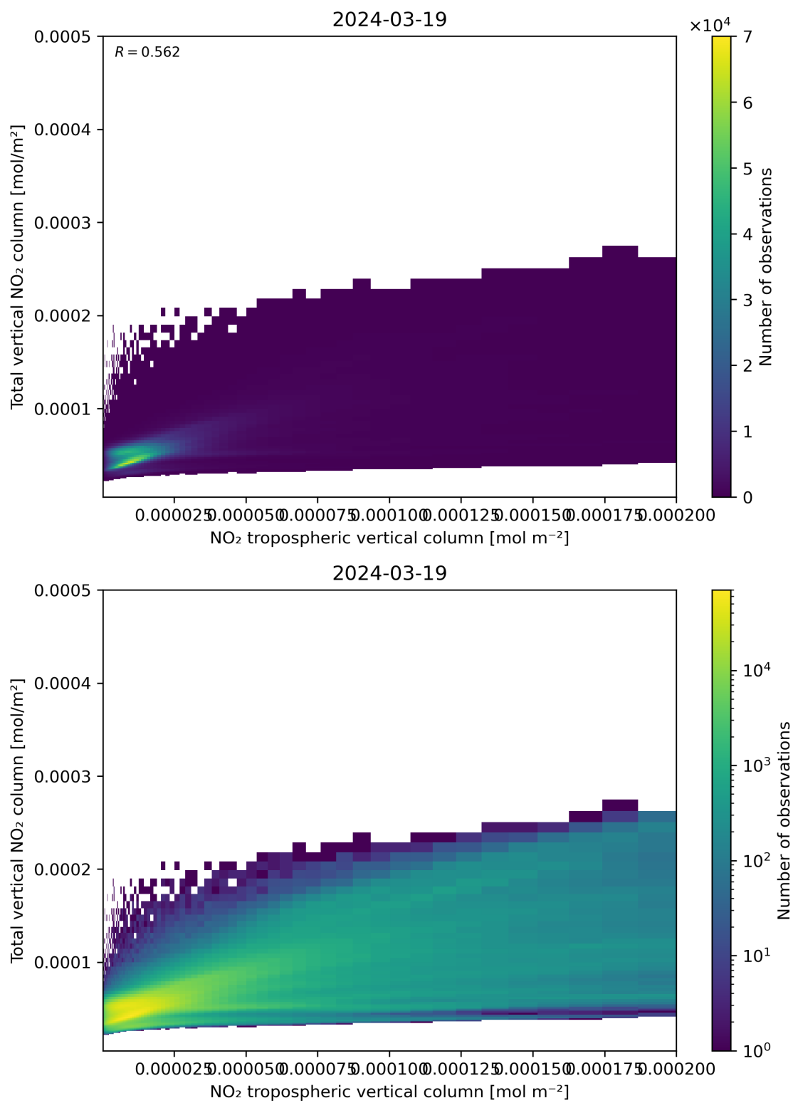
Figure 128: Scatter density plot of “NO 2 tropospheric vertical column” against “Total vertical NO 2 column” for 2024-03-18 to 2024-03-20.
