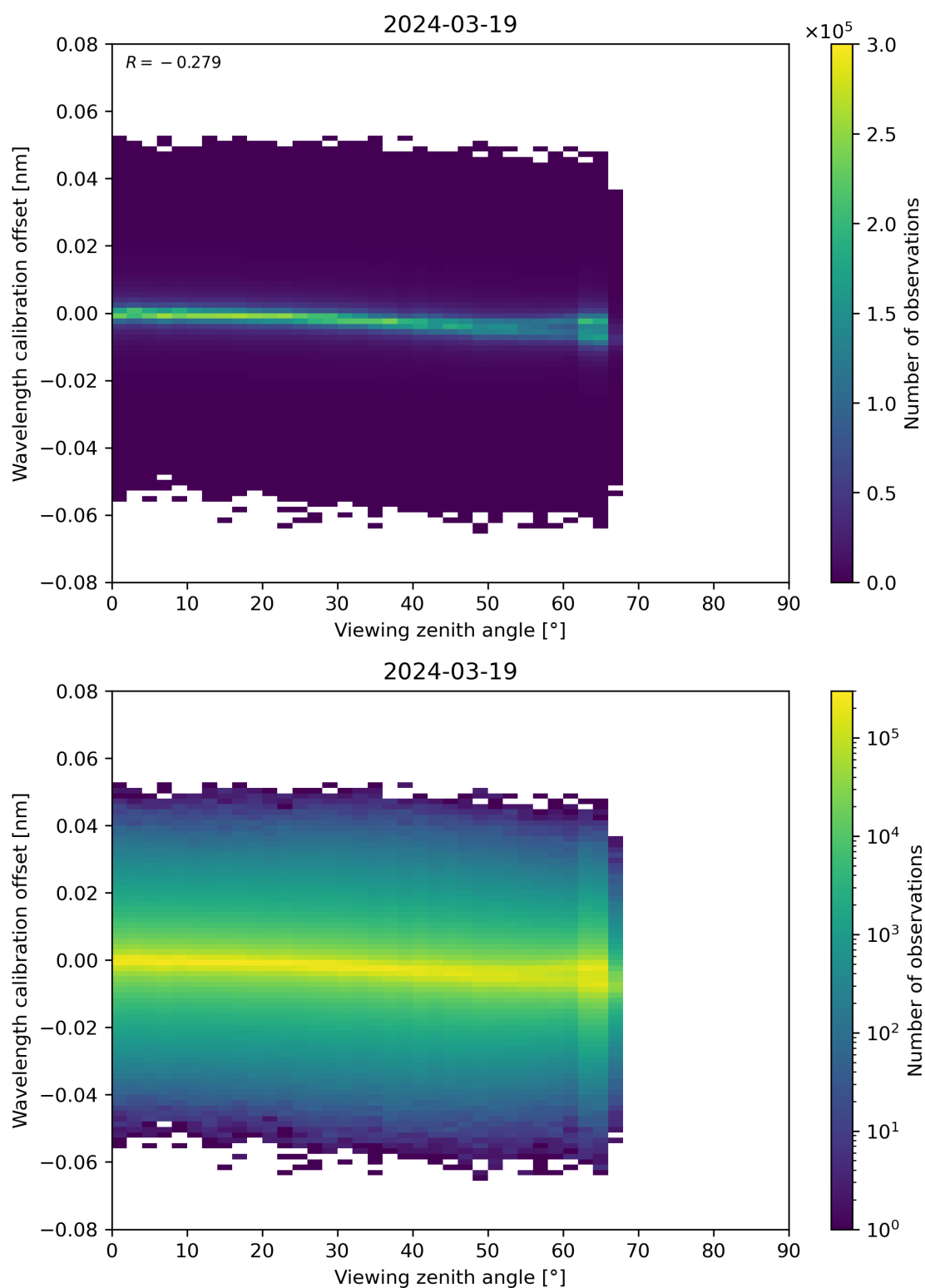
Figure 173: Scatter density plot of “Viewing zenith angle” against “Wavelength calibration offset” for 2024-03-18 to 2024-03-20.
