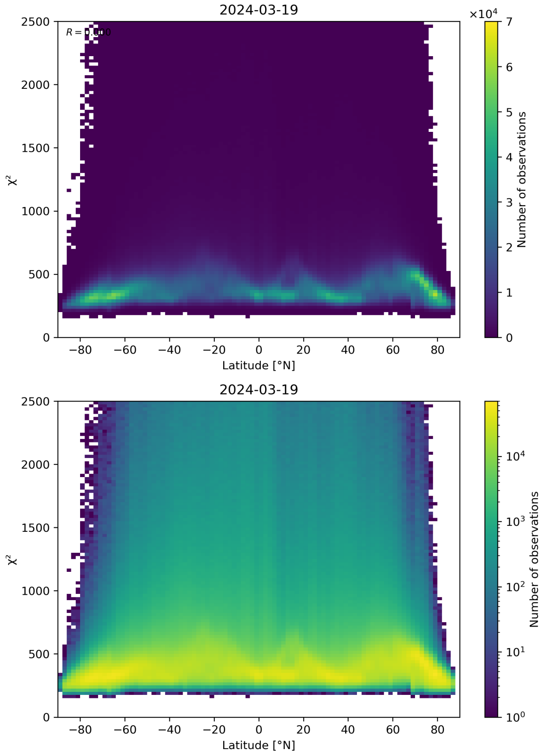
Figure 86: Scatter density plot of “Latitude” against “ \chi^2 ” for 2024-03-18 to 2024-03-20.
