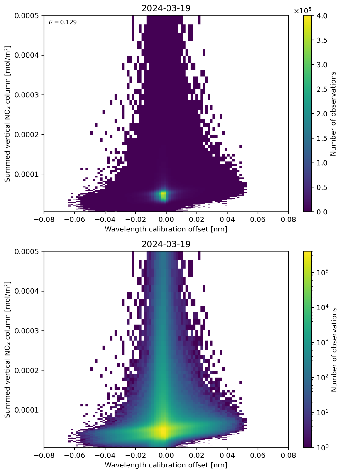
Figure 177: Scatter density plot of “Wavelength calibration offset” against “Summed vertical NO 2 column” for 2024-03-18 to 2024-03-20.
