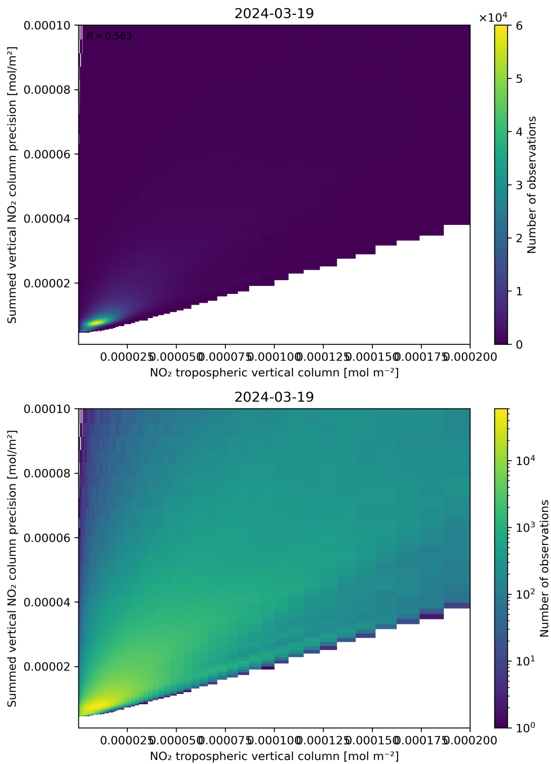
Figure 127: Scatter density plot of “NO 2 tropospheric vertical column” against “Summed vertical NO 2 column precision” for 2024-03-18 to 2024-03-20.
