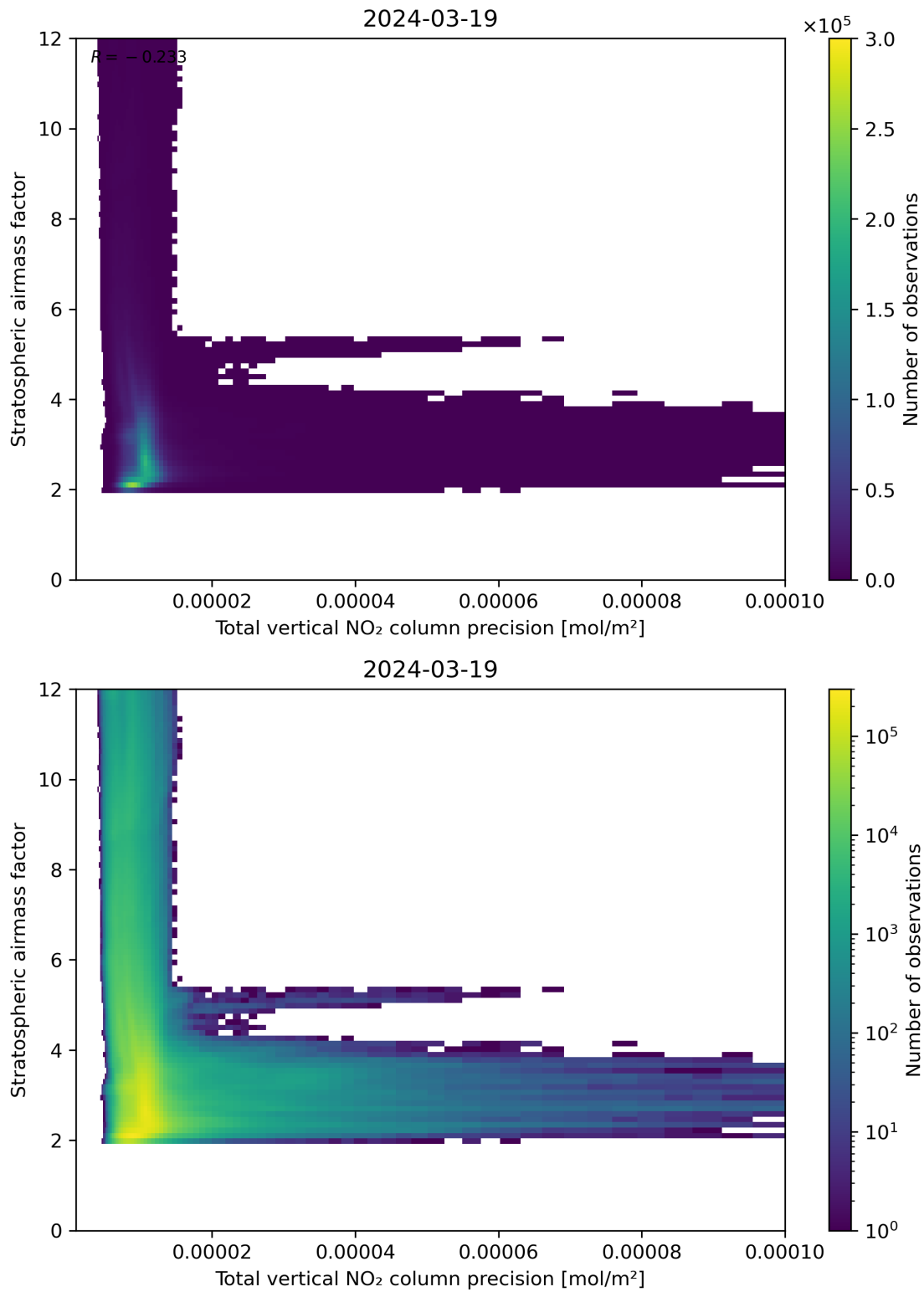
Figure 115: Scatter density plot of “Total vertical NO 2 column precision” against “Stratospheric air mass factor” for 2024-03-18 to 2024-03-20.
