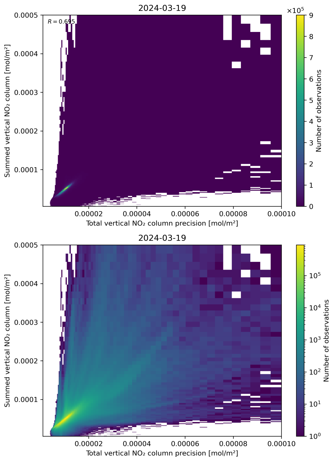
Figure 117: Scatter density plot of “Total vertical NO 2 column precision” against “Summed vertical NO 2 column” for 2024-03-18 to 2024-03-20.
