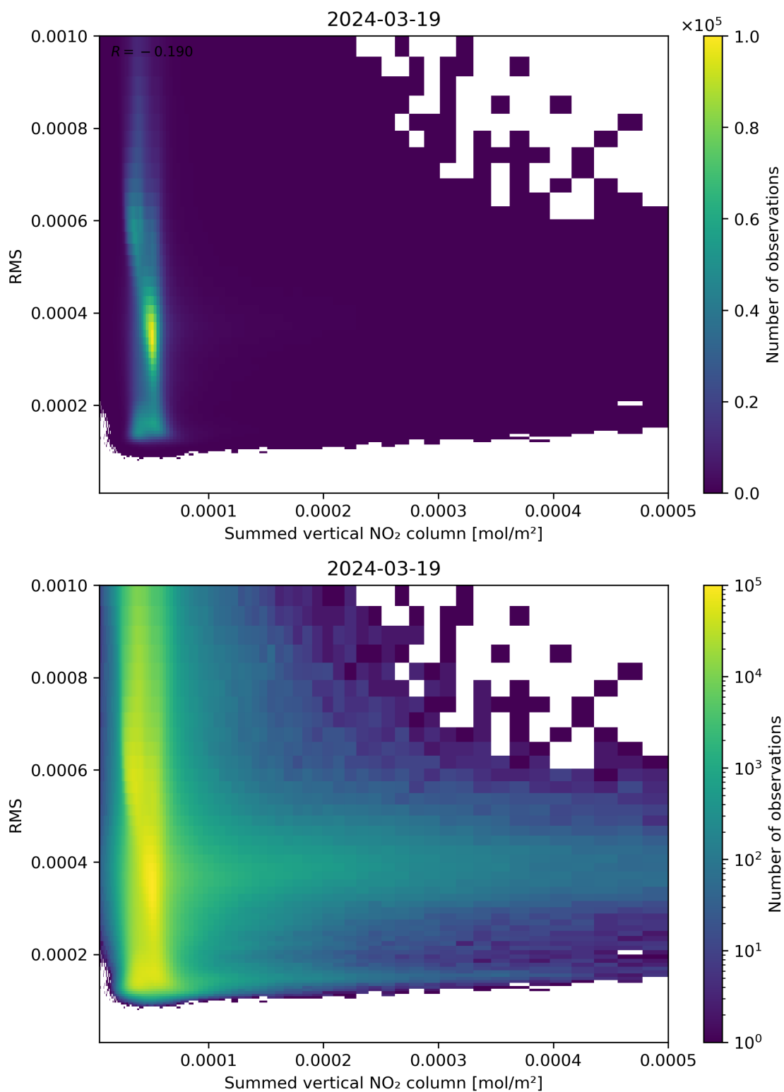
Figure 109: Scatter density plot of “Summed vertical NO 2 column” against “RMS” for 2024-03-18 to 2024-03-20.
