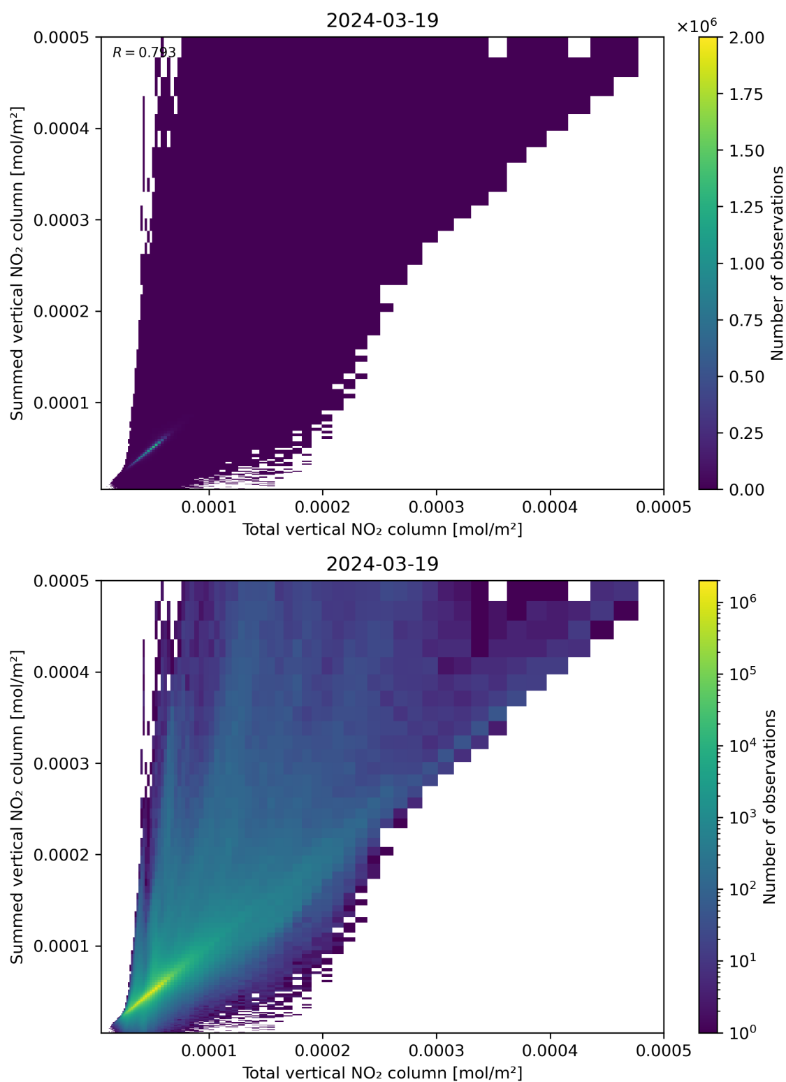
Figure 112: Scatter density plot of “Total vertical NO 2 column” against “Summed vertical NO 2 column” for 2024-03-18 to 2024-03-20.
