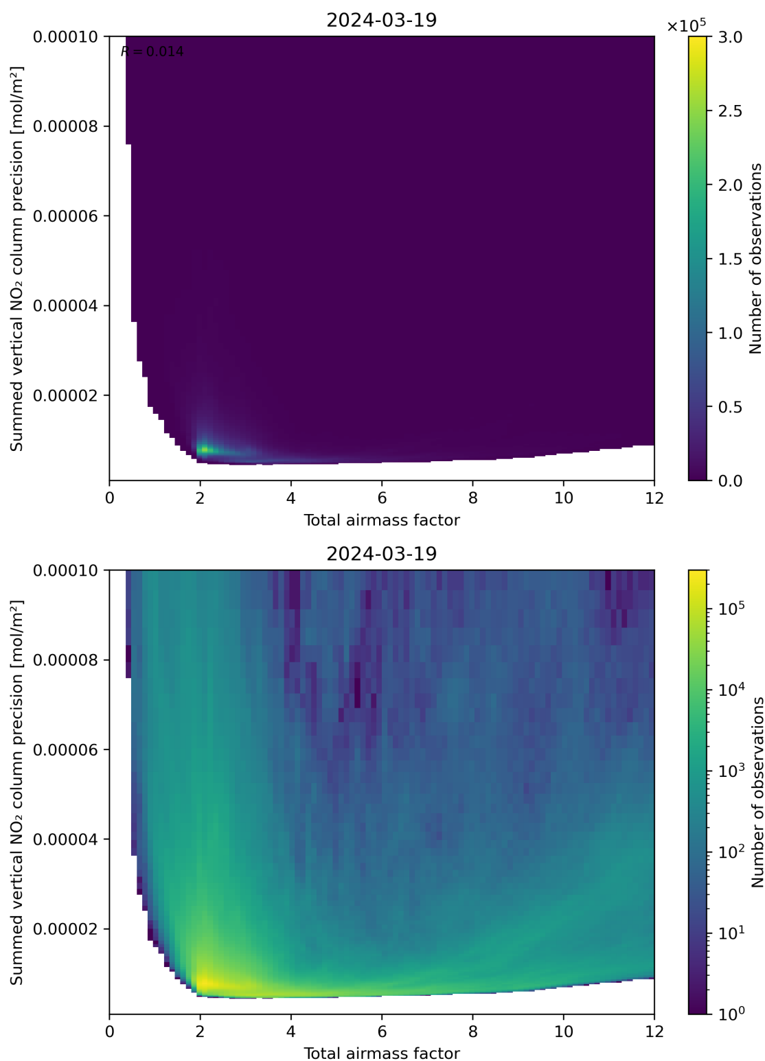
Figure 66: Scatter density plot of “Total airmass factor” against “Summed vertical NO 2 column precision” for 2024-03-18 to 2024-03-20.
