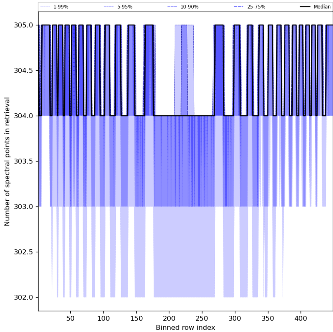
Figure 50: Along track statistics of “Number of spectral points in retrieval” for 2024-03-18 to 2024-03-20
