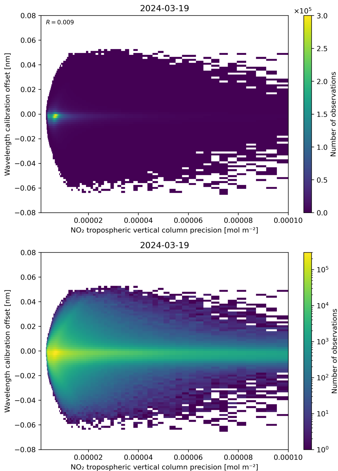
Figure 141: Scatter density plot of “NO 2 tropospheric vertical column precision” against “Wavelength calibration offset” for 2024-03-18 to 2024-03-20.
