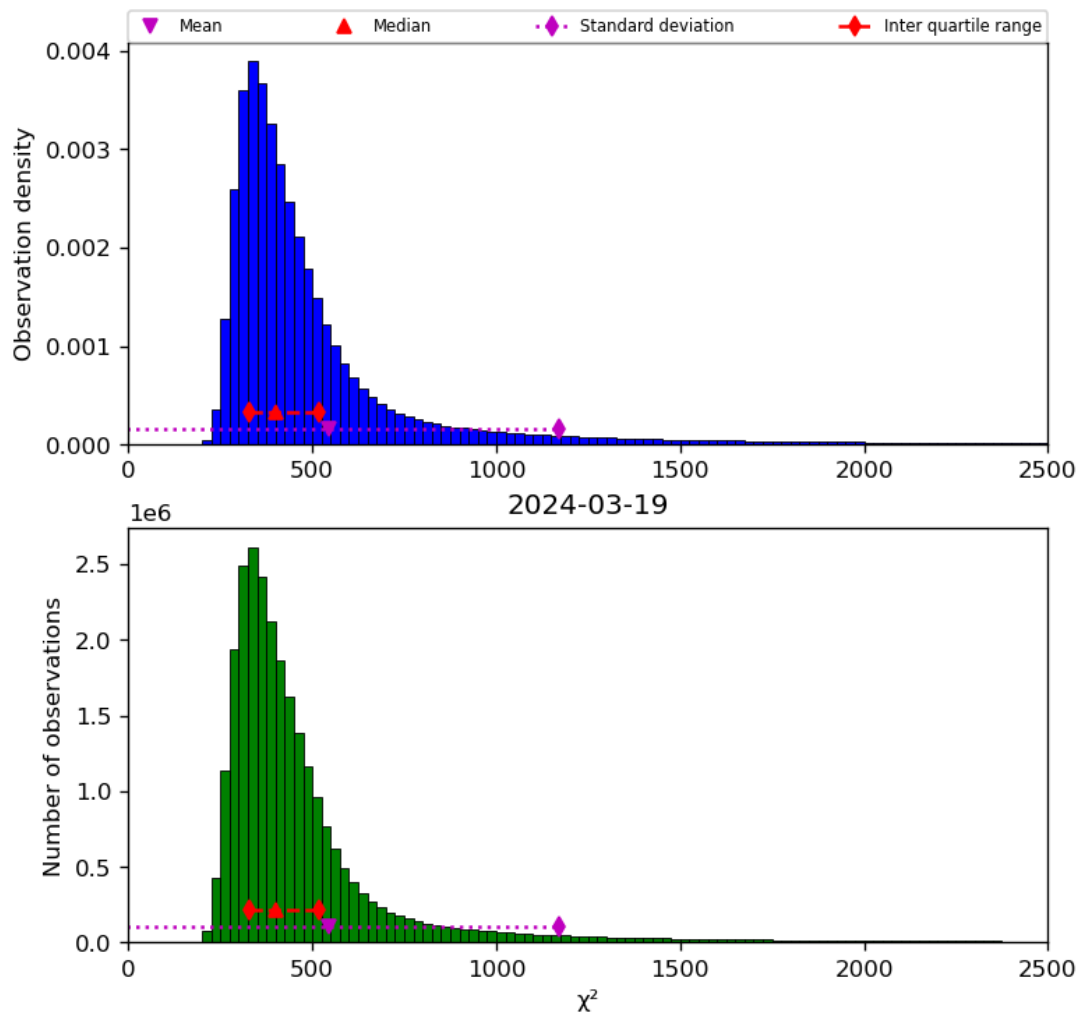
Figure 42: Histogram of “ \chi^2 ” for 2024-03-18 to 2024-03-20
