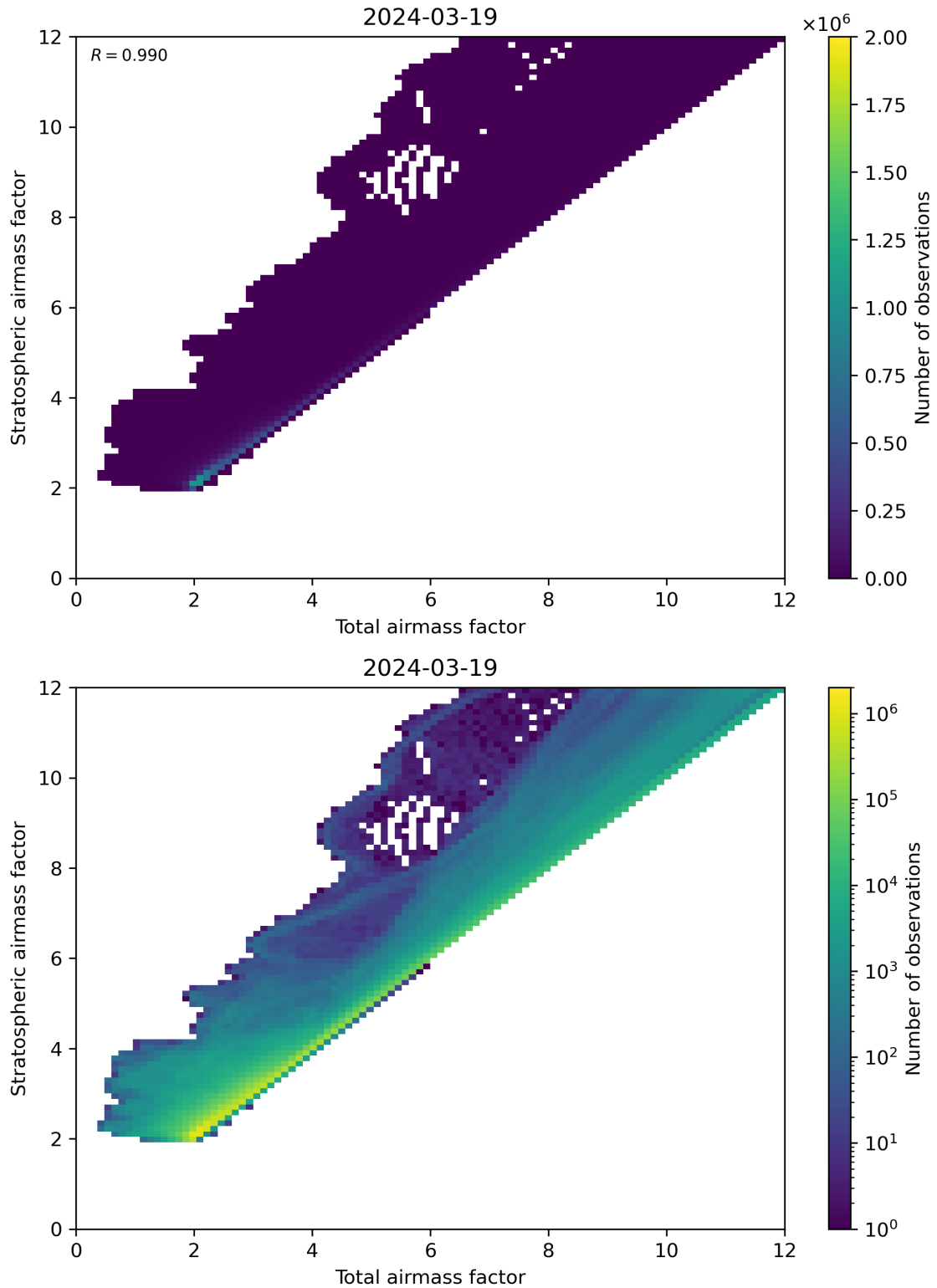
Figure 62: Scatter density plot of “Total airmass factor” against “Stratospheric airmass factor” for 2024-03-18 to 2024-03-20.
