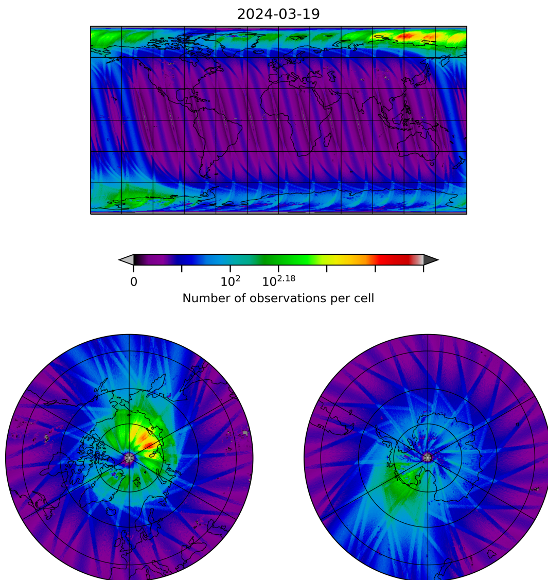
Figure 10: Map of the number of observations for 2024-03-18 to 2024-03-20
