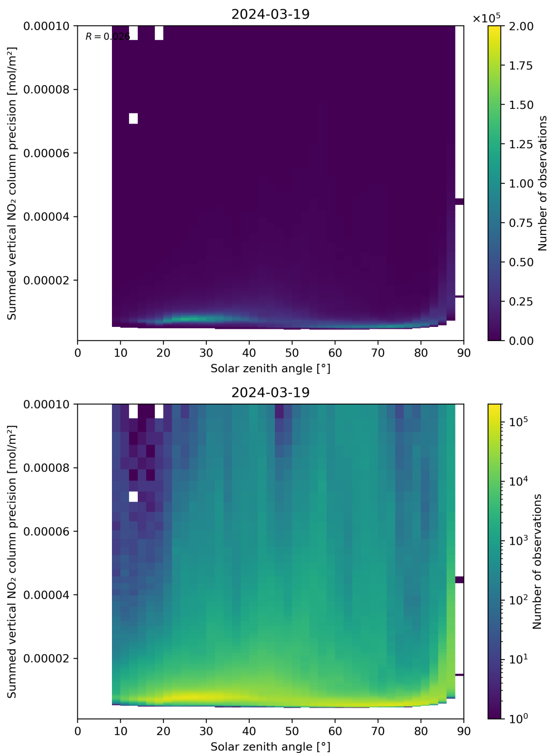
Figure 152: Scatter density plot of “Solar zenith angle” against “Summed vertical NO 2 column precision” for 2024-03-18 to 2024-03-20.
