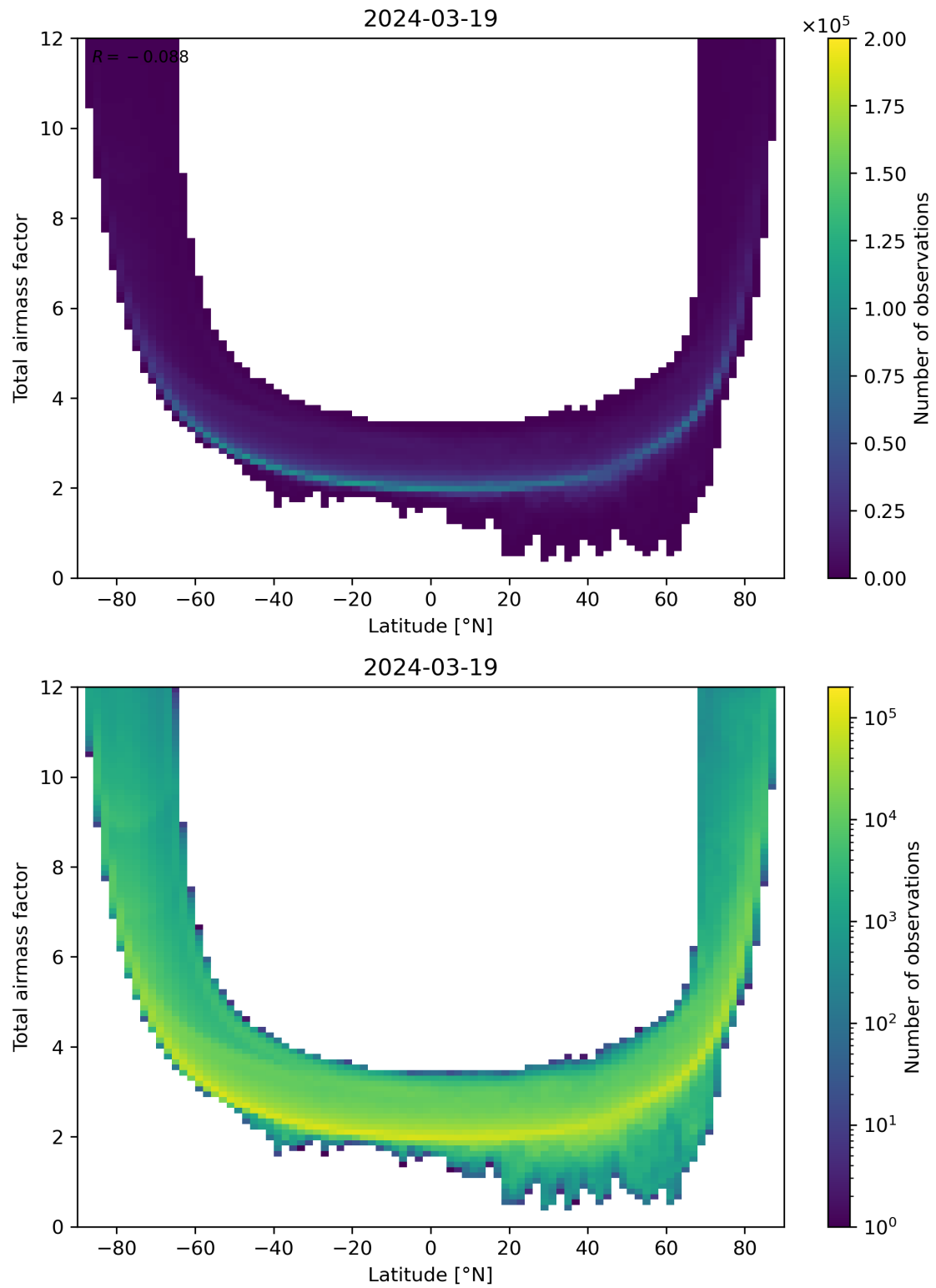
Figure 84: Scatter density plot of “Latitude” against “Total airmass factor” for 2024-03-18 to 2024-03-20.
