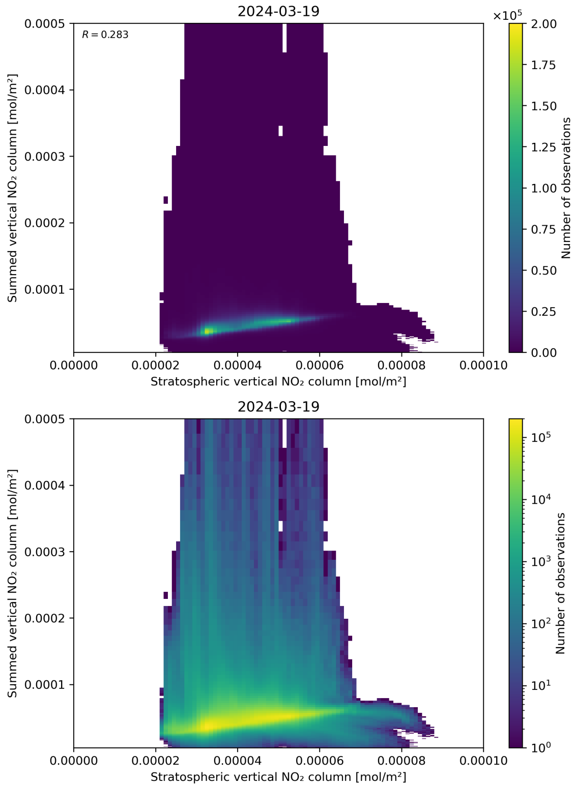
Figure 98: Scatter density plot of “Stratospheric vertical NO 2 column” against “Summed vertical NO 2 column” for 2024-03-18 to 2024-03-20.
