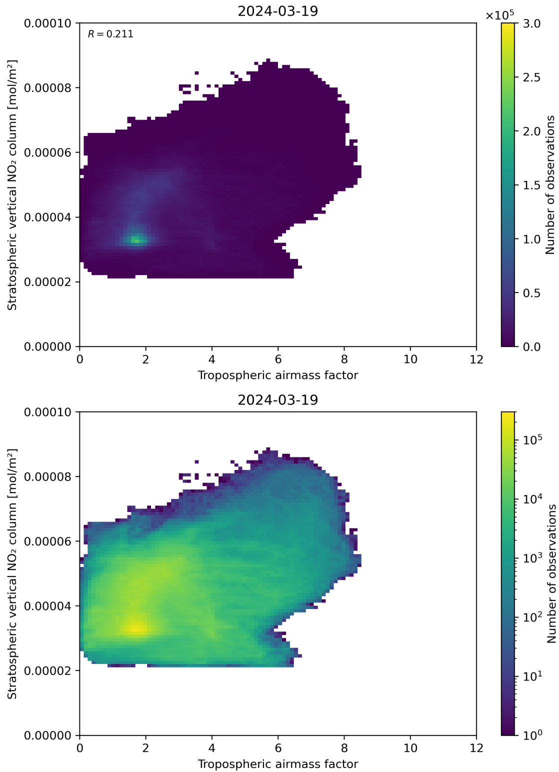
Figure 74: Scatter density plot of “Tropospheric airmass factor” against “Stratospheric vertical NO 2 column” for 2024-03-18 to 2024-03-20.
