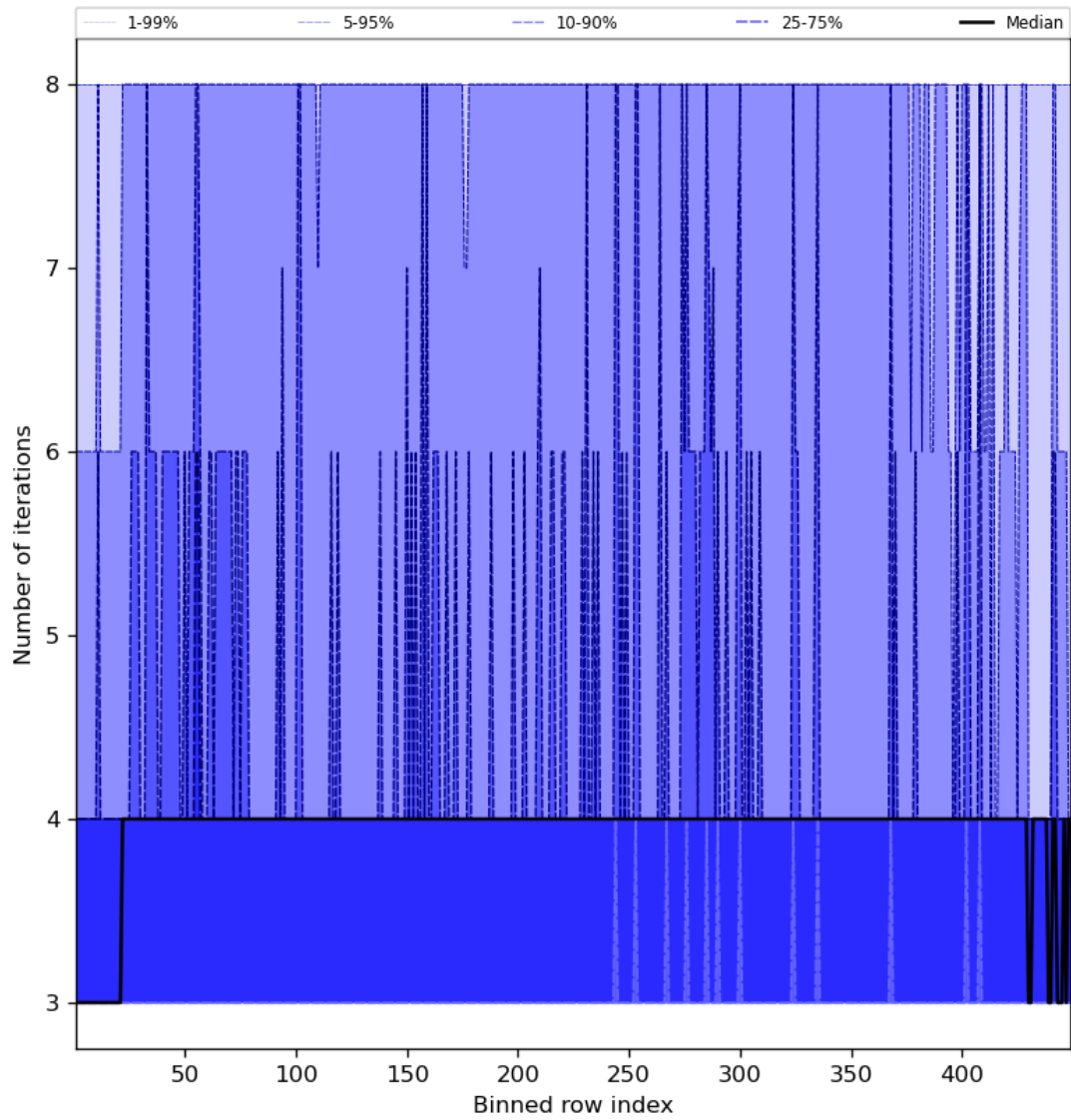
Figure 51: Along track statistics of “Number of iterations” for 2024-03-18 to 2024-03-20
