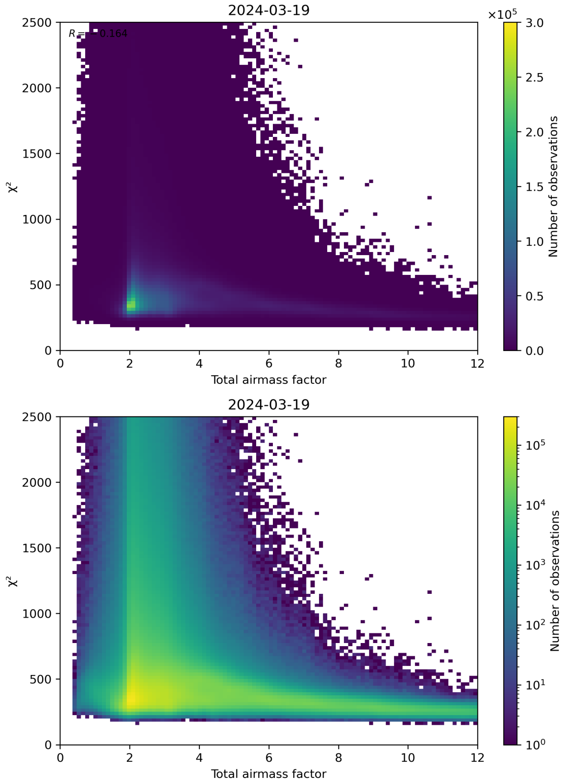
Figure 63: Scatter density plot of “Total airmass factor” against “ \chi^2 ” for 2024-03-18 to 2024-03-20.
