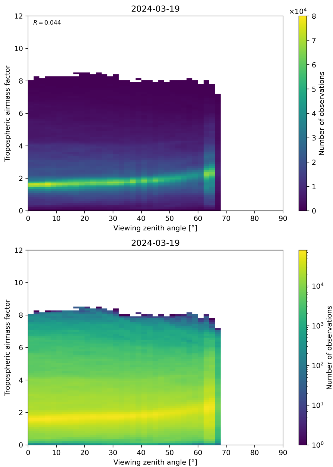
Figure 161: Scatter density plot of “Viewing zenith angle” against “Tropospheric airmass factor” for 2024-03-18 to 2024-03-20.
