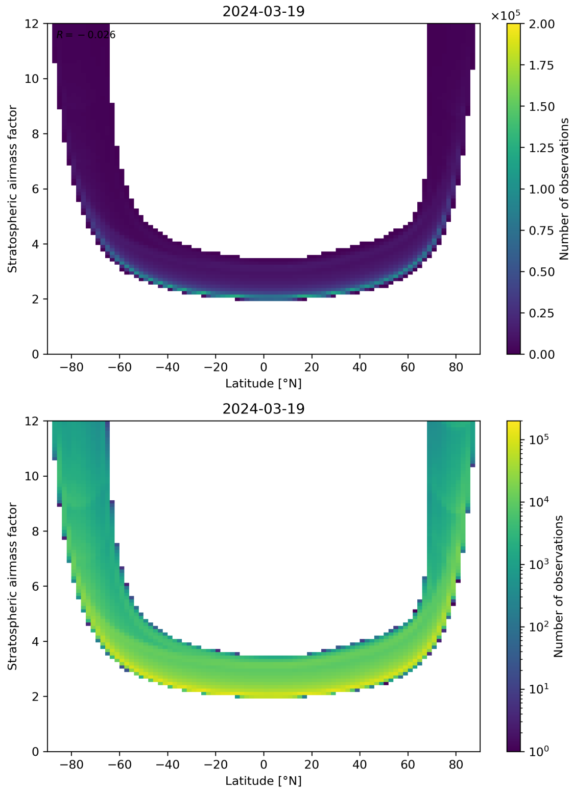
Figure 83: Scatter density plot of “Latitude” against “Stratospheric airmass factor” for 2024-03-18 to 2024-03-20.
