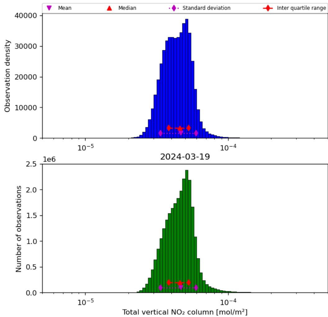
Figure 38: Histogram of "Total vertical NO 2 column" for 2024-03-18 to 2024-03-20
