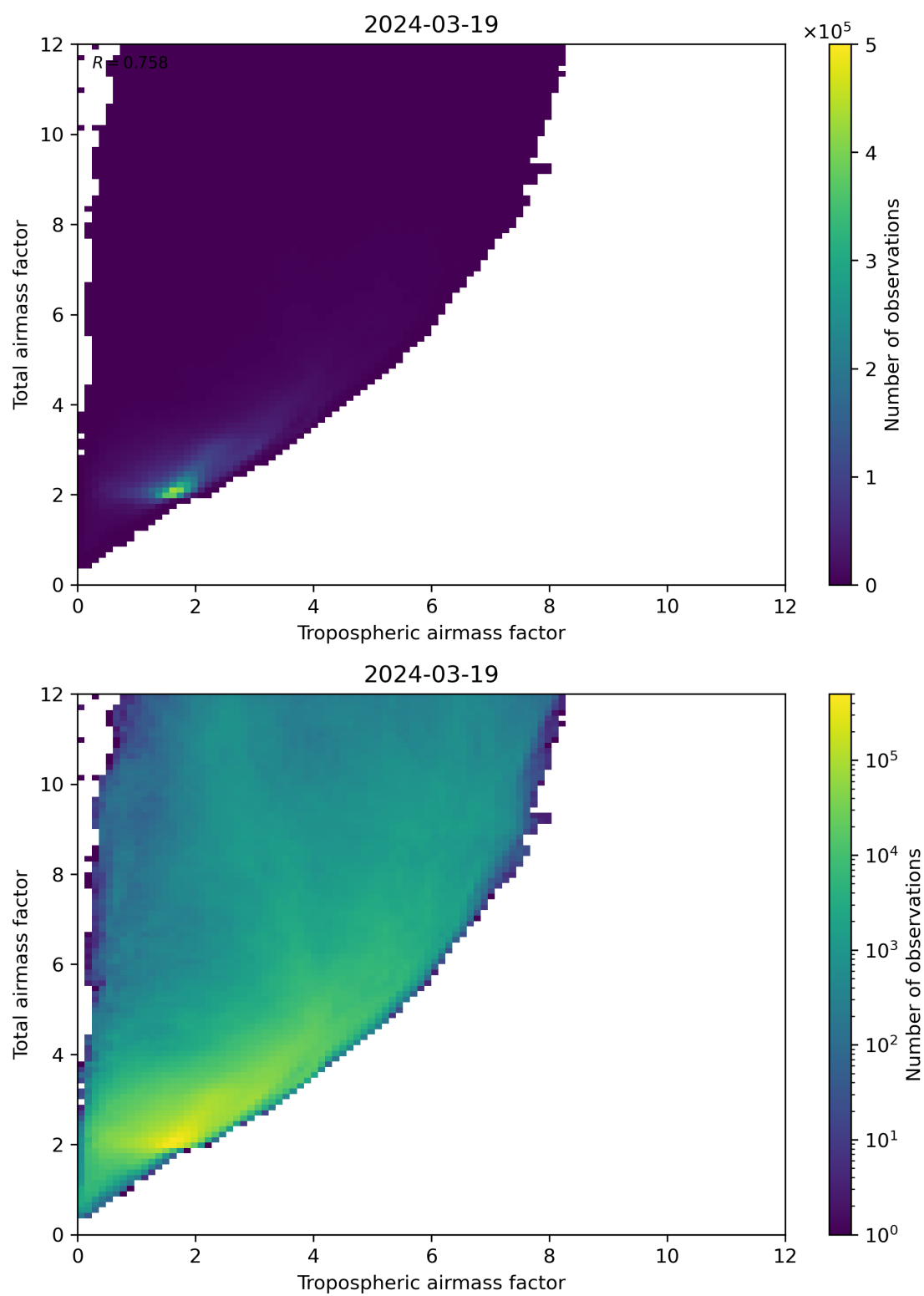
Figure 72: Scatter density plot of “Tropospheric airmass factor” against “Total airmass factor” for 2024-03-18 to 2024-03-20.
