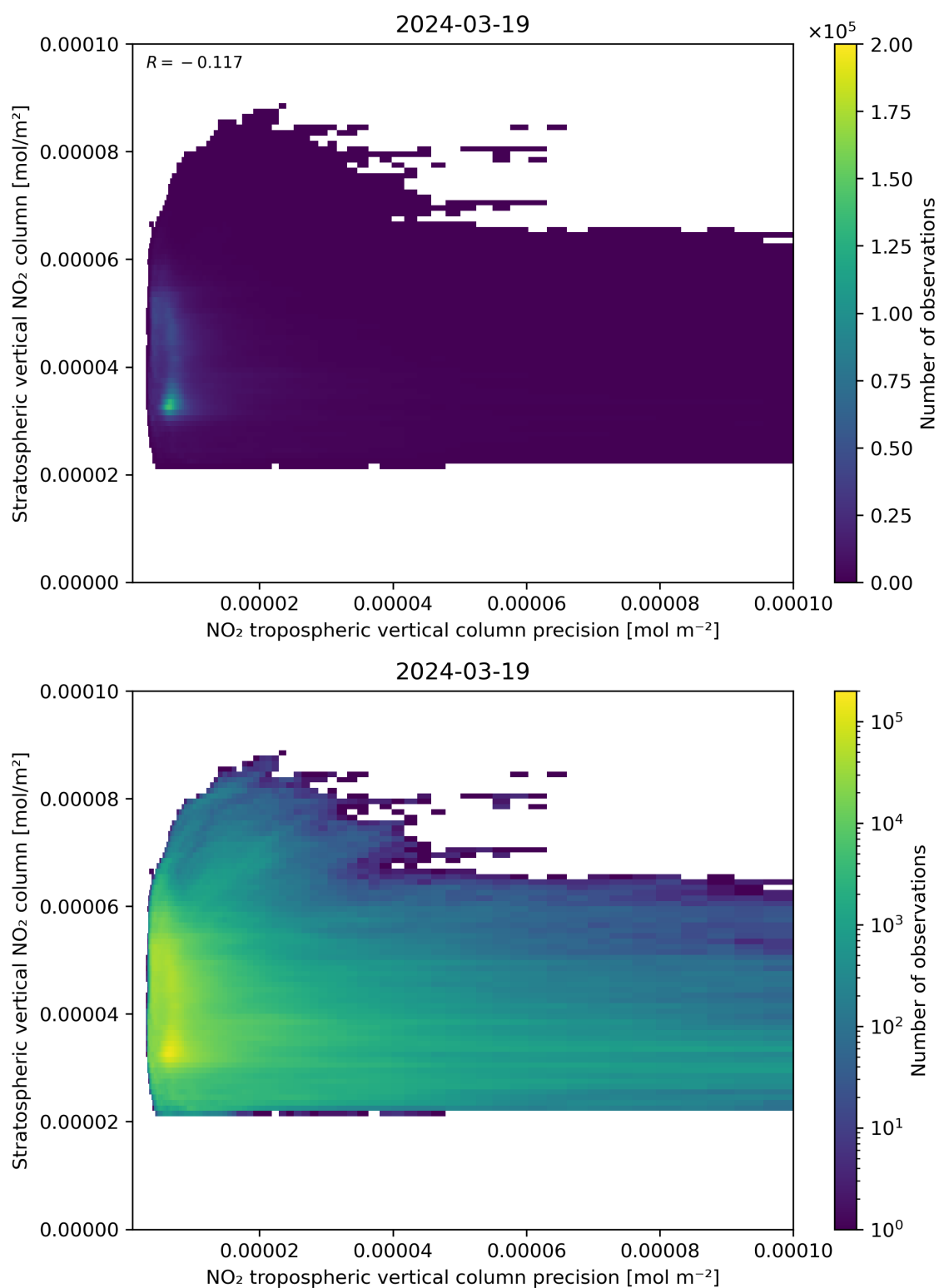
Figure 135: Scatter density plot of “NO 2 tropospheric vertical column precision” against “Stratospheric vertical NO 2 column” for 2024-03-18 to 2024-03-20.
