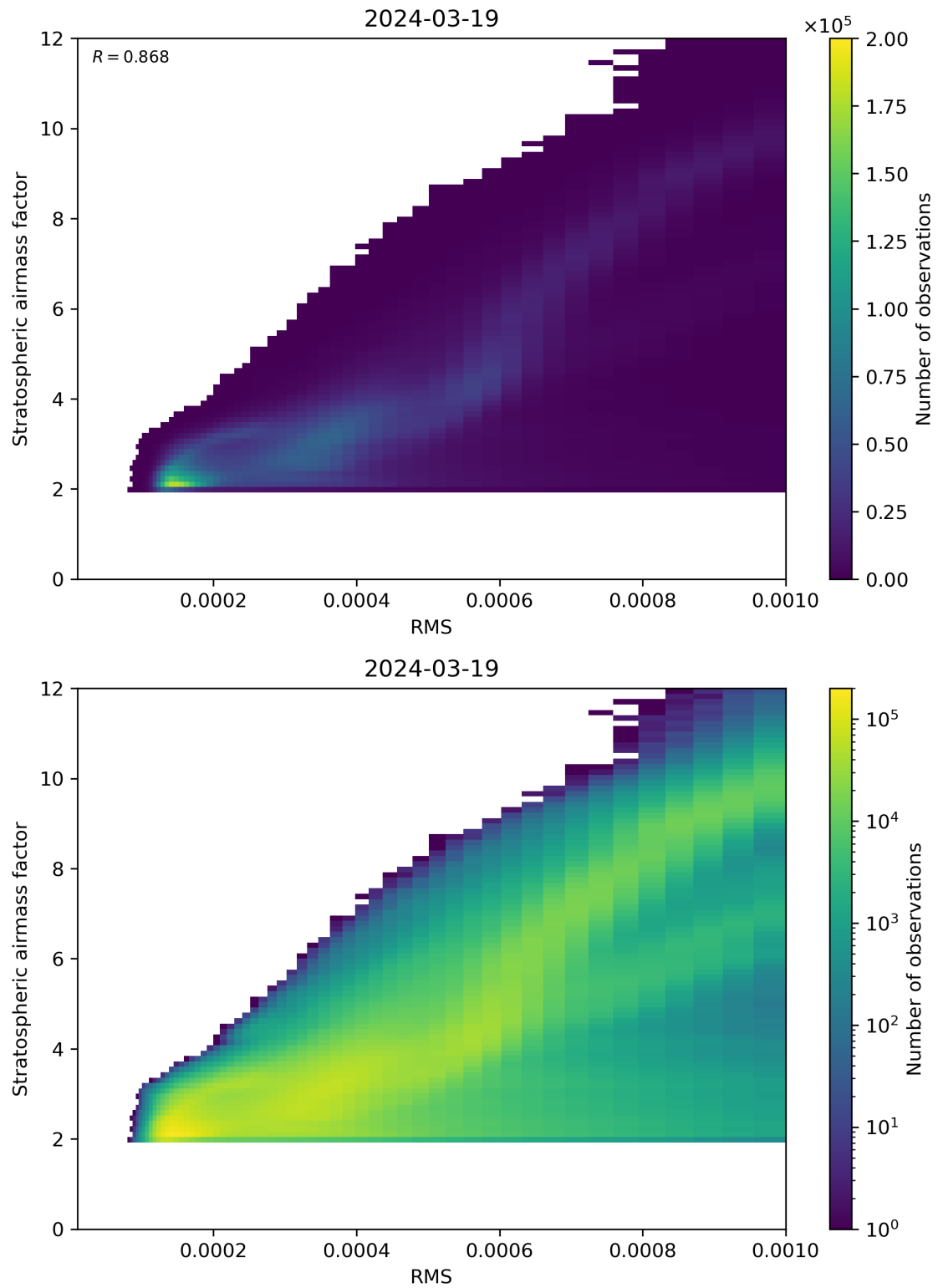
Figure 144: Scatter density plot of “RMS” against “Stratospheric airmass factor” for 2024-03-18 to 2024-03-20.
