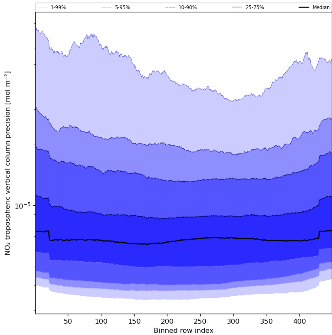
Figure 47: Along track statistics of “NO 2 tropospheric vertical column precision” for 2024-03-18 to 2024-03-20
