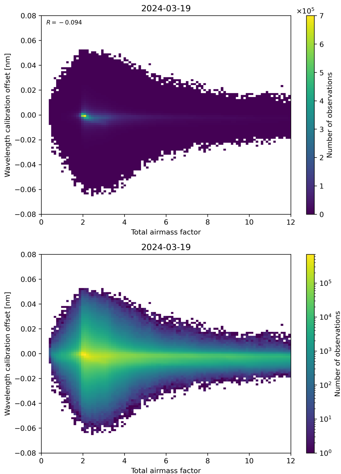
Figure 70: Scatter density plot of “Total airmass factor” against “Wavelength calibration offset” for 2024-03-18 to 2024-03-20.
