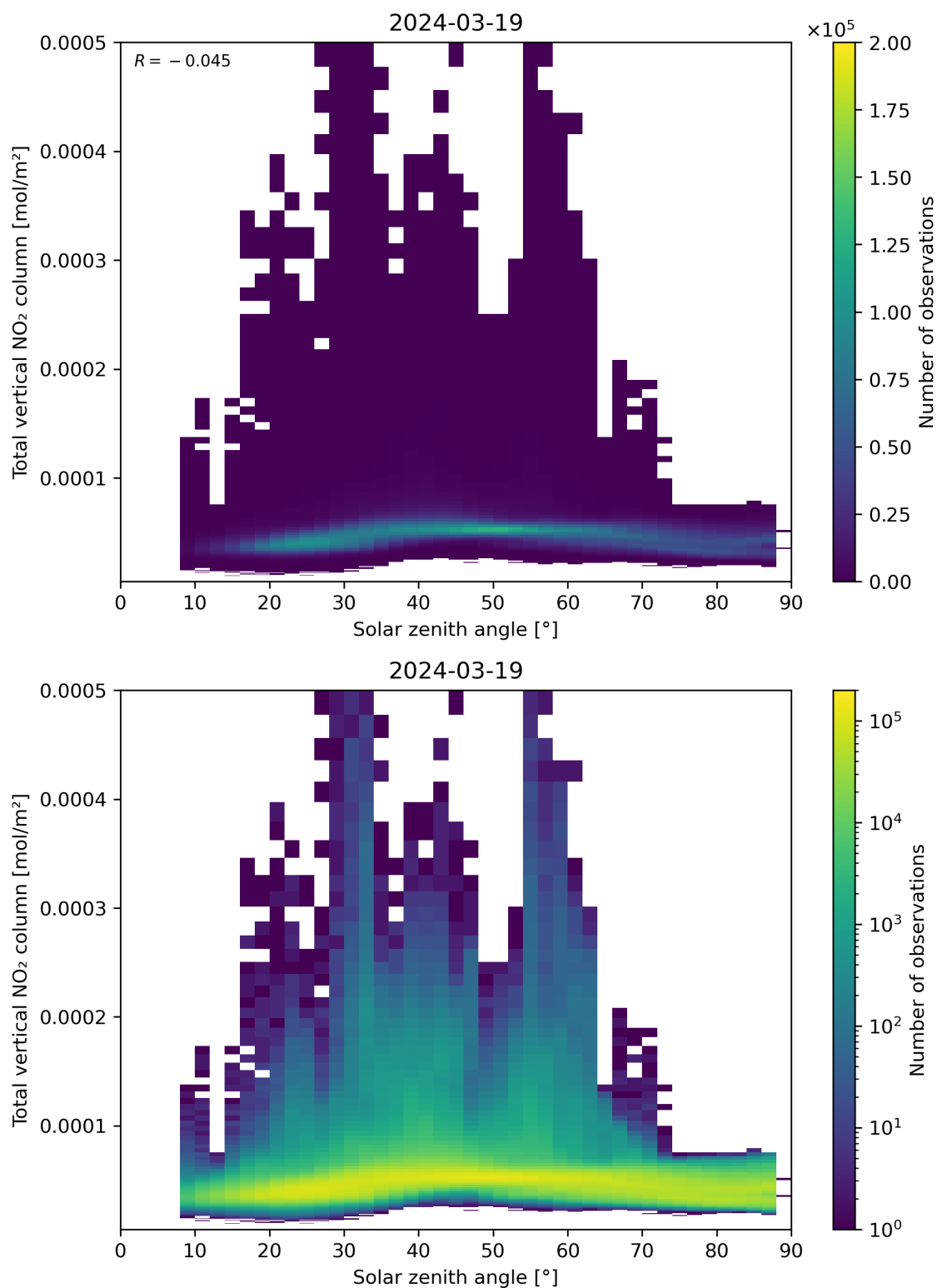
Figure 153: Scatter density plot of “Solar zenith angle” against “Total vertical NO 2 column” for 2024-03-18 to 2024-03-20.
