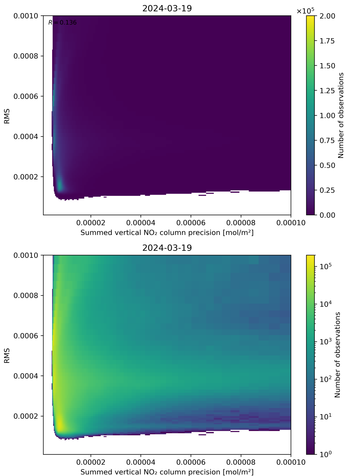
Figure 108: Scatter density plot of “Summed vertical NO 2 column precision” against “RMS” for 2024-03-18 to 2024-03-20.
