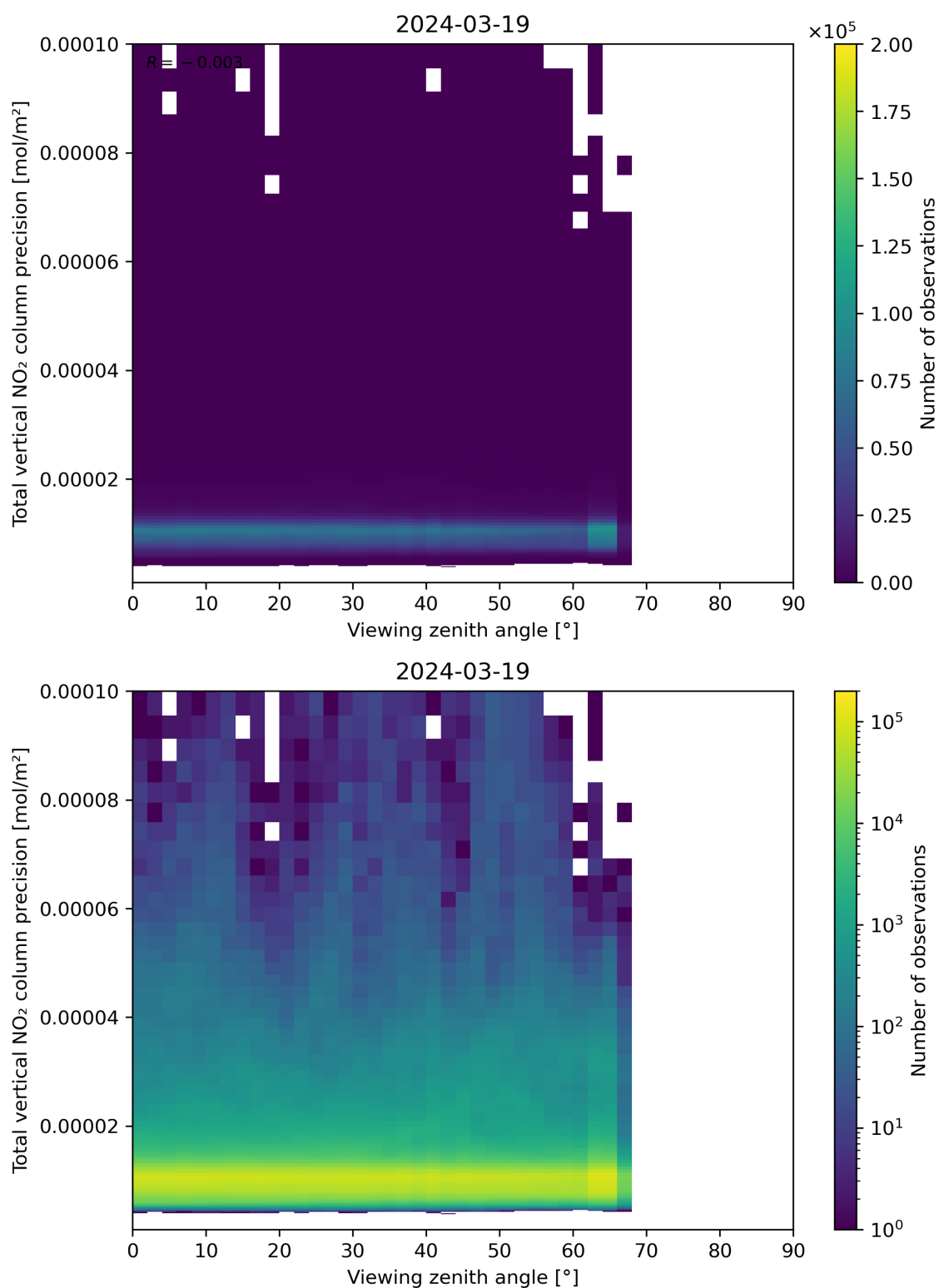
Figure 168: Scatter density plot of “Viewing zenith angle” against “Total vertical NO 2 column precision” for 2024-03-18 to 2024-03-20.
