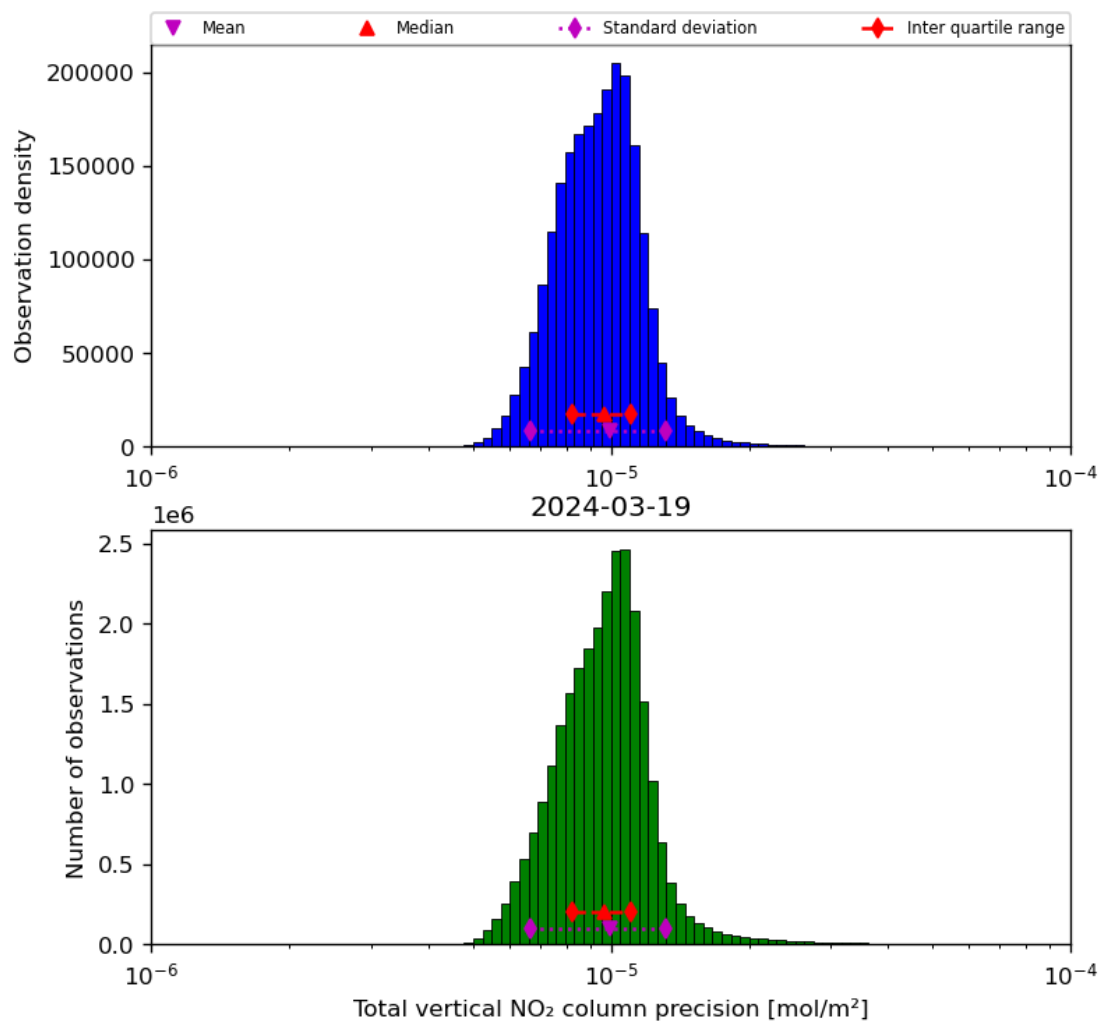
Figure 39: Histogram of “Total vertical NO 2 column precision” for 2024-03-18 to 2024-03-20
