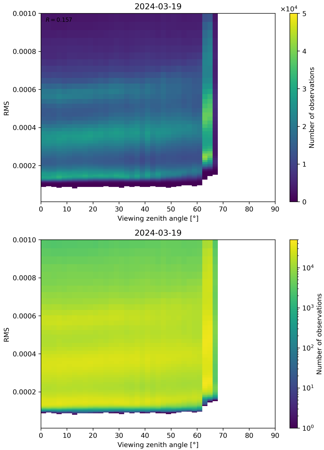
Figure 171: Scatter density plot of “Viewing zenith angle” against “RMS” for 2024-03-18 to 2024-03-20.
