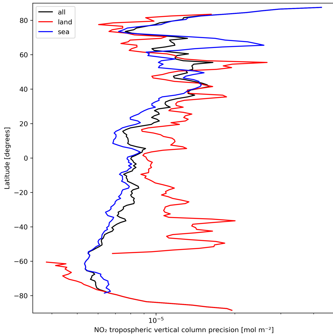
Figure 13: Zonal average of “NO 2 tropospheric vertical column precision” for 2024-03-18 to 2024-03-20.
