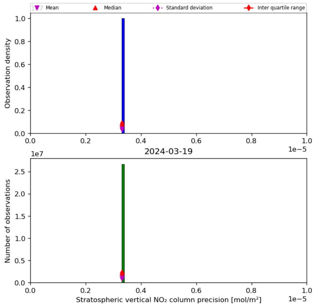
Figure 37: Histogram of “Stratospheric vertical NO 2 column precision” for 2024-03-18 to 2024-03-20
