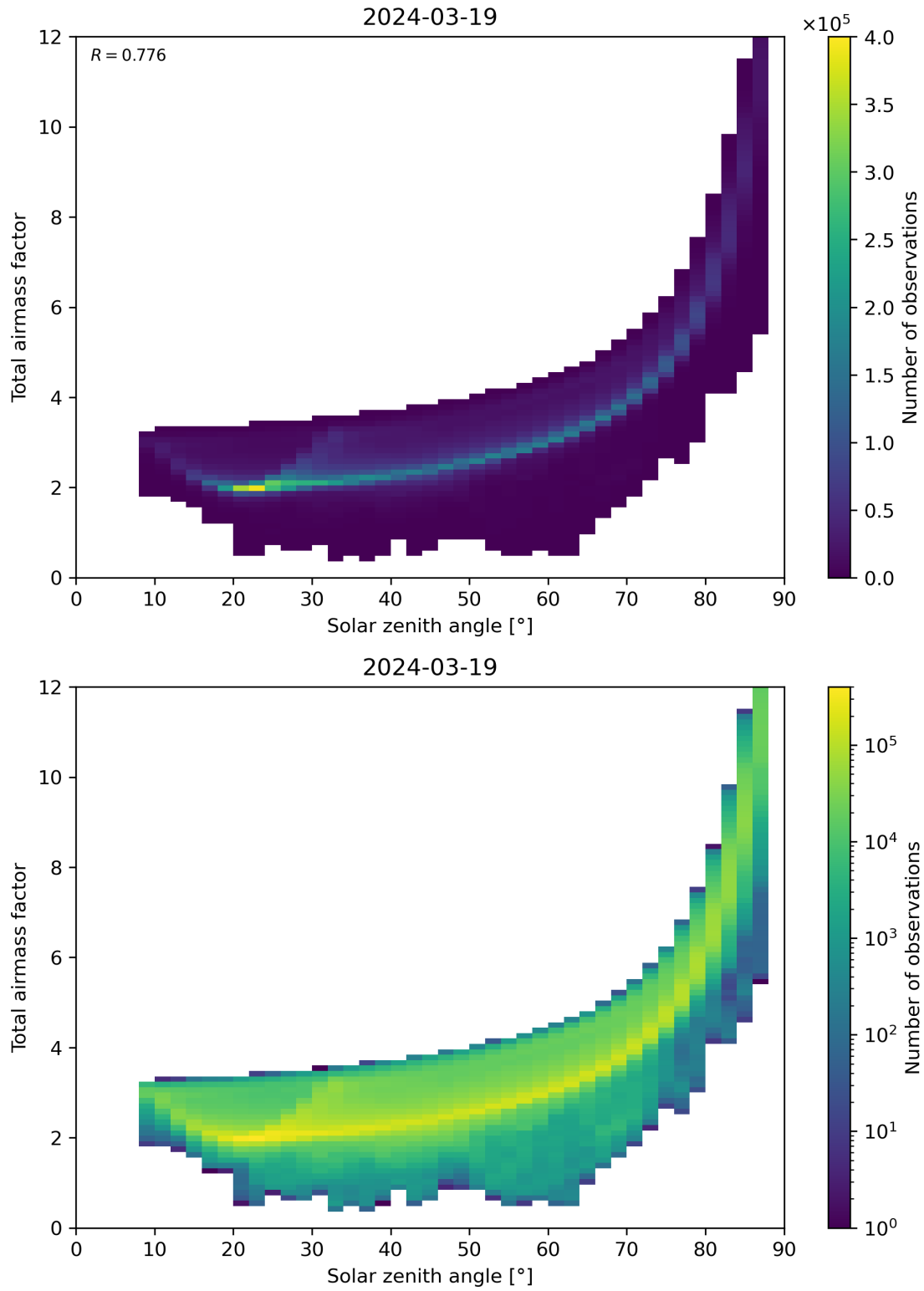
Figure 146: Scatter density plot of “Solar zenith angle” against “Total air mass factor” for 2024-03-18 to 2024-03-20.
