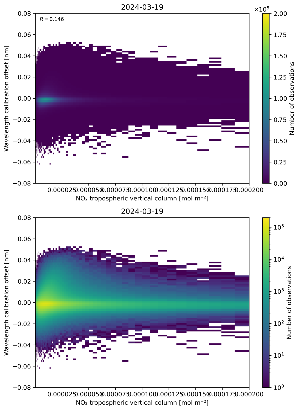
Figure 143: Scatter density plot of “NO 2 tropospheric vertical column” against “Wavelength calibration offset” for 2024-03-18 to 2024-03-20.
