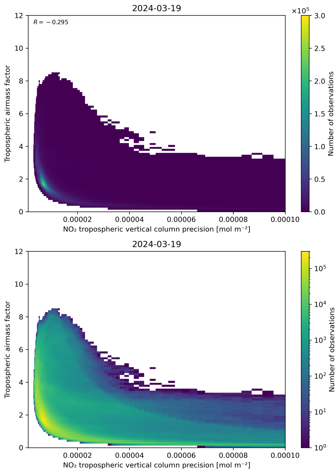
Figure 133: Scatter density plot of “NO 2 tropospheric vertical column precision” against “Tropospheric airmass factor” for 2024-03-18 to 2024-03-20.
