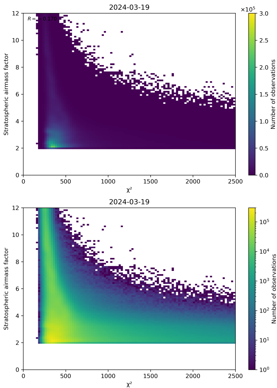
Figure 81: Scatter density plot of “ \chi^2 ” against “Stratospheric airmass factor” for 2024-03-18 to 2024-03-20.
