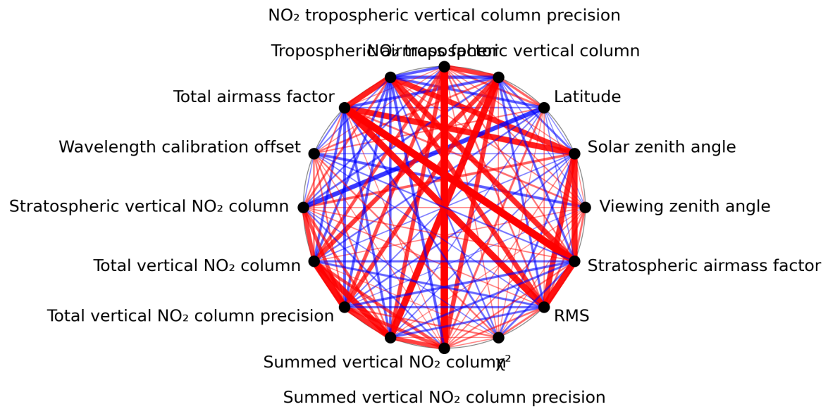
Figure 1: Map of correlation graph for 2024-03-18 to 2024-03-20.
