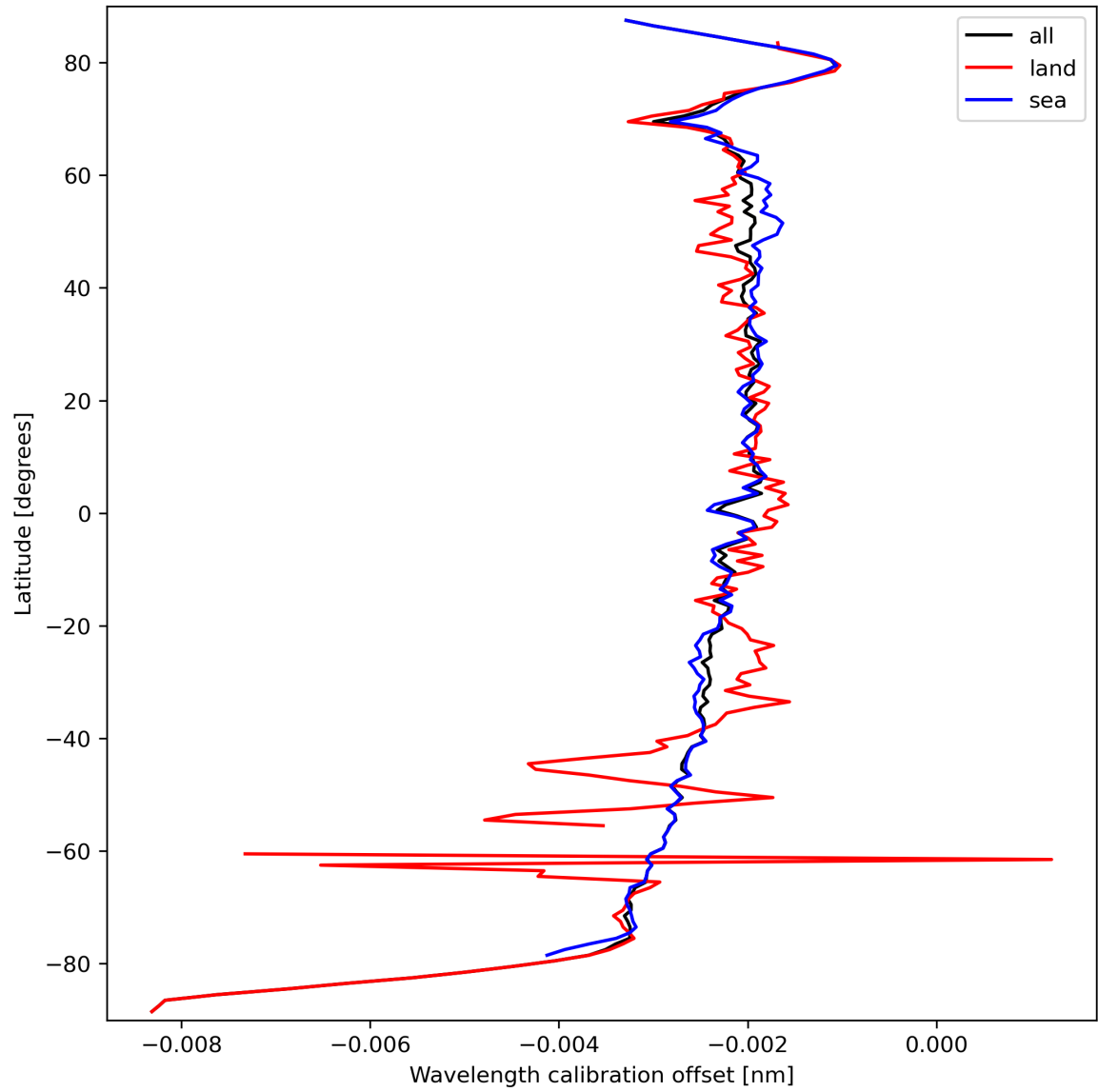
Figure 18: Zonal average of “Wavelength calibration offset” for 2024-03-18 to 2024-03-20.
