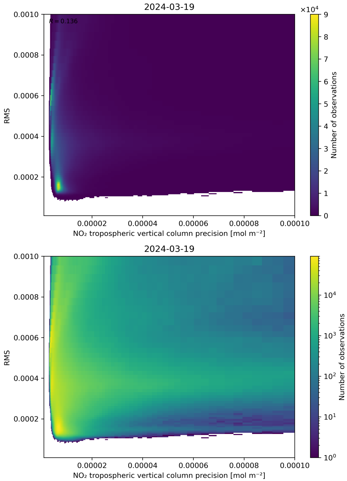
Figure 140: Scatter density plot of “NO 2 tropospheric vertical column precision” against “RMS” for 2024-03-18 to 2024-03-20.
