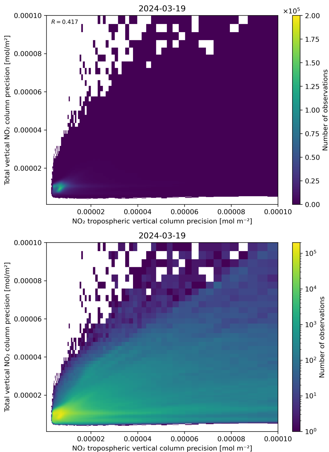
Figure 139: Scatter density plot of “NO 2 tropospheric vertical column precision” against “Total vertical NO 2 column precision” for 2024-03-18 to 2024-03-20.
