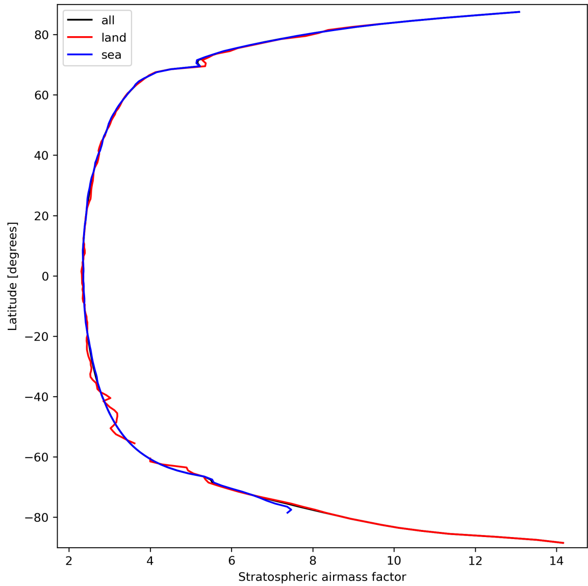
Figure 27: Zonal average of “Stratospheric air mass factor” for 2024-03-18 to 2024-03-20.
