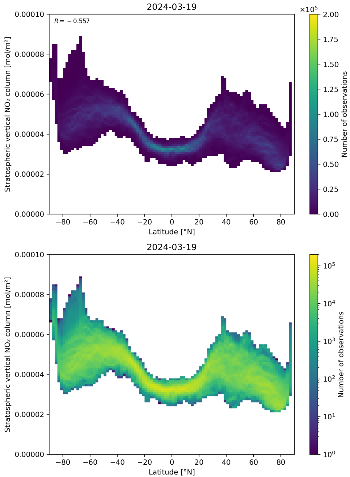
Figure 87: Scatter density plot of “Latitude” against “Stratospheric vertical NO 2 column” for 2024-03-18 to 2024-03-20.
