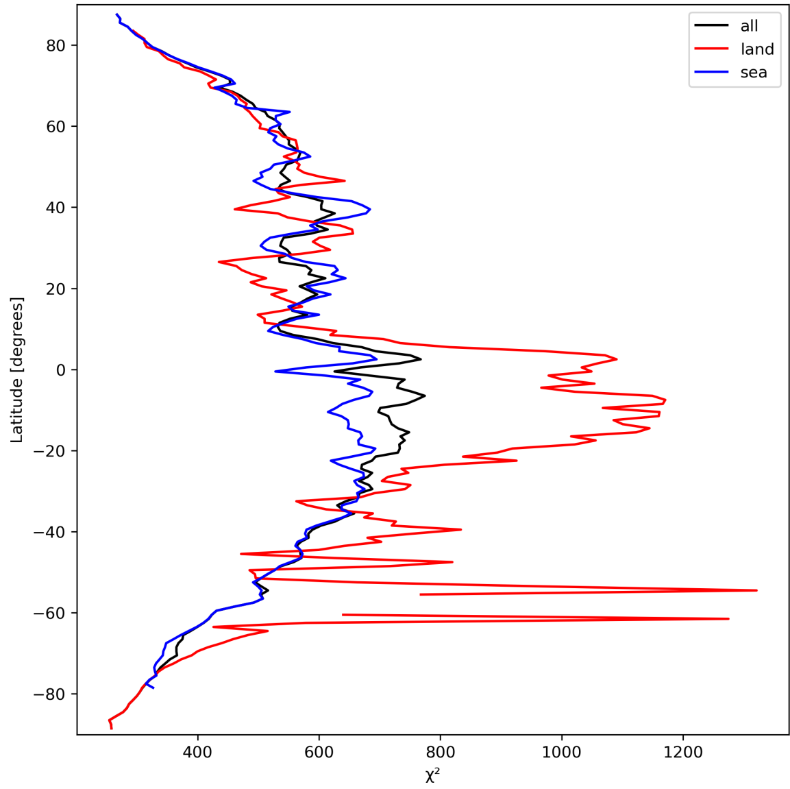
Figure 25: Zonal average of “ \chi^2 ” for 2024-03-18 to 2024-03-20.
