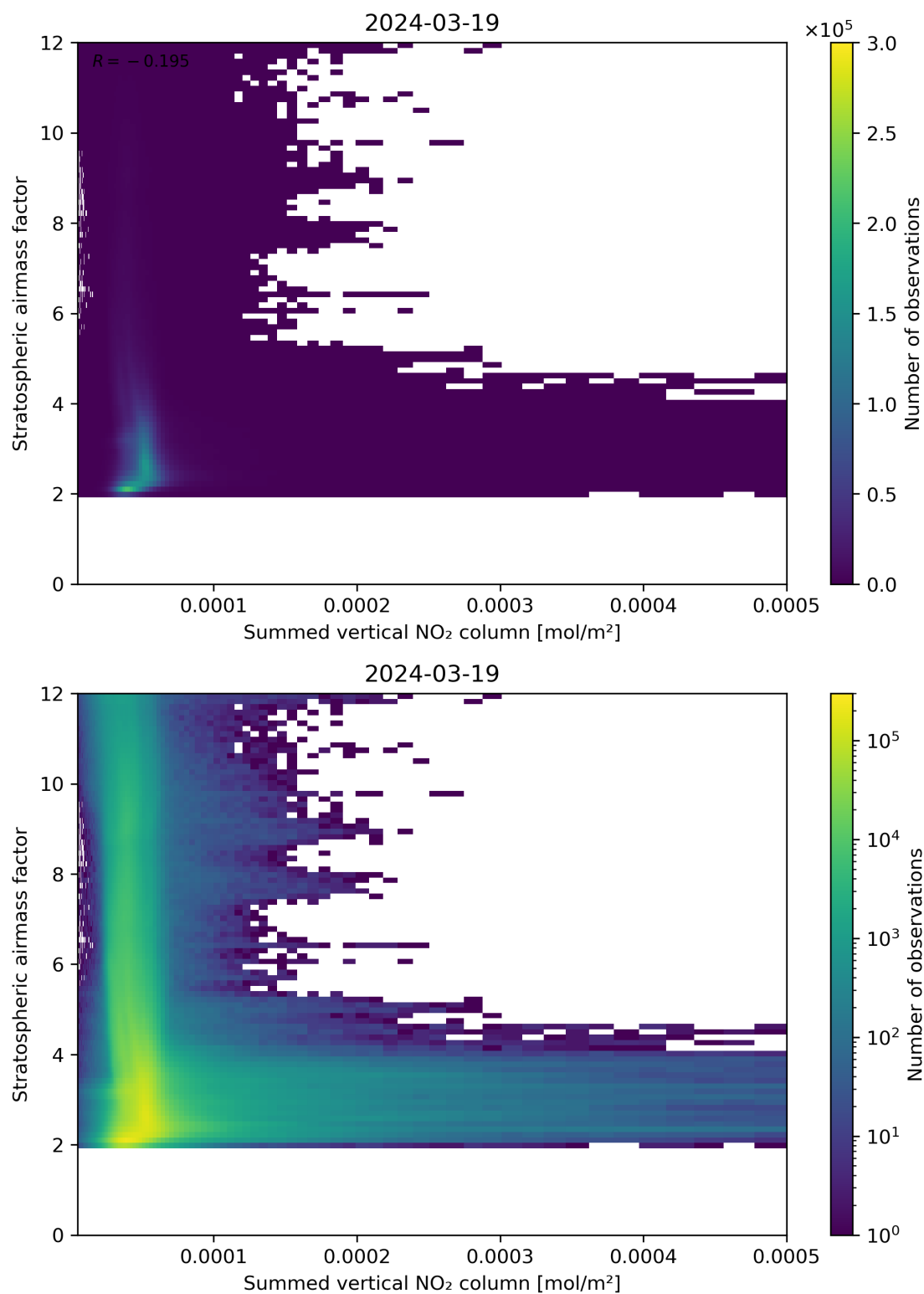
Figure 103: Scatter density plot of “Summed vertical NO 2 column” against “Stratospheric airmass factor” for 2024-03-18 to 2024-03-20.
