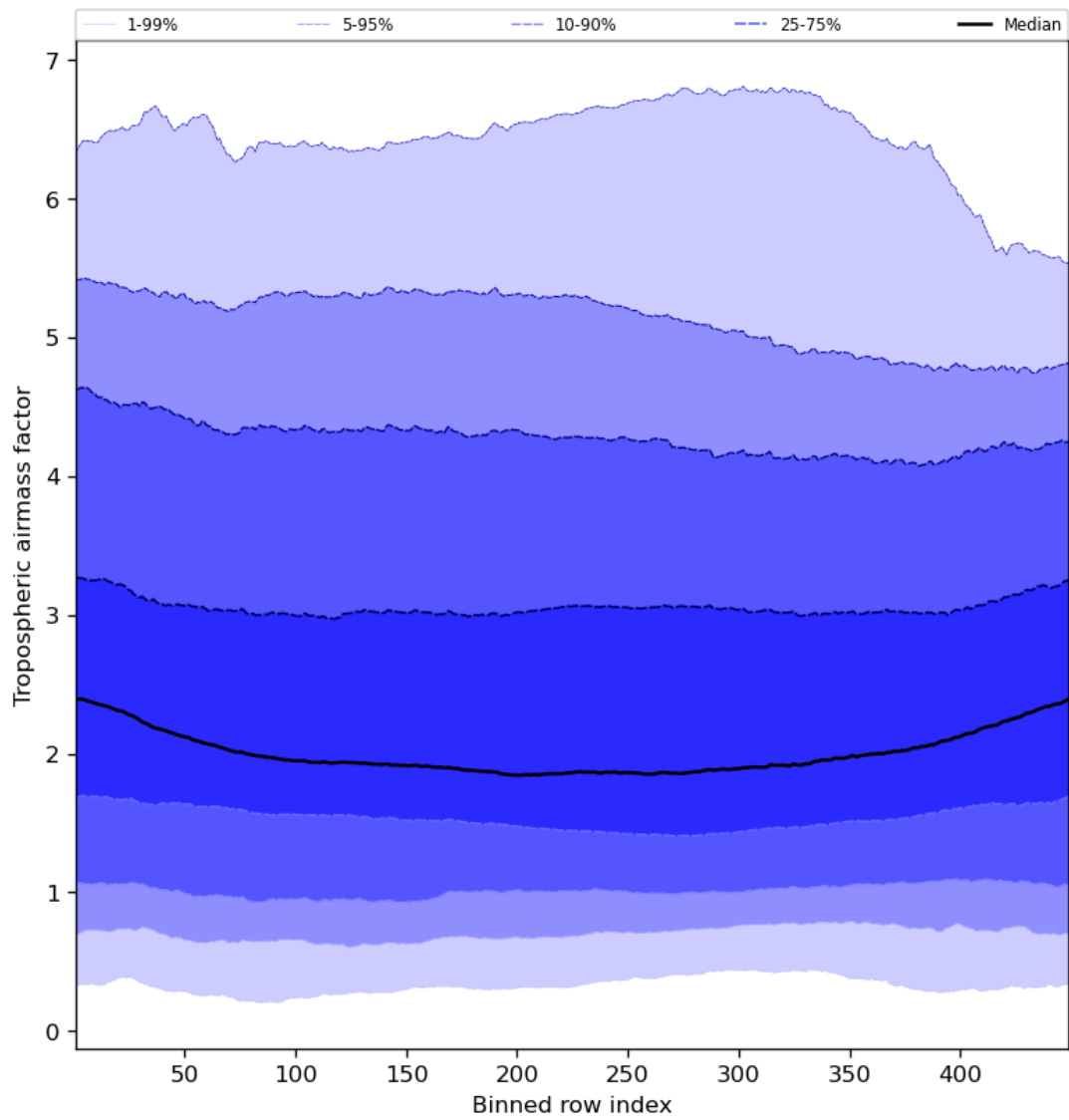
Figure 48: Along track statistics of “Tropospheric air mass factor” for 2024-03-18 to 2024-03-20
