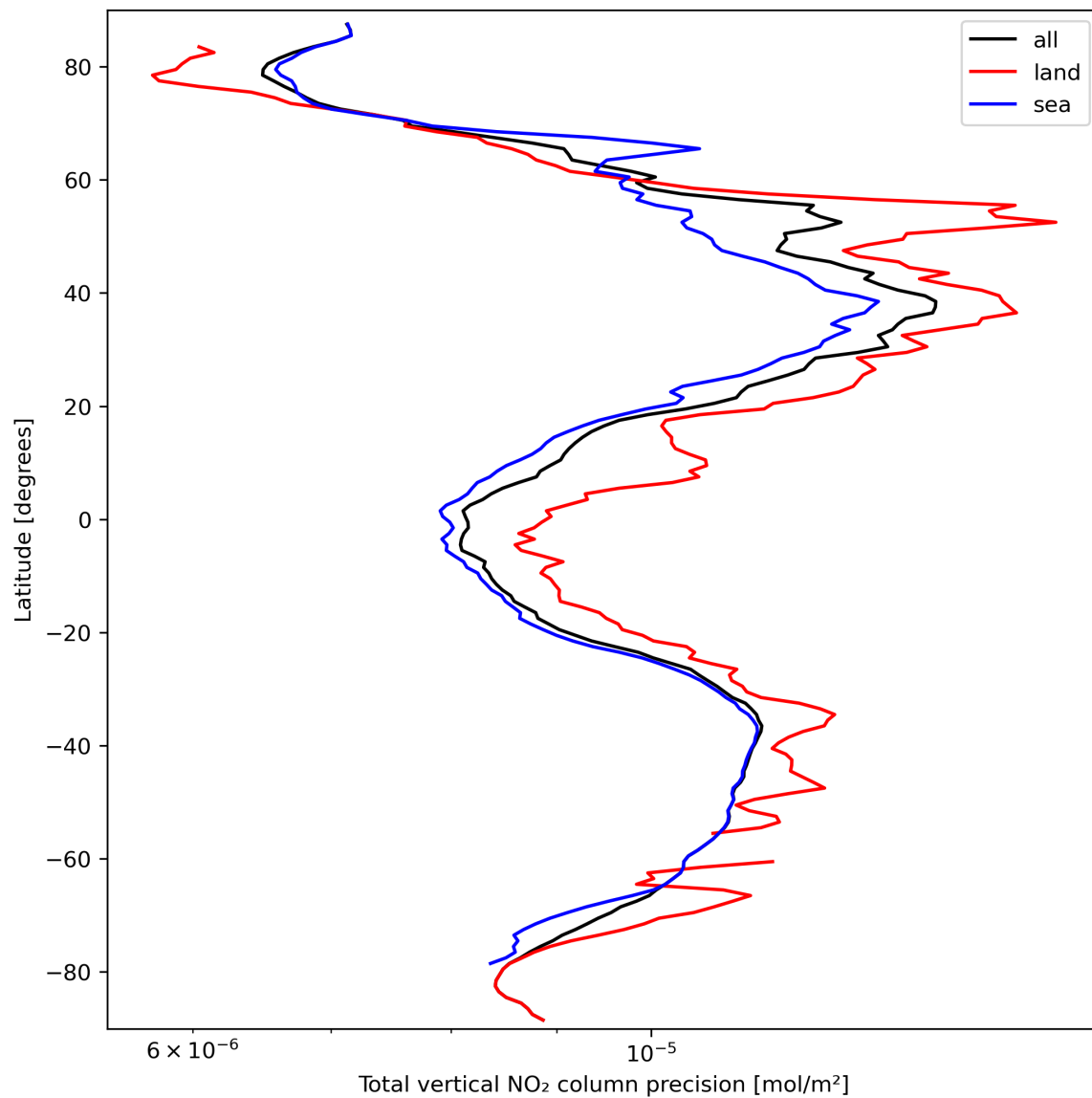
Figure 22: Zonal average of “Total vertical NO 2 column precision” for 2024-03-18 to 2024-03-20.
