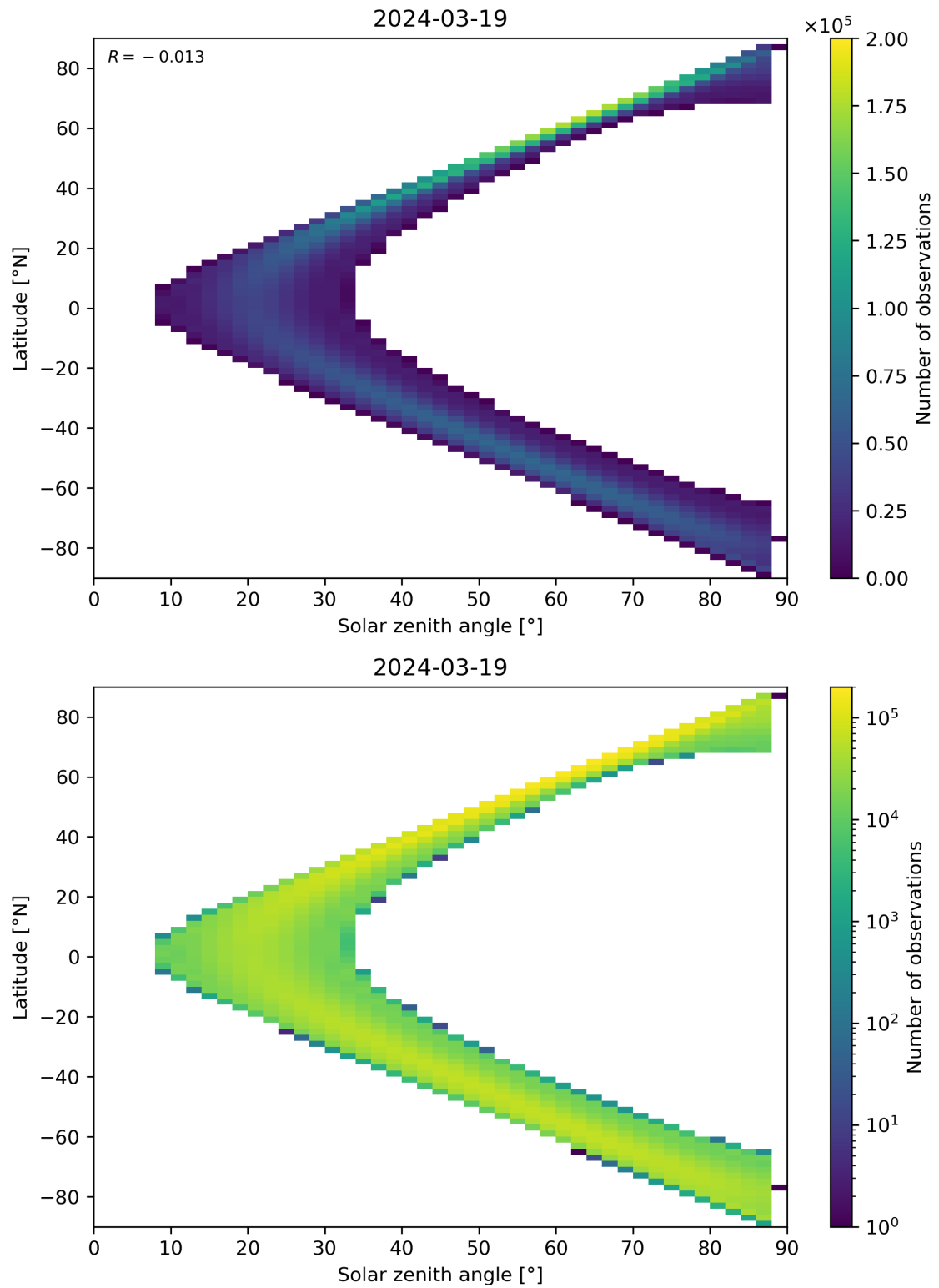
Figure 149: Scatter density plot of “Solar zenith angle” against “Latitude” for 2024-03-18 to 2024-03-20.
