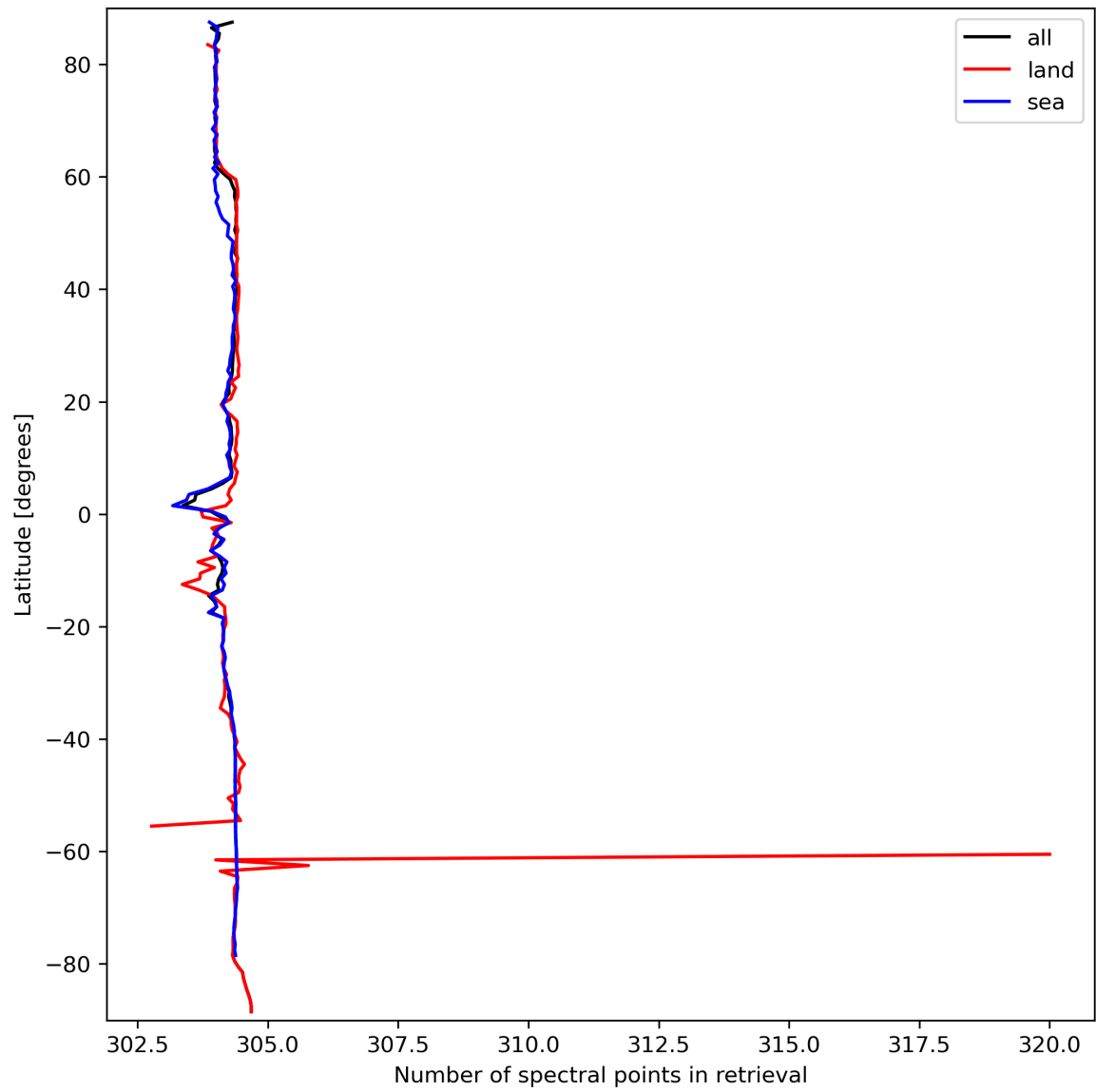
Figure 16: Zonal average of “Number of spectral points in retrieval” for 2024-03-18 to 2024-03-20.
