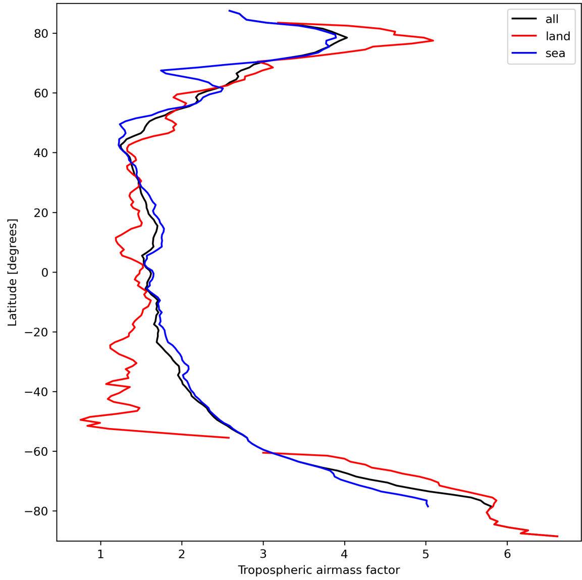
Figure 14: Zonal average of “Tropospheric airmass factor” for 2024-03-18 to 2024-03-20.
