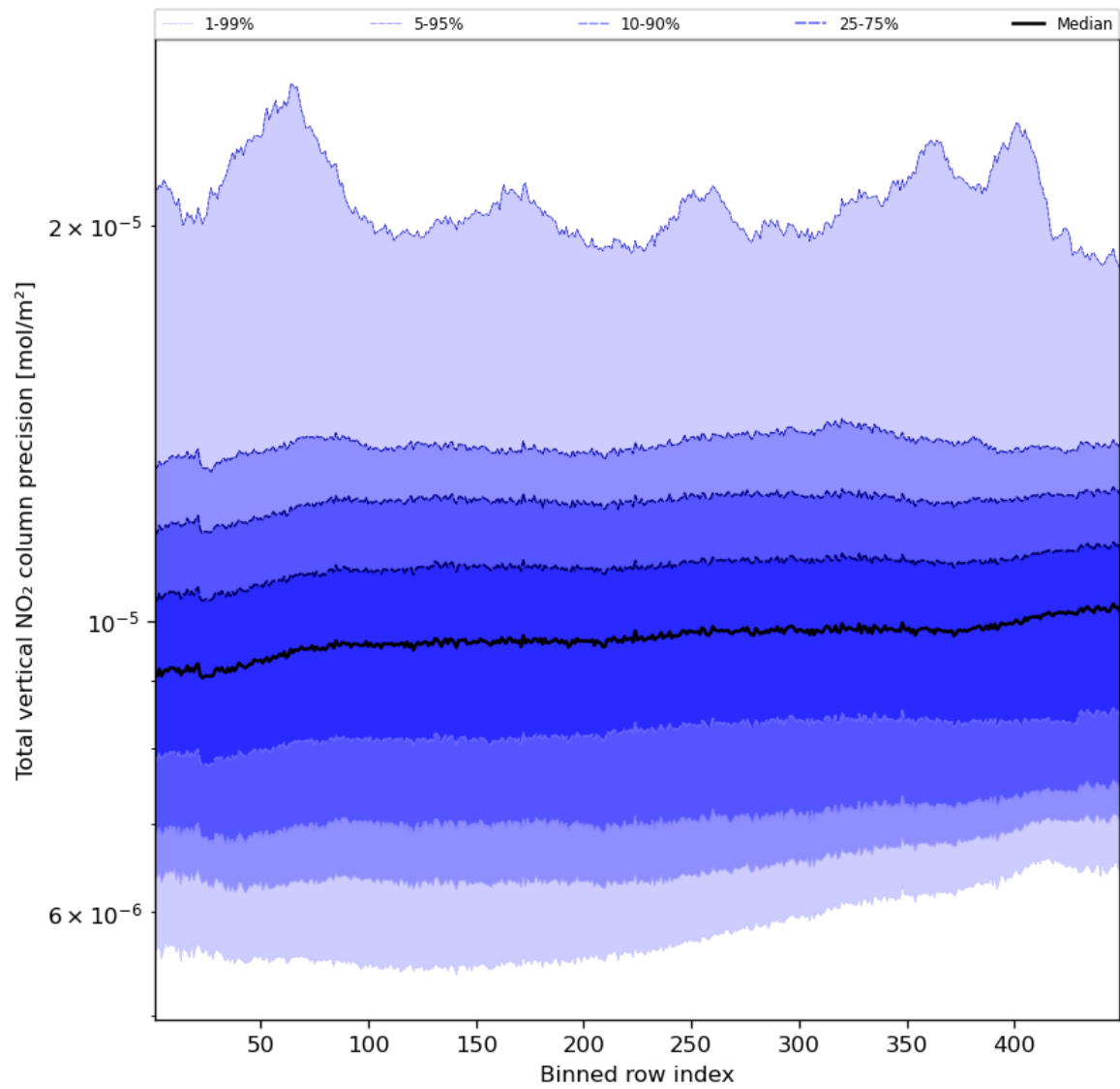
Figure 56: Along track statistics of “Total vertical NO 2 column precision” for 2024-03-18 to 2024-03-20
