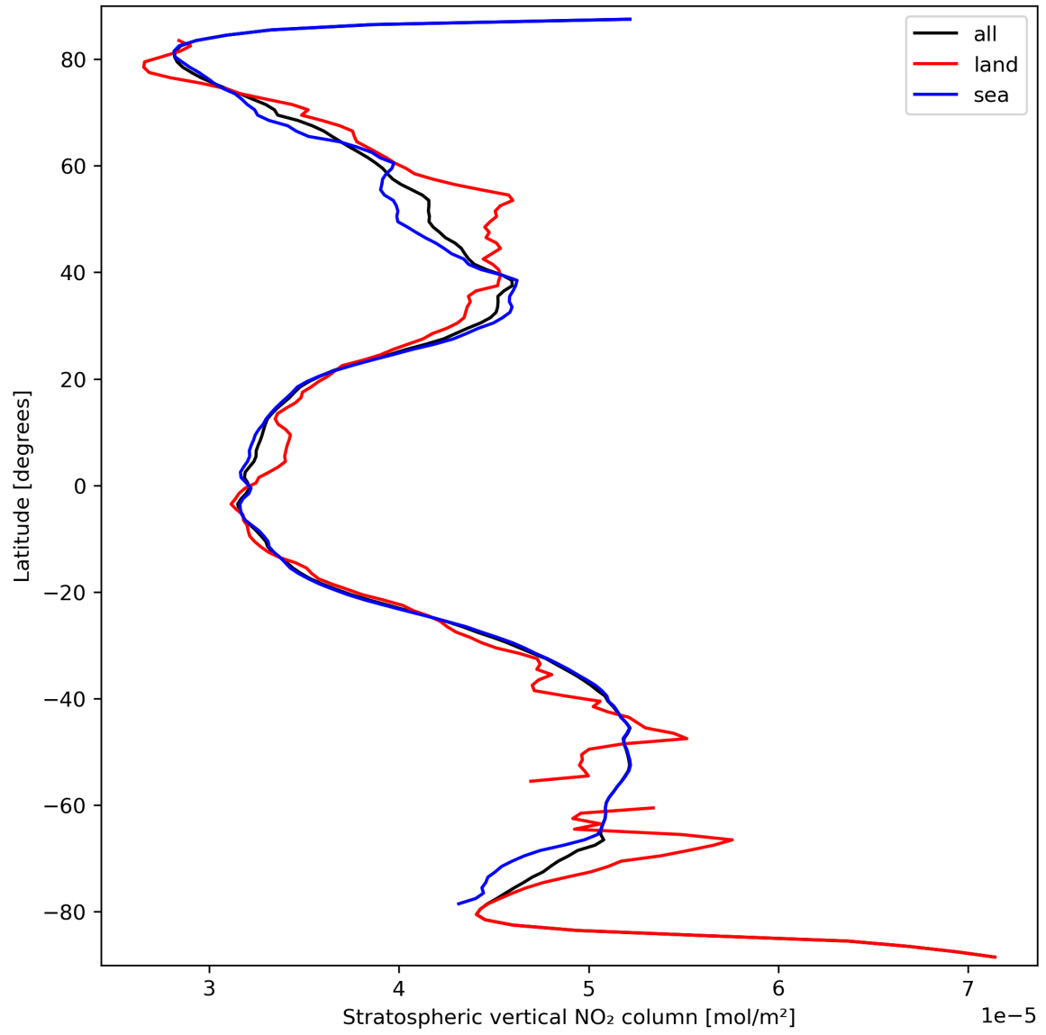
Figure 19: Zonal average of “Stratospheric vertical NO 2 column” for 2024-03-18 to 2024-03-20.
