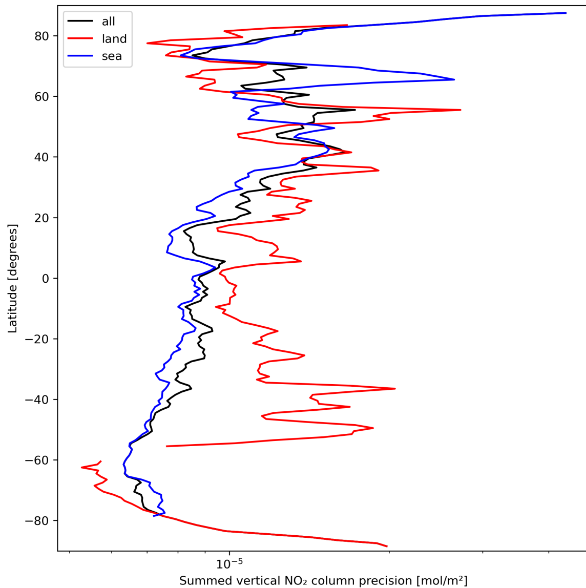
Figure 24: Zonal average of “Summed vertical NO 2 column precision” for 2024-03-18 to 2024-03-20.
