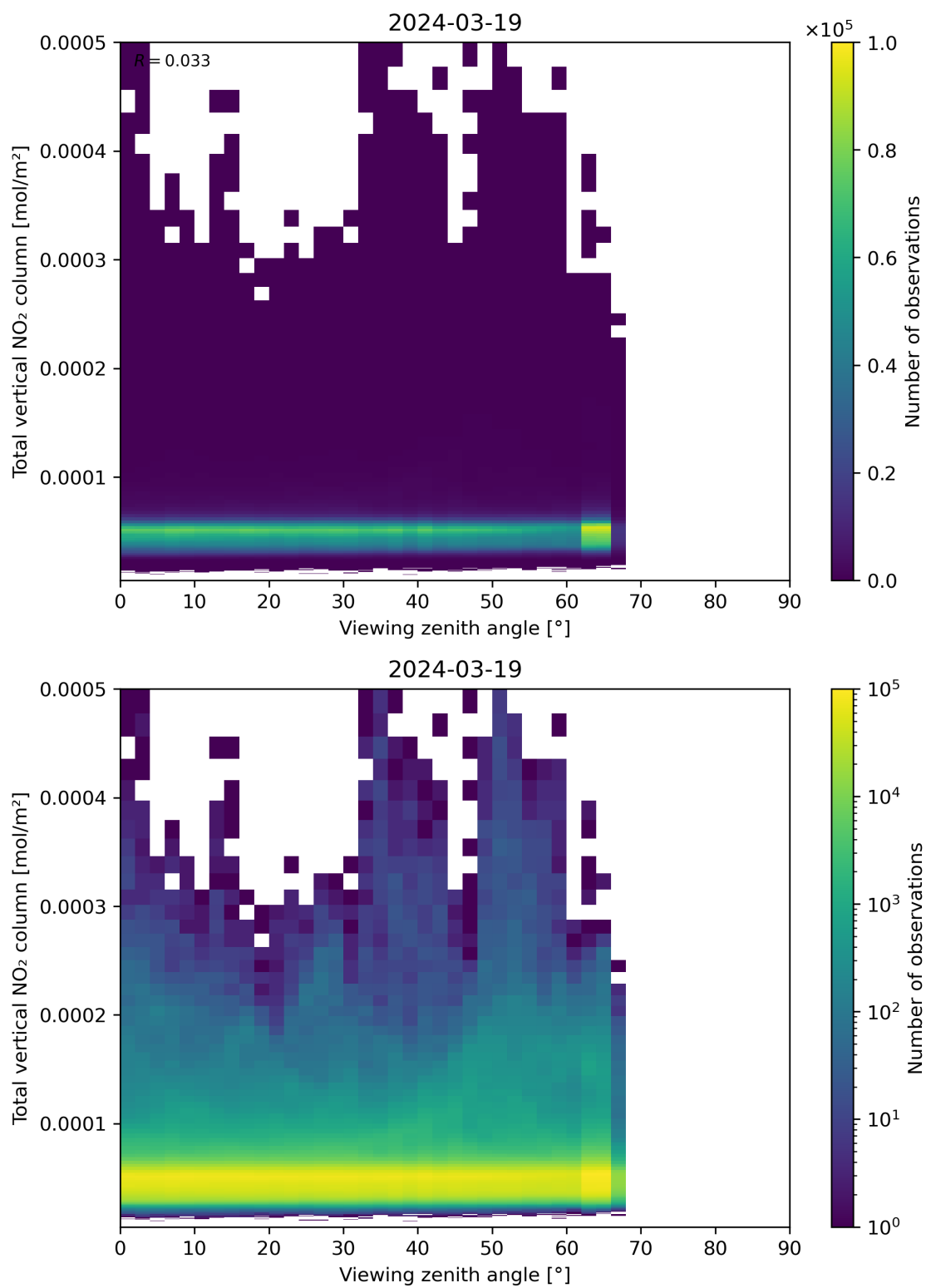
Figure 167: Scatter density plot of “Viewing zenith angle” against “Total vertical NO 2 column” for 2024-03-18 to 2024-03-20.
