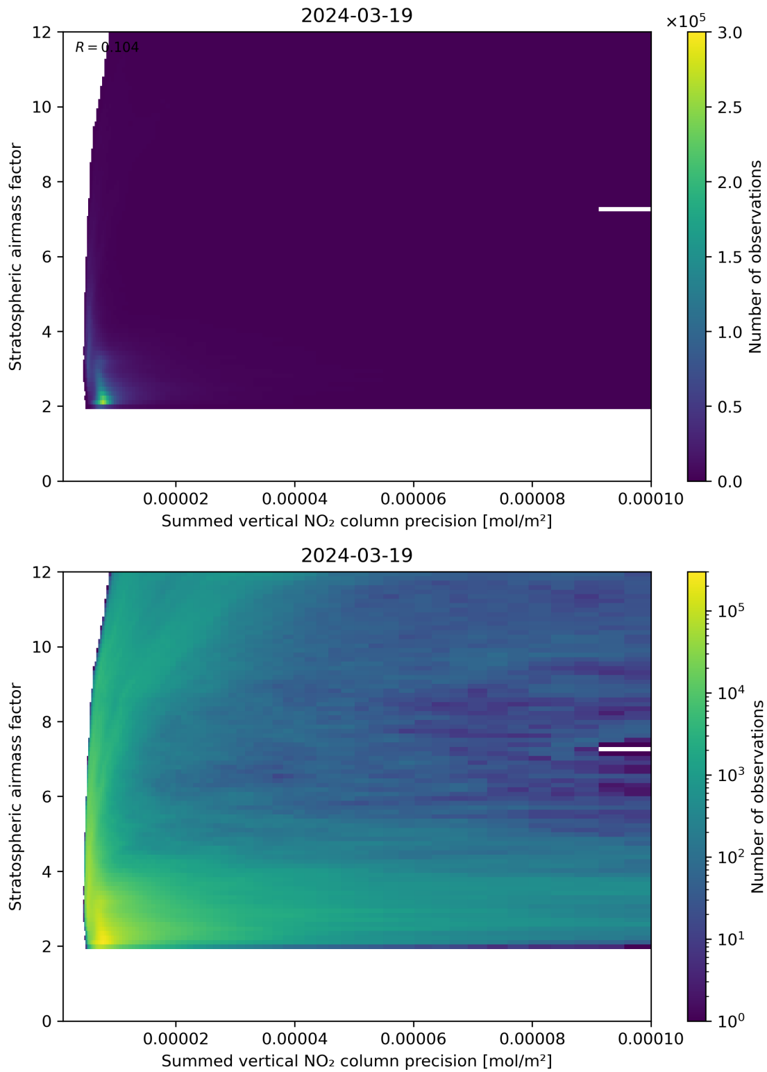
Figure 106: Scatter density plot of “Summed vertical NO 2 column precision” against “Stratospheric airmass factor” for 2024-03-18 to 2024-03-20.
