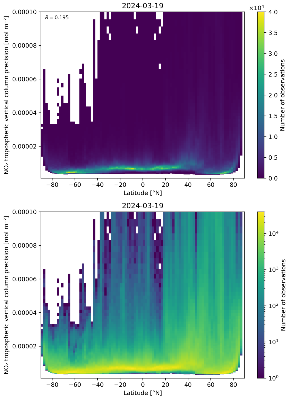
Figure 93: Scatter density plot of “Latitude” against “NO 2 tropospheric vertical column precision” for 2024-03-18 to 2024-03-20.
