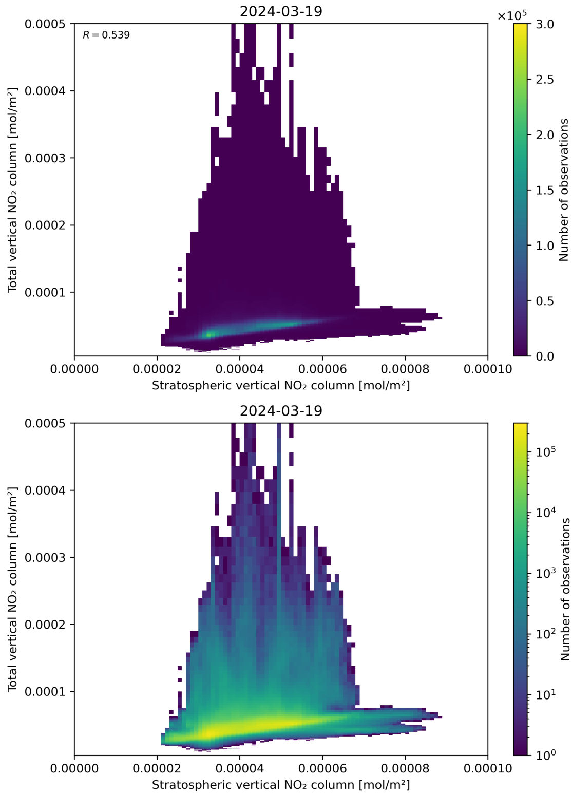
Figure 100: Scatter density plot of “Stratospheric vertical NO 2 column” against “Total vertical NO 2 column” for 2024-03-18 to 2024-03-20.
