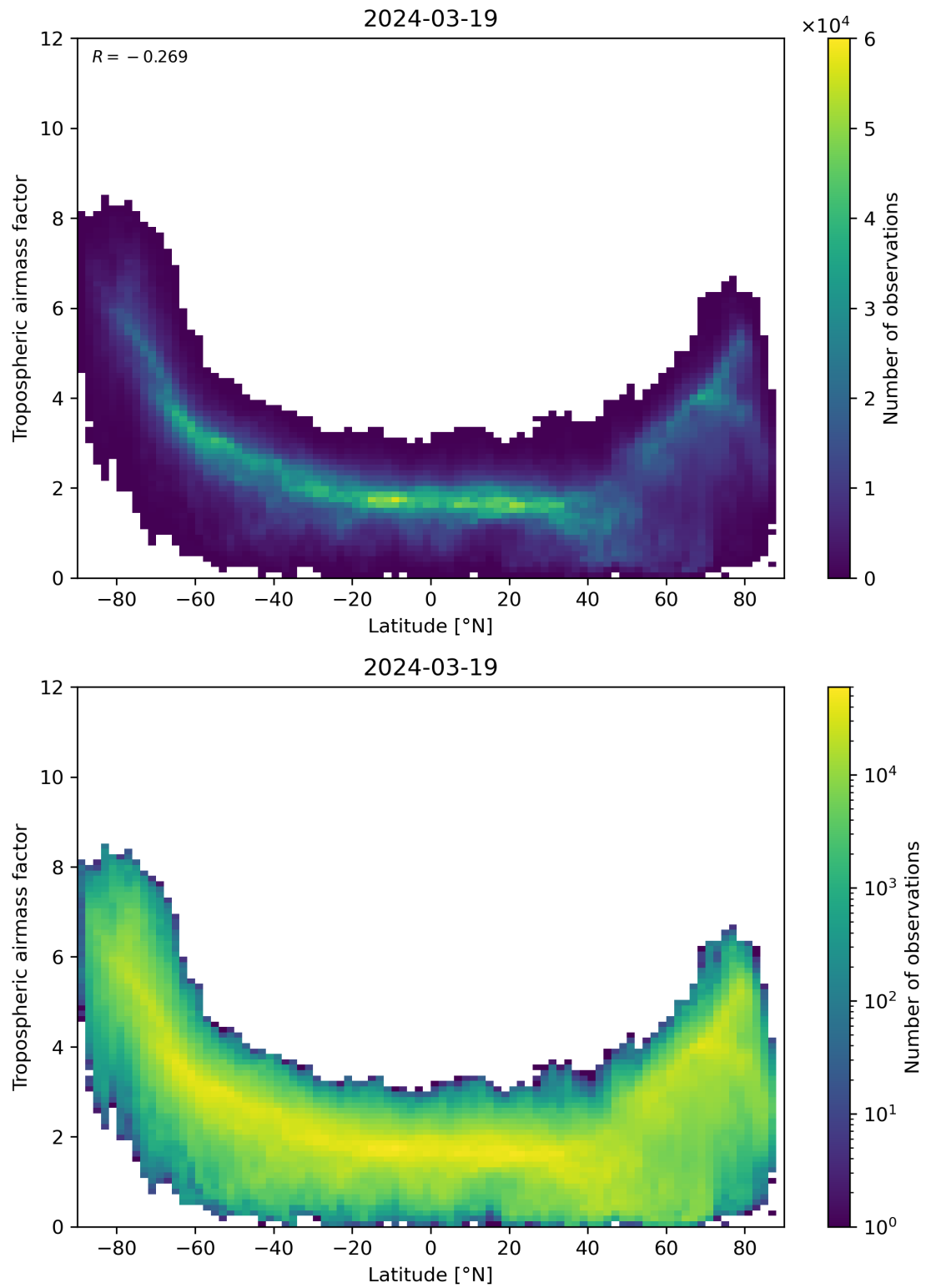
Figure 85: Scatter density plot of “Latitude” against “Tropospheric air mass factor” for 2024-03-18 to 2024-03-20.
