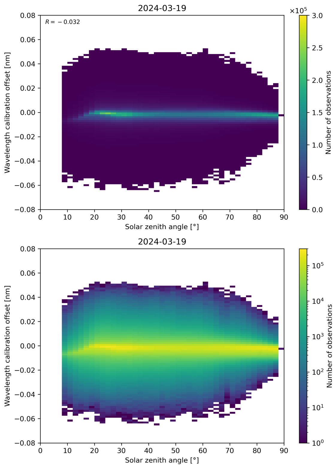
Figure 158: Scatter density plot of “Solar zenith angle” against “Wavelength calibration offset” for 2024-03-18 to 2024-03-20.
