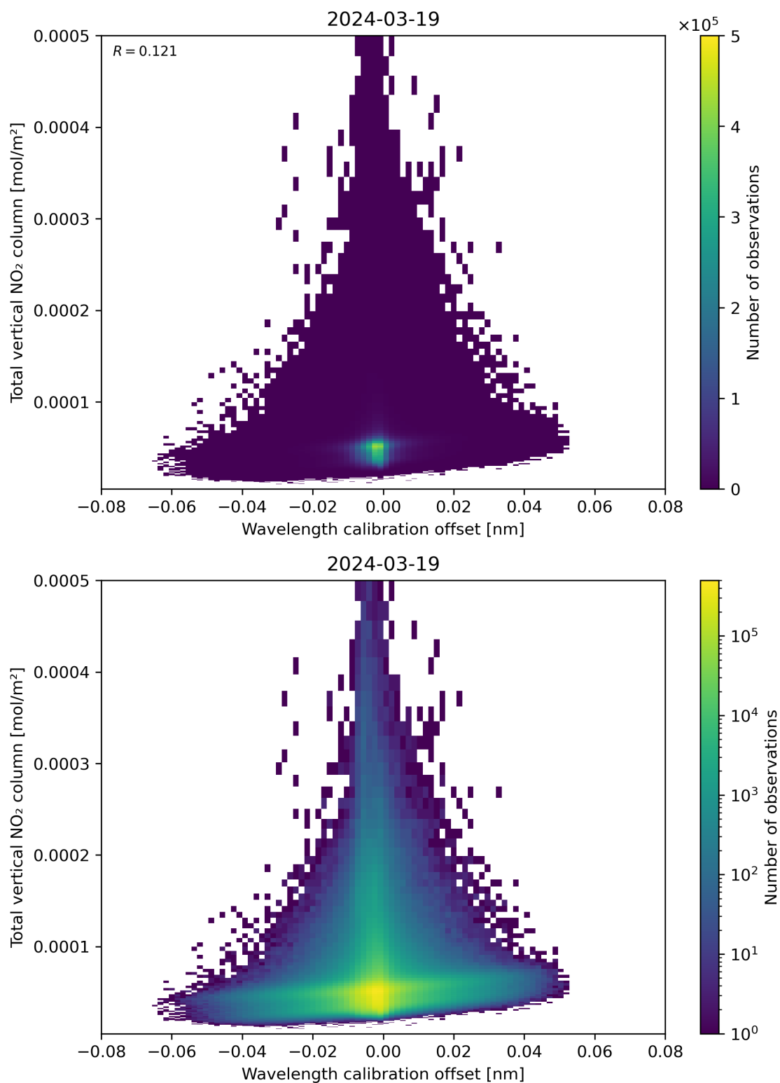
Figure 179: Scatter density plot of “Wavelength calibration offset” against “Total vertical NO 2 column” for 2024-03-18 to 2024-03-20.
