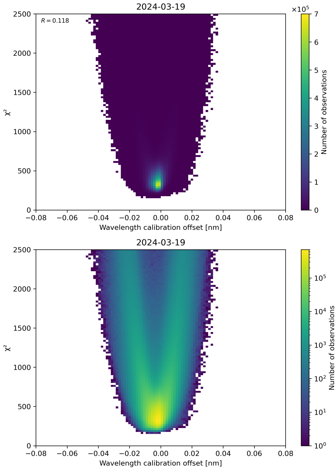
Figure 175: Scatter density plot of “Wavelength calibration offset” against “ \chi^2 ” for 2024-03-18 to 2024-03-20.
