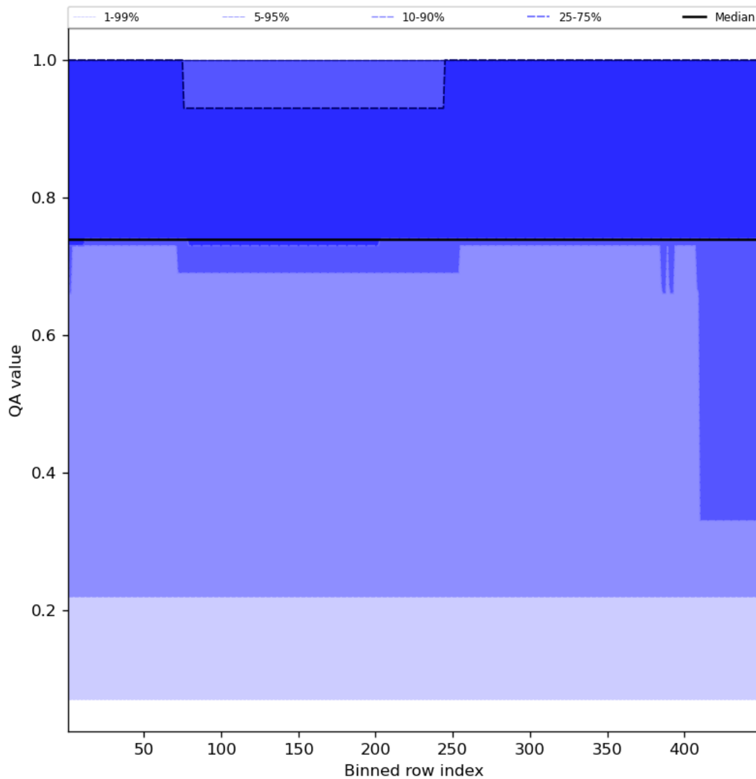
Figure 45: Along track statistics of “QA value” for 2024-03-18 to 2024-03-20
