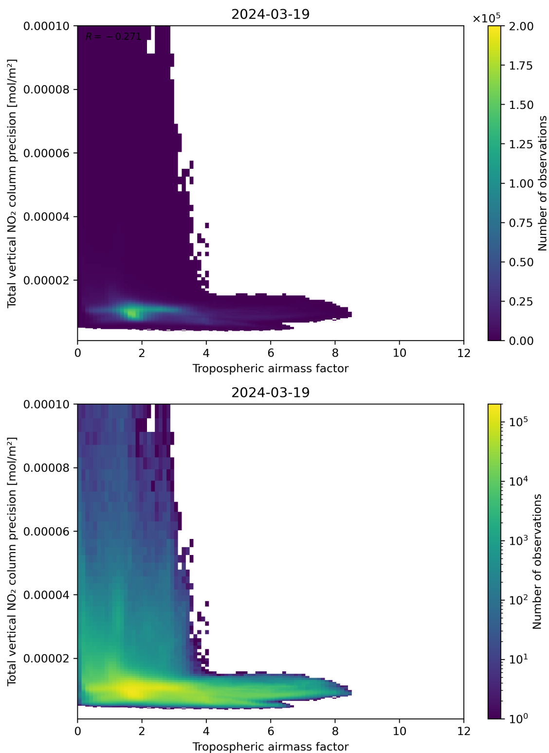
Figure 78: Scatter density plot of “Tropospheric air mass factor” against “Total vertical NO 2 column precision” for 2024-03-18 to 2024-03-20.
