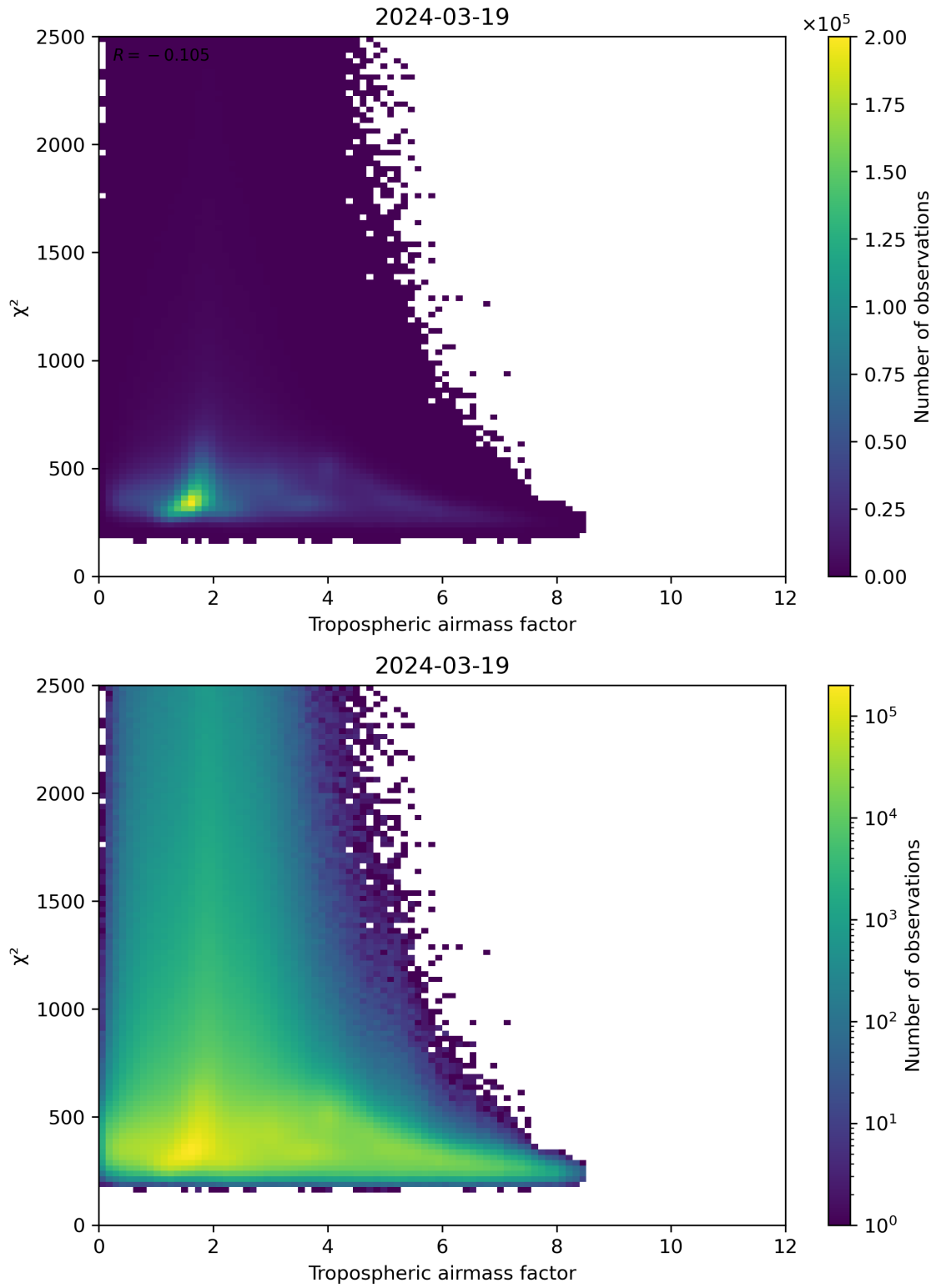
Figure 73: Scatter density plot of “Tropospheric airmass factor” against “ \chi^2 ” for 2024-03-18 to 2024-03-20.
