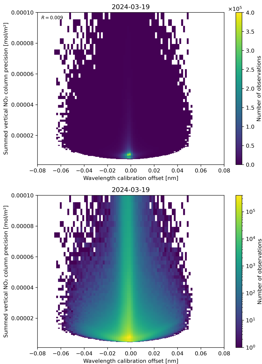
Figure 178: Scatter density plot of “Wavelength calibration offset” against “Summed vertical NO 2 column precision” for 2024-03-18 to 2024-03-20.
