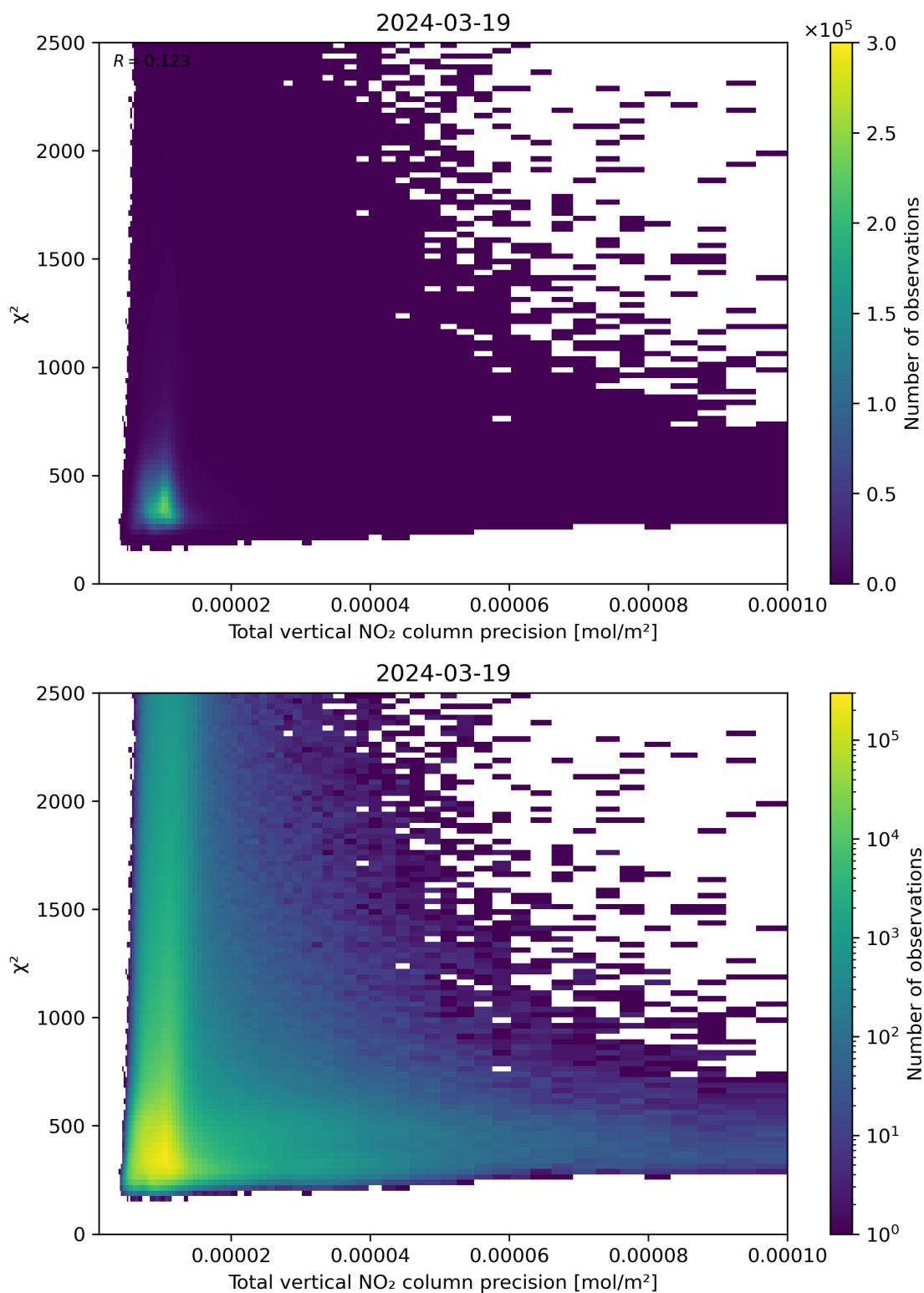
Figure 116: Scatter density plot of “Total vertical NO 2 column precision” against “ \chi^2 ” for 2024-03-18 to 2024-03-20.
