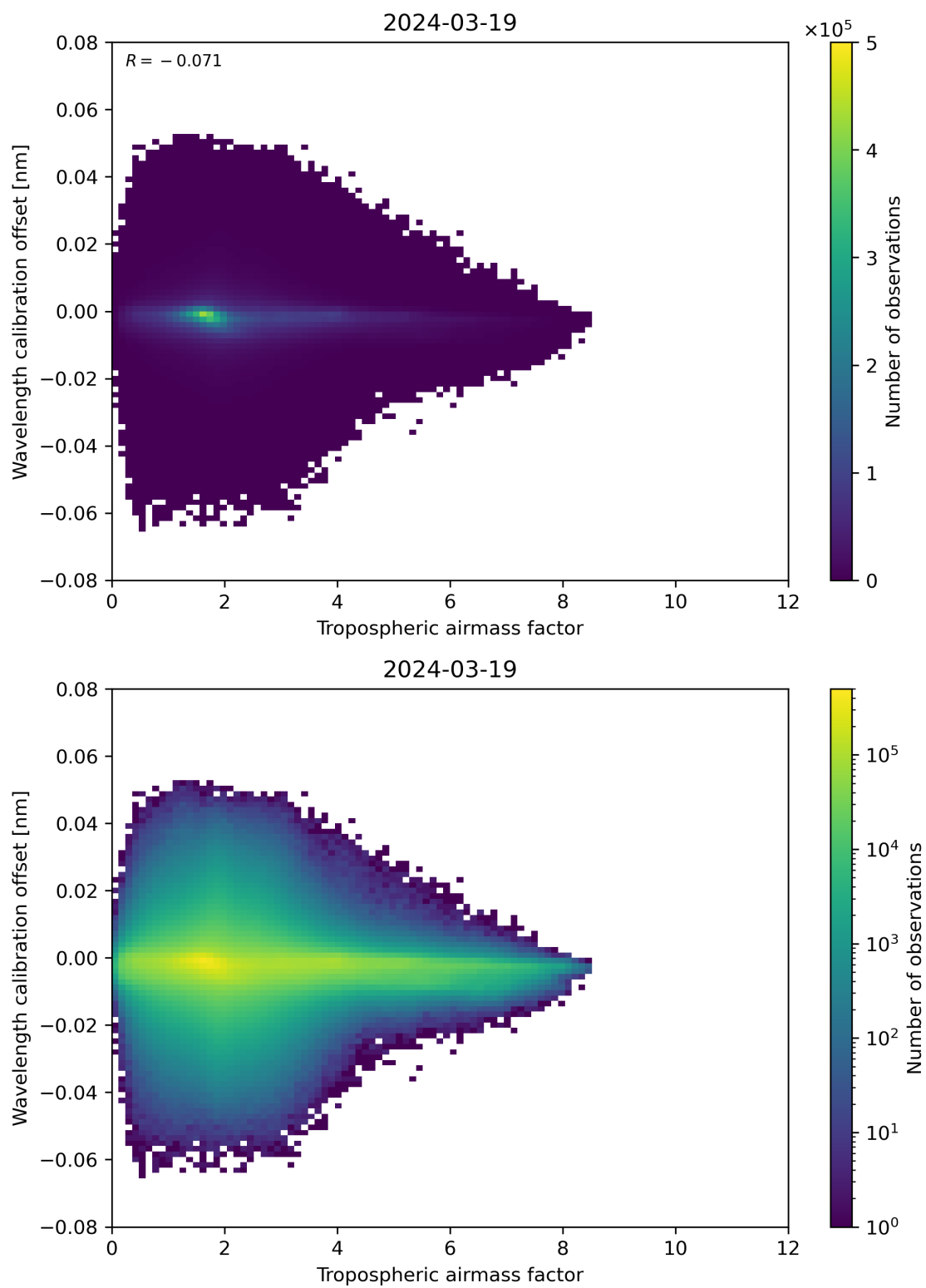
Figure 80: Scatter density plot of “Tropospheric airmass factor” against “Wavelength calibration offset” for 2024-03-18 to 2024-03-20.
