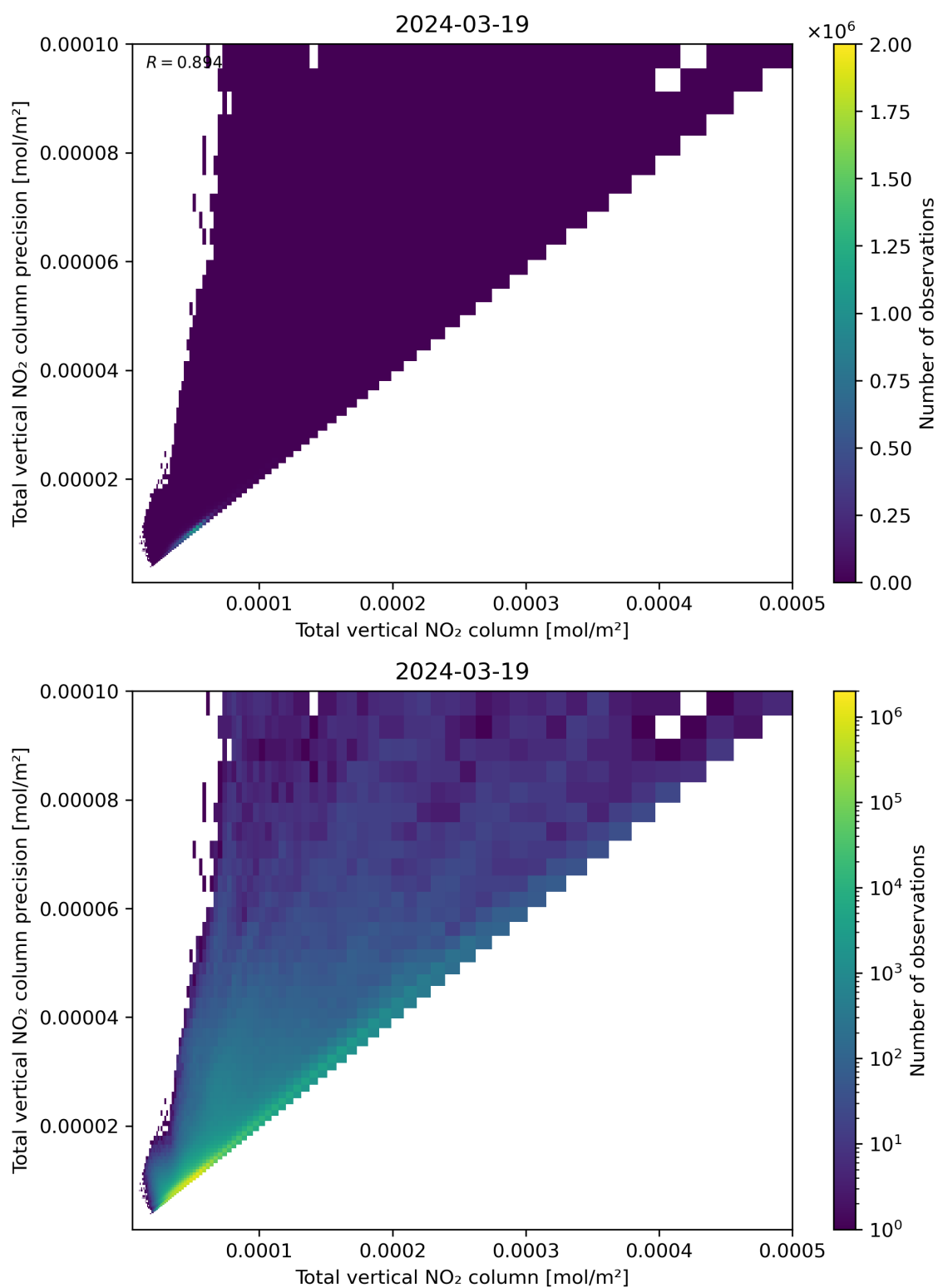
Figure 114: Scatter density plot of “Total vertical NO 2 column” against “Total vertical NO 2 column precision” for 2024-03-18 to 2024-03-20.
