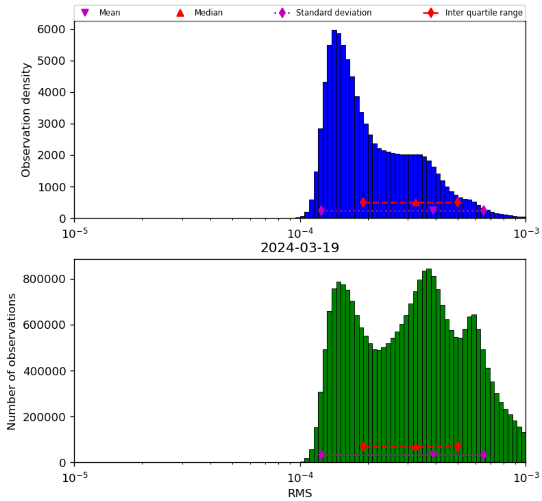
Figure 43: Histogram of “RMS” for 2024-03-18 to 2024-03-20
