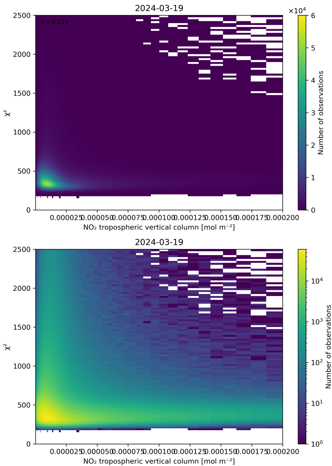
Figure 124: Scatter density plot of “NO 2 tropospheric vertical column” against “ \chi^2 ” for 2024-03-18 to 2024-03-20.
