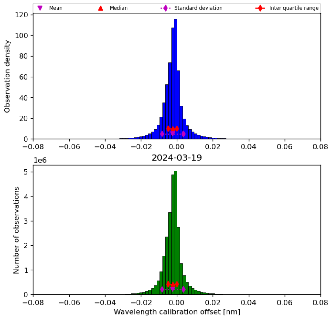
Figure 35: Histogram of “Wavelength calibration offset” for 2024-03-18 to 2024-03-20
