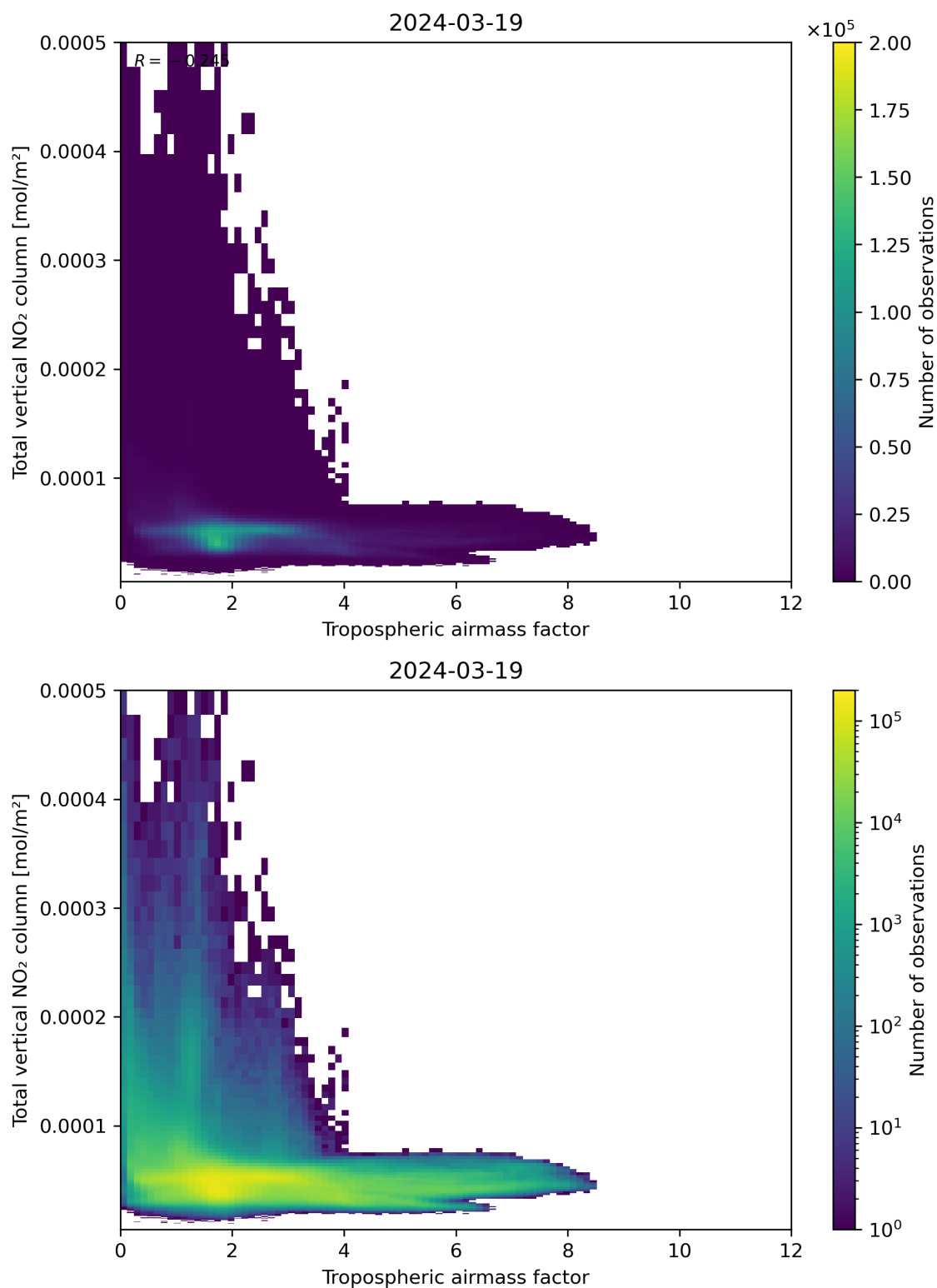
Figure 77: Scatter density plot of “Tropospheric airmass factor” against “Total vertical NO 2 column” for 2024-03-18 to 2024-03-20.
