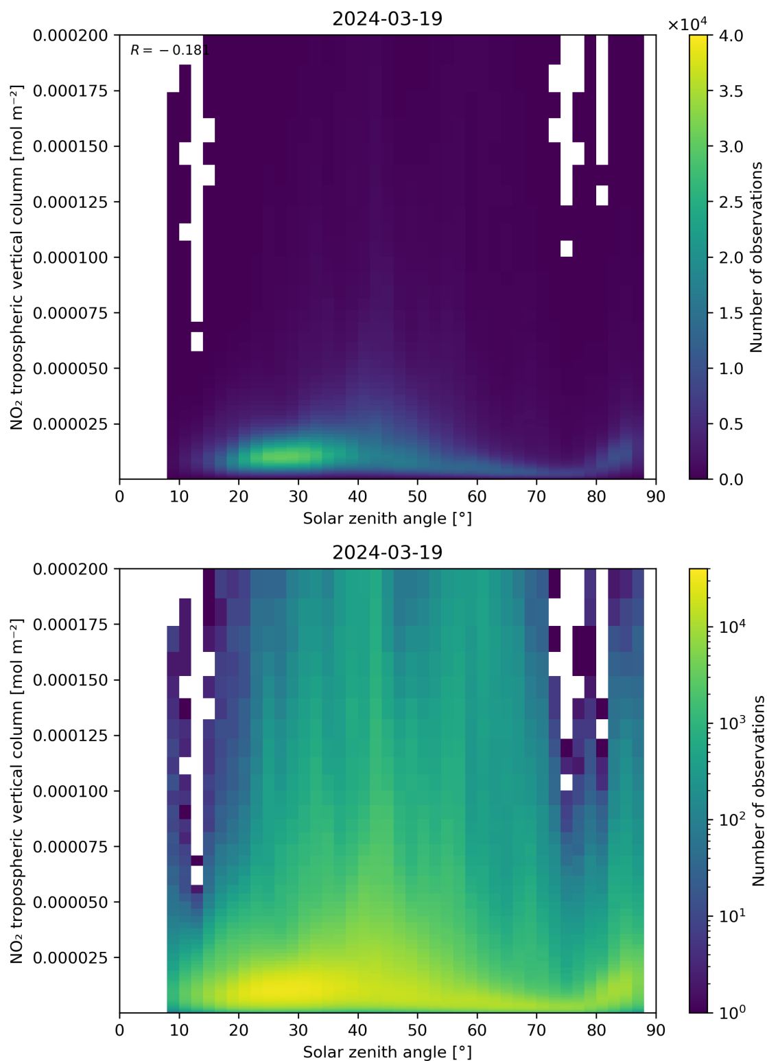
Figure 155: Scatter density plot of “Solar zenith angle” against “NO 2 tropospheric vertical column” for 2024-03-18 to 2024-03-20.
