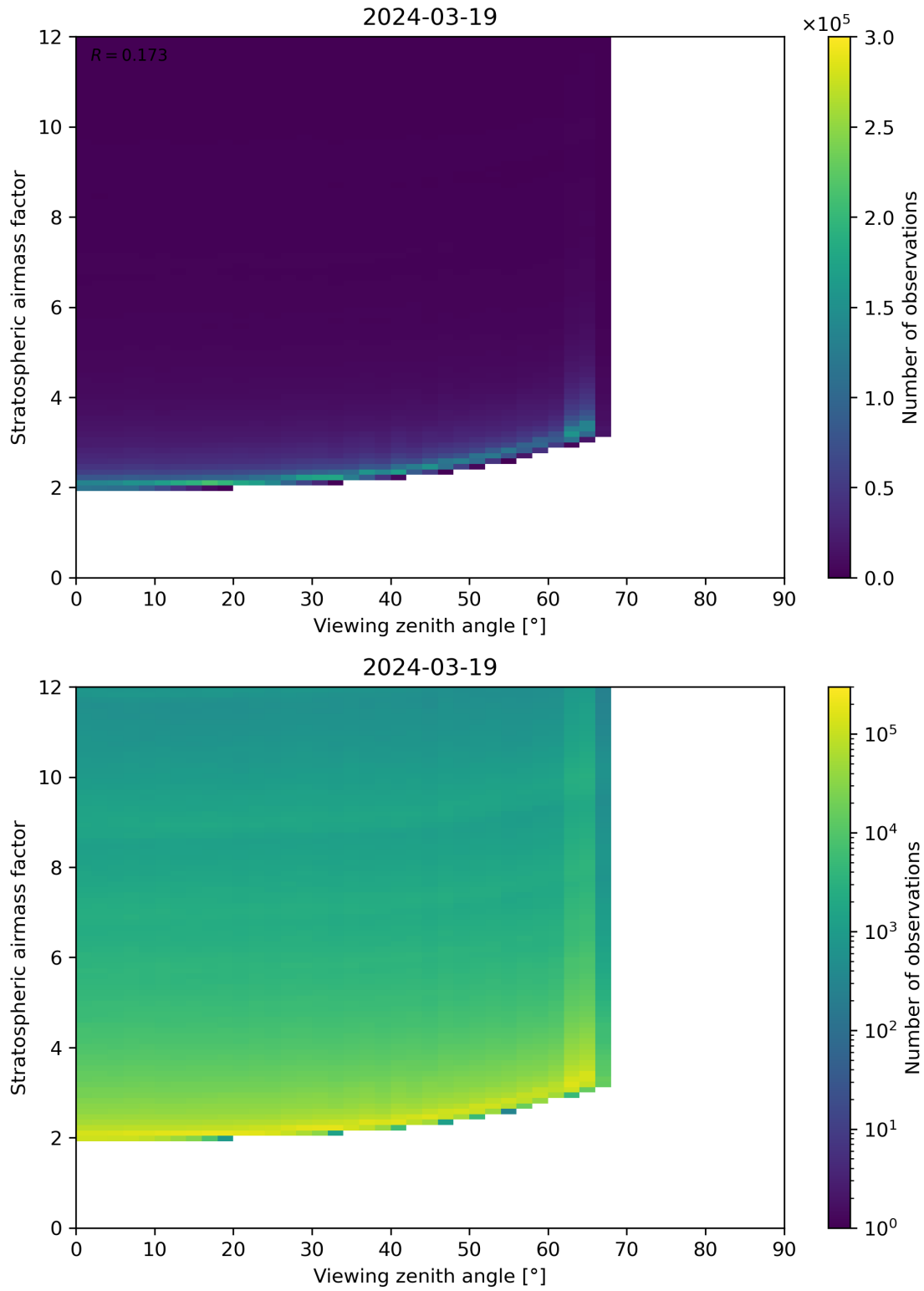
Figure 159: Scatter density plot of “Viewing zenith angle” against “Stratospheric airmass factor” for 2024-03-18 to 2024-03-20.
