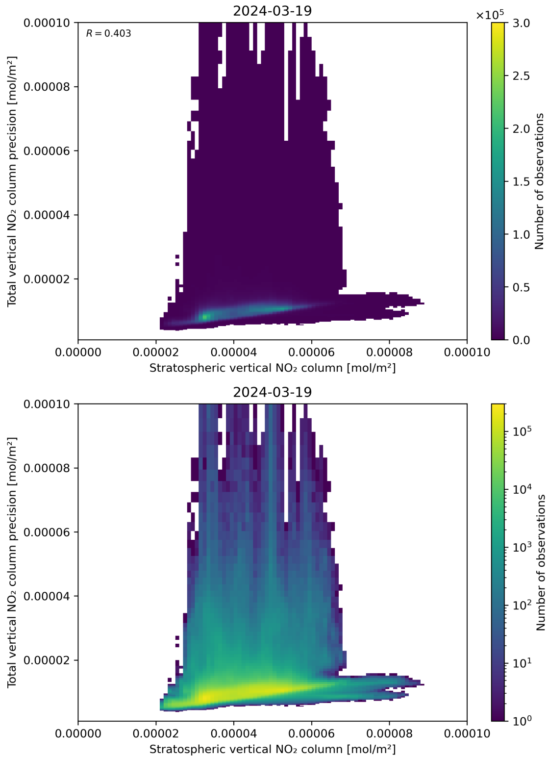
Figure 101: Scatter density plot of “Stratospheric vertical NO 2 column” against “Total vertical NO 2 column precision” for 2024-03-18 to 2024-03-20.
