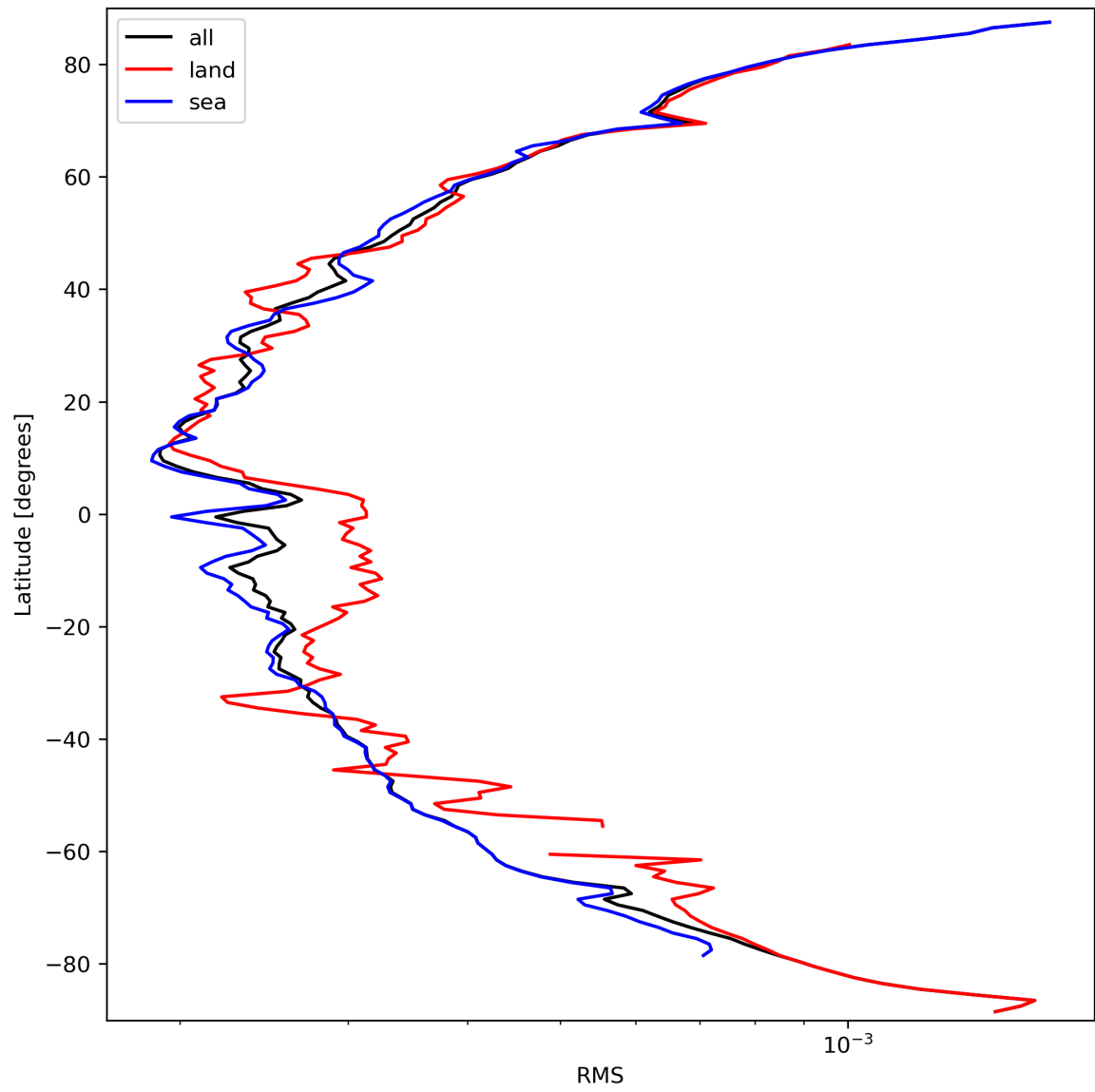
Figure 26: Zonal average of “RMS” for 2024-03-18 to 2024-03-20.
