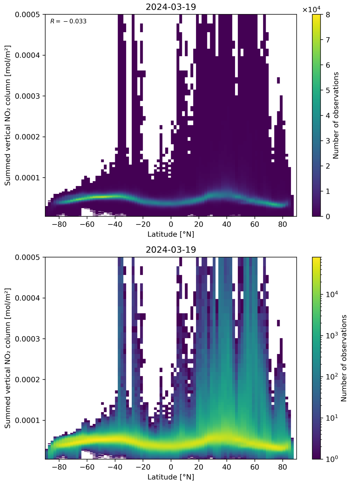
Figure 88: Scatter density plot of “Latitude” against “Summed vertical NO 2 column” for 2024-03-18 to 2024-03-20.
