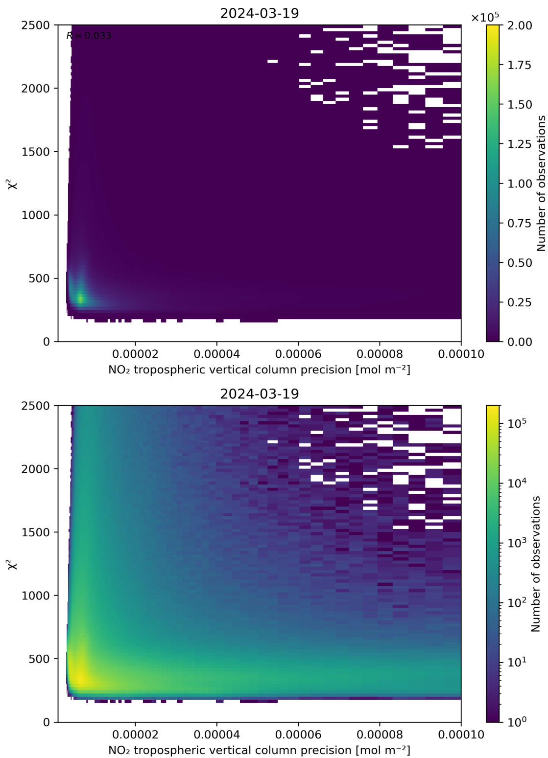
Figure 134: Scatter density plot of “NO 2 tropospheric vertical column precision” against “ \chi^2 ” for 2024-03-18 to 2024-03-20.
