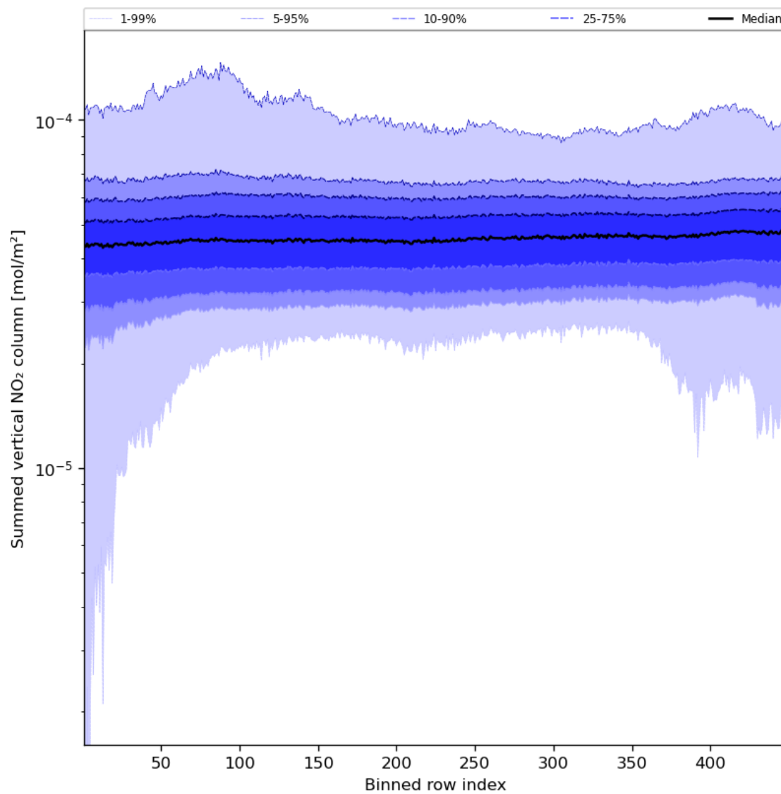
Figure 57: Along track statistics of “Summed vertical NO 2 column” for 2024-03-18 to 2024-03-20
