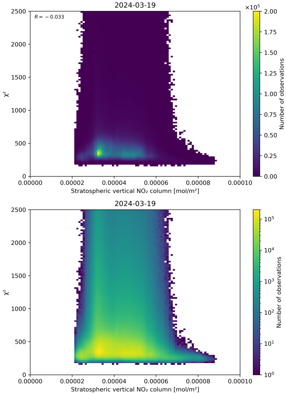
Figure 97: Scatter density plot of “Stratospheric vertical NO 2 column” against “ \chi^2 ” for 2024-03-18 to 2024-03-20.
