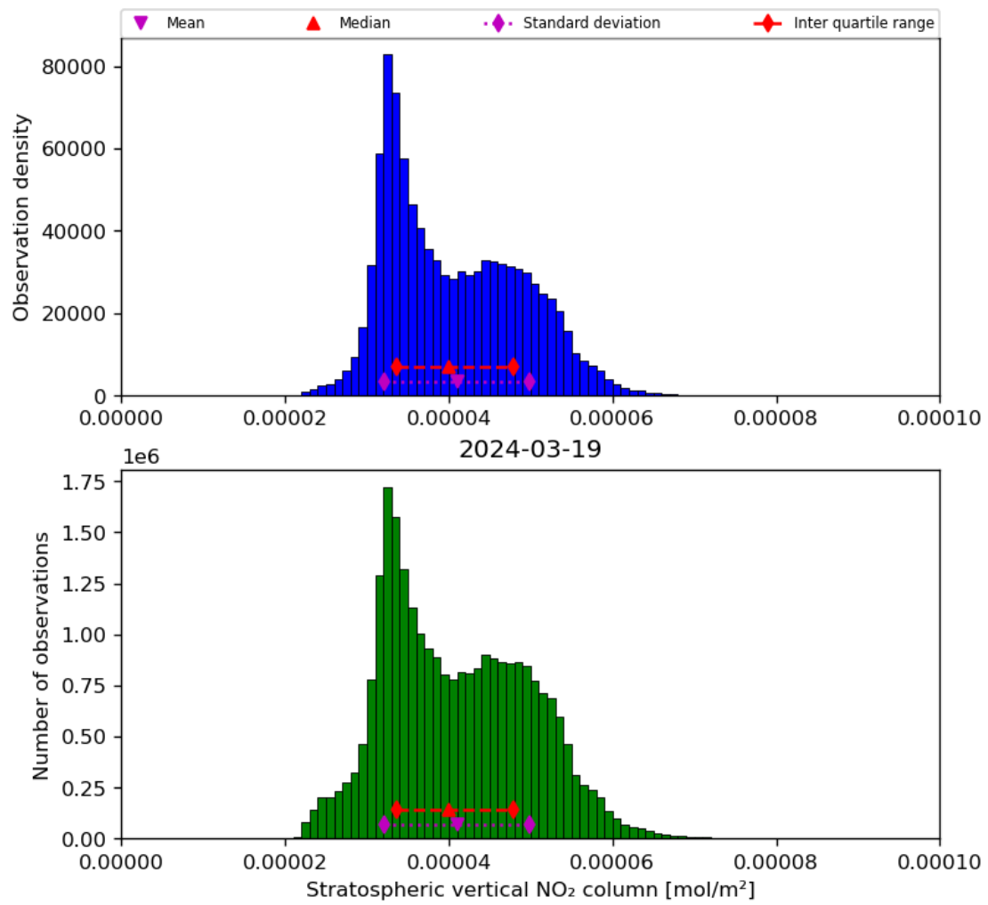
Figure 36: Histogram of “Stratospheric vertical NO 2 column” for 2024-03-18 to 2024-03-20
