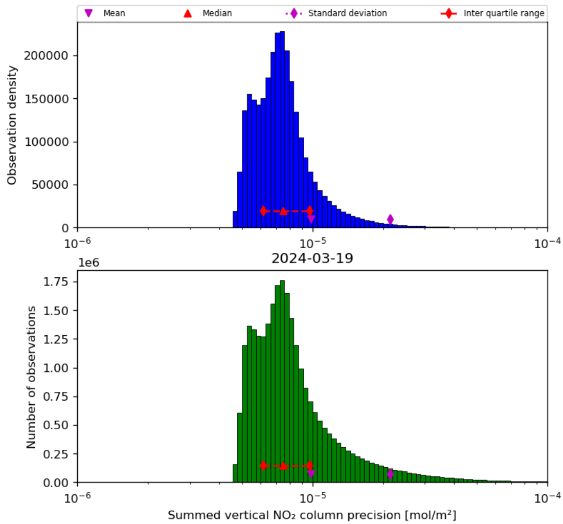
Figure 41: Histogram of "Summed vertical NO 2 column precision" for 2024-03-18 to 2024-03-20
