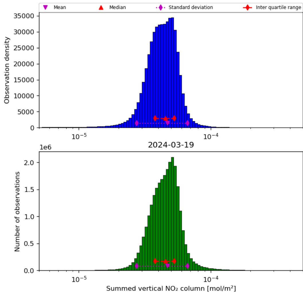
Figure 40: Histogram of “Summed vertical NO 2 column” for 2024-03-18 to 2024-03-20
