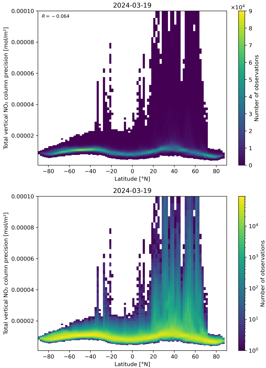
Figure 91: Scatter density plot of “Latitude” against “Total vertical NO 2 column precision” for 2024-03-18 to 2024-03-20.
