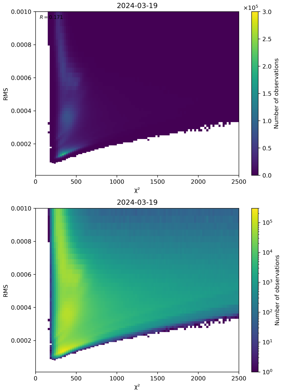
Figure 82: Scatter density plot of “ \chi^2 ” against “RMS” for 2024-03-18 to 2024-03-20.
