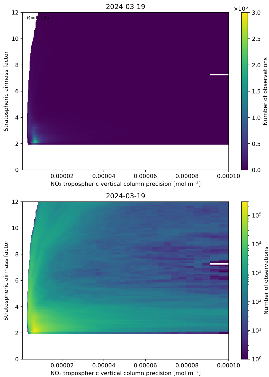
Figure 131: Scatter density plot of “NO 2 tropospheric vertical column precision” against “Stratospheric airmass factor” for 2024-03-18 to 2024-03-20.
