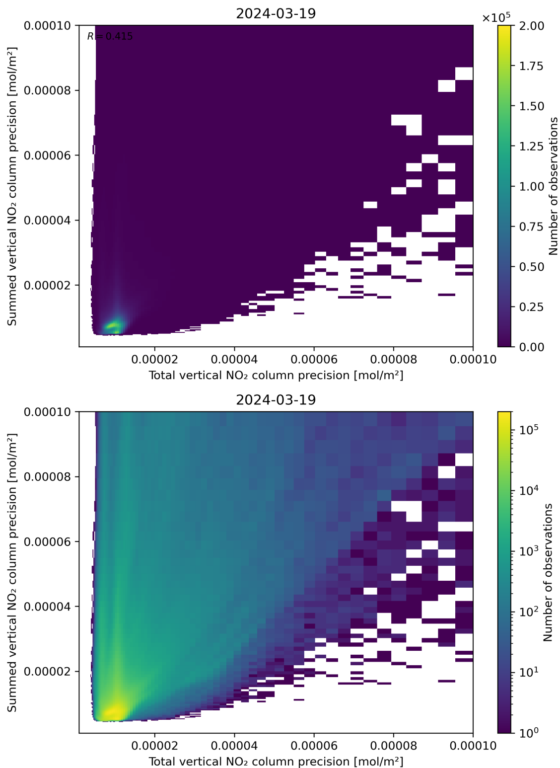
Figure 118: Scatter density plot of “Total vertical NO 2 column precision” against “Summed vertical NO 2 column precision” for 2024-03-18 to 2024-03-20.
