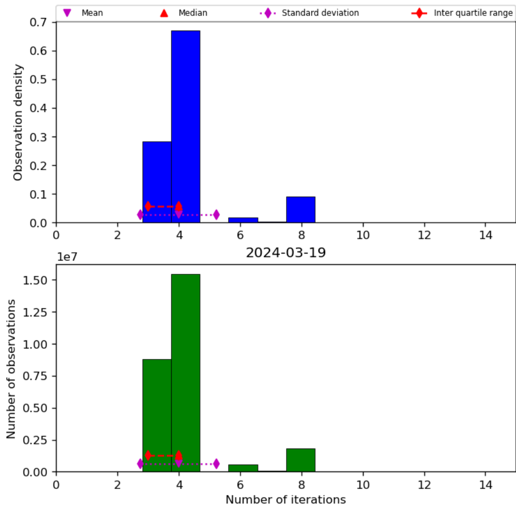
Figure 34: Histogram of “Number of iterations” for 2024-03-18 to 2024-03-20
