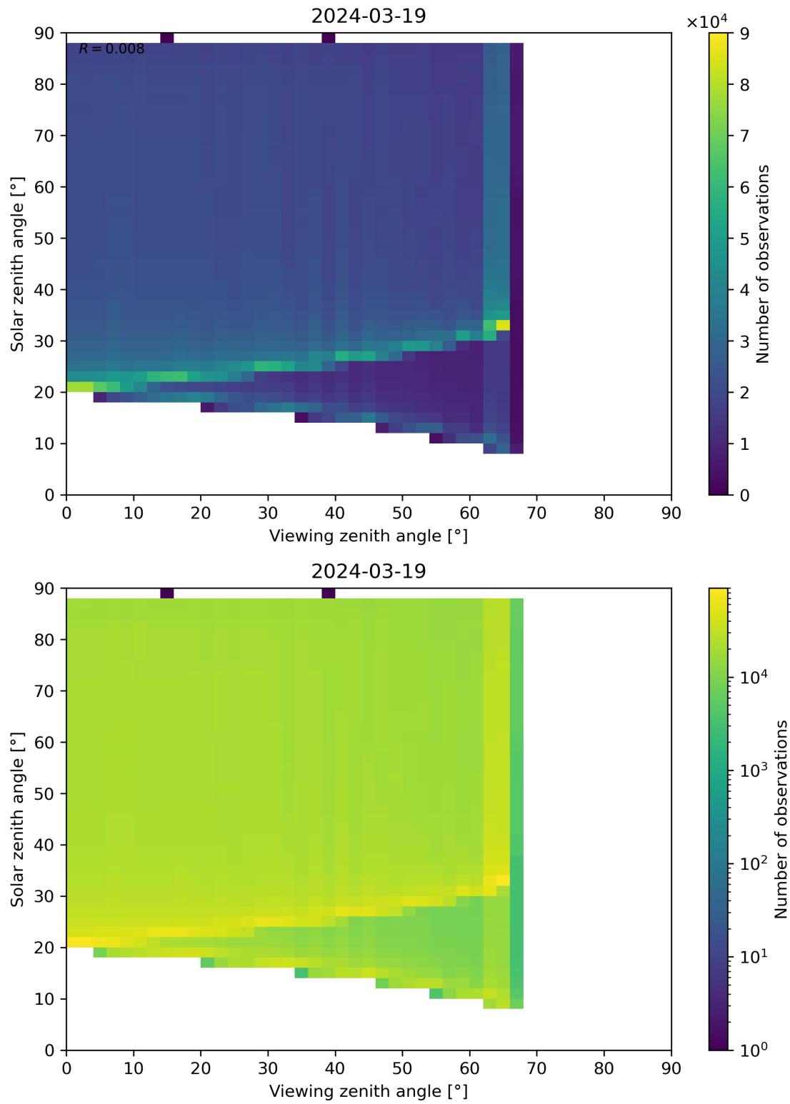
Figure 172: Scatter density plot of “Viewing zenith angle” against “Solar zenith angle” for 2024-03-18 to 2024-03-20.
