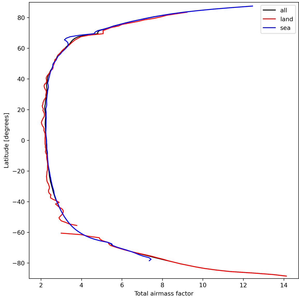
Figure 15: Zonal average of “Total airmass factor” for 2024-03-18 to 2024-03-20.
