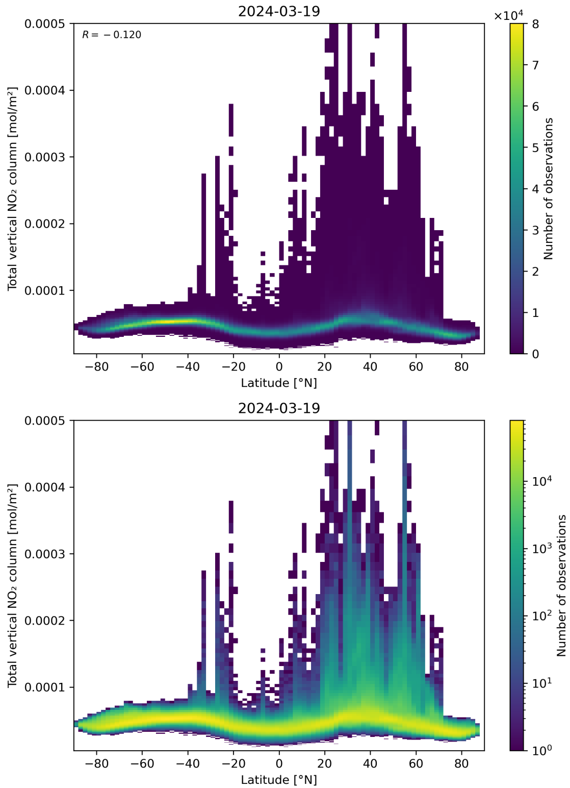
Figure 90: Scatter density plot of “Latitude” against “Total vertical NO 2 column” for 2024-03-18 to 2024-03-20.
