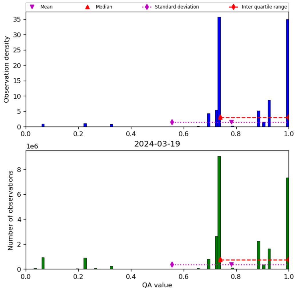
Figure 28: Histogram of “QA value” for 2024-03-18 to 2024-03-20
