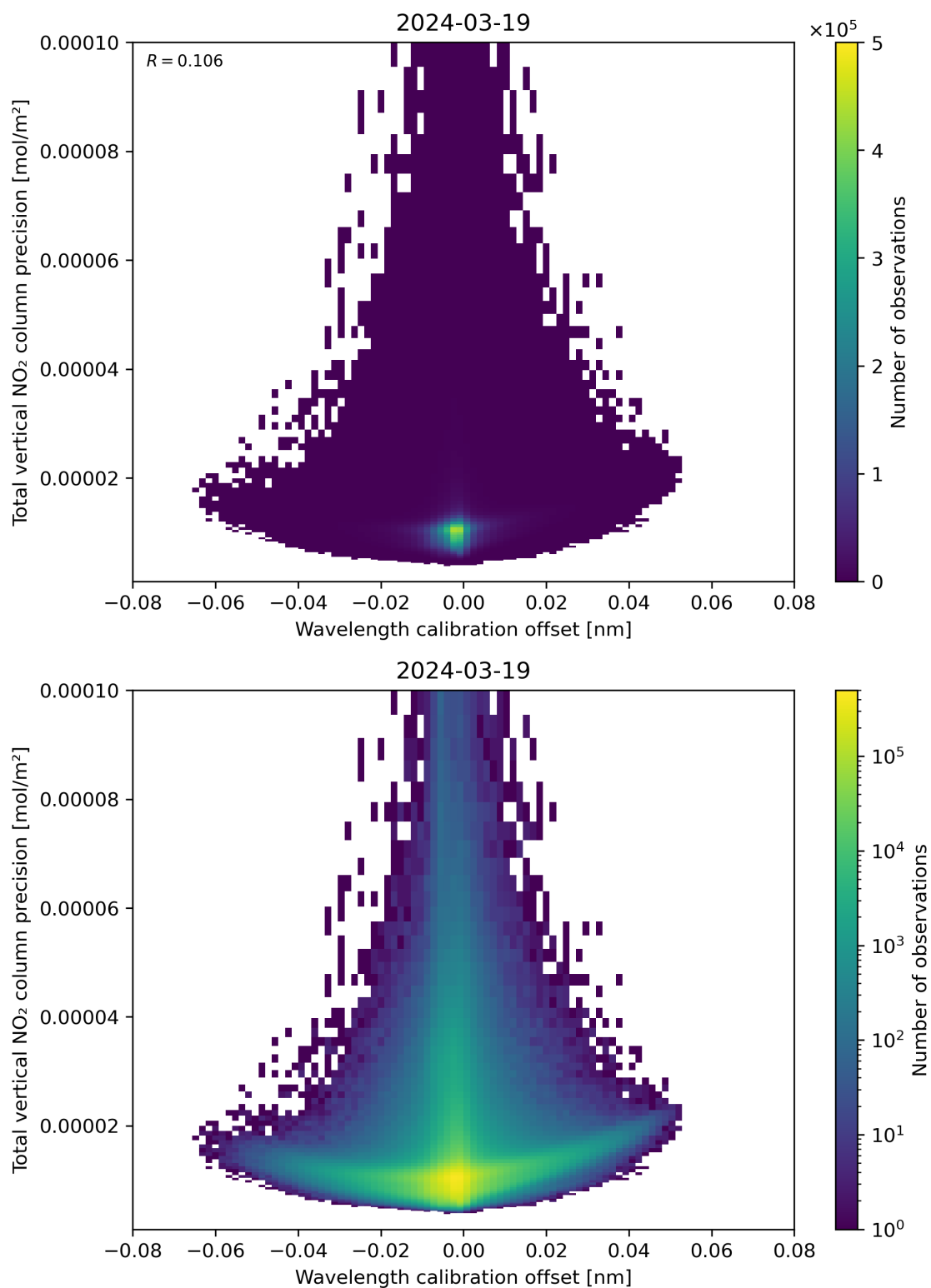
Figure 180: Scatter density plot of “Wavelength calibration offset” against “Total vertical NO 2 column precision” for 2024-03-18 to 2024-03-20.
