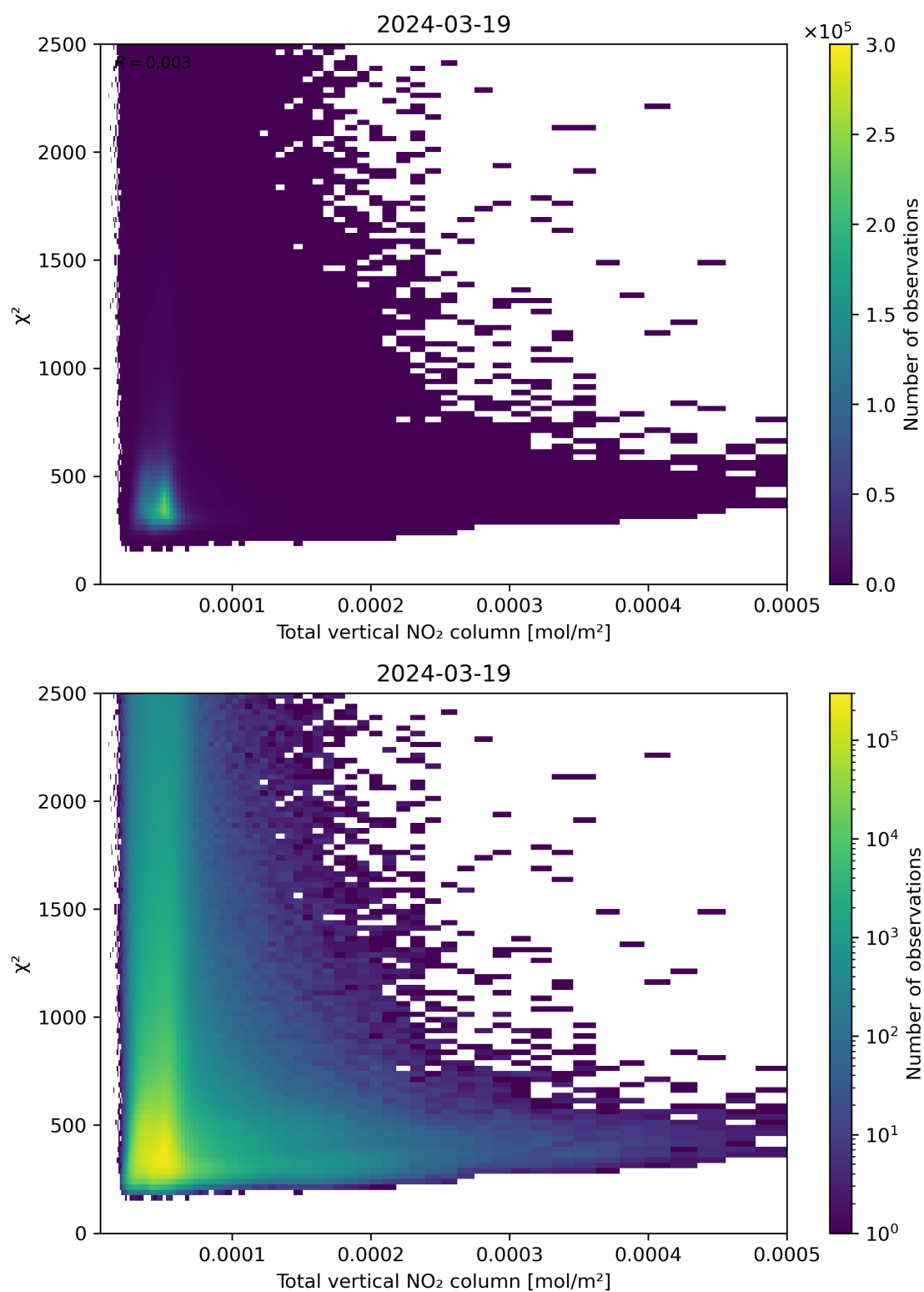
Figure 111: Scatter density plot of “Total vertical NO 2 column” against “ \chi^2 ” for 2024-03-18 to 2024-03-20.
