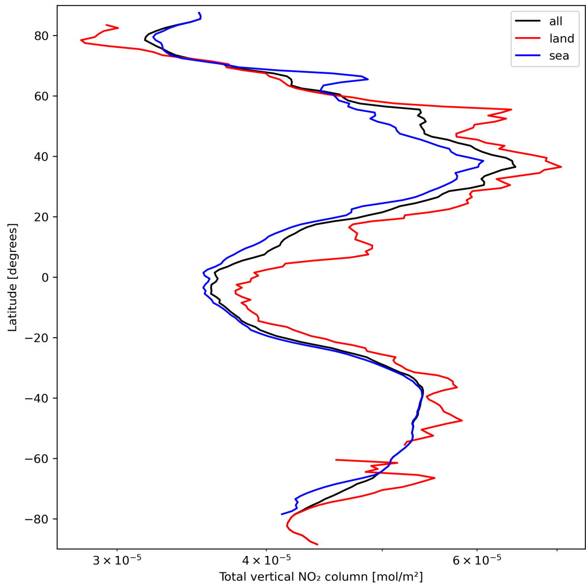
Figure 21: Zonal average of “Total vertical NO 2 column” for 2024-03-18 to 2024-03-20.
