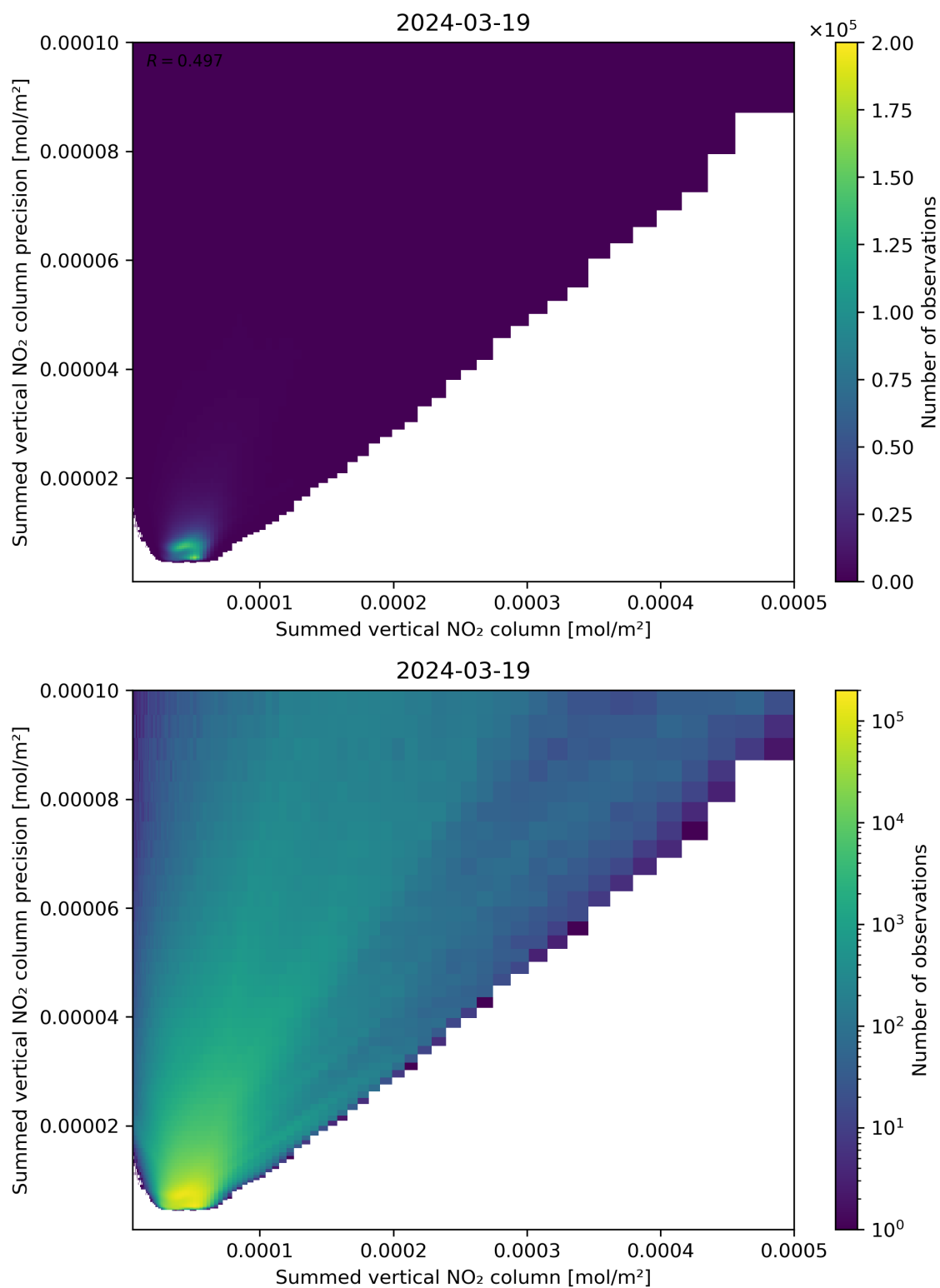
Figure 105: Scatter density plot of “Summed vertical NO 2 column” against “Summed vertical NO 2 column precision” for 2024-03-18 to 2024-03-20.
