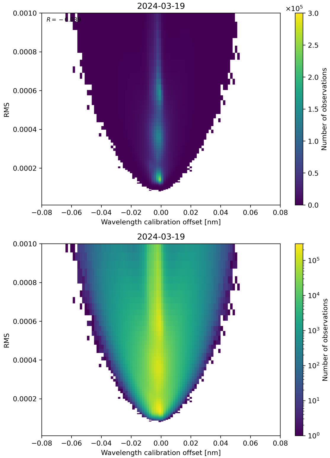
Figure 181: Scatter density plot of “Wavelength calibration offset” against “RMS” for 2024-03-18 to 2024-03-20.
