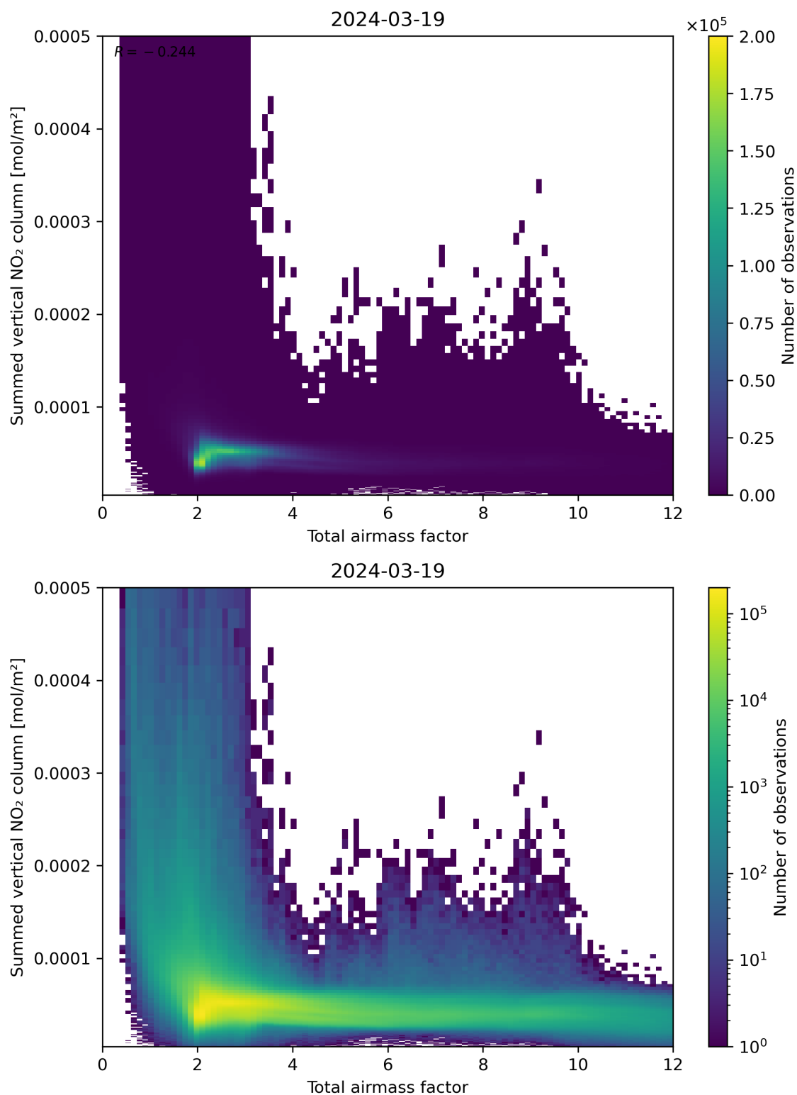
Figure 65: Scatter density plot of “Total airmass factor” against “Summed vertical NO 2 column” for 2024-03-18 to 2024-03-20.
