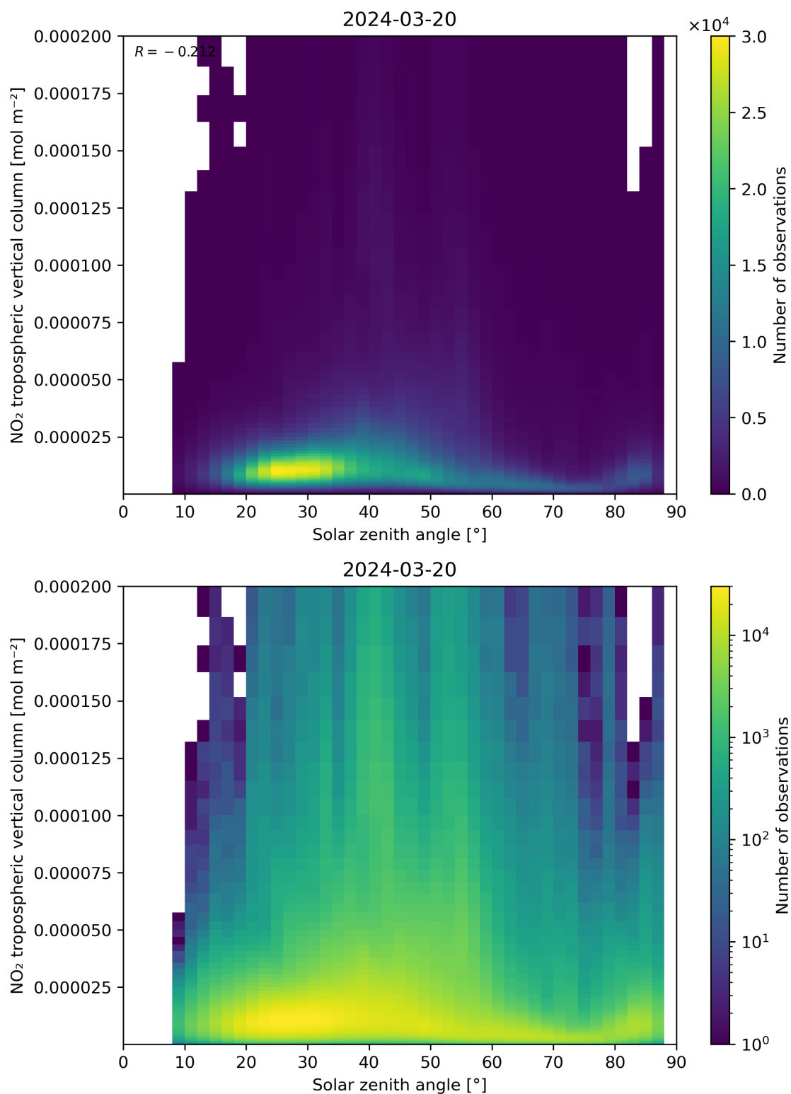
Figure 155: Scatter density plot of “Solar zenith angle” against “NO 2 tropospheric vertical column” for 2024-03-20 to 2024-03-21.
