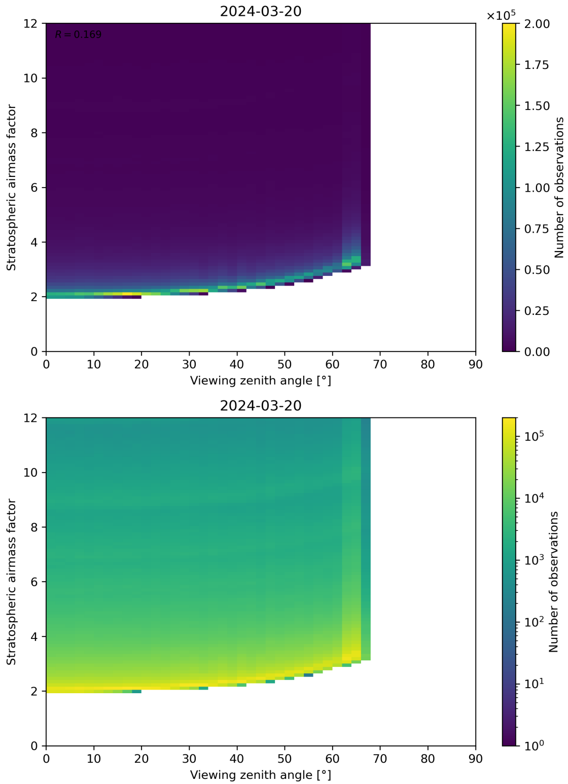
Figure 159: Scatter density plot of “Viewing zenith angle” against “Stratospheric airmass factor” for 2024-03-20 to 2024-03-21.
