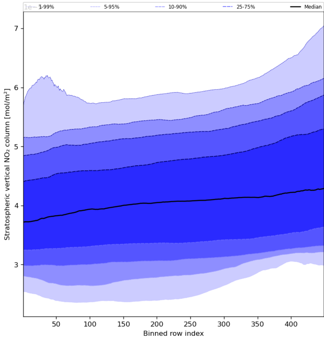
Figure 53: Along track statistics of “Stratospheric vertical NO 2 column” for 2024-03-20 to 2024-03-21
