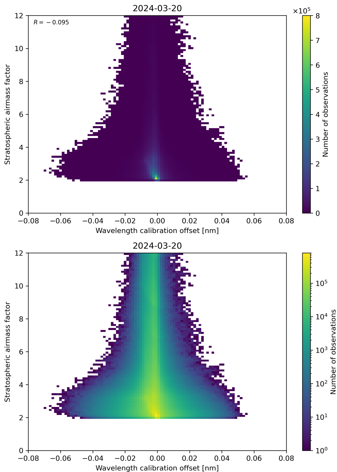
Figure 174: Scatter density plot of “Wavelength calibration offset” against “Stratospheric air mass factor” for 2024-03-20 to 2024-03-21.
