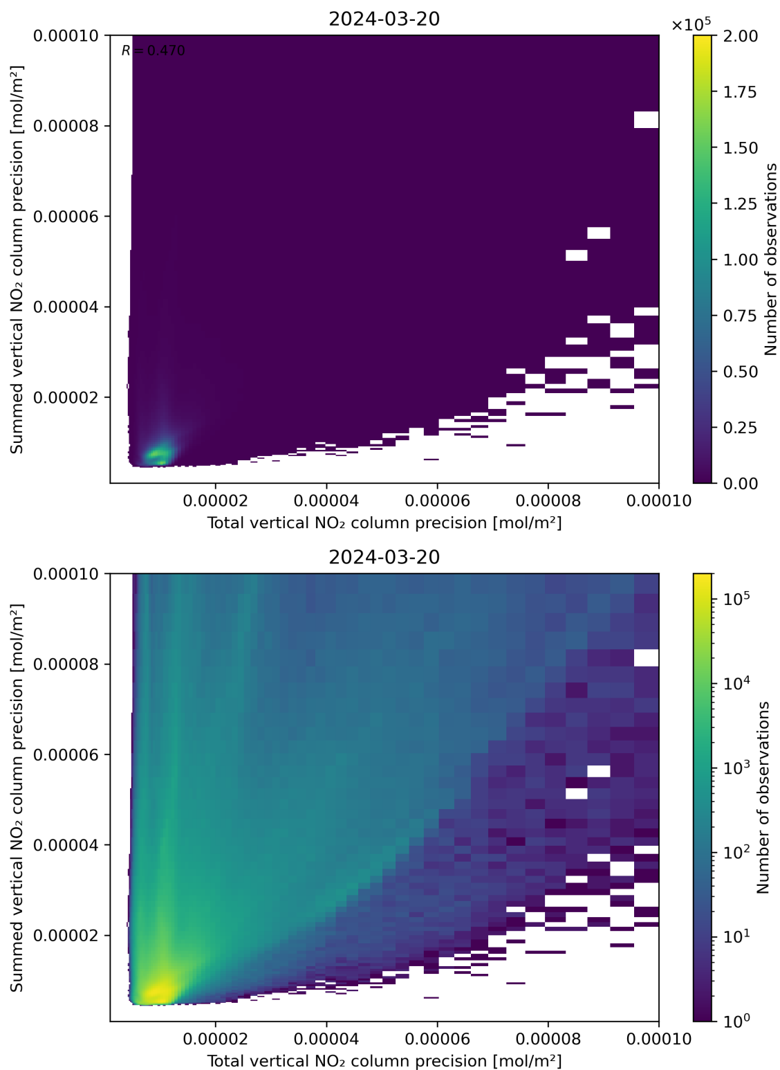
Figure 118: Scatter density plot of “Total vertical NO 2 column precision” against “Summed vertical NO 2 column precision” for 2024-03-20 to 2024-03-21.
