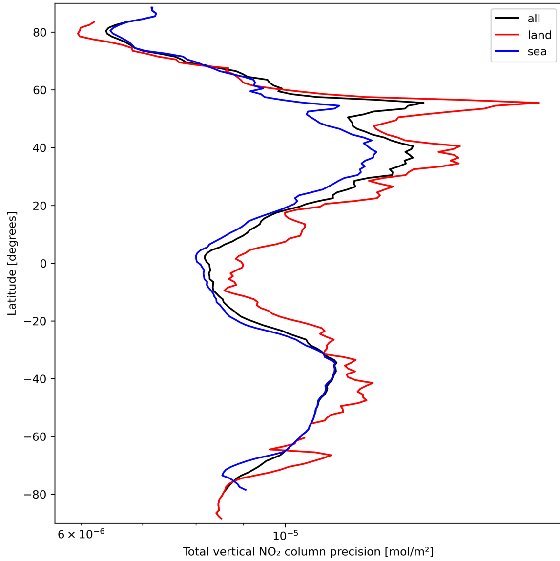
Figure 22: Zonal average of “Total vertical NO 2 column precision” for 2024-03-20 to 2024-03-21.
