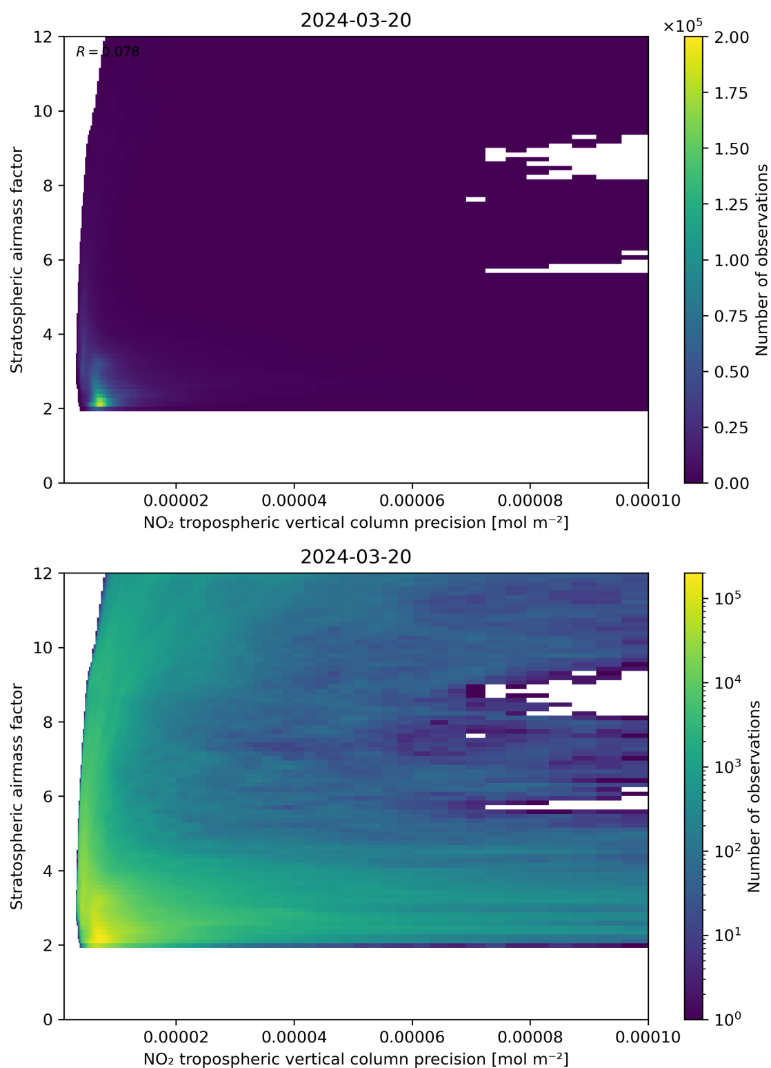
Figure 131: Scatter density plot of “NO 2 tropospheric vertical column precision” against “Stratospheric airmass factor” for 2024-03-20 to 2024-03-21.
