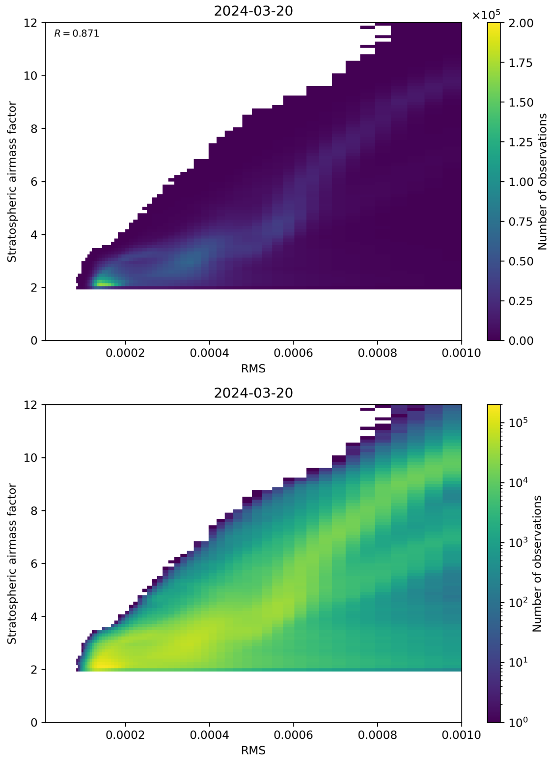
Figure 144: Scatter density plot of “RMS” against “Stratospheric airmass factor” for 2024-03-20 to 2024-03-21.
