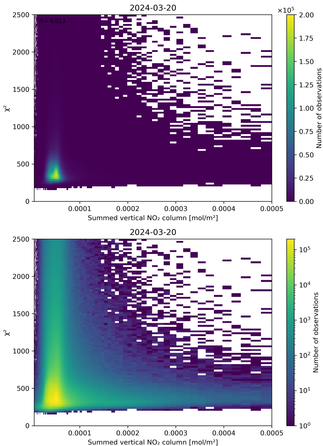
Figure 104: Scatter density plot of “Summed vertical NO 2 column” against “ \chi^2 ” for 2024-03-20 to 2024-03-21.
