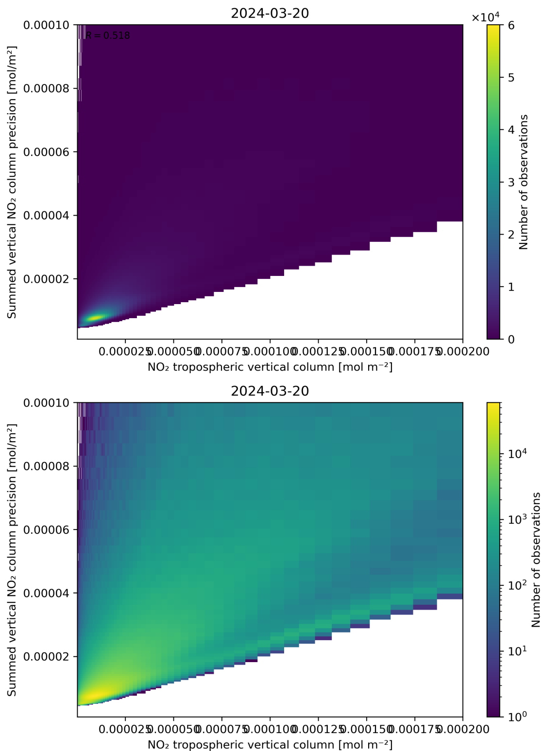
Figure 127: Scatter density plot of “NO 2 tropospheric vertical column” against “Summed vertical NO 2 column precision” for 2024-03-20 to 2024-03-21.
