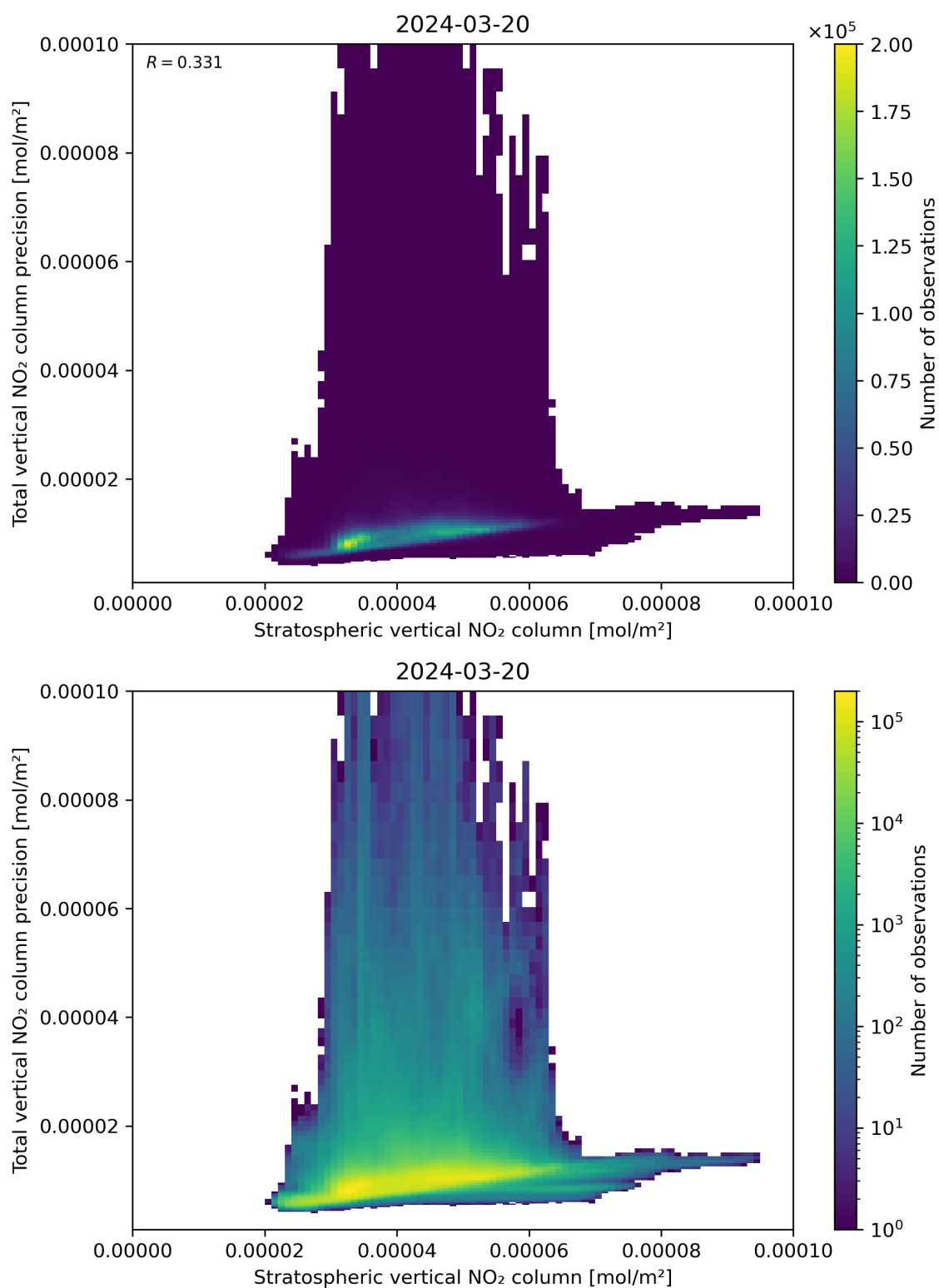
Figure 101: Scatter density plot of “Stratospheric vertical NO 2 column” against “Total vertical NO 2 column precision” for 2024-03-20 to 2024-03-21.
