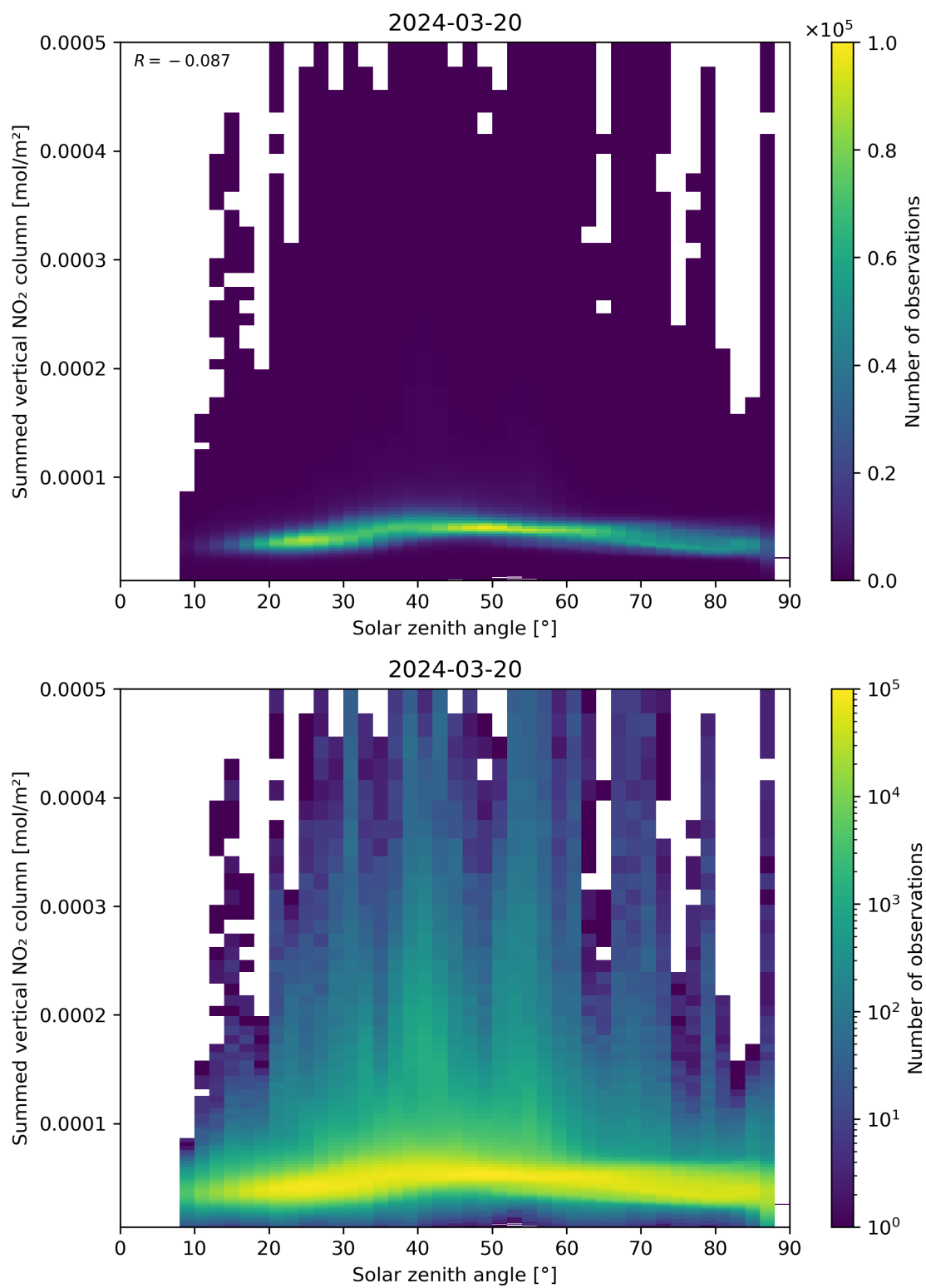
Figure 151: Scatter density plot of “Solar zenith angle” against “Summed vertical NO 2 column” for 2024-03-20 to 2024-03-21.
