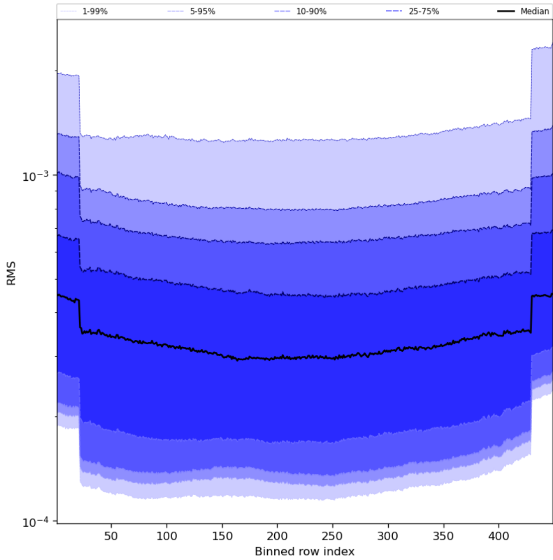
Figure 60: Along track statistics of “RMS” for 2024-03-20 to 2024-03-21
