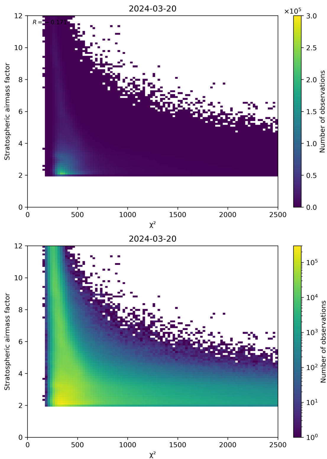
Figure 81: Scatter density plot of “ \chi^2 ” against “Stratospheric airmass factor” for 2024-03-20 to 2024-03-21.
