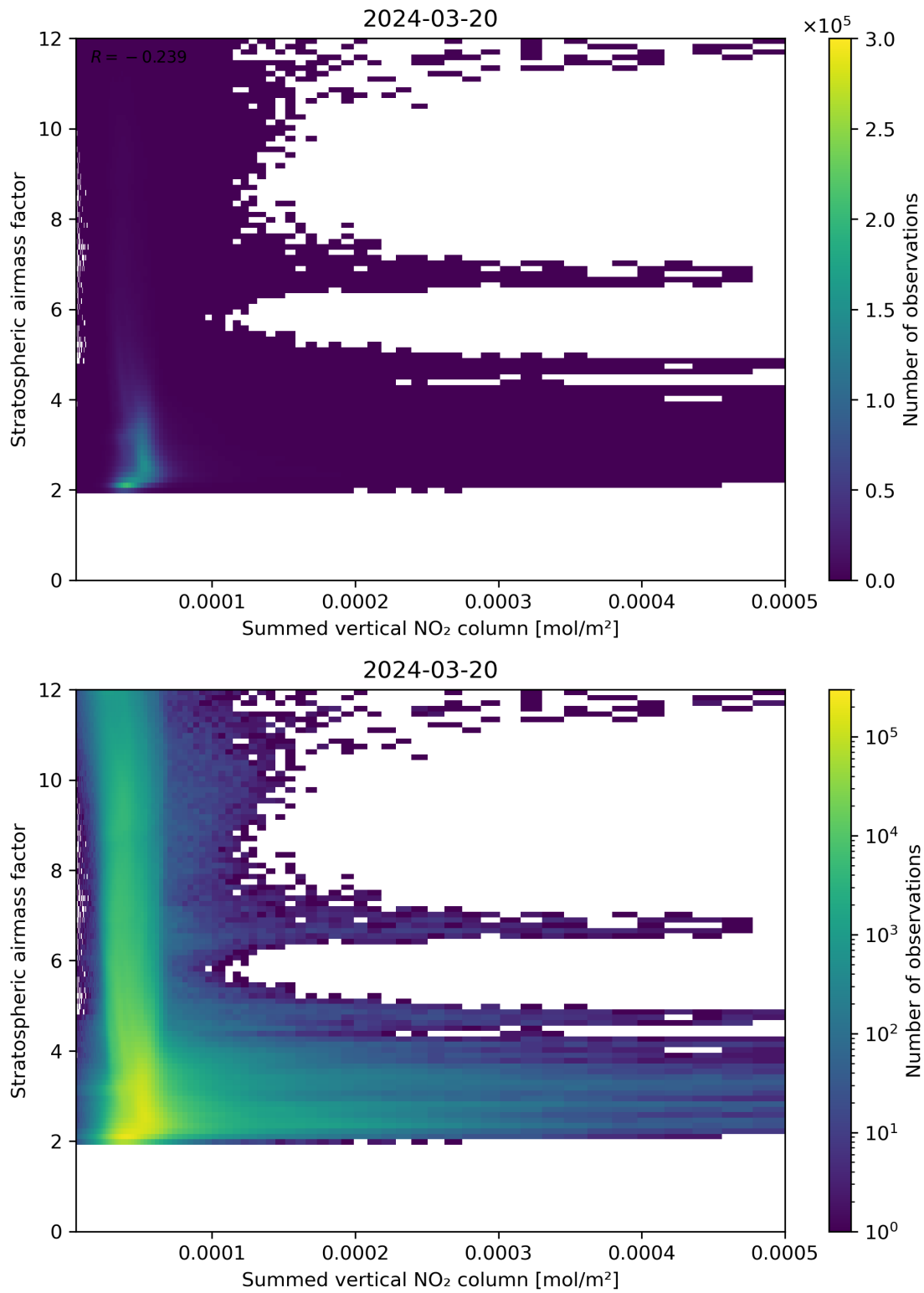
Figure 103: Scatter density plot of “Summed vertical NO 2 column” against “Stratospheric airmass factor” for 2024-03-20 to 2024-03-21.
