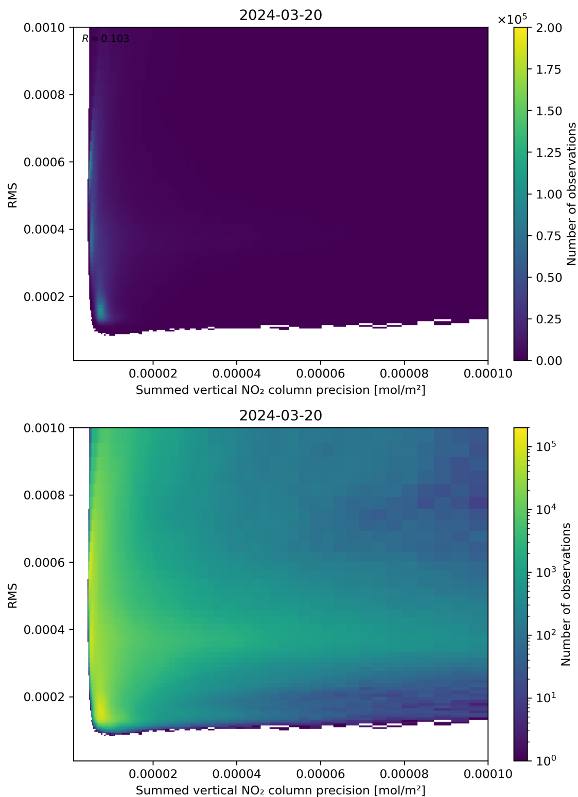
Figure 108: Scatter density plot of “Summed vertical NO 2 column precision” against “RMS” for 2024-03-20 to 2024-03-21.
