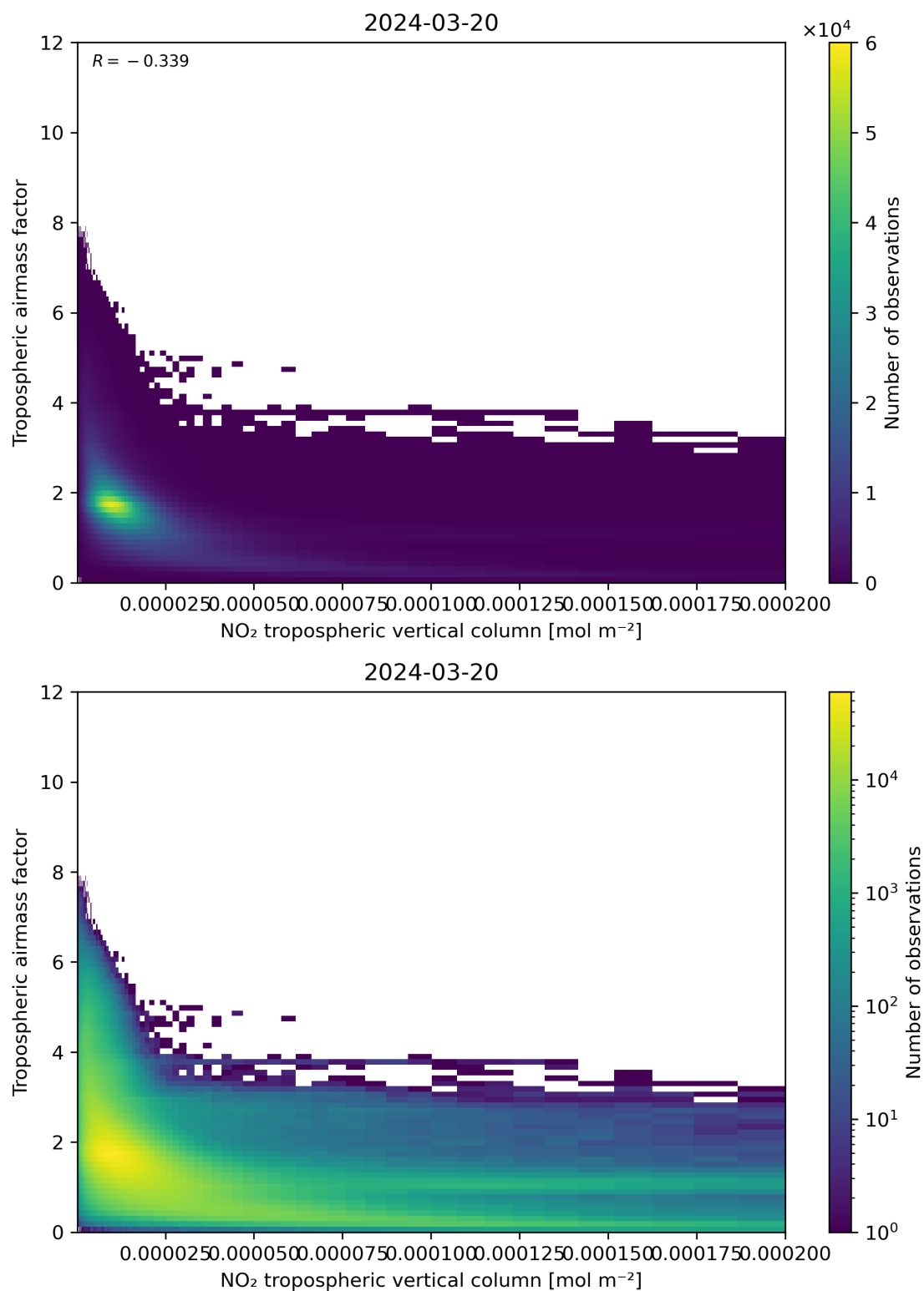
Figure 123: Scatter density plot of “NO 2 tropospheric vertical column” against “Tropospheric air mass factor” for 2024-03-20 to 2024-03-21.
