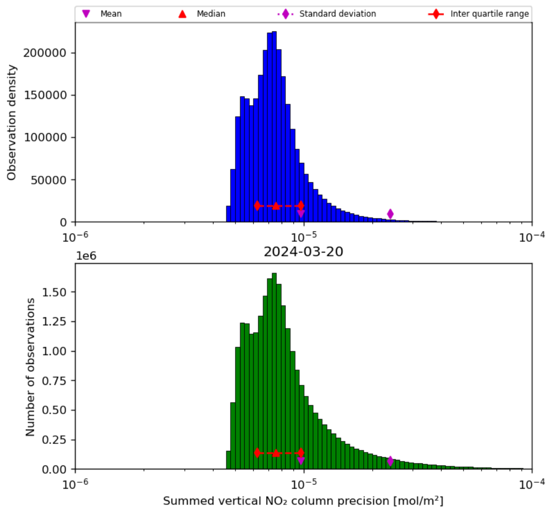
Figure 41: Histogram of “Summed vertical NO 2 column precision” for 2024-03-20 to 2024-03-21
