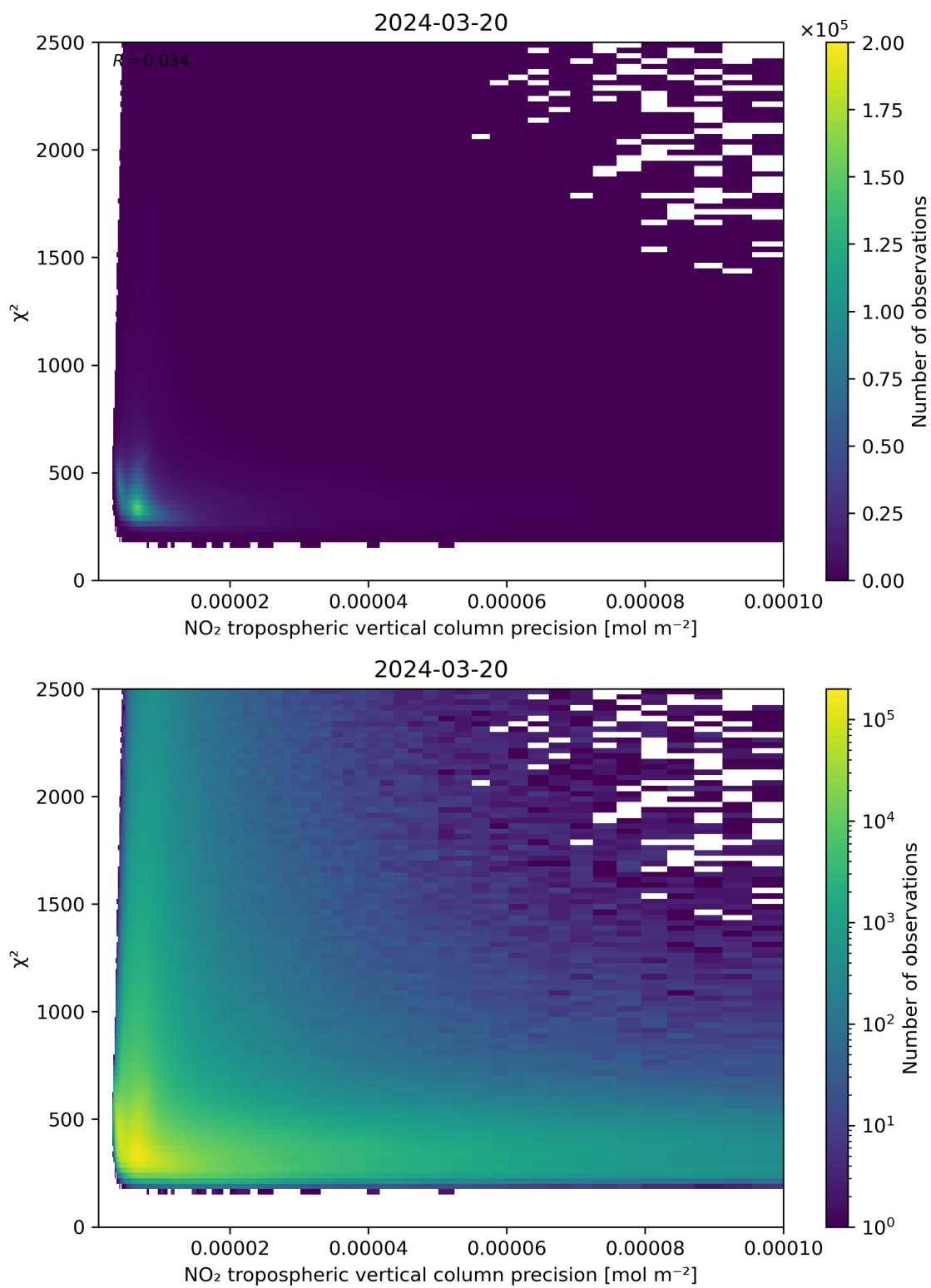
Figure 134: Scatter density plot of “NO 2 tropospheric vertical column precision” against “ \chi^2 ” for 2024-03-20 to 2024-03-21.
