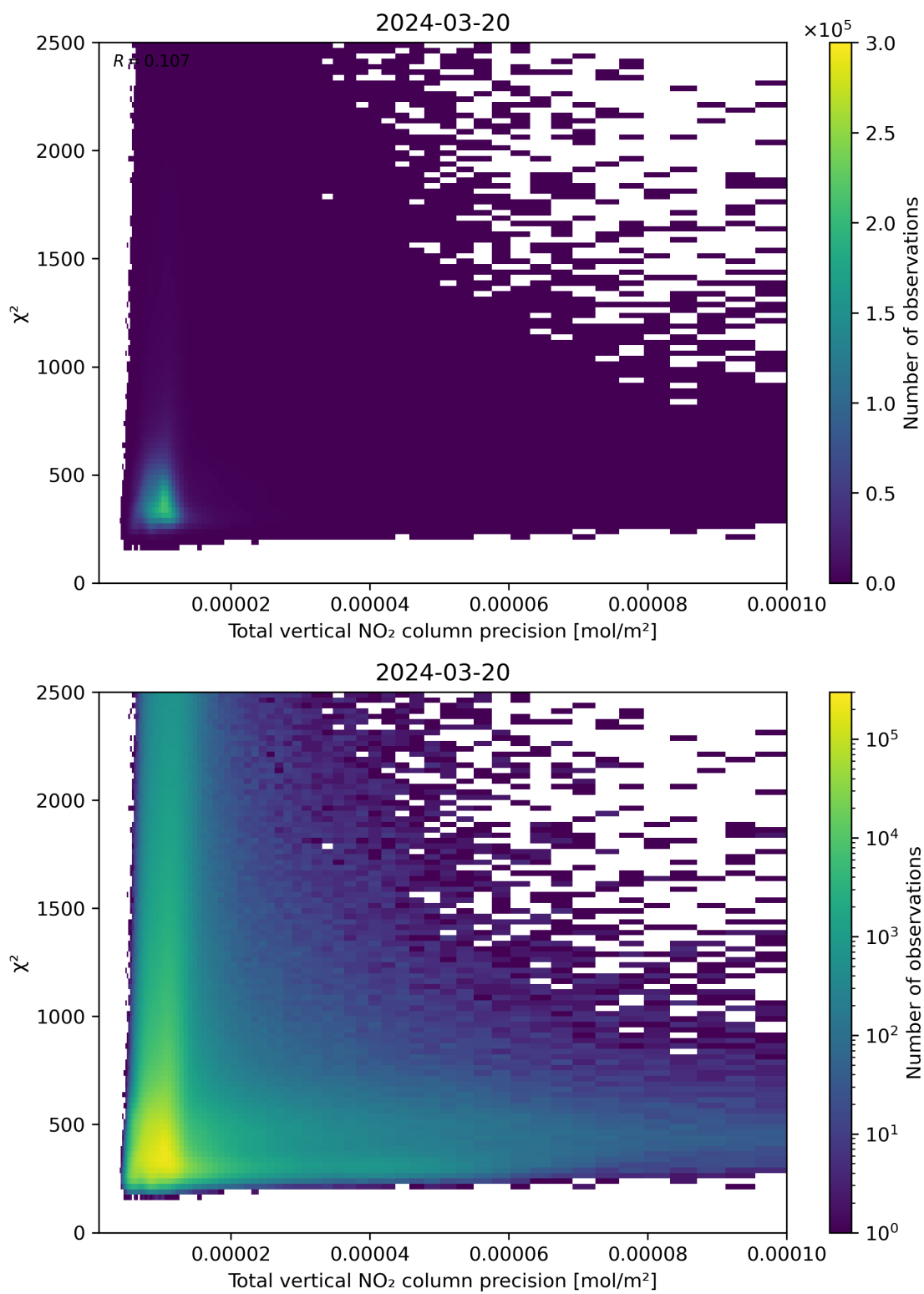
Figure 116: Scatter density plot of “Total vertical NO 2 column precision” against “ \chi^2 ” for 2024-03-20 to 2024-03-21.
