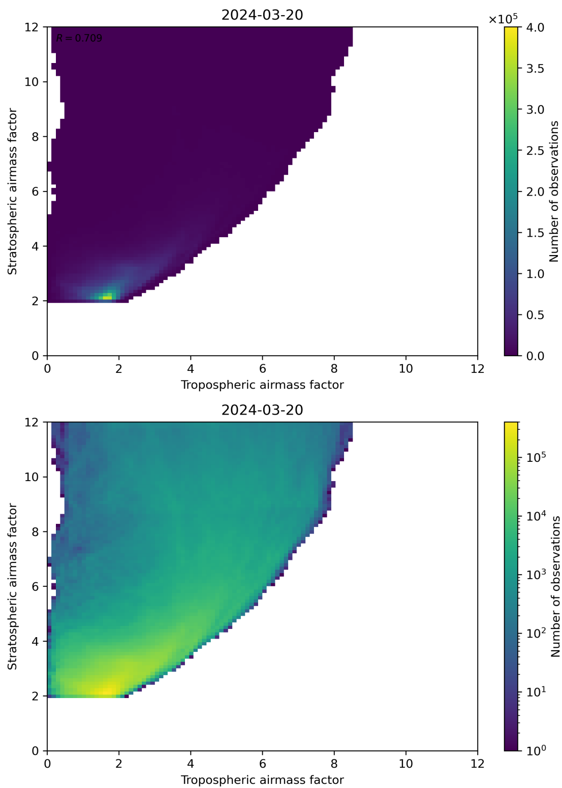
Figure 71: Scatter density plot of “Tropospheric airmass factor” against “Stratospheric airmass factor” for 2024-03-20 to 2024-03-21.
