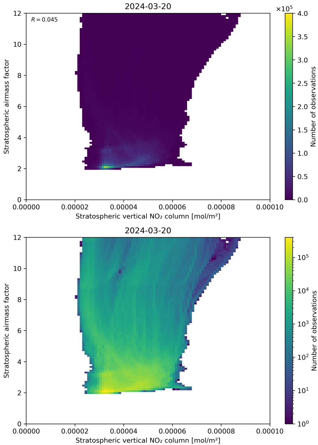
Figure 96: Scatter density plot of “Stratospheric vertical NO 2 column” against “Stratospheric airmass factor” for 2024-03-20 to 2024-03-21.
