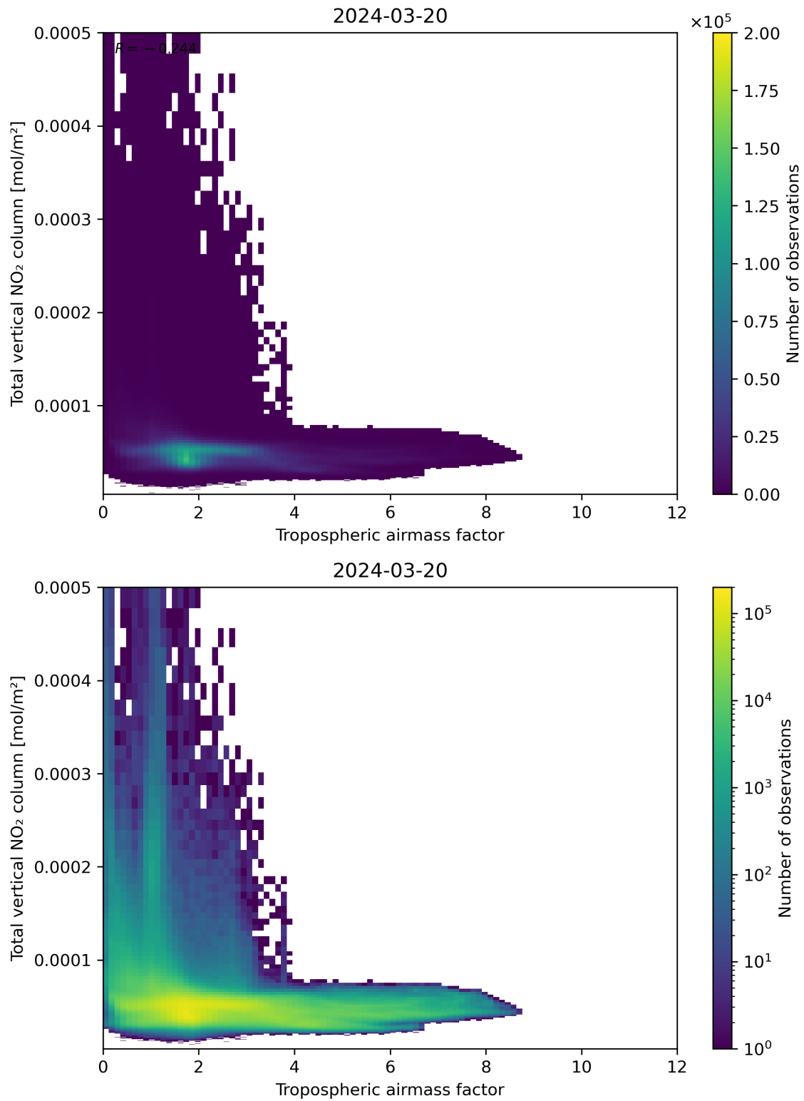
Figure 77: Scatter density plot of “Tropospheric airmass factor” against “Total vertical NO 2 column” for 2024-03-20 to 2024-03-21.
