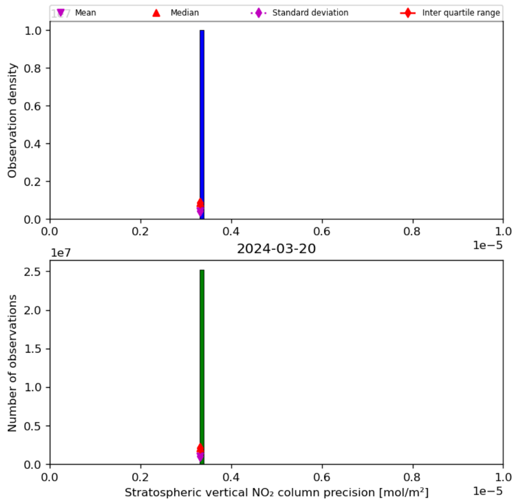
Figure 37: Histogram of “Stratospheric vertical NO 2 column precision” for 2024-03-20 to 2024-03-21
