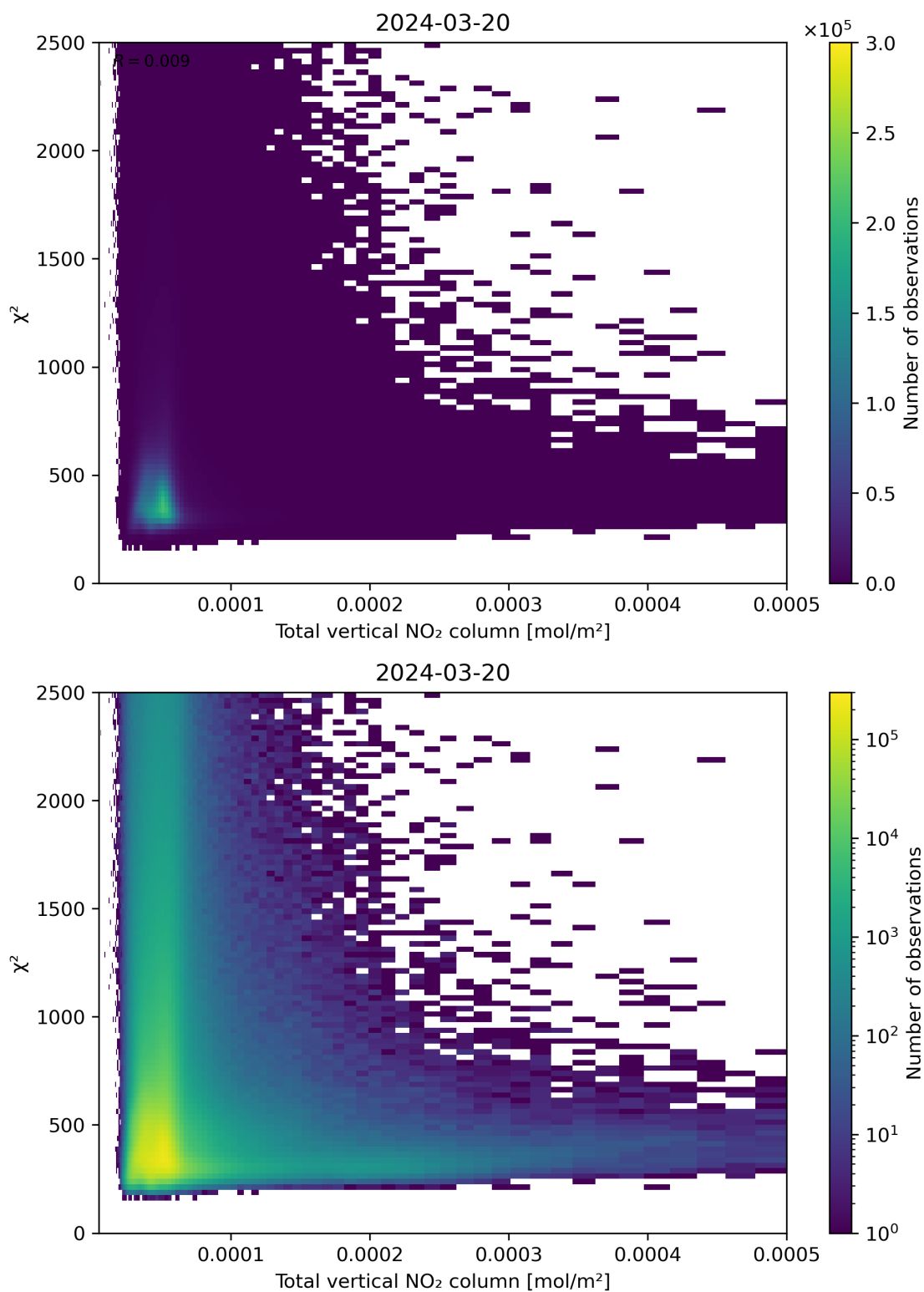
Figure 111: Scatter density plot of “Total vertical NO 2 column” against “ \chi^2 ” for 2024-03-20 to 2024-03-21.
