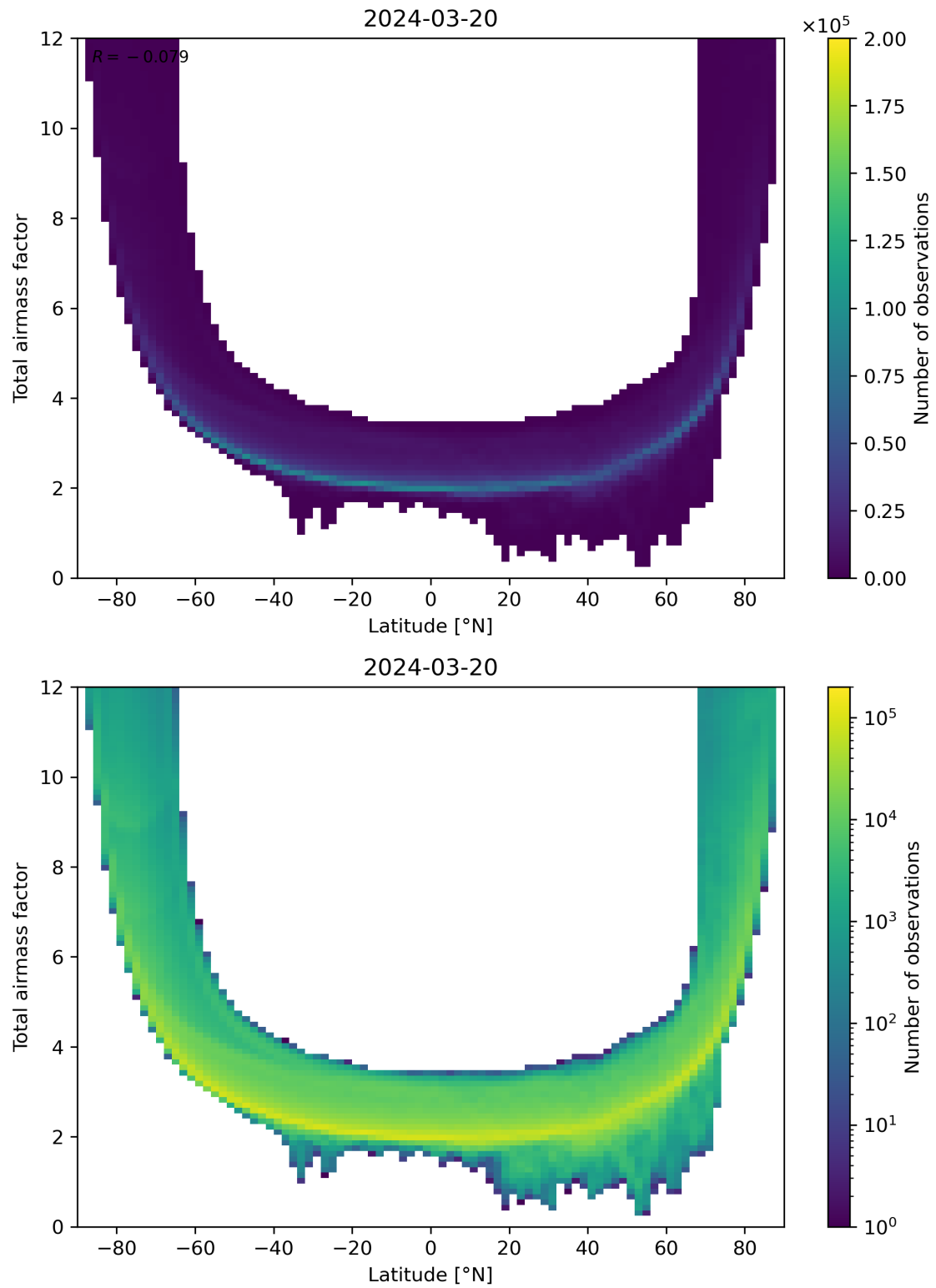
Figure 84: Scatter density plot of “Latitude” against “Total airmass factor” for 2024-03-20 to 2024-03-21.
