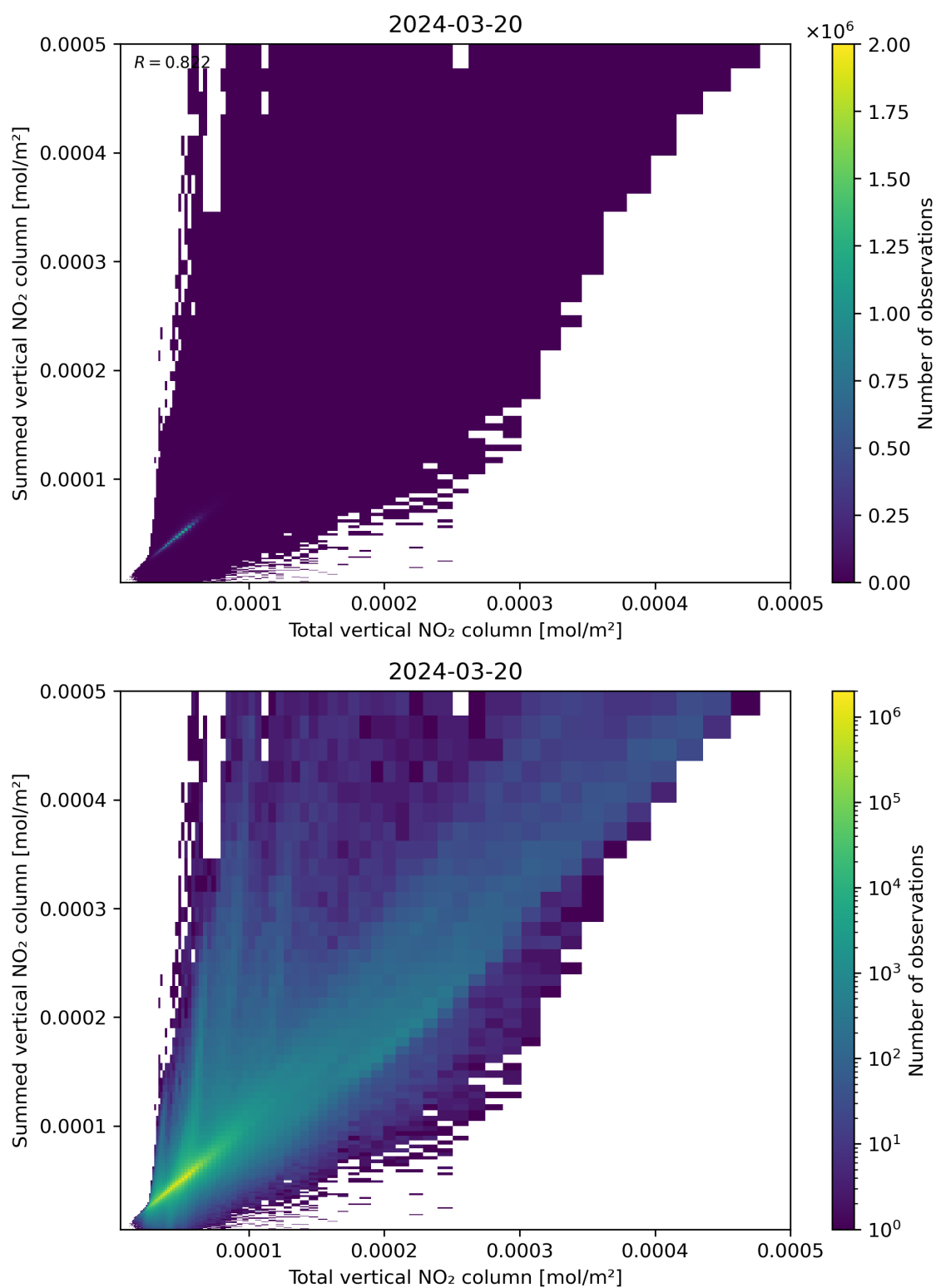
Figure 112: Scatter density plot of “Total vertical NO 2 column” against “Summed vertical NO 2 column” for 2024-03-20 to 2024-03-21.
