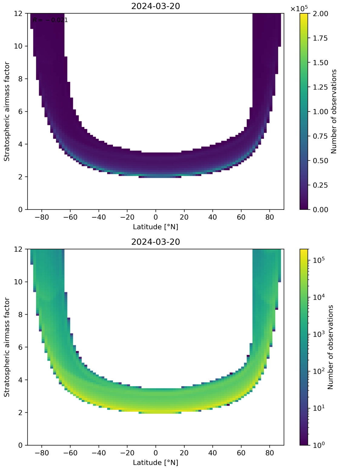
Figure 83: Scatter density plot of “Latitude” against “Stratospheric air mass factor” for 2024-03-20 to 2024-03-21.
