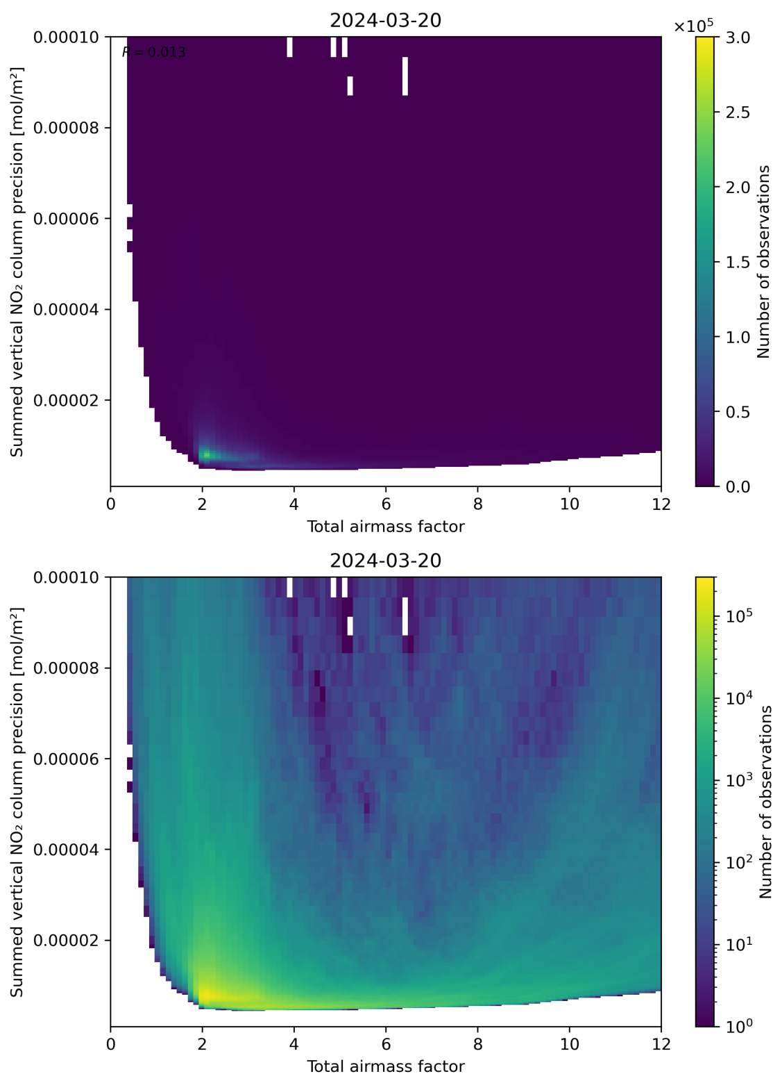
Figure 66: Scatter density plot of “Total airmass factor” against “Summed vertical NO 2 column precision” for 2024-03-20 to 2024-03-21.
