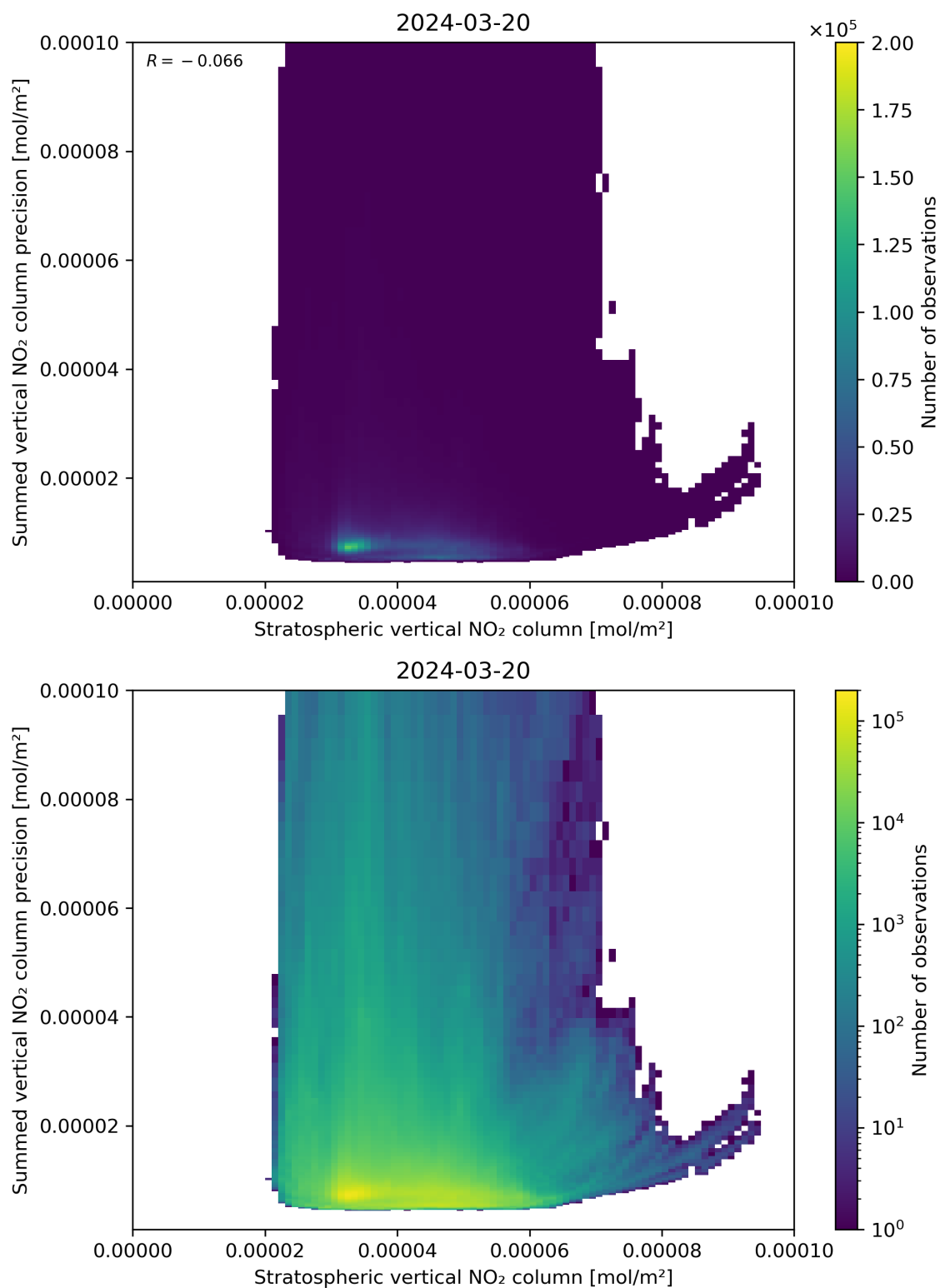
Figure 99: Scatter density plot of “Stratospheric vertical NO 2 column” against “Summed vertical NO 2 column precision” for 2024-03-20 to 2024-03-21.
