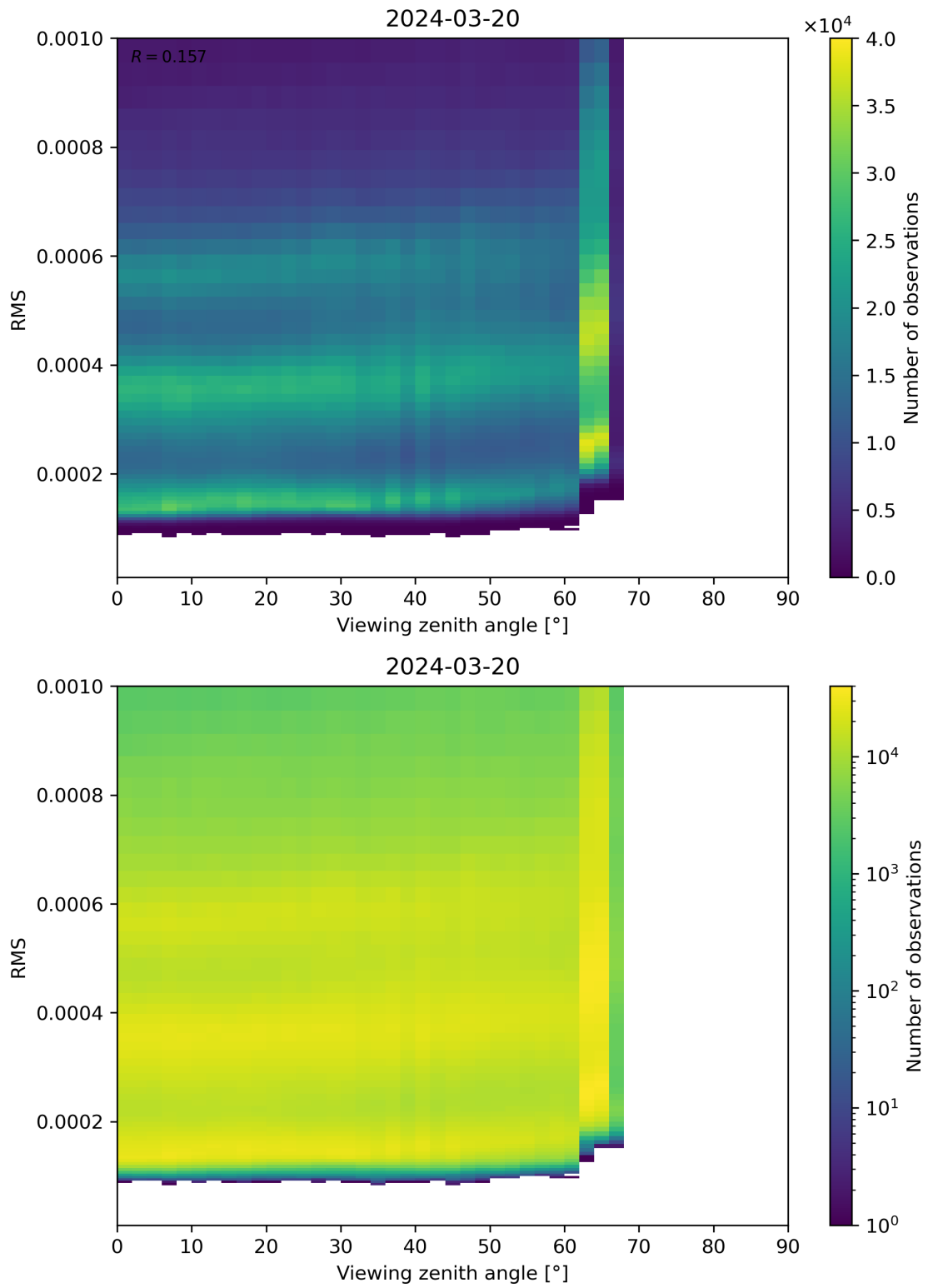
Figure 171: Scatter density plot of “Viewing zenith angle” against “RMS” for 2024-03-20 to 2024-03-21.
