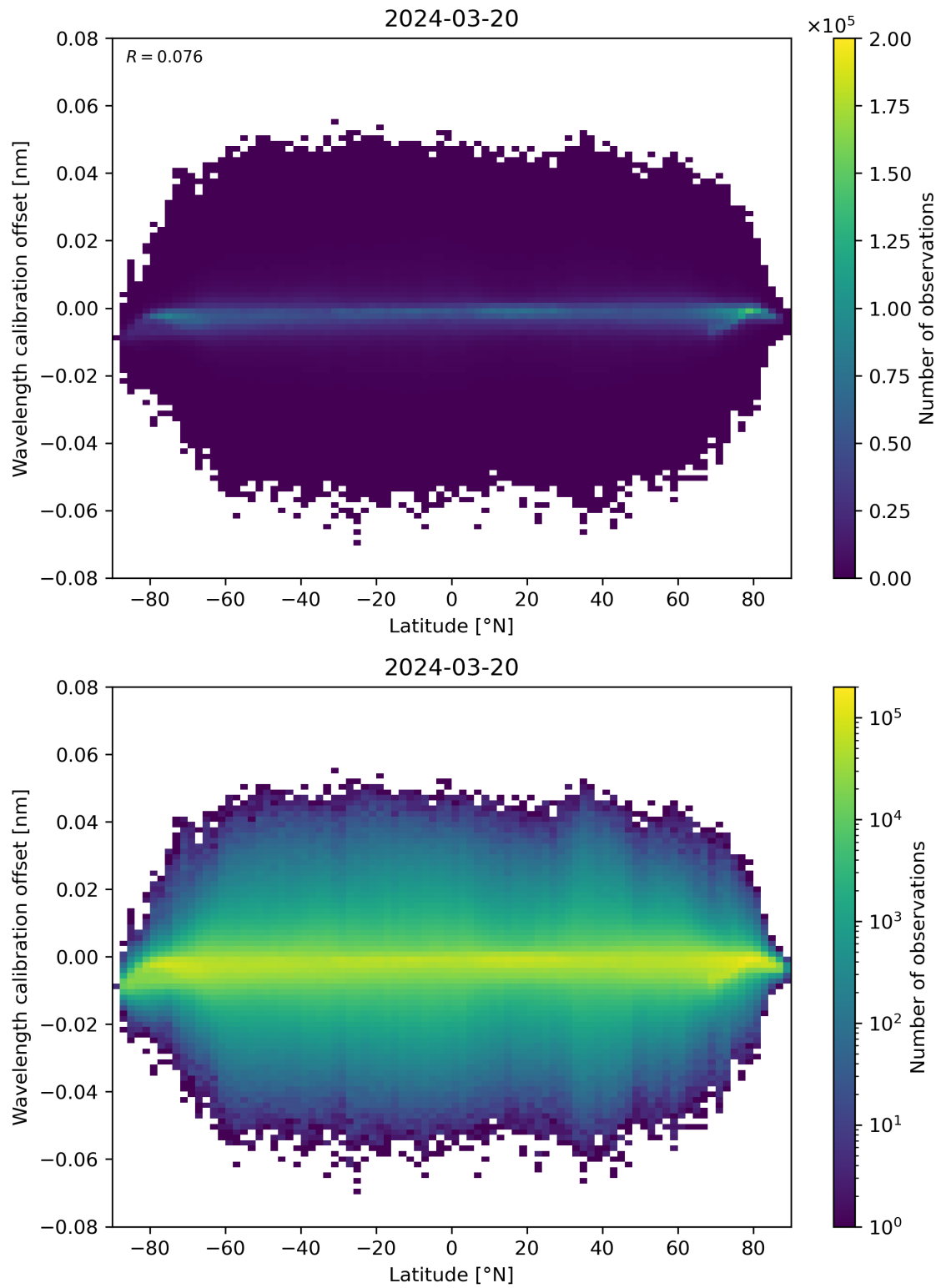
Figure 95: Scatter density plot of “Latitude” against “Wavelength calibration offset” for 2024-03-20 to 2024-03-21.
