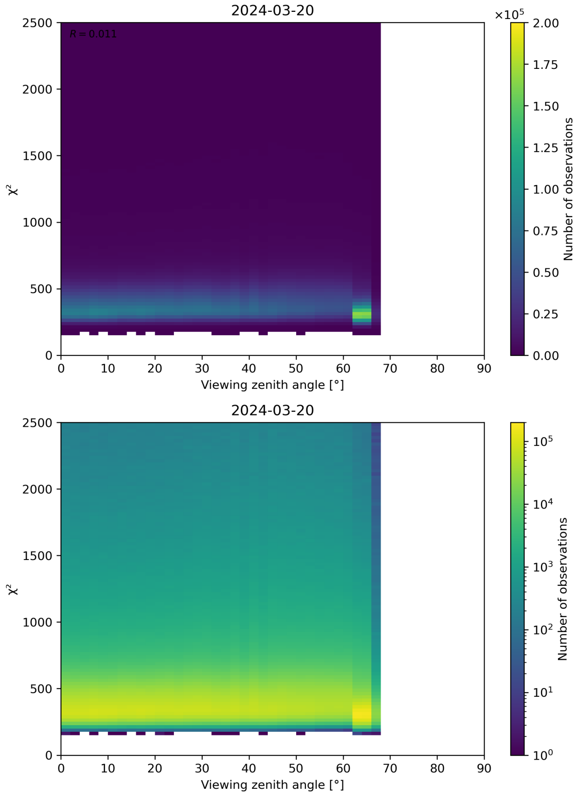
Figure 162: Scatter density plot of “Viewing zenith angle” against “ \chi^2 ” for 2024-03-20 to 2024-03-21.
