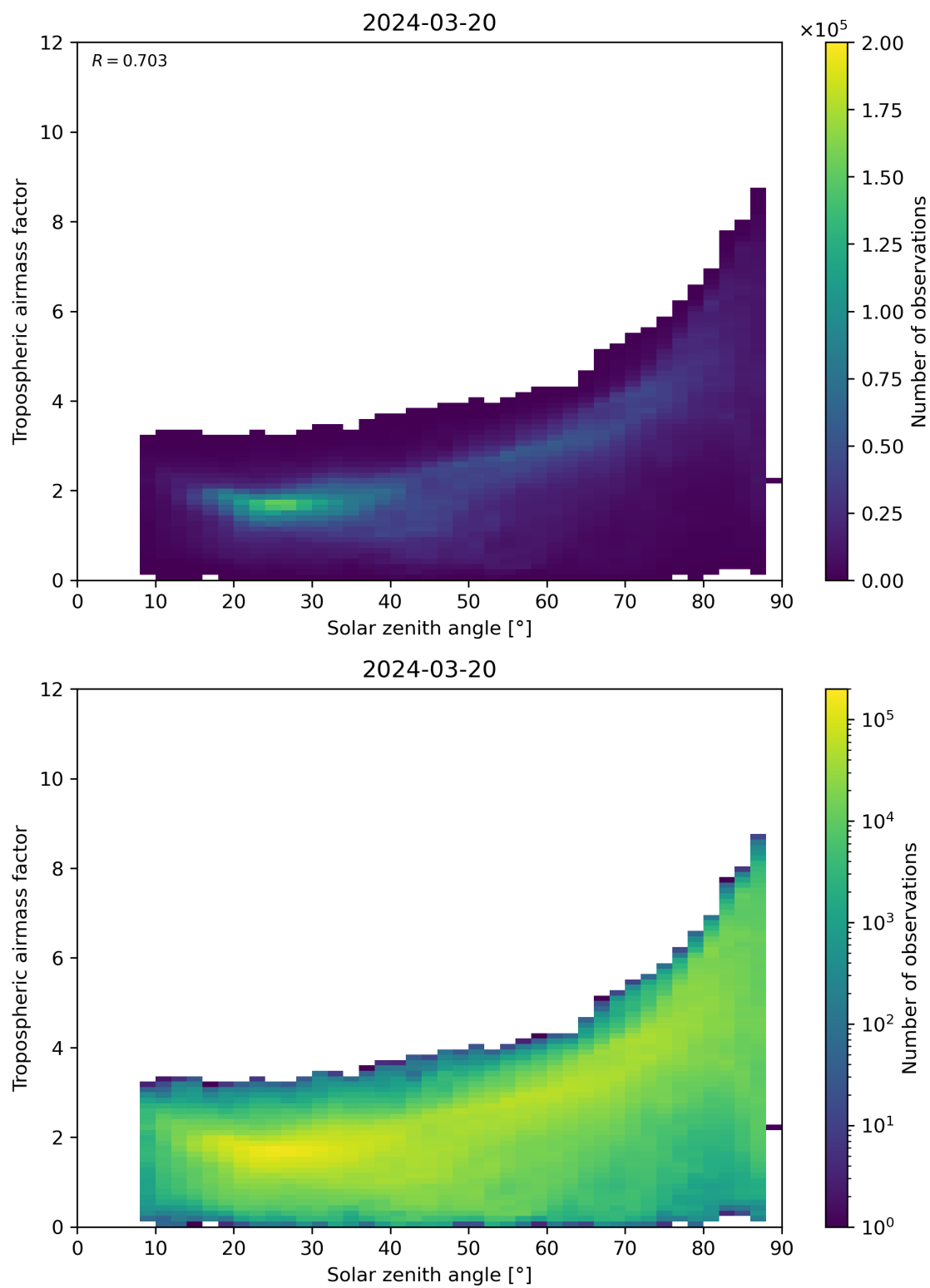
Figure 147: Scatter density plot of “Solar zenith angle” against “Tropospheric airmass factor” for 2024-03-20 to 2024-03-21.
