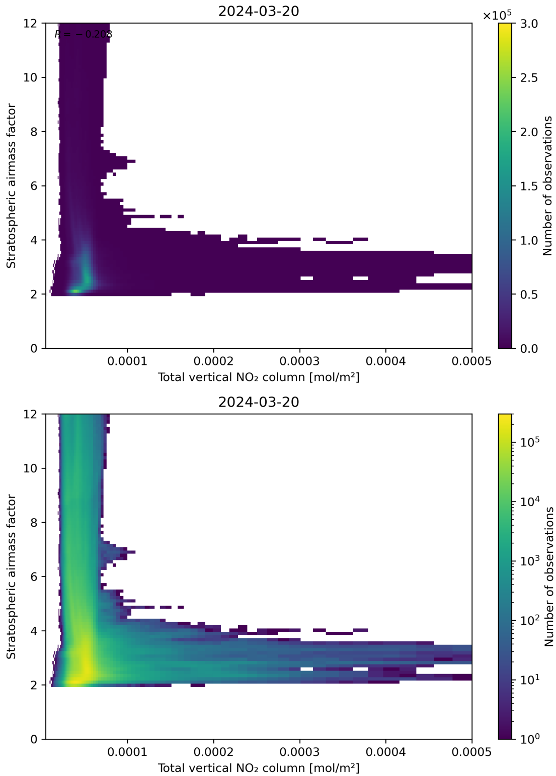
Figure 110: Scatter density plot of “Total vertical NO 2 column” against “Stratospheric air mass factor” for 2024-03-20 to 2024-03-21.
