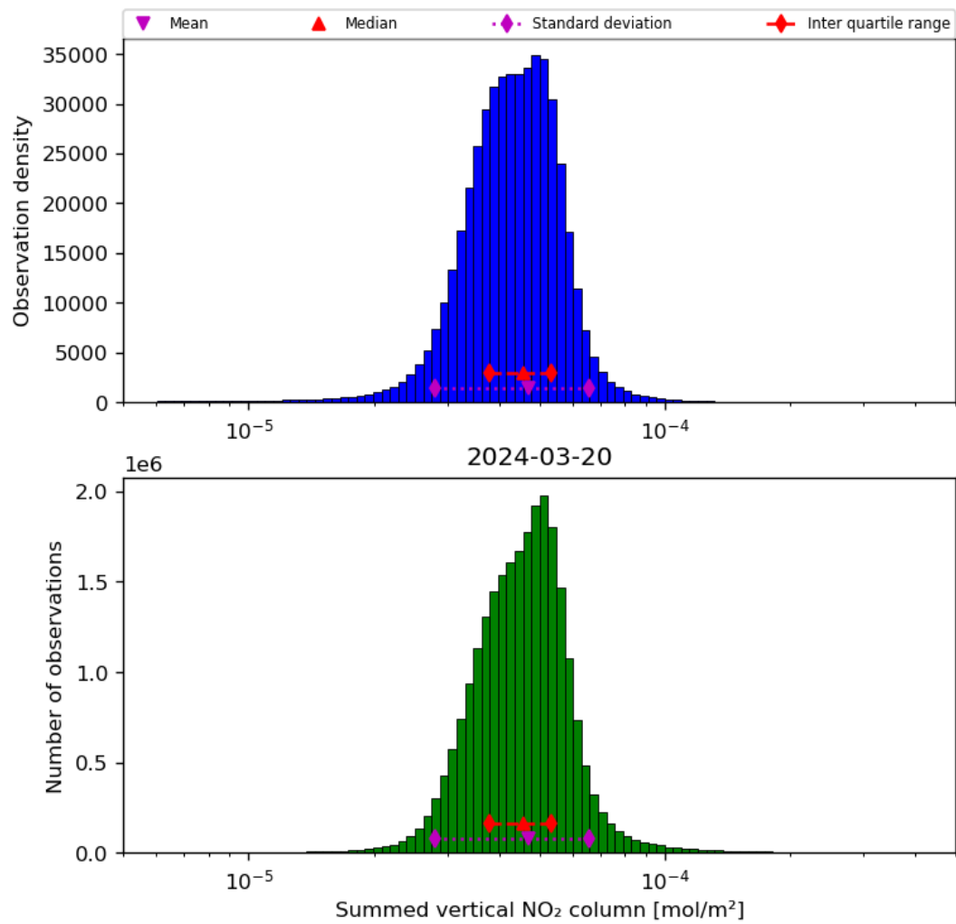
Figure 40: Histogram of “Summed vertical NO 2 column” for 2024-03-20 to 2024-03-21
