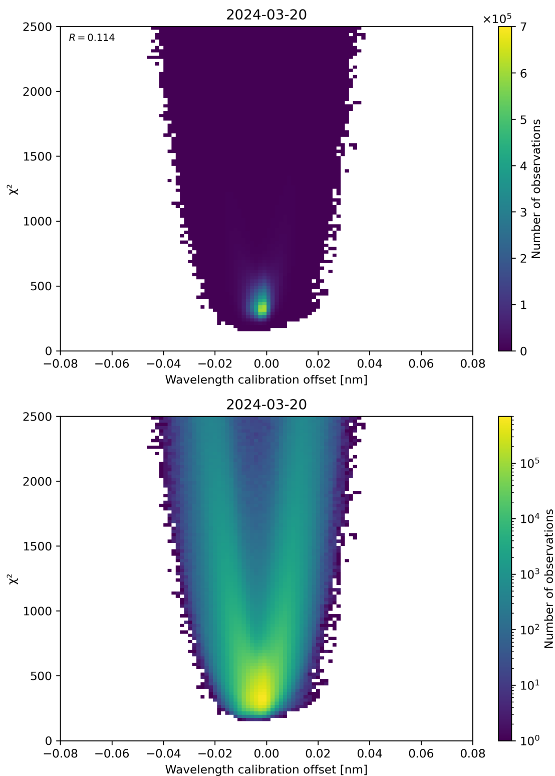
Figure 175: Scatter density plot of “Wavelength calibration offset” against “ \chi^2 ” for 2024-03-20 to 2024-03-21.
