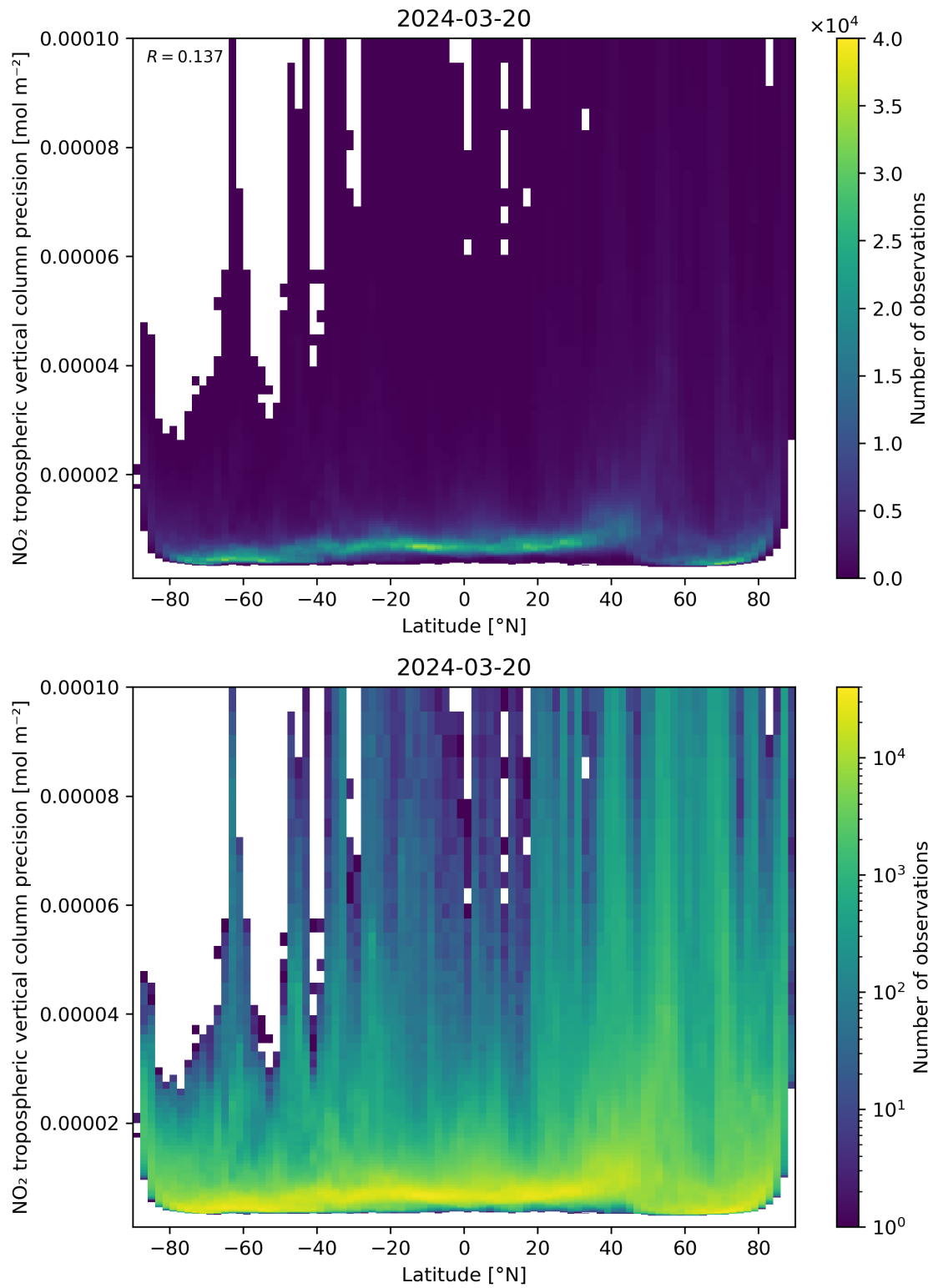
Figure 93: Scatter density plot of “Latitude” against “NO 2 tropospheric vertical column precision” for 2024-03-20 to 2024-03-21.
