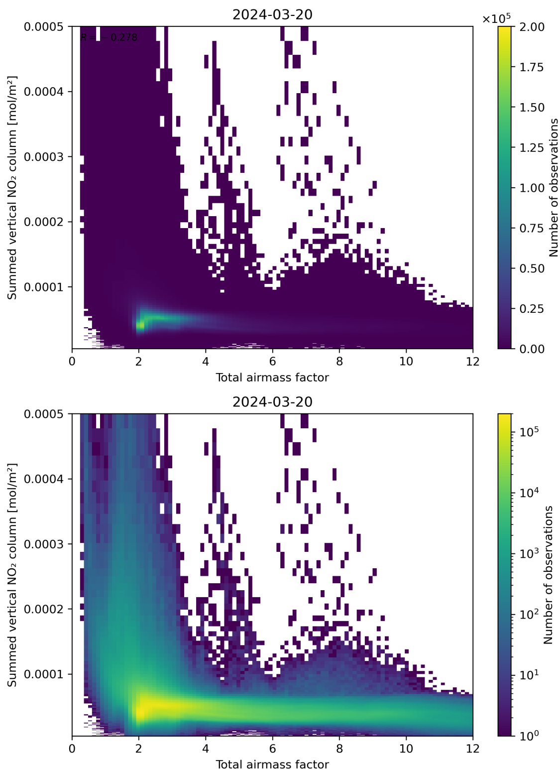
Figure 65: Scatter density plot of “Total airmass factor” against “Summed vertical NO 2 column” for 2024-03-20 to 2024-03-21.
