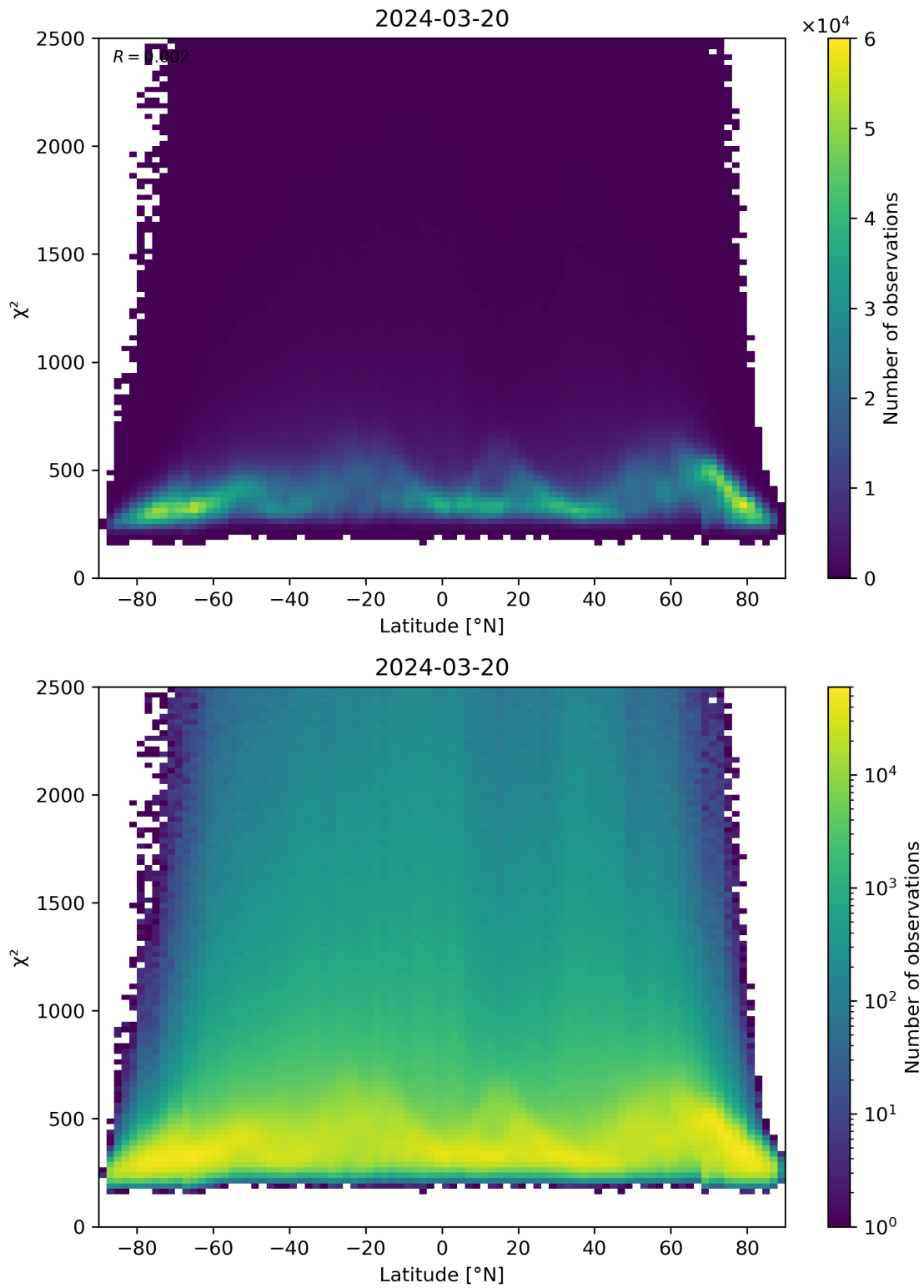
Figure 86: Scatter density plot of “Latitude” against “ \chi^2 ” for 2024-03-20 to 2024-03-21.
