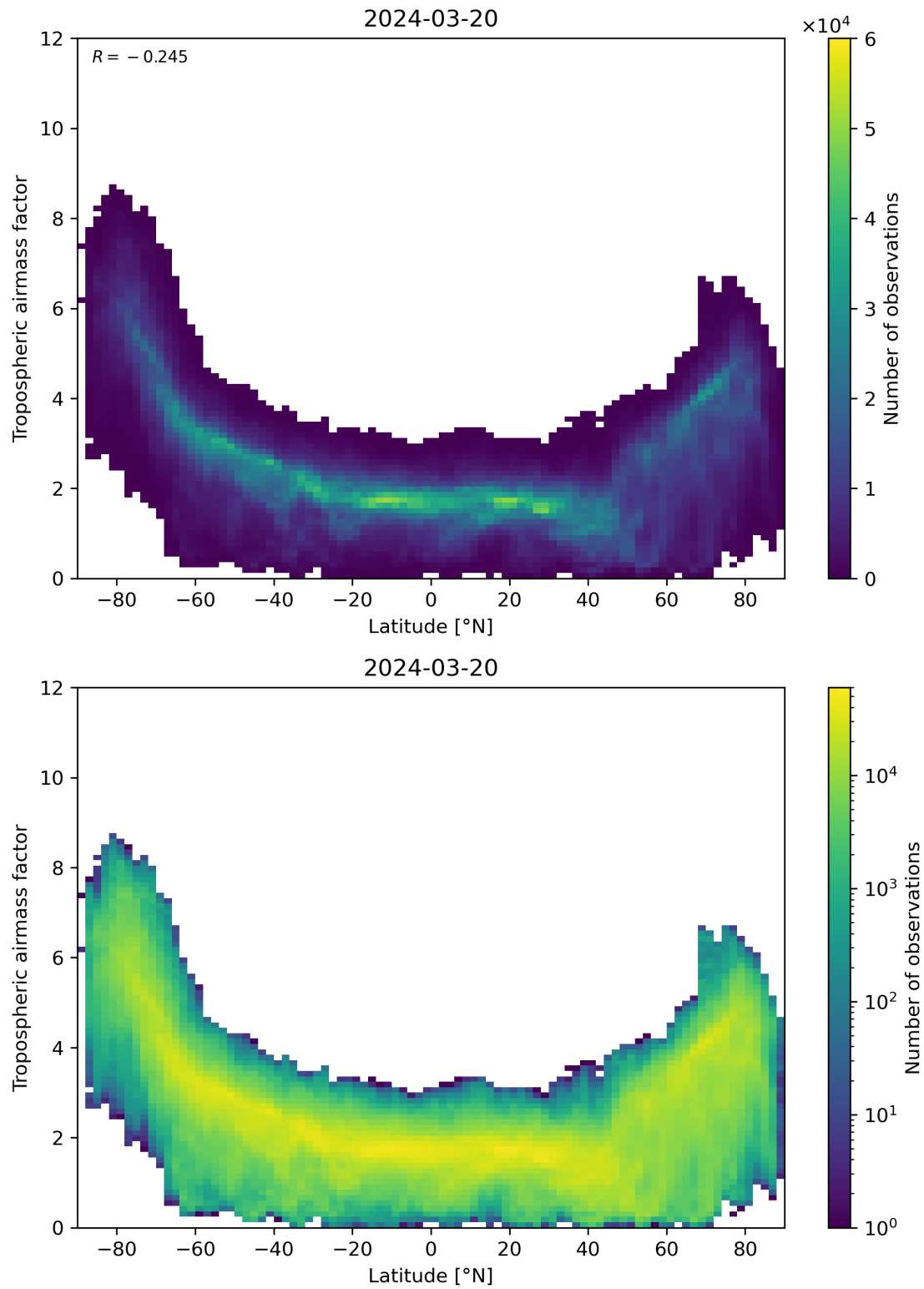
Figure 85: Scatter density plot of “Latitude” against “Tropospheric air mass factor” for 2024-03-20 to 2024-03-21.
