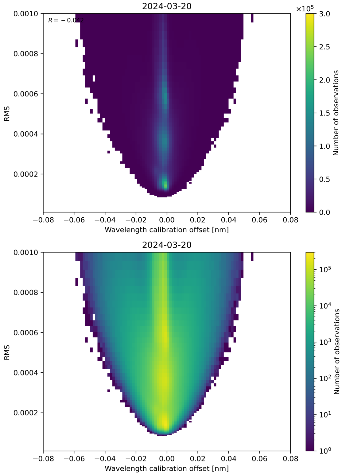
Figure 181: Scatter density plot of “Wavelength calibration offset” against “RMS” for 2024-03-20 to 2024-03-21.
