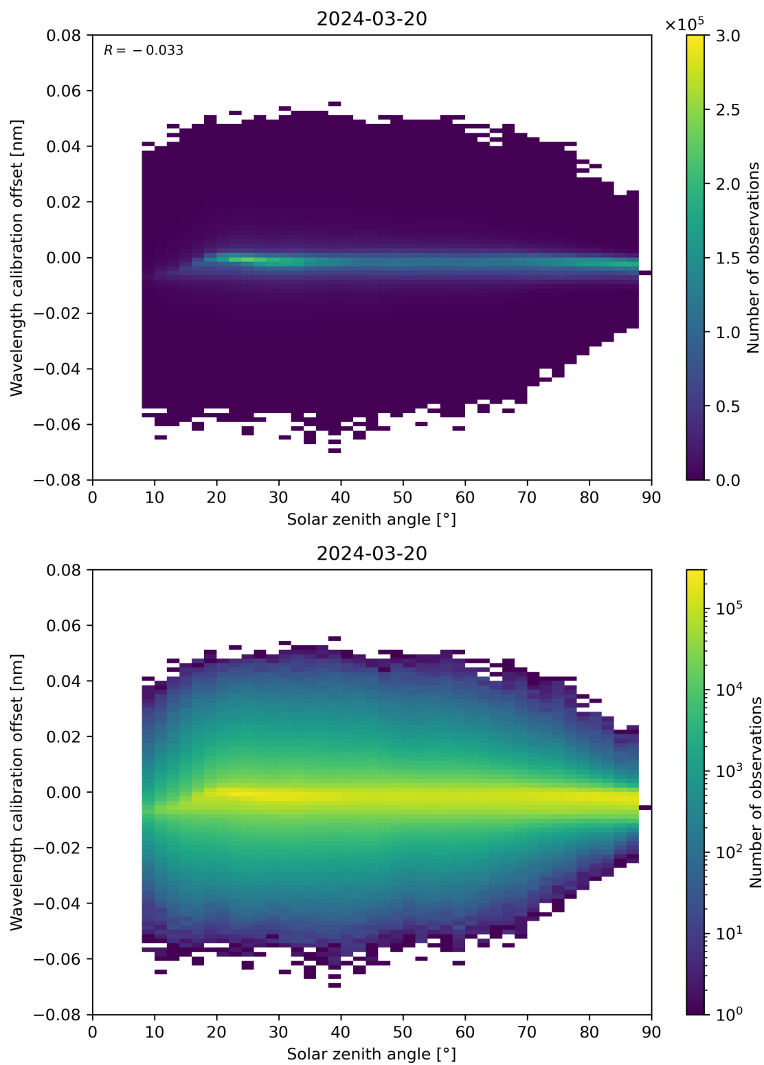
Figure 158: Scatter density plot of “Solar zenith angle” against “Wavelength calibration offset” for 2024-03-20 to 2024-03-21.
