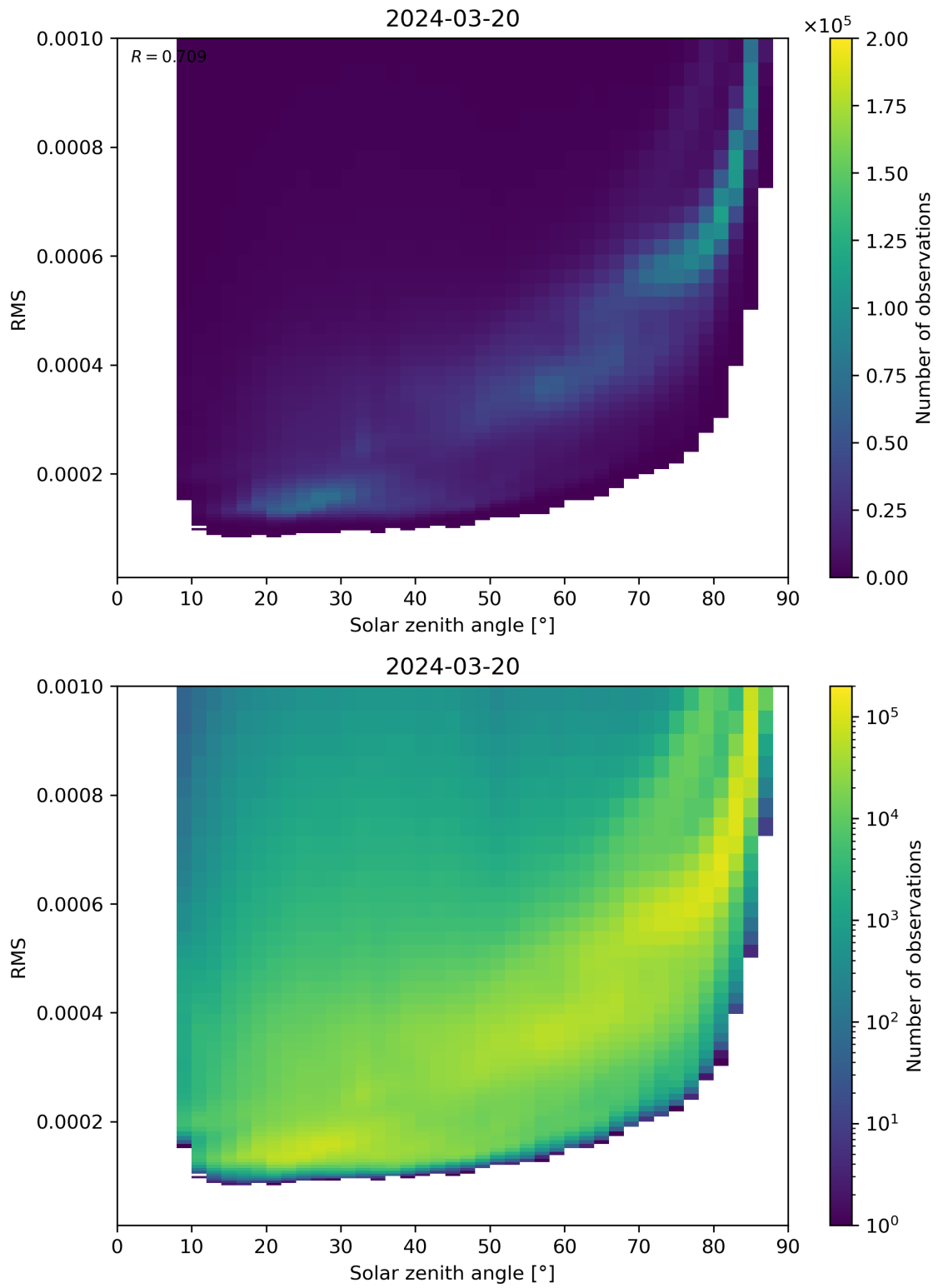
Figure 157: Scatter density plot of “Solar zenith angle” against “RMS” for 2024-03-20 to 2024-03-21.
