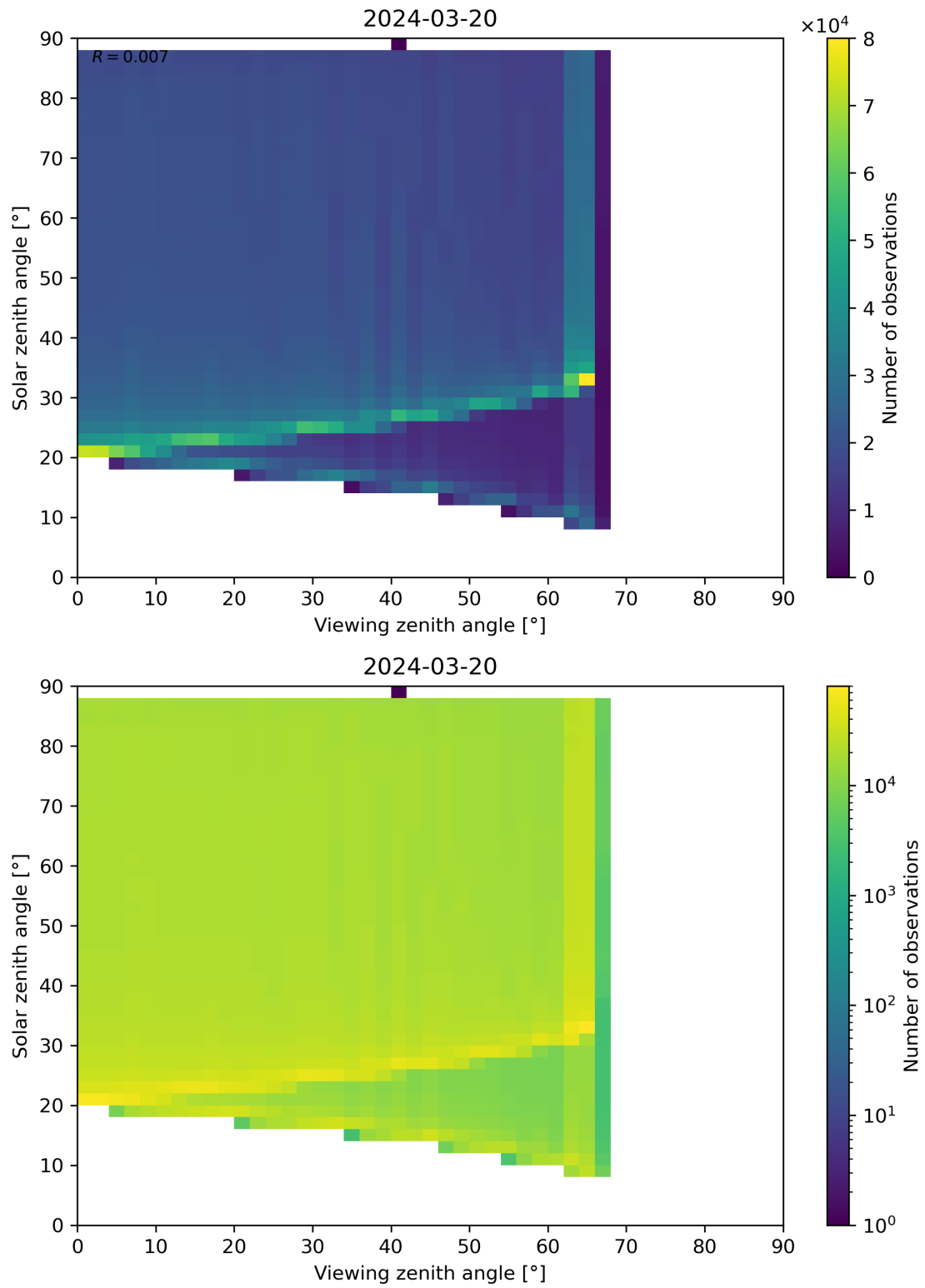
Figure 172: Scatter density plot of “Viewing zenith angle” against “Solar zenith angle” for 2024-03-20 to 2024-03-21.
