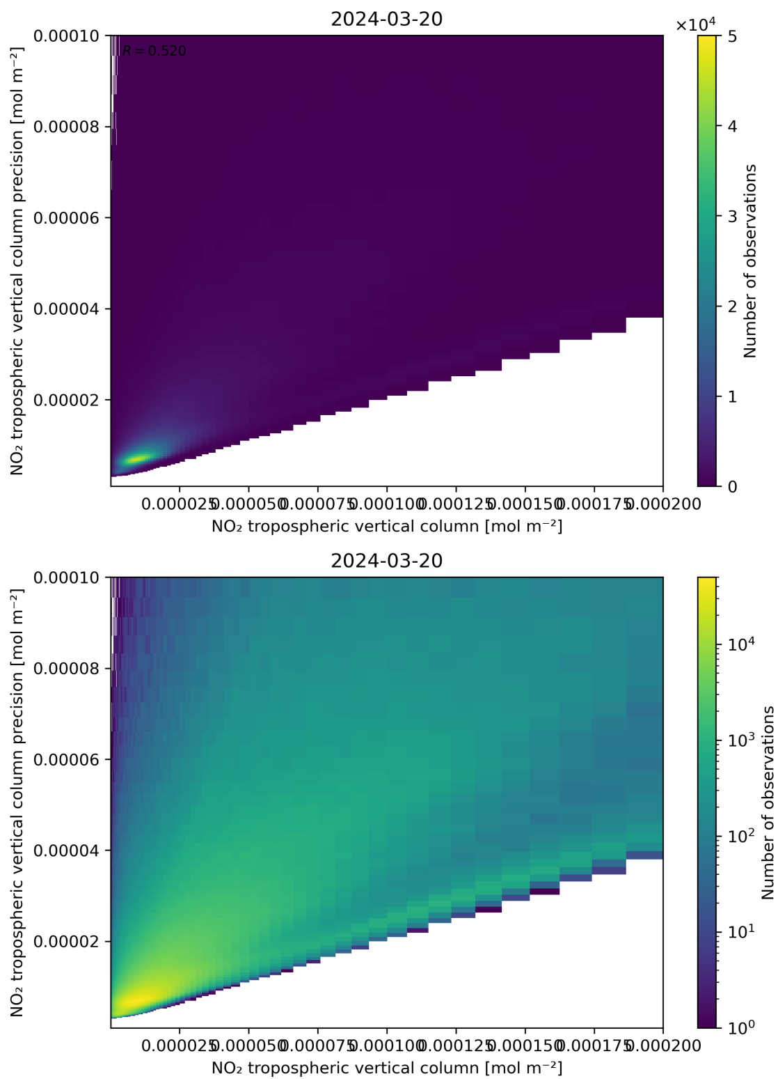
Figure 130: Scatter density plot of “NO 2 tropospheric vertical column” against “NO 2 tropospheric vertical column precision” for 2024-03-20 to 2024-03-21.
