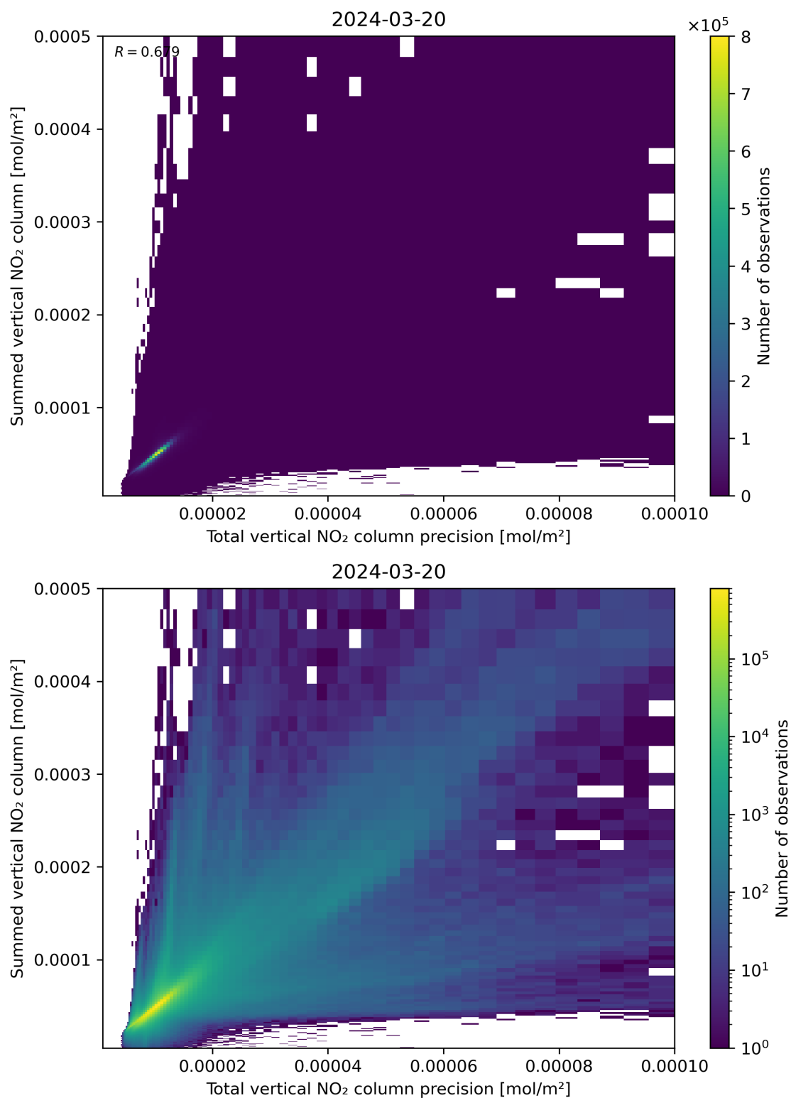
Figure 117: Scatter density plot of “Total vertical NO 2 column precision” against “Summed vertical NO 2 column” for 2024-03-20 to 2024-03-21.
