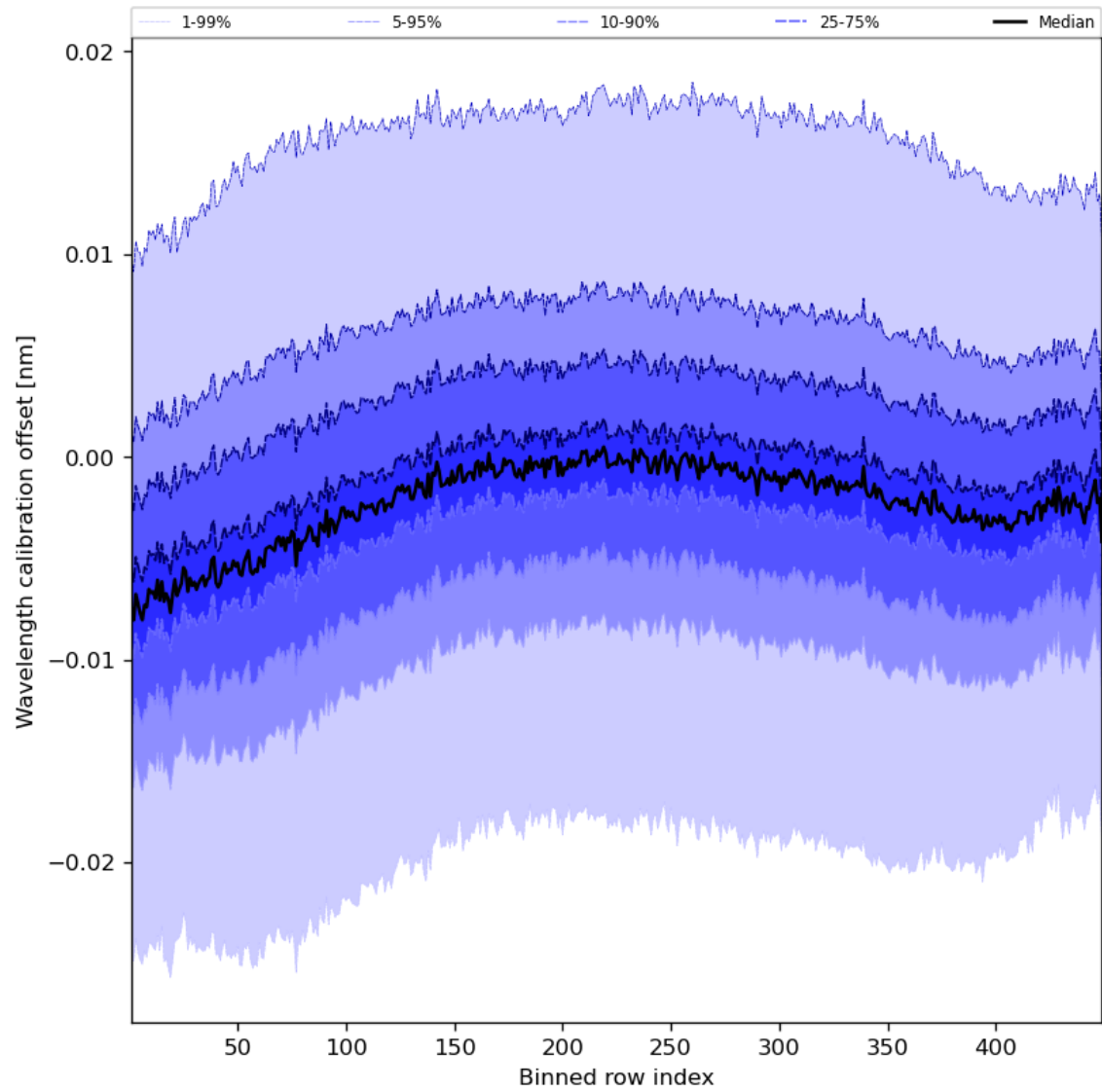
Figure 52: Along track statistics of “Wavelength calibration offset” for 2024-03-20 to 2024-03-21
