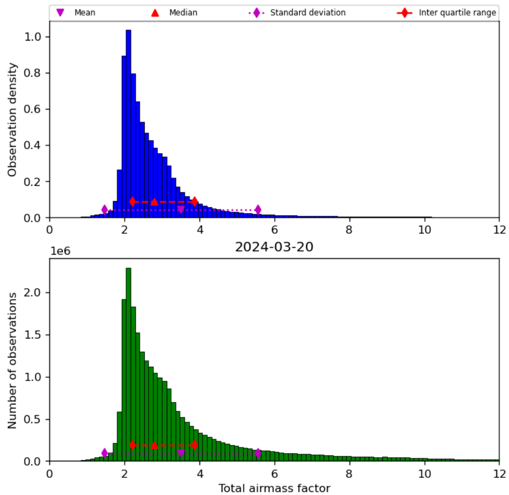
Figure 32: Histogram of “Total airmass factor” for 2024-03-20 to 2024-03-21
