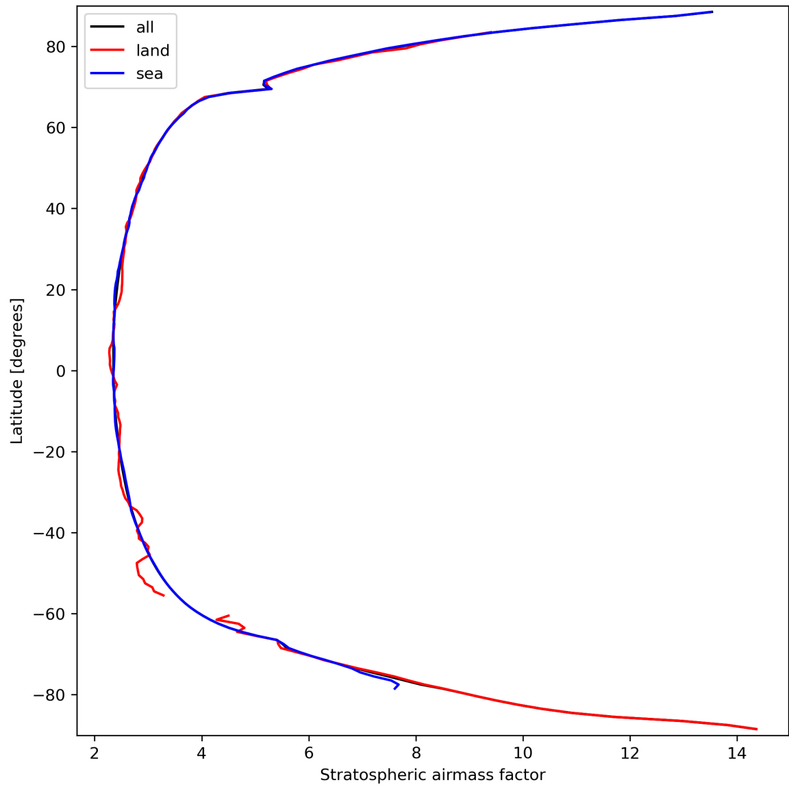
Figure 27: Zonal average of “Stratospheric air mass factor” for 2024-03-20 to 2024-03-21.
