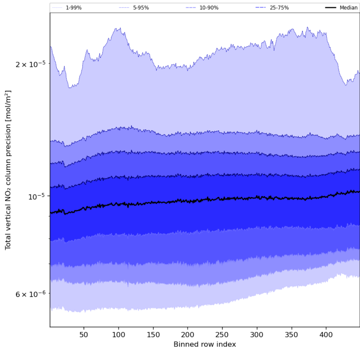
Figure 56: Along track statistics of “Total vertical NO 2 column precision” for 2024-03-20 to 2024-03-21
