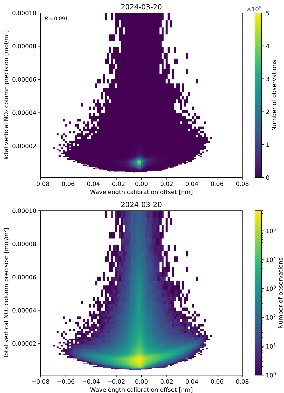
Figure 180: Scatter density plot of “Wavelength calibration offset” against “Total vertical NO 2 column precision” for 2024-03-20 to 2024-03-21.
