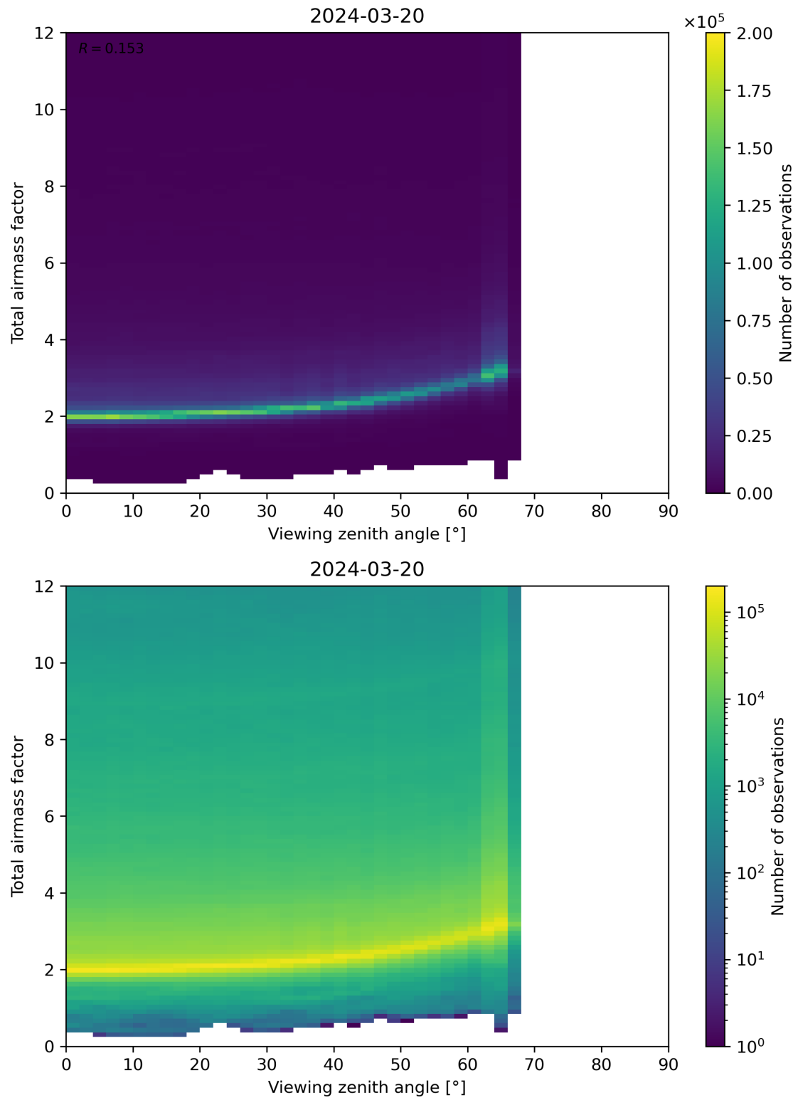
Figure 160: Scatter density plot of “Viewing zenith angle” against “Total airmass factor” for 2024-03-20 to 2024-03-21.
