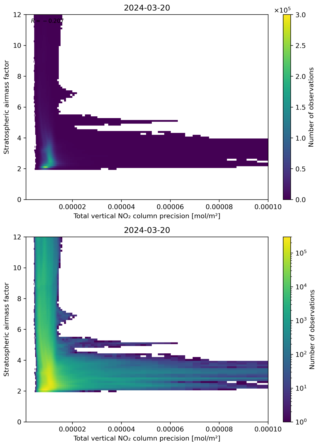
Figure 115: Scatter density plot of “Total vertical NO 2 column precision” against “Stratospheric air mass factor” for 2024-03-20 to 2024-03-21.
