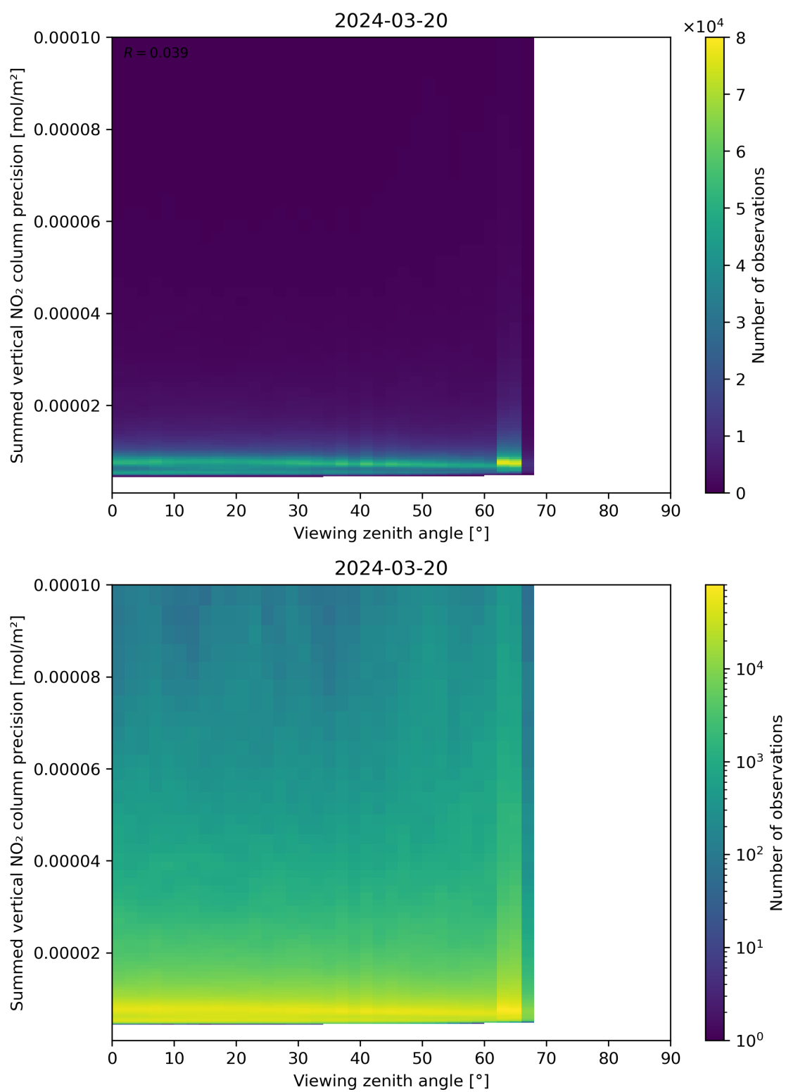
Figure 166: Scatter density plot of “Viewing zenith angle” against “Summed vertical NO 2 column precision” for 2024-03-20 to 2024-03-21.
