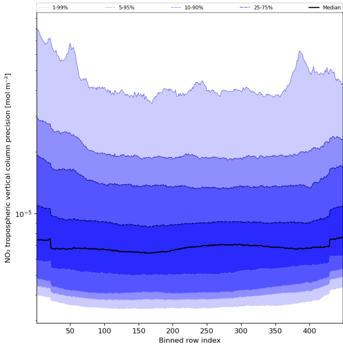
Figure 47: Along track statistics of “NO 2 tropospheric vertical column precision” for 2024-03-20 to 2024-03-21
