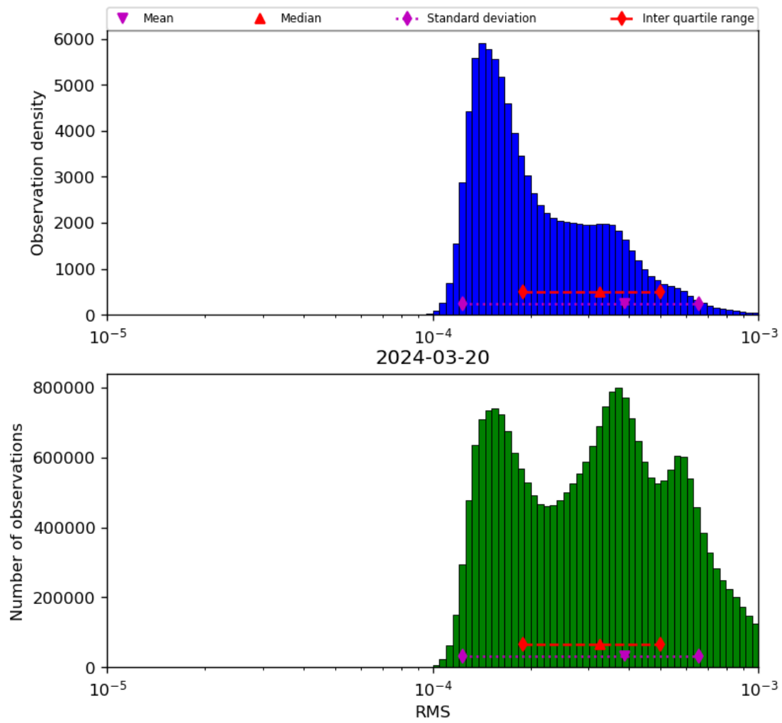
Figure 43: Histogram of “RMS” for 2024-03-20 to 2024-03-21
