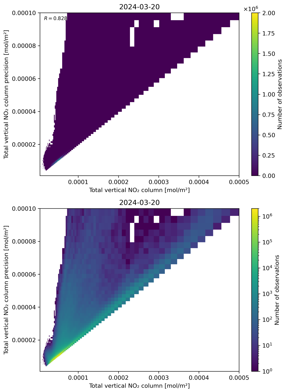
Figure 114: Scatter density plot of “Total vertical NO 2 column” against “Total vertical NO 2 column precision” for 2024-03-20 to 2024-03-21.
