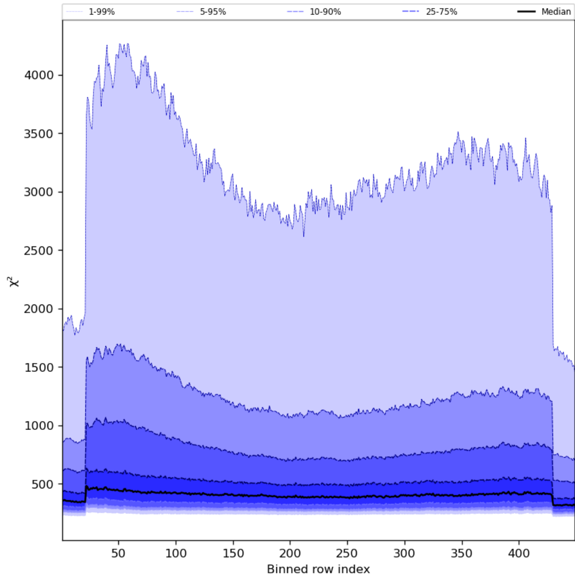
Figure 59: Along track statistics of “ \chi^2 ” for 2024-03-20 to 2024-03-21
