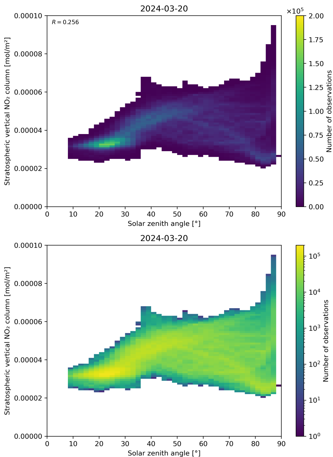
Figure 150: Scatter density plot of “Solar zenith angle” against “Stratospheric vertical NO 2 column” for 2024-03-20 to 2024-03-21.
