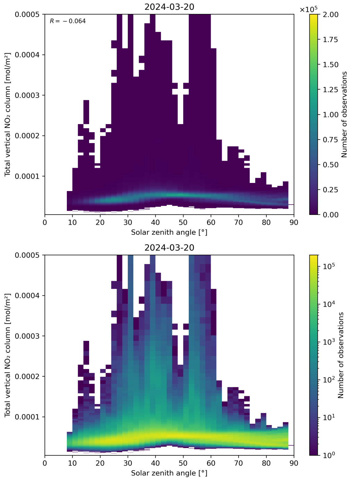
Figure 153: Scatter density plot of “Solar zenith angle” against “Total vertical NO 2 column” for 2024-03-20 to 2024-03-21.
