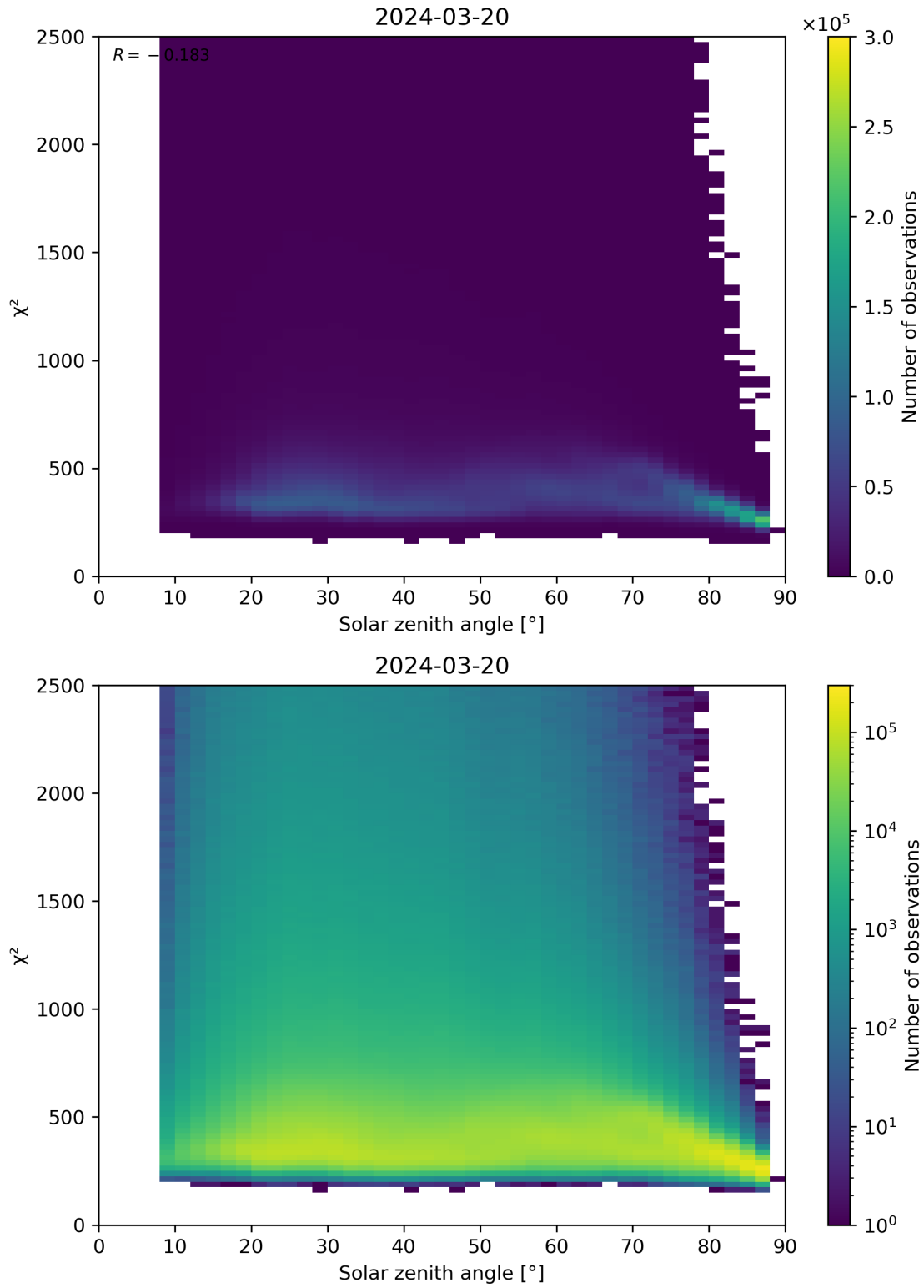
Figure 148: Scatter density plot of “Solar zenith angle” against “ \chi^2 ” for 2024-03-20 to 2024-03-21.
