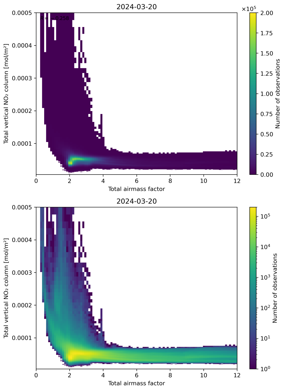
Figure 67: Scatter density plot of “Total airmass factor” against “Total vertical NO 2 column” for 2024-03-20 to 2024-03-21.
