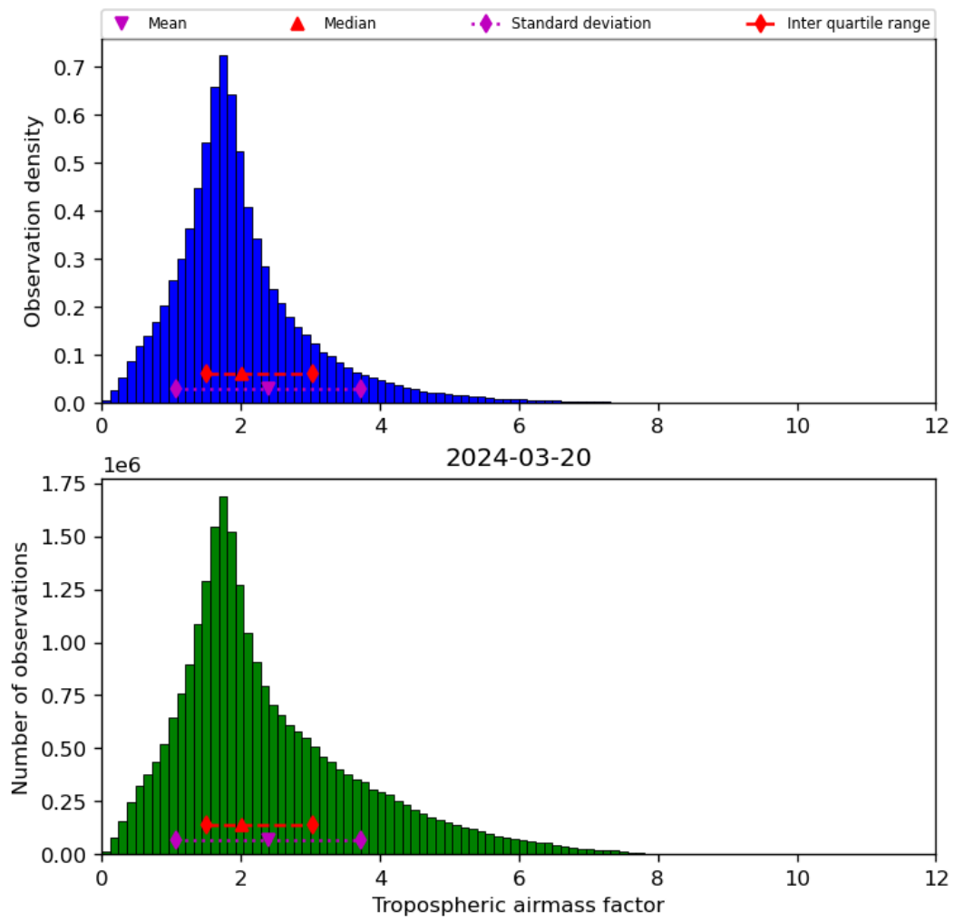
Figure 31: Histogram of “Tropospheric airmass factor” for 2024-03-20 to 2024-03-21
