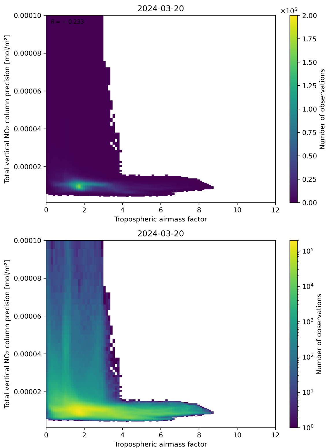
Figure 78: Scatter density plot of “Tropospheric air mass factor” against “Total vertical NO 2 column precision” for 2024-03-20 to 2024-03-21.
