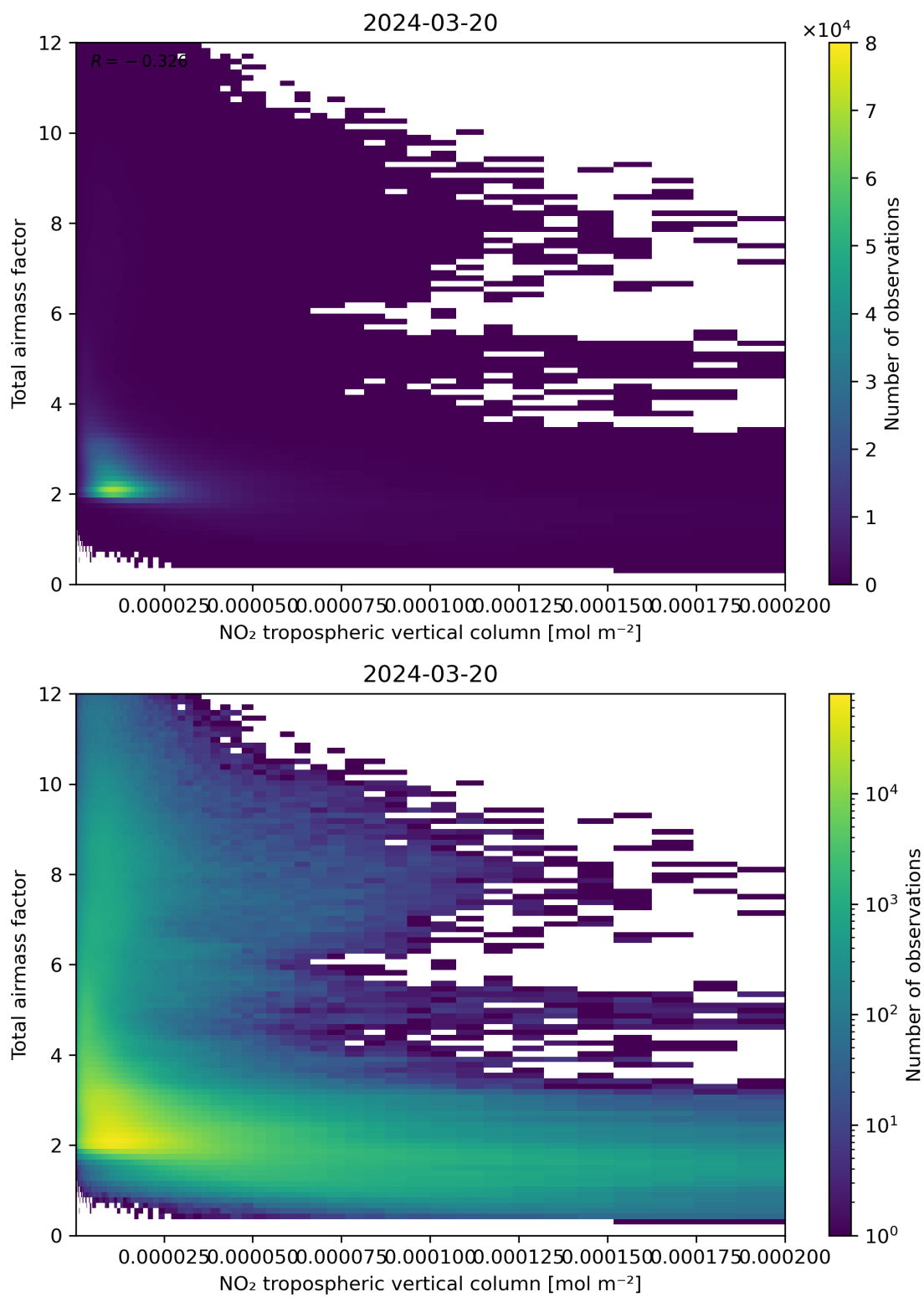
Figure 122: Scatter density plot of “NO 2 tropospheric vertical column” against “Total air mass factor” for 2024-03-20 to 2024-03-21.
