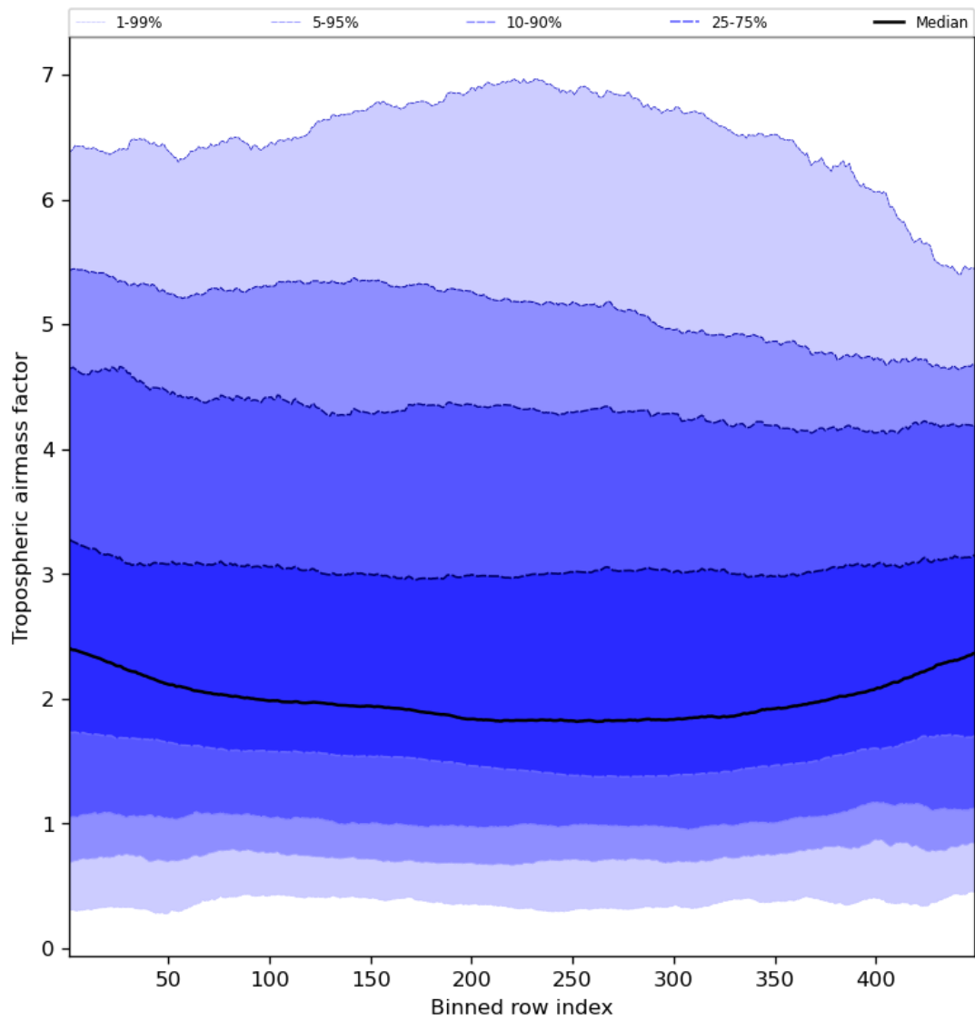
Figure 48: Along track statistics of “Tropospheric airmass factor” for 2024-03-20 to 2024-03-21
