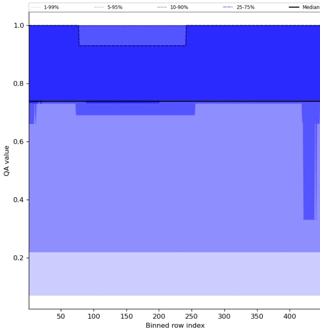
Figure 45: Along track statistics of “QA value” for 2024-03-20 to 2024-03-21
