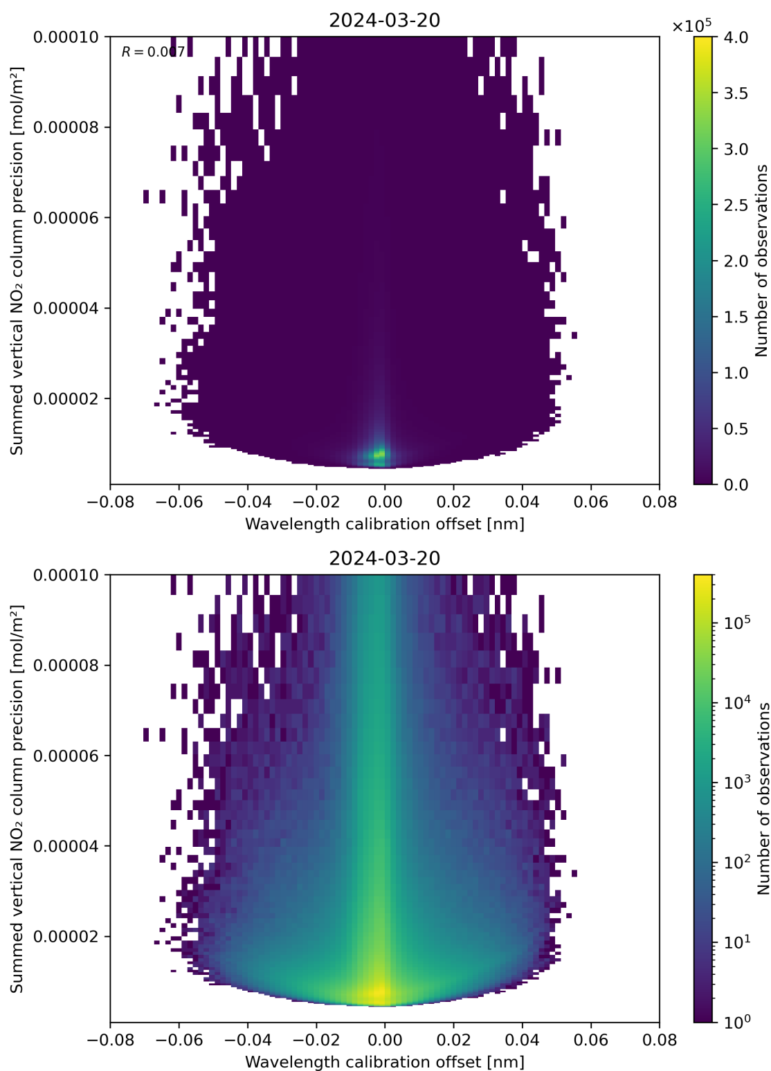
Figure 178: Scatter density plot of “Wavelength calibration offset” against “Summed vertical NO 2 column precision” for 2024-03-20 to 2024-03-21.
