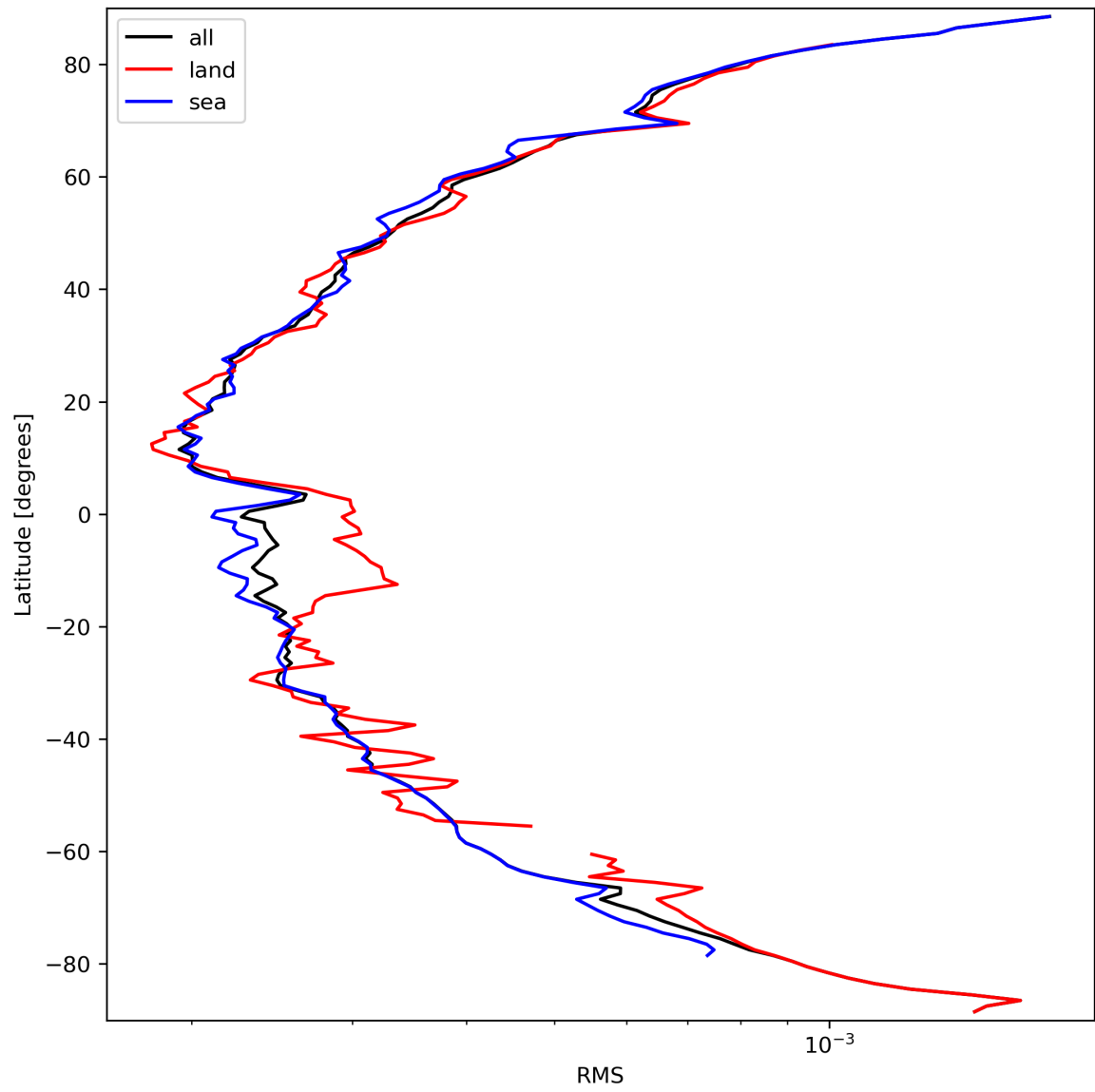
Figure 26: Zonal average of “RMS” for 2024-03-20 to 2024-03-21.
