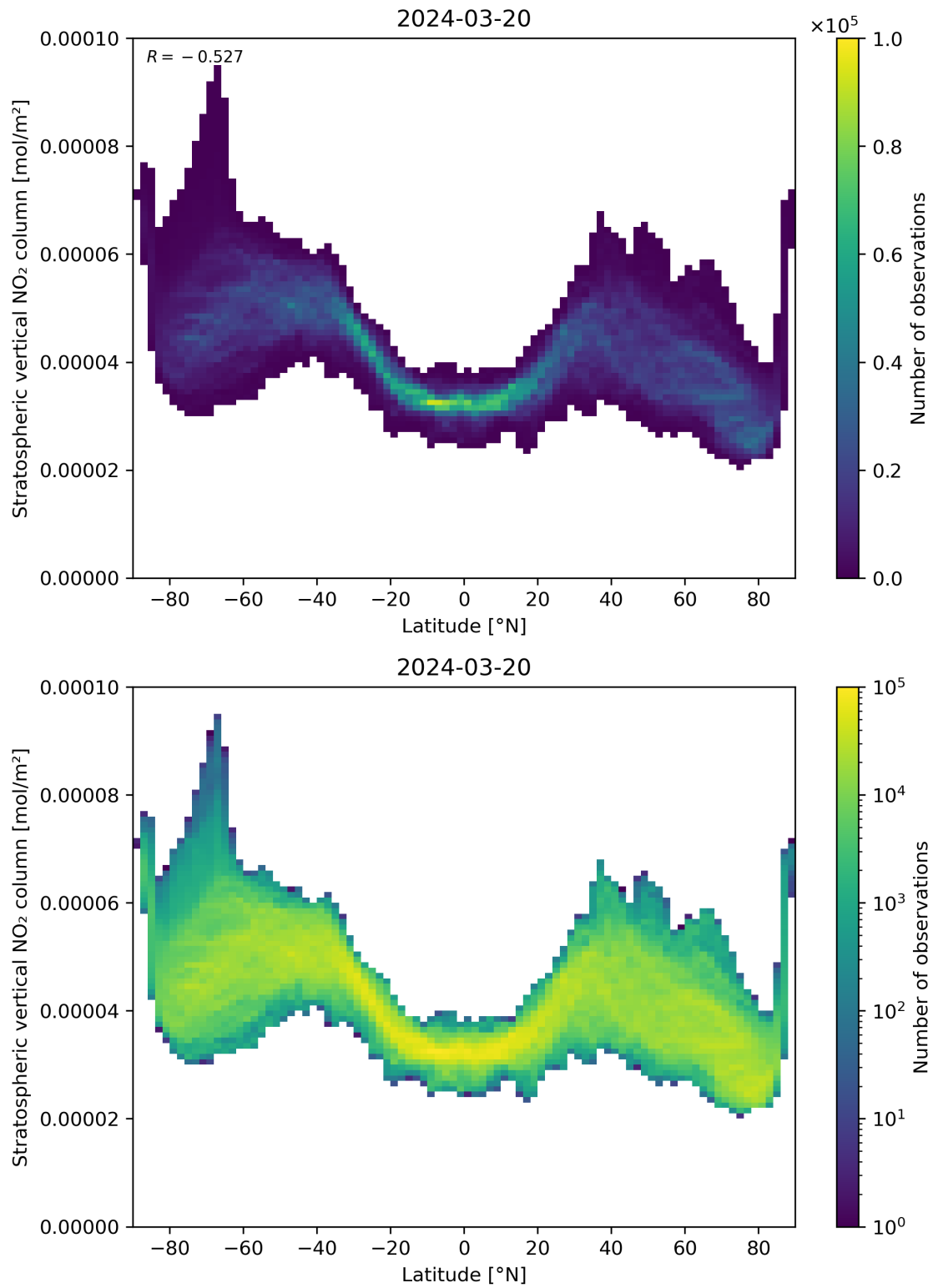
Figure 87: Scatter density plot of “Latitude” against “Stratospheric vertical NO 2 column” for 2024-03-20 to 2024-03-21.
