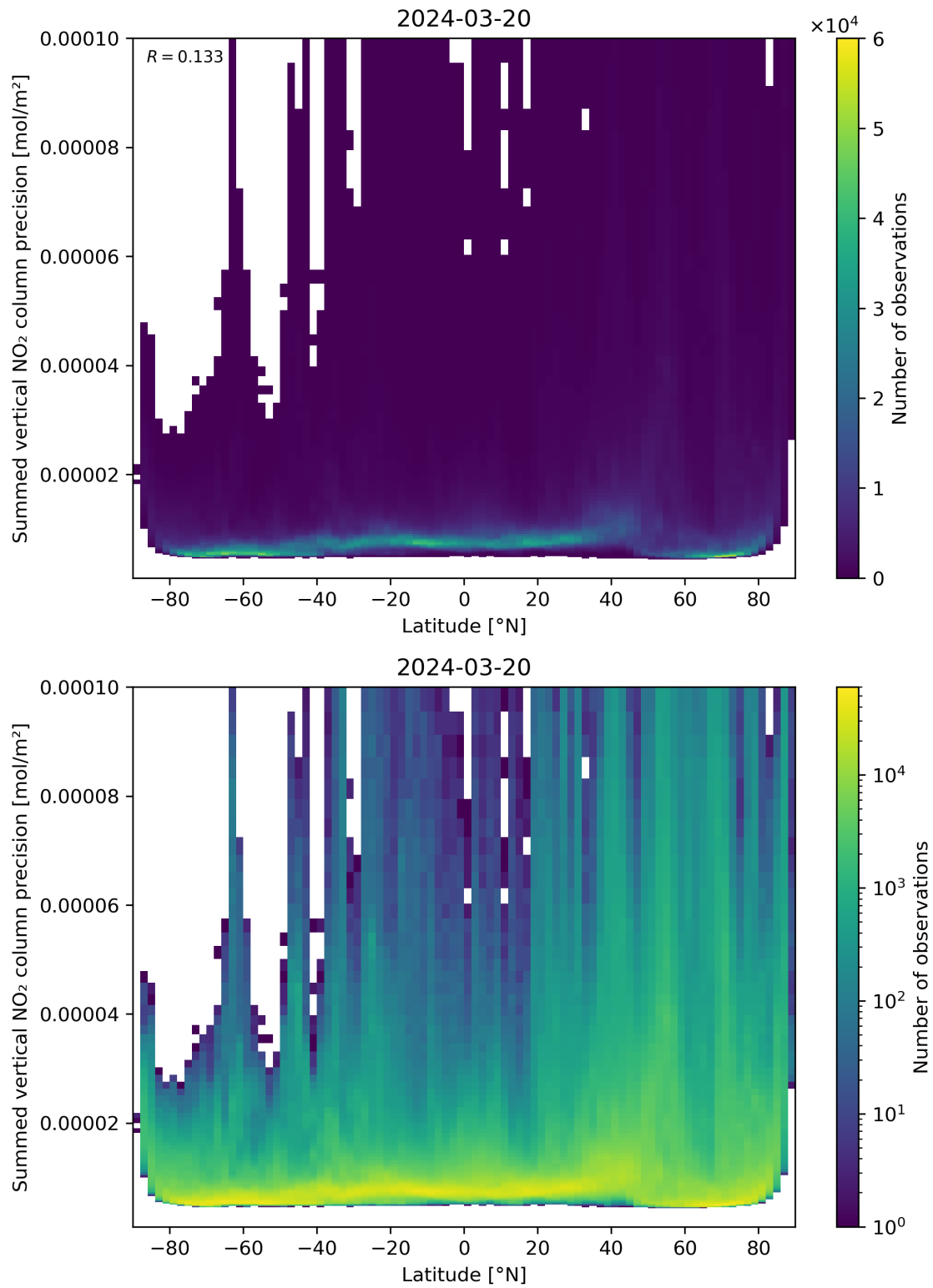
Figure 89: Scatter density plot of “Latitude” against “Summed vertical NO 2 column precision” for 2024-03-20 to 2024-03-21.
