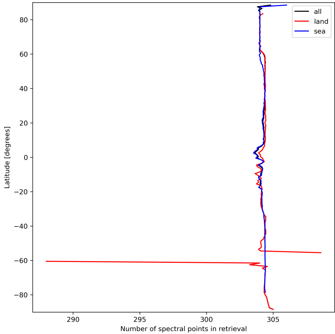
Figure 16: Zonal average of “Number of spectral points in retrieval” for 2024-03-20 to 2024-03-21.
