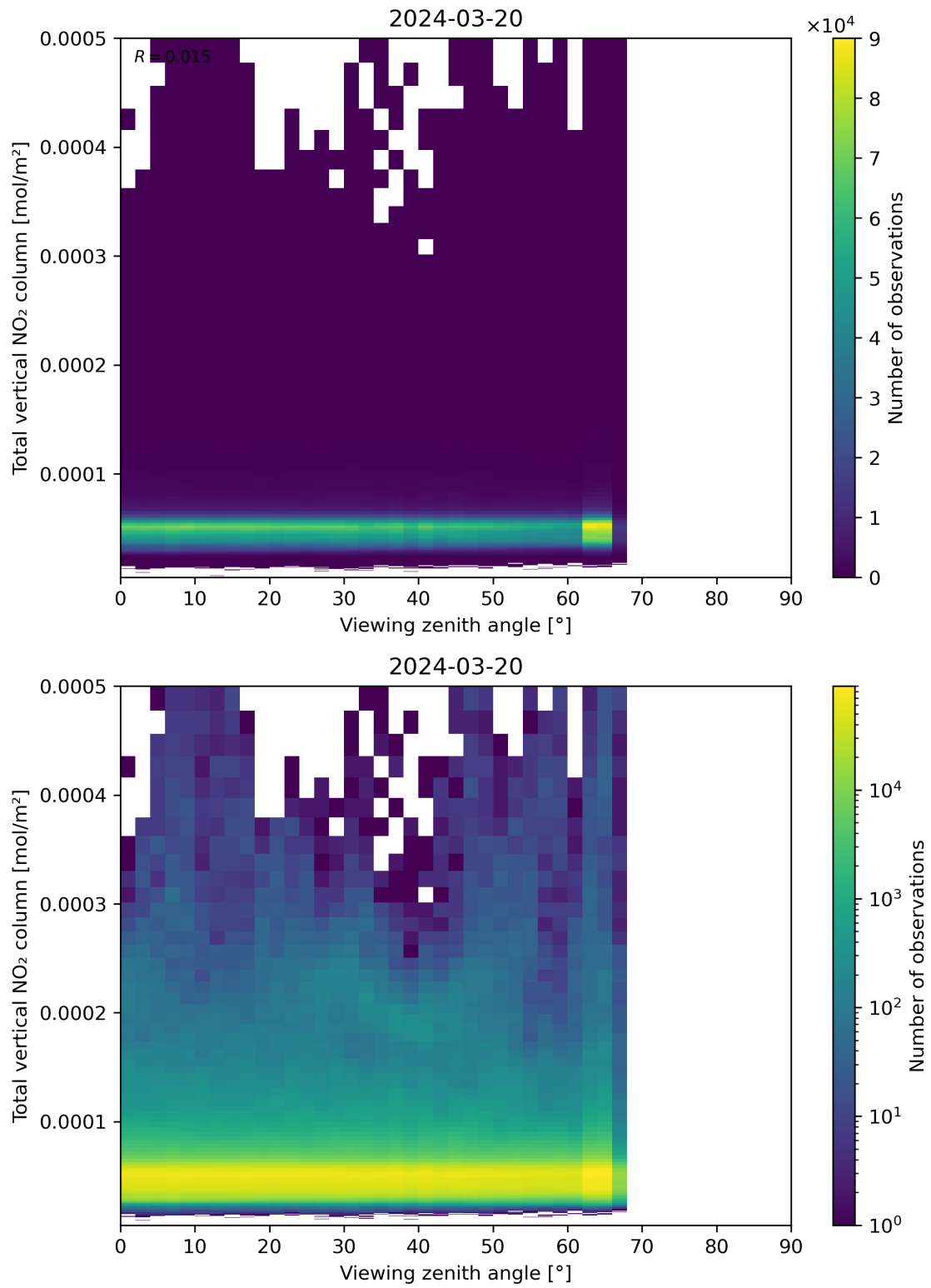
Figure 167: Scatter density plot of “Viewing zenith angle” against “Total vertical NO 2 column” for 2024-03-20 to 2024-03-21.
