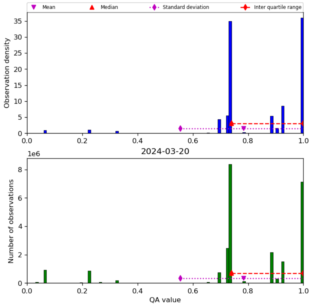
Figure 28: Histogram of “QA value” for 2024-03-20 to 2024-03-21
