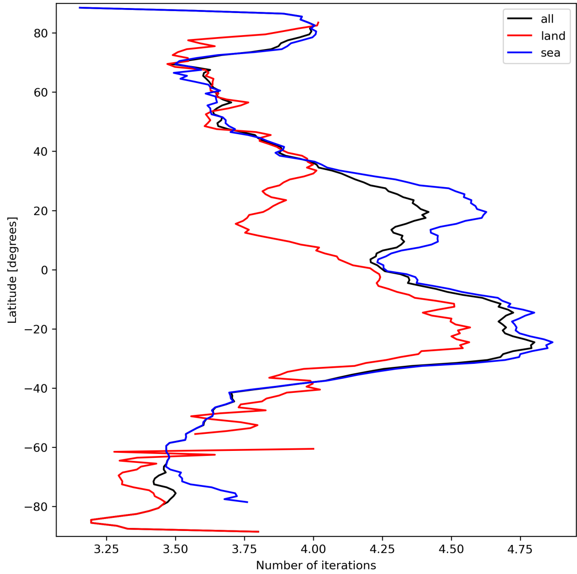
Figure 17: Zonal average of “Number of iterations” for 2024-03-20 to 2024-03-21.
