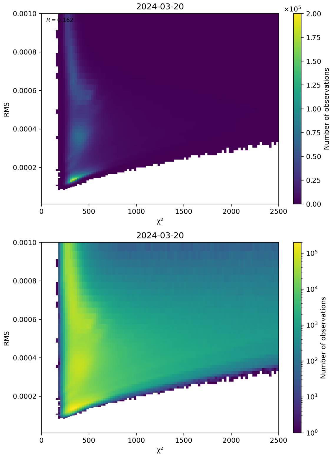
Figure 82: Scatter density plot of “ \chi^2 ” against “RMS” for 2024-03-20 to 2024-03-21.
