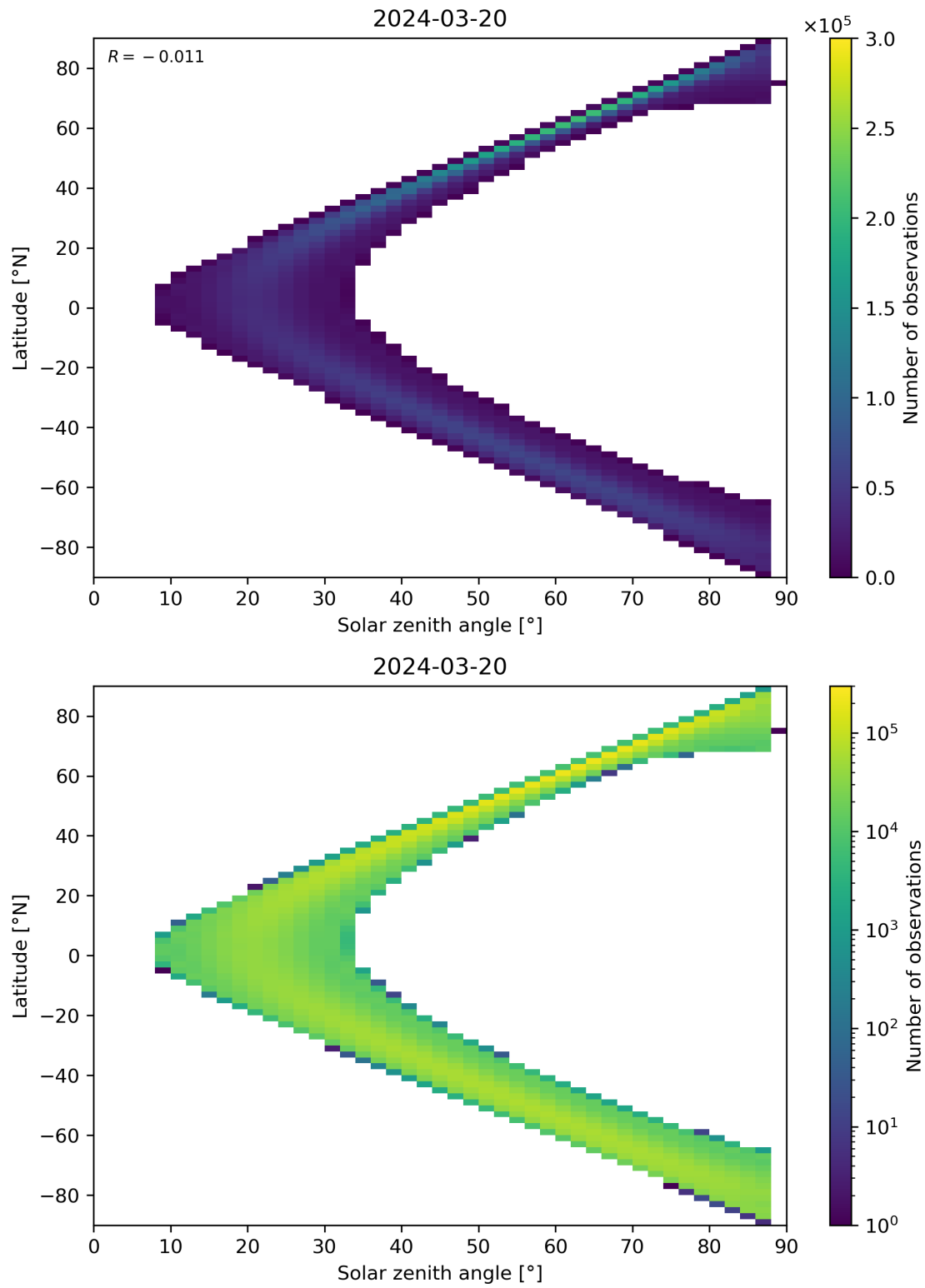
Figure 149: Scatter density plot of “Solar zenith angle” against “Latitude” for 2024-03-20 to 2024-03-21.
