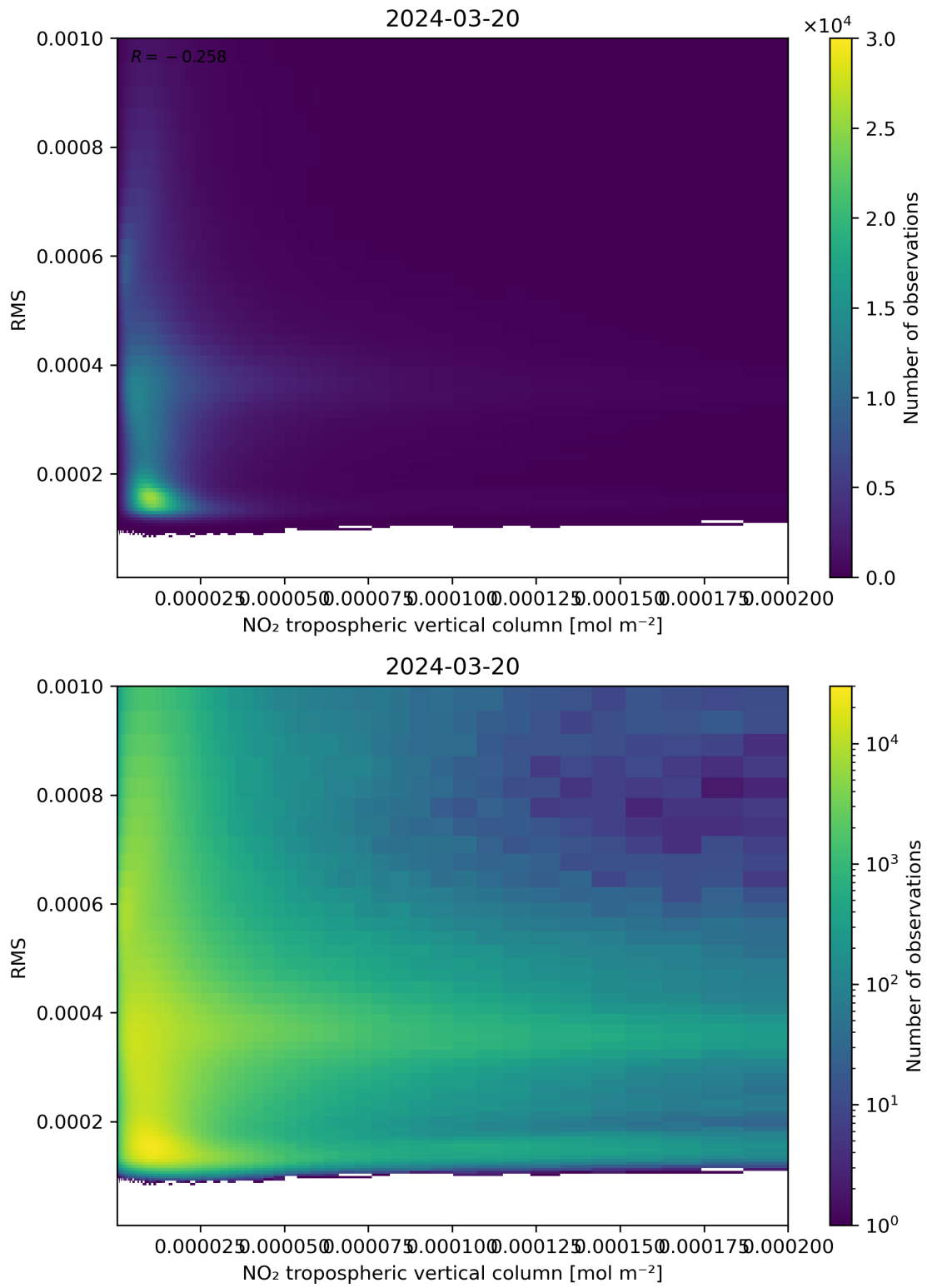
Figure 142: Scatter density plot of “NO 2 tropospheric vertical column” against “RMS” for 2024-03-20 to 2024-03-21.
