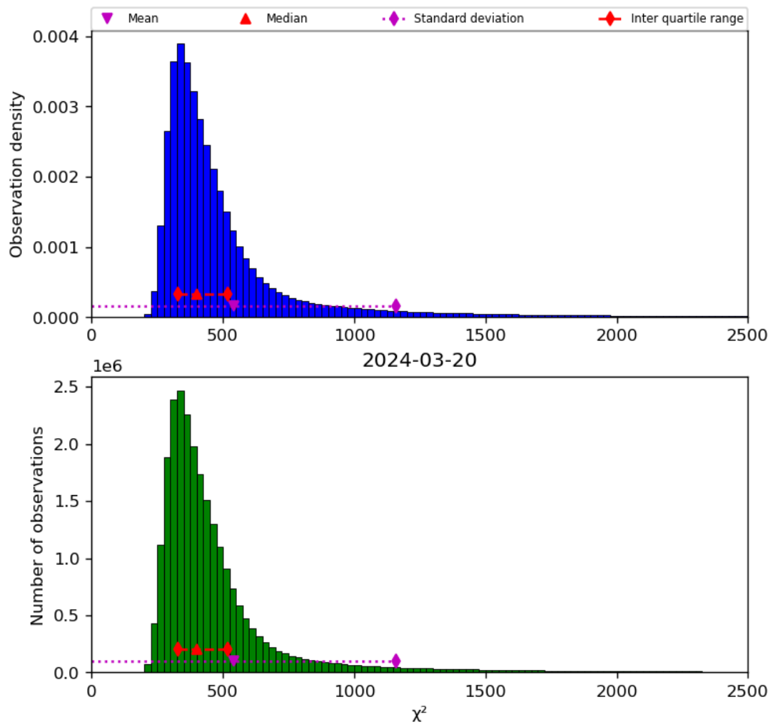
Figure 42: Histogram of “ \chi^2 ” for 2024-03-20 to 2024-03-21
