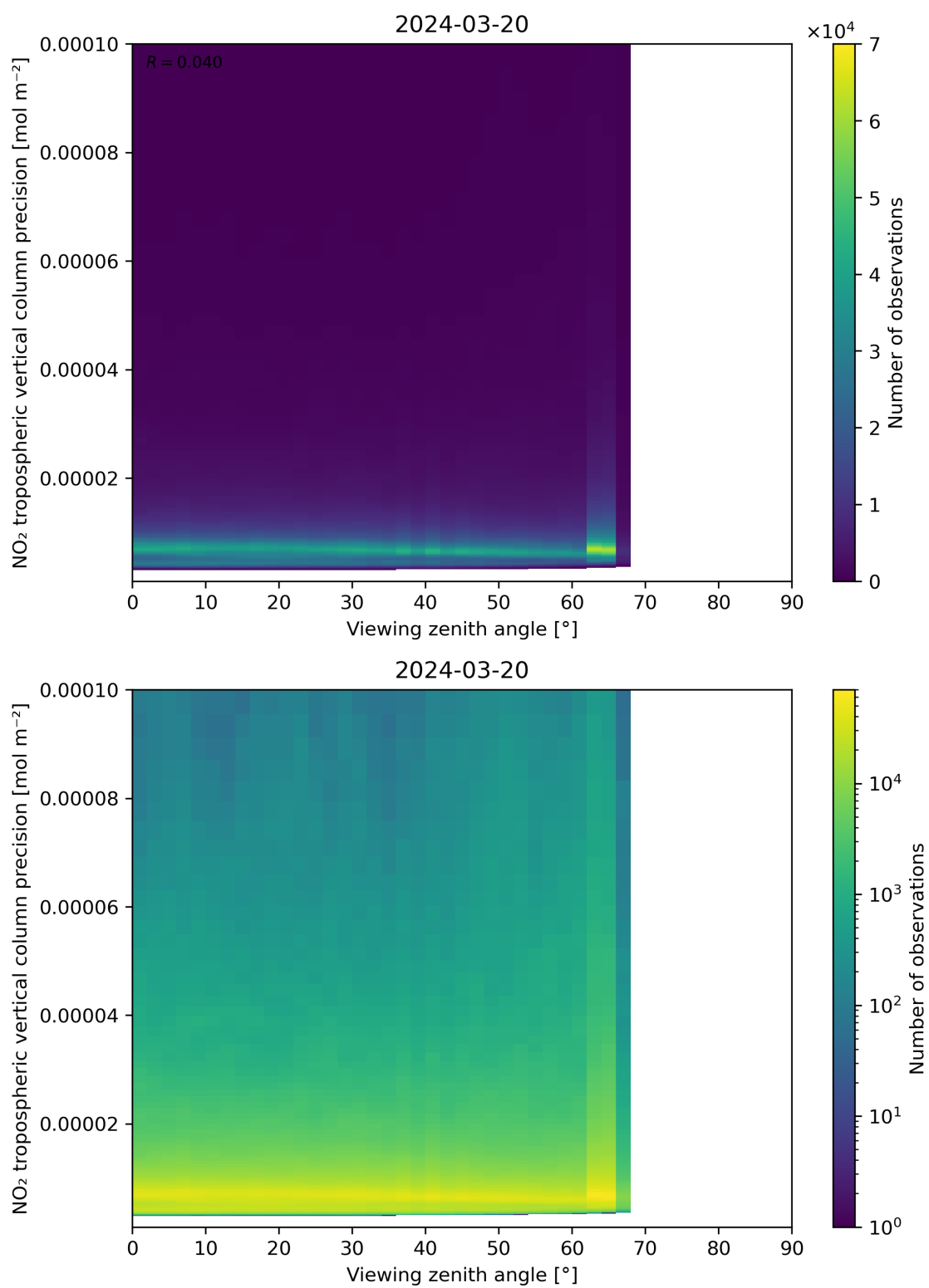
Figure 170: Scatter density plot of “Viewing zenith angle” against “NO 2 tropospheric vertical column precision” for 2024-03-20 to 2024-03-21.
