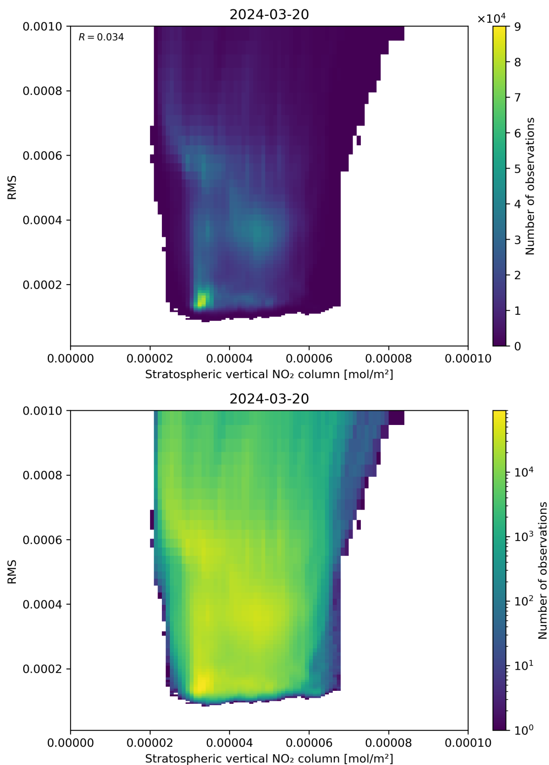
Figure 102: Scatter density plot of “Stratospheric vertical NO 2 column” against “RMS” for 2024-03-20 to 2024-03-21.
