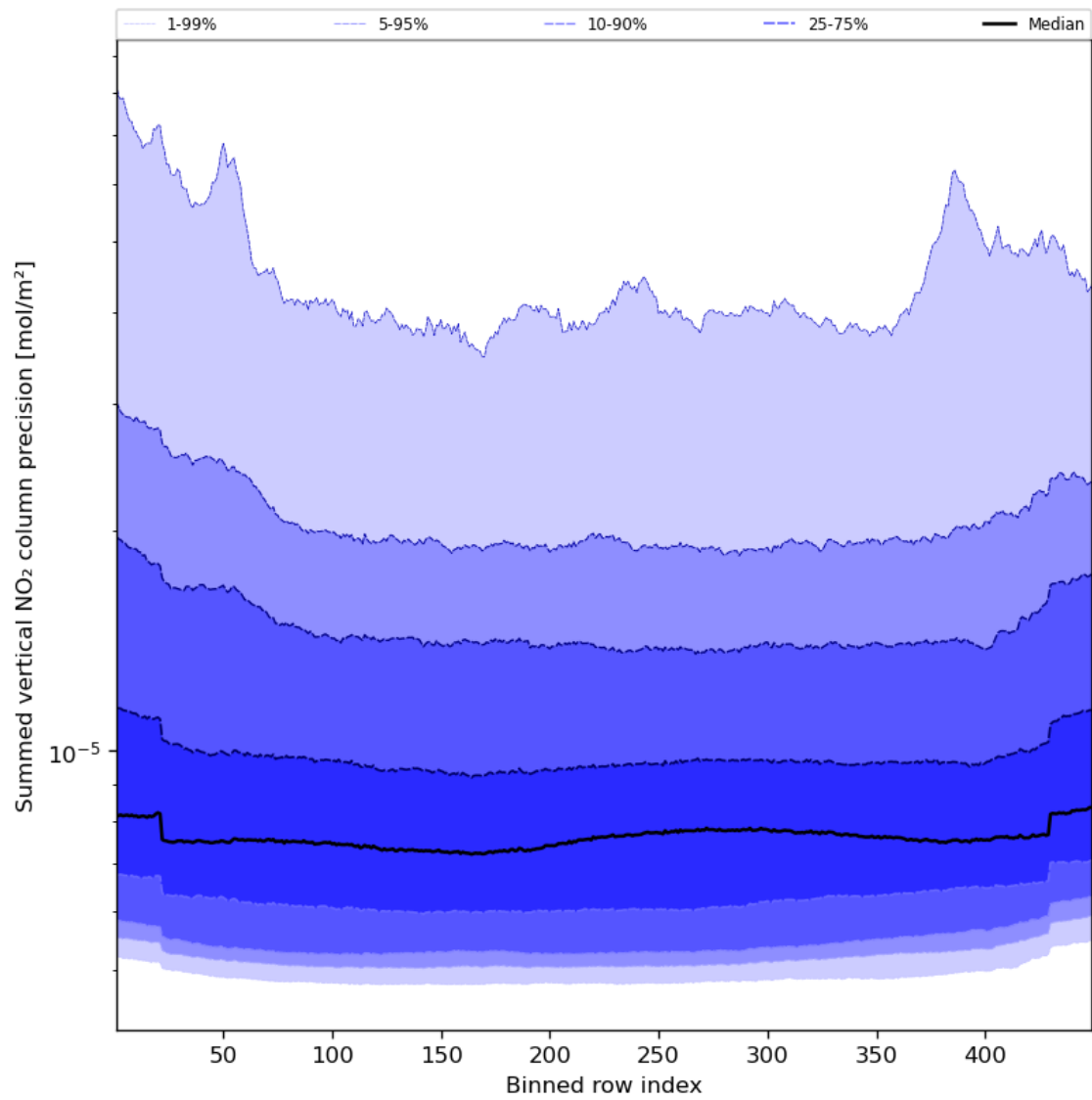
Figure 58: Along track statistics of “Summed vertical NO 2 column precision” for 2024-03-20 to 2024-03-21
