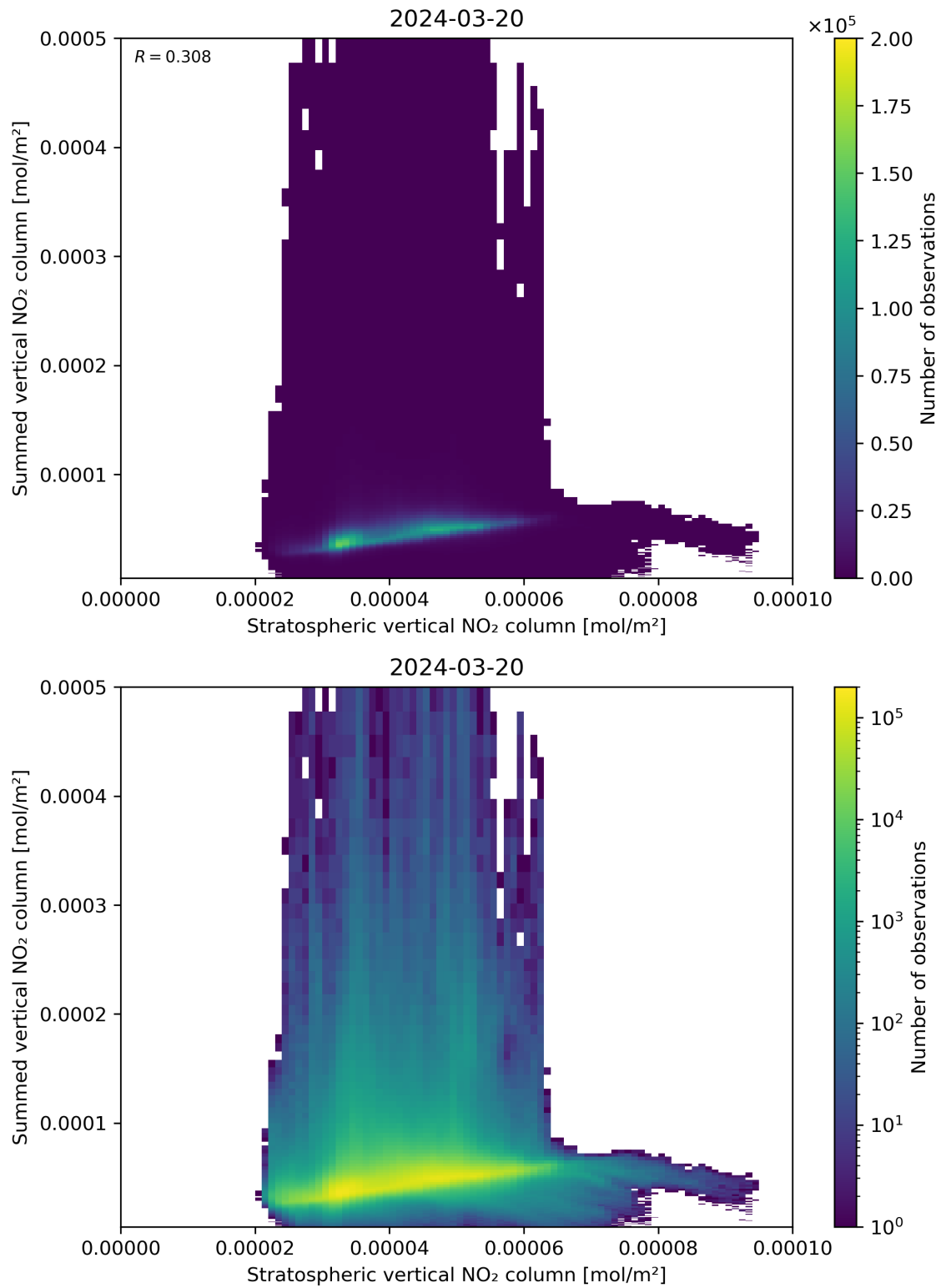
Figure 98: Scatter density plot of “Stratospheric vertical NO 2 column” against “Summed vertical NO 2 column” for 2024-03-20 to 2024-03-21.
