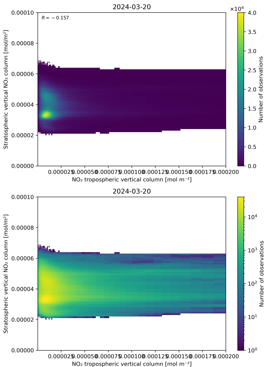
Figure 125: Scatter density plot of “NO 2 tropospheric vertical column” against “Stratospheric vertical NO 2 column” for 2024-03-20 to 2024-03-21.
