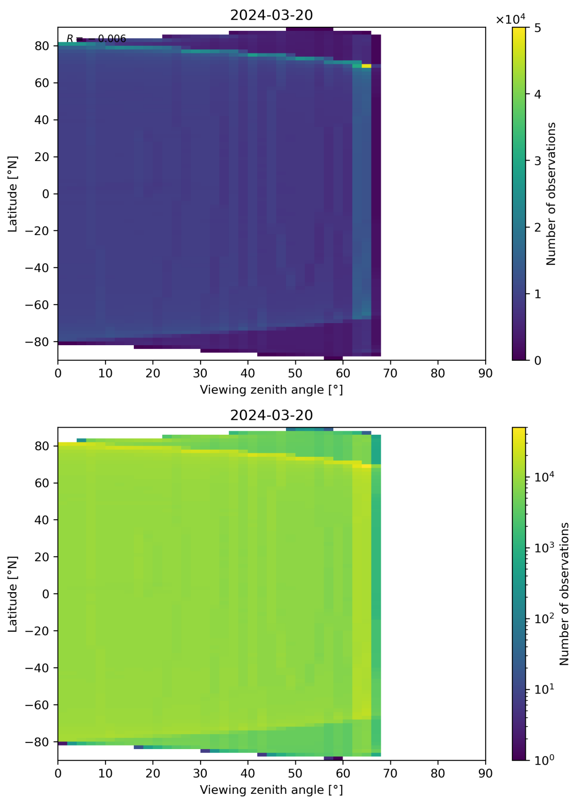
Figure 163: Scatter density plot of “Viewing zenith angle” against “Latitude” for 2024-03-20 to 2024-03-21.
