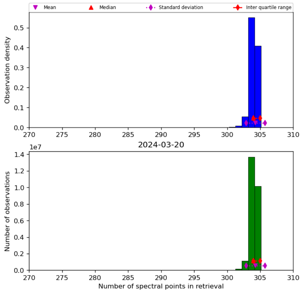
Figure 33: Histogram of “Number of spectral points in retrieval” for 2024-03-20 to 2024-03-21
