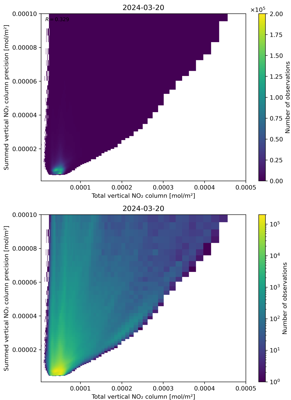
Figure 113: Scatter density plot of “Total vertical NO 2 column” against “Summed vertical NO 2 column precision” for 2024-03-20 to 2024-03-21.
