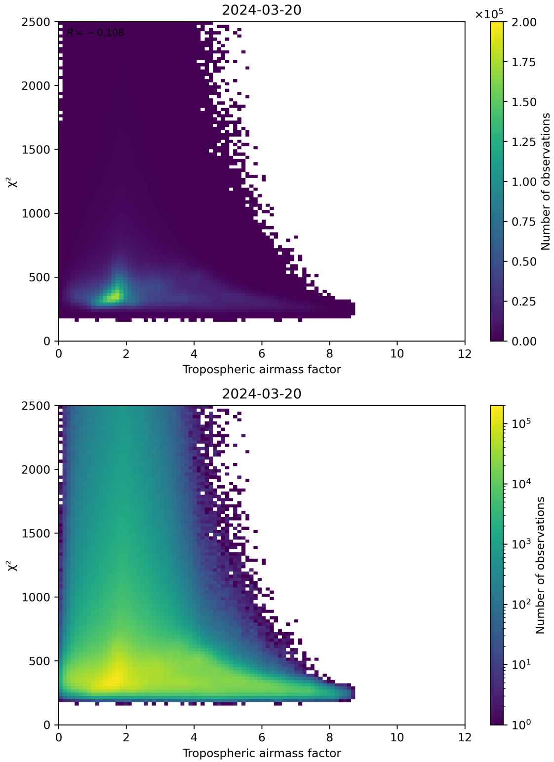
Figure 73: Scatter density plot of “Tropospheric airmass factor” against “ \chi^2 ” for 2024-03-20 to 2024-03-21.
