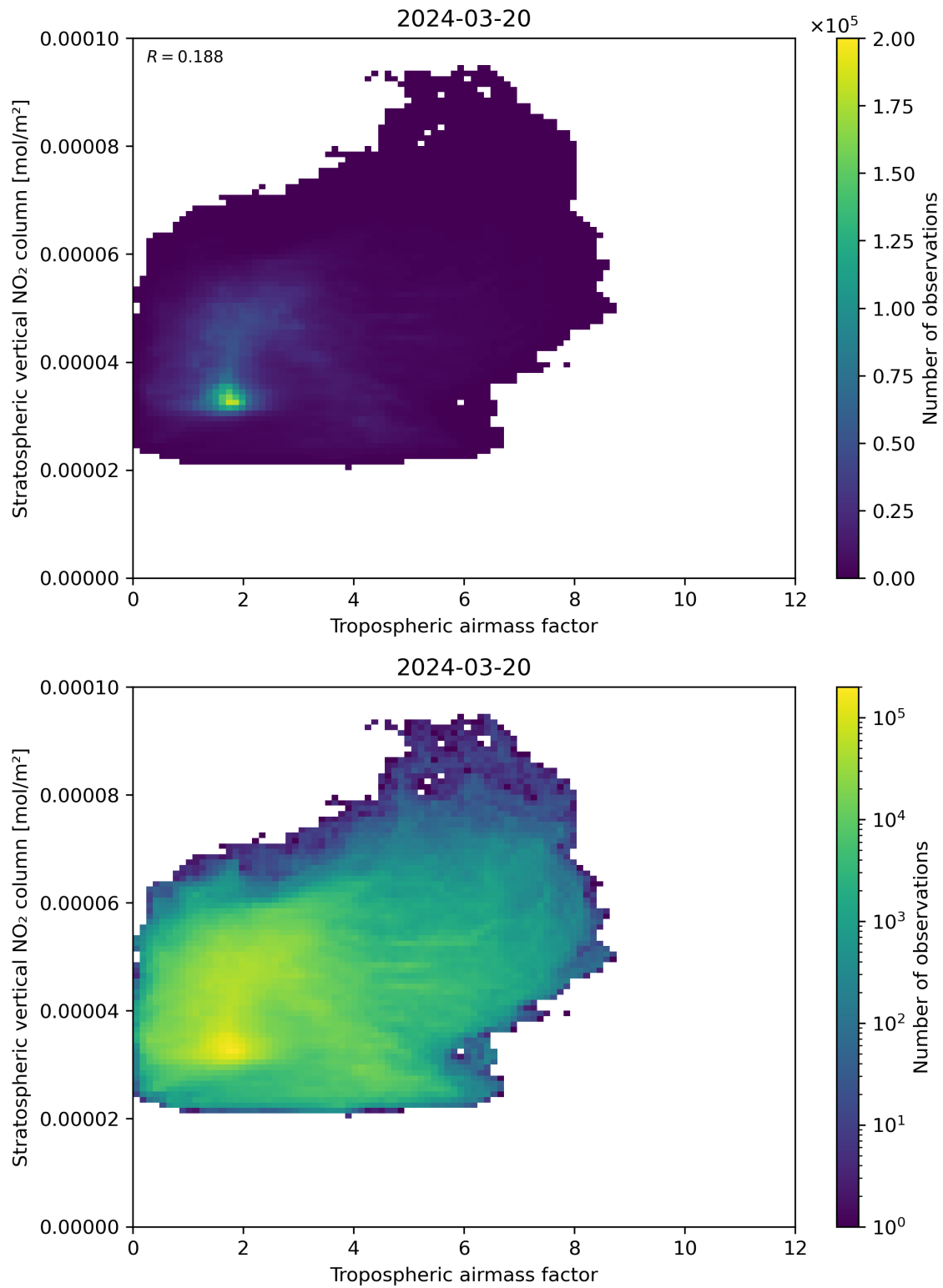
Figure 74: Scatter density plot of “Tropospheric air mass factor” against “Stratospheric vertical NO 2 column” for 2024-03-20 to 2024-03-21.
