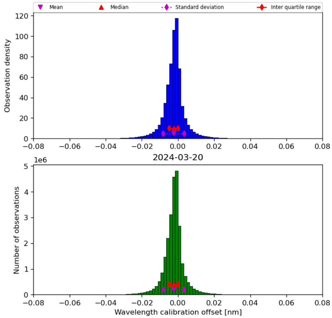
Figure 35: Histogram of “Wavelength calibration offset” for 2024-03-20 to 2024-03-21
