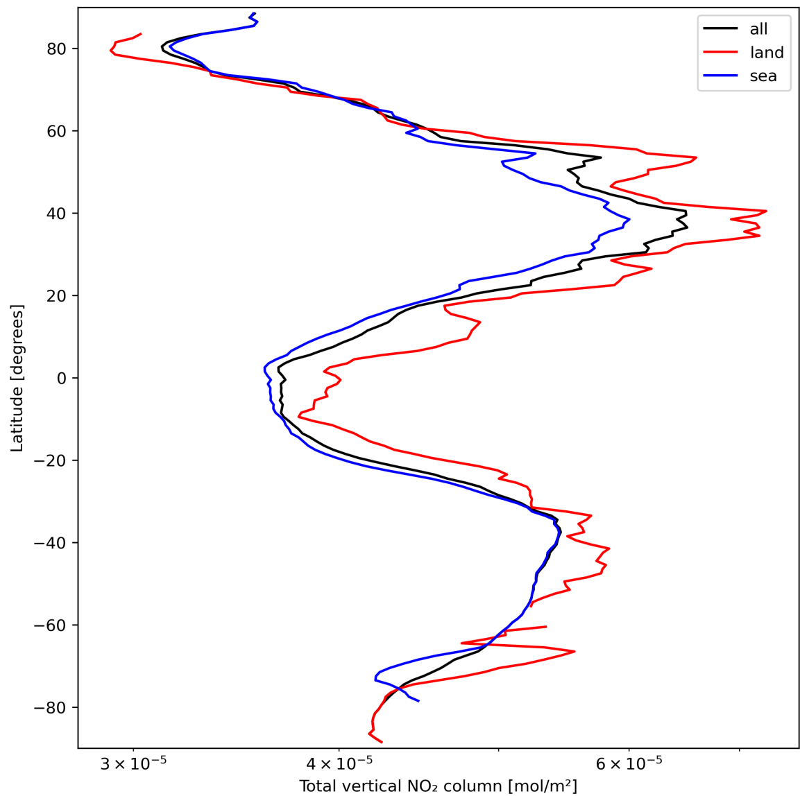
Figure 21: Zonal average of “Total vertical NO 2 column” for 2024-03-20 to 2024-03-21.
