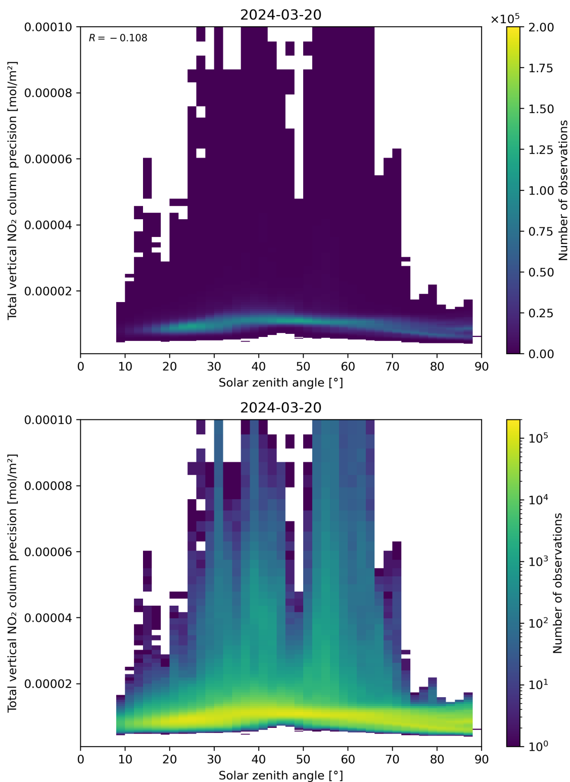
Figure 154: Scatter density plot of “Solar zenith angle” against “Total vertical NO 2 column precision” for 2024-03-20 to 2024-03-21.
