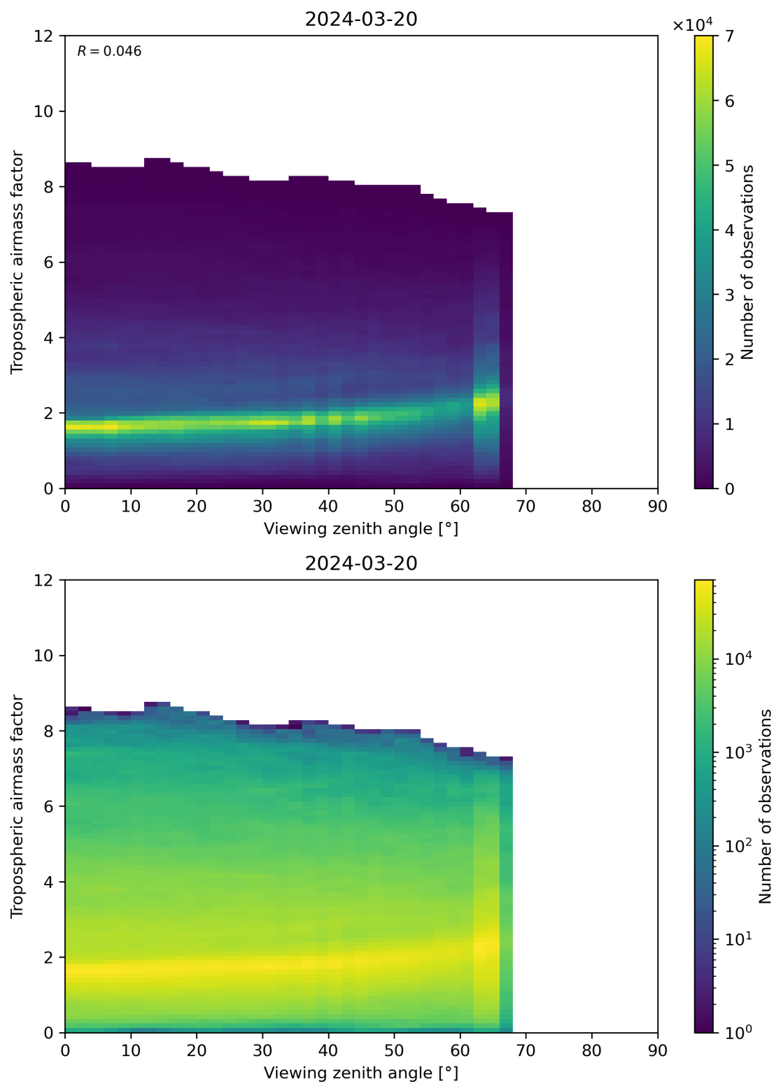
Figure 161: Scatter density plot of “Viewing zenith angle” against “Tropospheric airmass factor” for 2024-03-20 to 2024-03-21.
