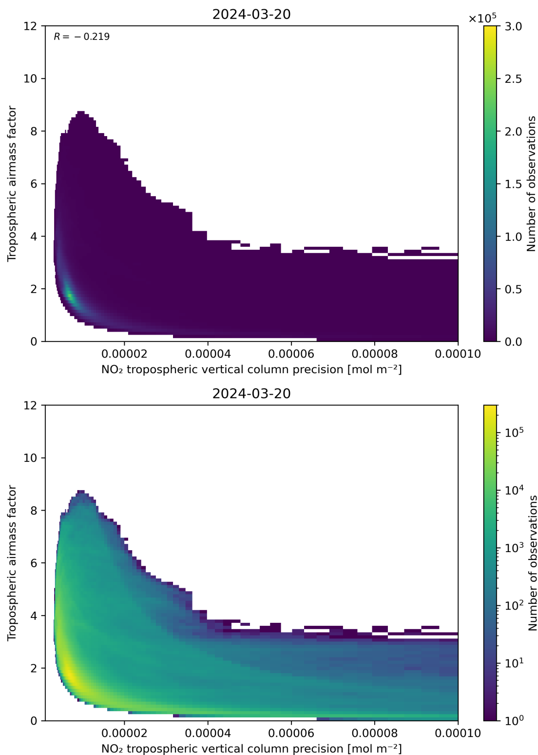
Figure 133: Scatter density plot of “NO 2 tropospheric vertical column precision” against “Tropospheric airmass factor” for 2024-03-20 to 2024-03-21.
