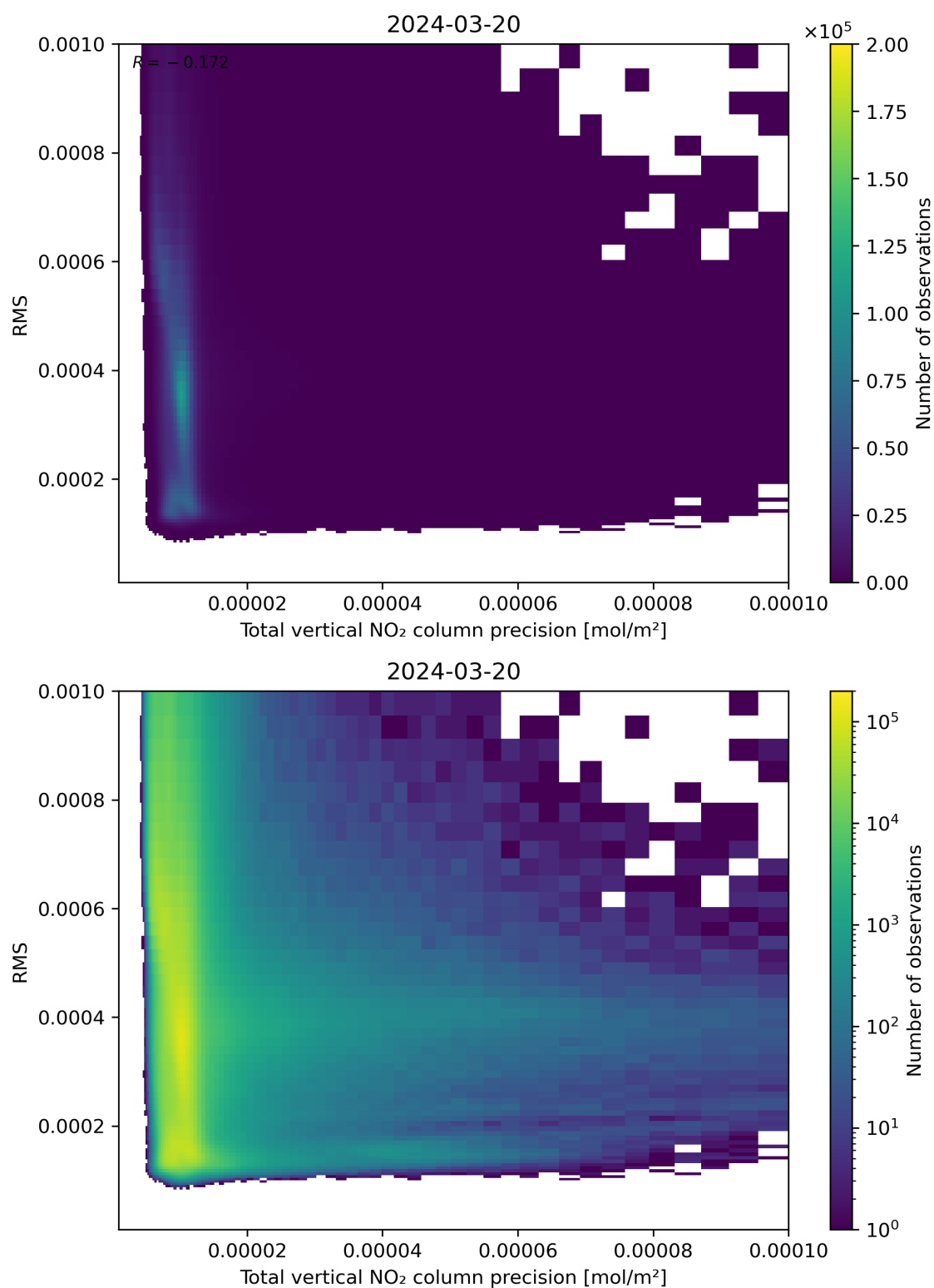
Figure 119: Scatter density plot of “Total vertical NO 2 column precision” against “RMS” for 2024-03-20 to 2024-03-21.
