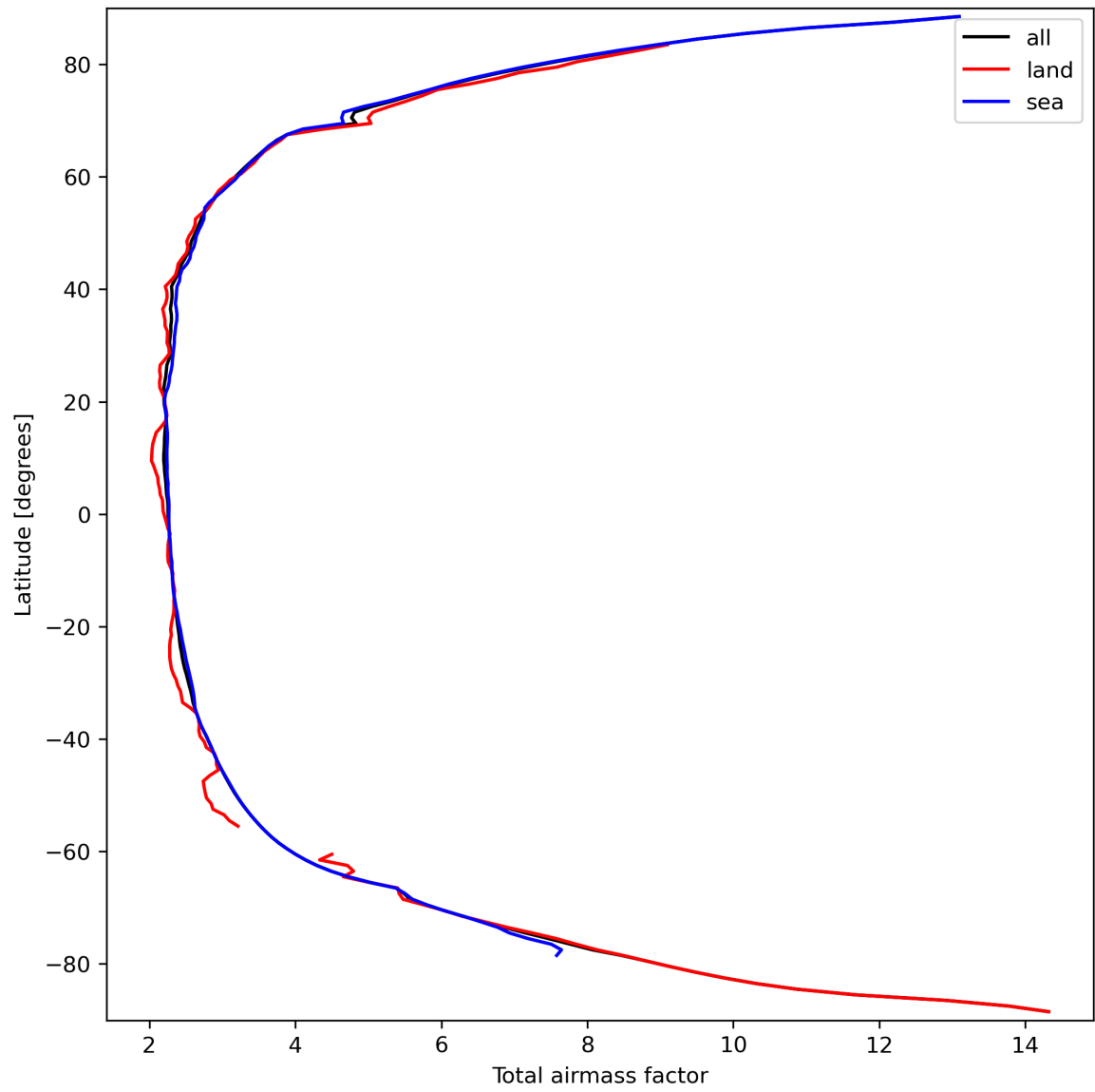
Figure 15: Zonal average of “Total airmass factor” for 2024-03-20 to 2024-03-21.
