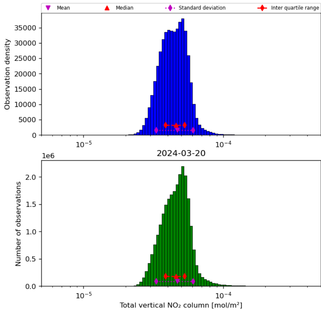
Figure 38: Histogram of “Total vertical NO 2 column” for 2024-03-20 to 2024-03-21
