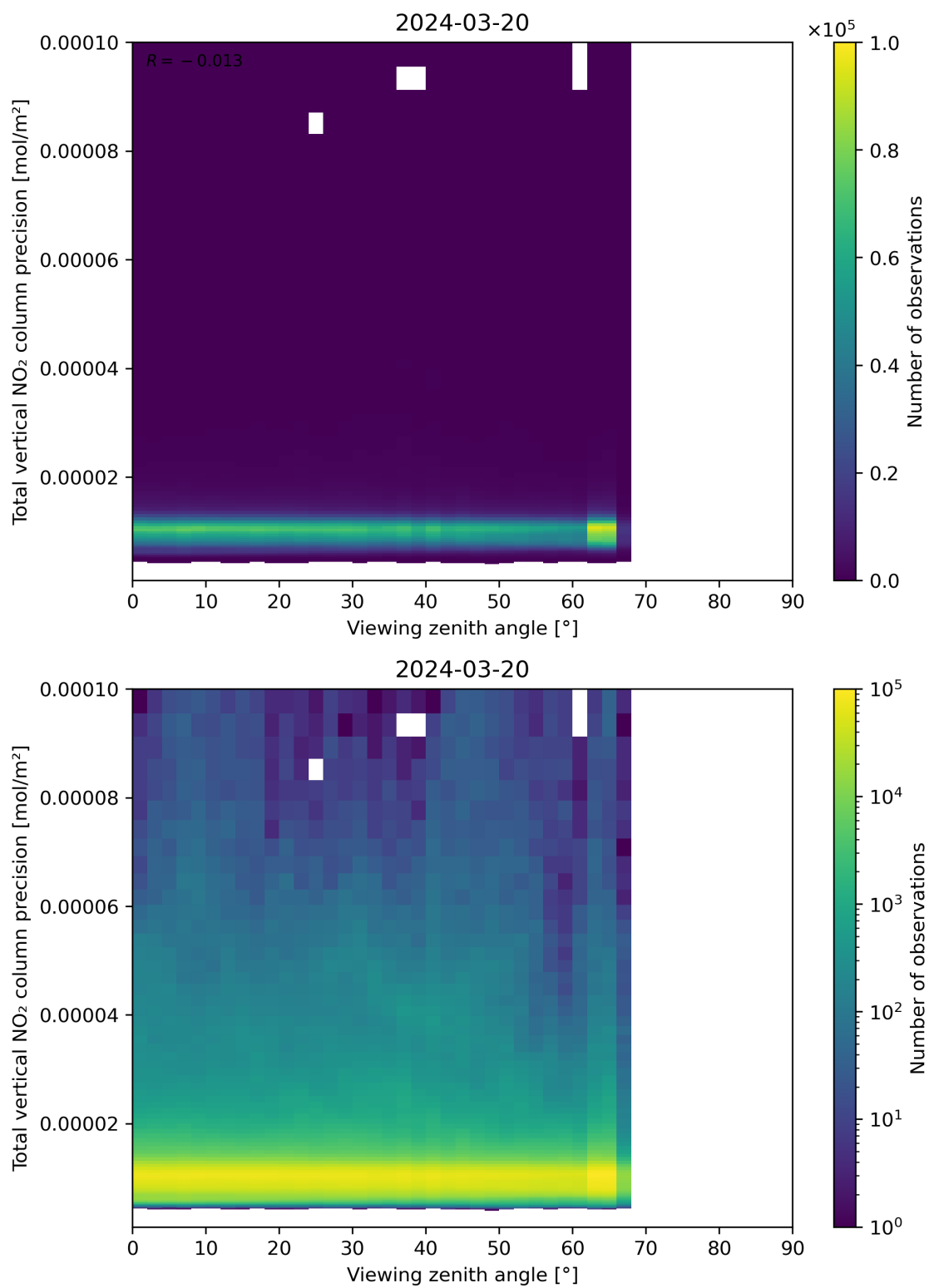
Figure 168: Scatter density plot of “Viewing zenith angle” against “Total vertical NO 2 column precision” for 2024-03-20 to 2024-03-21.
