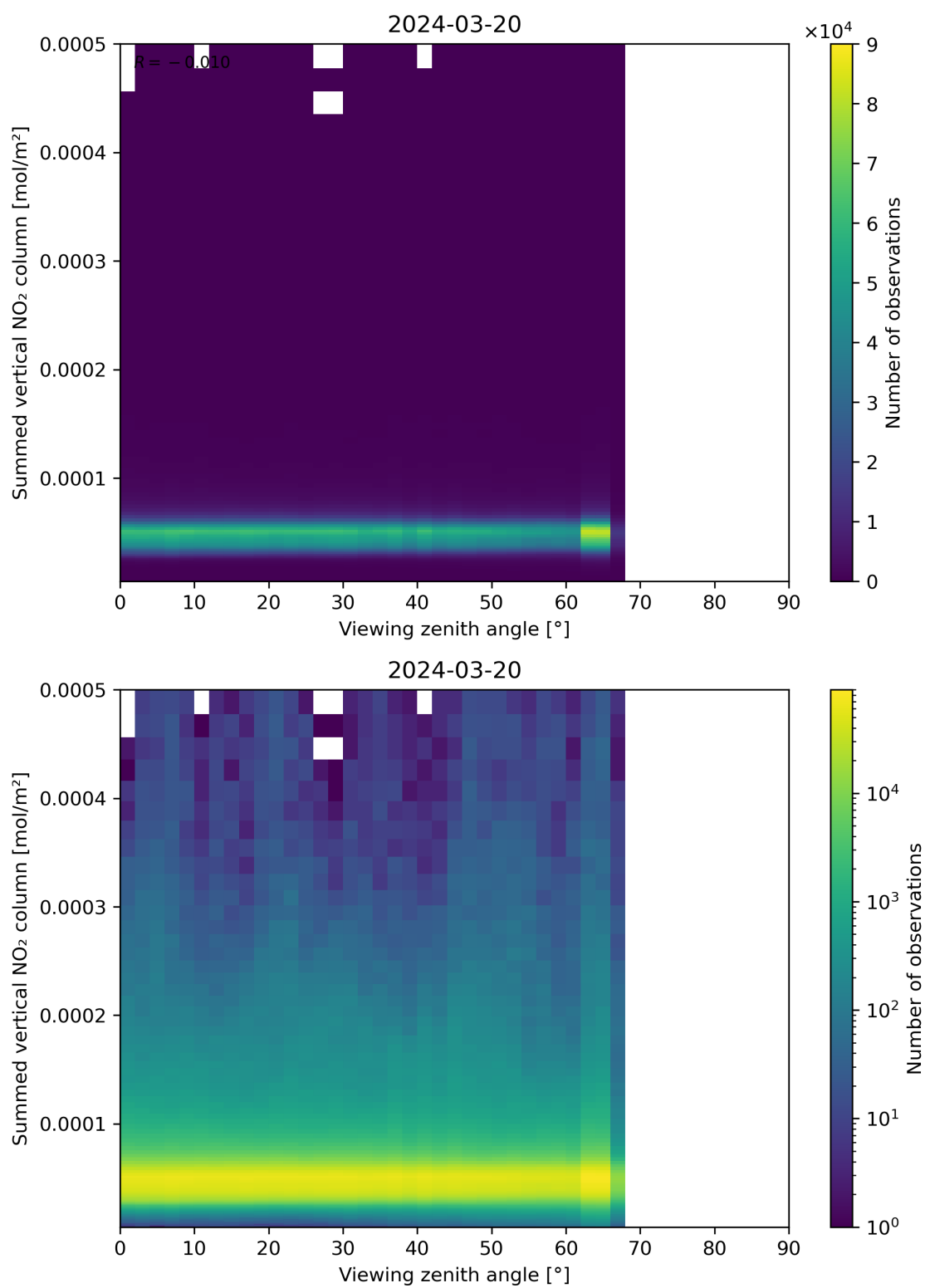
Figure 165: Scatter density plot of “Viewing zenith angle” against “Summed vertical NO 2 column” for 2024-03-20 to 2024-03-21.
