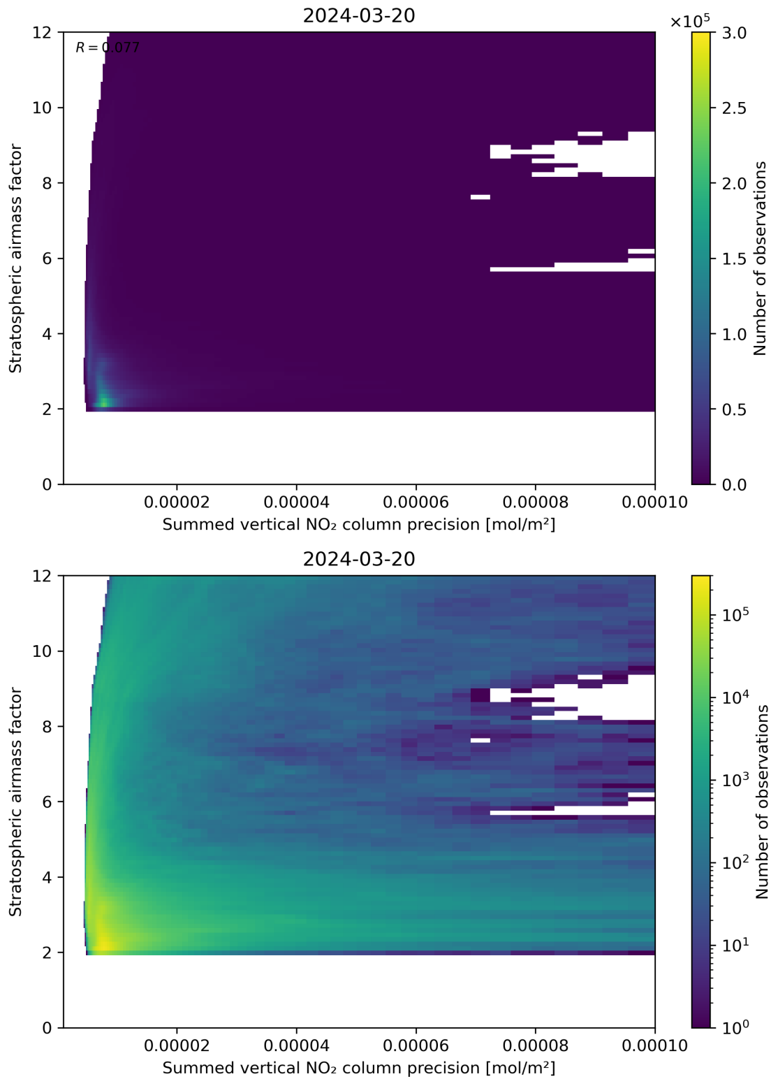
Figure 106: Scatter density plot of “Summed vertical NO 2 column precision” against “Stratospheric airmass factor” for 2024-03-20 to 2024-03-21.
