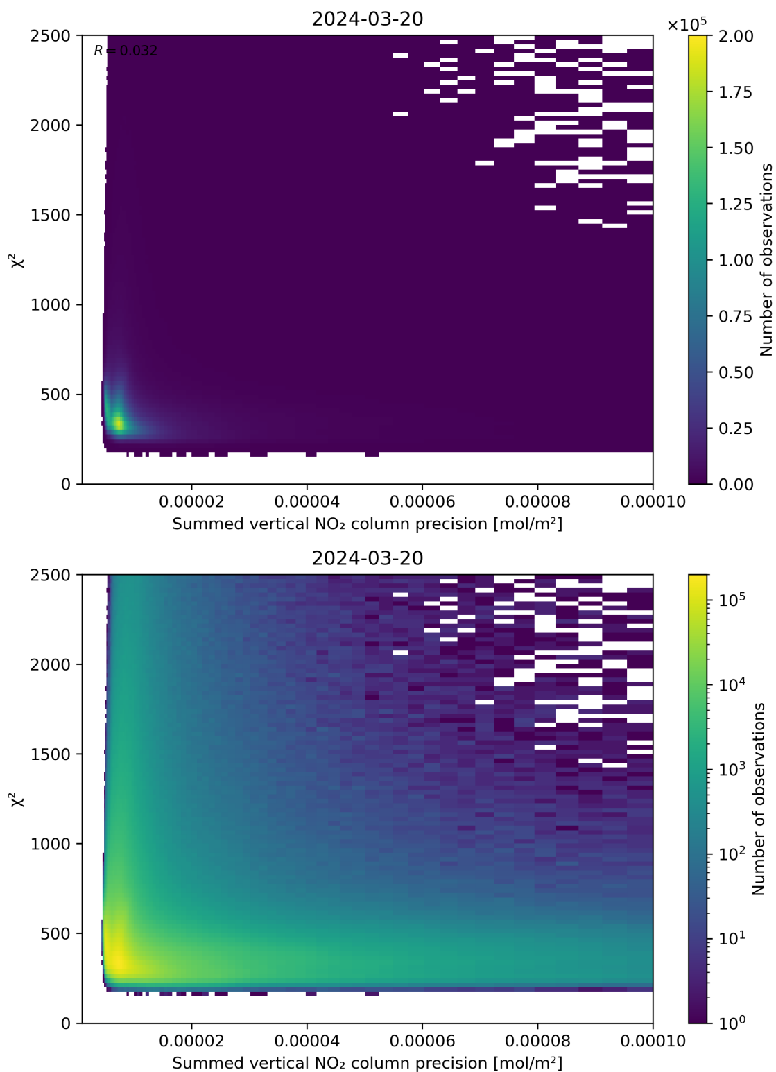
Figure 107: Scatter density plot of “Summed vertical NO 2 column precision” against “ \chi^2 ” for 2024-03-20 to 2024-03-21.
