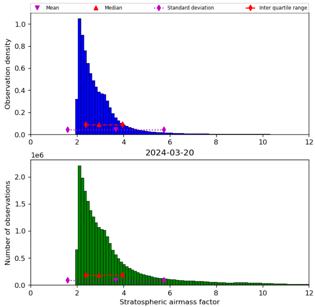
Figure 44: Histogram of “Stratospheric airmass factor” for 2024-03-20 to 2024-03-21
