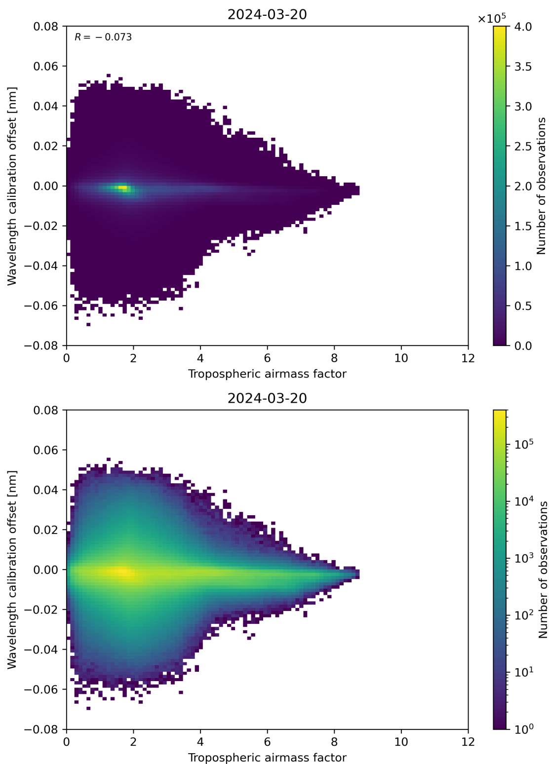
Figure 80: Scatter density plot of “Tropospheric airmass factor” against “Wavelength calibration offset” for 2024-03-20 to 2024-03-21.
