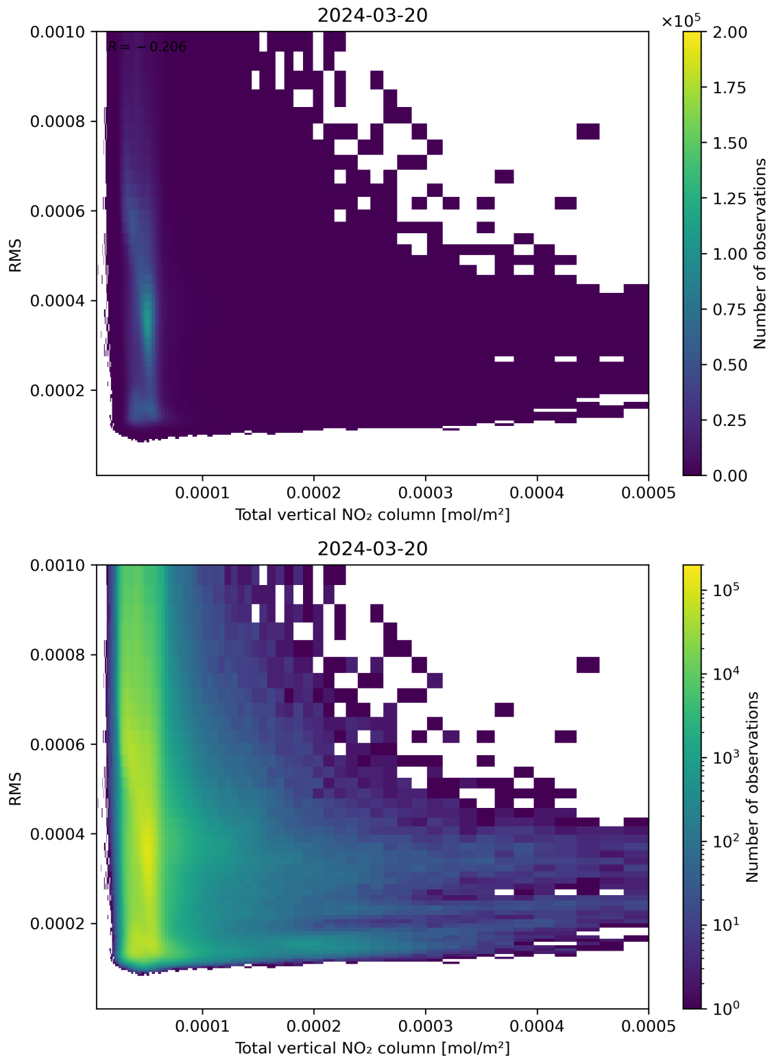
Figure 120: Scatter density plot of “Total vertical NO 2 column” against “RMS” for 2024-03-20 to 2024-03-21.
