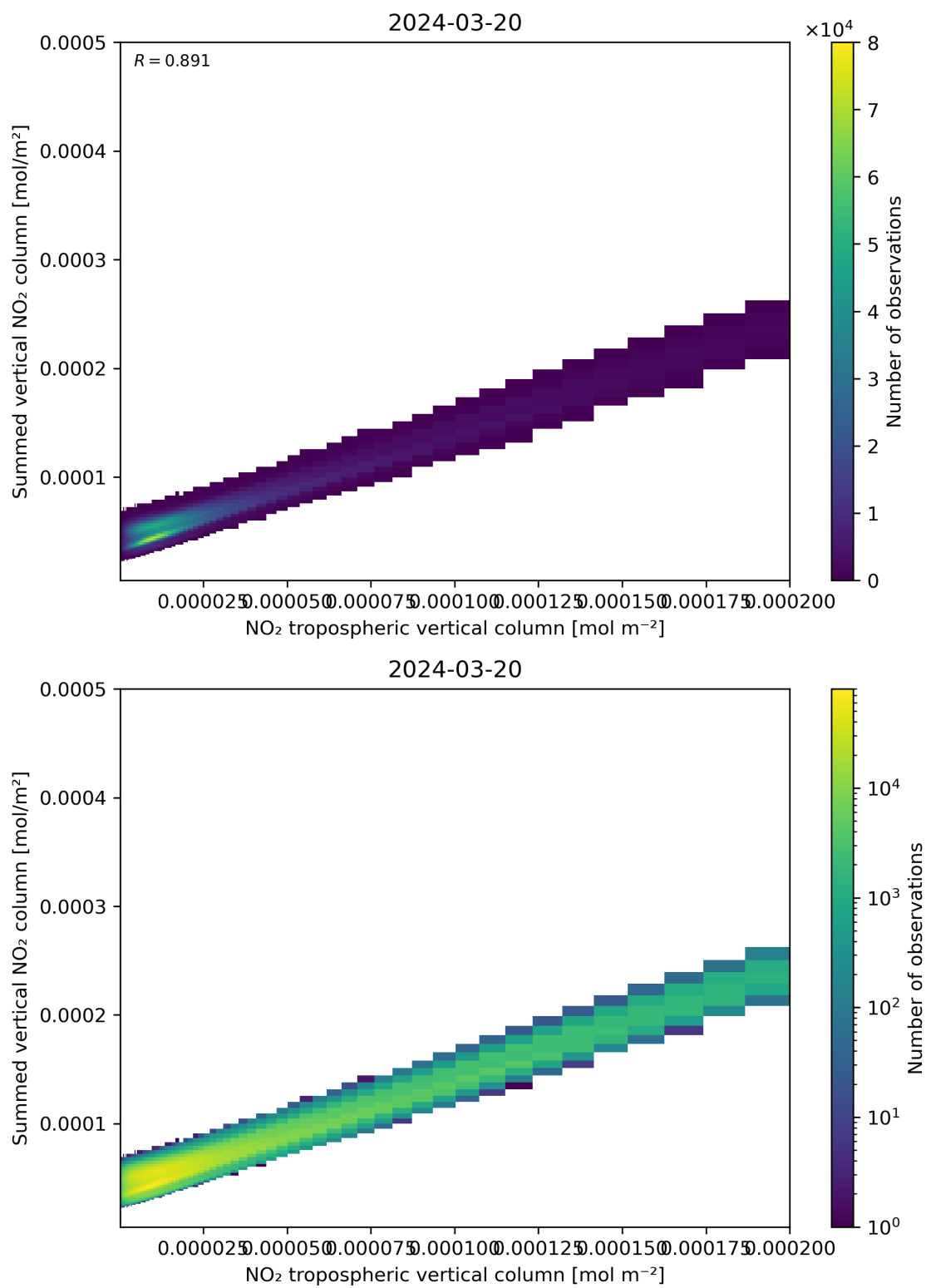
Figure 126: Scatter density plot of “NO 2 tropospheric vertical column” against “Summed vertical NO 2 column” for 2024-03-20 to 2024-03-21.
