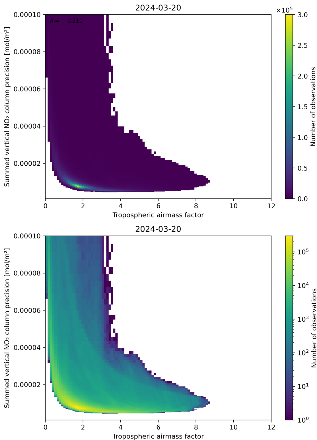
Figure 76: Scatter density plot of “Tropospheric air mass factor” against “Summed vertical NO 2 column precision” for 2024-03-20 to 2024-03-21.
