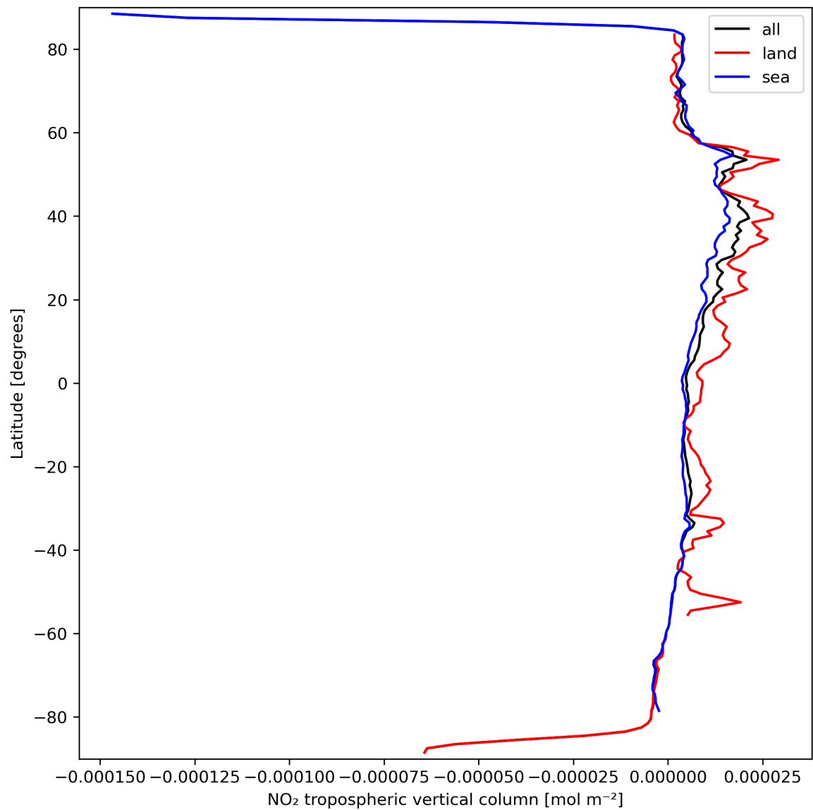
Figure 12: Zonal average of “NO 2 tropospheric vertical column” for 2024-03-20 to 2024-03-21.
