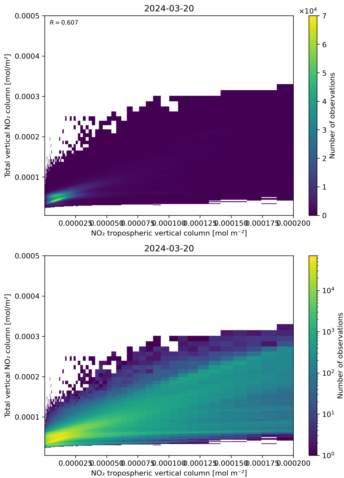
Figure 128: Scatter density plot of “NO 2 tropospheric vertical column” against “Total vertical NO 2 column” for 2024-03-20 to 2024-03-21.
