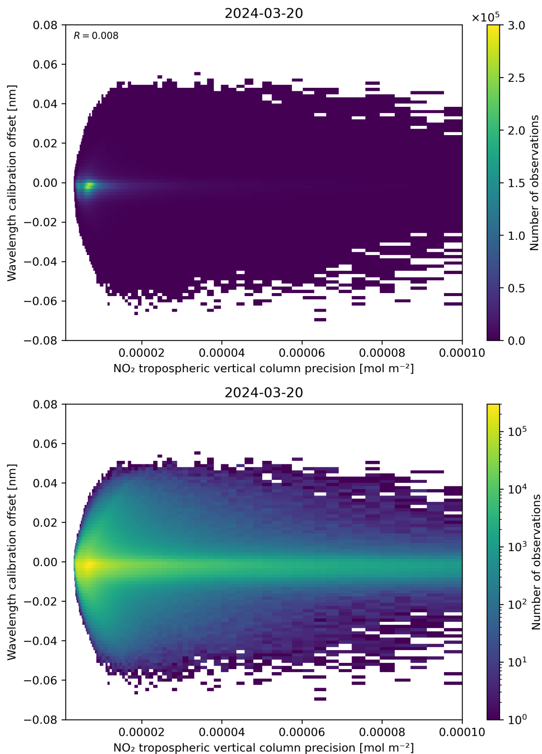
Figure 141: Scatter density plot of “NO 2 tropospheric vertical column precision” against “Wavelength calibration offset” for 2024-03-20 to 2024-03-21.
