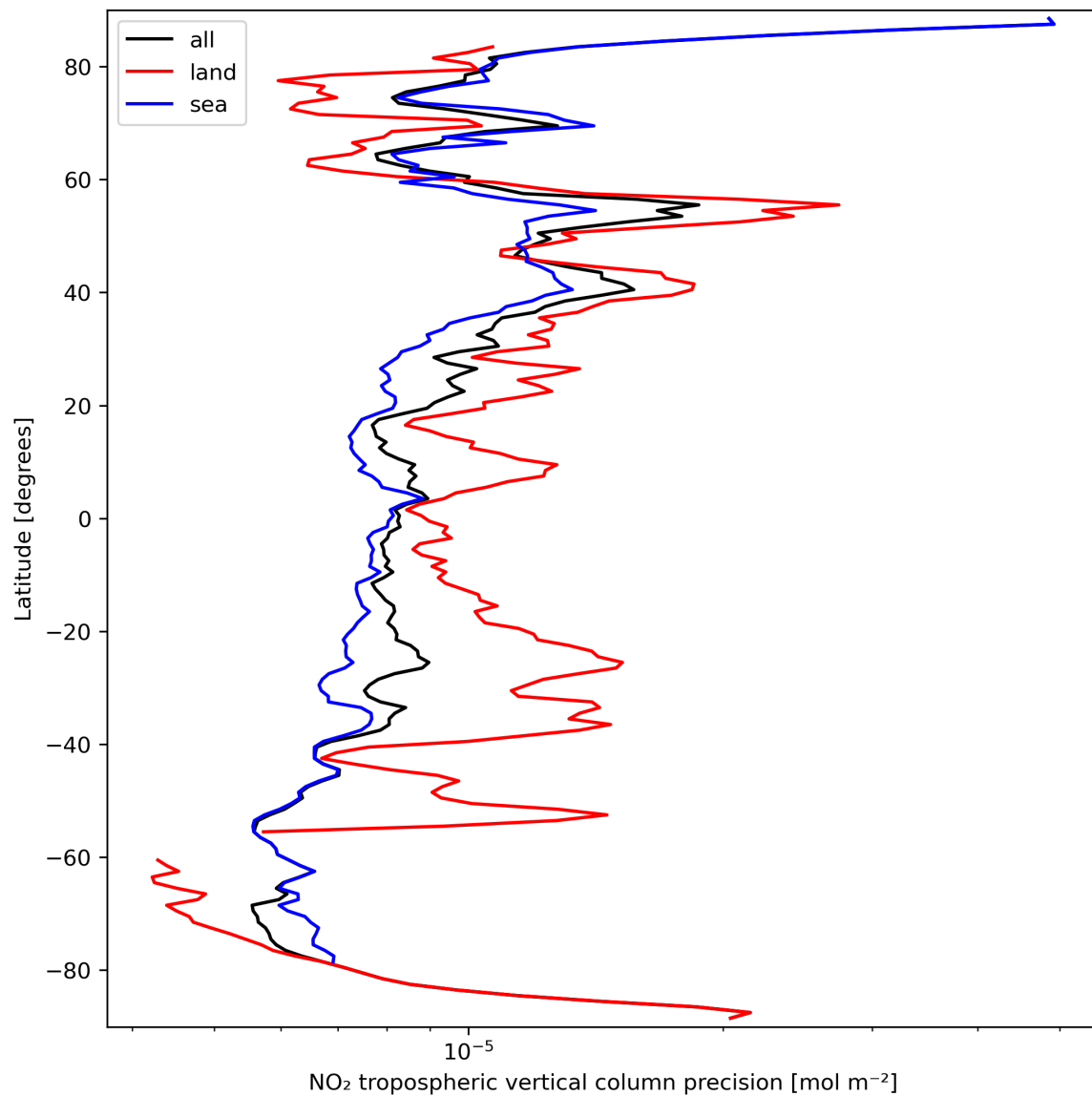
Figure 13: Zonal average of “NO 2 tropospheric vertical column precision” for 2024-03-20 to 2024-03-21.
