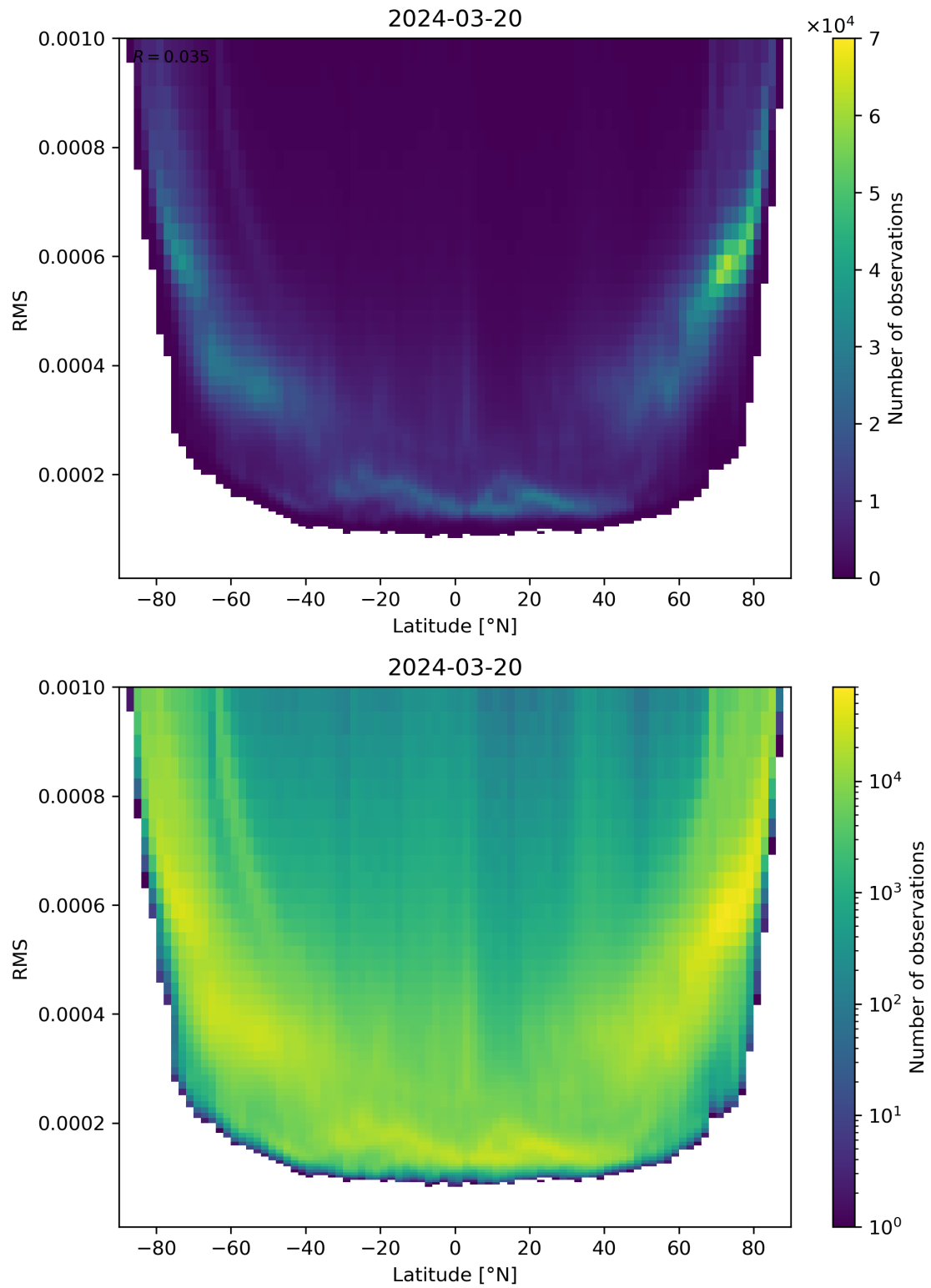
Figure 94: Scatter density plot of “Latitude” against “RMS” for 2024-03-20 to 2024-03-21.
