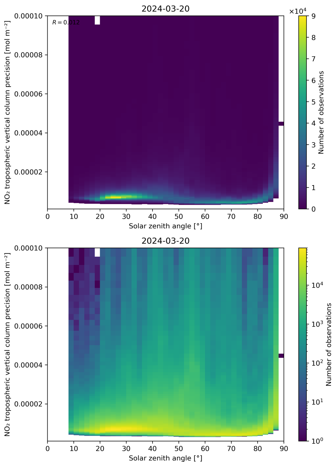
Figure 156: Scatter density plot of “Solar zenith angle” against “NO 2 tropospheric vertical column precision” for 2024-03-20 to 2024-03-21.
