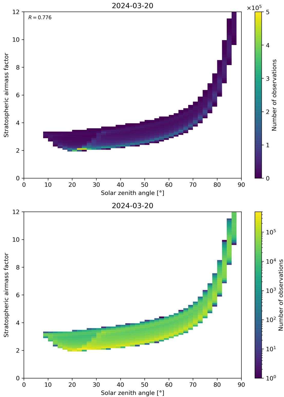
Figure 145: Scatter density plot of “Solar zenith angle” against “Stratospheric airmass factor” for 2024-03-20 to 2024-03-21.
