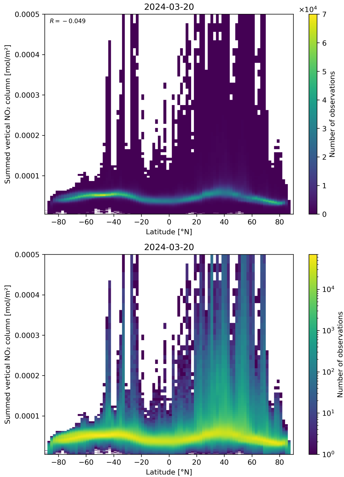
Figure 88: Scatter density plot of “Latitude” against “Summed vertical NO 2 column” for 2024-03-20 to 2024-03-21.
