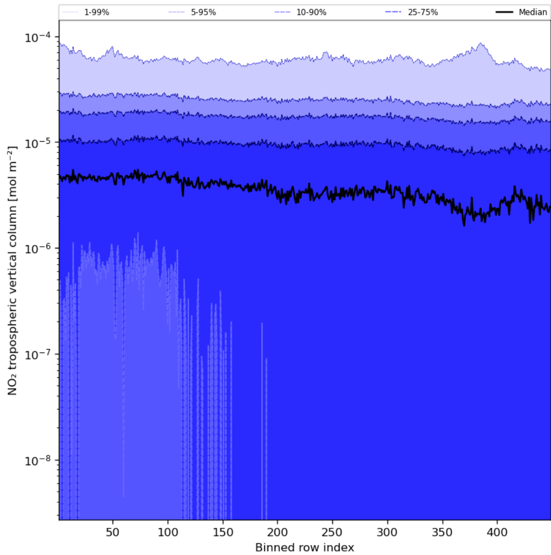
Figure 46: Along track statistics of “NO 2 tropospheric vertical column” for 2024-03-20 to 2024-03-21
