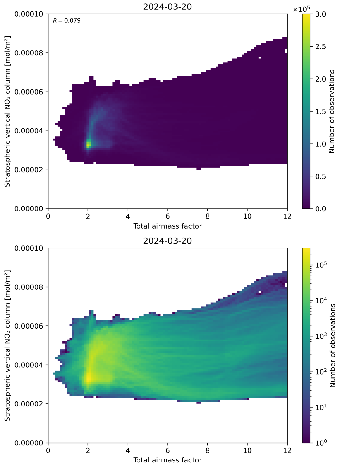
Figure 64: Scatter density plot of “Total airmass factor” against “Stratospheric vertical NO 2 column” for 2024-03-20 to 2024-03-21.
