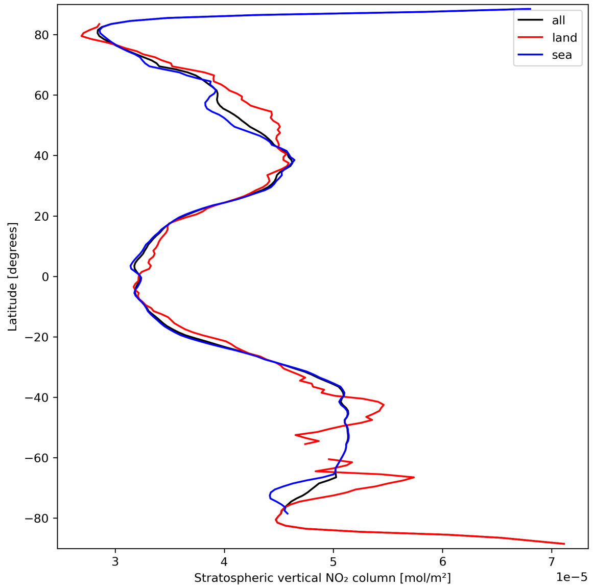
Figure 19: Zonal average of “Stratospheric vertical NO 2 column” for 2024-03-20 to 2024-03-21.
