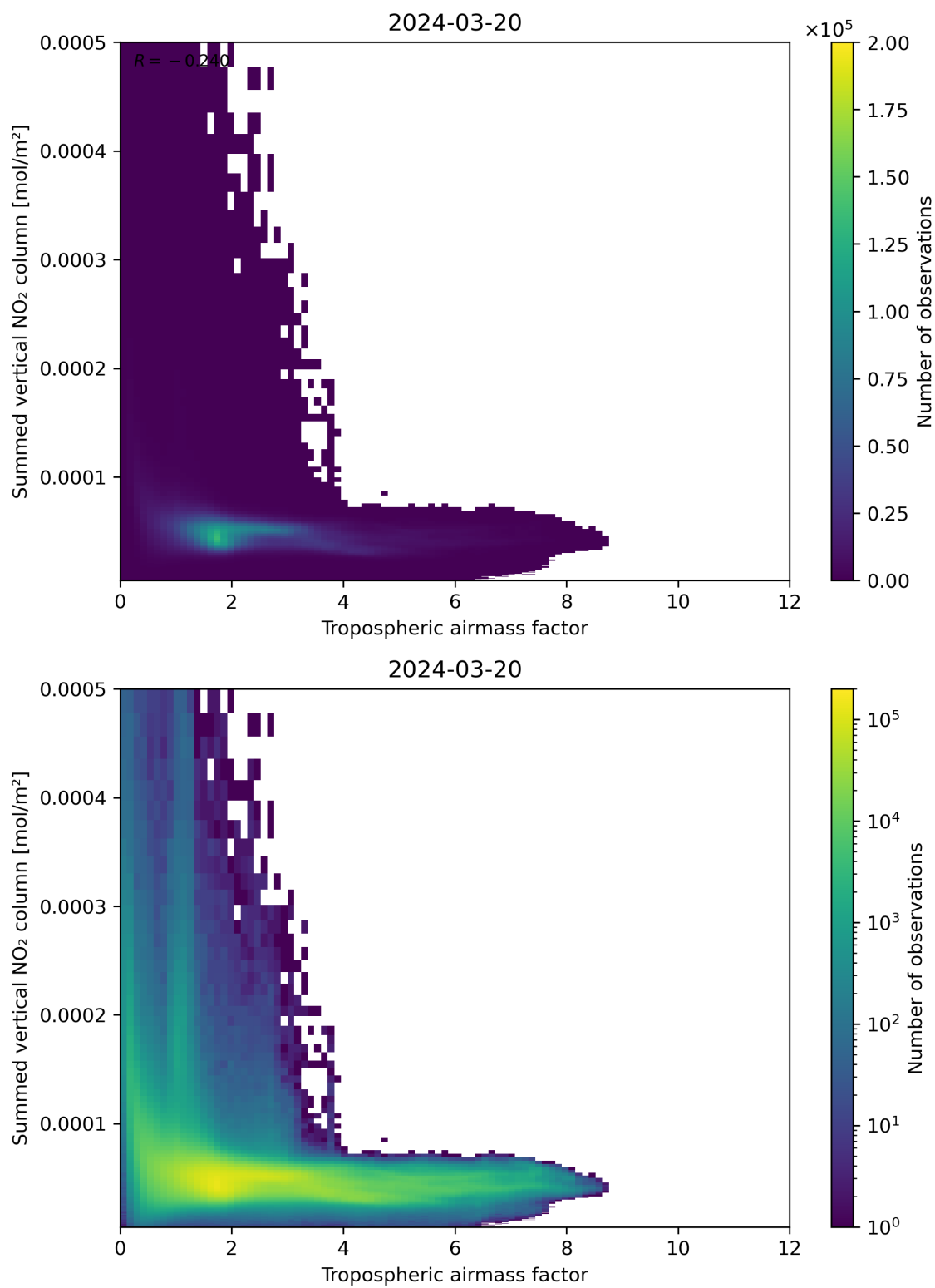
Figure 75: Scatter density plot of “Tropospheric air mass factor” against “Summed vertical NO 2 column” for 2024-03-20 to 2024-03-21.
