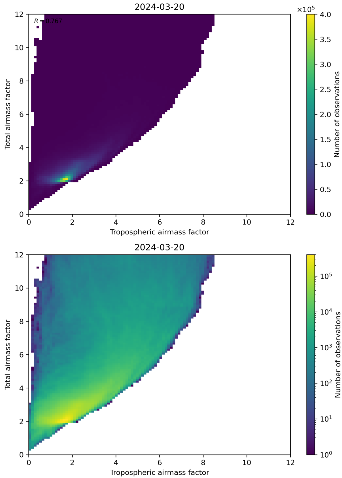
Figure 72: Scatter density plot of “Tropospheric airmass factor” against “Total airmass factor” for 2024-03-20 to 2024-03-21.
