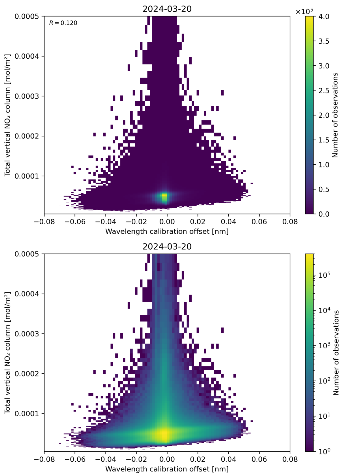
Figure 179: Scatter density plot of “Wavelength calibration offset” against “Total vertical NO 2 column” for 2024-03-20 to 2024-03-21.
