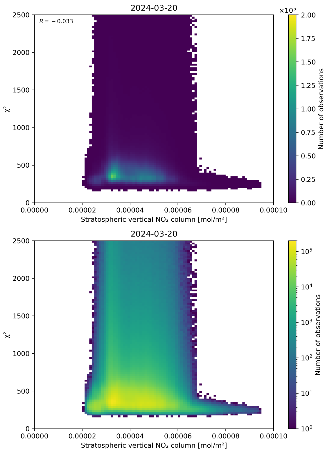
Figure 97: Scatter density plot of “Stratospheric vertical NO 2 column” against “ \chi^2 ” for 2024-03-20 to 2024-03-21.
