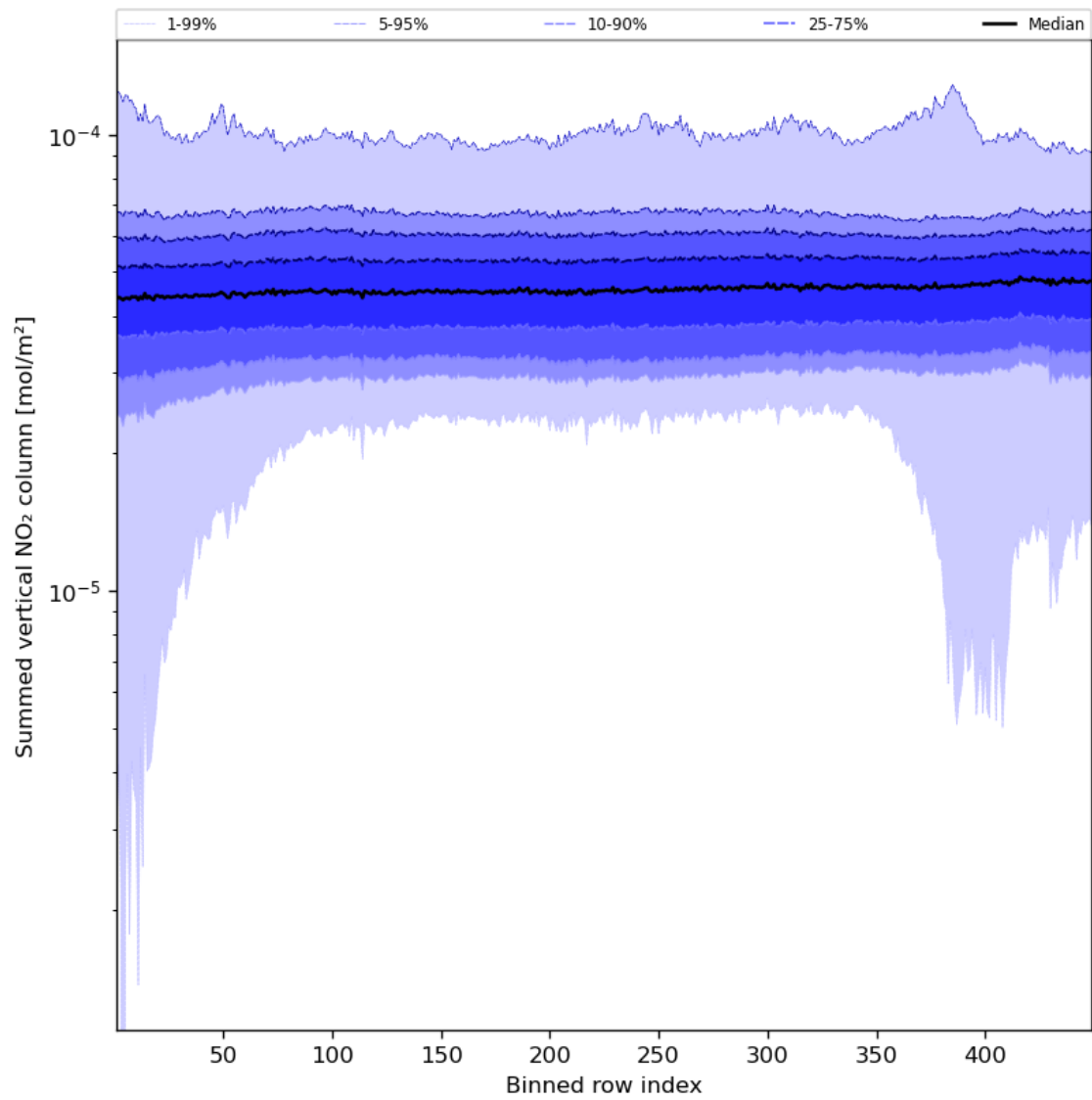
Figure 57: Along track statistics of “Summed vertical NO 2 column” for 2024-03-20 to 2024-03-21
