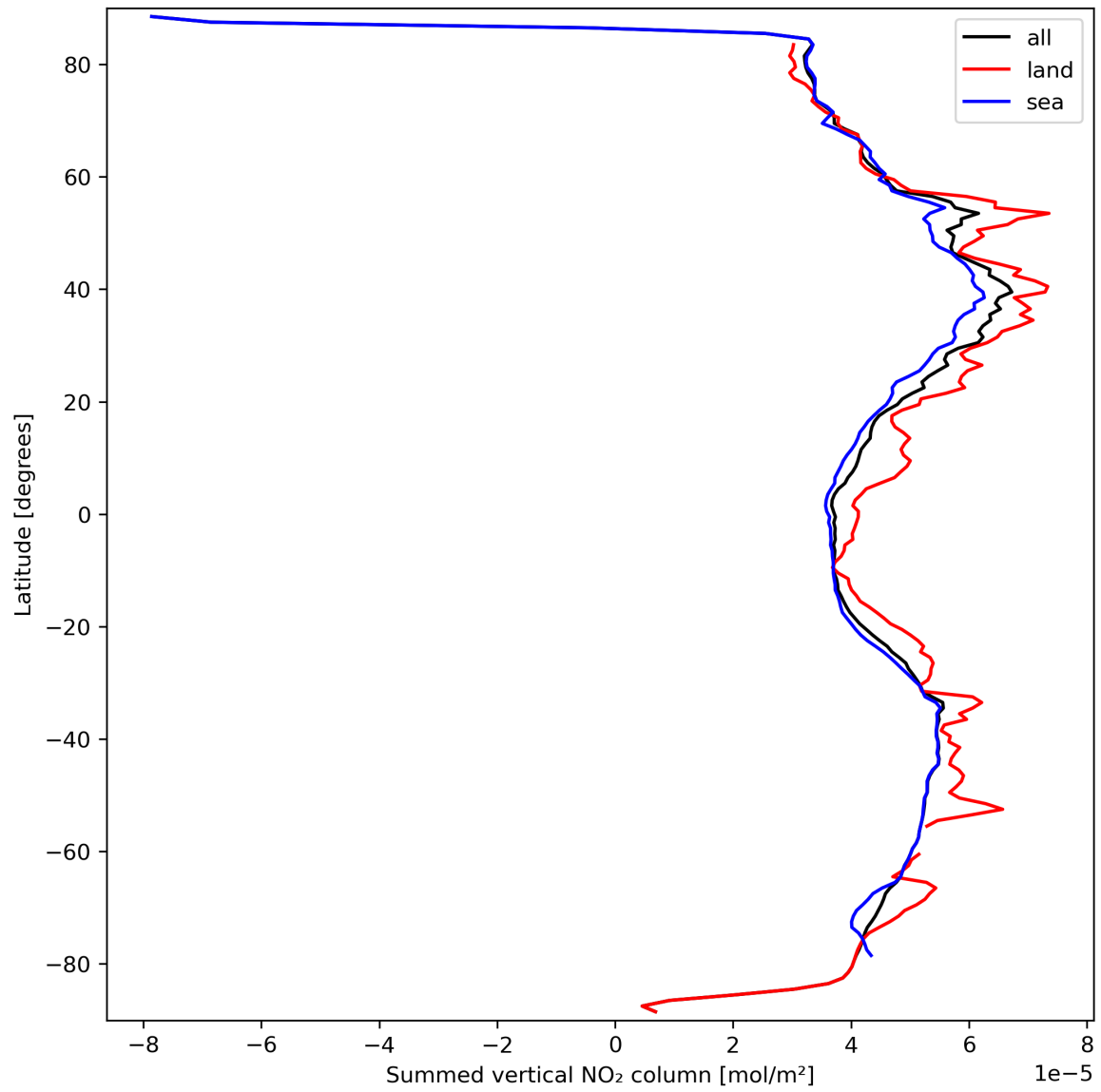
Figure 23: Zonal average of “Summed vertical NO 2 column” for 2024-03-20 to 2024-03-21.
