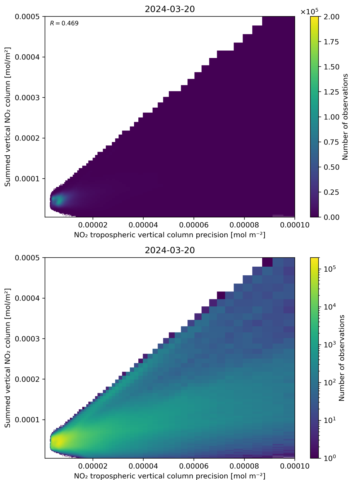
Figure 136: Scatter density plot of “NO 2 tropospheric vertical column precision” against “Summed vertical NO 2 column” for 2024-03-20 to 2024-03-21.
