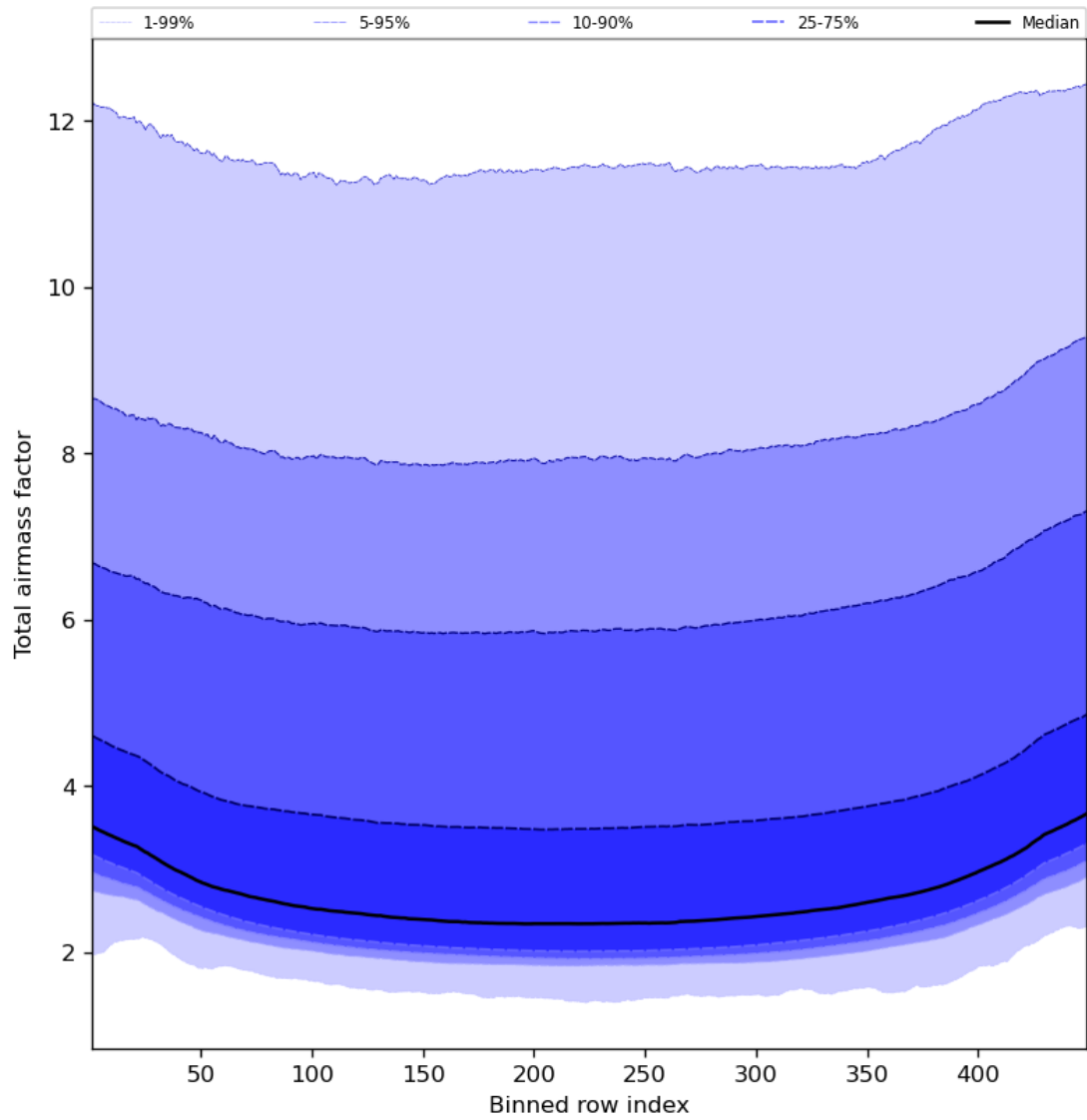
Figure 49: Along track statistics of “Total airmass factor” for 2024-03-20 to 2024-03-21
