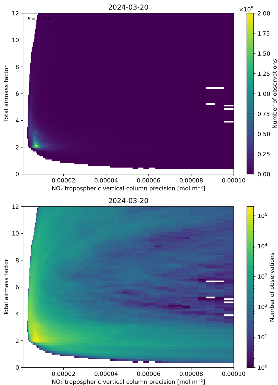
Figure 132: Scatter density plot of “NO 2 tropospheric vertical column precision” against “Total air mass factor” for 2024-03-20 to 2024-03-21.
