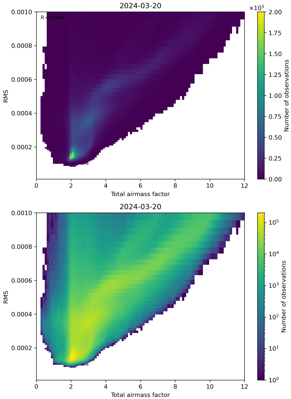
Figure 69: Scatter density plot of “Total airmass factor” against “RMS” for 2024-03-20 to 2024-03-21.
