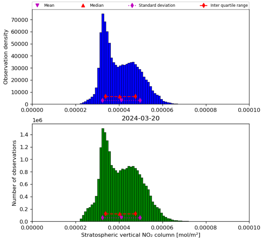
Figure 36: Histogram of “Stratospheric vertical NO 2 column” for 2024-03-20 to 2024-03-21
