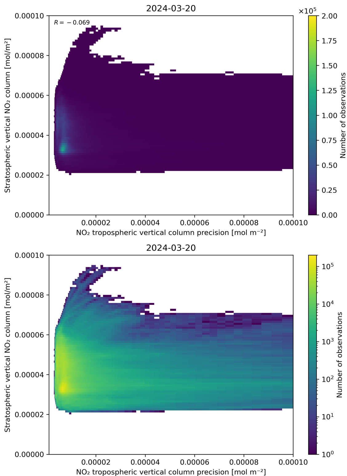
Figure 135: Scatter density plot of “NO 2 tropospheric vertical column precision” against “Stratospheric vertical NO 2 column” for 2024-03-20 to 2024-03-21.
