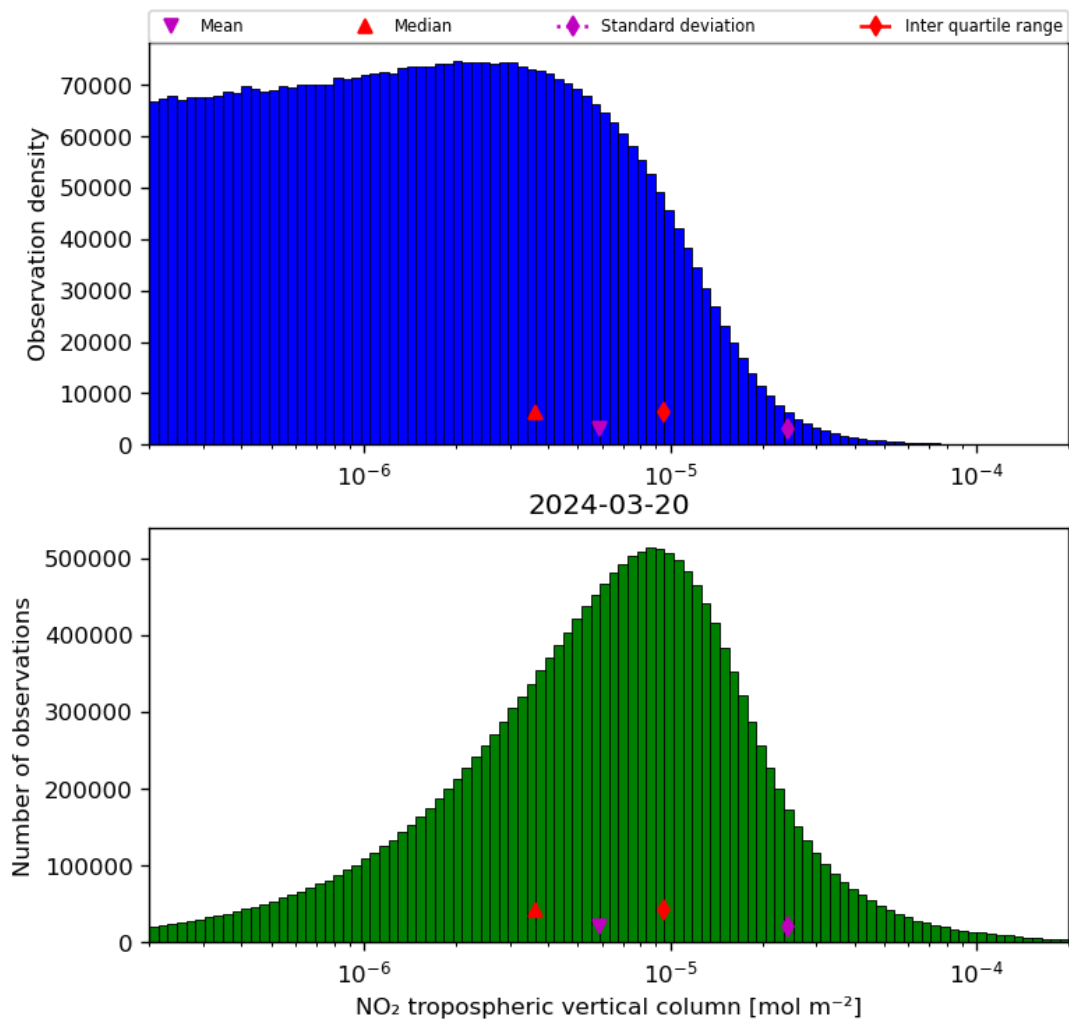
Figure 29: Histogram of “ \text{NO}_2 tropospheric vertical column” for 2024-03-20 to 2024-03-21
