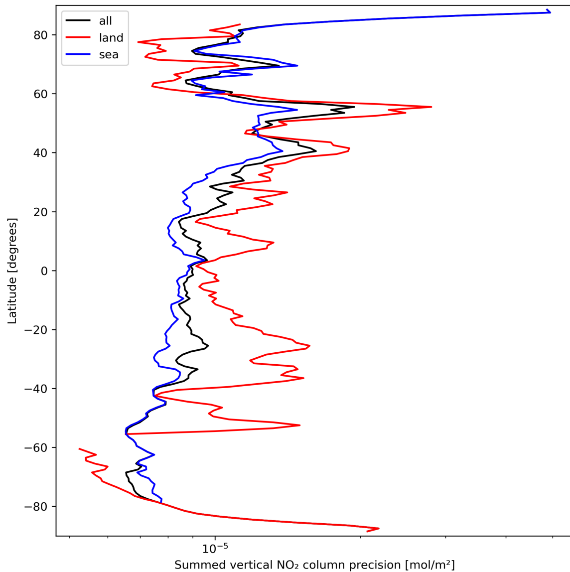
Figure 24: Zonal average of “Summed vertical NO 2 column precision” for 2024-03-20 to 2024-03-21.
