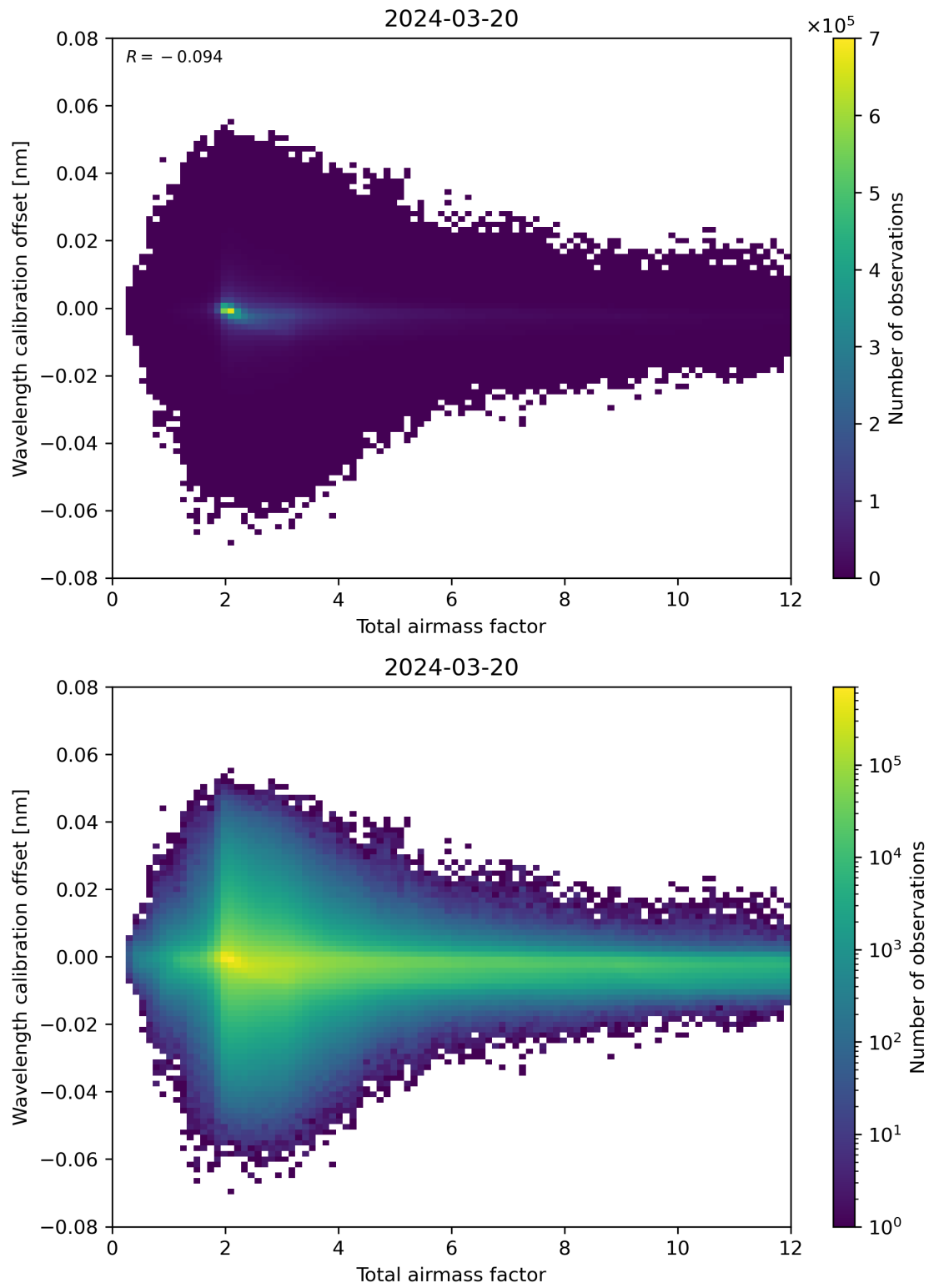
Figure 70: Scatter density plot of “Total airmass factor” against “Wavelength calibration offset” for 2024-03-20 to 2024-03-21.
