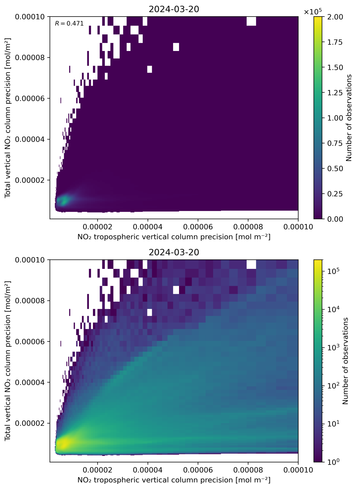
Figure 139: Scatter density plot of “NO 2 tropospheric vertical column precision” against “Total vertical NO 2 column precision” for 2024-03-20 to 2024-03-21.
