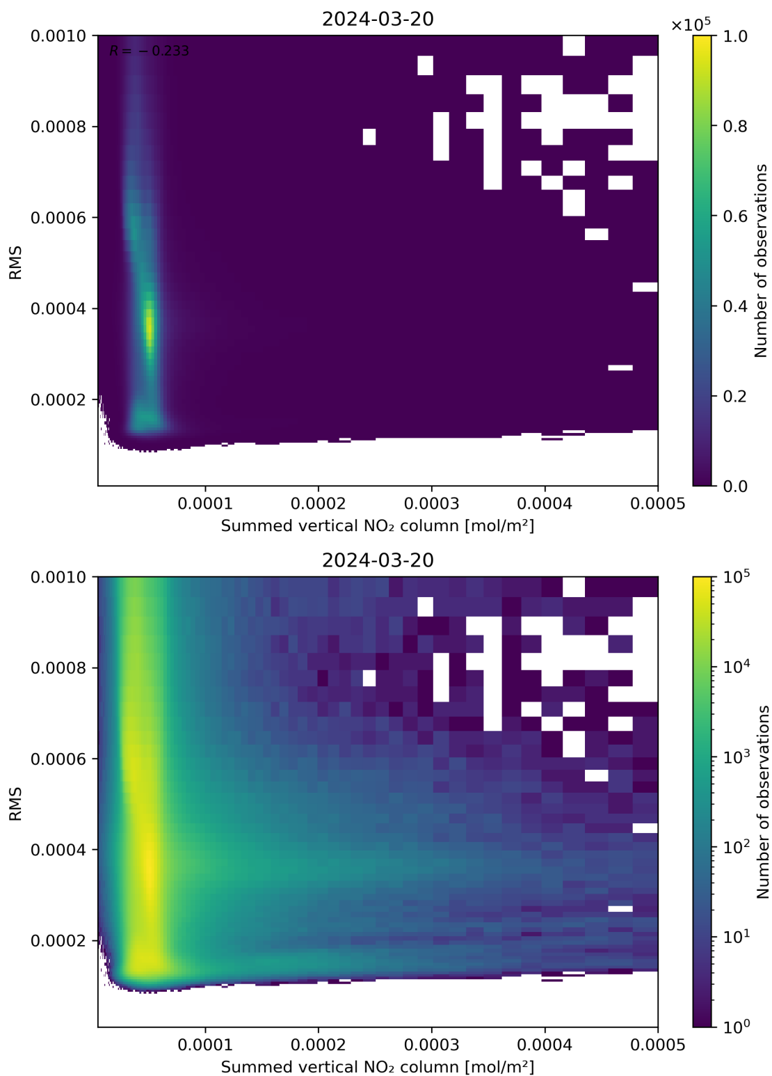
Figure 109: Scatter density plot of “Summed vertical NO 2 column” against “RMS” for 2024-03-20 to 2024-03-21.
