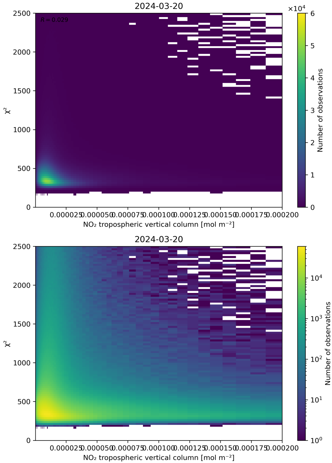
Figure 124: Scatter density plot of “NO 2 tropospheric vertical column” against “ \chi^2 ” for 2024-03-20 to 2024-03-21.
