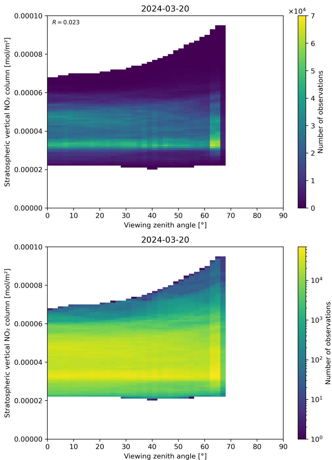
Figure 164: Scatter density plot of “Viewing zenith angle” against “Stratospheric vertical NO 2 column” for 2024-03-20 to 2024-03-21.
