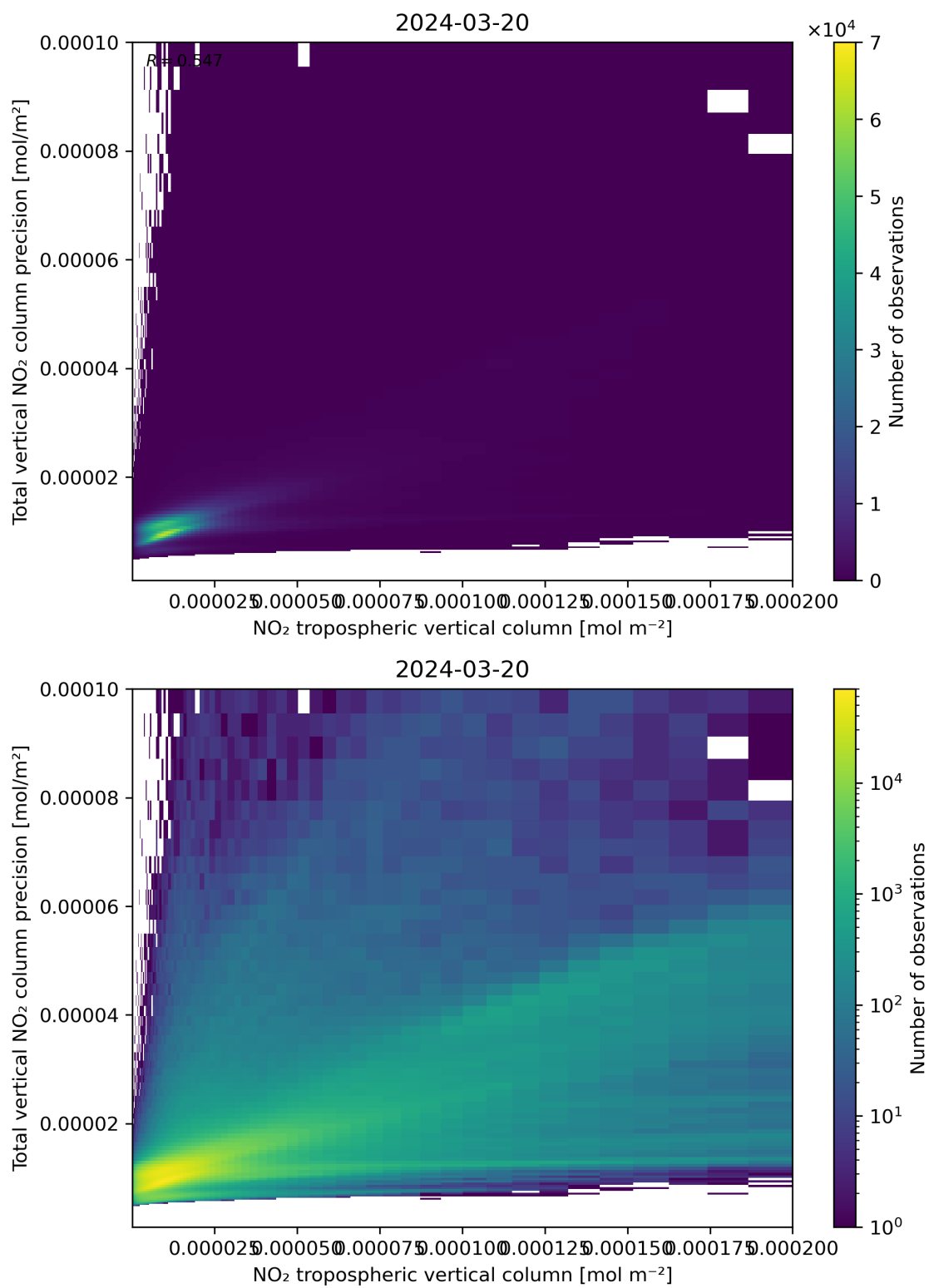
Figure 129: Scatter density plot of “NO 2 tropospheric vertical column” against “Total vertical NO 2 column precision” for 2024-03-20 to 2024-03-21.
