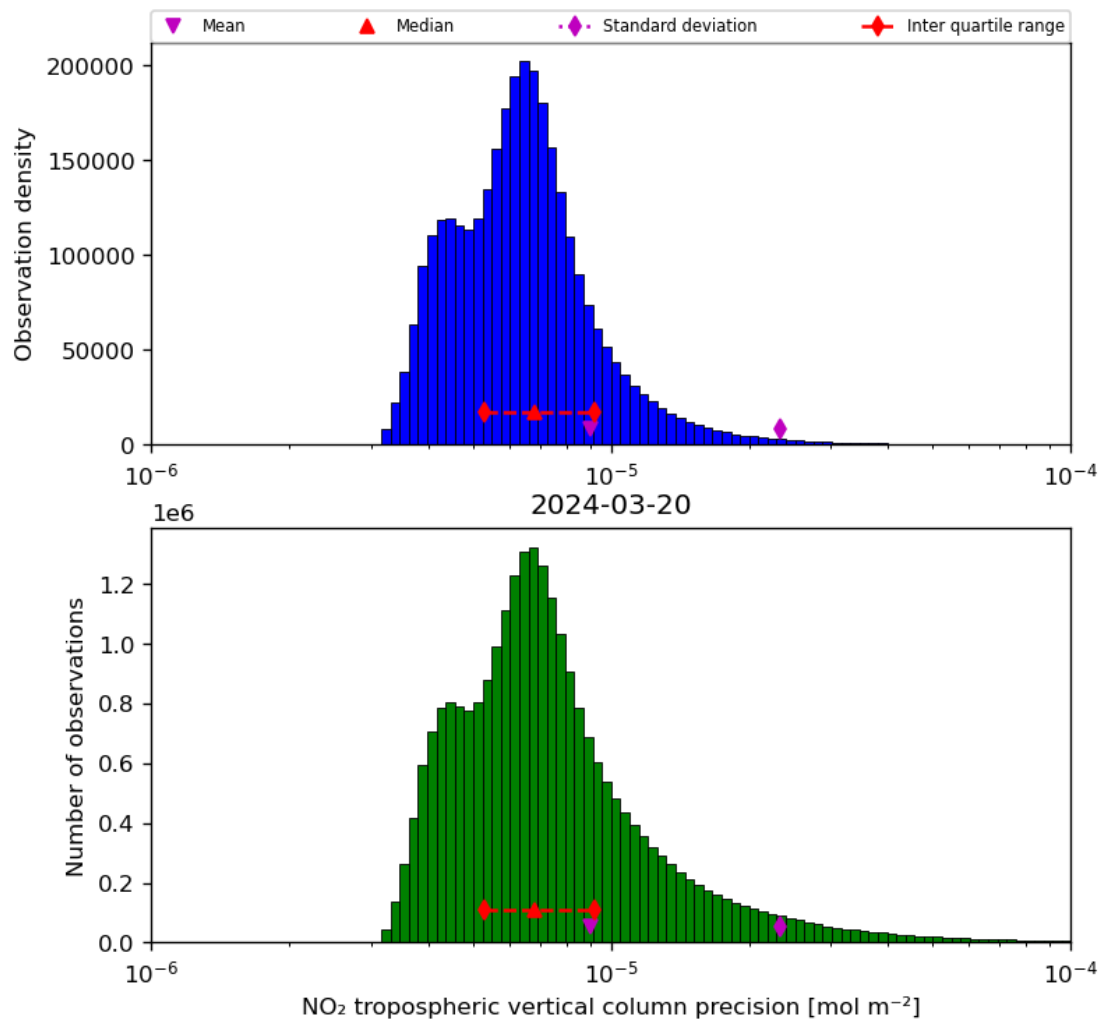
Figure 30: Histogram of “NO 2 tropospheric vertical column precision” for 2024-03-20 to 2024-03-21
