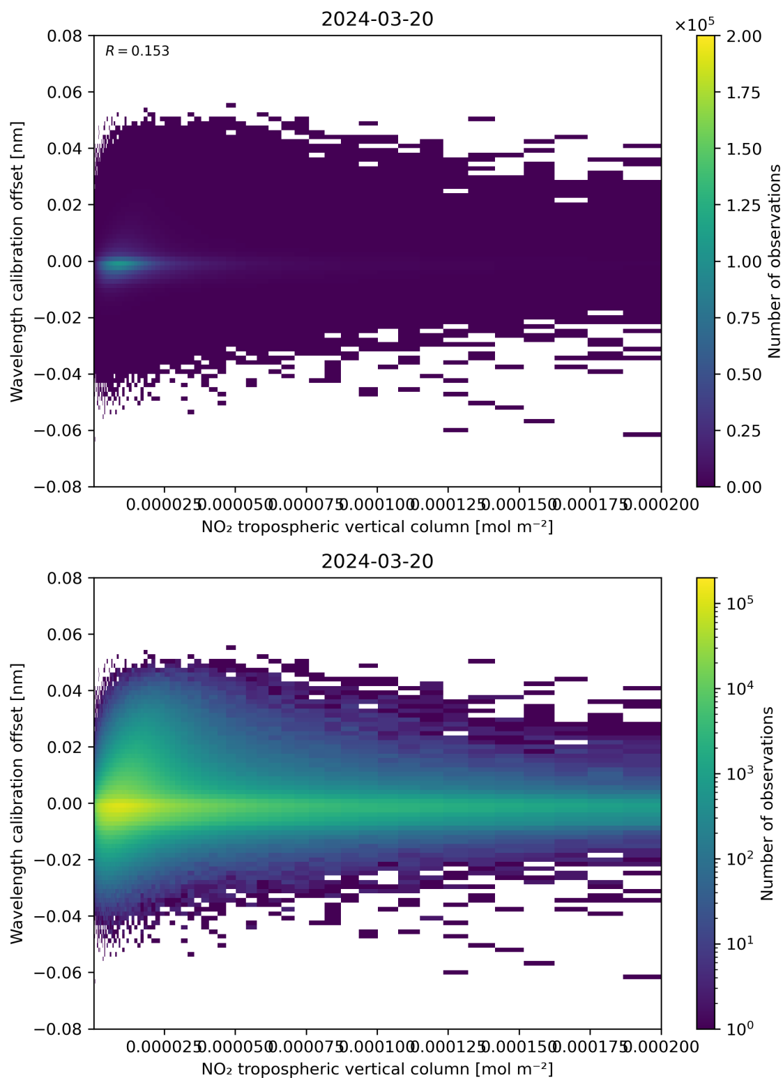
Figure 143: Scatter density plot of “NO 2 tropospheric vertical column” against “Wavelength calibration offset” for 2024-03-20 to 2024-03-21.
