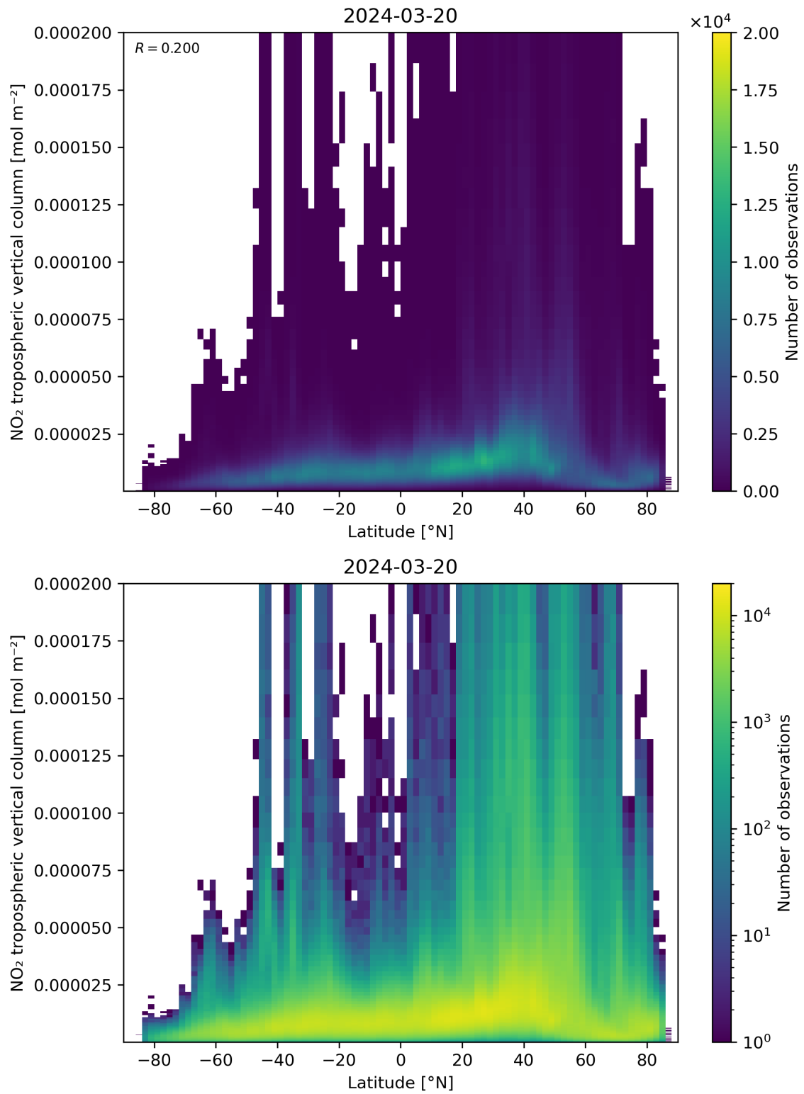
Figure 92: Scatter density plot of “Latitude” against “NO 2 tropospheric vertical column” for 2024-03-20 to 2024-03-21.
