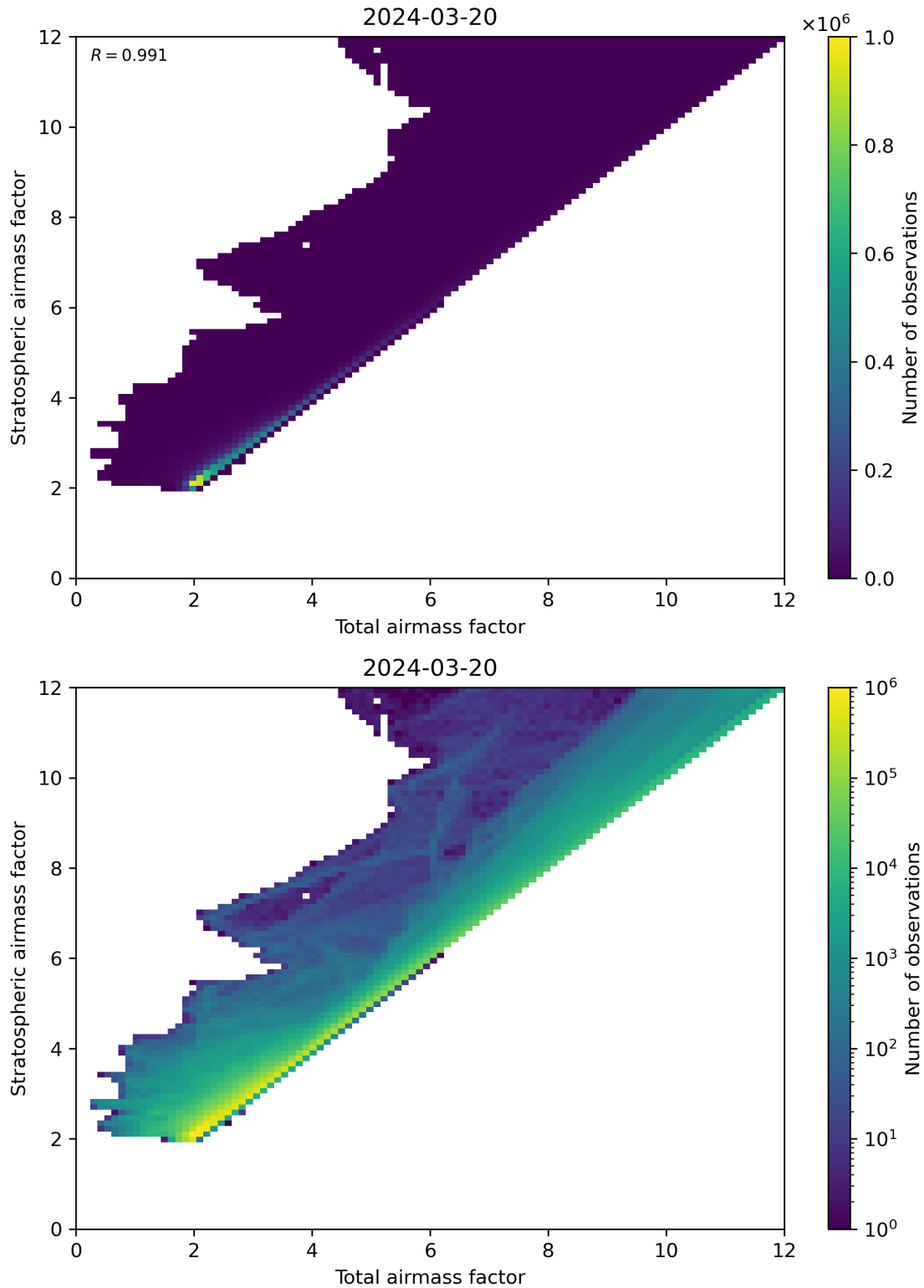
Figure 62: Scatter density plot of “Total airmass factor” against “Stratospheric airmass factor” for 2024-03-20 to 2024-03-21.
