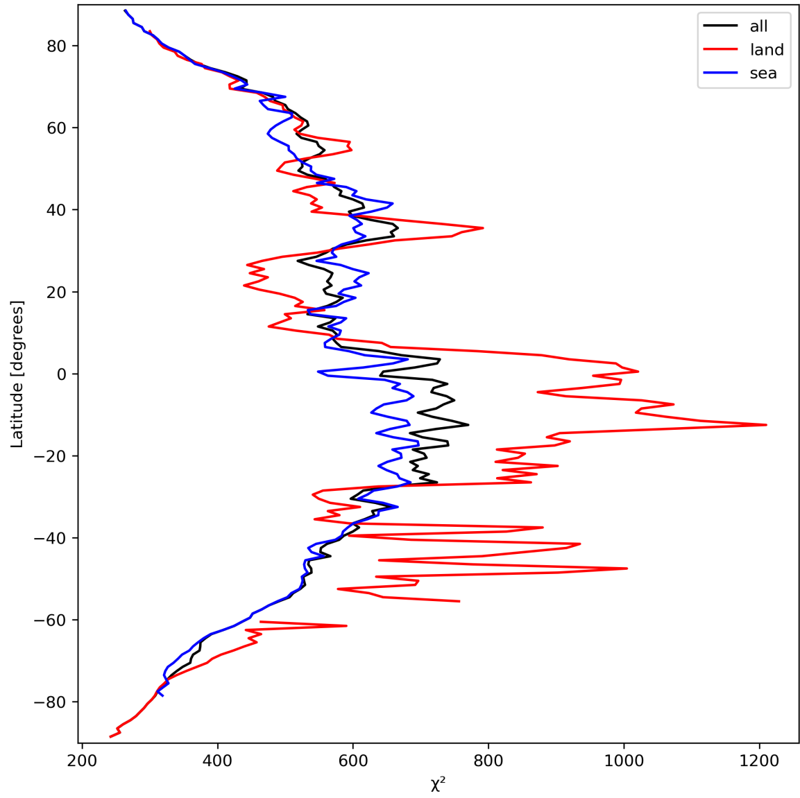
Figure 25: Zonal average of “ \chi^2 ” for 2024-03-20 to 2024-03-21.
