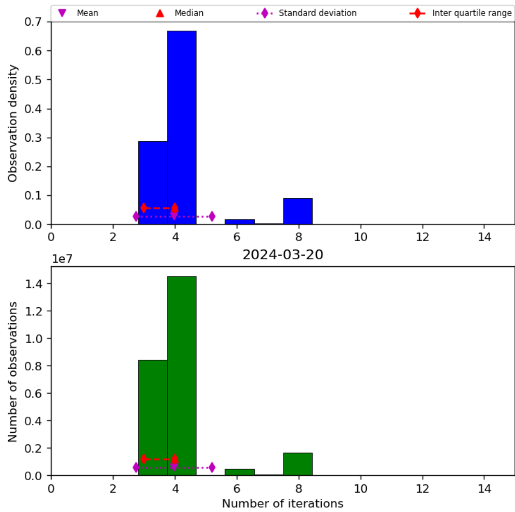
Figure 34: Histogram of “Number of iterations” for 2024-03-20 to 2024-03-21
