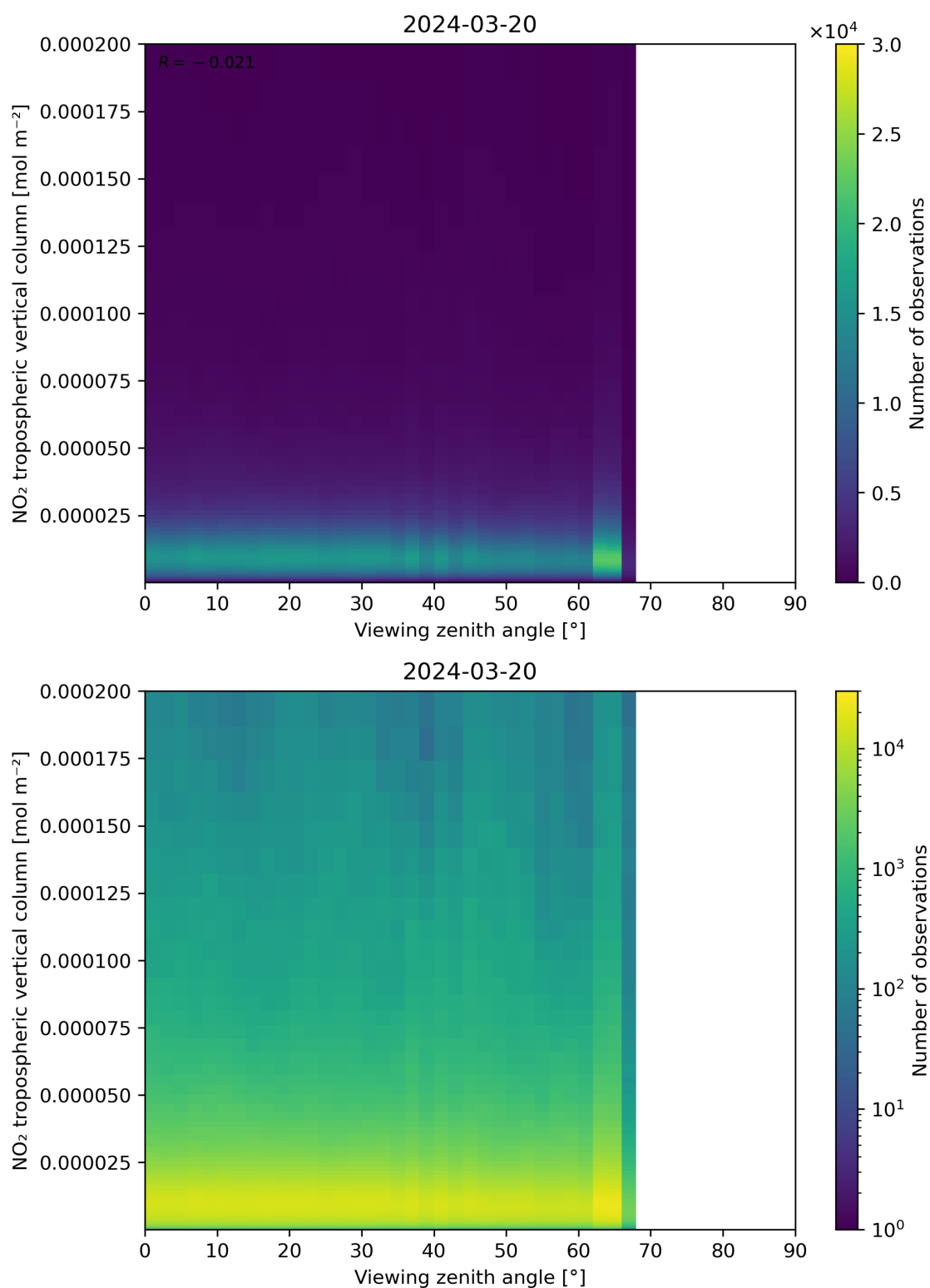
Figure 169: Scatter density plot of “Viewing zenith angle” against “NO 2 tropospheric vertical column” for 2024-03-20 to 2024-03-21.
