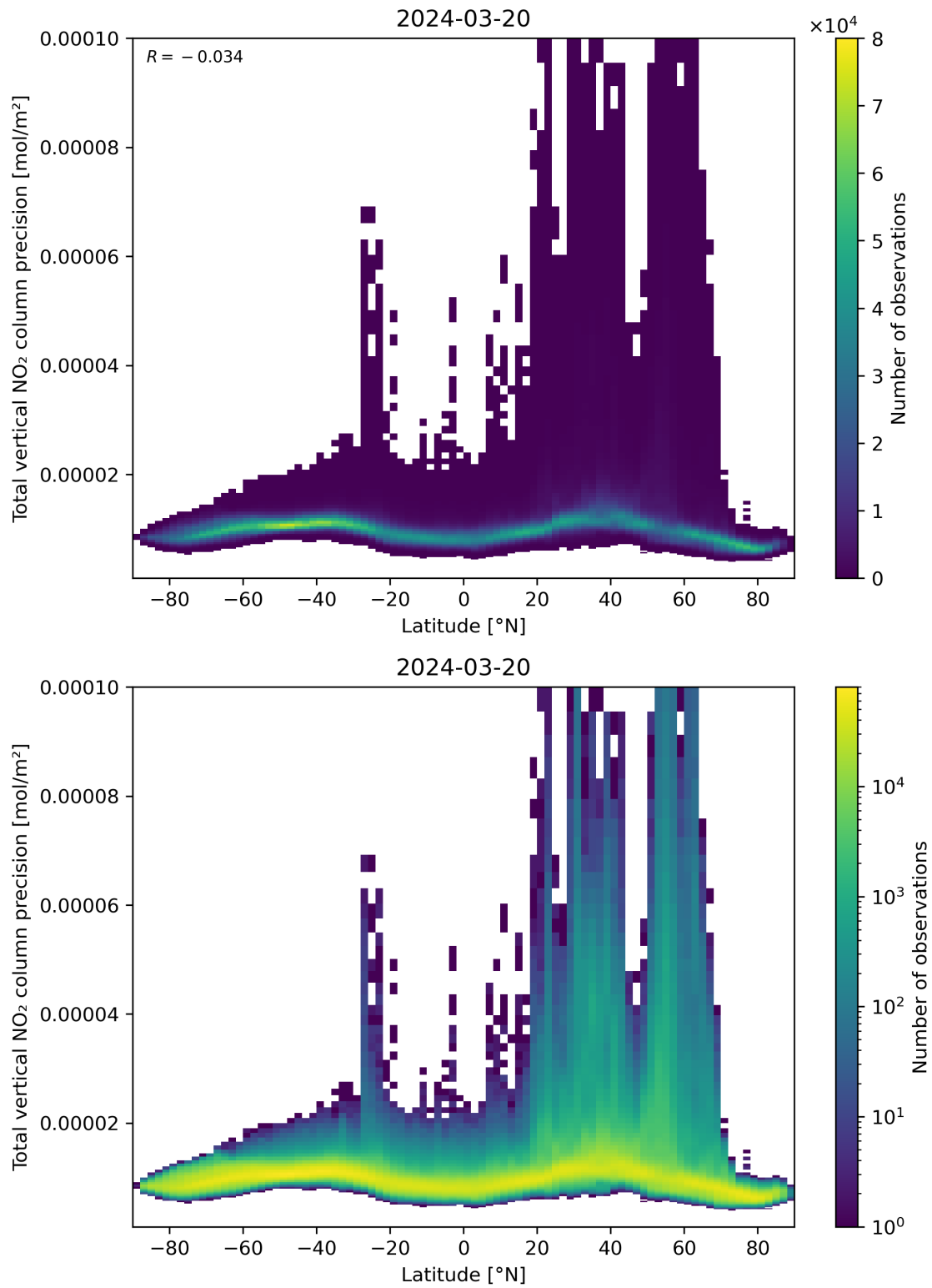
Figure 91: Scatter density plot of “Latitude” against “Total vertical NO 2 column precision” for 2024-03-20 to 2024-03-21.
