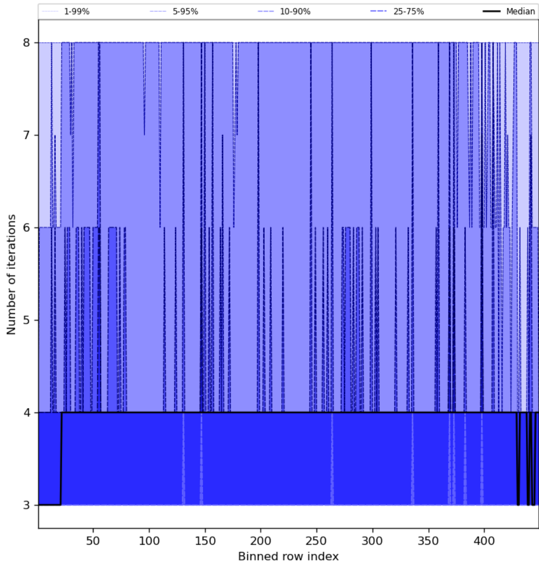
Figure 51: Along track statistics of “Number of iterations” for 2024-03-20 to 2024-03-21
