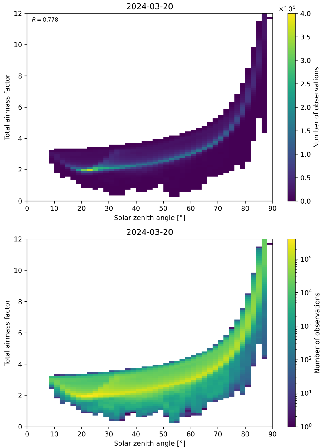
Figure 146: Scatter density plot of “Solar zenith angle” against “Total air mass factor” for 2024-03-20 to 2024-03-21.
