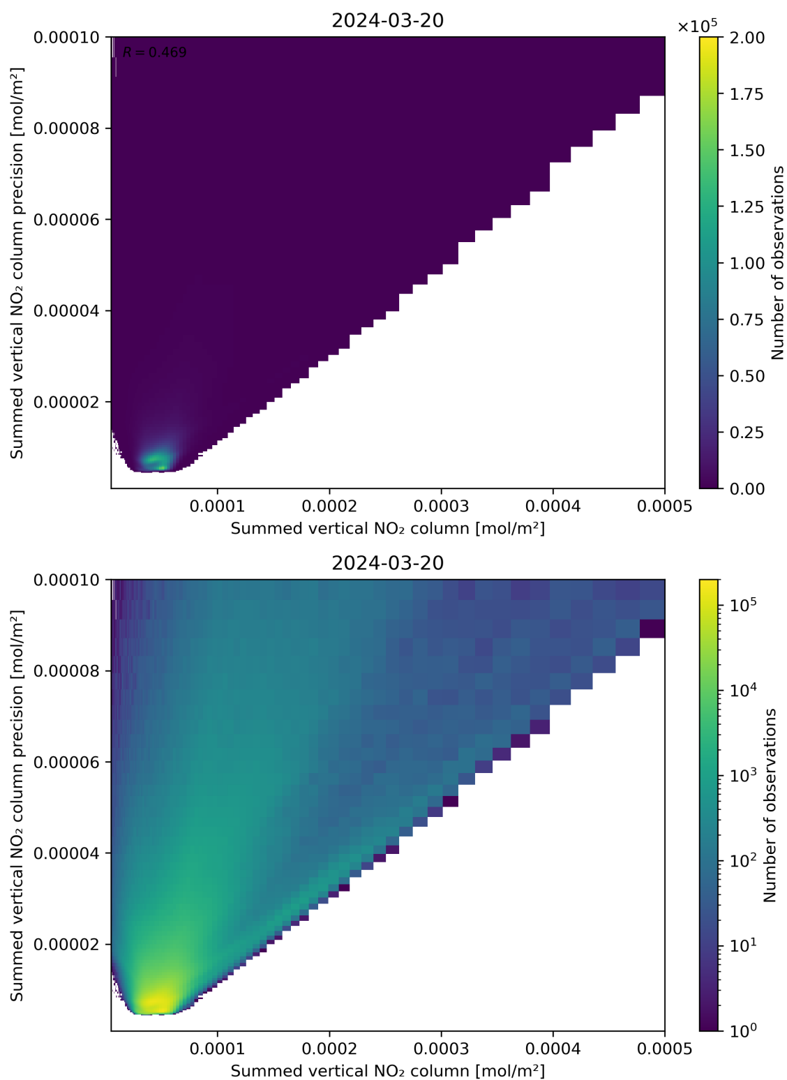
Figure 105: Scatter density plot of “Summed vertical NO 2 column” against “Summed vertical NO 2 column precision” for 2024-03-20 to 2024-03-21.
