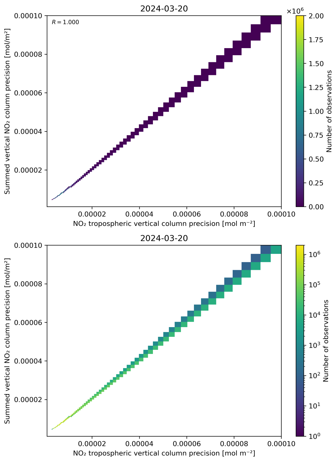
Figure 137: Scatter density plot of “NO 2 tropospheric vertical column precision” against “Summed vertical NO 2 column precision” for 2024-03-20 to 2024-03-21.
