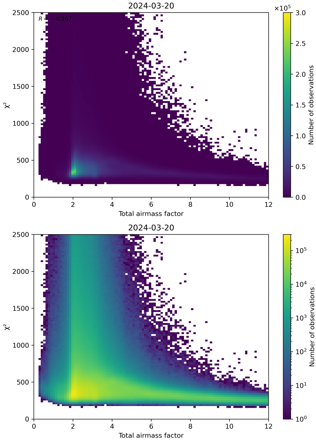
Figure 63: Scatter density plot of “Total airmass factor” against “ \chi^2 ” for 2024-03-20 to 2024-03-21.
