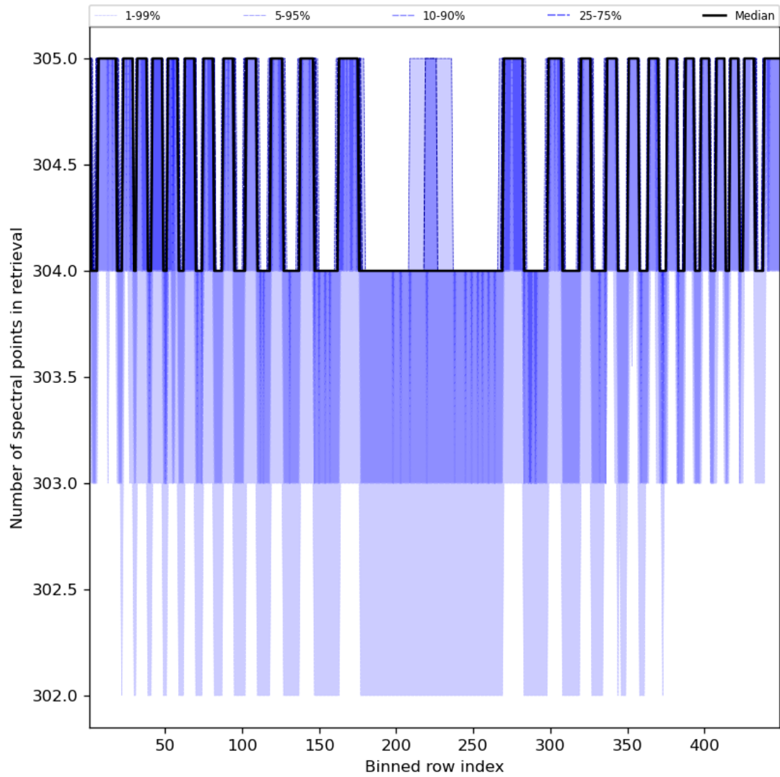
Figure 50: Along track statistics of “Number of spectral points in retrieval” for 2024-03-20 to 2024-03-21
