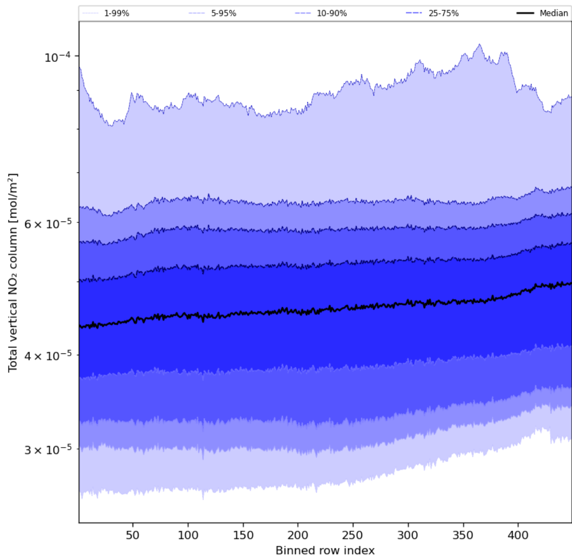
Figure 55: Along track statistics of “Total vertical NO 2 column” for 2024-03-20 to 2024-03-21
