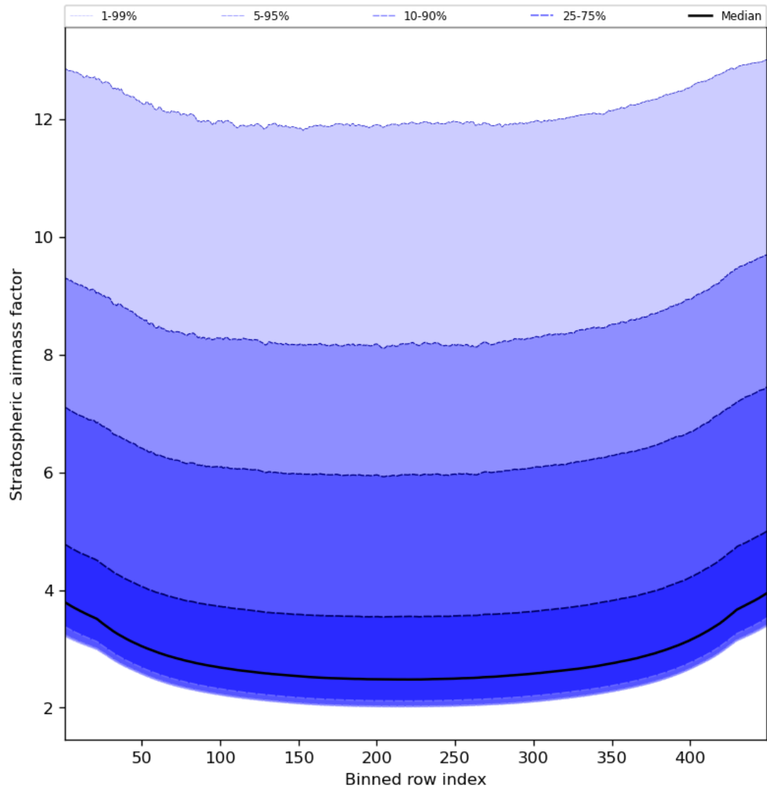
Figure 61: Along track statistics of “Stratospheric airmass factor” for 2024-03-20 to 2024-03-21
