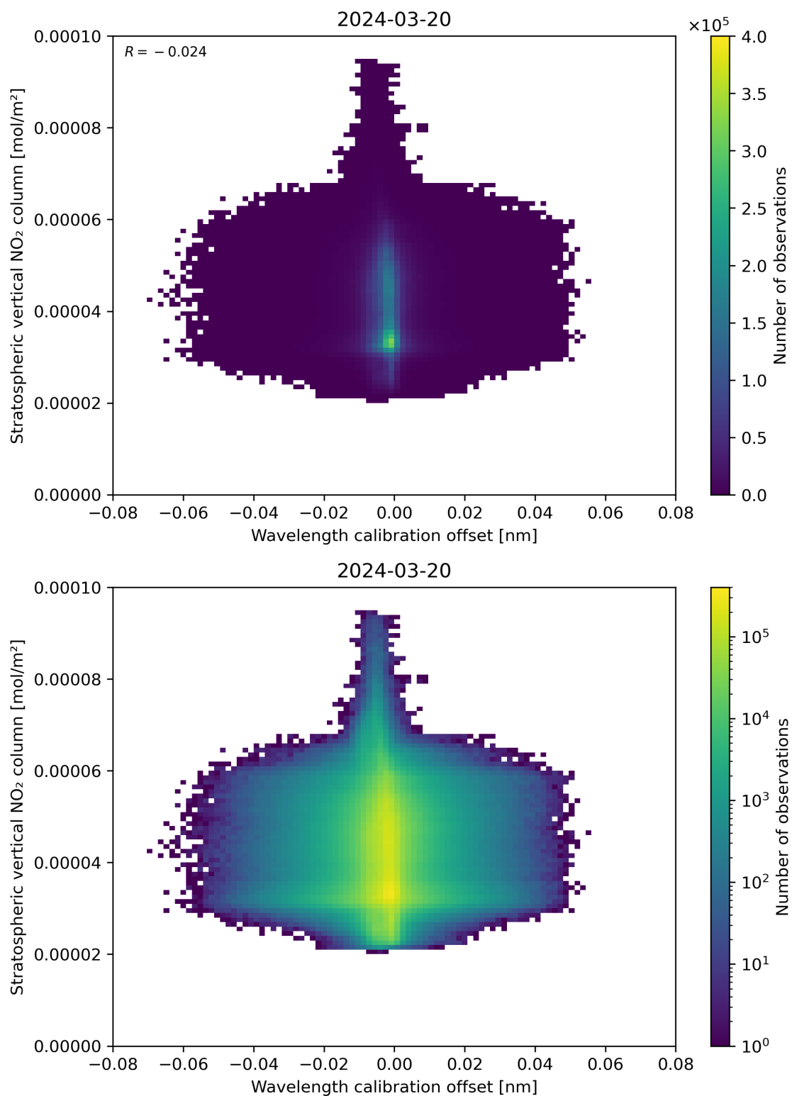
Figure 176: Scatter density plot of “Wavelength calibration offset” against “Stratospheric vertical NO 2 column” for 2024-03-20 to 2024-03-21.
