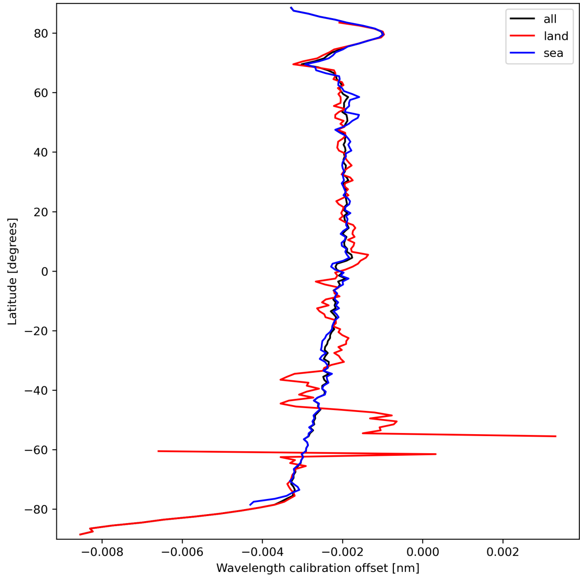
Figure 18: Zonal average of “Wavelength calibration offset” for 2024-03-20 to 2024-03-21.
