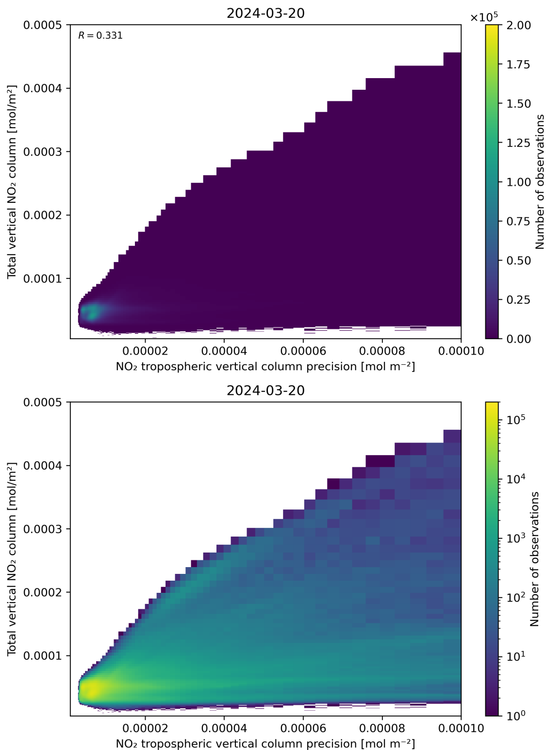
Figure 138: Scatter density plot of “NO 2 tropospheric vertical column precision” against “Total vertical NO 2 column” for 2024-03-20 to 2024-03-21.
