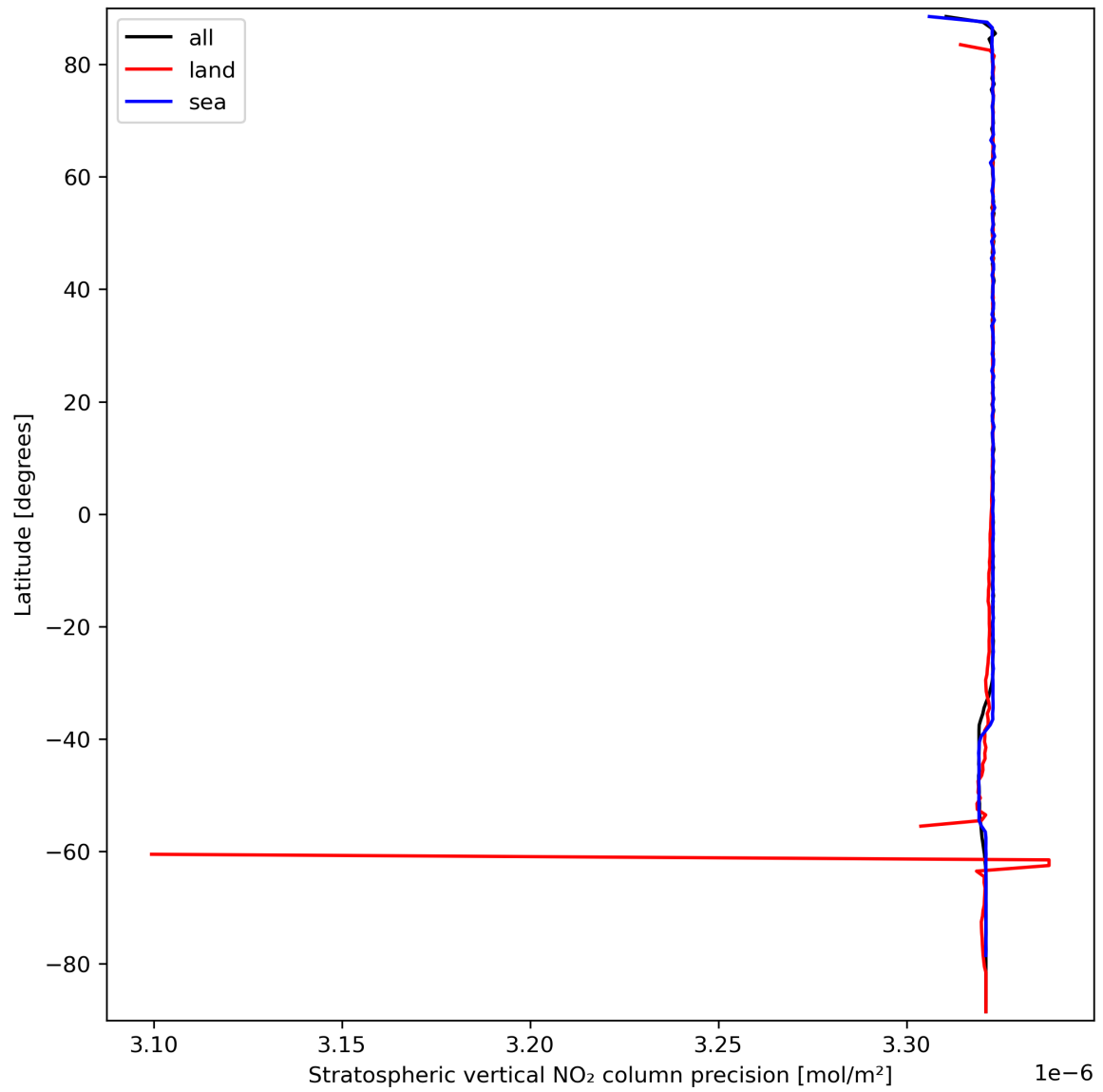
Figure 20: Zonal average of “Stratospheric vertical NO 2 column precision” for 2024-03-20 to 2024-03-21.
