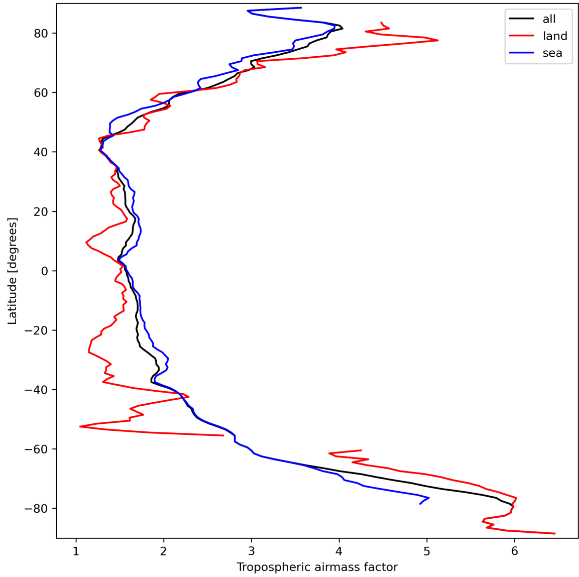
Figure 14: Zonal average of “Tropospheric airmass factor” for 2024-03-20 to 2024-03-21.
