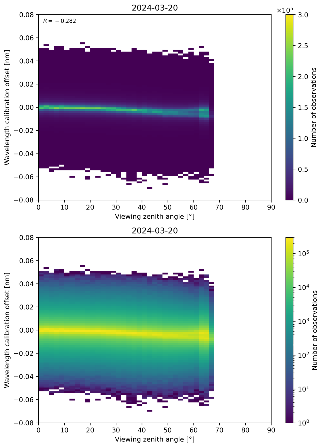
Figure 173: Scatter density plot of “Viewing zenith angle” against “Wavelength calibration offset” for 2024-03-20 to 2024-03-21.
