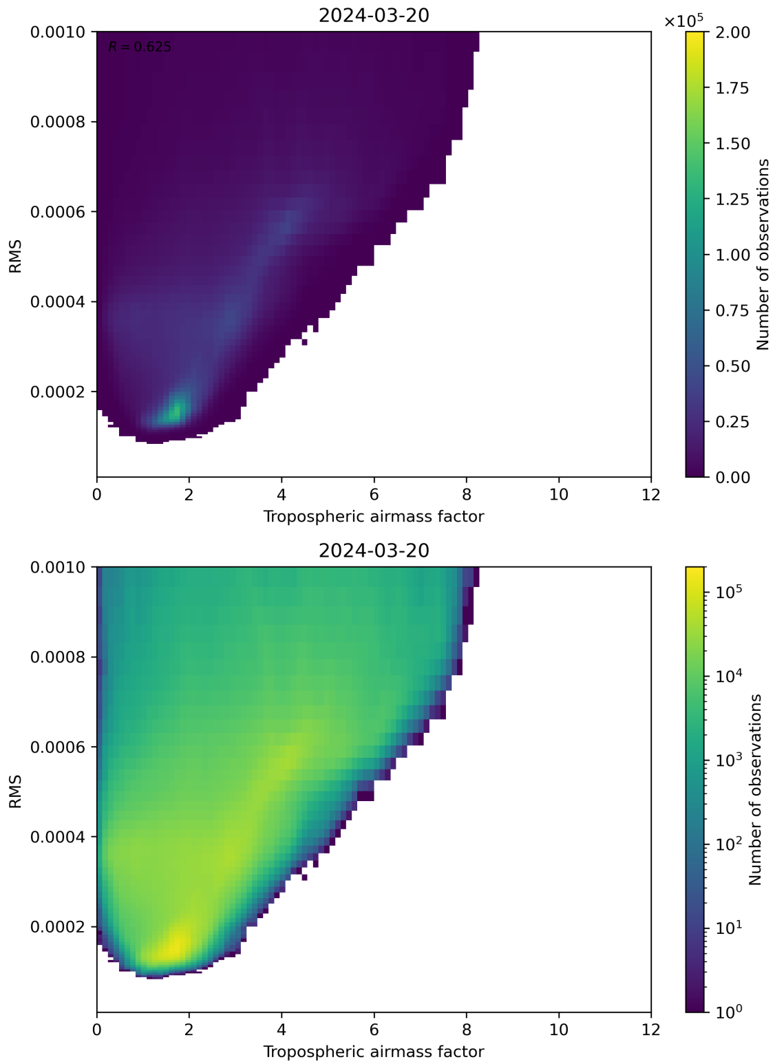
Figure 79: Scatter density plot of “Tropospheric airmass factor” against “RMS” for 2024-03-20 to 2024-03-21.
