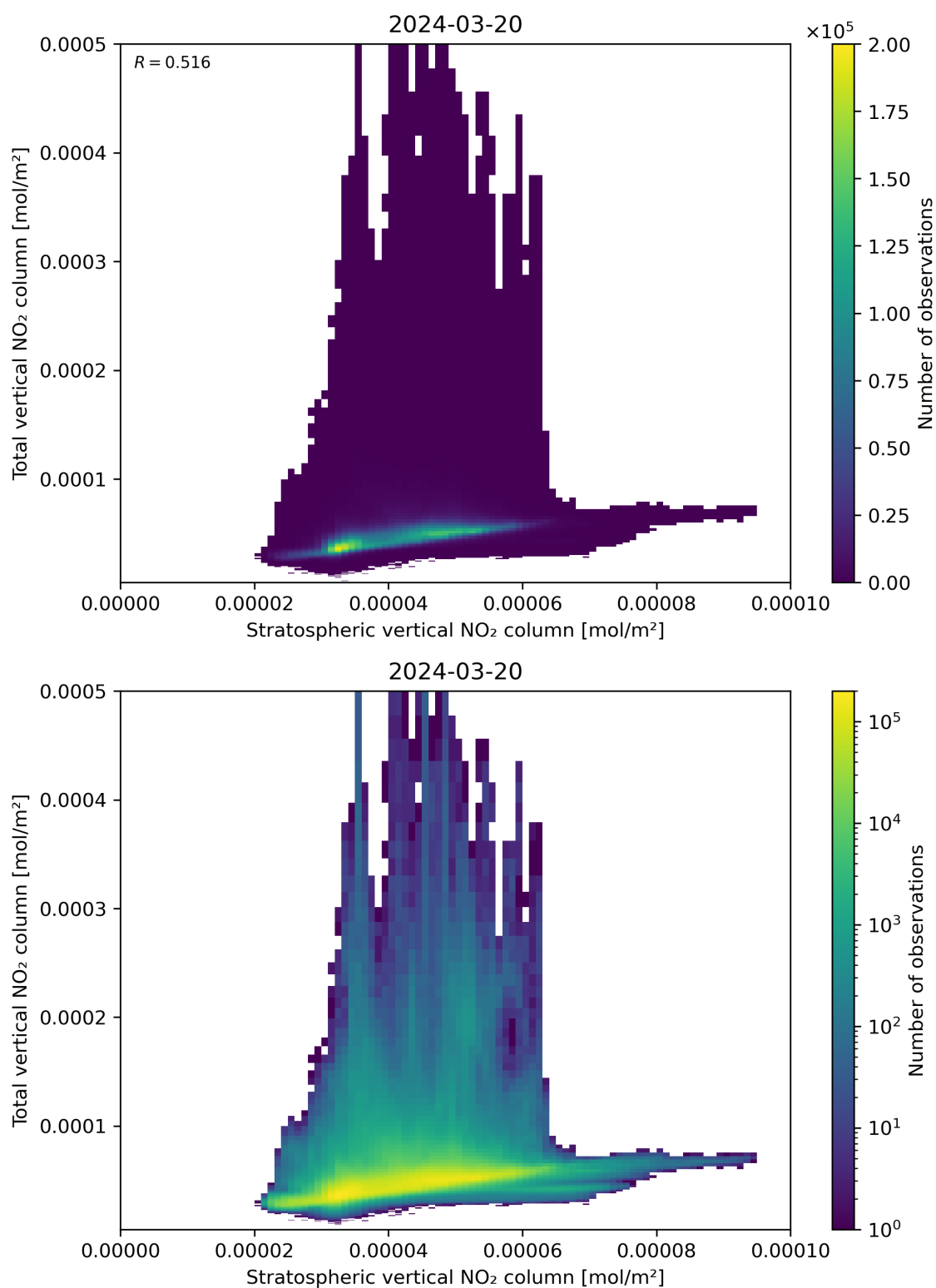
Figure 100: Scatter density plot of “Stratospheric vertical NO 2 column” against “Total vertical NO 2 column” for 2024-03-20 to 2024-03-21.
