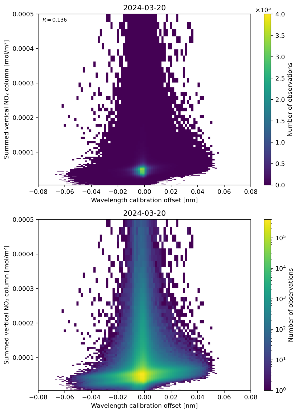
Figure 177: Scatter density plot of “Wavelength calibration offset” against “Summed vertical NO 2 column” for 2024-03-20 to 2024-03-21.
