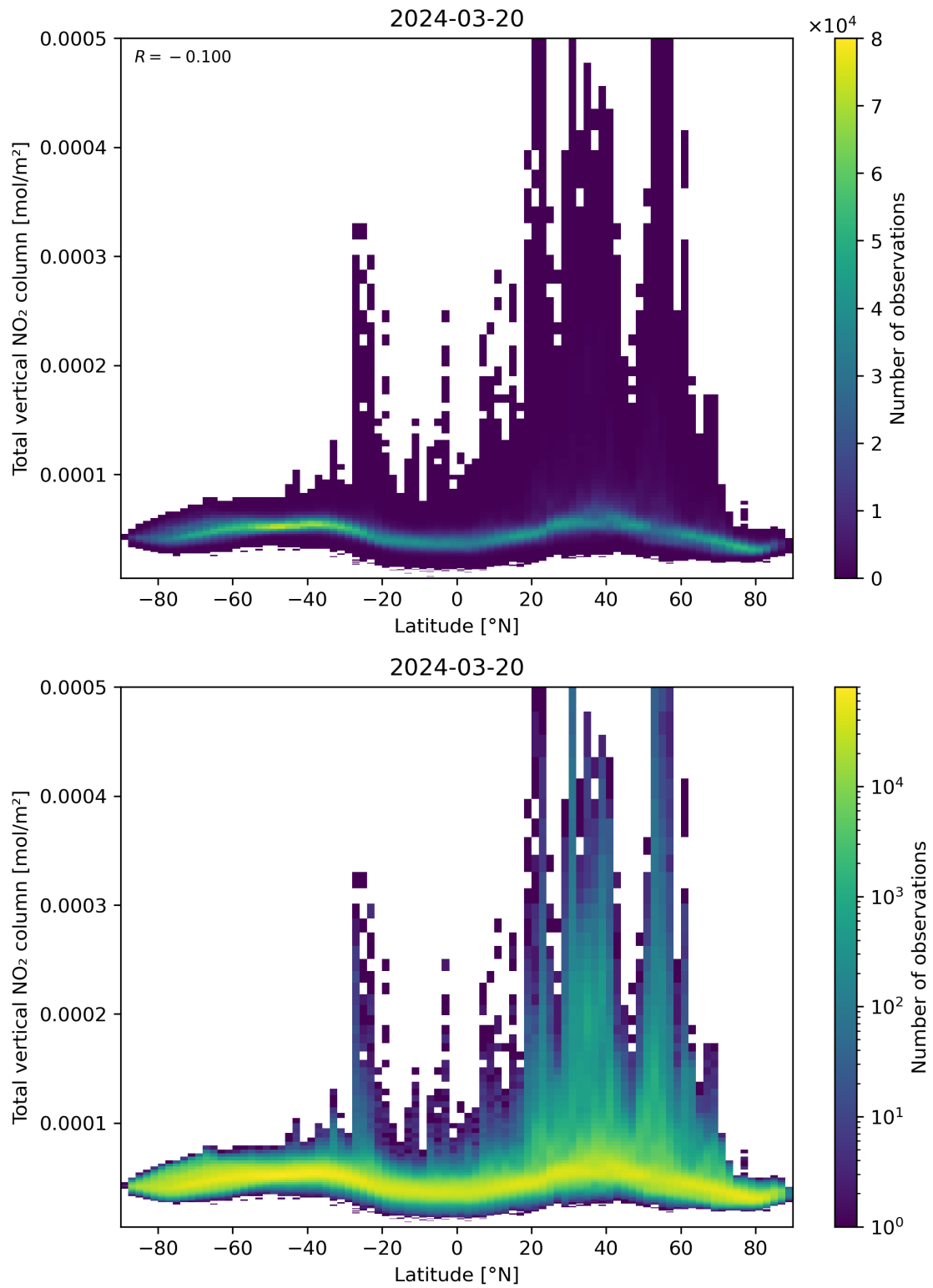
Figure 90: Scatter density plot of “Latitude” against “Total vertical NO 2 column” for 2024-03-20 to 2024-03-21.
