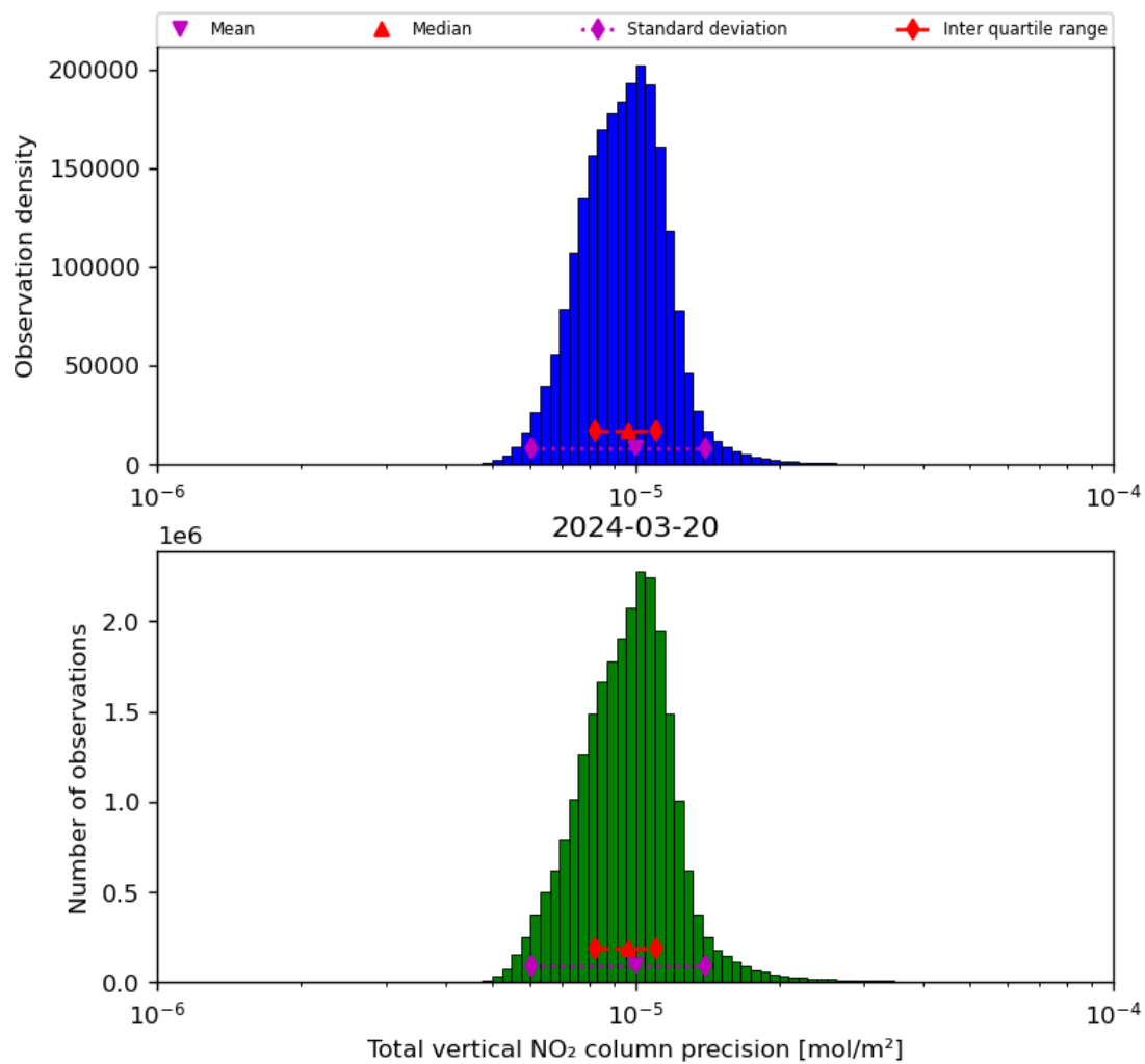
Figure 39: Histogram of “Total vertical NO 2 column precision” for 2024-03-20 to 2024-03-21
