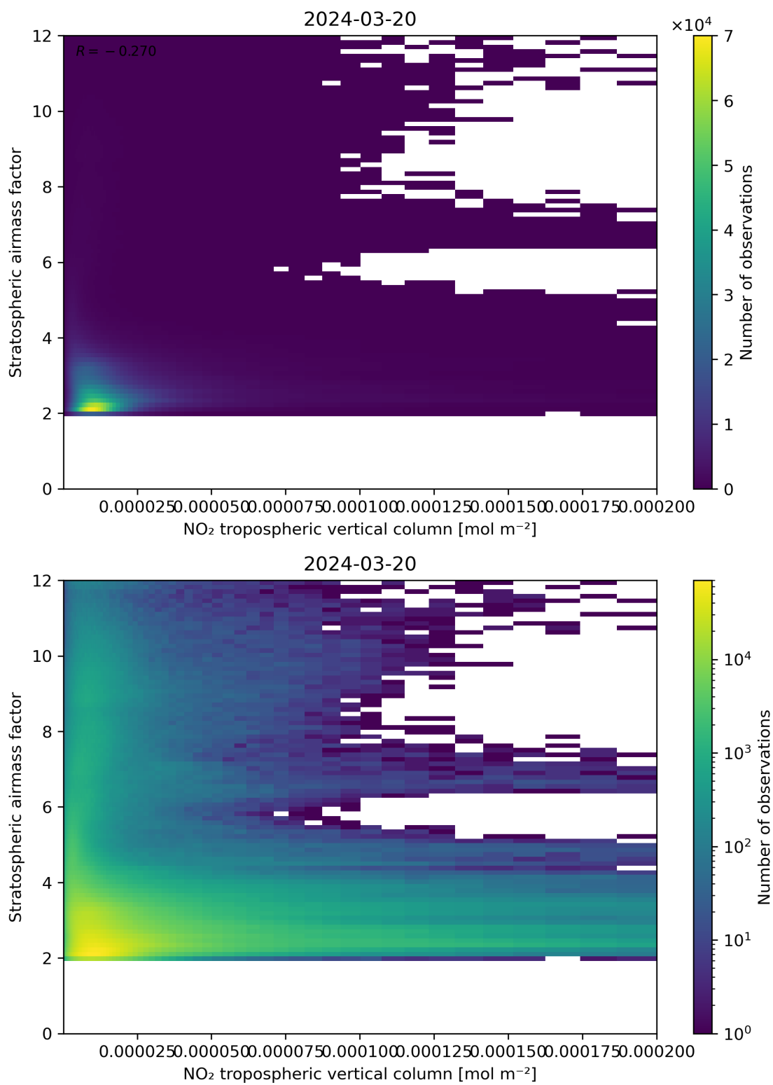
Figure 121: Scatter density plot of “NO 2 tropospheric vertical column” against “Stratospheric air mass factor” for 2024-03-20 to 2024-03-21.
