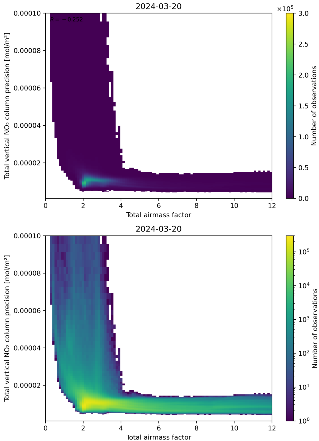
Figure 68: Scatter density plot of “Total airmass factor” against “Total vertical NO 2 column precision” for 2024-03-20 to 2024-03-21.
