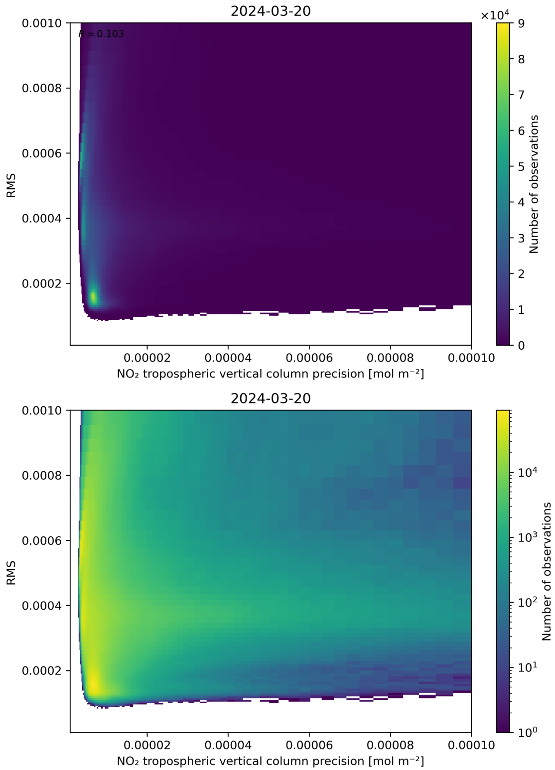
Figure 140: Scatter density plot of “NO 2 tropospheric vertical column precision” against “RMS” for 2024-03-20 to 2024-03-21.
