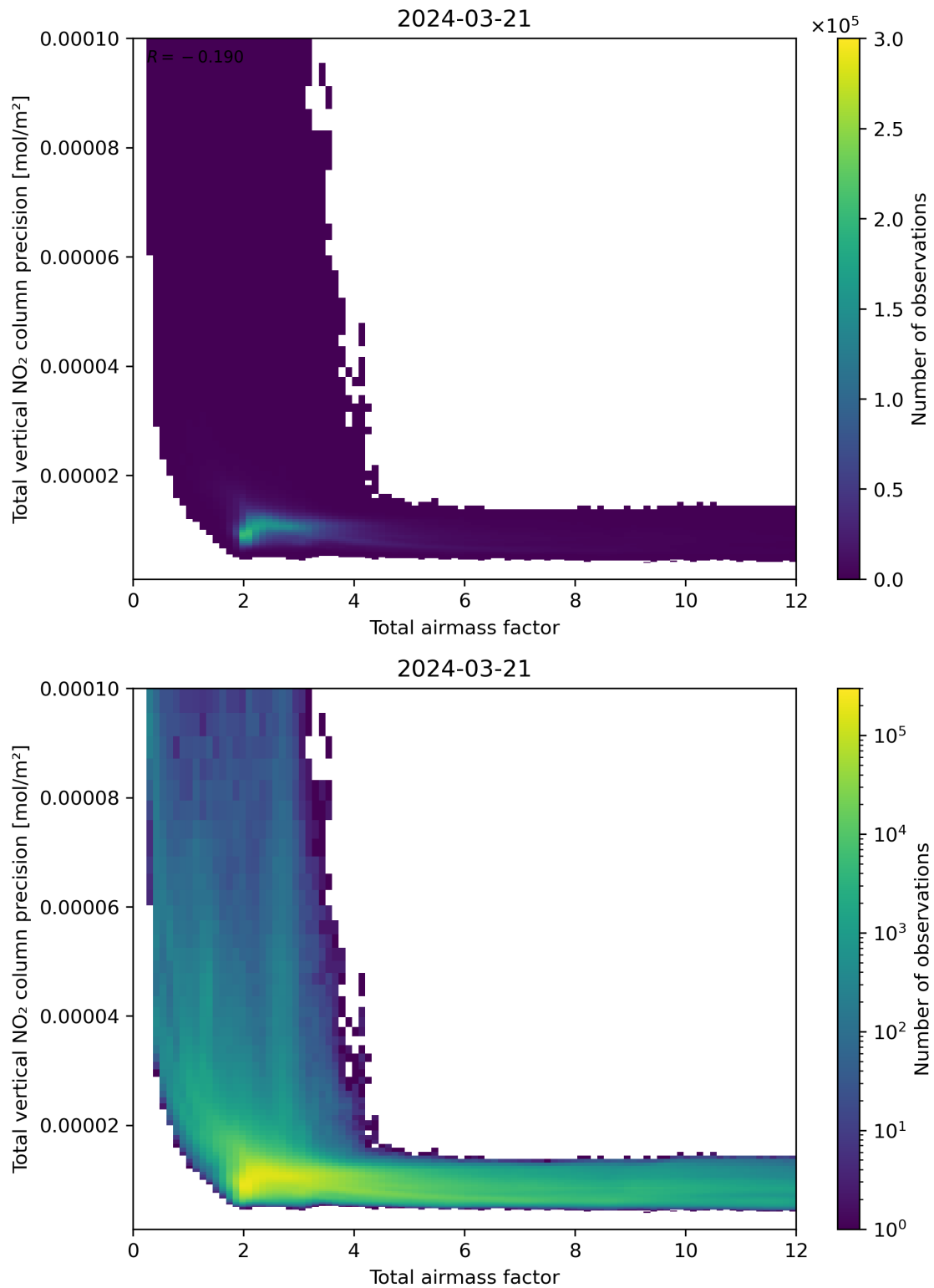
Figure 68: Scatter density plot of “Total airmass factor” against “Total vertical NO 2 column precision” for 2024-03-20 to 2024-03-22.
