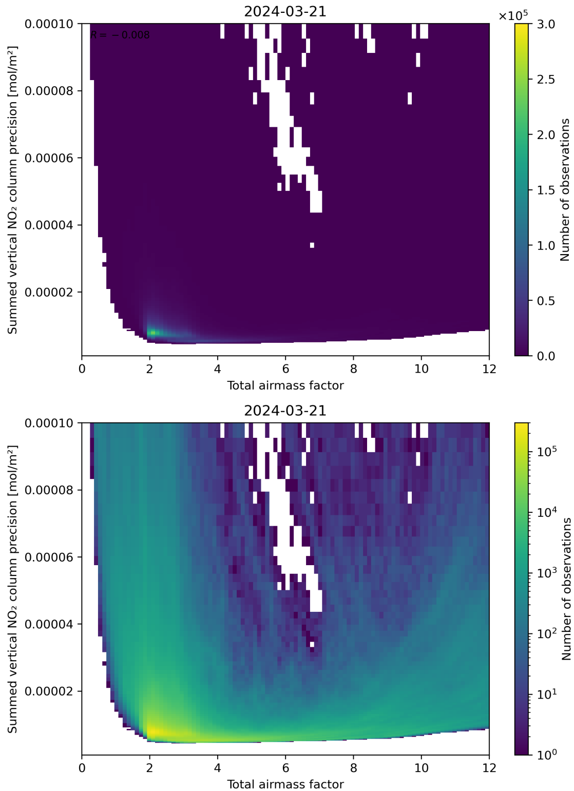
Figure 66: Scatter density plot of “Total airmass factor” against “Summed vertical NO 2 column precision” for 2024-03-20 to 2024-03-22.
