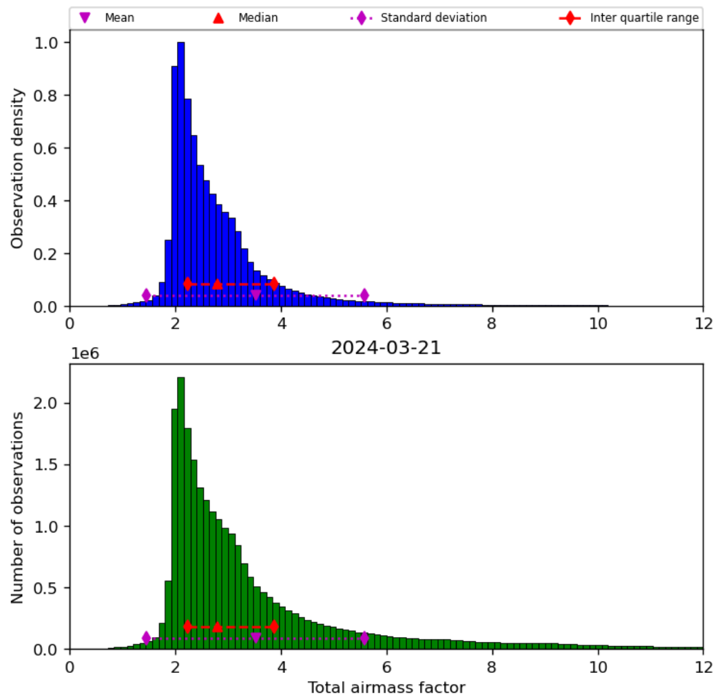
Figure 32: Histogram of “Total airmass factor” for 2024-03-20 to 2024-03-22
