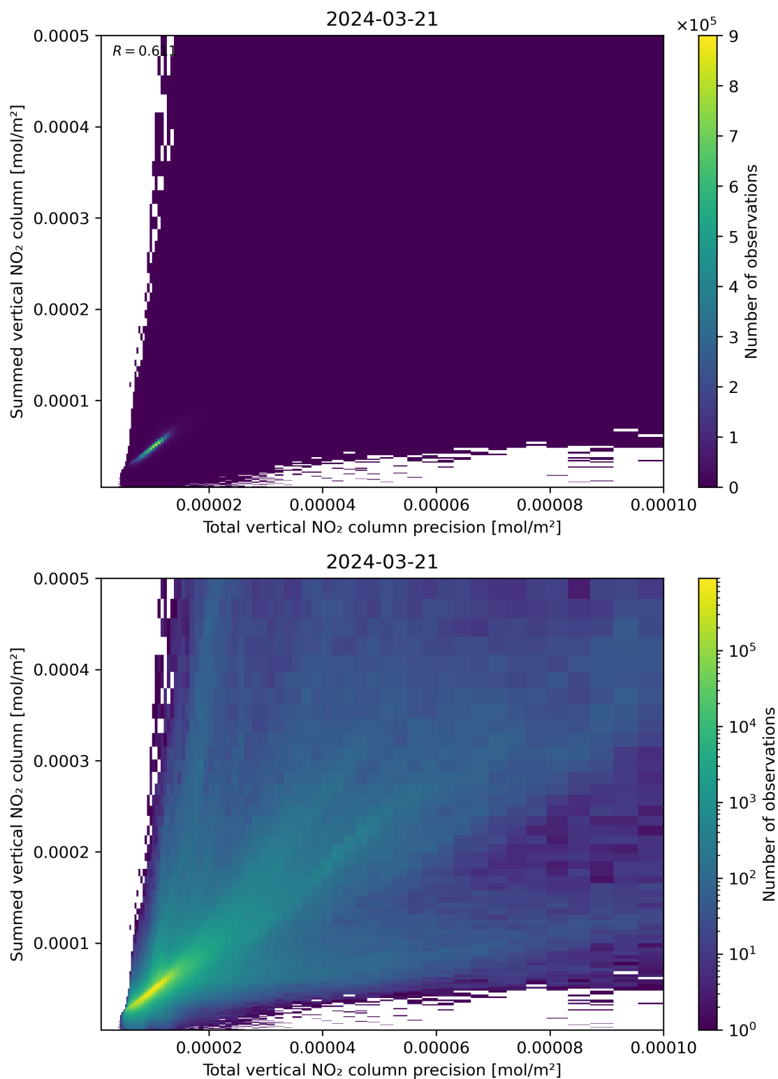
Figure 117: Scatter density plot of “Total vertical NO 2 column precision” against “Summed vertical NO 2 column” for 2024-03-20 to 2024-03-22.
