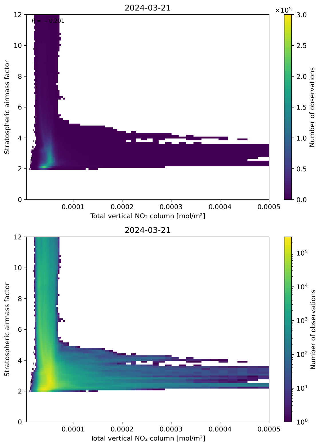
Figure 110: Scatter density plot of “Total vertical NO 2 column” against “Stratospheric airmass factor” for 2024-03-20 to 2024-03-22.
