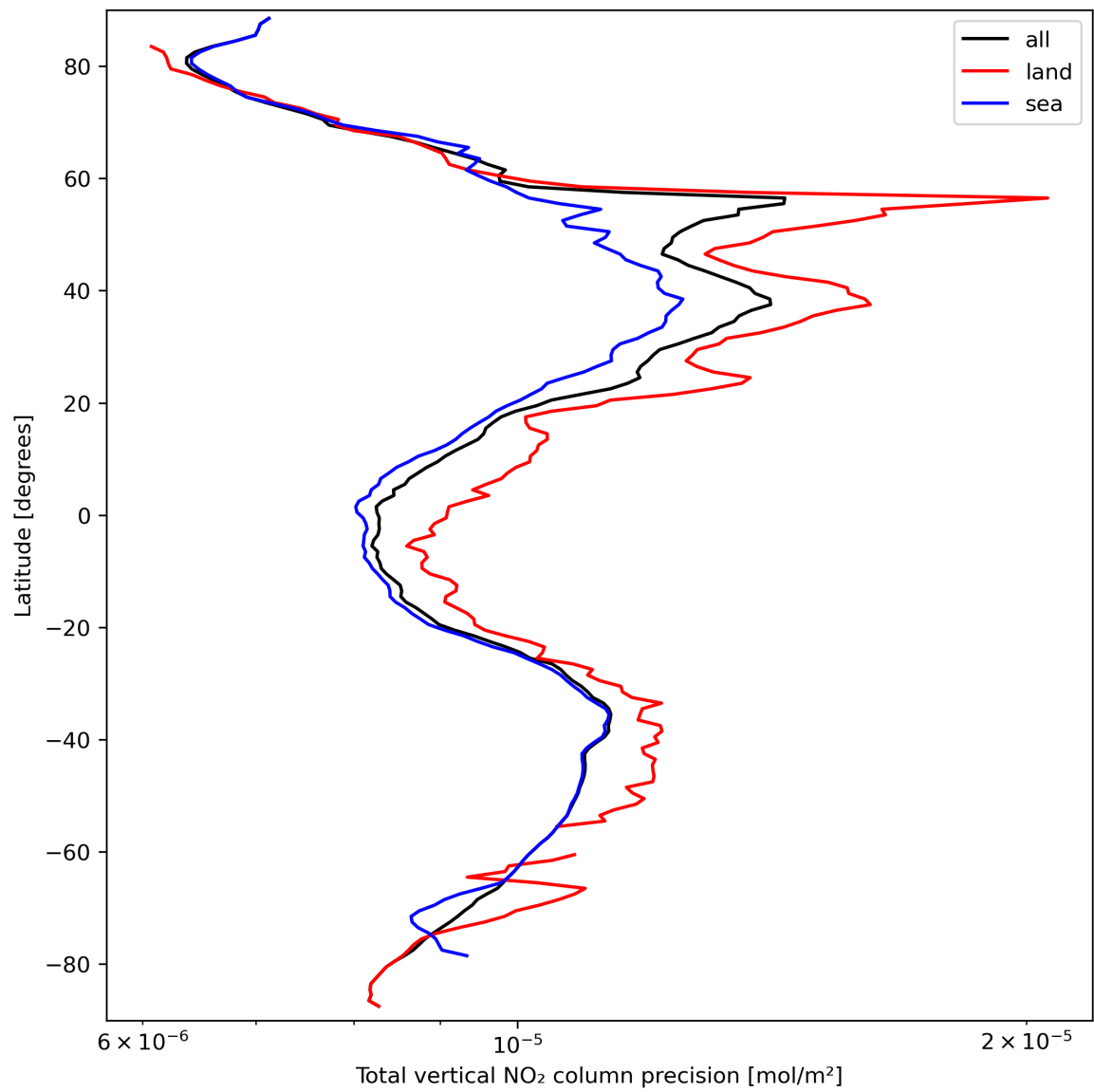
Figure 22: Zonal average of “Total vertical NO 2 column precision” for 2024-03-20 to 2024-03-22.
