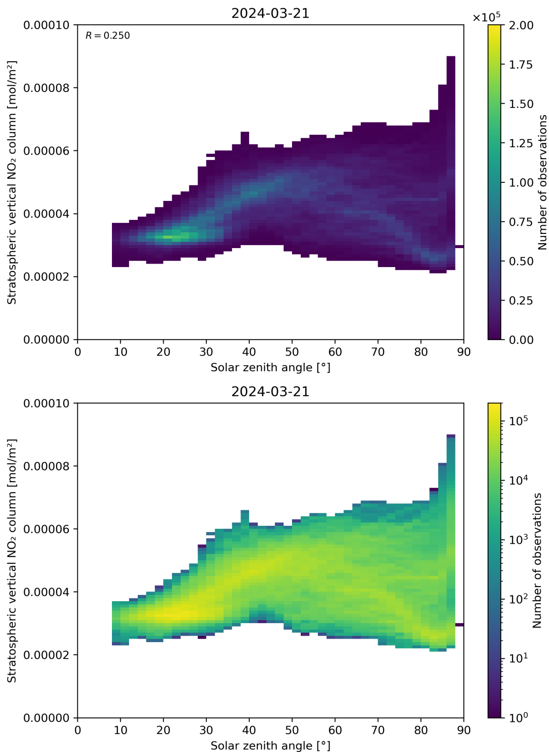
Figure 150: Scatter density plot of “Solar zenith angle” against “Stratospheric vertical \text{NO}_2 column” for 2024-03-20 to 2024-03-22.
