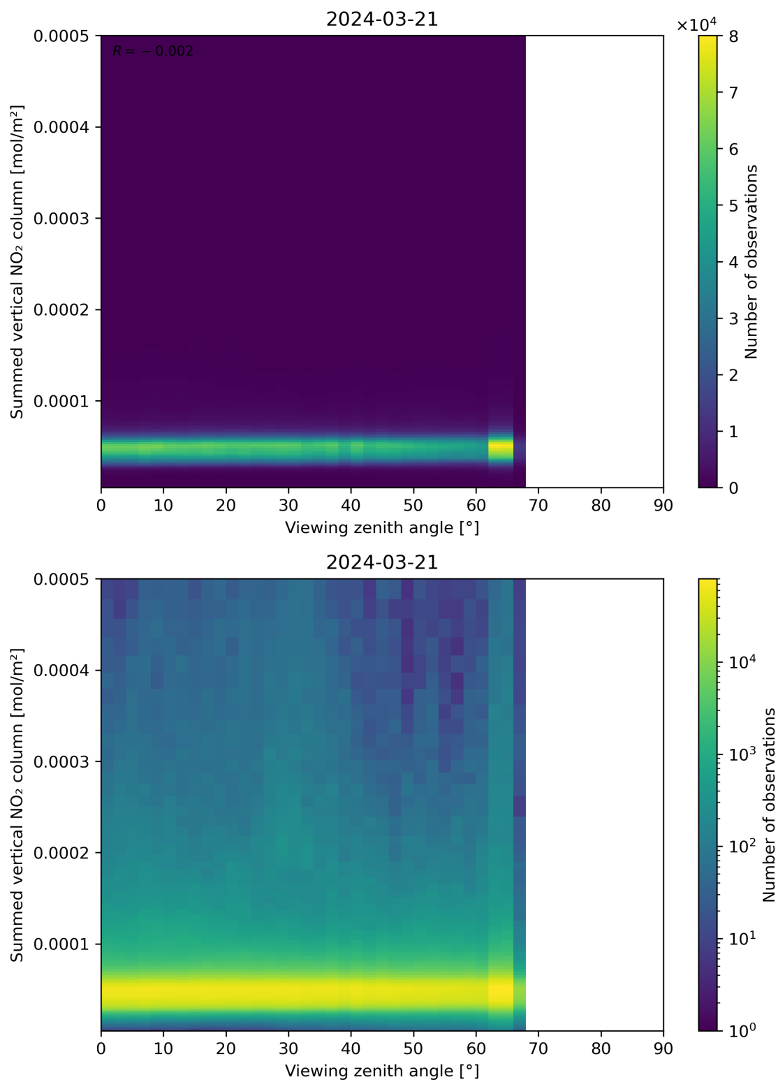
Figure 165: Scatter density plot of “Viewing zenith angle” against “Summed vertical NO 2 column” for 2024-03-20 to 2024-03-22.
