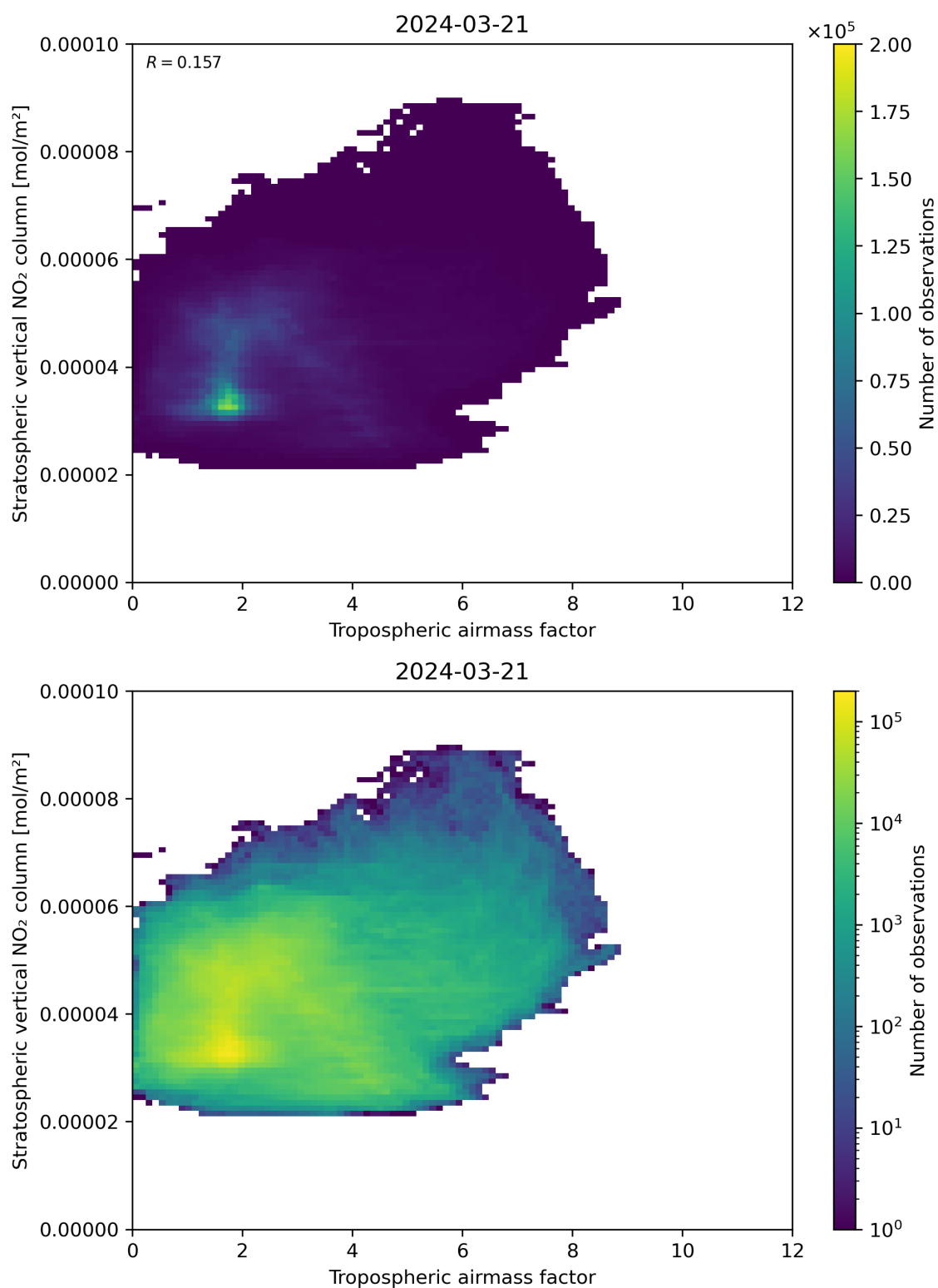
Figure 74: Scatter density plot of “Tropospheric air mass factor” against “Stratospheric vertical NO 2 column” for 2024-03-20 to 2024-03-22.
