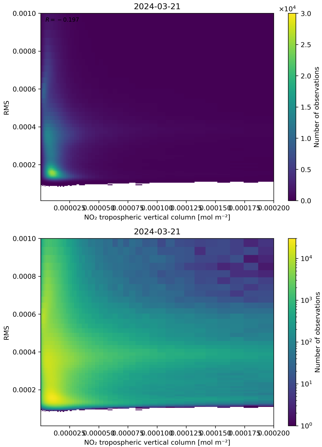
Figure 142: Scatter density plot of “NO 2 tropospheric vertical column” against “RMS” for 2024-03-20 to 2024-03-22.
