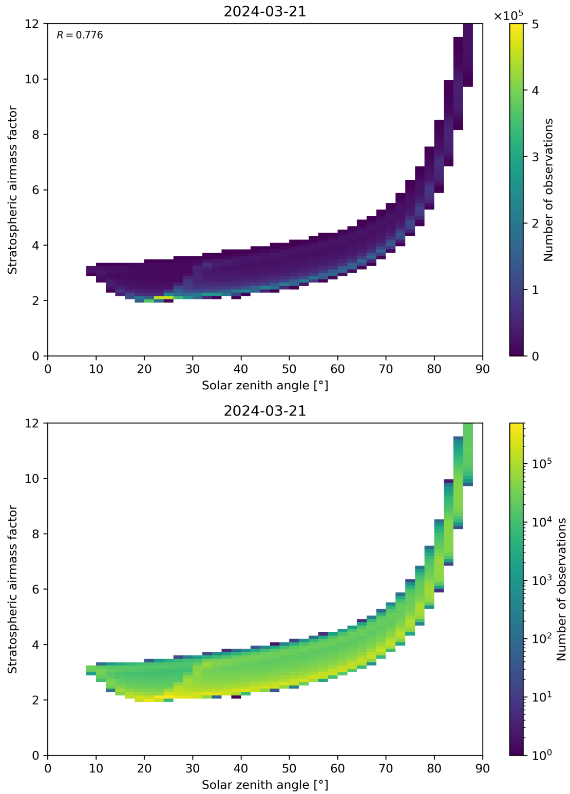
Figure 145: Scatter density plot of “Solar zenith angle” against “Stratospheric airmass factor” for 2024-03-20 to 2024-03-22.
