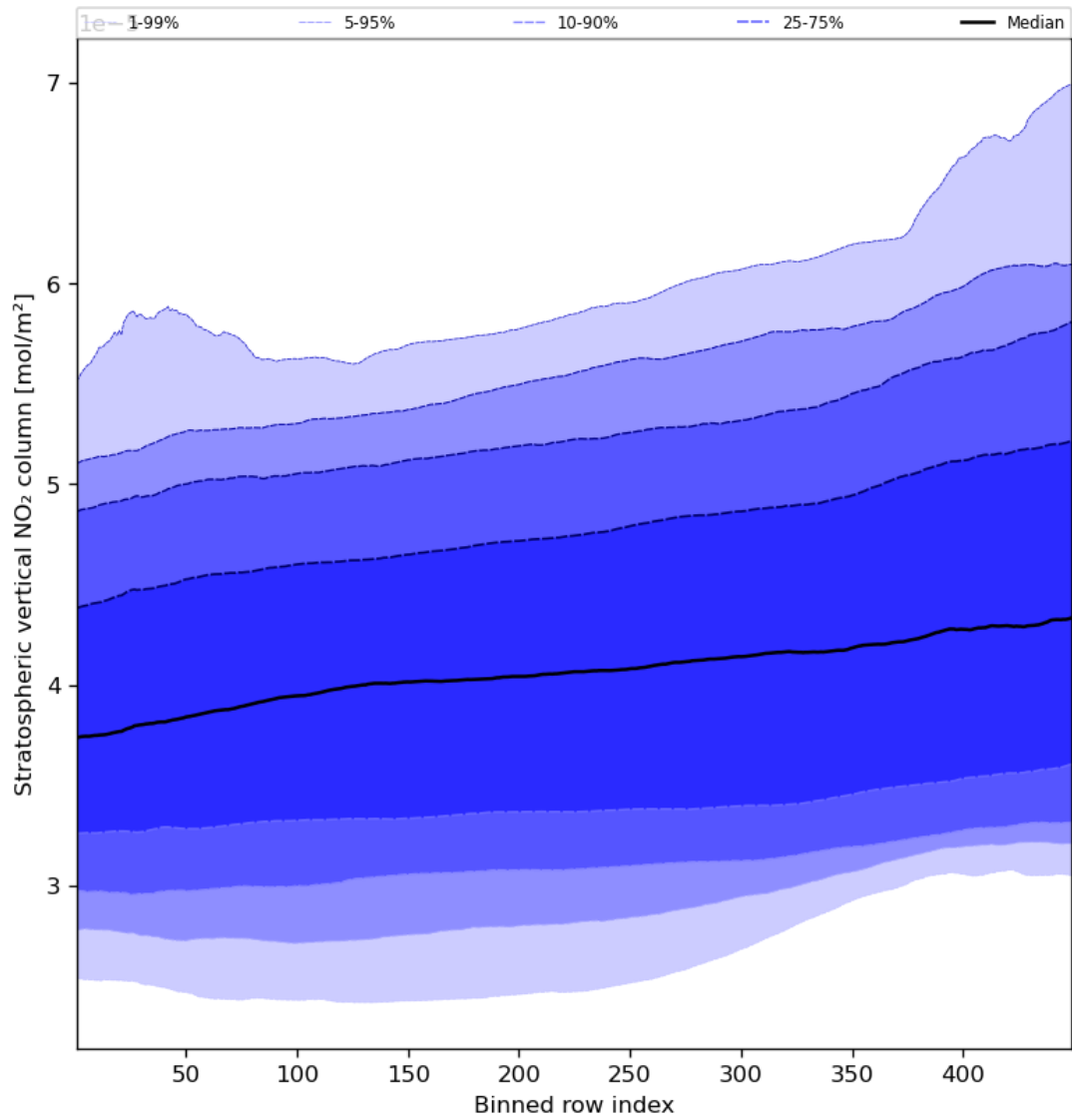
Figure 53: Along track statistics of “Stratospheric vertical NO 2 column” for 2024-03-20 to 2024-03-22
