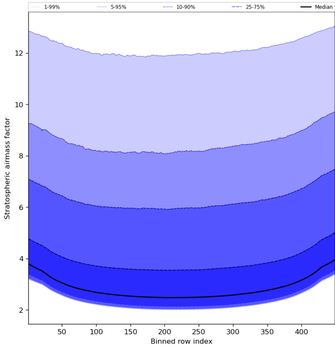
Figure 61: Along track statistics of “Stratospheric air mass factor” for 2024-03-20 to 2024-03-22
