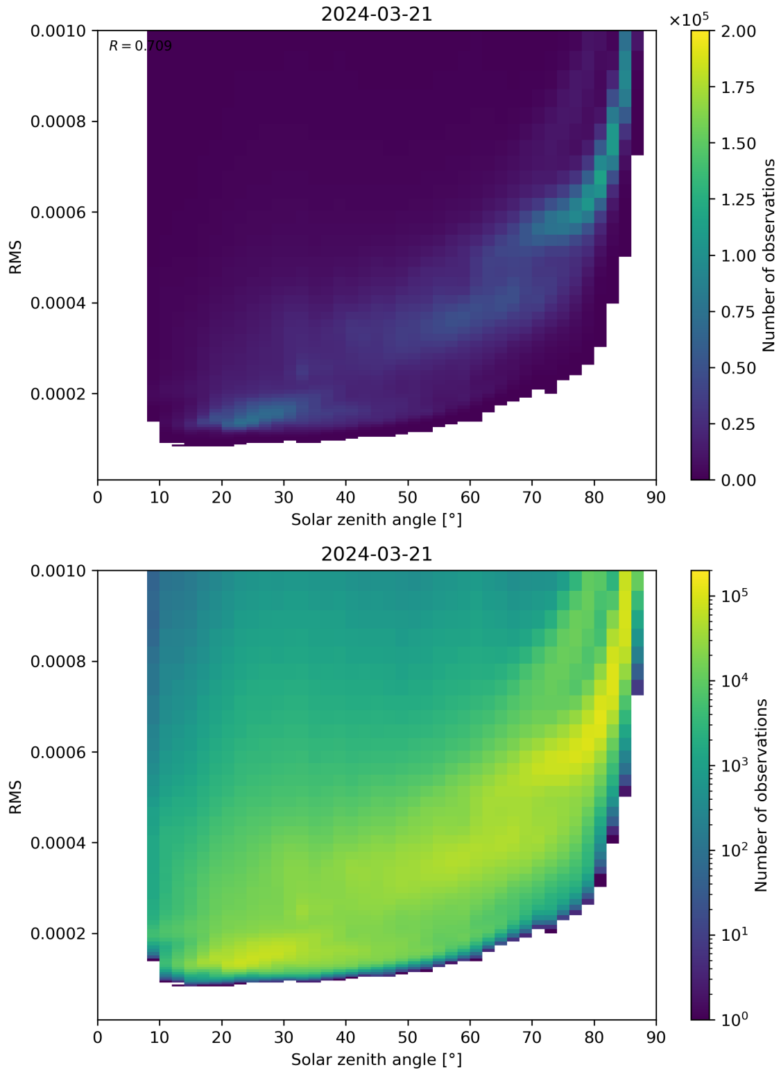
Figure 157: Scatter density plot of “Solar zenith angle” against “RMS” for 2024-03-20 to 2024-03-22.
