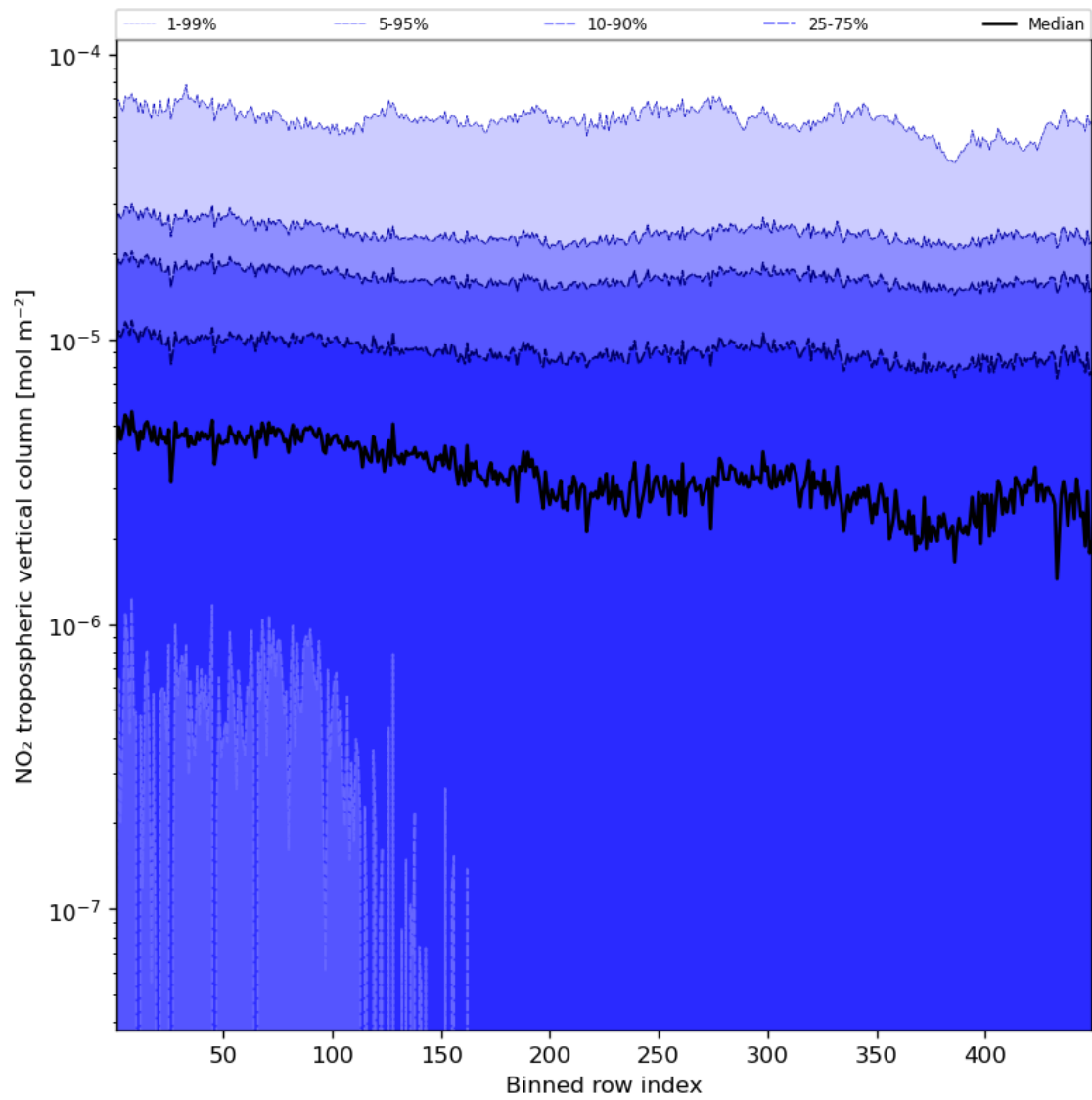
Figure 46: Along track statistics of “NO 2 tropospheric vertical column” for 2024-03-20 to 2024-03-22
