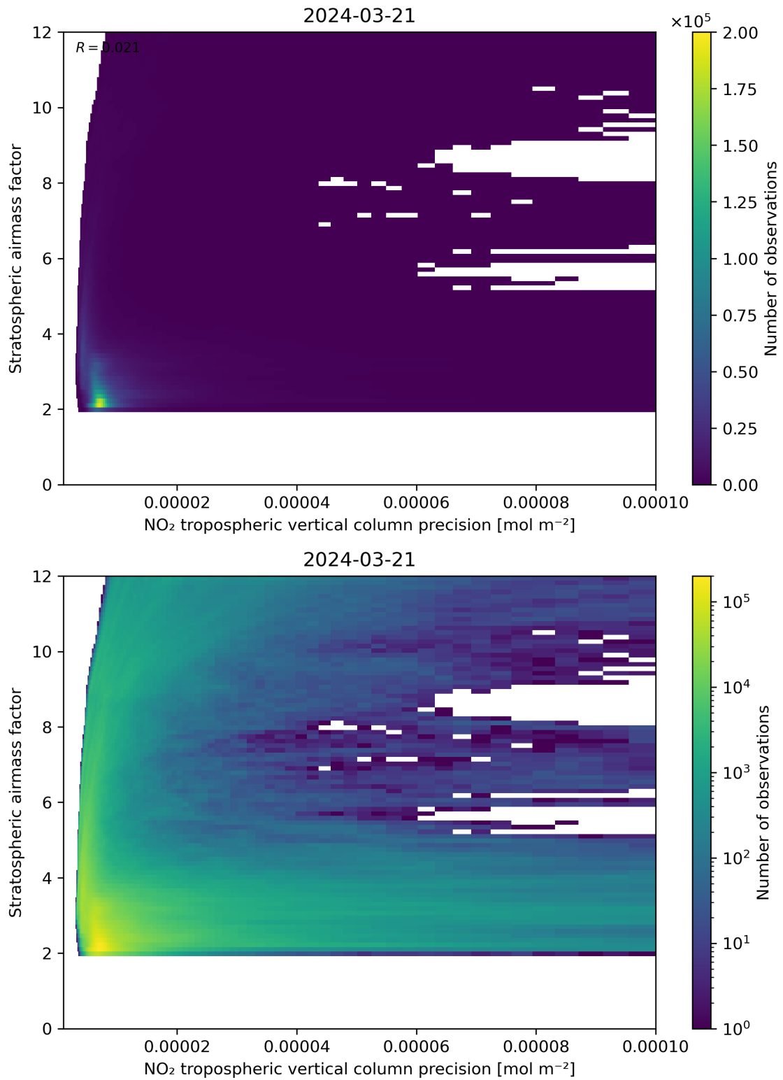
Figure 131: Scatter density plot of “NO 2 tropospheric vertical column precision” against “Stratospheric airmass factor” for 2024-03-20 to 2024-03-22.
