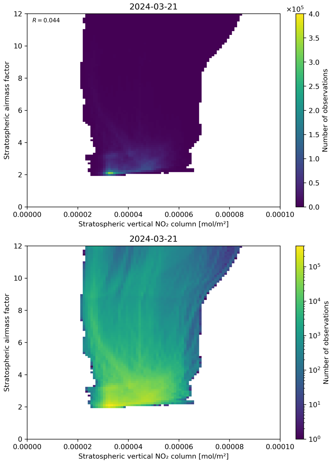
Figure 96: Scatter density plot of “Stratospheric vertical NO 2 column” against “Stratospheric airmass factor” for 2024-03-20 to 2024-03-22.
