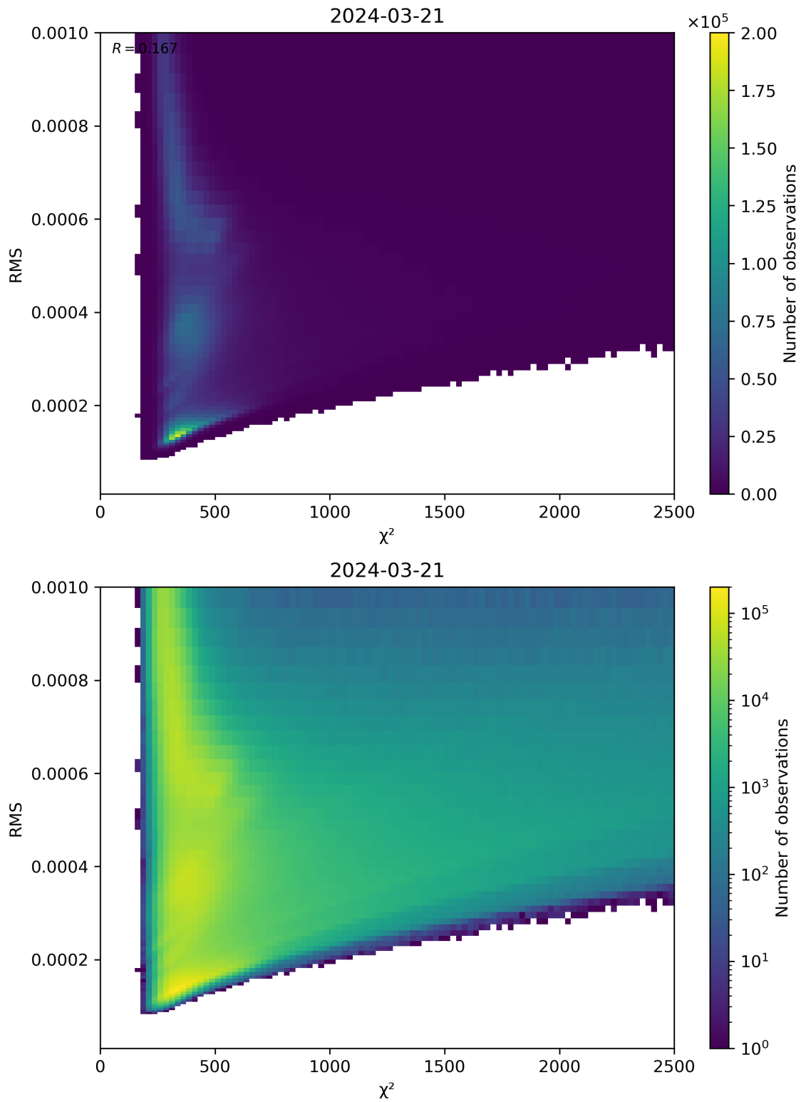
Figure 82: Scatter density plot of “ \chi^2 ” against “RMS” for 2024-03-20 to 2024-03-22.
