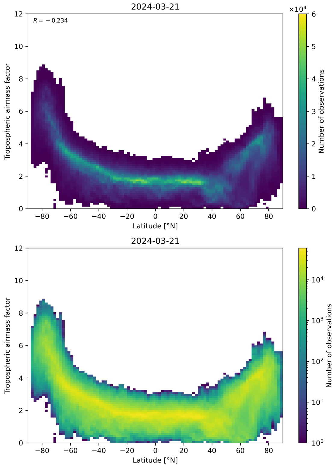
Figure 85: Scatter density plot of “Latitude” against “Tropospheric airmass factor” for 2024-03-20 to 2024-03-22.
