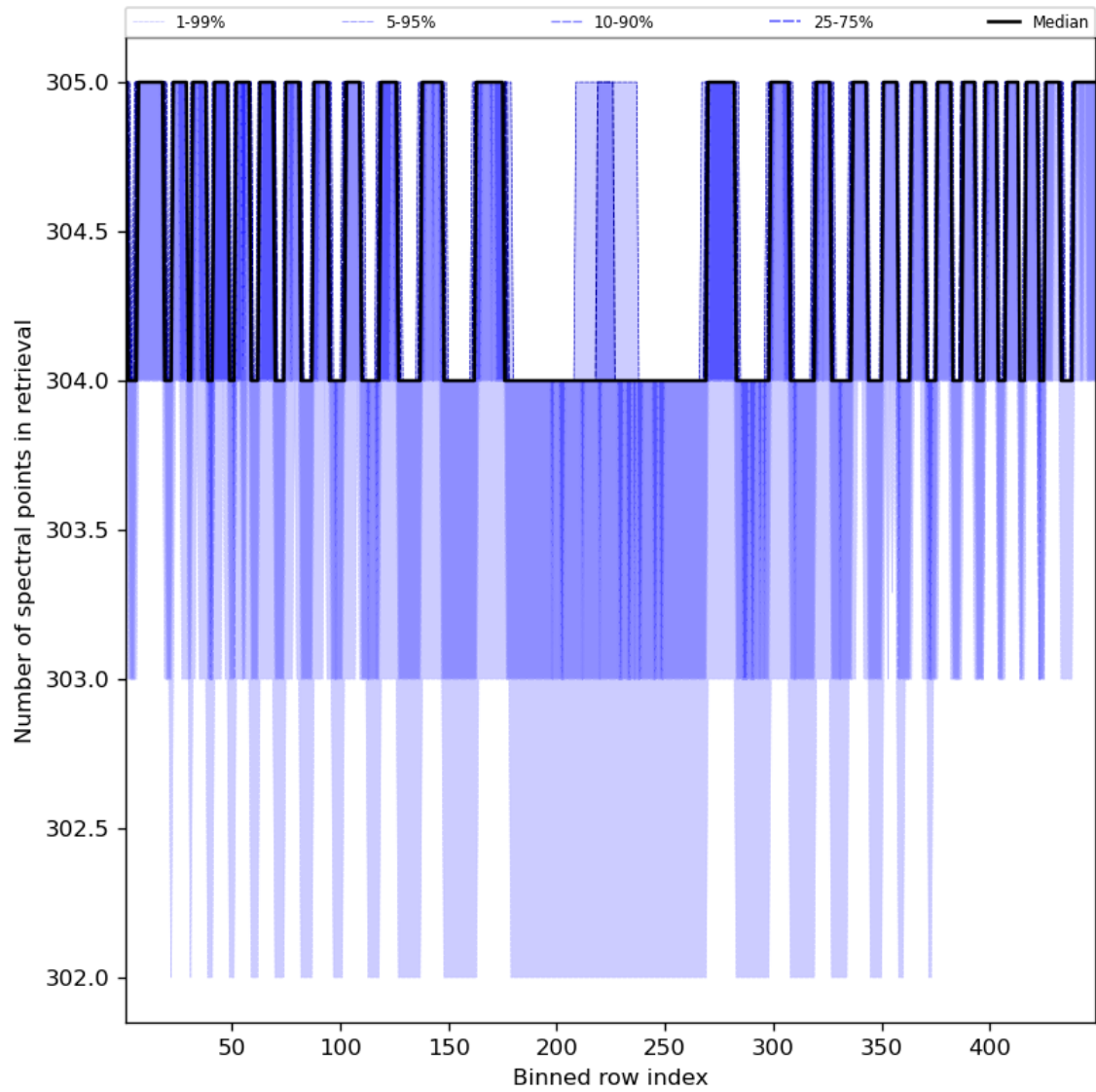
Figure 50: Along track statistics of “Number of spectral points in retrieval” for 2024-03-20 to 2024-03-22
