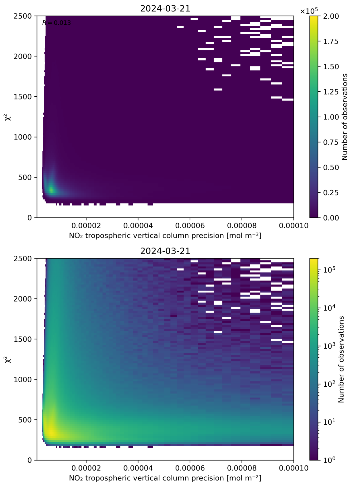
Figure 134: Scatter density plot of “NO 2 tropospheric vertical column precision” against “ \chi^2 ” for 2024-03-20 to 2024-03-22.
