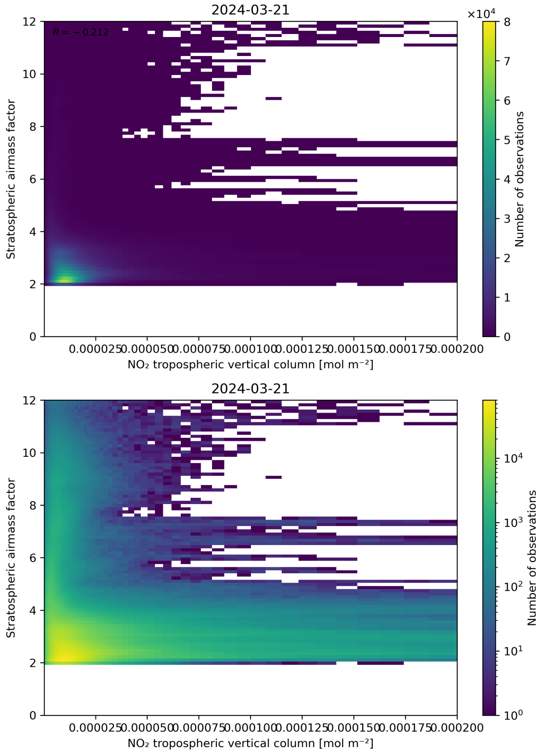
Figure 121: Scatter density plot of “NO 2 tropospheric vertical column” against “Stratospheric air mass factor” for 2024-03-20 to 2024-03-22.
