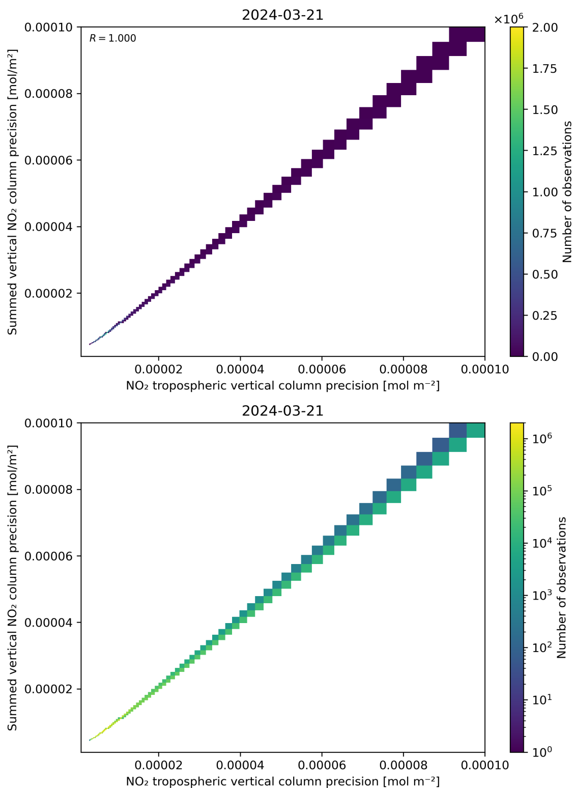
Figure 137: Scatter density plot of “NO 2 tropospheric vertical column precision” against “Summed vertical NO 2 column precision” for 2024-03-20 to 2024-03-22.
