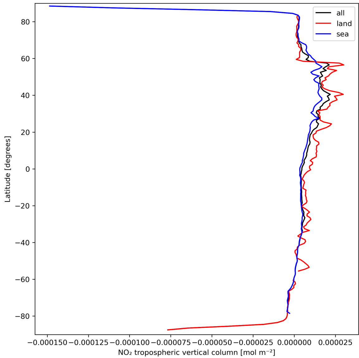
Figure 12: Zonal average of “NO 2 tropospheric vertical column” for 2024-03-20 to 2024-03-22.
