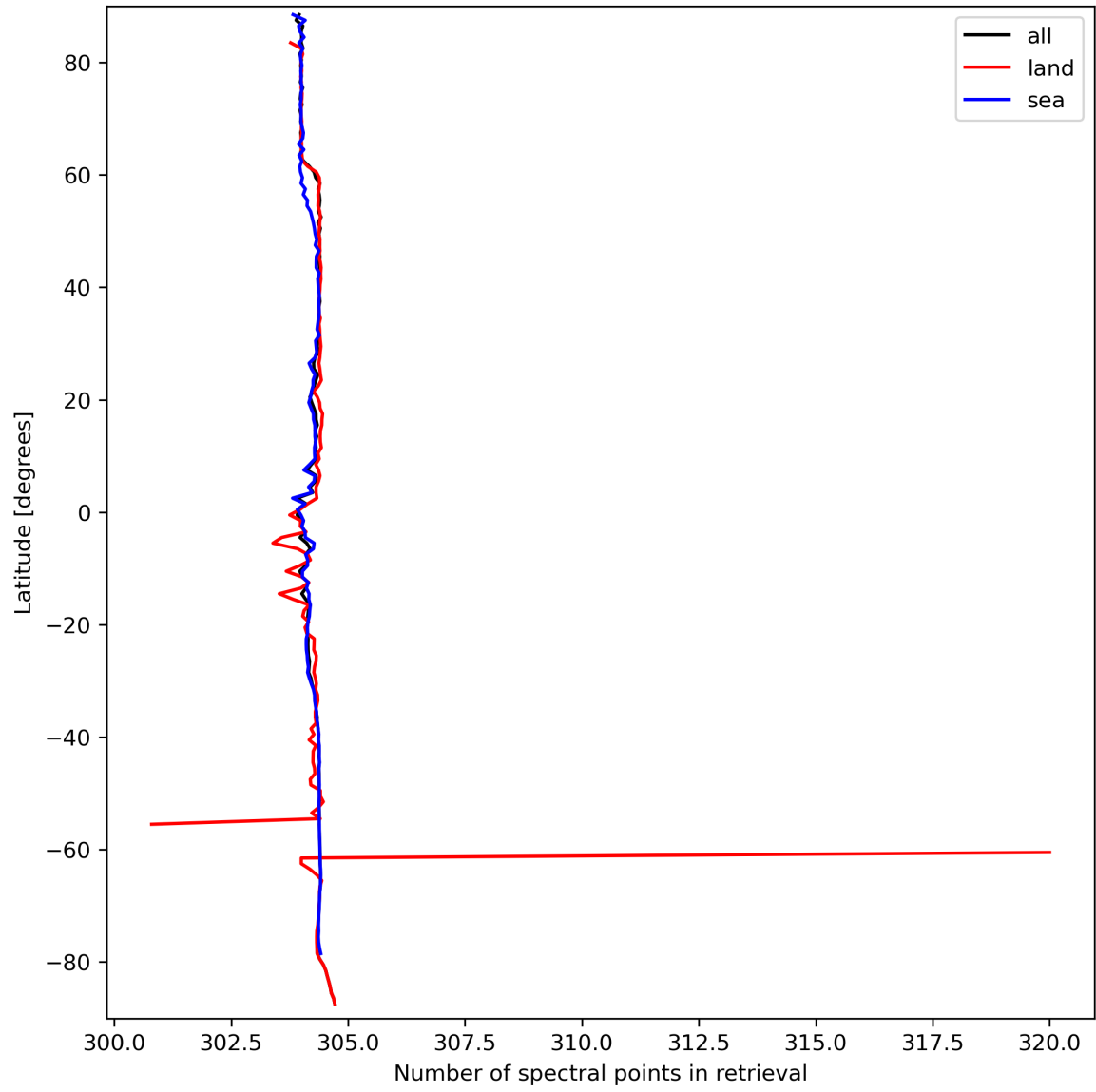
Figure 16: Zonal average of “Number of spectral points in retrieval” for 2024-03-20 to 2024-03-22.
