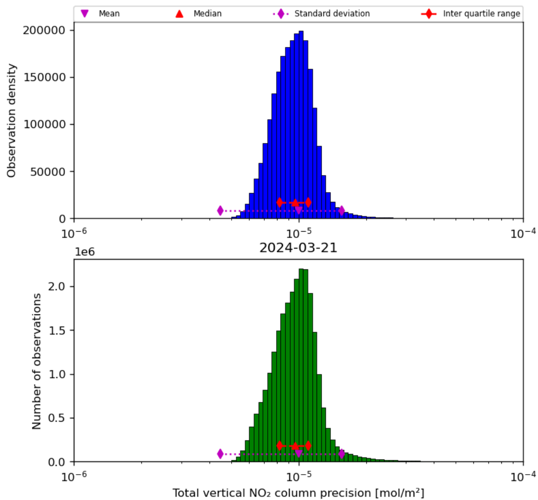
Figure 39: Histogram of "Total vertical NO 2 column precision" for 2024-03-20 to 2024-03-22
