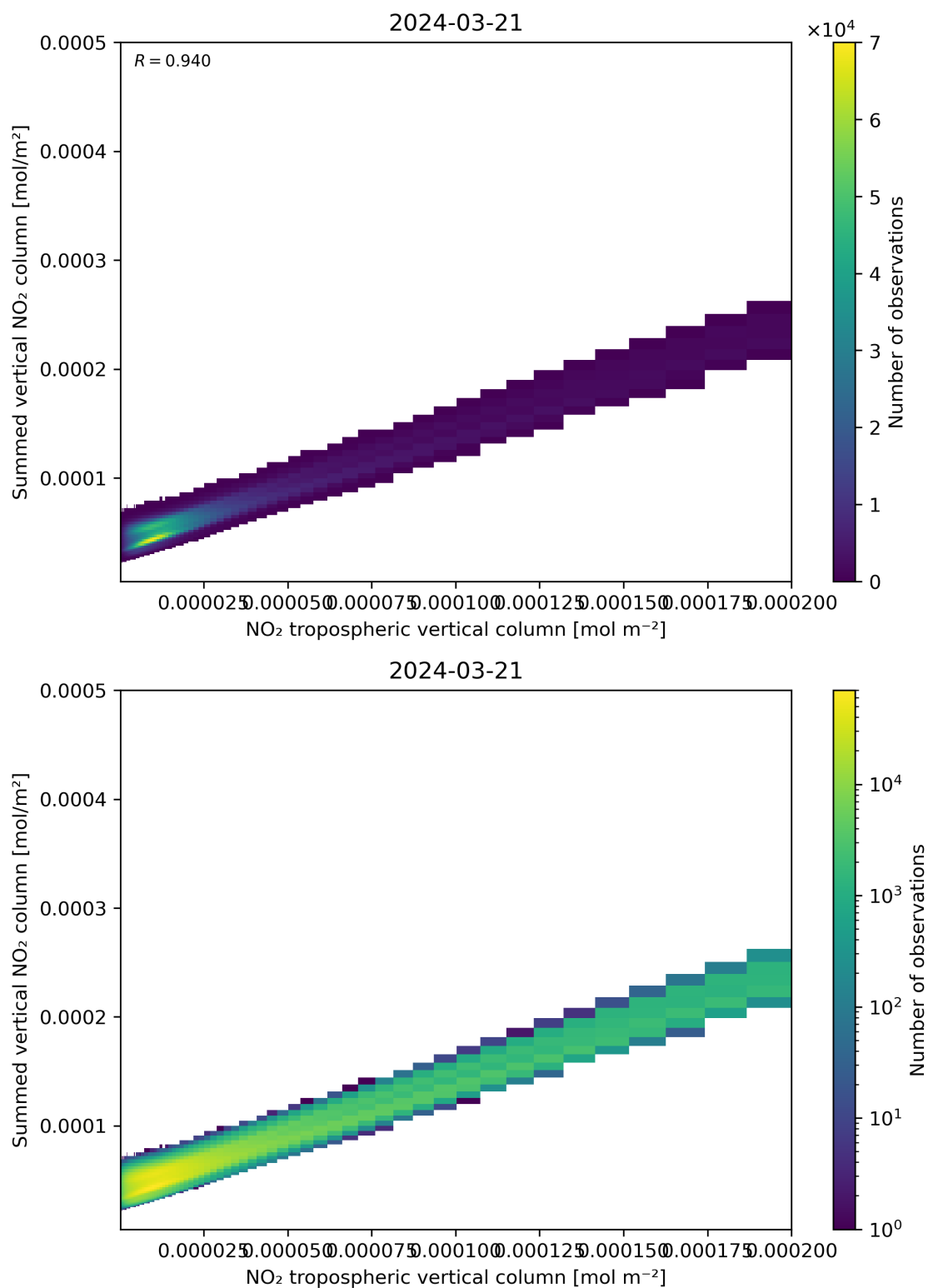
Figure 126: Scatter density plot of “NO 2 tropospheric vertical column” against “Summed vertical NO 2 column” for 2024-03-20 to 2024-03-22.
