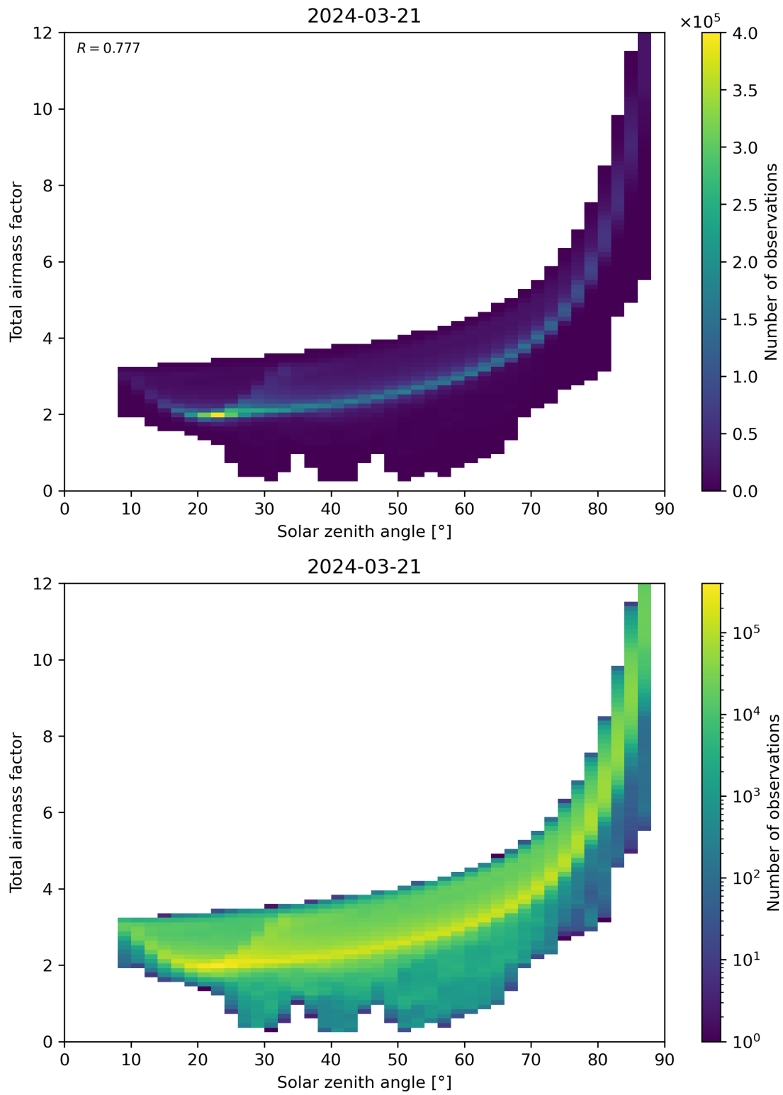
Figure 146: Scatter density plot of “Solar zenith angle” against “Total air mass factor” for 2024-03-20 to 2024-03-22.
