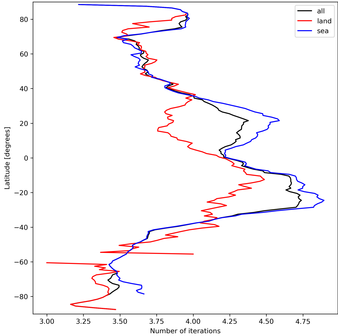
Figure 17: Zonal average of “Number of iterations” for 2024-03-20 to 2024-03-22.
