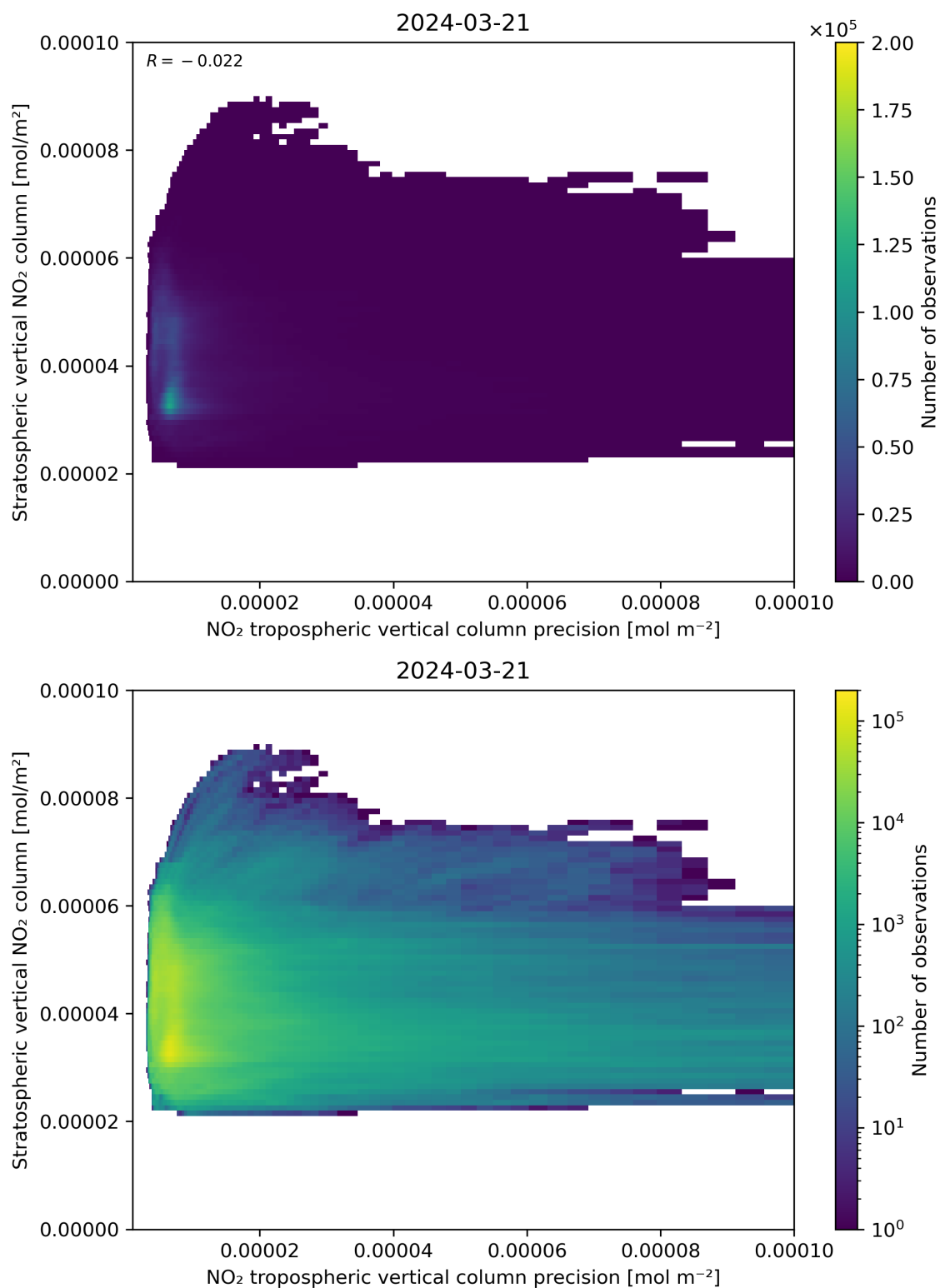
Figure 135: Scatter density plot of “NO 2 tropospheric vertical column precision” against “Stratospheric vertical NO 2 column” for 2024-03-20 to 2024-03-22.
