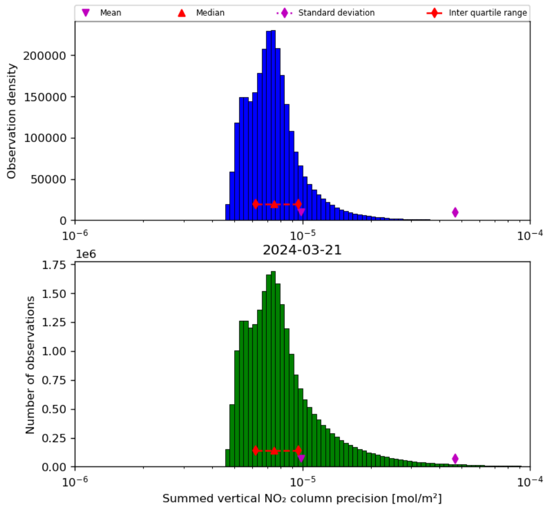
Figure 41: Histogram of "Summed vertical NO 2 column precision" for 2024-03-20 to 2024-03-22
