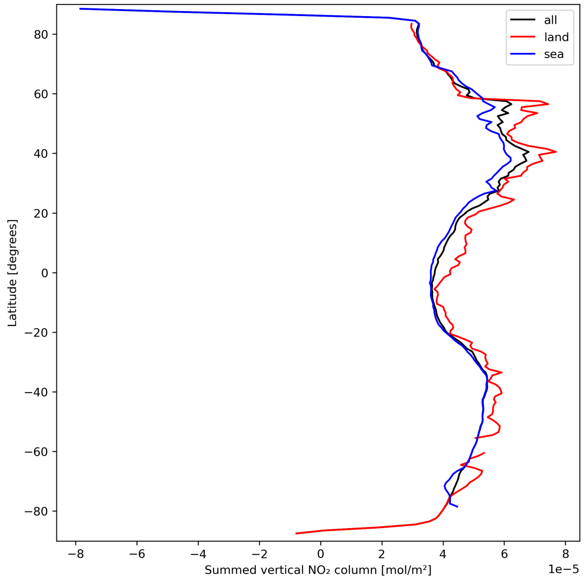
Figure 23: Zonal average of “Summed vertical NO 2 column” for 2024-03-20 to 2024-03-22.
