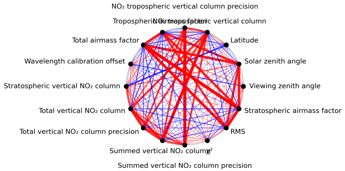
Figure 1: Map of correlation graph for 2024-03-20 to 2024-03-22.
