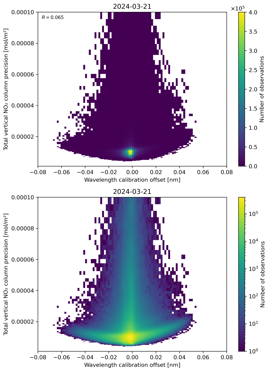
Figure 180: Scatter density plot of “Wavelength calibration offset” against “Total vertical NO 2 column precision” for 2024-03-20 to 2024-03-22.
