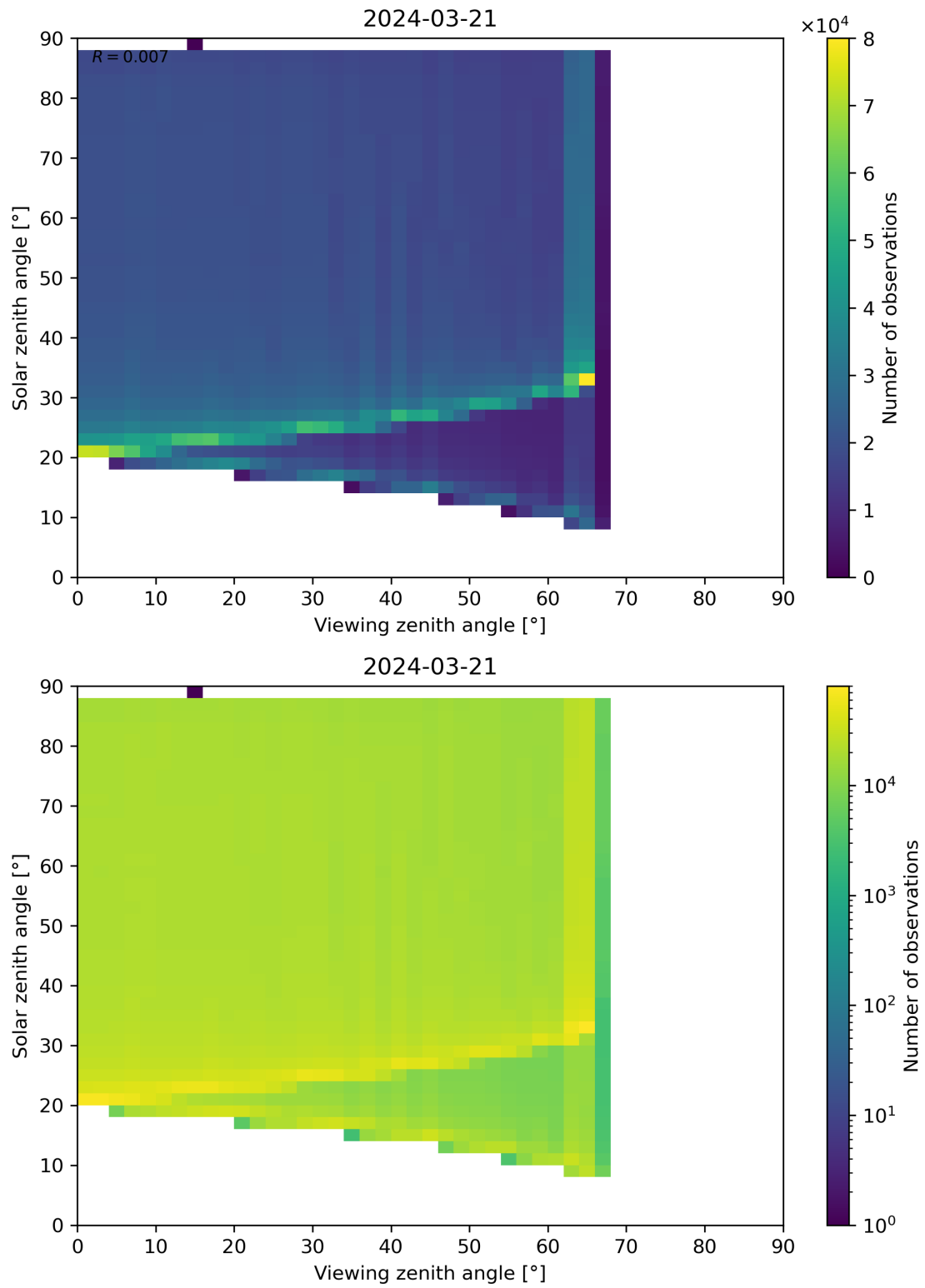
Figure 172: Scatter density plot of “Viewing zenith angle” against “Solar zenith angle” for 2024-03-20 to 2024-03-22.
