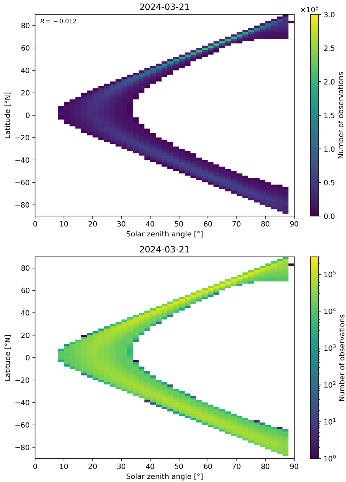
Figure 149: Scatter density plot of “Solar zenith angle” against “Latitude” for 2024-03-20 to 2024-03-22.
