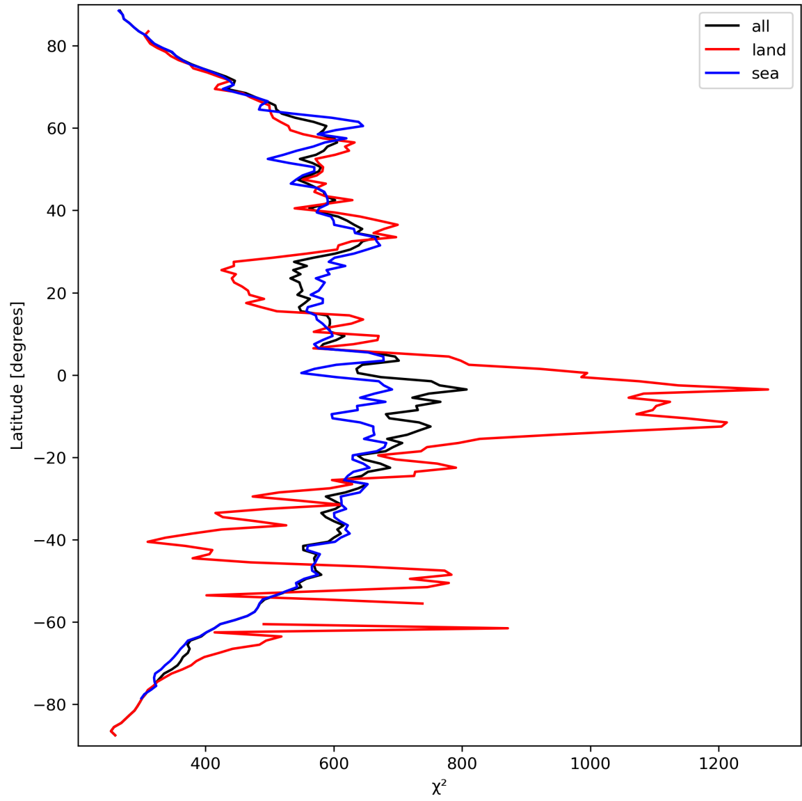
Figure 25: Zonal average of “ \chi^2 ” for 2024-03-20 to 2024-03-22.
