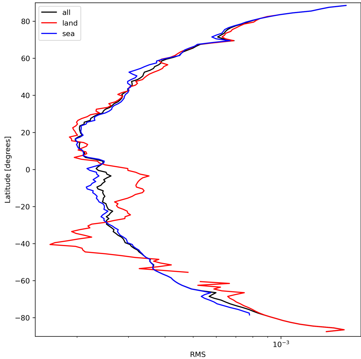
Figure 26: Zonal average of “RMS” for 2024-03-20 to 2024-03-22.
