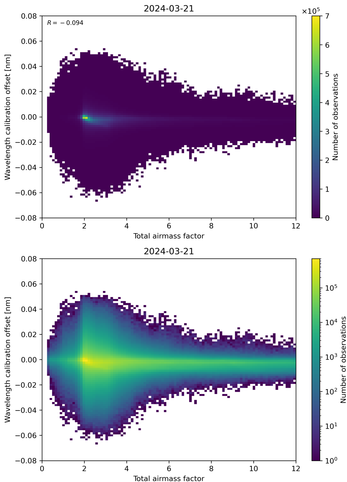
Figure 70: Scatter density plot of “Total airmass factor” against “Wavelength calibration offset” for 2024-03-20 to 2024-03-22.
