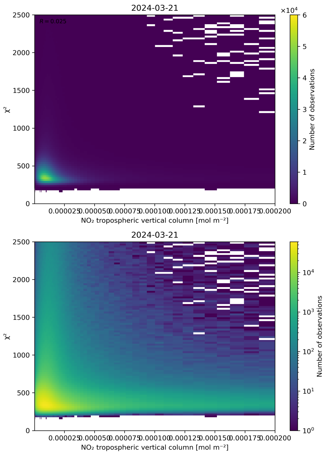
Figure 124: Scatter density plot of “NO 2 tropospheric vertical column” against “ \chi^2 ” for 2024-03-20 to 2024-03-22.
