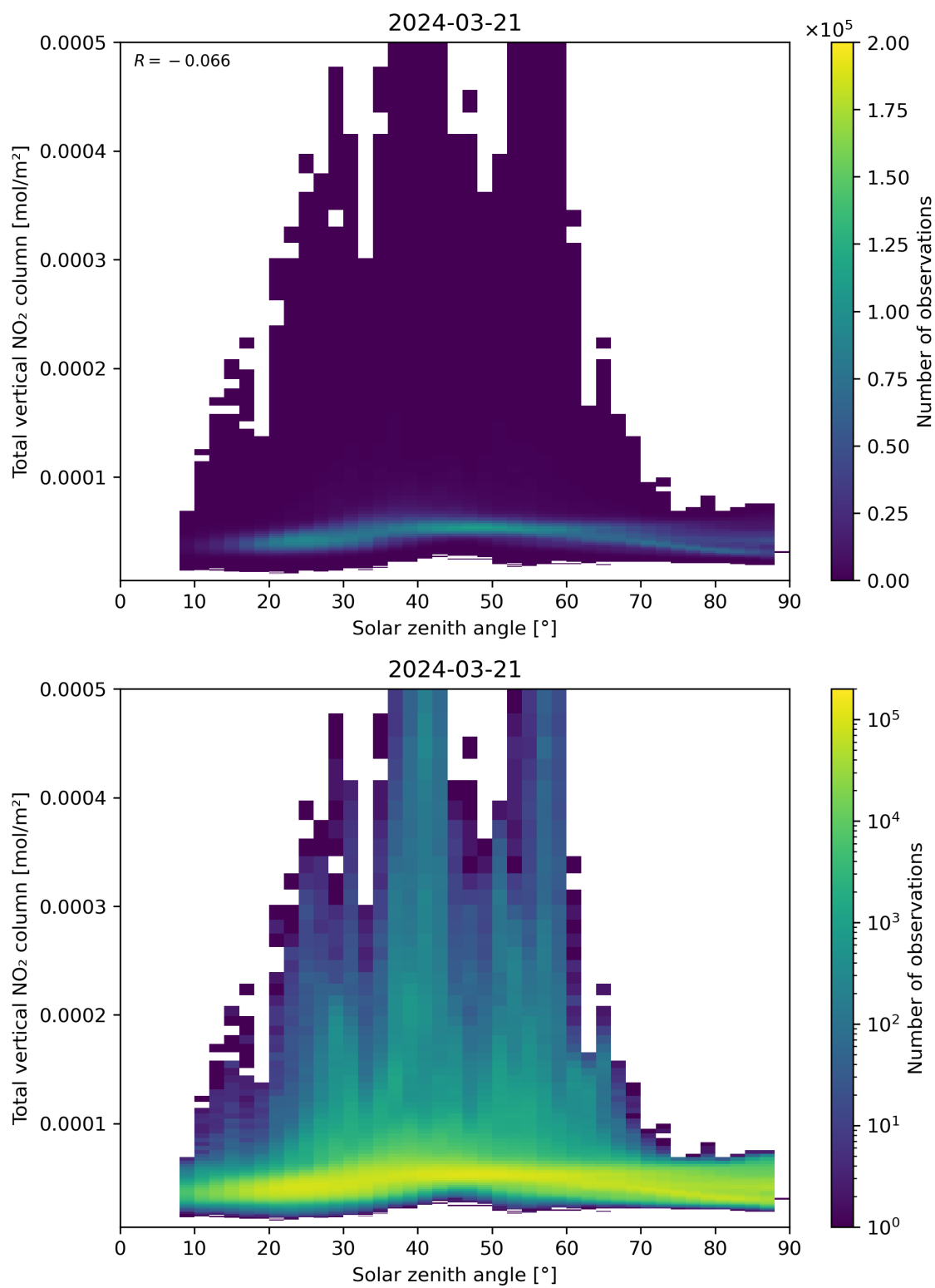
Figure 153: Scatter density plot of “Solar zenith angle” against “Total vertical NO 2 column” for 2024-03-20 to 2024-03-22.
