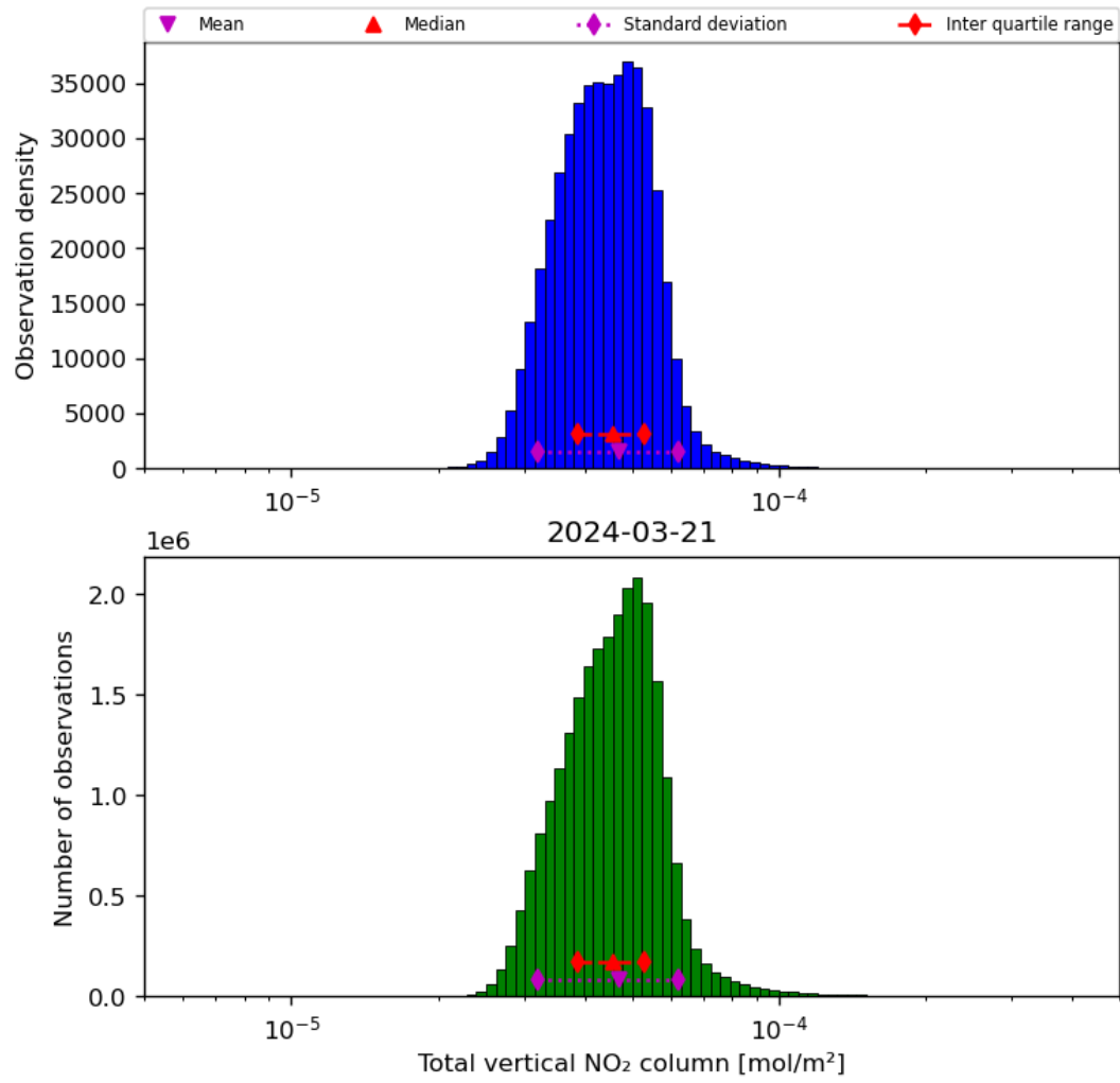
Figure 38: Histogram of "Total vertical NO 2 column" for 2024-03-20 to 2024-03-22
