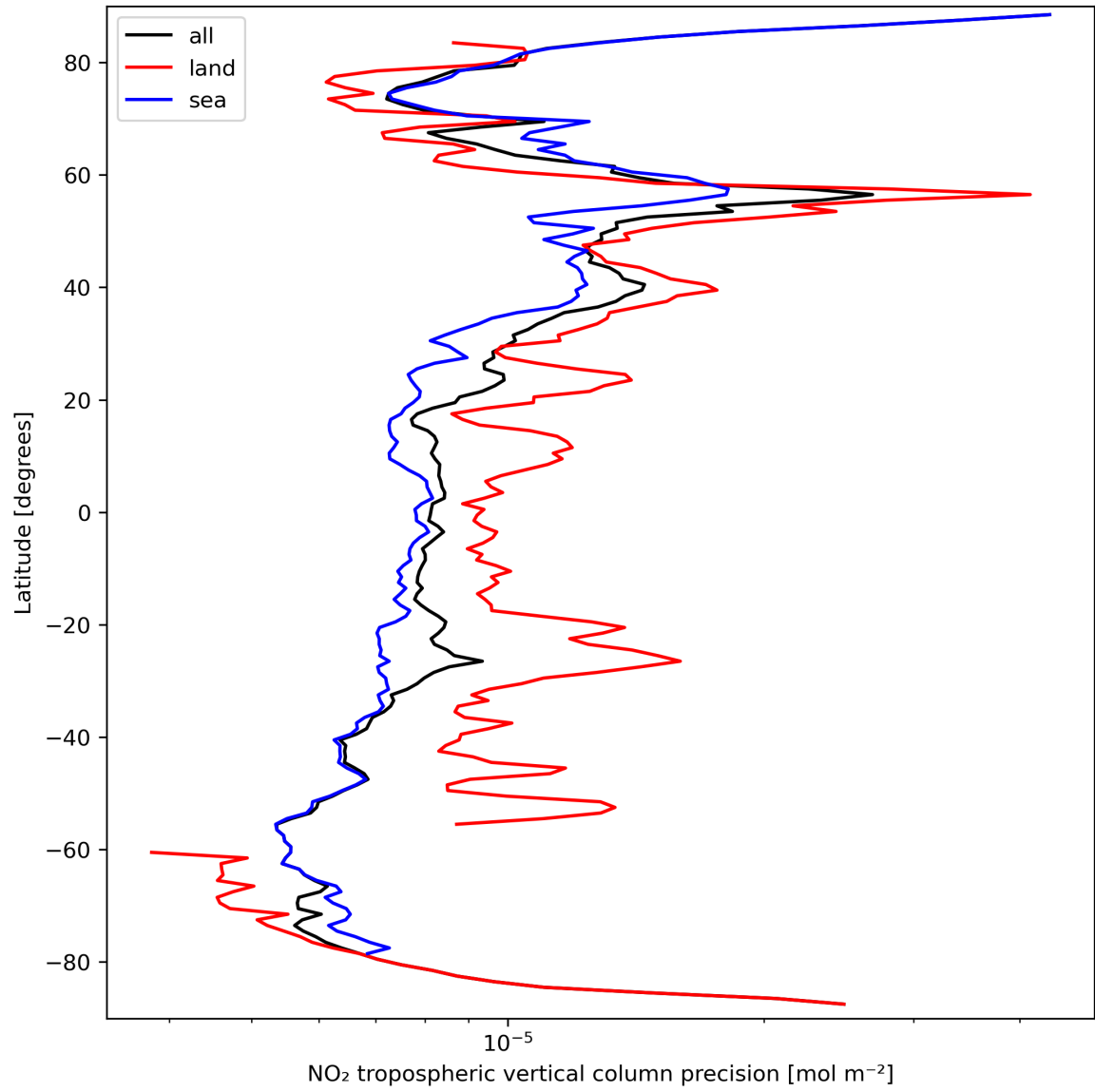
Figure 13: Zonal average of “NO 2 tropospheric vertical column precision” for 2024-03-20 to 2024-03-22.
