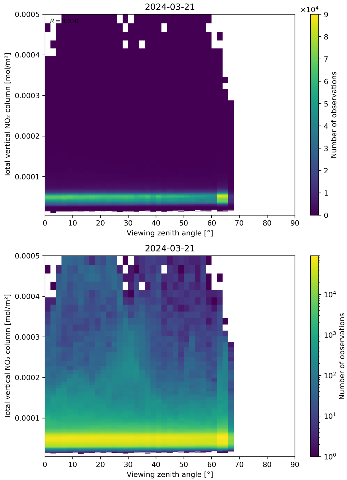
Figure 167: Scatter density plot of “Viewing zenith angle” against “Total vertical NO 2 column” for 2024-03-20 to 2024-03-22.
