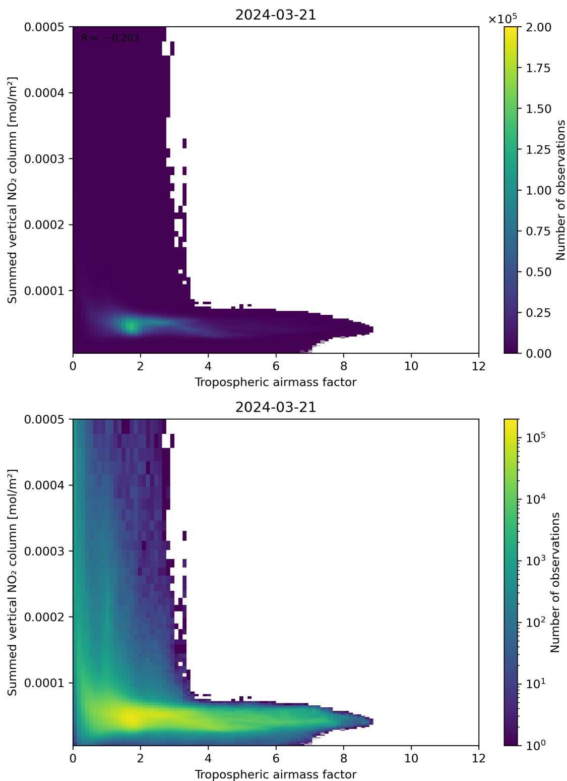
Figure 75: Scatter density plot of “Tropospheric air mass factor” against “Summed vertical NO 2 column” for 2024-03-20 to 2024-03-22.
