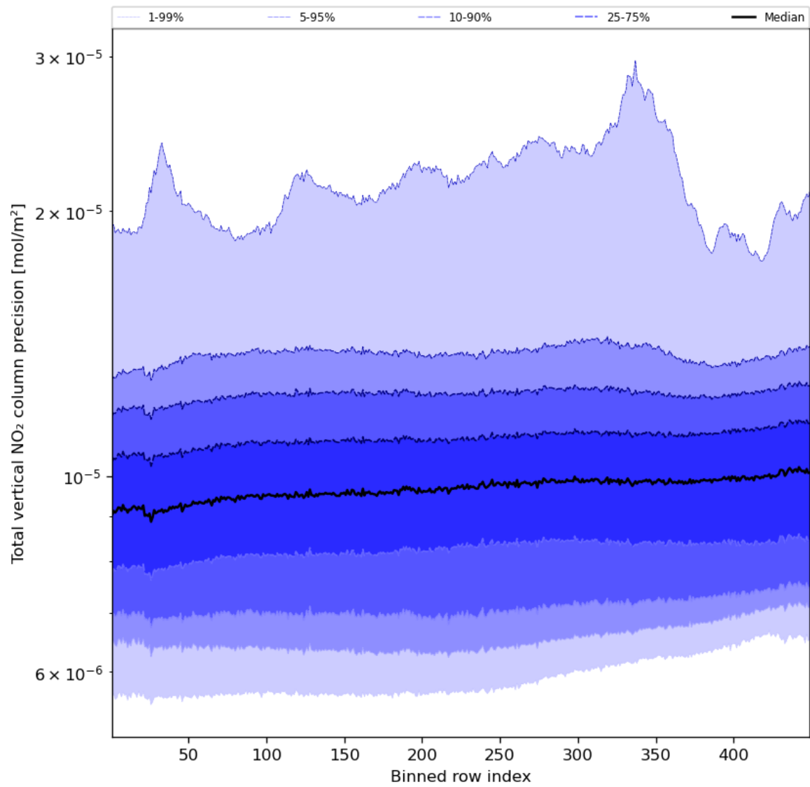
Figure 56: Along track statistics of “Total vertical NO 2 column precision” for 2024-03-20 to 2024-03-22
