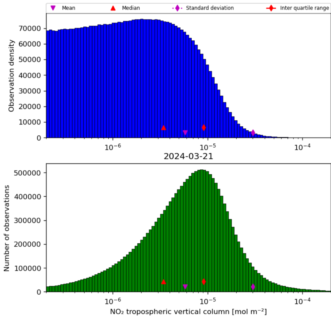
Figure 29: Histogram of “NO 2 tropospheric vertical column” for 2024-03-20 to 2024-03-22
