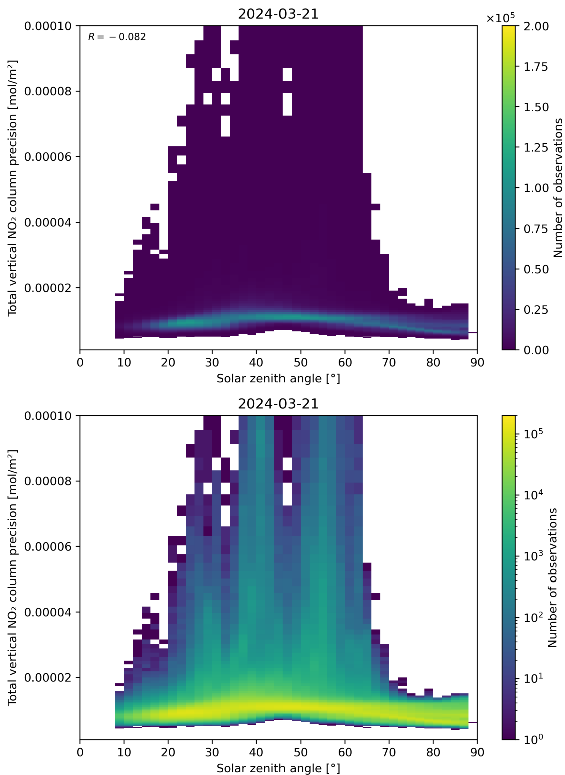
Figure 154: Scatter density plot of “Solar zenith angle” against “Total vertical NO 2 column precision” for 2024-03-20 to 2024-03-22.
