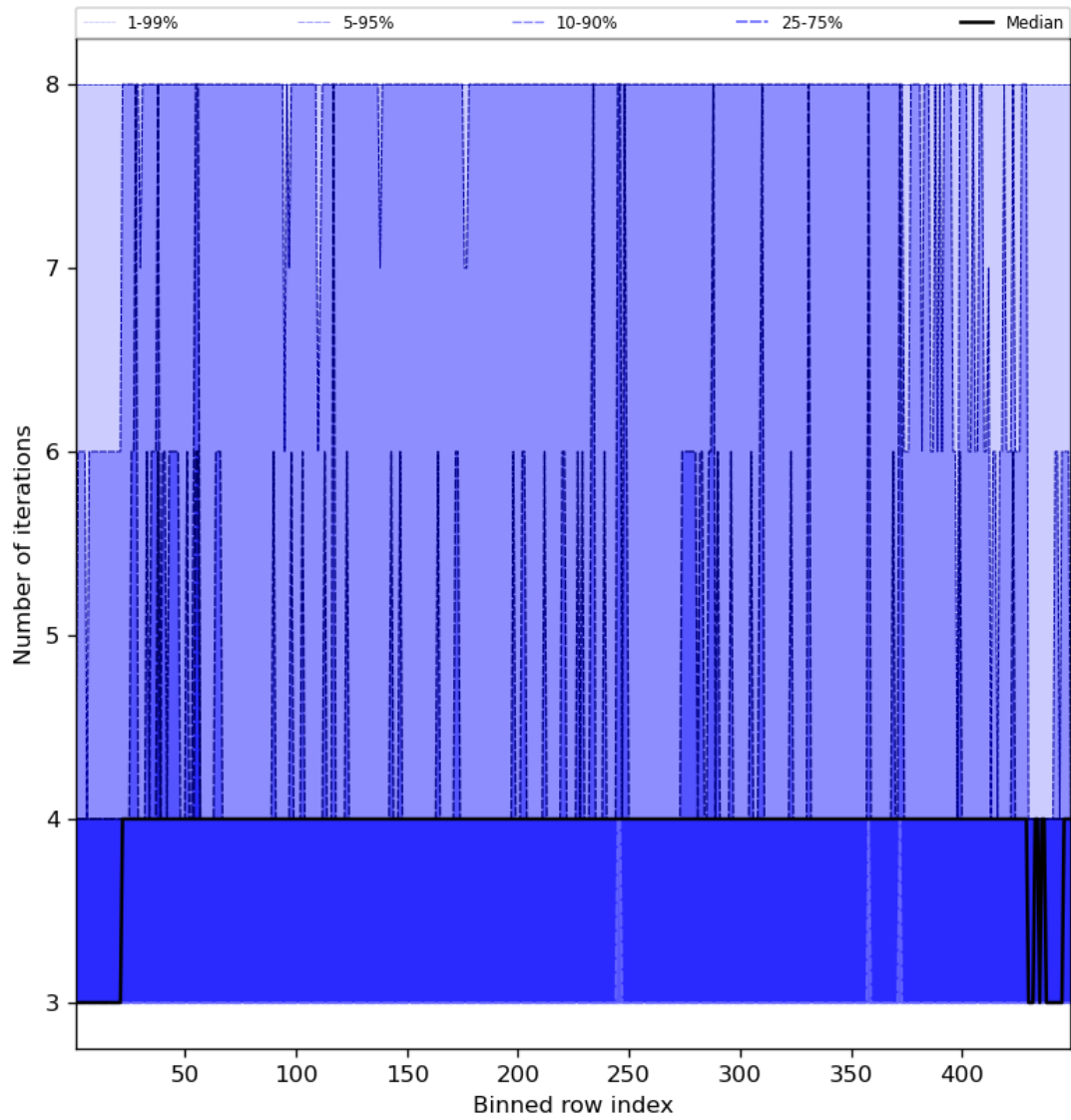
Figure 51: Along track statistics of “Number of iterations” for 2024-03-20 to 2024-03-22
