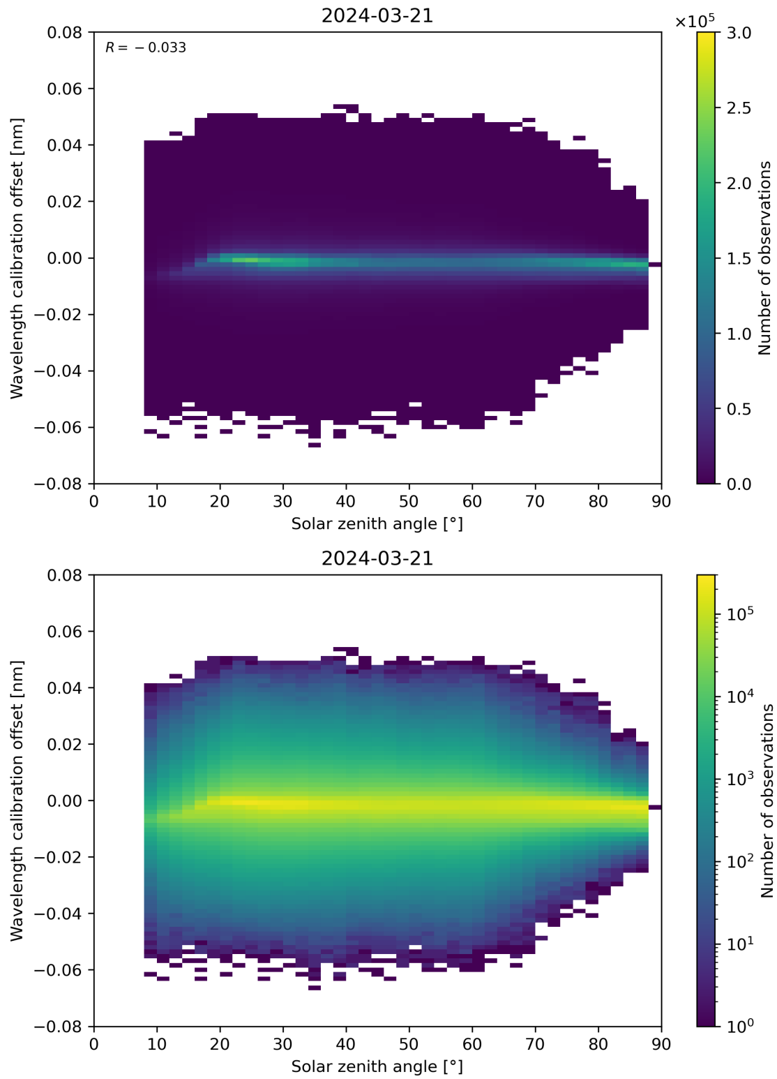
Figure 158: Scatter density plot of “Solar zenith angle” against “Wavelength calibration offset” for 2024-03-20 to 2024-03-22.
