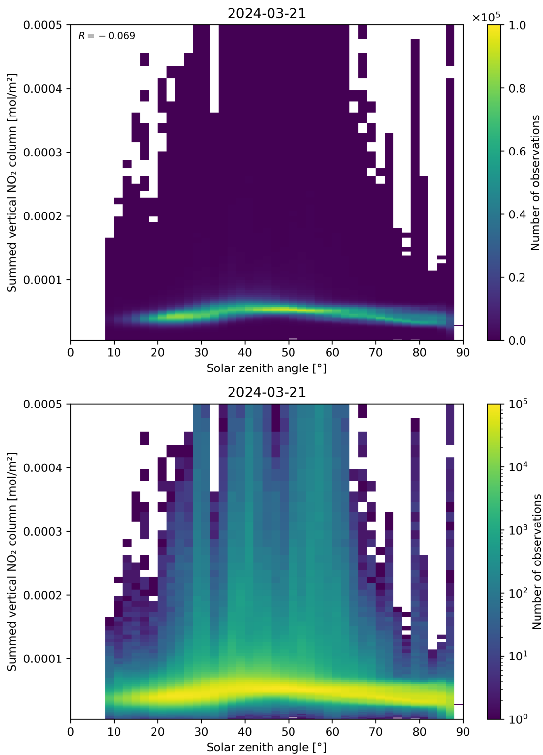
Figure 151: Scatter density plot of “Solar zenith angle” against “Summed vertical NO 2 column” for 2024-03-20 to 2024-03-22.
