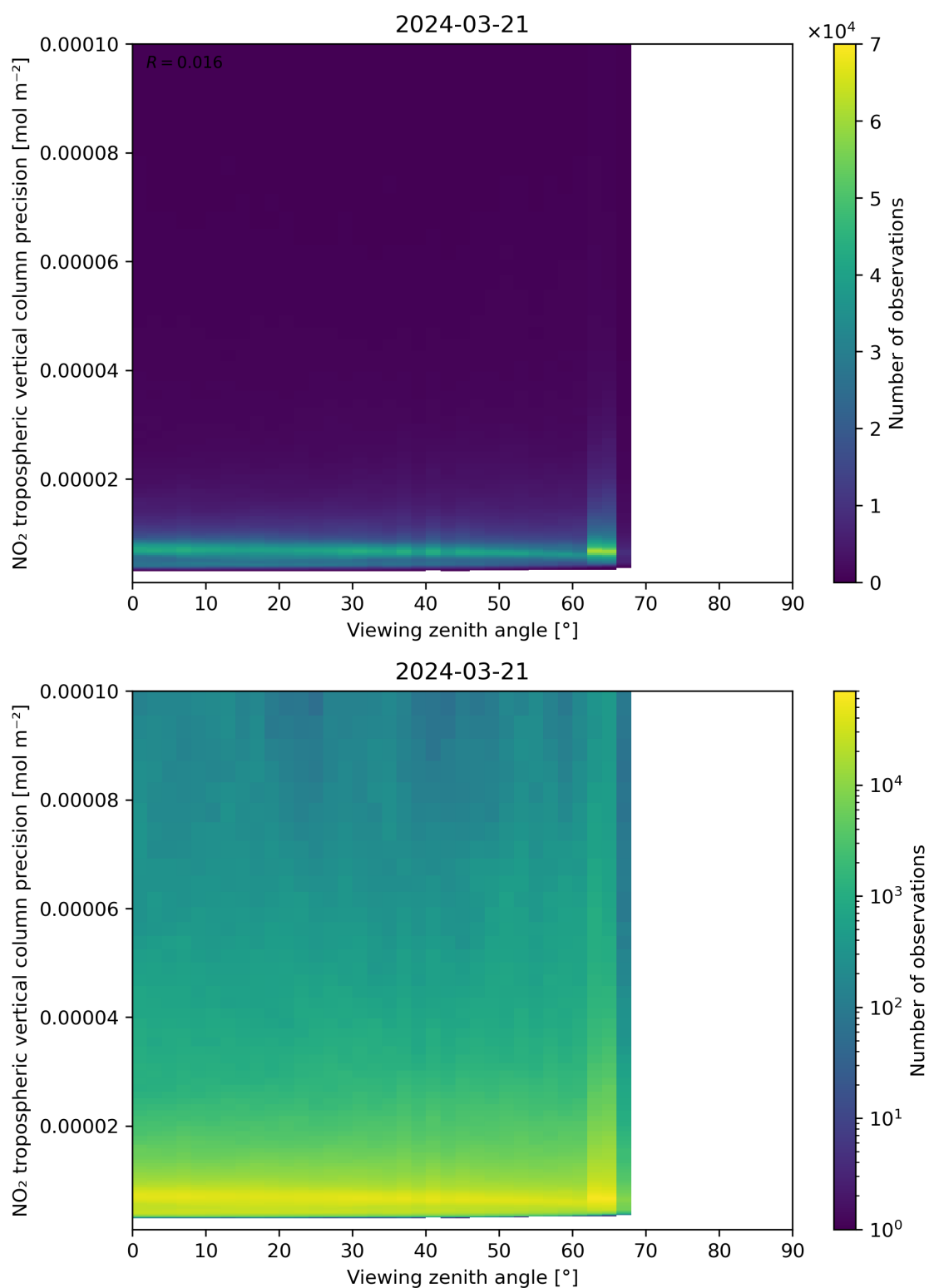
Figure 170: Scatter density plot of “Viewing zenith angle” against “NO 2 tropospheric vertical column precision” for 2024-03-20 to 2024-03-22.
