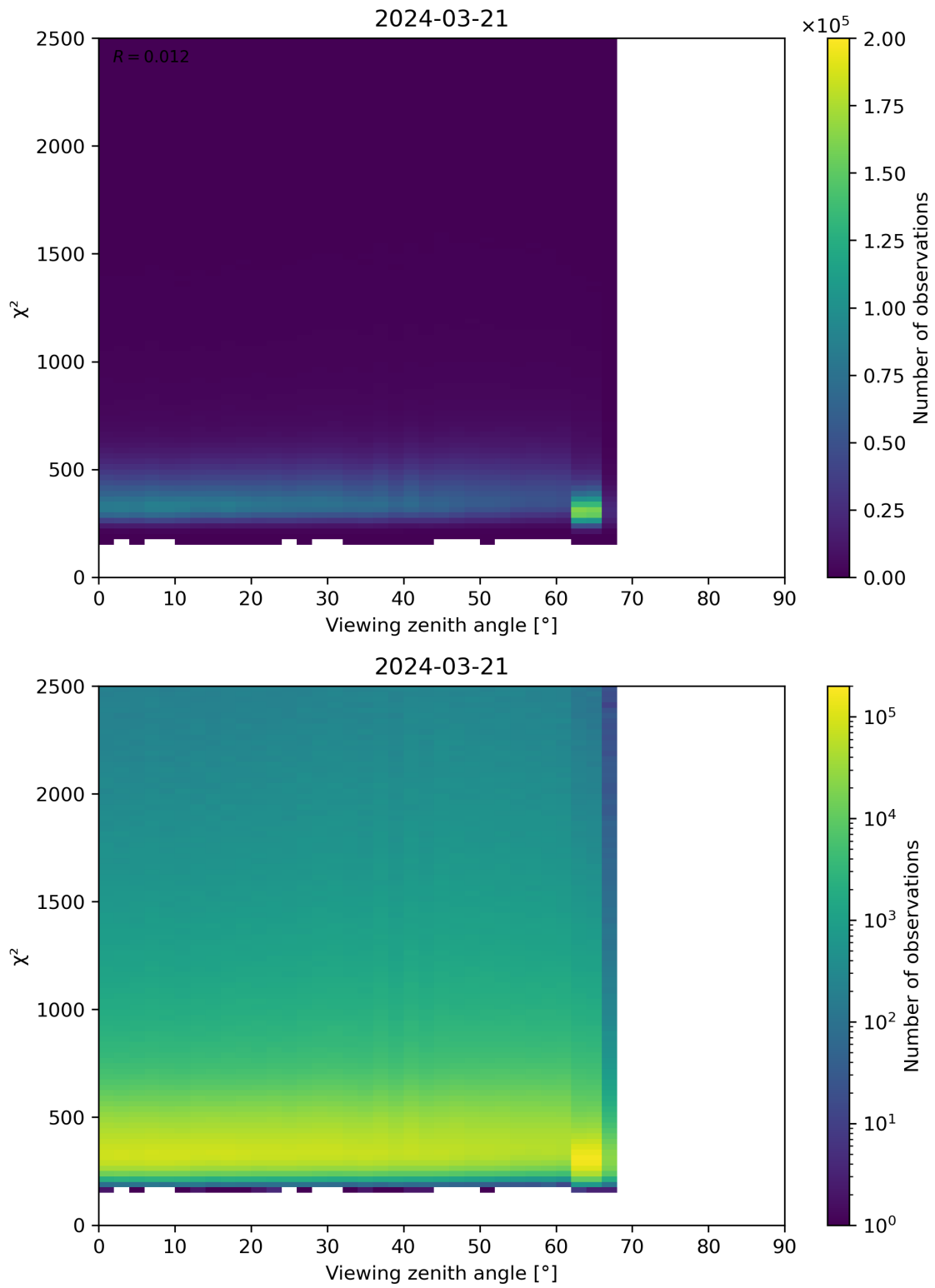
Figure 162: Scatter density plot of “Viewing zenith angle” against “ \chi^2 ” for 2024-03-20 to 2024-03-22.
