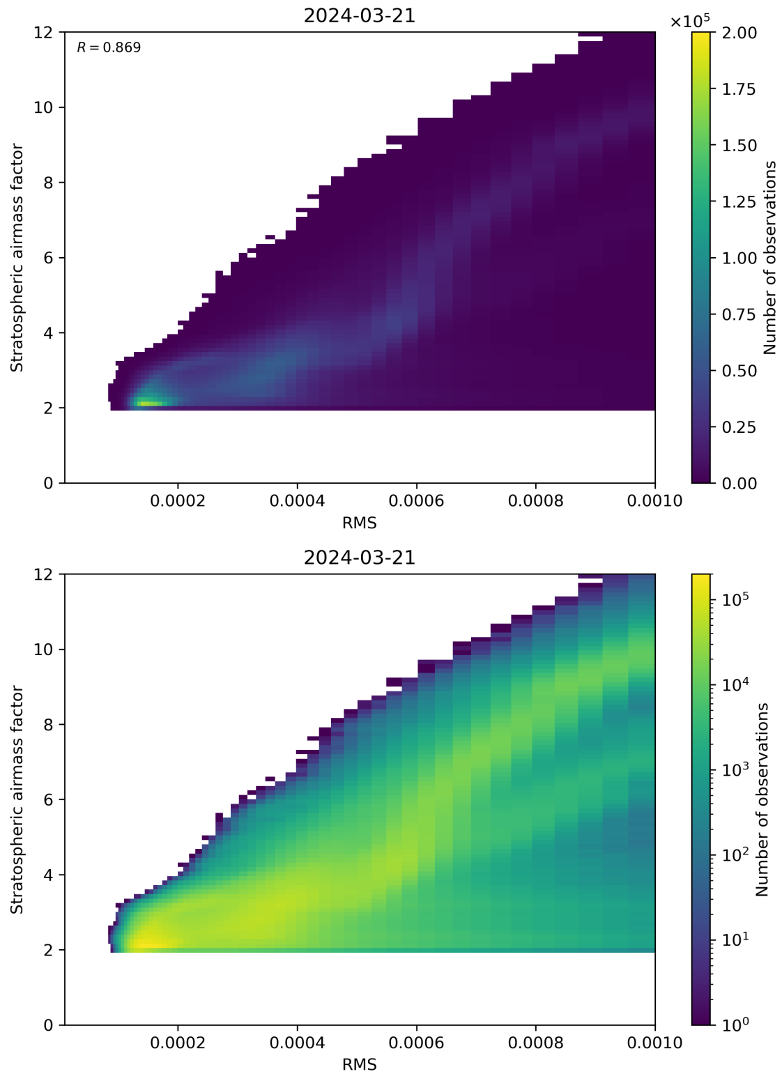
Figure 144: Scatter density plot of “RMS” against “Stratospheric airmass factor” for 2024-03-20 to 2024-03-22.
