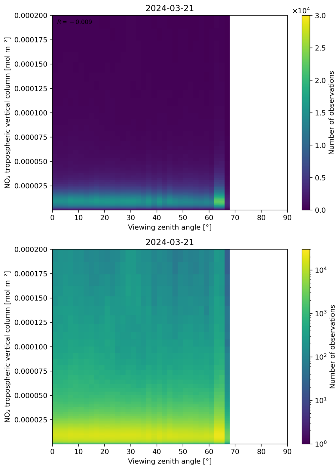
Figure 169: Scatter density plot of “Viewing zenith angle” against “NO 2 tropospheric vertical column” for 2024-03-20 to 2024-03-22.
