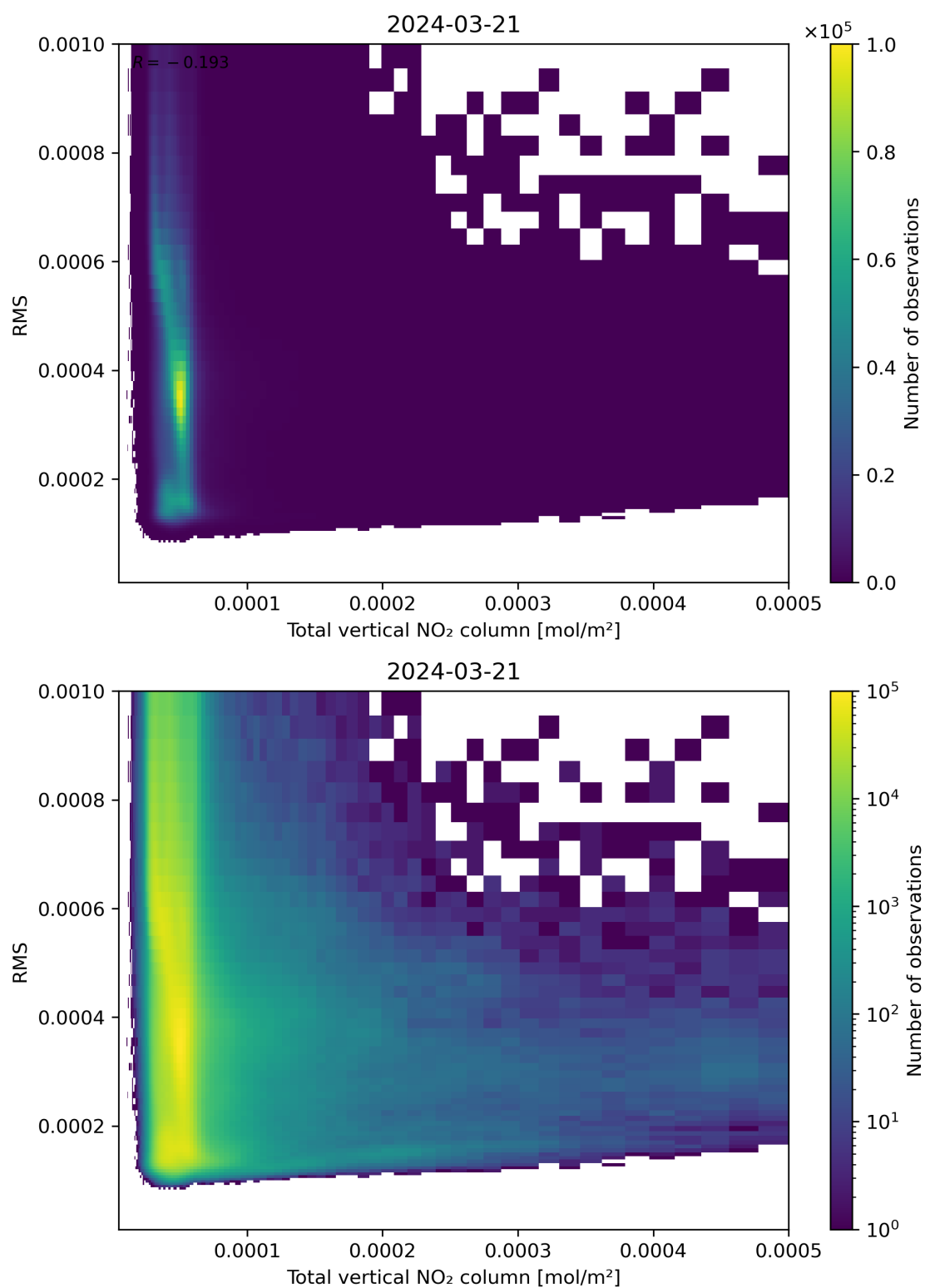
Figure 120: Scatter density plot of “Total vertical NO 2 column” against “RMS” for 2024-03-20 to 2024-03-22.
