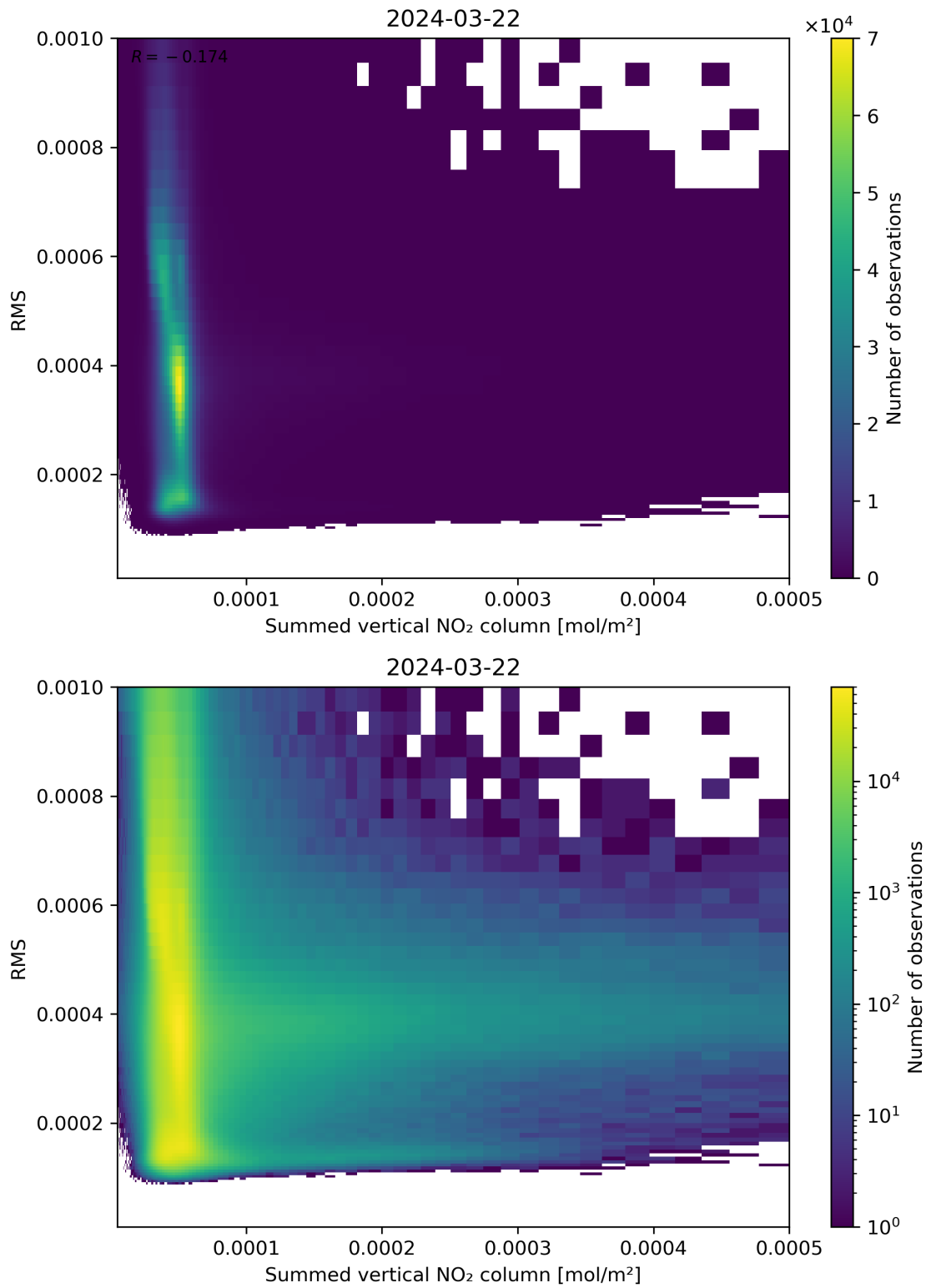
Figure 109: Scatter density plot of “Summed vertical NO 2 column” against “RMS” for 2024-03-21 to 2024-03-22.
