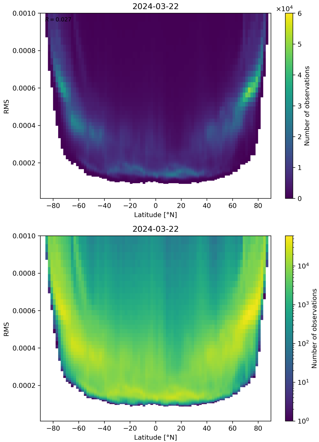
Figure 94: Scatter density plot of “Latitude” against “RMS” for 2024-03-21 to 2024-03-22.
