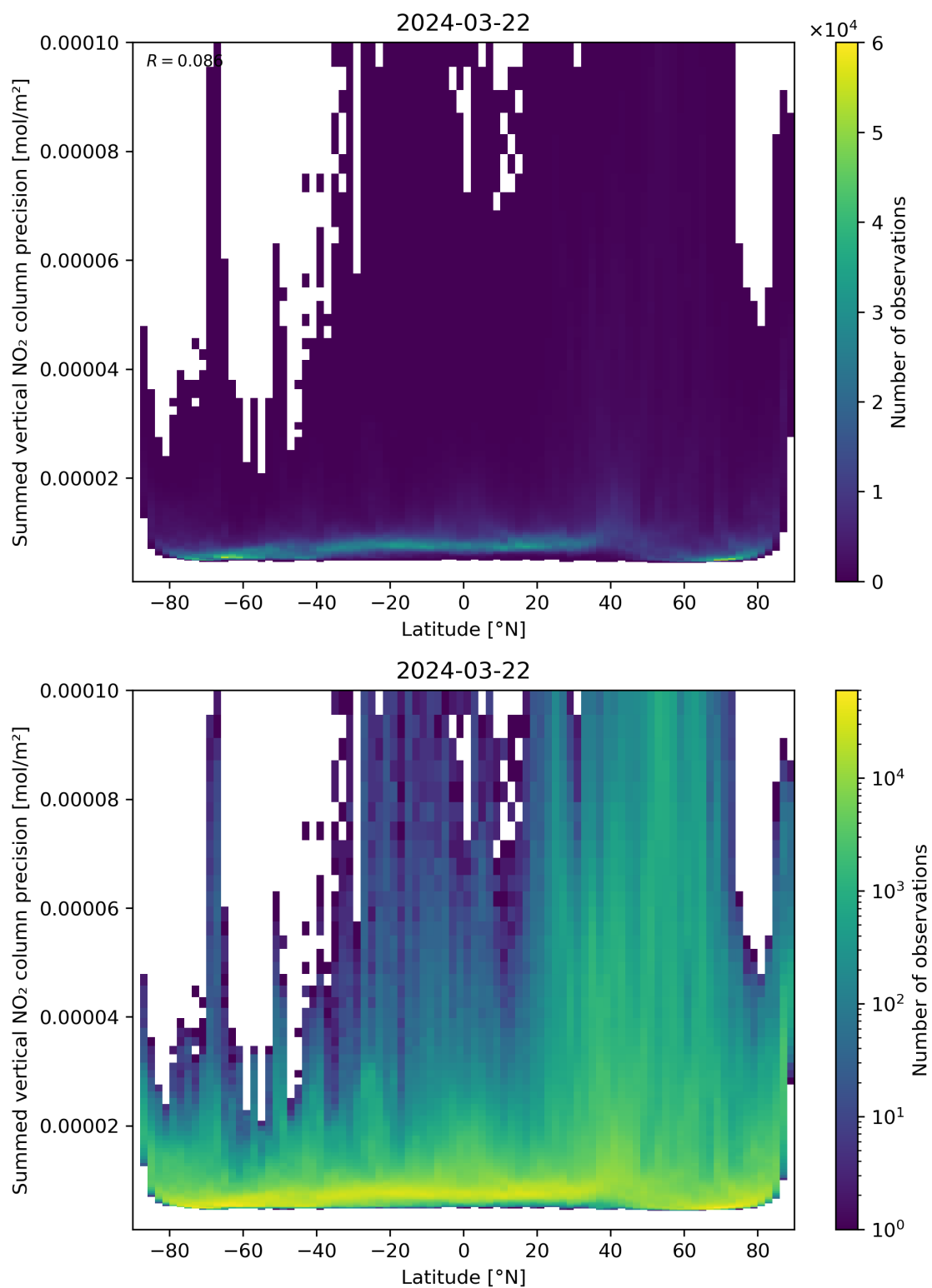
Figure 89: Scatter density plot of “Latitude” against “Summed vertical NO 2 column precision” for 2024-03-21 to 2024-03-22.
