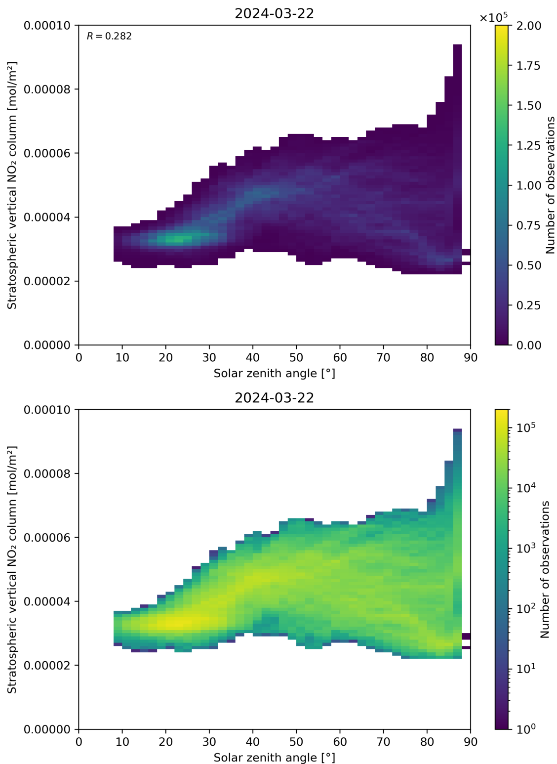
Figure 150: Scatter density plot of “Solar zenith angle” against “Stratospheric vertical \text{NO}_2 column” for 2024-03-21 to 2024-03-22.
