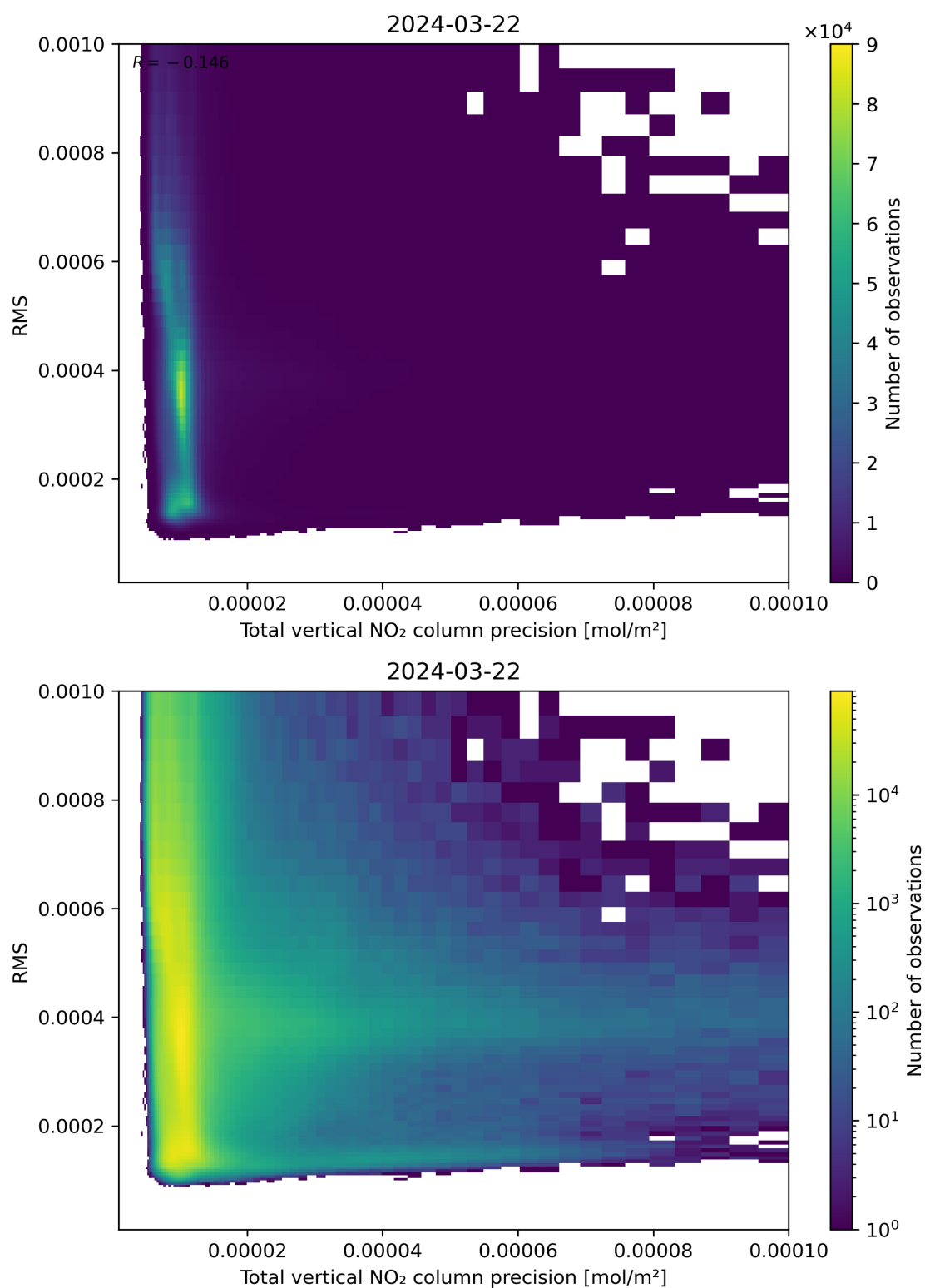
Figure 119: Scatter density plot of “Total vertical NO 2 column precision” against “RMS” for 2024-03-21 to 2024-03-22.
