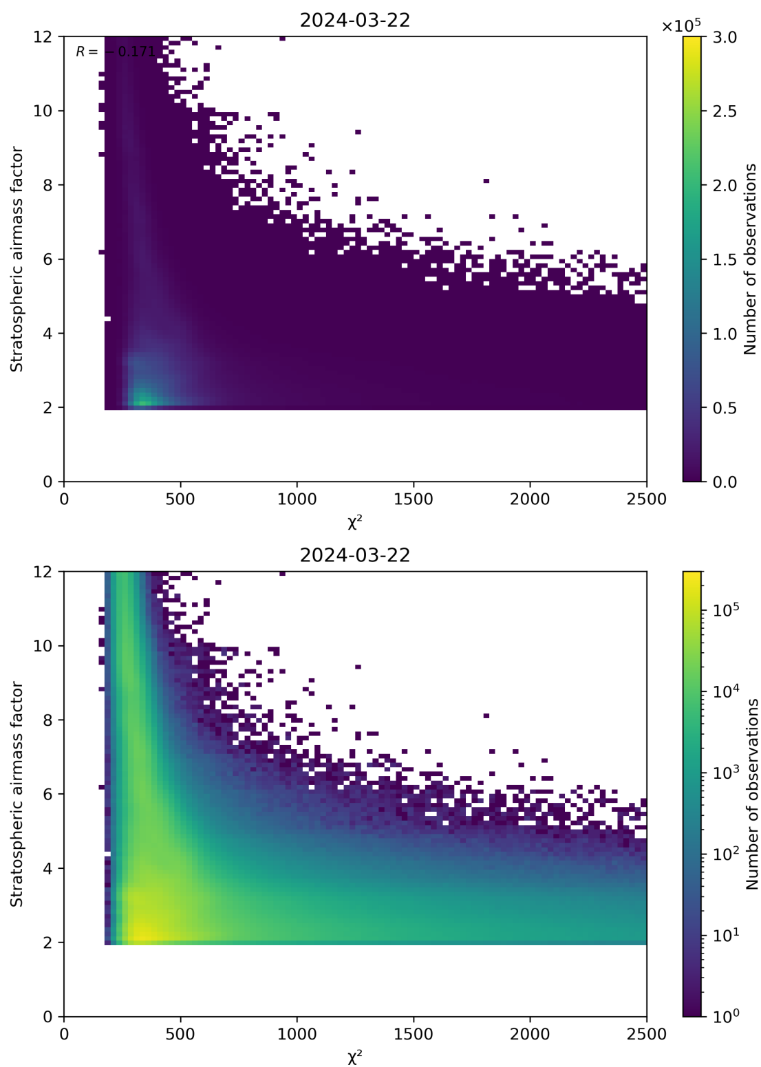
Figure 81: Scatter density plot of “ \chi^2 ” against “Stratospheric airmass factor” for 2024-03-21 to 2024-03-22.
