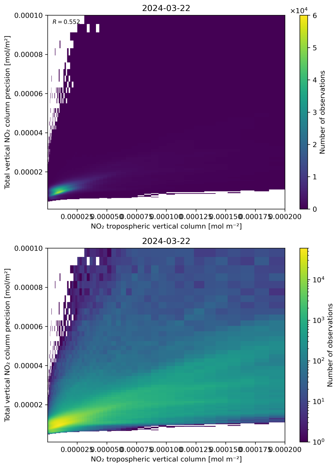
Figure 129: Scatter density plot of “NO 2 tropospheric vertical column” against “Total vertical NO 2 column precision” for 2024-03-21 to 2024-03-22.
