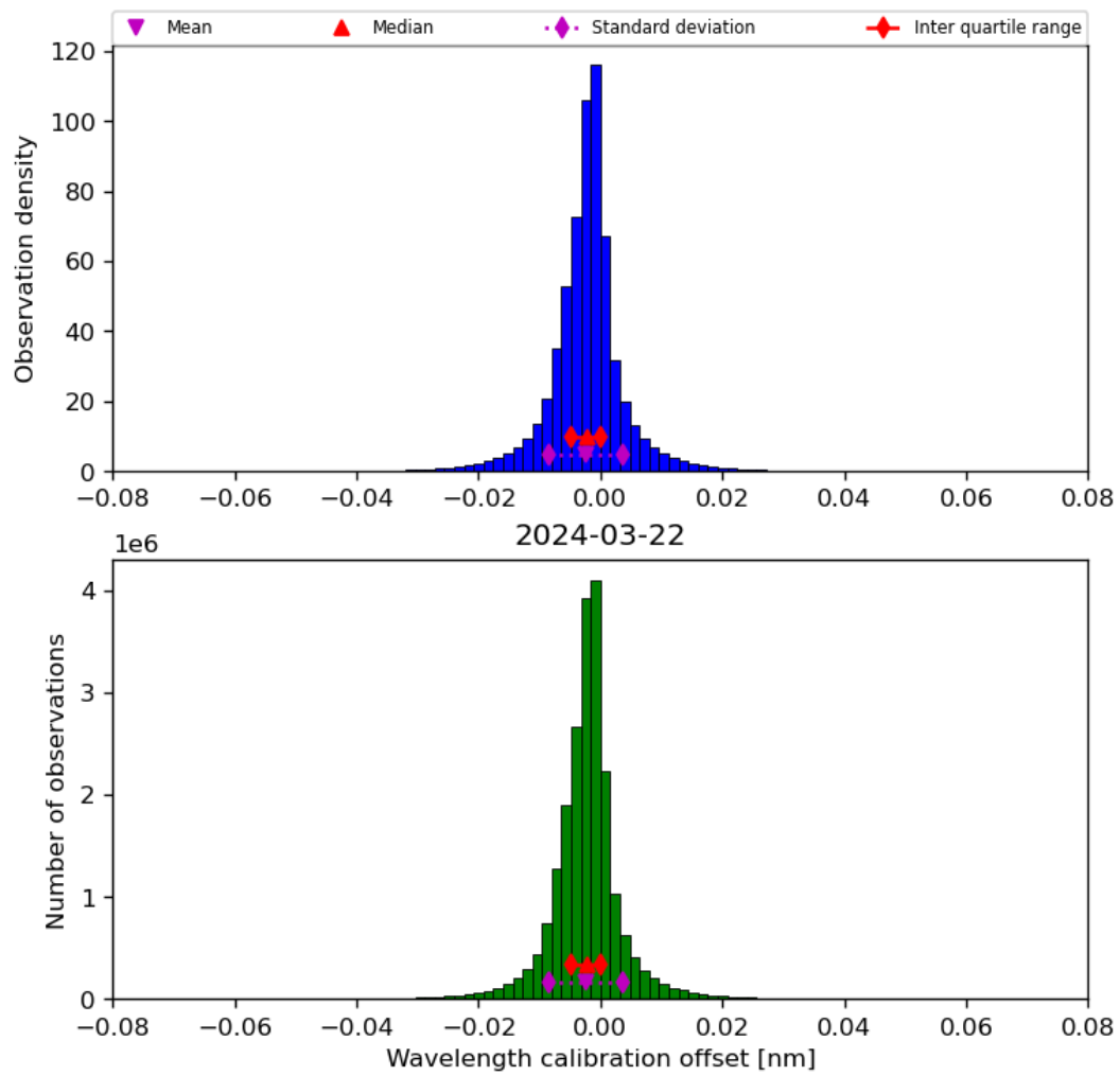
Figure 35: Histogram of “Wavelength calibration offset” for 2024-03-21 to 2024-03-22
