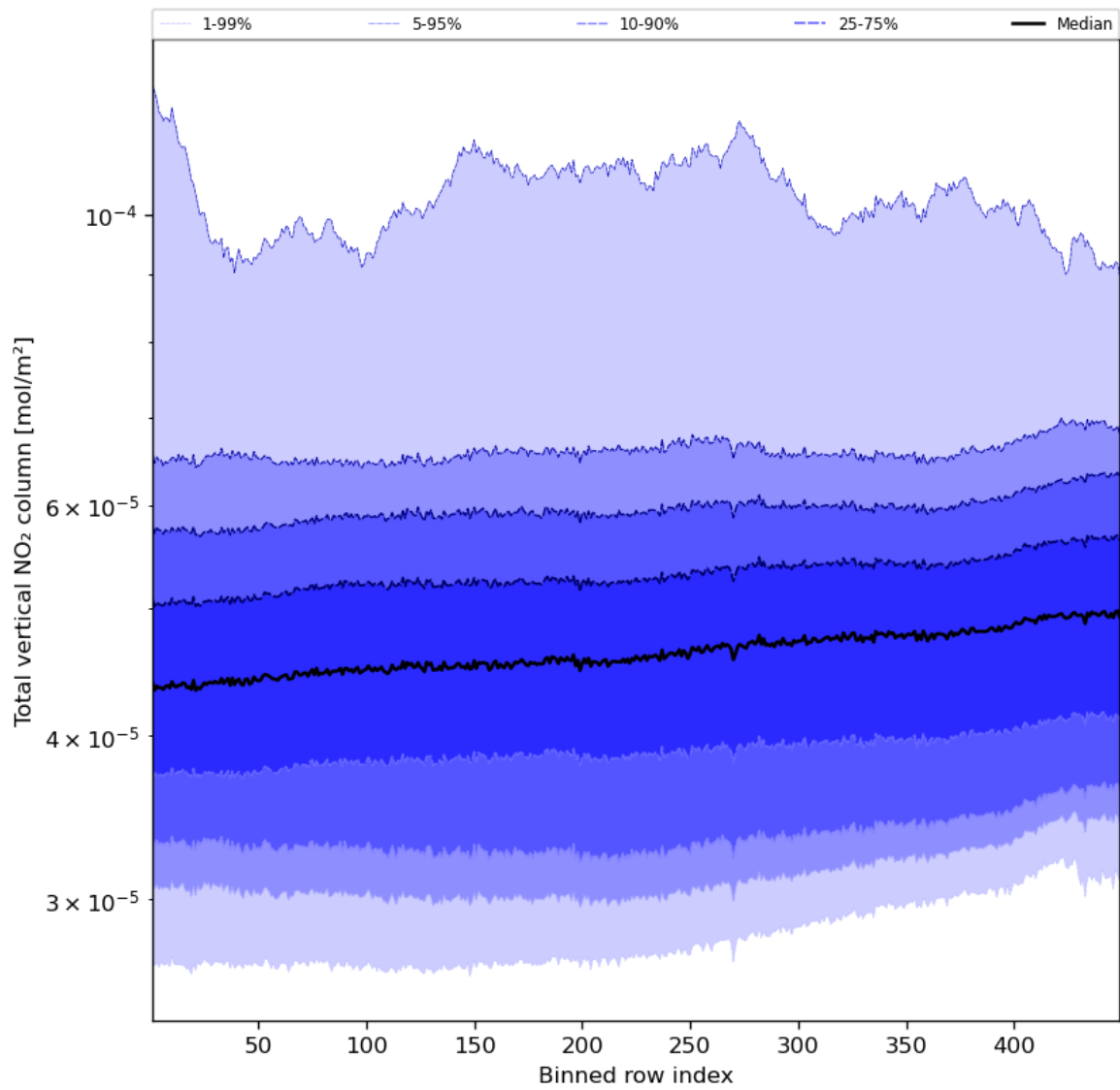
Figure 55: Along track statistics of “Total vertical NO 2 column” for 2024-03-21 to 2024-03-22
