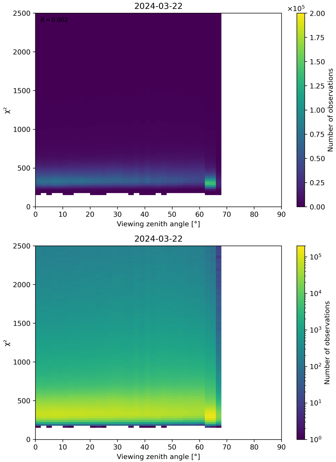
Figure 162: Scatter density plot of “Viewing zenith angle” against “ \chi^2 ” for 2024-03-21 to 2024-03-22.
