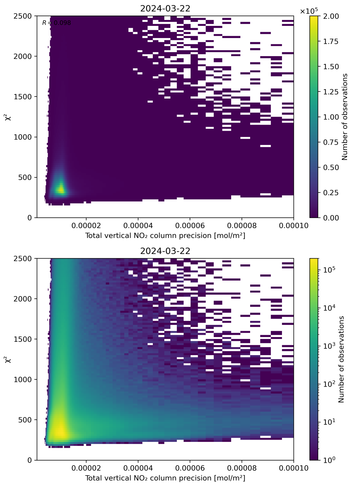
Figure 116: Scatter density plot of “Total vertical NO 2 column precision” against “ \chi^2 ” for 2024-03-21 to 2024-03-22.
