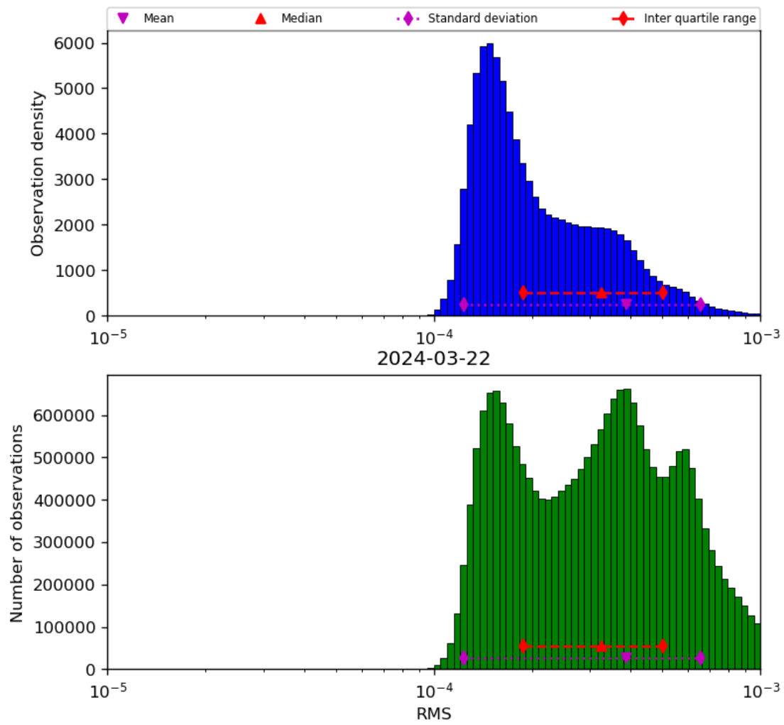
Figure 43: Histogram of “RMS” for 2024-03-21 to 2024-03-22
