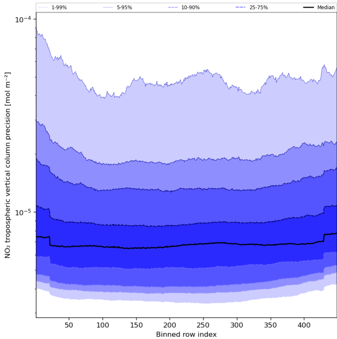
Figure 47: Along track statistics of “NO 2 tropospheric vertical column precision” for 2024-03-21 to 2024-03-22
