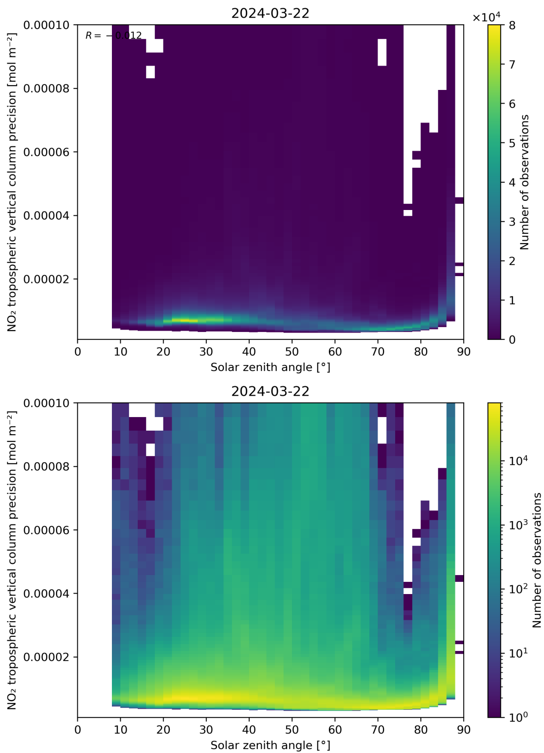
Figure 156: Scatter density plot of “Solar zenith angle” against “NO 2 tropospheric vertical column precision” for 2024-03-21 to 2024-03-22.
