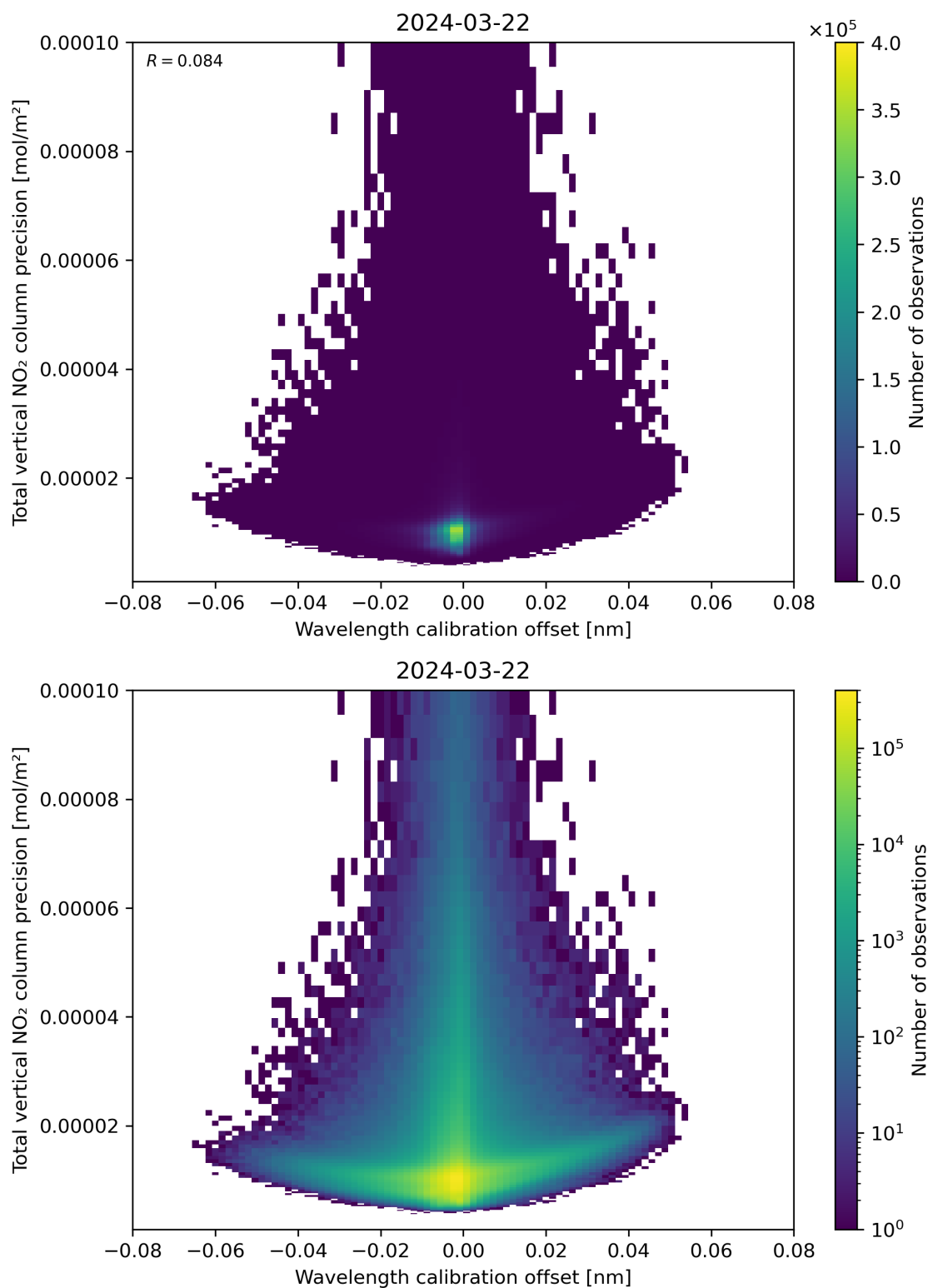
Figure 180: Scatter density plot of “Wavelength calibration offset” against “Total vertical NO 2 column precision” for 2024-03-21 to 2024-03-22.
