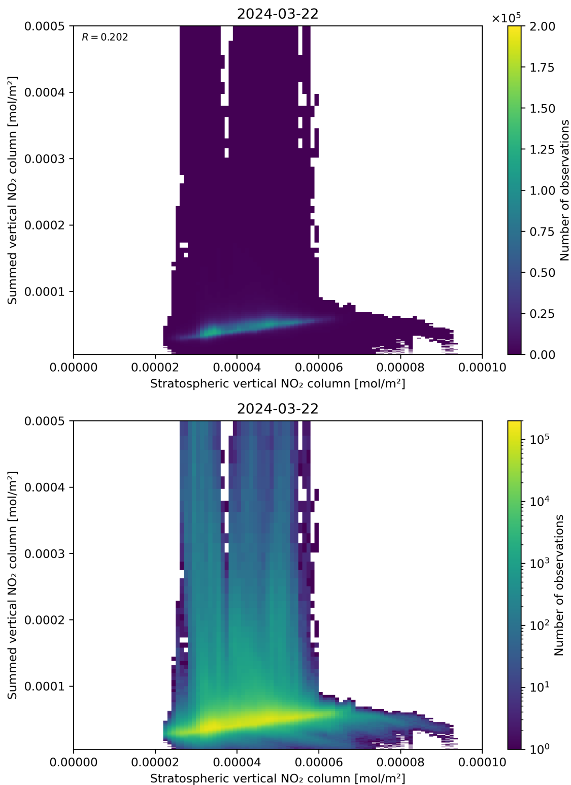
Figure 98: Scatter density plot of “Stratospheric vertical NO 2 column” against “Summed vertical NO 2 column” for 2024-03-21 to 2024-03-22.
