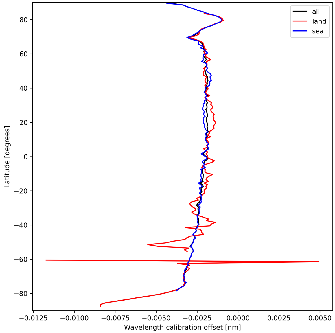
Figure 18: Zonal average of “Wavelength calibration offset” for 2024-03-21 to 2024-03-22.
