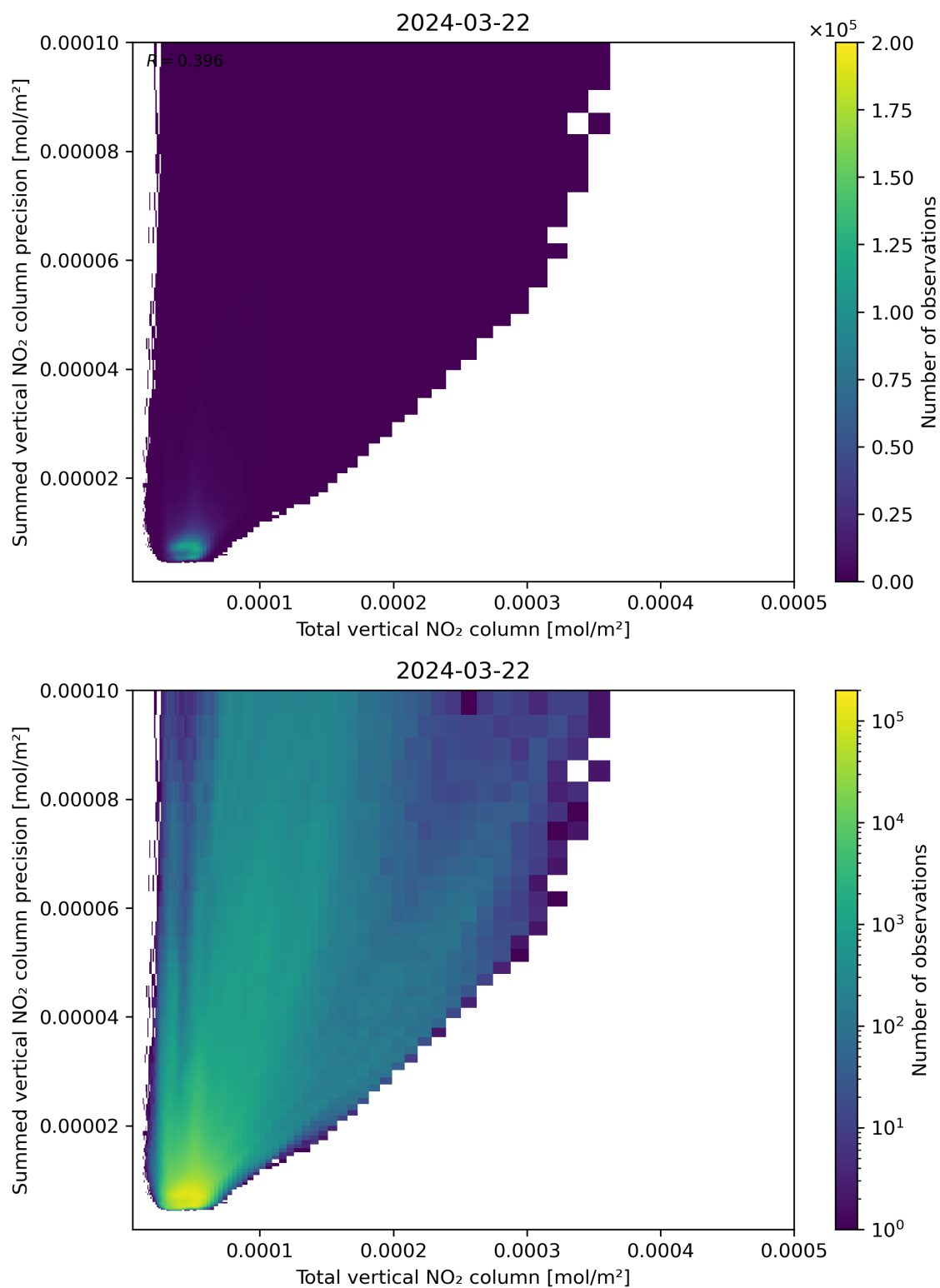
Figure 113: Scatter density plot of “Total vertical NO 2 column” against “Summed vertical NO 2 column precision” for 2024-03-21 to 2024-03-22.
