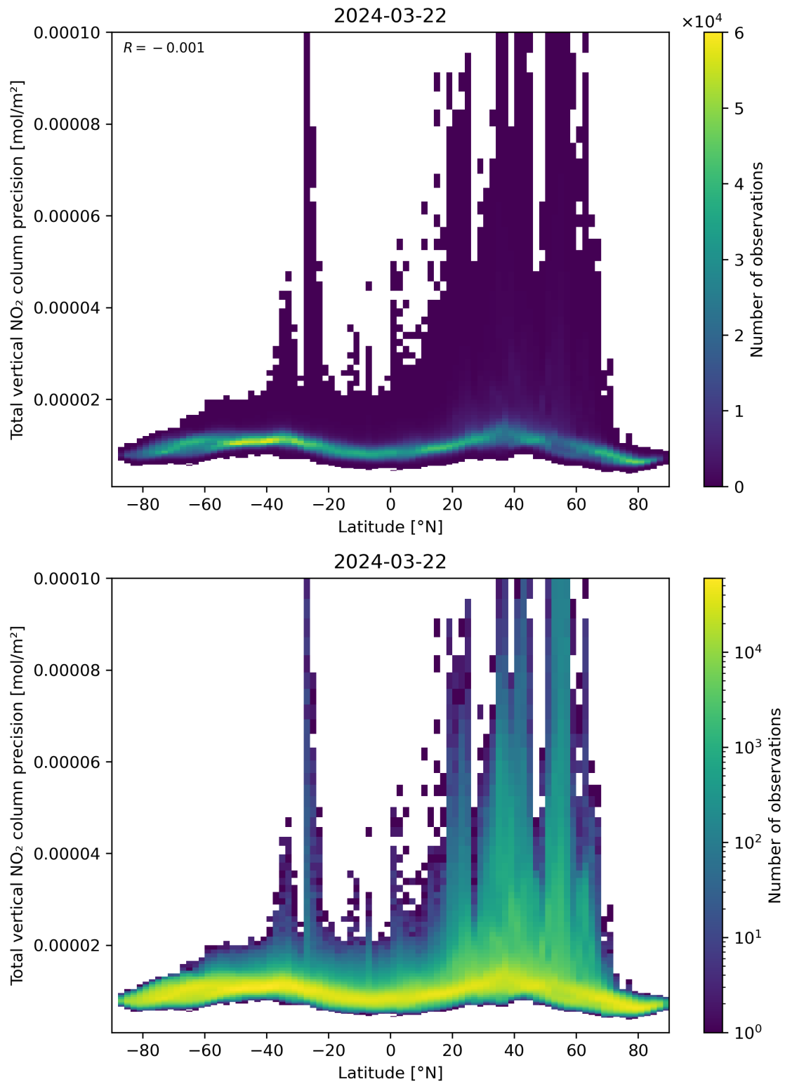
Figure 91: Scatter density plot of “Latitude” against “Total vertical NO 2 column precision” for 2024-03-21 to 2024-03-22.
