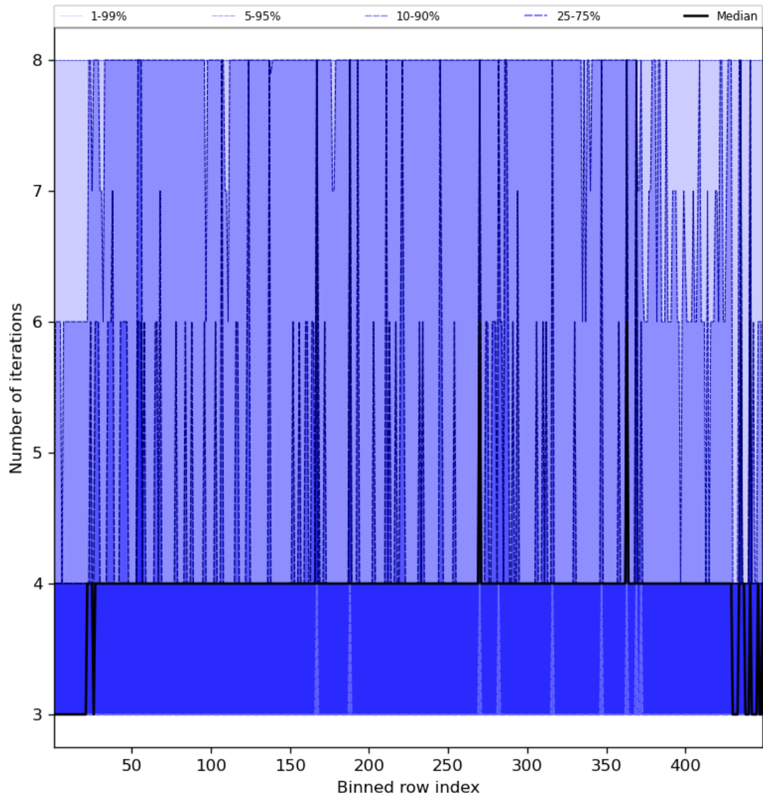
Figure 51: Along track statistics of “Number of iterations” for 2024-03-21 to 2024-03-22
