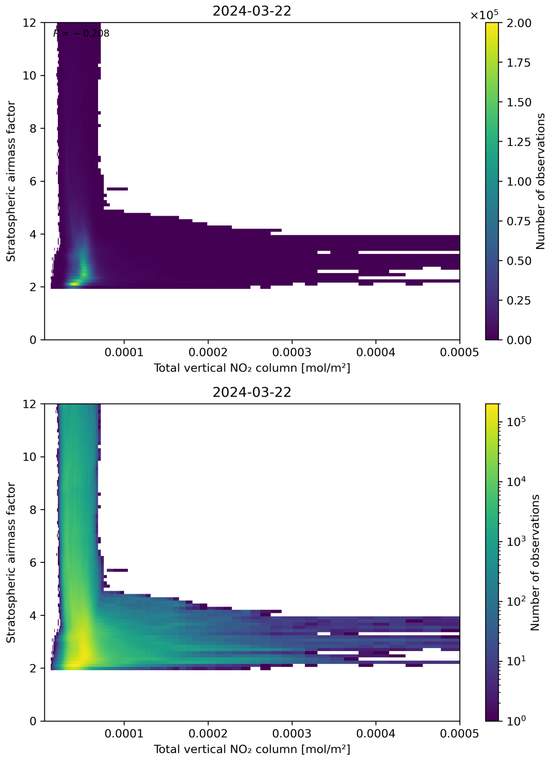
Figure 110: Scatter density plot of “Total vertical NO 2 column” against “Stratospheric airmass factor” for 2024-03-21 to 2024-03-22.
