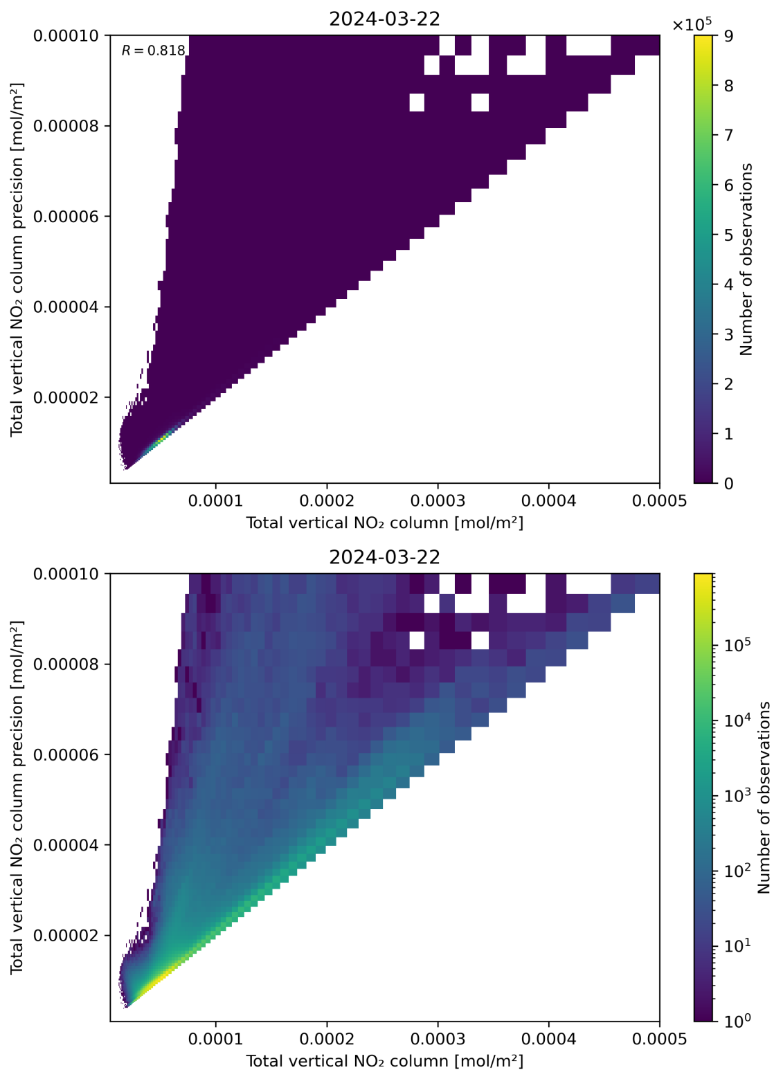
Figure 114: Scatter density plot of “Total vertical NO 2 column” against “Total vertical NO 2 column precision” for 2024-03-21 to 2024-03-22.
