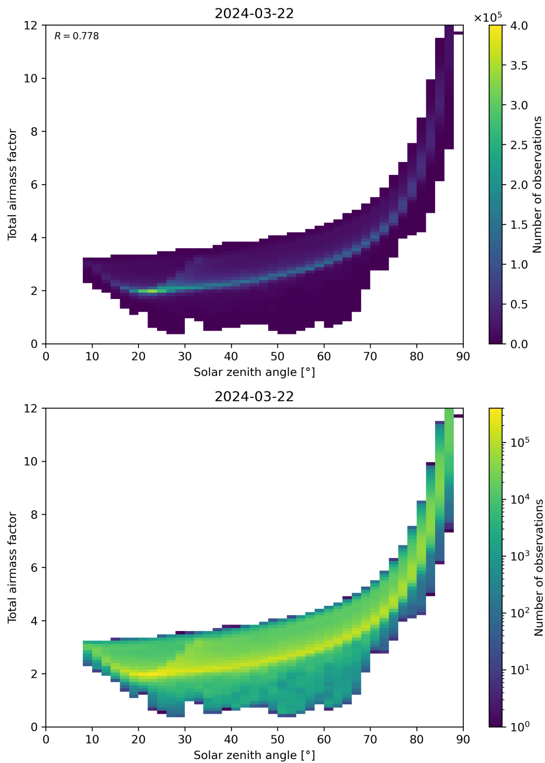
Figure 146: Scatter density plot of “Solar zenith angle” against “Total air mass factor” for 2024-03-21 to 2024-03-22.
