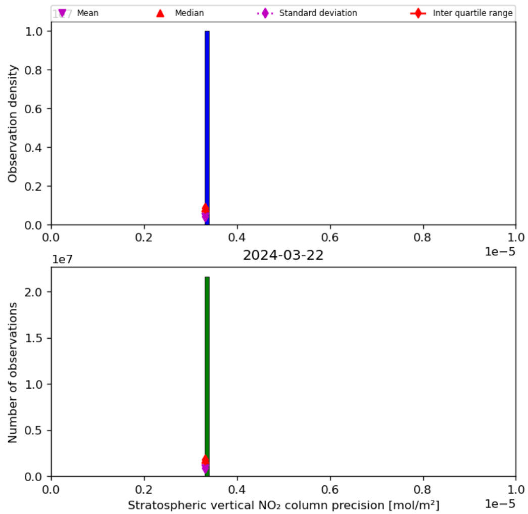
Figure 37: Histogram of “Stratospheric vertical NO 2 column precision” for 2024-03-21 to 2024-03-22
