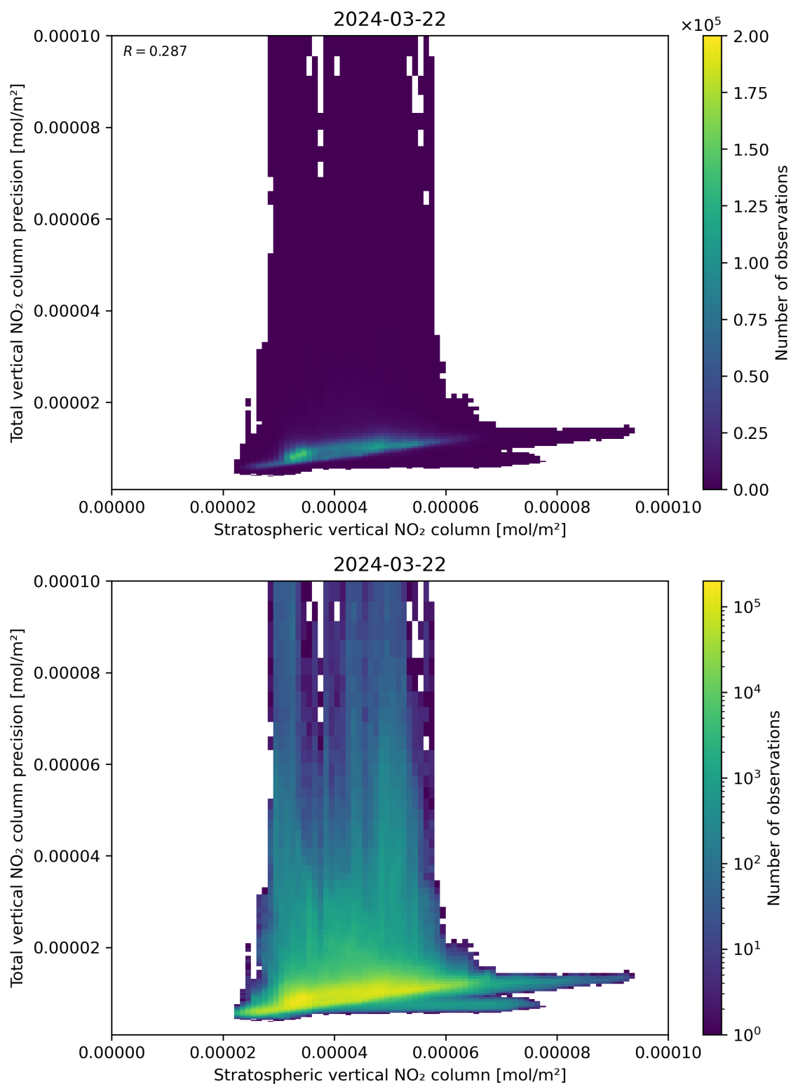
Figure 101: Scatter density plot of “Stratospheric vertical NO 2 column” against “Total vertical NO 2 column precision” for 2024-03-21 to 2024-03-22.
