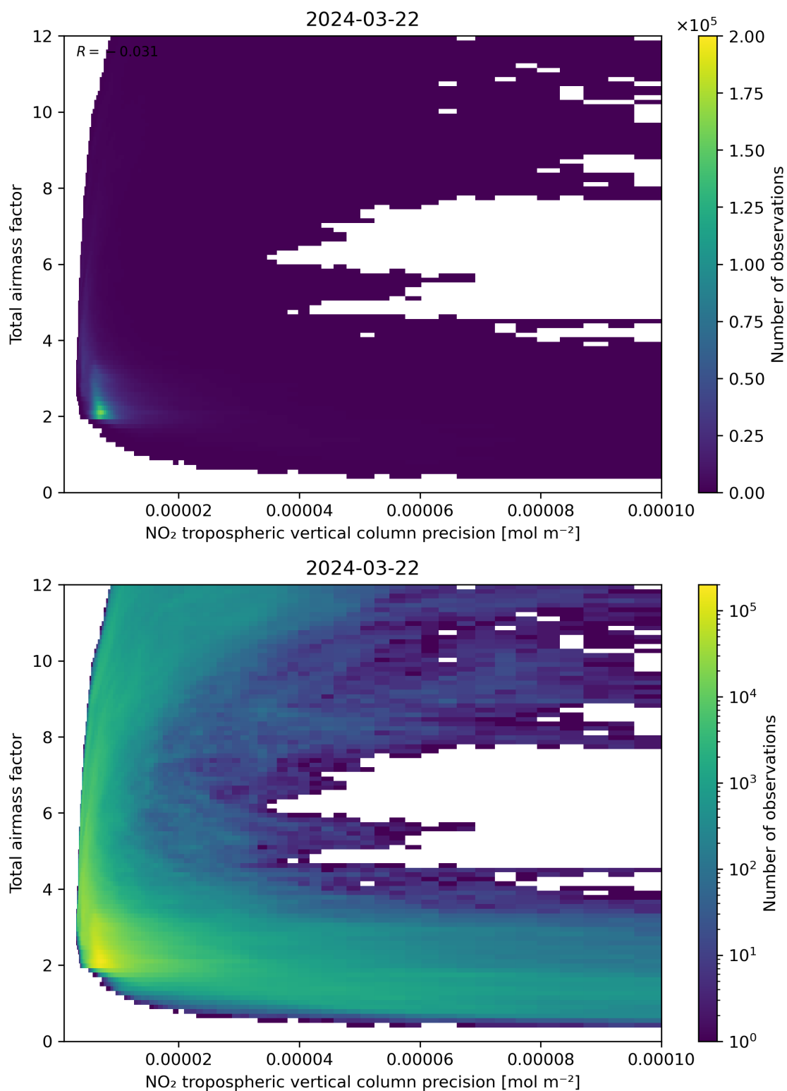
Figure 132: Scatter density plot of “NO 2 tropospheric vertical column precision” against “Total air mass factor” for 2024-03-21 to 2024-03-22.
