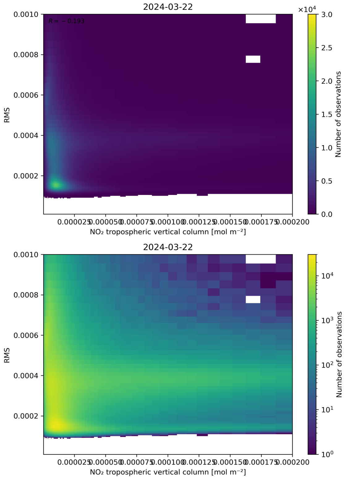
Figure 142: Scatter density plot of “NO 2 tropospheric vertical column” against “RMS” for 2024-03-21 to 2024-03-22.
