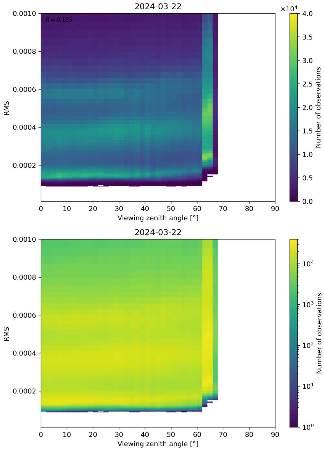
Figure 171: Scatter density plot of “Viewing zenith angle” against “RMS” for 2024-03-21 to 2024-03-22.
