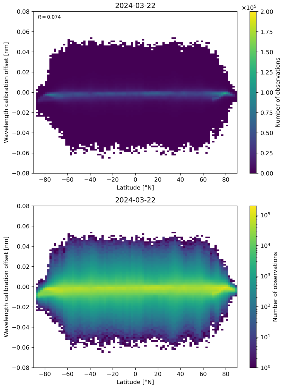
Figure 95: Scatter density plot of “Latitude” against “Wavelength calibration offset” for 2024-03-21 to 2024-03-22.
