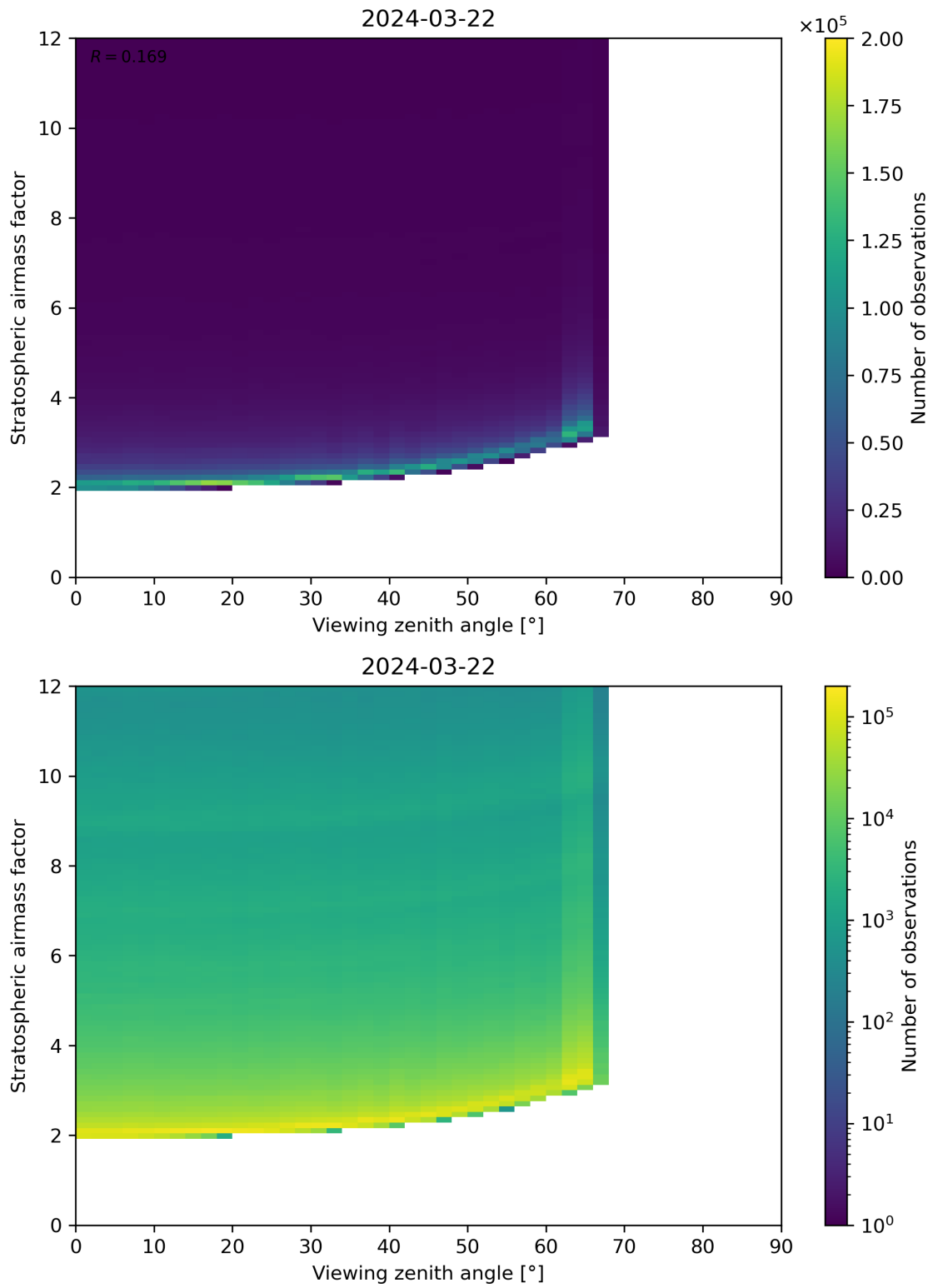
Figure 159: Scatter density plot of “Viewing zenith angle” against “Stratospheric airmass factor” for 2024-03-21 to 2024-03-22.
