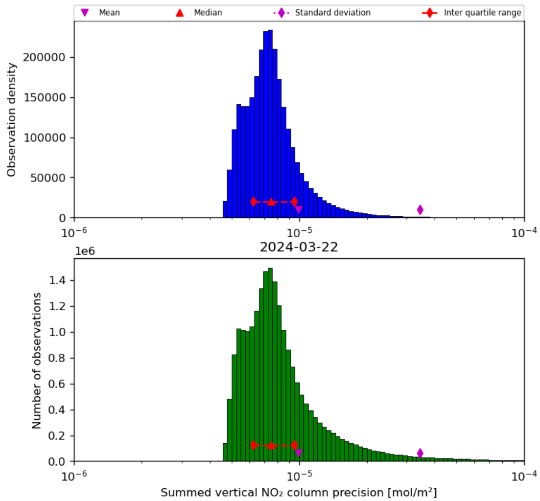
Figure 41: Histogram of "Summed vertical NO 2 column precision" for 2024-03-21 to 2024-03-22
