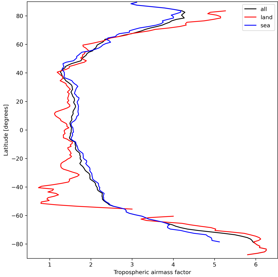
Figure 14: Zonal average of “Tropospheric airmass factor” for 2024-03-21 to 2024-03-22.
