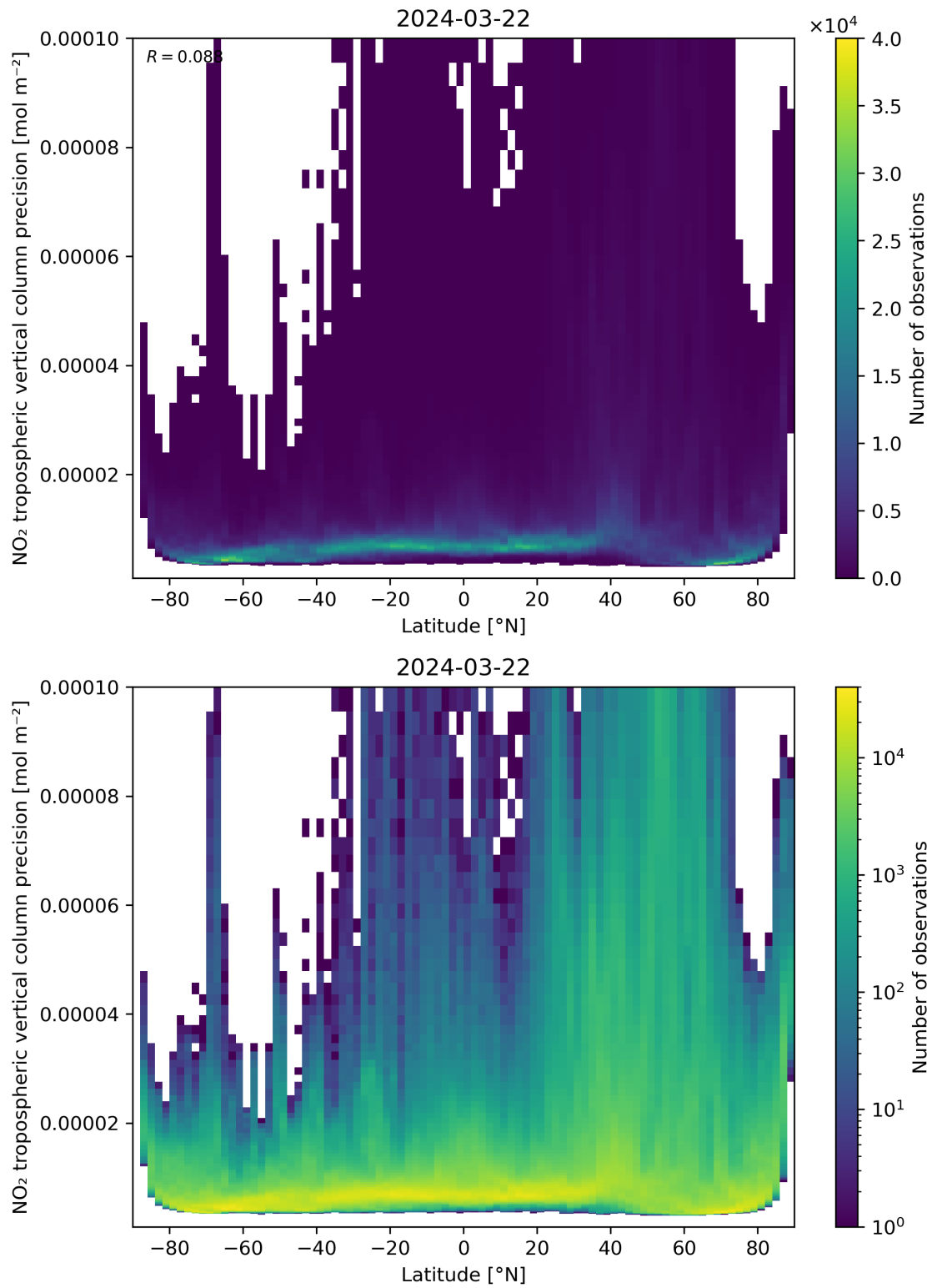
Figure 93: Scatter density plot of “Latitude” against “NO 2 tropospheric vertical column precision” for 2024-03-21 to 2024-03-22.
