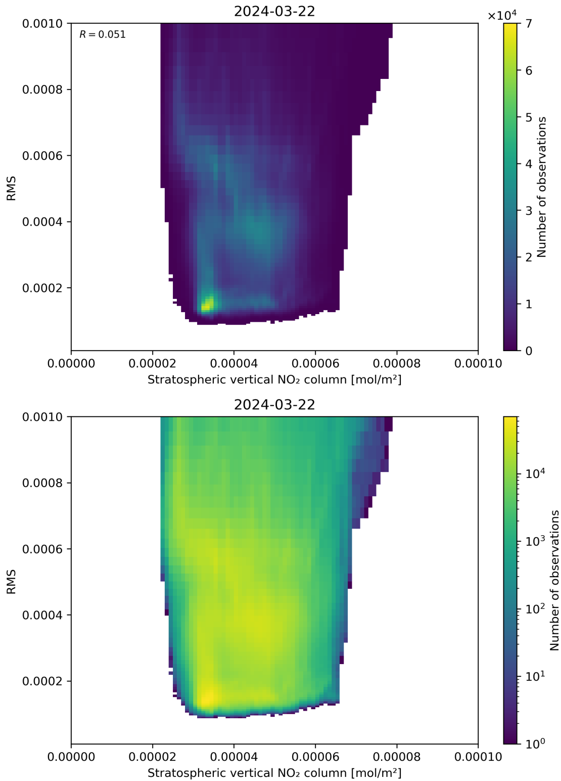
Figure 102: Scatter density plot of “Stratospheric vertical NO 2 column” against “RMS” for 2024-03-21 to 2024-03-22.
