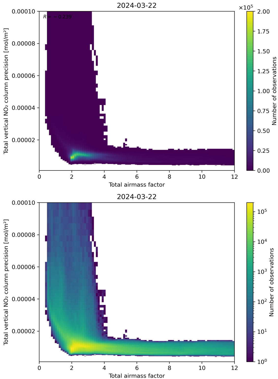
Figure 68: Scatter density plot of “Total airmass factor” against “Total vertical NO 2 column precision” for 2024-03-21 to 2024-03-22.
