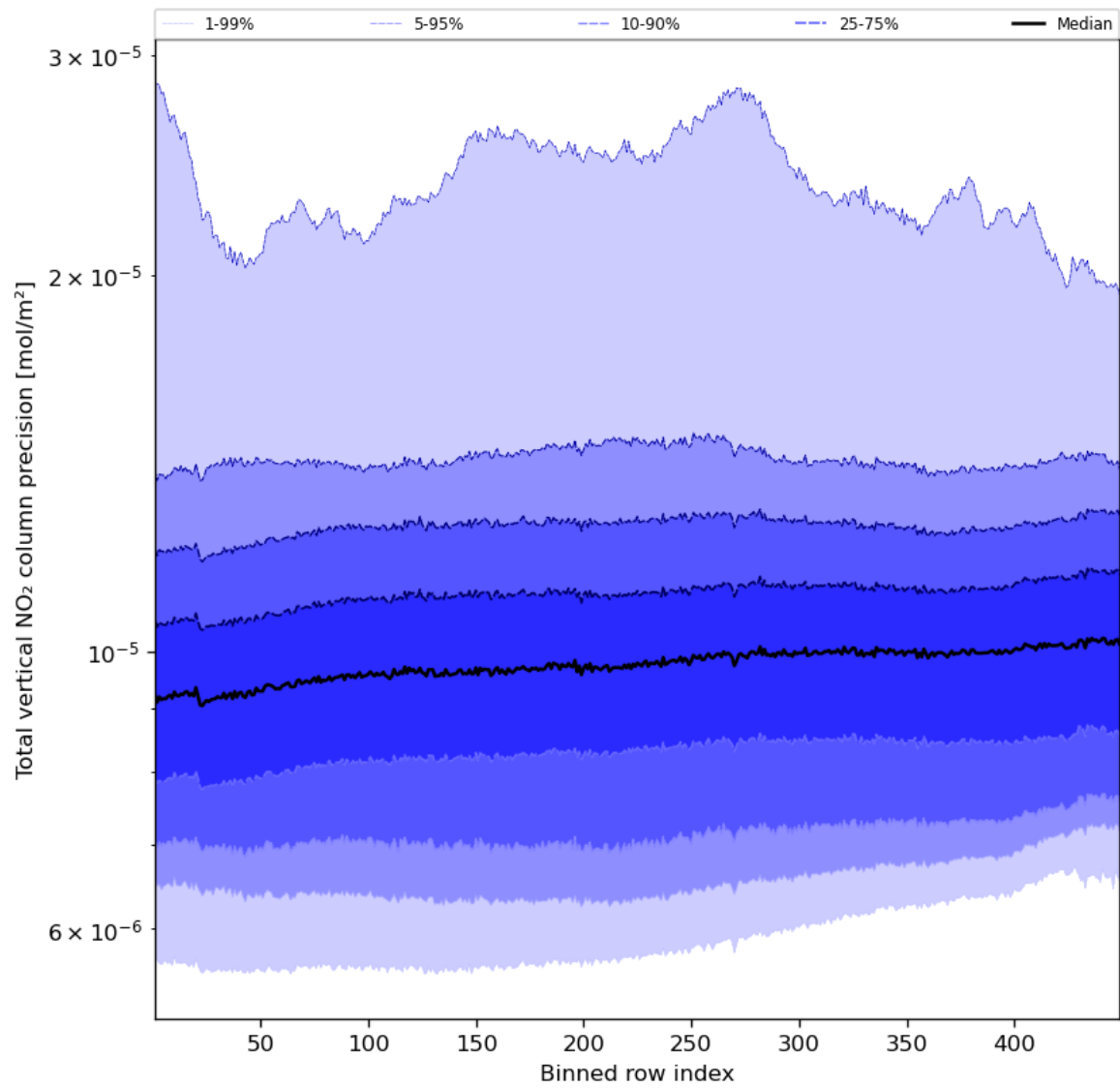
Figure 56: Along track statistics of “Total vertical NO 2 column precision” for 2024-03-21 to 2024-03-22
