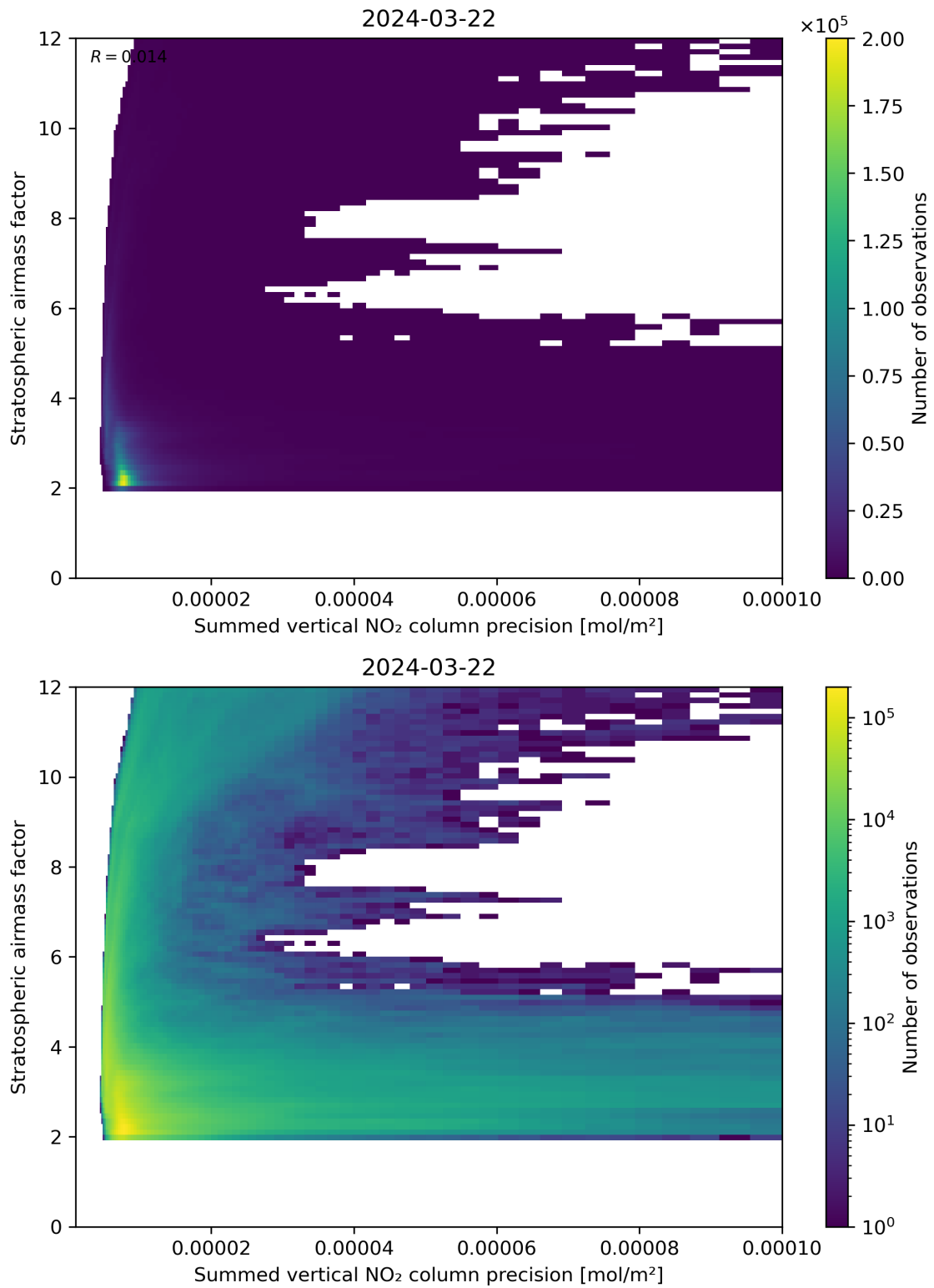
Figure 106: Scatter density plot of “Summed vertical NO 2 column precision” against “Stratospheric airmass factor” for 2024-03-21 to 2024-03-22.
