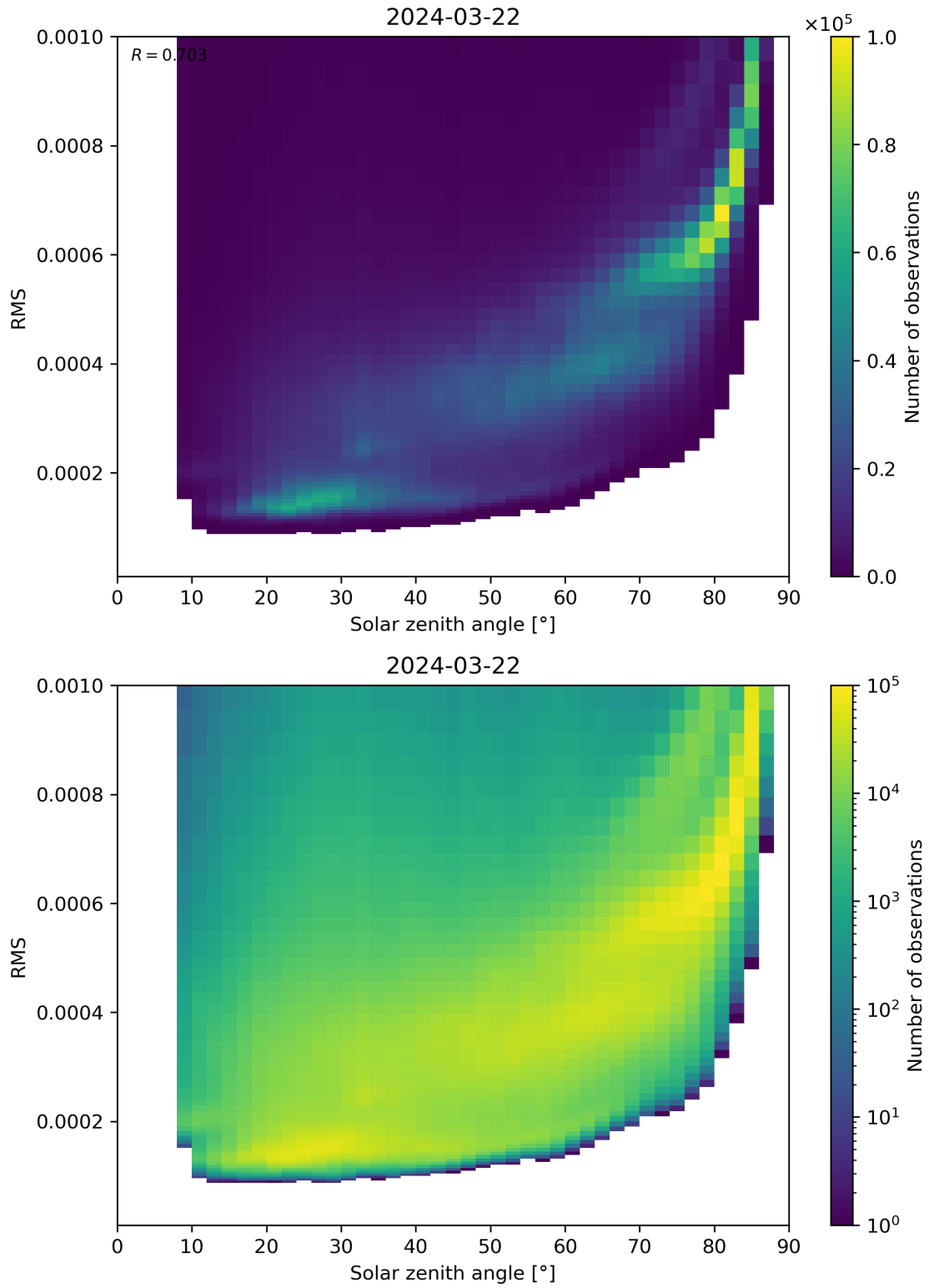
Figure 157: Scatter density plot of “Solar zenith angle” against “RMS” for 2024-03-21 to 2024-03-22.
