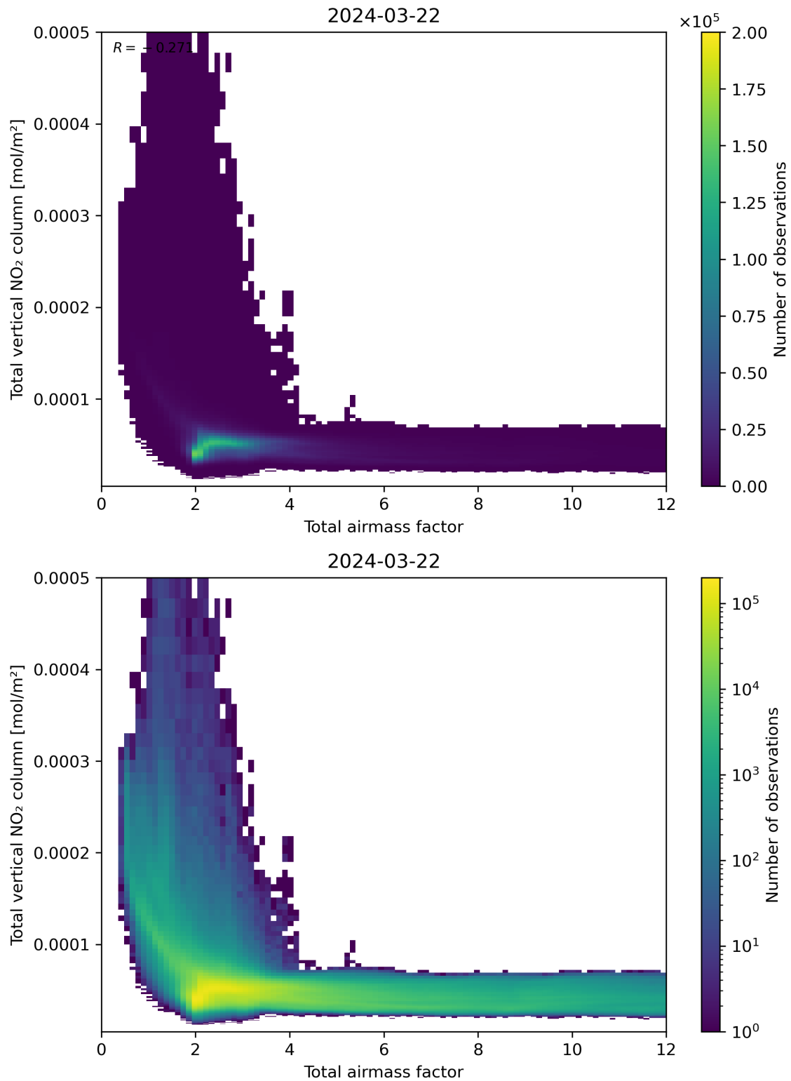
Figure 67: Scatter density plot of “Total airmass factor” against “Total vertical NO 2 column” for 2024-03-21 to 2024-03-22.
