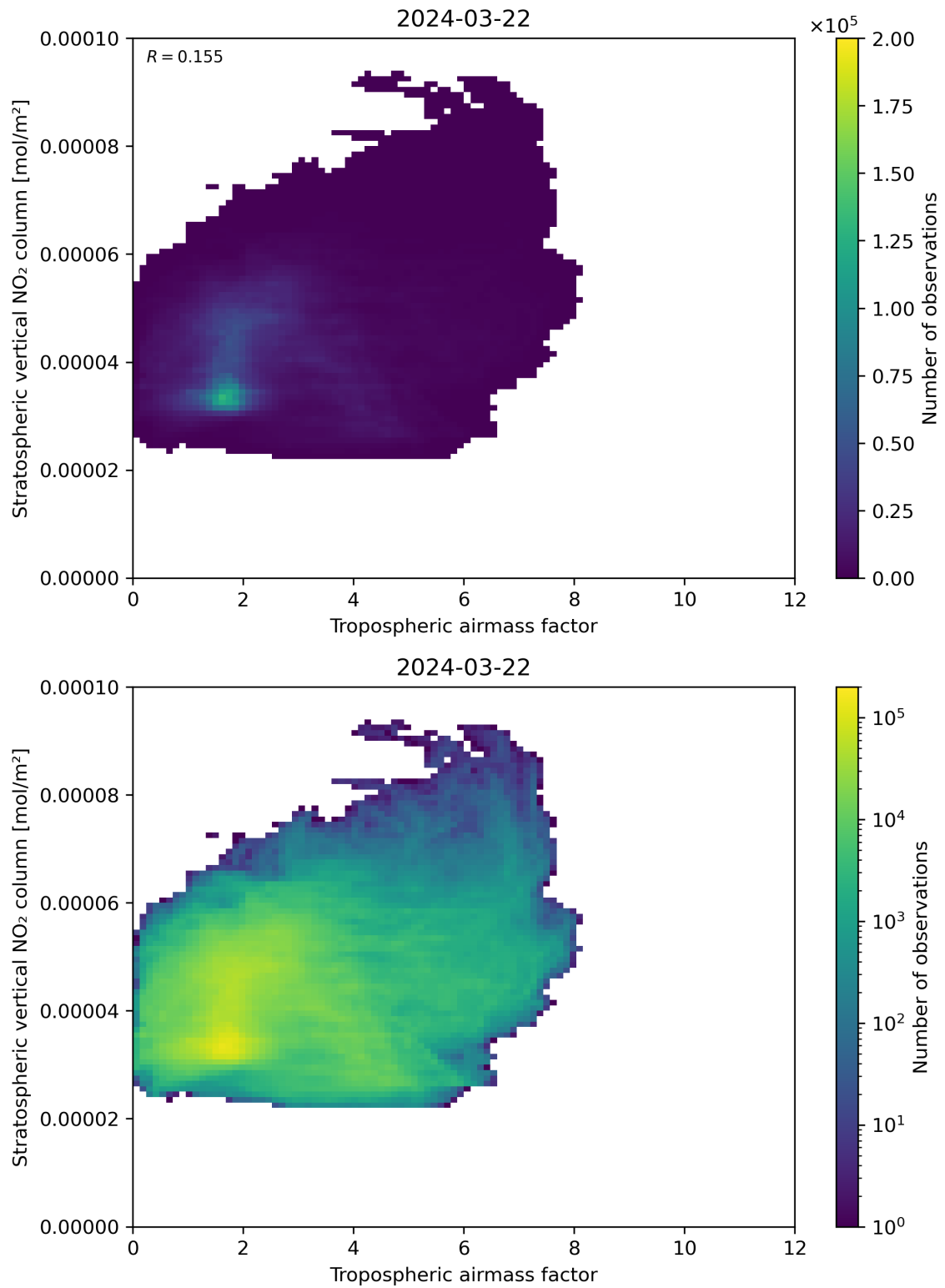
Figure 74: Scatter density plot of “Tropospheric air mass factor” against “Stratospheric vertical NO 2 column” for 2024-03-21 to 2024-03-22.
