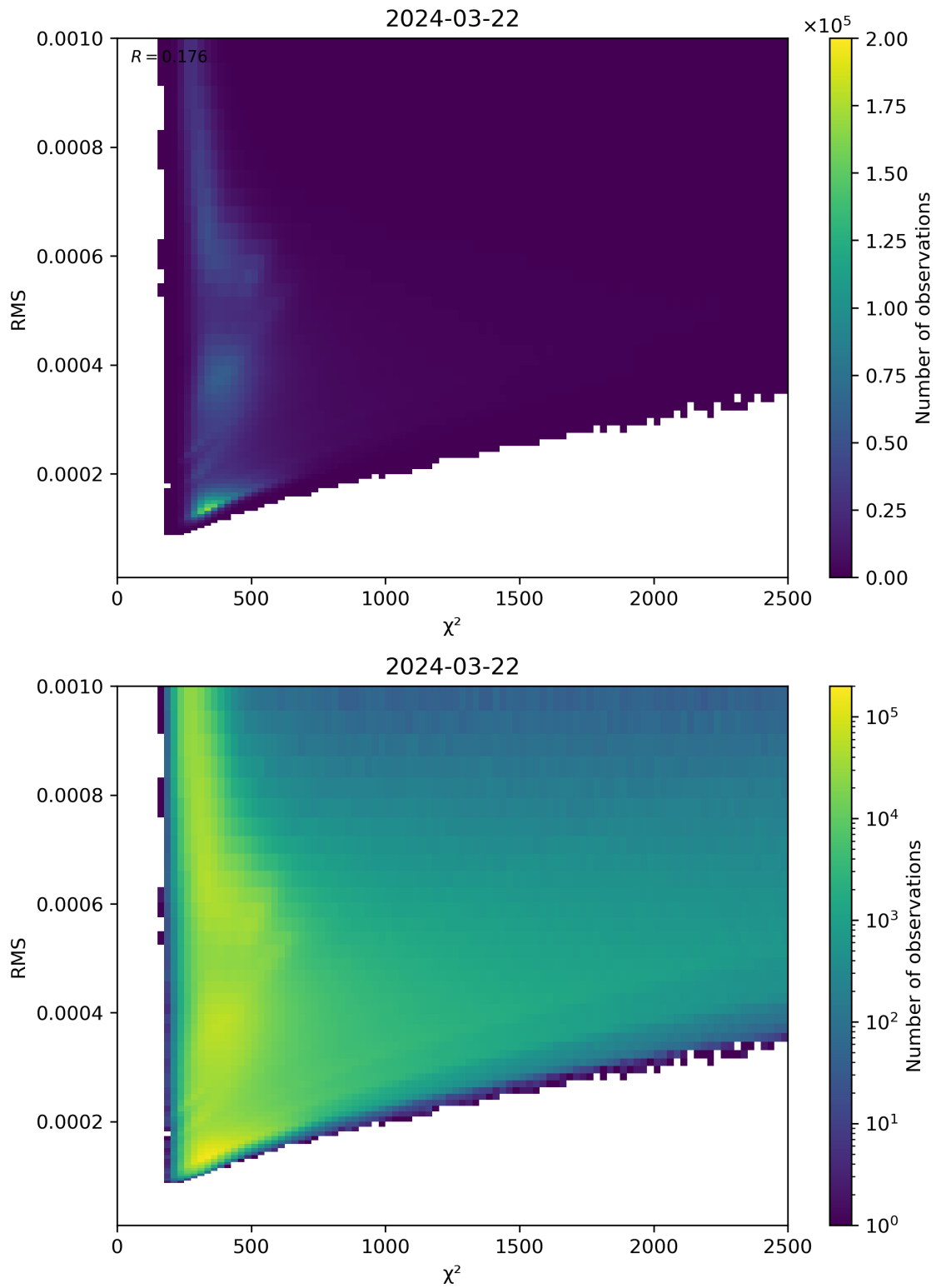
Figure 82: Scatter density plot of “ \chi^2 ” against “RMS” for 2024-03-21 to 2024-03-22.
