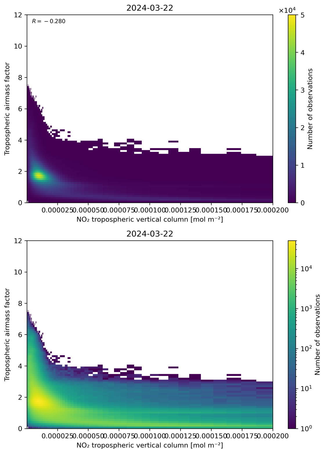
Figure 123: Scatter density plot of “NO 2 tropospheric vertical column” against “Tropospheric air mass factor” for 2024-03-21 to 2024-03-22.
