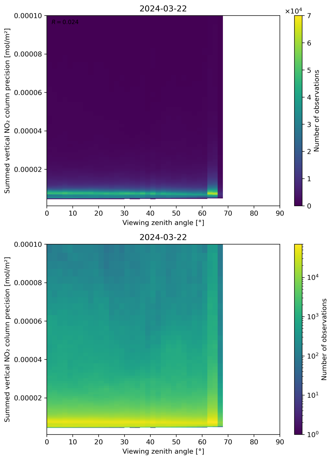
Figure 166: Scatter density plot of “Viewing zenith angle” against “Summed vertical NO 2 column precision” for 2024-03-21 to 2024-03-22.
