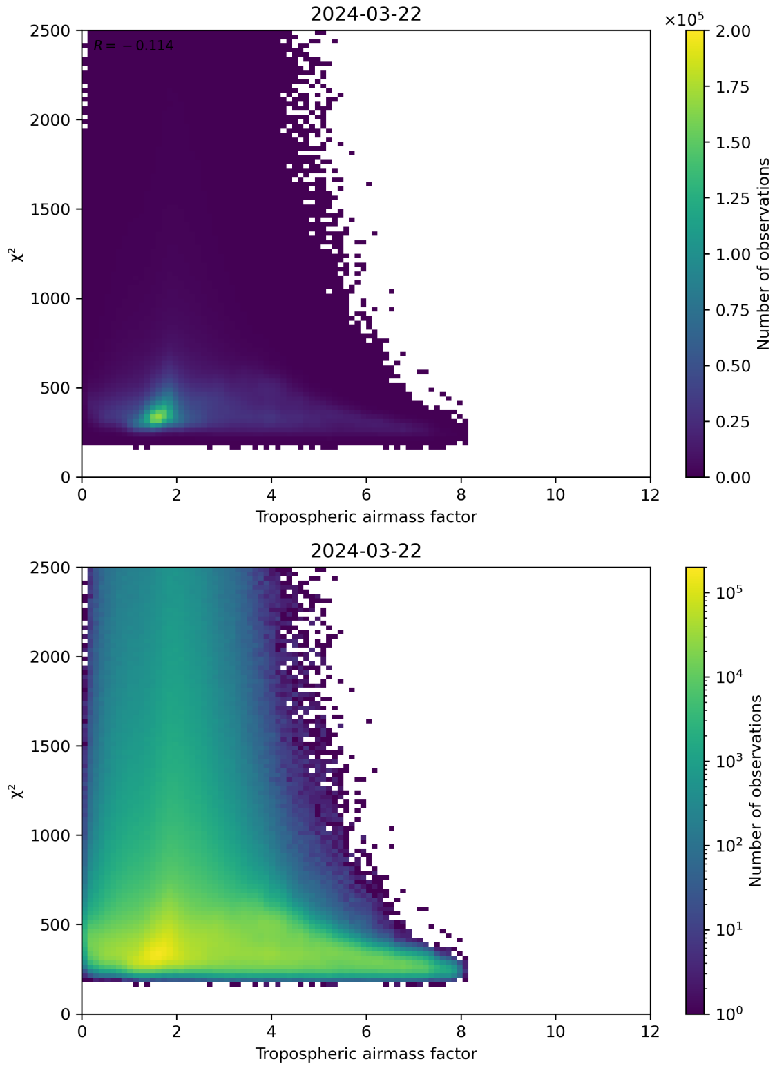
Figure 73: Scatter density plot of “Tropospheric airmass factor” against “ \chi^2 ” for 2024-03-21 to 2024-03-22.
