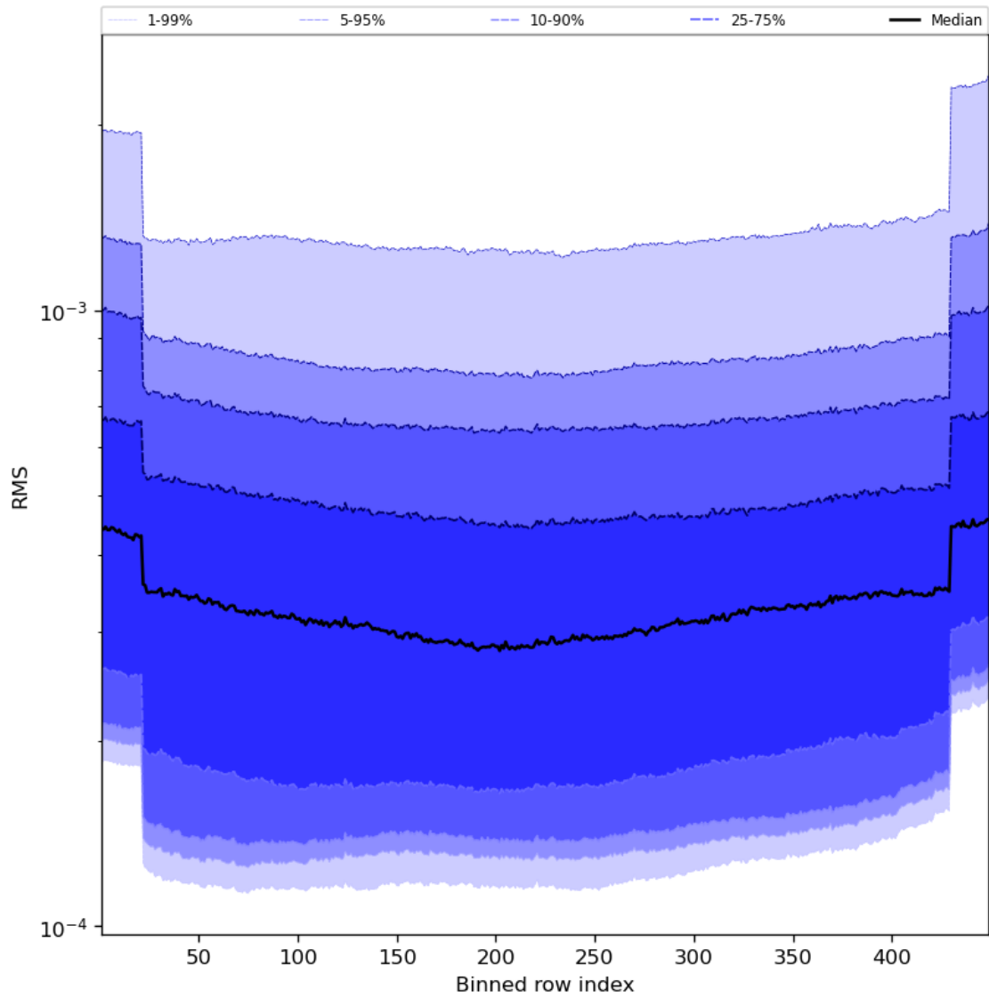
Figure 60: Along track statistics of “RMS” for 2024-03-21 to 2024-03-22
