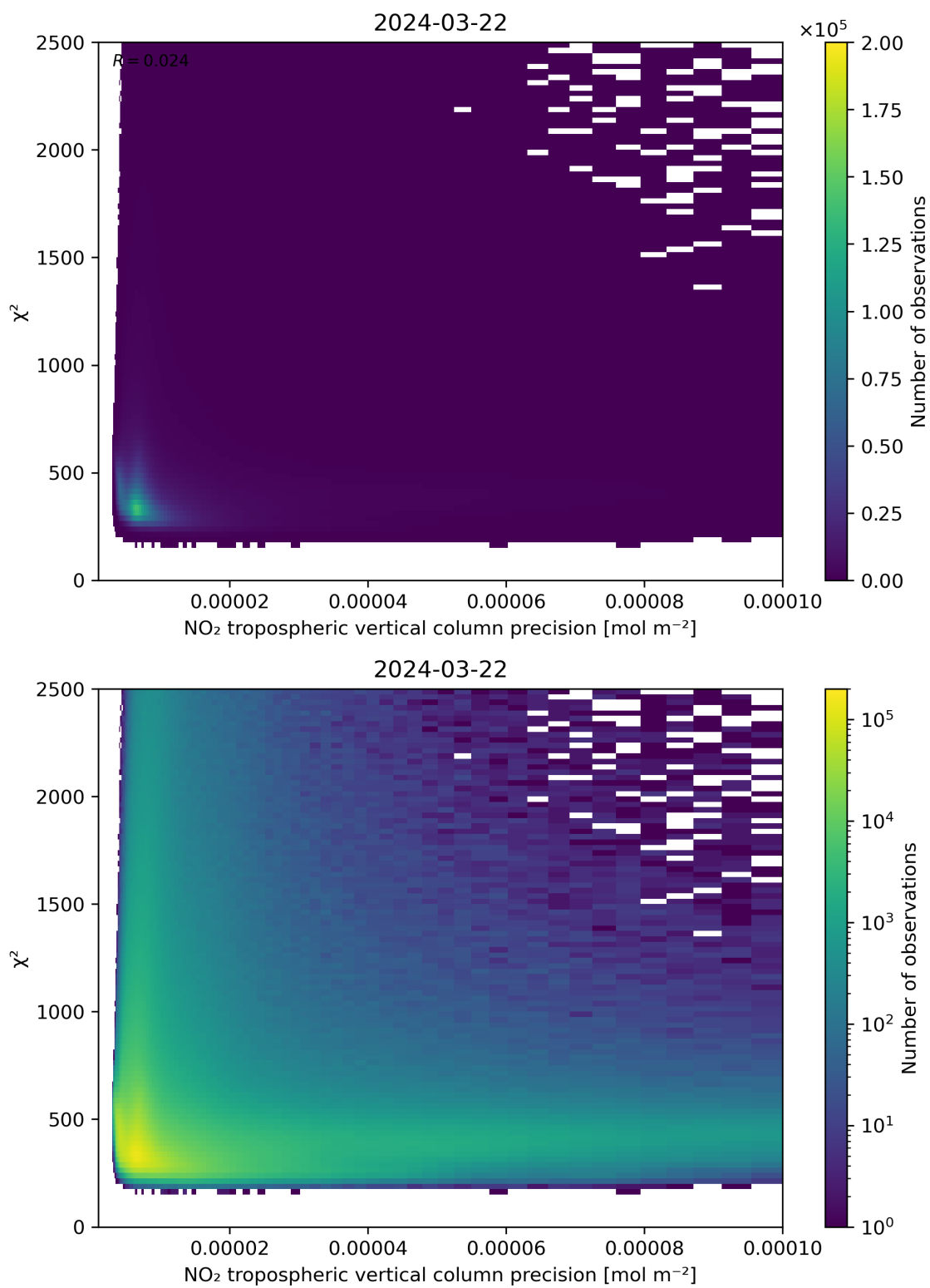
Figure 134: Scatter density plot of “NO 2 tropospheric vertical column precision” against “ \chi^2 ” for 2024-03-21 to 2024-03-22.
