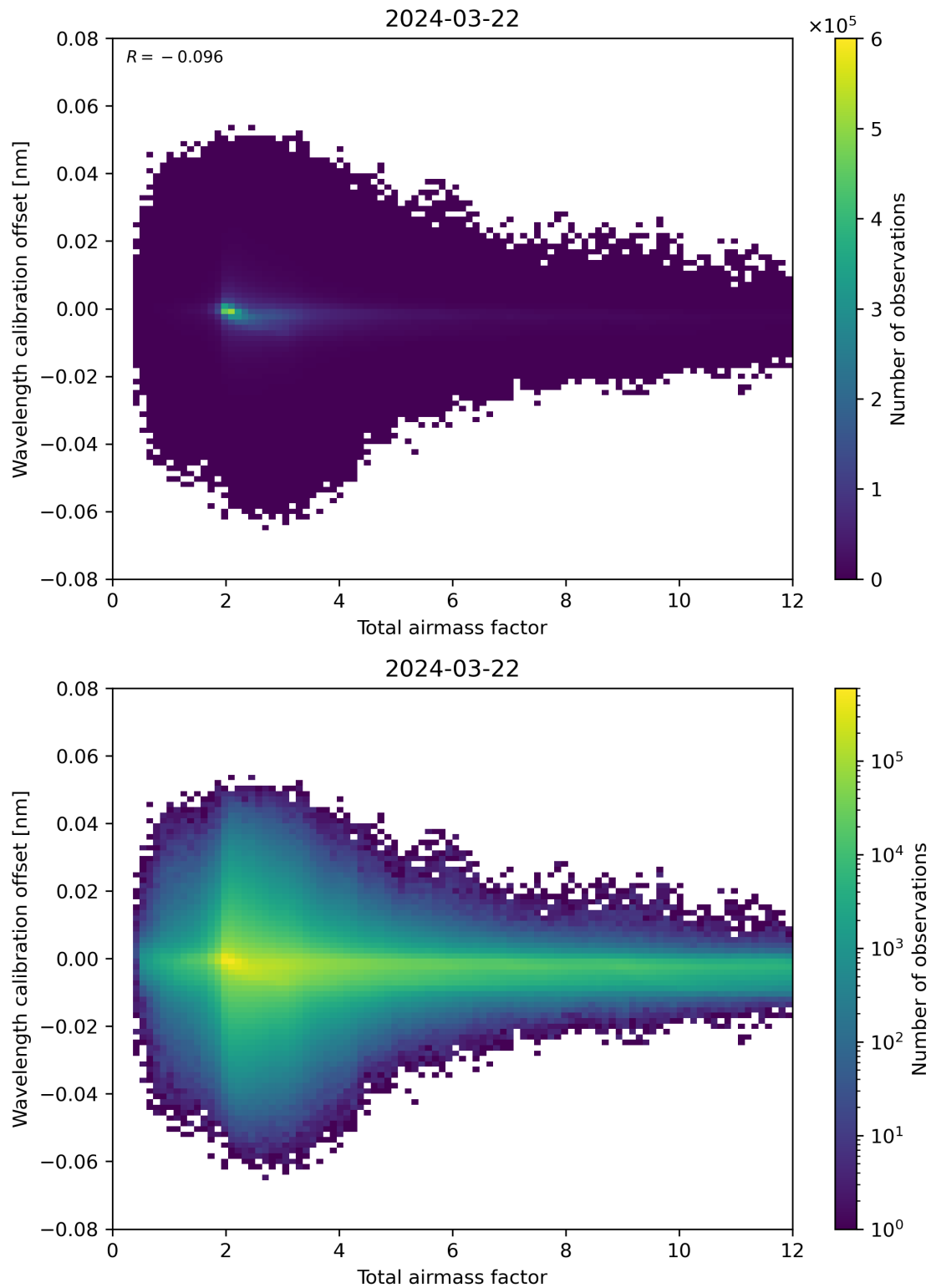
Figure 70: Scatter density plot of “Total airmass factor” against “Wavelength calibration offset” for 2024-03-21 to 2024-03-22.
