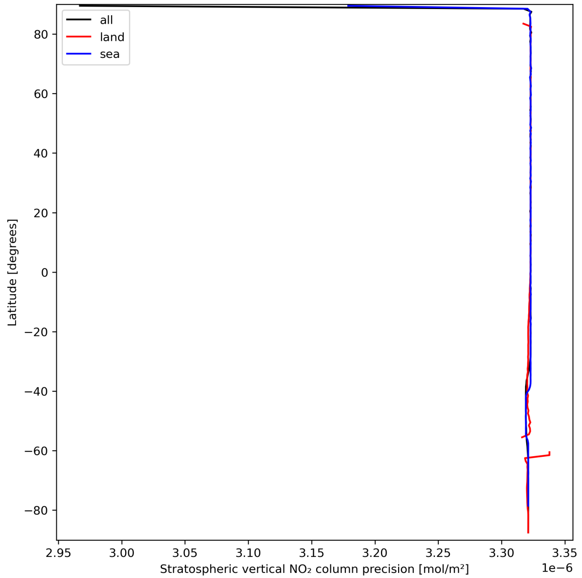
Figure 20: Zonal average of “Stratospheric vertical NO 2 column precision” for 2024-03-21 to 2024-03-22.
