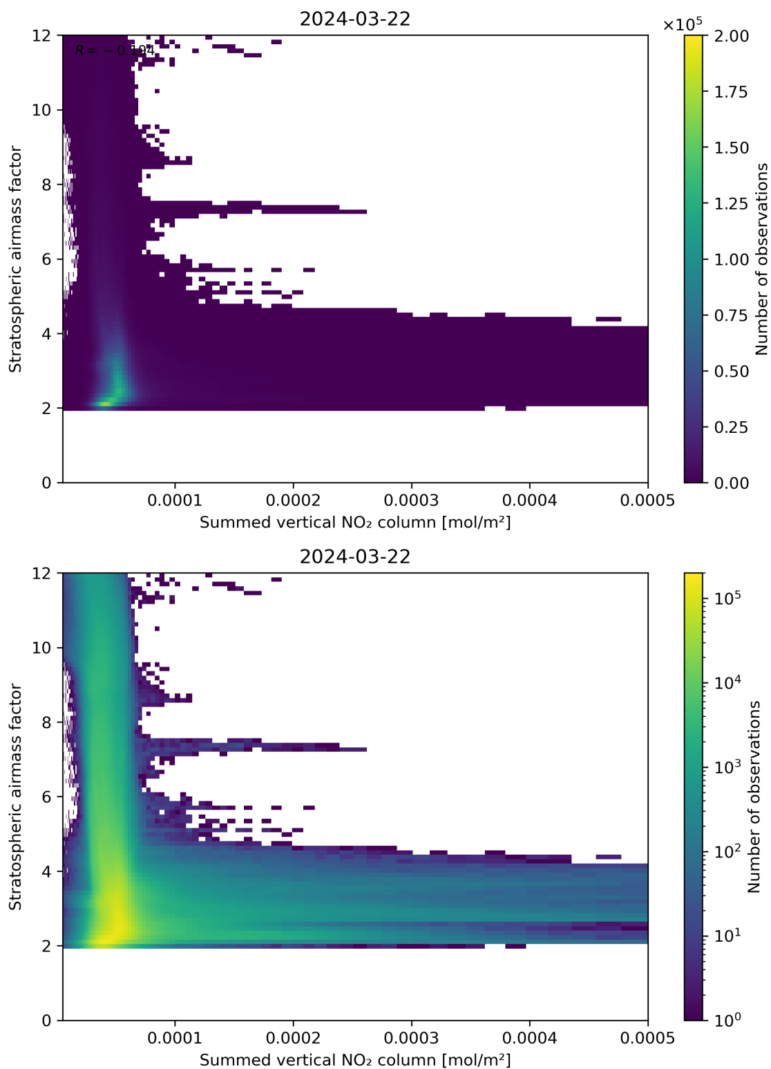
Figure 103: Scatter density plot of “Summed vertical NO 2 column” against “Stratospheric air mass factor” for 2024-03-21 to 2024-03-22.
