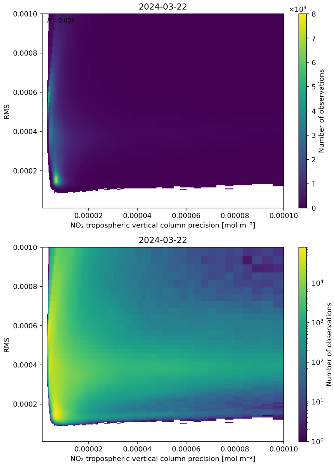
Figure 140: Scatter density plot of “NO 2 tropospheric vertical column precision” against “RMS” for 2024-03-21 to 2024-03-22.
