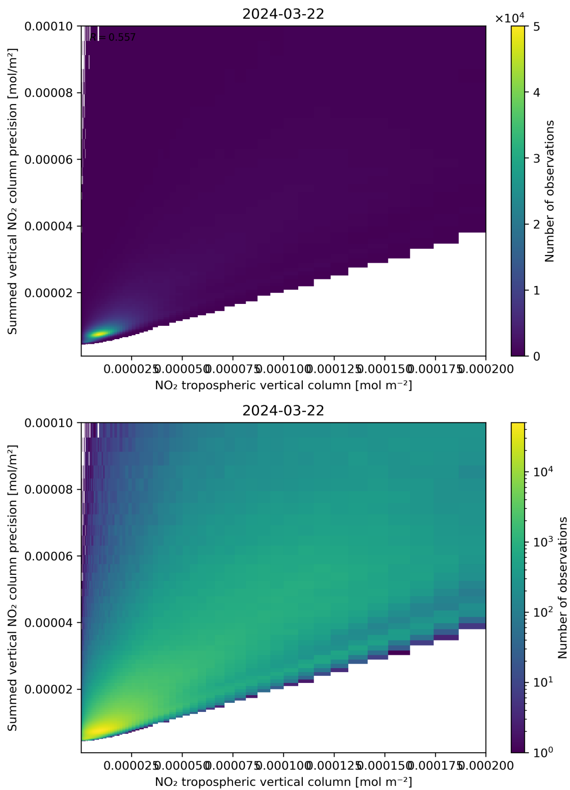
Figure 127: Scatter density plot of “NO 2 tropospheric vertical column” against “Summed vertical NO 2 column precision” for 2024-03-21 to 2024-03-22.
