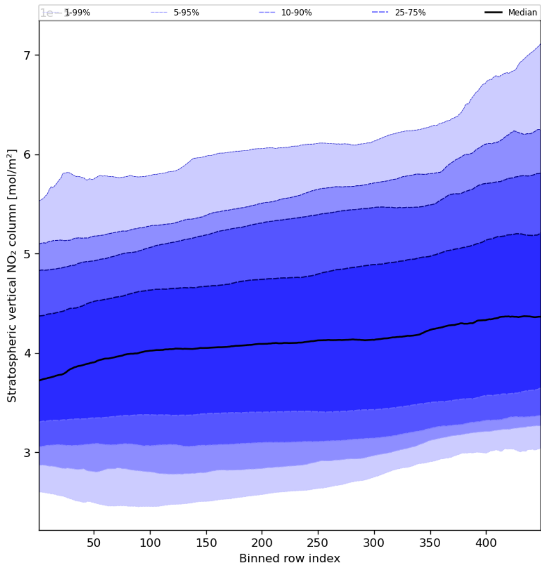
Figure 53: Along track statistics of “Stratospheric vertical NO 2 column” for 2024-03-21 to 2024-03-22
