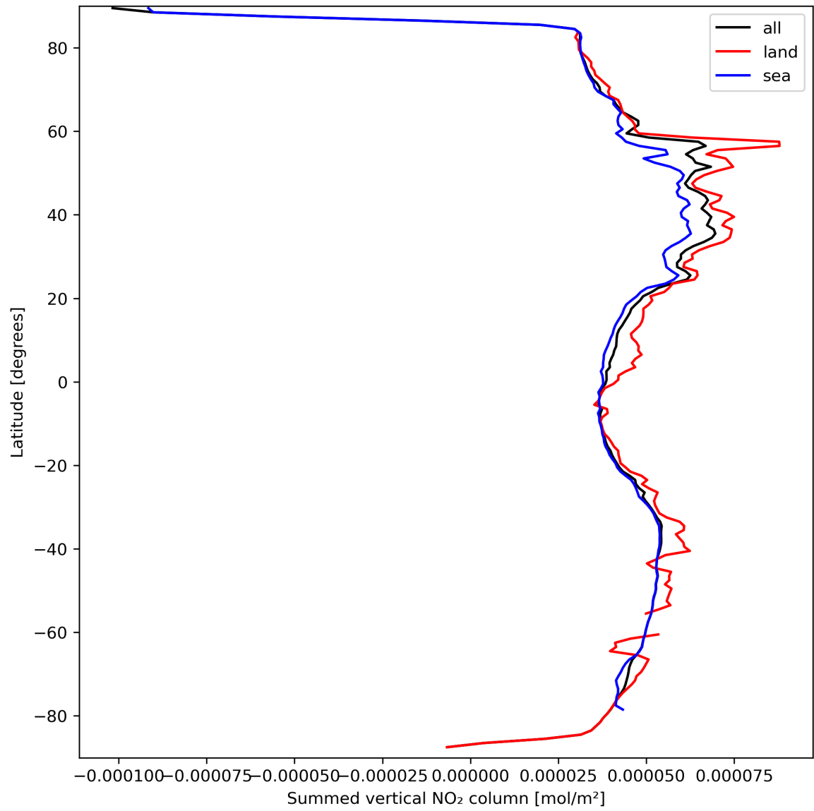
Figure 23: Zonal average of “Summed vertical NO 2 column” for 2024-03-21 to 2024-03-22.
