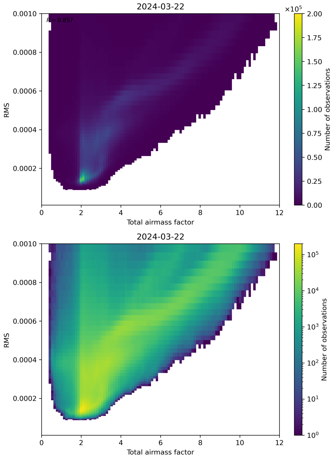
Figure 69: Scatter density plot of “Total airmass factor” against “RMS” for 2024-03-21 to 2024-03-22.
