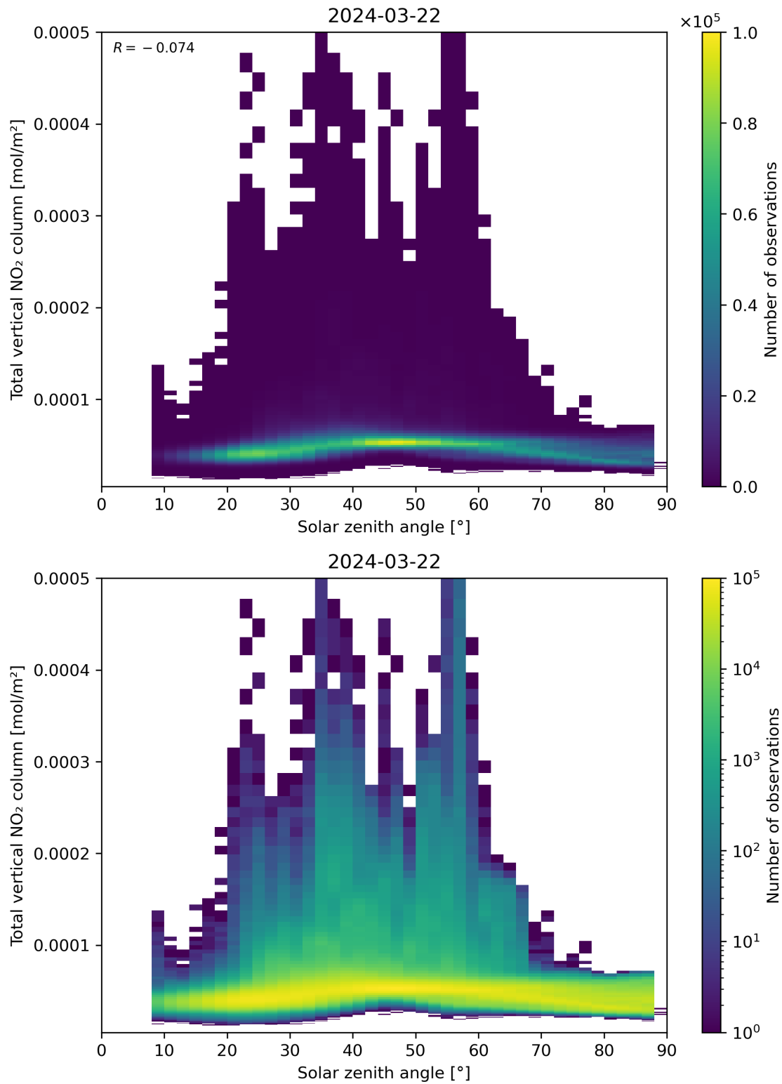
Figure 153: Scatter density plot of “Solar zenith angle” against “Total vertical NO 2 column” for 2024-03-21 to 2024-03-22.
