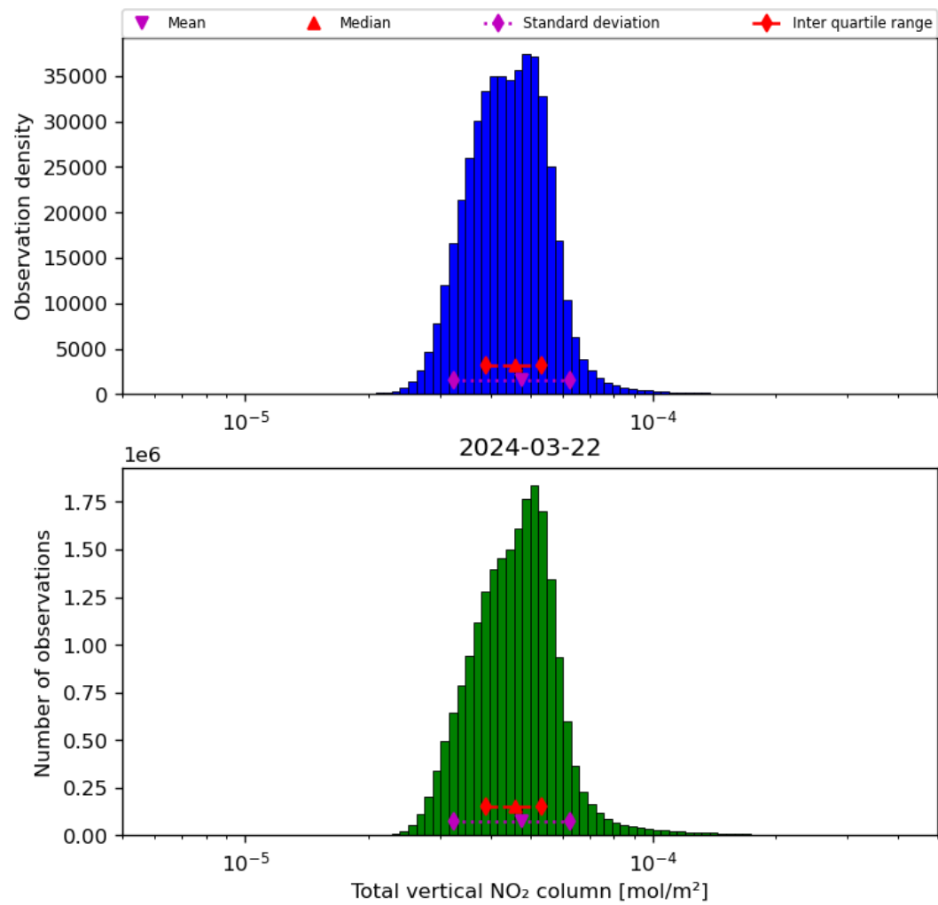
Figure 38: Histogram of “Total vertical NO 2 column” for 2024-03-21 to 2024-03-22
