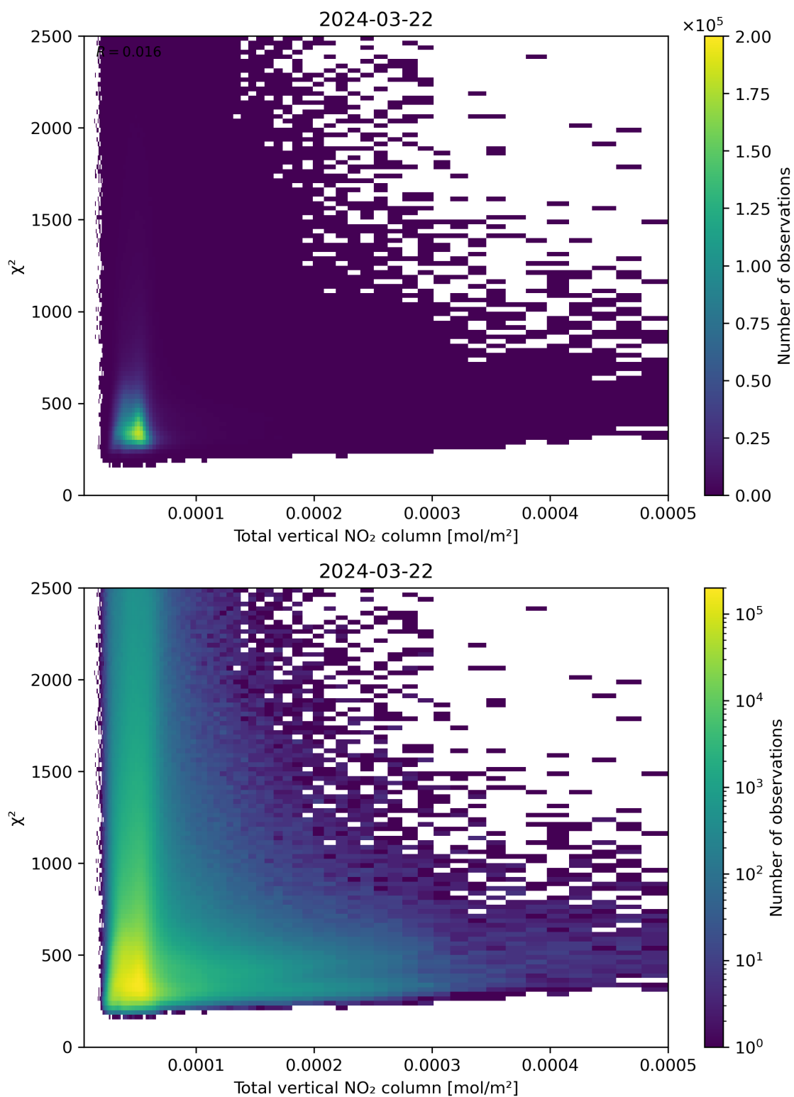
Figure 111: Scatter density plot of “Total vertical NO 2 column” against “ \chi^2 ” for 2024-03-21 to 2024-03-22.
