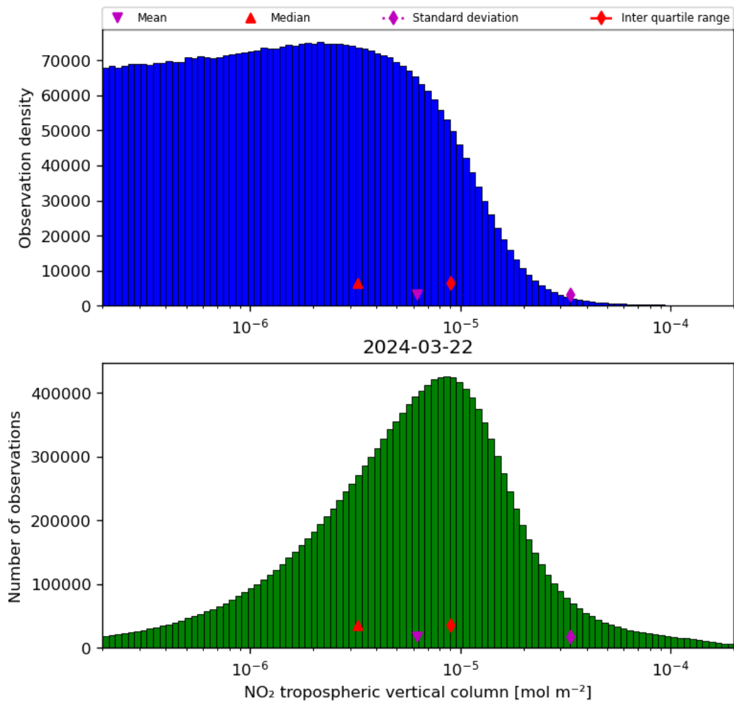
Figure 29: Histogram of “NO 2 tropospheric vertical column” for 2024-03-21 to 2024-03-22
