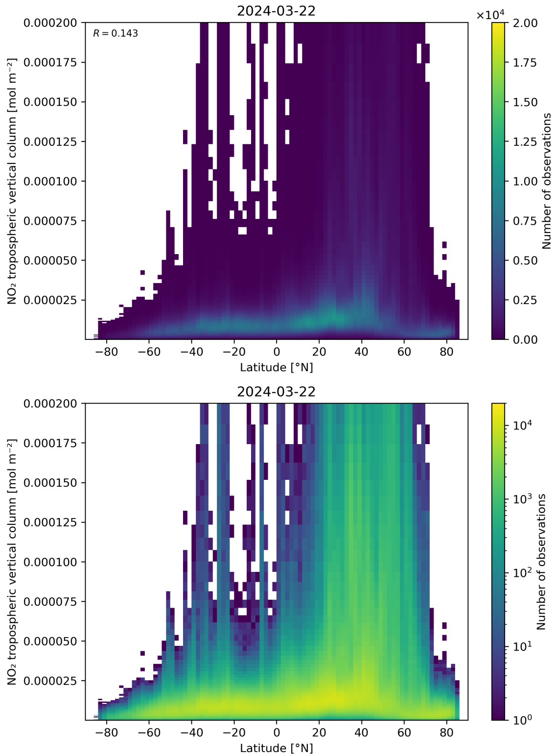
Figure 92: Scatter density plot of “Latitude” against “NO 2 tropospheric vertical column” for 2024-03-21 to 2024-03-22.
