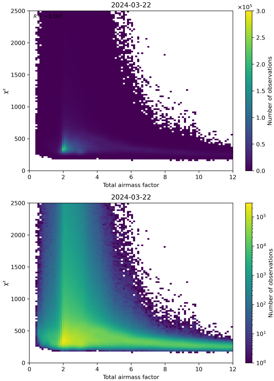
Figure 63: Scatter density plot of “Total airmass factor” against “ \chi^2 ” for 2024-03-21 to 2024-03-22.
