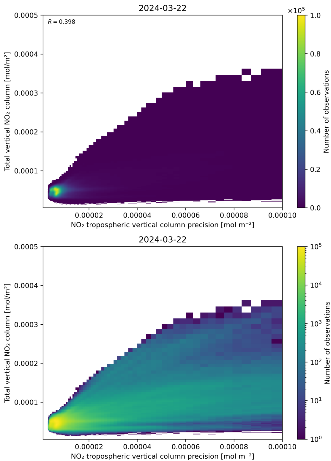
Figure 138: Scatter density plot of “NO 2 tropospheric vertical column precision” against “Total vertical NO 2 column” for 2024-03-21 to 2024-03-22.
