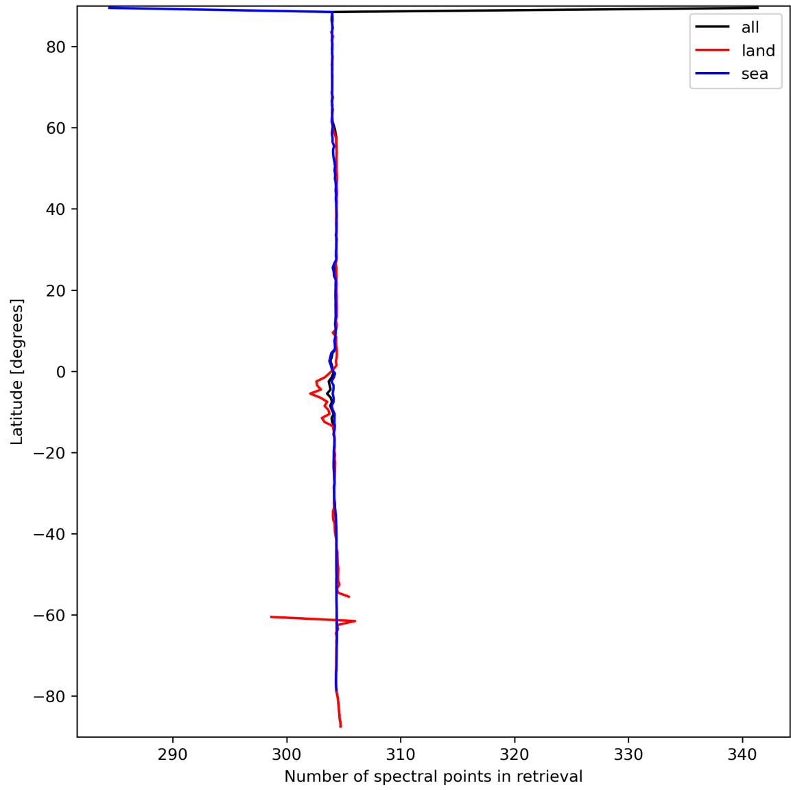
Figure 16: Zonal average of “Number of spectral points in retrieval” for 2024-03-21 to 2024-03-22.
