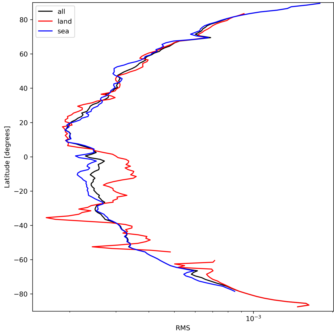
Figure 26: Zonal average of “RMS” for 2024-03-21 to 2024-03-22.
