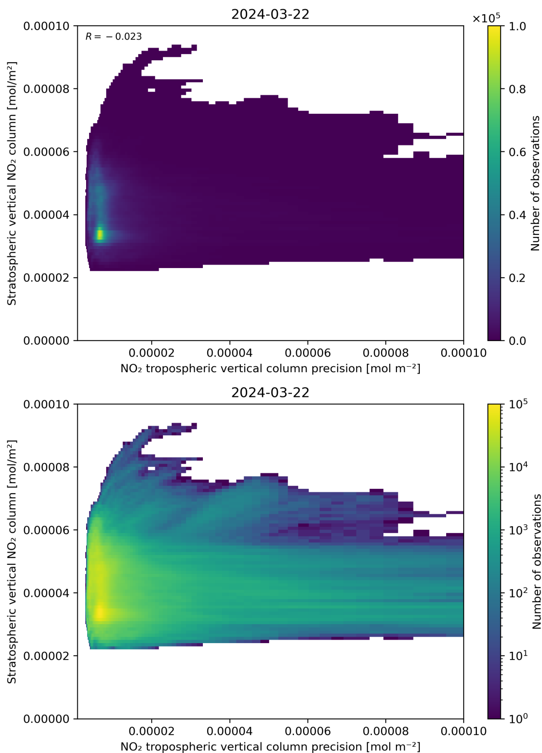
Figure 135: Scatter density plot of “NO 2 tropospheric vertical column precision” against “Stratospheric vertical NO 2 column” for 2024-03-21 to 2024-03-22.
