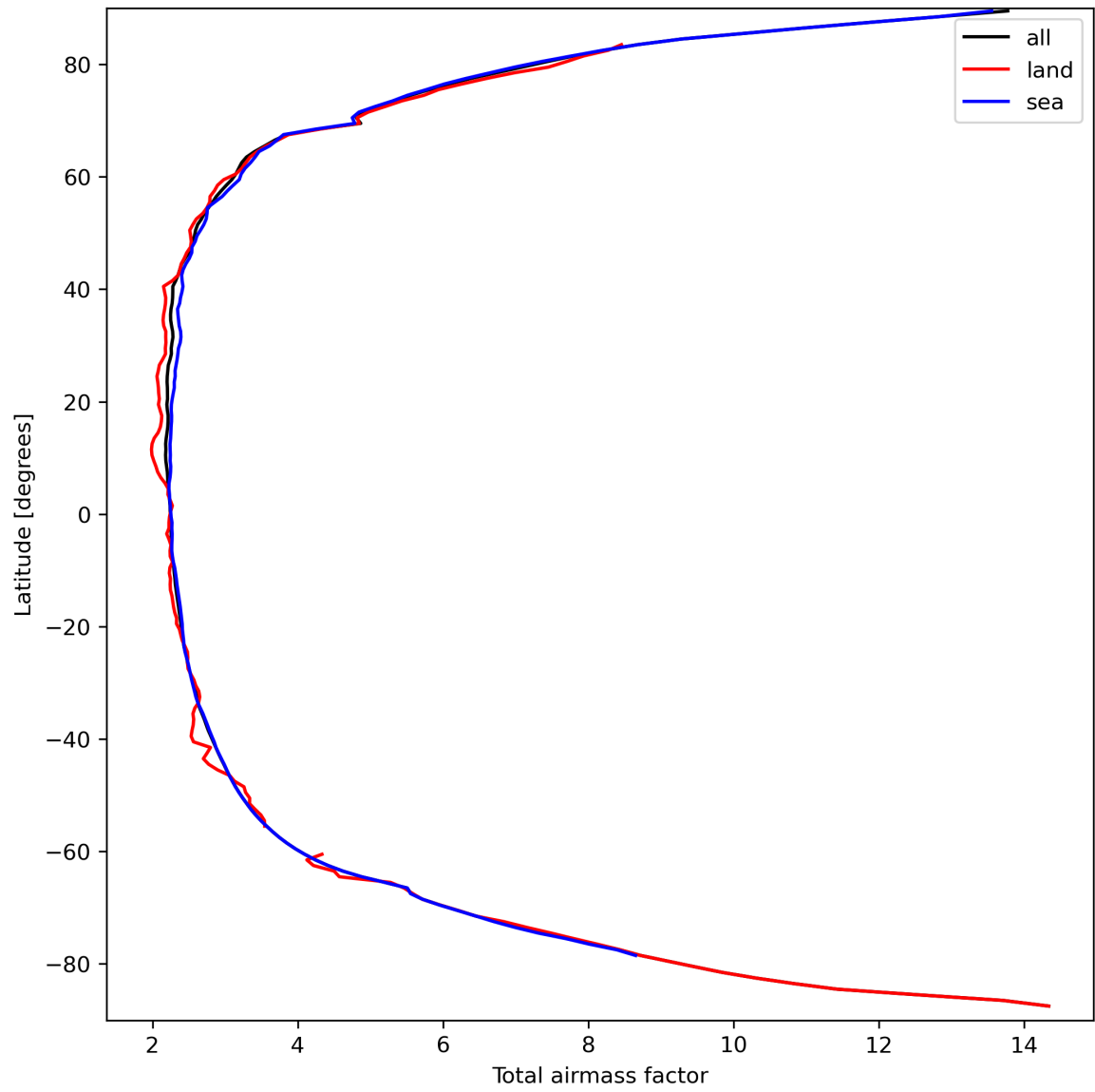
Figure 15: Zonal average of “Total airmass factor” for 2024-03-21 to 2024-03-22.
