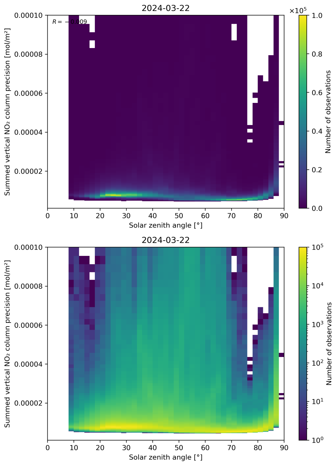
Figure 152: Scatter density plot of “Solar zenith angle” against “Summed vertical NO 2 column precision” for 2024-03-21 to 2024-03-22.
