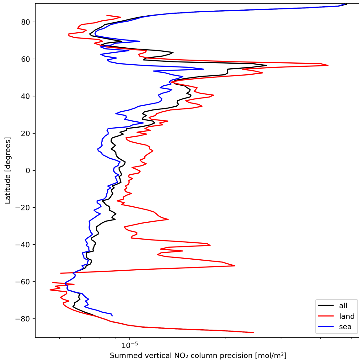
Figure 24: Zonal average of “Summed vertical NO 2 column precision” for 2024-03-21 to 2024-03-22.
