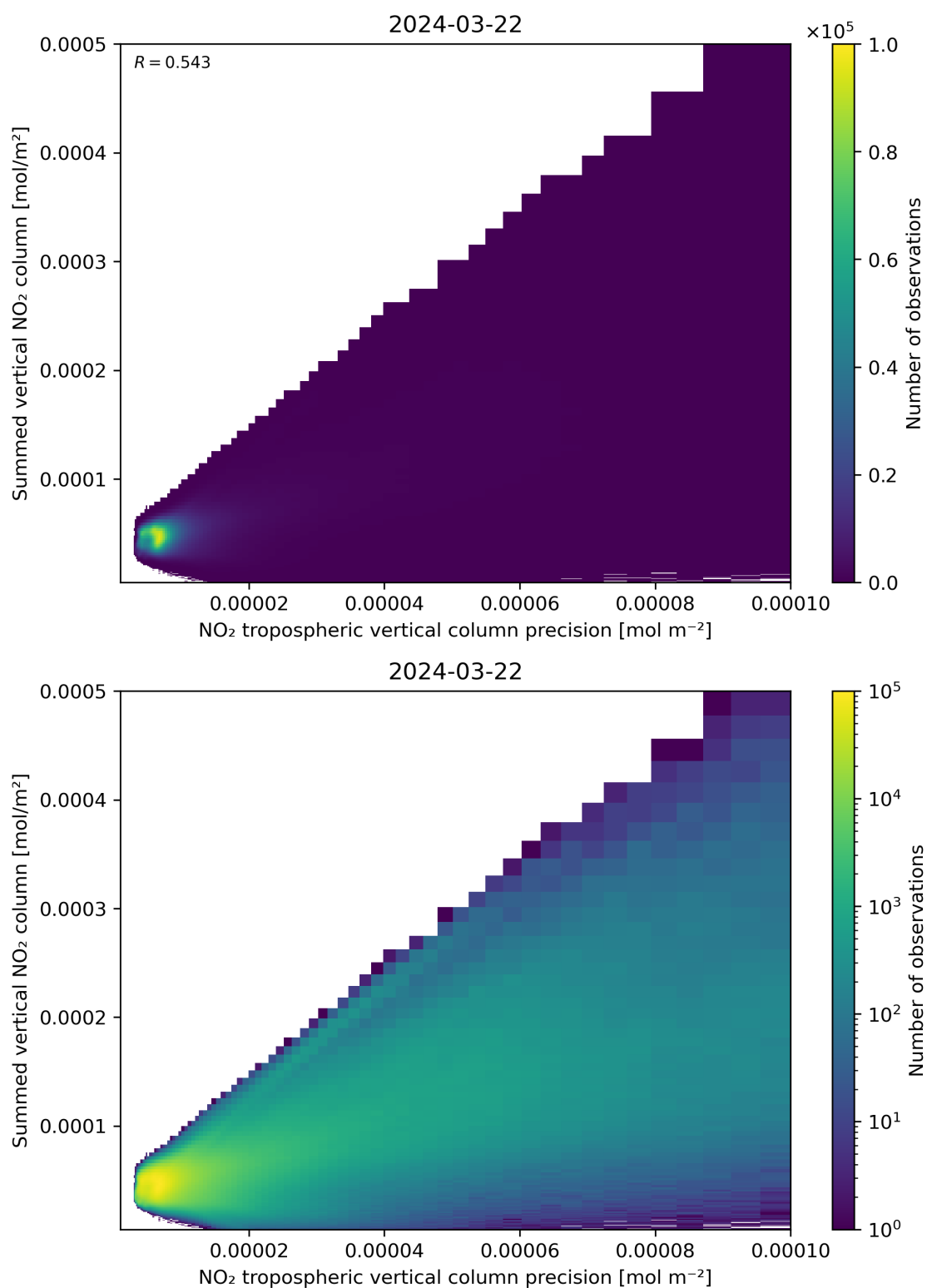
Figure 136: Scatter density plot of “NO 2 tropospheric vertical column precision” against “Summed vertical NO 2 column” for 2024-03-21 to 2024-03-22.
