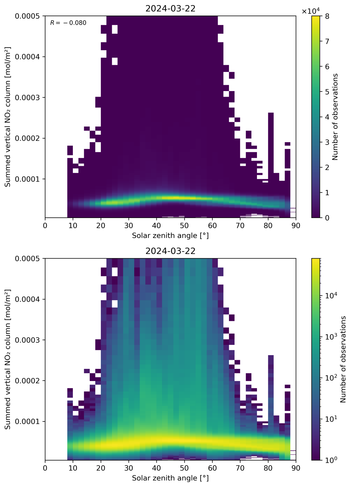
Figure 151: Scatter density plot of “Solar zenith angle” against “Summed vertical NO 2 column” for 2024-03-21 to 2024-03-22.
