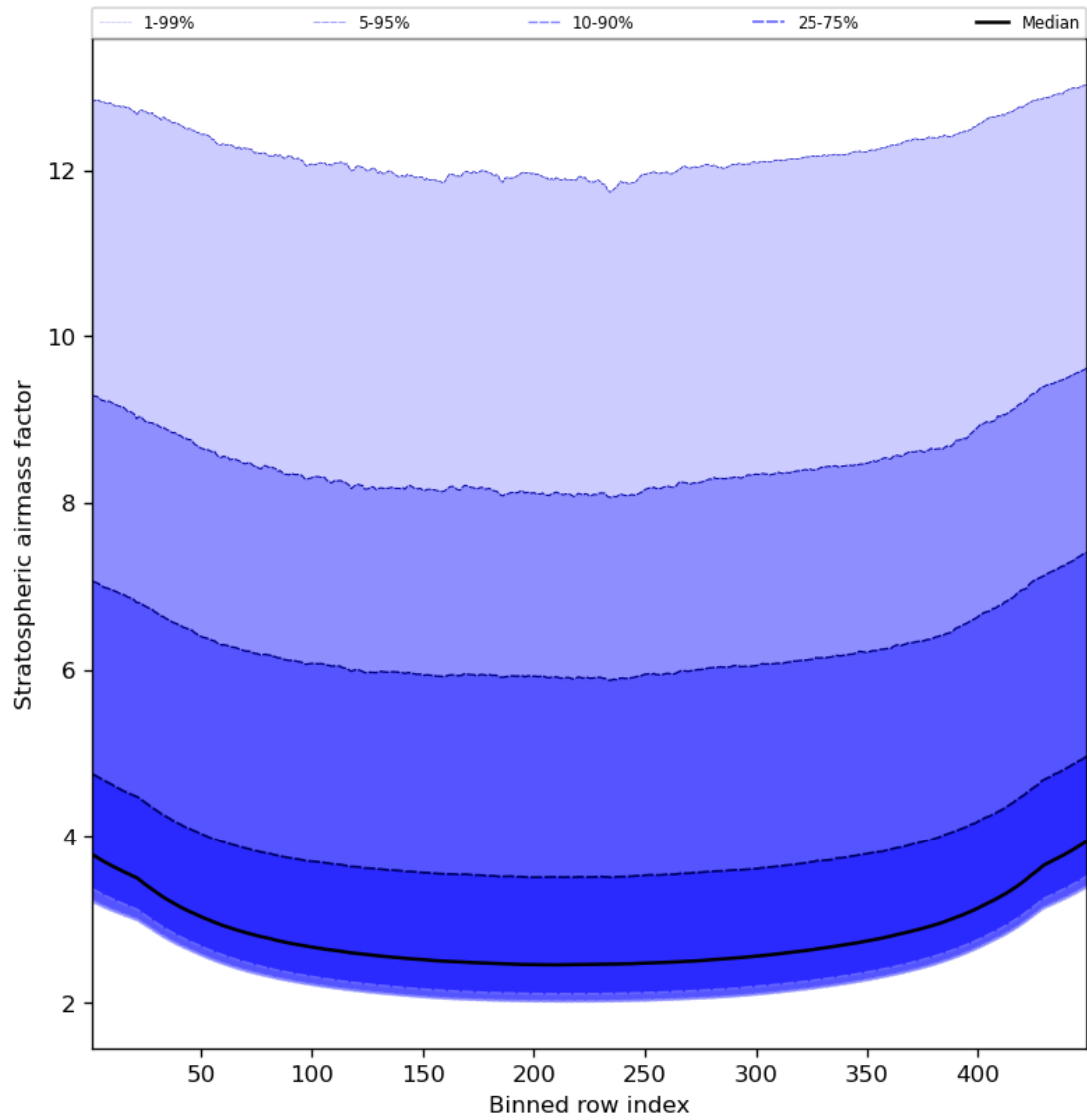
Figure 61: Along track statistics of “Stratospheric airmass factor” for 2024-03-21 to 2024-03-22
