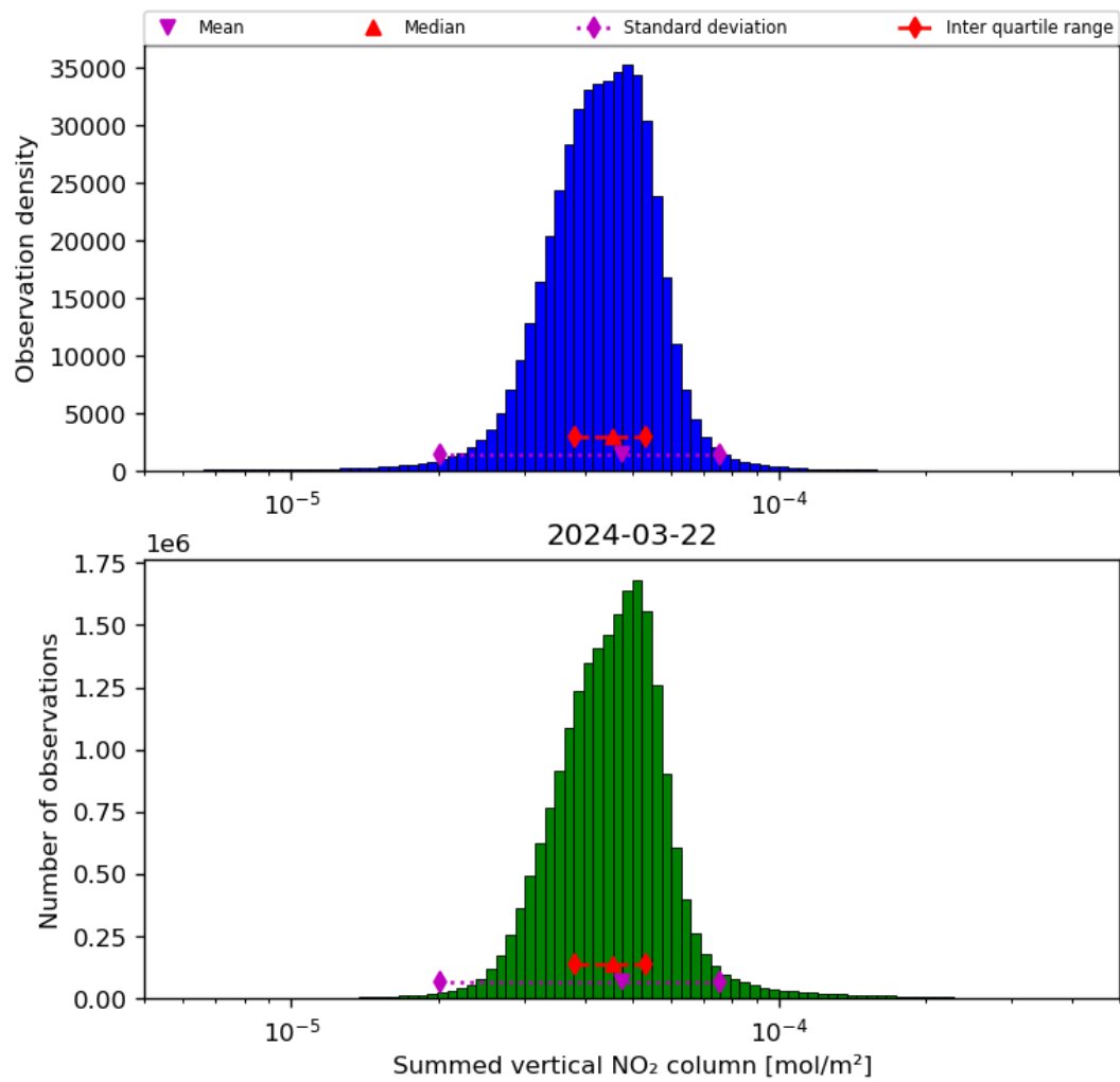
Figure 40: Histogram of “Summed vertical NO 2 column” for 2024-03-21 to 2024-03-22
