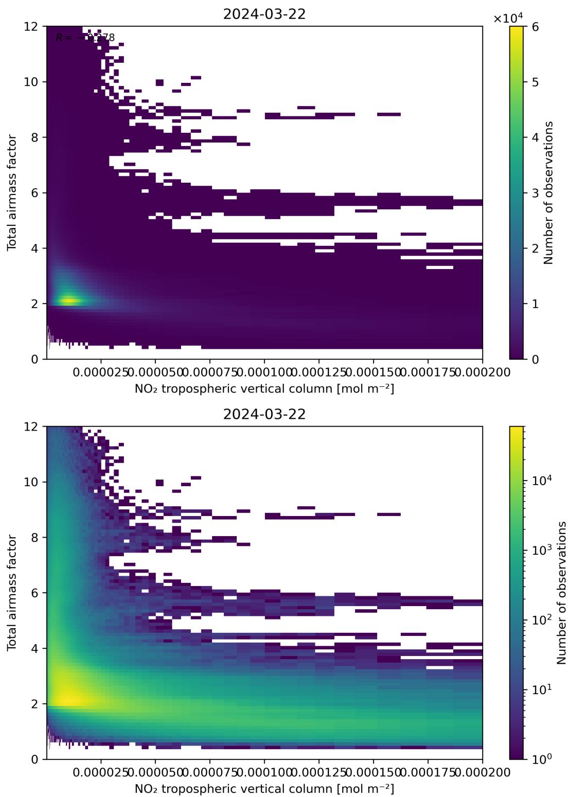
Figure 122: Scatter density plot of “NO 2 tropospheric vertical column” against “Total air mass factor” for 2024-03-21 to 2024-03-22.
