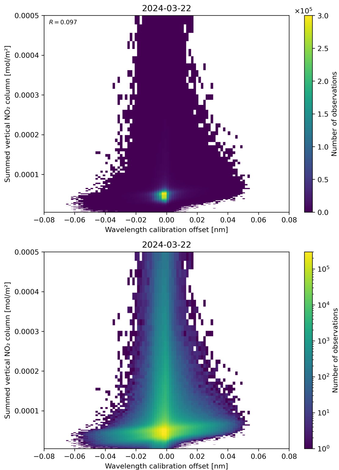
Figure 177: Scatter density plot of “Wavelength calibration offset” against “Summed vertical NO 2 column” for 2024-03-21 to 2024-03-22.
