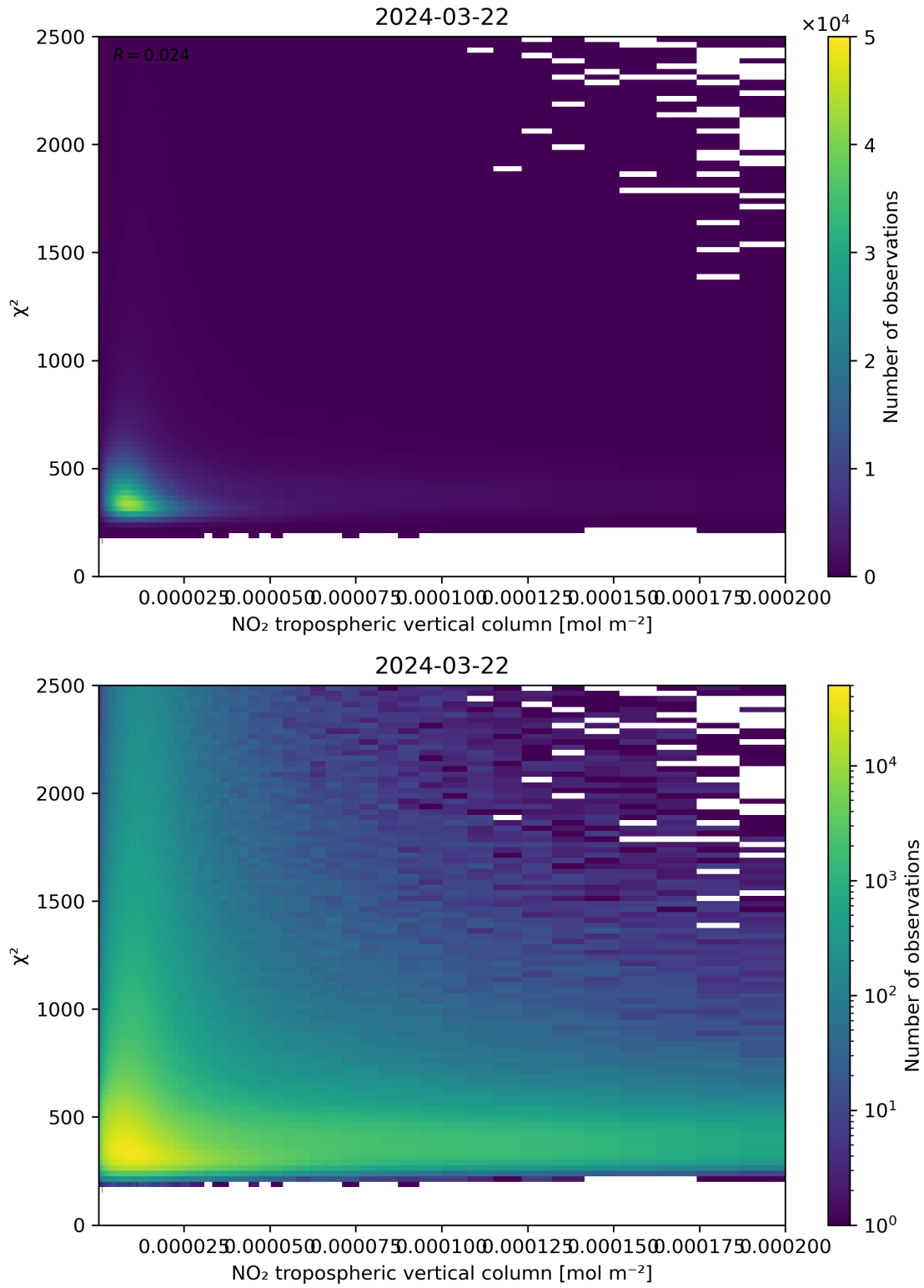
Figure 124: Scatter density plot of “NO 2 tropospheric vertical column” against “ \chi^2 ” for 2024-03-21 to 2024-03-22.
