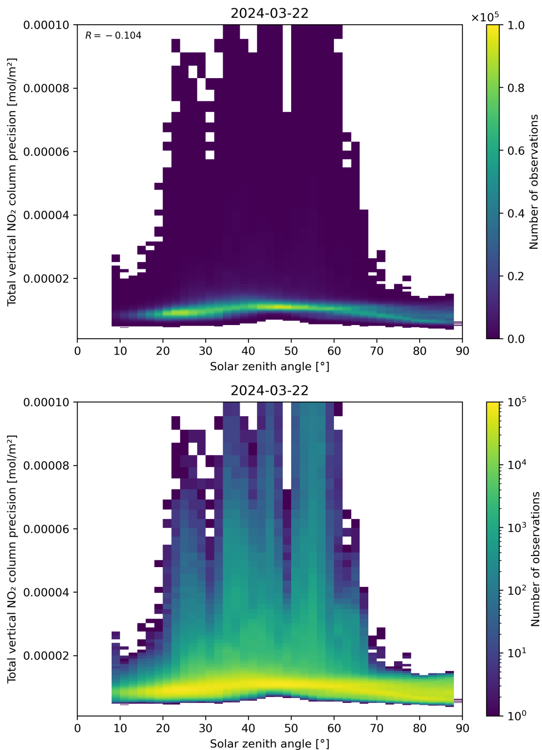
Figure 154: Scatter density plot of “Solar zenith angle” against “Total vertical NO 2 column precision” for 2024-03-21 to 2024-03-22.
