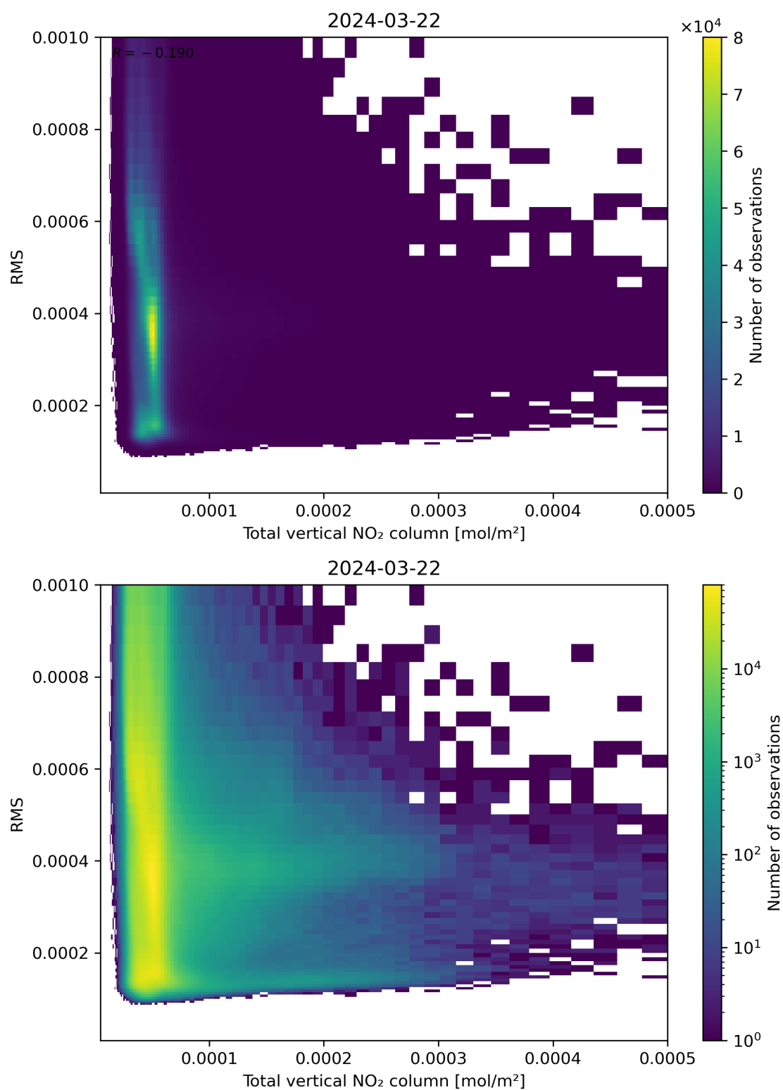
Figure 120: Scatter density plot of “Total vertical NO 2 column” against “RMS” for 2024-03-21 to 2024-03-22.
