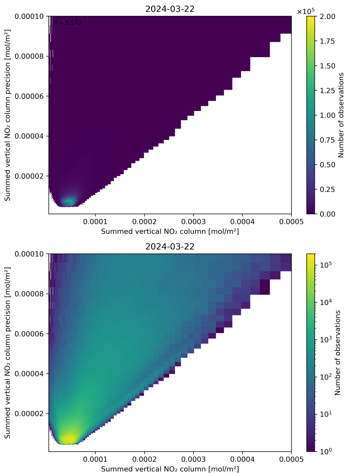
Figure 105: Scatter density plot of “Summed vertical NO 2 column” against “Summed vertical NO 2 column precision” for 2024-03-21 to 2024-03-22.
