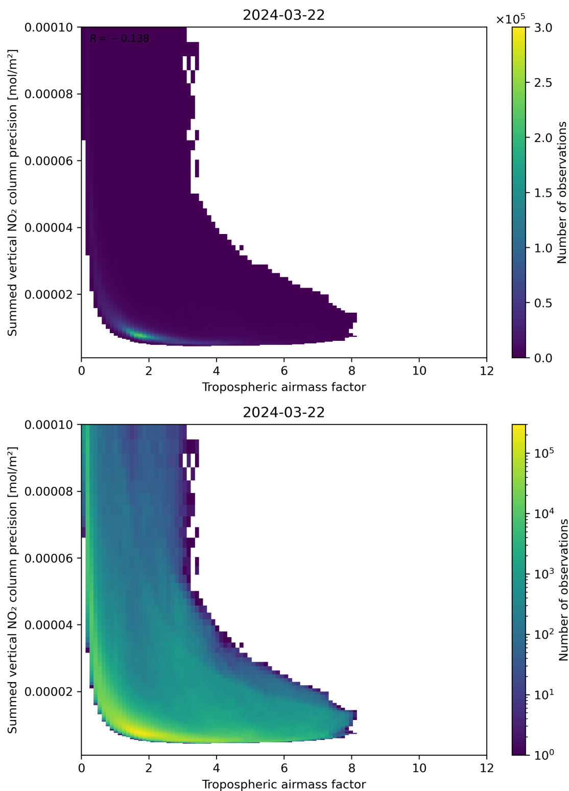
Figure 76: Scatter density plot of “Tropospheric air mass factor” against “Summed vertical NO 2 column precision” for 2024-03-21 to 2024-03-22.
