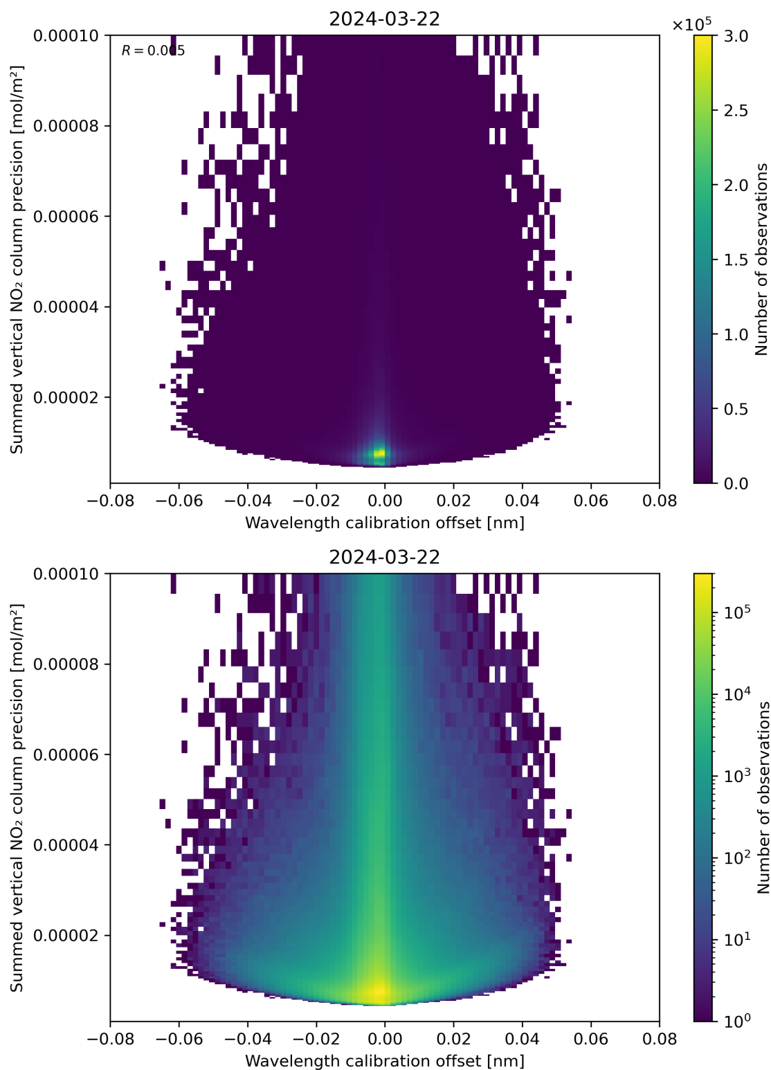
Figure 178: Scatter density plot of “Wavelength calibration offset” against “Summed vertical NO 2 column precision” for 2024-03-21 to 2024-03-22.
