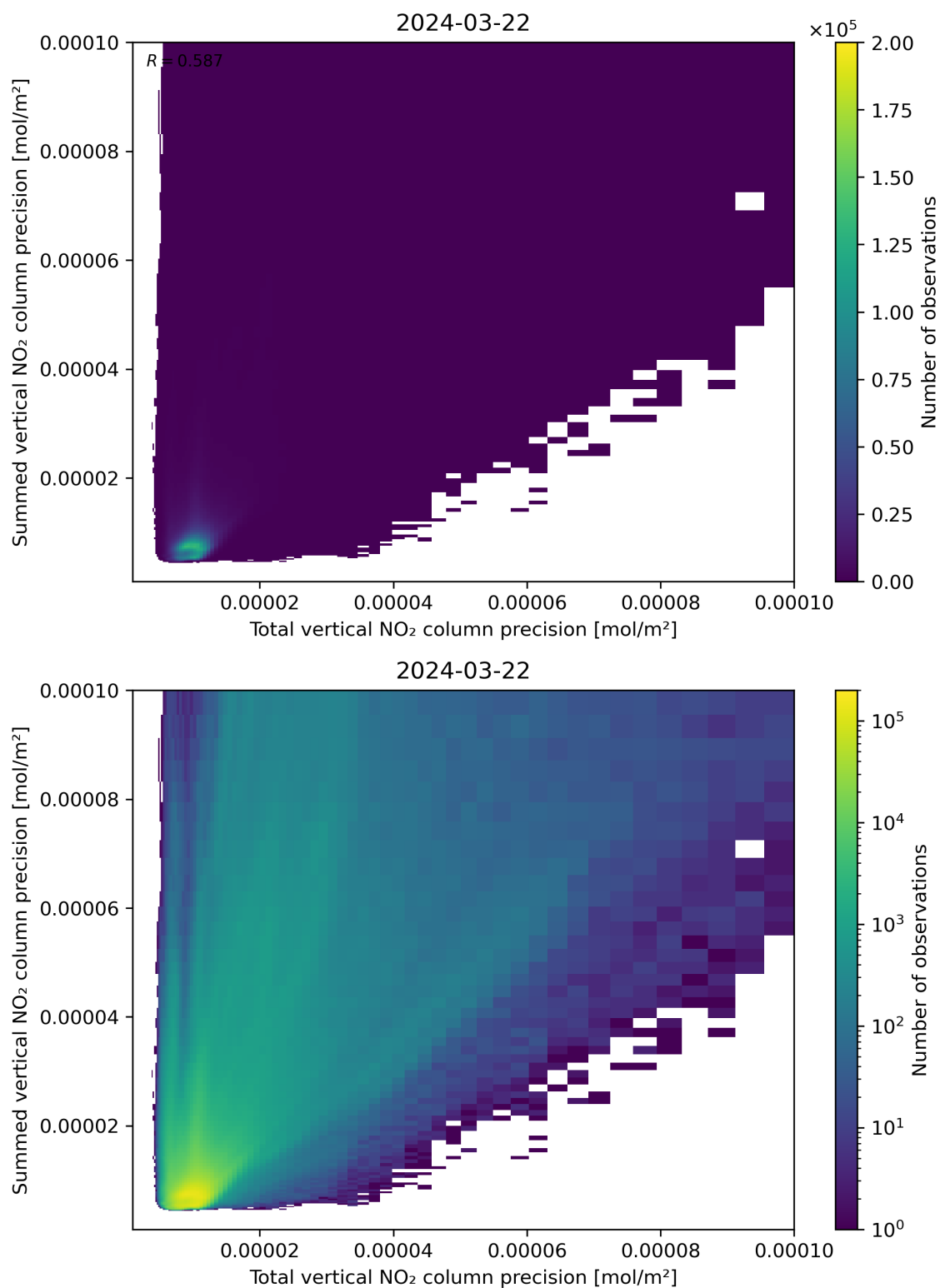
Figure 118: Scatter density plot of “Total vertical NO 2 column precision” against “Summed vertical NO 2 column precision” for 2024-03-21 to 2024-03-22.
