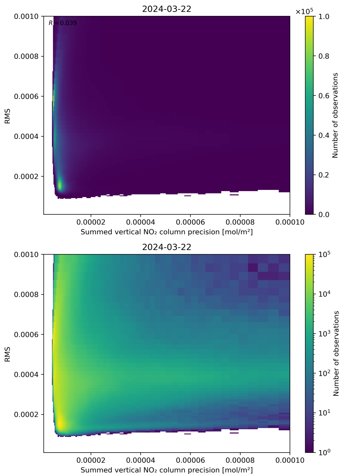
Figure 108: Scatter density plot of “Summed vertical NO 2 column precision” against “RMS” for 2024-03-21 to 2024-03-22.
