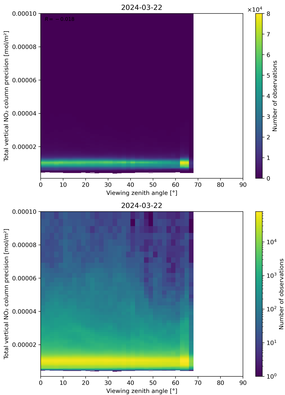
Figure 168: Scatter density plot of “Viewing zenith angle” against “Total vertical NO 2 column precision” for 2024-03-21 to 2024-03-22.
