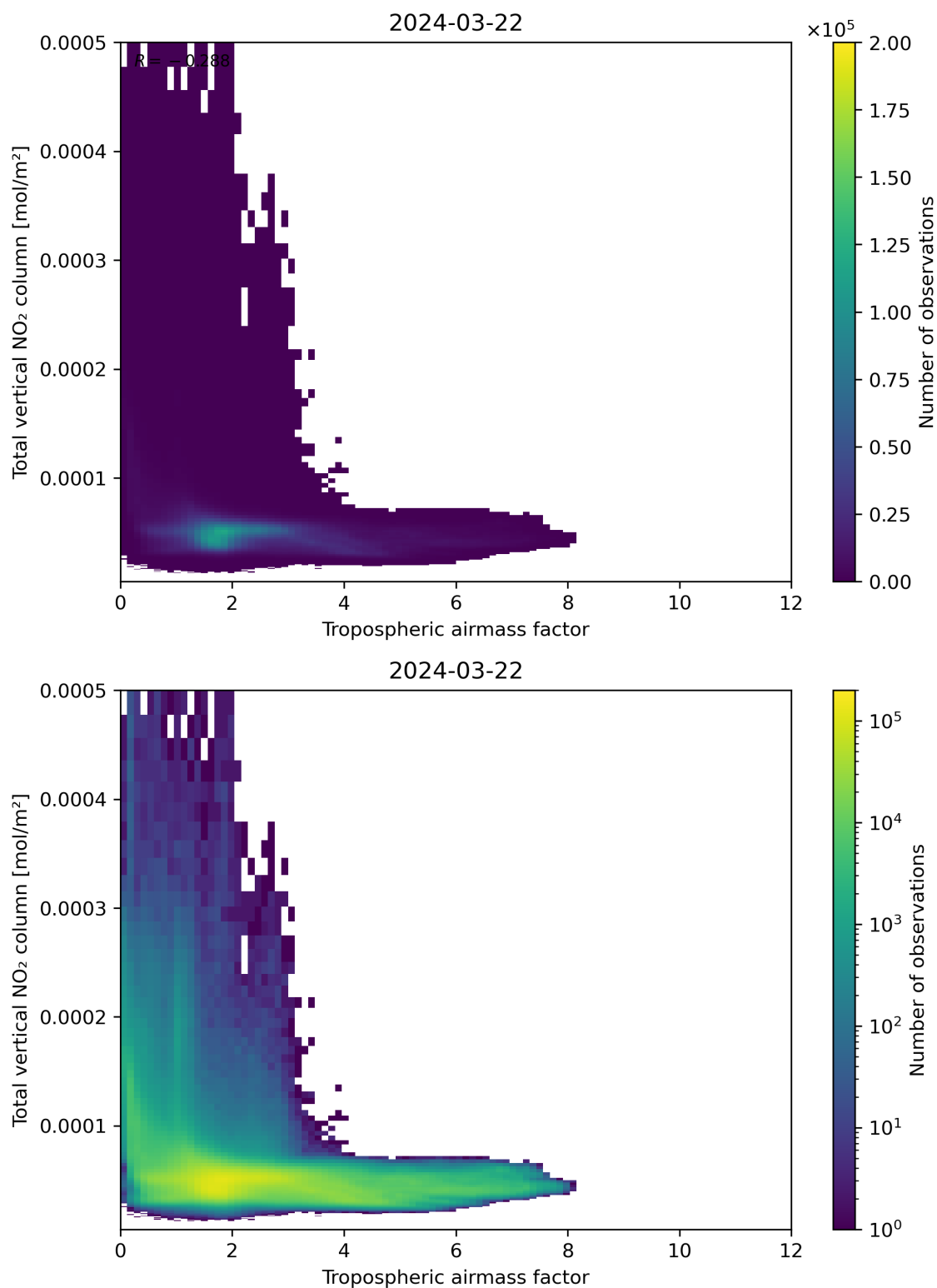
Figure 77: Scatter density plot of “Tropospheric airmass factor” against “Total vertical NO 2 column” for 2024-03-21 to 2024-03-22.
