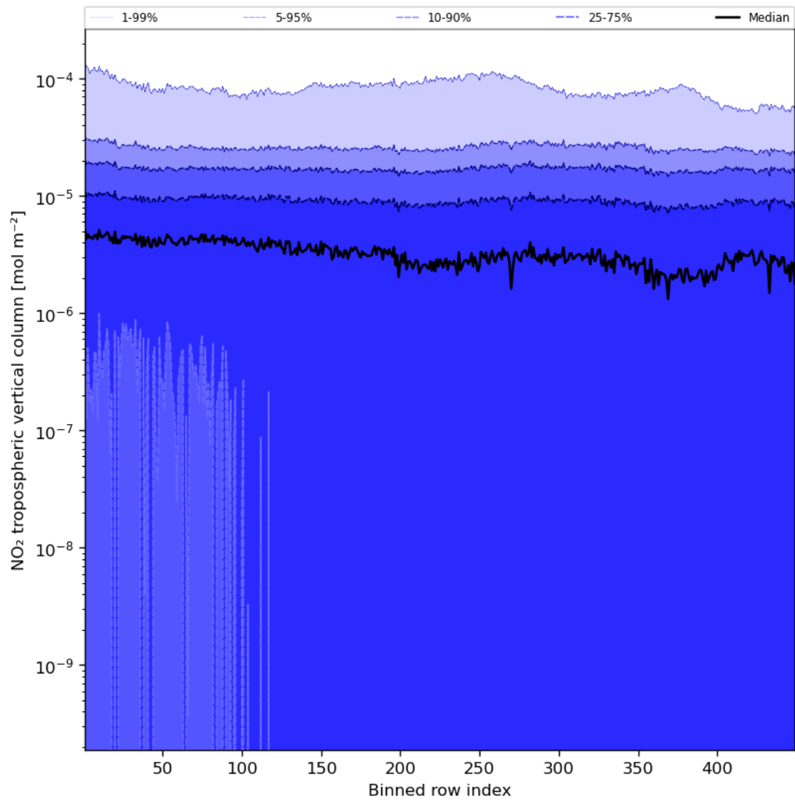
Figure 46: Along track statistics of “NO 2 tropospheric vertical column” for 2024-03-21 to 2024-03-22
