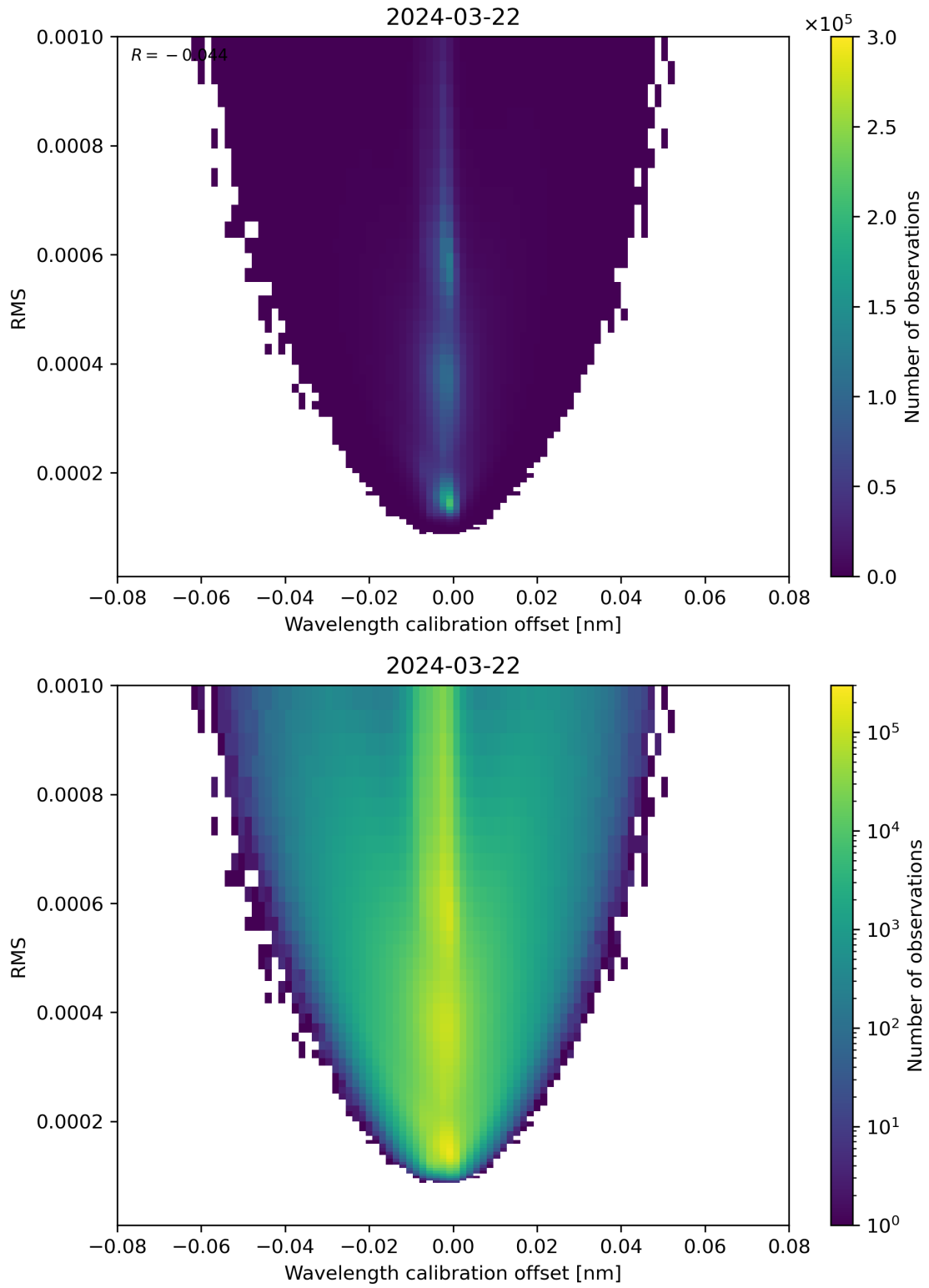
Figure 181: Scatter density plot of “Wavelength calibration offset” against “RMS” for 2024-03-21 to 2024-03-22.
