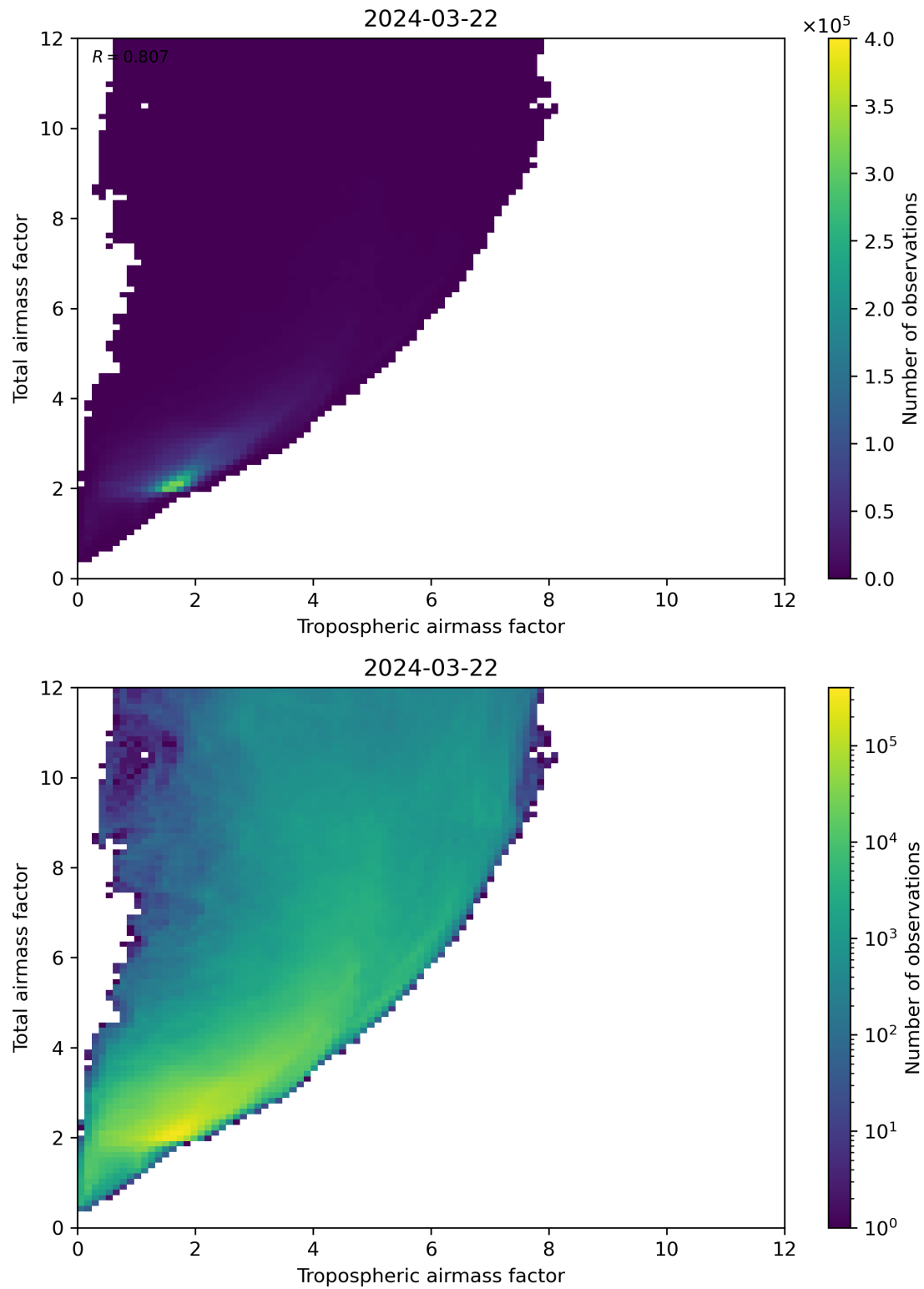
Figure 72: Scatter density plot of “Tropospheric airmass factor” against “Total airmass factor” for 2024-03-21 to 2024-03-22.
