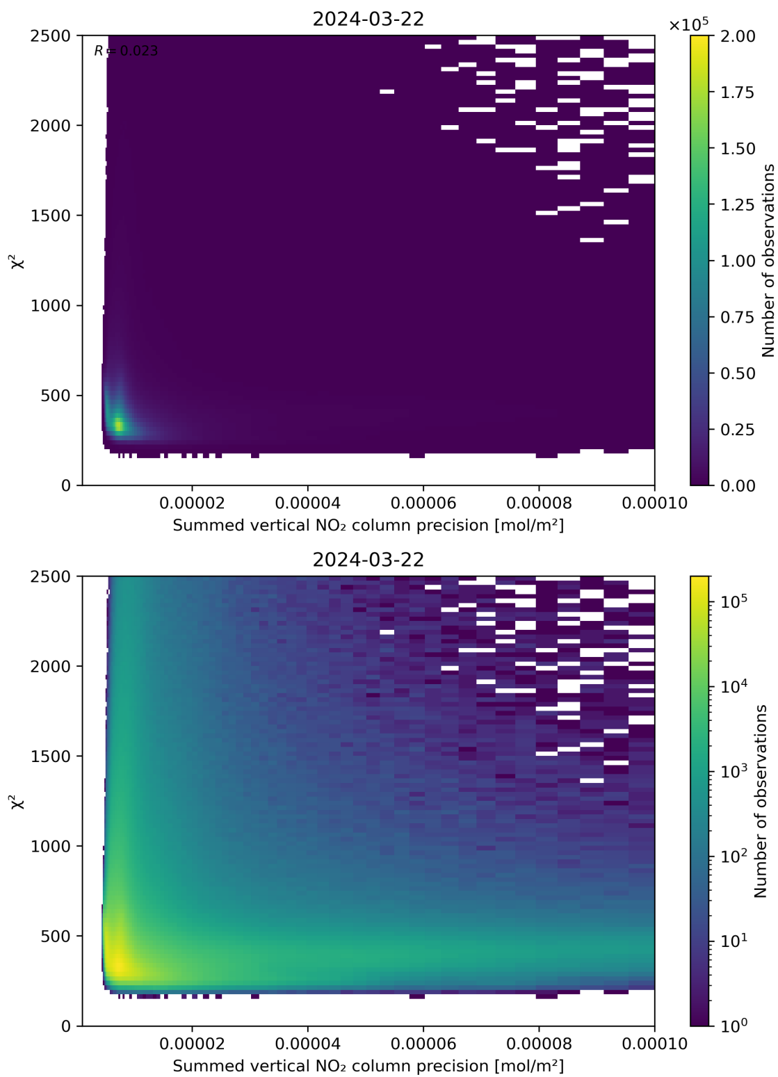
Figure 107: Scatter density plot of “Summed vertical NO 2 column precision” against “ \chi^2 ” for 2024-03-21 to 2024-03-22.
