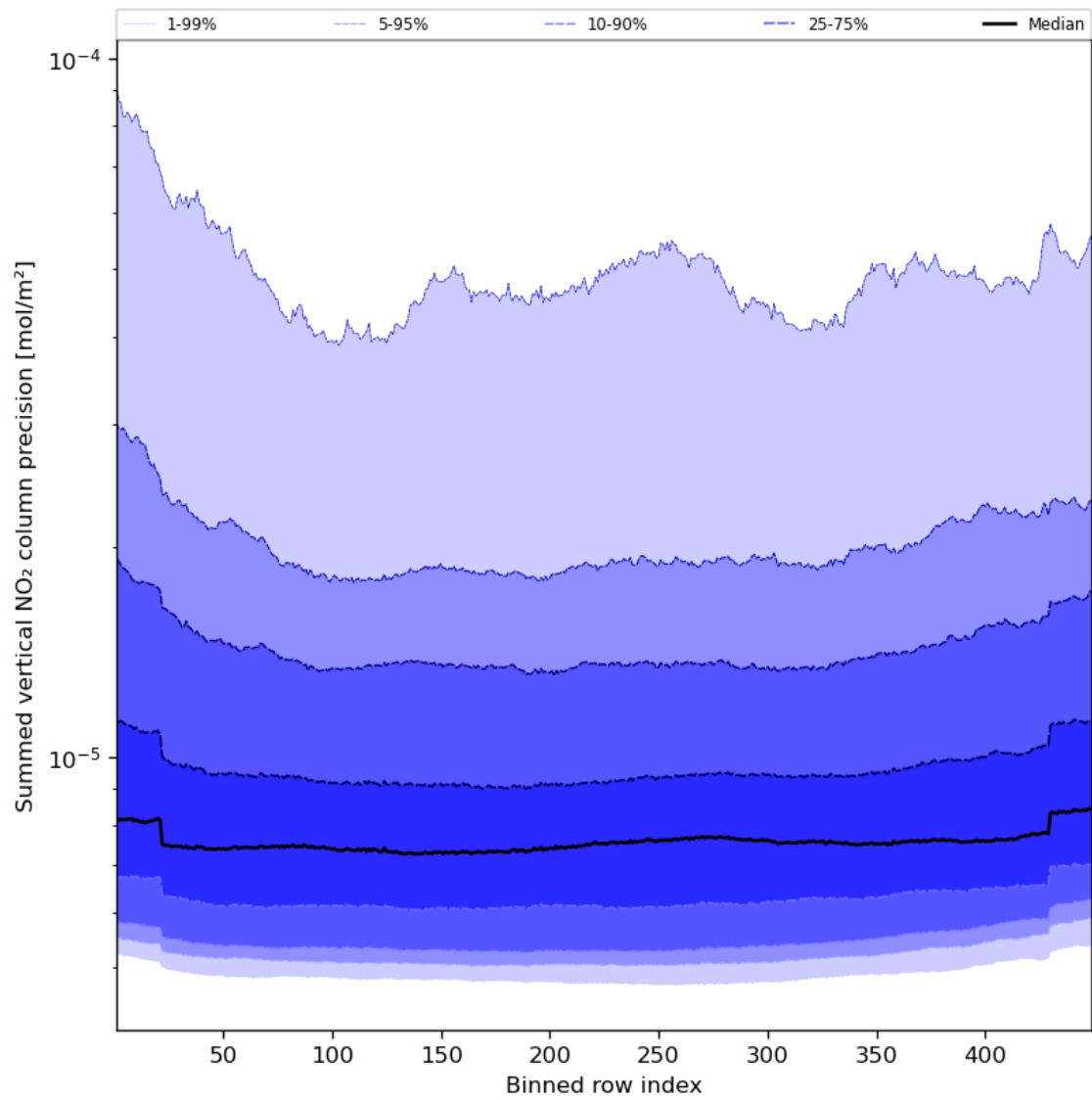
Figure 58: Along track statistics of “Summed vertical NO 2 column precision” for 2024-03-21 to 2024-03-22
