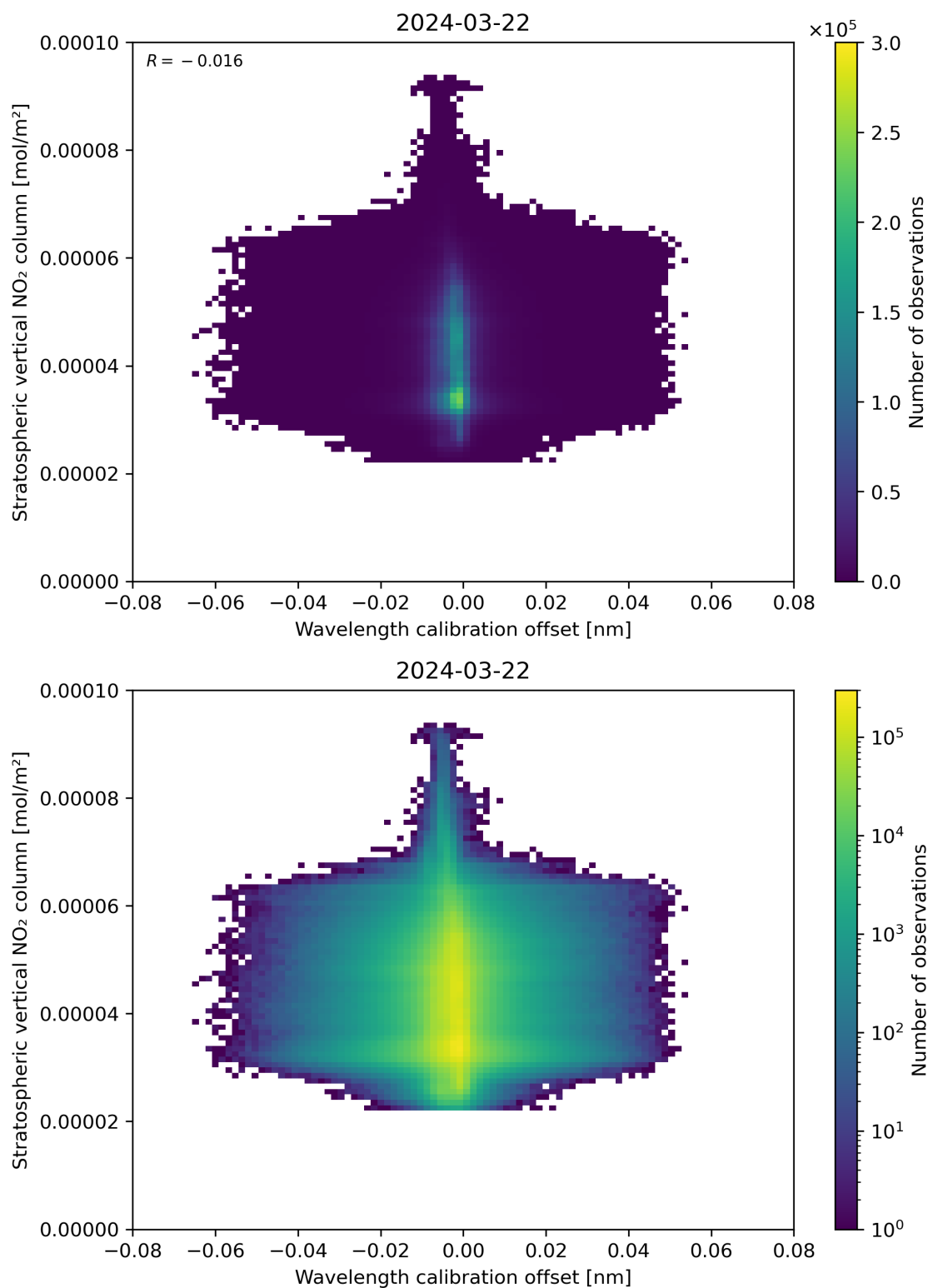
Figure 176: Scatter density plot of “Wavelength calibration offset” against “Stratospheric vertical NO 2 column” for 2024-03-21 to 2024-03-22.
