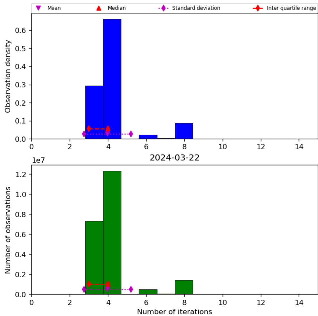
Figure 34: Histogram of “Number of iterations” for 2024-03-21 to 2024-03-22
