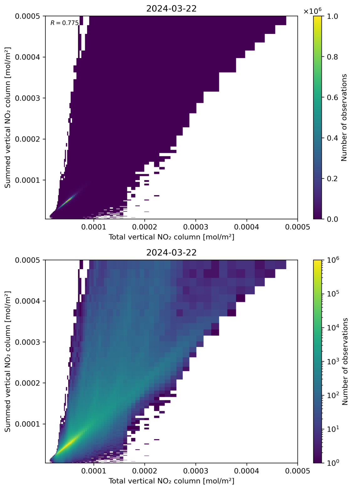
Figure 112: Scatter density plot of “Total vertical NO 2 column” against “Summed vertical NO 2 column” for 2024-03-21 to 2024-03-22.
