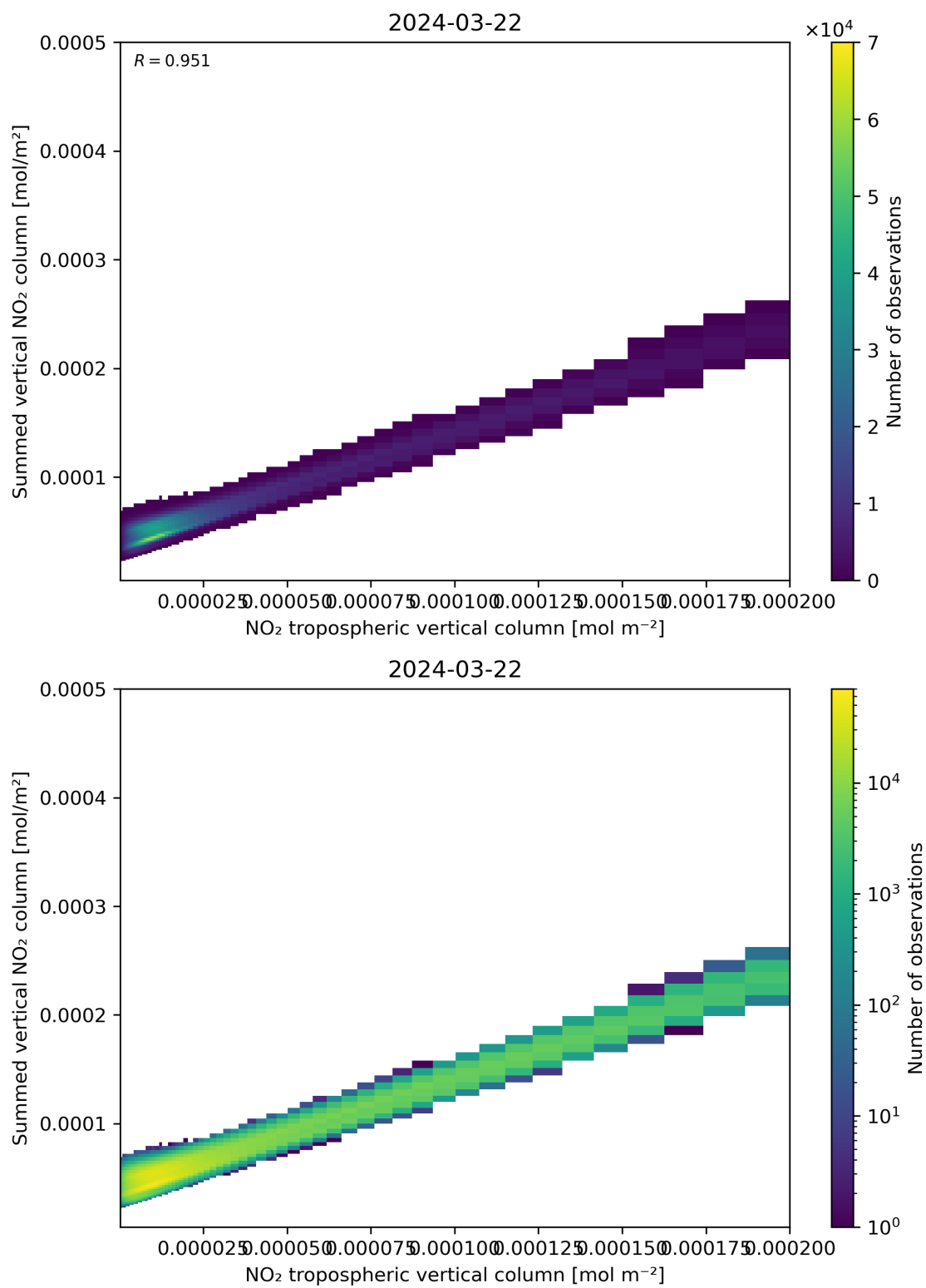
Figure 126: Scatter density plot of “NO 2 tropospheric vertical column” against “Summed vertical NO 2 column” for 2024-03-21 to 2024-03-22.
