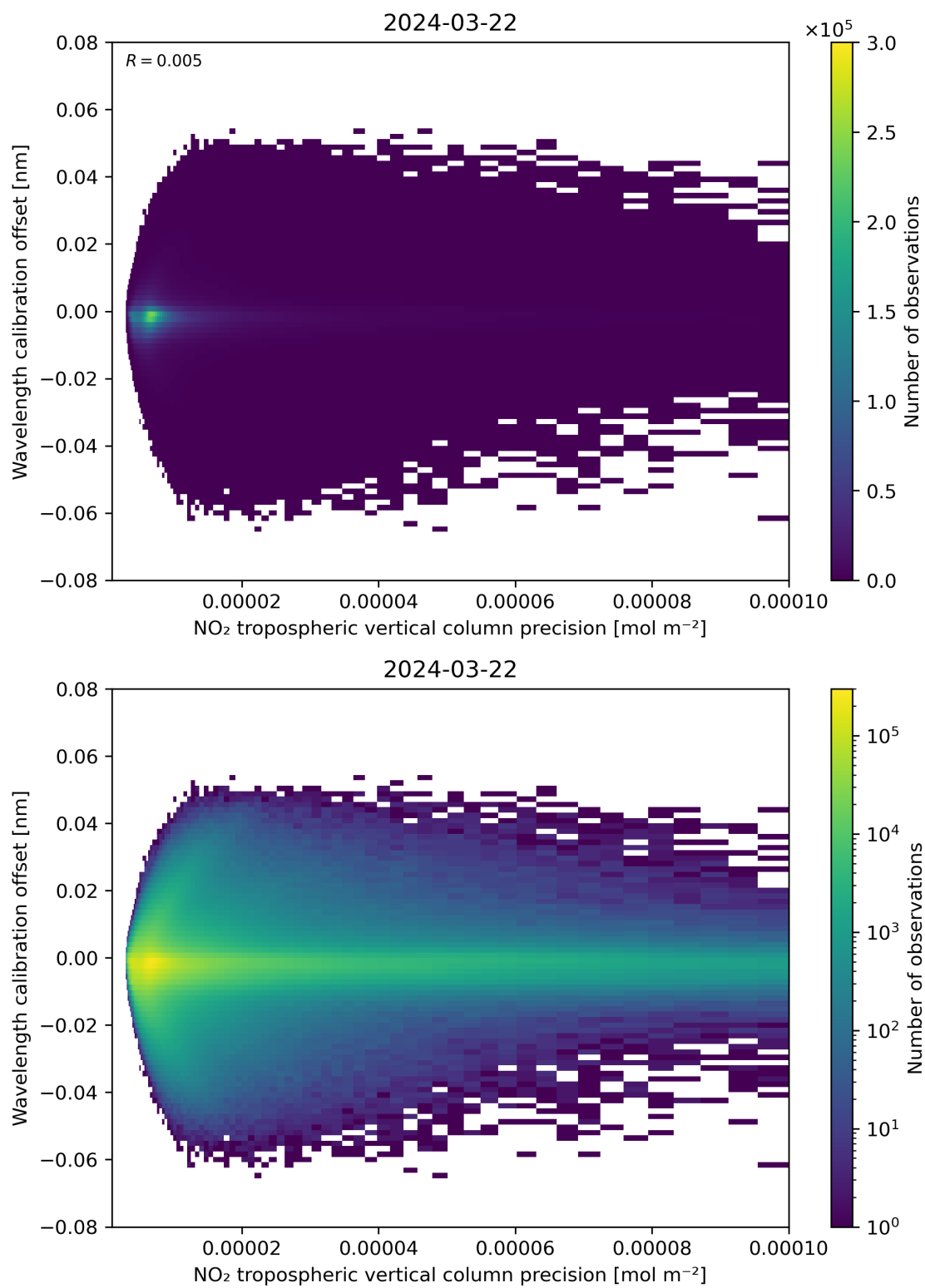
Figure 141: Scatter density plot of “NO 2 tropospheric vertical column precision” against “Wavelength calibration offset” for 2024-03-21 to 2024-03-22.
