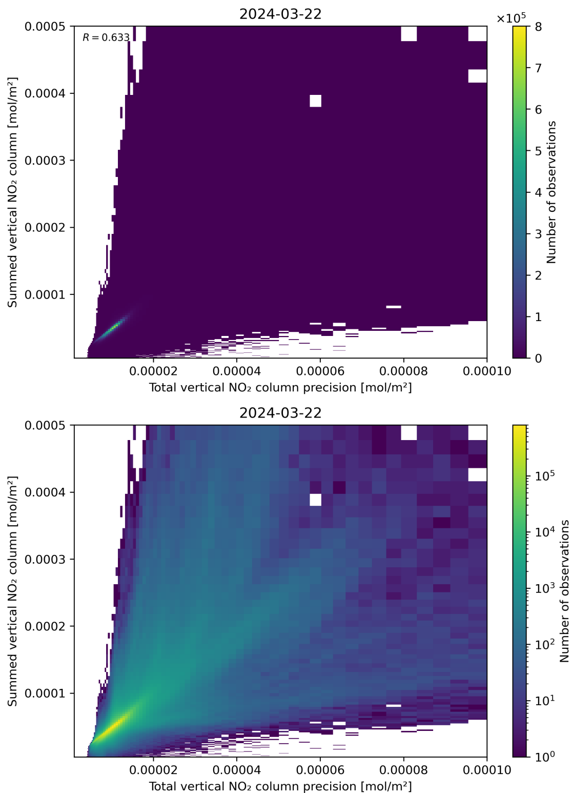
Figure 117: Scatter density plot of “Total vertical NO 2 column precision” against “Summed vertical NO 2 column” for 2024-03-21 to 2024-03-22.
