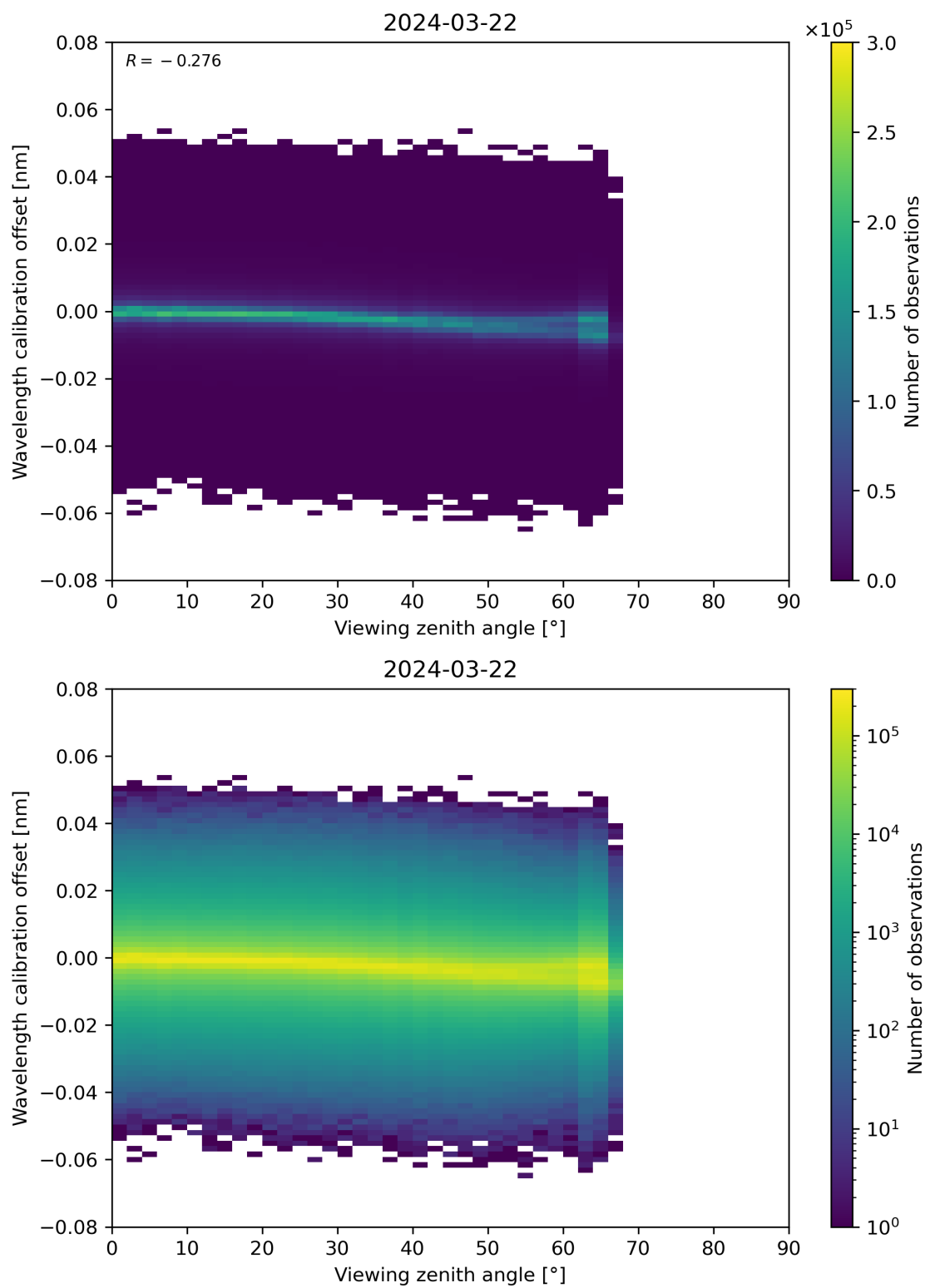
Figure 173: Scatter density plot of “Viewing zenith angle” against “Wavelength calibration offset” for 2024-03-21 to 2024-03-22.
