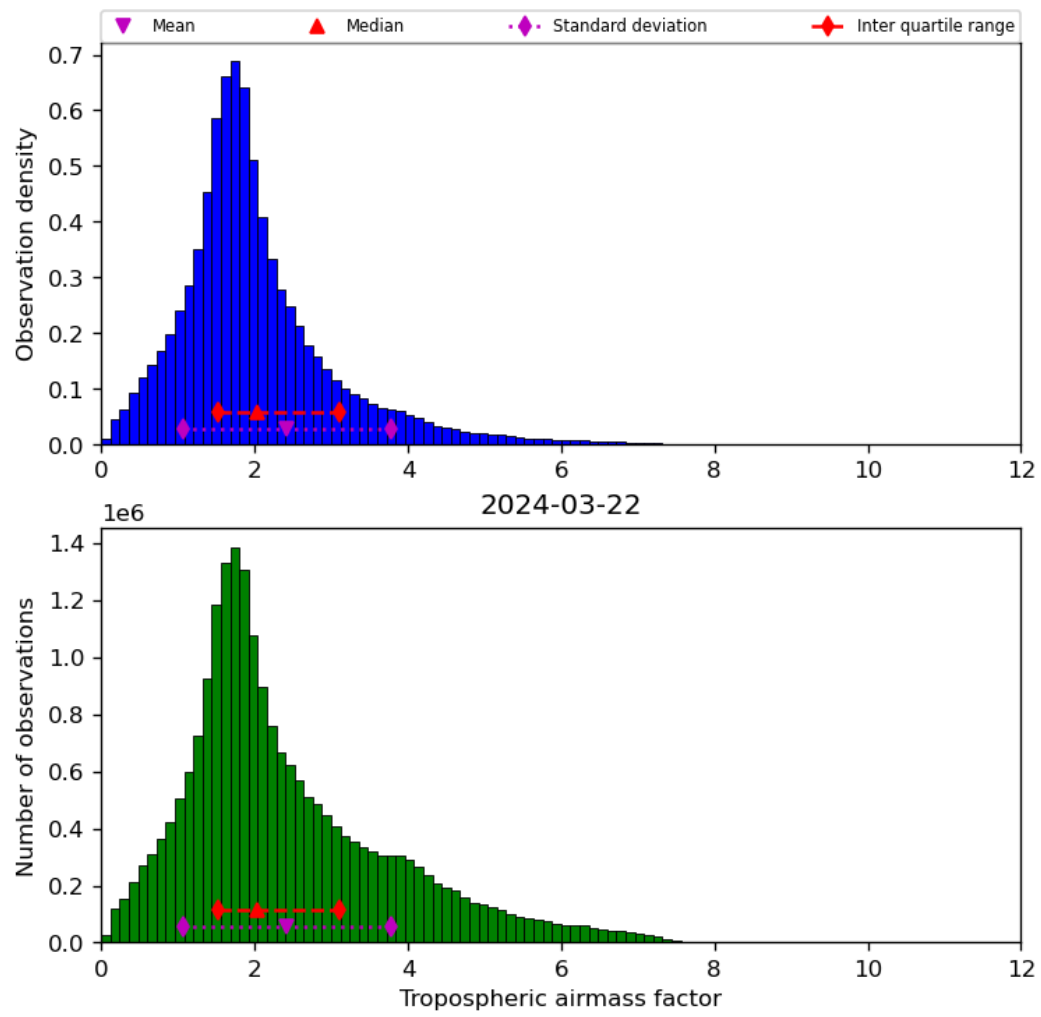
Figure 31: Histogram of “Tropospheric airmass factor” for 2024-03-21 to 2024-03-22
