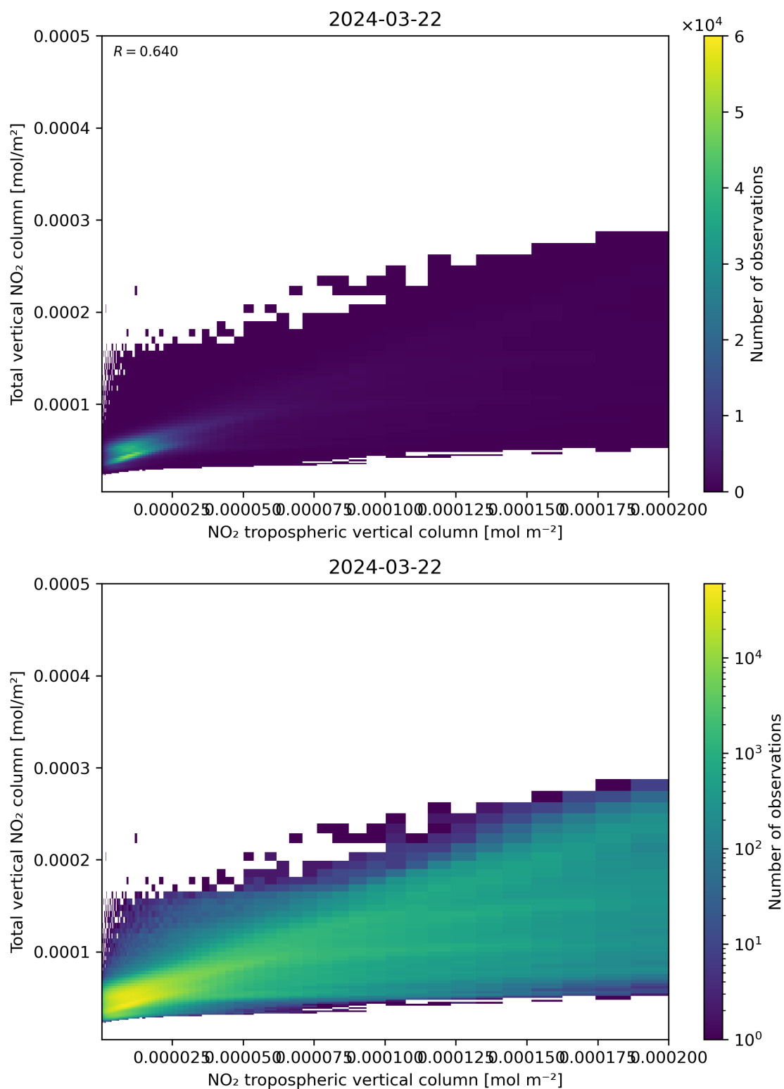
Figure 128: Scatter density plot of “NO 2 tropospheric vertical column” against “Total vertical NO 2 column” for 2024-03-21 to 2024-03-22.
