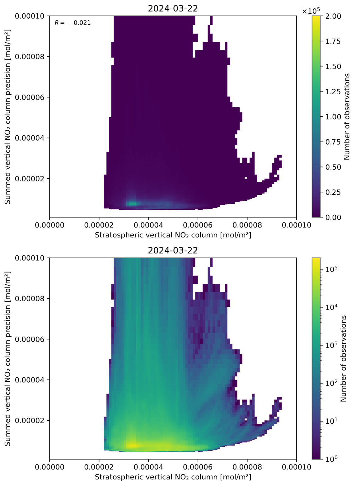
Figure 99: Scatter density plot of “Stratospheric vertical NO 2 column” against “Summed vertical NO 2 column precision” for 2024-03-21 to 2024-03-22.
