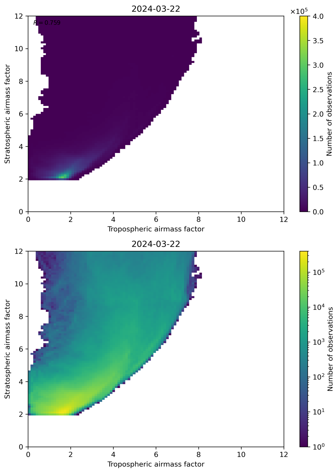
Figure 71: Scatter density plot of “Tropospheric airmass factor” against “Stratospheric airmass factor” for 2024-03-21 to 2024-03-22.
