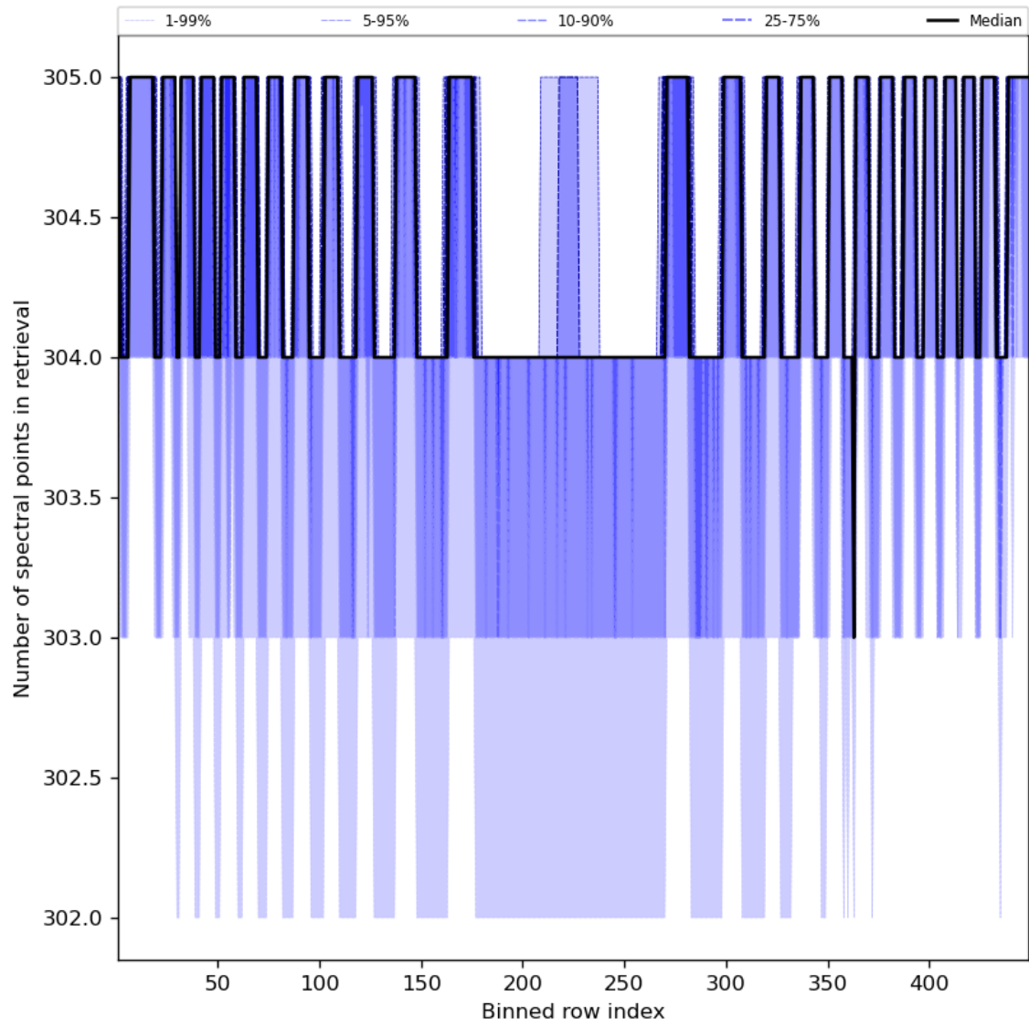
Figure 50: Along track statistics of “Number of spectral points in retrieval” for 2024-03-21 to 2024-03-22
