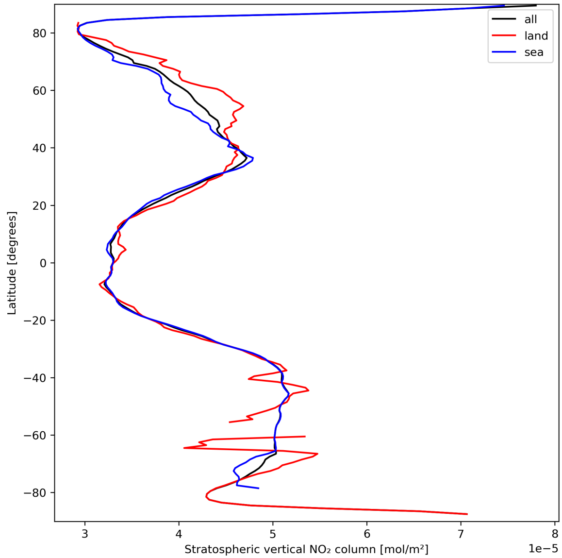
Figure 19: Zonal average of “Stratospheric vertical NO 2 column” for 2024-03-21 to 2024-03-22.
