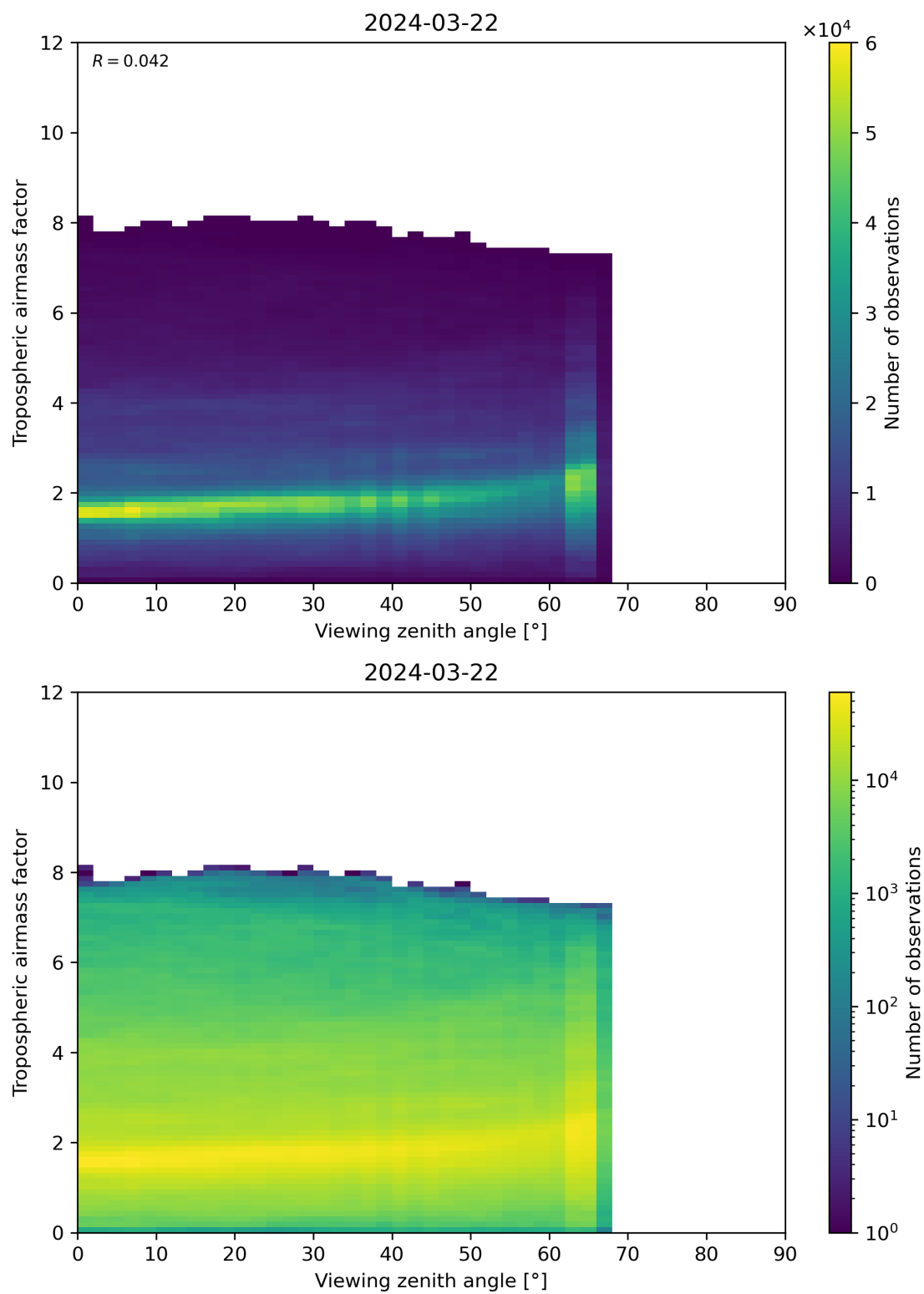
Figure 161: Scatter density plot of “Viewing zenith angle” against “Tropospheric airmass factor” for 2024-03-21 to 2024-03-22.
