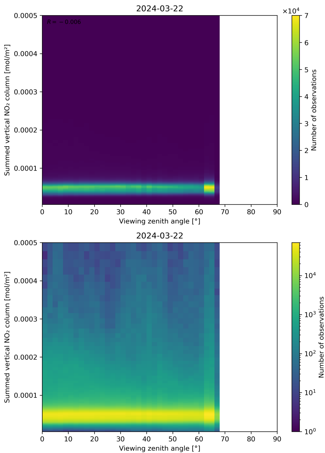
Figure 165: Scatter density plot of “Viewing zenith angle” against “Summed vertical NO 2 column” for 2024-03-21 to 2024-03-22.
