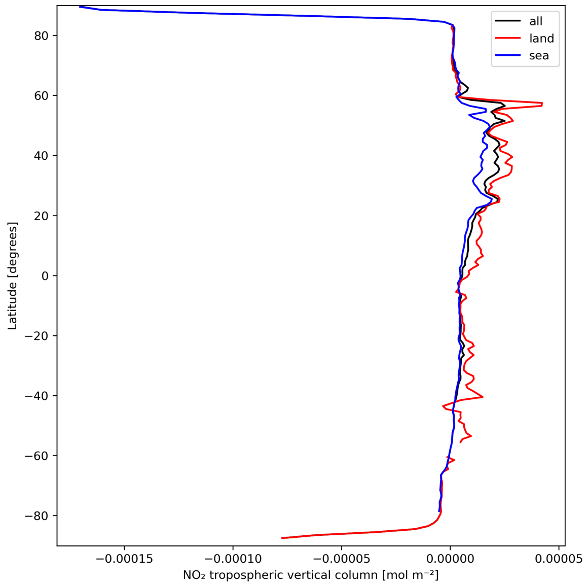
Figure 12: Zonal average of “NO 2 tropospheric vertical column” for 2024-03-21 to 2024-03-22.
