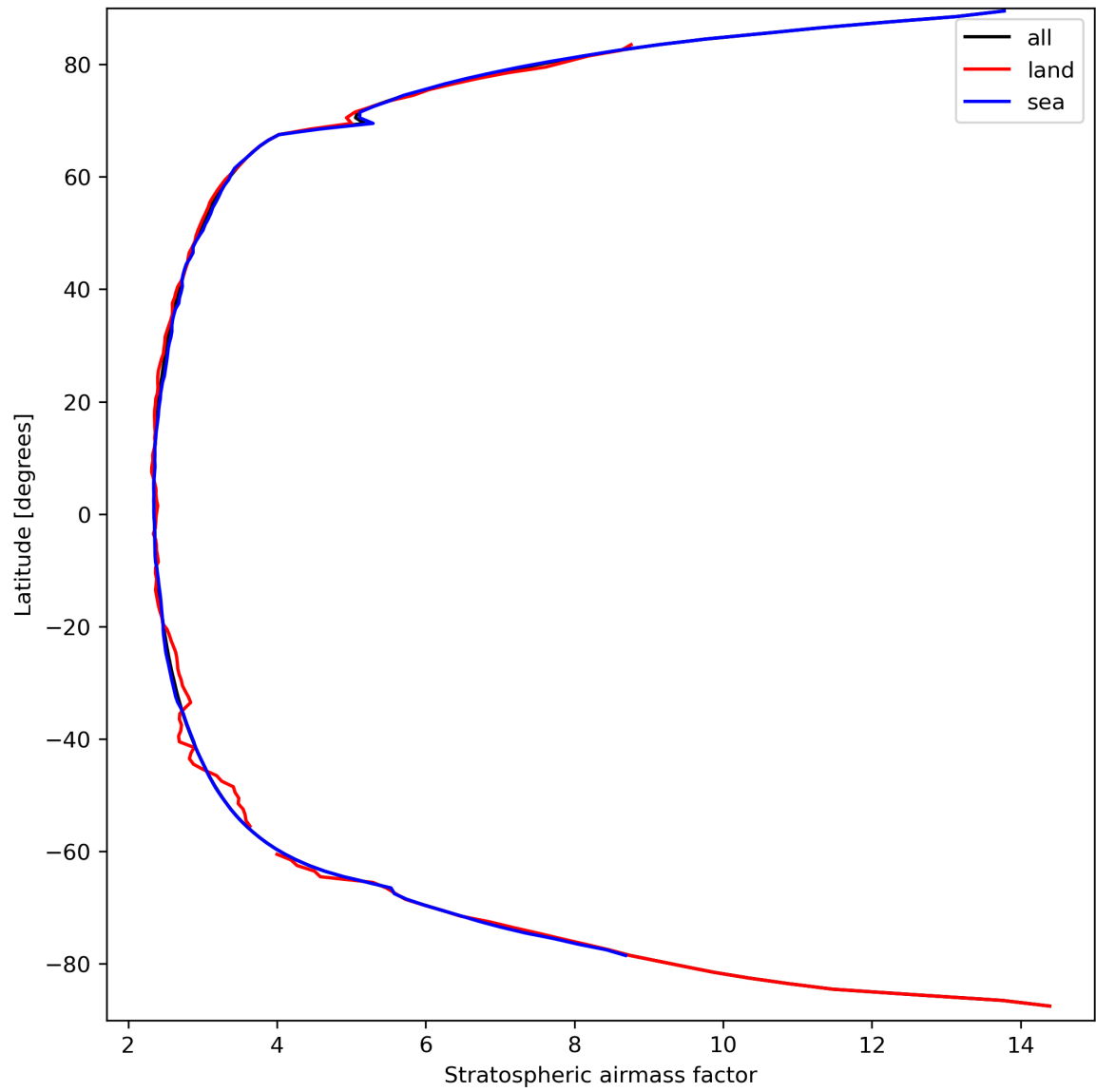
Figure 27: Zonal average of “Stratospheric air mass factor” for 2024-03-21 to 2024-03-22.
