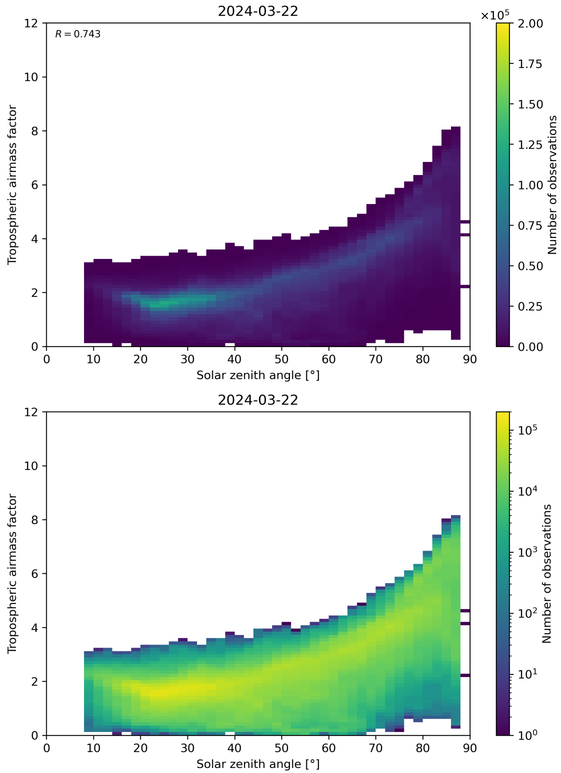
Figure 147: Scatter density plot of “Solar zenith angle” against “Tropospheric airmass factor” for 2024-03-21 to 2024-03-22.
