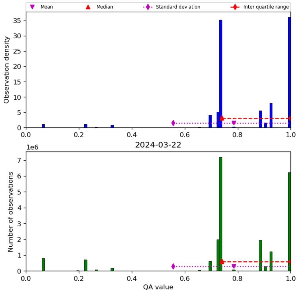
Figure 28: Histogram of “QA value” for 2024-03-21 to 2024-03-22
