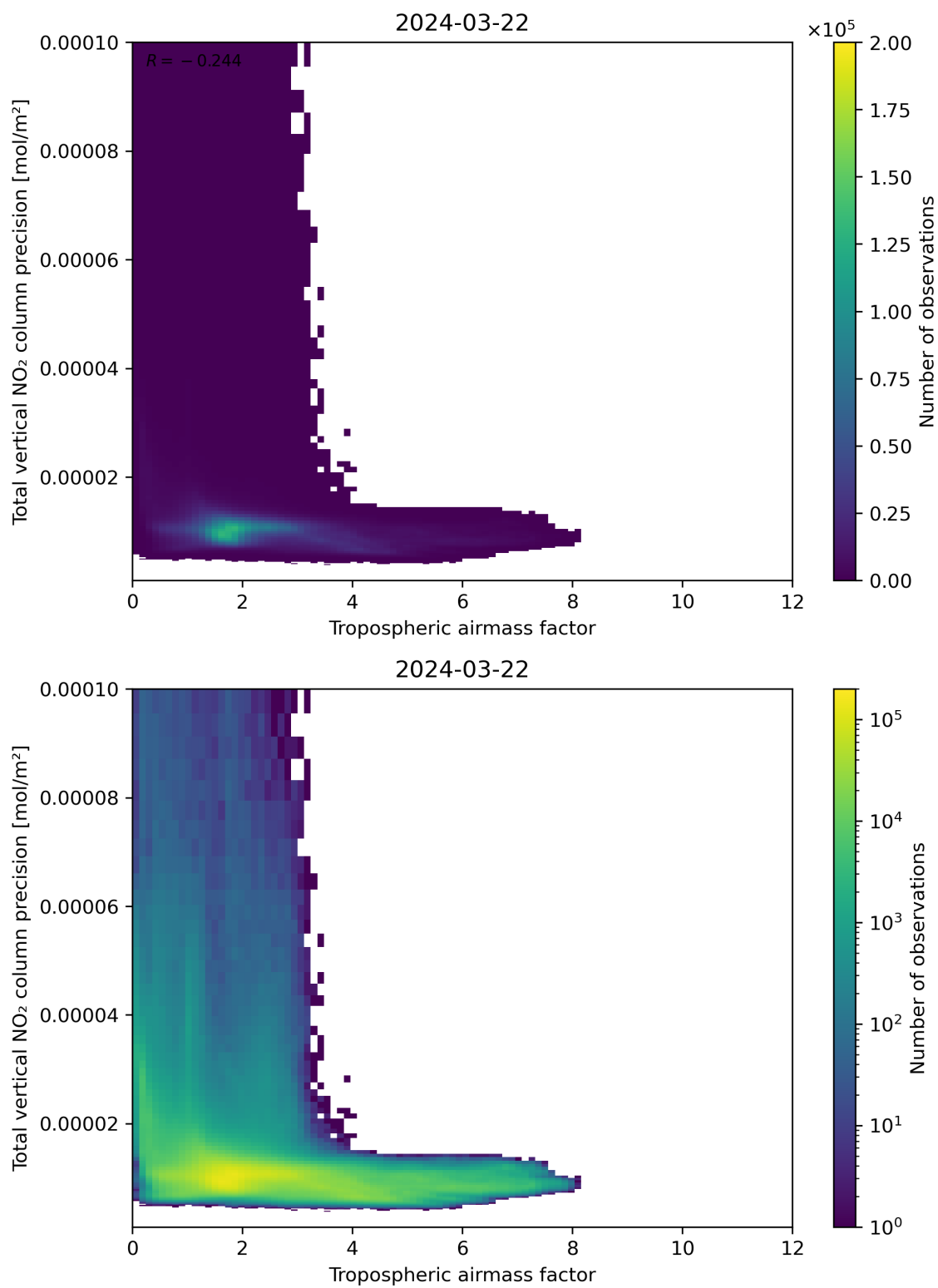
Figure 78: Scatter density plot of “Tropospheric air mass factor” against “Total vertical NO 2 column precision” for 2024-03-21 to 2024-03-22.
