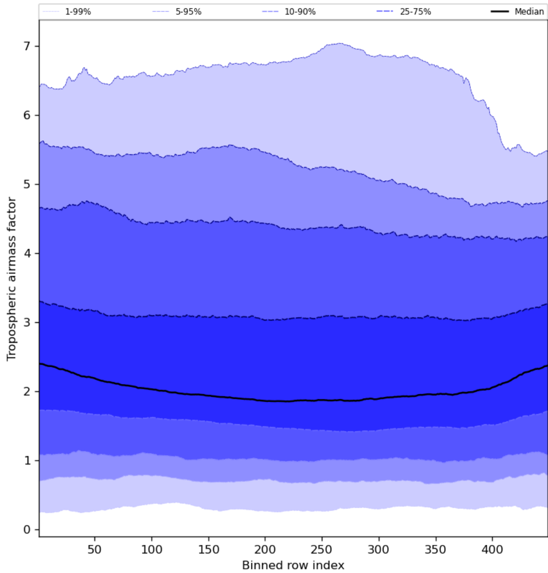
Figure 48: Along track statistics of “Tropospheric airmass factor” for 2024-03-21 to 2024-03-22
