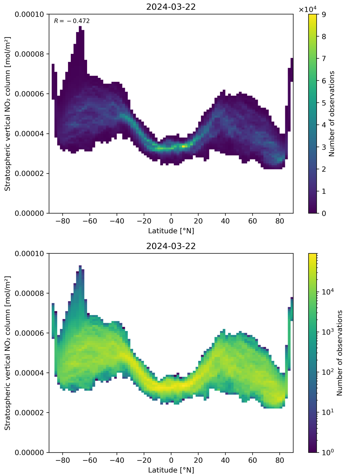
Figure 87: Scatter density plot of “Latitude” against “Stratospheric vertical NO 2 column” for 2024-03-21 to 2024-03-22.
