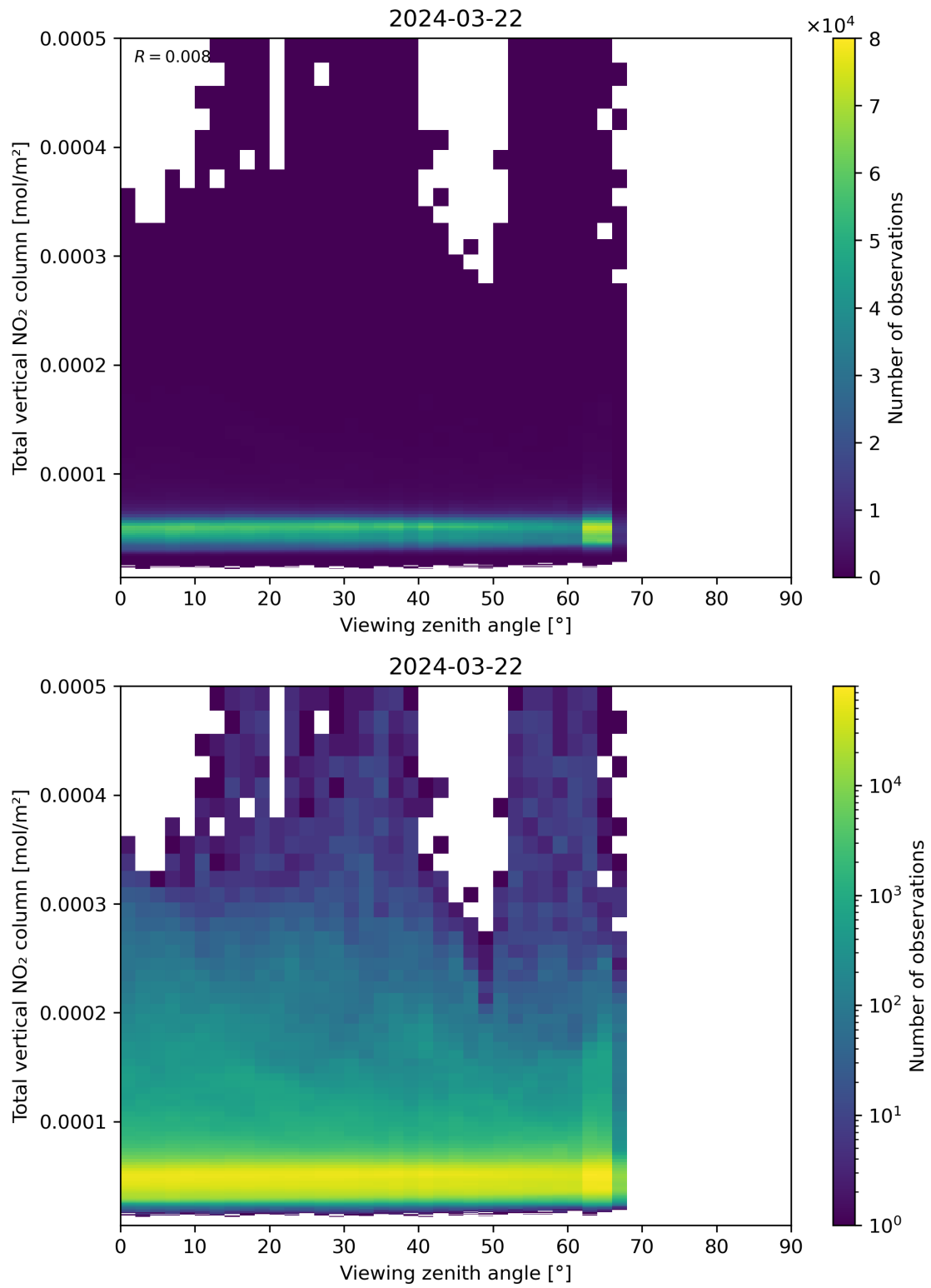
Figure 167: Scatter density plot of “Viewing zenith angle” against “Total vertical NO 2 column” for 2024-03-21 to 2024-03-22.
