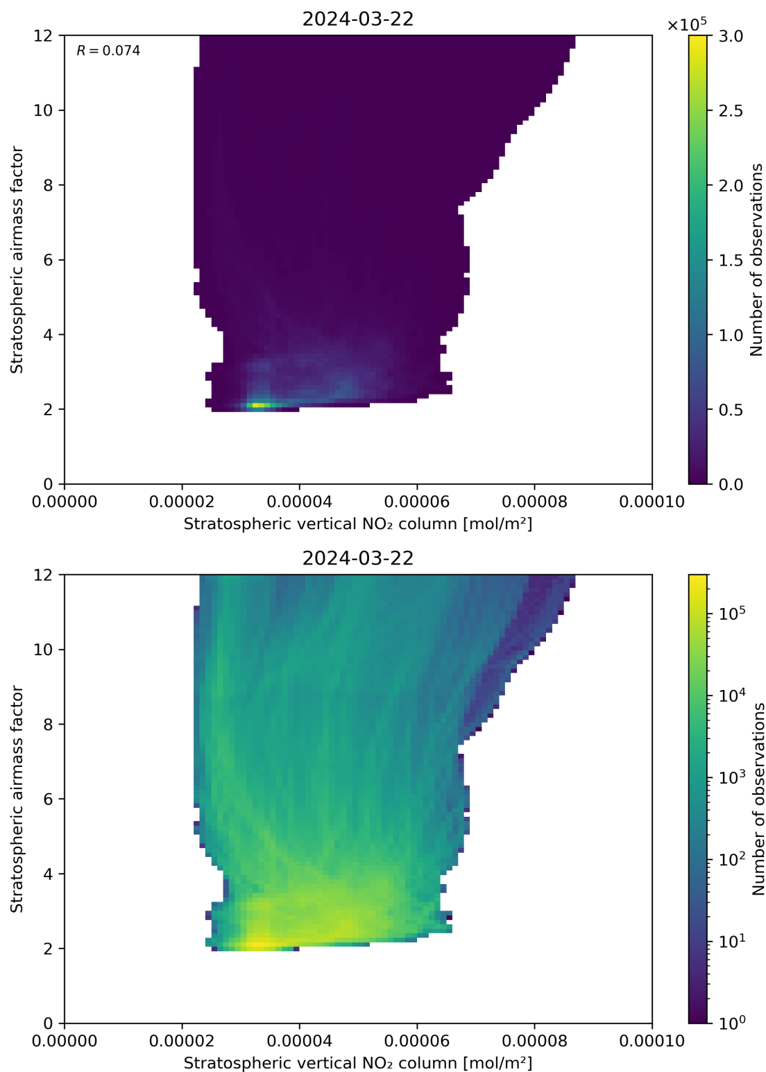
Figure 96: Scatter density plot of “Stratospheric vertical NO 2 column” against “Stratospheric airmass factor” for 2024-03-21 to 2024-03-22.
