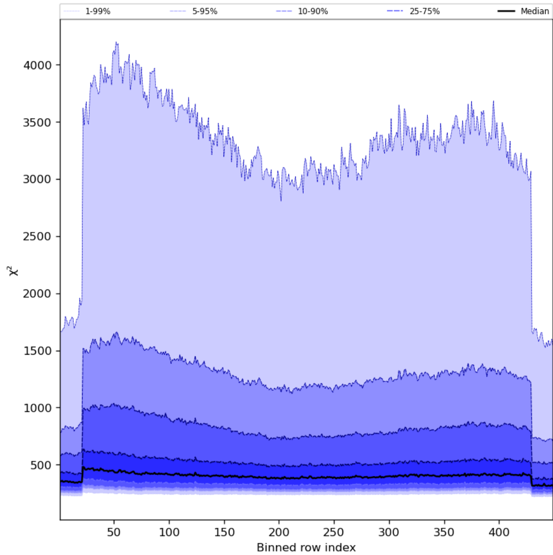
Figure 59: Along track statistics of “ \chi^2 ” for 2024-03-21 to 2024-03-22
