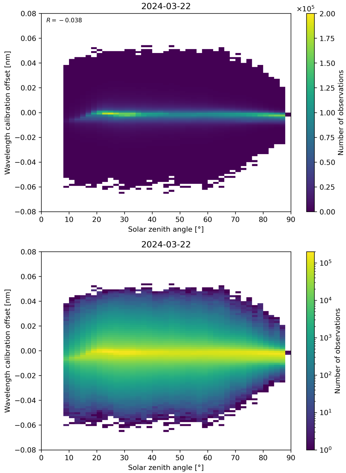
Figure 158: Scatter density plot of “Solar zenith angle” against “Wavelength calibration offset” for 2024-03-21 to 2024-03-22.
