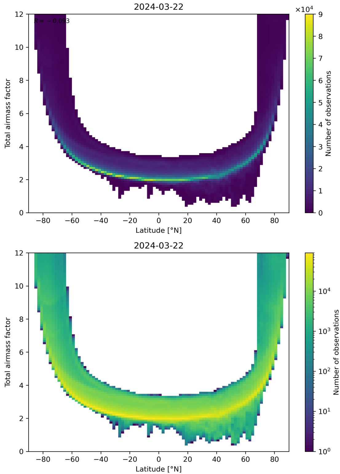
Figure 84: Scatter density plot of “Latitude” against “Total airmass factor” for 2024-03-21 to 2024-03-22.
