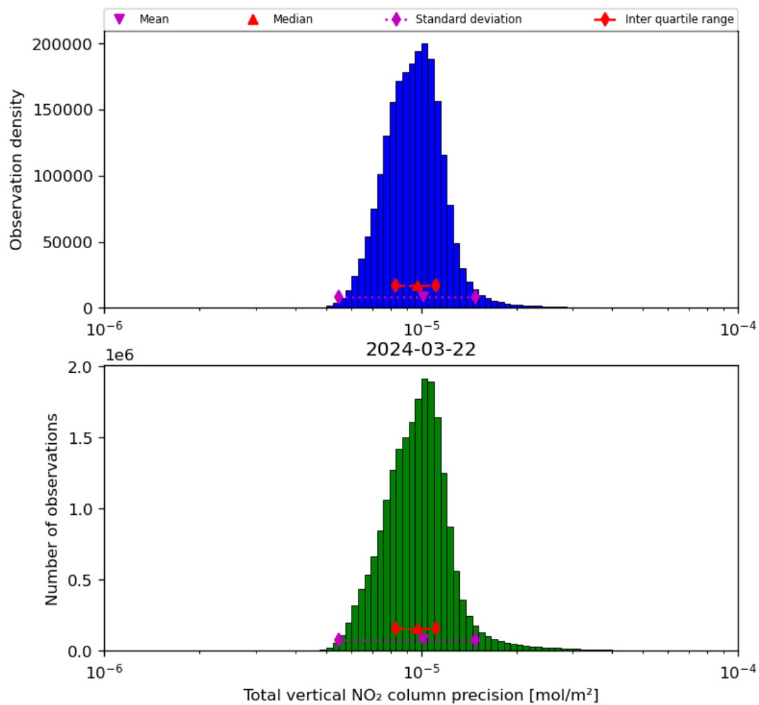
Figure 39: Histogram of “Total vertical NO 2 column precision” for 2024-03-21 to 2024-03-22
