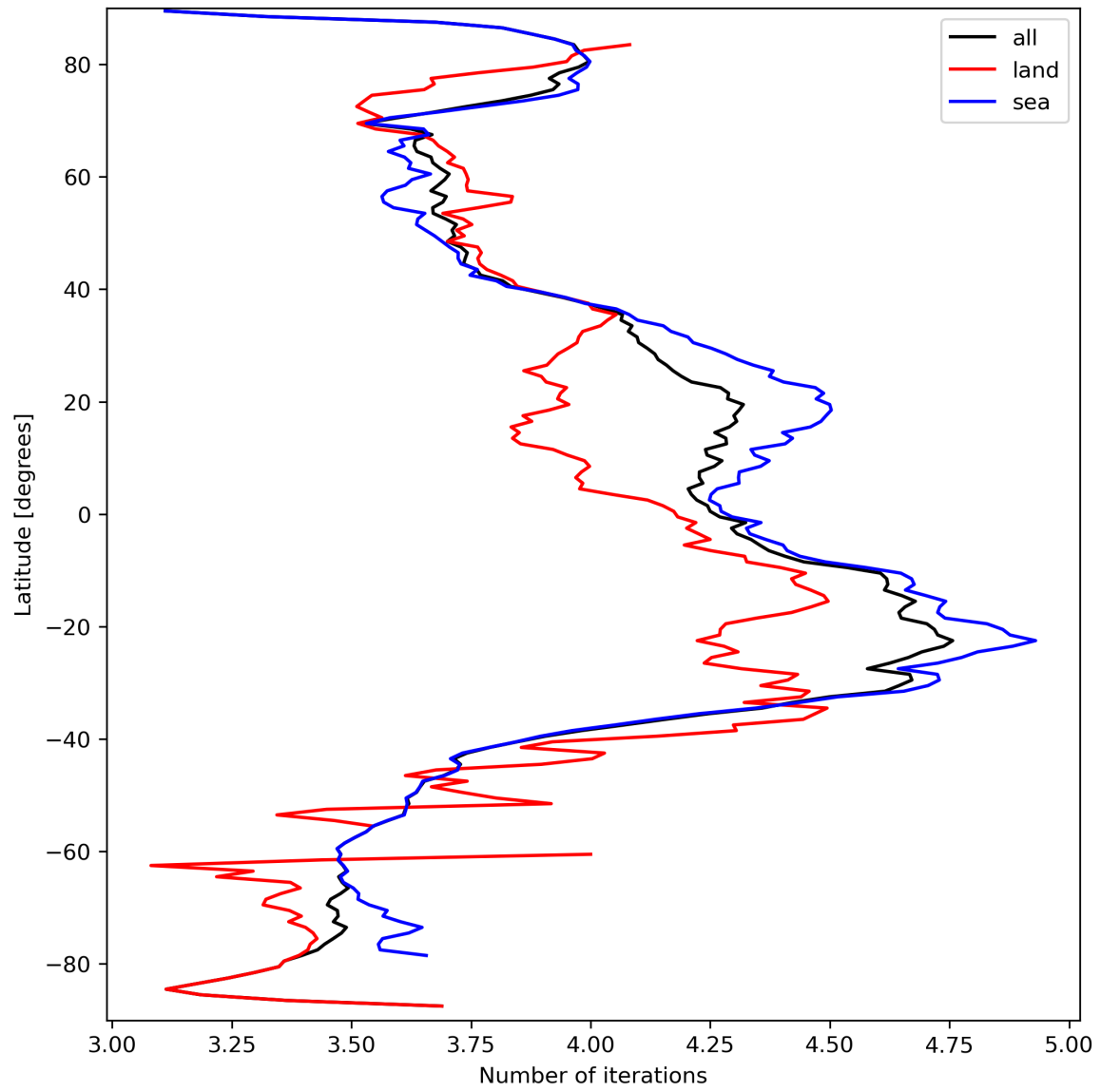
Figure 17: Zonal average of “Number of iterations” for 2024-03-21 to 2024-03-22.
