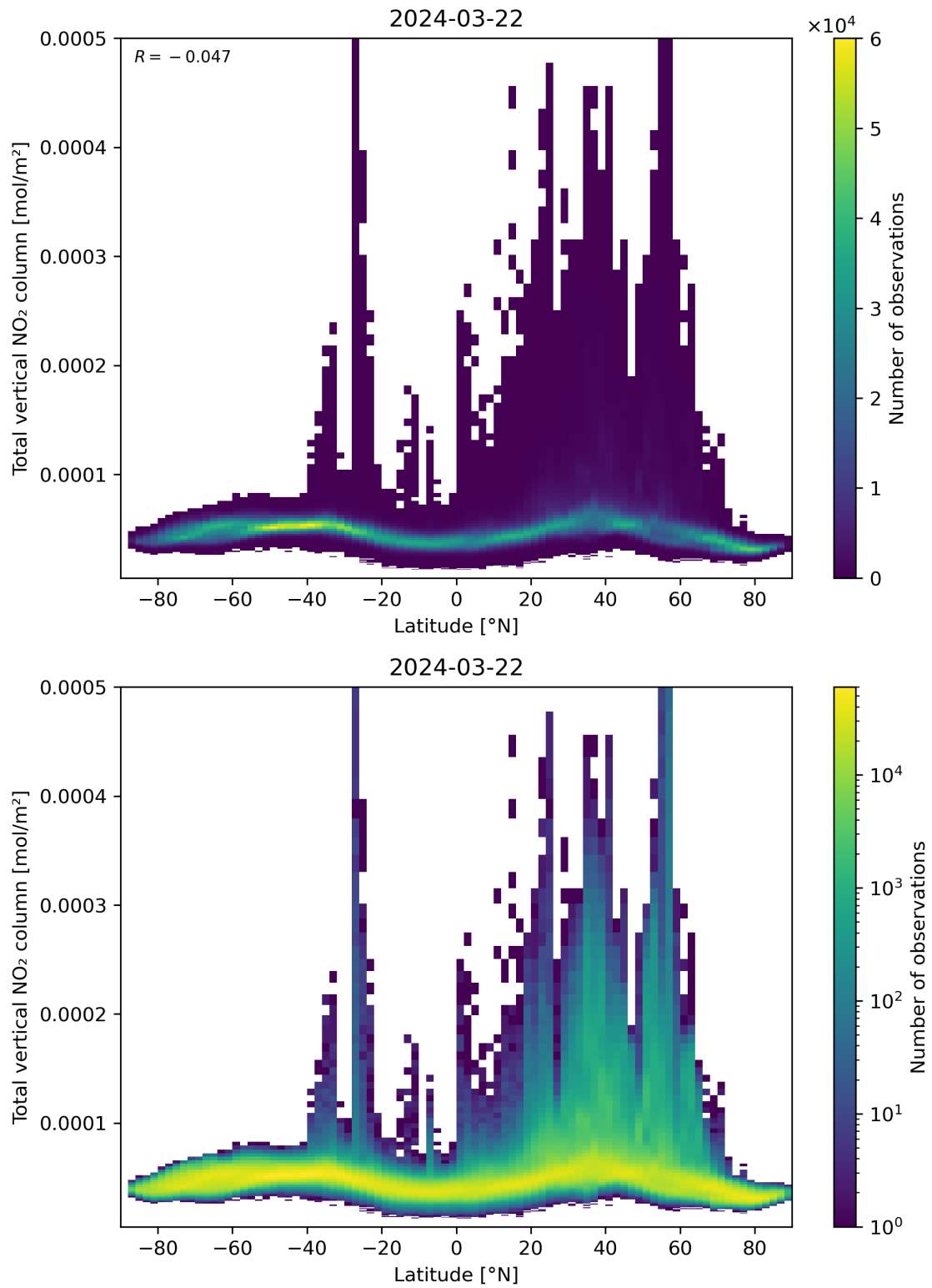
Figure 90: Scatter density plot of “Latitude” against “Total vertical NO 2 column” for 2024-03-21 to 2024-03-22.
