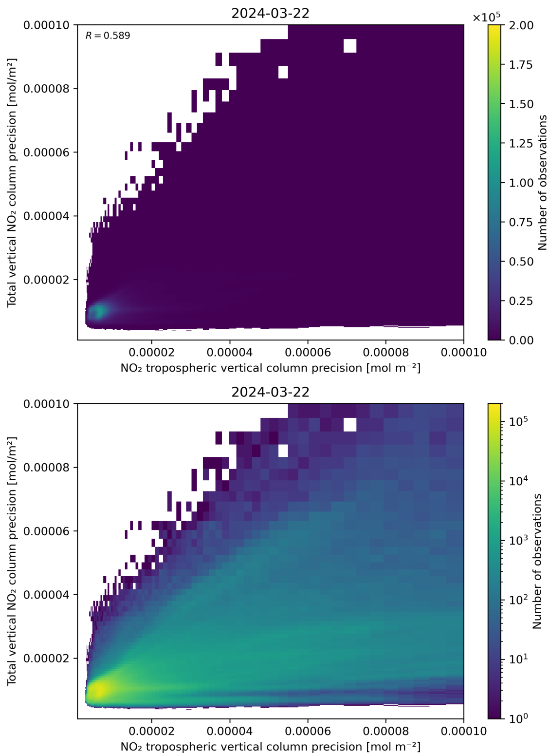
Figure 139: Scatter density plot of “NO 2 tropospheric vertical column precision” against “Total vertical NO 2 column precision” for 2024-03-21 to 2024-03-22.
