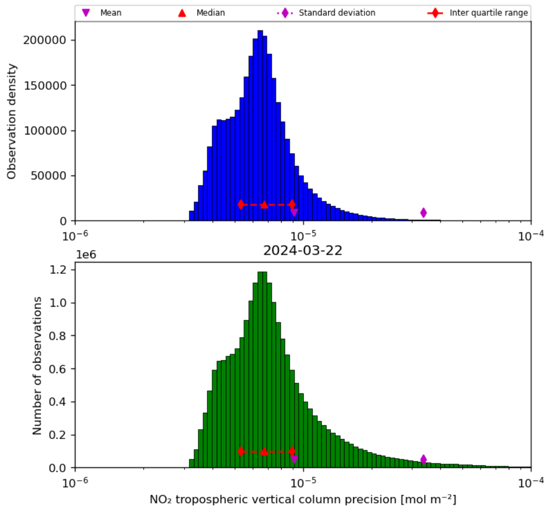
Figure 30: Histogram of “NO 2 tropospheric vertical column precision” for 2024-03-21 to 2024-03-22
