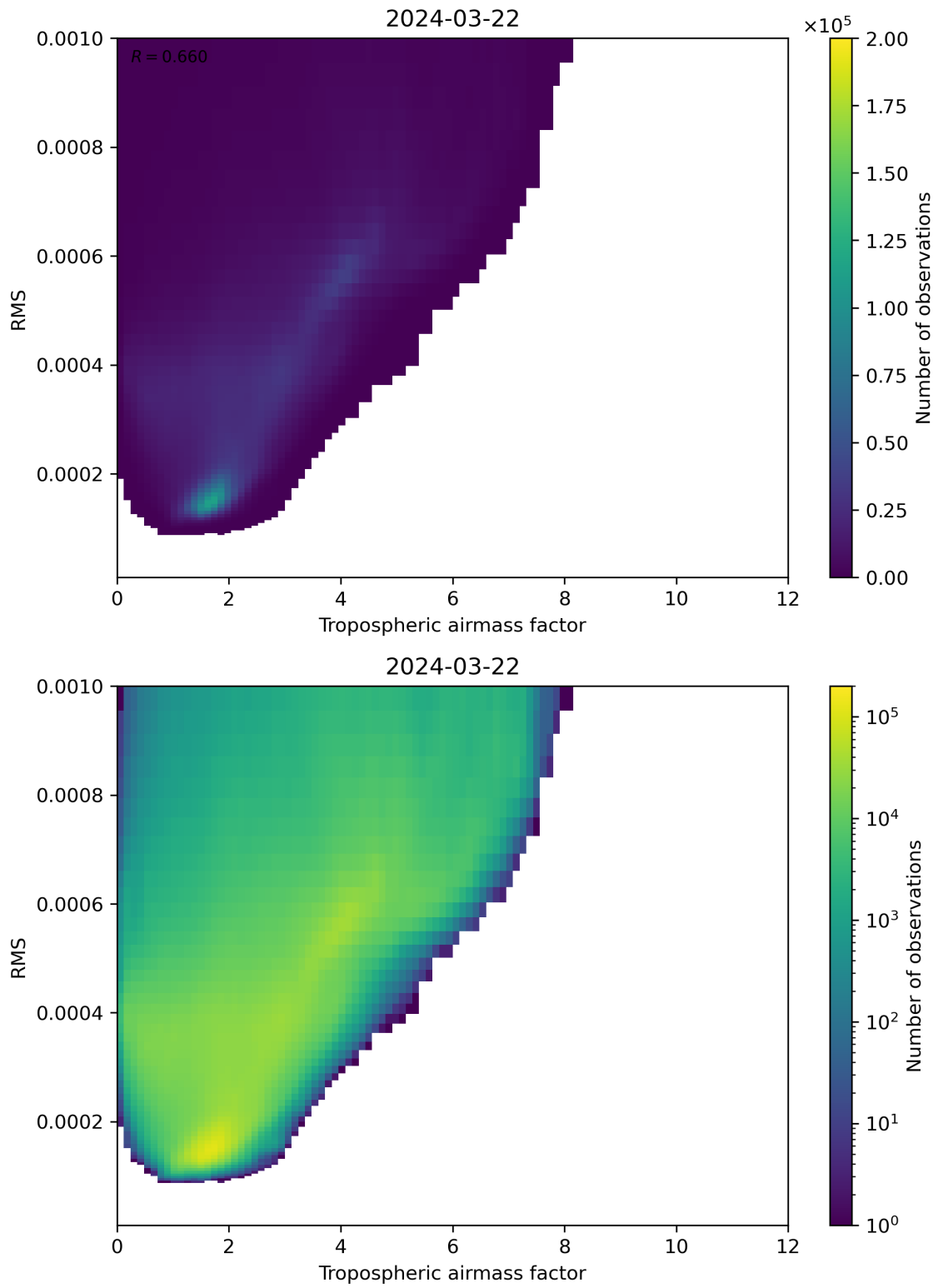
Figure 79: Scatter density plot of “Tropospheric airmass factor” against “RMS” for 2024-03-21 to 2024-03-22.
