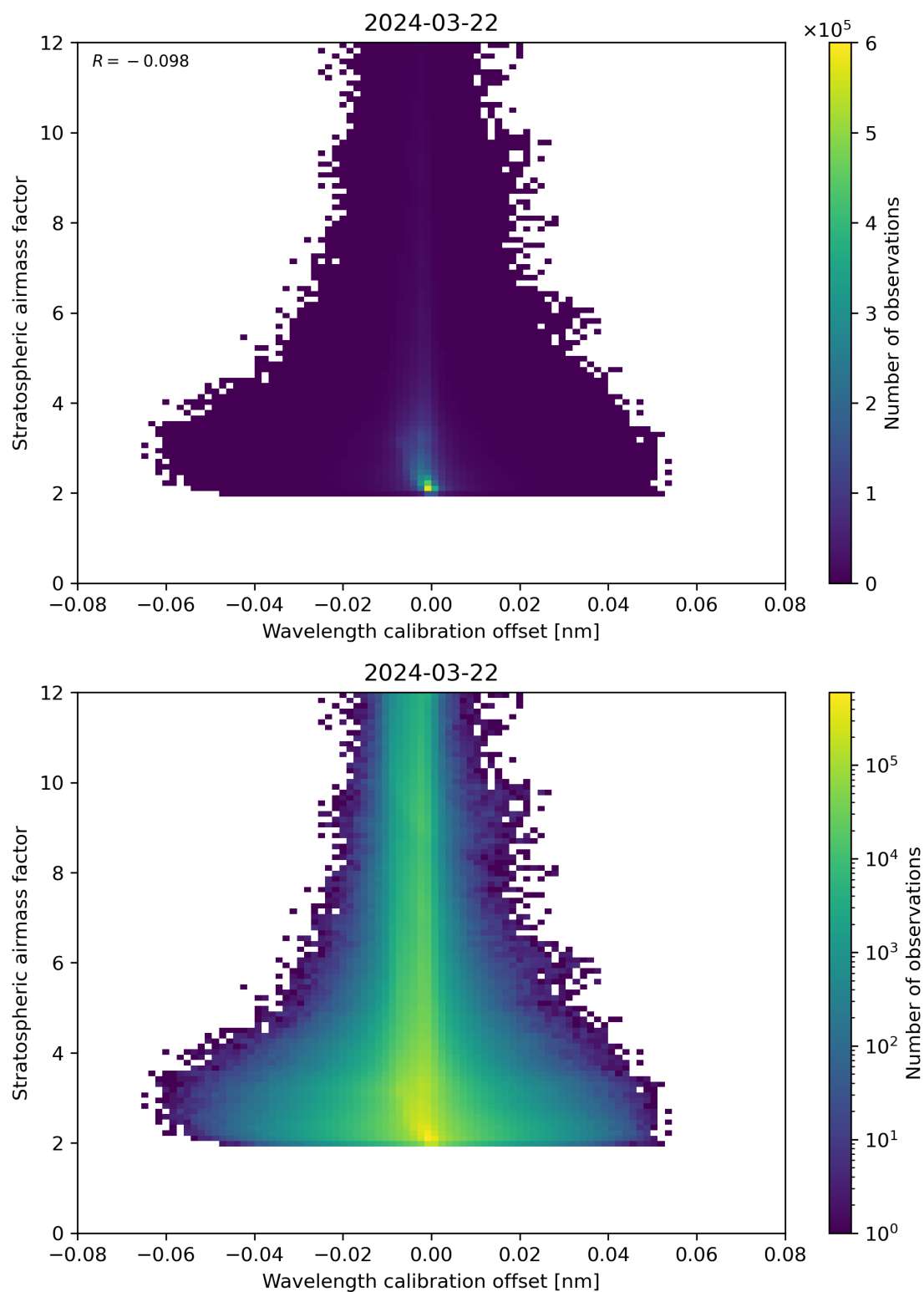
Figure 174: Scatter density plot of “Wavelength calibration offset” against “Stratospheric airmass factor” for 2024-03-21 to 2024-03-22.
