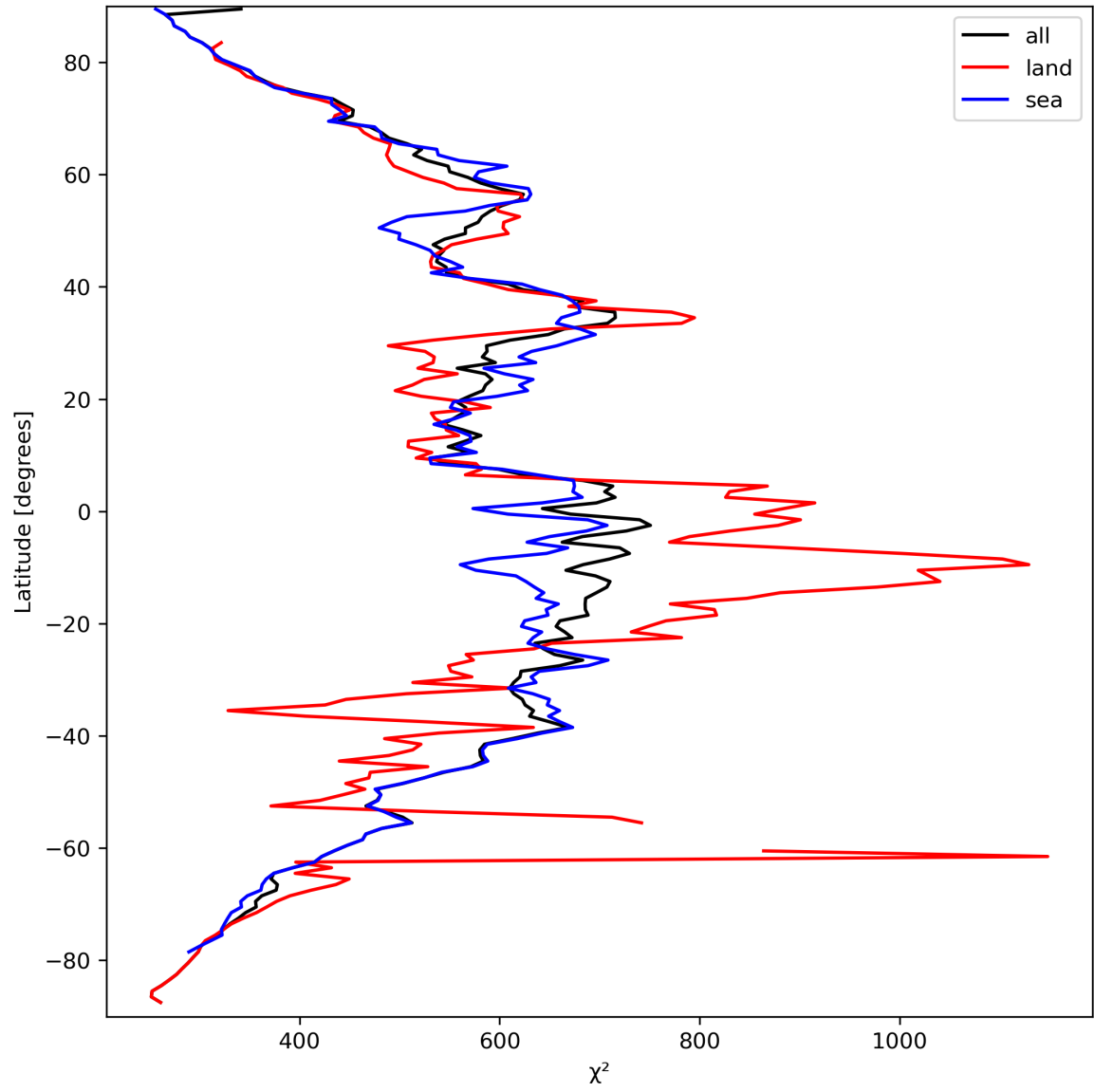
Figure 25: Zonal average of “ \chi^2 ” for 2024-03-21 to 2024-03-22.
