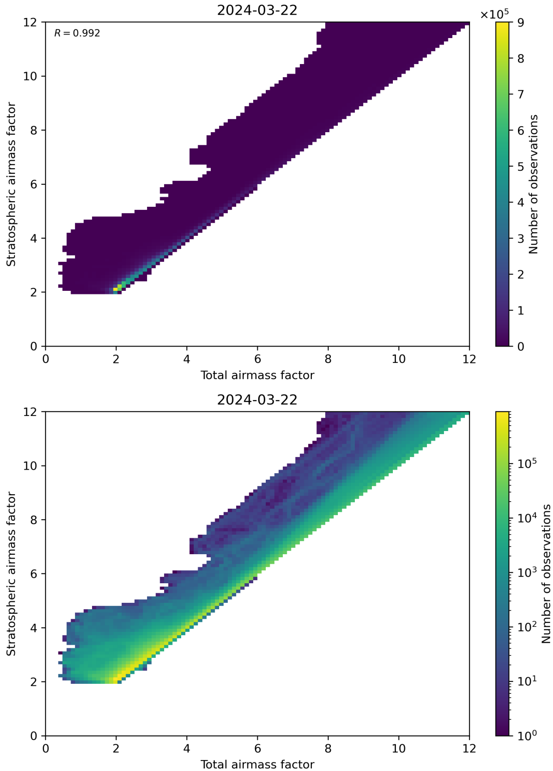
Figure 62: Scatter density plot of “Total airmass factor” against “Stratospheric airmass factor” for 2024-03-21 to 2024-03-22.
