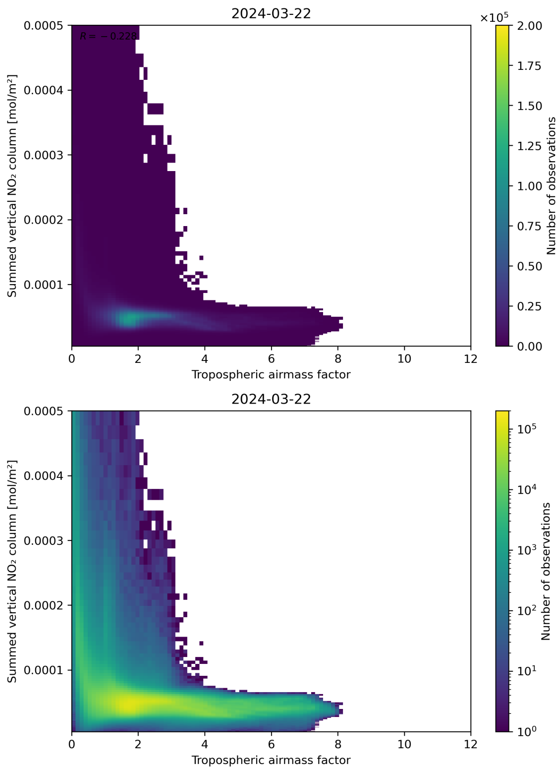
Figure 75: Scatter density plot of “Tropospheric airmass factor” against “Summed vertical NO 2 column” for 2024-03-21 to 2024-03-22.
