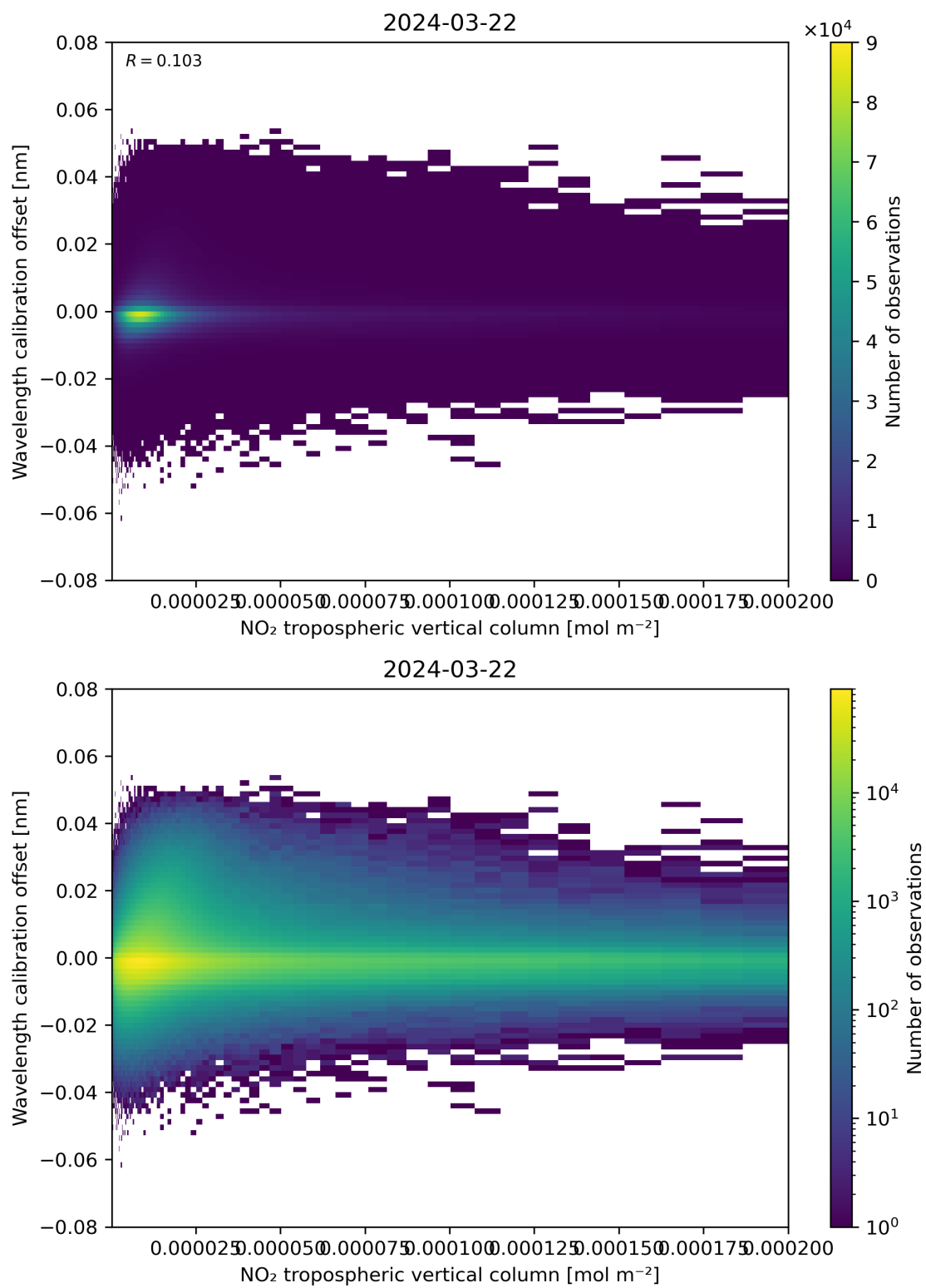
Figure 143: Scatter density plot of “NO 2 tropospheric vertical column” against “Wavelength calibration offset” for 2024-03-21 to 2024-03-22.
