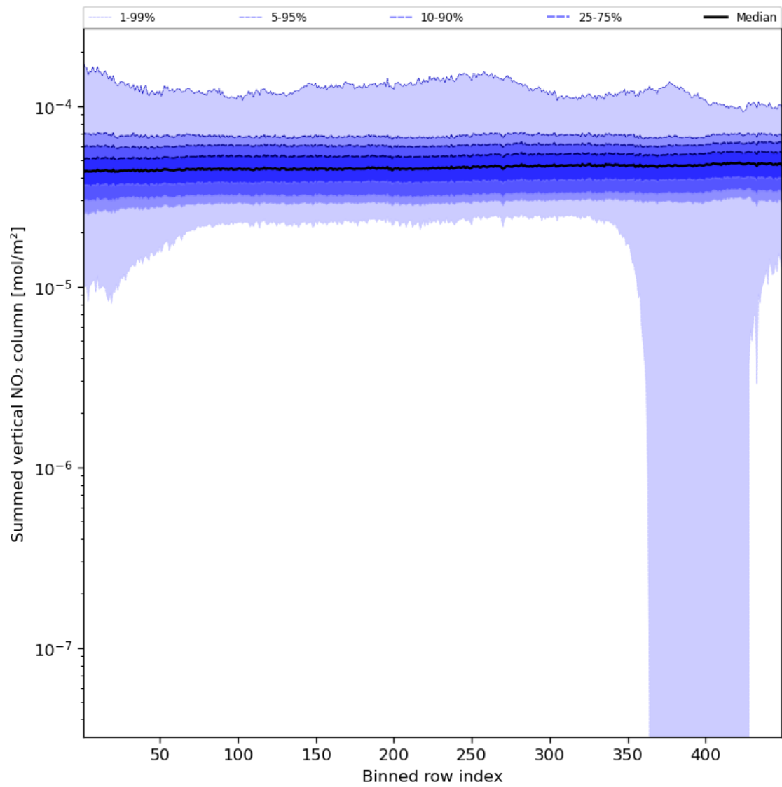
Figure 57: Along track statistics of “Summed vertical NO 2 column” for 2024-03-21 to 2024-03-22
