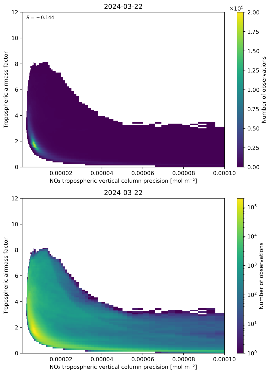
Figure 133: Scatter density plot of “NO 2 tropospheric vertical column precision” against “Tropospheric airmass factor” for 2024-03-21 to 2024-03-22.
