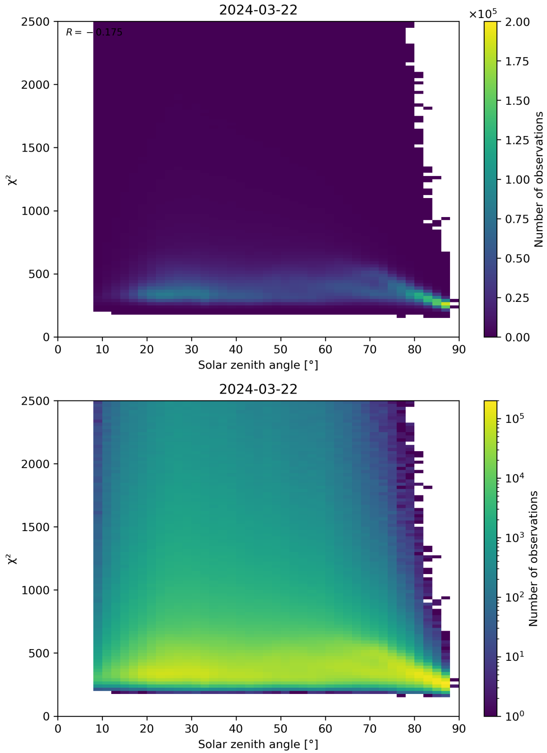
Figure 148: Scatter density plot of “Solar zenith angle” against “ \chi^2 ” for 2024-03-21 to 2024-03-22.
