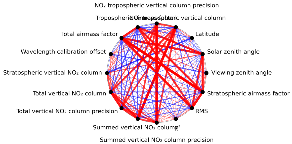
Figure 1: Map of correlation graph for 2024-03-21 to 2024-03-22.
