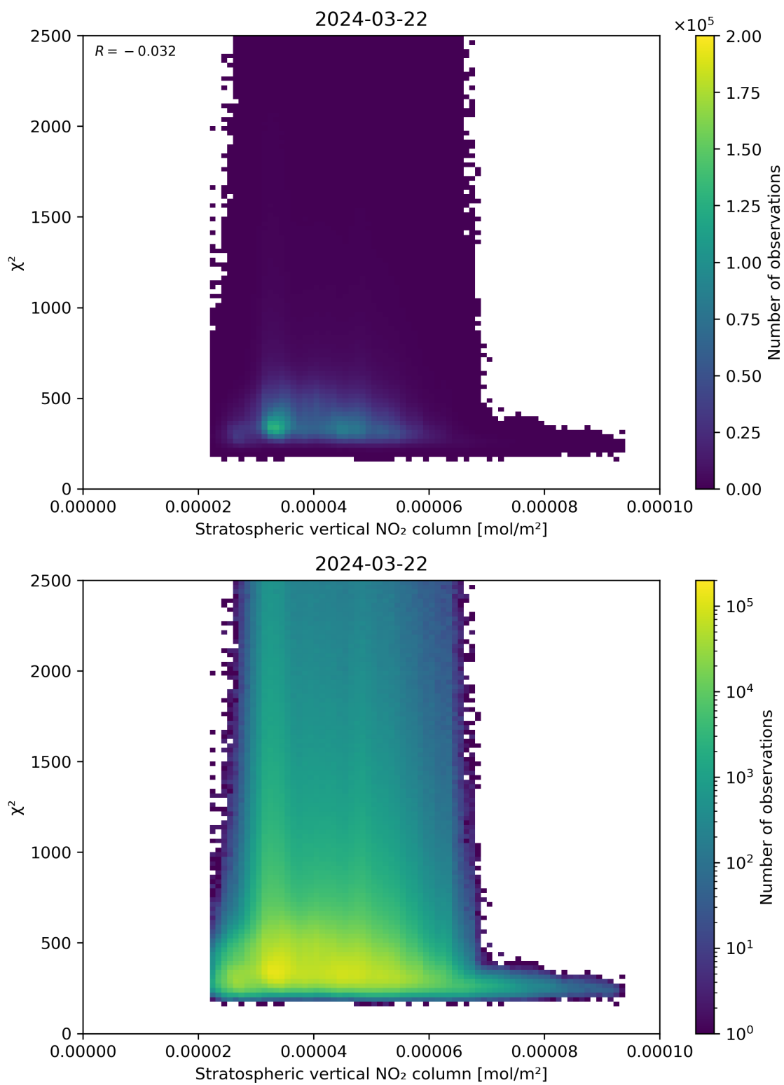
Figure 97: Scatter density plot of “Stratospheric vertical NO 2 column” against “ \chi^2 ” for 2024-03-21 to 2024-03-22.
