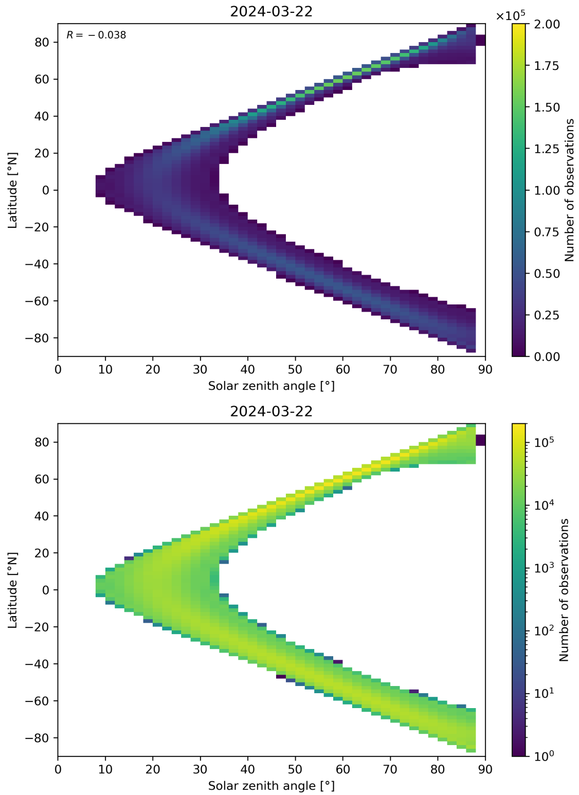
Figure 149: Scatter density plot of “Solar zenith angle” against “Latitude” for 2024-03-21 to 2024-03-22.
