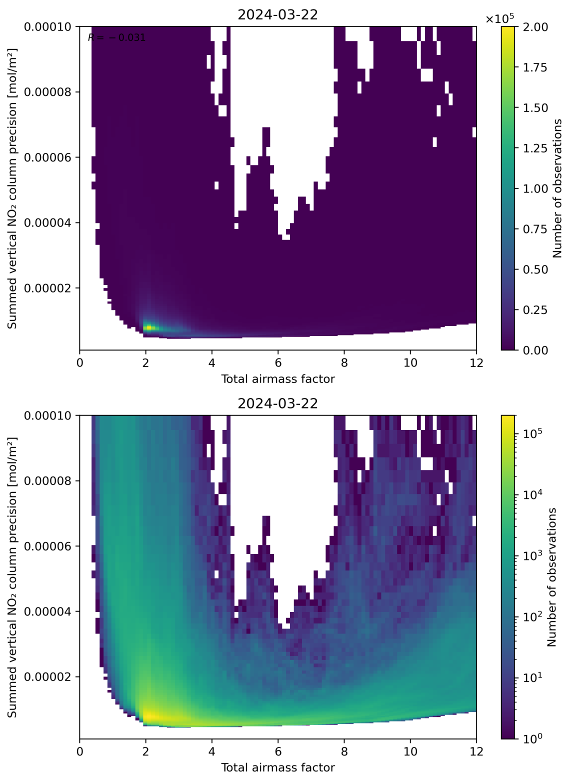
Figure 66: Scatter density plot of “Total airmass factor” against “Summed vertical NO 2 column precision” for 2024-03-21 to 2024-03-22.
