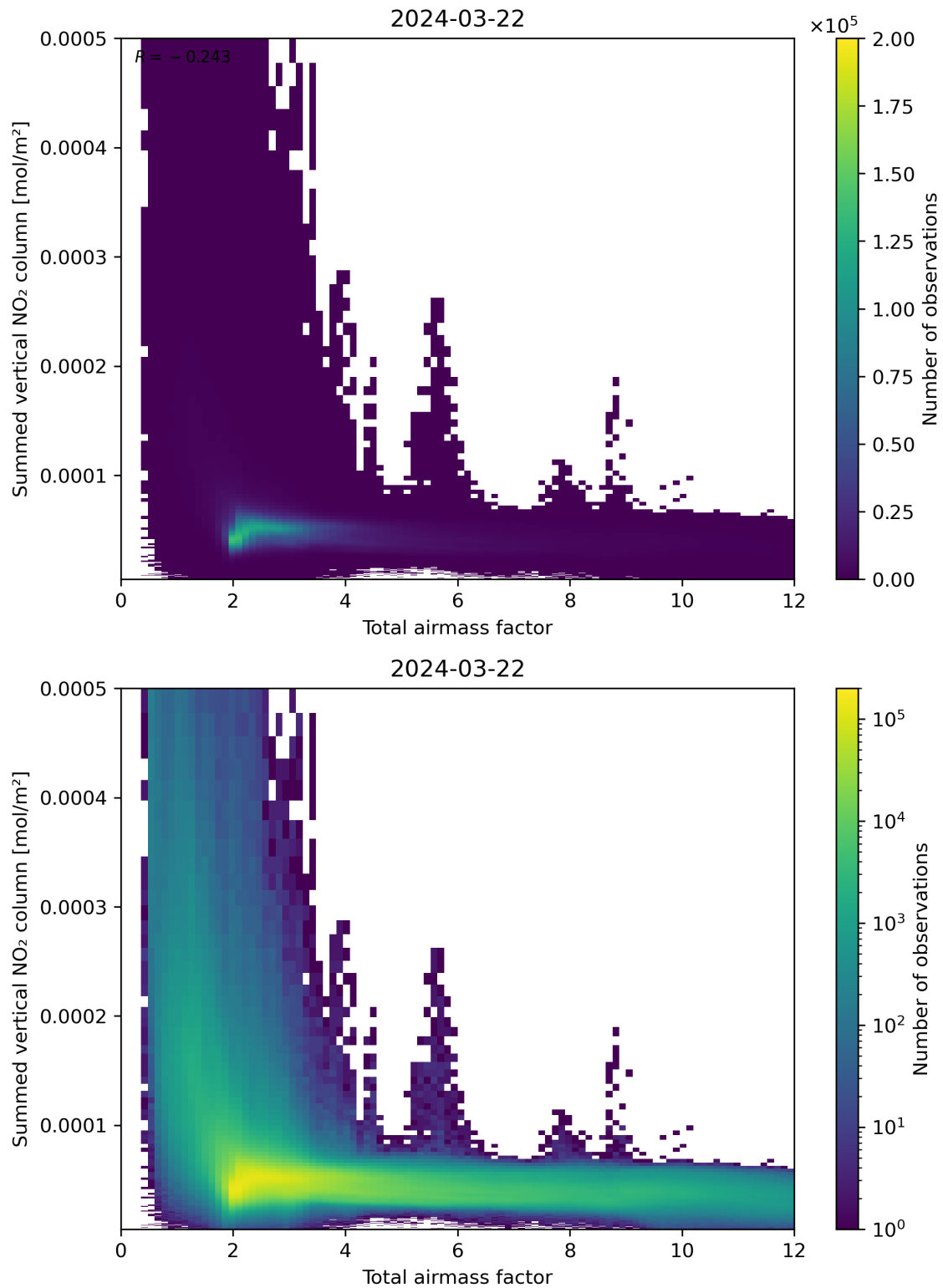
Figure 65: Scatter density plot of “Total airmass factor” against “Summed vertical NO 2 column” for 2024-03-21 to 2024-03-22.
