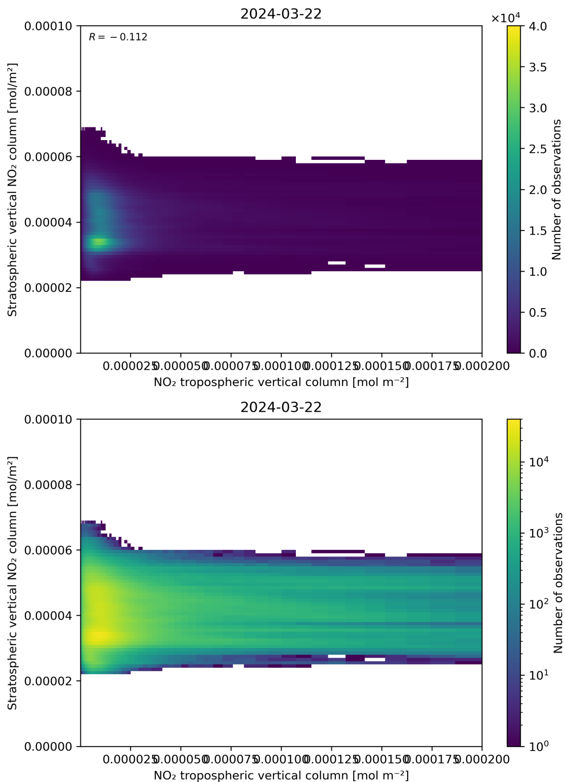
Figure 125: Scatter density plot of “NO 2 tropospheric vertical column” against “Stratospheric vertical NO 2 column” for 2024-03-21 to 2024-03-22.
