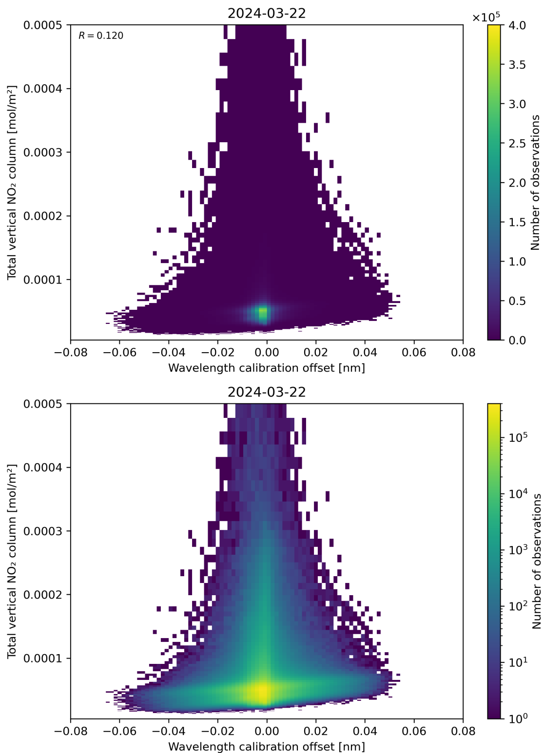
Figure 179: Scatter density plot of “Wavelength calibration offset” against “Total vertical NO 2 column” for 2024-03-21 to 2024-03-22.
