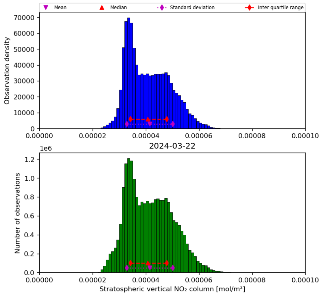
Figure 36: Histogram of “Stratospheric vertical NO 2 column” for 2024-03-21 to 2024-03-22
