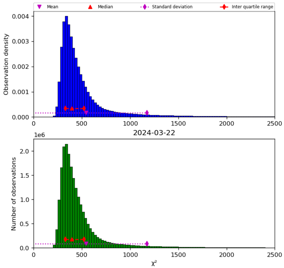
Figure 42: Histogram of “ \chi^2 ” for 2024-03-21 to 2024-03-22
