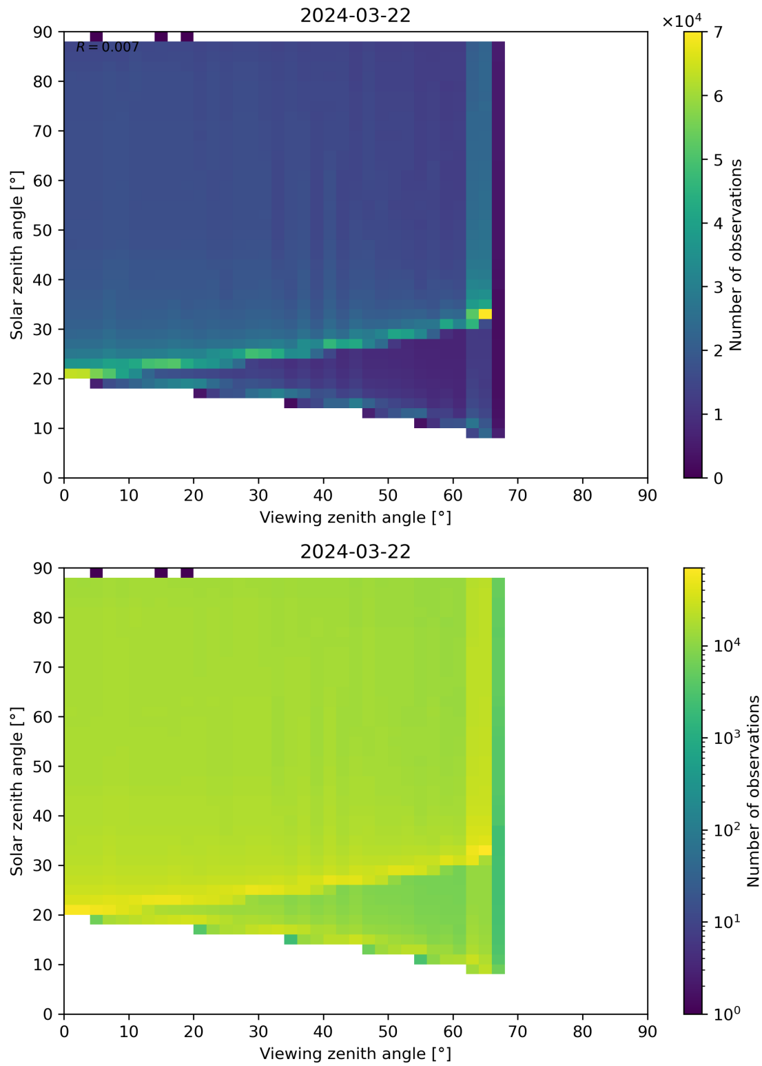
Figure 172: Scatter density plot of “Viewing zenith angle” against “Solar zenith angle” for 2024-03-21 to 2024-03-22.
