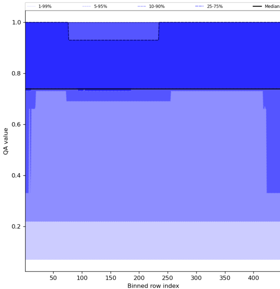
Figure 45: Along track statistics of "QA value" for 2024-03-21 to 2024-03-22
