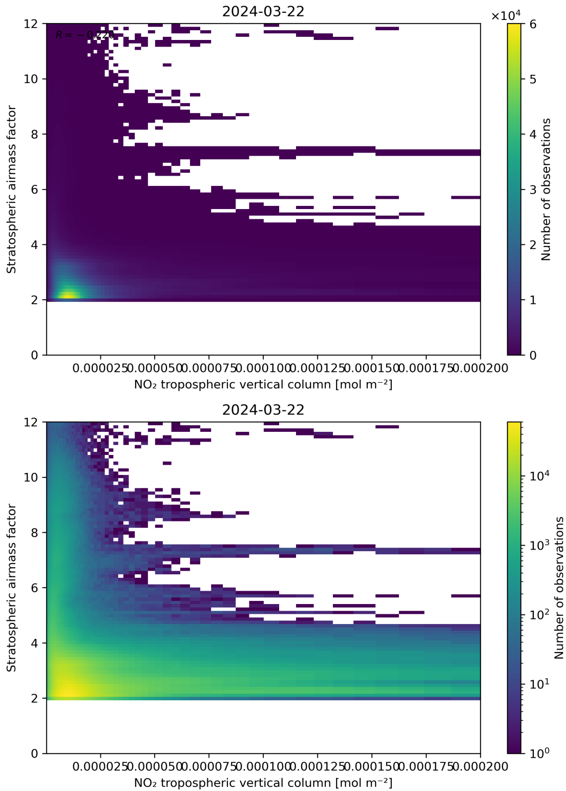
Figure 121: Scatter density plot of “NO 2 tropospheric vertical column” against “Stratospheric air mass factor” for 2024-03-21 to 2024-03-22.
