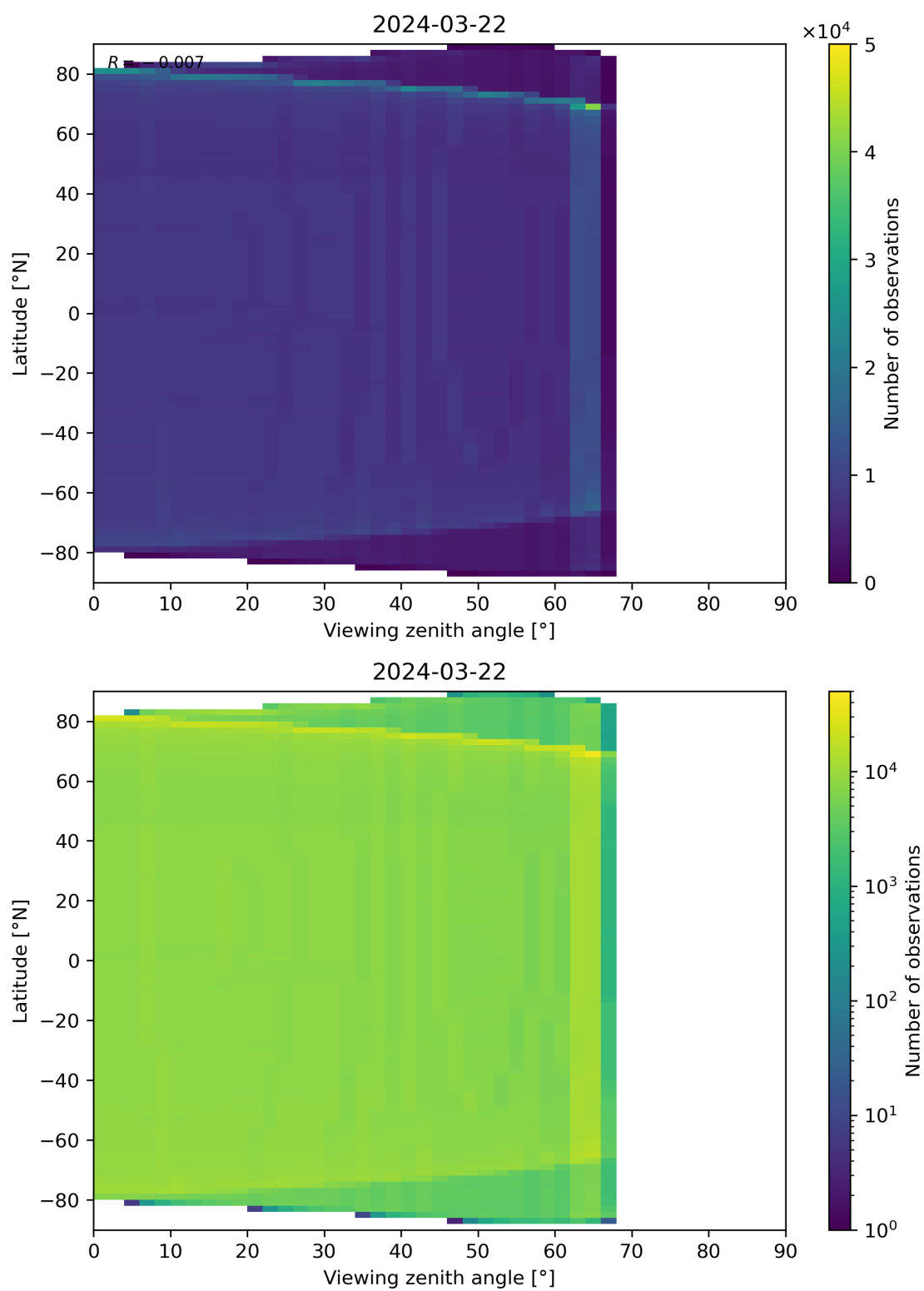
Figure 163: Scatter density plot of “Viewing zenith angle” against “Latitude” for 2024-03-21 to 2024-03-22.
