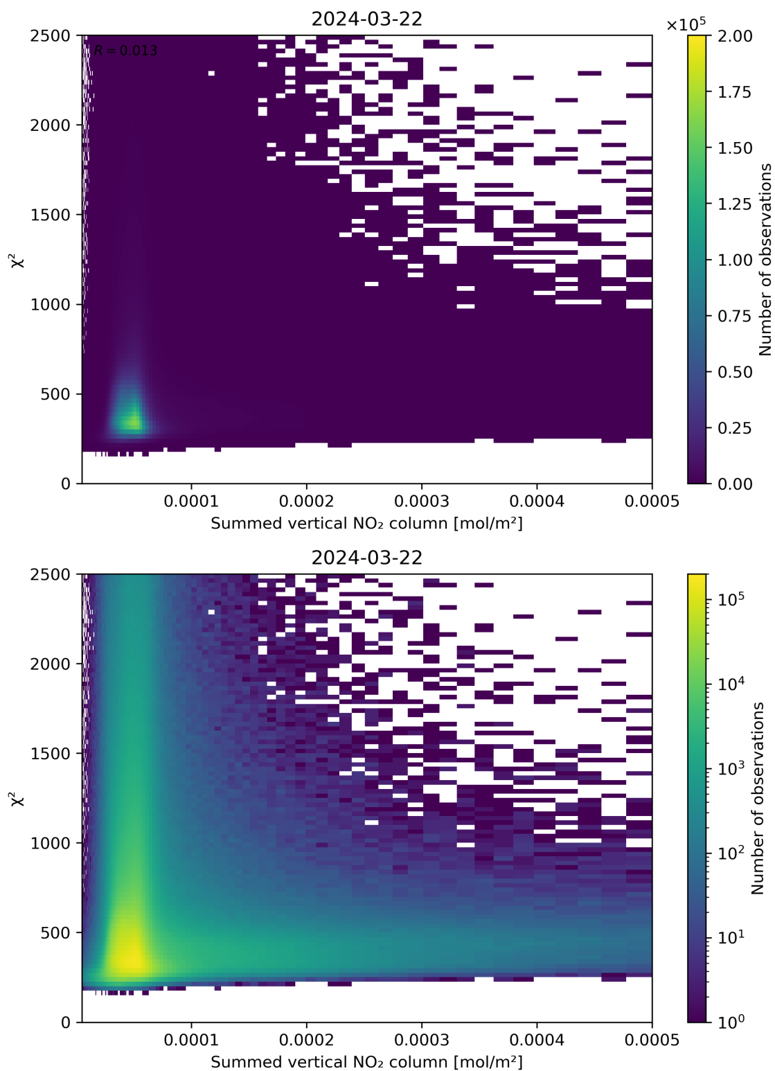
Figure 104: Scatter density plot of “Summed vertical NO 2 column” against “ \chi^2 ” for 2024-03-21 to 2024-03-22.
