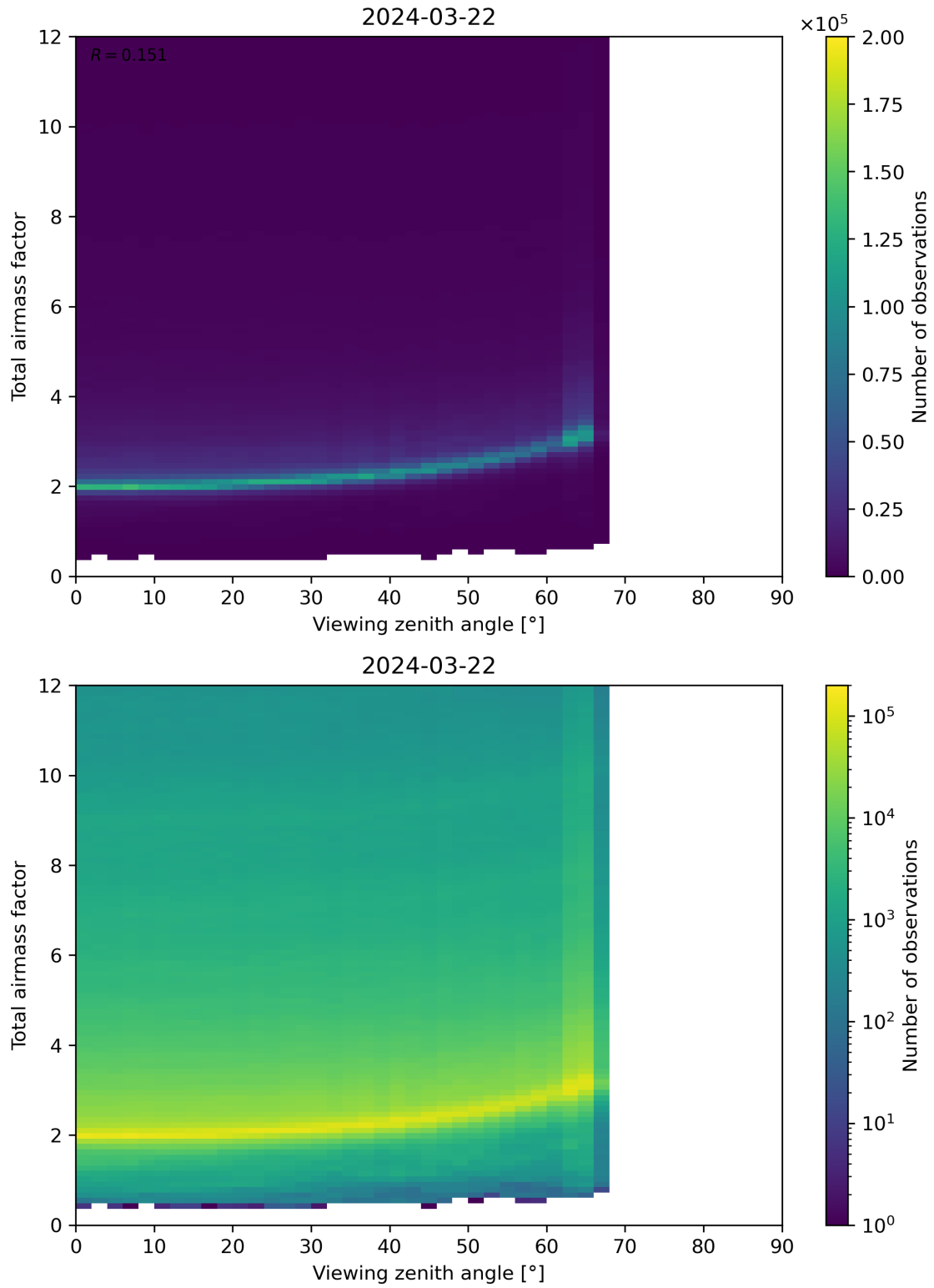
Figure 160: Scatter density plot of “Viewing zenith angle” against “Total airmass factor” for 2024-03-21 to 2024-03-22.
