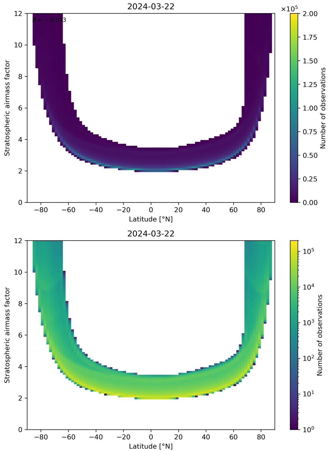
Figure 83: Scatter density plot of “Latitude” against “Stratospheric air mass factor” for 2024-03-21 to 2024-03-22.
