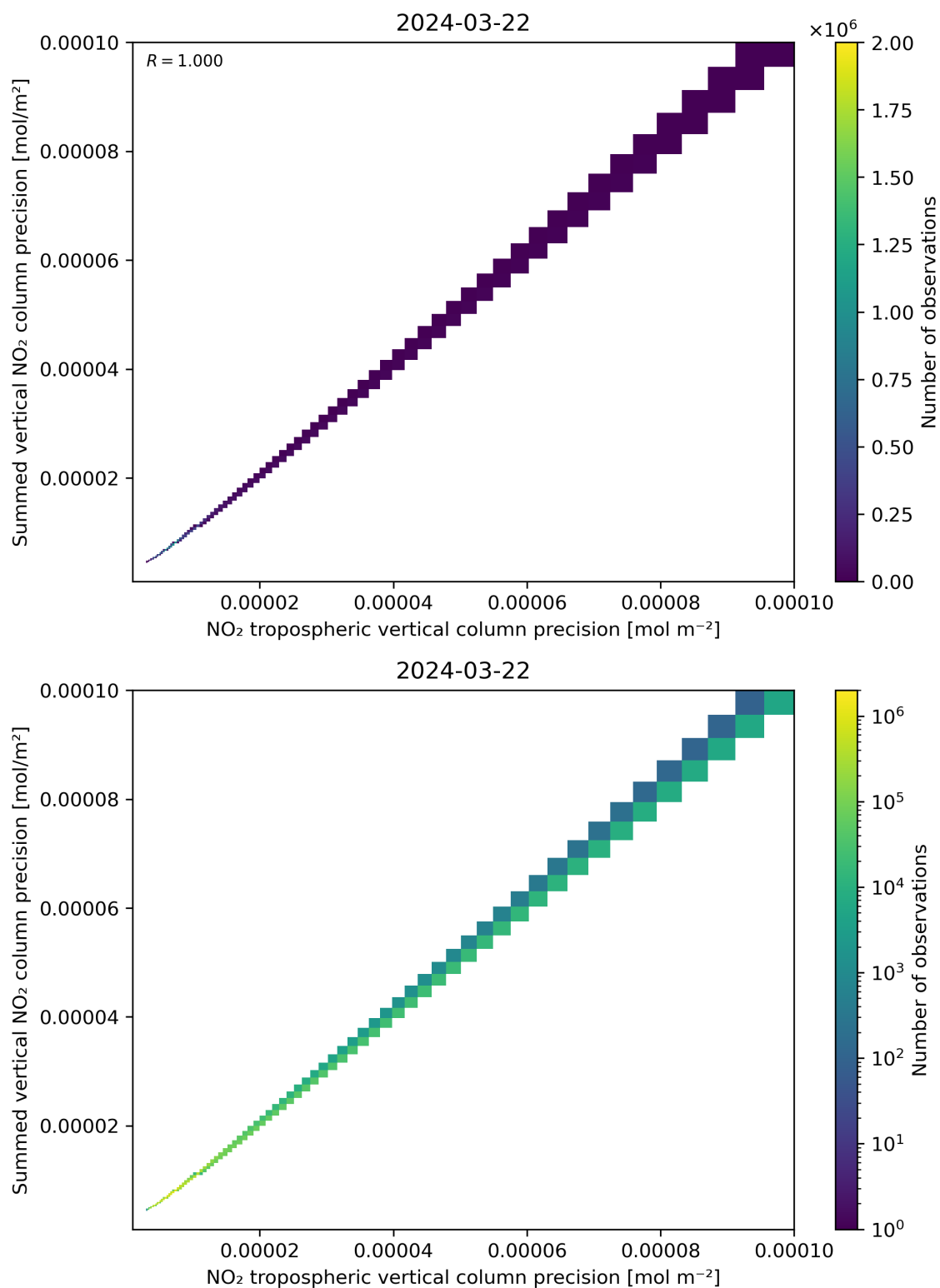
Figure 137: Scatter density plot of “NO 2 tropospheric vertical column precision” against “Summed vertical NO 2 column precision” for 2024-03-21 to 2024-03-22.
