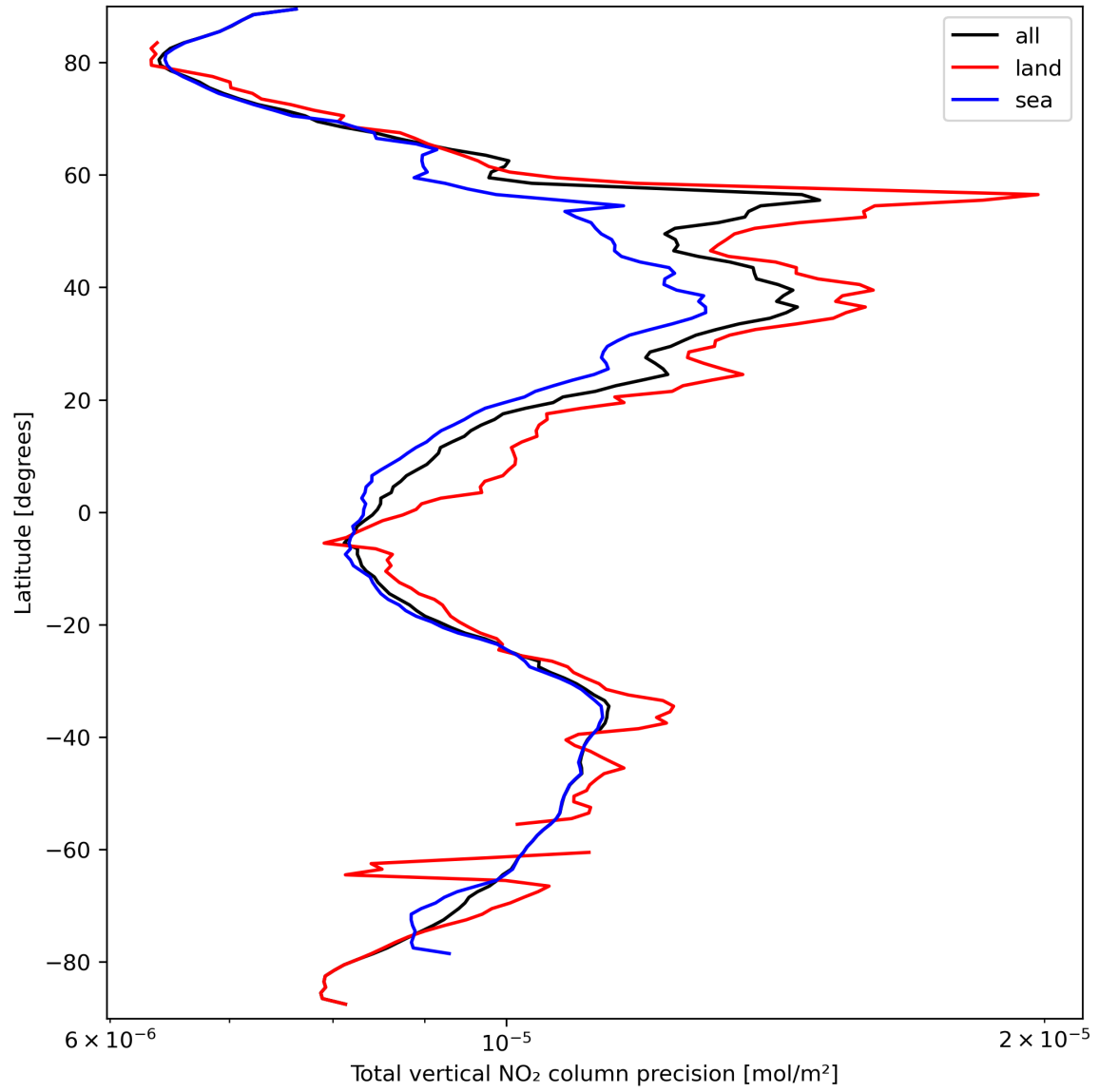
Figure 22: Zonal average of “Total vertical NO 2 column precision” for 2024-03-21 to 2024-03-22.
