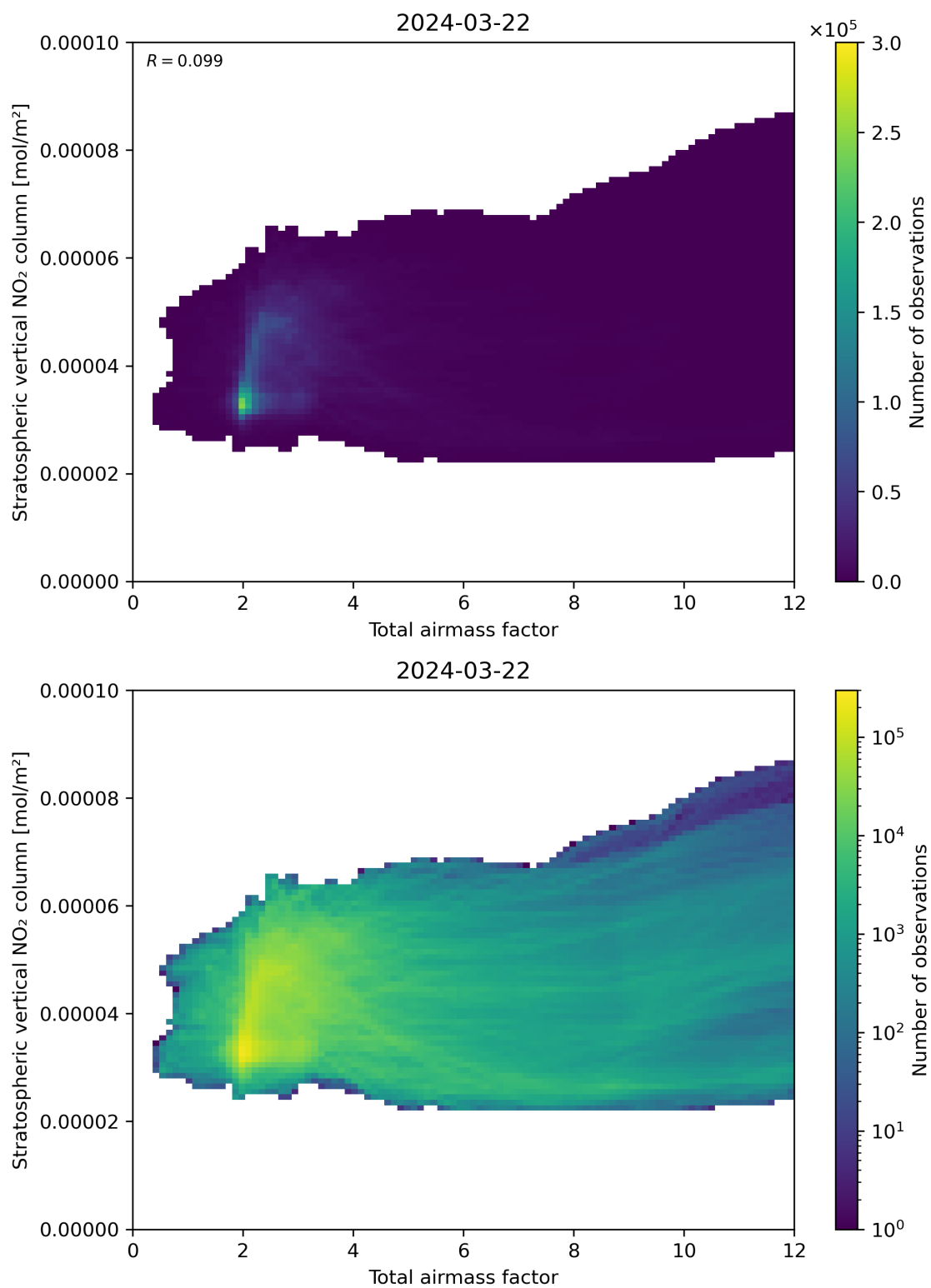
Figure 64: Scatter density plot of “Total airmass factor” against “Stratospheric vertical NO 2 column” for 2024-03-21 to 2024-03-22.
