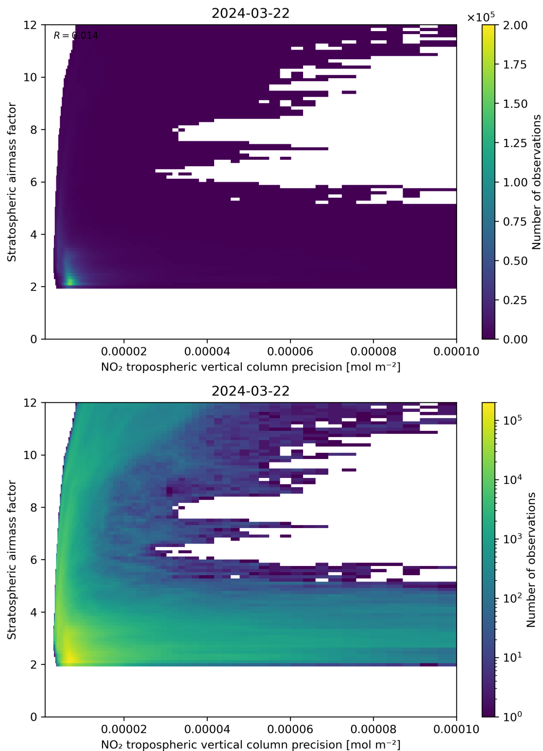
Figure 131: Scatter density plot of “NO 2 tropospheric vertical column precision” against “Stratospheric airmass factor” for 2024-03-21 to 2024-03-22.
