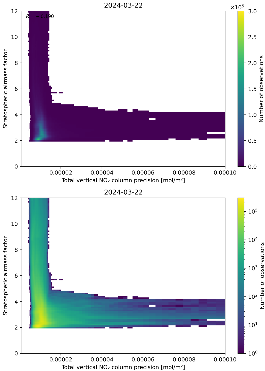
Figure 115: Scatter density plot of “Total vertical NO 2 column precision” against “Stratospheric air mass factor” for 2024-03-21 to 2024-03-22.
