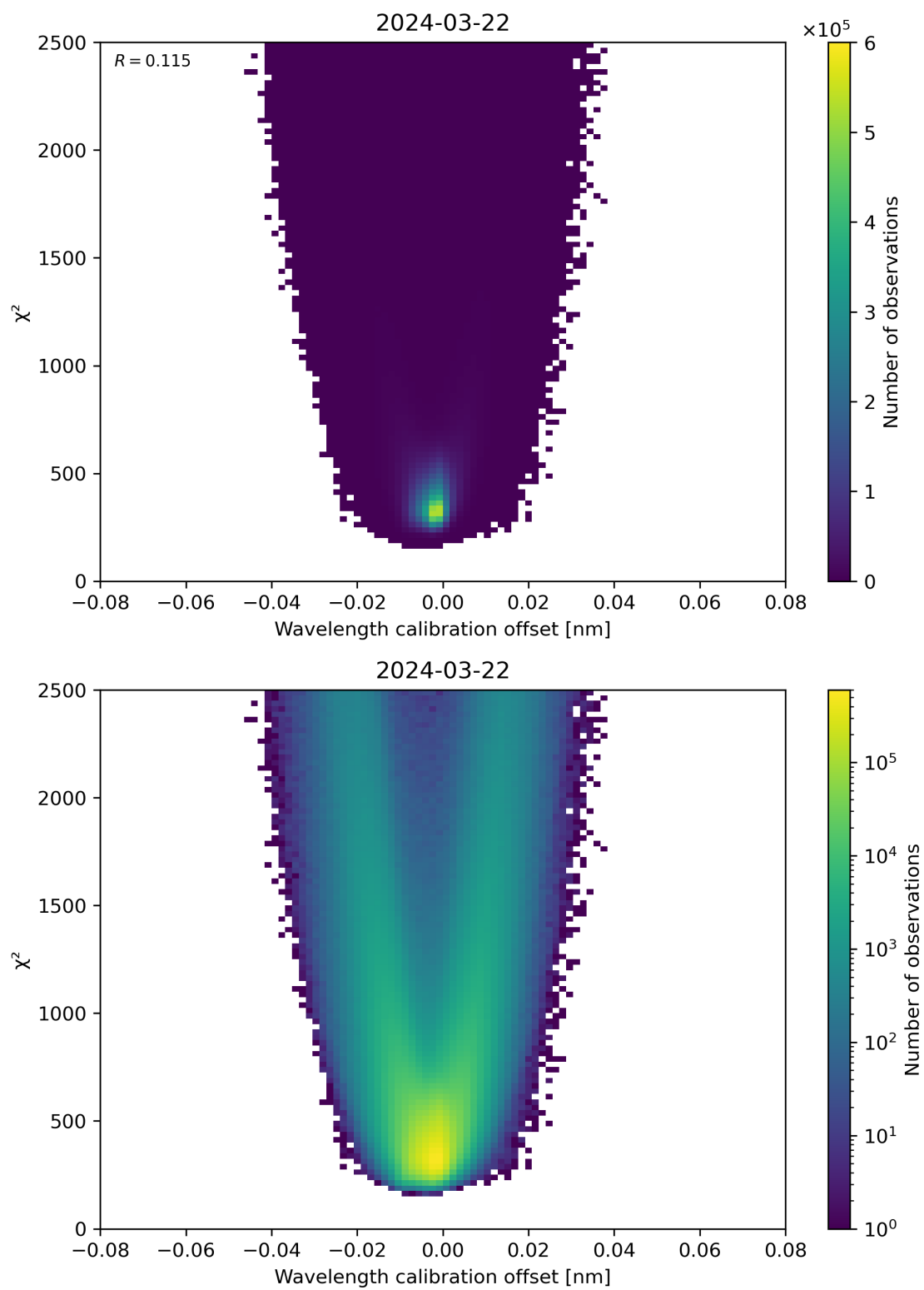
Figure 175: Scatter density plot of “Wavelength calibration offset” against “ \chi^2 ” for 2024-03-21 to 2024-03-22.
