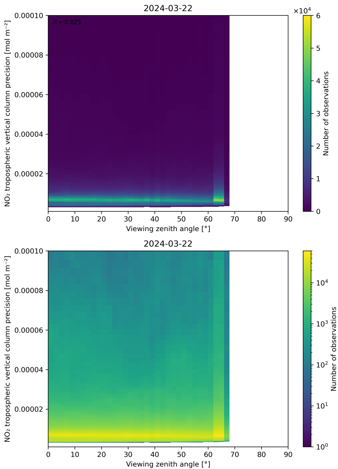
Figure 170: Scatter density plot of “Viewing zenith angle” against “NO 2 tropospheric vertical column precision” for 2024-03-21 to 2024-03-22.
