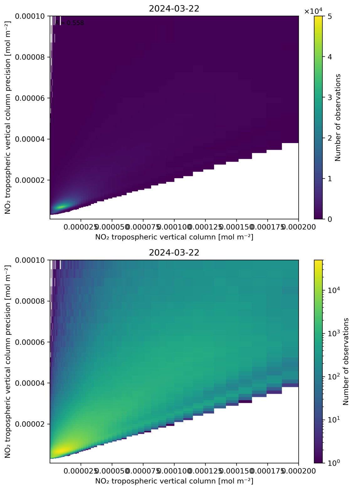
Figure 130: Scatter density plot of “NO 2 tropospheric vertical column” against “NO 2 tropospheric vertical column precision” for 2024-03-21 to 2024-03-22.
