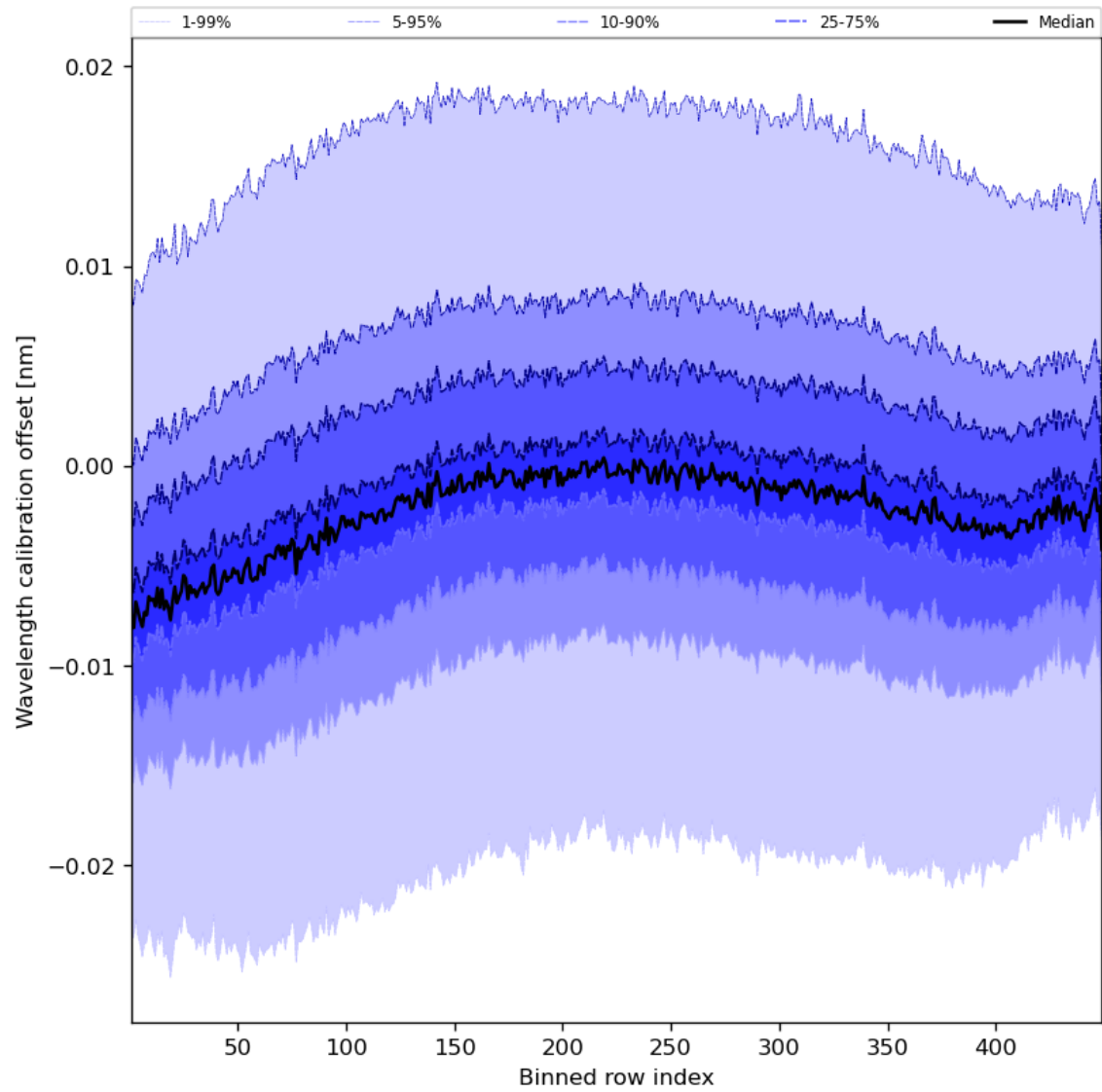
Figure 52: Along track statistics of “Wavelength calibration offset” for 2024-03-21 to 2024-03-22
