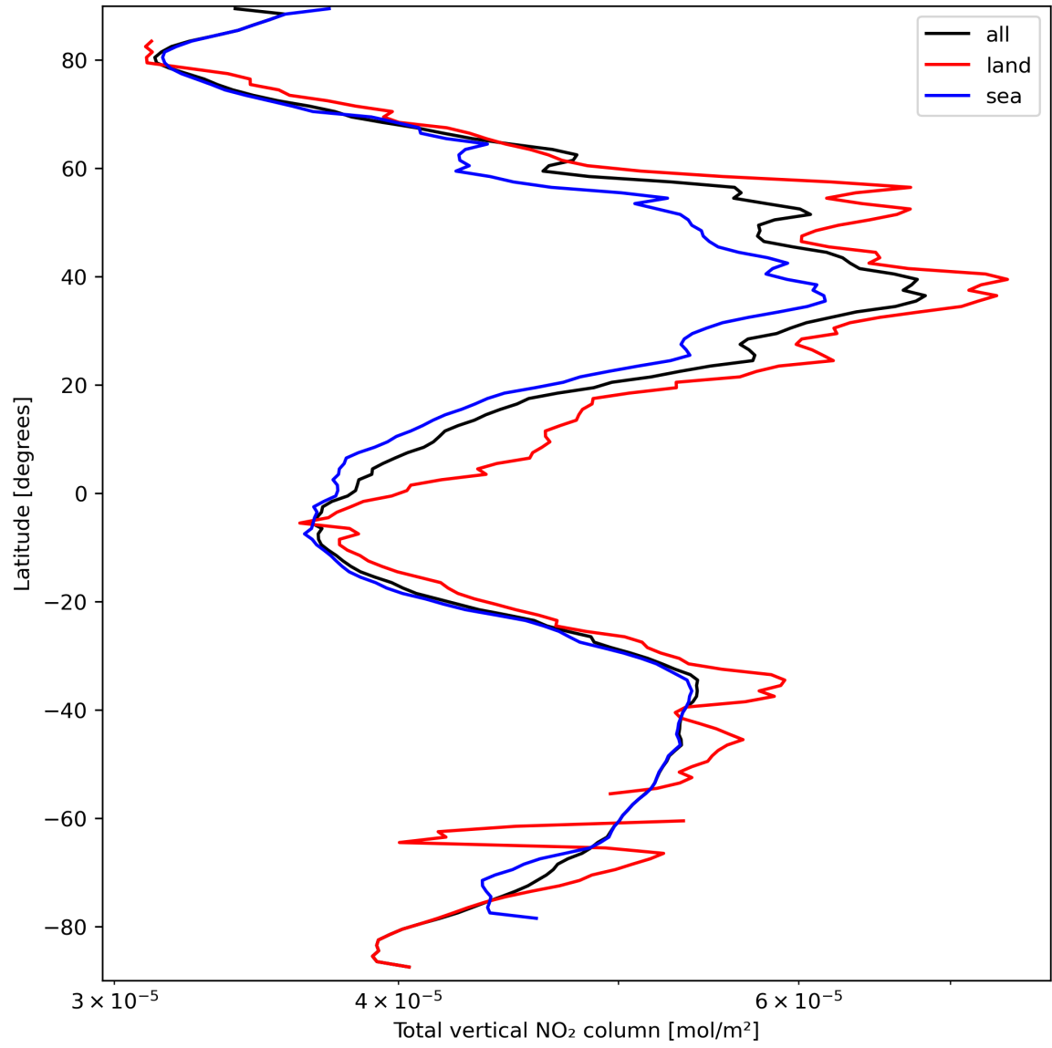
Figure 21: Zonal average of “Total vertical NO 2 column” for 2024-03-21 to 2024-03-22.
