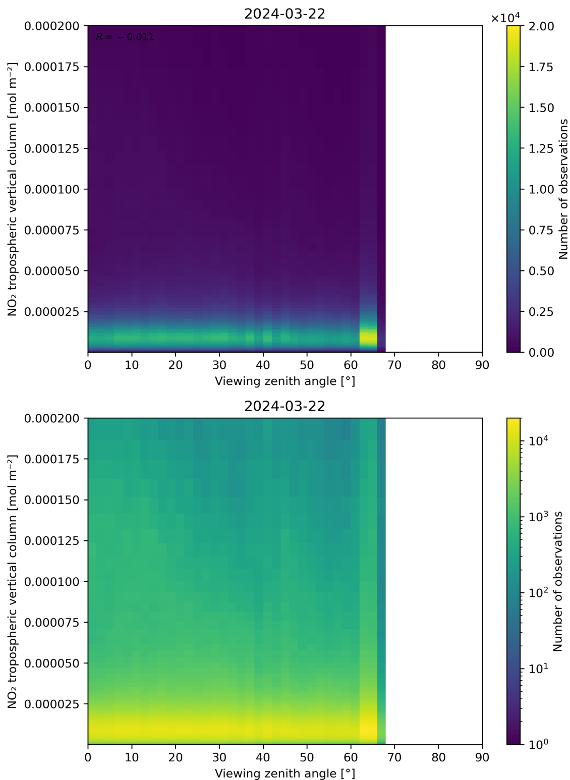
Figure 169: Scatter density plot of “Viewing zenith angle” against “NO 2 tropospheric vertical column” for 2024-03-21 to 2024-03-22.
