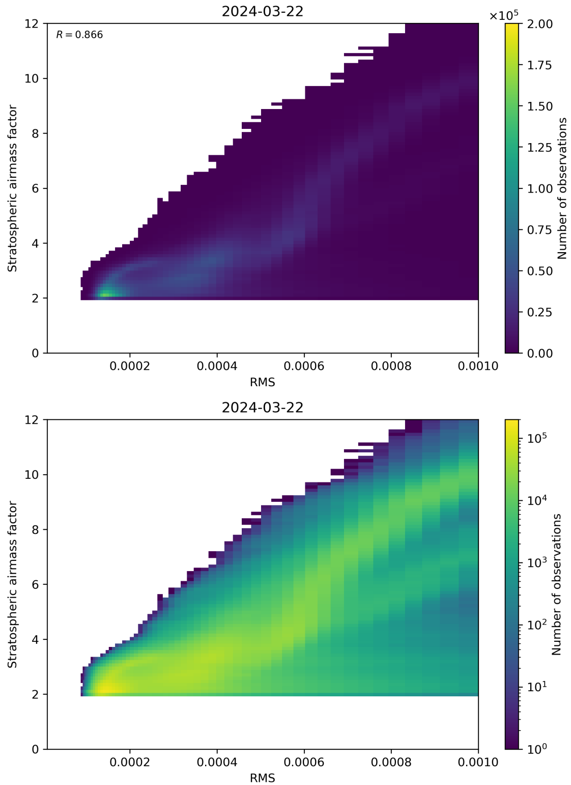
Figure 144: Scatter density plot of “RMS” against “Stratospheric airmass factor” for 2024-03-21 to 2024-03-22.
