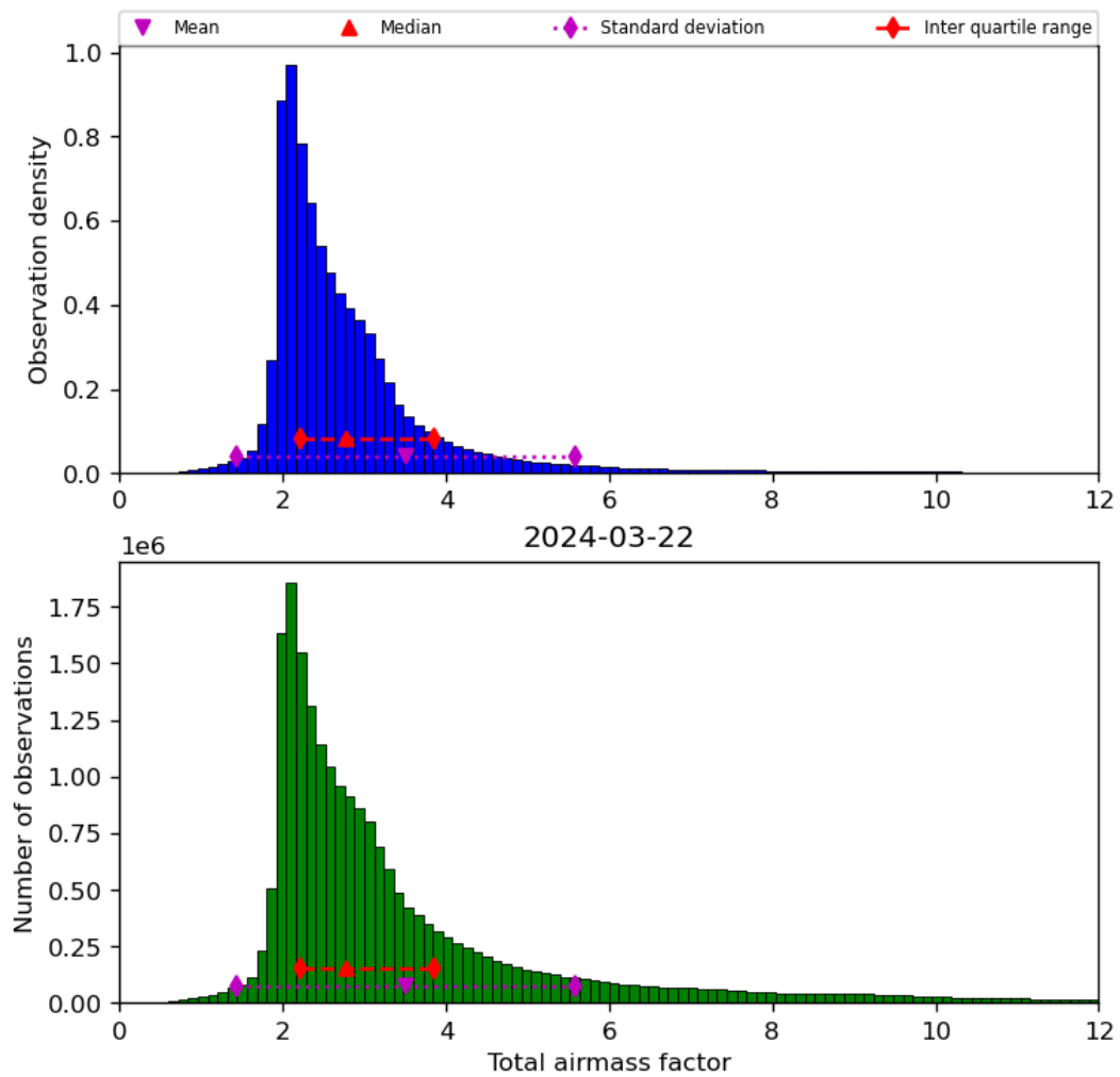
Figure 32: Histogram of “Total airmass factor” for 2024-03-21 to 2024-03-22
