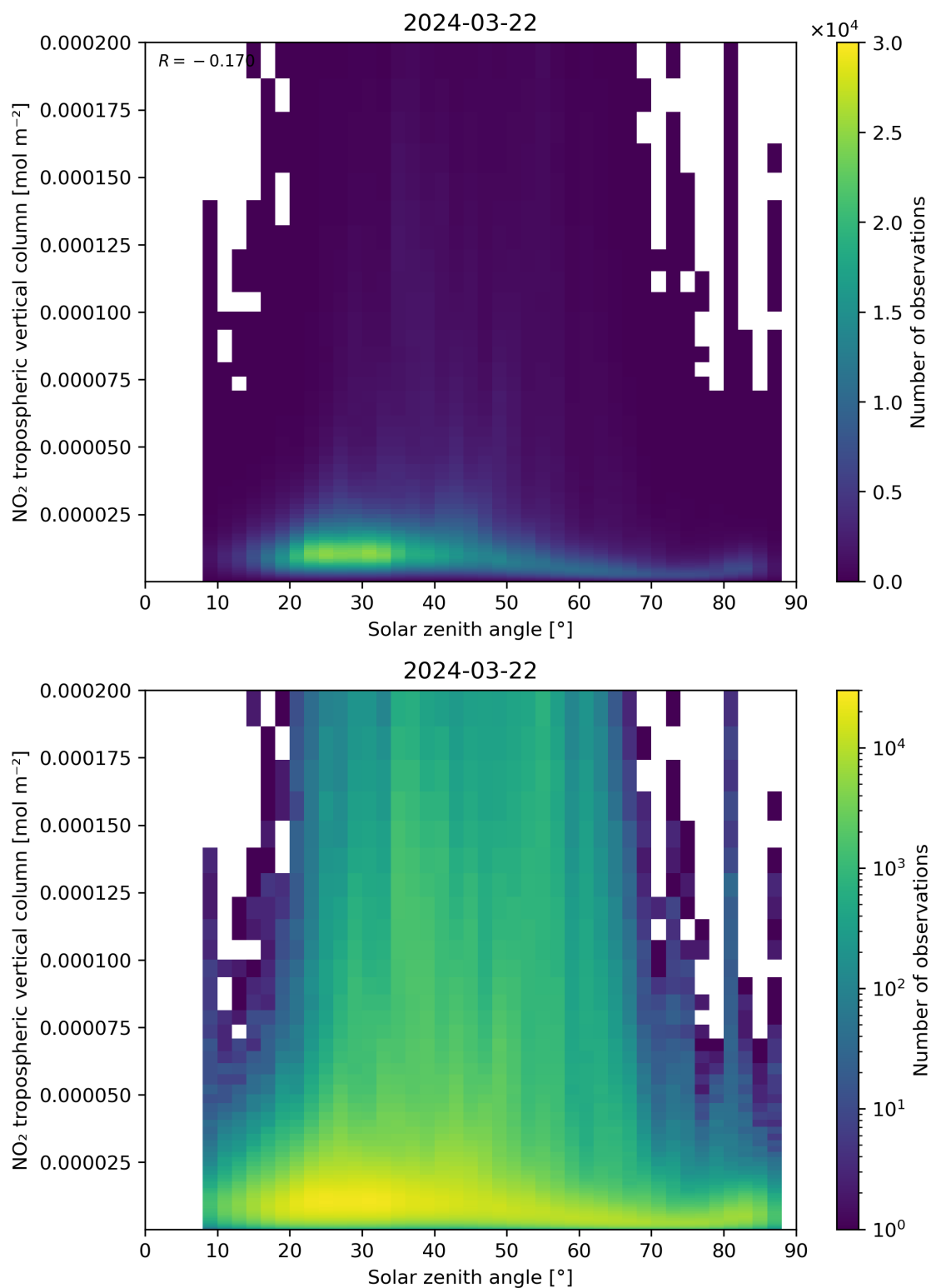
Figure 155: Scatter density plot of “Solar zenith angle” against “NO 2 tropospheric vertical column” for 2024-03-21 to 2024-03-22.
