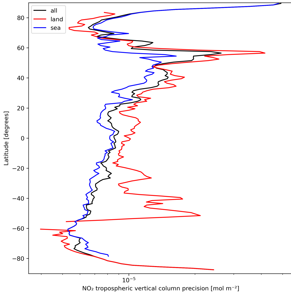
Figure 13: Zonal average of “NO 2 tropospheric vertical column precision” for 2024-03-21 to 2024-03-22.
