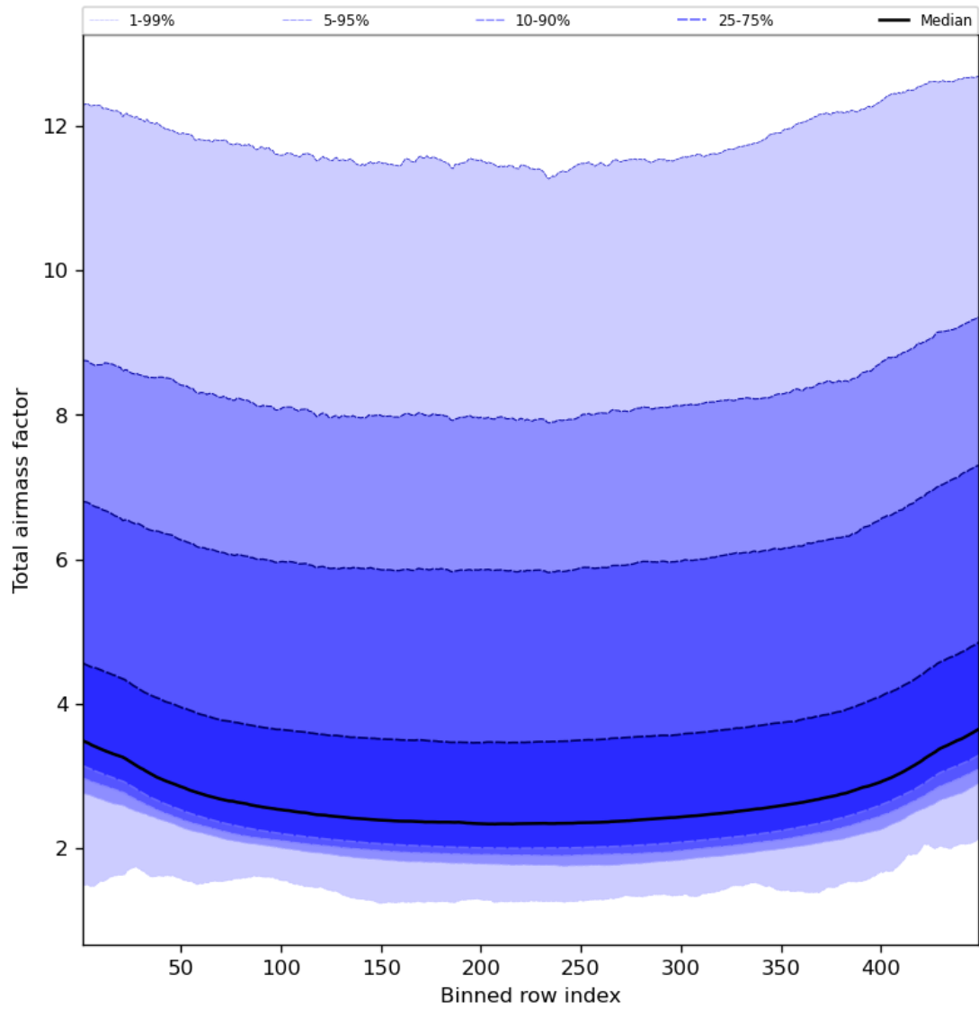
Figure 49: Along track statistics of “Total airmass factor” for 2024-03-21 to 2024-03-22
