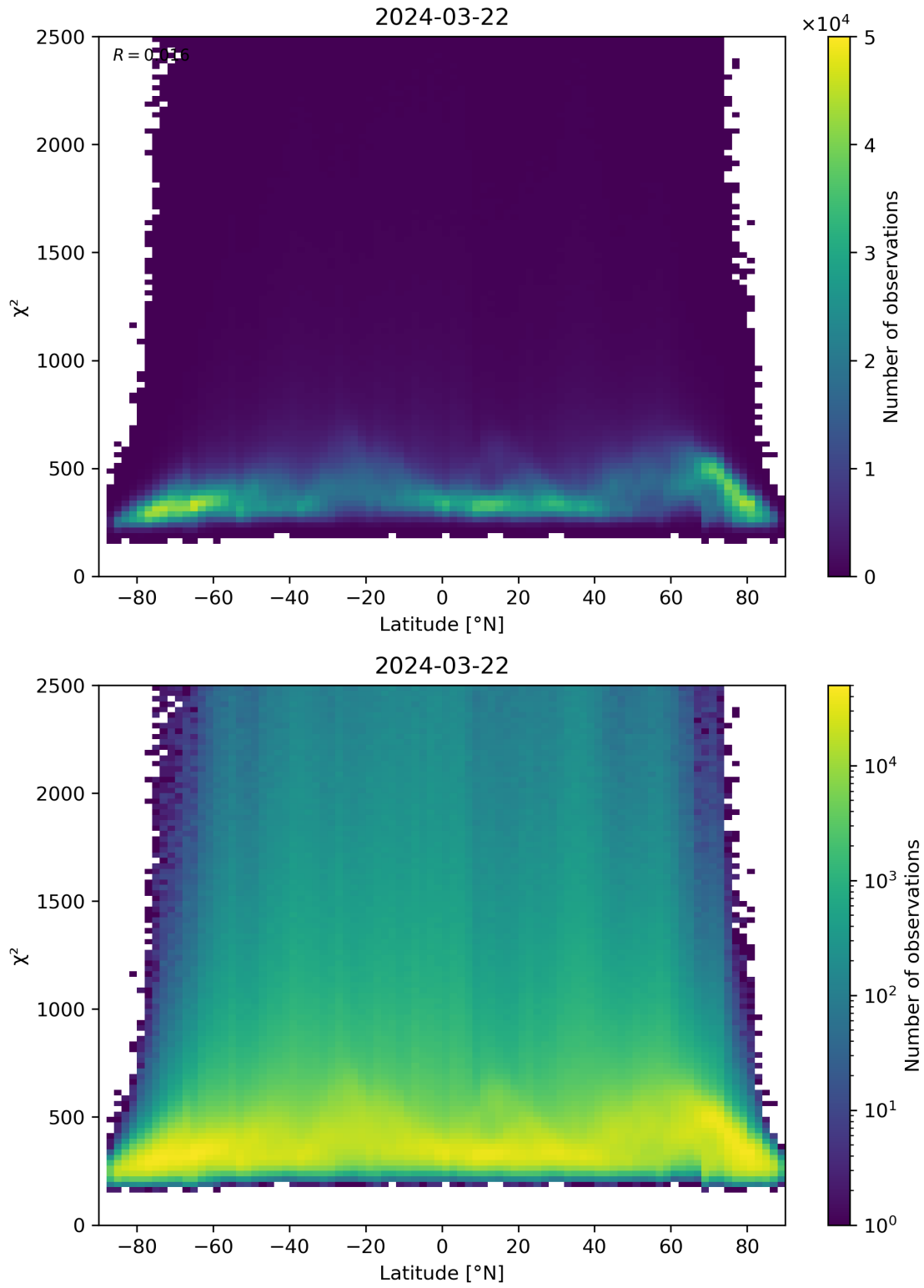
Figure 86: Scatter density plot of “Latitude” against “ \chi^2 ” for 2024-03-21 to 2024-03-22.
