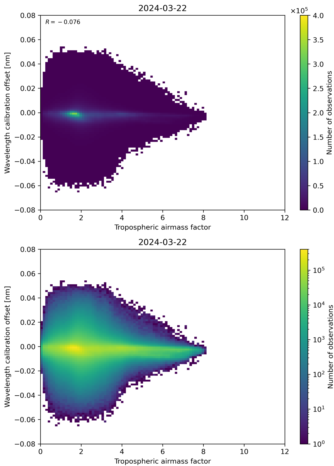
Figure 80: Scatter density plot of “Tropospheric airmass factor” against “Wavelength calibration offset” for 2024-03-21 to 2024-03-22.
