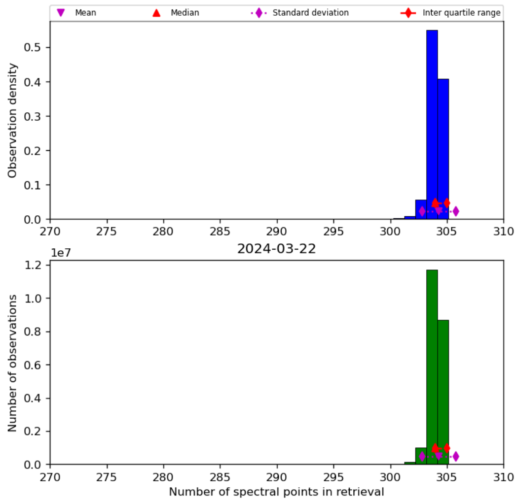
Figure 33: Histogram of “Number of spectral points in retrieval” for 2024-03-21 to 2024-03-22
