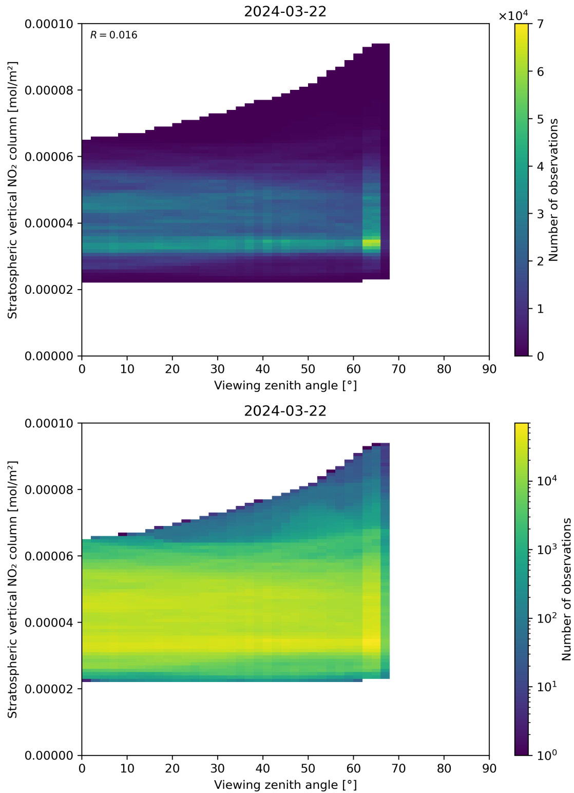
Figure 164: Scatter density plot of “Viewing zenith angle” against “Stratospheric vertical NO 2 column” for 2024-03-21 to 2024-03-22.
