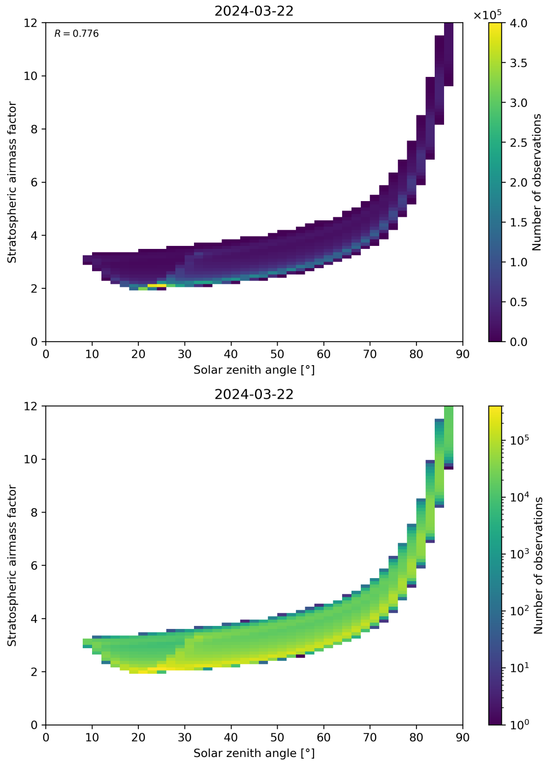
Figure 145: Scatter density plot of “Solar zenith angle” against “Stratospheric airmass factor” for 2024-03-21 to 2024-03-22.
