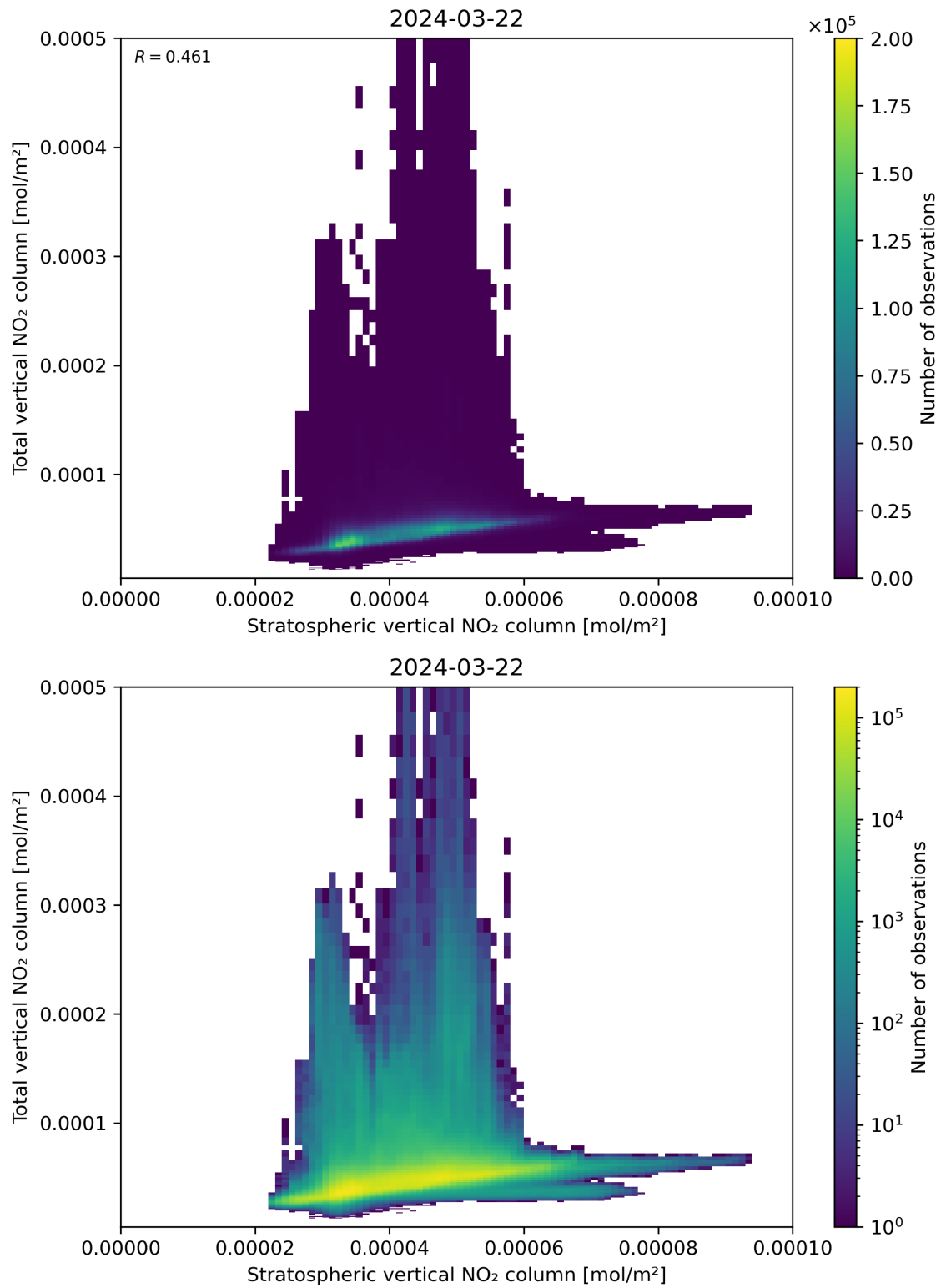
Figure 100: Scatter density plot of “Stratospheric vertical NO 2 column” against “Total vertical NO 2 column” for 2024-03-21 to 2024-03-22.
