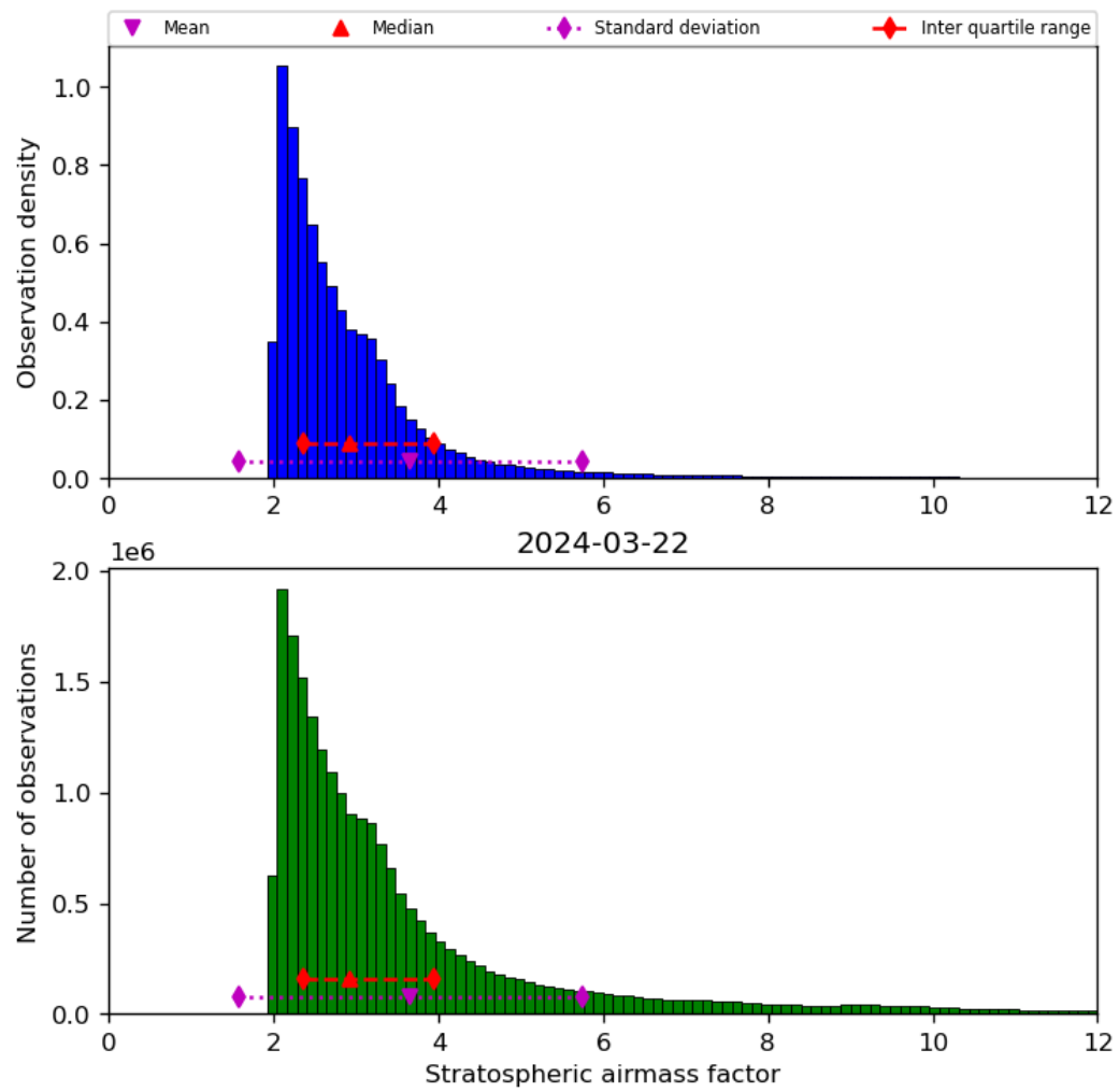
Figure 44: Histogram of “Stratospheric airmass factor” for 2024-03-21 to 2024-03-22
