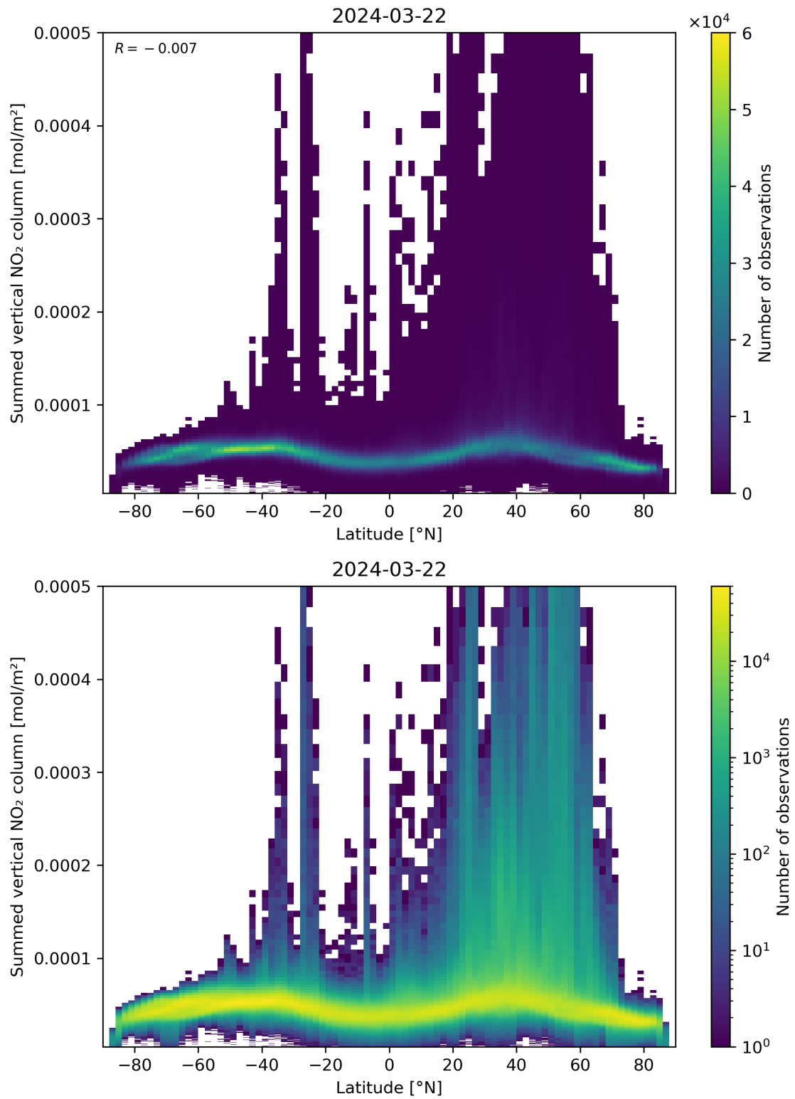
Figure 88: Scatter density plot of “Latitude” against “Summed vertical NO 2 column” for 2024-03-21 to 2024-03-22.
