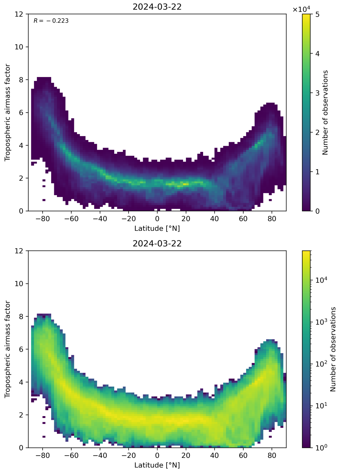
Figure 85: Scatter density plot of “Latitude” against “Tropospheric airmass factor” for 2024-03-21 to 2024-03-22.
