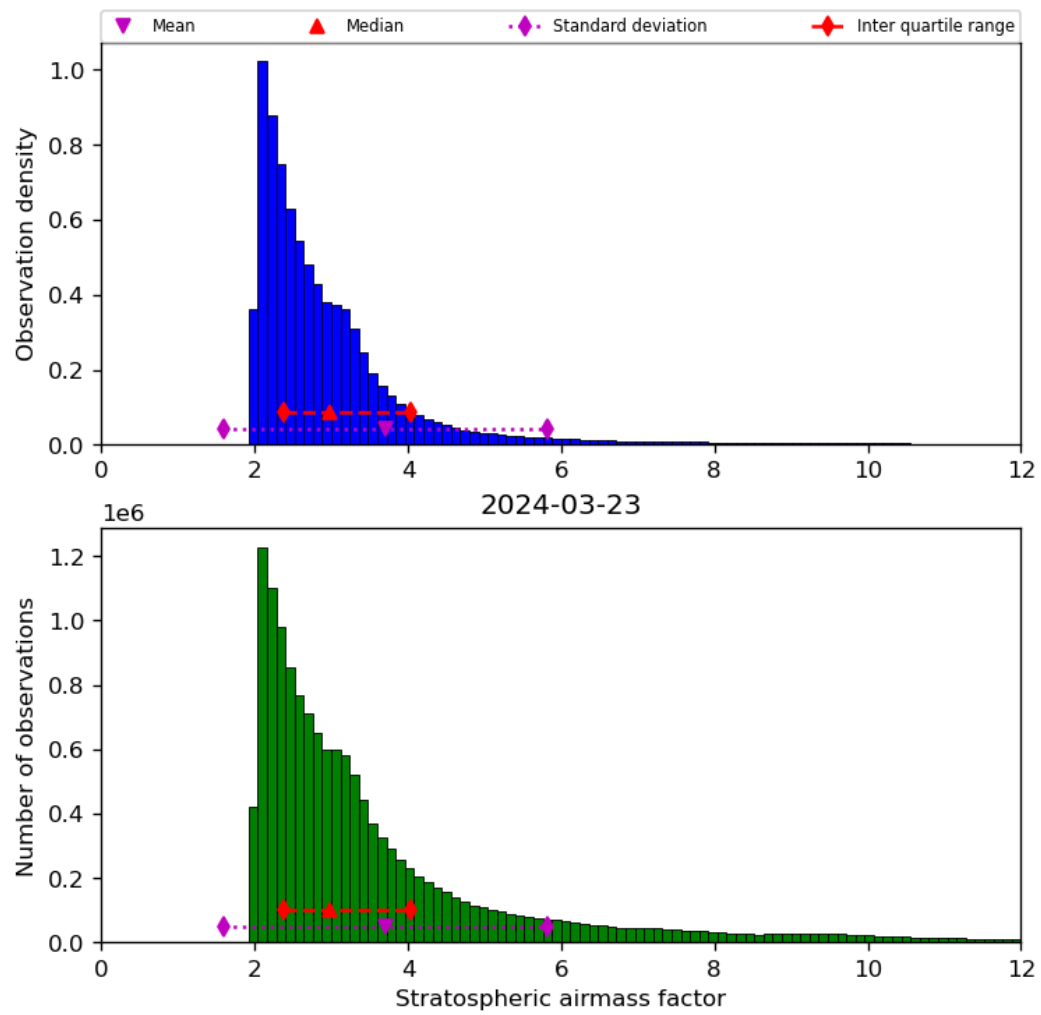
Figure 44: Histogram of “Stratospheric airmass factor” for 2024-03-23 to 2024-03-24
