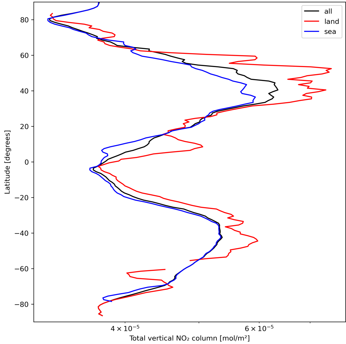
Figure 21: Zonal average of “Total vertical NO 2 column” for 2024-03-23 to 2024-03-24.
