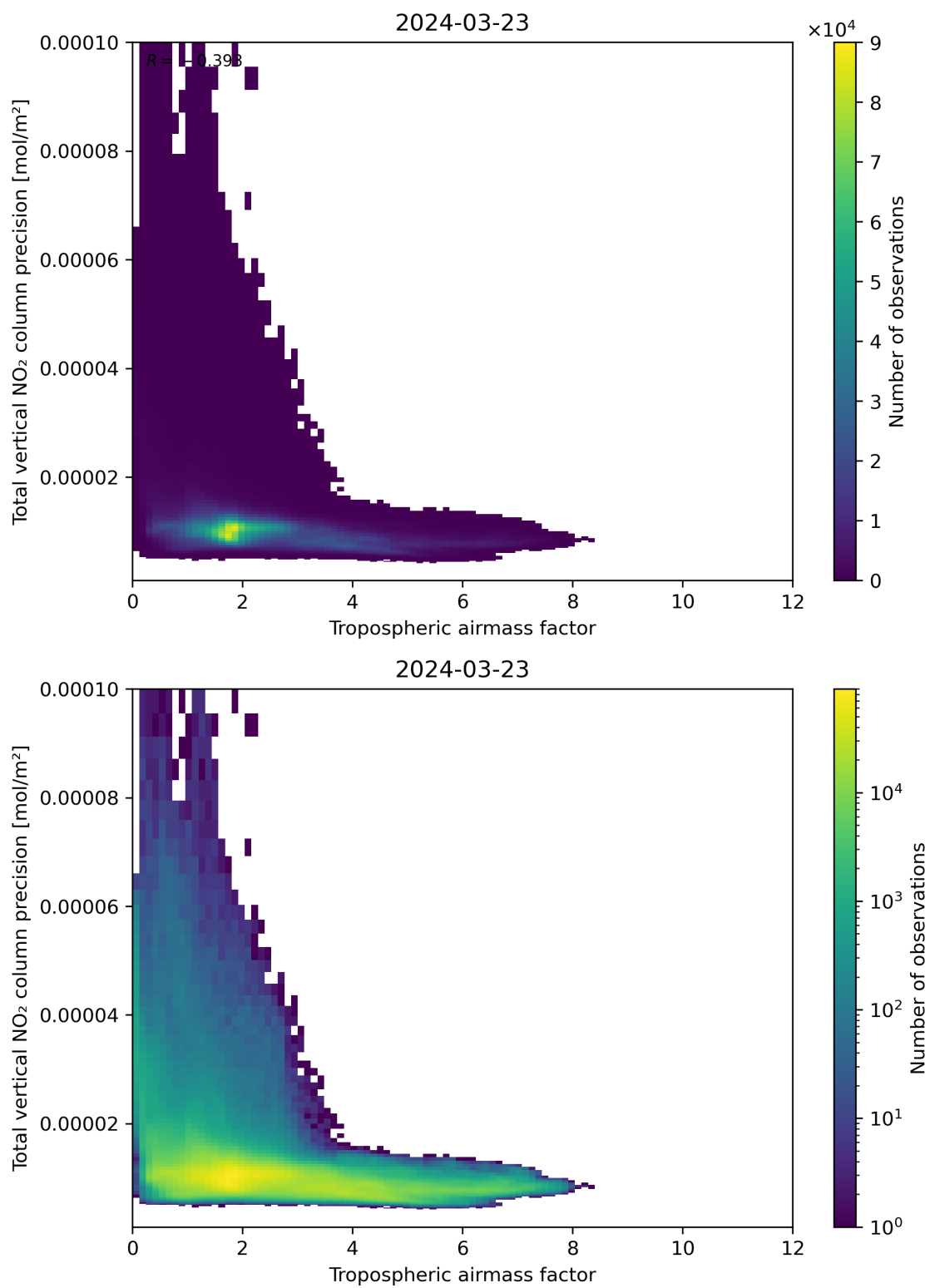
Figure 78: Scatter density plot of “Tropospheric air mass factor” against “Total vertical NO 2 column precision” for 2024-03-23 to 2024-03-24.
