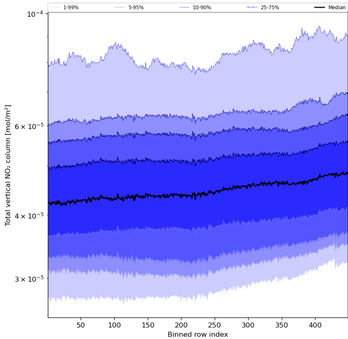
Figure 55: Along track statistics of “Total vertical NO 2 column” for 2024-03-23 to 2024-03-24
