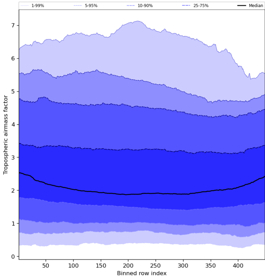
Figure 48: Along track statistics of “Tropospheric air mass factor” for 2024-03-23 to 2024-03-24
