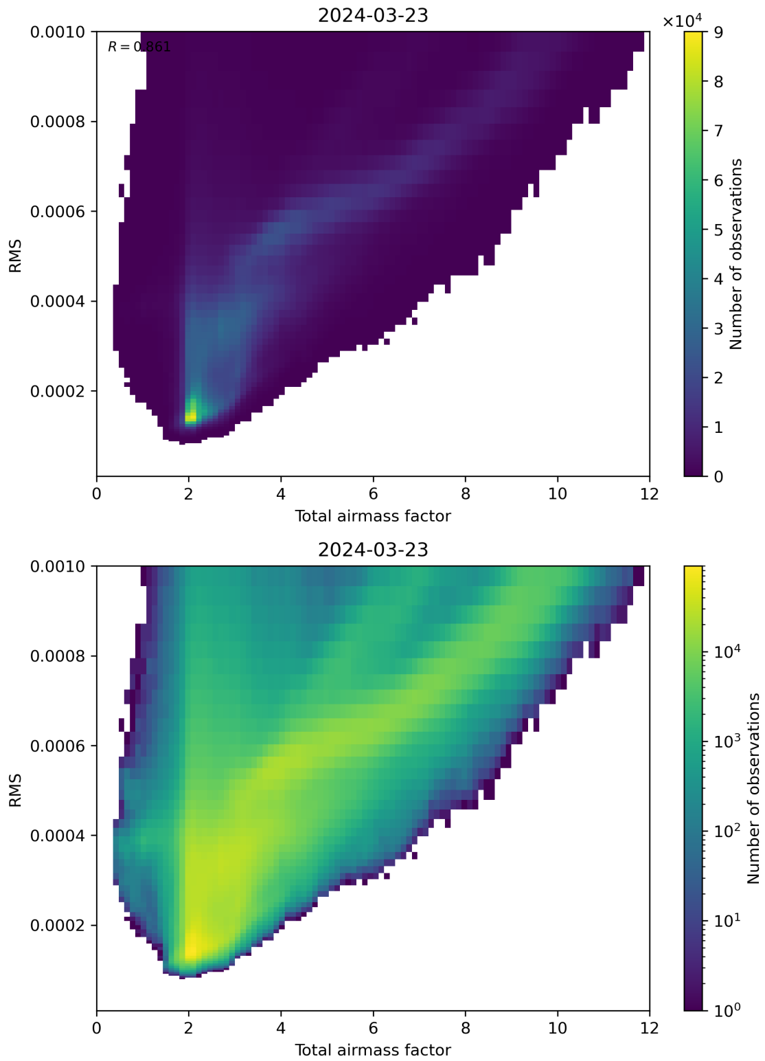
Figure 69: Scatter density plot of “Total airmass factor” against “RMS” for 2024-03-23 to 2024-03-24.
