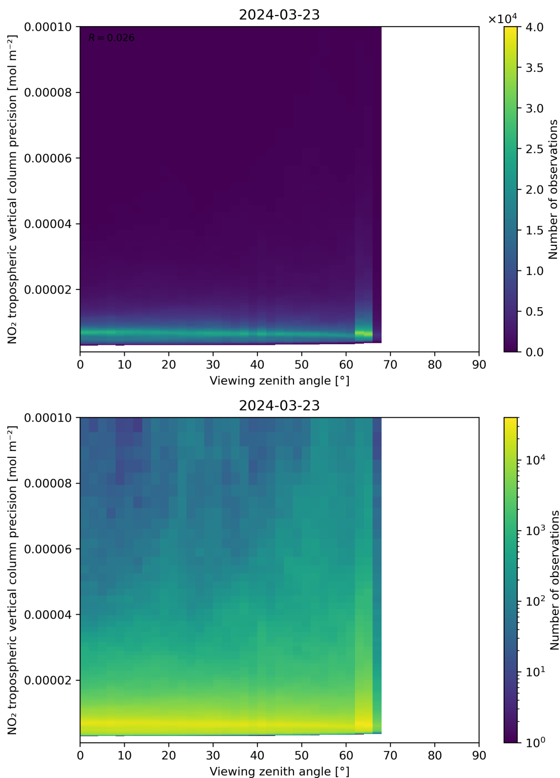
Figure 170: Scatter density plot of “Viewing zenith angle” against “NO 2 tropospheric vertical column precision” for 2024-03-23 to 2024-03-24.
