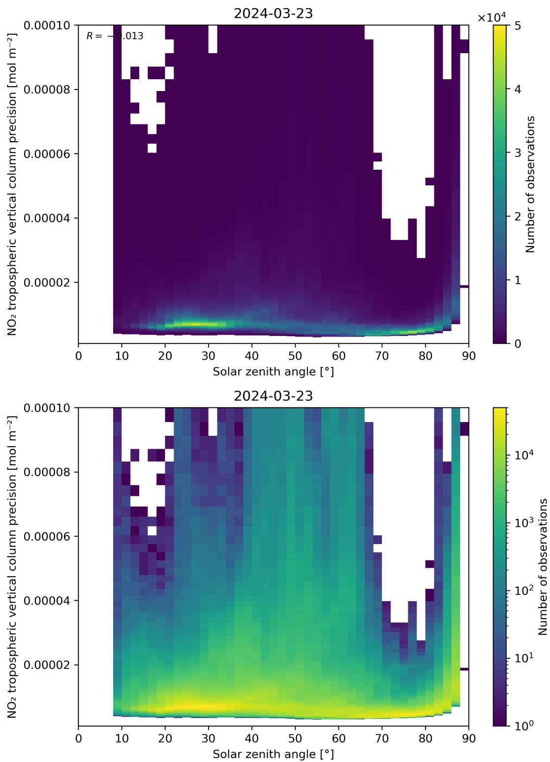
Figure 156: Scatter density plot of “Solar zenith angle” against “NO 2 tropospheric vertical column precision” for 2024-03-23 to 2024-03-24.
