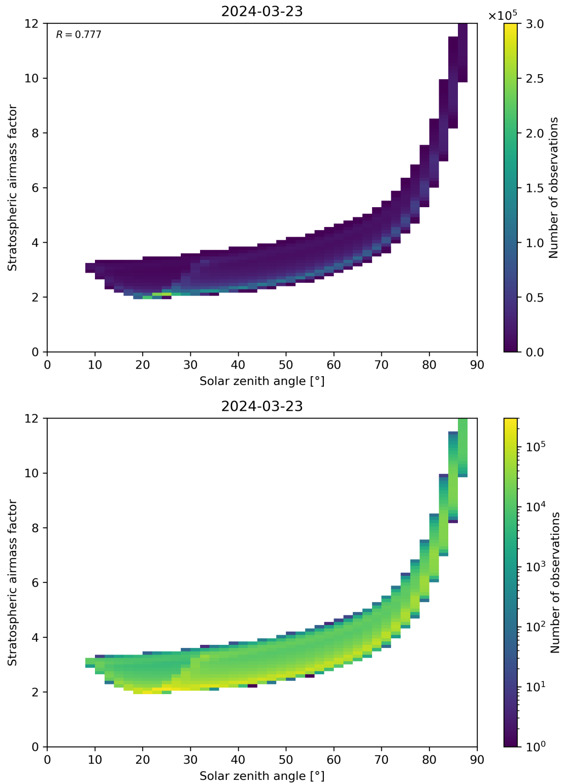
Figure 145: Scatter density plot of “Solar zenith angle” against “Stratospheric airmass factor” for 2024-03-23 to 2024-03-24.
