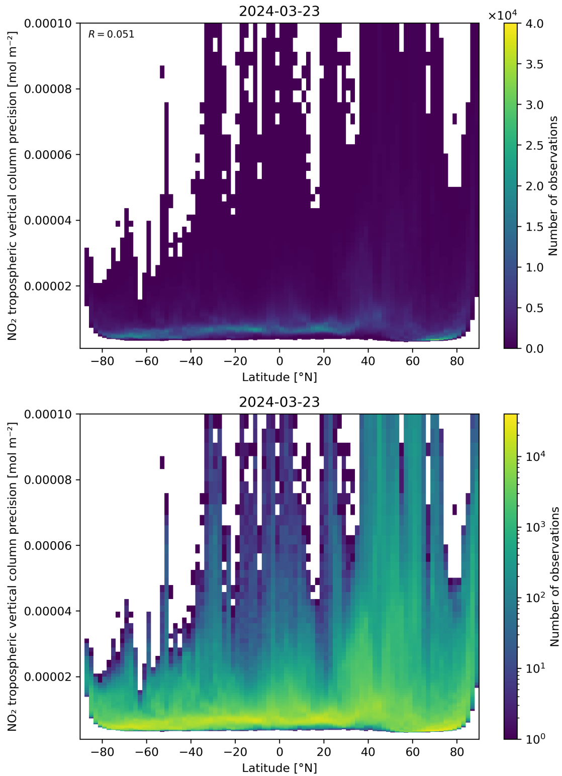
Figure 93: Scatter density plot of “Latitude” against “NO 2 tropospheric vertical column precision” for 2024-03-23 to 2024-03-24.
