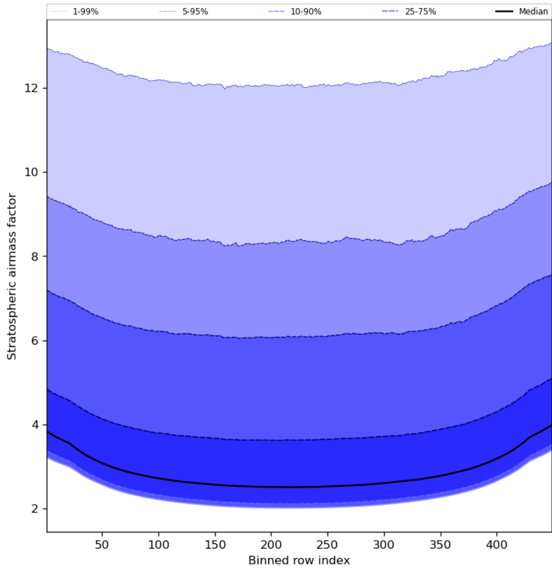
Figure 61: Along track statistics of “Stratospheric airmass factor” for 2024-03-23 to 2024-03-24
