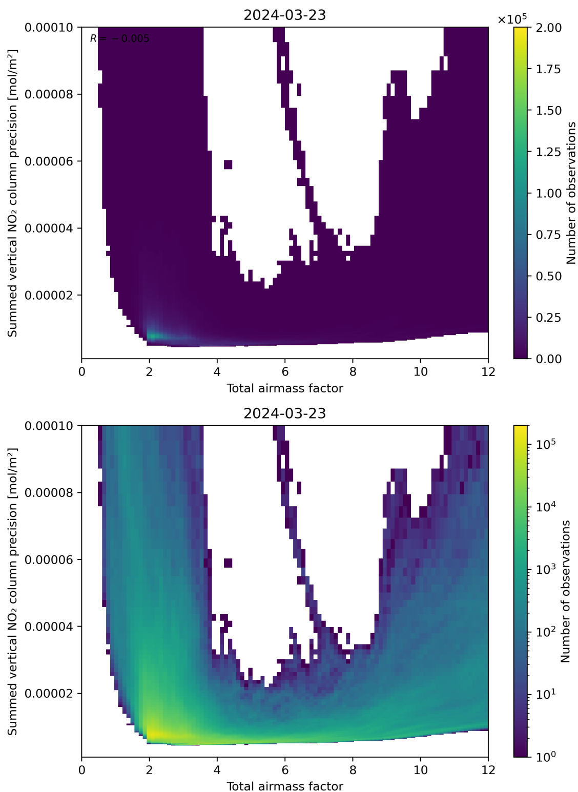
Figure 66: Scatter density plot of “Total airmass factor” against “Summed vertical NO 2 column precision” for 2024-03-23 to 2024-03-24.
