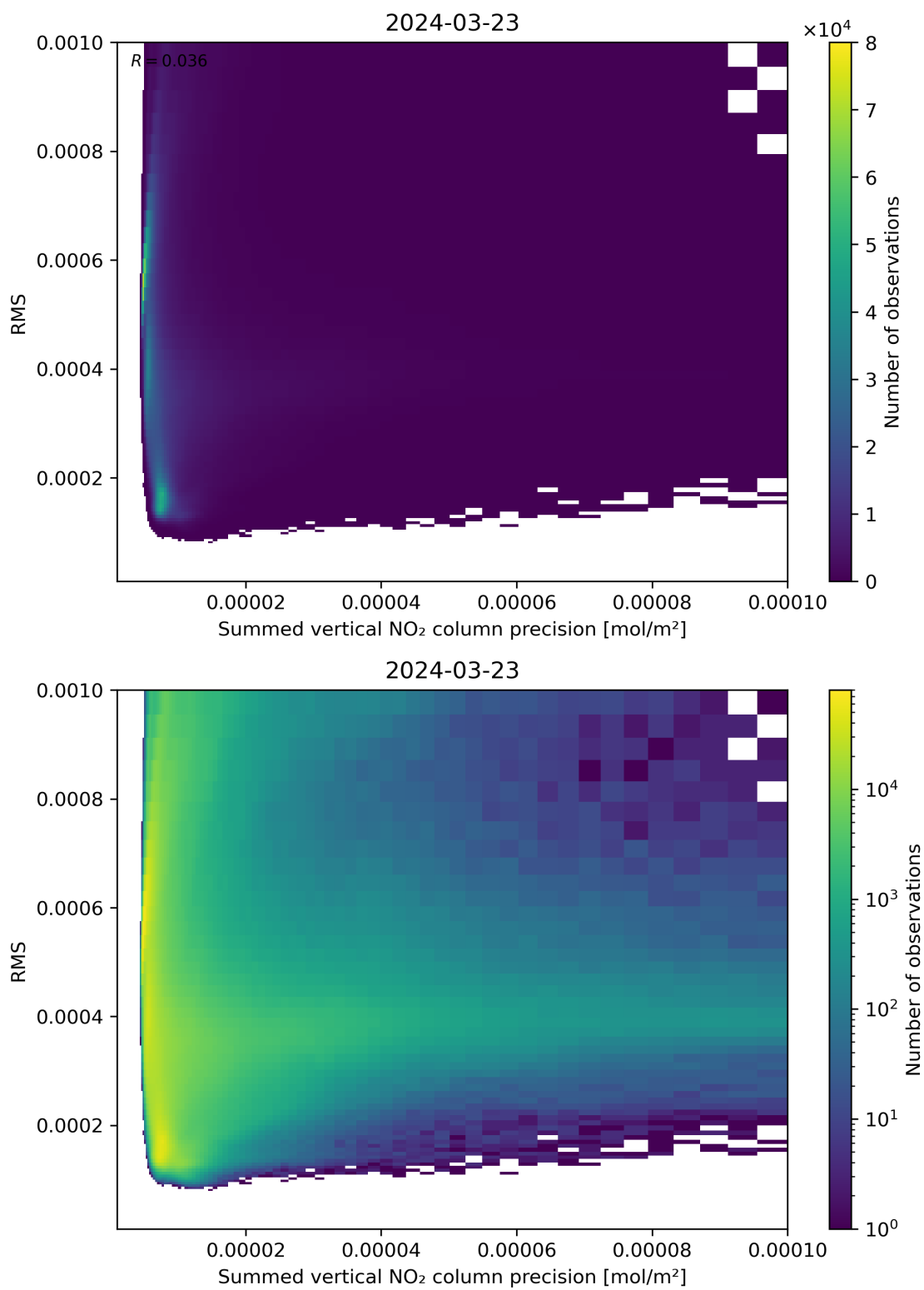
Figure 108: Scatter density plot of “Summed vertical NO 2 column precision” against “RMS” for 2024-03-23 to 2024-03-24.
