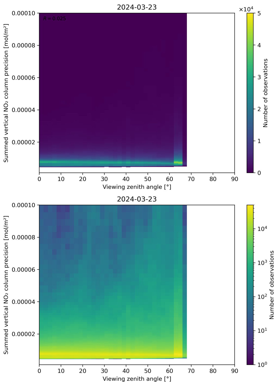
Figure 166: Scatter density plot of “Viewing zenith angle” against “Summed vertical NO 2 column precision” for 2024-03-23 to 2024-03-24.
