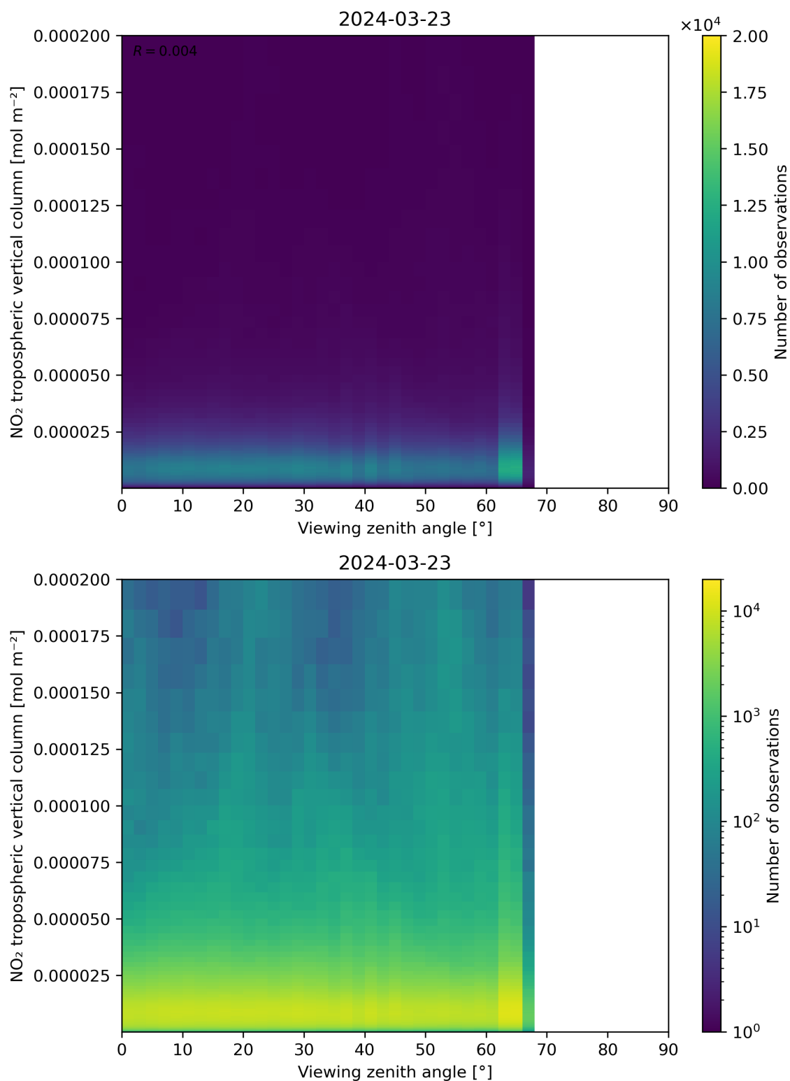
Figure 169: Scatter density plot of “Viewing zenith angle” against “NO 2 tropospheric vertical column” for 2024-03-23 to 2024-03-24.
