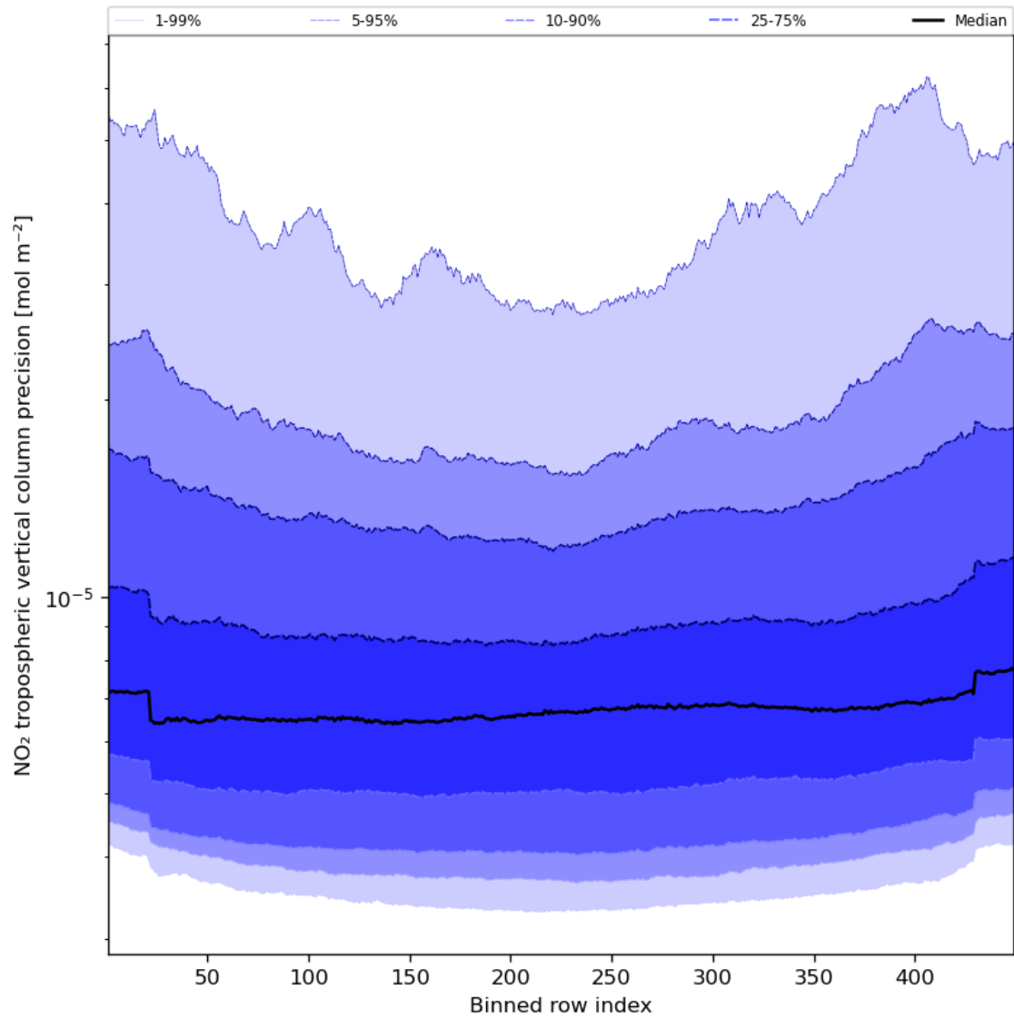
Figure 47: Along track statistics of “NO 2 tropospheric vertical column precision” for 2024-03-23 to 2024-03-24
