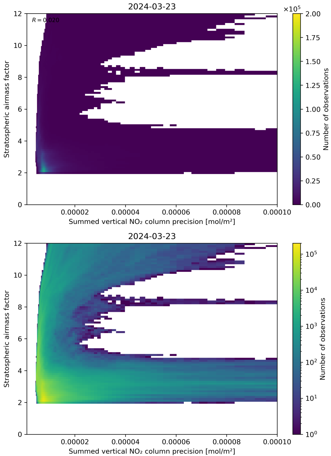
Figure 106: Scatter density plot of “Summed vertical NO 2 column precision” against “Stratospheric airmass factor” for 2024-03-23 to 2024-03-24.
