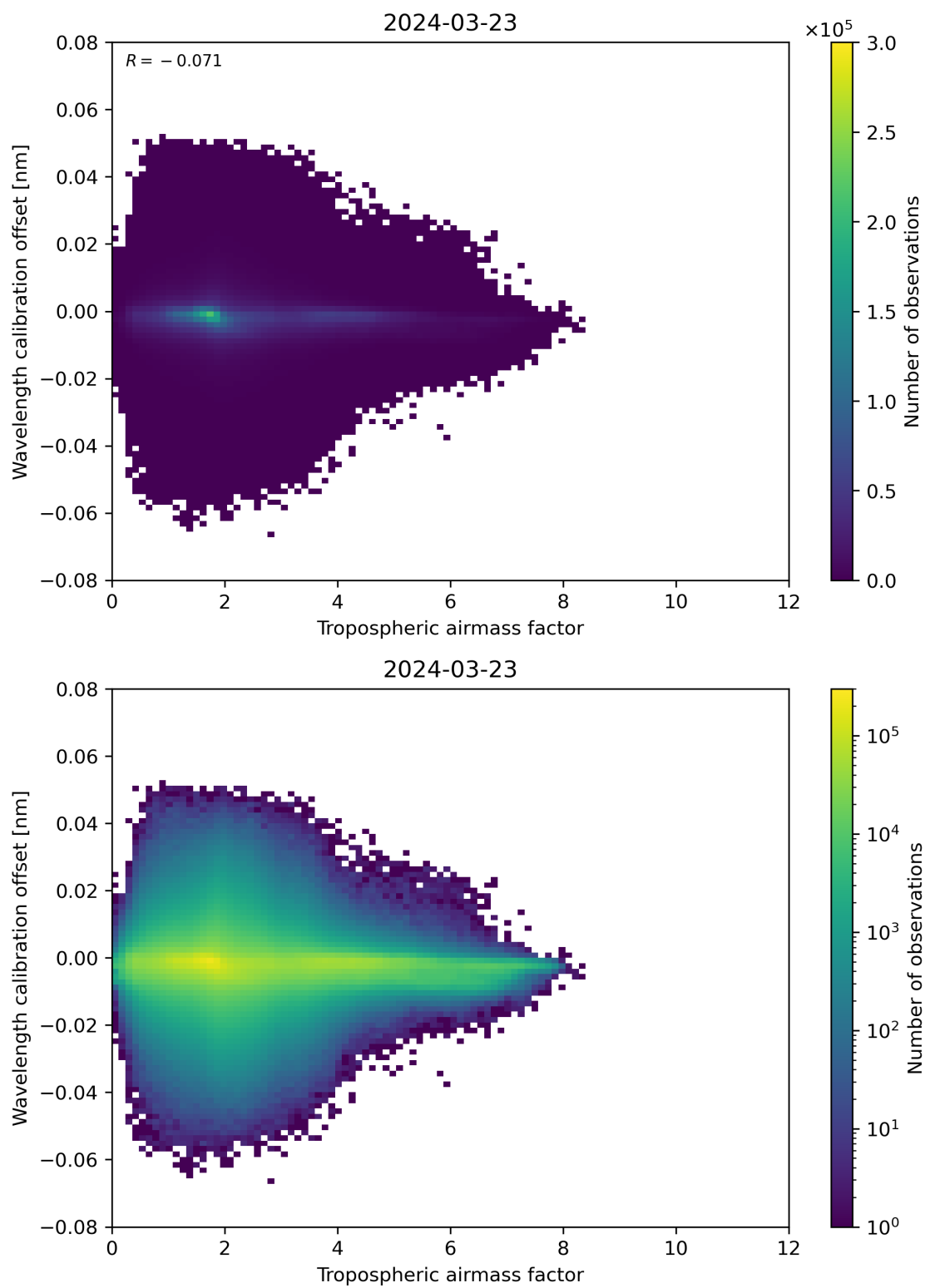
Figure 80: Scatter density plot of “Tropospheric airmass factor” against “Wavelength calibration offset” for 2024-03-23 to 2024-03-24.
