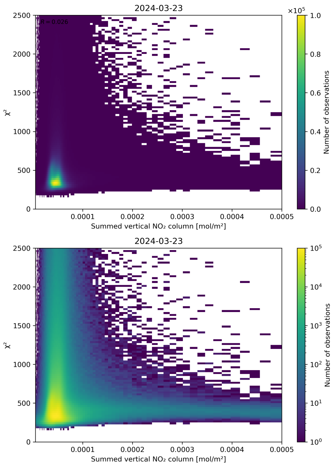
Figure 104: Scatter density plot of “Summed vertical NO 2 column” against “ \chi^2 ” for 2024-03-23 to 2024-03-24.
