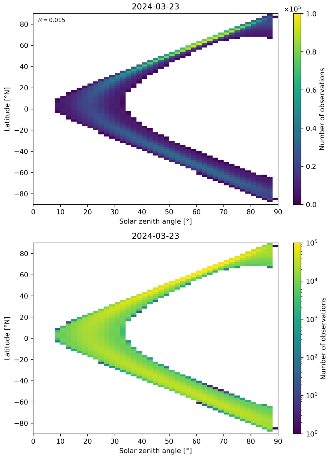
Figure 149: Scatter density plot of “Solar zenith angle” against “Latitude” for 2024-03-23 to 2024-03-24.
