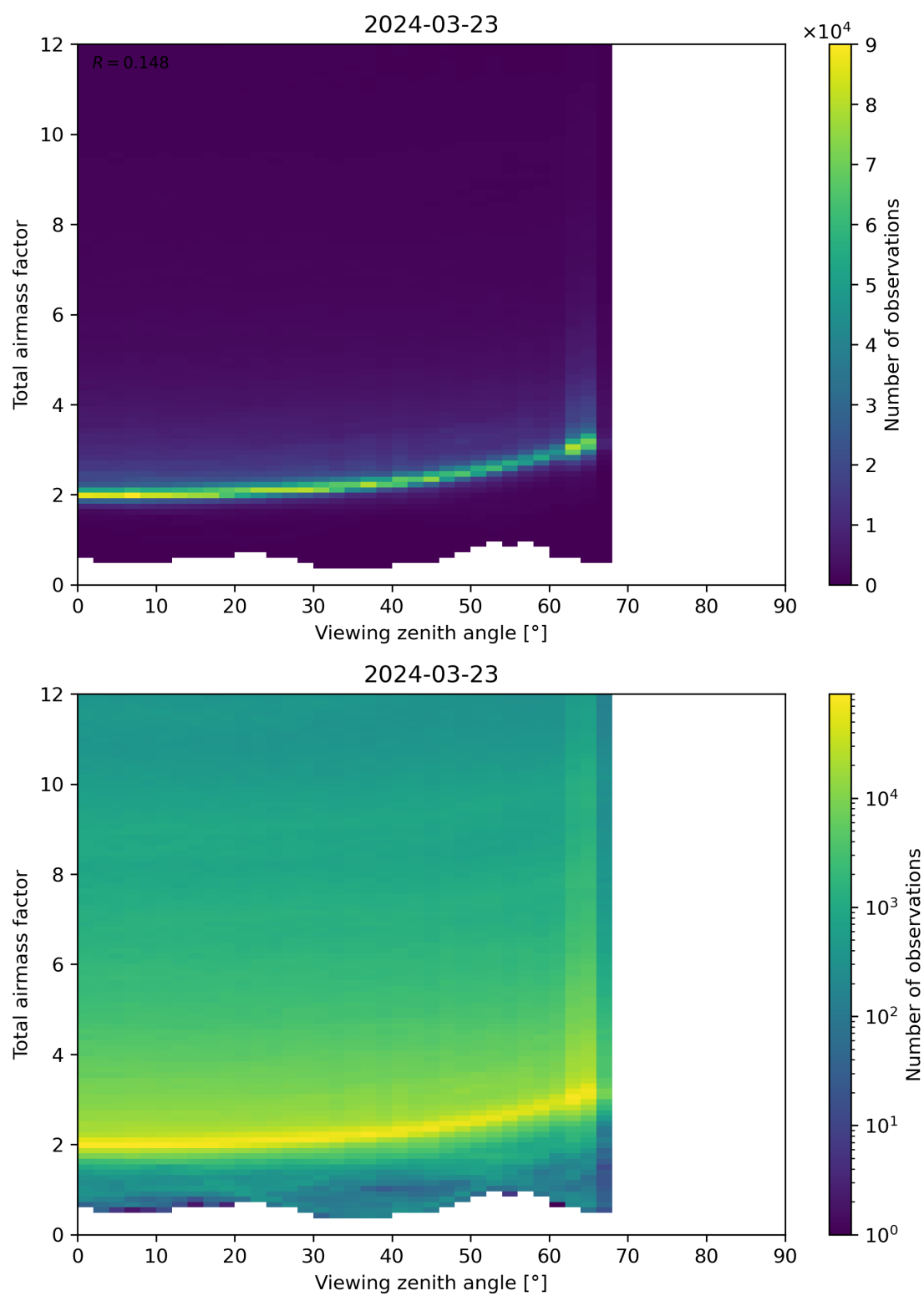
Figure 160: Scatter density plot of “Viewing zenith angle” against “Total airmass factor” for 2024-03-23 to 2024-03-24.
