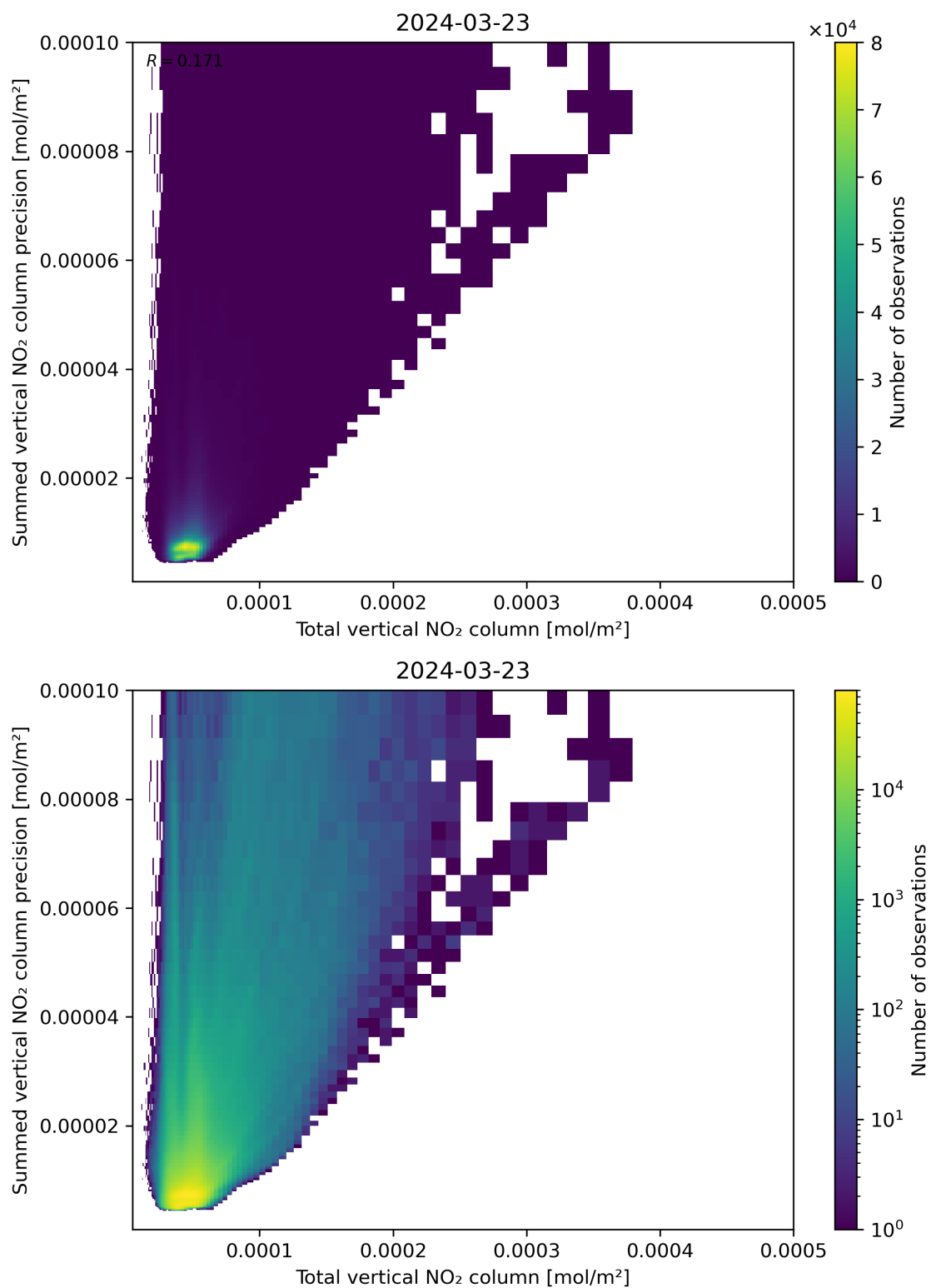
Figure 113: Scatter density plot of “Total vertical NO 2 column” against “Summed vertical NO 2 column precision” for 2024-03-23 to 2024-03-24.
