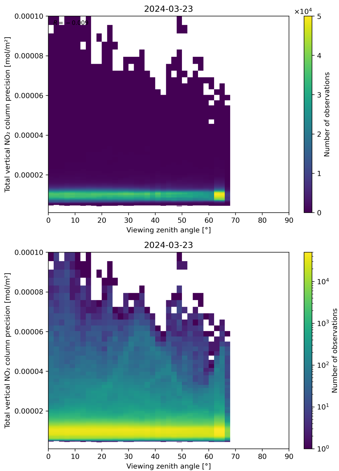
Figure 168: Scatter density plot of “Viewing zenith angle” against “Total vertical NO 2 column precision” for 2024-03-23 to 2024-03-24.
