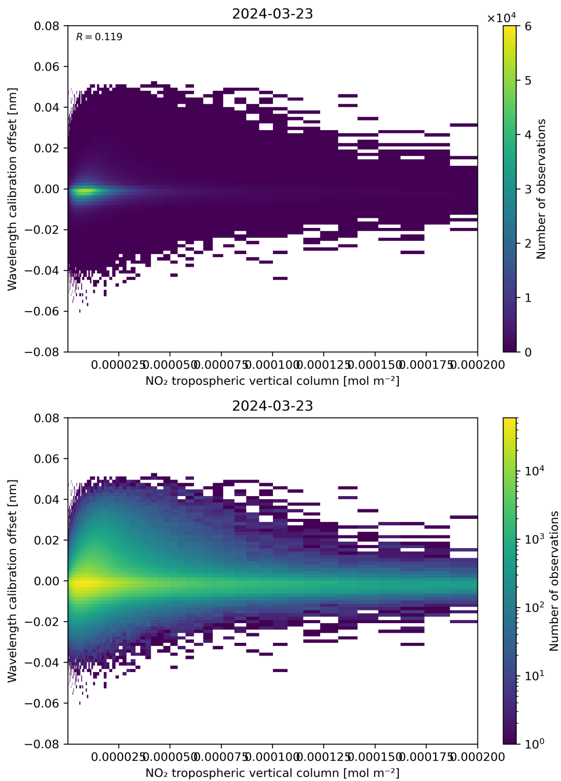
Figure 143: Scatter density plot of “NO 2 tropospheric vertical column” against “Wavelength calibration offset” for 2024-03-23 to 2024-03-24.
