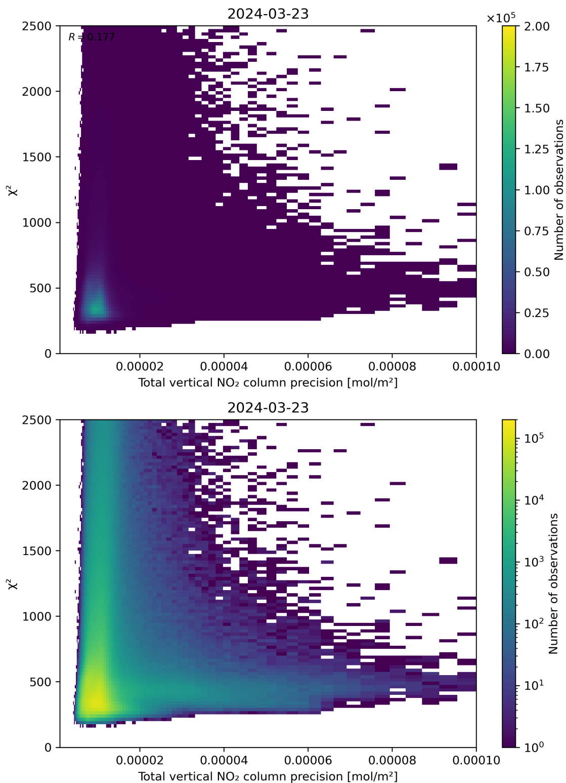
Figure 116: Scatter density plot of “Total vertical NO 2 column precision” against “ \chi^2 ” for 2024-03-23 to 2024-03-24.
