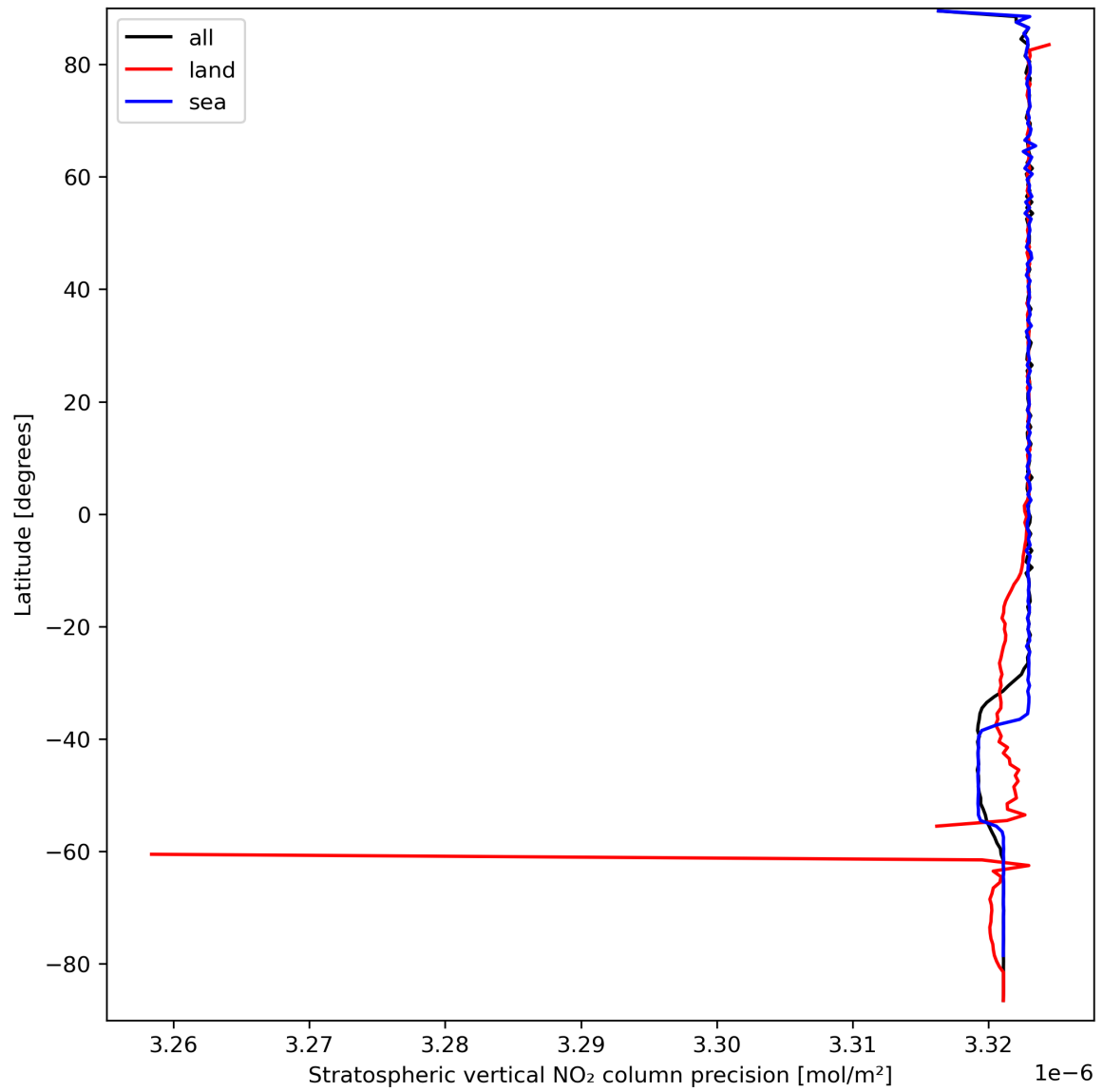
Figure 20: Zonal average of “Stratospheric vertical NO 2 column precision” for 2024-03-23 to 2024-03-24.
