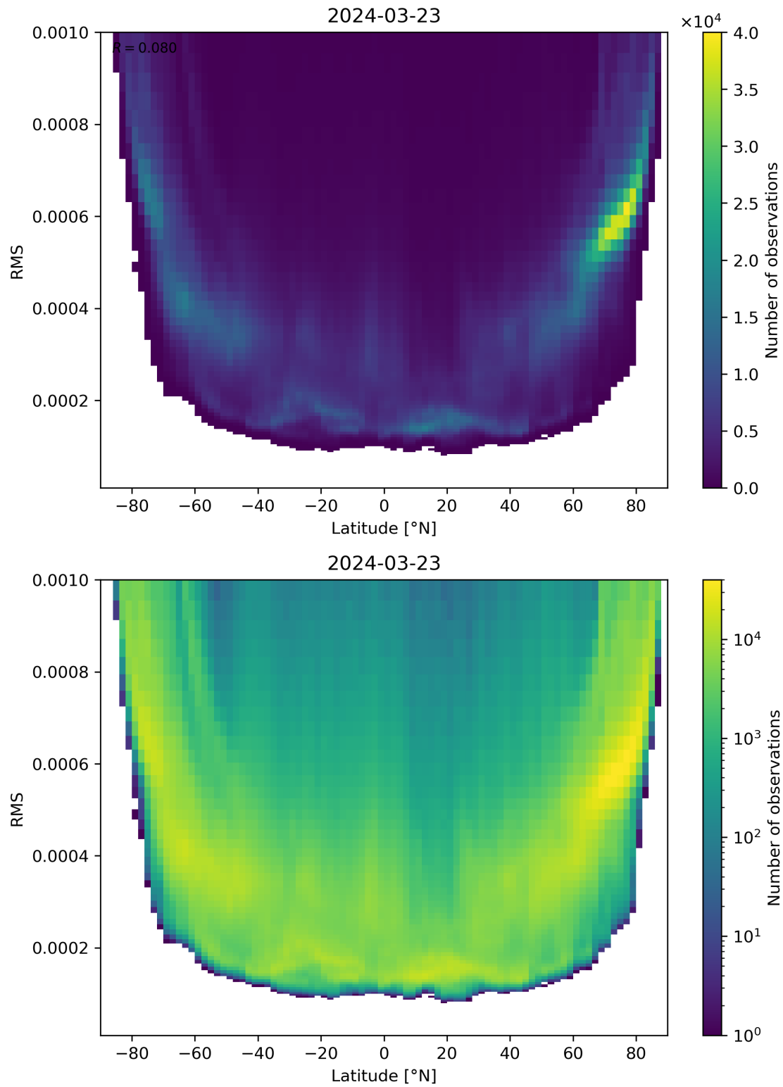
Figure 94: Scatter density plot of “Latitude” against “RMS” for 2024-03-23 to 2024-03-24.
