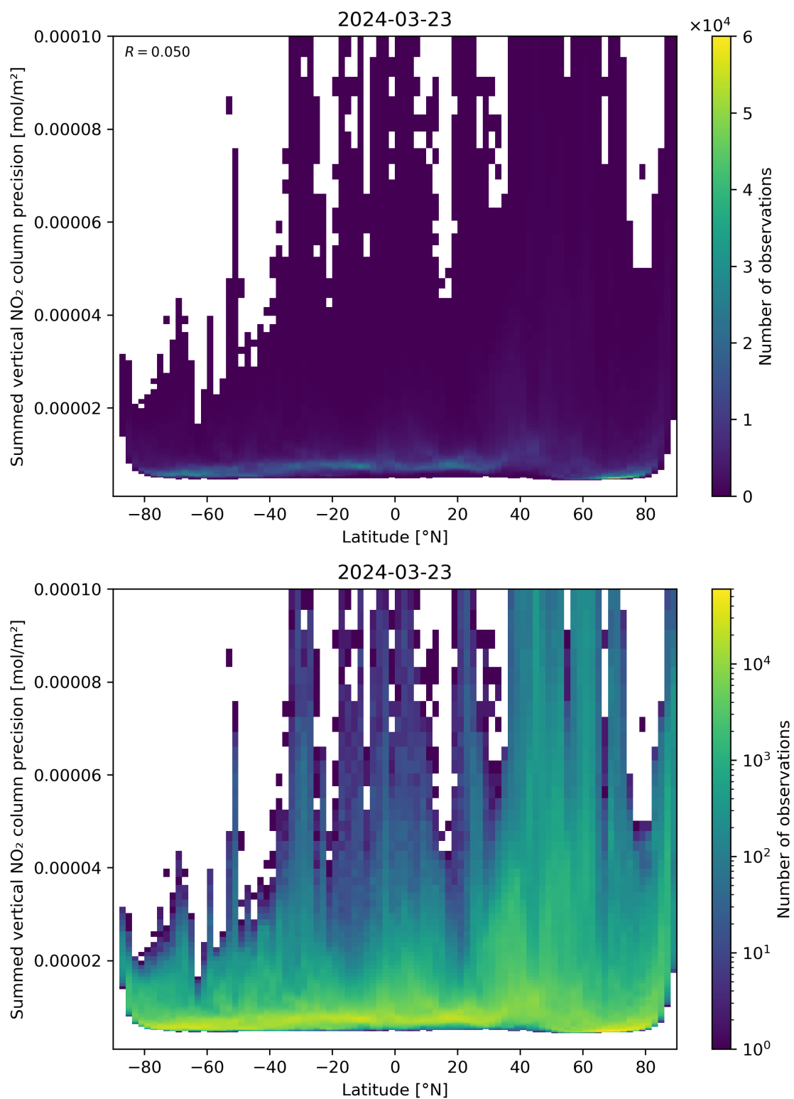
Figure 89: Scatter density plot of “Latitude” against “Summed vertical NO 2 column precision” for 2024-03-23 to 2024-03-24.
