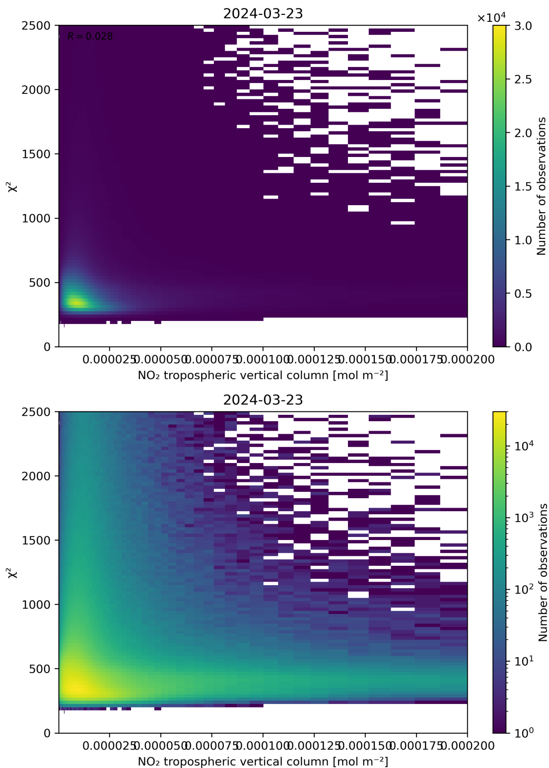
Figure 124: Scatter density plot of “NO 2 tropospheric vertical column” against “ \chi^2 ” for 2024-03-23 to 2024-03-24.
