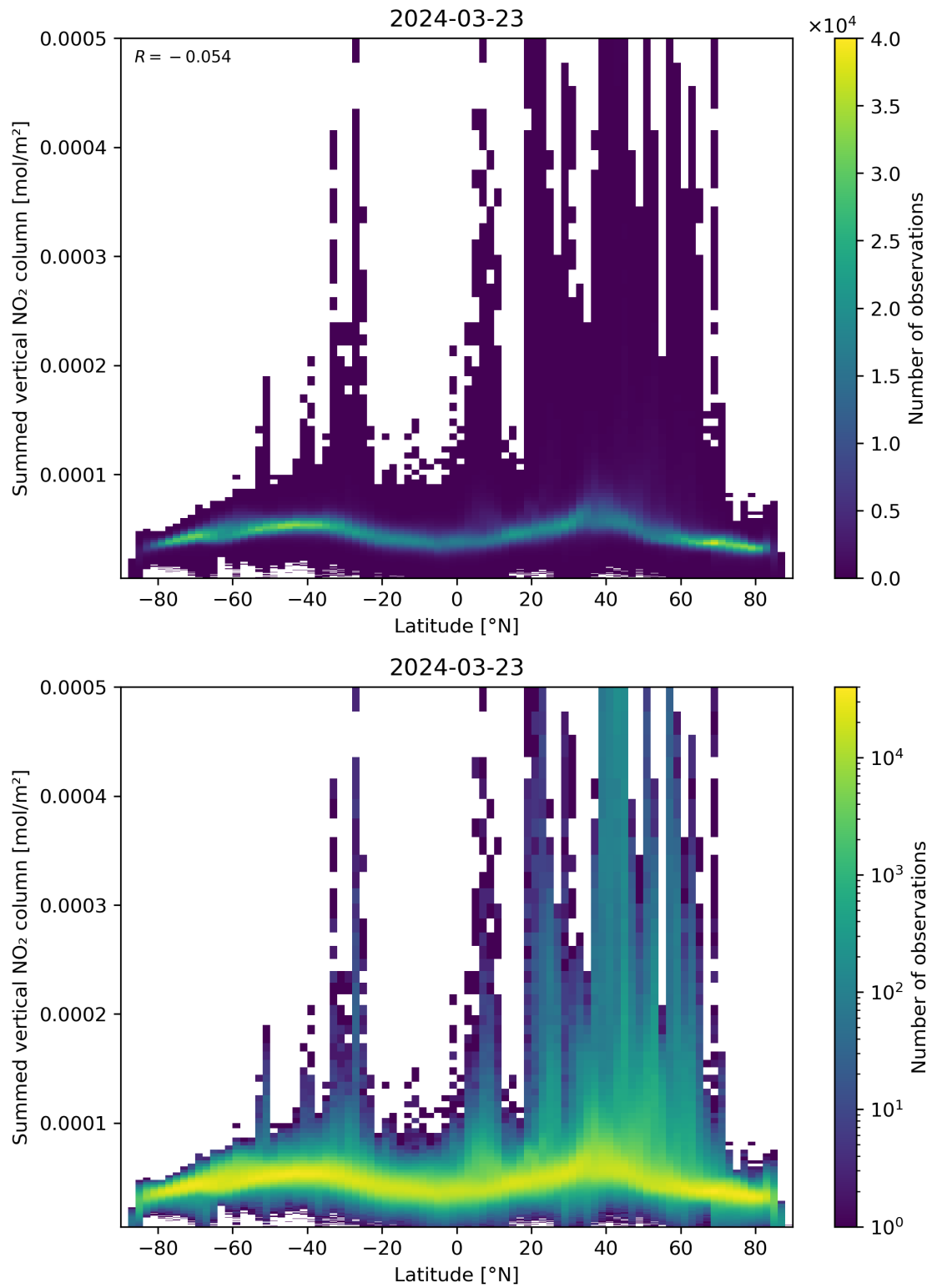
Figure 88: Scatter density plot of “Latitude” against “Summed vertical NO 2 column” for 2024-03-23 to 2024-03-24.
