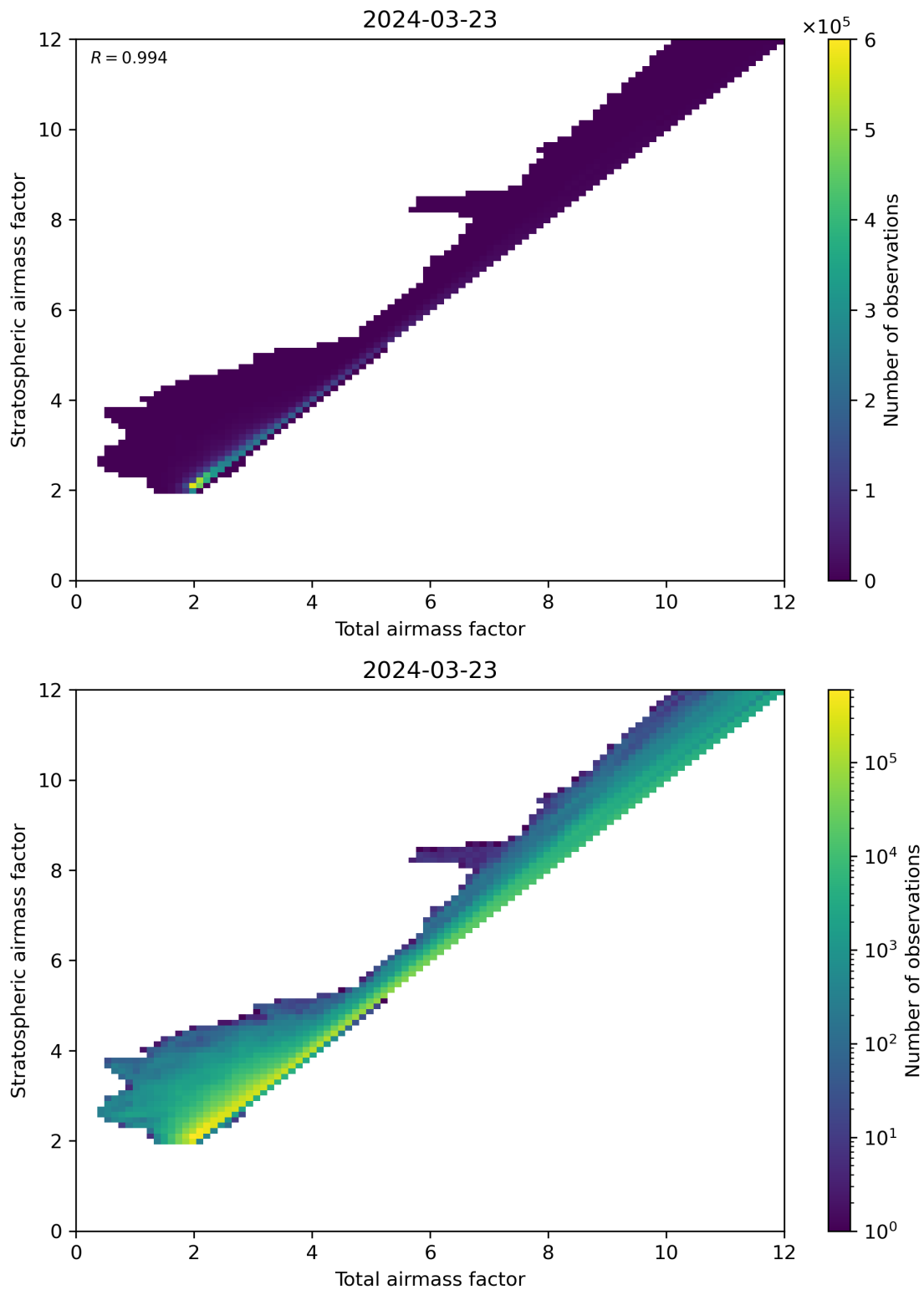
Figure 62: Scatter density plot of “Total airmass factor” against “Stratospheric airmass factor” for 2024-03-23 to 2024-03-24.
