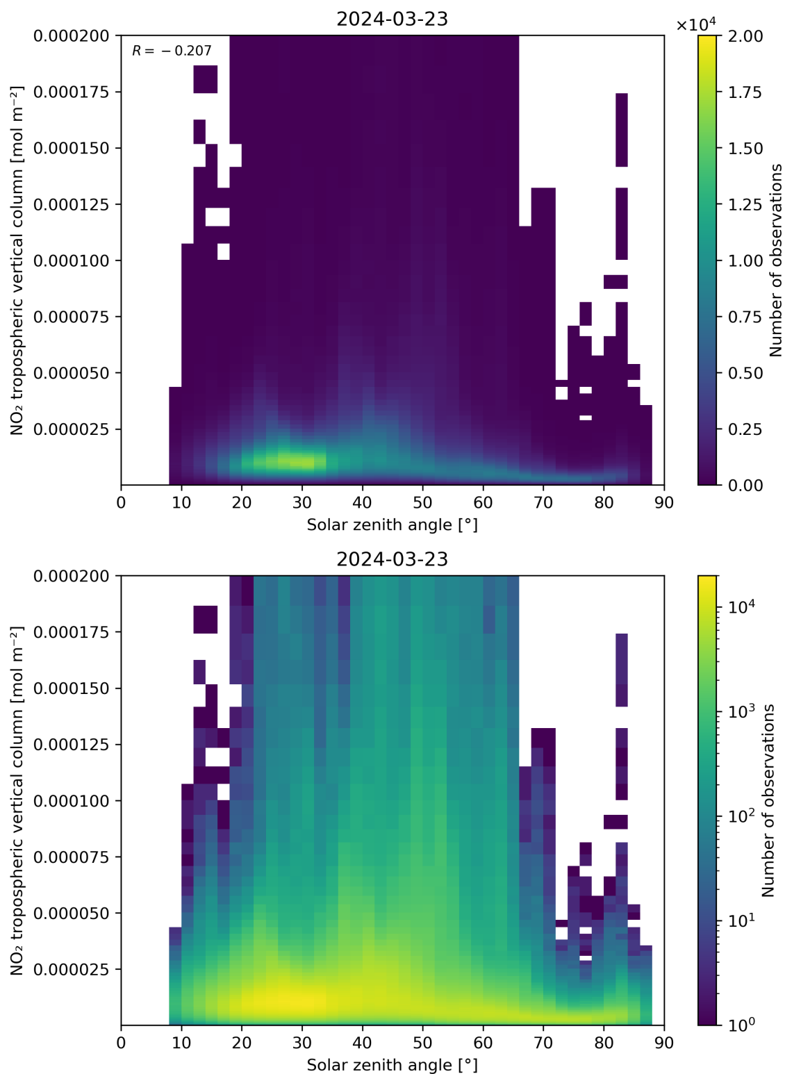
Figure 155: Scatter density plot of “Solar zenith angle” against “NO 2 tropospheric vertical column” for 2024-03-23 to 2024-03-24.
