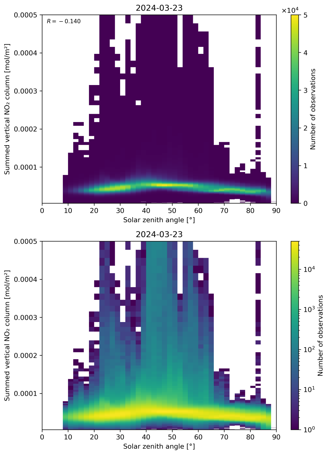
Figure 151: Scatter density plot of “Solar zenith angle” against “Summed vertical NO 2 column” for 2024-03-23 to 2024-03-24.
