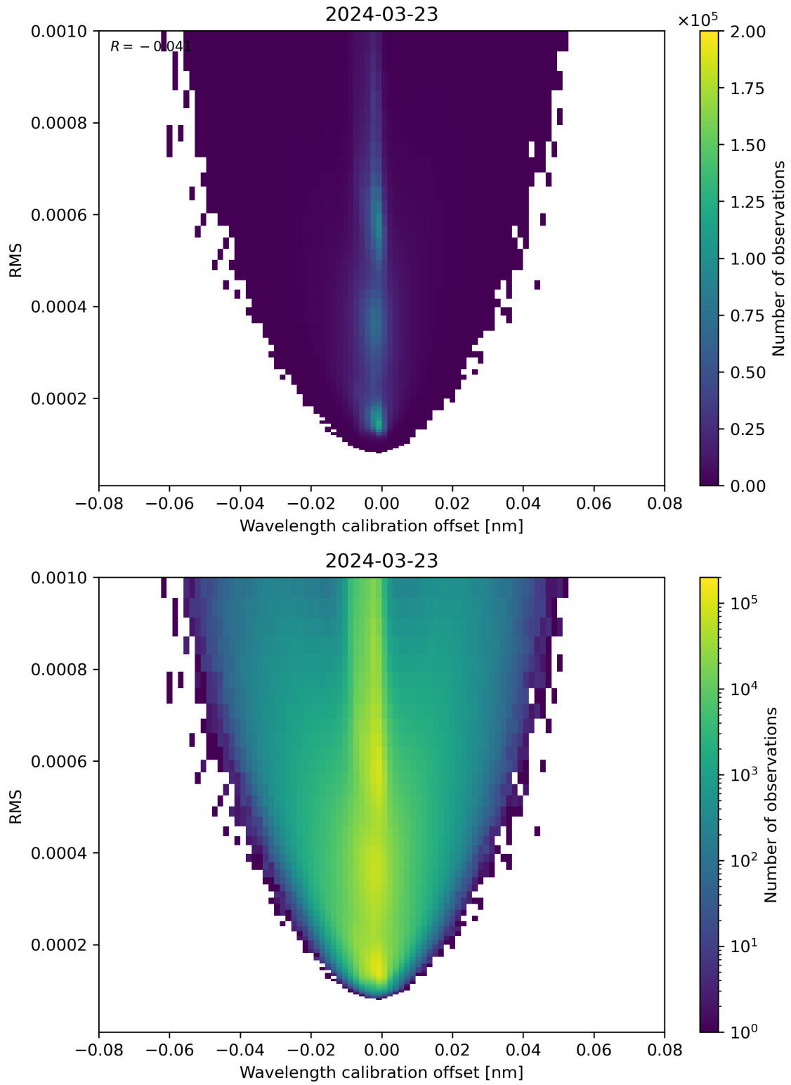
Figure 181: Scatter density plot of “Wavelength calibration offset” against “RMS” for 2024-03-23 to 2024-03-24.
