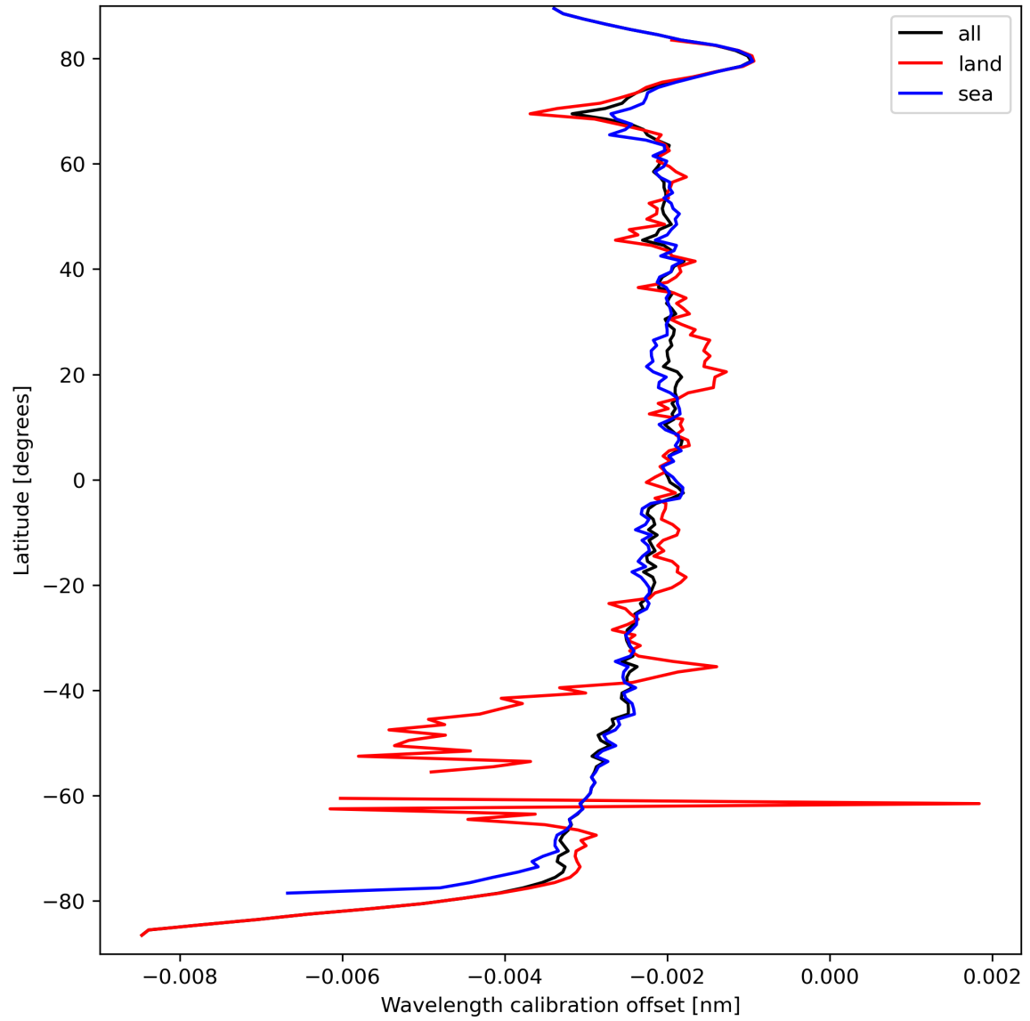
Figure 18: Zonal average of “Wavelength calibration offset” for 2024-03-23 to 2024-03-24.
