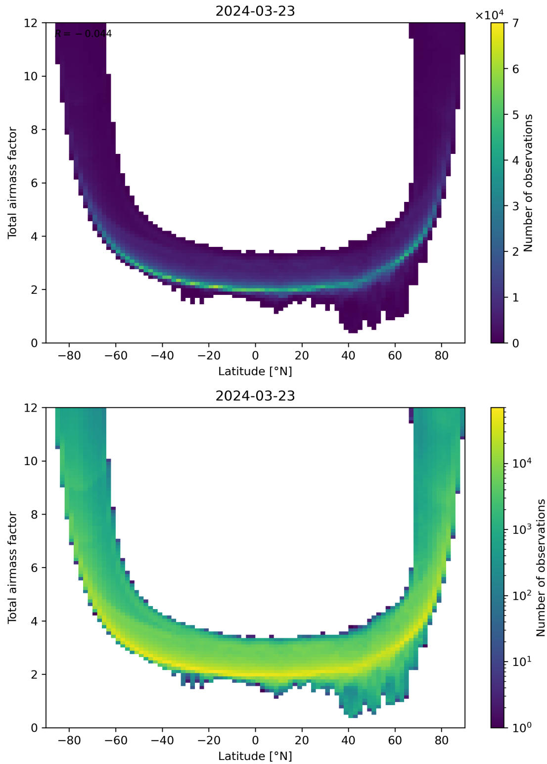
Figure 84: Scatter density plot of “Latitude” against “Total airmass factor” for 2024-03-23 to 2024-03-24.
