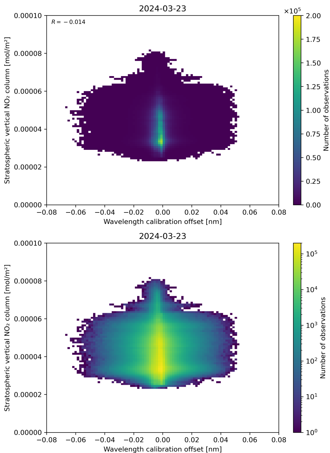
Figure 176: Scatter density plot of “Wavelength calibration offset” against “Stratospheric vertical NO 2 column” for 2024-03-23 to 2024-03-24.
