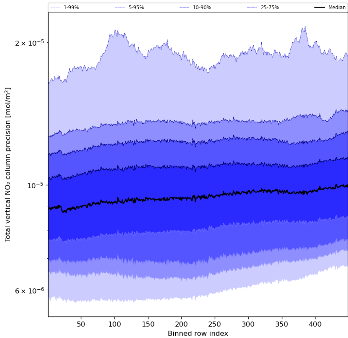
Figure 56: Along track statistics of “Total vertical NO 2 column precision” for 2024-03-23 to 2024-03-24
