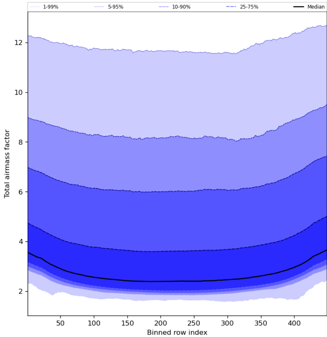
Figure 49: Along track statistics of “Total airmass factor” for 2024-03-23 to 2024-03-24
