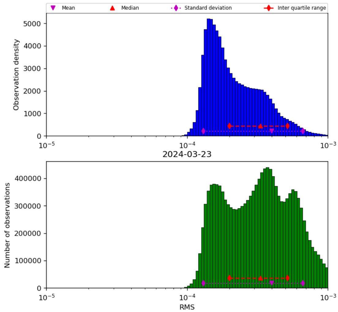
Figure 43: Histogram of “RMS” for 2024-03-23 to 2024-03-24
