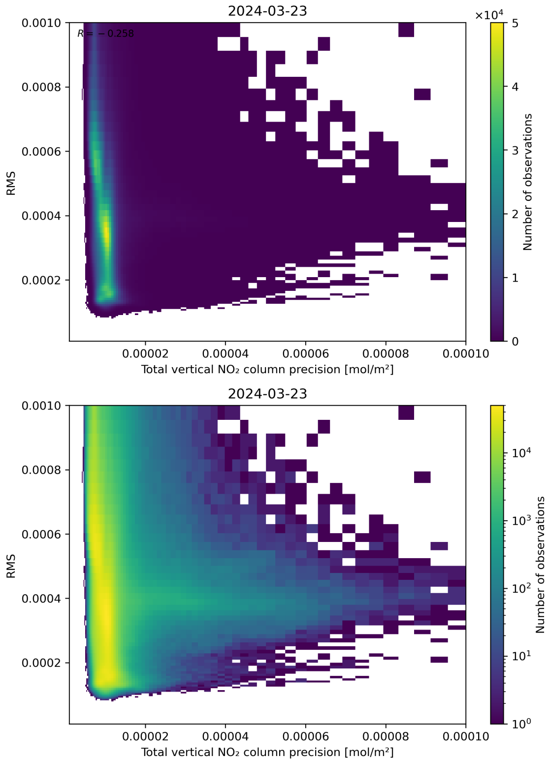
Figure 119: Scatter density plot of “Total vertical NO 2 column precision” against “RMS” for 2024-03-23 to 2024-03-24.
