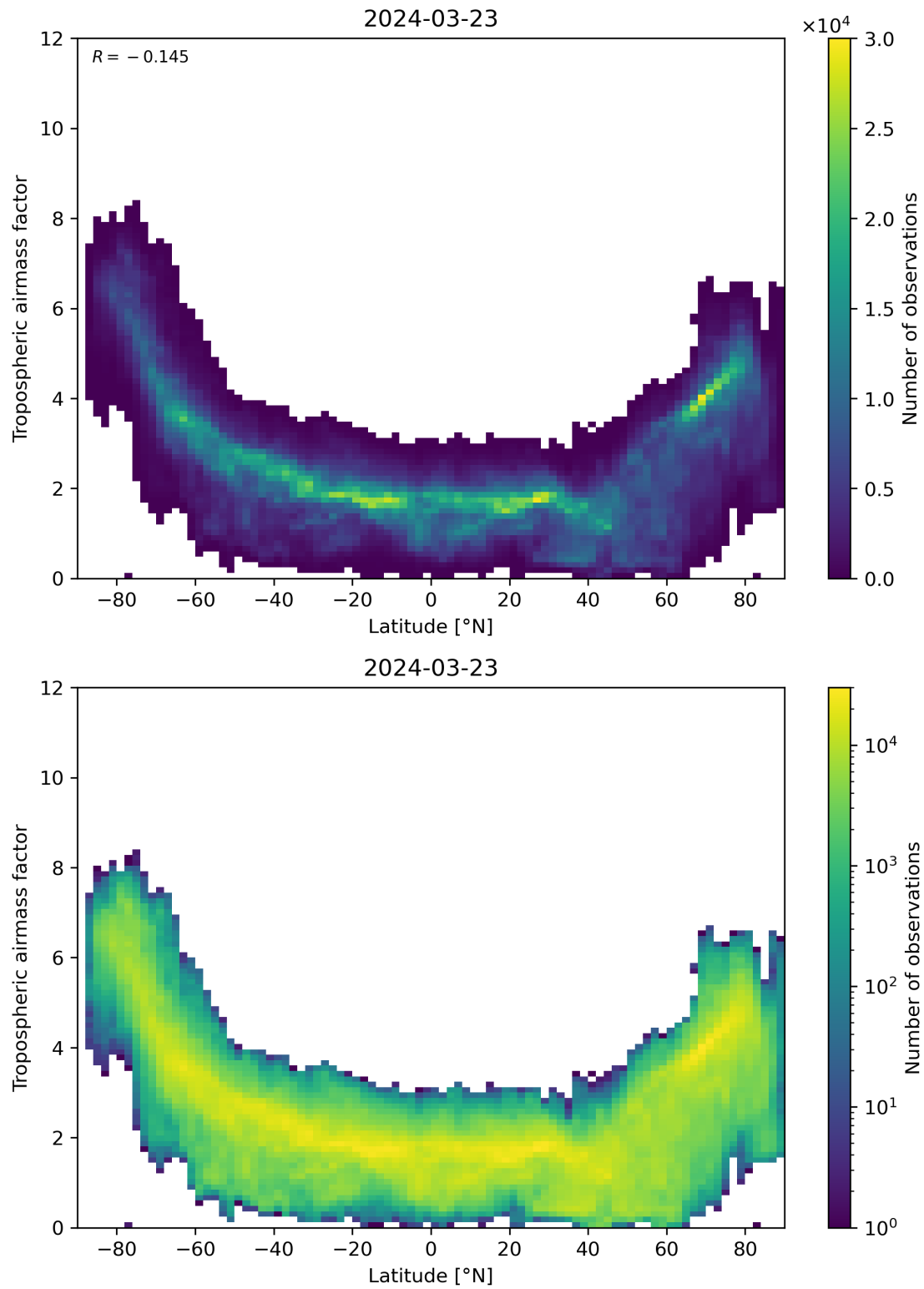
Figure 85: Scatter density plot of “Latitude” against “Tropospheric air mass factor” for 2024-03-23 to 2024-03-24.
