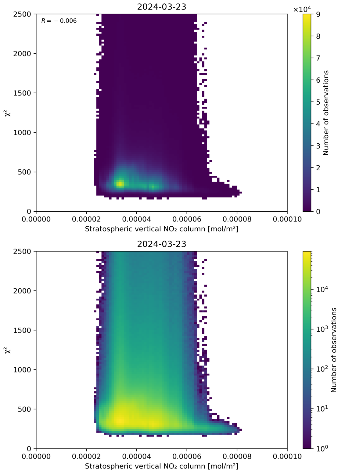
Figure 97: Scatter density plot of “Stratospheric vertical NO 2 column” against “ \chi^2 ” for 2024-03-23 to 2024-03-24.
