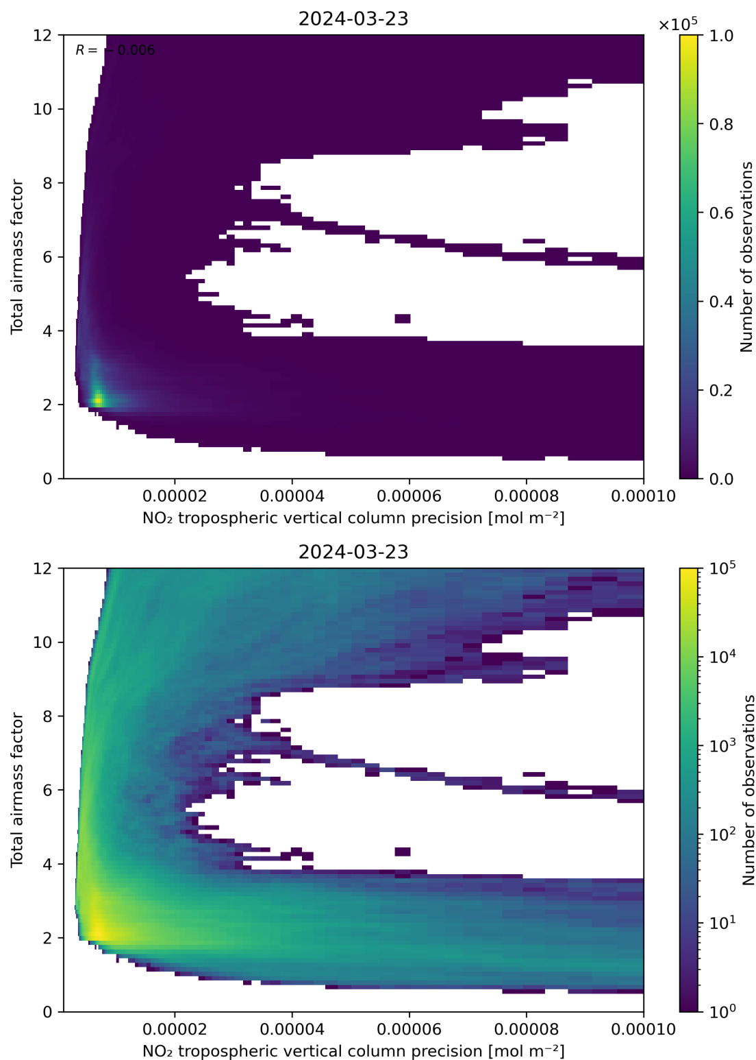
Figure 132: Scatter density plot of “NO 2 tropospheric vertical column precision” against “Total air mass factor” for 2024-03-23 to 2024-03-24.
