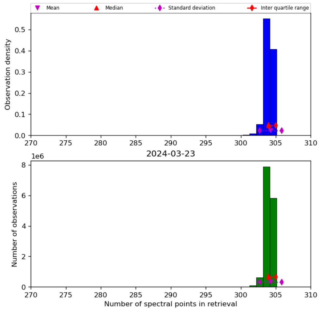
Figure 33: Histogram of “Number of spectral points in retrieval” for 2024-03-23 to 2024-03-24
