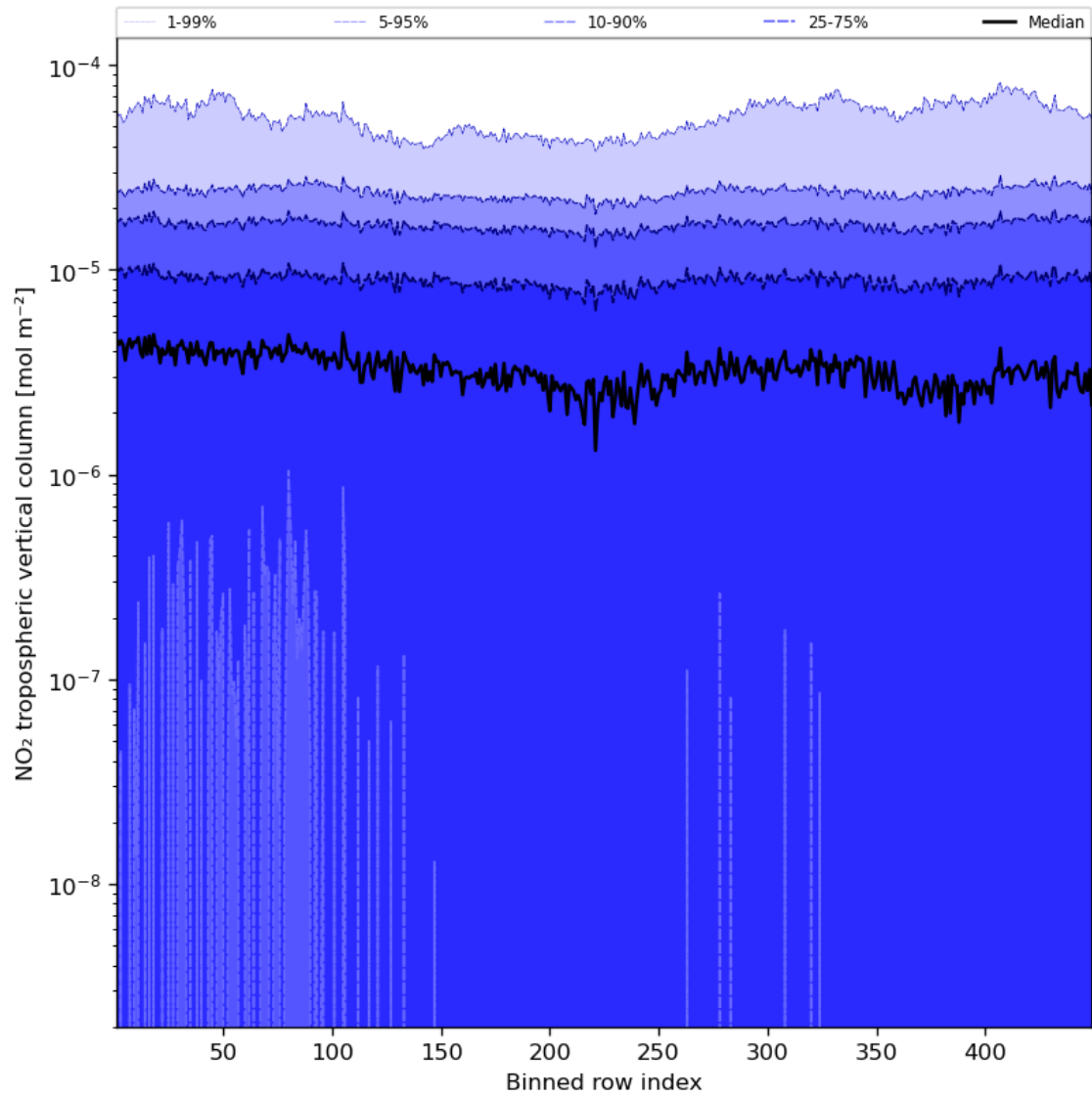
Figure 46: Along track statistics of “NO 2 tropospheric vertical column” for 2024-03-23 to 2024-03-24
