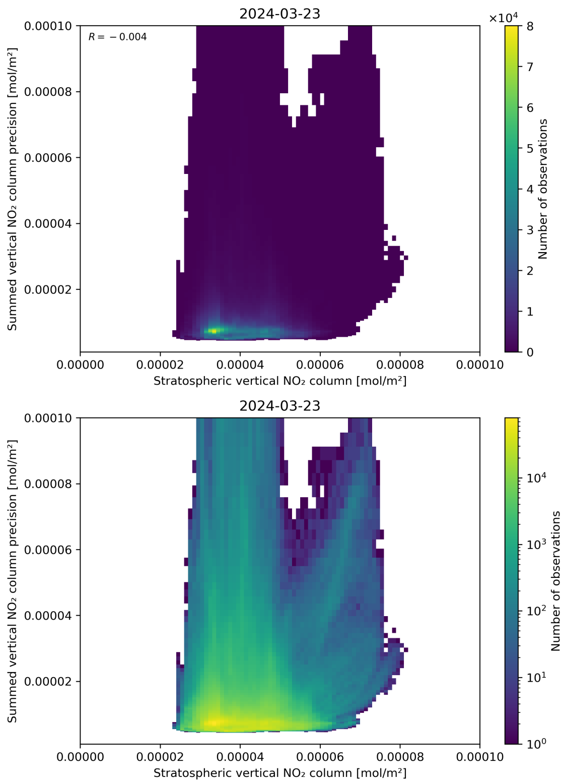
Figure 99: Scatter density plot of “Stratospheric vertical NO 2 column” against “Summed vertical NO 2 column precision” for 2024-03-23 to 2024-03-24.
