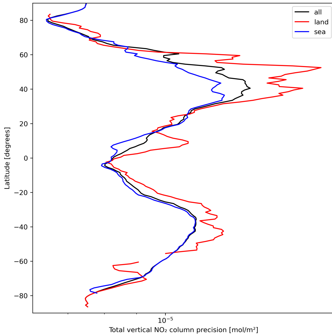
Figure 22: Zonal average of “Total vertical NO 2 column precision” for 2024-03-23 to 2024-03-24.
