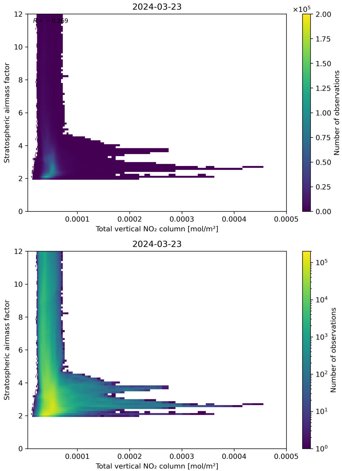
Figure 110: Scatter density plot of “Total vertical NO 2 column” against “Stratospheric airmass factor” for 2024-03-23 to 2024-03-24.
