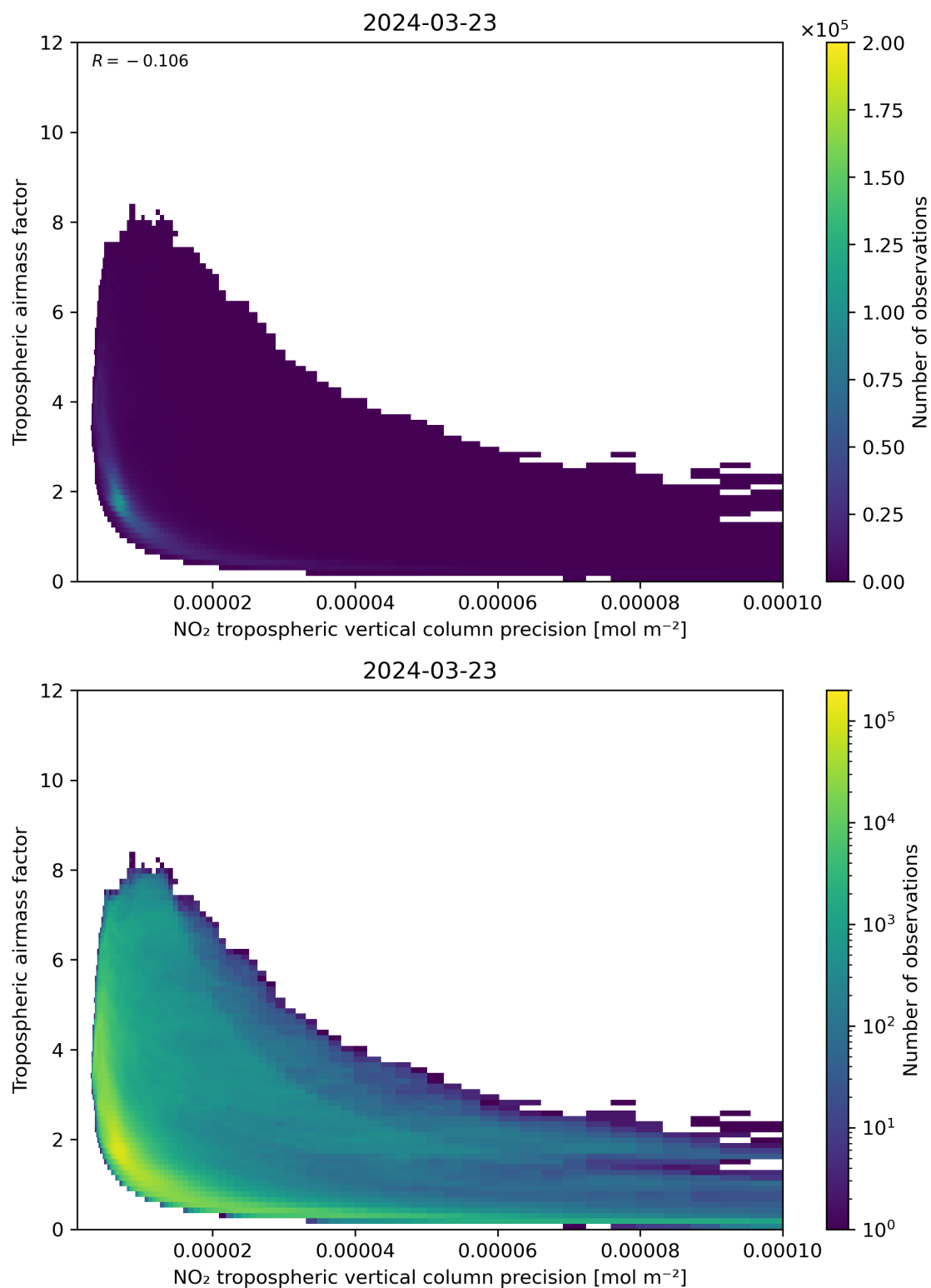
Figure 133: Scatter density plot of “NO 2 tropospheric vertical column precision” against “Tropospheric airmass factor” for 2024-03-23 to 2024-03-24.
