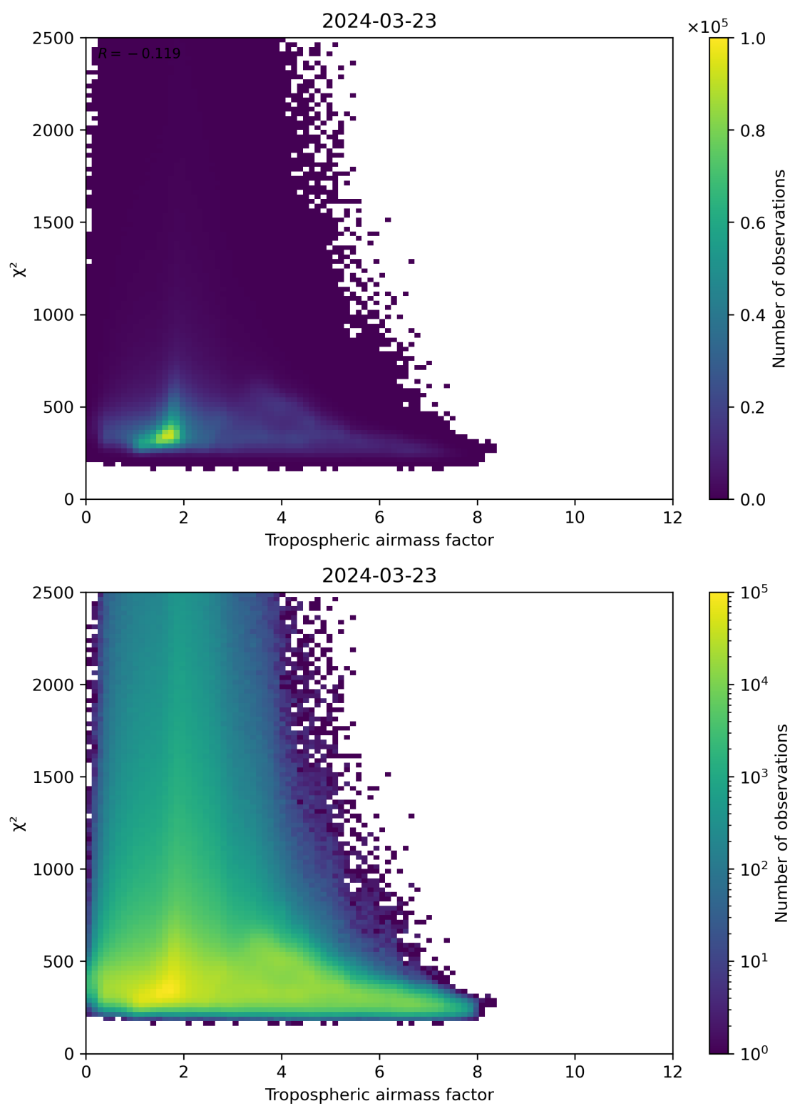
Figure 73: Scatter density plot of “Tropospheric airmass factor” against “ \chi^2 ” for 2024-03-23 to 2024-03-24.
