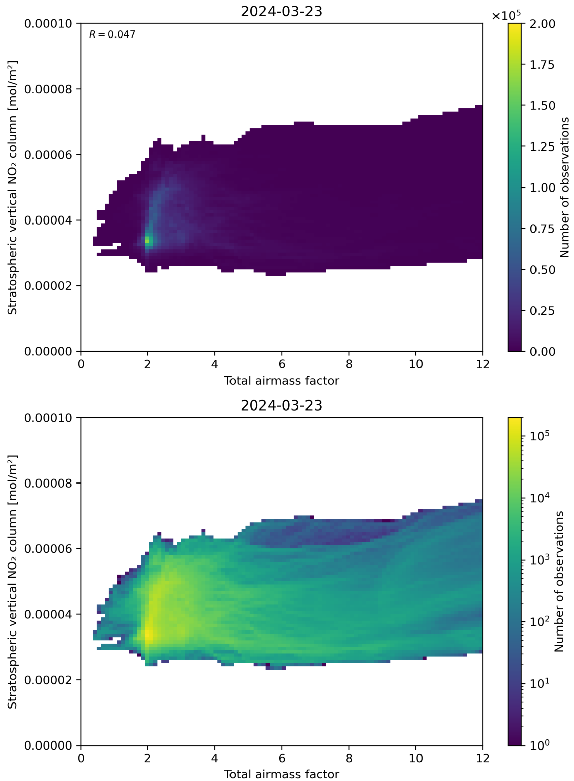
Figure 64: Scatter density plot of “Total airmass factor” against “Stratospheric vertical NO 2 column” for 2024-03-23 to 2024-03-24.
