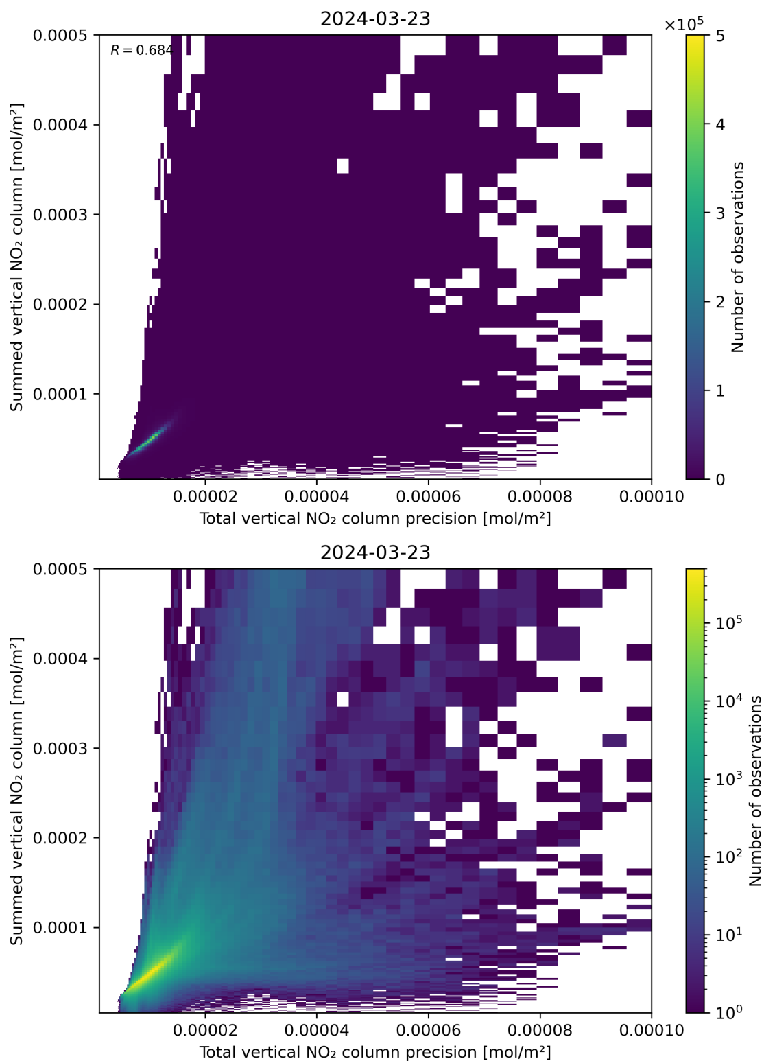
Figure 117: Scatter density plot of “Total vertical NO 2 column precision” against “Summed vertical NO 2 column” for 2024-03-23 to 2024-03-24.
