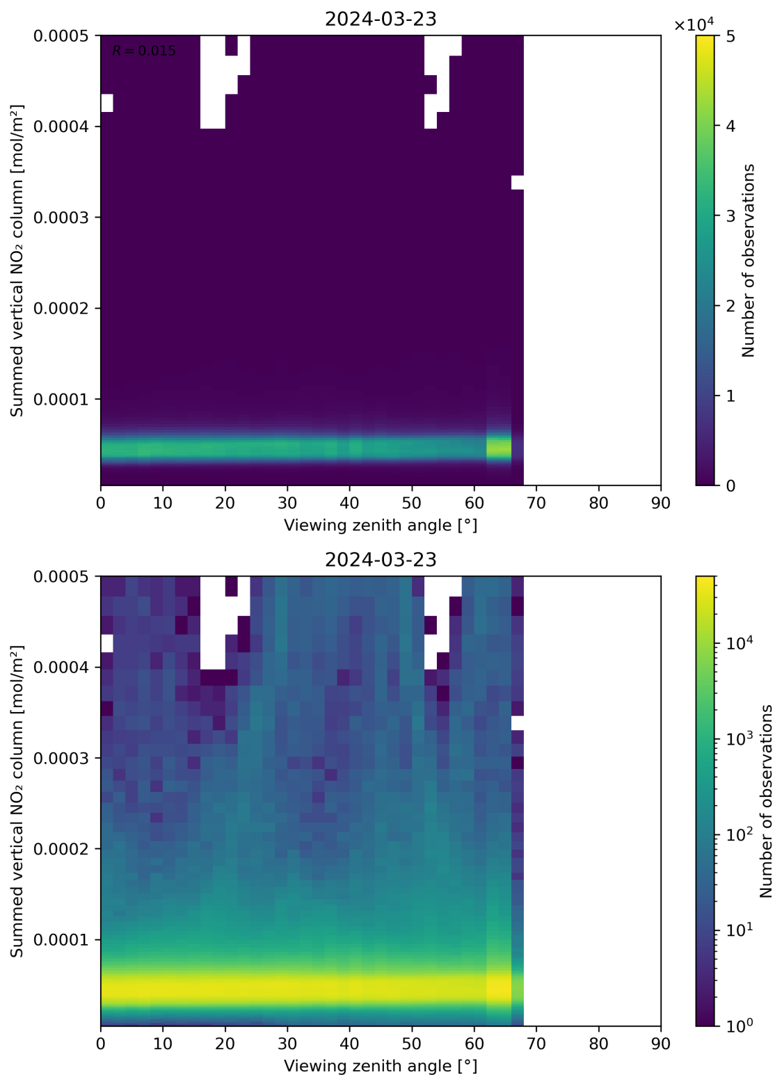
Figure 165: Scatter density plot of “Viewing zenith angle” against “Summed vertical NO 2 column” for 2024-03-23 to 2024-03-24.
