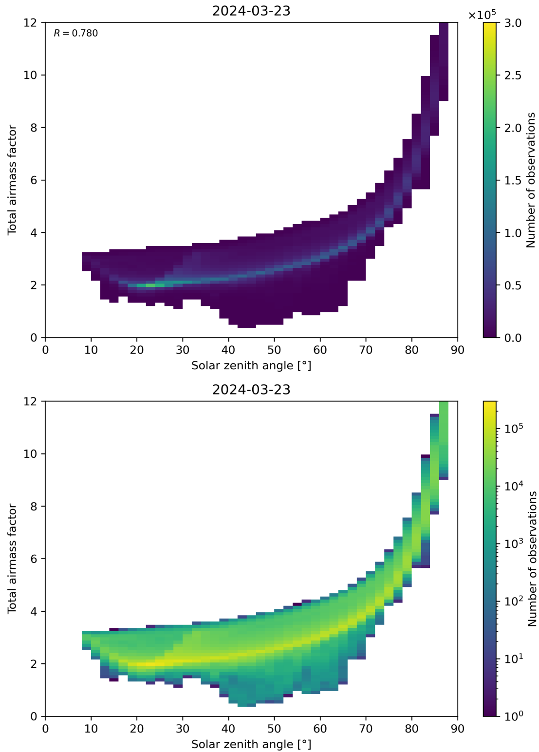
Figure 146: Scatter density plot of “Solar zenith angle” against “Total air mass factor” for 2024-03-23 to 2024-03-24.
