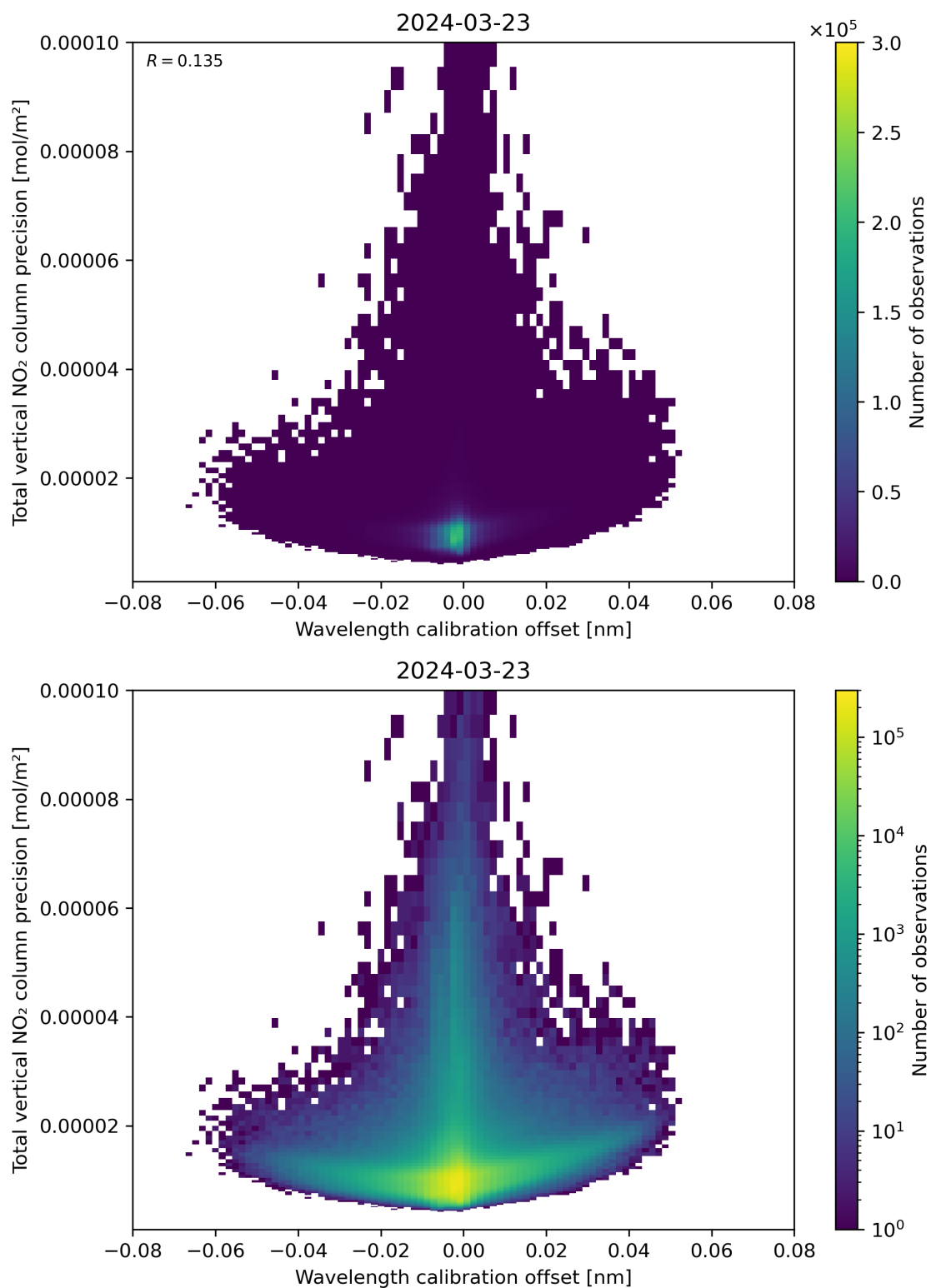
Figure 180: Scatter density plot of “Wavelength calibration offset” against “Total vertical NO 2 column precision” for 2024-03-23 to 2024-03-24.
