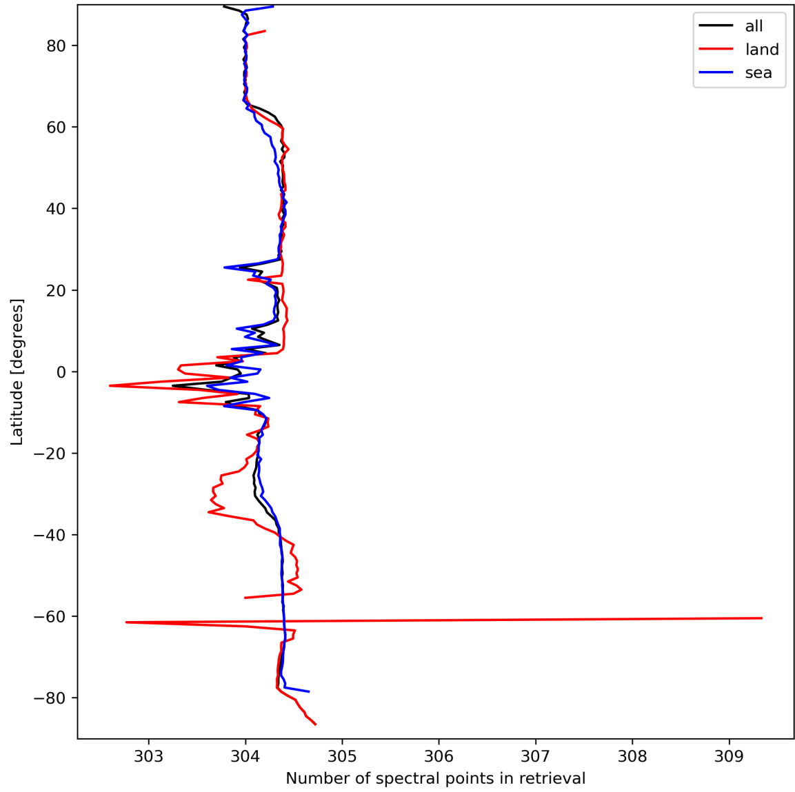
Figure 16: Zonal average of “Number of spectral points in retrieval” for 2024-03-23 to 2024-03-24.
