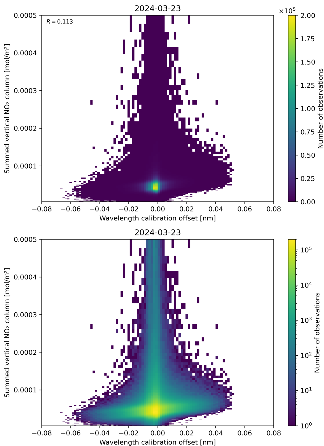
Figure 177: Scatter density plot of “Wavelength calibration offset” against “Summed vertical NO 2 column” for 2024-03-23 to 2024-03-24.
