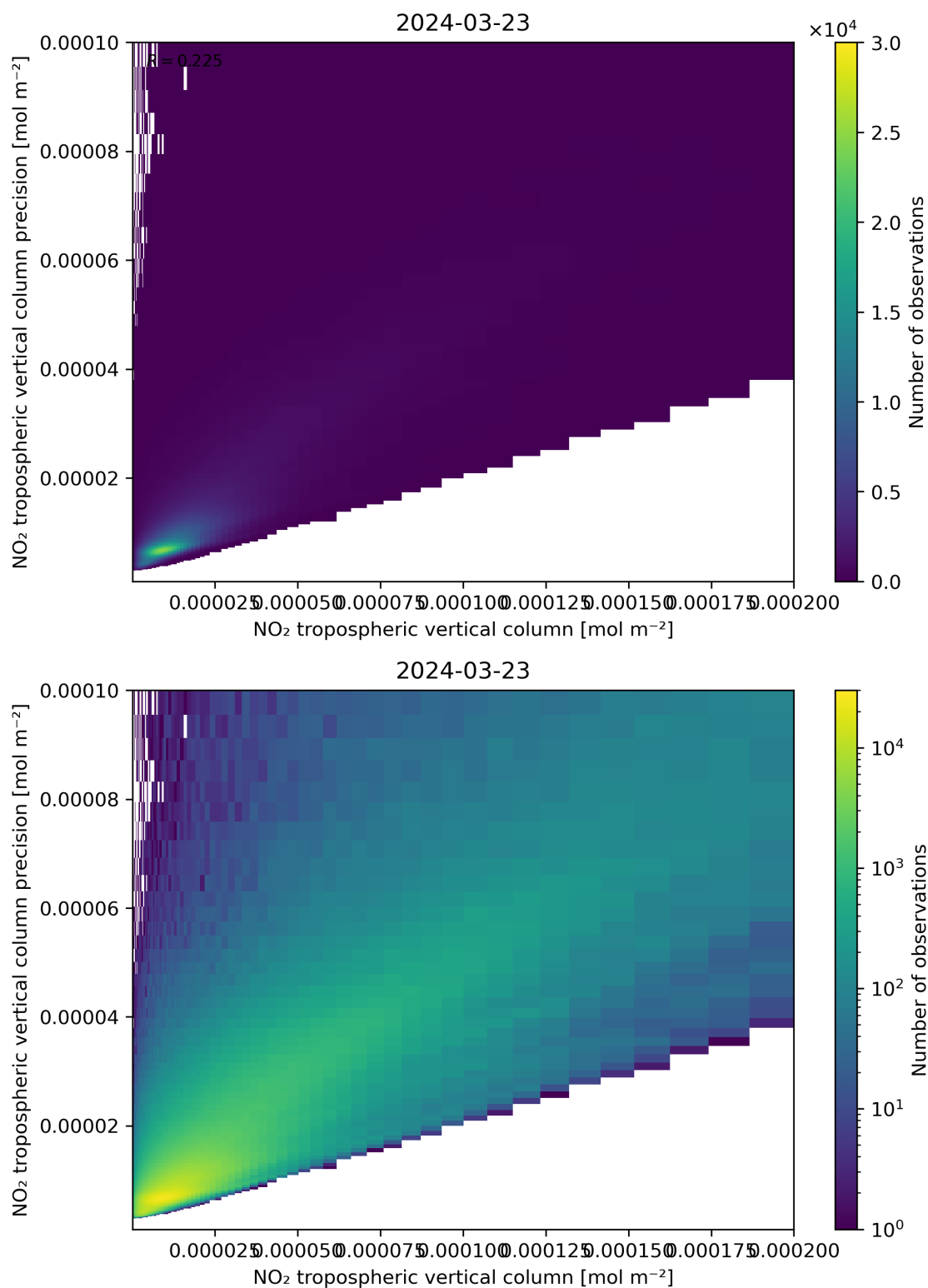
Figure 130: Scatter density plot of “NO 2 tropospheric vertical column” against “NO 2 tropospheric vertical column precision” for 2024-03-23 to 2024-03-24.
