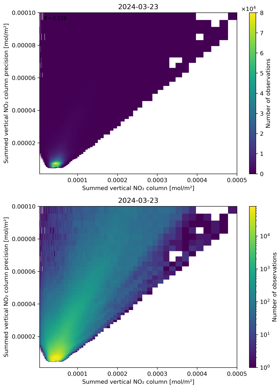
Figure 105: Scatter density plot of “Summed vertical NO 2 column” against “Summed vertical NO 2 column precision” for 2024-03-23 to 2024-03-24.
