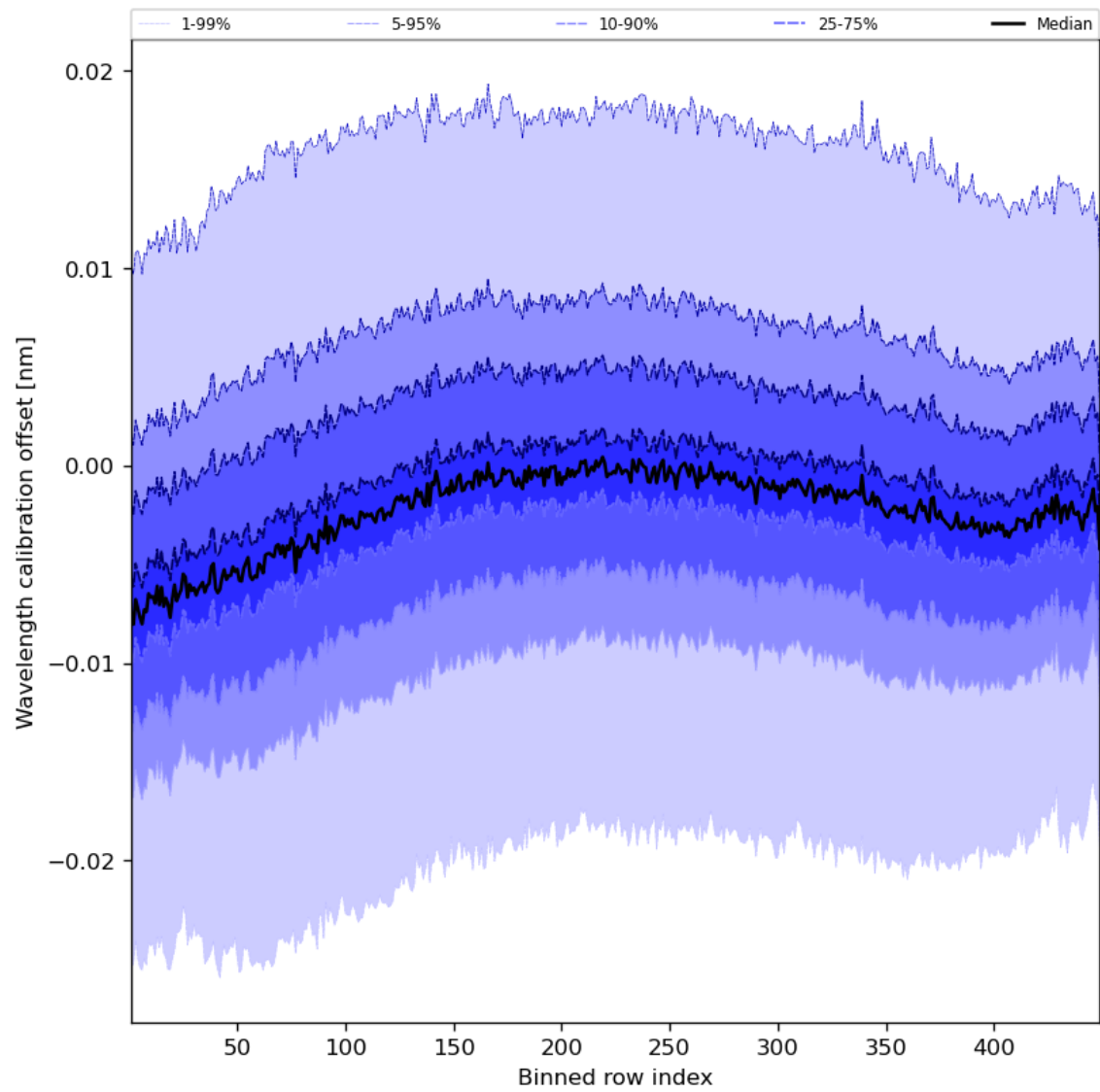
Figure 52: Along track statistics of “Wavelength calibration offset” for 2024-03-23 to 2024-03-24
