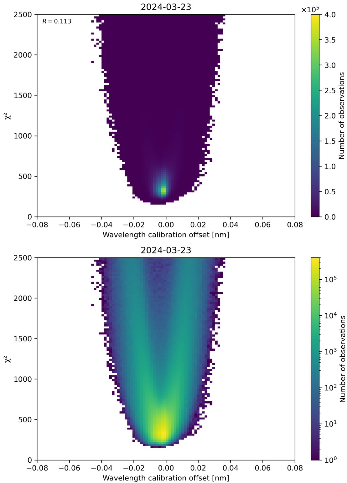
Figure 175: Scatter density plot of “Wavelength calibration offset” against “ \chi^2 ” for 2024-03-23 to 2024-03-24.
