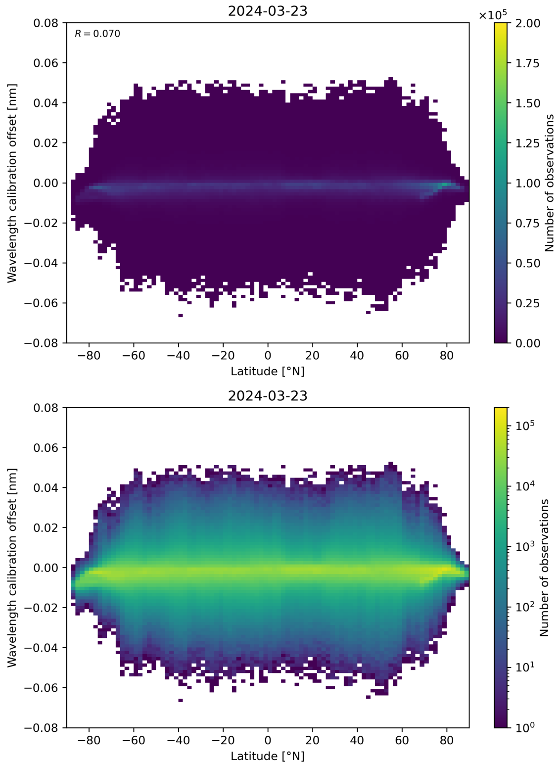
Figure 95: Scatter density plot of “Latitude” against “Wavelength calibration offset” for 2024-03-23 to 2024-03-24.
