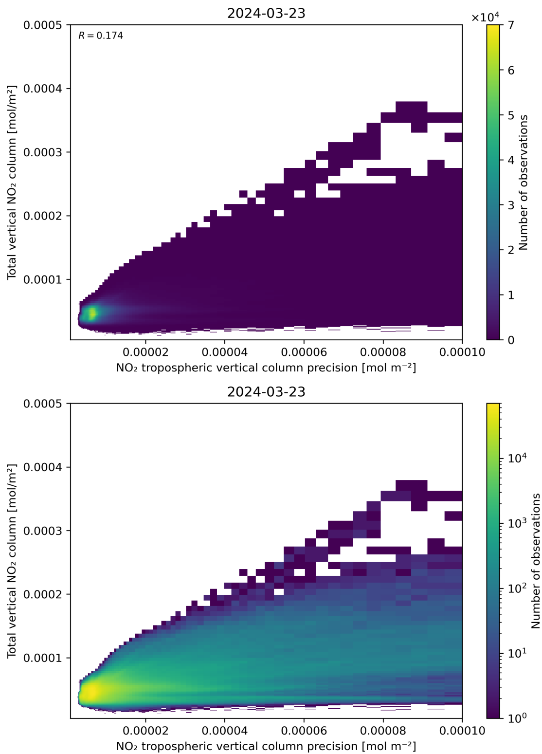
Figure 138: Scatter density plot of “NO 2 tropospheric vertical column precision” against “Total vertical NO 2 column” for 2024-03-23 to 2024-03-24.
