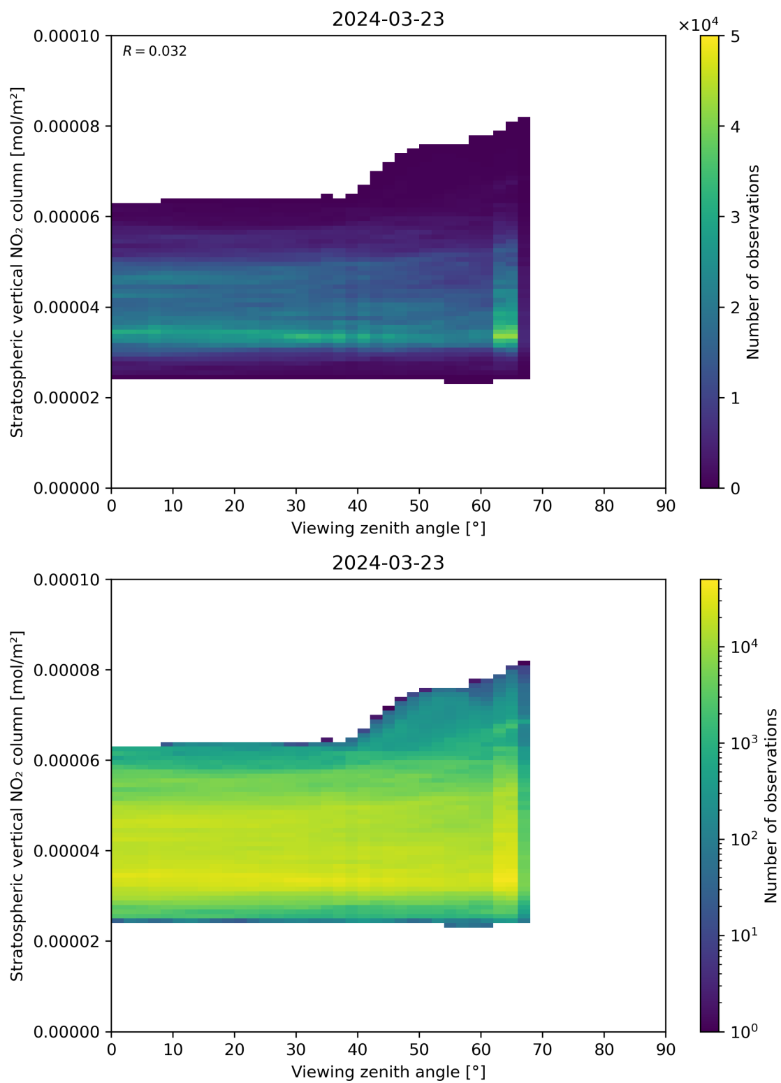
Figure 164: Scatter density plot of “Viewing zenith angle” against “Stratospheric vertical NO 2 column” for 2024-03-23 to 2024-03-24.
