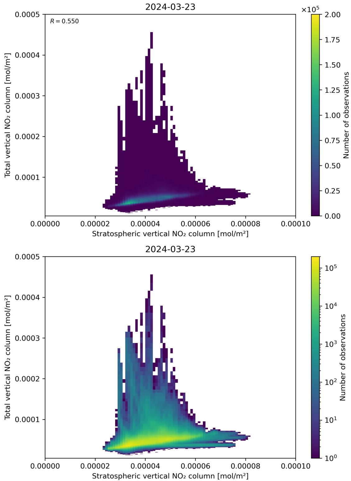
Figure 100: Scatter density plot of “Stratospheric vertical NO 2 column” against “Total vertical NO 2 column” for 2024-03-23 to 2024-03-24.
