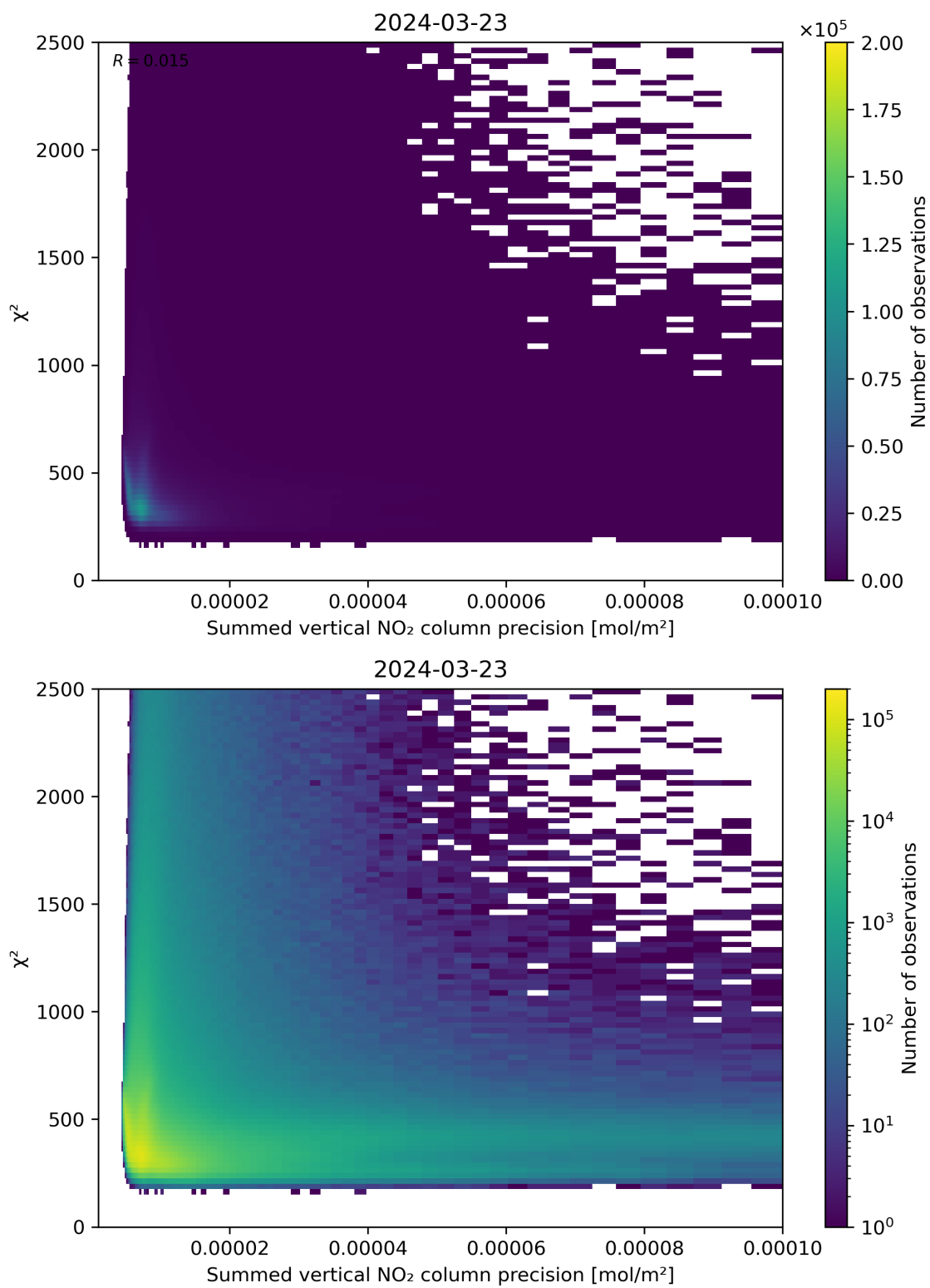
Figure 107: Scatter density plot of “Summed vertical NO 2 column precision” against “ \chi^2 ” for 2024-03-23 to 2024-03-24.
