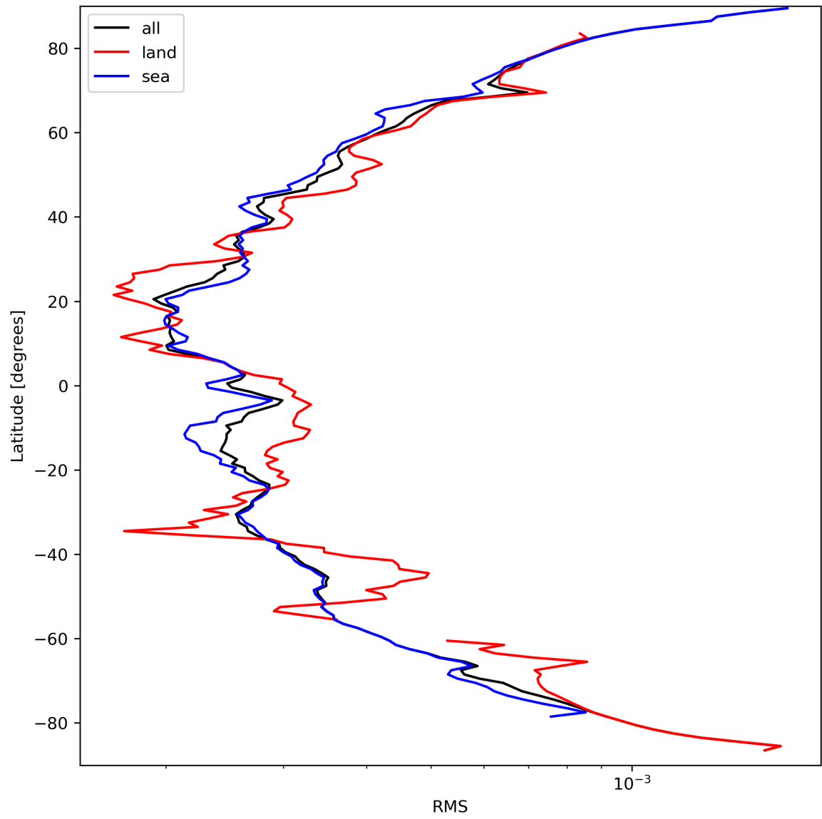
Figure 26: Zonal average of “RMS” for 2024-03-23 to 2024-03-24.
