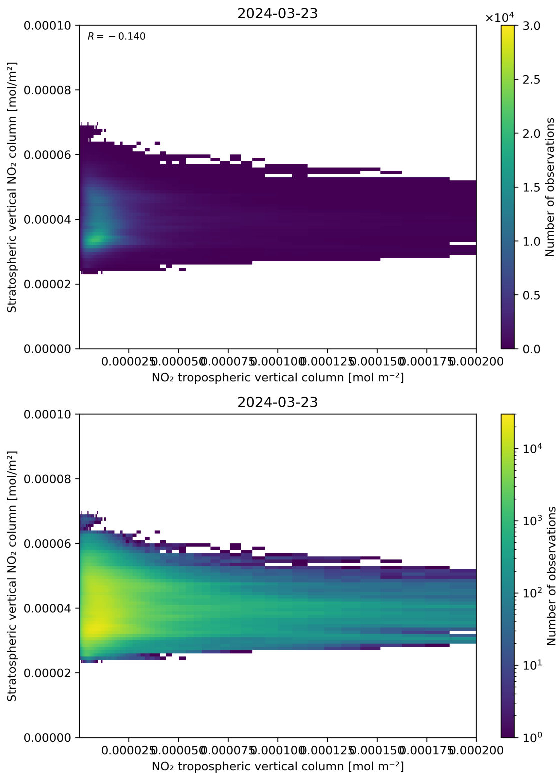
Figure 125: Scatter density plot of “NO 2 tropospheric vertical column” against “Stratospheric vertical NO 2 column” for 2024-03-23 to 2024-03-24.
