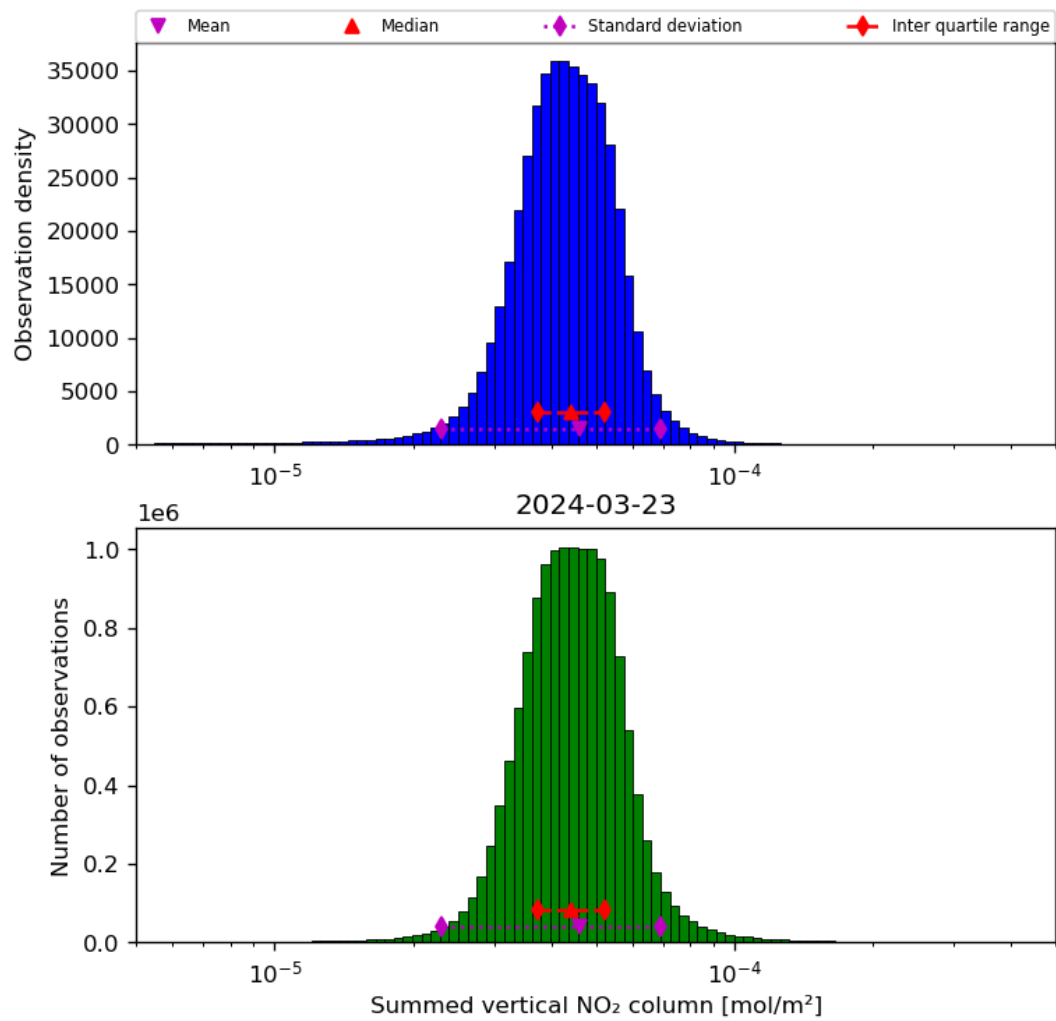
Figure 40: Histogram of “Summed vertical NO 2 column” for 2024-03-23 to 2024-03-24
