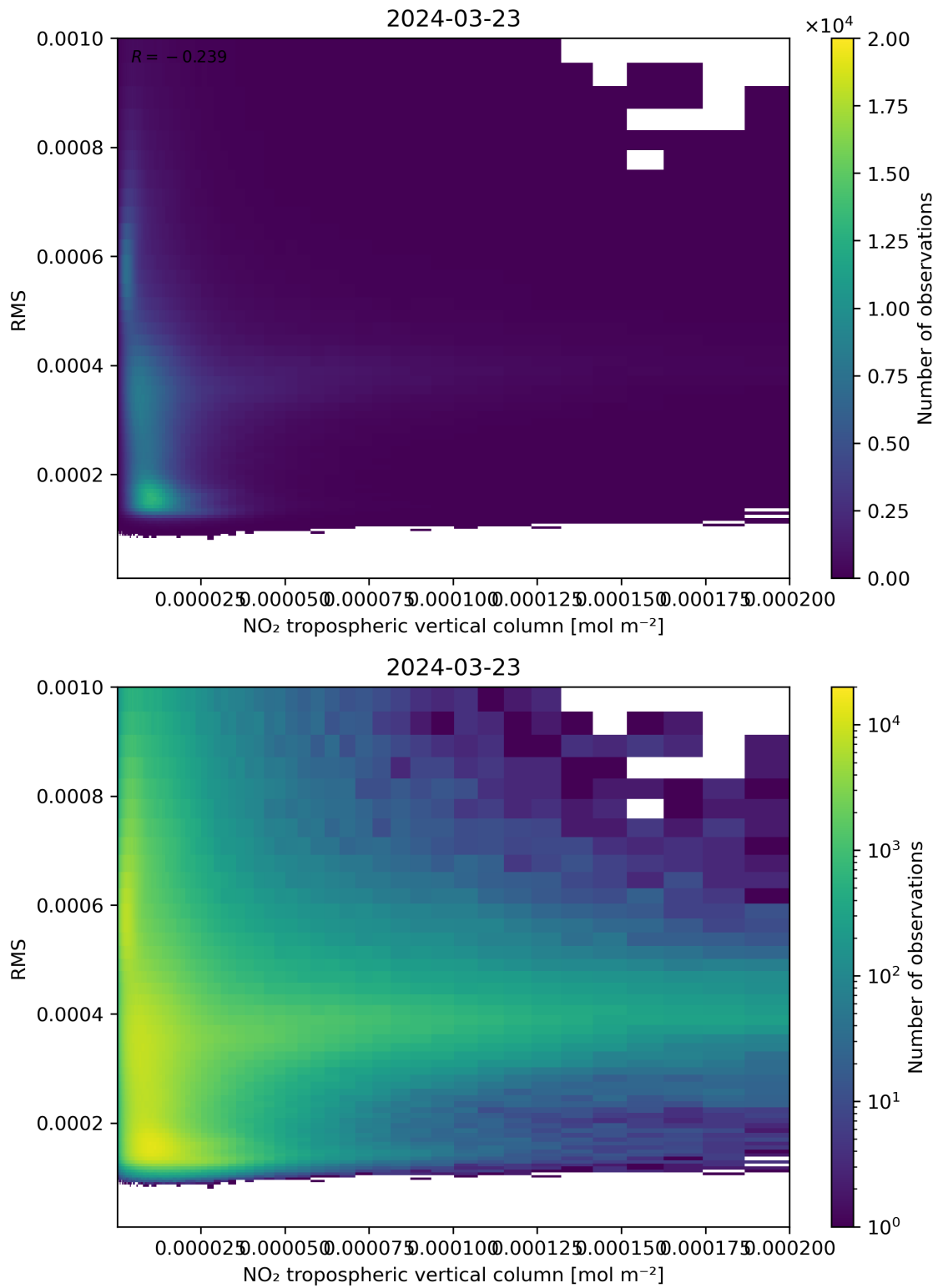
Figure 142: Scatter density plot of “NO 2 tropospheric vertical column” against “RMS” for 2024-03-23 to 2024-03-24.
