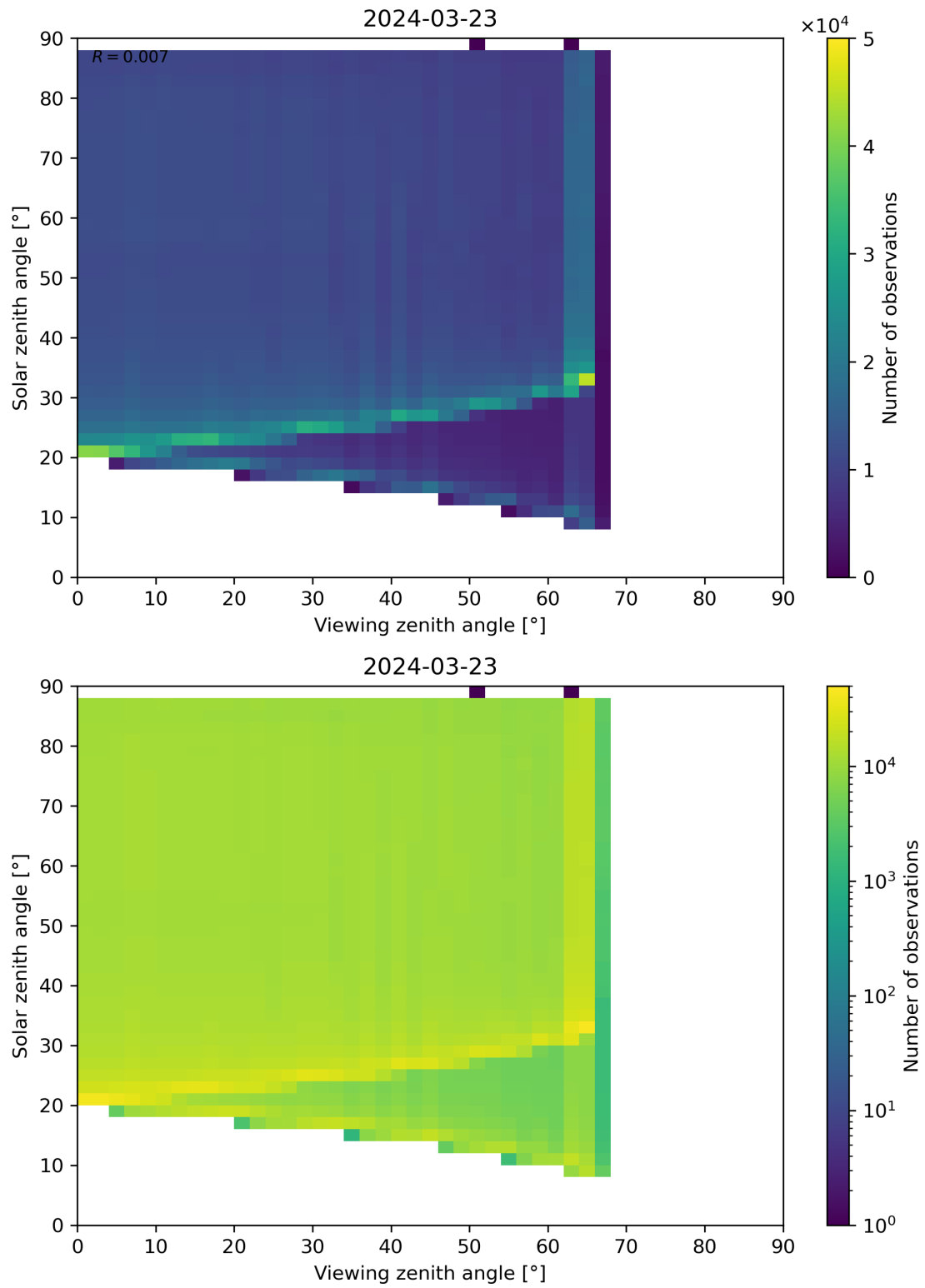
Figure 172: Scatter density plot of “Viewing zenith angle” against “Solar zenith angle” for 2024-03-23 to 2024-03-24.
