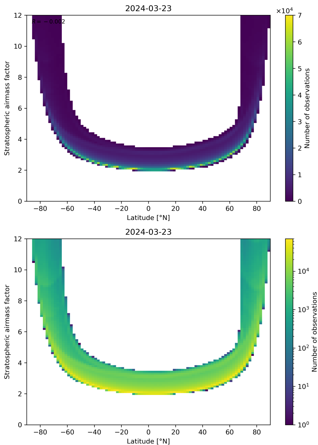
Figure 83: Scatter density plot of “Latitude” against “Stratospheric airmass factor” for 2024-03-23 to 2024-03-24.
