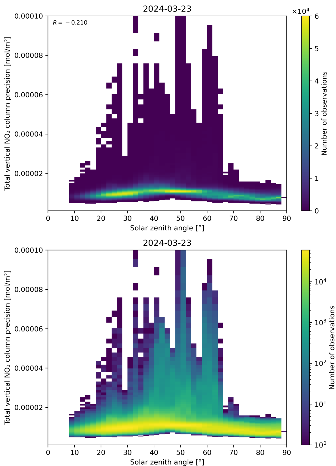
Figure 154: Scatter density plot of “Solar zenith angle” against “Total vertical NO 2 column precision” for 2024-03-23 to 2024-03-24.
