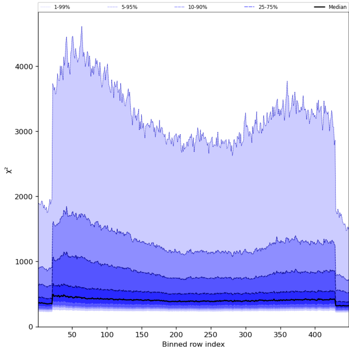
Figure 59: Along track statistics of “ \chi^2 ” for 2024-03-23 to 2024-03-24
