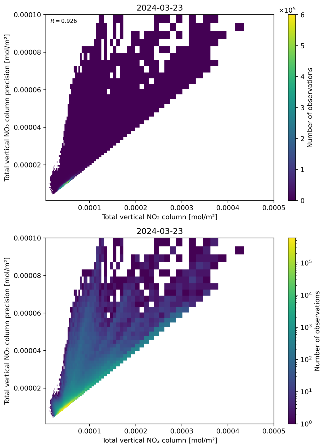
Figure 114: Scatter density plot of “Total vertical NO 2 column” against “Total vertical NO 2 column precision” for 2024-03-23 to 2024-03-24.
