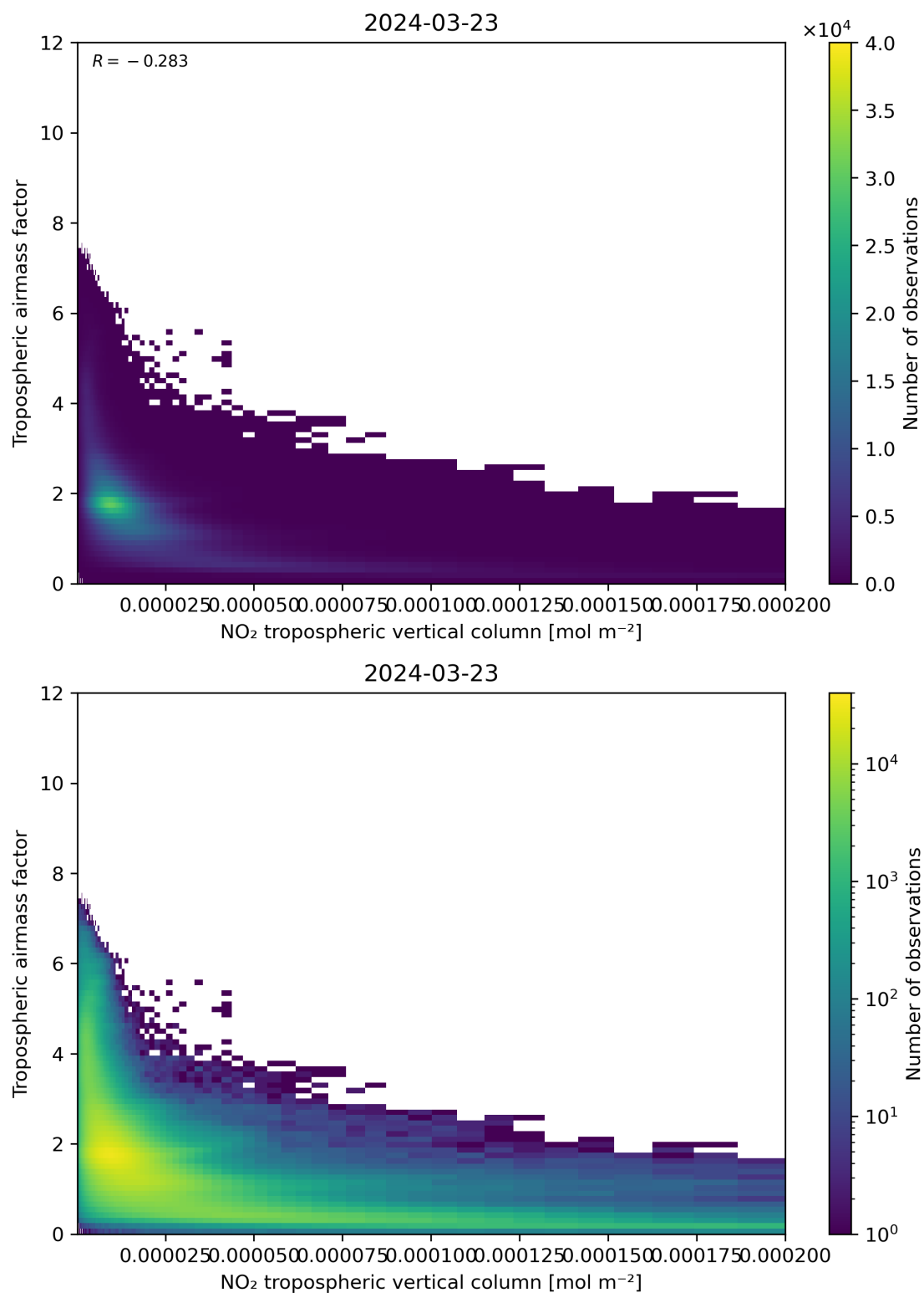
Figure 123: Scatter density plot of “NO 2 tropospheric vertical column” against “Tropospheric airmass factor” for 2024-03-23 to 2024-03-24.
