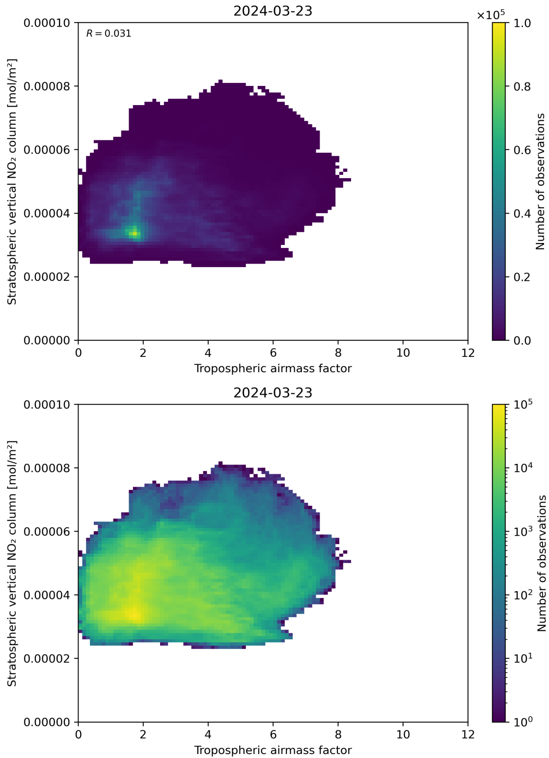
Figure 74: Scatter density plot of “Tropospheric air mass factor” against “Stratospheric vertical NO 2 column” for 2024-03-23 to 2024-03-24.
