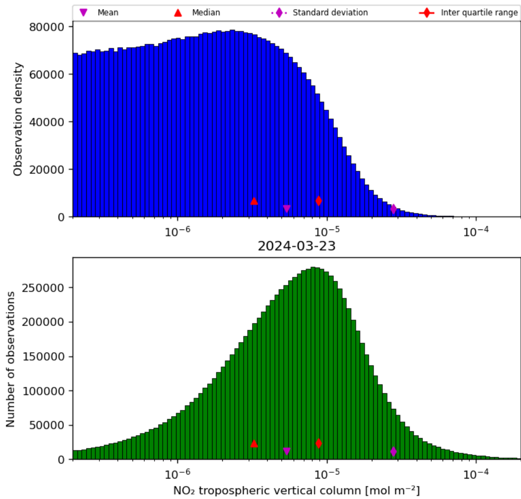
Figure 29: Histogram of “NO 2 tropospheric vertical column” for 2024-03-23 to 2024-03-24
