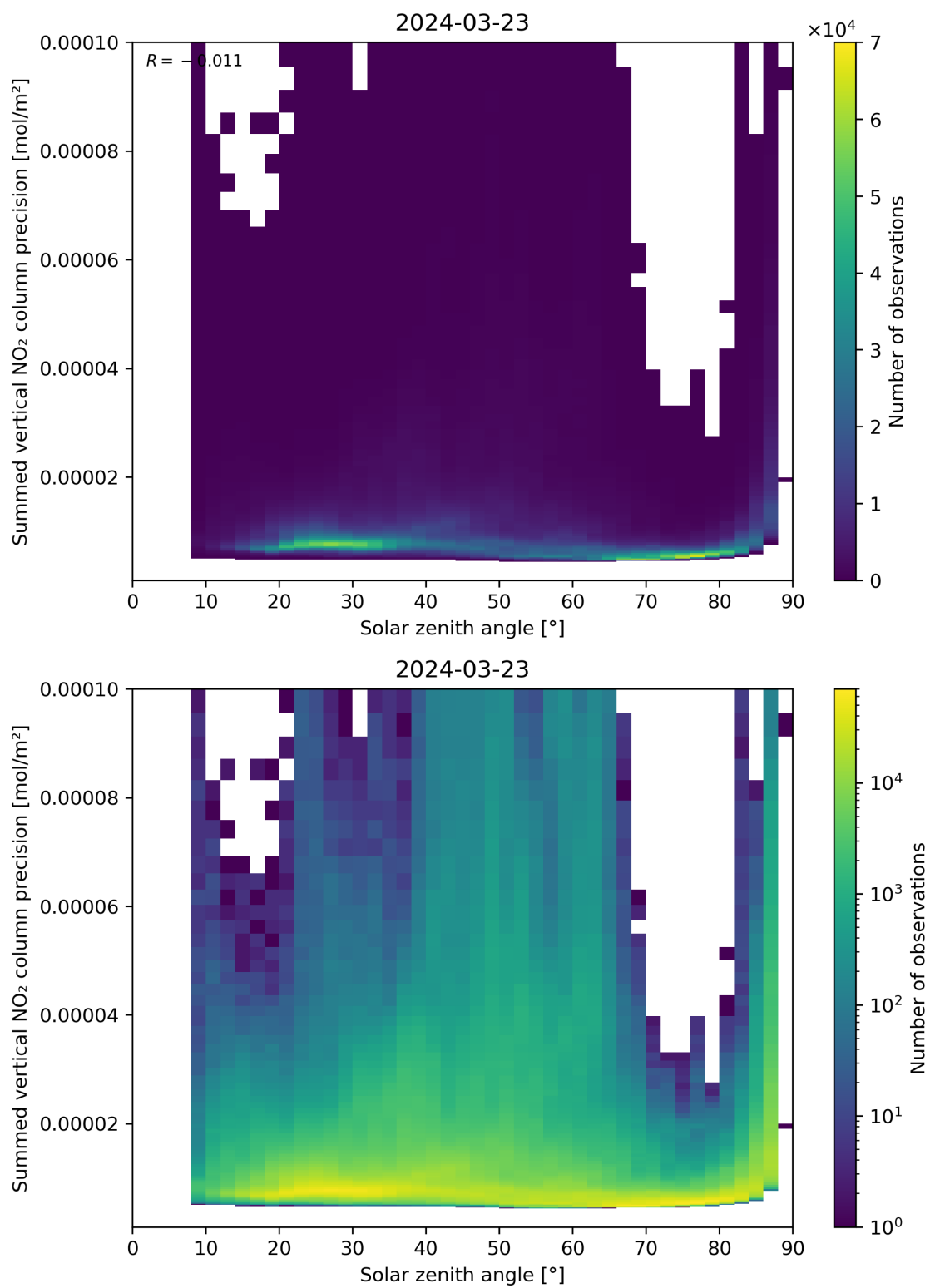
Figure 152: Scatter density plot of “Solar zenith angle” against “Summed vertical NO 2 column precision” for 2024-03-23 to 2024-03-24.
