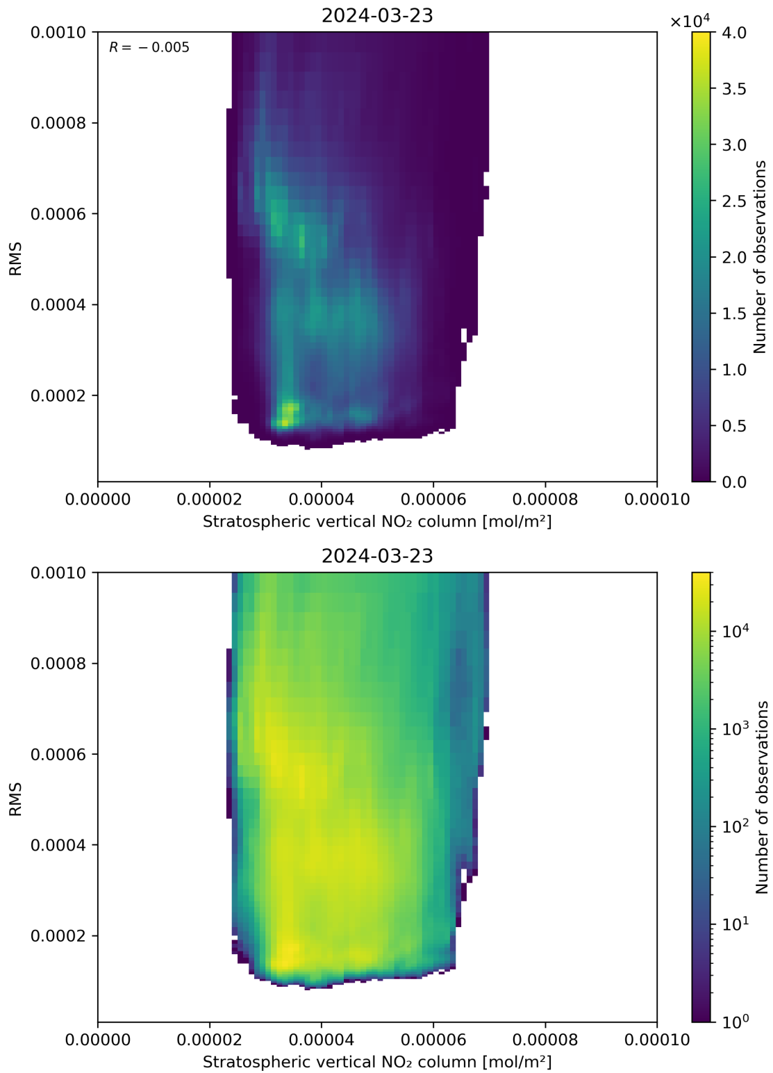
Figure 102: Scatter density plot of “Stratospheric vertical NO 2 column” against “RMS” for 2024-03-23 to 2024-03-24.
