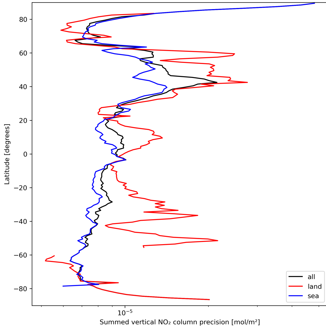
Figure 24: Zonal average of “Summed vertical NO 2 column precision” for 2024-03-23 to 2024-03-24.
