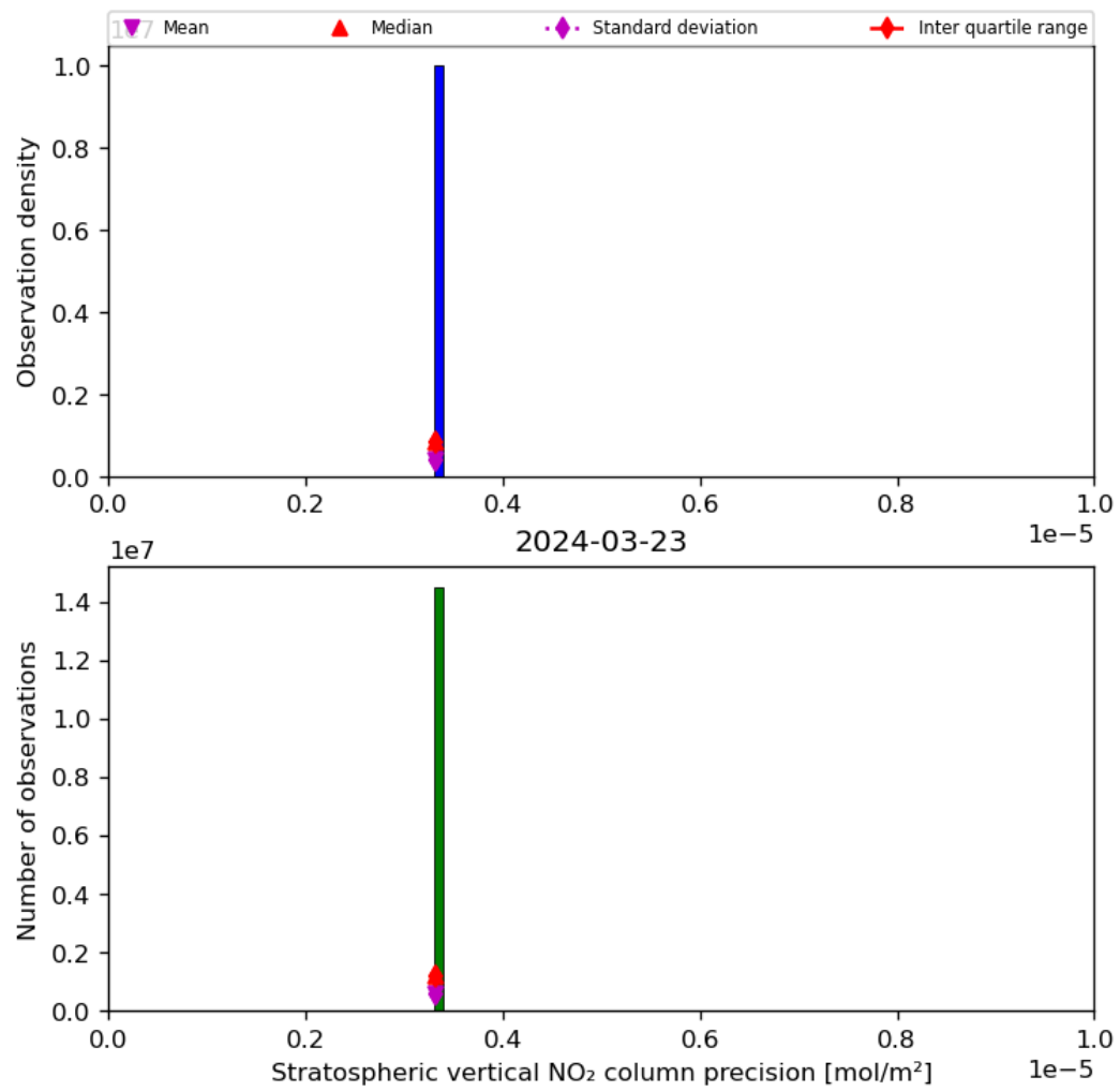
Figure 37: Histogram of “Stratospheric vertical NO 2 column precision” for 2024-03-23 to 2024-03-24
