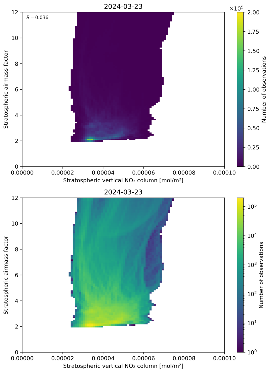
Figure 96: Scatter density plot of “Stratospheric vertical NO 2 column” against “Stratospheric airmass factor” for 2024-03-23 to 2024-03-24.
