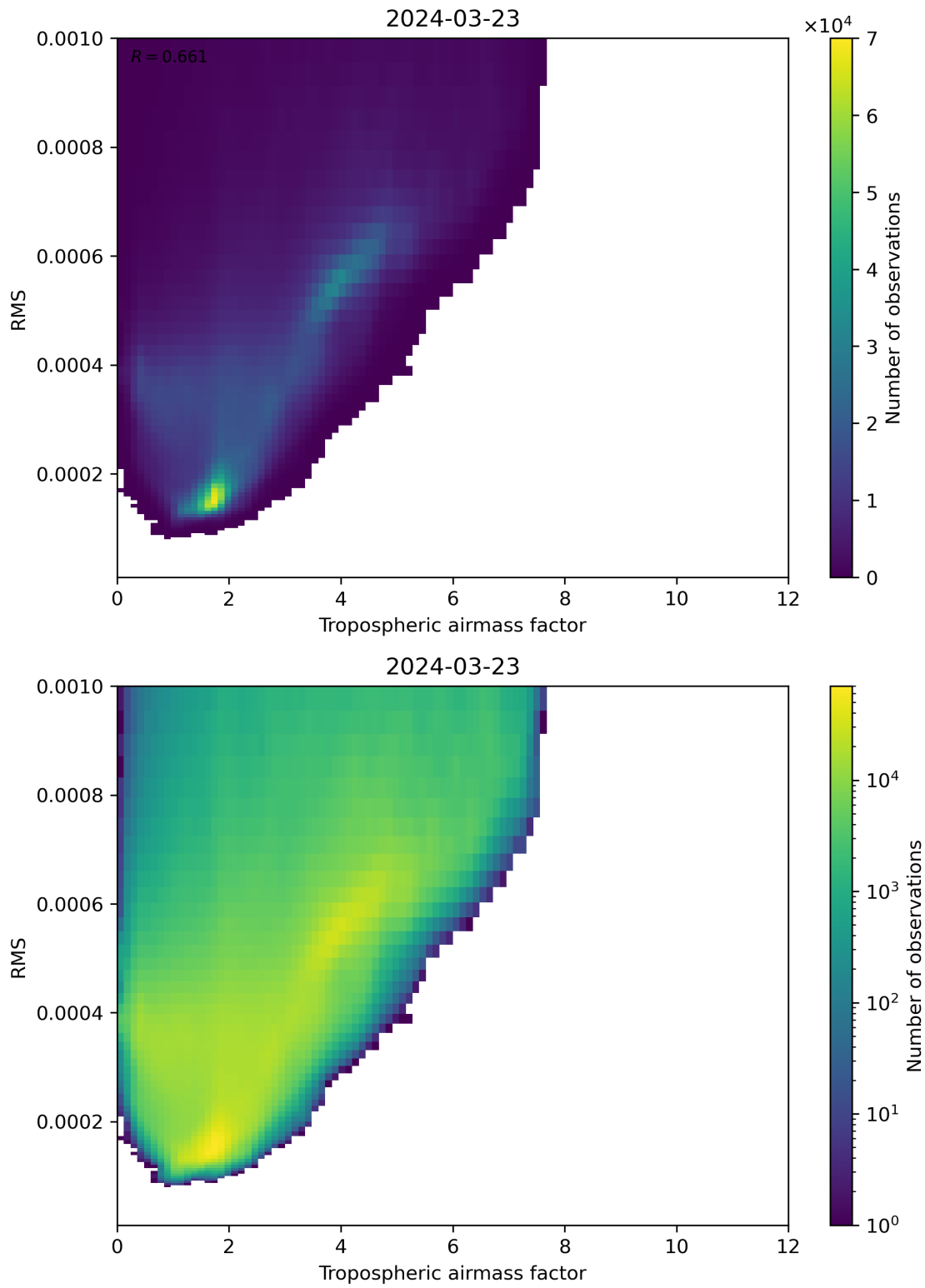
Figure 79: Scatter density plot of “Tropospheric airmass factor” against “RMS” for 2024-03-23 to 2024-03-24.
