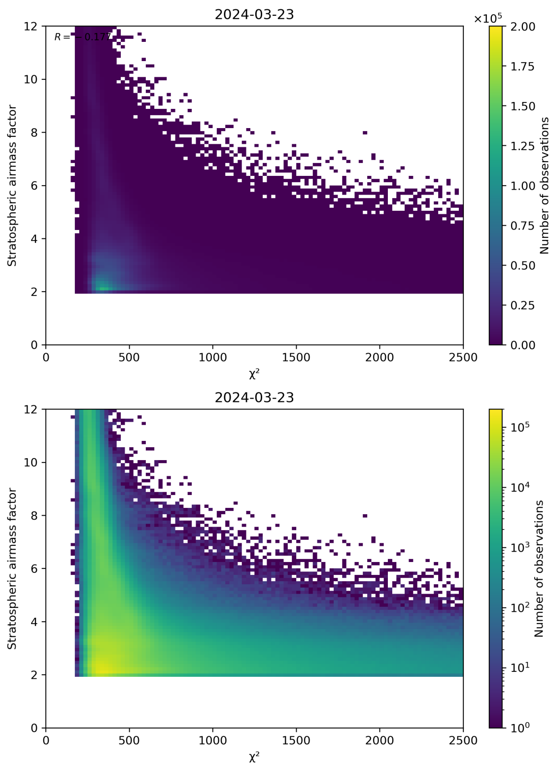
Figure 81: Scatter density plot of “ \chi^2 ” against “Stratospheric airmass factor” for 2024-03-23 to 2024-03-24.
