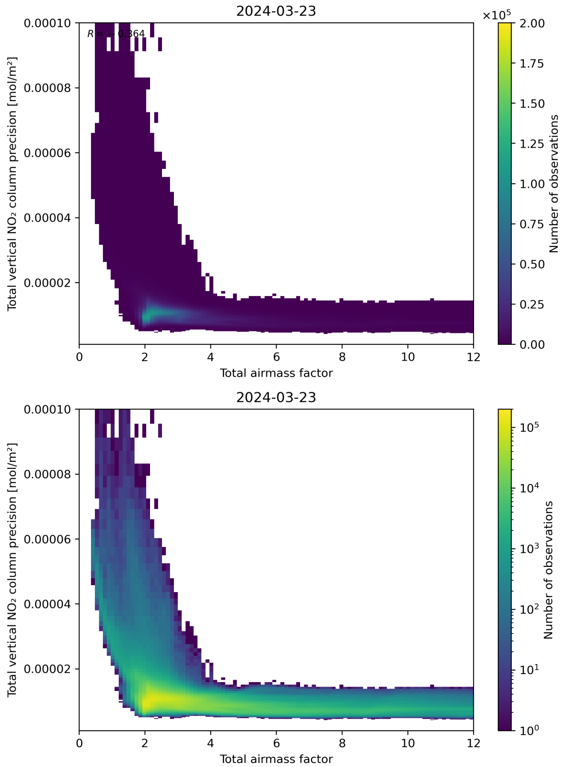
Figure 68: Scatter density plot of “Total airmass factor” against “Total vertical NO 2 column precision” for 2024-03-23 to 2024-03-24.
