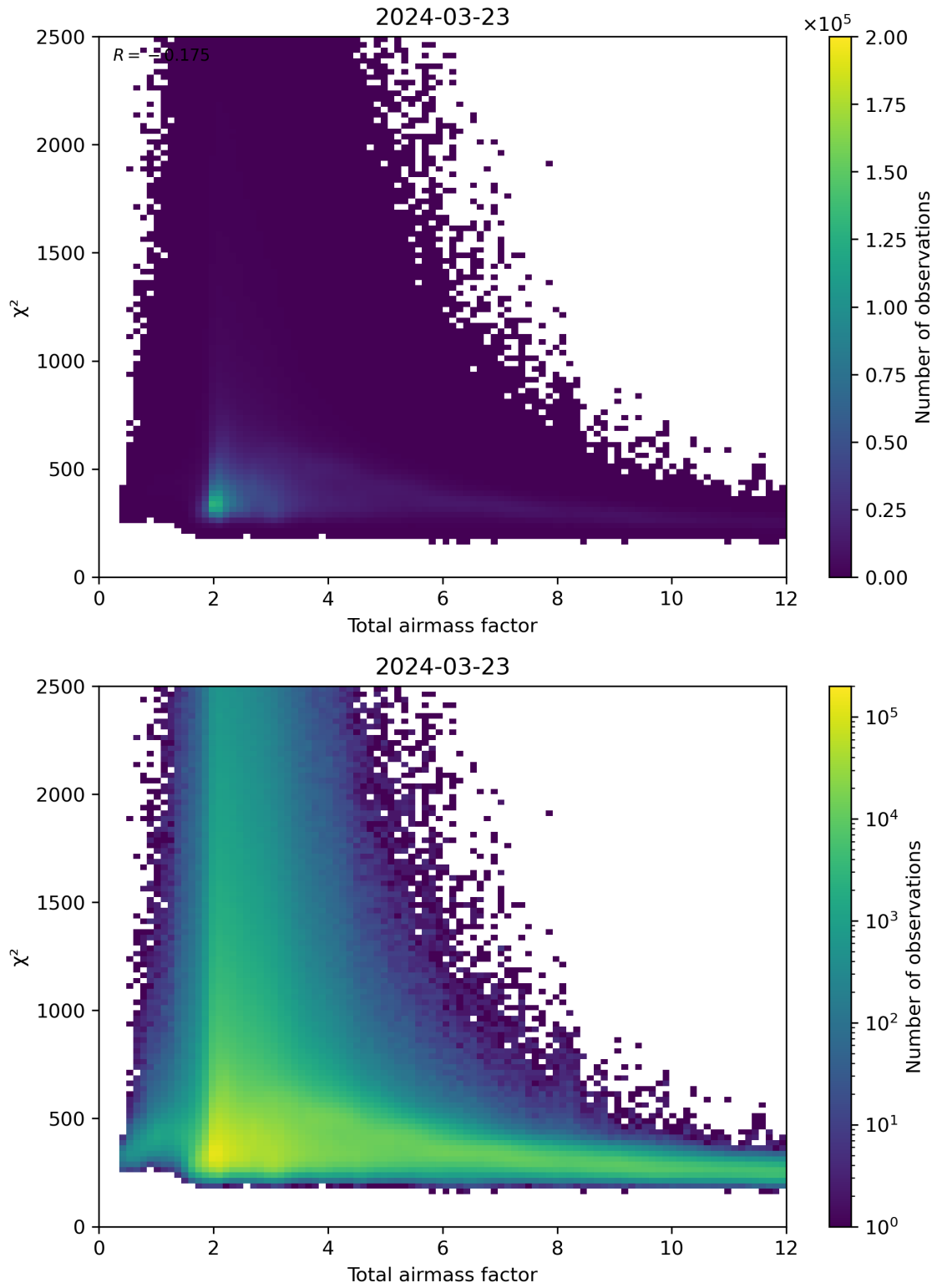
Figure 63: Scatter density plot of “Total airmass factor” against “ \chi^2 ” for 2024-03-23 to 2024-03-24.
