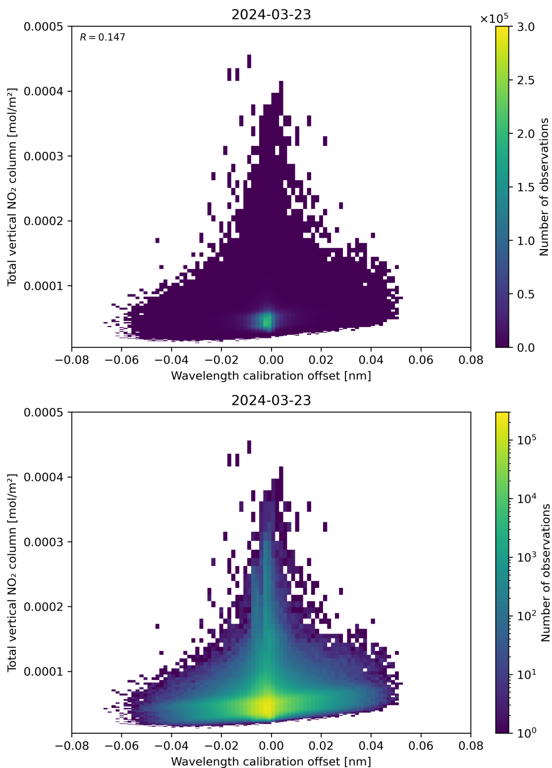
Figure 179: Scatter density plot of “Wavelength calibration offset” against “Total vertical NO 2 column” for 2024-03-23 to 2024-03-24.
