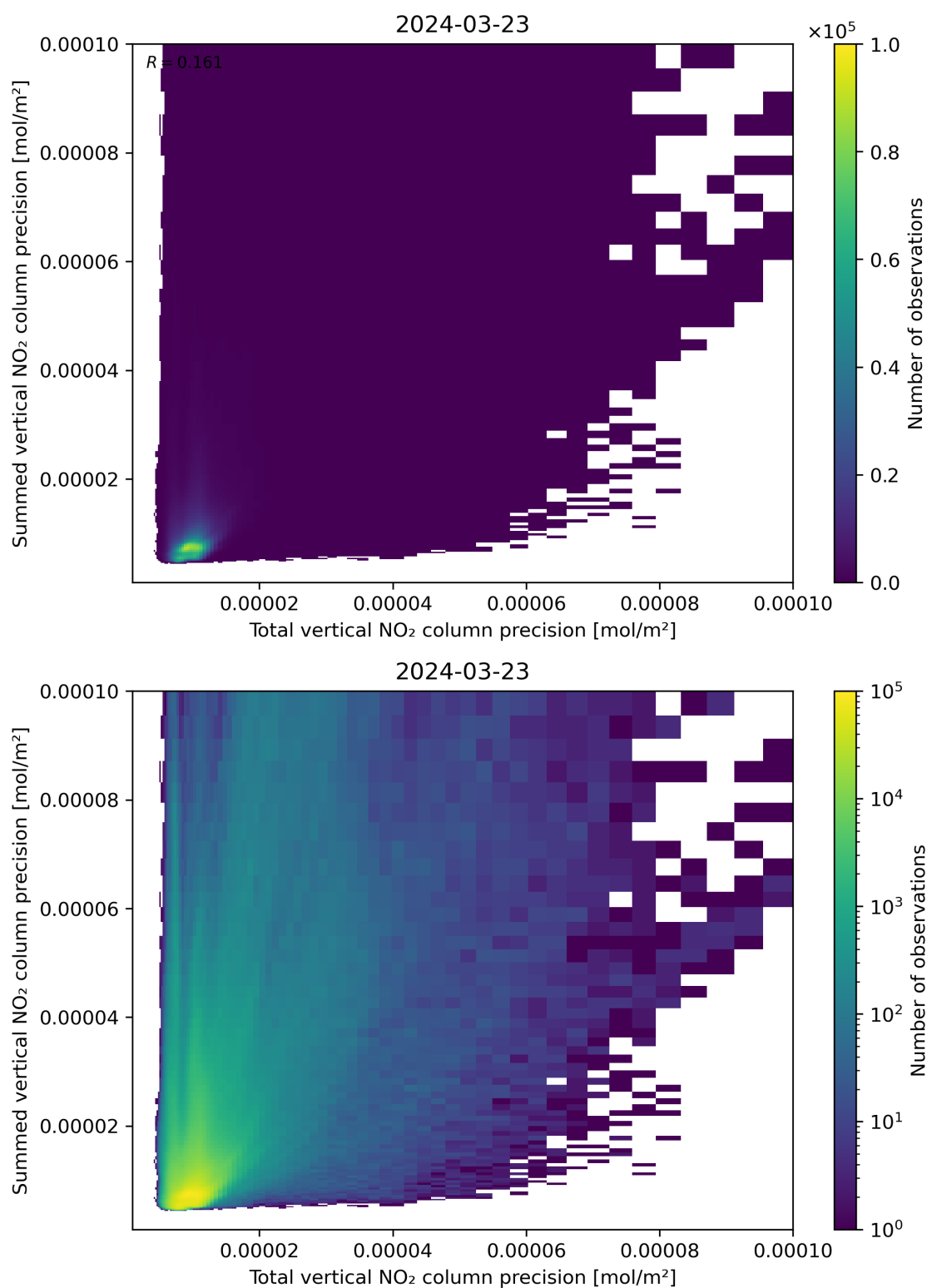
Figure 118: Scatter density plot of “Total vertical NO 2 column precision” against “Summed vertical NO 2 column precision” for 2024-03-23 to 2024-03-24.
