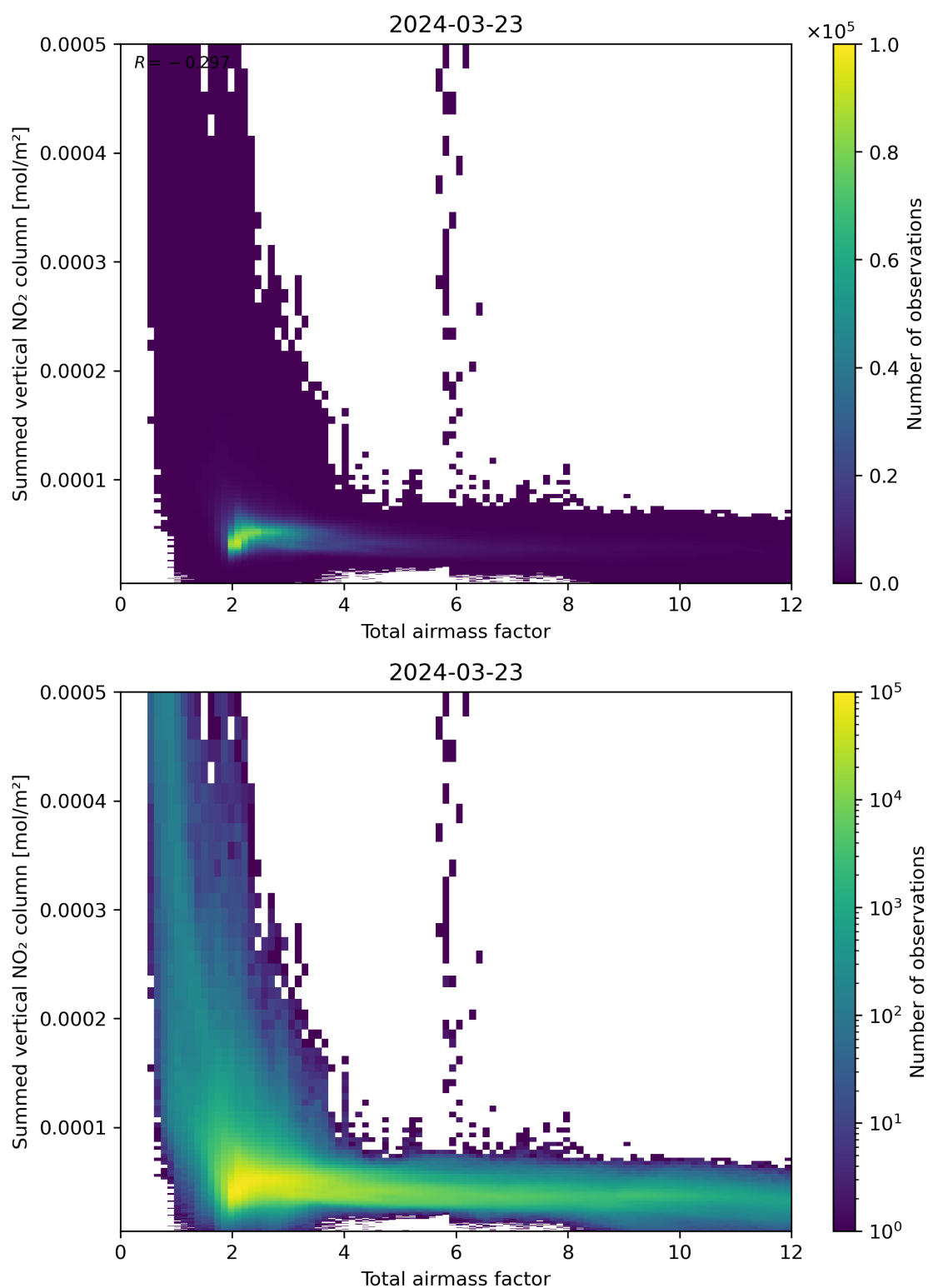
Figure 65: Scatter density plot of “Total airmass factor” against “Summed vertical NO 2 column” for 2024-03-23 to 2024-03-24.
