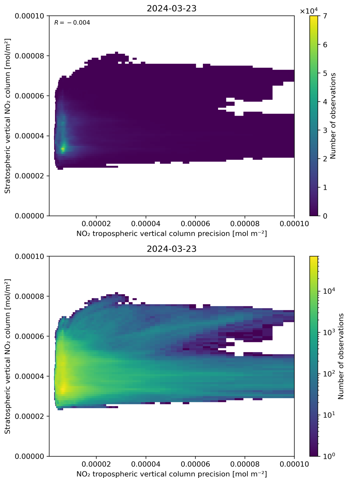
Figure 135: Scatter density plot of “NO 2 tropospheric vertical column precision” against “Stratospheric vertical NO 2 column” for 2024-03-23 to 2024-03-24.
