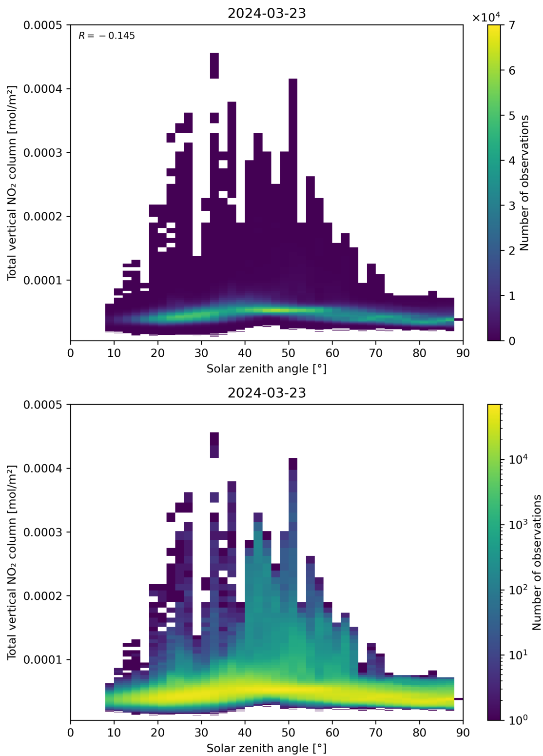
Figure 153: Scatter density plot of “Solar zenith angle” against “Total vertical NO 2 column” for 2024-03-23 to 2024-03-24.
