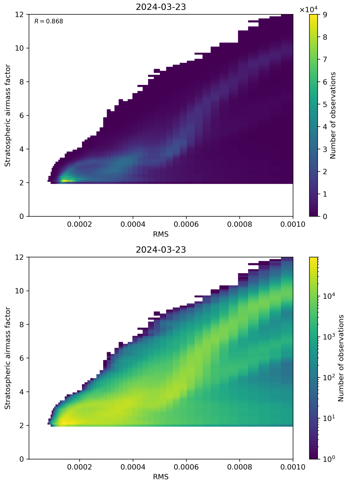
Figure 144: Scatter density plot of “RMS” against “Stratospheric airmass factor” for 2024-03-23 to 2024-03-24.
