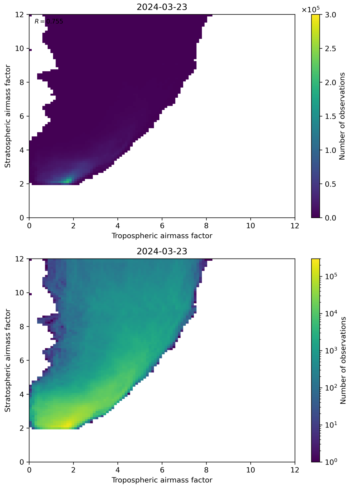
Figure 71: Scatter density plot of “Tropospheric airmass factor” against “Stratospheric airmass factor” for 2024-03-23 to 2024-03-24.
