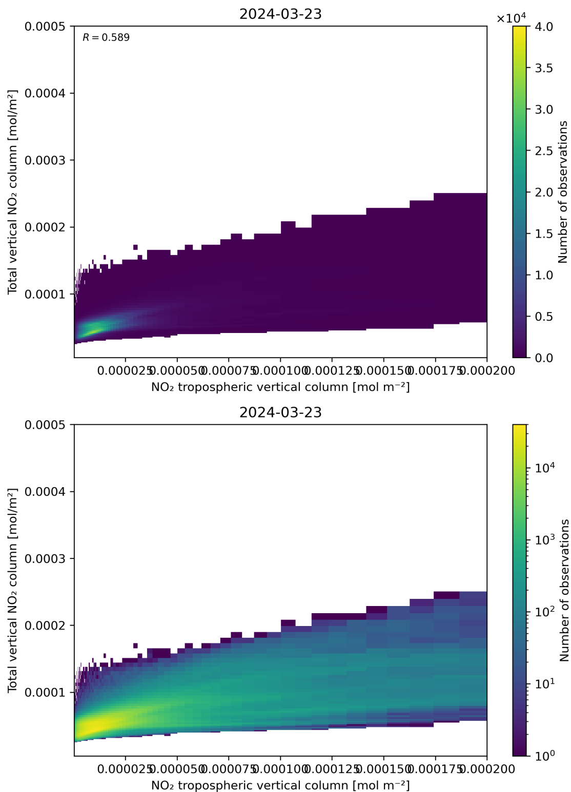
Figure 128: Scatter density plot of “NO 2 tropospheric vertical column” against “Total vertical NO 2 column” for 2024-03-23 to 2024-03-24.
