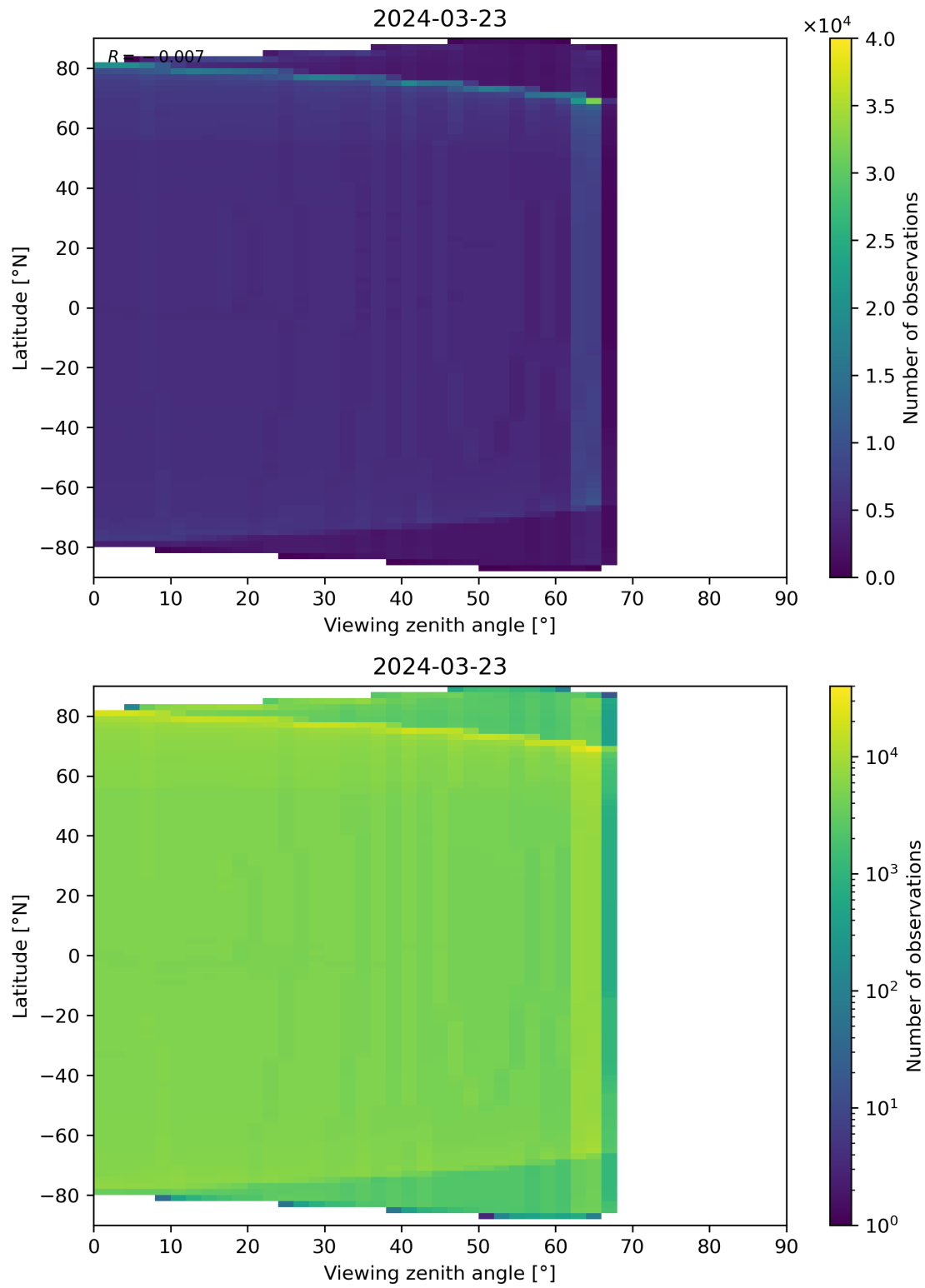
Figure 163: Scatter density plot of “Viewing zenith angle” against “Latitude” for 2024-03-23 to 2024-03-24.
