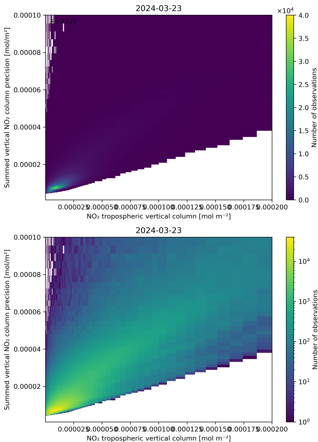
Figure 127: Scatter density plot of “NO 2 tropospheric vertical column” against “Summed vertical NO 2 column precision” for 2024-03-23 to 2024-03-24.
