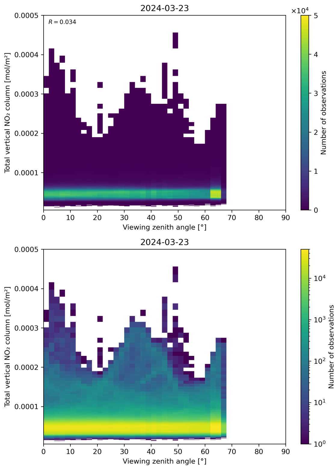
Figure 167: Scatter density plot of “Viewing zenith angle” against “Total vertical NO 2 column” for 2024-03-23 to 2024-03-24.
