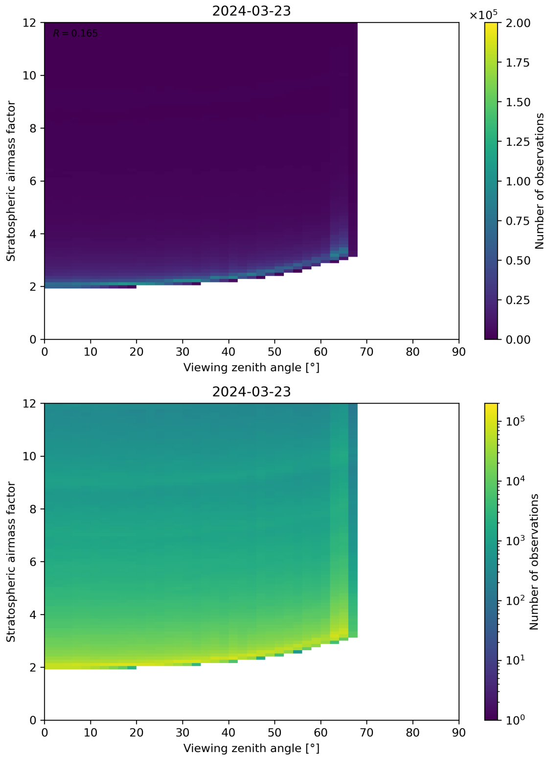
Figure 159: Scatter density plot of “Viewing zenith angle” against “Stratospheric airmass factor” for 2024-03-23 to 2024-03-24.
