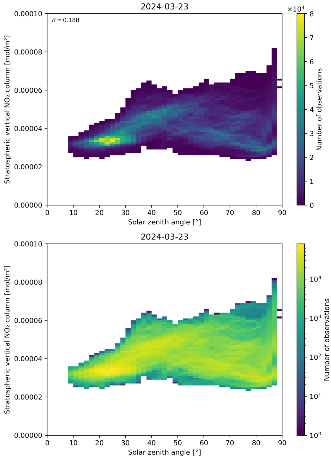
Figure 150: Scatter density plot of “Solar zenith angle” against “Stratospheric vertical NO 2 column” for 2024-03-23 to 2024-03-24.
