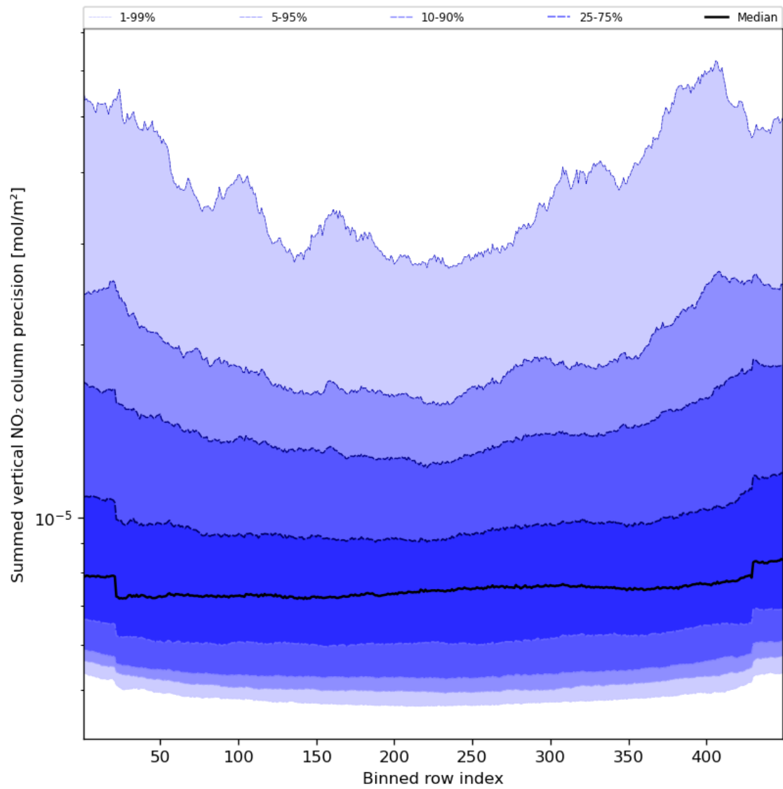
Figure 58: Along track statistics of “Summed vertical NO 2 column precision” for 2024-03-23 to 2024-03-24
