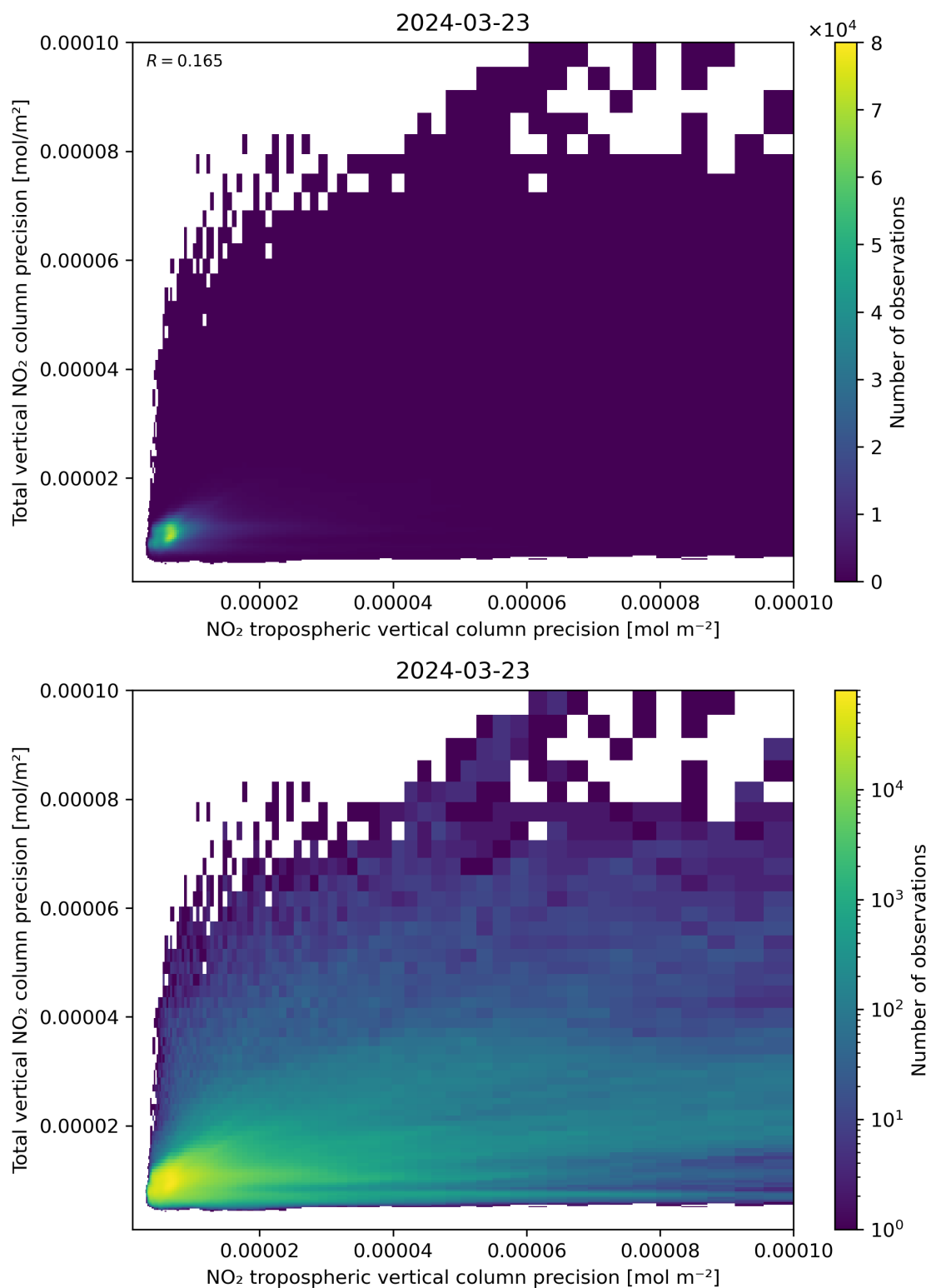
Figure 139: Scatter density plot of “NO 2 tropospheric vertical column precision” against “Total vertical NO 2 column precision” for 2024-03-23 to 2024-03-24.
