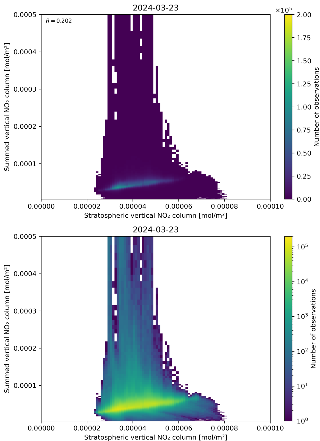
Figure 98: Scatter density plot of “Stratospheric vertical NO 2 column” against “Summed vertical NO 2 column” for 2024-03-23 to 2024-03-24.
