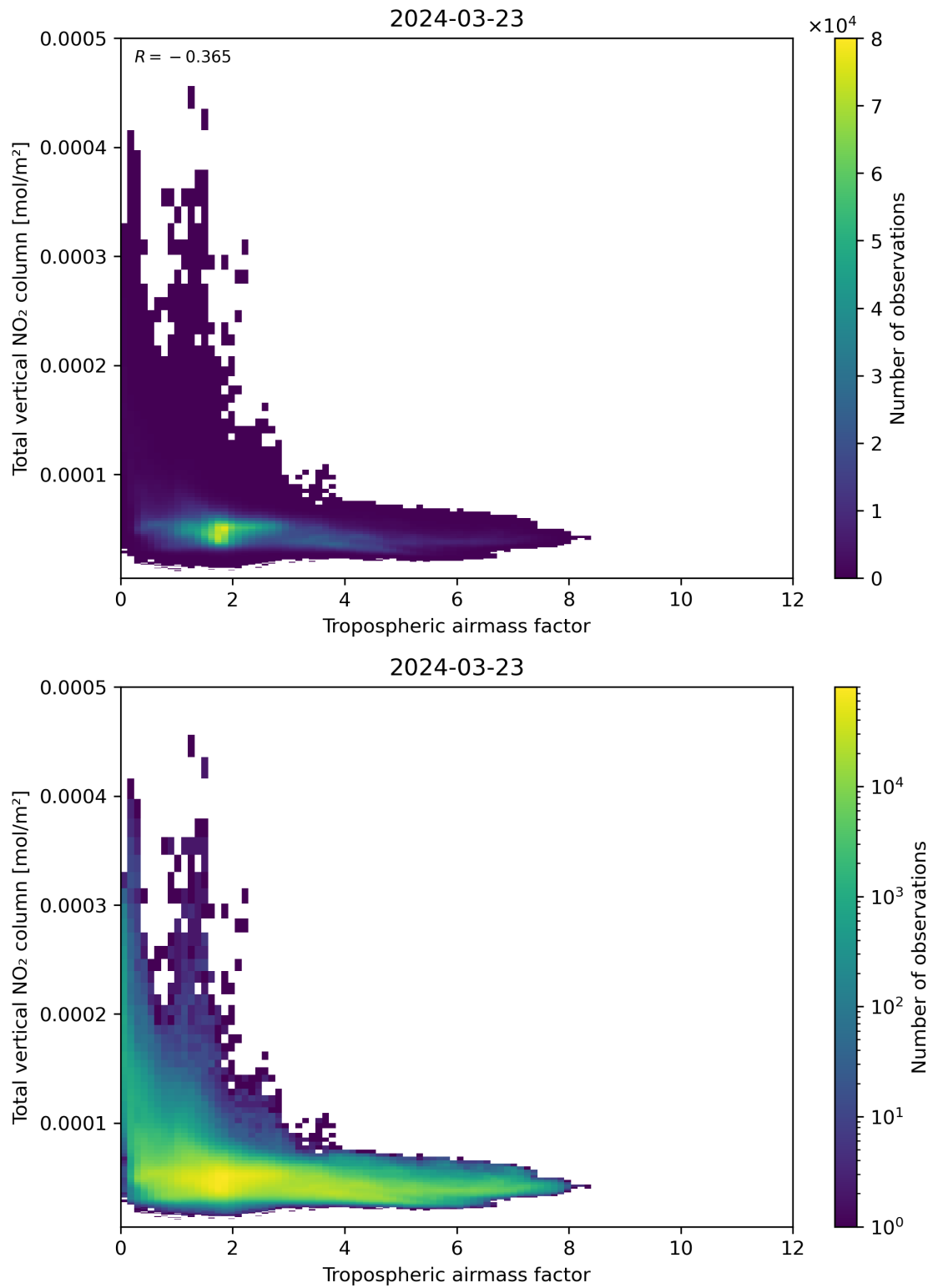
Figure 77: Scatter density plot of “Tropospheric airmass factor” against “Total vertical NO 2 column” for 2024-03-23 to 2024-03-24.
