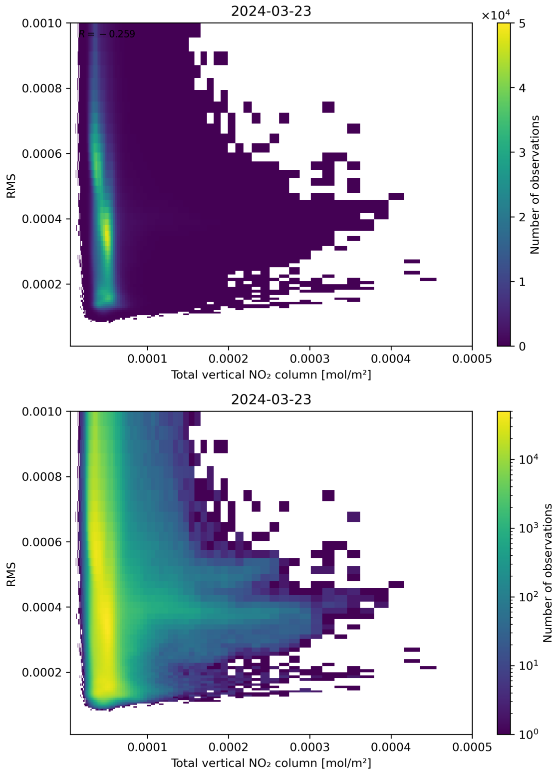
Figure 120: Scatter density plot of “Total vertical NO 2 column” against “RMS” for 2024-03-23 to 2024-03-24.
