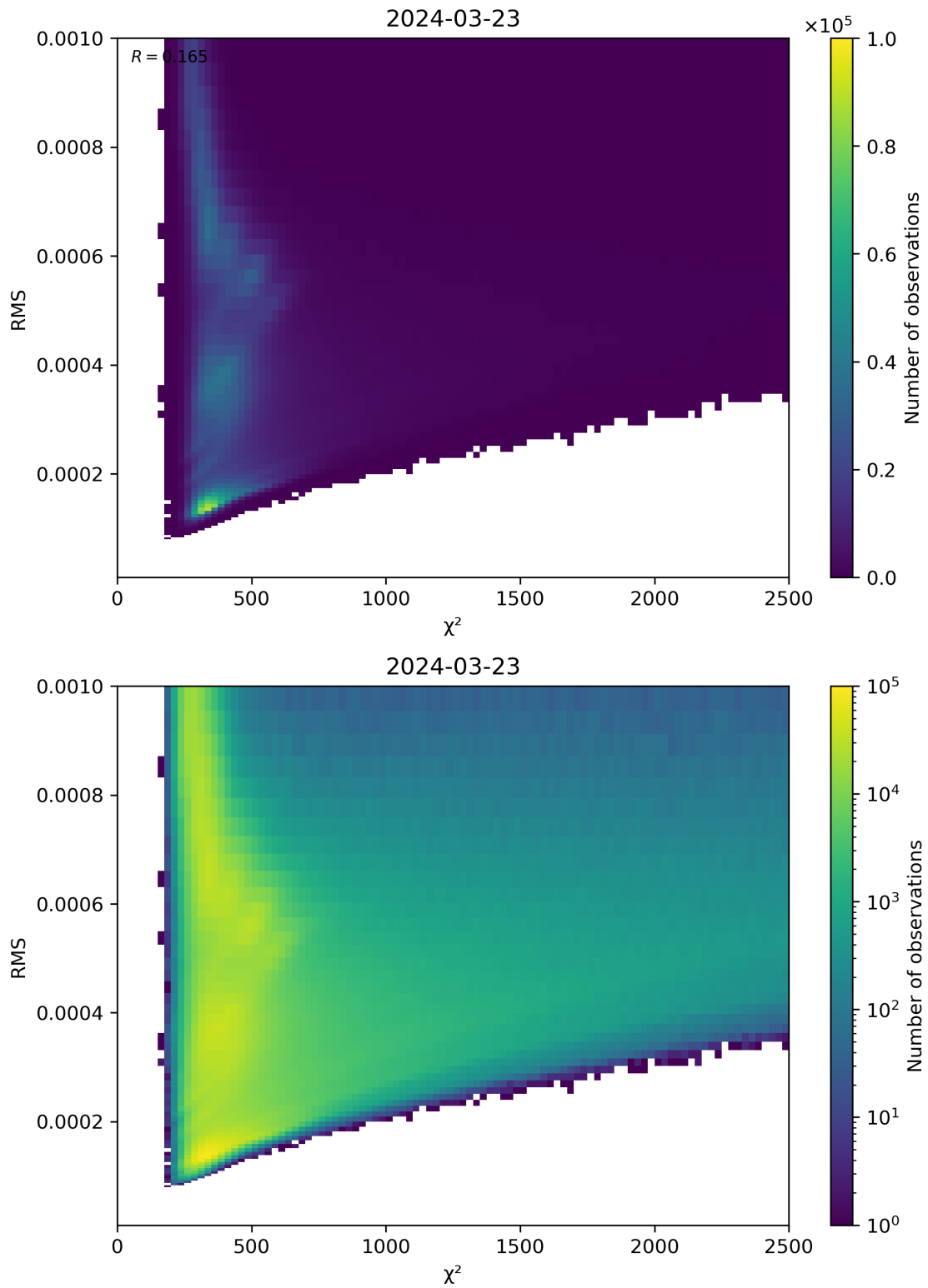
Figure 82: Scatter density plot of “ \chi^2 ” against “RMS” for 2024-03-23 to 2024-03-24.
