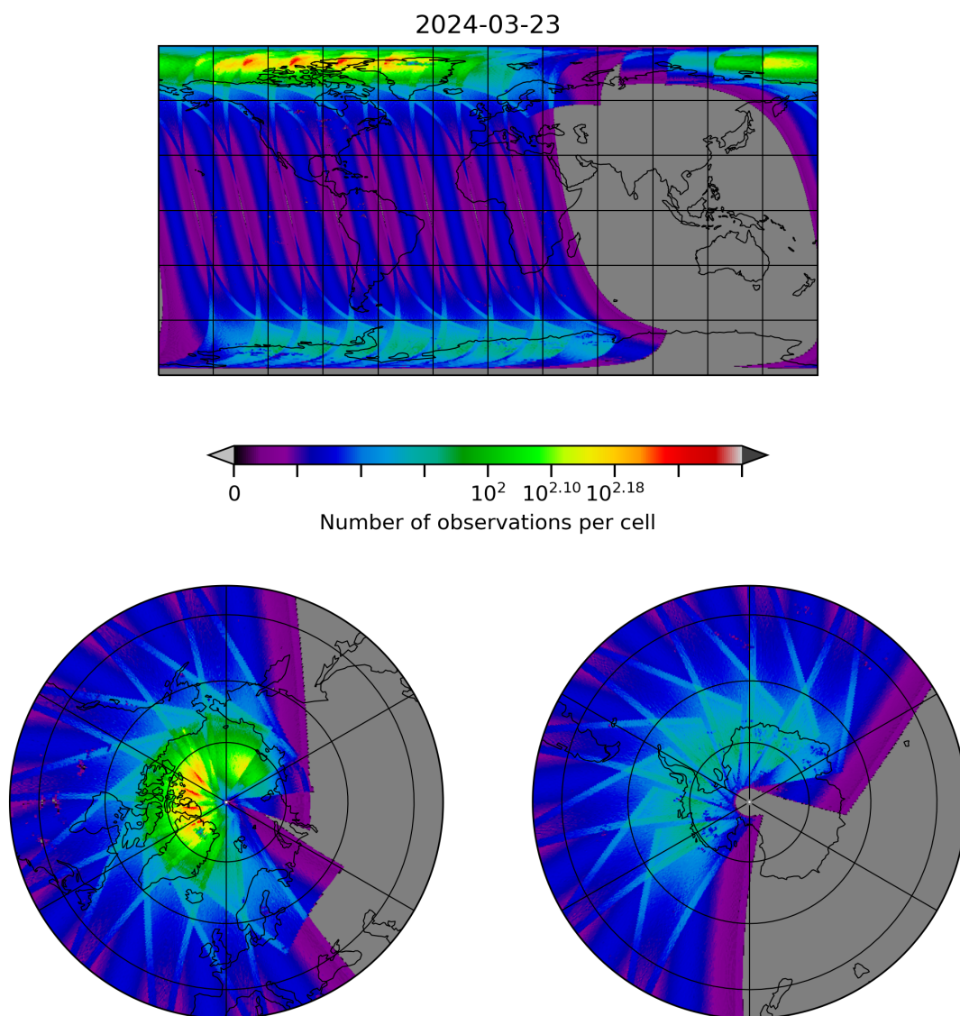
Figure 10: Map of the number of observations for 2024-03-23 to 2024-03-24
