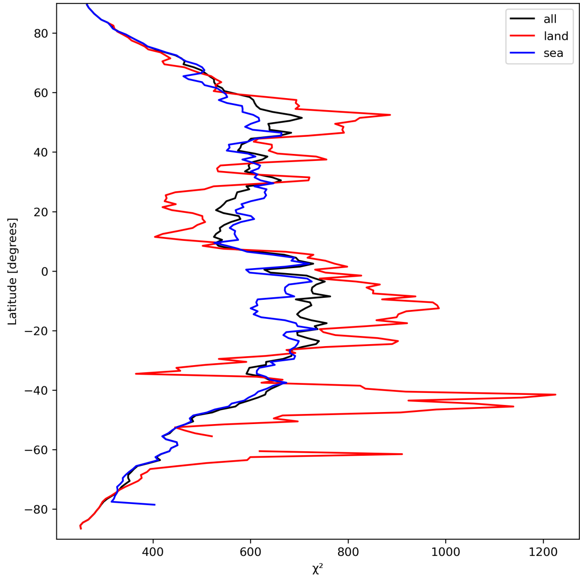
Figure 25: Zonal average of “ \chi^2 ” for 2024-03-23 to 2024-03-24.
