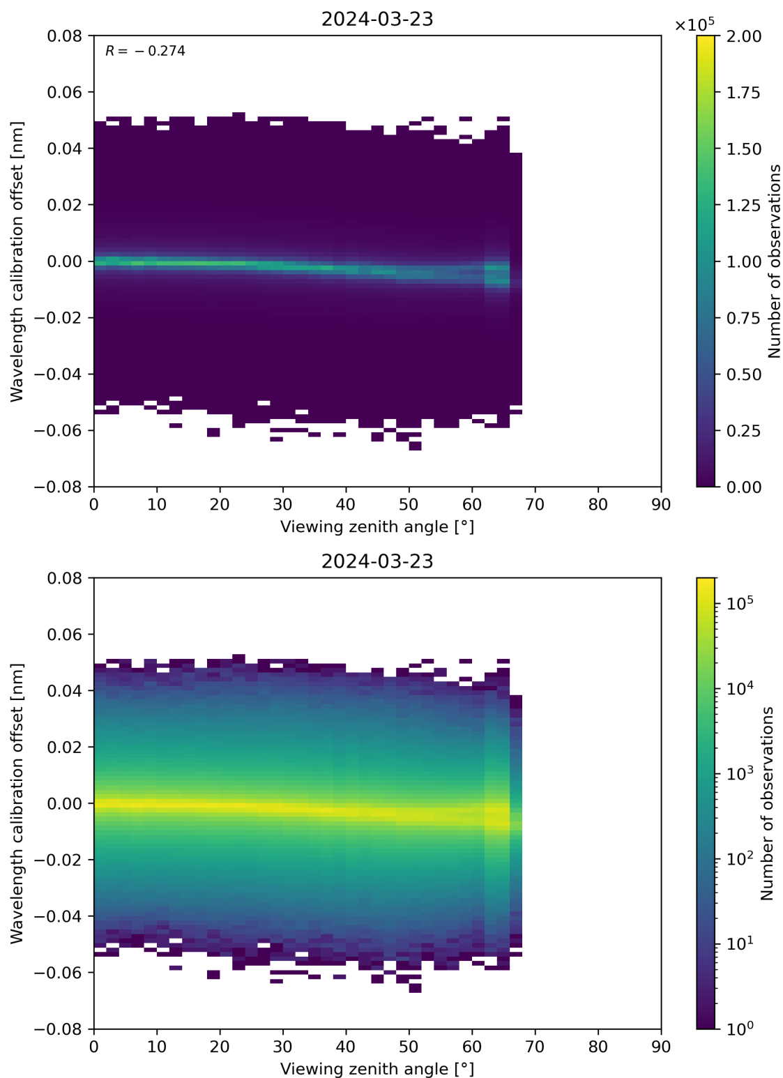
Figure 173: Scatter density plot of “Viewing zenith angle” against “Wavelength calibration offset” for 2024-03-23 to 2024-03-24.
