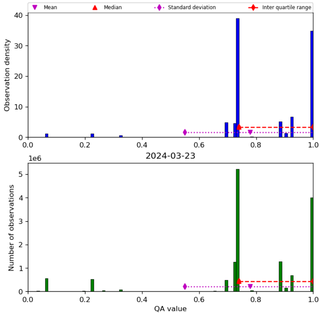
Figure 28: Histogram of “QA value” for 2024-03-23 to 2024-03-24
