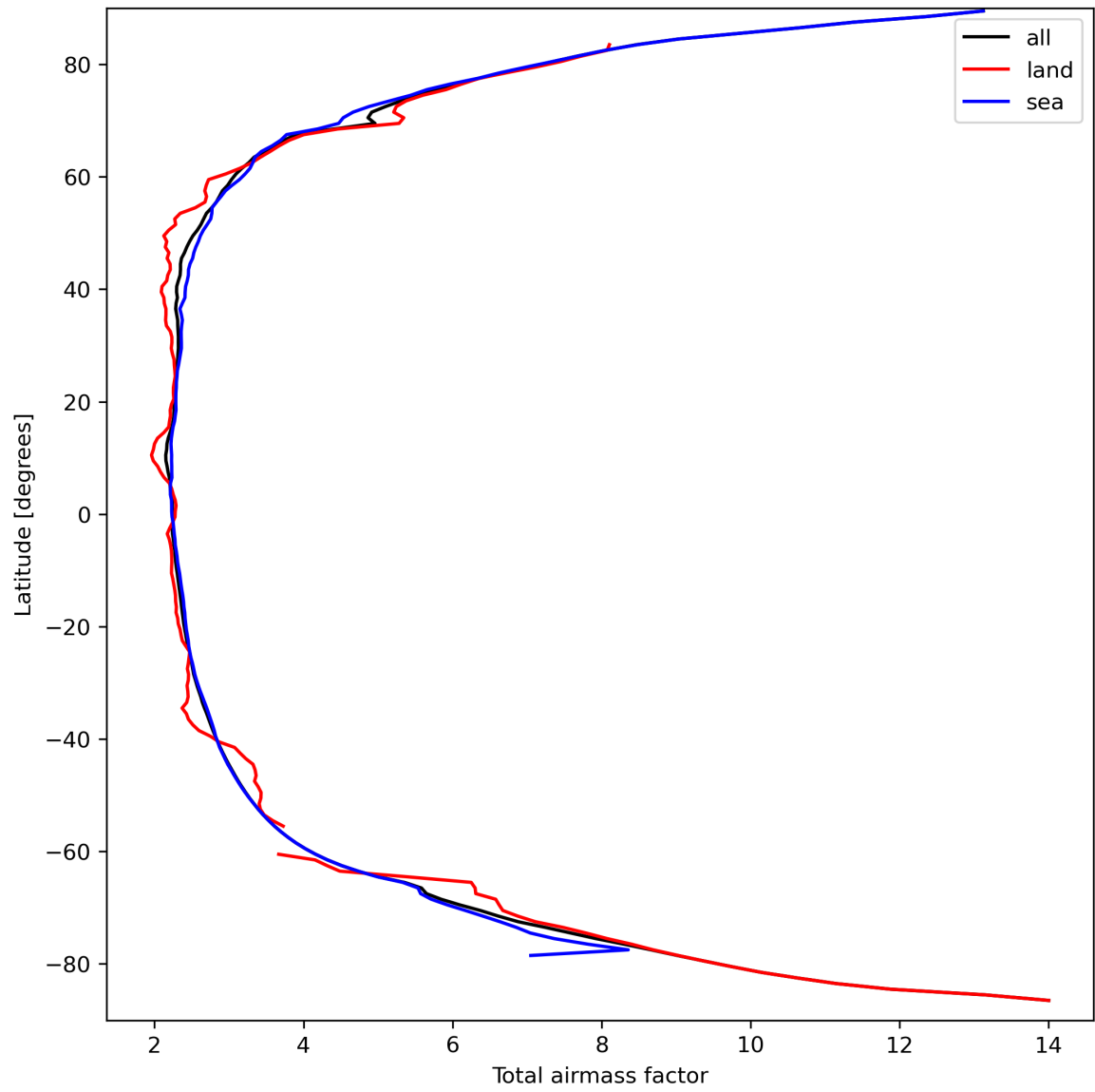
Figure 15: Zonal average of “Total airmass factor” for 2024-03-23 to 2024-03-24.
