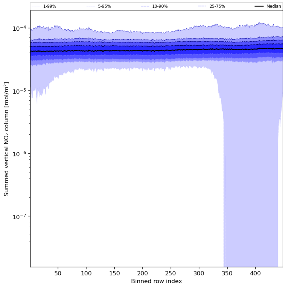
Figure 57: Along track statistics of “Summed vertical NO 2 column” for 2024-03-23 to 2024-03-24
