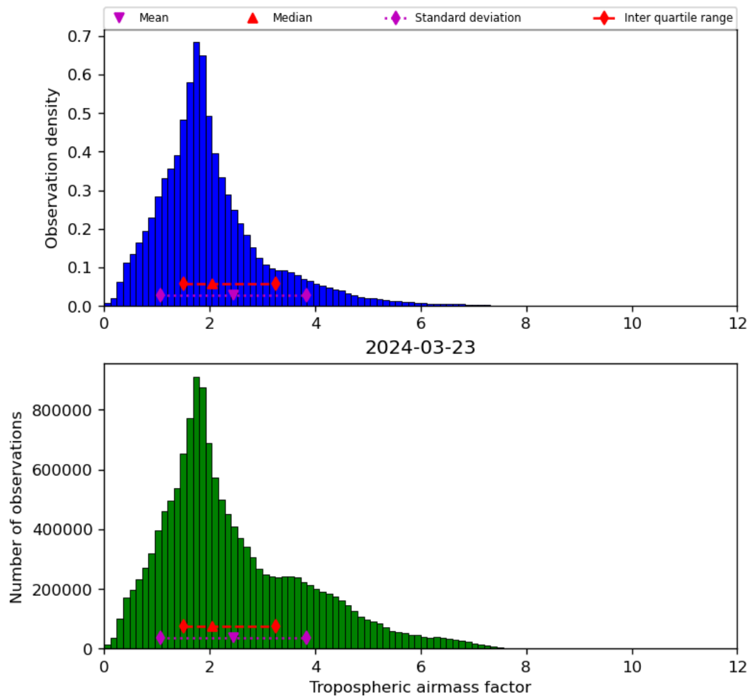
Figure 31: Histogram of “Tropospheric airmass factor” for 2024-03-23 to 2024-03-24
