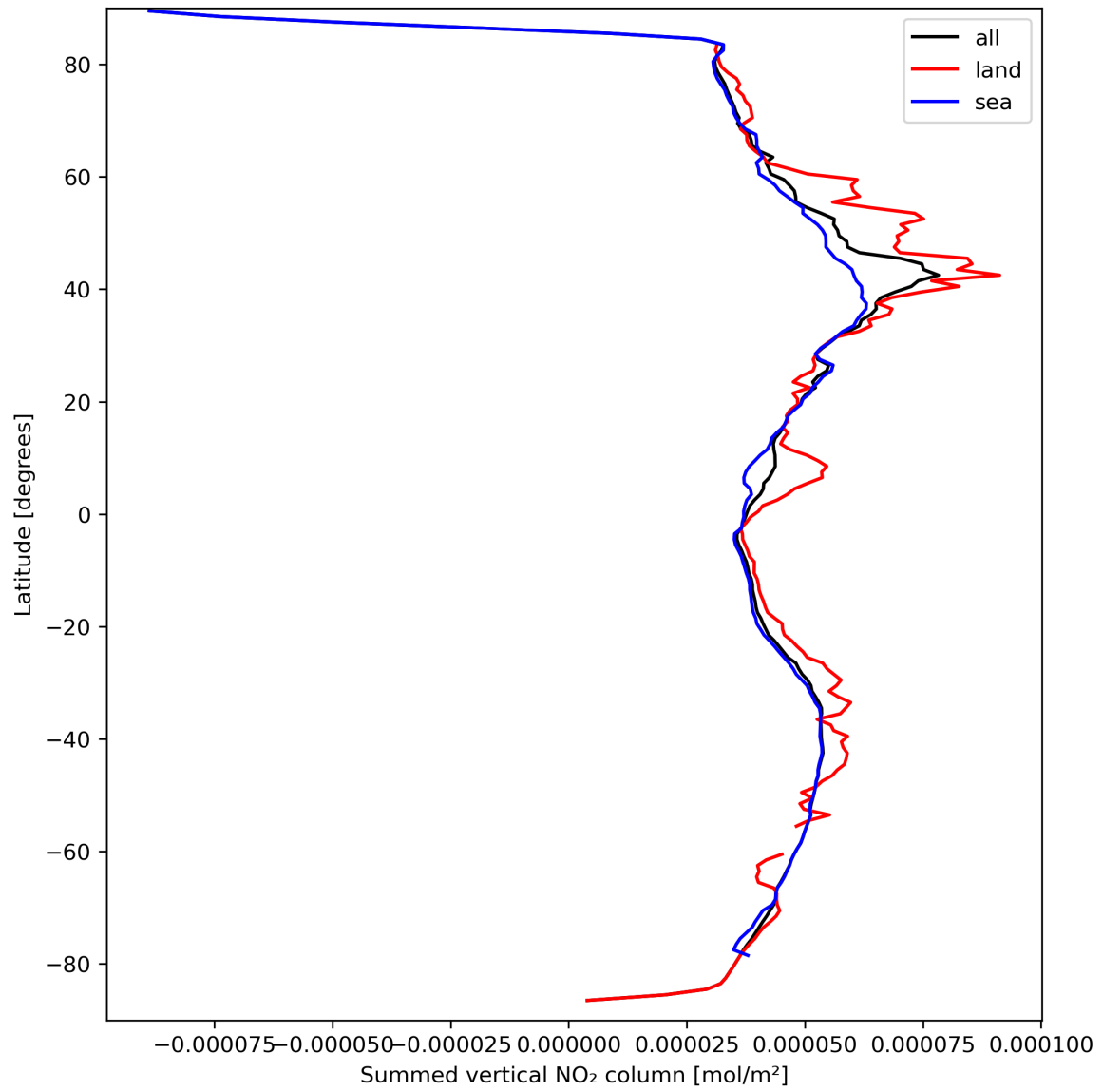
Figure 23: Zonal average of “Summed vertical NO 2 column” for 2024-03-23 to 2024-03-24.
