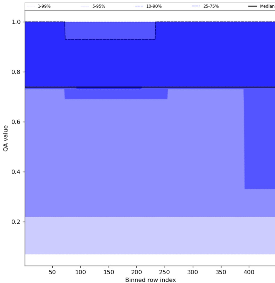
Figure 45: Along track statistics of "QA value" for 2024-03-23 to 2024-03-24
