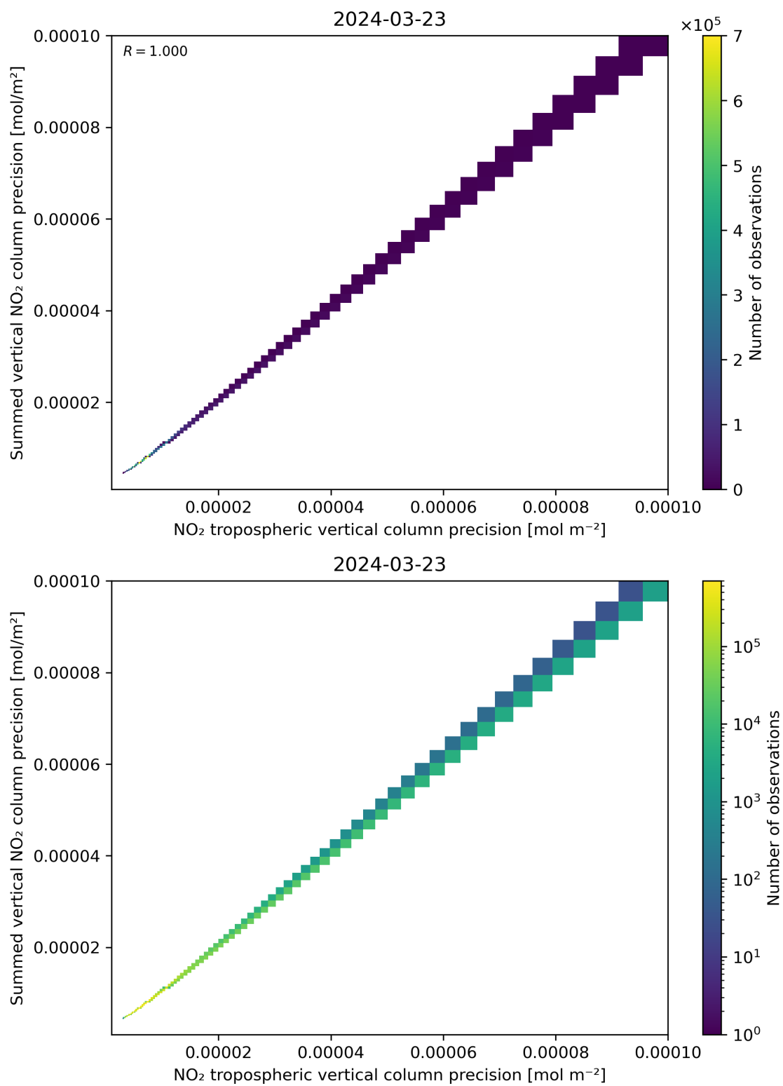
Figure 137: Scatter density plot of “NO 2 tropospheric vertical column precision” against “Summed vertical NO 2 column precision” for 2024-03-23 to 2024-03-24.
