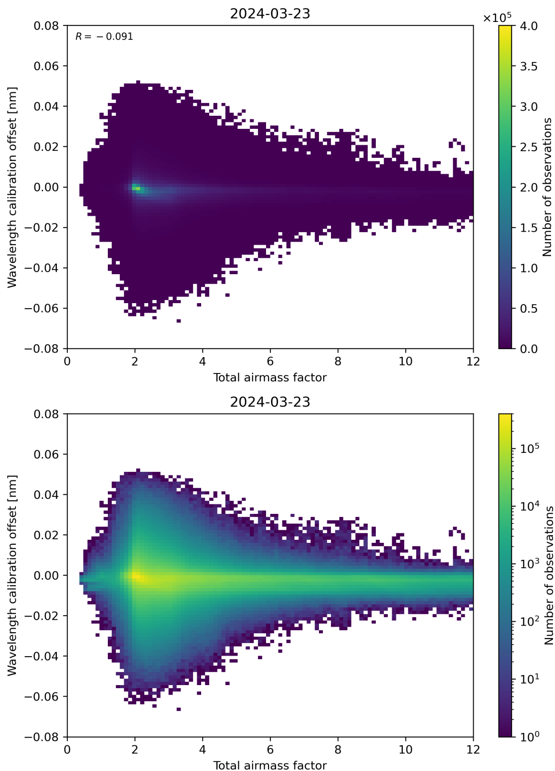
Figure 70: Scatter density plot of “Total airmass factor” against “Wavelength calibration offset” for 2024-03-23 to 2024-03-24.
