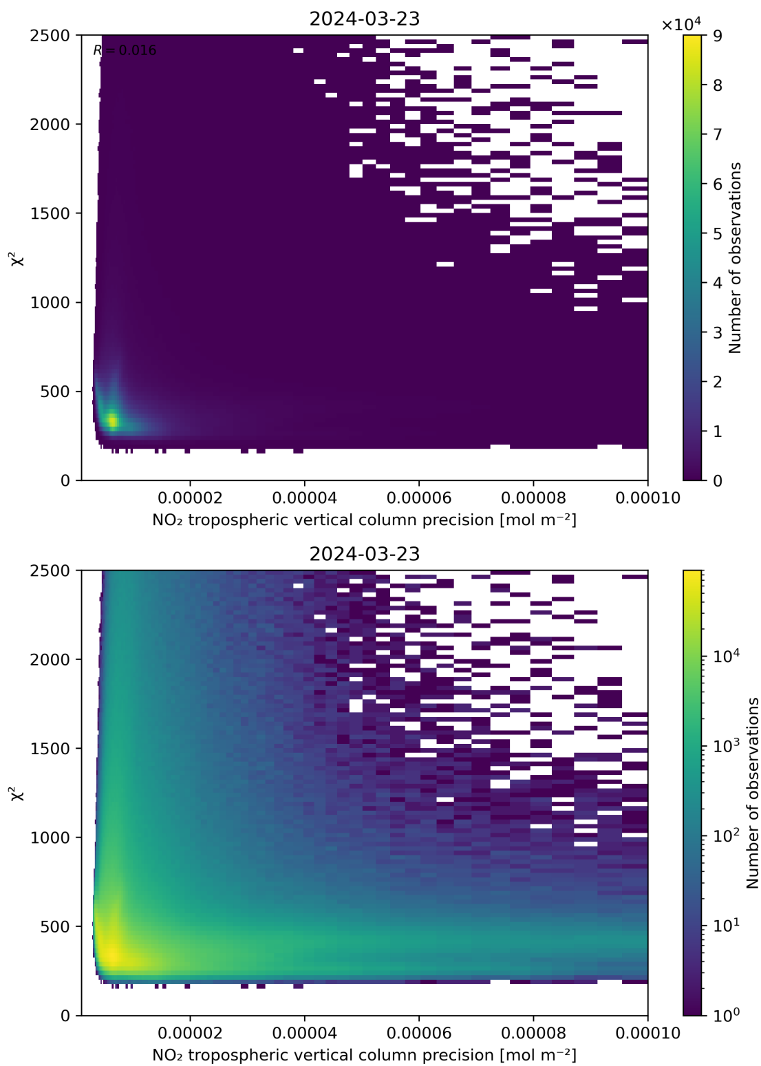
Figure 134: Scatter density plot of “NO 2 tropospheric vertical column precision” against “ \chi^2 ” for 2024-03-23 to 2024-03-24.
