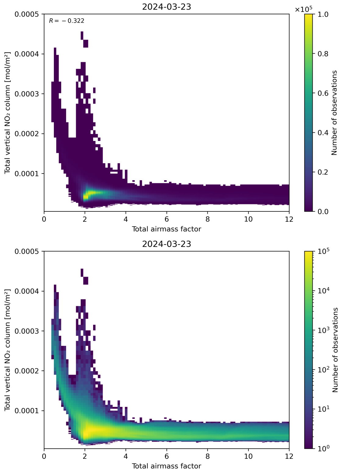
Figure 67: Scatter density plot of “Total airmass factor” against “Total vertical NO 2 column” for 2024-03-23 to 2024-03-24.
