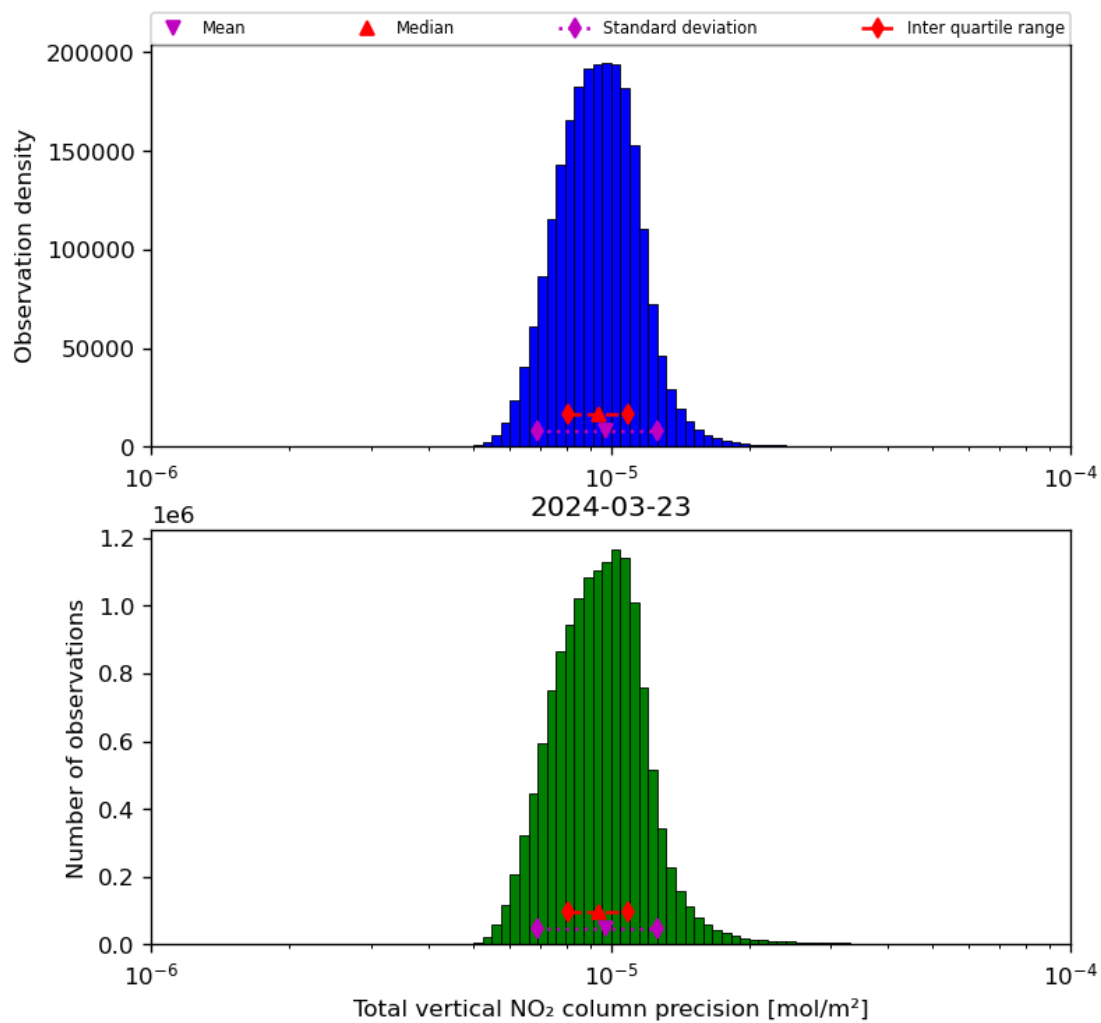
Figure 39: Histogram of “Total vertical NO 2 column precision” for 2024-03-23 to 2024-03-24
