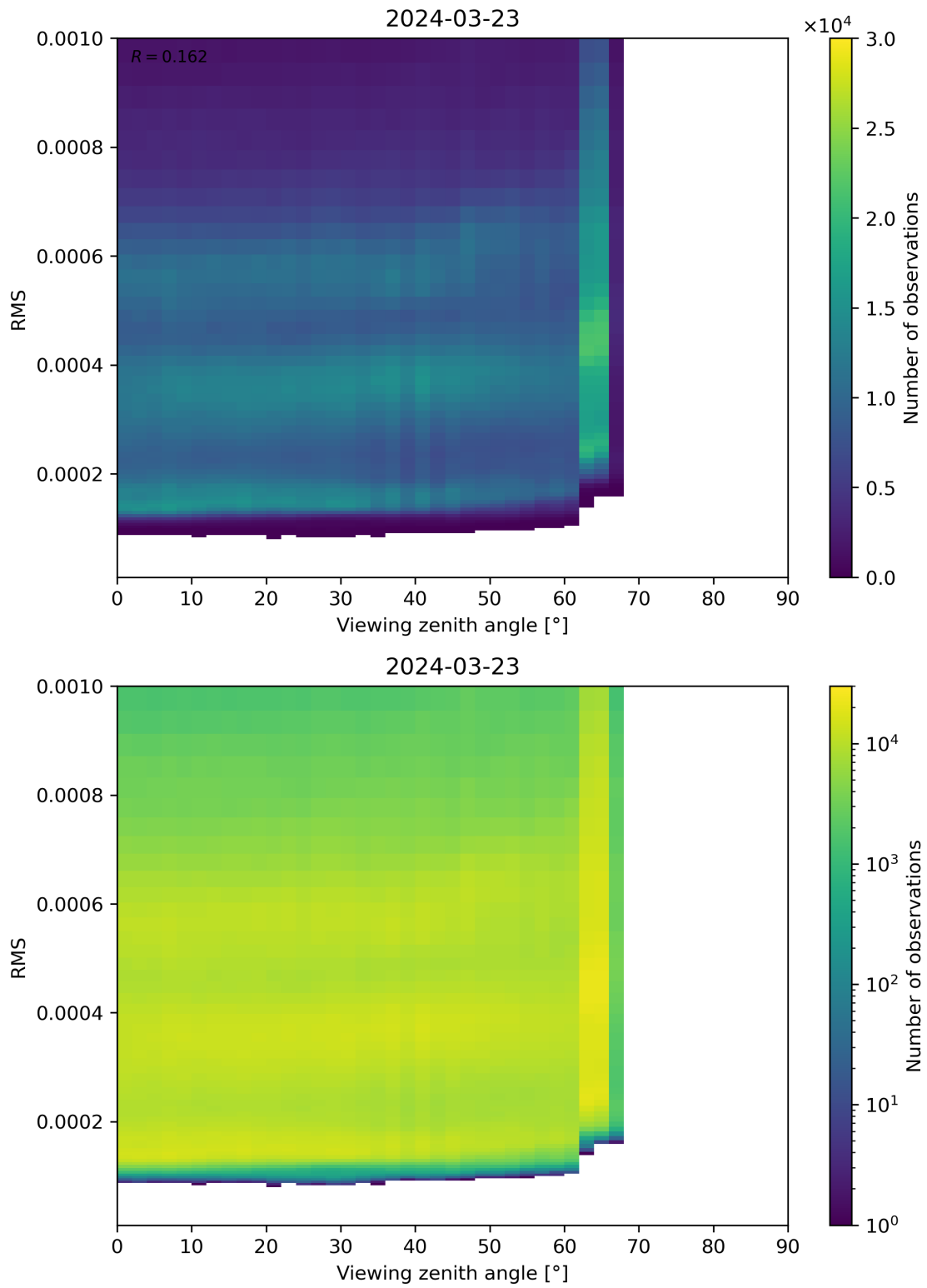
Figure 171: Scatter density plot of “Viewing zenith angle” against “RMS” for 2024-03-23 to 2024-03-24.
