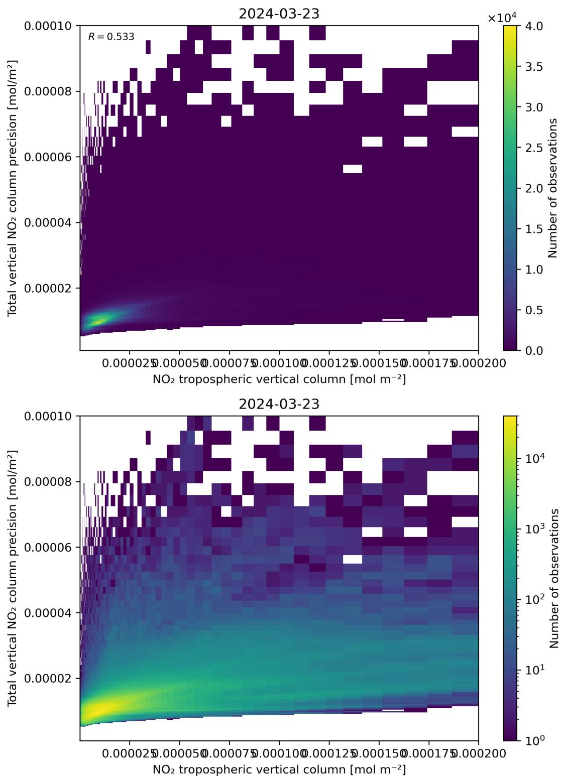
Figure 129: Scatter density plot of “NO 2 tropospheric vertical column” against “Total vertical NO 2 column precision” for 2024-03-23 to 2024-03-24.
