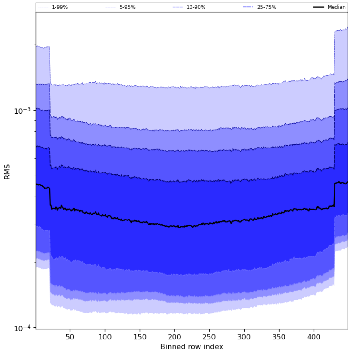
Figure 60: Along track statistics of “RMS” for 2024-03-23 to 2024-03-24
