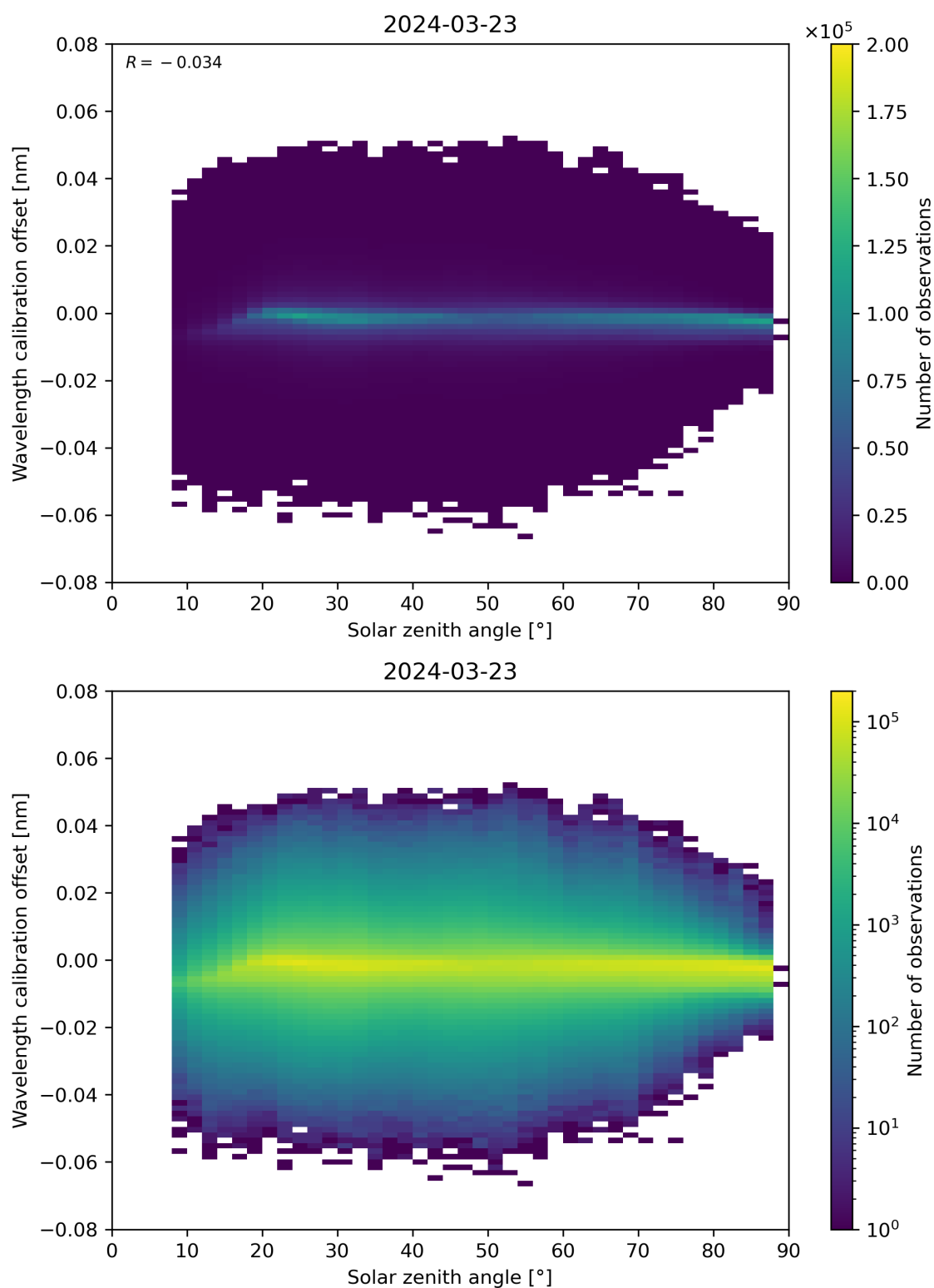
Figure 158: Scatter density plot of “Solar zenith angle” against “Wavelength calibration offset” for 2024-03-23 to 2024-03-24.
