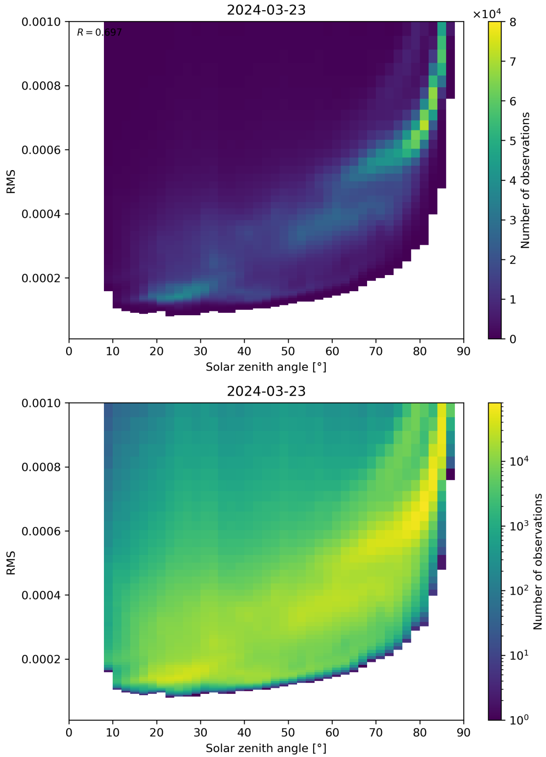
Figure 157: Scatter density plot of “Solar zenith angle” against “RMS” for 2024-03-23 to 2024-03-24.
