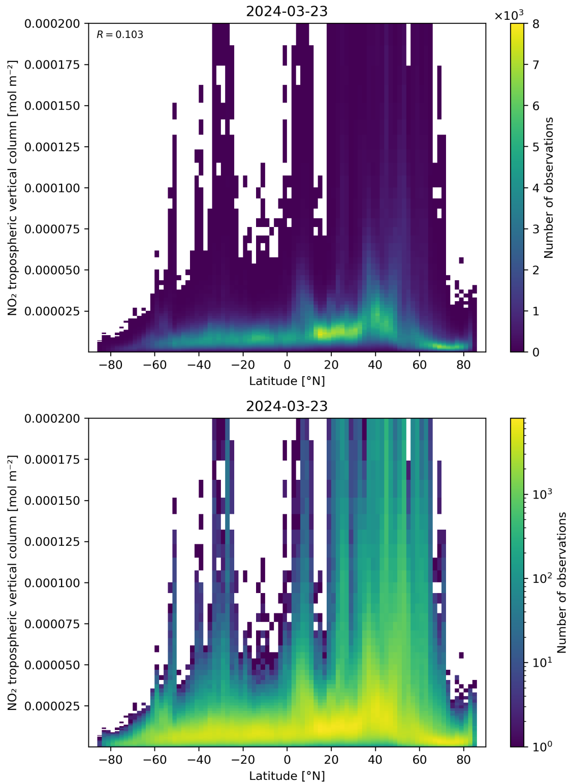
Figure 92: Scatter density plot of “Latitude” against “NO 2 tropospheric vertical column” for 2024-03-23 to 2024-03-24.
