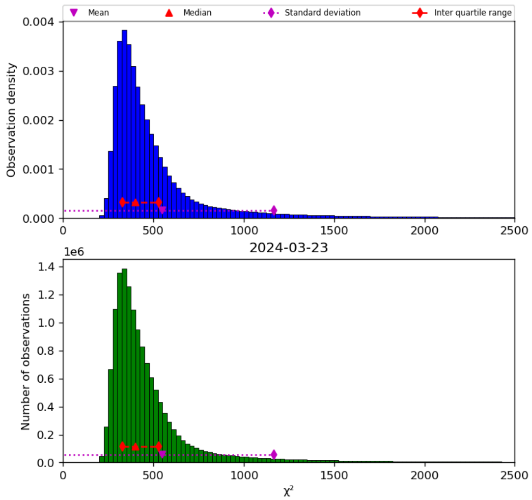
Figure 42: Histogram of “ \chi^2 ” for 2024-03-23 to 2024-03-24
