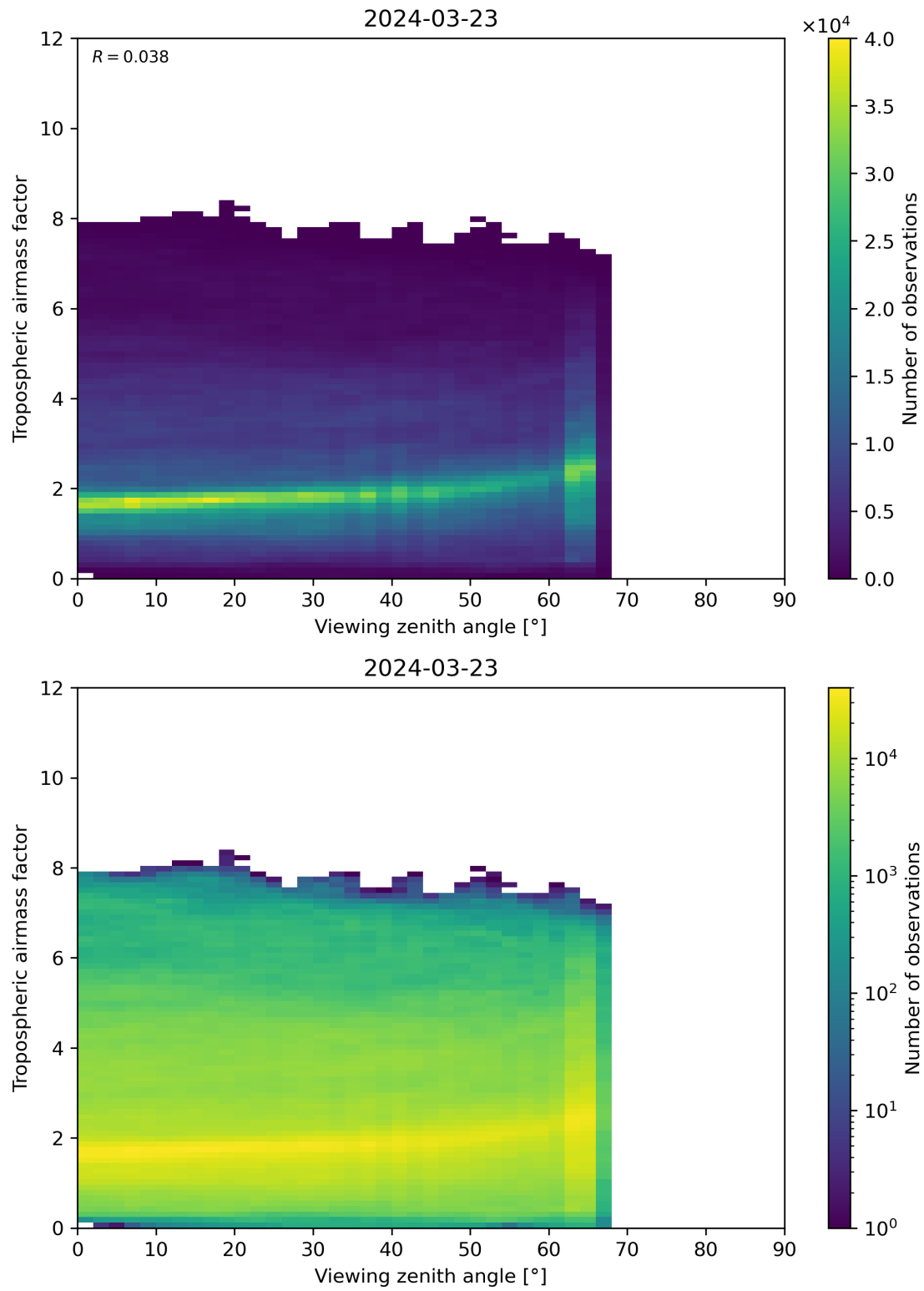
Figure 161: Scatter density plot of “Viewing zenith angle” against “Tropospheric airmass factor” for 2024-03-23 to 2024-03-24.
