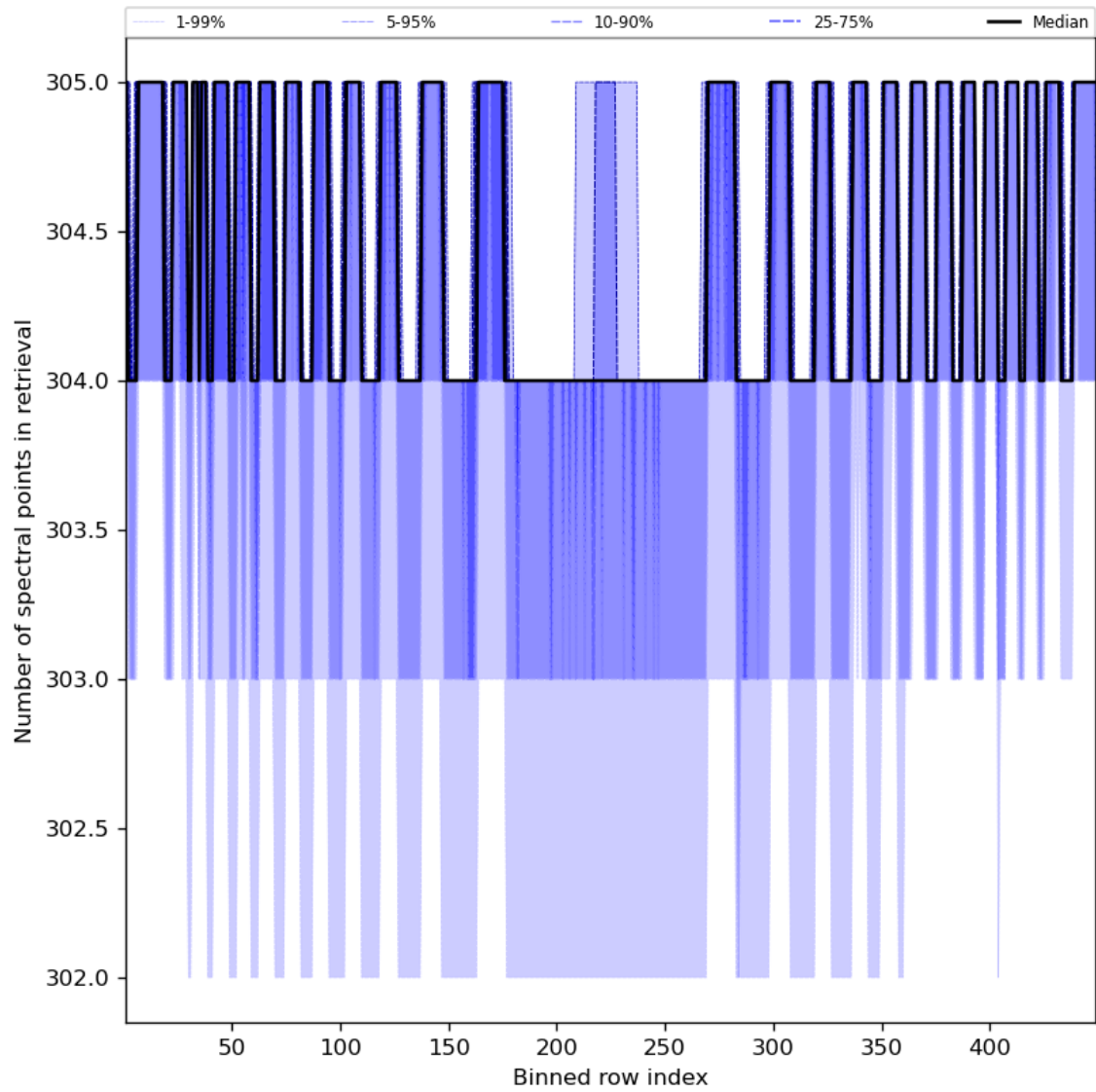
Figure 50: Along track statistics of “Number of spectral points in retrieval” for 2024-03-23 to 2024-03-24
