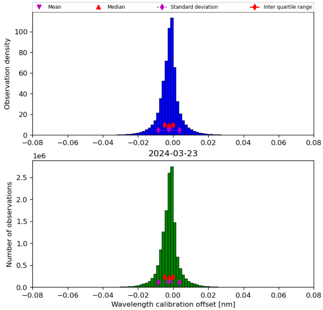
Figure 35: Histogram of “Wavelength calibration offset” for 2024-03-23 to 2024-03-24
