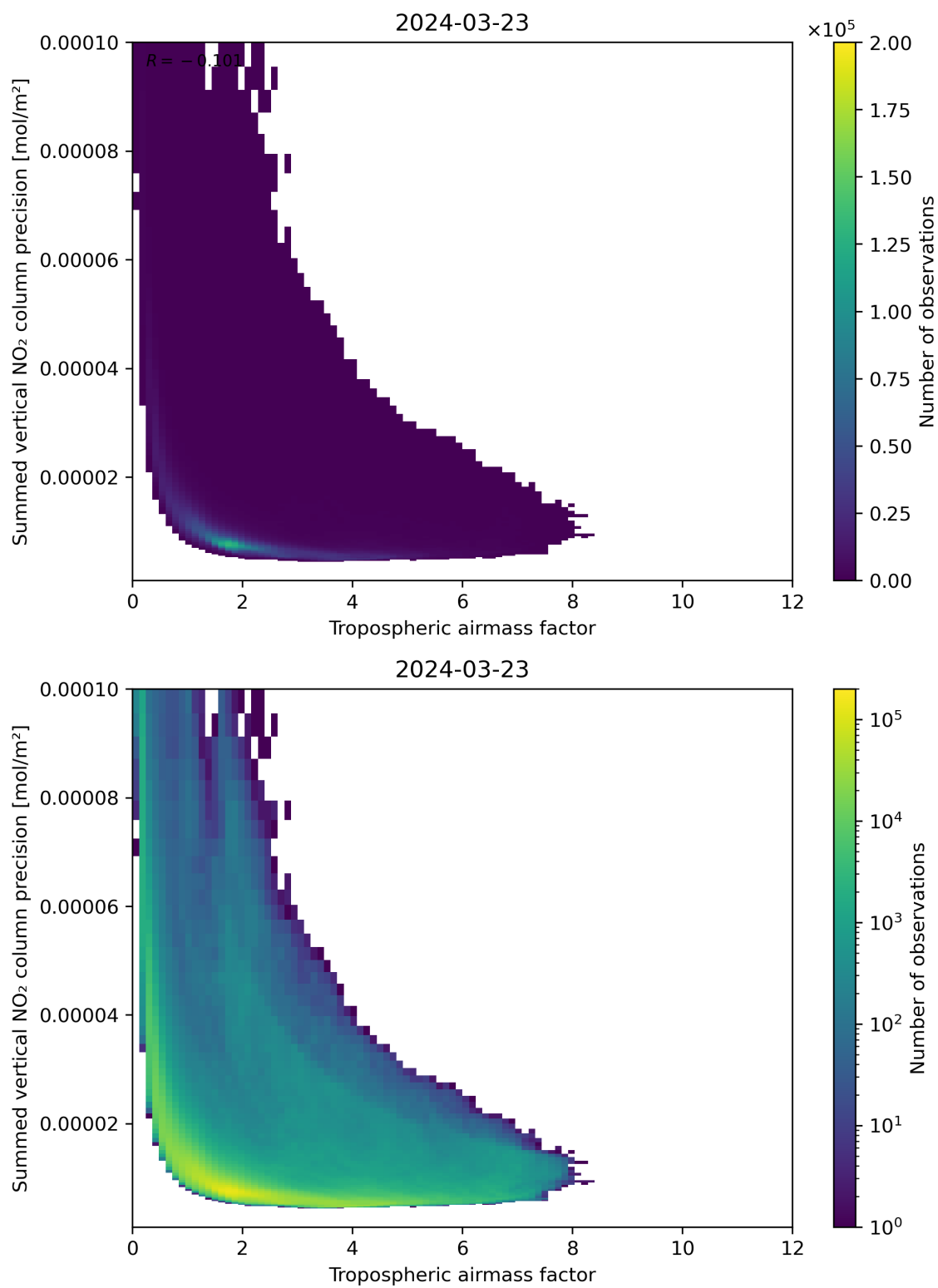
Figure 76: Scatter density plot of “Tropospheric air mass factor” against “Summed vertical NO 2 column precision” for 2024-03-23 to 2024-03-24.
