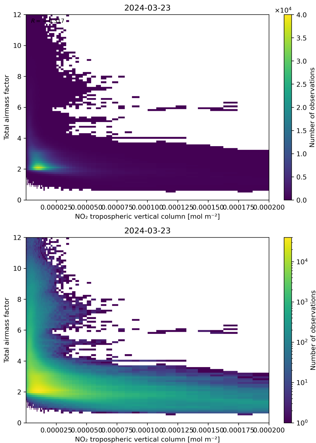
Figure 122: Scatter density plot of “NO 2 tropospheric vertical column” against “Total air mass factor” for 2024-03-23 to 2024-03-24.
