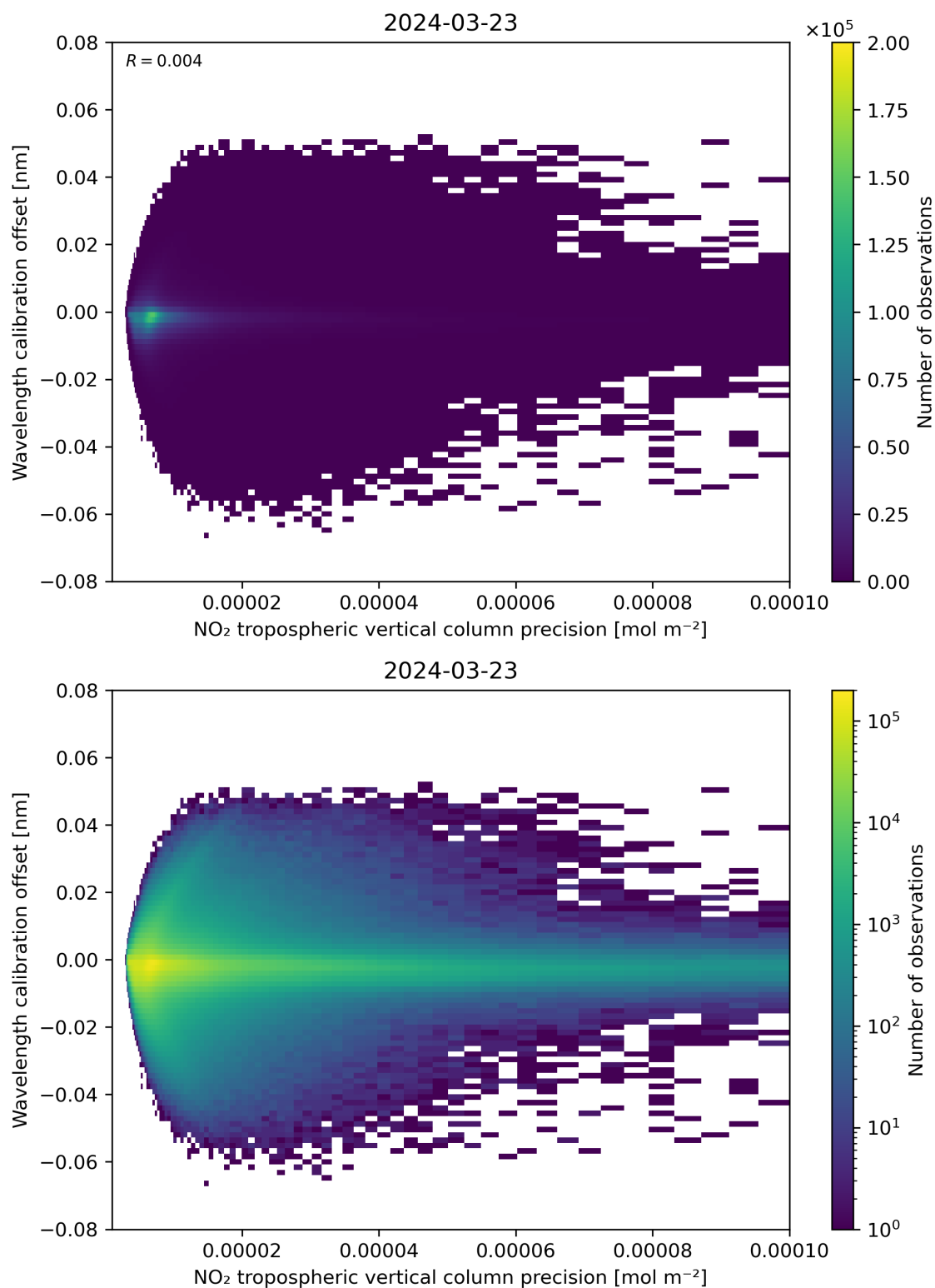
Figure 141: Scatter density plot of “NO 2 tropospheric vertical column precision” against “Wavelength calibration offset” for 2024-03-23 to 2024-03-24.
