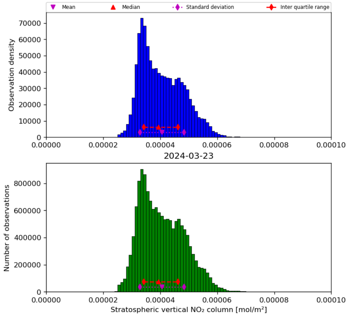
Figure 36: Histogram of “Stratospheric vertical NO 2 column” for 2024-03-23 to 2024-03-24
