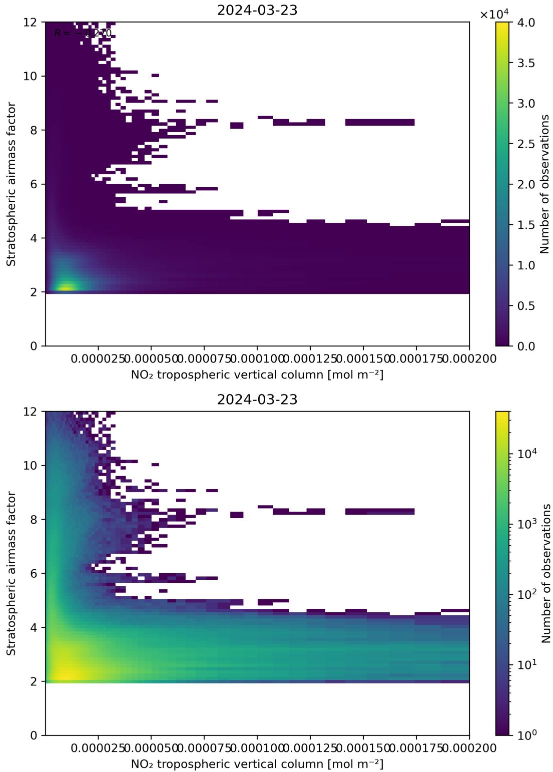
Figure 121: Scatter density plot of “NO 2 tropospheric vertical column” against “Stratospheric air mass factor” for 2024-03-23 to 2024-03-24.
