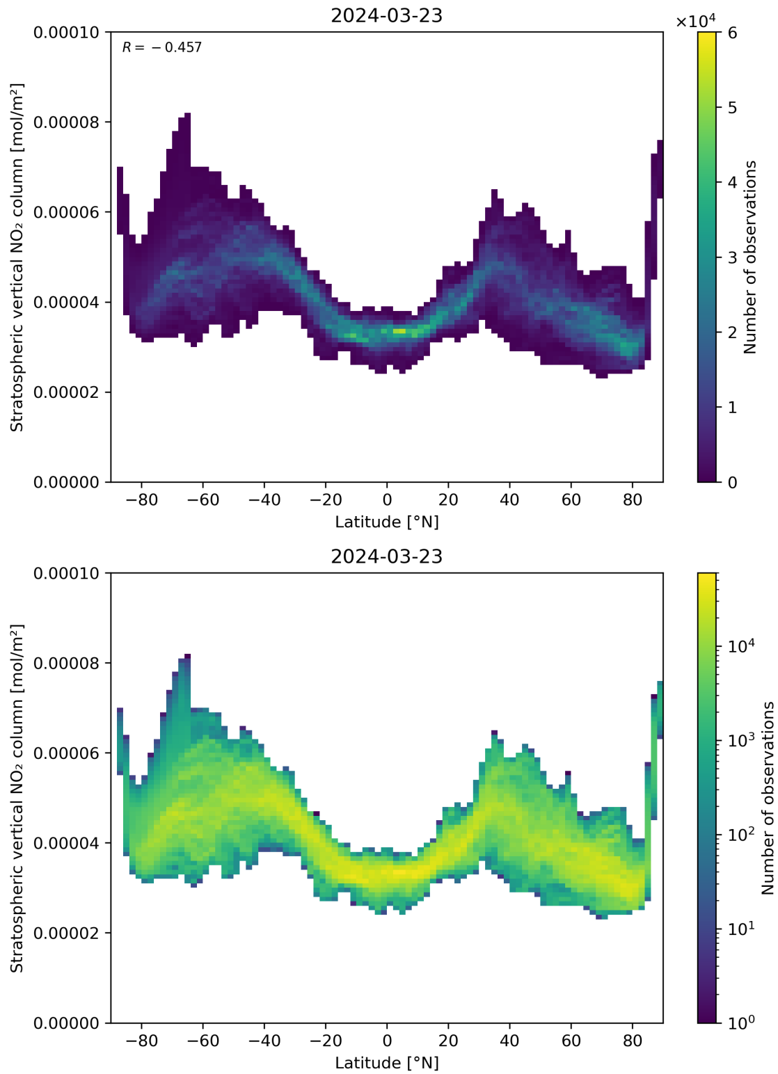
Figure 87: Scatter density plot of “Latitude” against “Stratospheric vertical NO 2 column” for 2024-03-23 to 2024-03-24.
