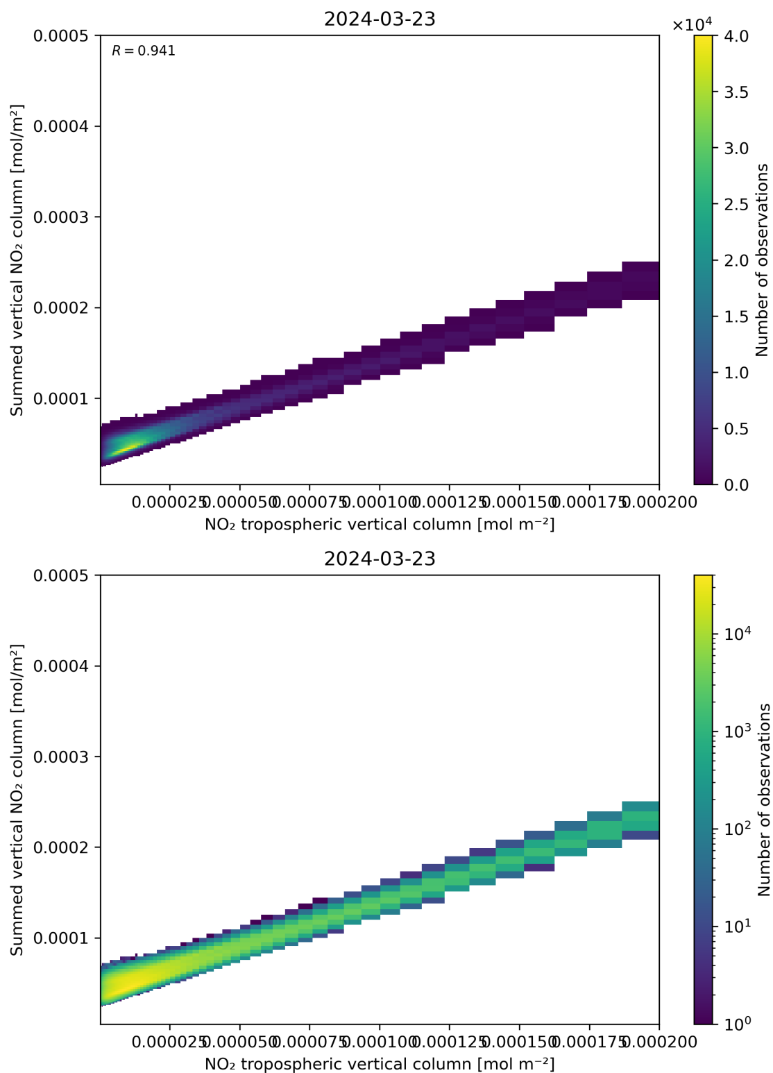
Figure 126: Scatter density plot of “NO 2 tropospheric vertical column” against “Summed vertical NO 2 column” for 2024-03-23 to 2024-03-24.
