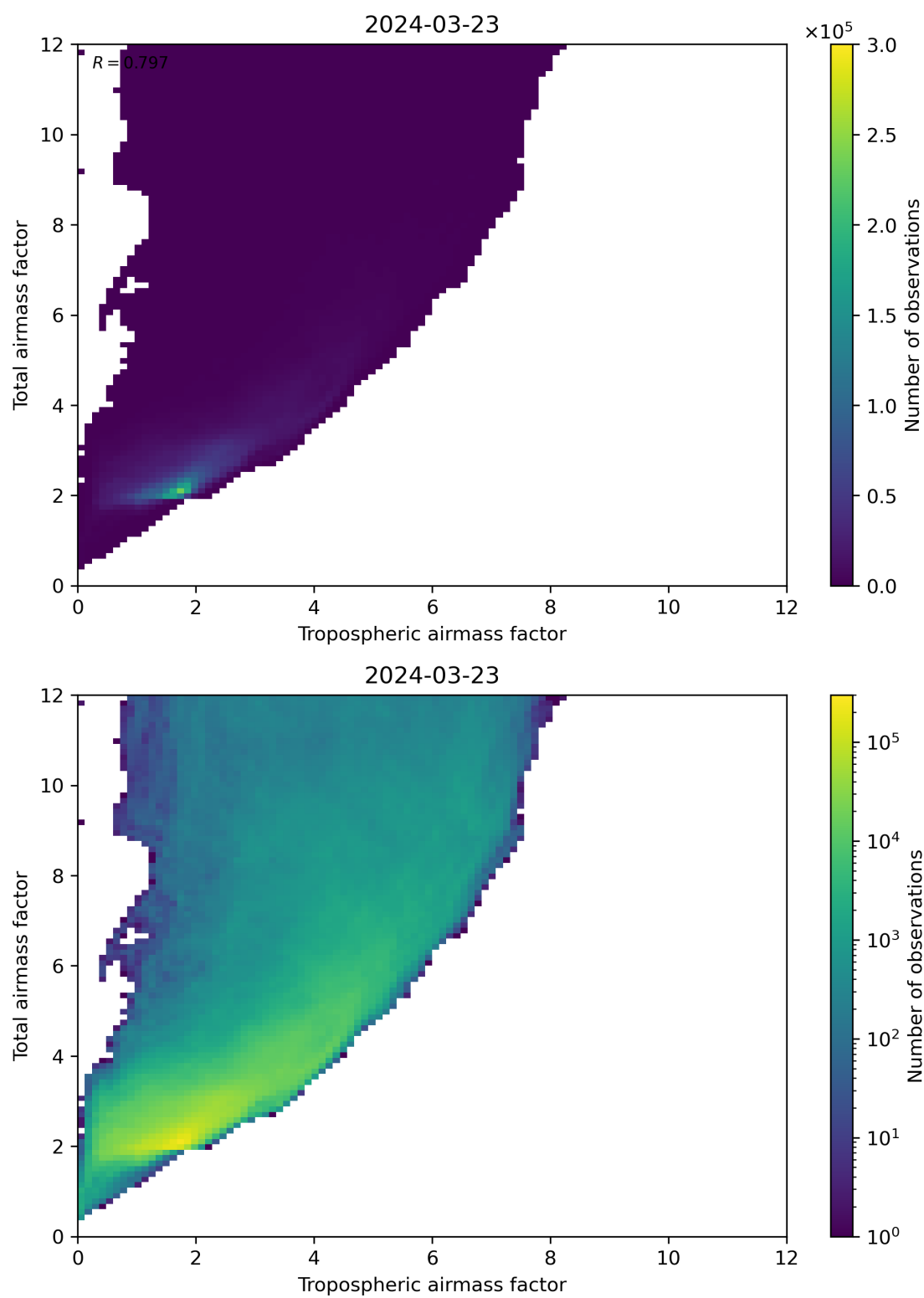
Figure 72: Scatter density plot of “Tropospheric airmass factor” against “Total airmass factor” for 2024-03-23 to 2024-03-24.
