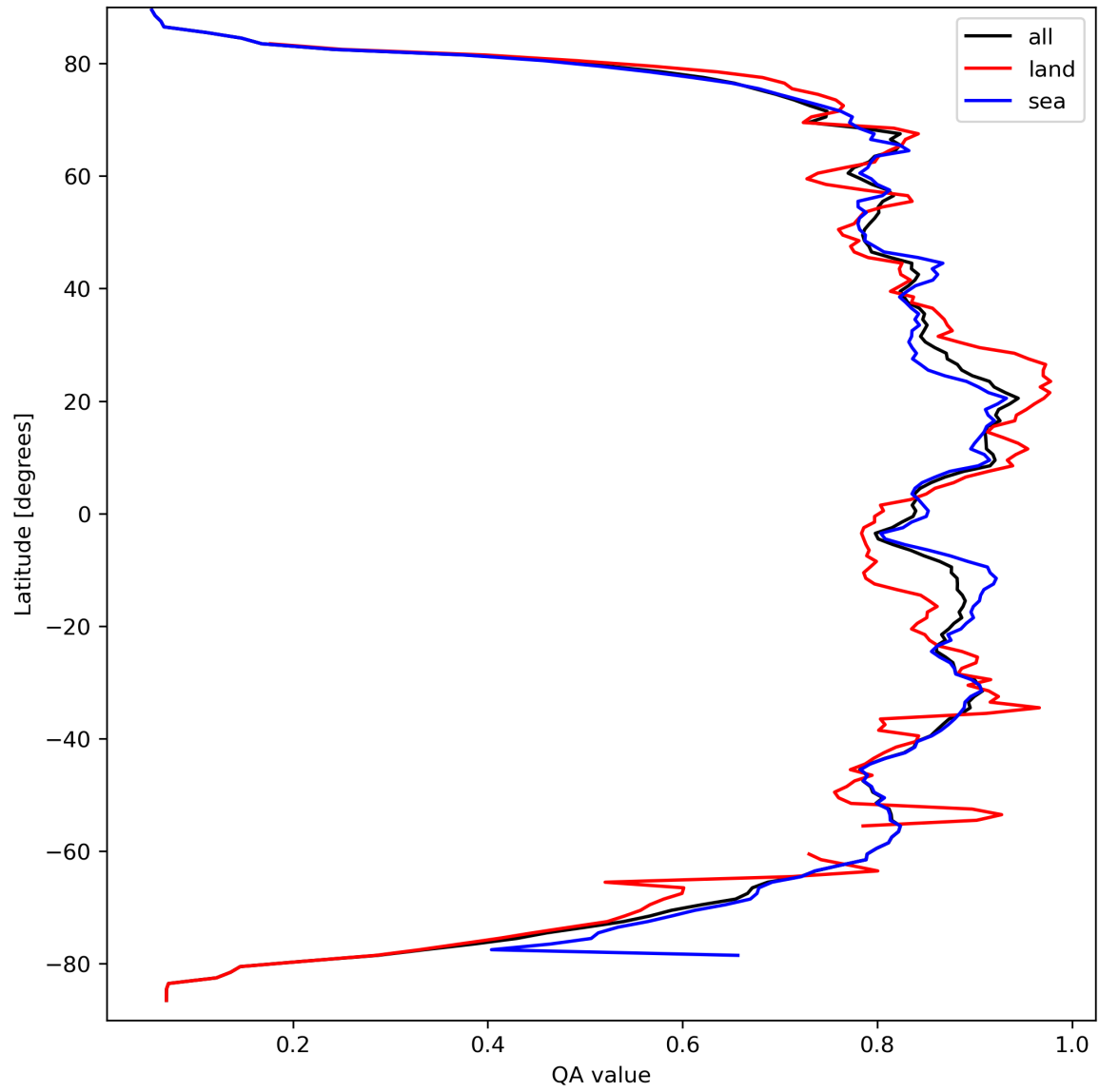
Figure 11: Zonal average of “QA value” for 2024-03-23 to 2024-03-24.
