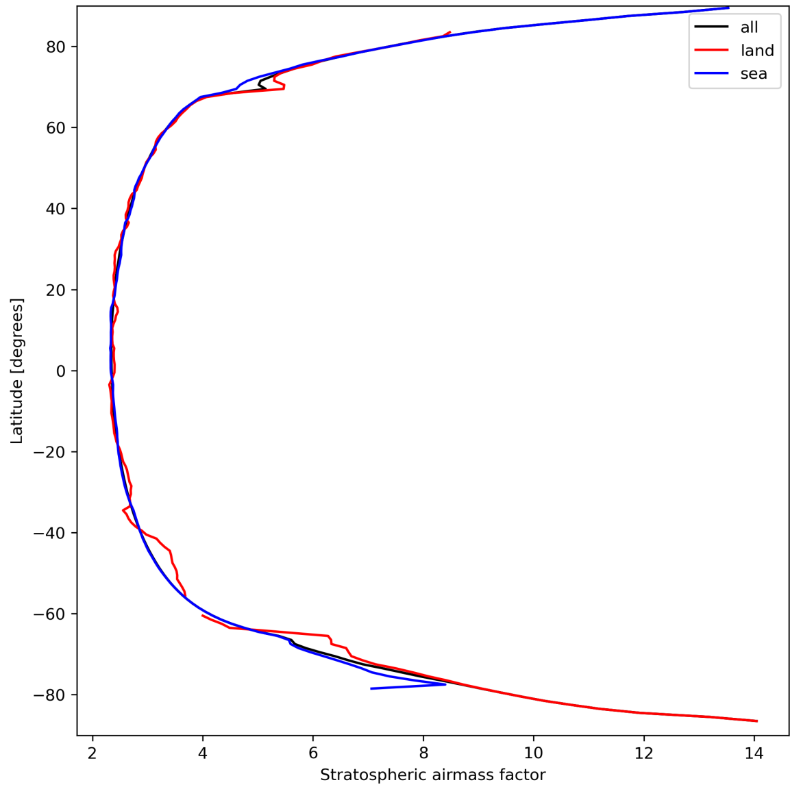
Figure 27: Zonal average of “Stratospheric airmass factor” for 2024-03-23 to 2024-03-24.
