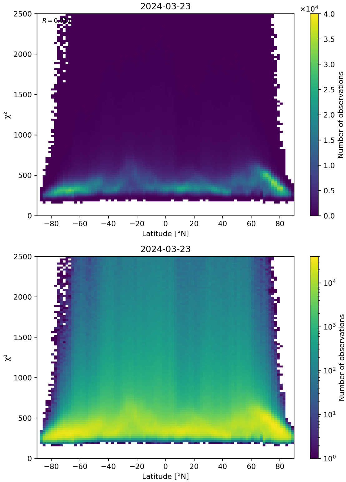
Figure 86: Scatter density plot of “Latitude” against “ \chi^2 ” for 2024-03-23 to 2024-03-24.
