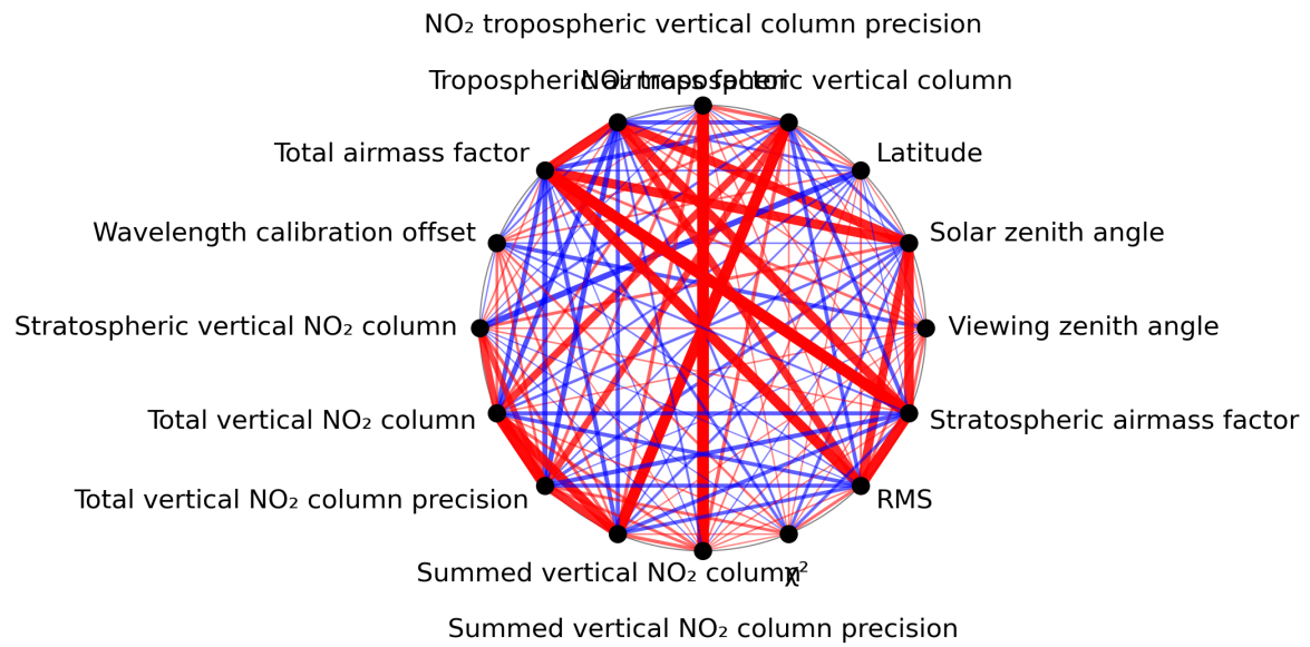
Figure 1: Map of correlation graph for 2024-03-23 to 2024-03-24.
