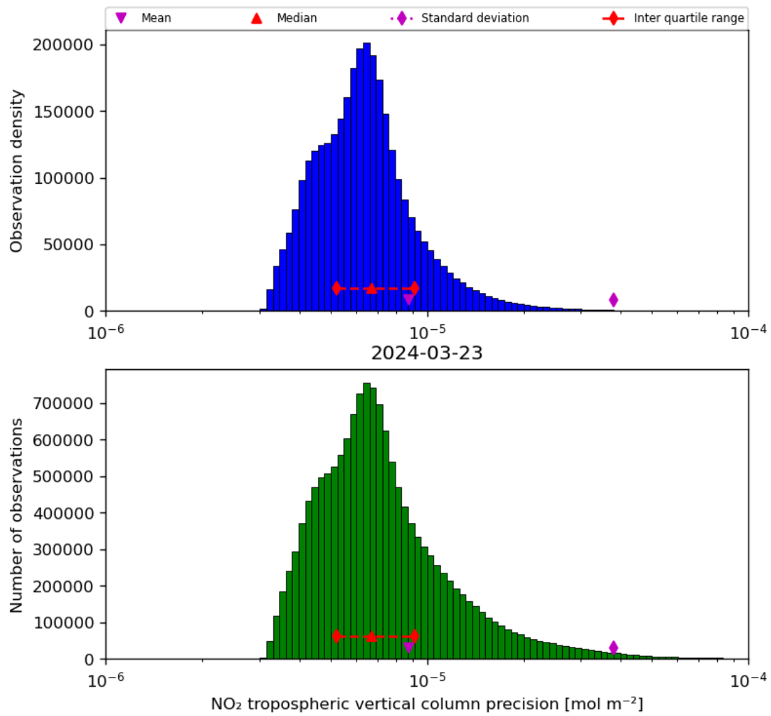
Figure 30: Histogram of “NO 2 tropospheric vertical column precision” for 2024-03-23 to 2024-03-24
