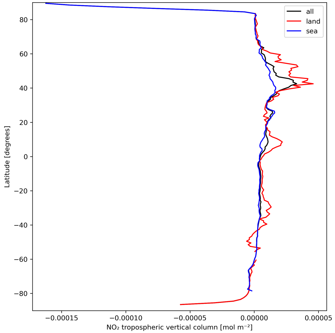
Figure 12: Zonal average of “NO 2 tropospheric vertical column” for 2024-03-23 to 2024-03-24.
