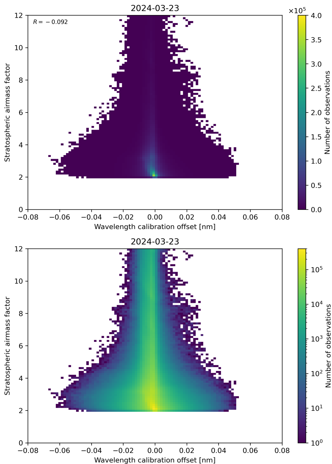
Figure 174: Scatter density plot of “Wavelength calibration offset” against “Stratospheric air mass factor” for 2024-03-23 to 2024-03-24.
