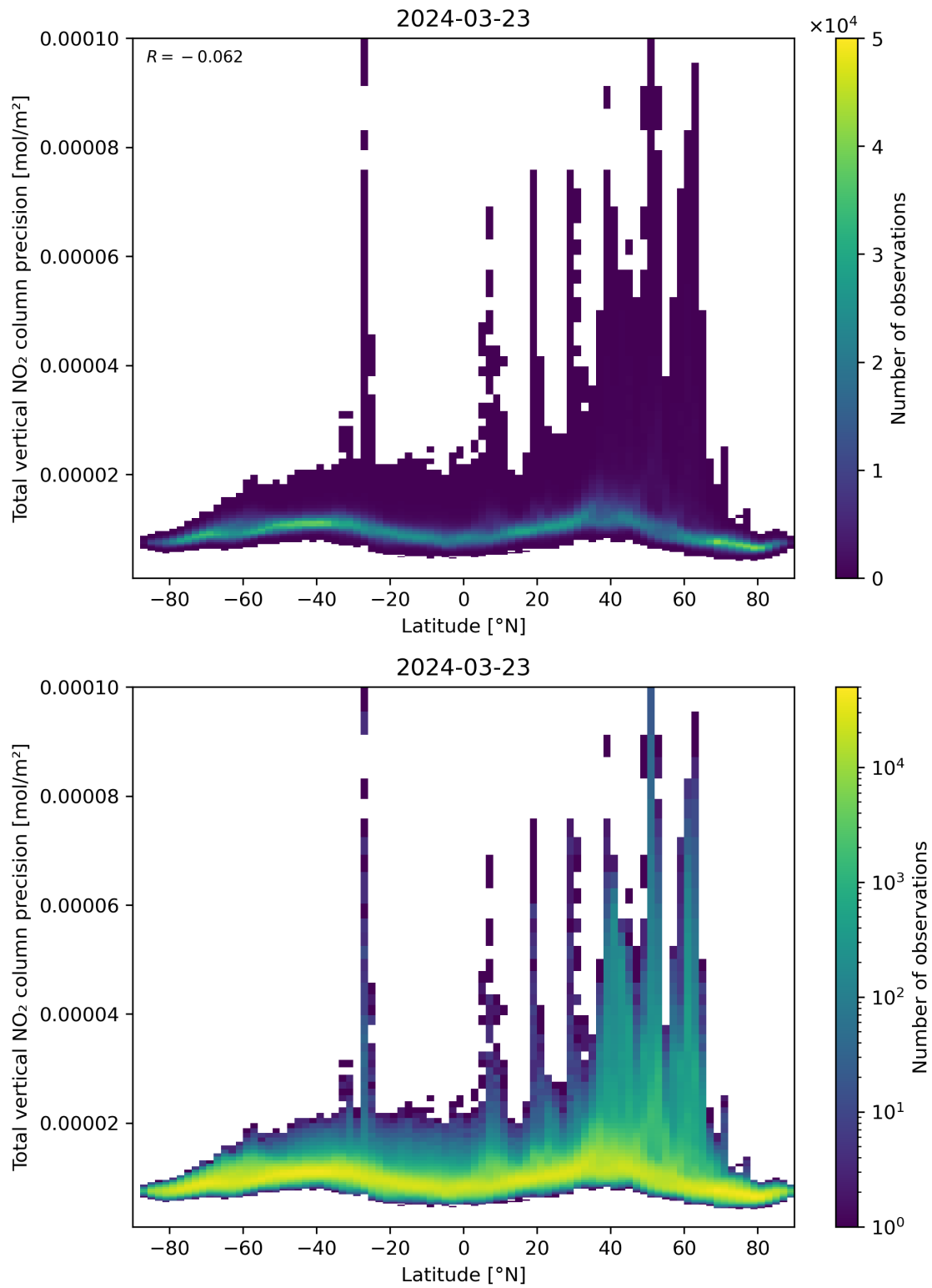
Figure 91: Scatter density plot of “Latitude” against “Total vertical NO 2 column precision” for 2024-03-23 to 2024-03-24.
