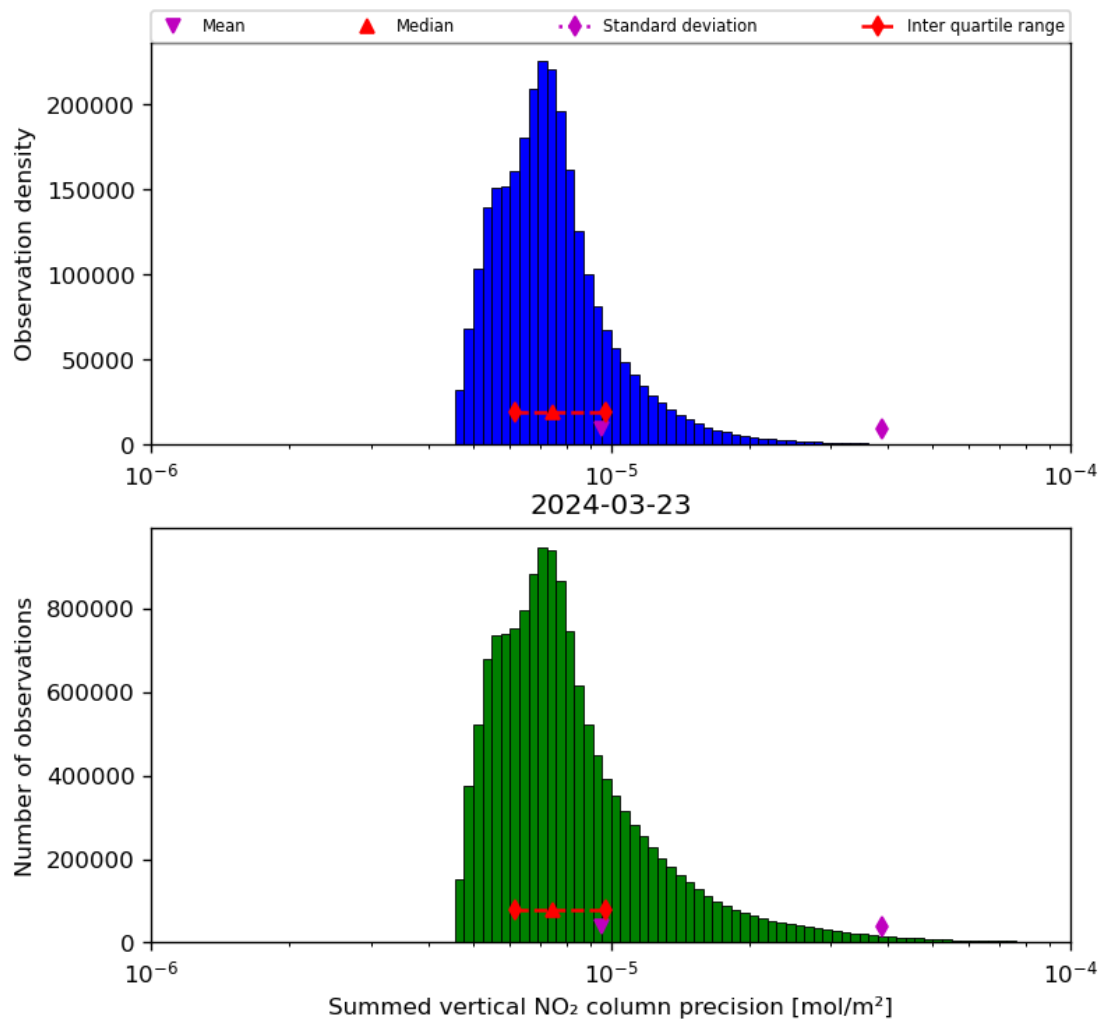
Figure 41: Histogram of “Summed vertical NO 2 column precision” for 2024-03-23 to 2024-03-24
