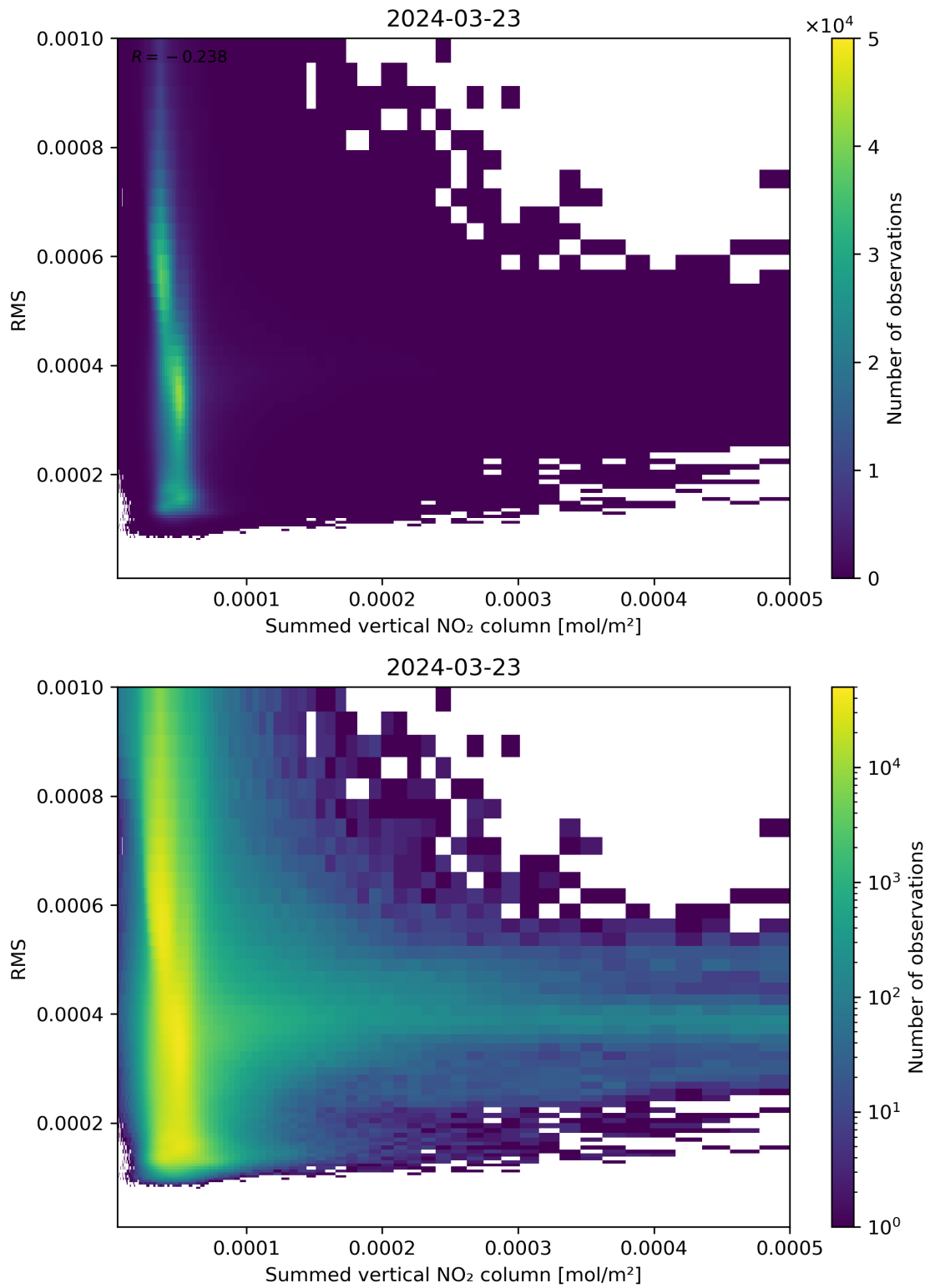
Figure 109: Scatter density plot of “Summed vertical NO 2 column” against “RMS” for 2024-03-23 to 2024-03-24.
