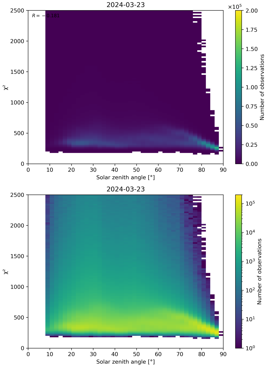
Figure 148: Scatter density plot of “Solar zenith angle” against “ \chi^2 ” for 2024-03-23 to 2024-03-24.
