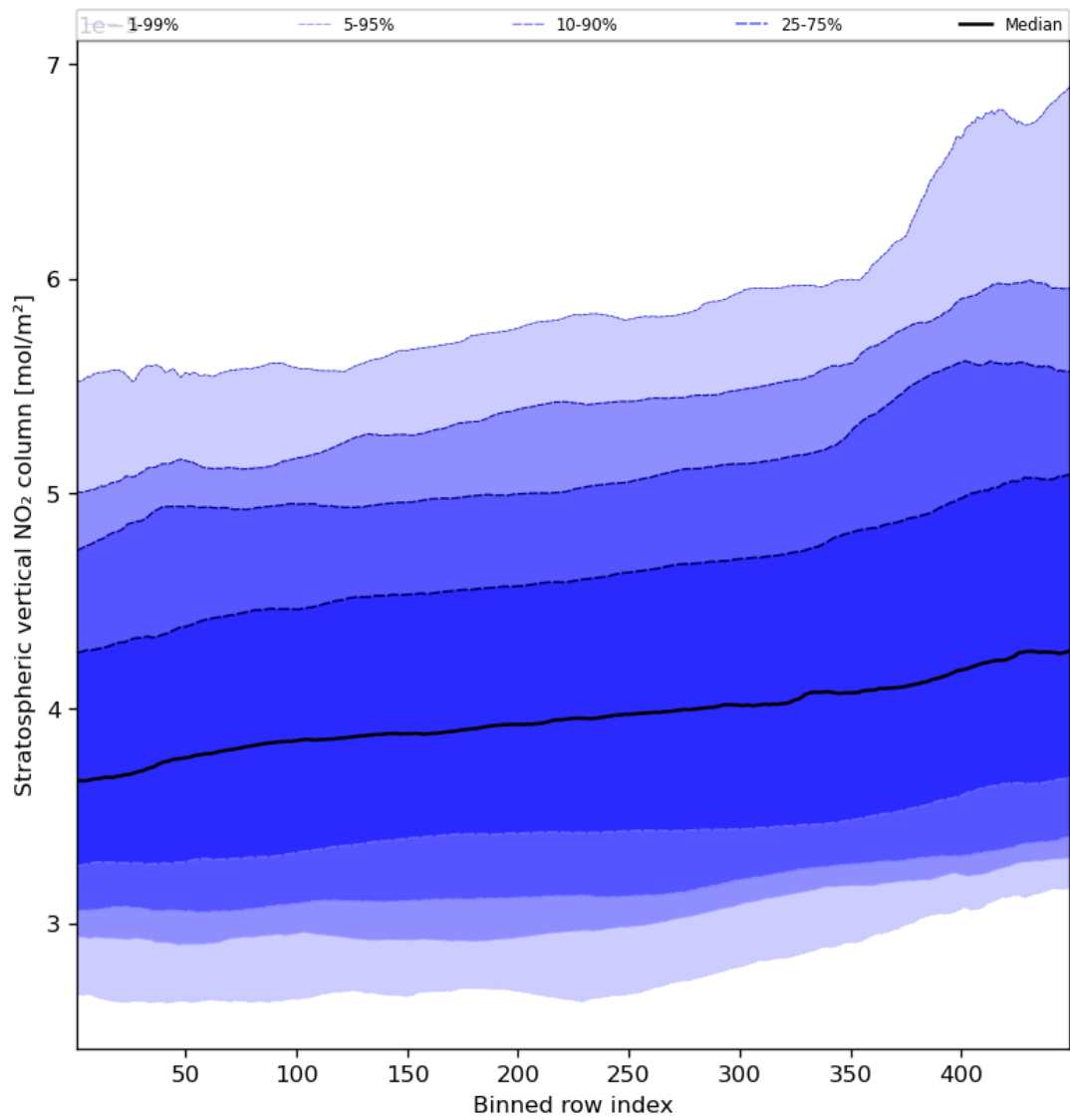
Figure 53: Along track statistics of “Stratospheric vertical NO 2 column” for 2024-03-23 to 2024-03-24
