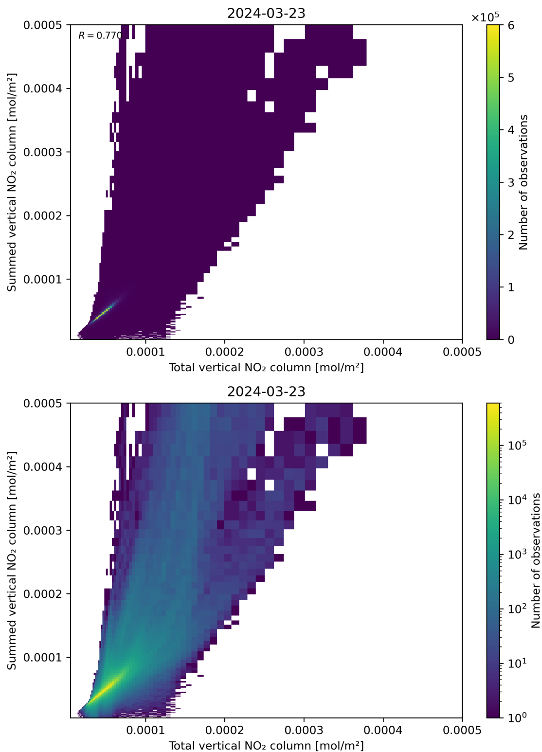
Figure 112: Scatter density plot of “Total vertical NO 2 column” against “Summed vertical NO 2 column” for 2024-03-23 to 2024-03-24.
