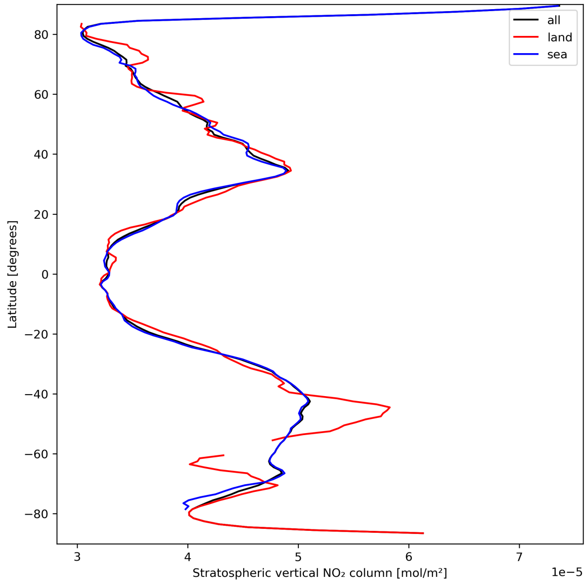
Figure 19: Zonal average of “Stratospheric vertical NO 2 column” for 2024-03-23 to 2024-03-24.
