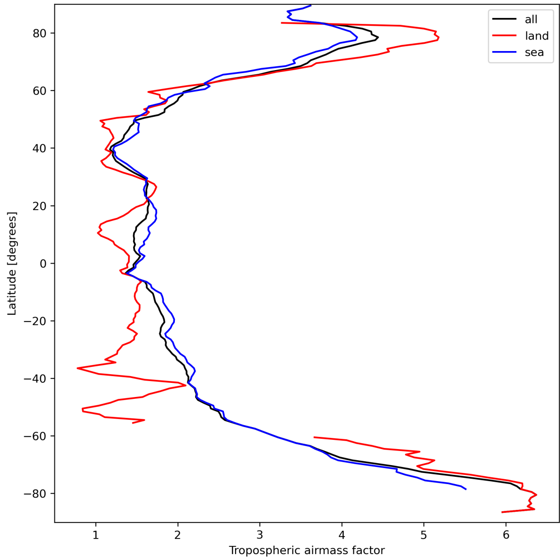
Figure 14: Zonal average of “Tropospheric airmass factor” for 2024-03-23 to 2024-03-24.
