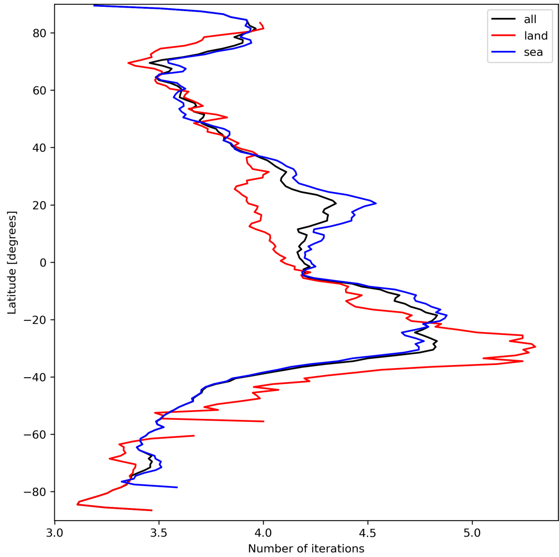
Figure 17: Zonal average of “Number of iterations” for 2024-03-23 to 2024-03-24.
