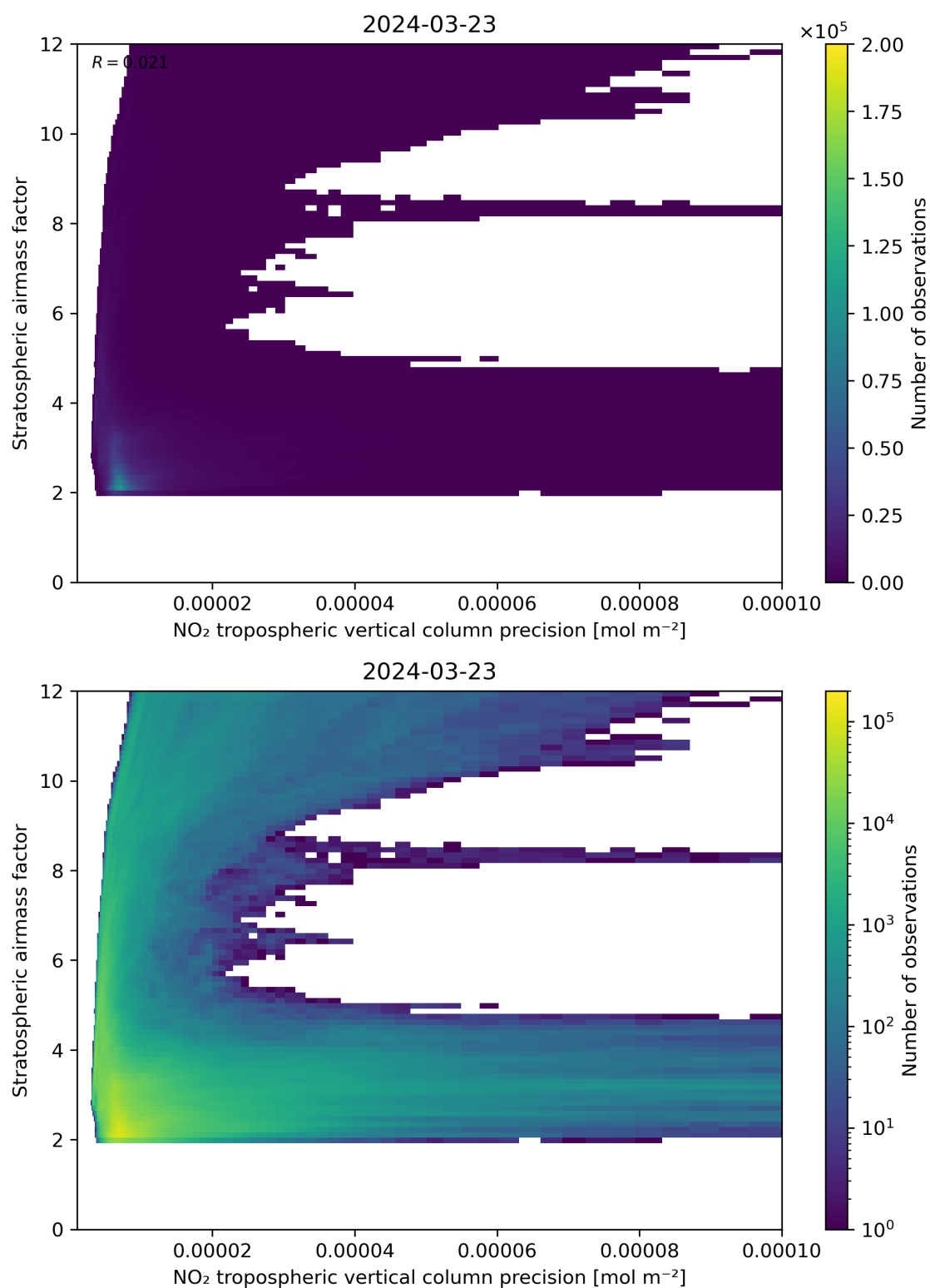
Figure 131: Scatter density plot of “NO 2 tropospheric vertical column precision” against “Stratospheric airmass factor” for 2024-03-23 to 2024-03-24.
