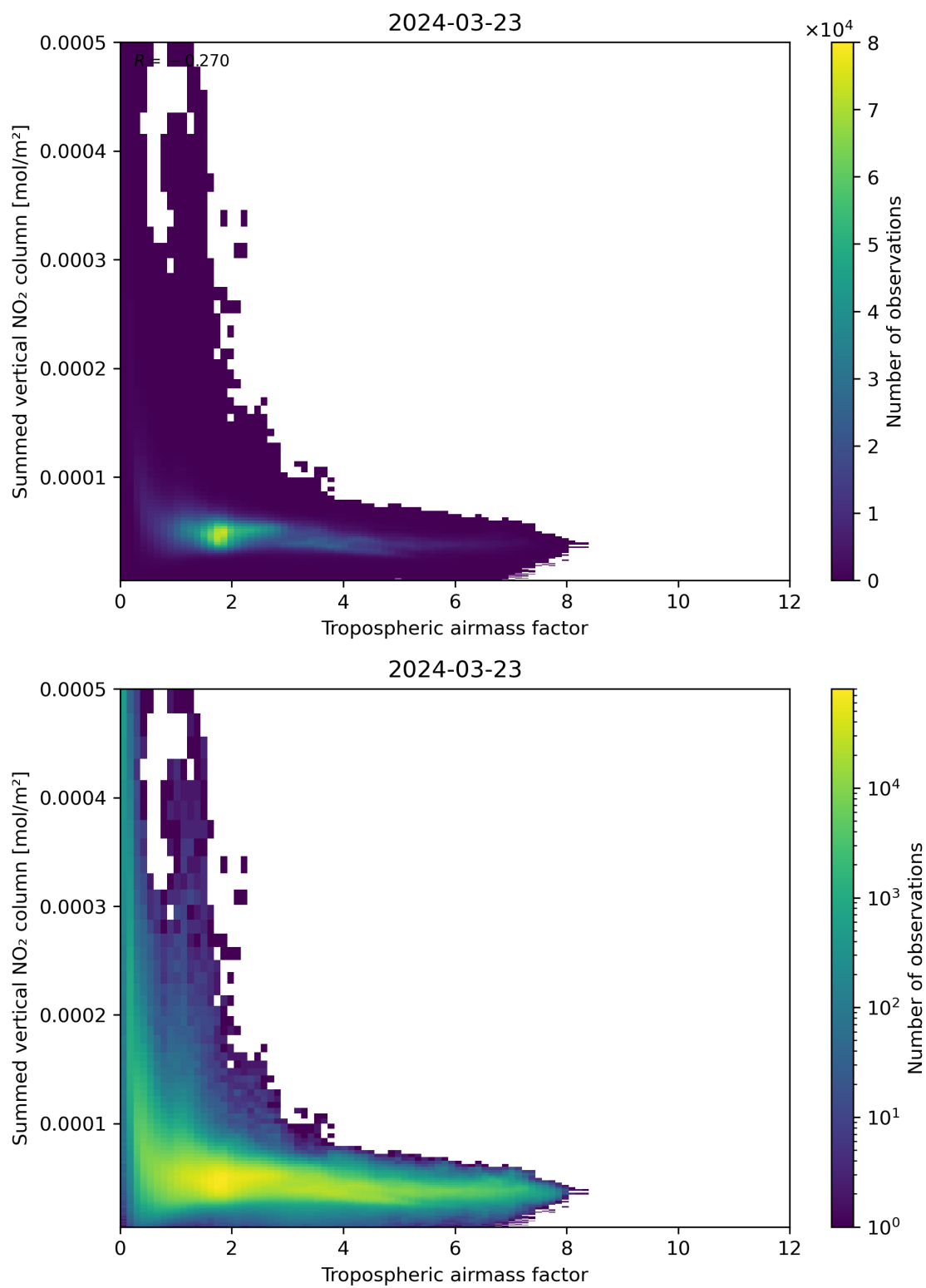
Figure 75: Scatter density plot of “Tropospheric airmass factor” against “Summed vertical NO 2 column” for 2024-03-23 to 2024-03-24.
