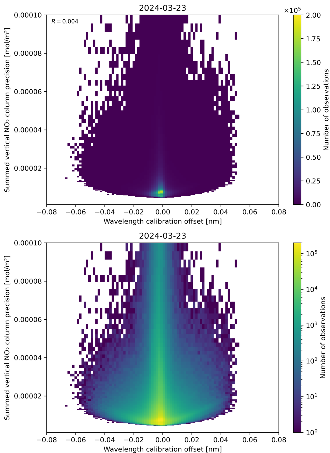
Figure 178: Scatter density plot of “Wavelength calibration offset” against “Summed vertical NO 2 column precision” for 2024-03-23 to 2024-03-24.
