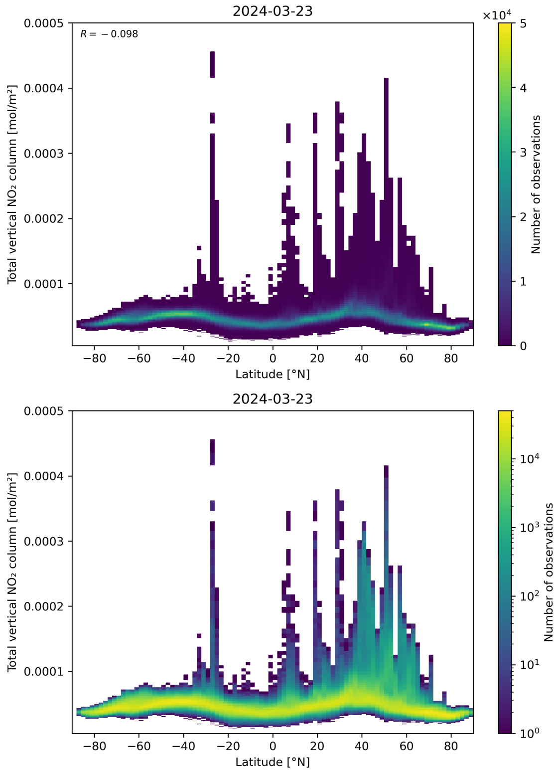
Figure 90: Scatter density plot of “Latitude” against “Total vertical NO 2 column” for 2024-03-23 to 2024-03-24.
