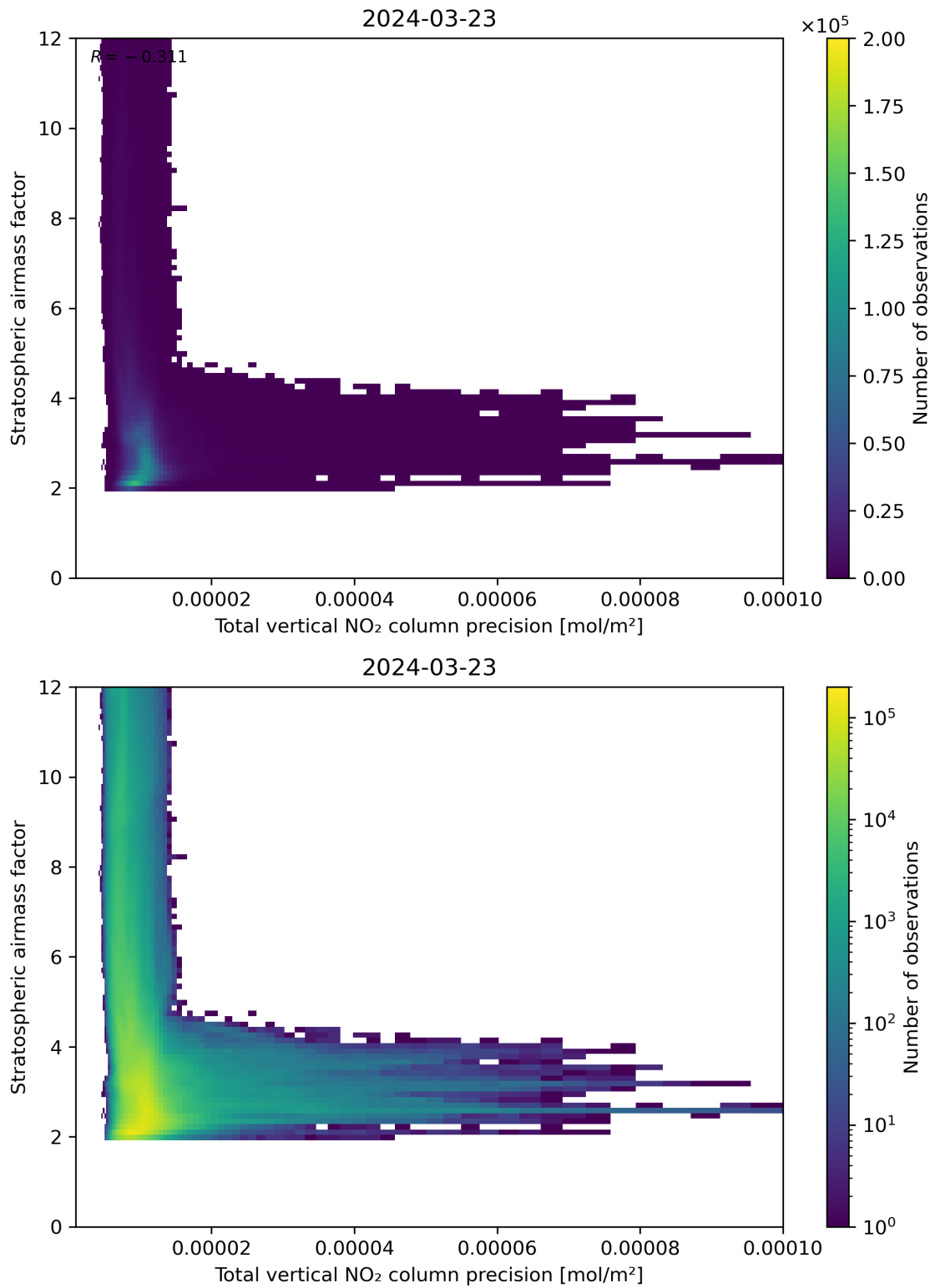
Figure 115: Scatter density plot of “Total vertical NO 2 column precision” against “Stratospheric air mass factor” for 2024-03-23 to 2024-03-24.
