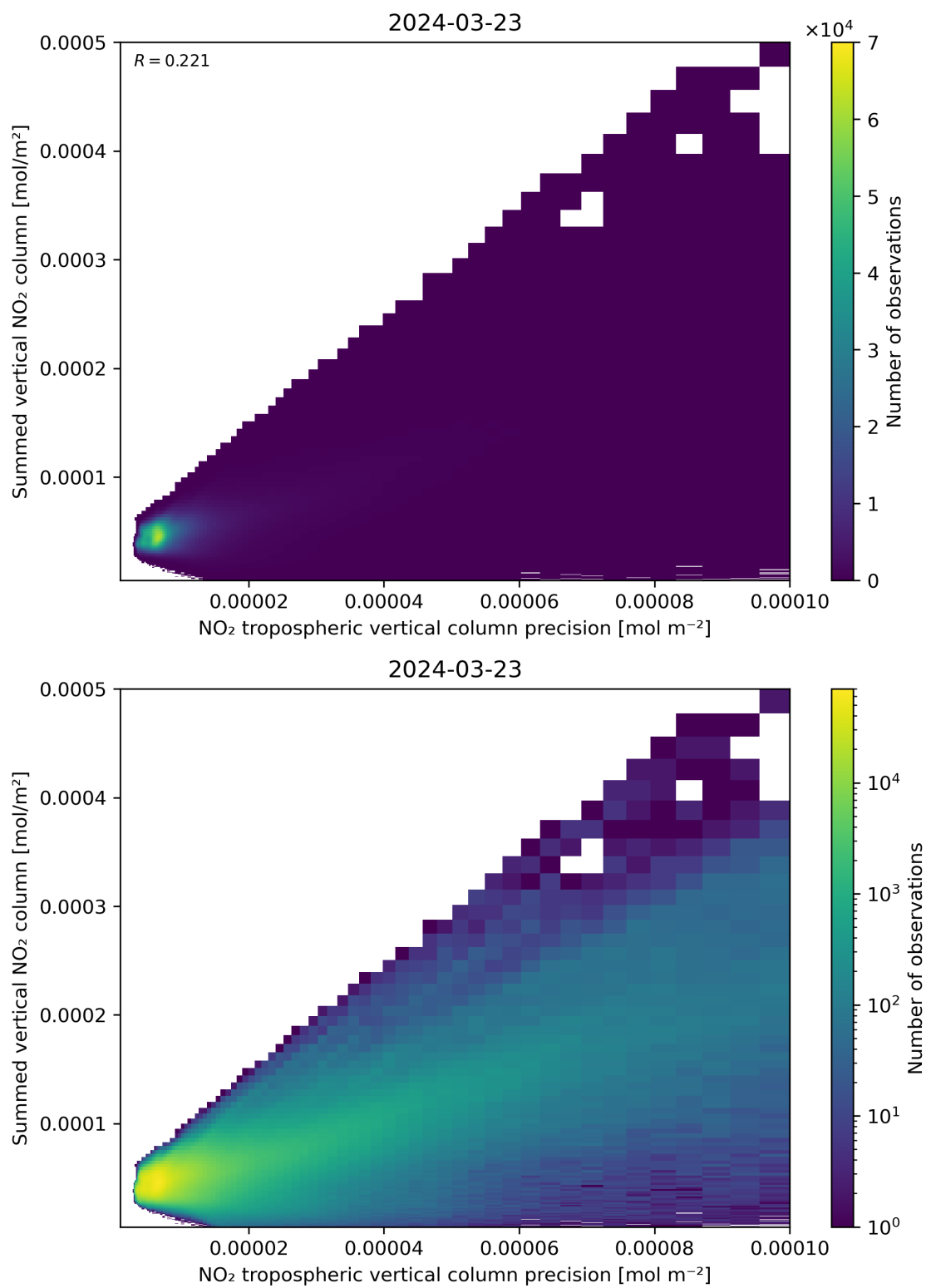
Figure 136: Scatter density plot of “NO 2 tropospheric vertical column precision” against “Summed vertical NO 2 column” for 2024-03-23 to 2024-03-24.
