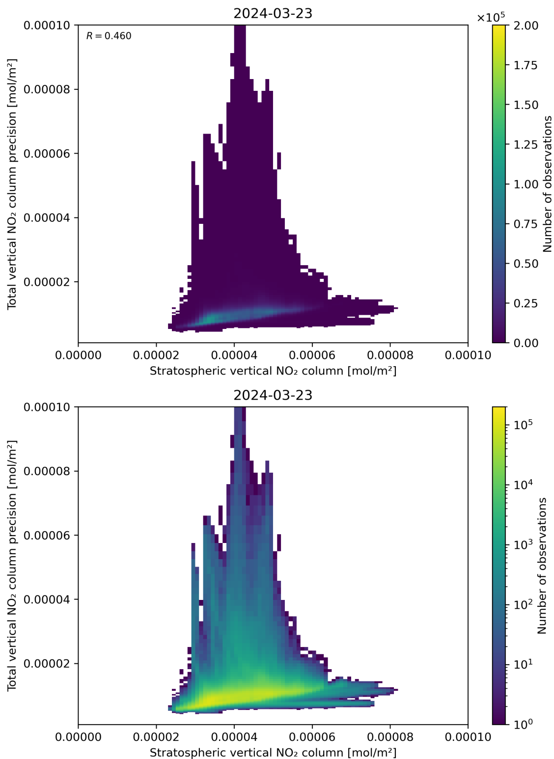
Figure 101: Scatter density plot of “Stratospheric vertical NO 2 column” against “Total vertical NO 2 column precision” for 2024-03-23 to 2024-03-24.
