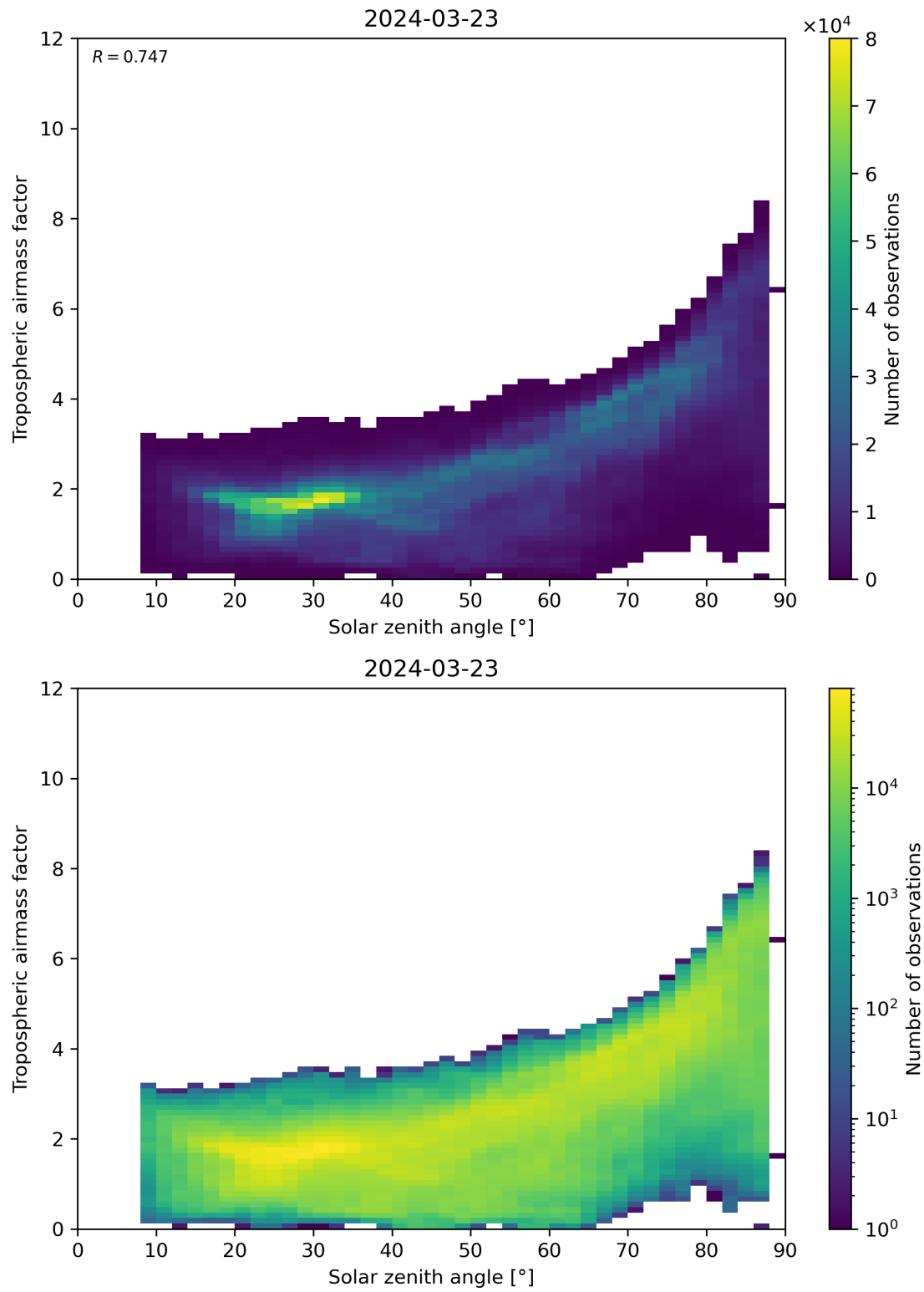
Figure 147: Scatter density plot of “Solar zenith angle” against “Tropospheric airmass factor” for 2024-03-23 to 2024-03-24.
