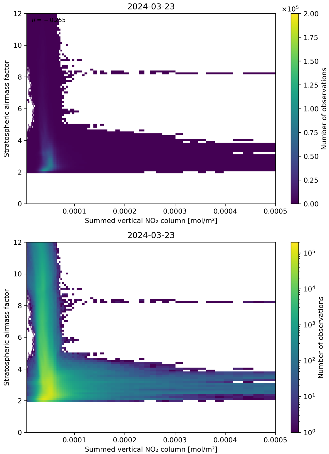
Figure 103: Scatter density plot of “Summed vertical NO 2 column” against “Stratospheric airmass factor” for 2024-03-23 to 2024-03-24.
