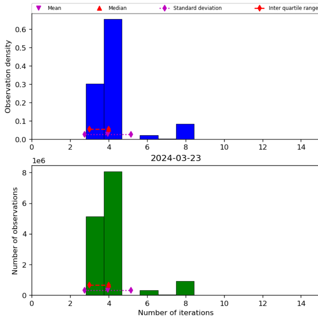
Figure 34: Histogram of “Number of iterations” for 2024-03-23 to 2024-03-24
