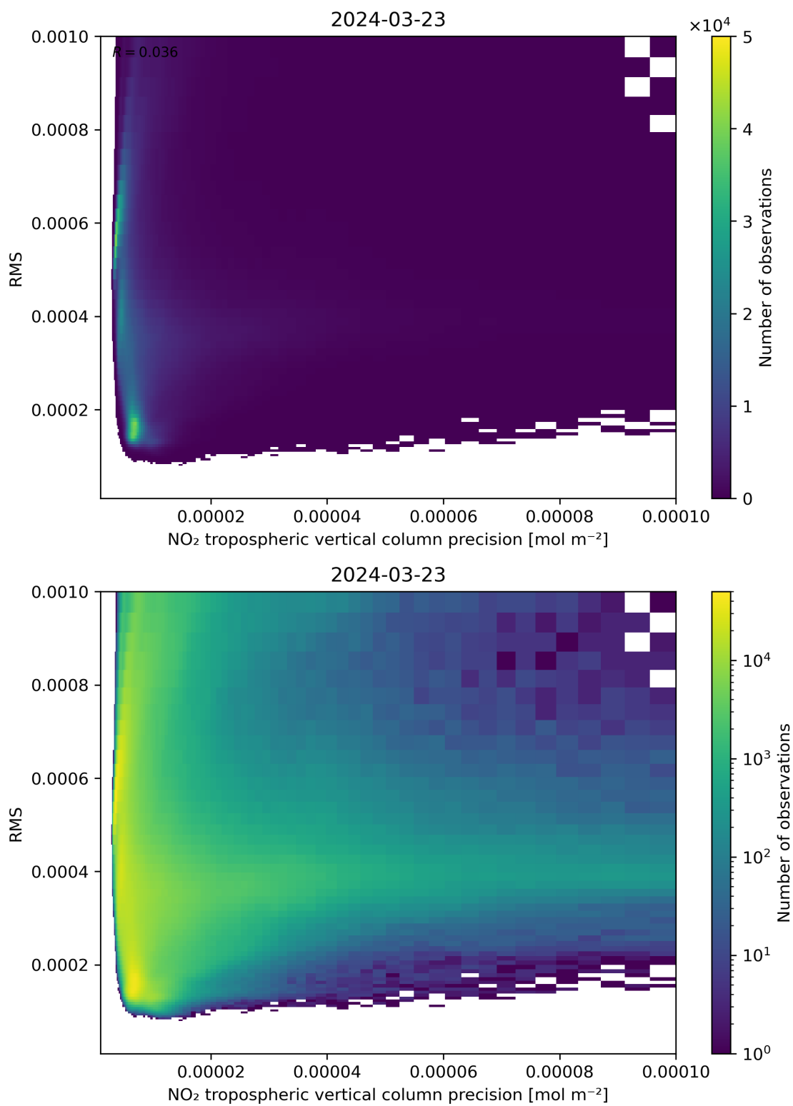
Figure 140: Scatter density plot of “NO 2 tropospheric vertical column precision” against “RMS” for 2024-03-23 to 2024-03-24.
