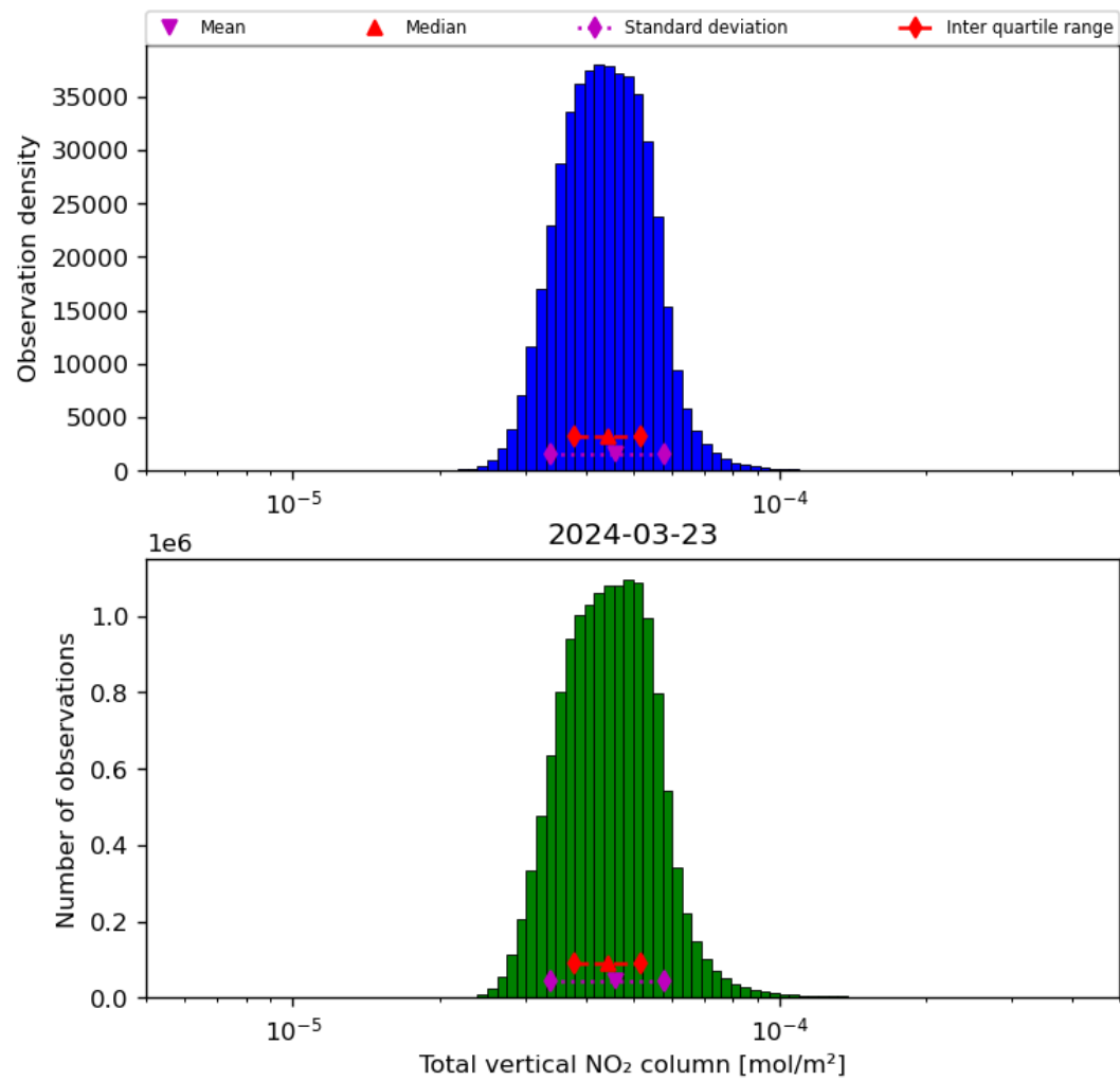
Figure 38: Histogram of "Total vertical NO 2 column" for 2024-03-23 to 2024-03-24
