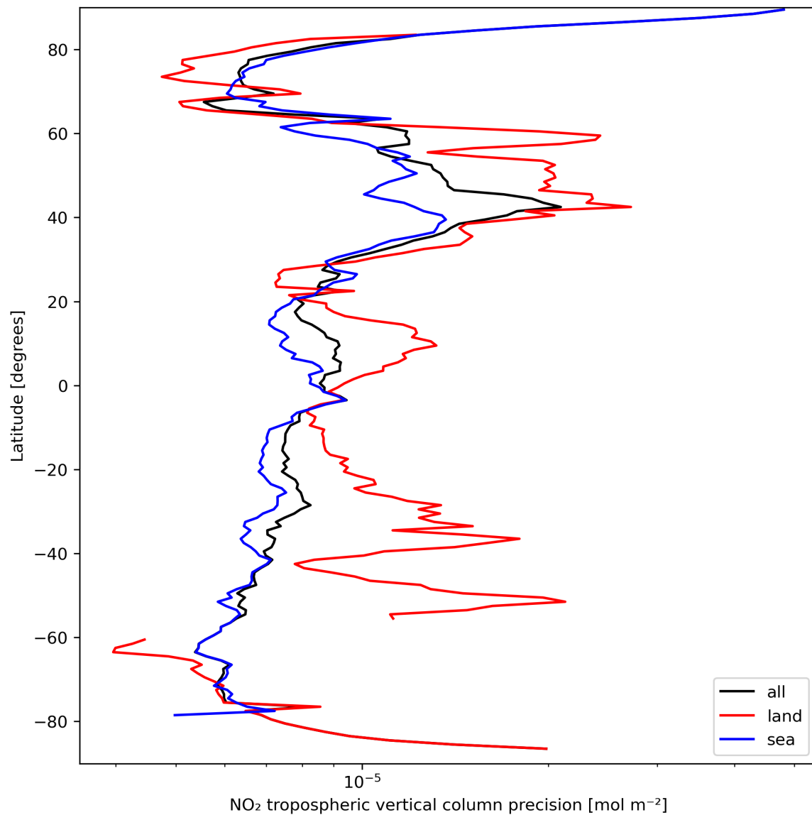
Figure 13: Zonal average of “NO 2 tropospheric vertical column precision” for 2024-03-23 to 2024-03-24.
