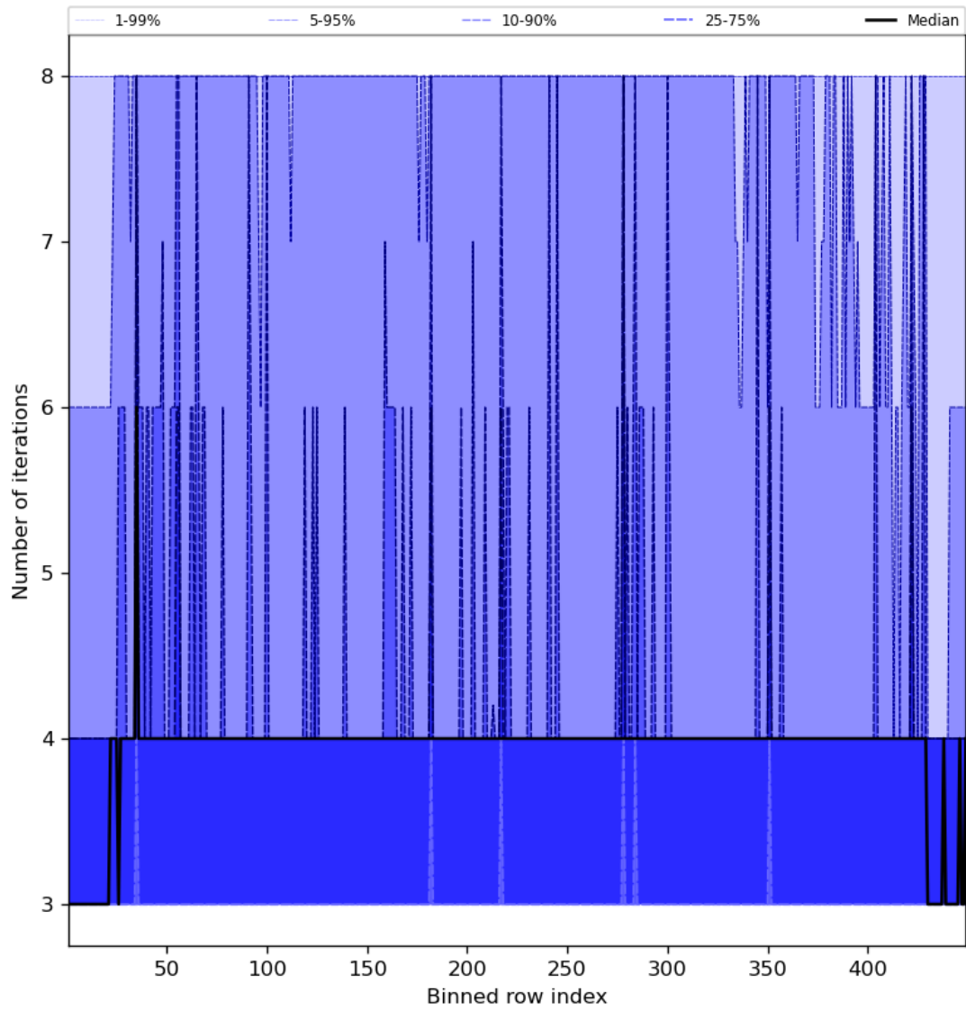
Figure 51: Along track statistics of “Number of iterations” for 2024-03-23 to 2024-03-24
