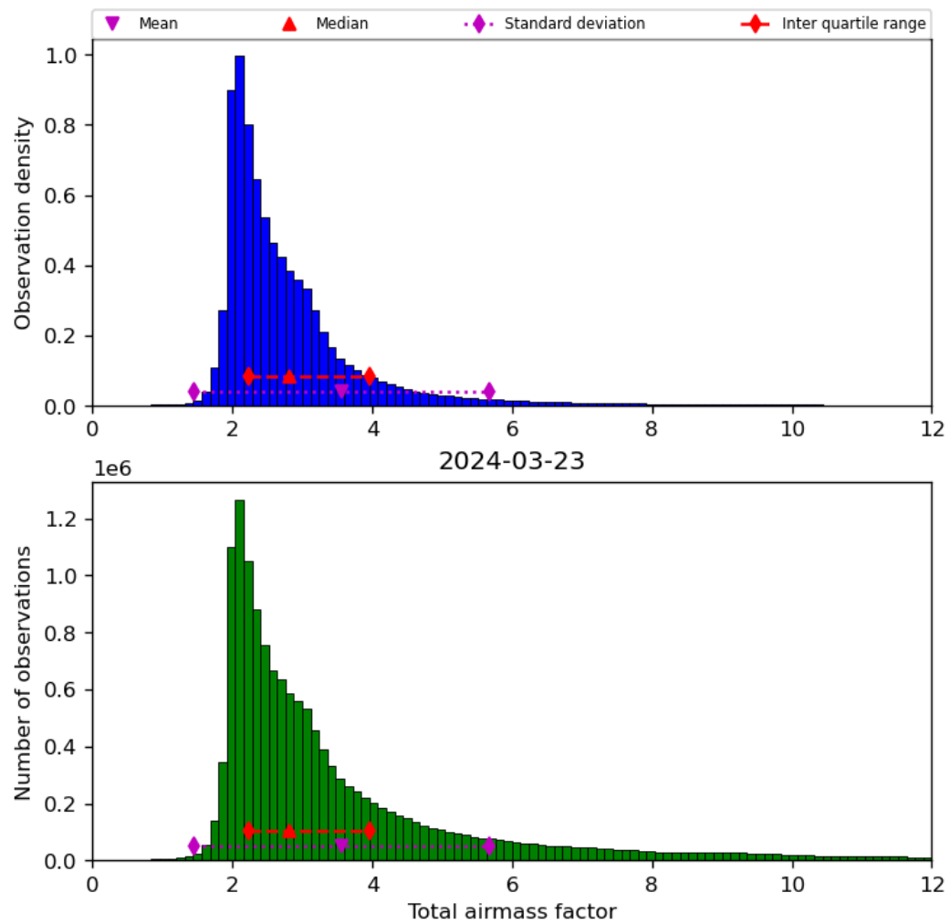
Figure 32: Histogram of “Total airmass factor” for 2024-03-23 to 2024-03-24
