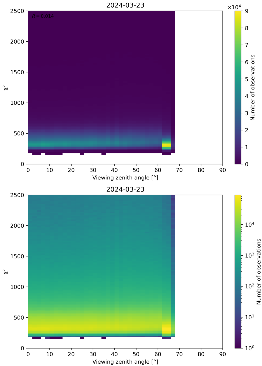
Figure 162: Scatter density plot of “Viewing zenith angle” against “ \chi^2 ” for 2024-03-23 to 2024-03-24.
