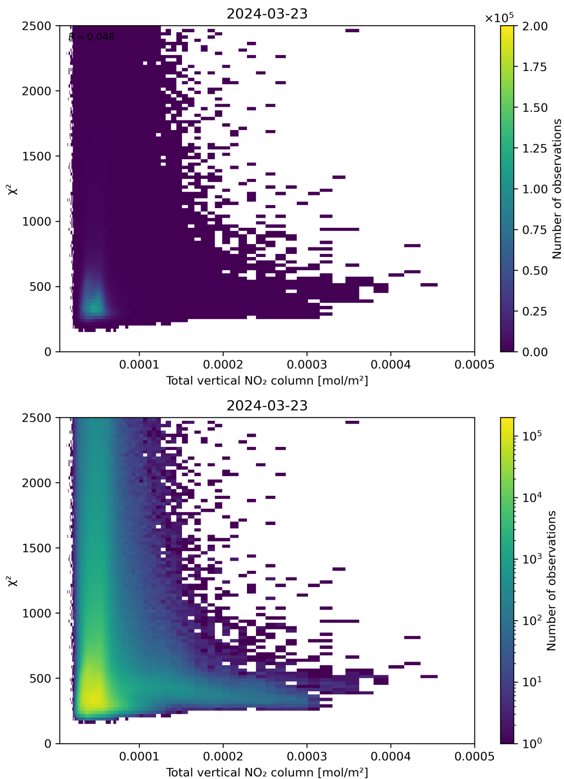
Figure 111: Scatter density plot of “Total vertical NO 2 column” against “ \chi^2 ” for 2024-03-23 to 2024-03-24.
