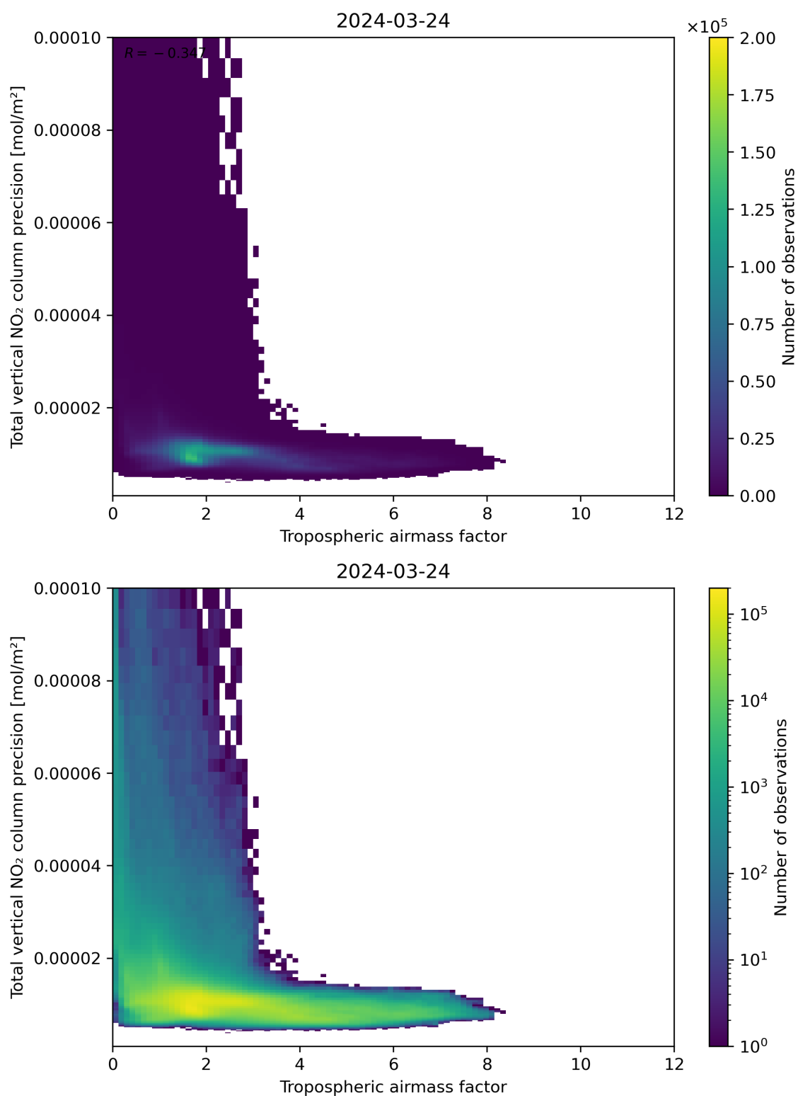
Figure 78: Scatter density plot of “Tropospheric air mass factor” against “Total vertical NO 2 column precision” for 2024-03-23 to 2024-03-25.
