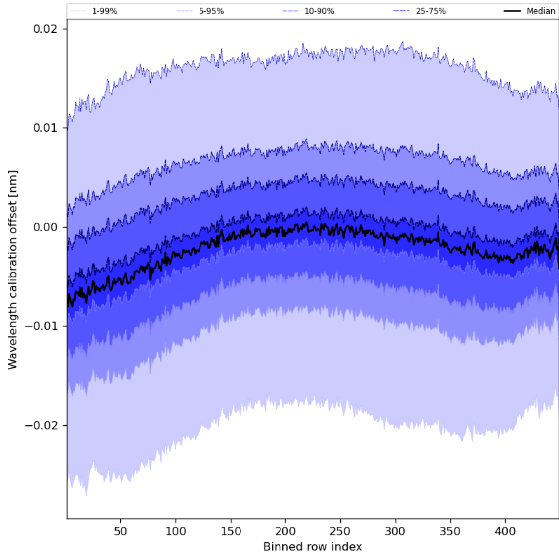
Figure 52: Along track statistics of “Wavelength calibration offset” for 2024-03-23 to 2024-03-25
