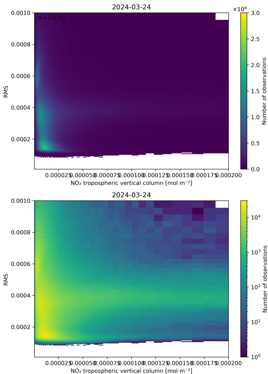
Figure 142: Scatter density plot of “NO 2 tropospheric vertical column” against “RMS” for 2024-03-23 to 2024-03-25.
