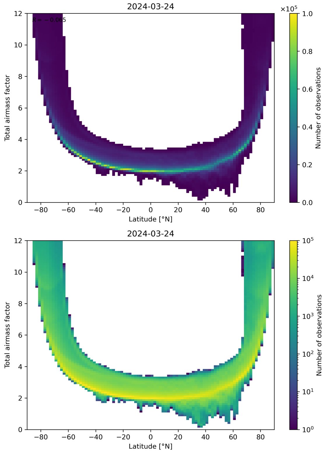
Figure 84: Scatter density plot of “Latitude” against “Total airmass factor” for 2024-03-23 to 2024-03-25.
