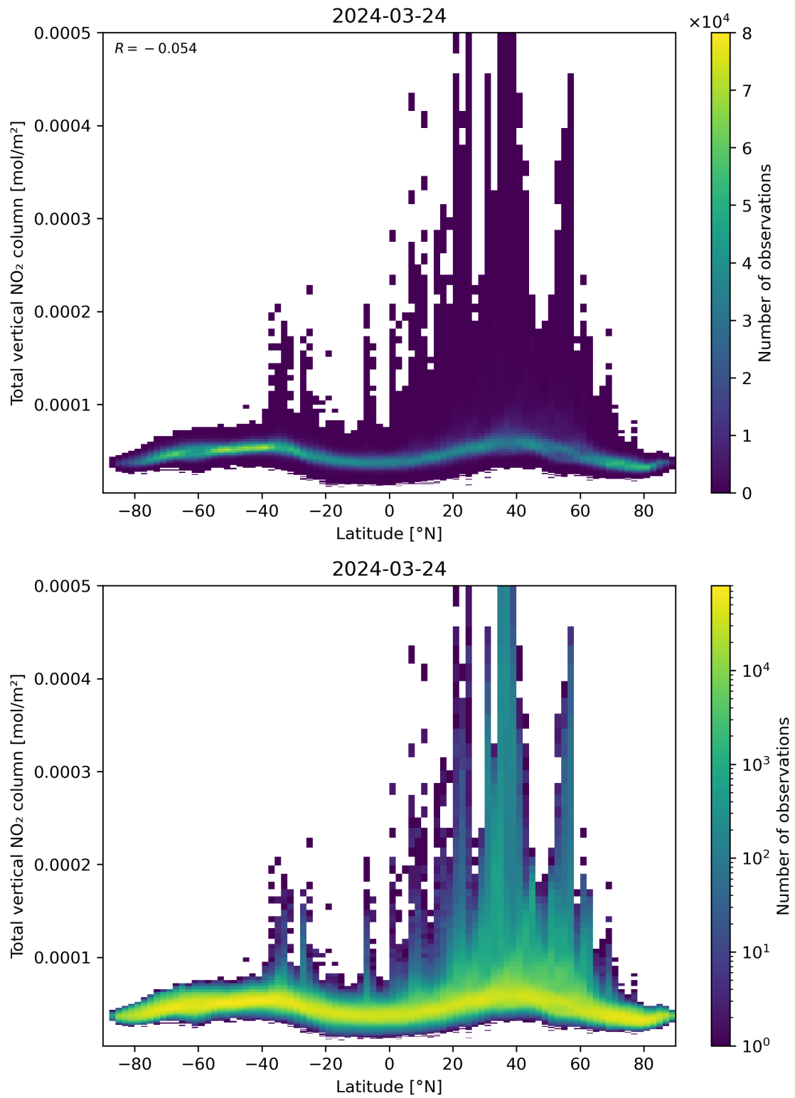
Figure 90: Scatter density plot of “Latitude” against “Total vertical NO 2 column” for 2024-03-23 to 2024-03-25.
