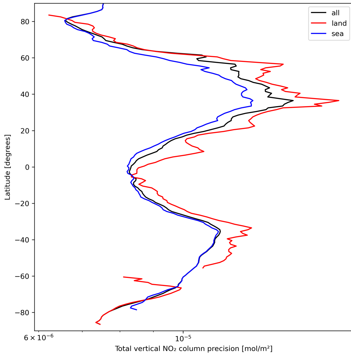
Figure 22: Zonal average of “Total vertical NO 2 column precision” for 2024-03-23 to 2024-03-25.
