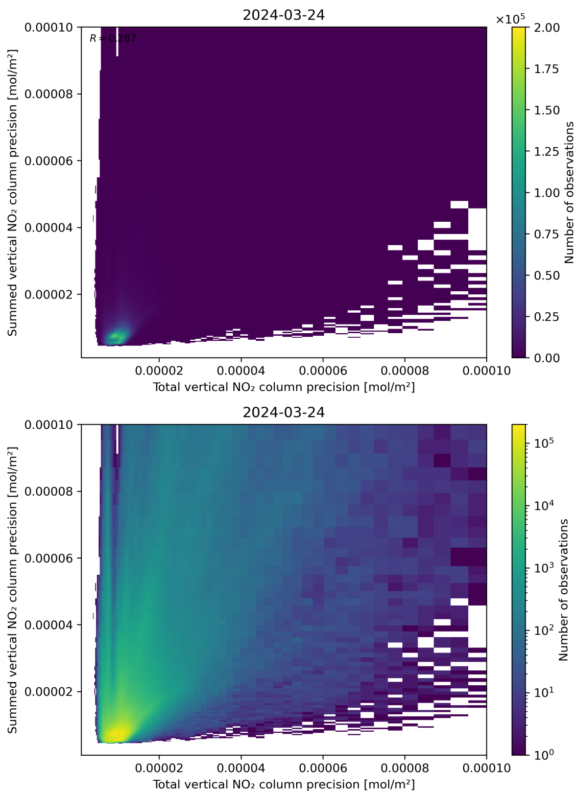
Figure 118: Scatter density plot of “Total vertical NO 2 column precision” against “Summed vertical NO 2 column precision” for 2024-03-23 to 2024-03-25.
