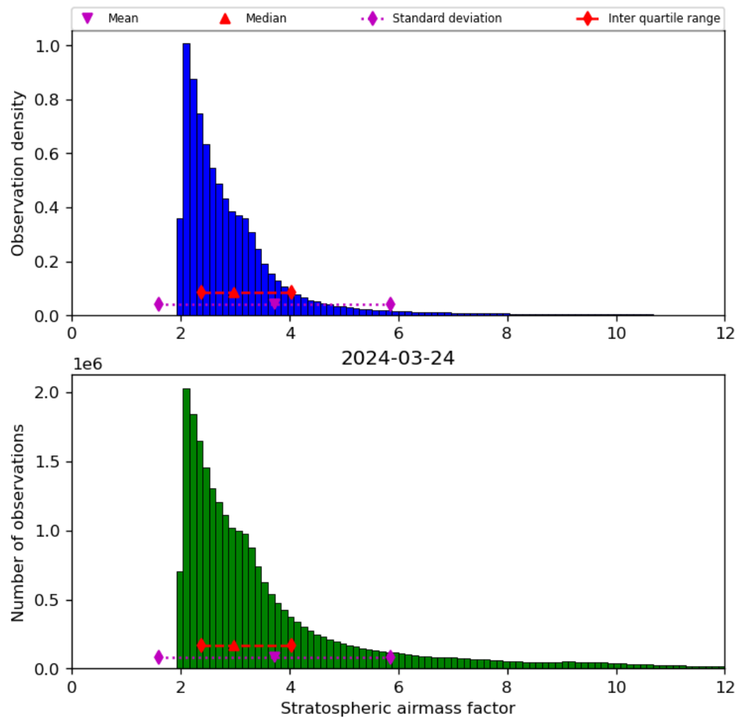
Figure 44: Histogram of “Stratospheric airmass factor” for 2024-03-23 to 2024-03-25
