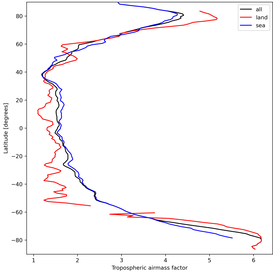
Figure 14: Zonal average of “Tropospheric airmass factor” for 2024-03-23 to 2024-03-25.
