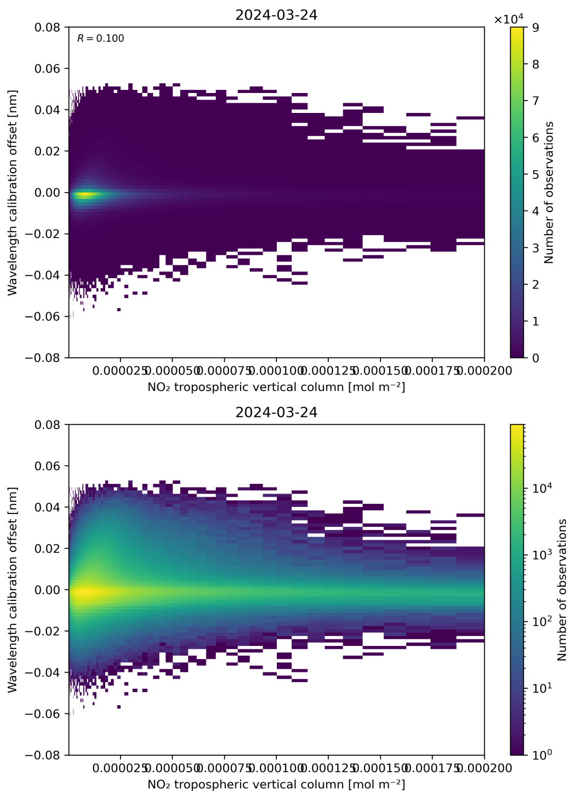
Figure 143: Scatter density plot of “NO 2 tropospheric vertical column” against “Wavelength calibration offset” for 2024-03-23 to 2024-03-25.
