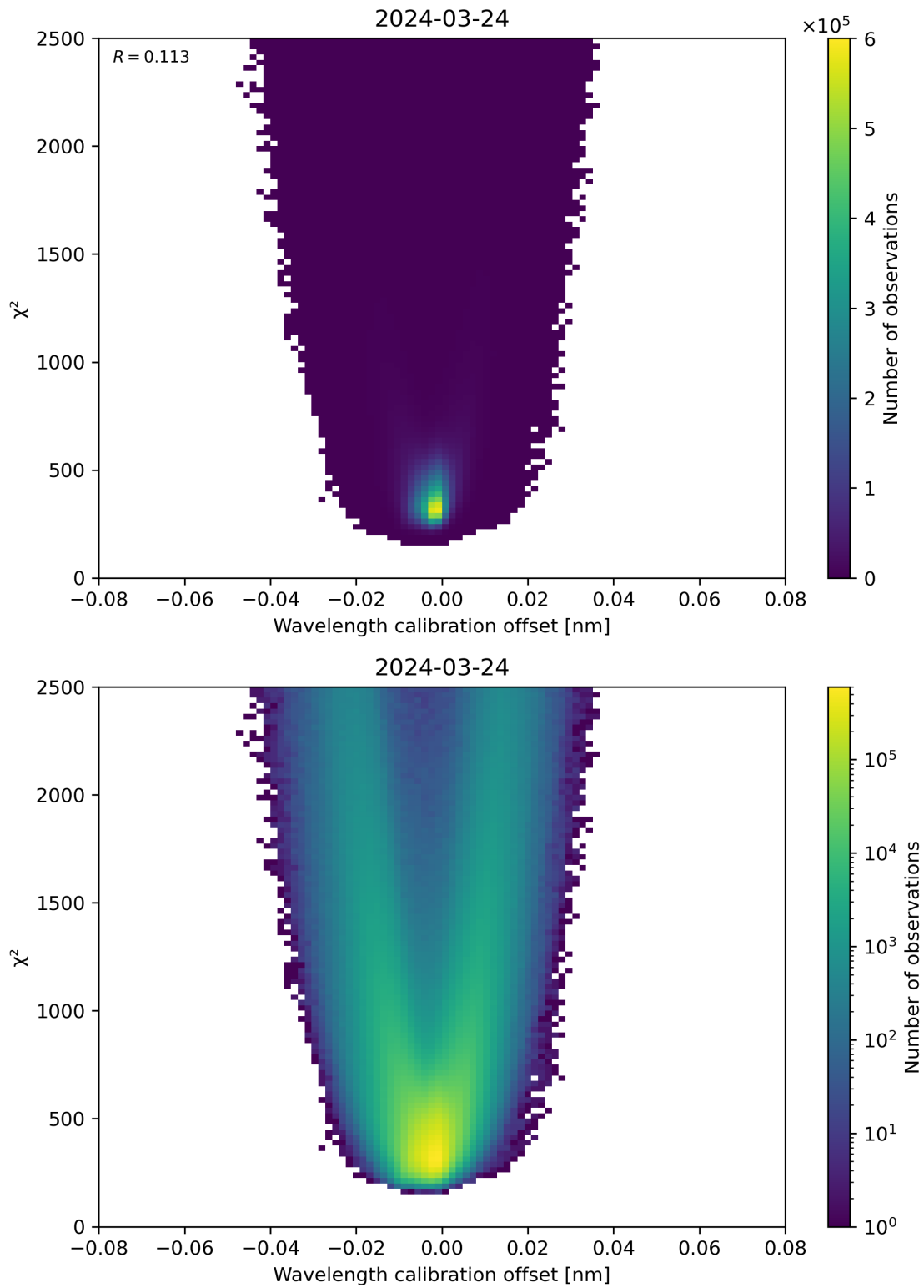
Figure 175: Scatter density plot of “Wavelength calibration offset” against “ \chi^2 ” for 2024-03-23 to 2024-03-25.
