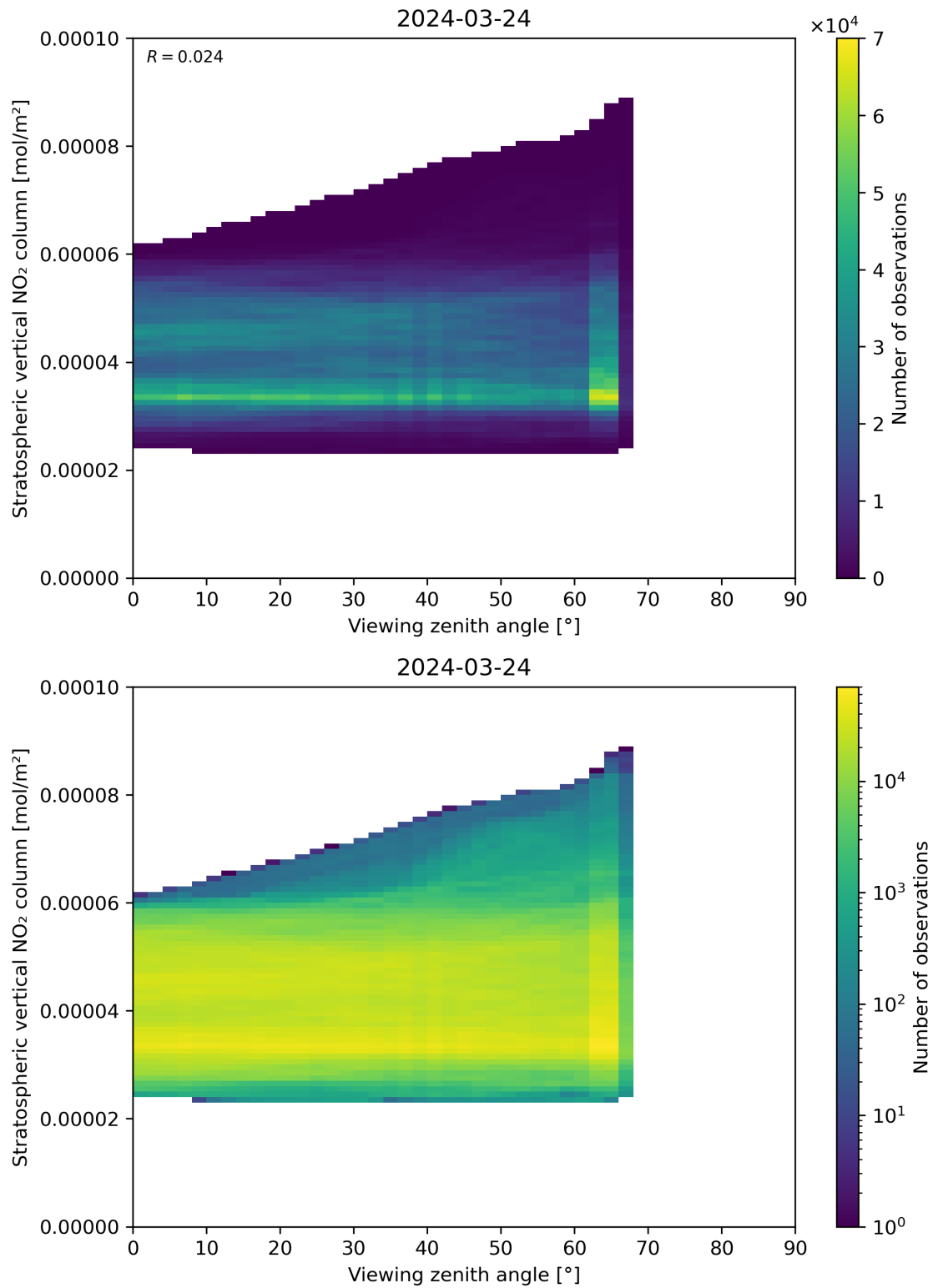
Figure 164: Scatter density plot of “Viewing zenith angle” against “Stratospheric vertical NO 2 column” for 2024-03-23 to 2024-03-25.
