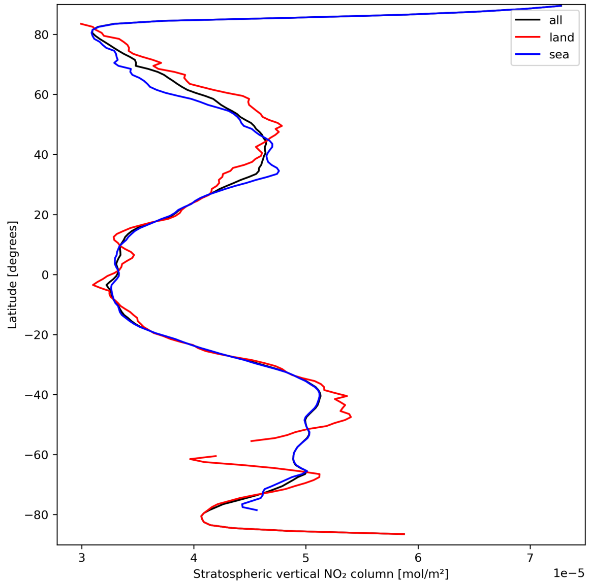
Figure 19: Zonal average of “Stratospheric vertical NO 2 column” for 2024-03-23 to 2024-03-25.
