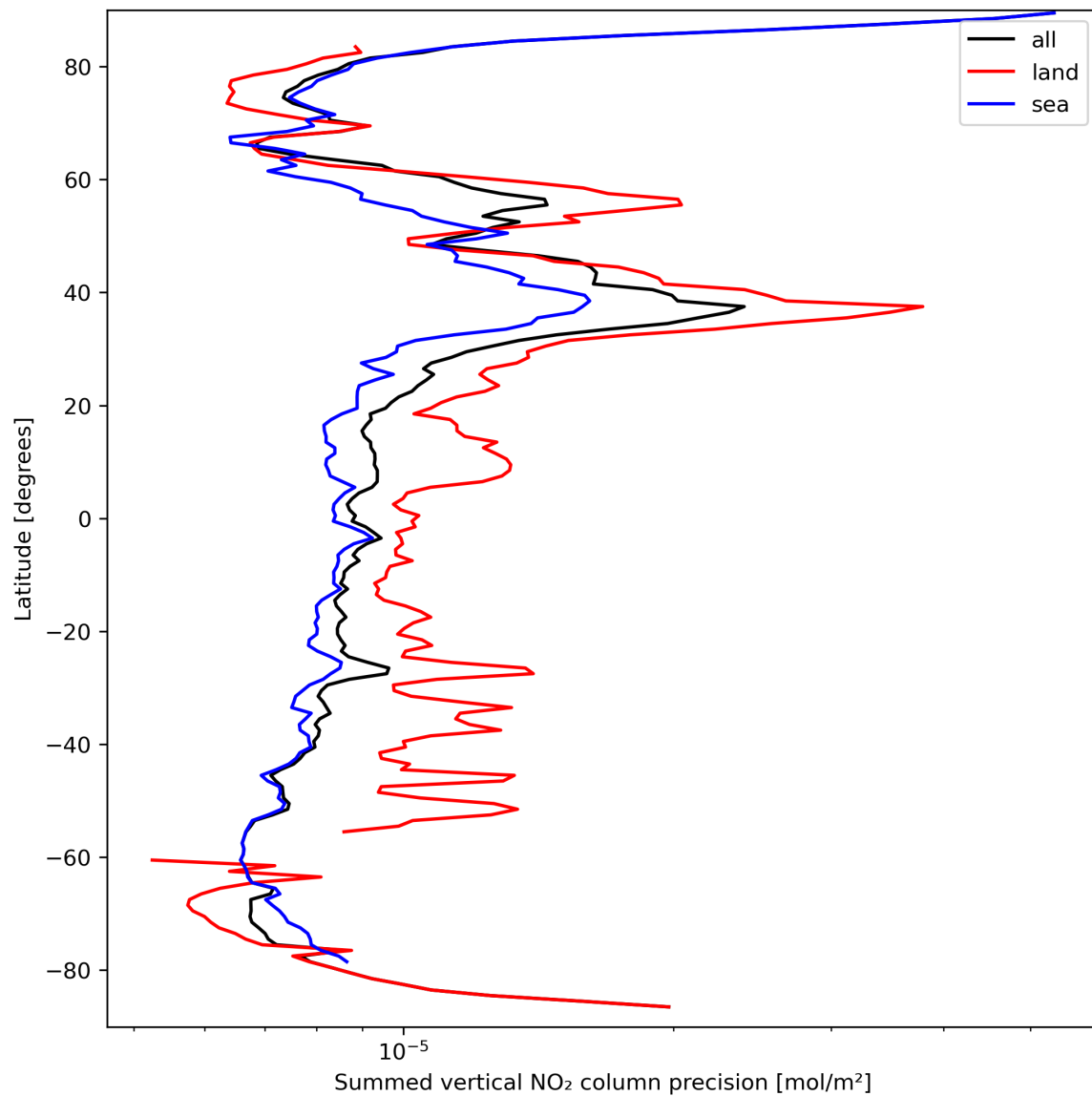
Figure 24: Zonal average of “Summed vertical NO 2 column precision” for 2024-03-23 to 2024-03-25.
