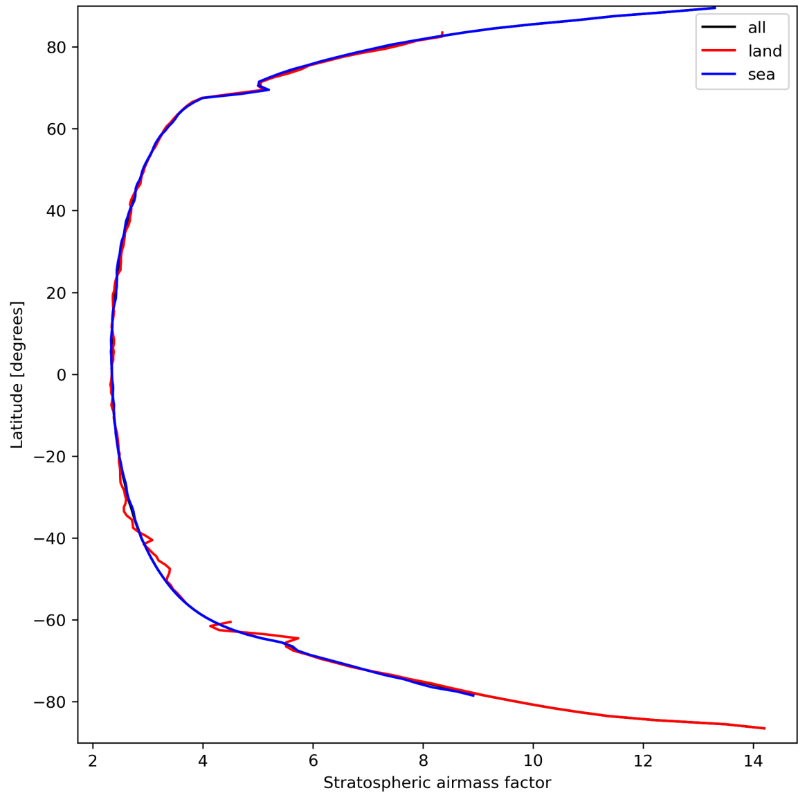
Figure 27: Zonal average of “Stratospheric airmass factor” for 2024-03-23 to 2024-03-25.
