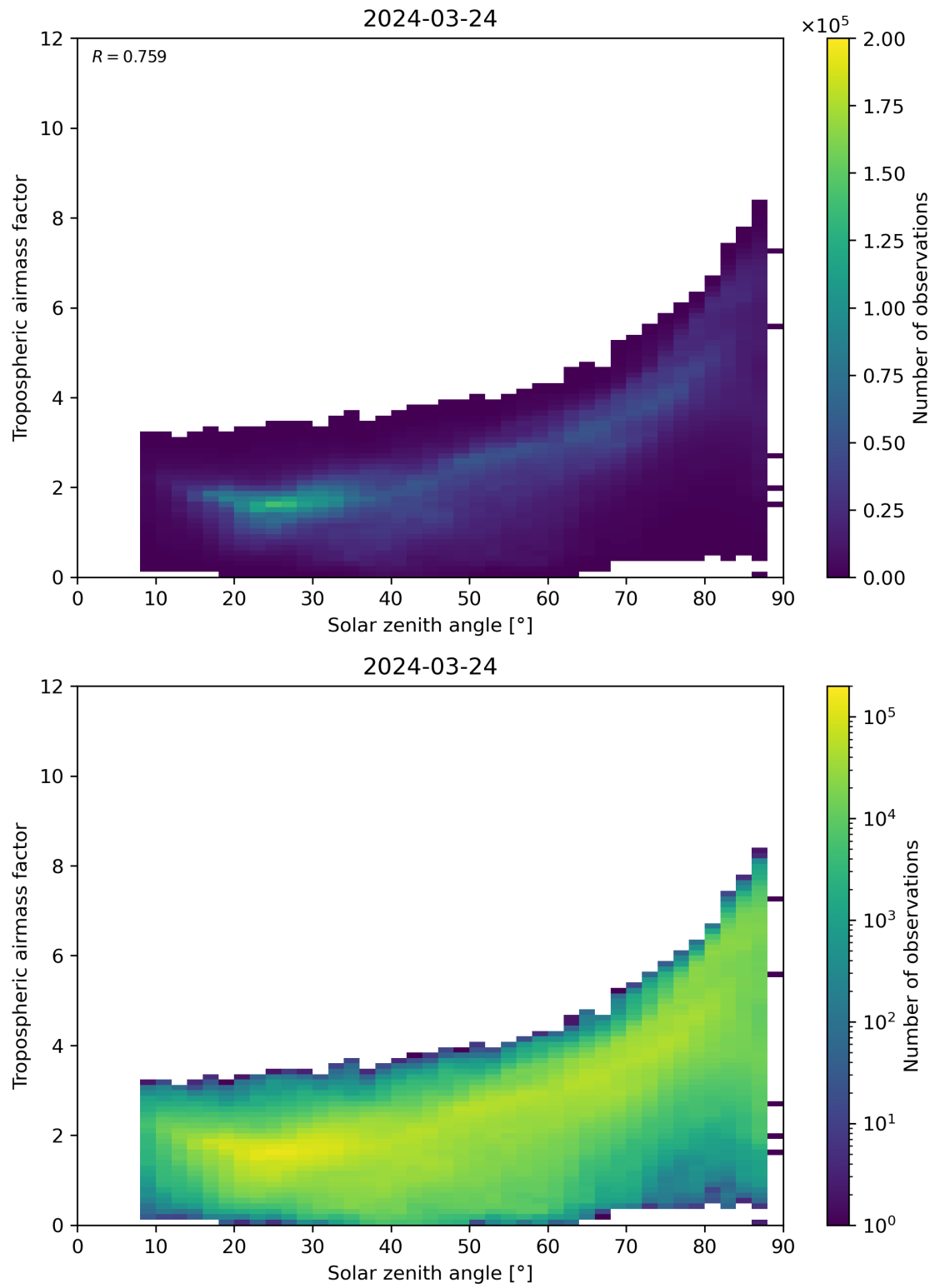
Figure 147: Scatter density plot of “Solar zenith angle” against “Tropospheric airmass factor” for 2024-03-23 to 2024-03-25.
