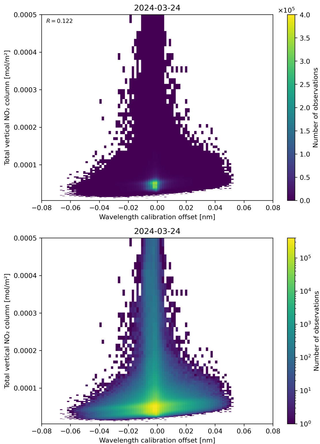
Figure 179: Scatter density plot of “Wavelength calibration offset” against “Total vertical NO 2 column” for 2024-03-23 to 2024-03-25.
