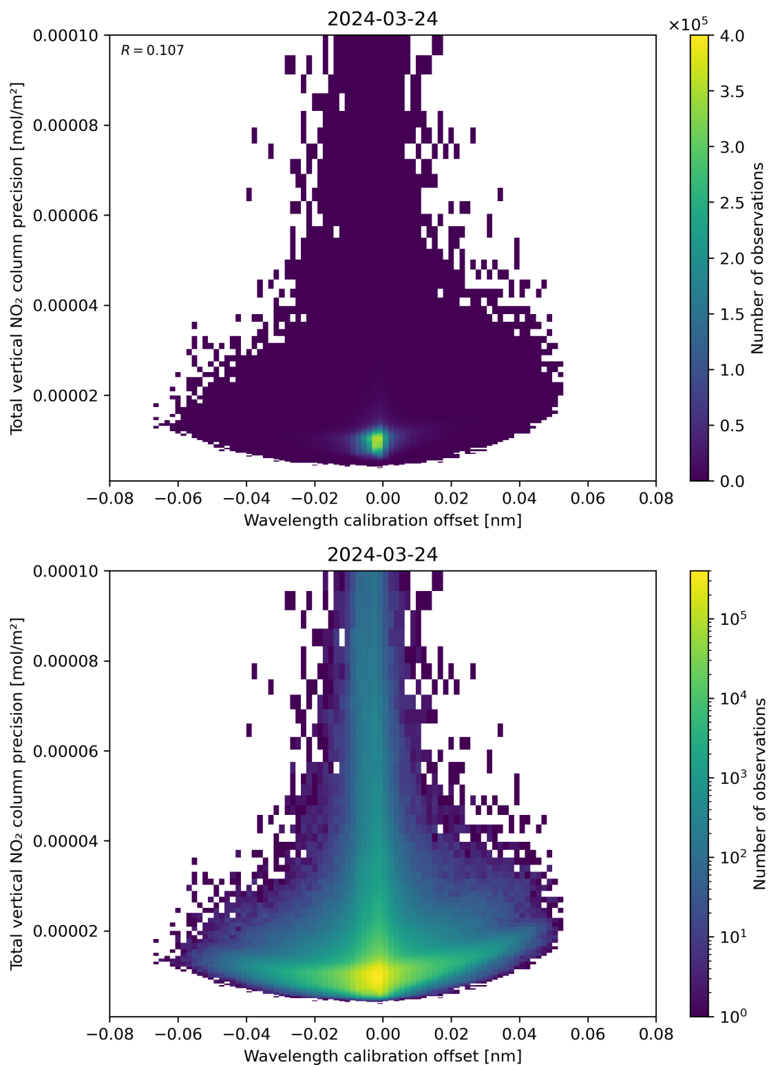
Figure 180: Scatter density plot of “Wavelength calibration offset” against “Total vertical NO 2 column precision” for 2024-03-23 to 2024-03-25.
