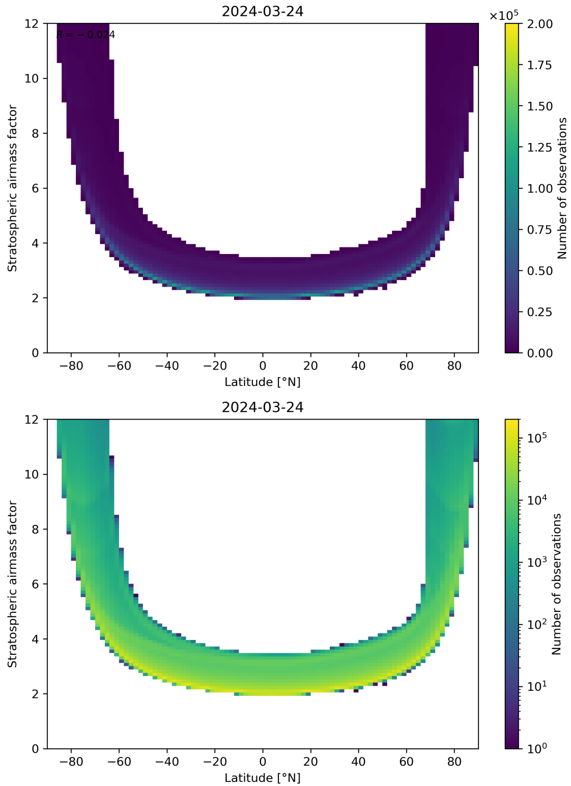
Figure 83: Scatter density plot of “Latitude” against “Stratospheric air mass factor” for 2024-03-23 to 2024-03-25.
