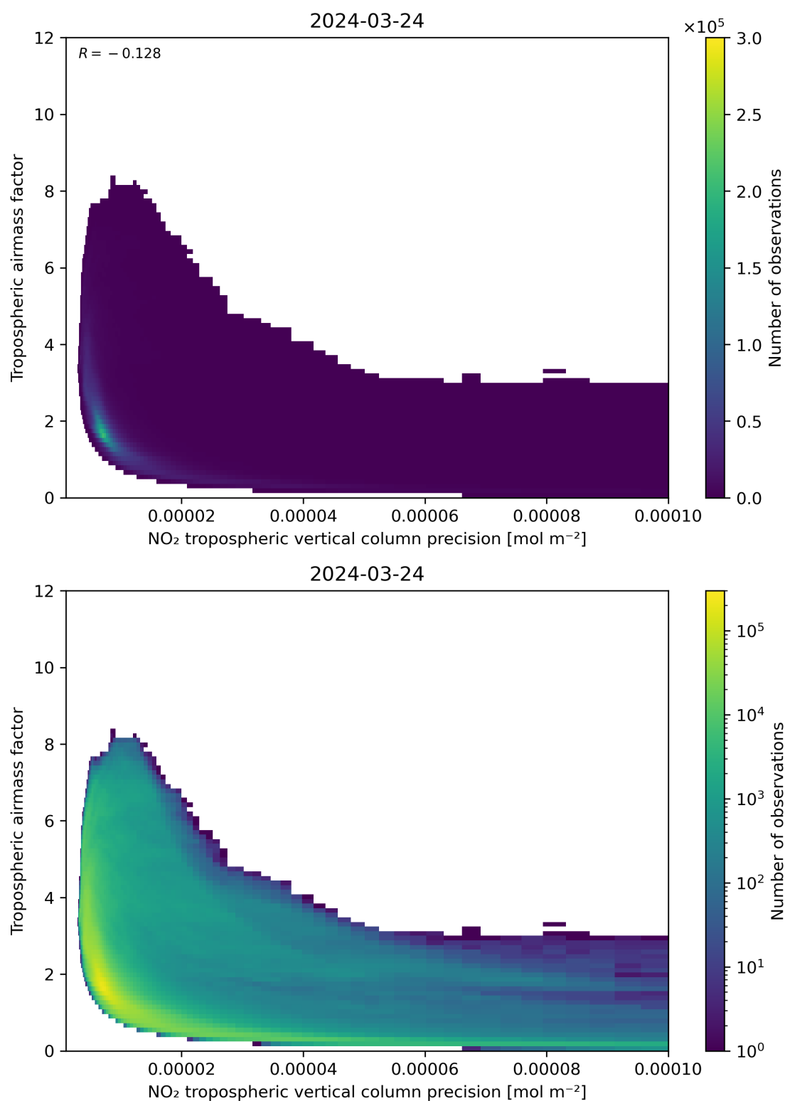
Figure 133: Scatter density plot of “NO 2 tropospheric vertical column precision” against “Tropospheric airmass factor” for 2024-03-23 to 2024-03-25.
