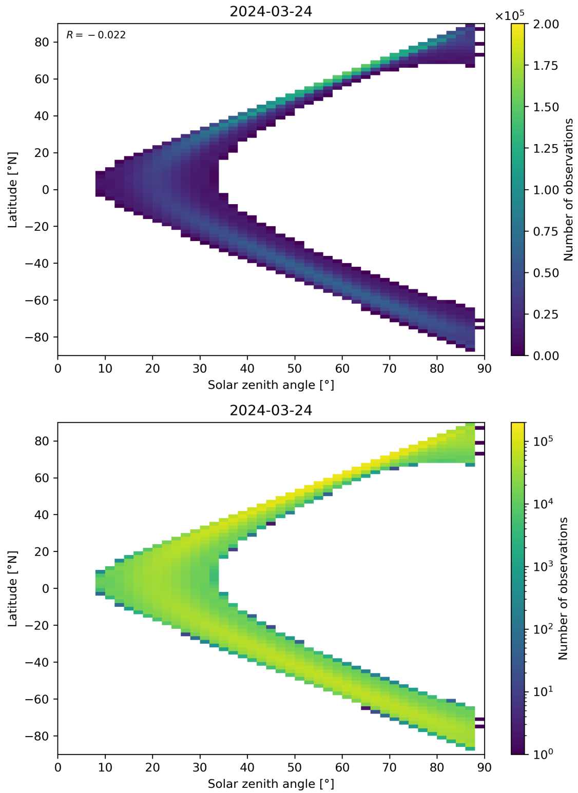
Figure 149: Scatter density plot of “Solar zenith angle” against “Latitude” for 2024-03-23 to 2024-03-25.
