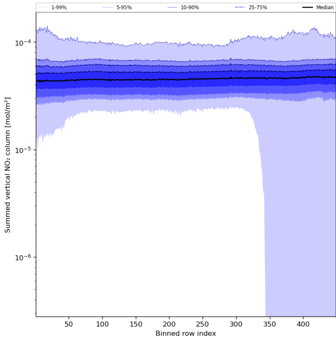
Figure 57: Along track statistics of “Summed vertical NO 2 column” for 2024-03-23 to 2024-03-25
