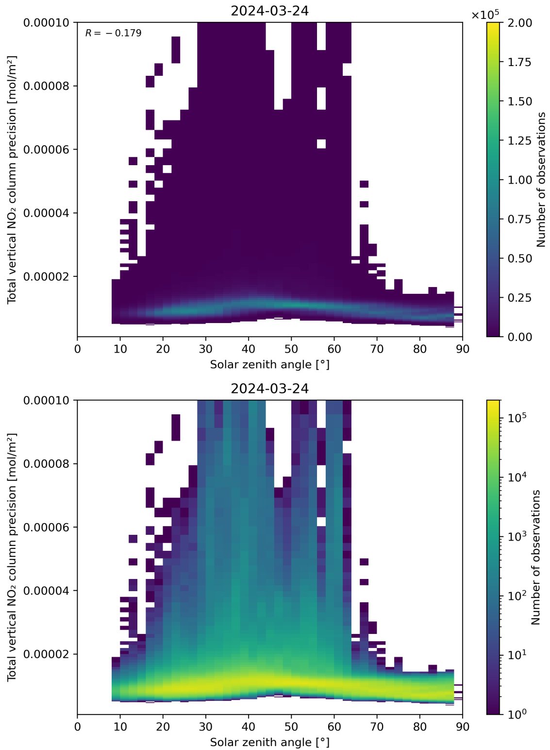
Figure 154: Scatter density plot of “Solar zenith angle” against “Total vertical NO 2 column precision” for 2024-03-23 to 2024-03-25.
