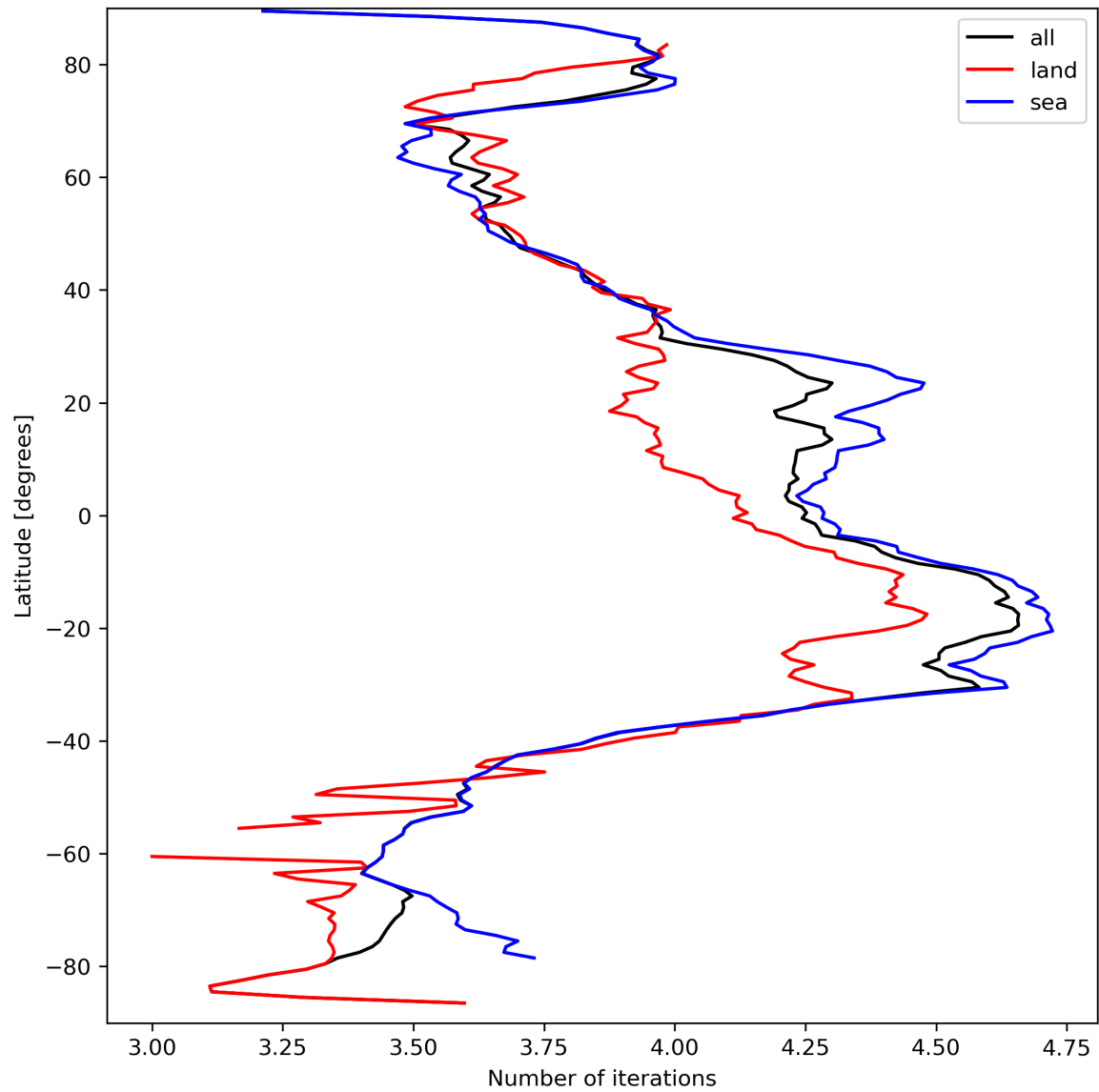
Figure 17: Zonal average of “Number of iterations” for 2024-03-23 to 2024-03-25.
