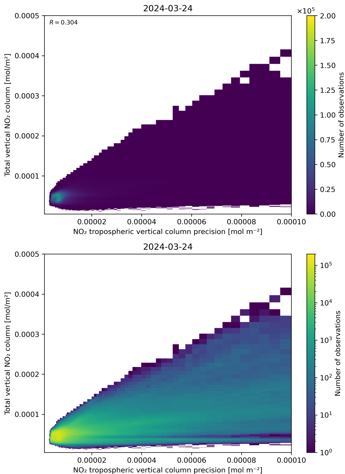
Figure 138: Scatter density plot of “NO 2 tropospheric vertical column precision” against “Total vertical NO 2 column” for 2024-03-23 to 2024-03-25.
