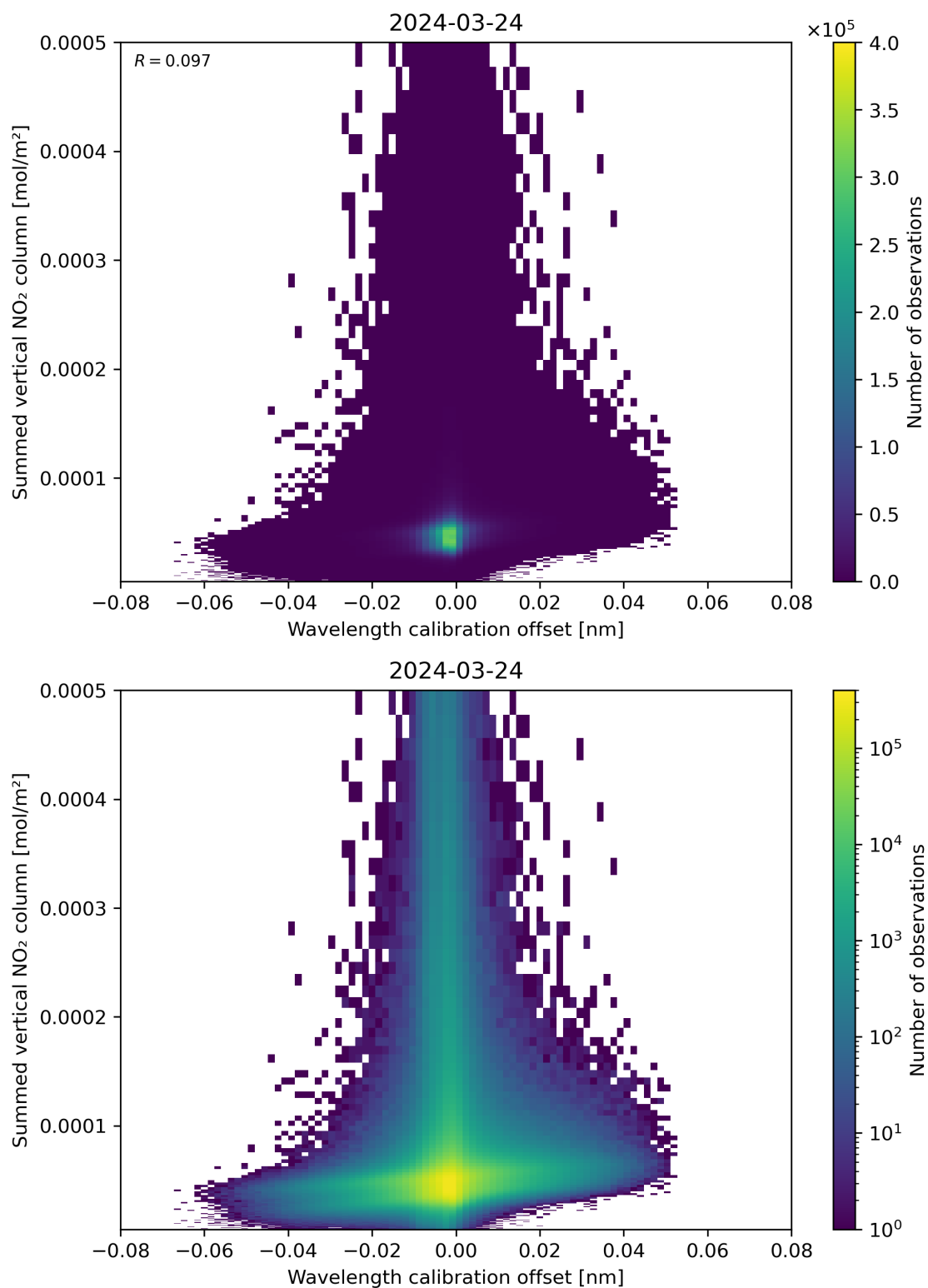
Figure 177: Scatter density plot of “Wavelength calibration offset” against “Summed vertical NO 2 column” for 2024-03-23 to 2024-03-25.
