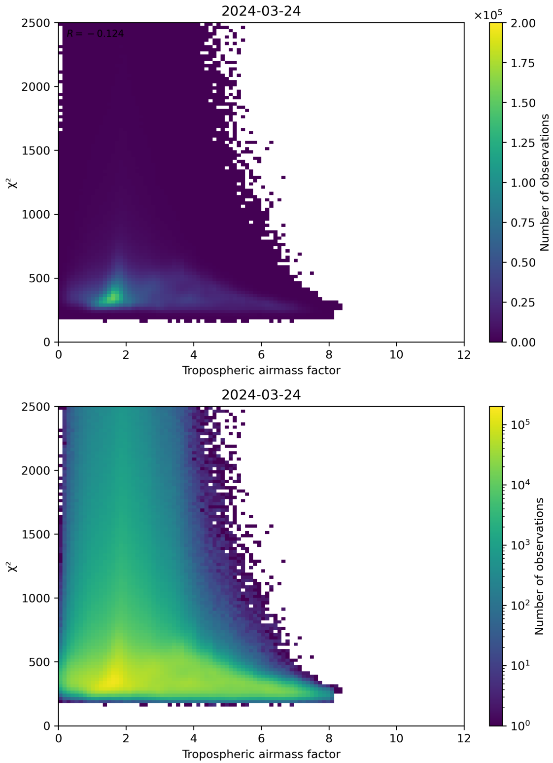
Figure 73: Scatter density plot of “Tropospheric airmass factor” against “ \chi^2 ” for 2024-03-23 to 2024-03-25.
