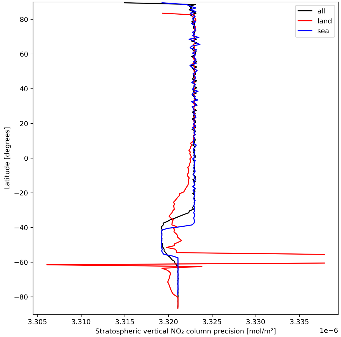
Figure 20: Zonal average of “Stratospheric vertical NO 2 column precision” for 2024-03-23 to 2024-03-25.
