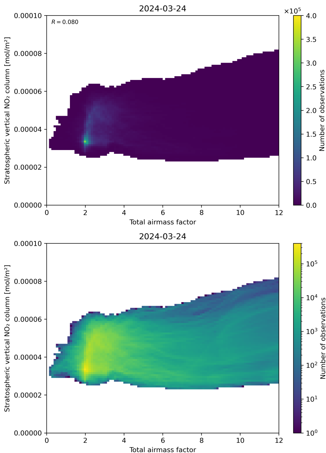
Figure 64: Scatter density plot of “Total airmass factor” against “Stratospheric vertical \text{NO}_2 column” for 2024-03-23 to 2024-03-25.
