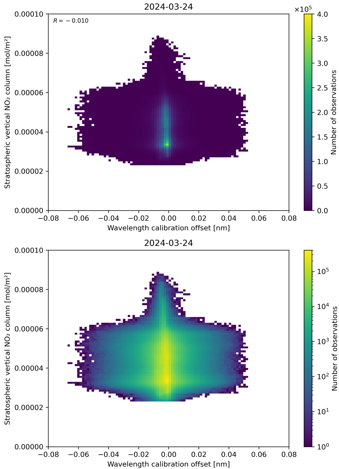
Figure 176: Scatter density plot of “Wavelength calibration offset” against “Stratospheric vertical NO 2 column” for 2024-03-23 to 2024-03-25.
