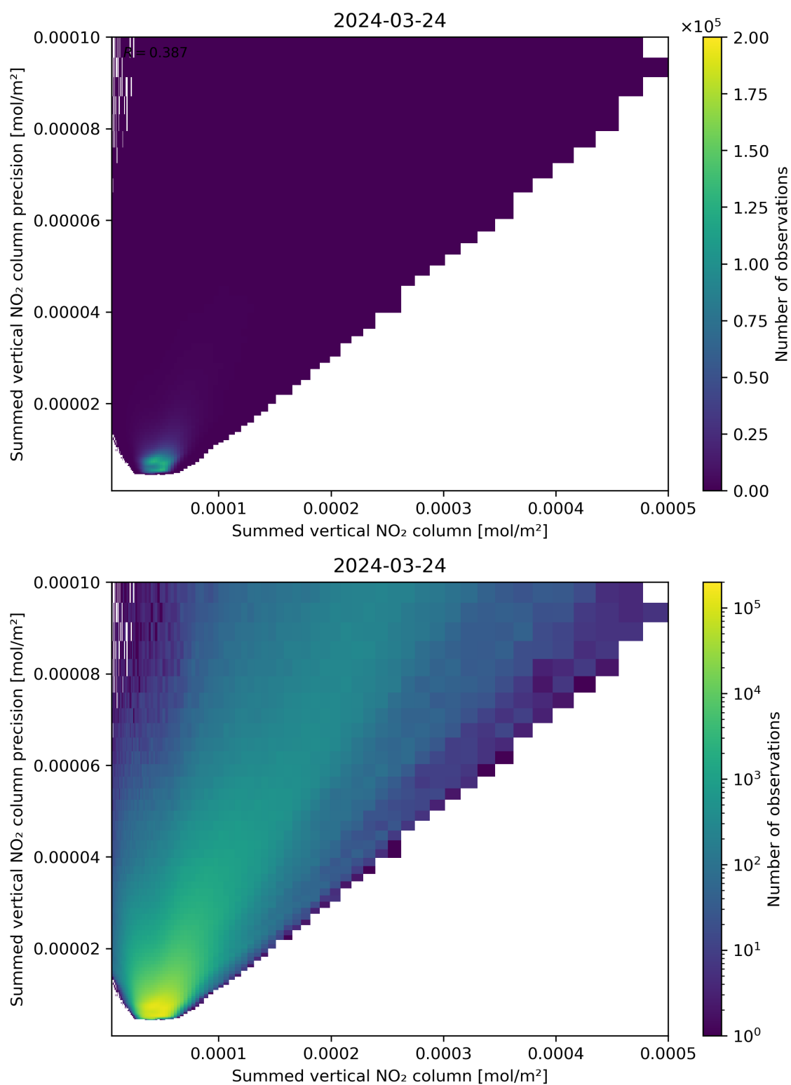
Figure 105: Scatter density plot of “Summed vertical NO 2 column” against “Summed vertical NO 2 column precision” for 2024-03-23 to 2024-03-25.
