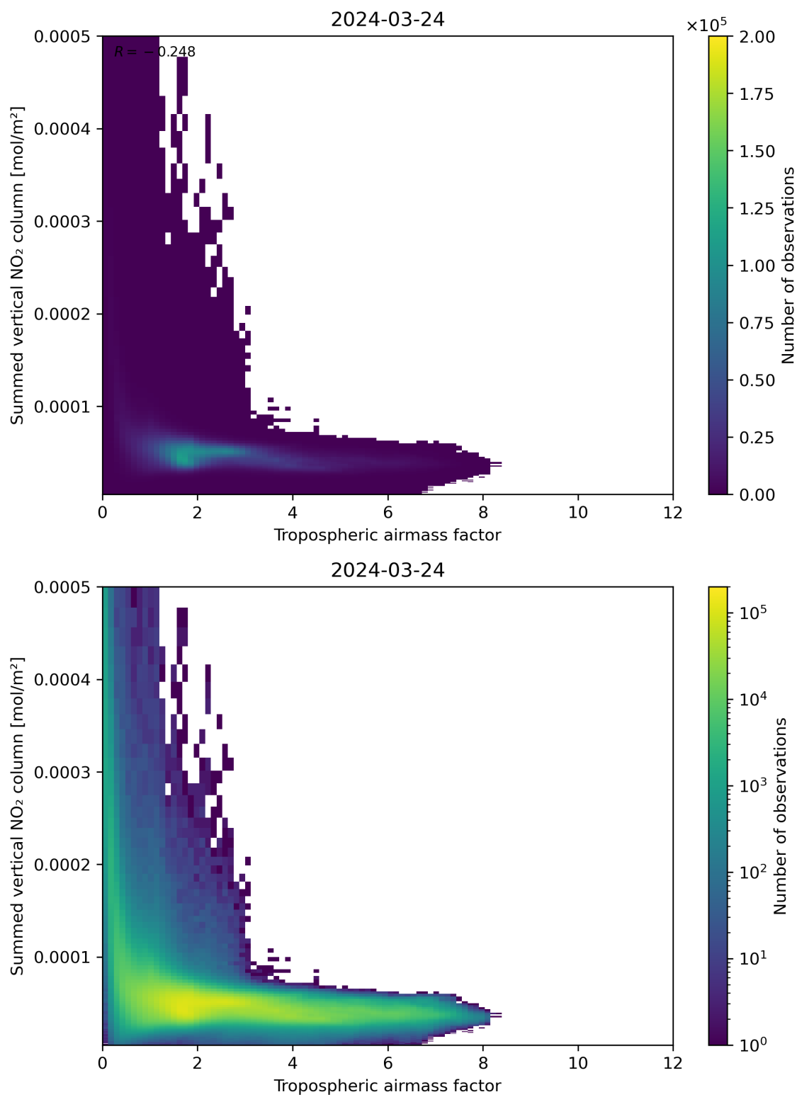
Figure 75: Scatter density plot of “Tropospheric airmass factor” against “Summed vertical NO 2 column” for 2024-03-23 to 2024-03-25.
