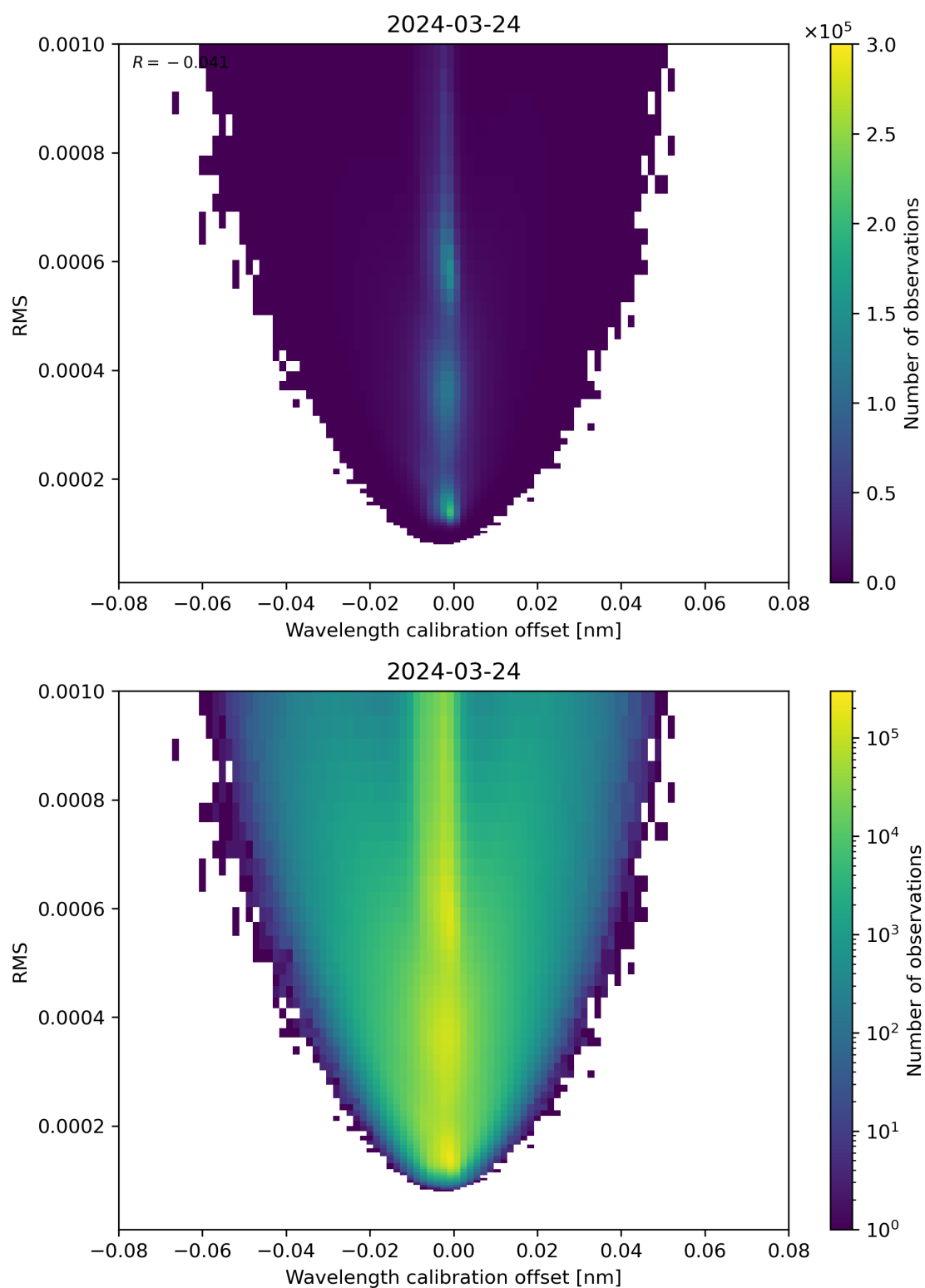
Figure 181: Scatter density plot of “Wavelength calibration offset” against “RMS” for 2024-03-23 to 2024-03-25.
