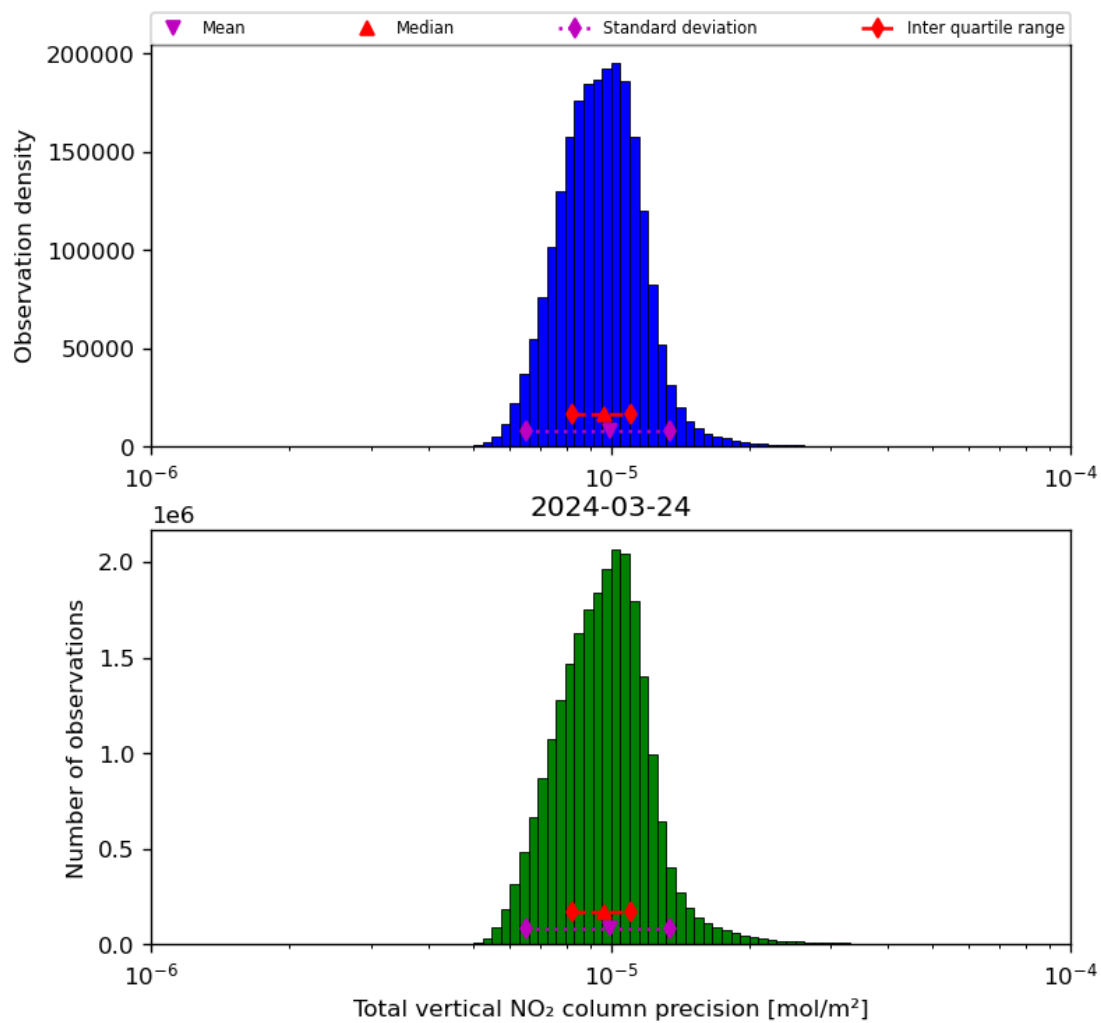
Figure 39: Histogram of “Total vertical NO 2 column precision” for 2024-03-23 to 2024-03-25
