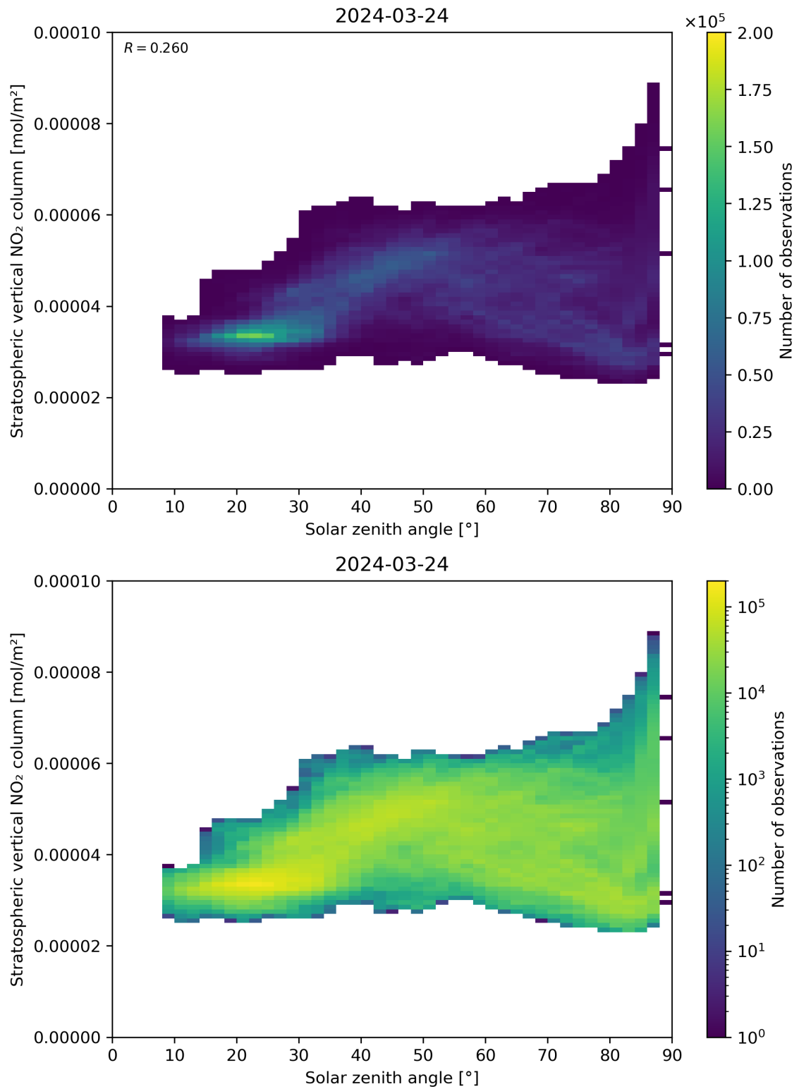
Figure 150: Scatter density plot of “Solar zenith angle” against “Stratospheric vertical NO 2 column” for 2024-03-23 to 2024-03-25.
