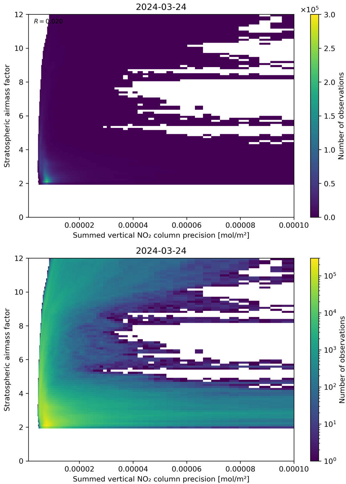
Figure 106: Scatter density plot of “Summed vertical NO 2 column precision” against “Stratospheric airmass factor” for 2024-03-23 to 2024-03-25.
