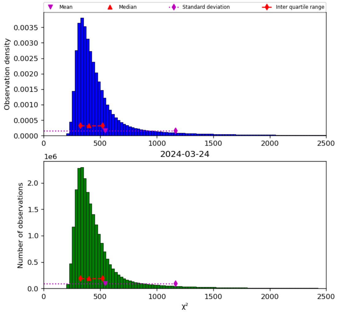
Figure 42: Histogram of “ \chi^2 ” for 2024-03-23 to 2024-03-25
