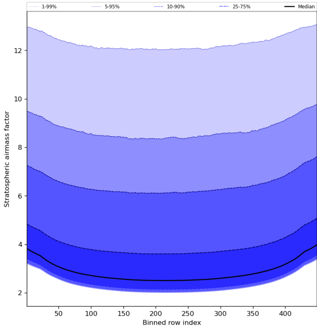
Figure 61: Along track statistics of “Stratospheric airmass factor” for 2024-03-23 to 2024-03-25
