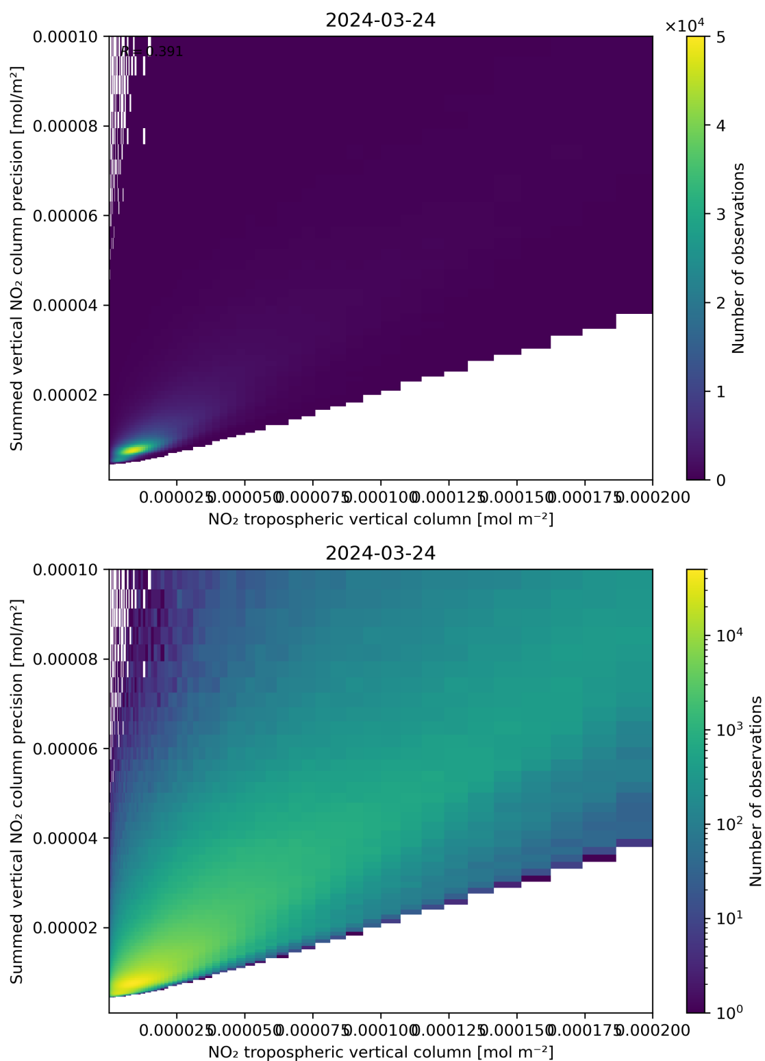
Figure 127: Scatter density plot of “NO 2 tropospheric vertical column” against “Summed vertical NO 2 column precision” for 2024-03-23 to 2024-03-25.
