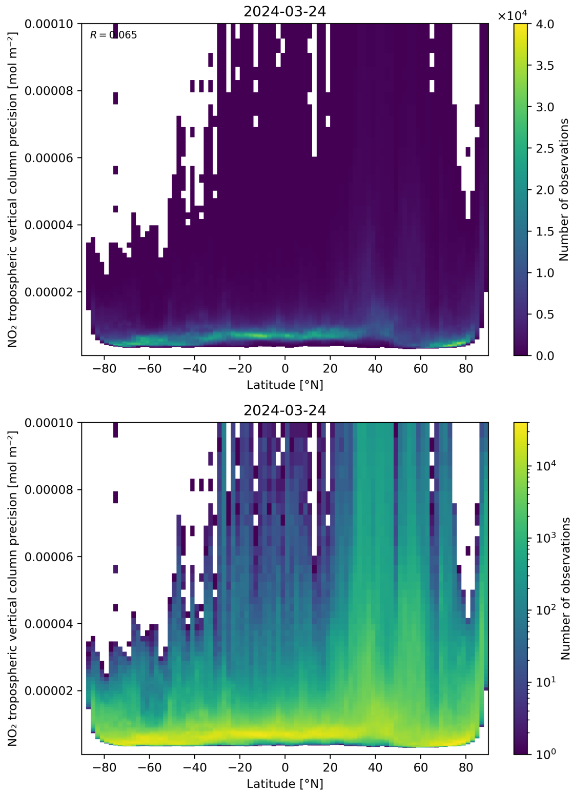
Figure 93: Scatter density plot of “Latitude” against “NO 2 tropospheric vertical column precision” for 2024-03-23 to 2024-03-25.
