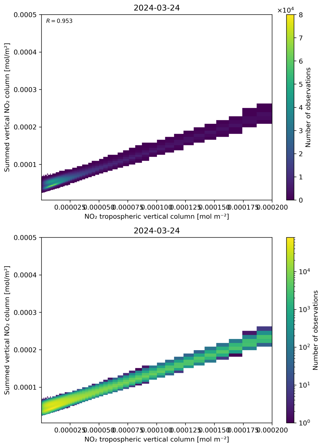
Figure 126: Scatter density plot of “NO 2 tropospheric vertical column” against “Summed vertical NO 2 column” for 2024-03-23 to 2024-03-25.
