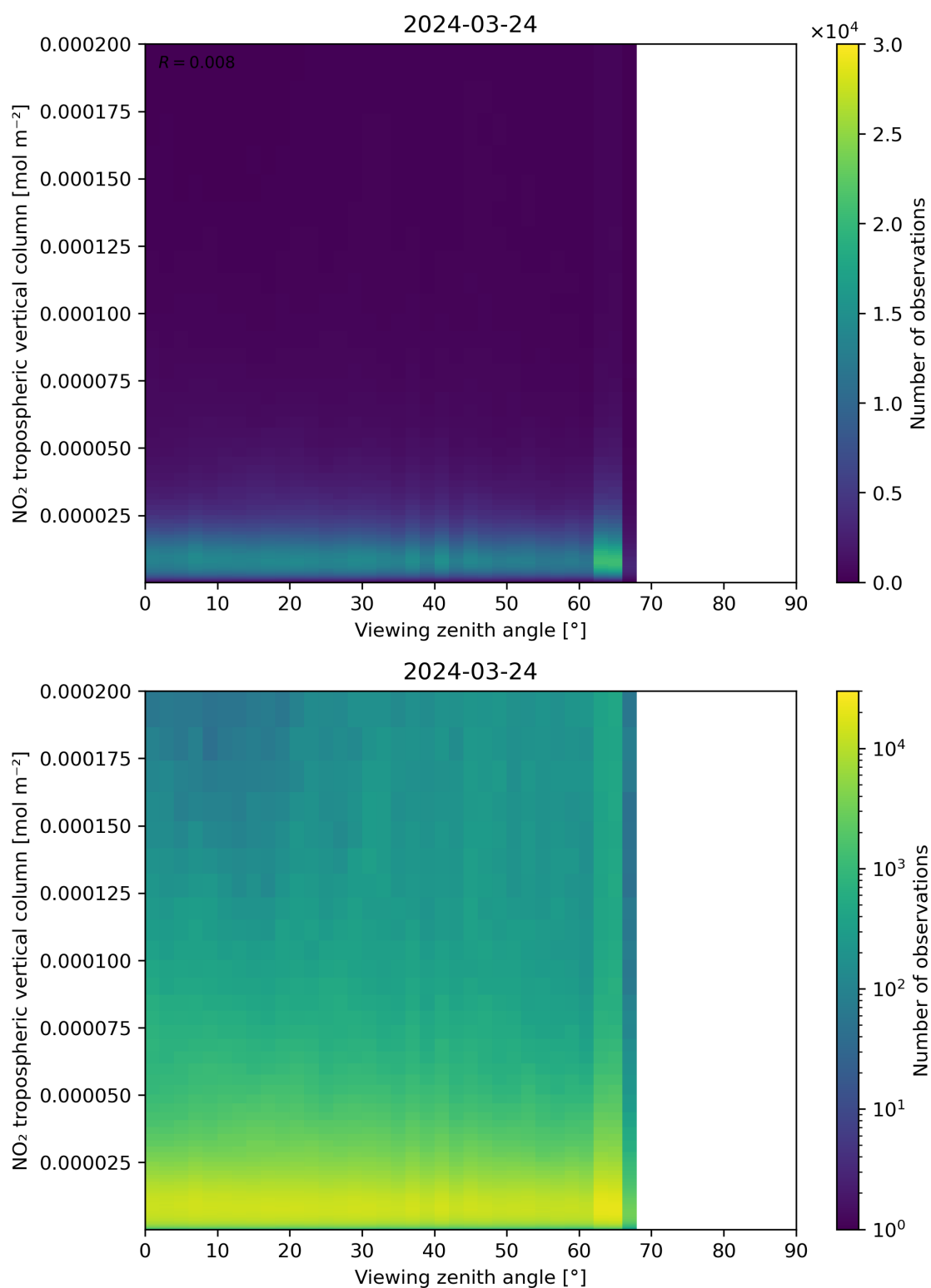
Figure 169: Scatter density plot of “Viewing zenith angle” against “NO 2 tropospheric vertical column” for 2024-03-23 to 2024-03-25.
