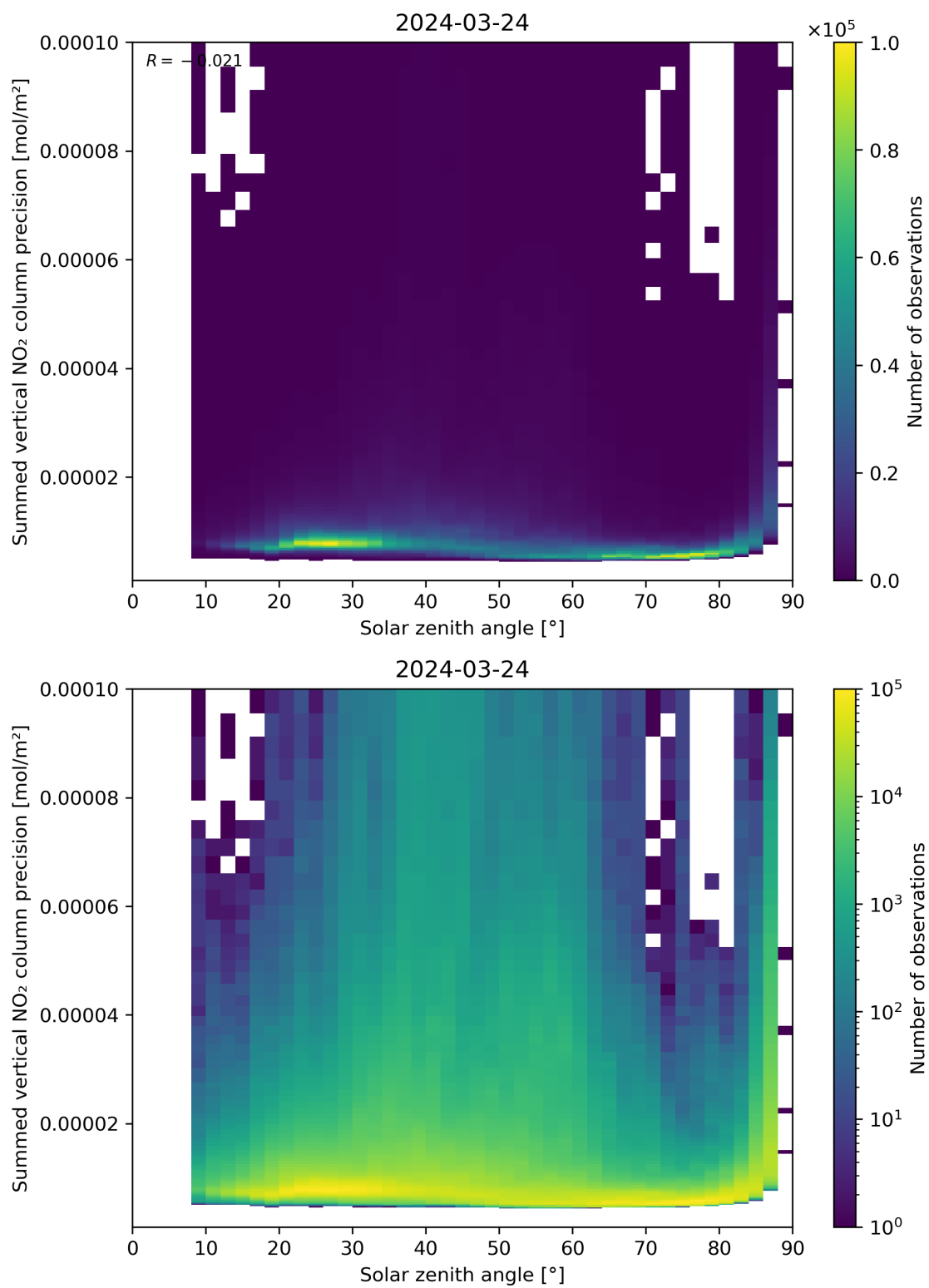
Figure 152: Scatter density plot of “Solar zenith angle” against “Summed vertical NO 2 column precision” for 2024-03-23 to 2024-03-25.
