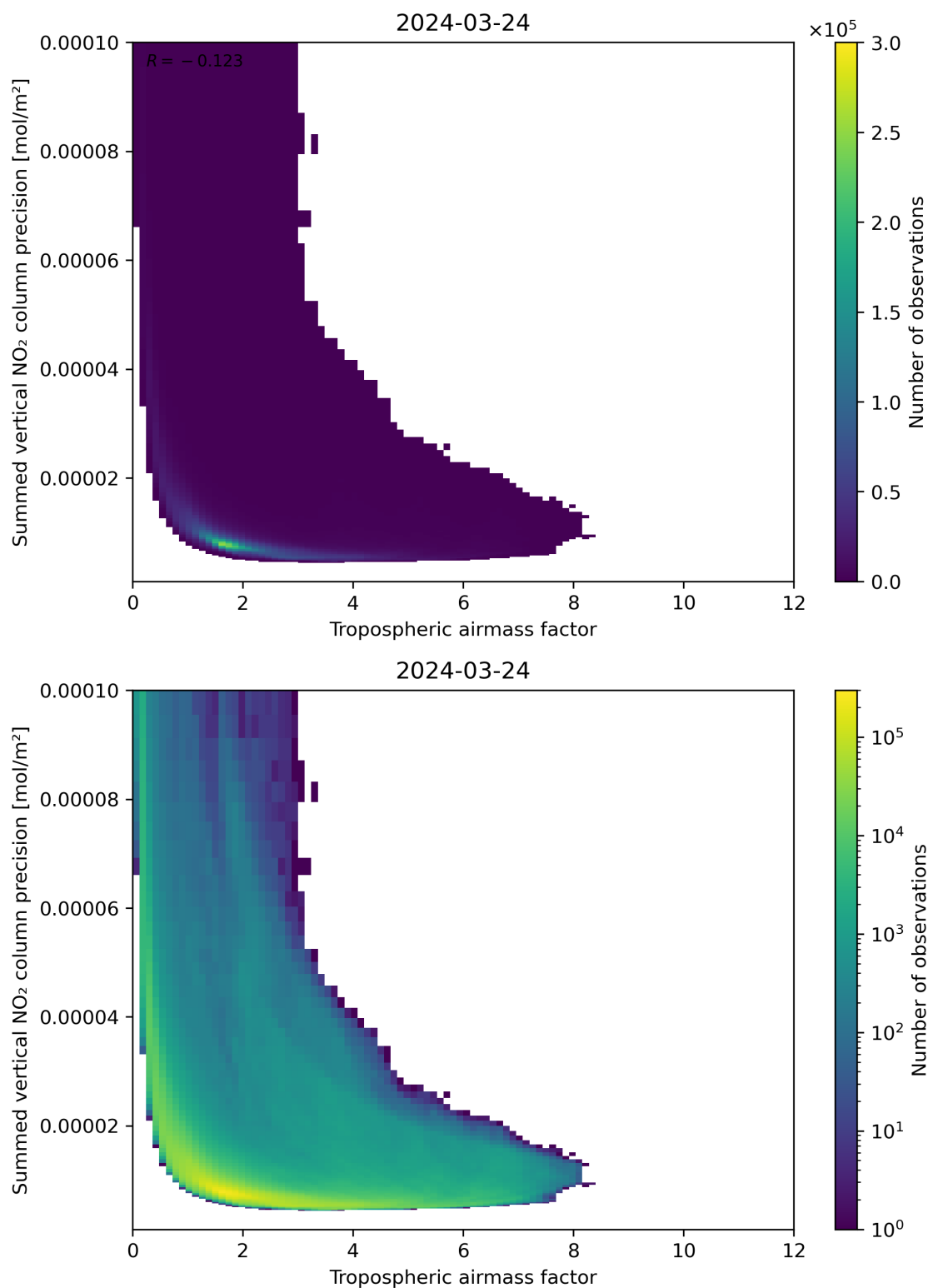
Figure 76: Scatter density plot of “Tropospheric air mass factor” against “Summed vertical NO 2 column precision” for 2024-03-23 to 2024-03-25.
