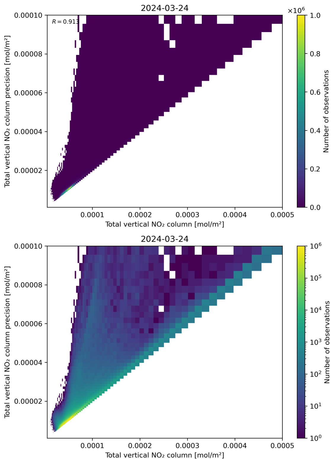
Figure 114: Scatter density plot of “Total vertical NO 2 column” against “Total vertical NO 2 column precision” for 2024-03-23 to 2024-03-25.
