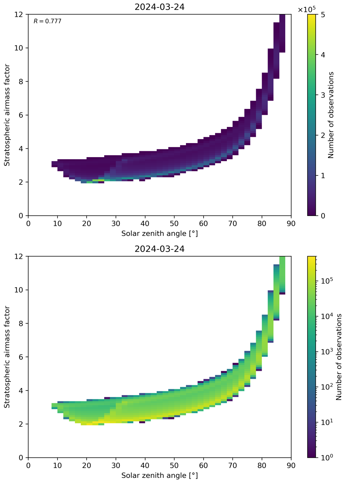
Figure 145: Scatter density plot of “Solar zenith angle” against “Stratospheric airmass factor” for 2024-03-23 to 2024-03-25.
