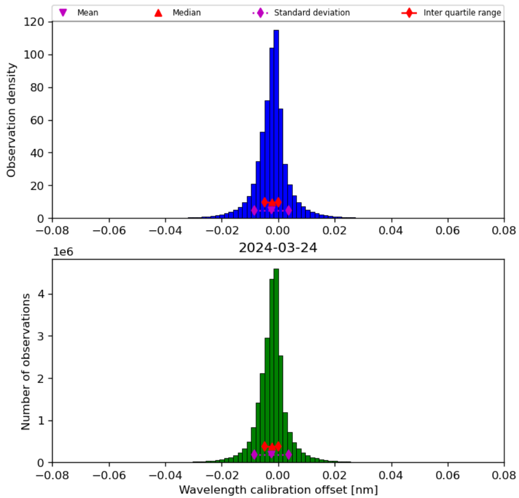
Figure 35: Histogram of “Wavelength calibration offset” for 2024-03-23 to 2024-03-25
