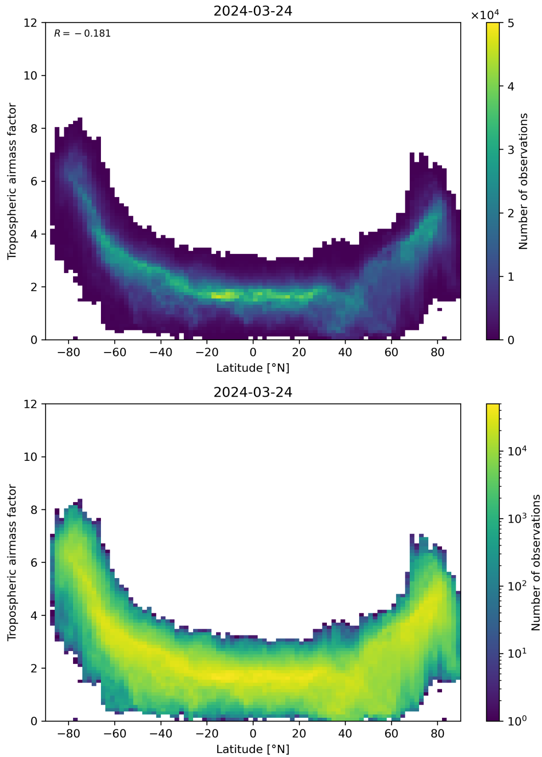
Figure 85: Scatter density plot of “Latitude” against “Tropospheric airmass factor” for 2024-03-23 to 2024-03-25.
