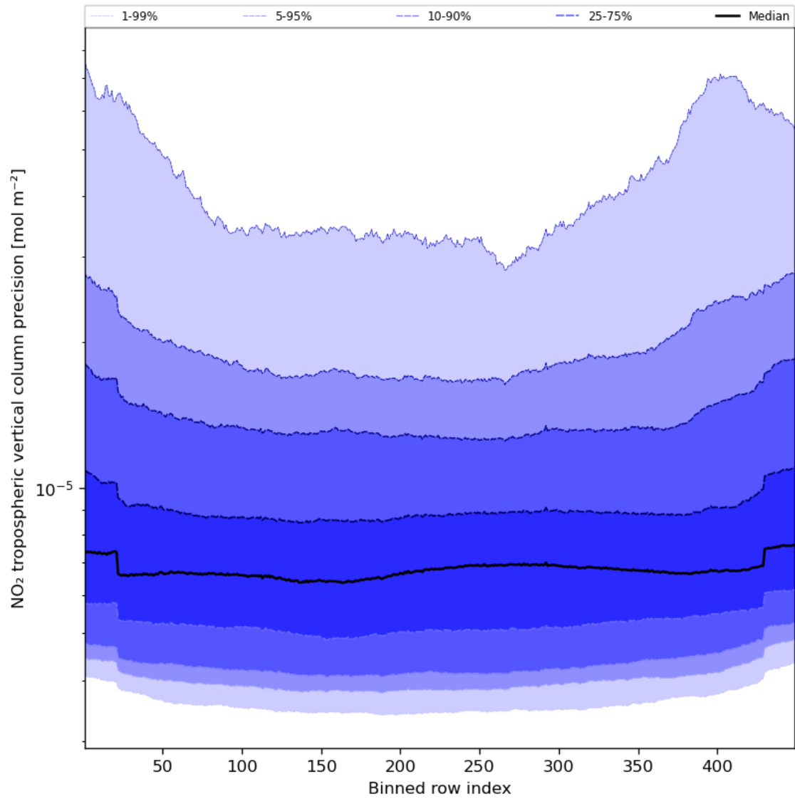
Figure 47: Along track statistics of “NO 2 tropospheric vertical column precision” for 2024-03-23 to 2024-03-25
