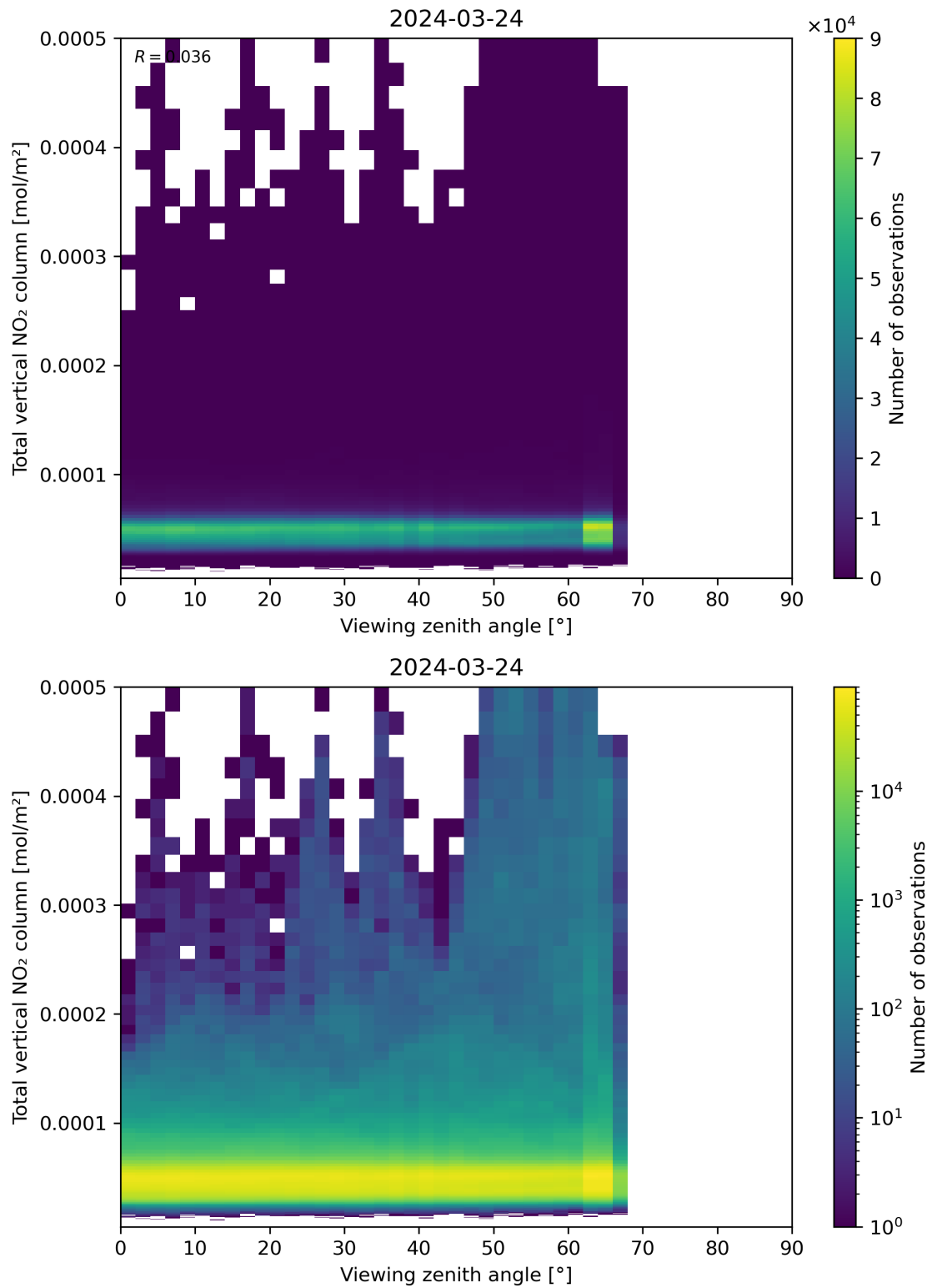
Figure 167: Scatter density plot of “Viewing zenith angle” against “Total vertical NO 2 column” for 2024-03-23 to 2024-03-25.
