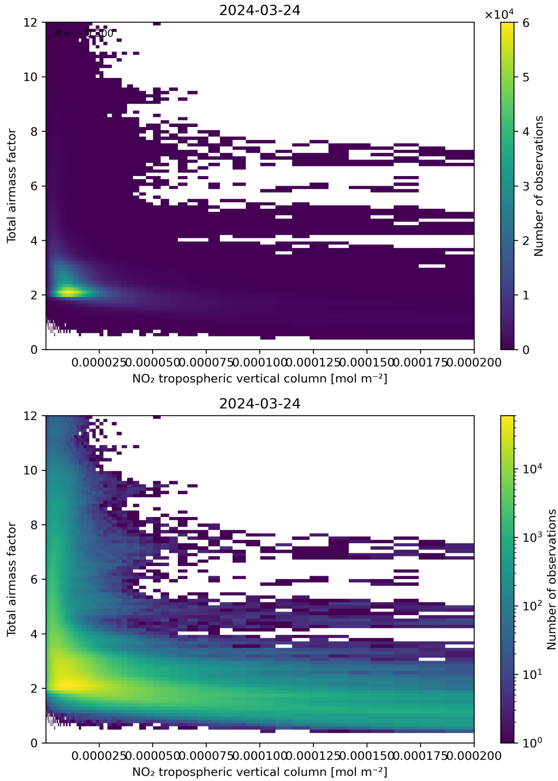
Figure 122: Scatter density plot of “NO 2 tropospheric vertical column” against “Total air mass factor” for 2024-03-23 to 2024-03-25.
