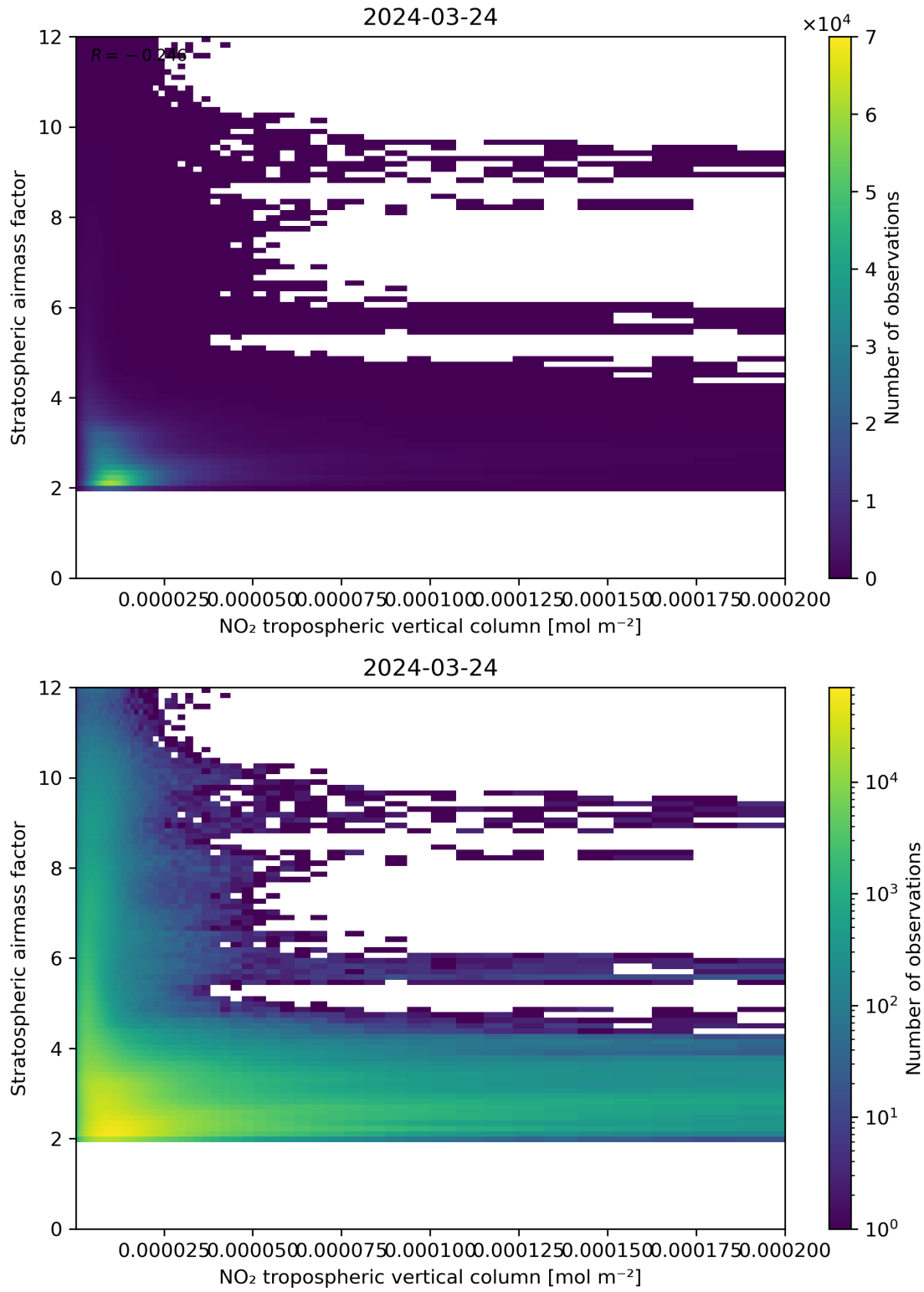
Figure 121: Scatter density plot of “NO 2 tropospheric vertical column” against “Stratospheric airmass factor” for 2024-03-23 to 2024-03-25.
