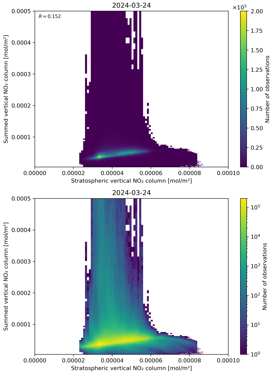
Figure 98: Scatter density plot of “Stratospheric vertical NO 2 column” against “Summed vertical NO 2 column” for 2024-03-23 to 2024-03-25.
