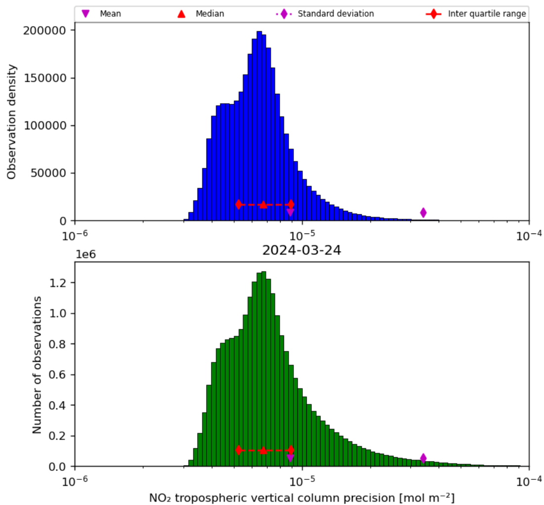
Figure 30: Histogram of “NO 2 tropospheric vertical column precision” for 2024-03-23 to 2024-03-25
