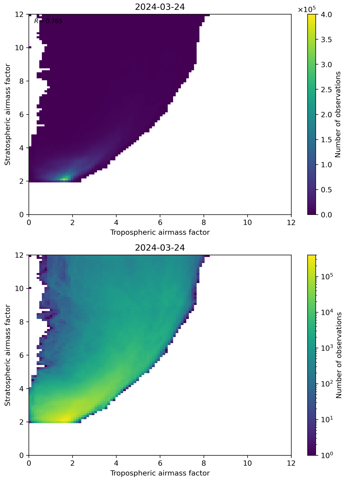
Figure 71: Scatter density plot of “Tropospheric airmass factor” against “Stratospheric airmass factor” for 2024-03-23 to 2024-03-25.
