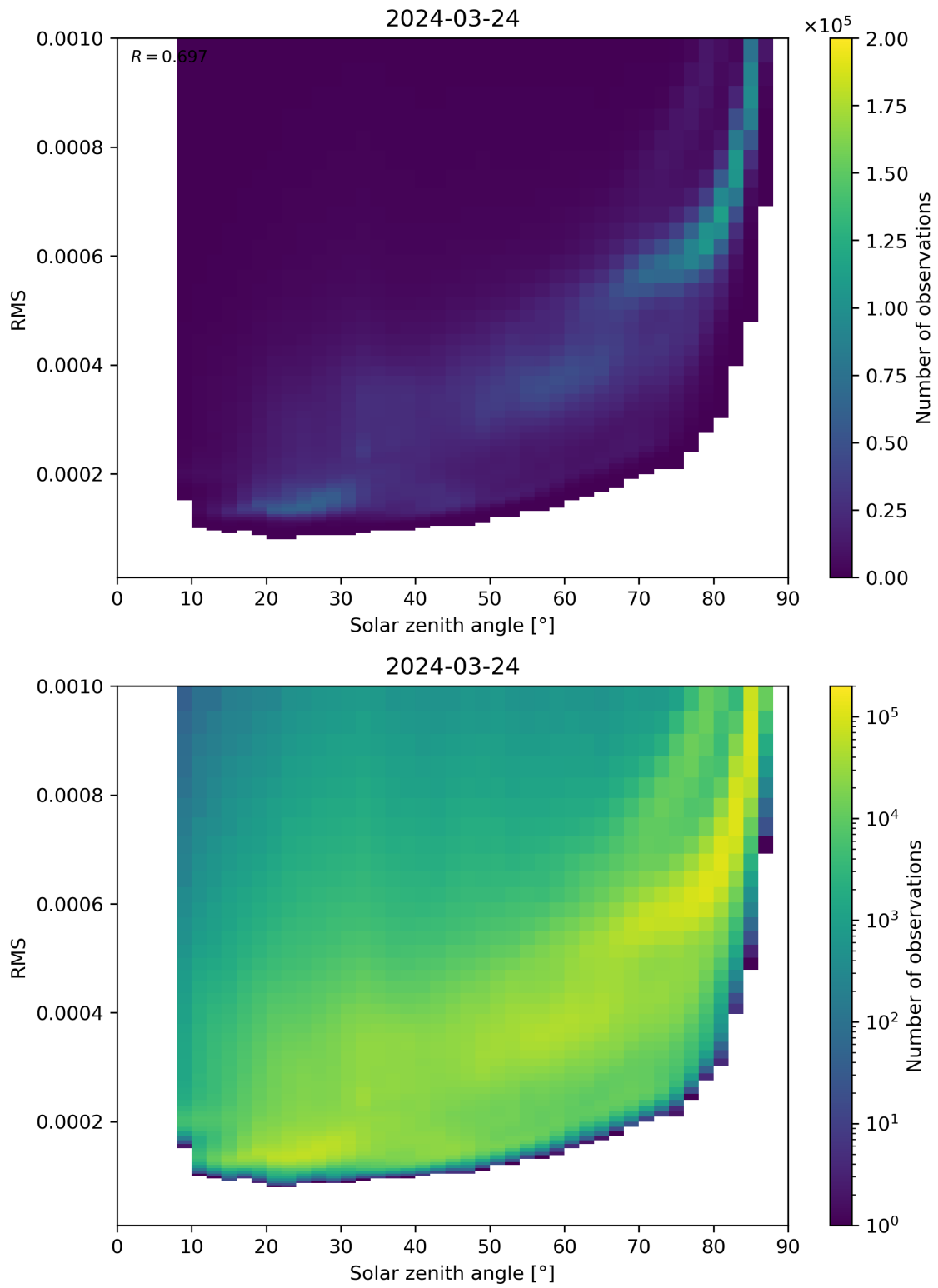
Figure 157: Scatter density plot of “Solar zenith angle” against “RMS” for 2024-03-23 to 2024-03-25.
