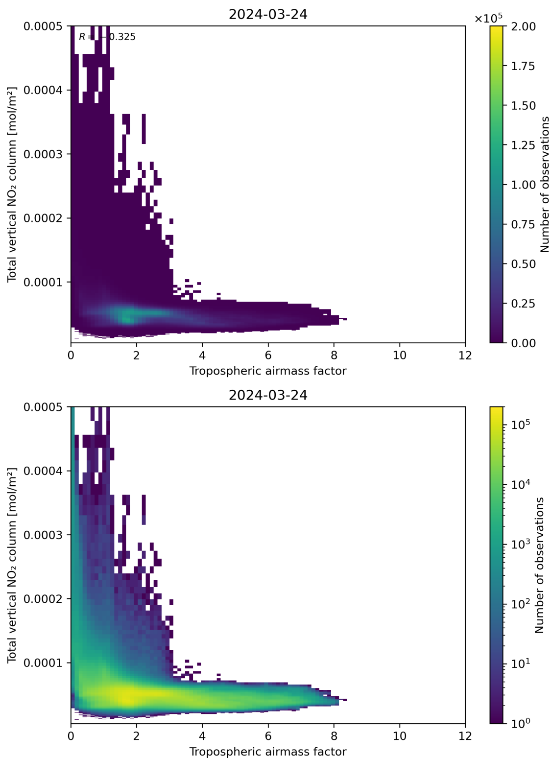
Figure 77: Scatter density plot of “Tropospheric airmass factor” against “Total vertical NO 2 column” for 2024-03-23 to 2024-03-25.
