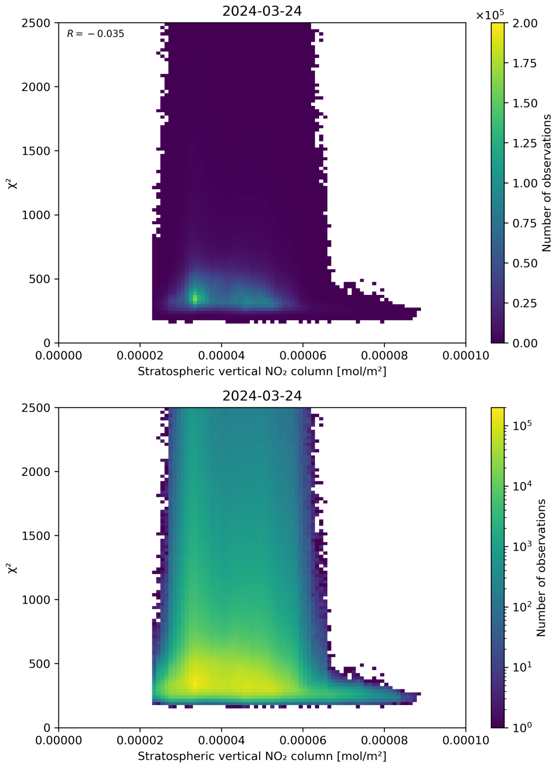
Figure 97: Scatter density plot of “Stratospheric vertical NO 2 column” against “ \chi^2 ” for 2024-03-23 to 2024-03-25.
