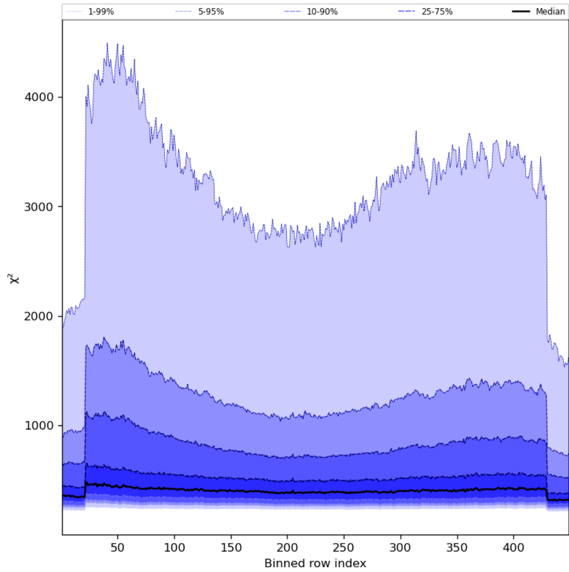
Figure 59: Along track statistics of “ \chi^2 ” for 2024-03-23 to 2024-03-25
