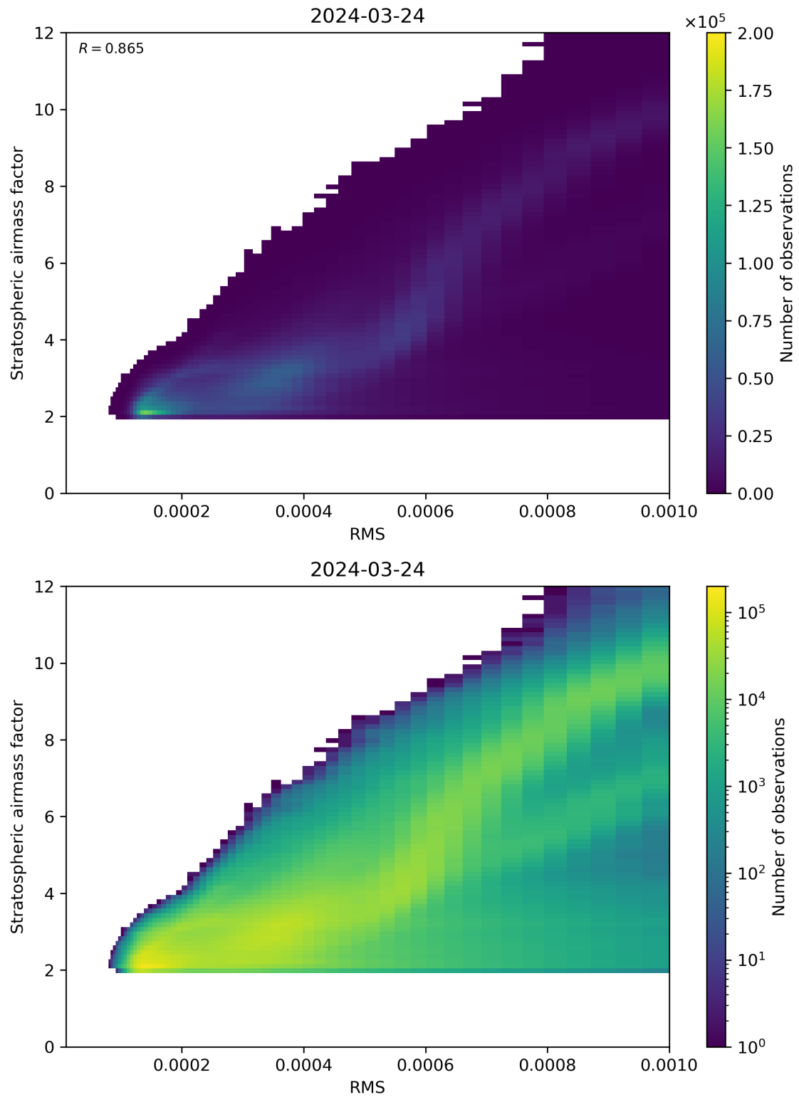
Figure 144: Scatter density plot of “RMS” against “Stratospheric airmass factor” for 2024-03-23 to 2024-03-25.
