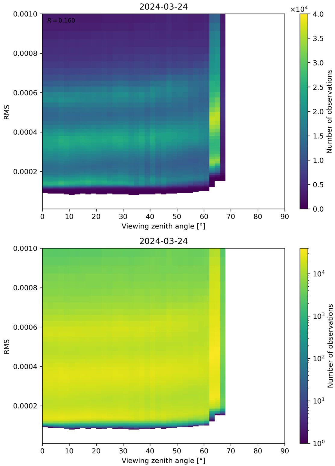
Figure 171: Scatter density plot of “Viewing zenith angle” against “RMS” for 2024-03-23 to 2024-03-25.
