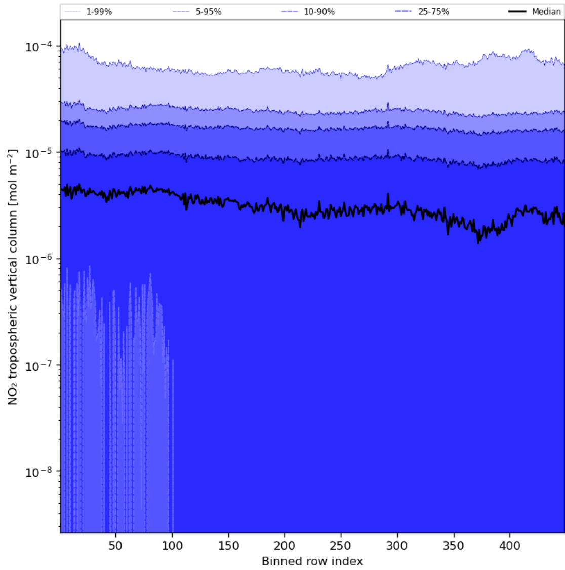
Figure 46: Along track statistics of “NO 2 tropospheric vertical column” for 2024-03-23 to 2024-03-25
