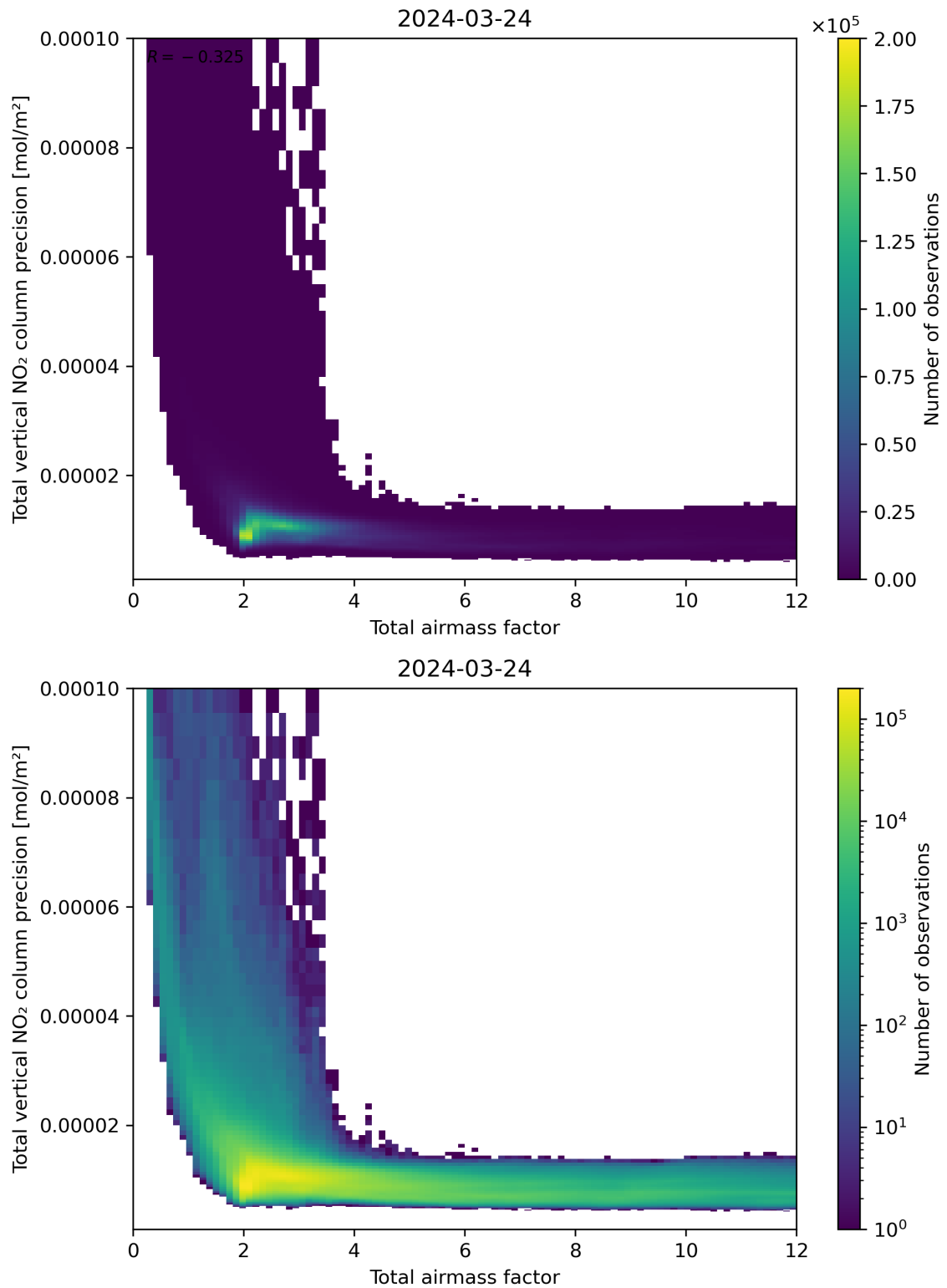
Figure 68: Scatter density plot of “Total airmass factor” against “Total vertical NO 2 column precision” for 2024-03-23 to 2024-03-25.
