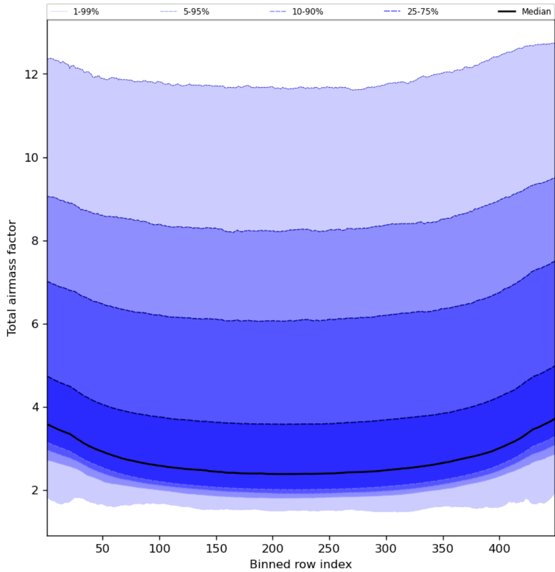
Figure 49: Along track statistics of “Total airmass factor” for 2024-03-23 to 2024-03-25
