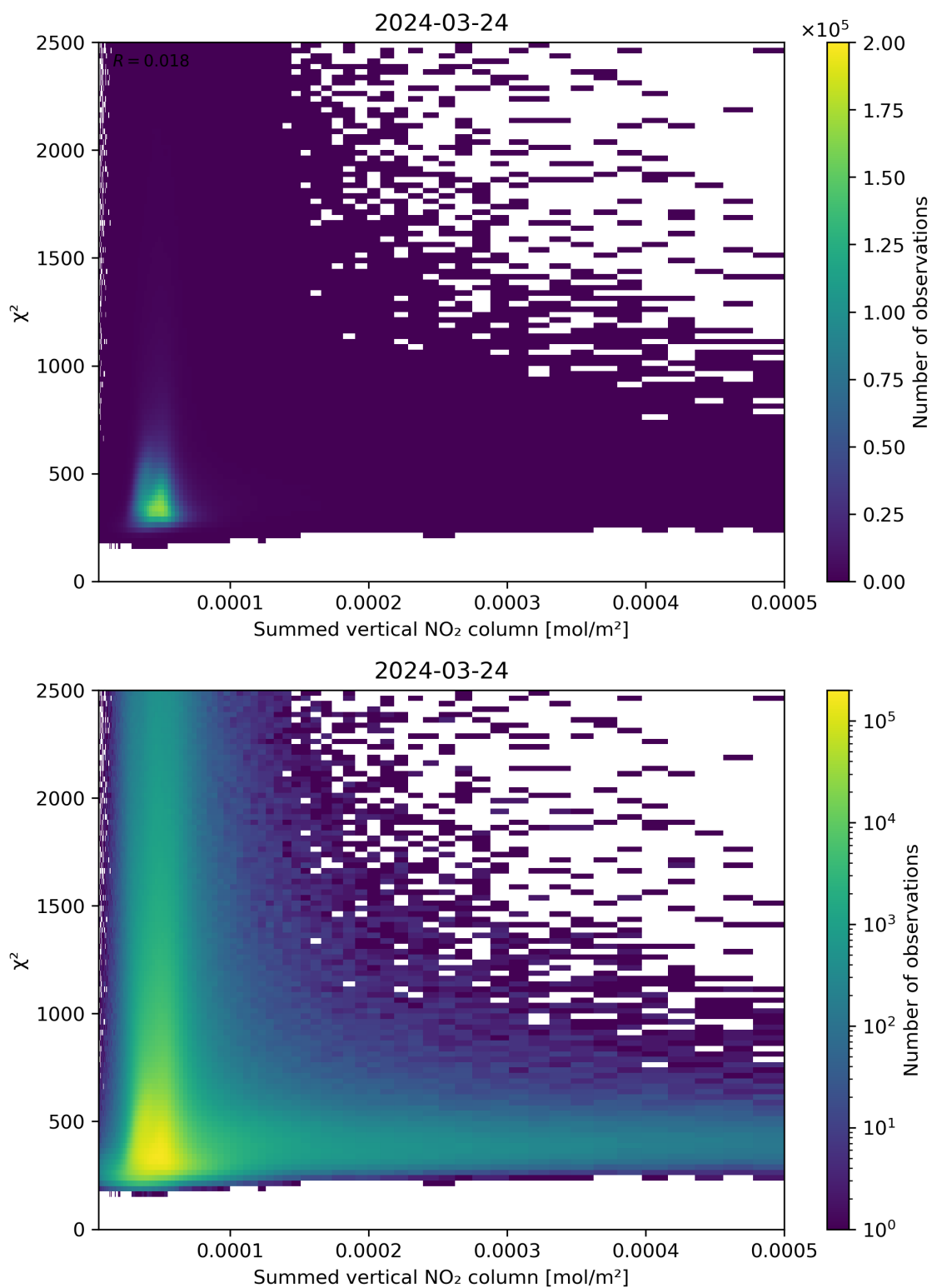
Figure 104: Scatter density plot of “Summed vertical NO 2 column” against “ \chi^2 ” for 2024-03-23 to 2024-03-25.
