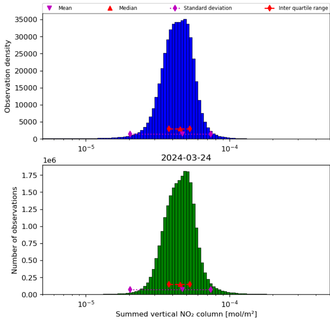
Figure 40: Histogram of “Summed vertical NO 2 column” for 2024-03-23 to 2024-03-25
