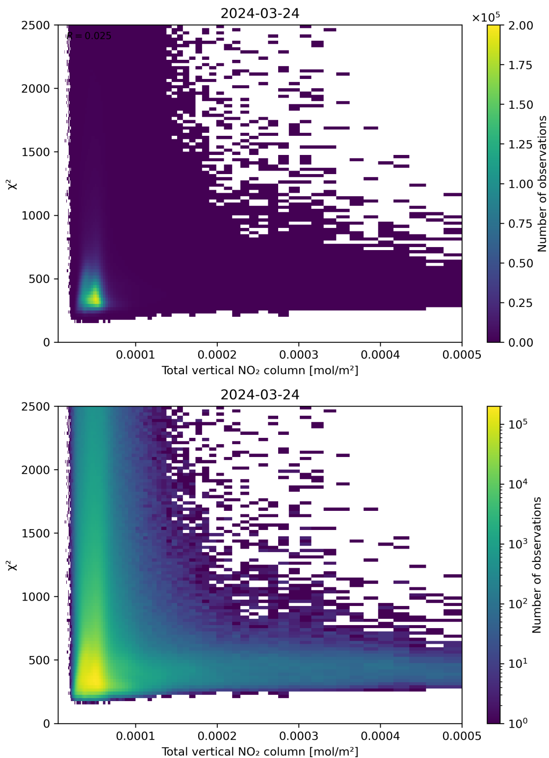
Figure 111: Scatter density plot of “Total vertical NO 2 column” against “ \chi^2 ” for 2024-03-23 to 2024-03-25.
