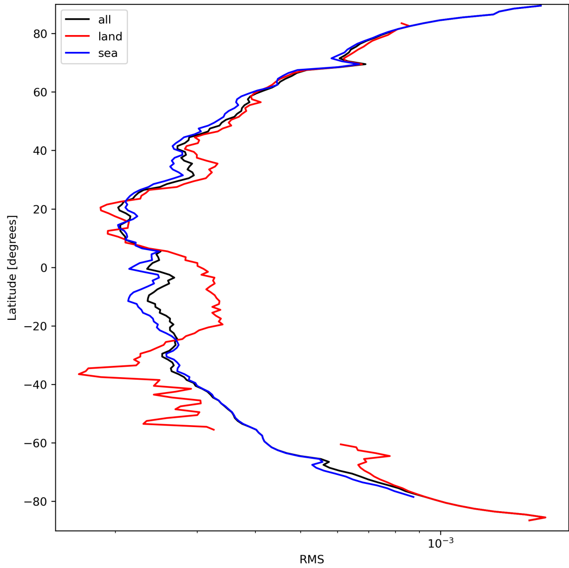
Figure 26: Zonal average of “RMS” for 2024-03-23 to 2024-03-25.
