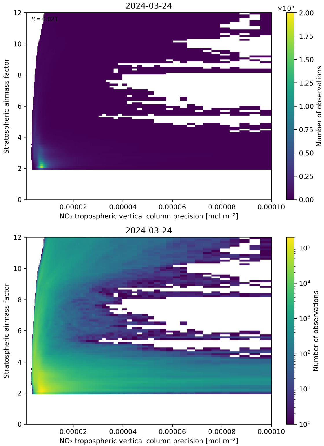
Figure 131: Scatter density plot of “NO 2 tropospheric vertical column precision” against “Stratospheric airmass factor” for 2024-03-23 to 2024-03-25.
