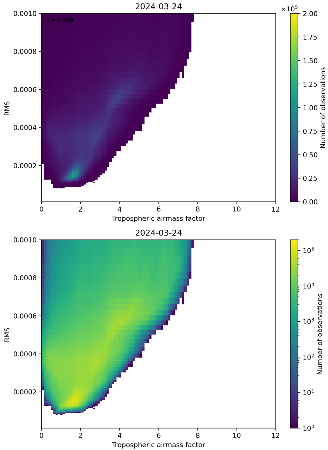
Figure 79: Scatter density plot of “Tropospheric airmass factor” against “RMS” for 2024-03-23 to 2024-03-25.
