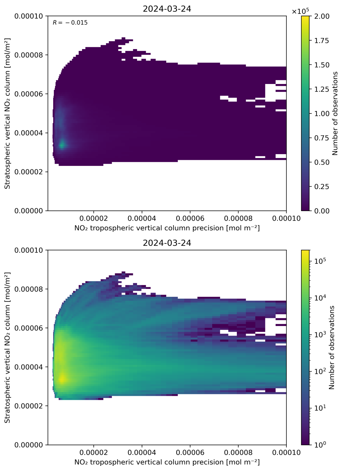
Figure 135: Scatter density plot of “NO 2 tropospheric vertical column precision” against “Stratospheric vertical NO 2 column” for 2024-03-23 to 2024-03-25.
