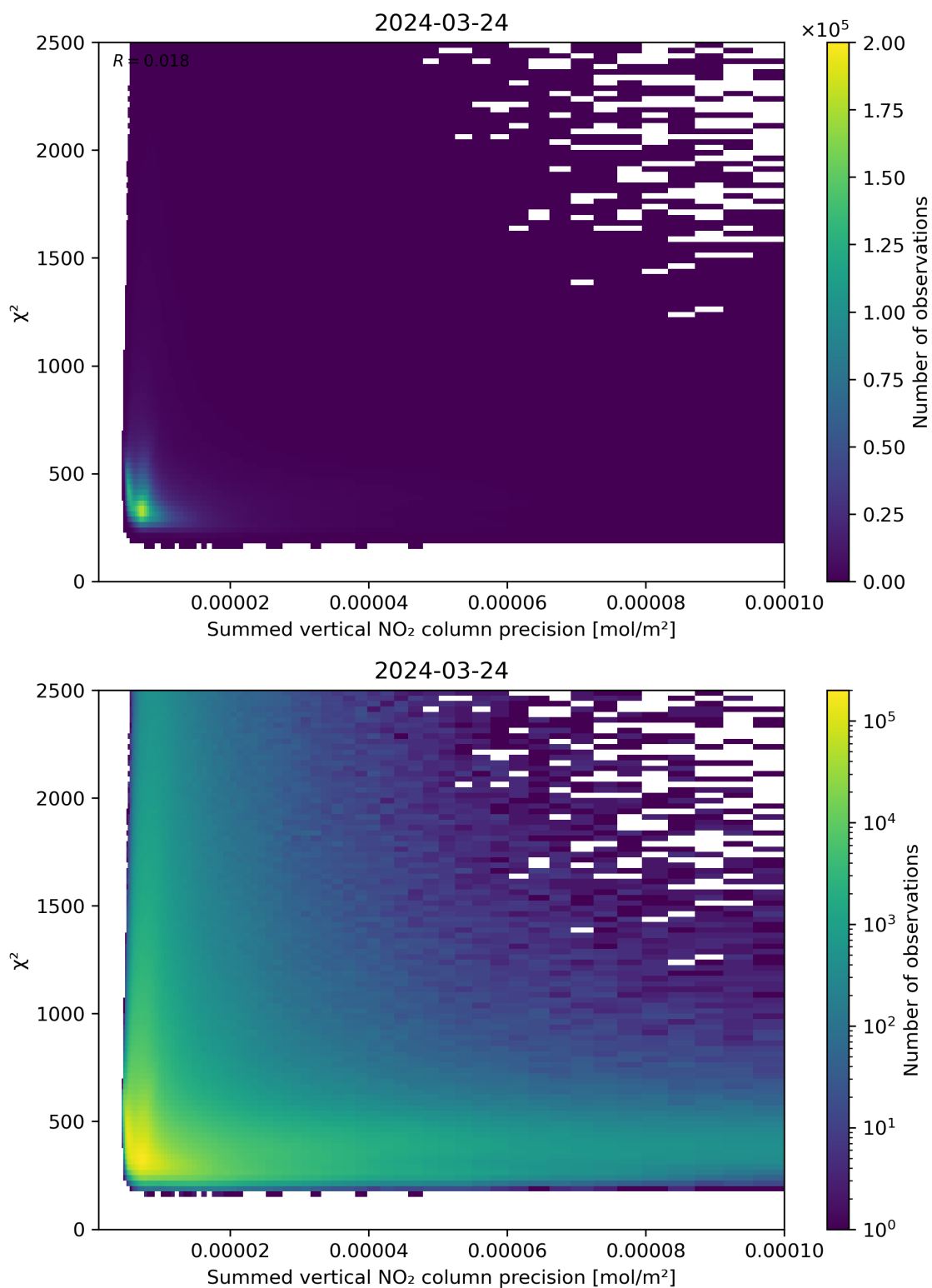
Figure 107: Scatter density plot of “Summed vertical NO 2 column precision” against “ \chi^2 ” for 2024-03-23 to 2024-03-25.
