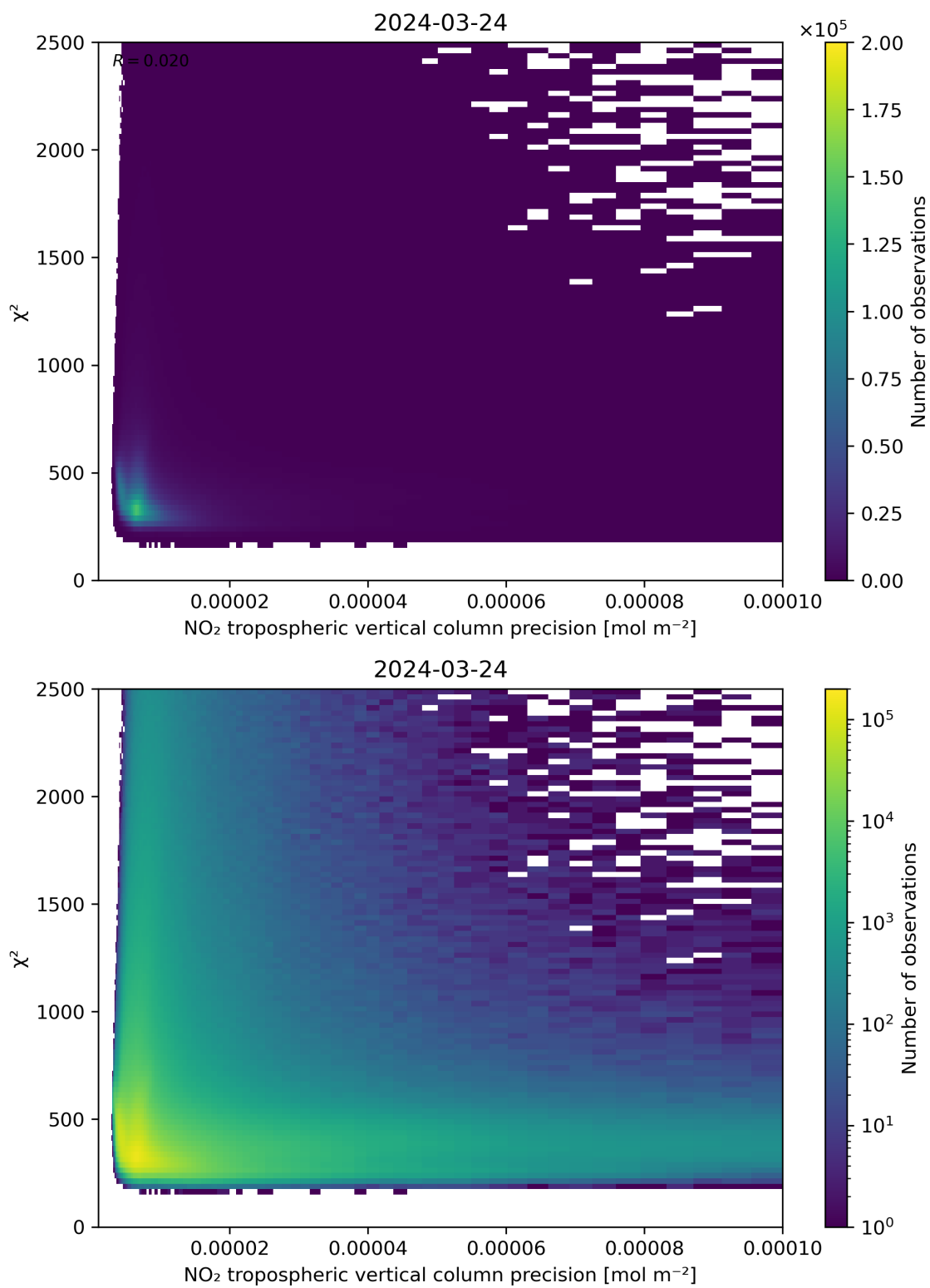
Figure 134: Scatter density plot of “NO 2 tropospheric vertical column precision” against “ \chi^2 ” for 2024-03-23 to 2024-03-25.
