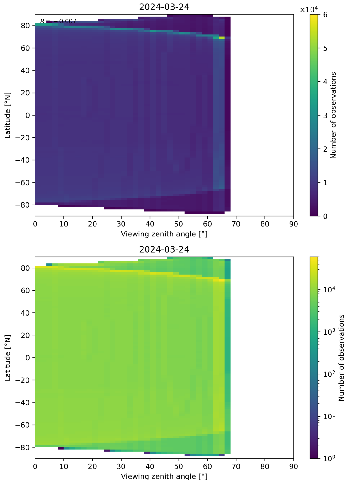
Figure 163: Scatter density plot of “Viewing zenith angle” against “Latitude” for 2024-03-23 to 2024-03-25.
