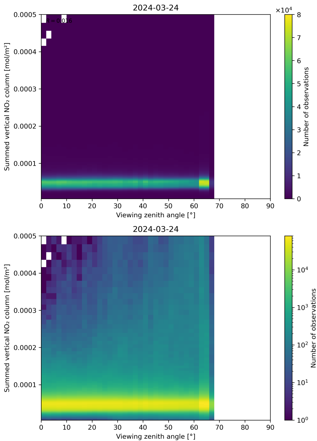
Figure 165: Scatter density plot of “Viewing zenith angle” against “Summed vertical NO 2 column” for 2024-03-23 to 2024-03-25.
