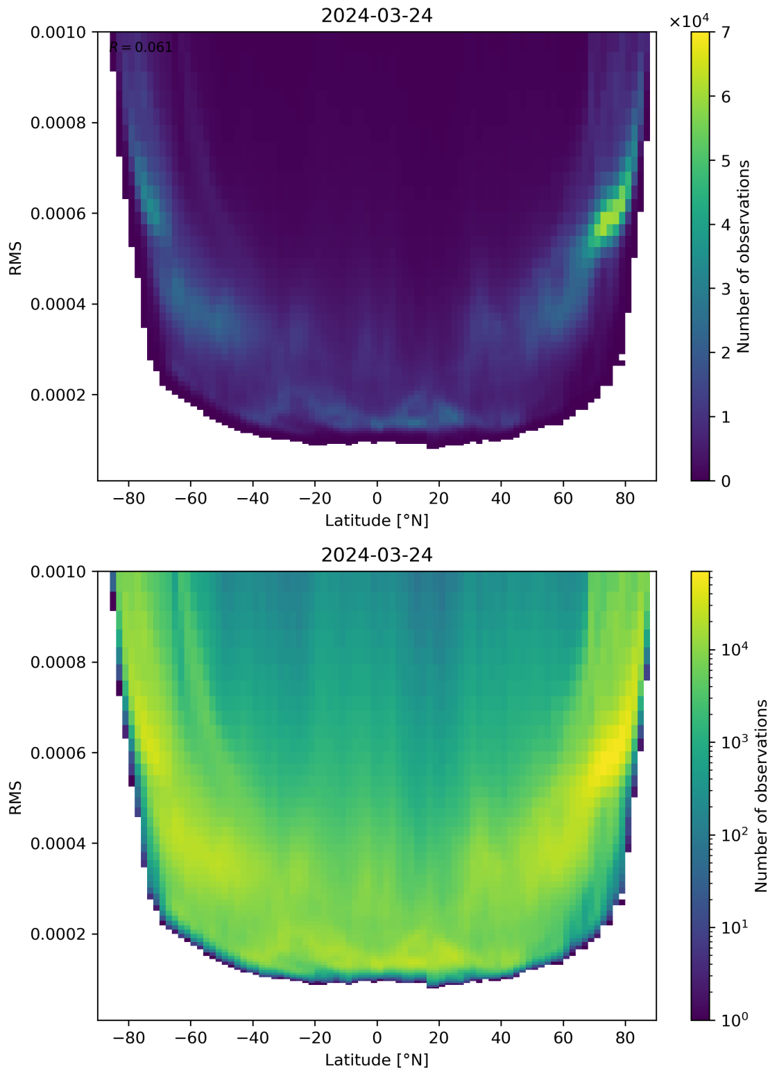
Figure 94: Scatter density plot of “Latitude” against “RMS” for 2024-03-23 to 2024-03-25.
