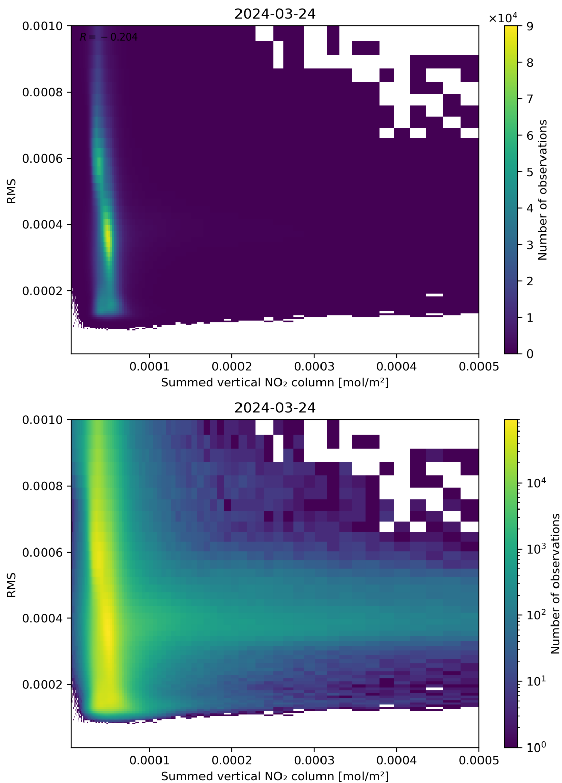
Figure 109: Scatter density plot of “Summed vertical NO 2 column” against “RMS” for 2024-03-23 to 2024-03-25.
