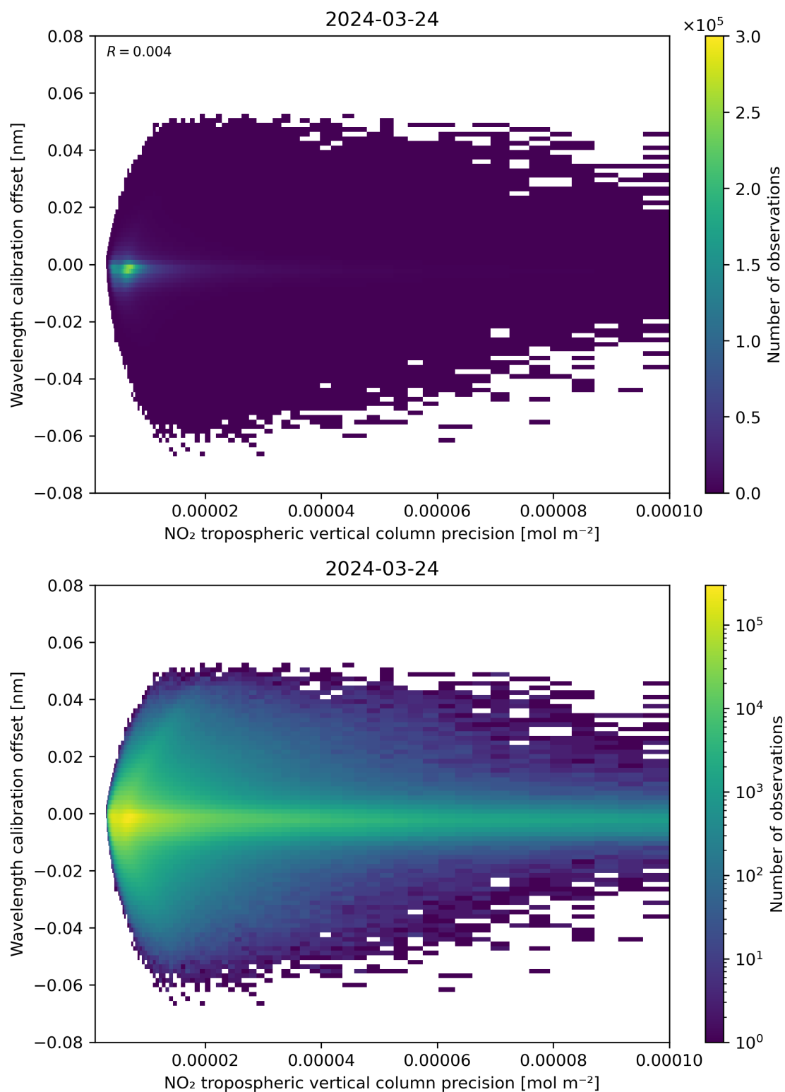
Figure 141: Scatter density plot of “NO 2 tropospheric vertical column precision” against “Wavelength calibration offset” for 2024-03-23 to 2024-03-25.
