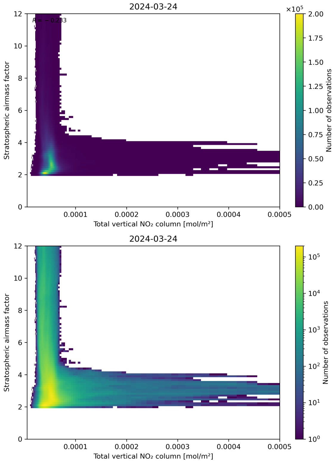
Figure 110: Scatter density plot of “Total vertical NO 2 column” against “Stratospheric airmass factor” for 2024-03-23 to 2024-03-25.
