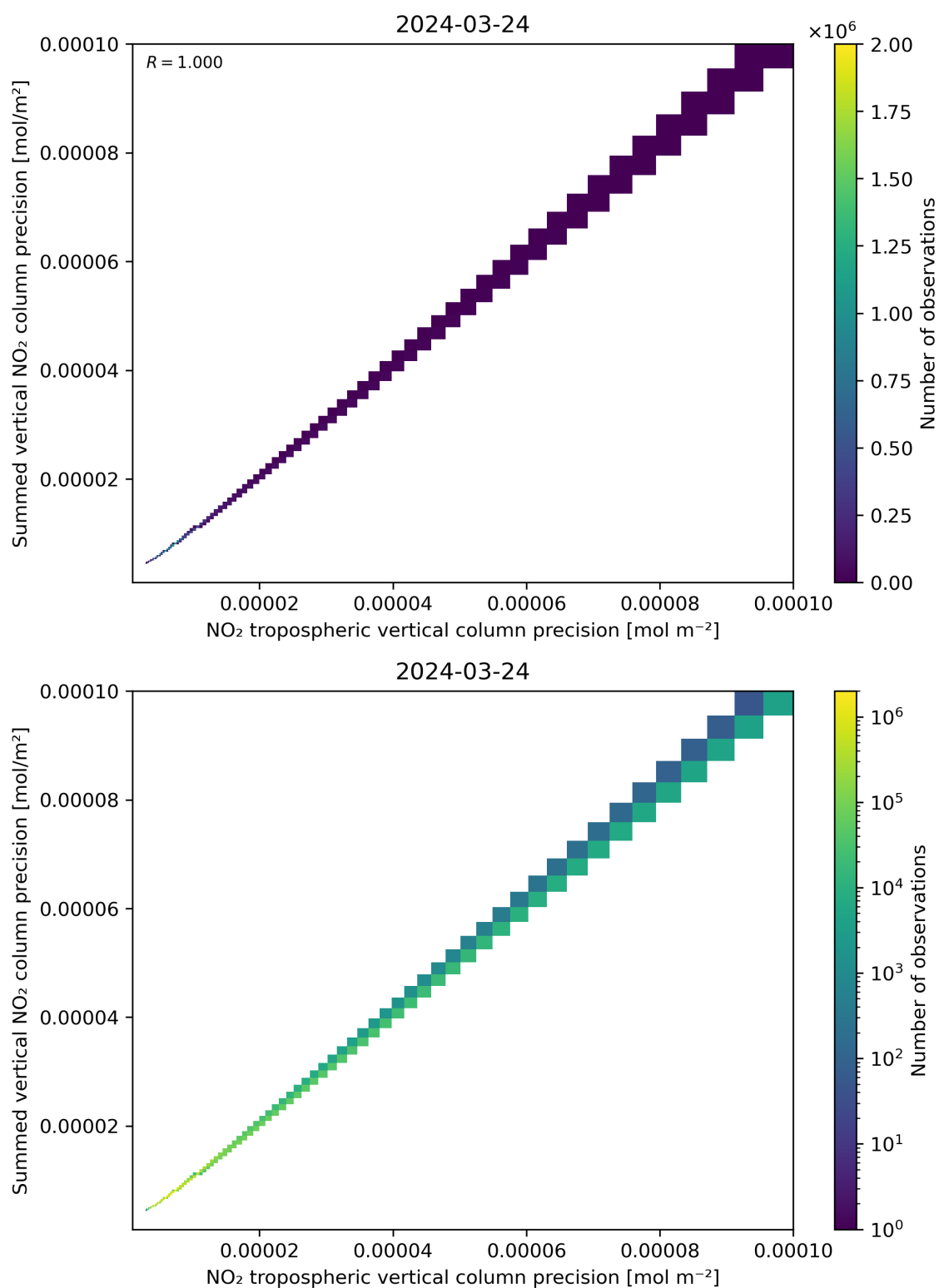
Figure 137: Scatter density plot of “NO 2 tropospheric vertical column precision” against “Summed vertical NO 2 column precision” for 2024-03-23 to 2024-03-25.
