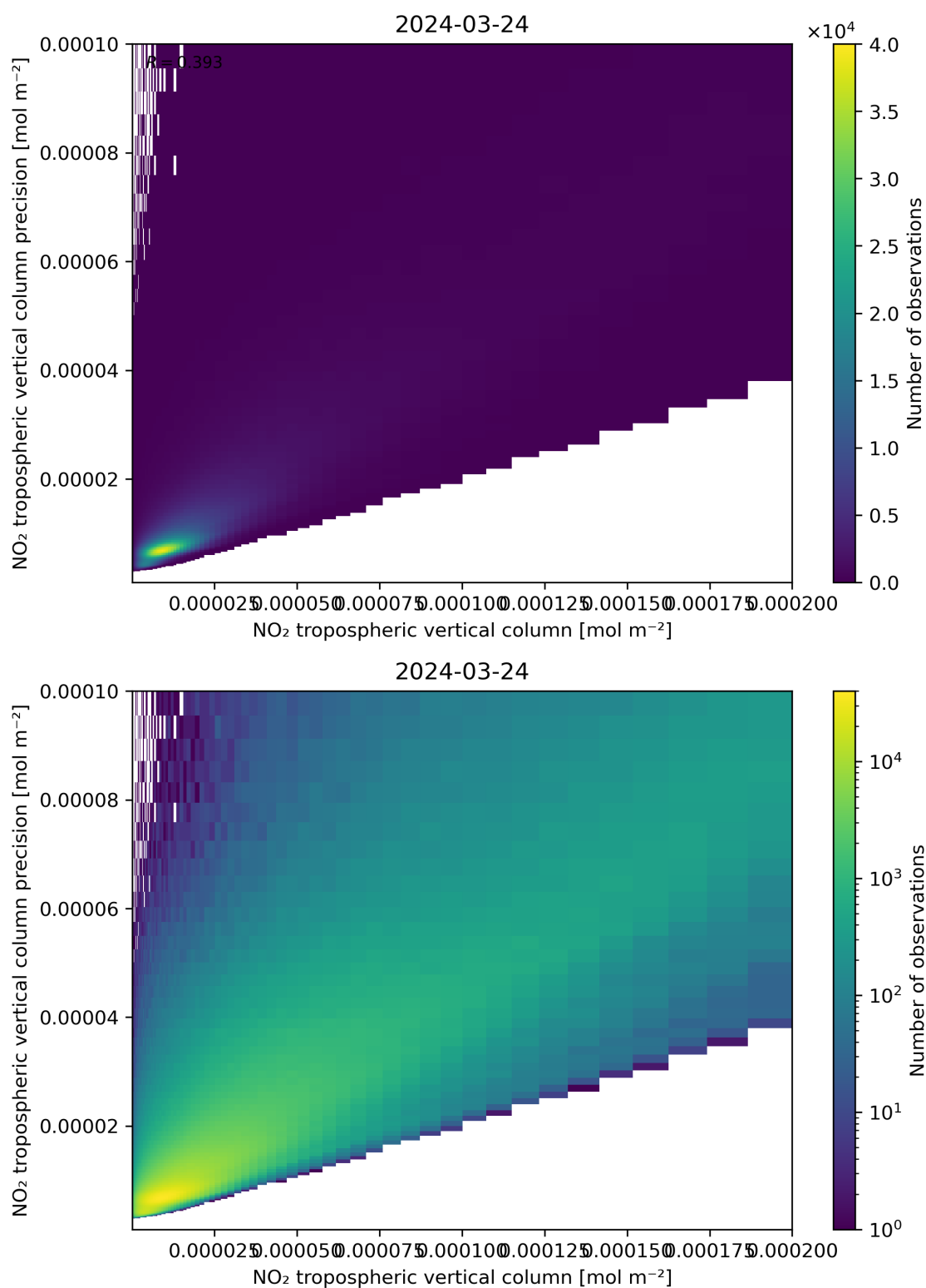
Figure 130: Scatter density plot of “NO 2 tropospheric vertical column” against “NO 2 tropospheric vertical column precision” for 2024-03-23 to 2024-03-25.
