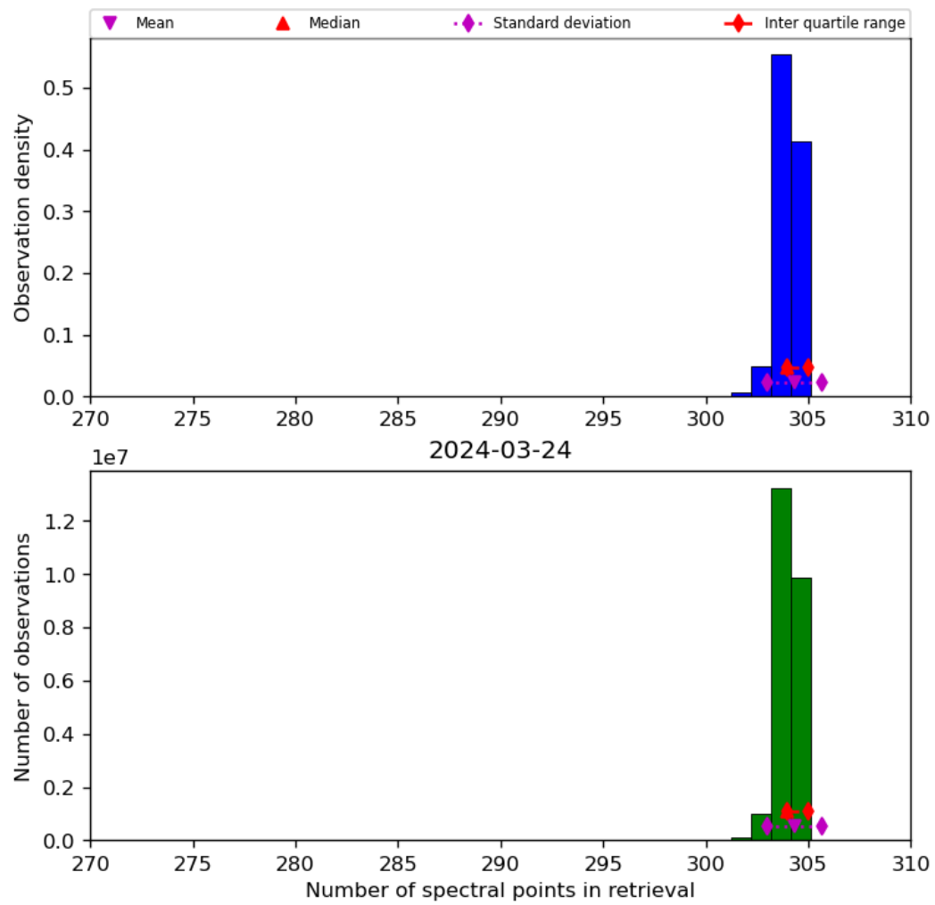
Figure 33: Histogram of “Number of spectral points in retrieval” for 2024-03-23 to 2024-03-25
