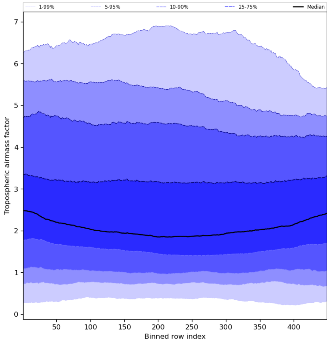
Figure 48: Along track statistics of “Tropospheric airmass factor” for 2024-03-23 to 2024-03-25
