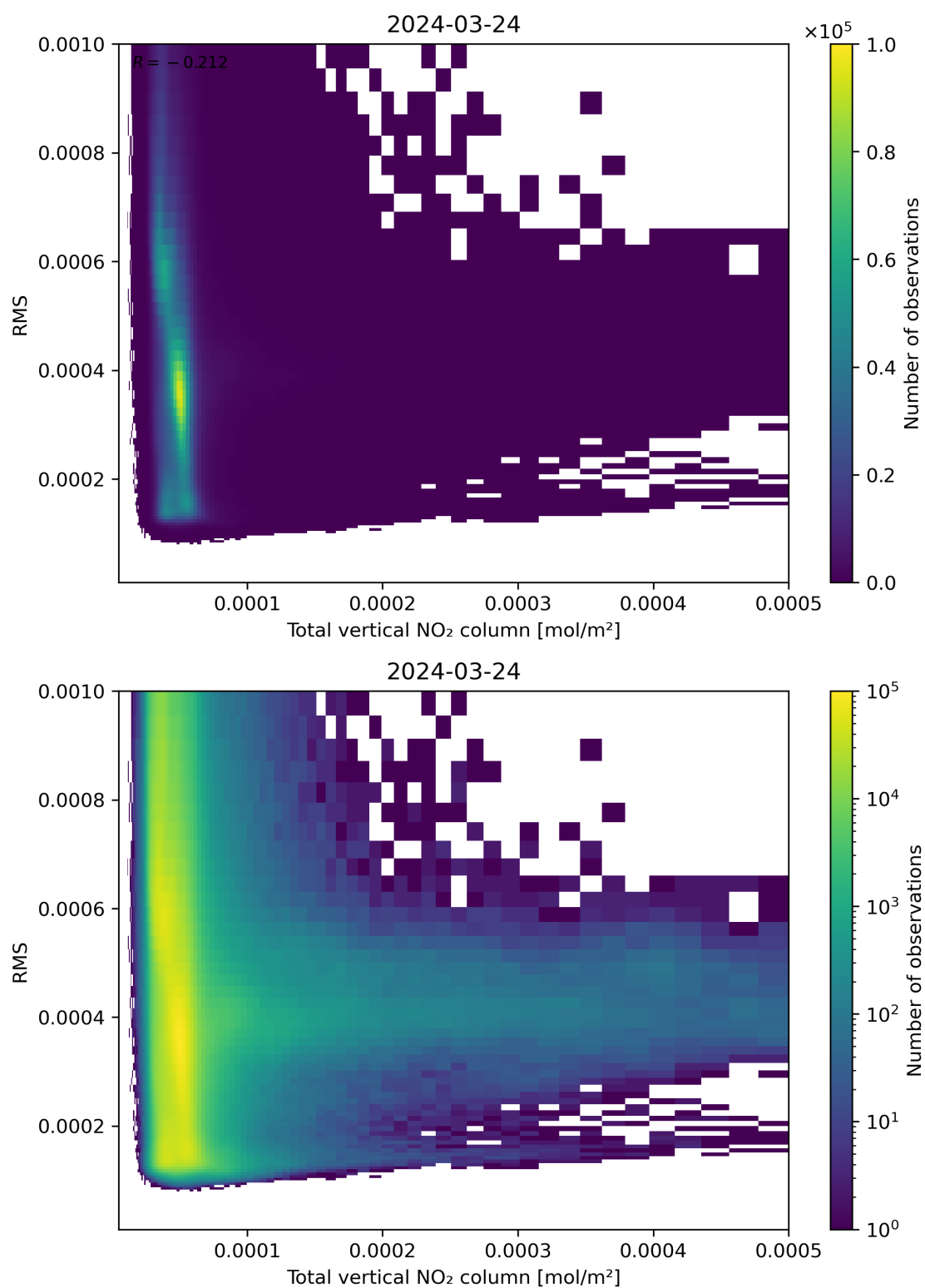
Figure 120: Scatter density plot of “Total vertical NO 2 column” against “RMS” for 2024-03-23 to 2024-03-25.
