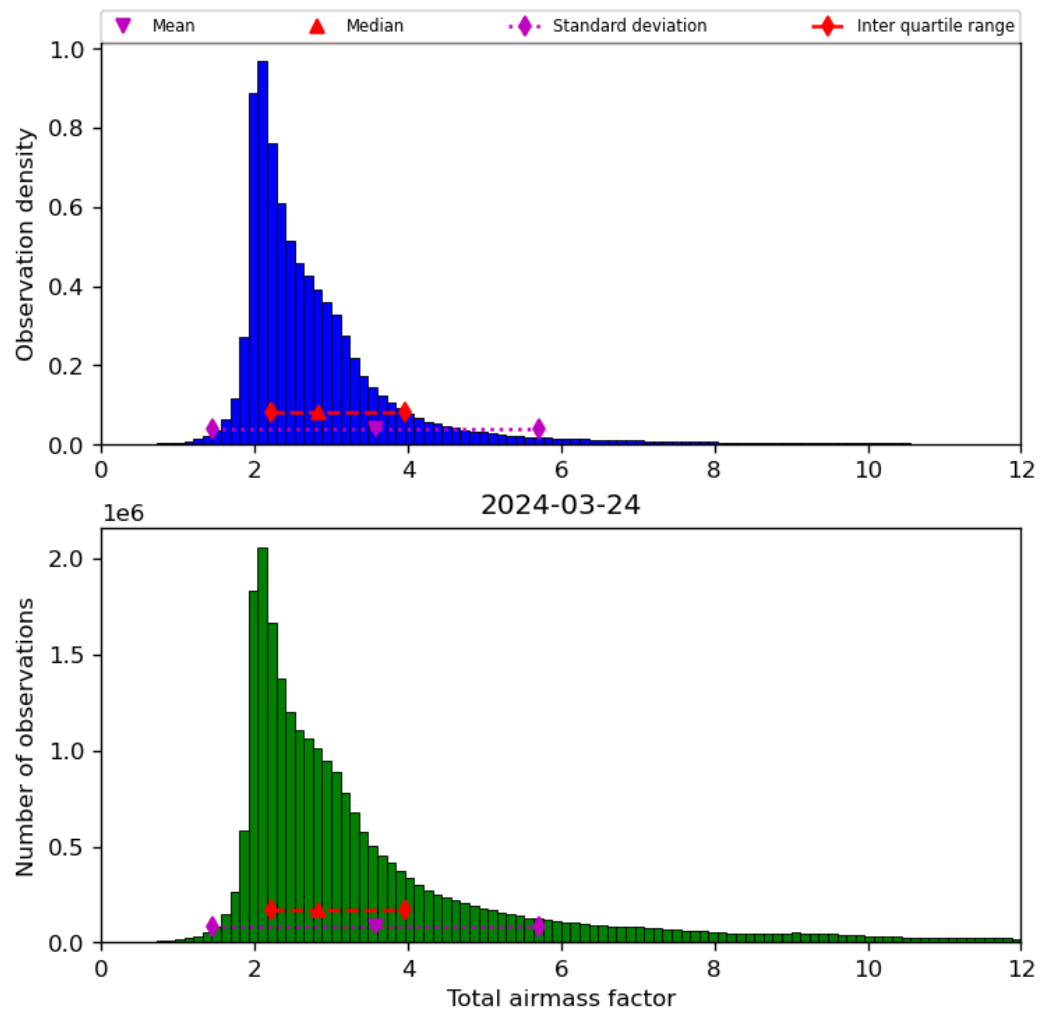
Figure 32: Histogram of “Total airmass factor” for 2024-03-23 to 2024-03-25
