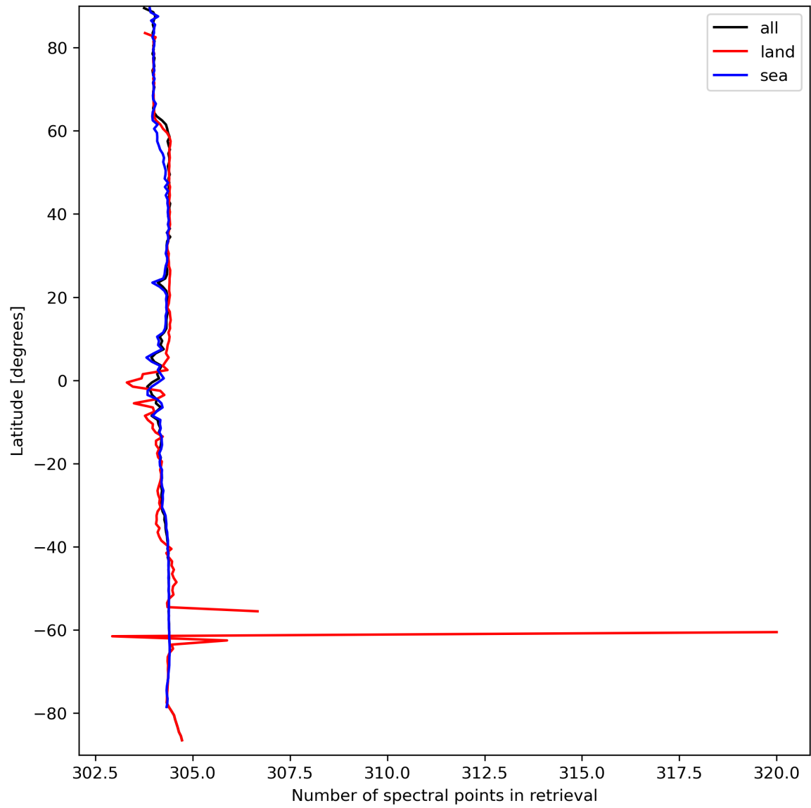
Figure 16: Zonal average of “Number of spectral points in retrieval” for 2024-03-23 to 2024-03-25.
