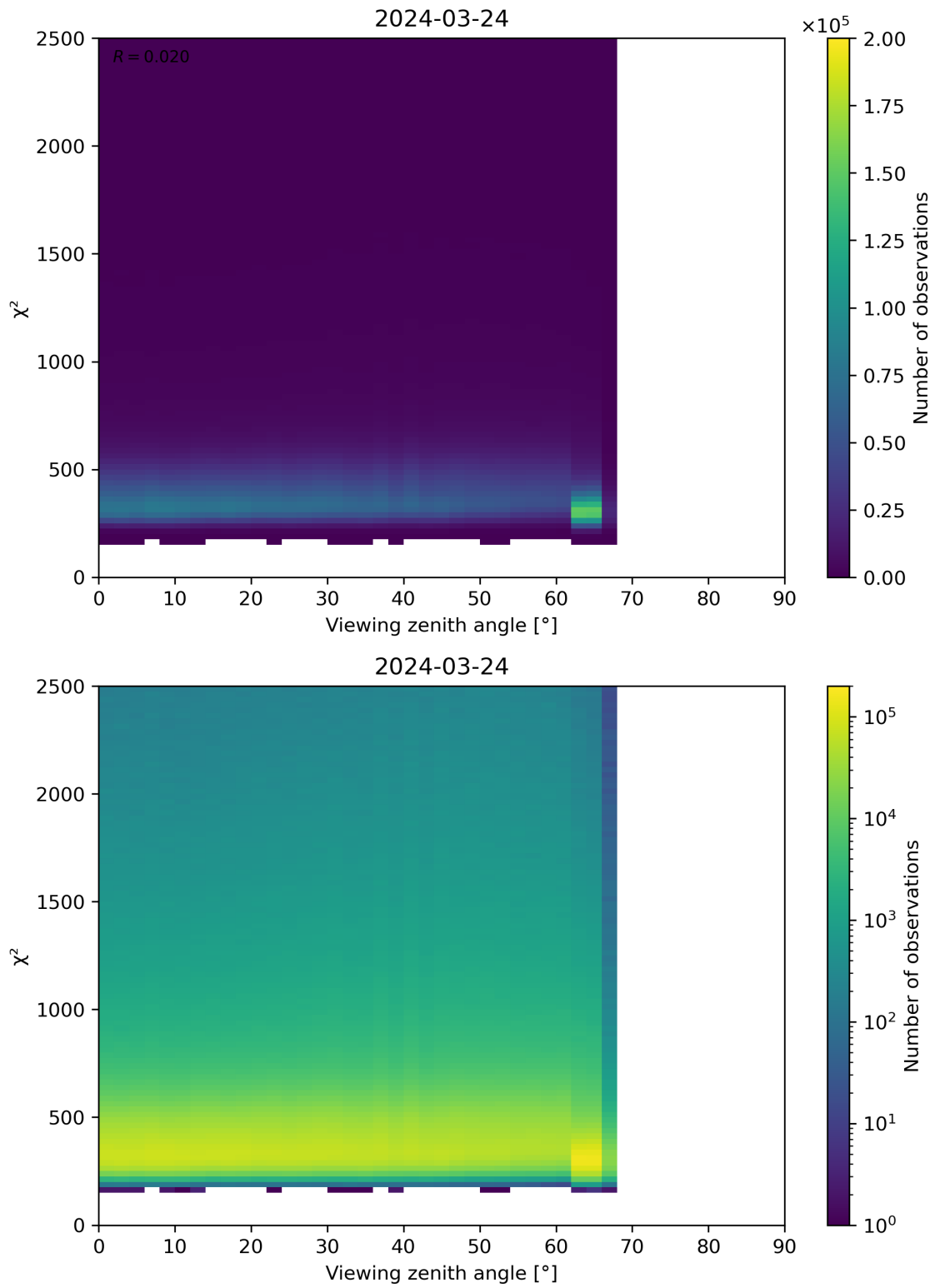
Figure 162: Scatter density plot of “Viewing zenith angle” against “ \chi^2 ” for 2024-03-23 to 2024-03-25.
