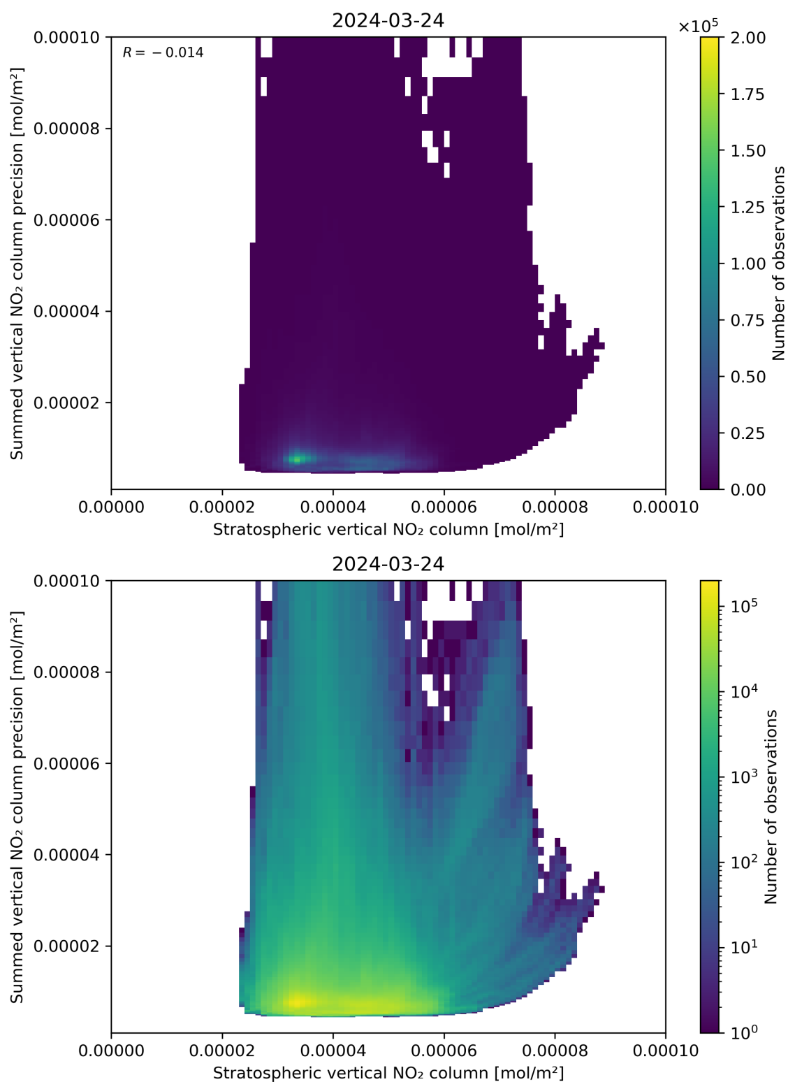
Figure 99: Scatter density plot of “Stratospheric vertical NO 2 column” against “Summed vertical NO 2 column precision” for 2024-03-23 to 2024-03-25.
