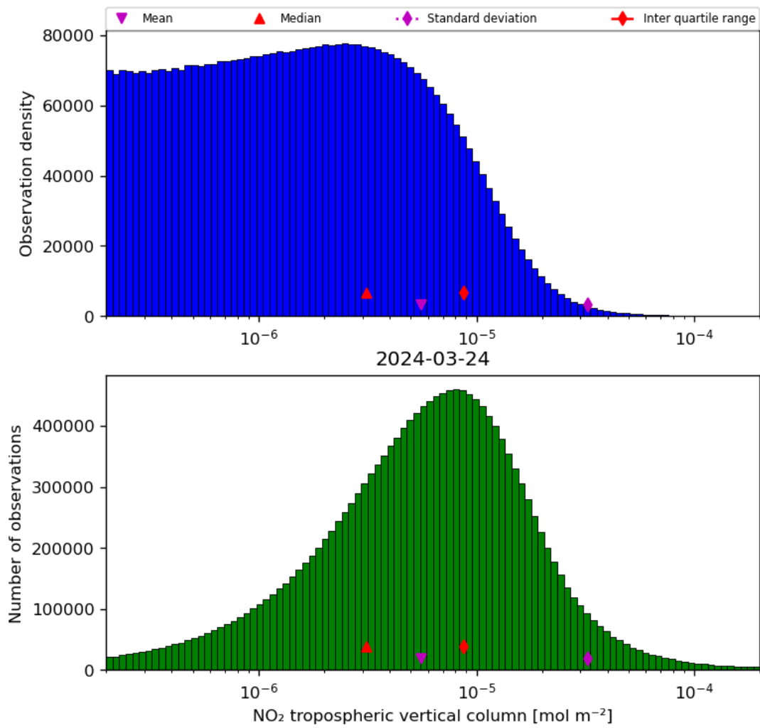
Figure 29: Histogram of “NO 2 tropospheric vertical column” for 2024-03-23 to 2024-03-25
