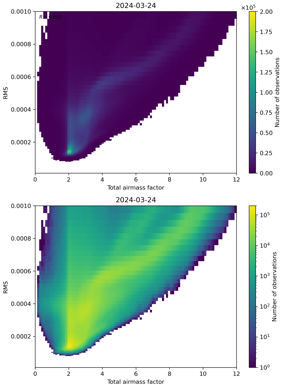
Figure 69: Scatter density plot of “Total airmass factor” against “RMS” for 2024-03-23 to 2024-03-25.
