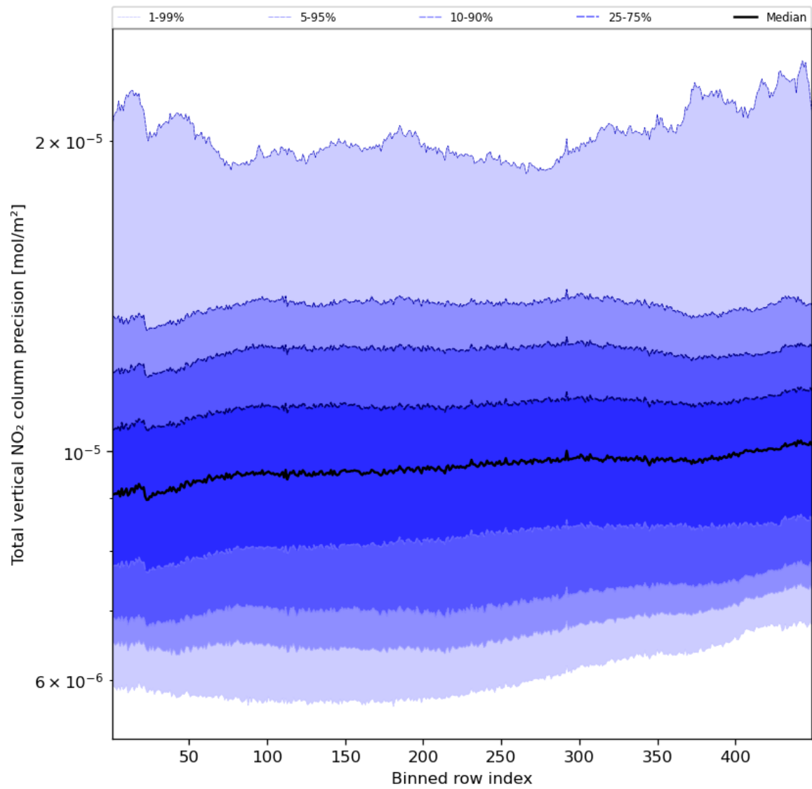
Figure 56: Along track statistics of “Total vertical NO 2 column precision” for 2024-03-23 to 2024-03-25
