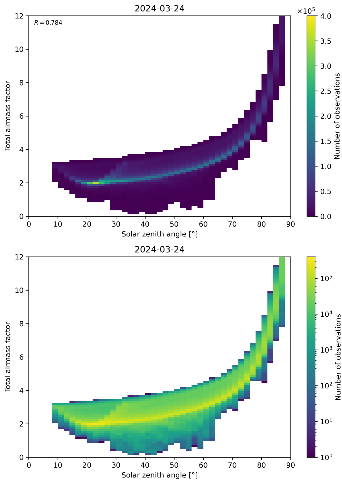
Figure 146: Scatter density plot of “Solar zenith angle” against “Total air mass factor” for 2024-03-23 to 2024-03-25.
