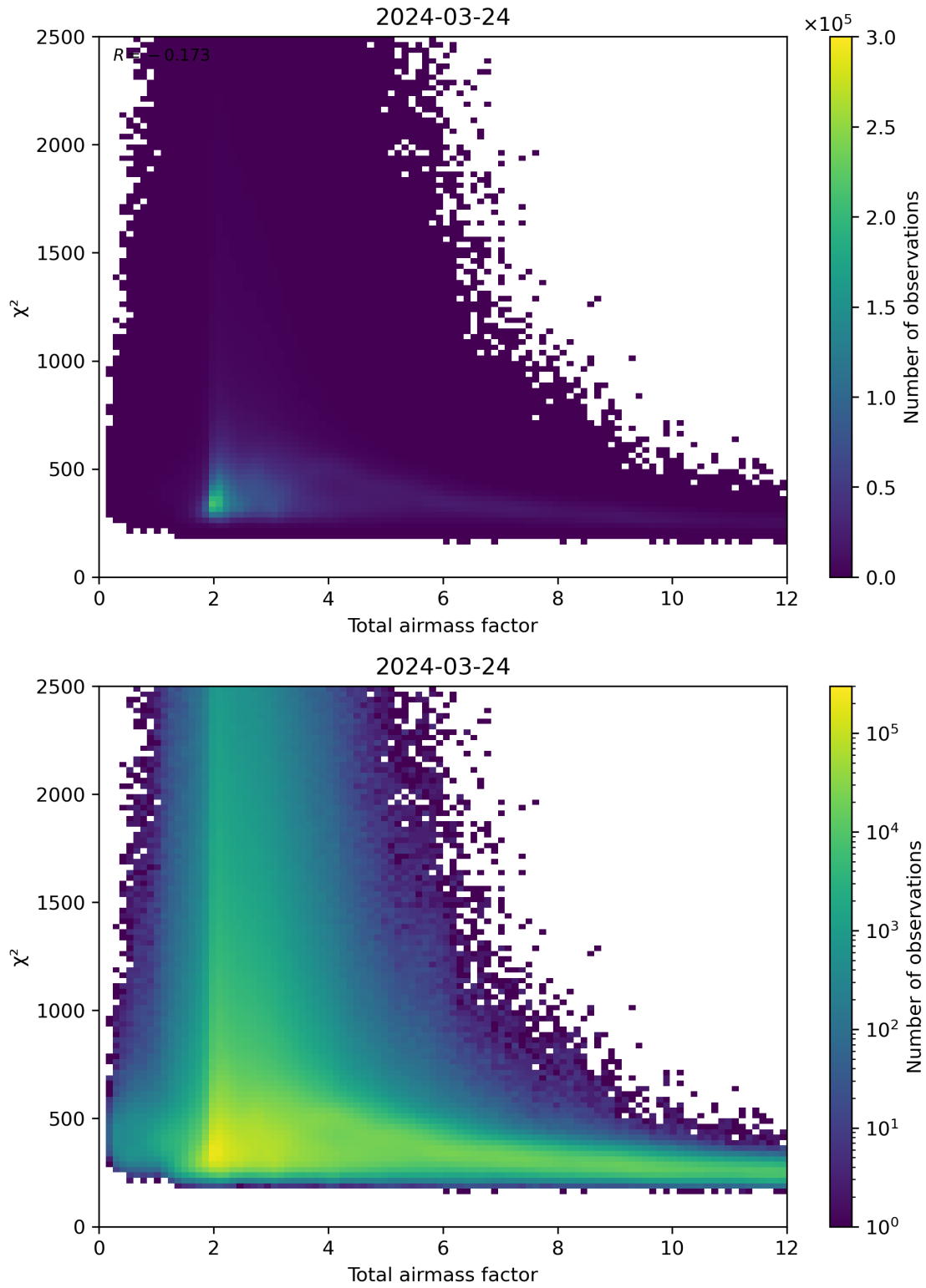
Figure 63: Scatter density plot of “Total airmass factor” against “ \chi^2 ” for 2024-03-23 to 2024-03-25.
