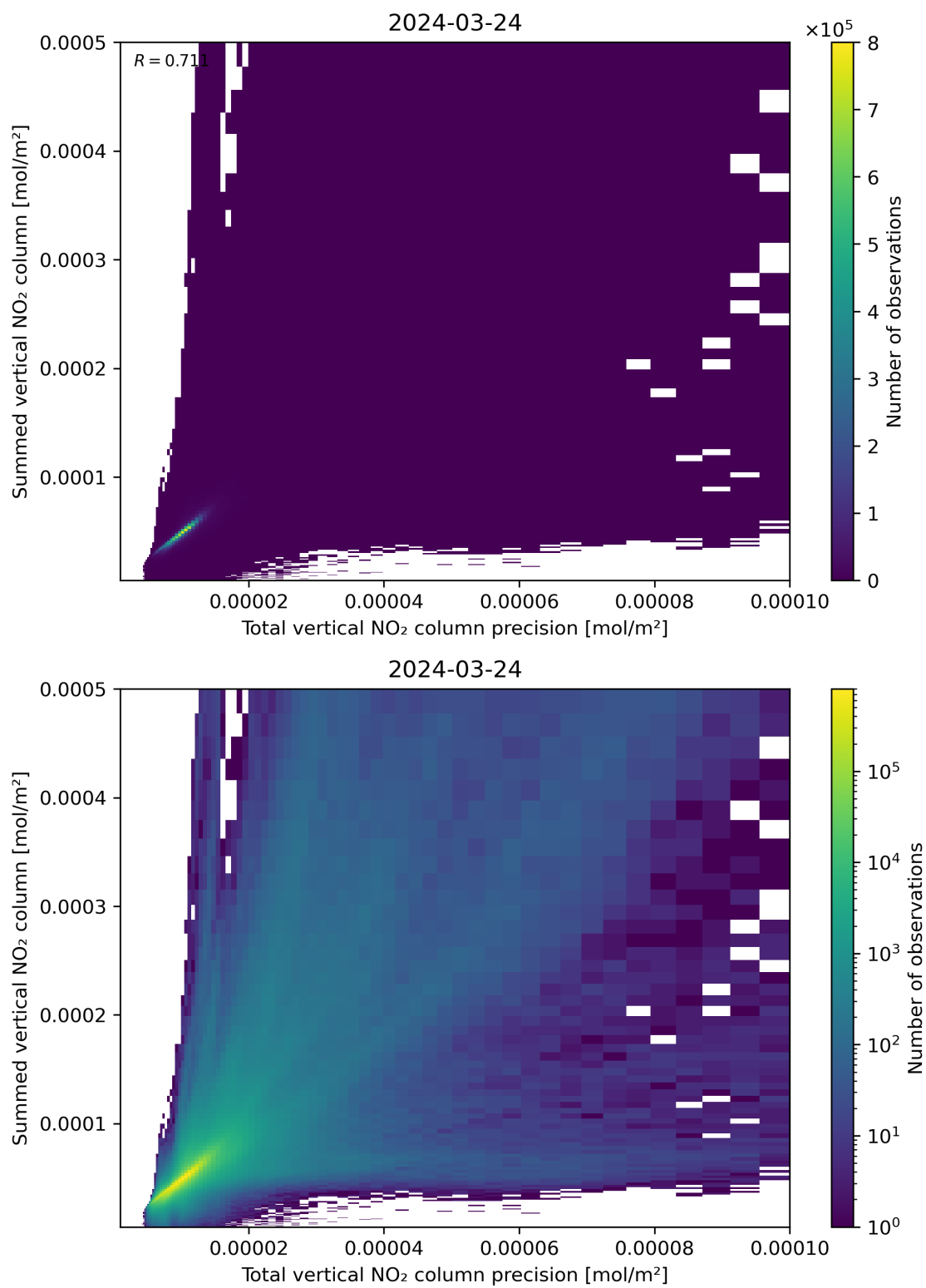
Figure 117: Scatter density plot of “Total vertical NO 2 column precision” against “Summed vertical NO 2 column” for 2024-03-23 to 2024-03-25.
