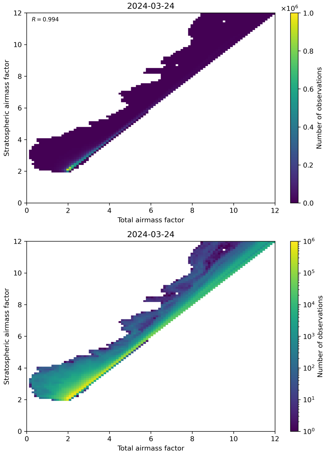
Figure 62: Scatter density plot of “Total airmass factor” against “Stratospheric airmass factor” for 2024-03-23 to 2024-03-25.
