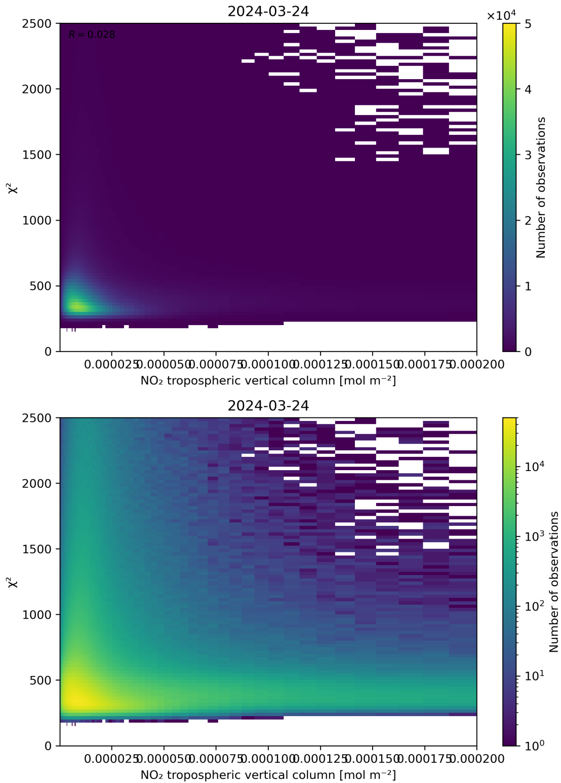
Figure 124: Scatter density plot of “NO 2 tropospheric vertical column” against “ \chi^2 ” for 2024-03-23 to 2024-03-25.
