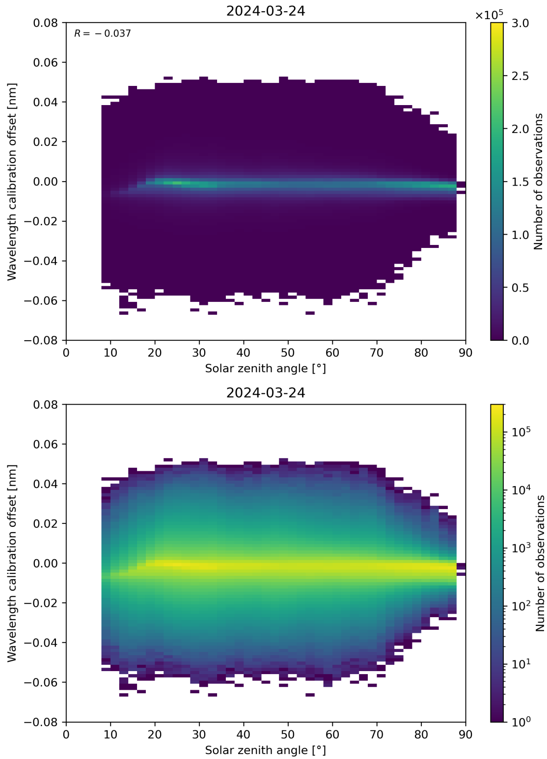
Figure 158: Scatter density plot of “Solar zenith angle” against “Wavelength calibration offset” for 2024-03-23 to 2024-03-25.
