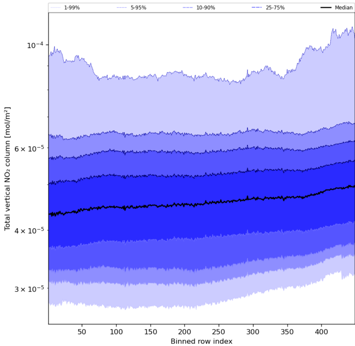
Figure 55: Along track statistics of “Total vertical NO 2 column” for 2024-03-23 to 2024-03-25
