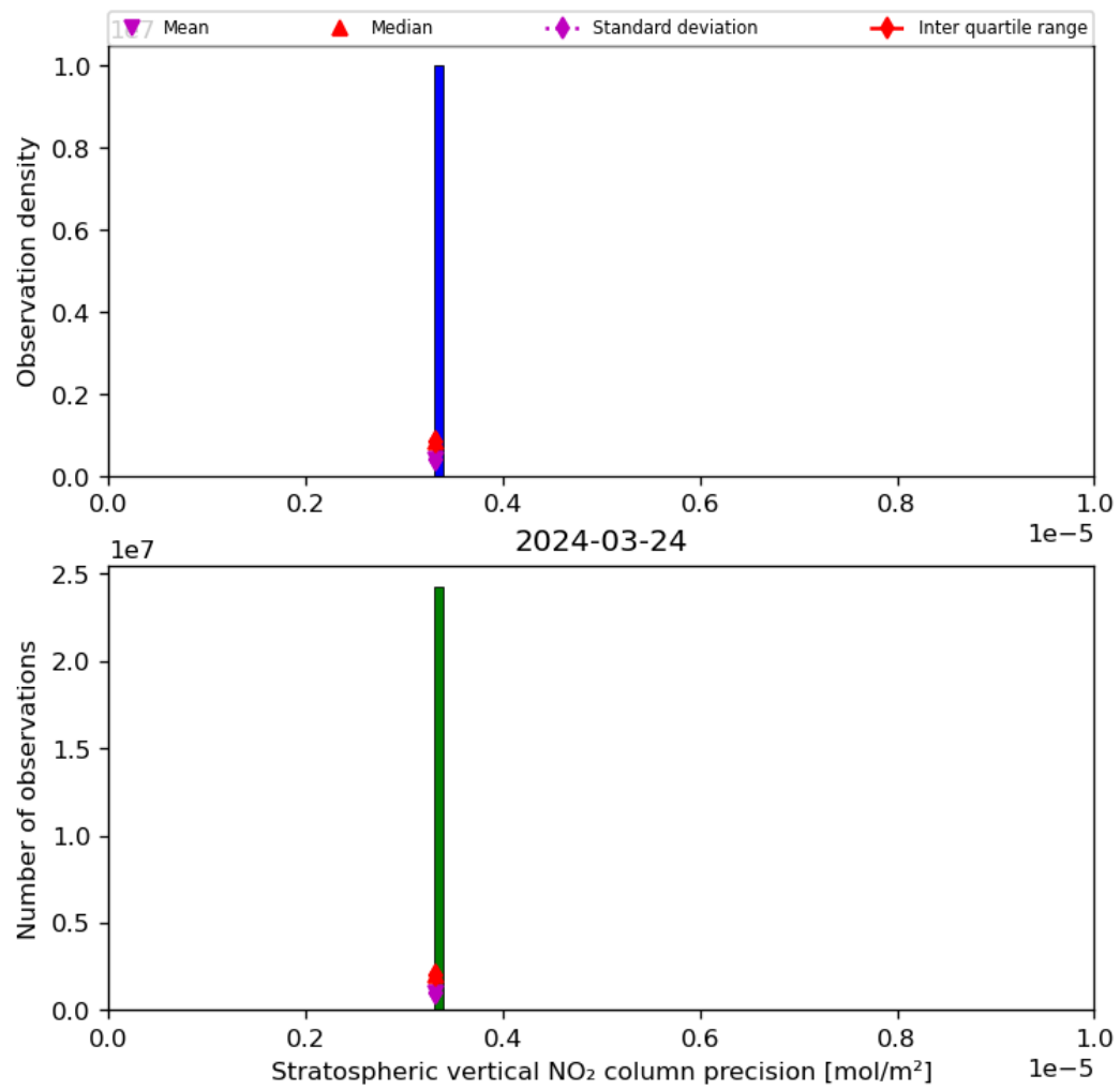
Figure 37: Histogram of “Stratospheric vertical NO 2 column precision” for 2024-03-23 to 2024-03-25
