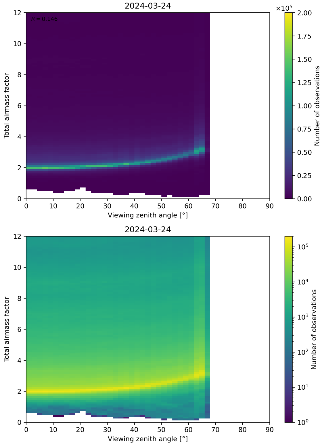
Figure 160: Scatter density plot of “Viewing zenith angle” against “Total airmass factor” for 2024-03-23 to 2024-03-25.
