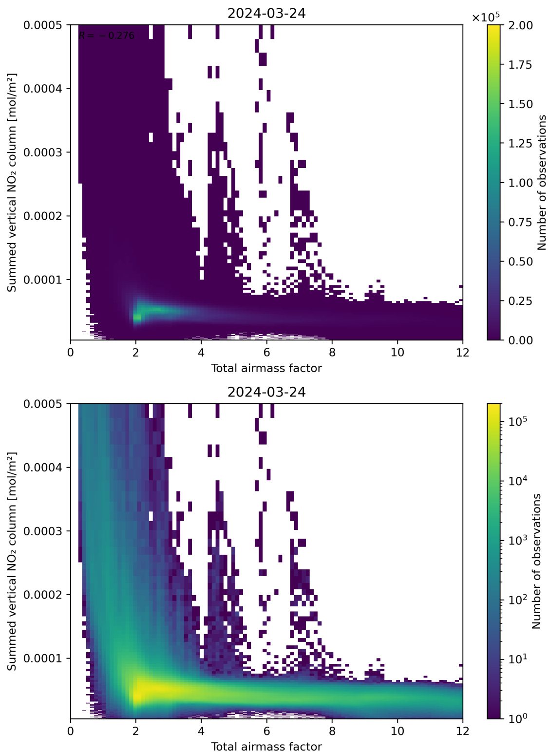
Figure 65: Scatter density plot of “Total airmass factor” against “Summed vertical NO 2 column” for 2024-03-23 to 2024-03-25.
