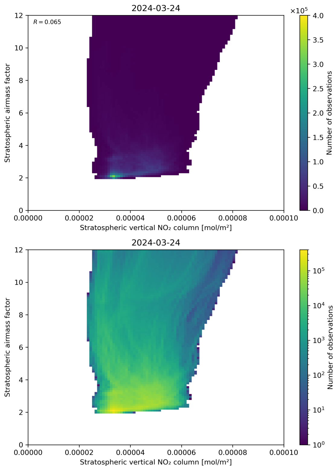
Figure 96: Scatter density plot of “Stratospheric vertical NO 2 column” against “Stratospheric airmass factor” for 2024-03-23 to 2024-03-25.
