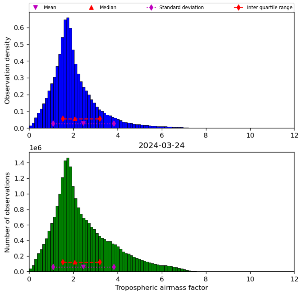
Figure 31: Histogram of “Tropospheric airmass factor” for 2024-03-23 to 2024-03-25
