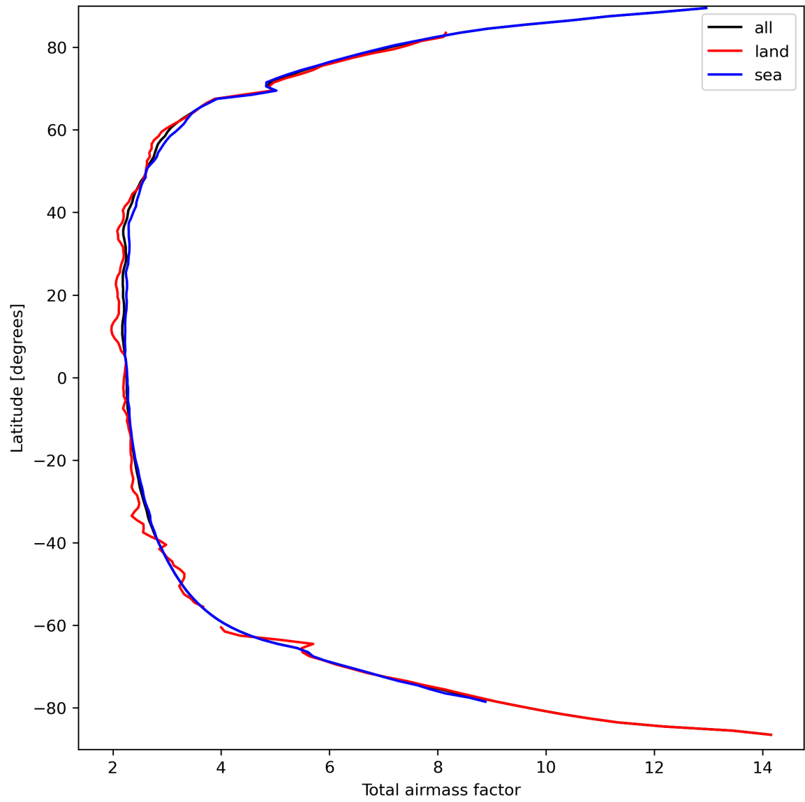
Figure 15: Zonal average of “Total airmass factor” for 2024-03-23 to 2024-03-25.
