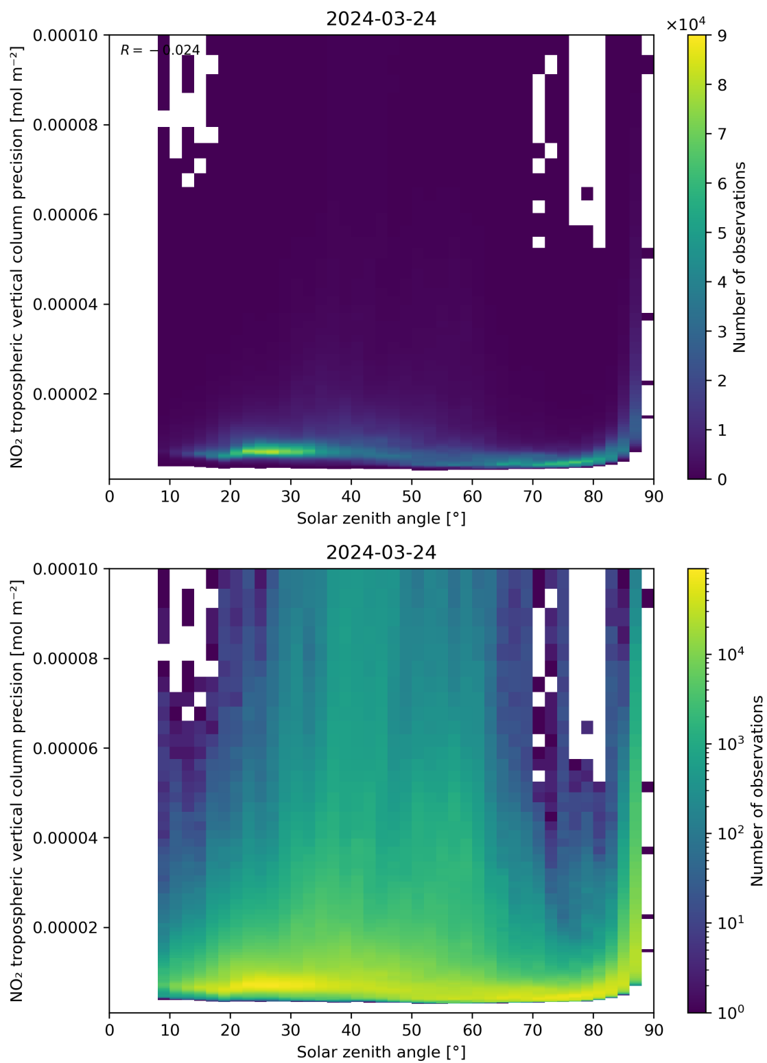
Figure 156: Scatter density plot of “Solar zenith angle” against “NO 2 tropospheric vertical column precision” for 2024-03-23 to 2024-03-25.
