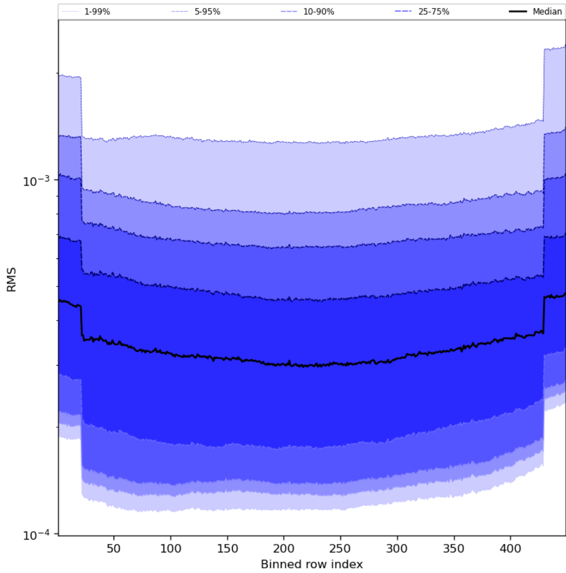
Figure 60: Along track statistics of “RMS” for 2024-03-23 to 2024-03-25
