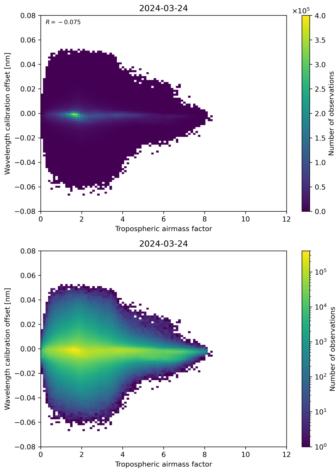
Figure 80: Scatter density plot of “Tropospheric airmass factor” against “Wavelength calibration offset” for 2024-03-23 to 2024-03-25.
