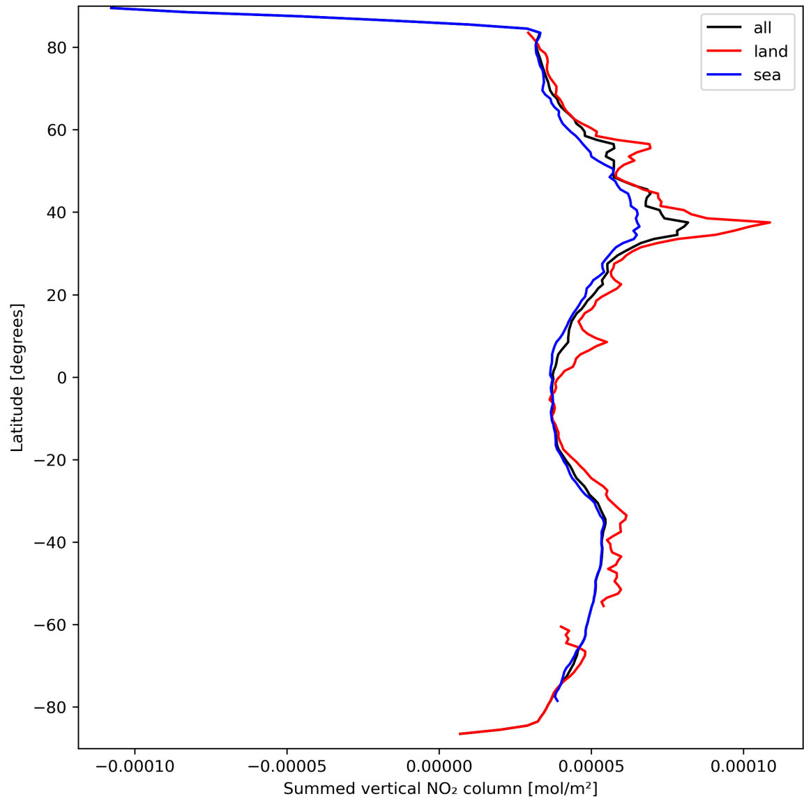
Figure 23: Zonal average of “Summed vertical NO 2 column” for 2024-03-23 to 2024-03-25.
