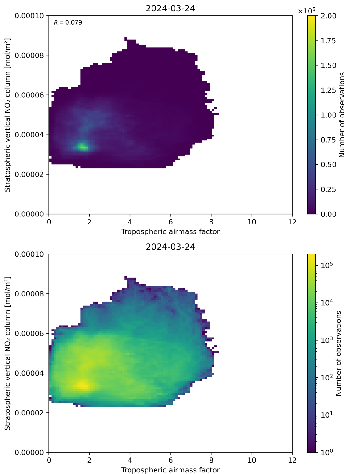
Figure 74: Scatter density plot of “Tropospheric air mass factor” against “Stratospheric vertical NO 2 column” for 2024-03-23 to 2024-03-25.
