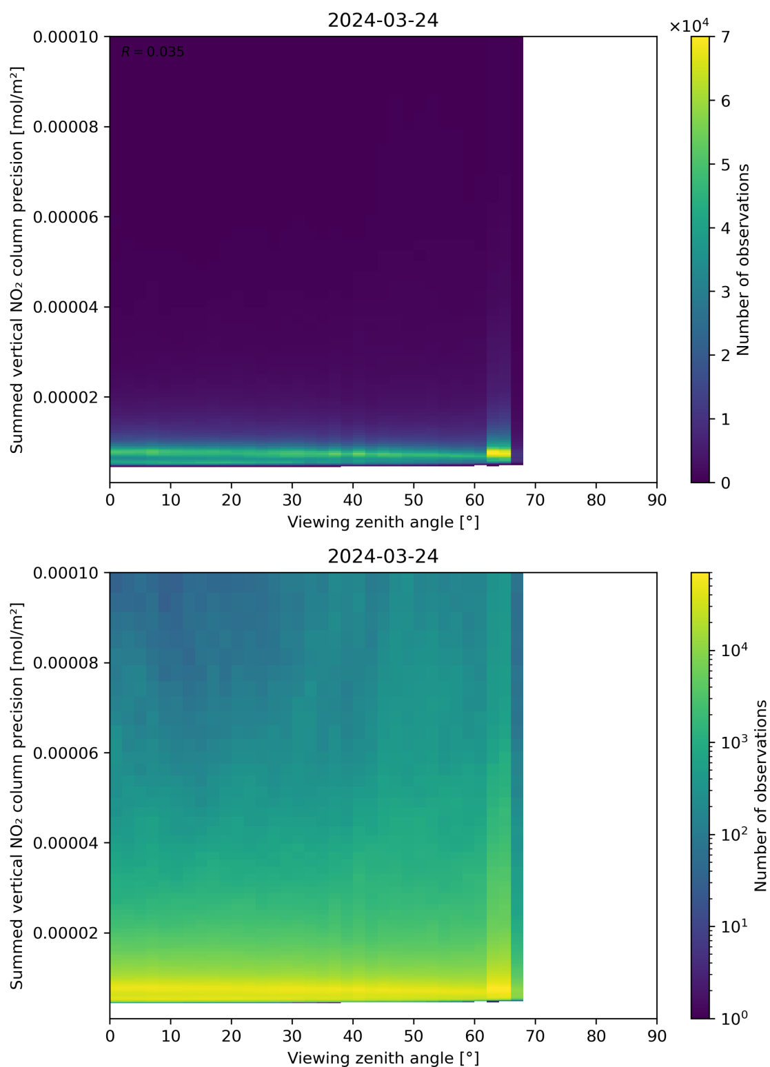
Figure 166: Scatter density plot of “Viewing zenith angle” against “Summed vertical NO 2 column precision” for 2024-03-23 to 2024-03-25.
