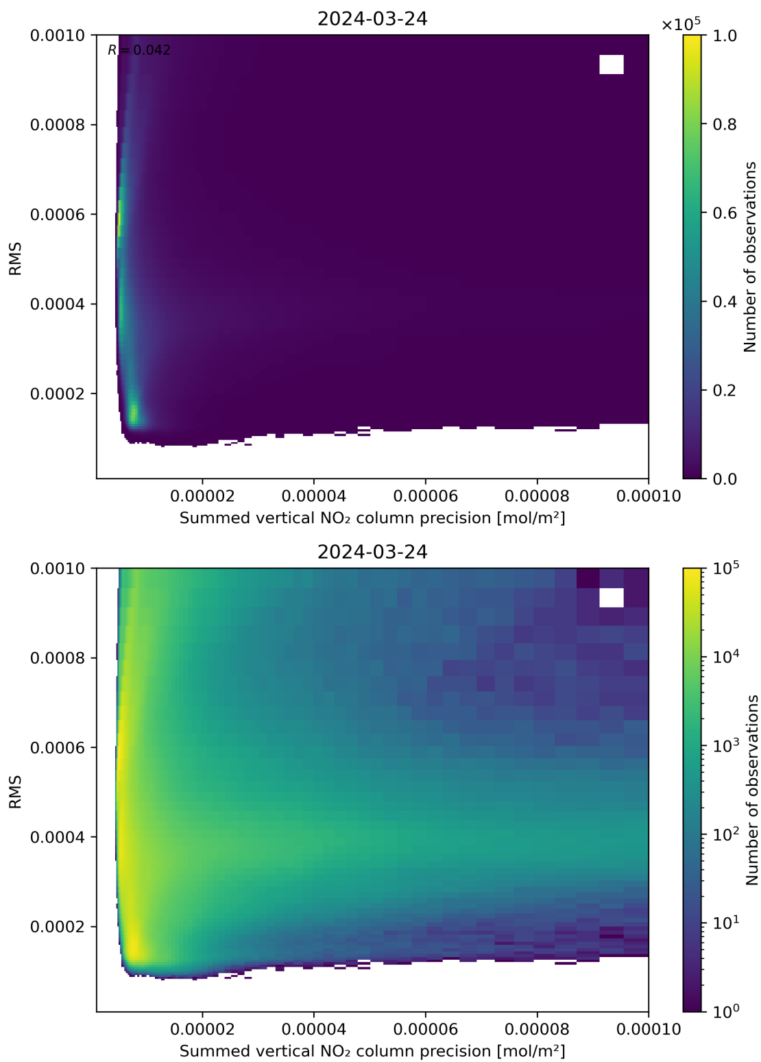
Figure 108: Scatter density plot of “Summed vertical NO 2 column precision” against “RMS” for 2024-03-23 to 2024-03-25.
