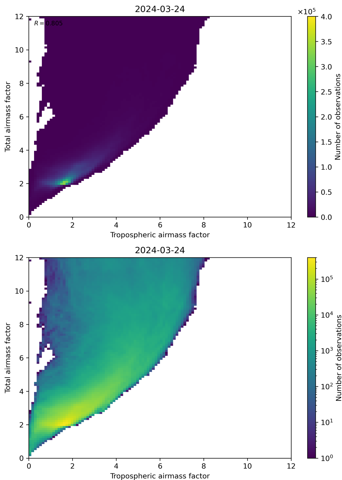
Figure 72: Scatter density plot of “Tropospheric airmass factor” against “Total airmass factor” for 2024-03-23 to 2024-03-25.
