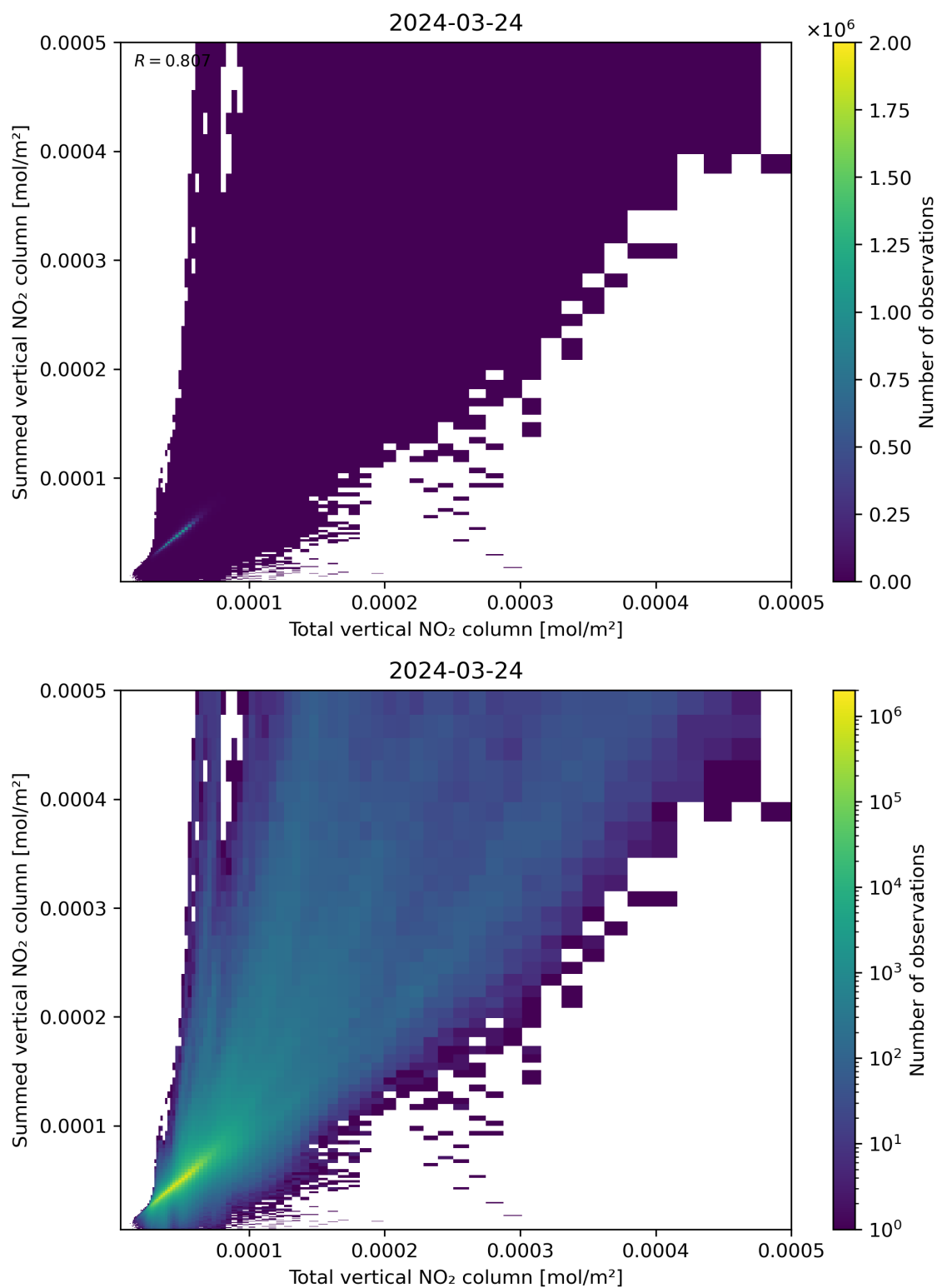
Figure 112: Scatter density plot of “Total vertical NO 2 column” against “Summed vertical NO 2 column” for 2024-03-23 to 2024-03-25.
