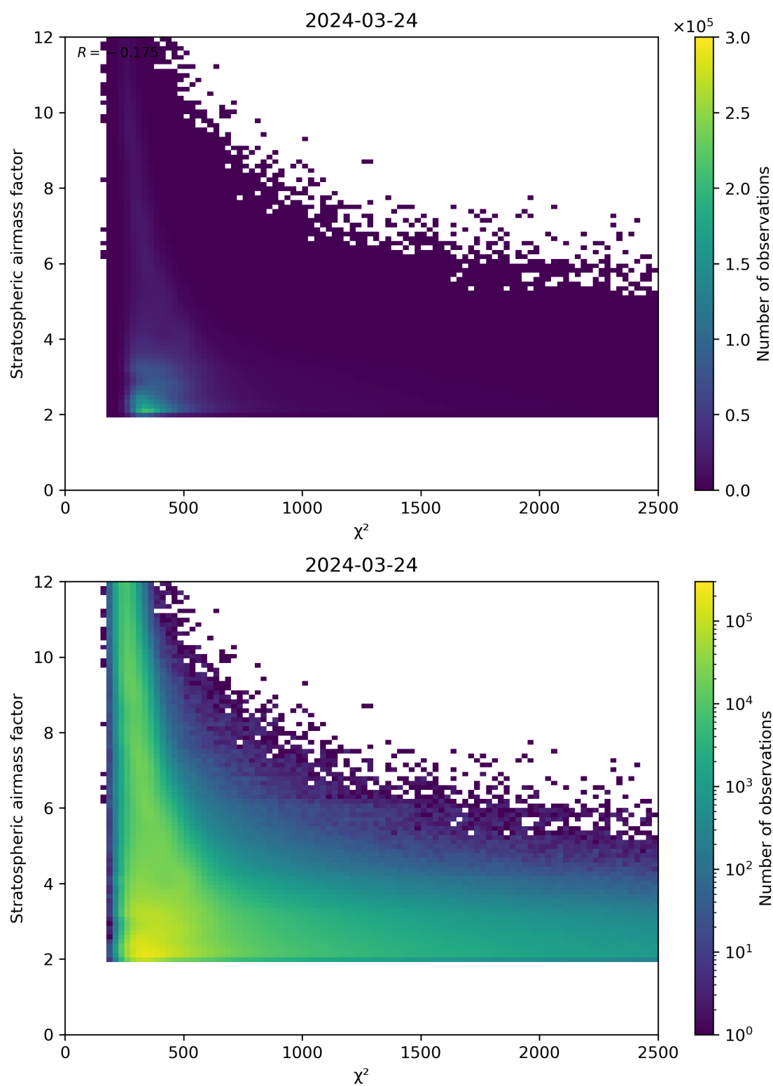
Figure 81: Scatter density plot of “ \chi^2 ” against “Stratospheric airmass factor” for 2024-03-23 to 2024-03-25.
