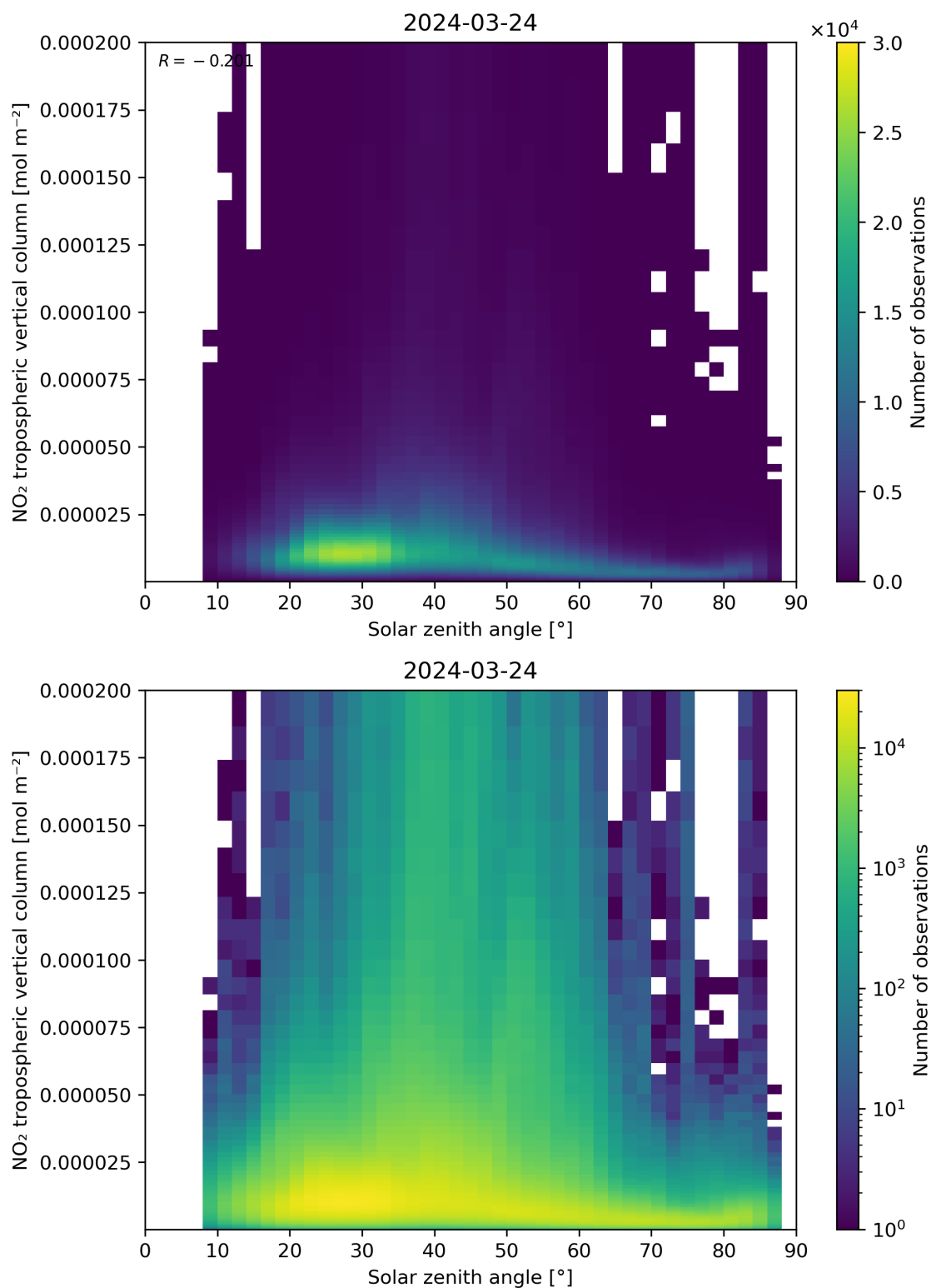
Figure 155: Scatter density plot of “Solar zenith angle” against “NO 2 tropospheric vertical column” for 2024-03-23 to 2024-03-25.
