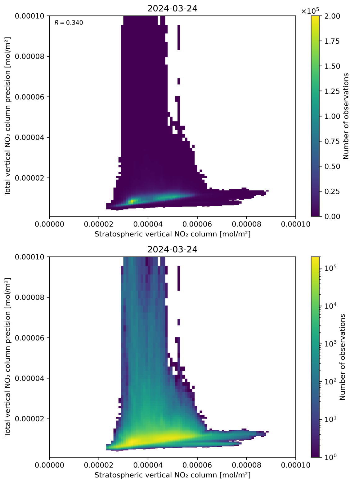
Figure 101: Scatter density plot of “Stratospheric vertical NO 2 column” against “Total vertical NO 2 column precision” for 2024-03-23 to 2024-03-25.
