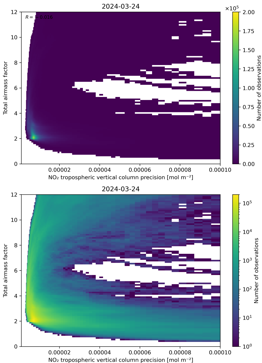
Figure 132: Scatter density plot of “NO 2 tropospheric vertical column precision” against “Total air mass factor” for 2024-03-23 to 2024-03-25.
