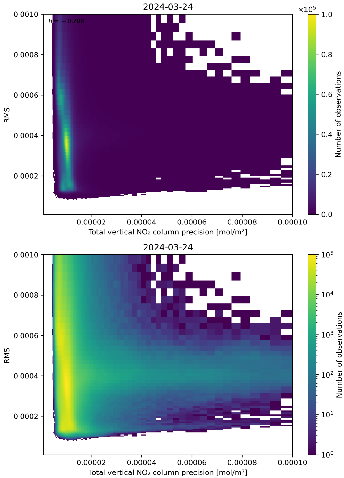
Figure 119: Scatter density plot of “Total vertical NO 2 column precision” against “RMS” for 2024-03-23 to 2024-03-25.
