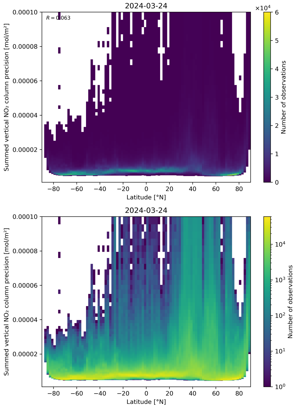
Figure 89: Scatter density plot of “Latitude” against “Summed vertical NO 2 column precision” for 2024-03-23 to 2024-03-25.
