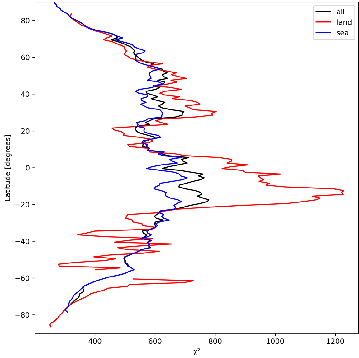
Figure 25: Zonal average of “ \chi^2 ” for 2024-03-23 to 2024-03-25.
