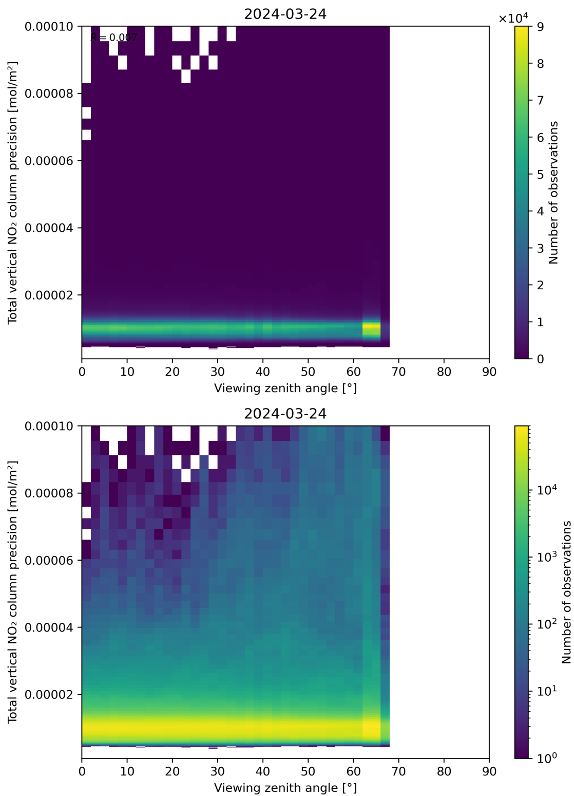
Figure 168: Scatter density plot of “Viewing zenith angle” against “Total vertical NO 2 column precision” for 2024-03-23 to 2024-03-25.
