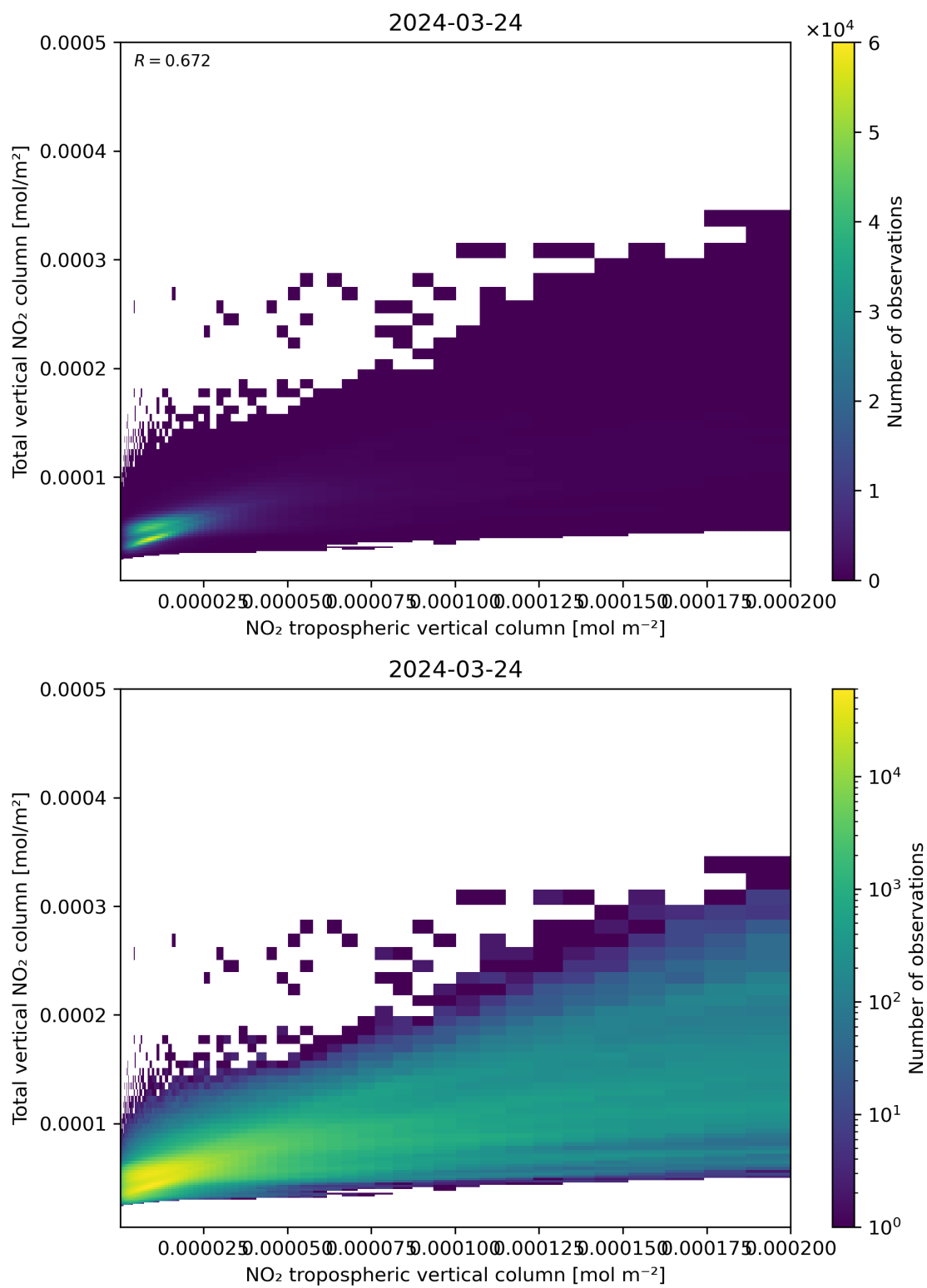
Figure 128: Scatter density plot of “NO 2 tropospheric vertical column” against “Total vertical NO 2 column” for 2024-03-23 to 2024-03-25.
