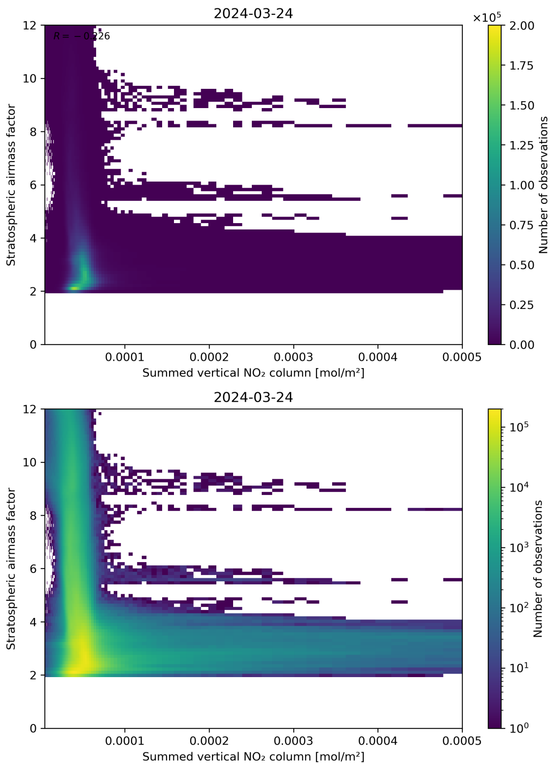
Figure 103: Scatter density plot of “Summed vertical NO 2 column” against “Stratospheric airmass factor” for 2024-03-23 to 2024-03-25.
