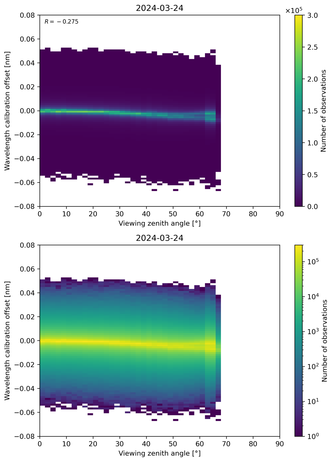
Figure 173: Scatter density plot of “Viewing zenith angle” against “Wavelength calibration offset” for 2024-03-23 to 2024-03-25.
