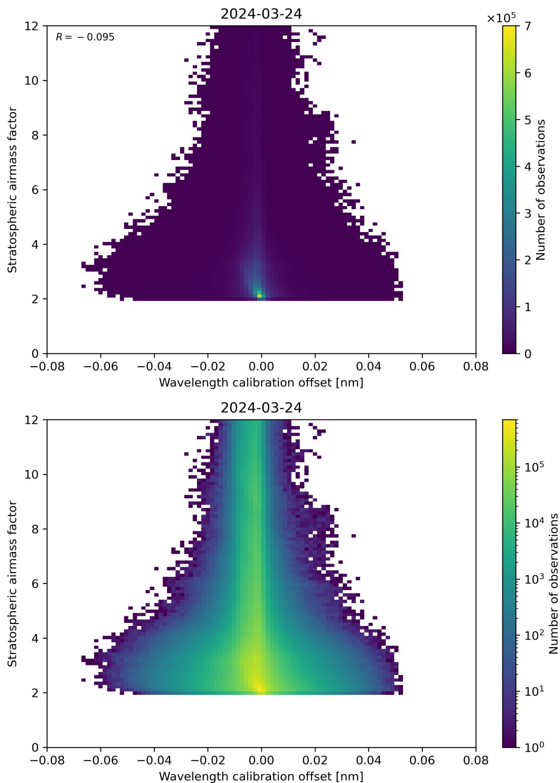
Figure 174: Scatter density plot of “Wavelength calibration offset” against “Stratospheric air mass factor” for 2024-03-23 to 2024-03-25.
