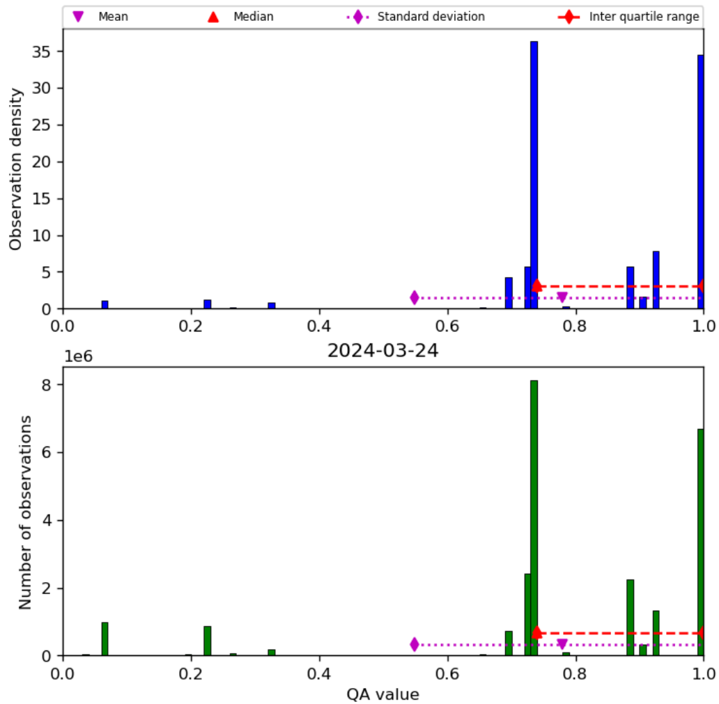
Figure 28: Histogram of “QA value” for 2024-03-23 to 2024-03-25
