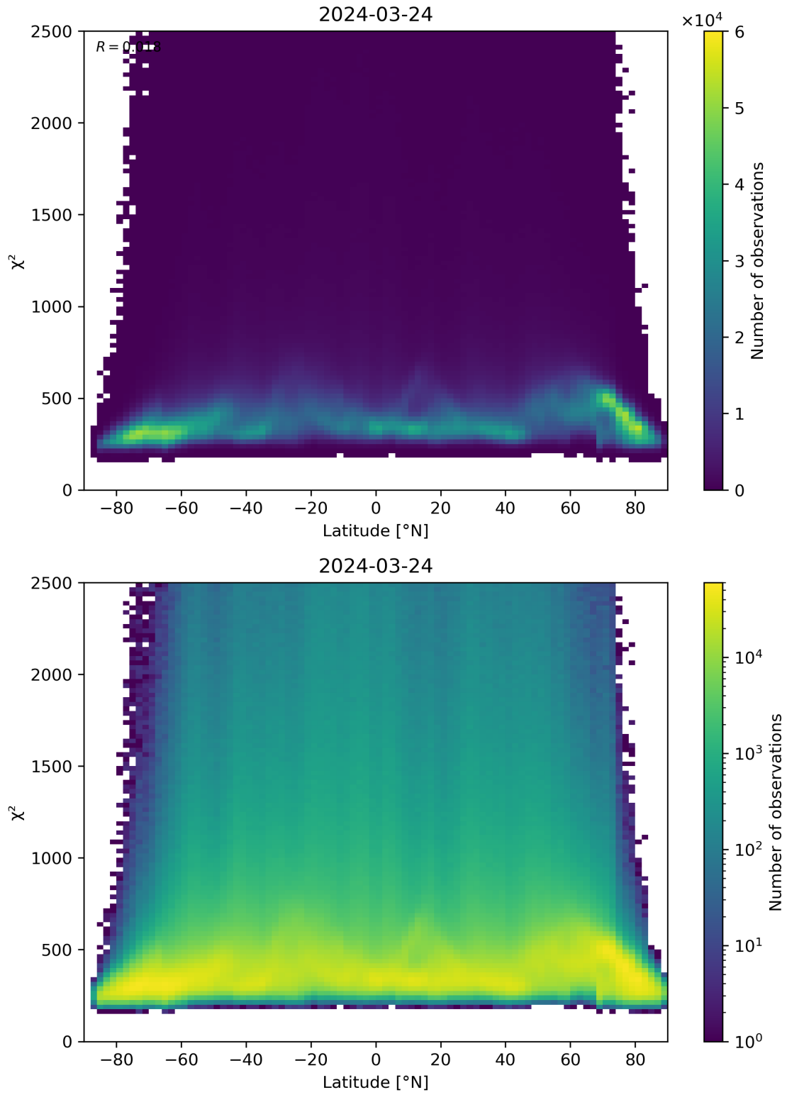
Figure 86: Scatter density plot of “Latitude” against “ \chi^2 ” for 2024-03-23 to 2024-03-25.
