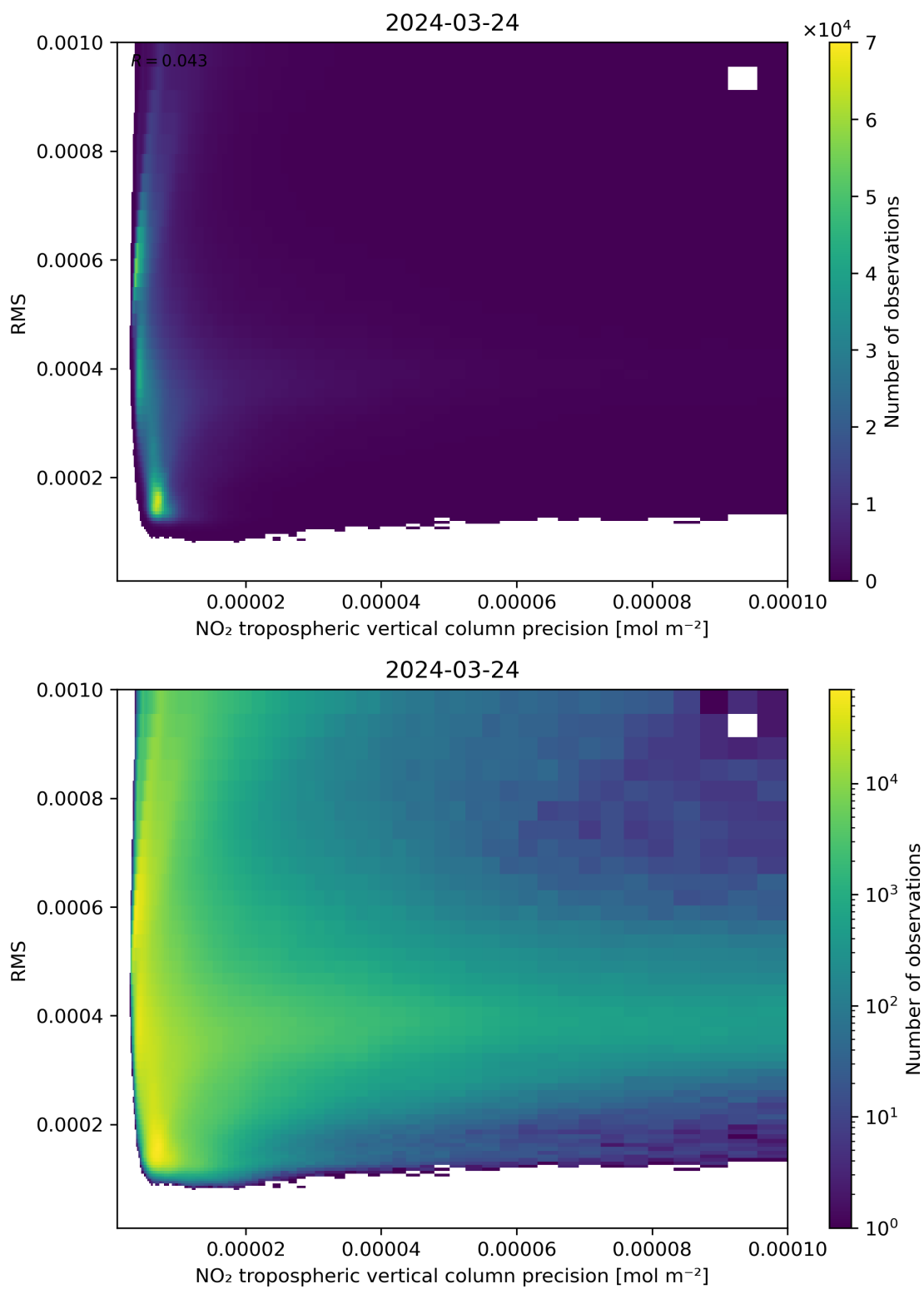
Figure 140: Scatter density plot of “NO 2 tropospheric vertical column precision” against “RMS” for 2024-03-23 to 2024-03-25.
