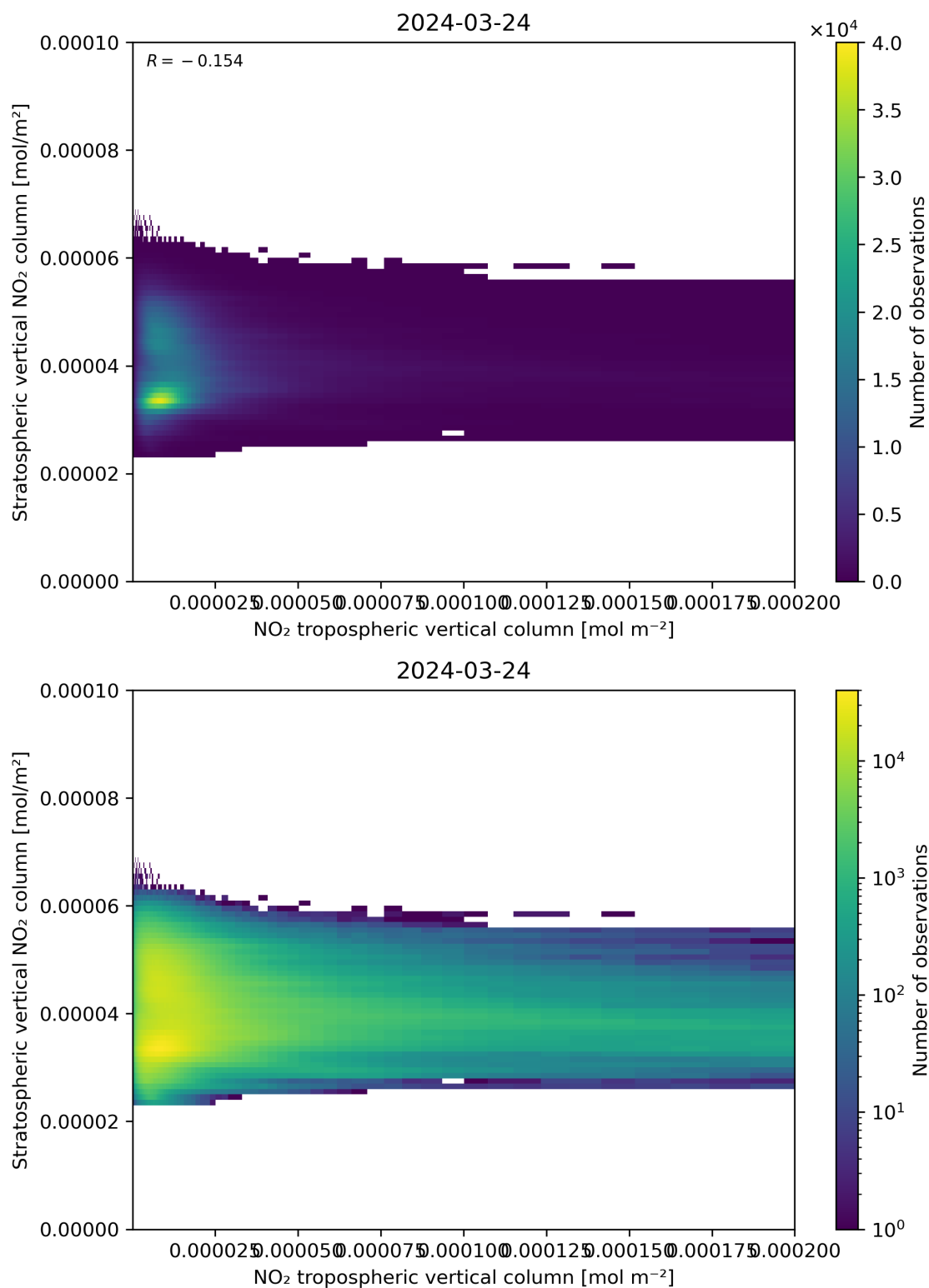
Figure 125: Scatter density plot of “NO 2 tropospheric vertical column” against “Stratospheric vertical NO 2 column” for 2024-03-23 to 2024-03-25.
