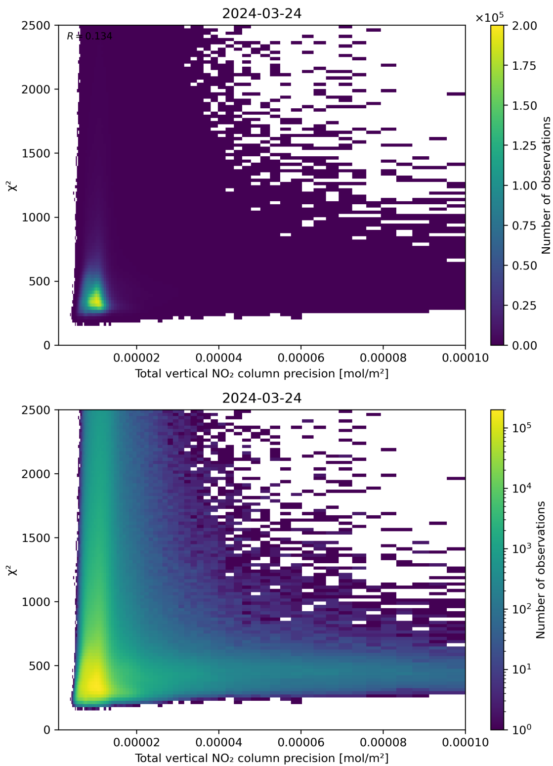
Figure 116: Scatter density plot of “Total vertical NO 2 column precision” against “ \chi^2 ” for 2024-03-23 to 2024-03-25.
