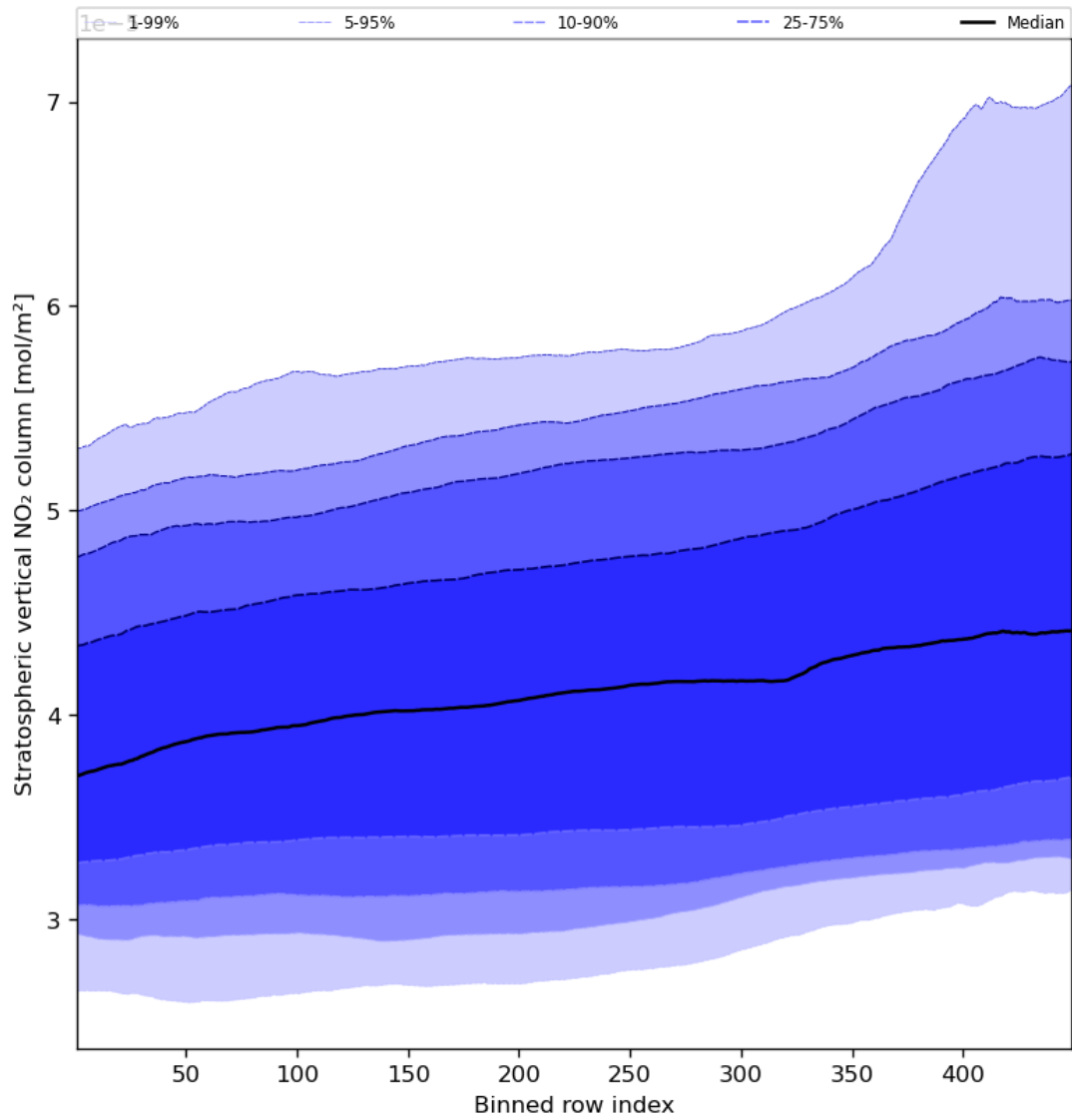
Figure 53: Along track statistics of “Stratospheric vertical NO 2 column” for 2024-03-23 to 2024-03-25
