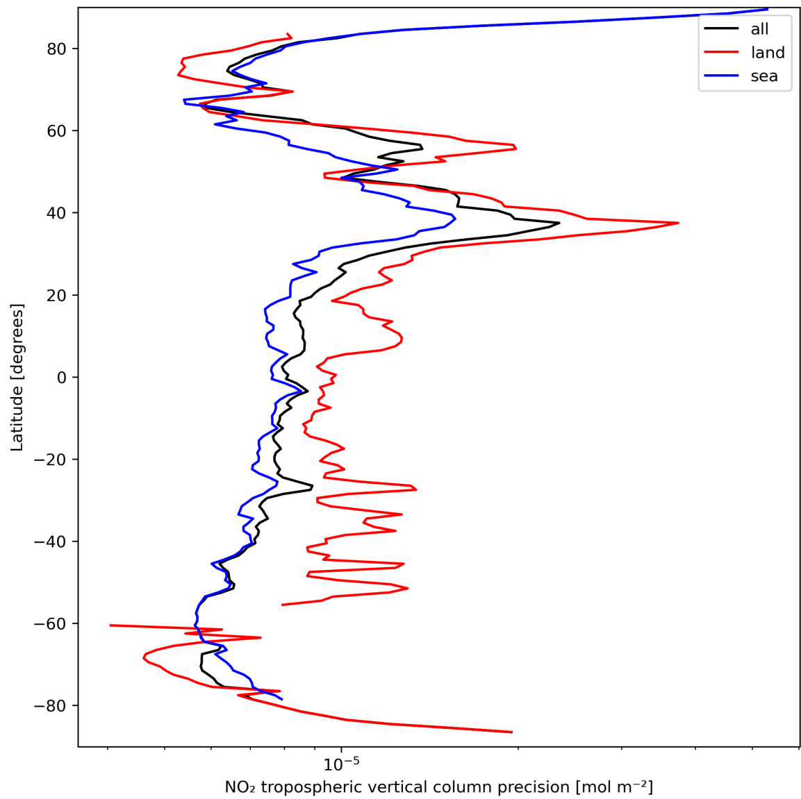
Figure 13: Zonal average of “NO 2 tropospheric vertical column precision” for 2024-03-23 to 2024-03-25.
