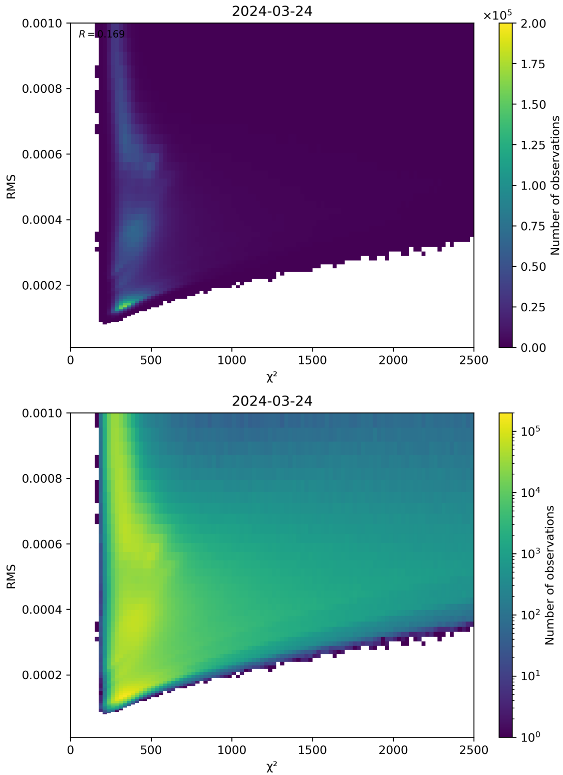
Figure 82: Scatter density plot of “ \chi^2 ” against “RMS” for 2024-03-23 to 2024-03-25.
