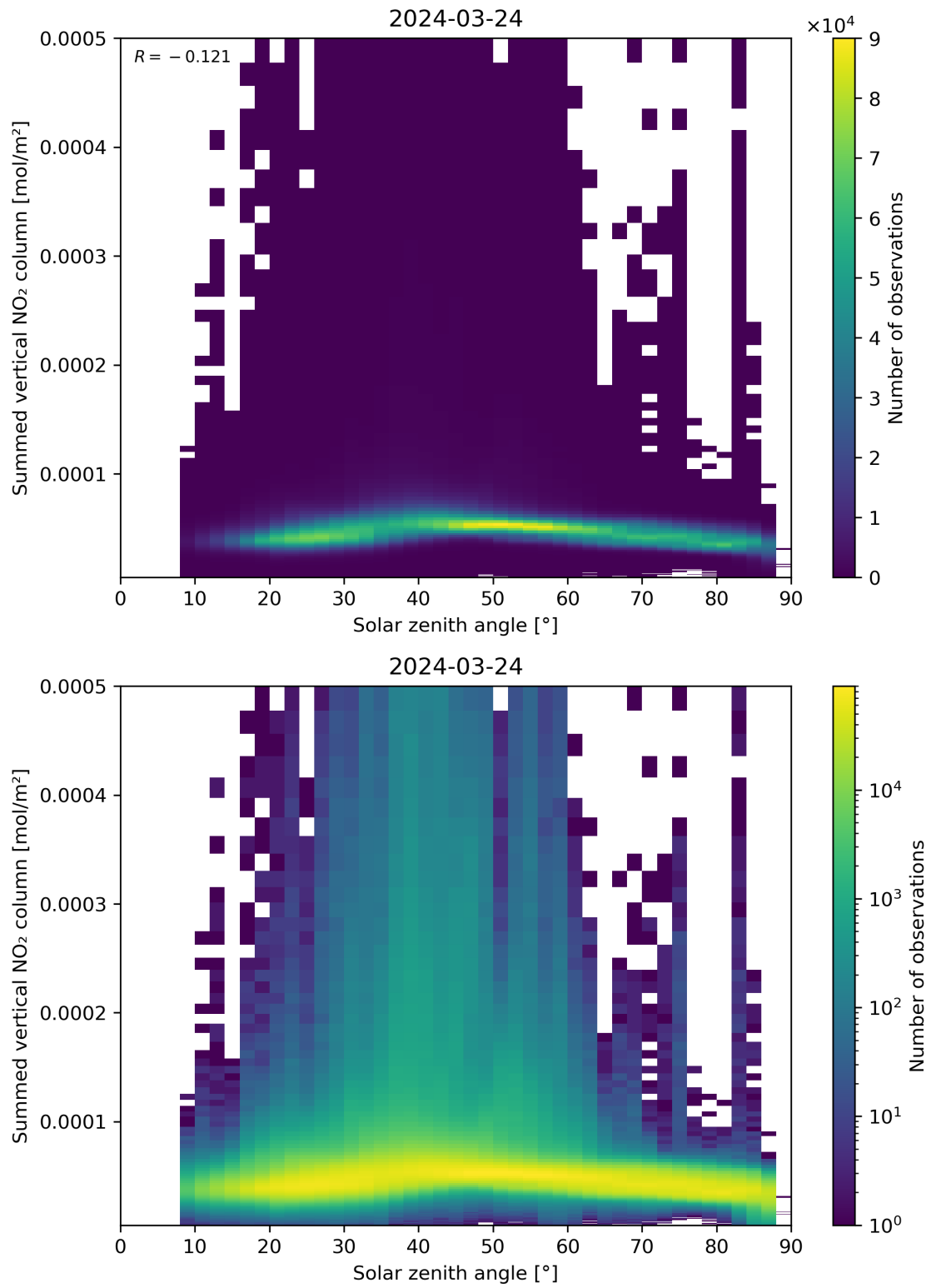
Figure 151: Scatter density plot of “Solar zenith angle” against “Summed vertical NO 2 column” for 2024-03-23 to 2024-03-25.
