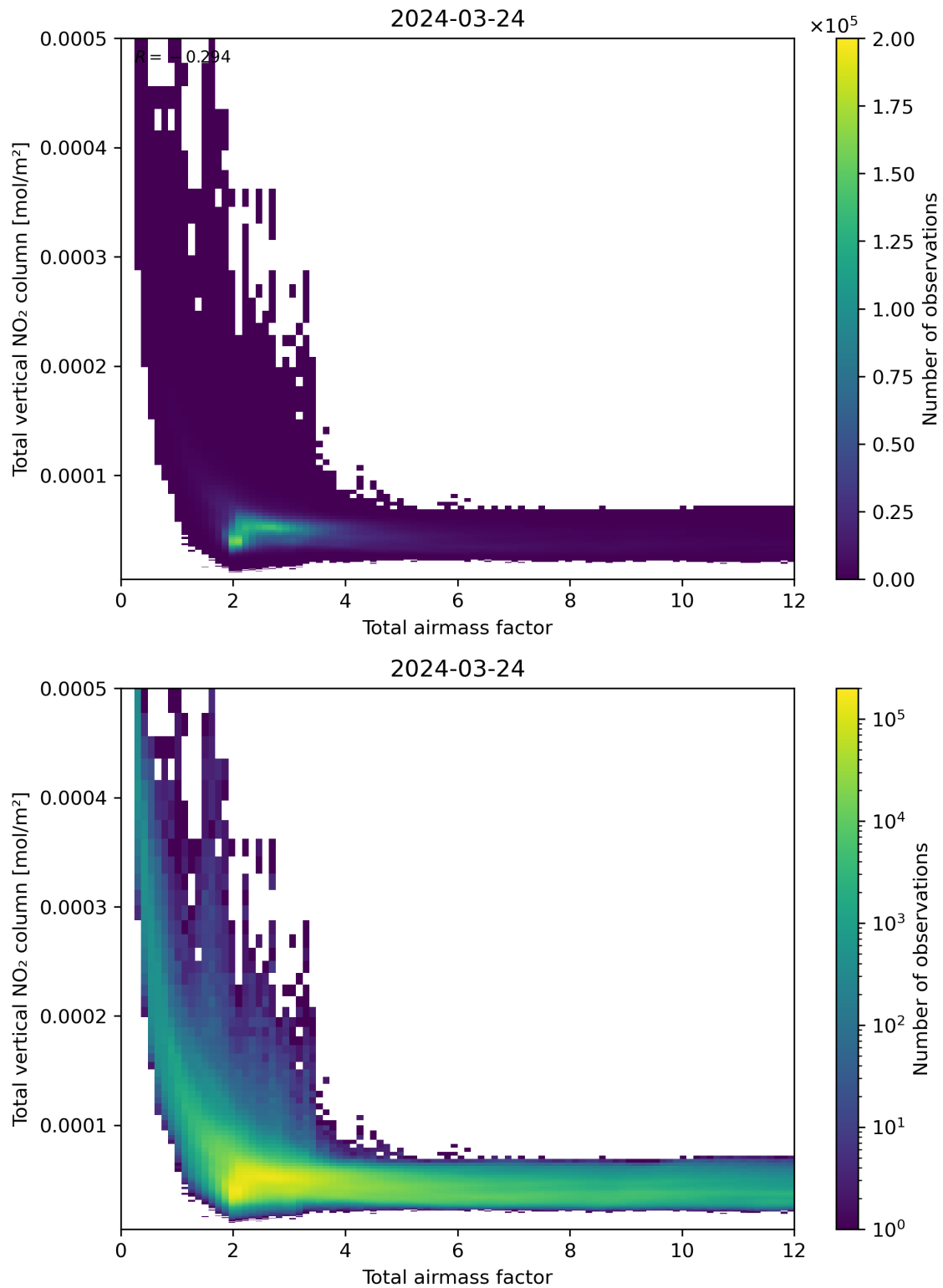
Figure 67: Scatter density plot of “Total airmass factor” against “Total vertical NO 2 column” for 2024-03-23 to 2024-03-25.
