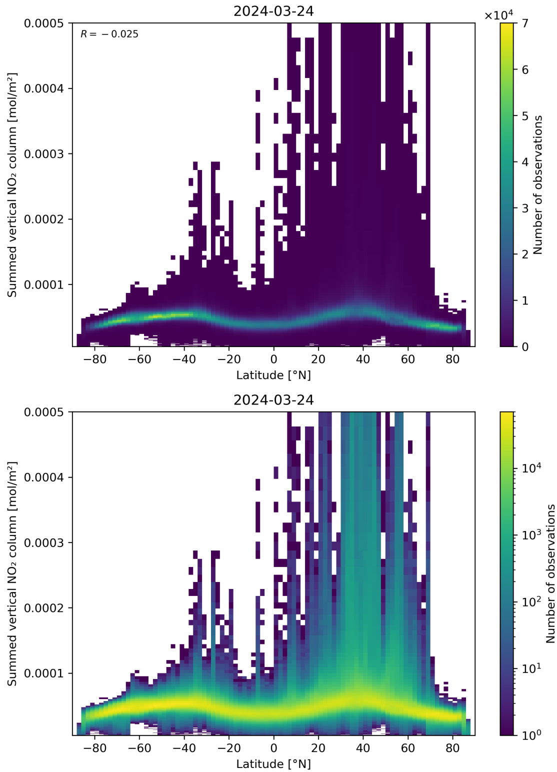
Figure 88: Scatter density plot of “Latitude” against “Summed vertical NO 2 column” for 2024-03-23 to 2024-03-25.
