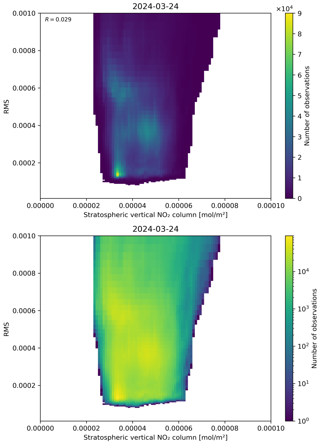
Figure 102: Scatter density plot of “Stratospheric vertical NO 2 column” against “RMS” for 2024-03-23 to 2024-03-25.
