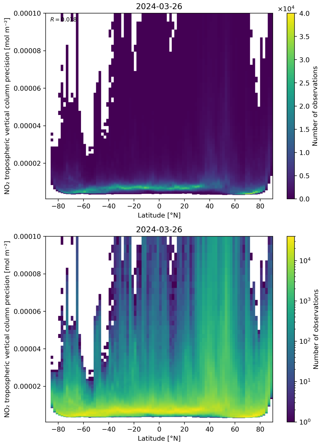
Figure 93: Scatter density plot of “Latitude” against “NO 2 tropospheric vertical column precision” for 2024-03-25 to 2024-03-27.
