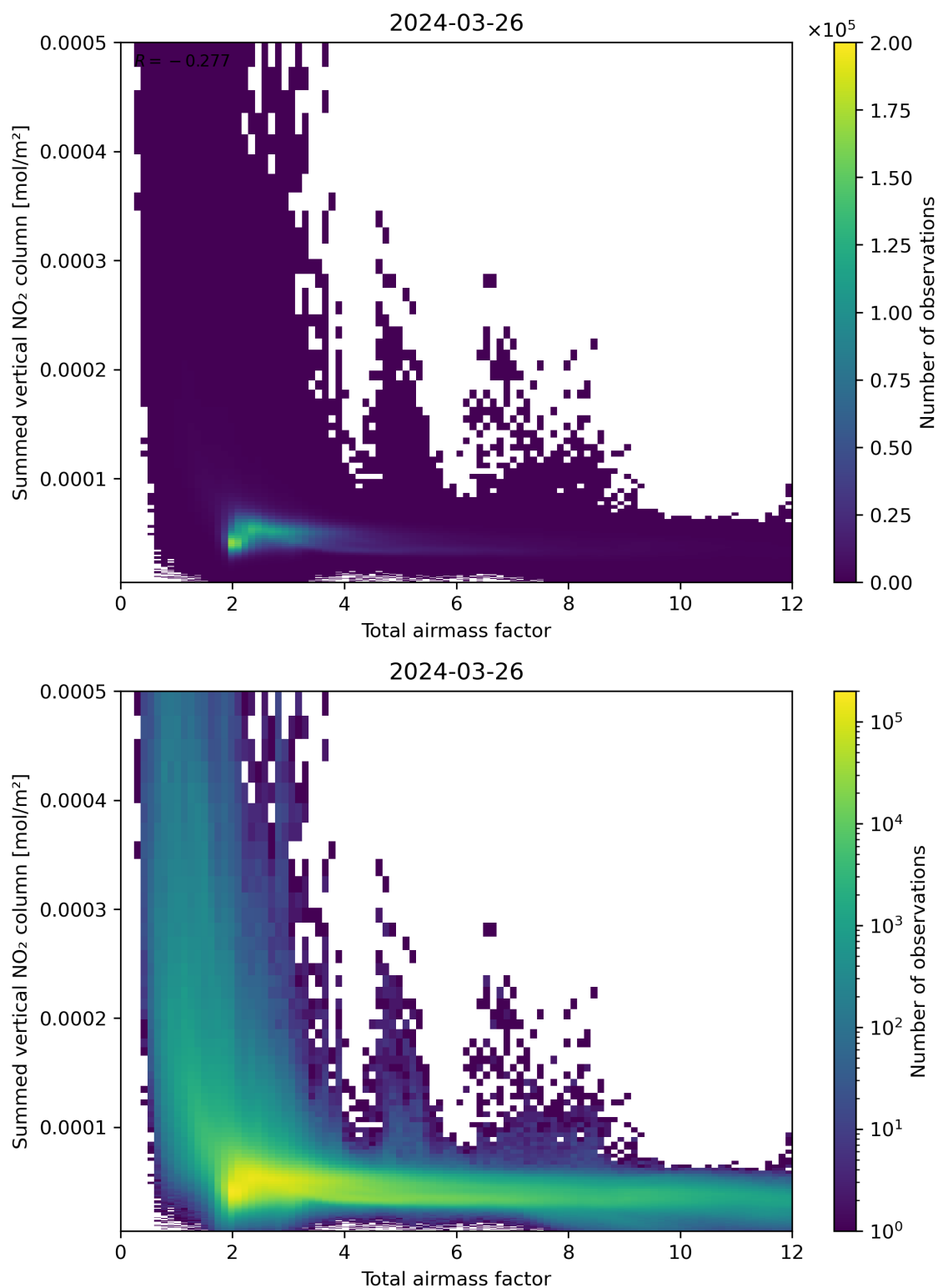
Figure 65: Scatter density plot of “Total airmass factor” against “Summed vertical NO 2 column” for 2024-03-25 to 2024-03-27.
