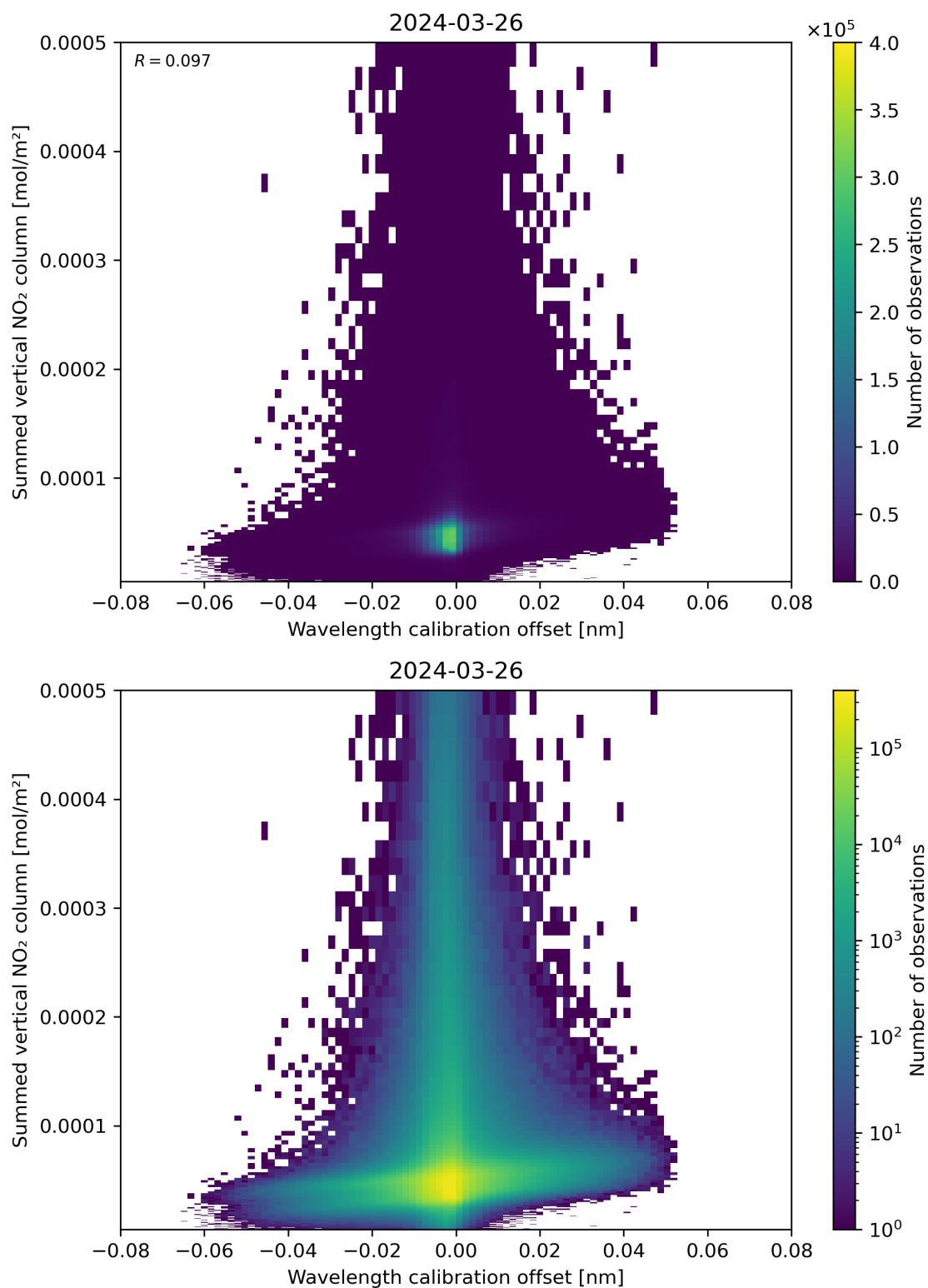
Figure 177: Scatter density plot of “Wavelength calibration offset” against “Summed vertical NO 2 column” for 2024-03-25 to 2024-03-27.
