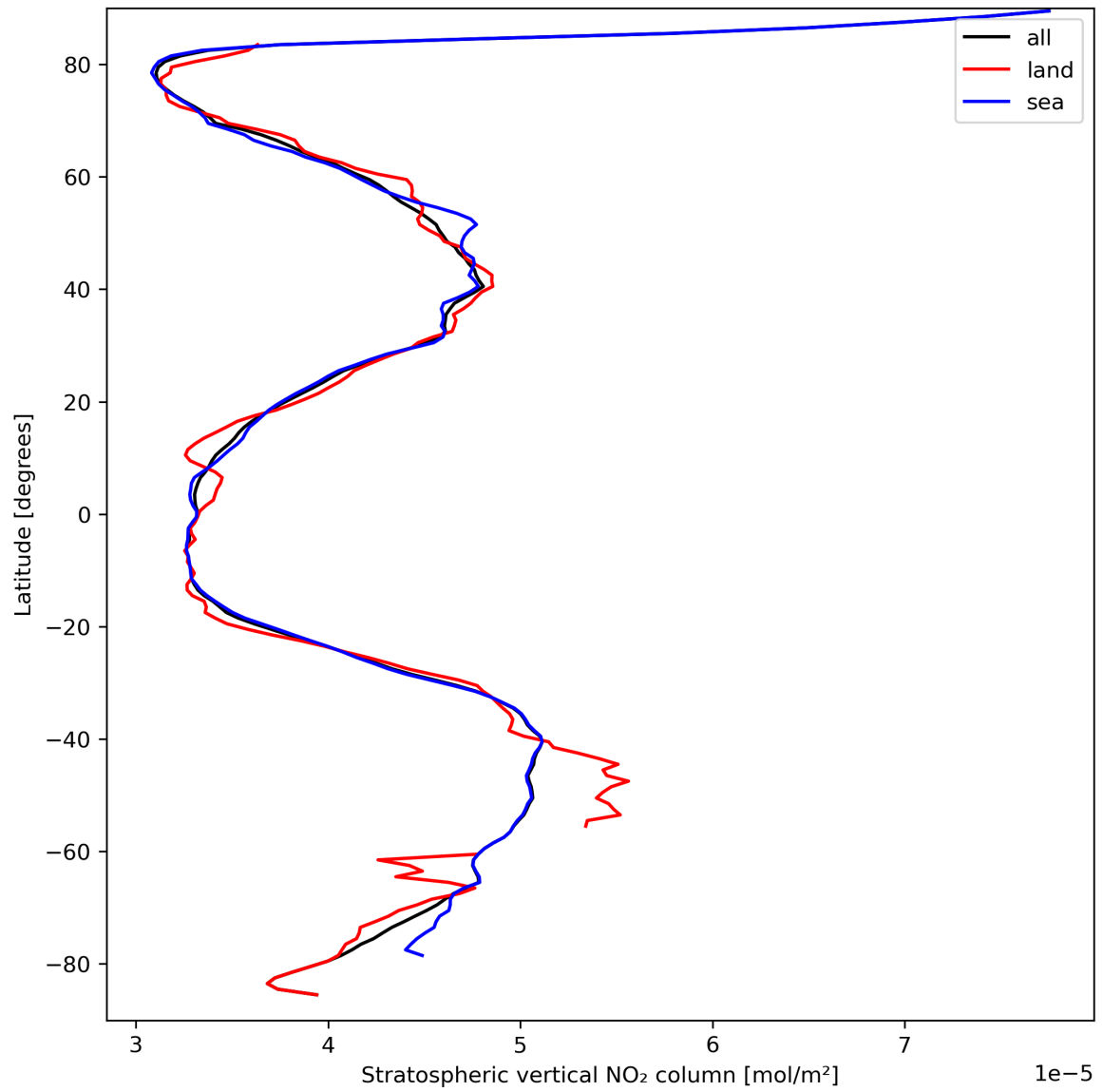
Figure 19: Zonal average of “Stratospheric vertical NO 2 column” for 2024-03-25 to 2024-03-27.
