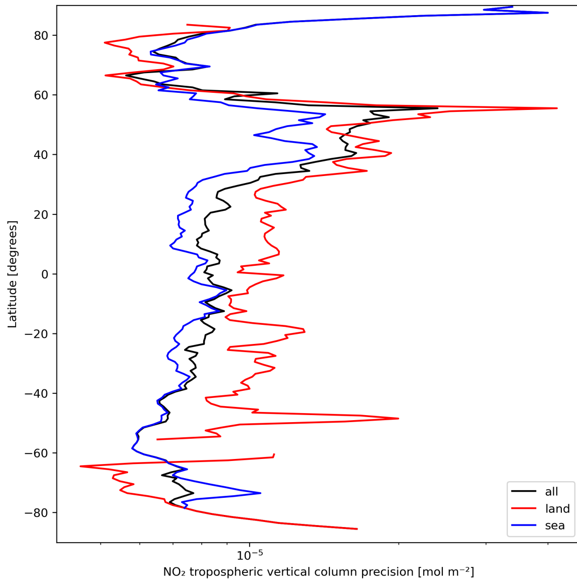
Figure 13: Zonal average of “NO 2 tropospheric vertical column precision” for 2024-03-25 to 2024-03-27.
