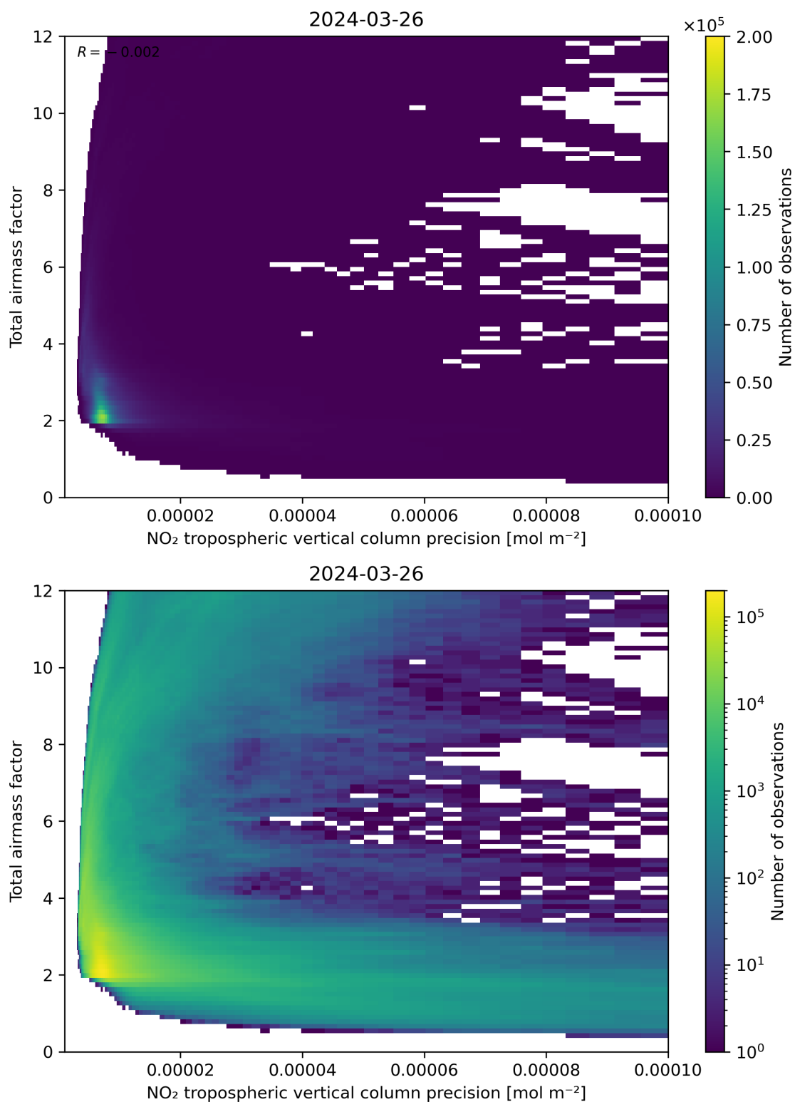
Figure 132: Scatter density plot of “NO 2 tropospheric vertical column precision” against “Total air mass factor” for 2024-03-25 to 2024-03-27.
