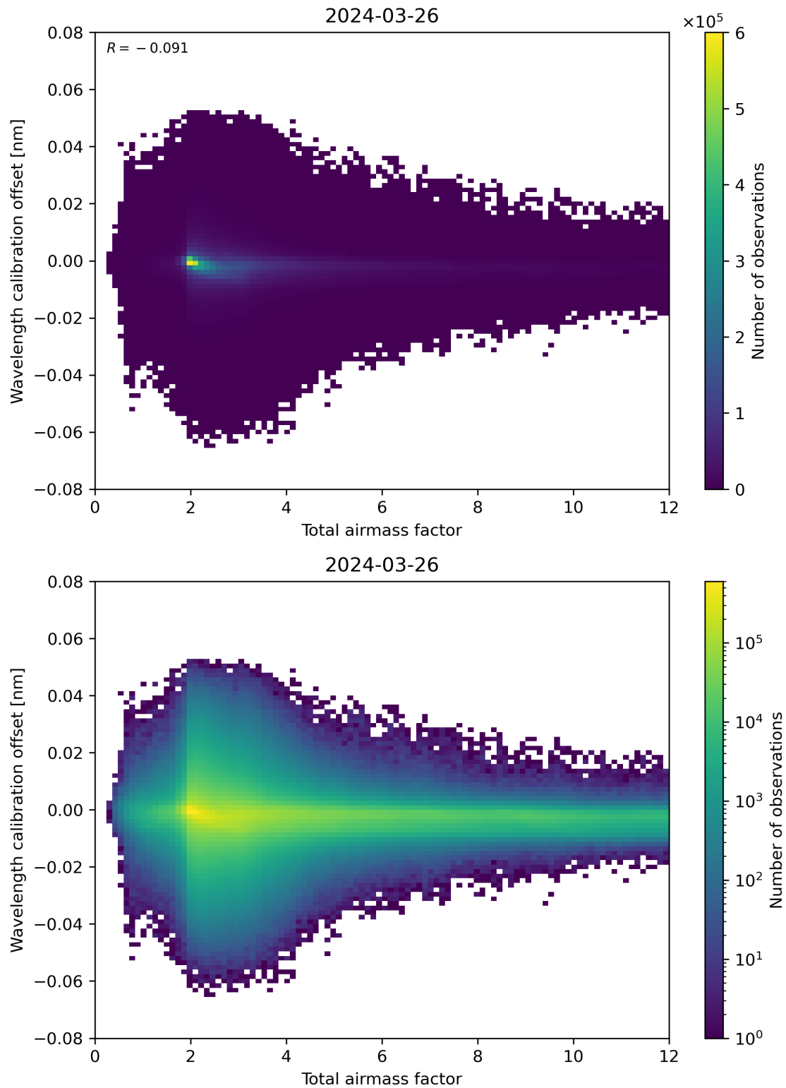
Figure 70: Scatter density plot of “Total airmass factor” against “Wavelength calibration offset” for 2024-03-25 to 2024-03-27.
