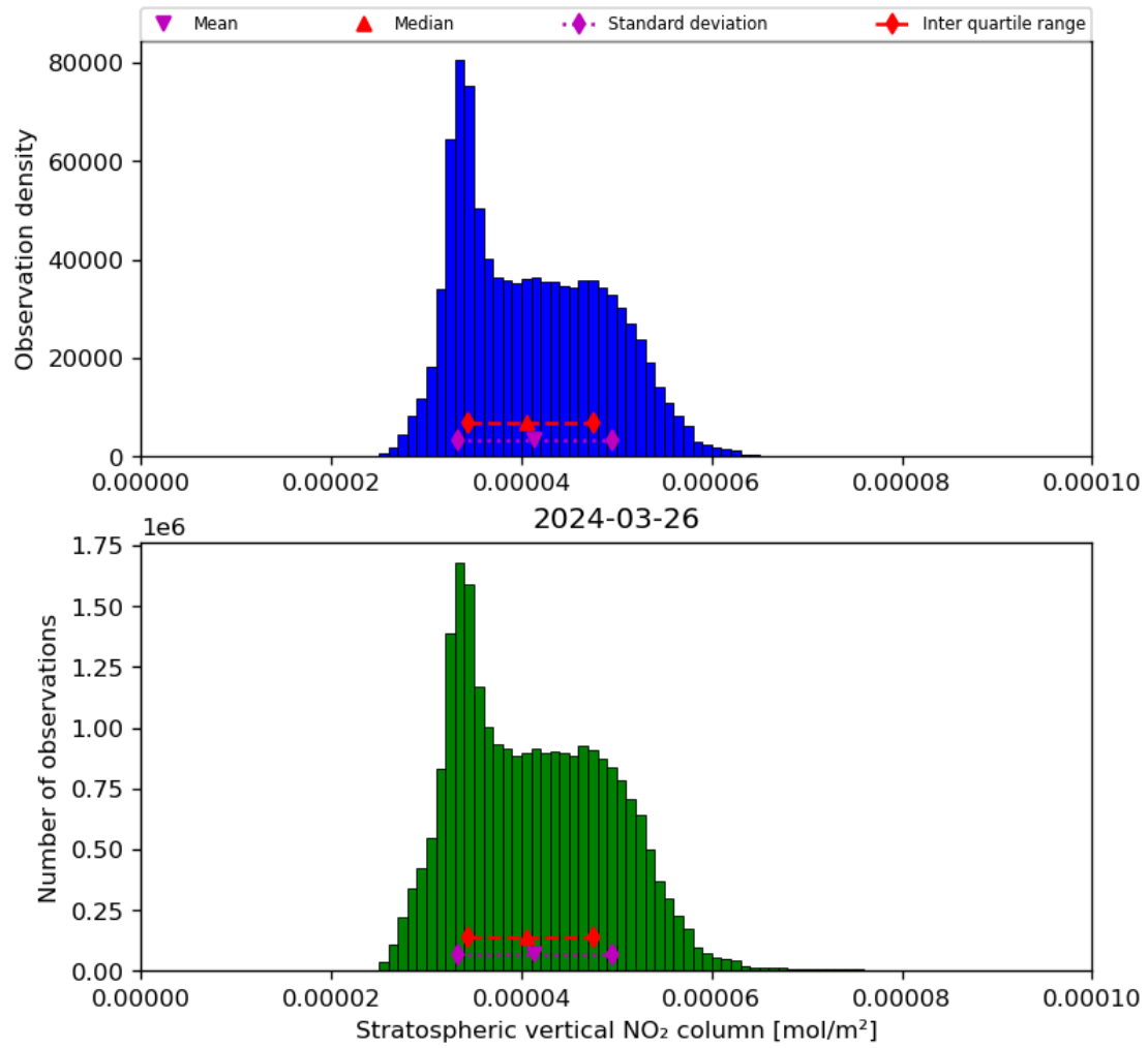
Figure 36: Histogram of “Stratospheric vertical NO 2 column” for 2024-03-25 to 2024-03-27
