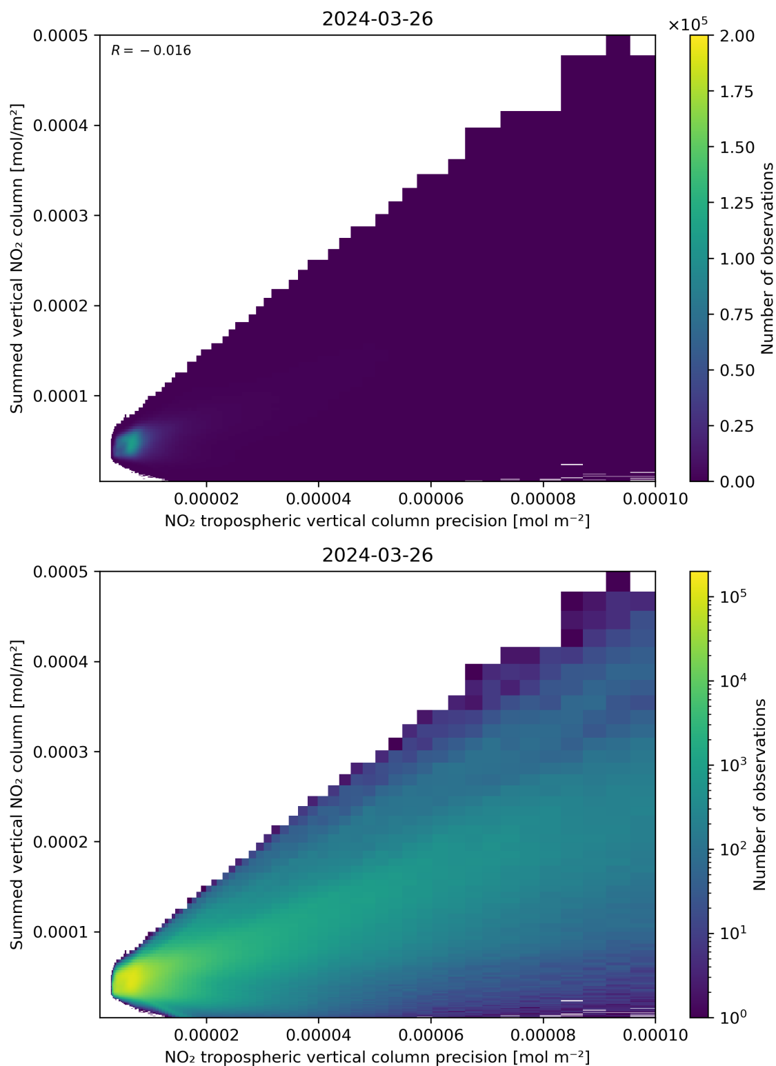
Figure 136: Scatter density plot of “NO 2 tropospheric vertical column precision” against “Summed vertical NO 2 column” for 2024-03-25 to 2024-03-27.
