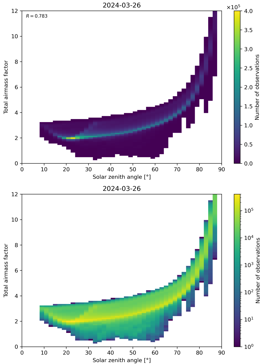
Figure 146: Scatter density plot of “Solar zenith angle” against “Total air mass factor” for 2024-03-25 to 2024-03-27.
