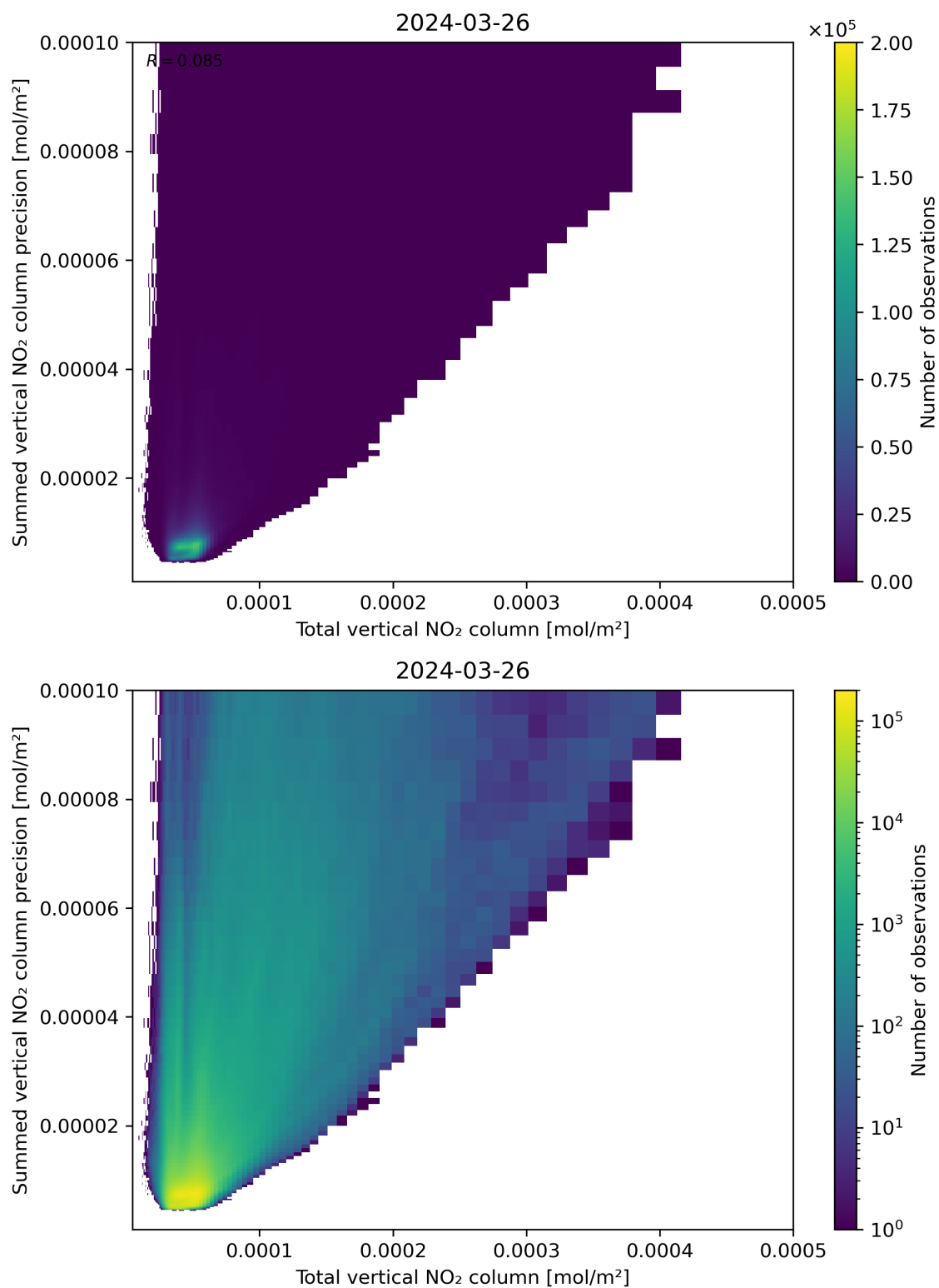
Figure 113: Scatter density plot of “Total vertical NO 2 column” against “Summed vertical NO 2 column precision” for 2024-03-25 to 2024-03-27.
