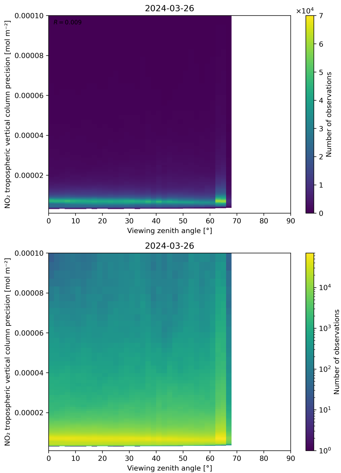
Figure 170: Scatter density plot of “Viewing zenith angle” against “NO 2 tropospheric vertical column precision” for 2024-03-25 to 2024-03-27.
