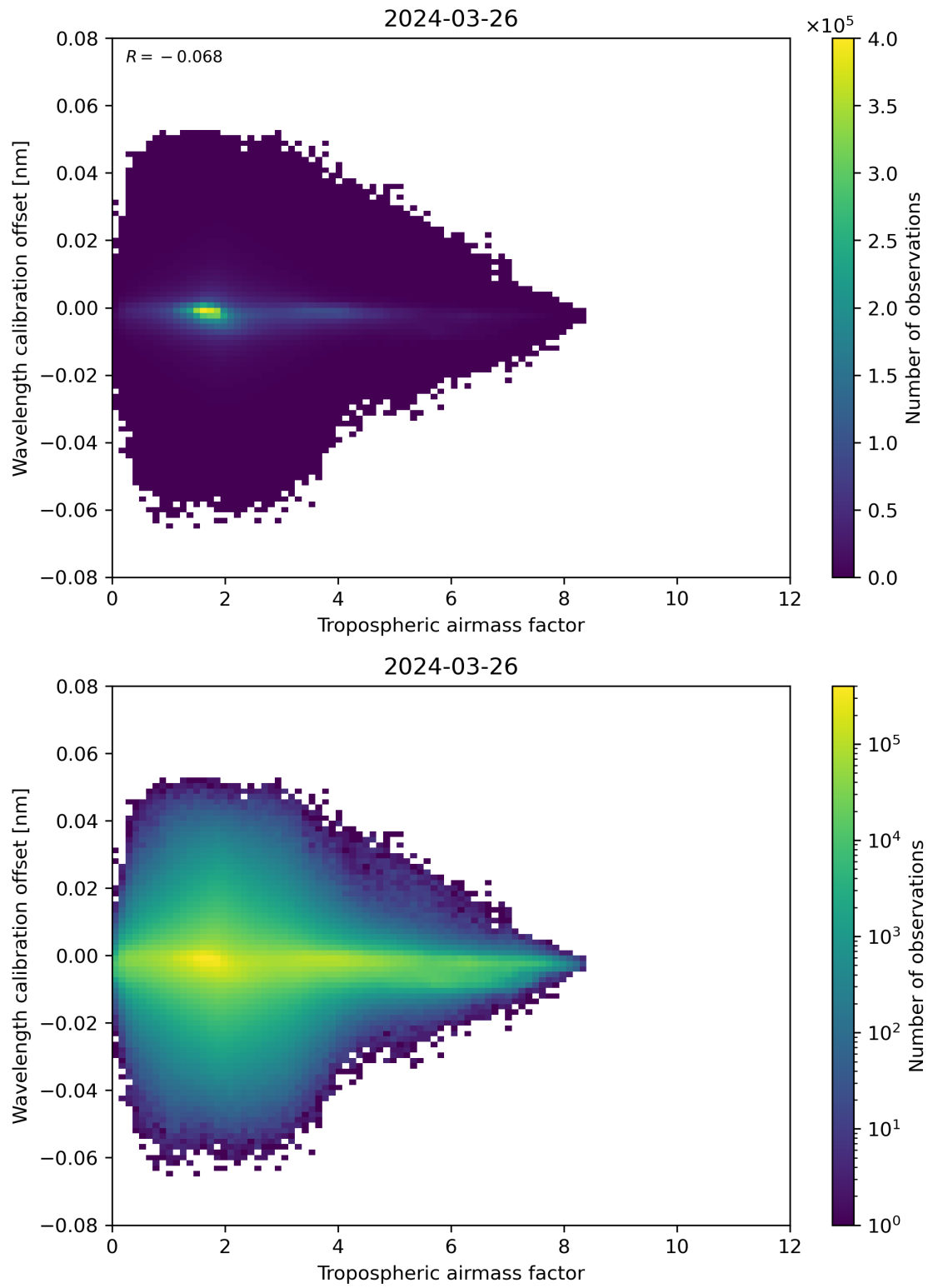
Figure 80: Scatter density plot of “Tropospheric airmass factor” against “Wavelength calibration offset” for 2024-03-25 to 2024-03-27.
