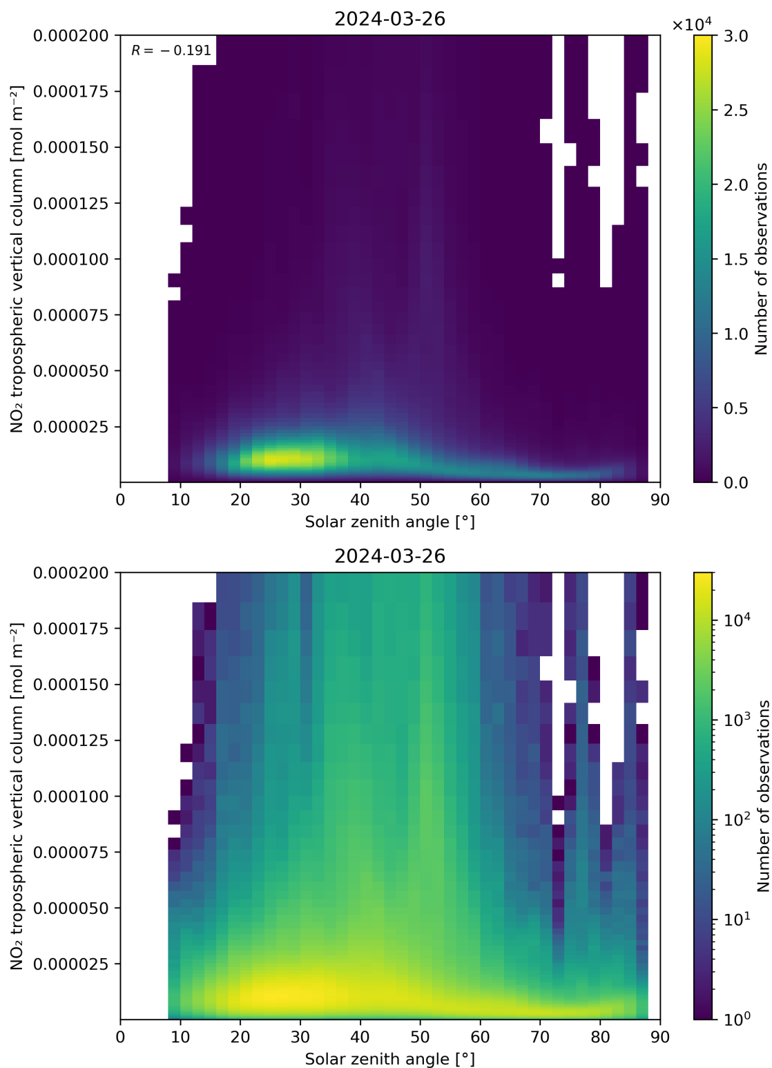
Figure 155: Scatter density plot of “Solar zenith angle” against “NO 2 tropospheric vertical column” for 2024-03-25 to 2024-03-27.
