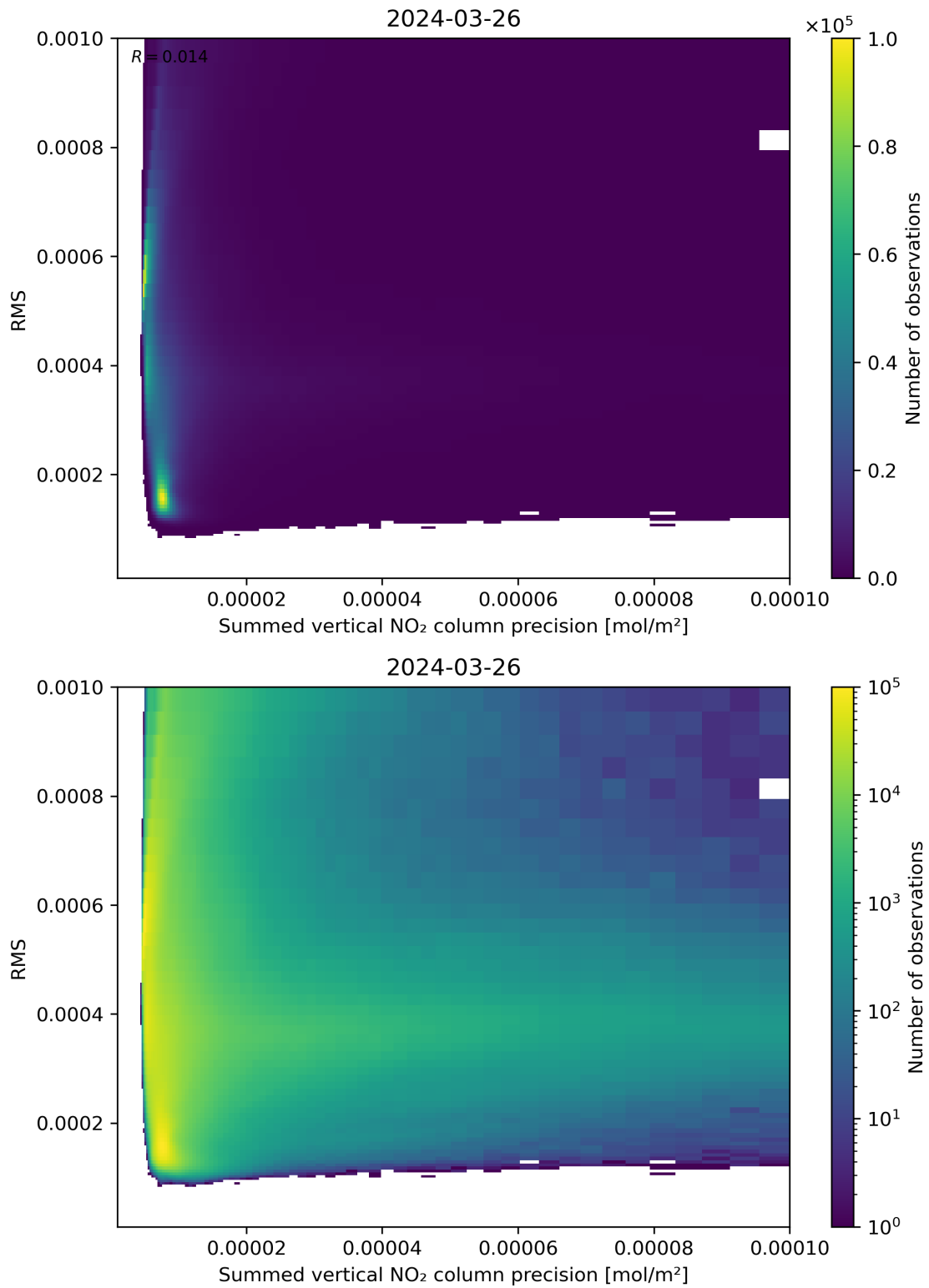
Figure 108: Scatter density plot of “Summed vertical NO 2 column precision” against “RMS” for 2024-03-25 to 2024-03-27.
