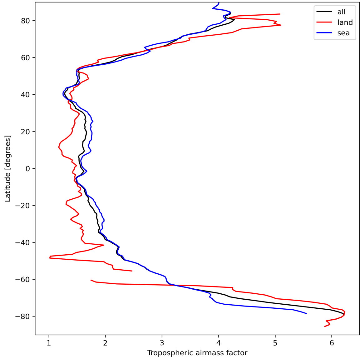
Figure 14: Zonal average of “Tropospheric airmass factor” for 2024-03-25 to 2024-03-27.
