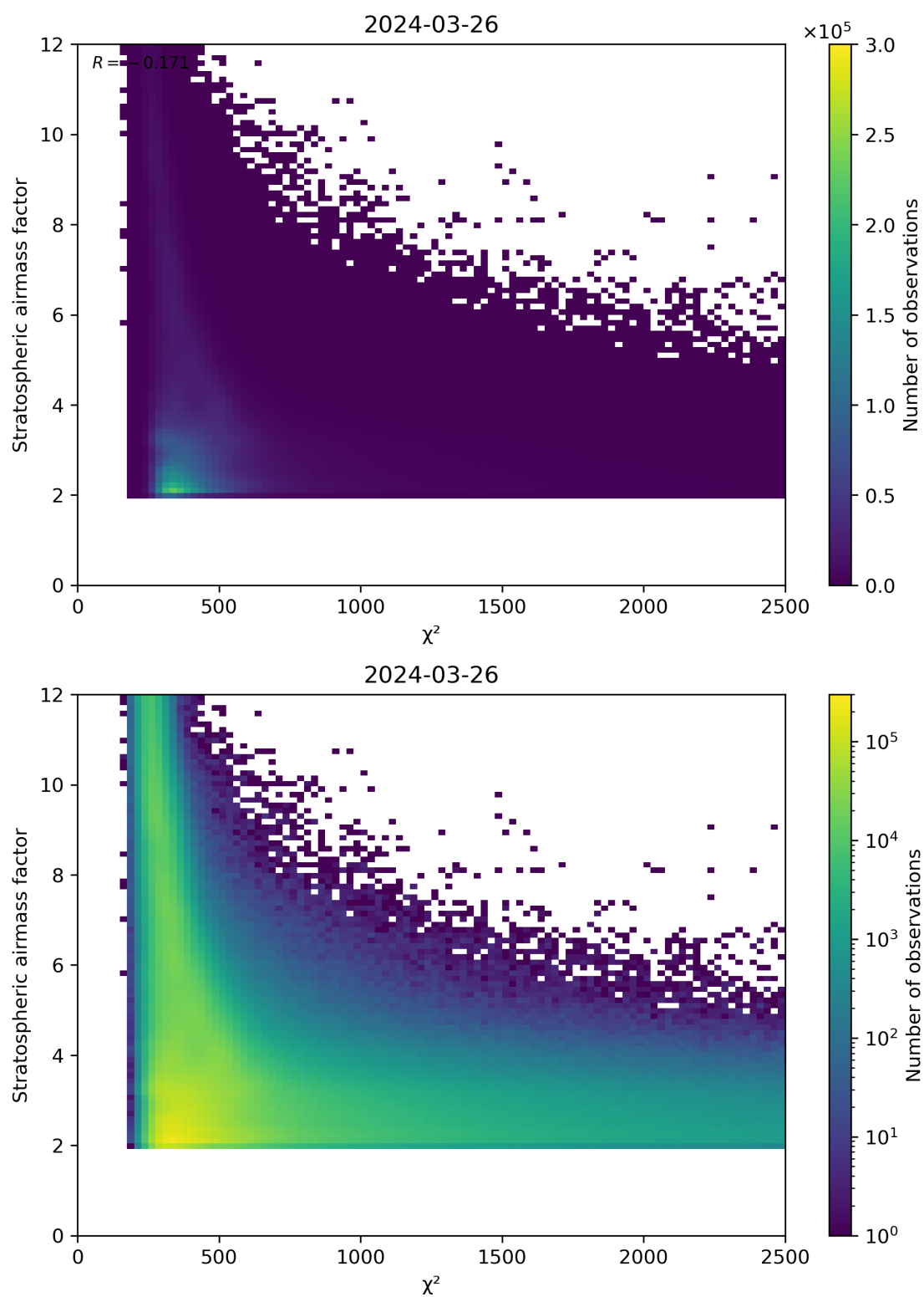
Figure 81: Scatter density plot of “ \chi^2 ” against “Stratospheric airmass factor” for 2024-03-25 to 2024-03-27.
