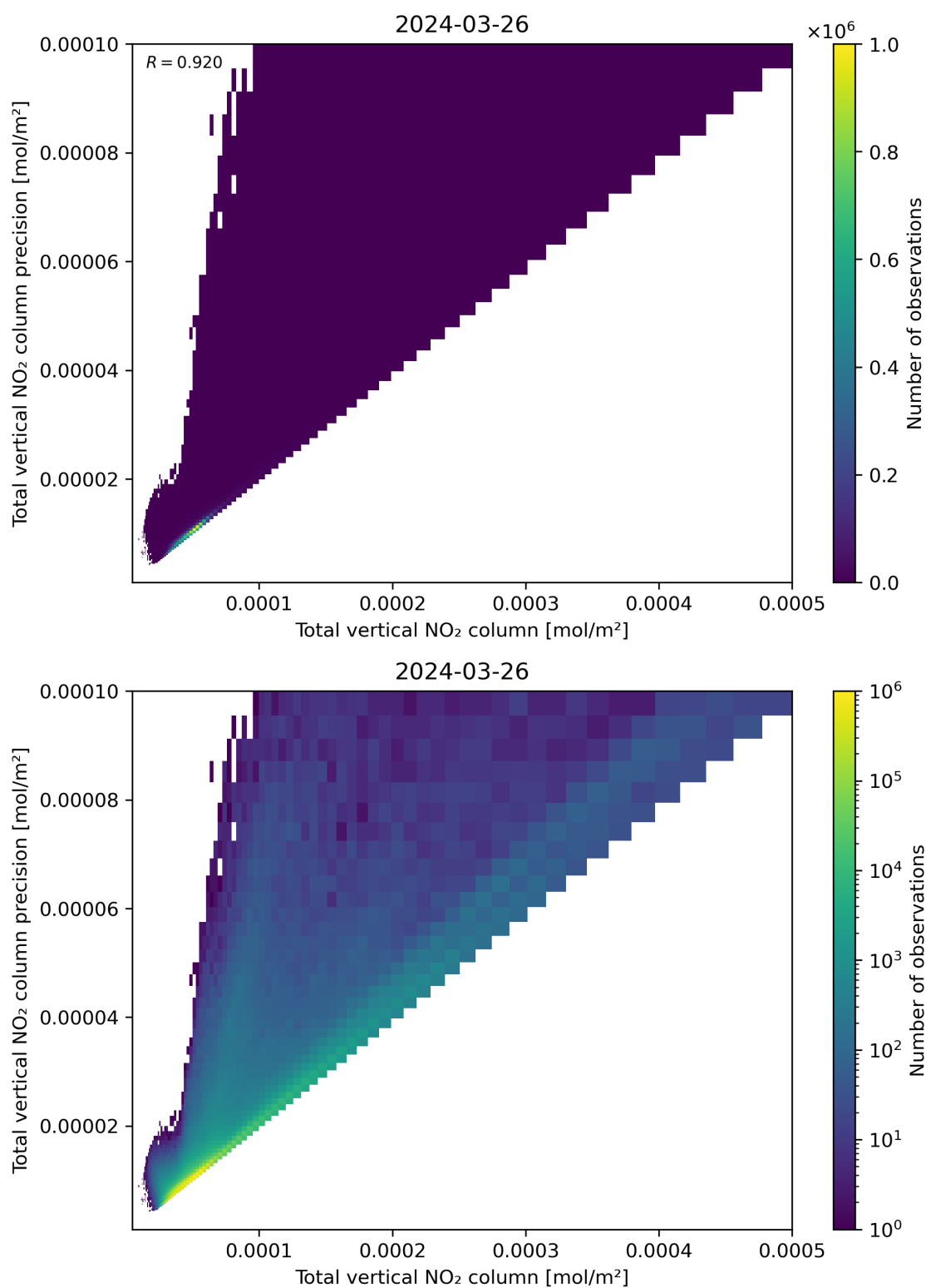
Figure 114: Scatter density plot of “Total vertical NO 2 column” against “Total vertical NO 2 column precision” for 2024-03-25 to 2024-03-27.
