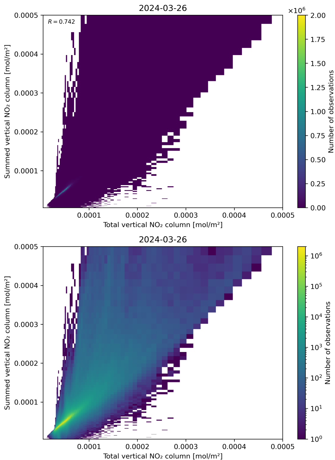
Figure 112: Scatter density plot of “Total vertical NO 2 column” against “Summed vertical NO 2 column” for 2024-03-25 to 2024-03-27.
