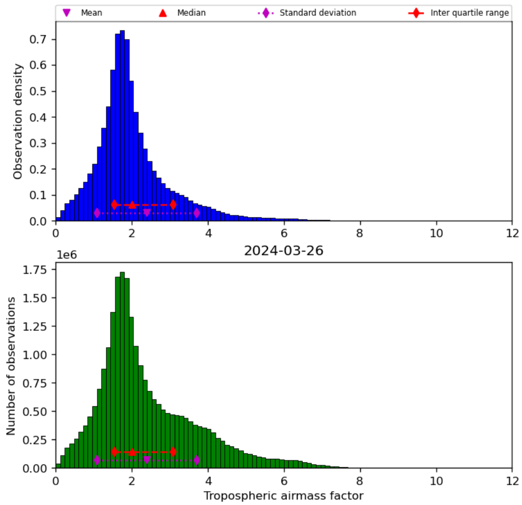
Figure 31: Histogram of “Tropospheric airmass factor” for 2024-03-25 to 2024-03-27
