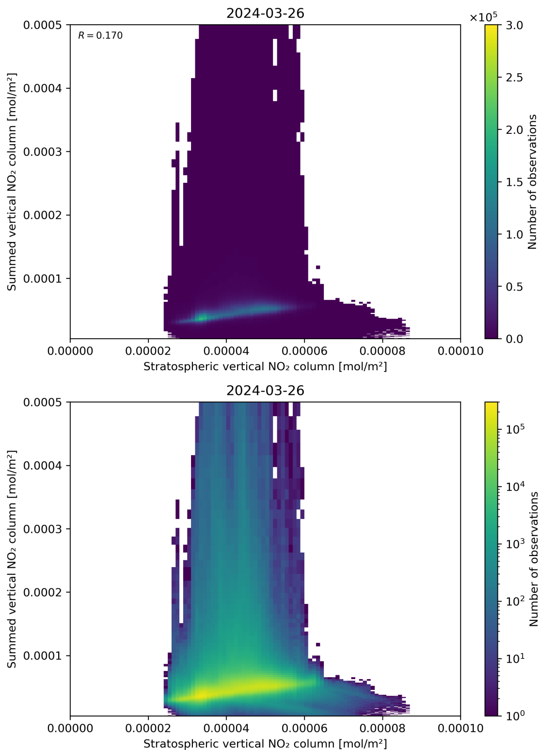
Figure 98: Scatter density plot of “Stratospheric vertical NO 2 column” against “Summed vertical NO 2 column” for 2024-03-25 to 2024-03-27.
