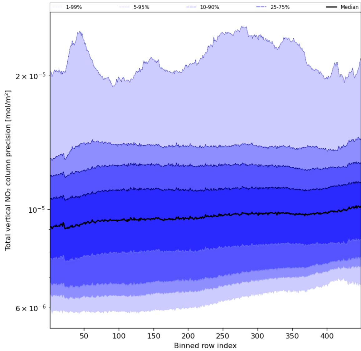
Figure 56: Along track statistics of “Total vertical NO 2 column precision” for 2024-03-25 to 2024-03-27
