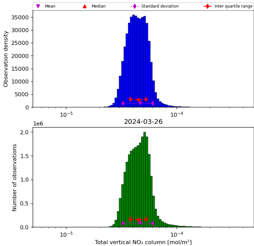
Figure 38: Histogram of “Total vertical NO 2 column” for 2024-03-25 to 2024-03-27
