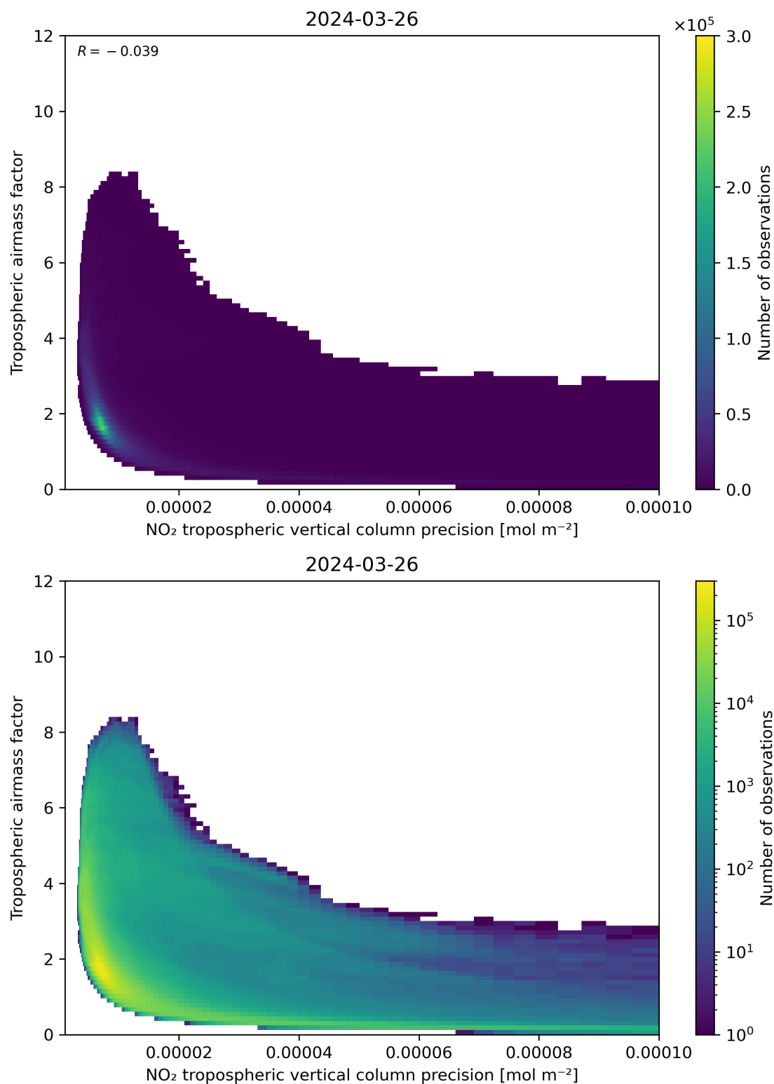
Figure 133: Scatter density plot of “NO 2 tropospheric vertical column precision” against “Tropospheric airmass factor” for 2024-03-25 to 2024-03-27.
