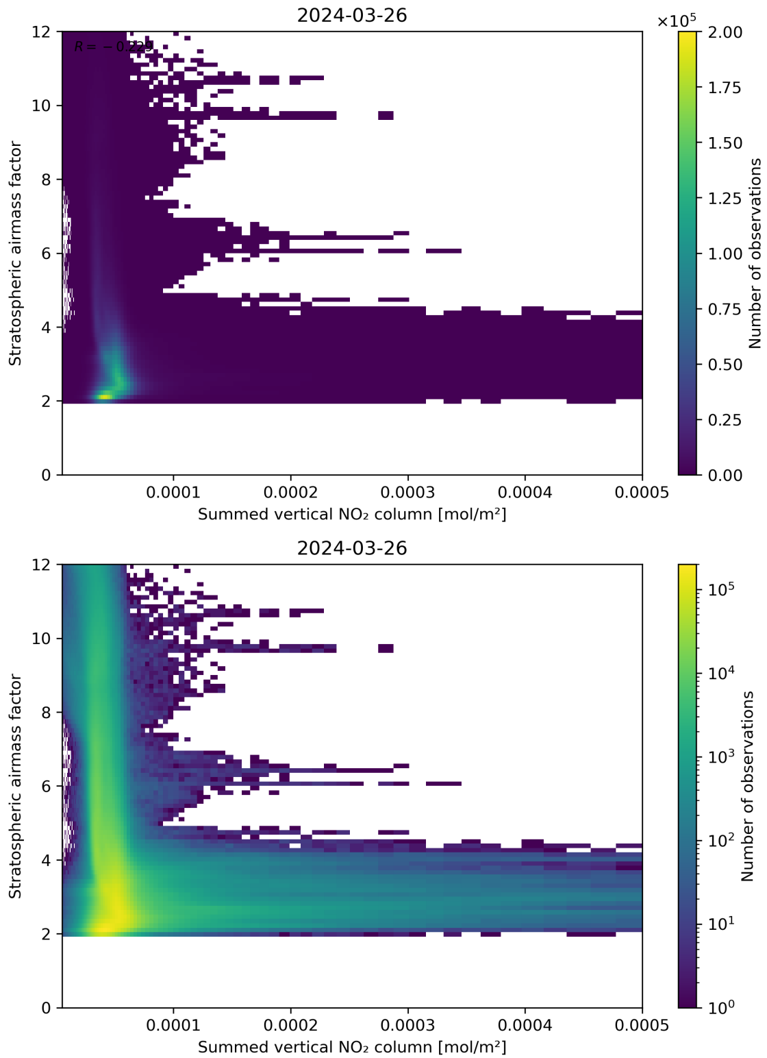
Figure 103: Scatter density plot of “Summed vertical NO 2 column” against “Stratospheric air mass factor” for 2024-03-25 to 2024-03-27.
