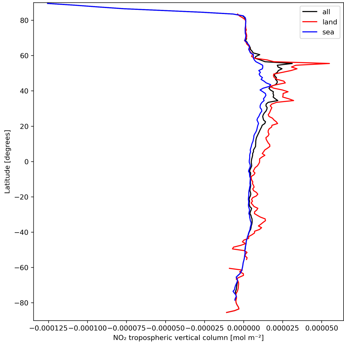
Figure 12: Zonal average of “NO 2 tropospheric vertical column” for 2024-03-25 to 2024-03-27.
