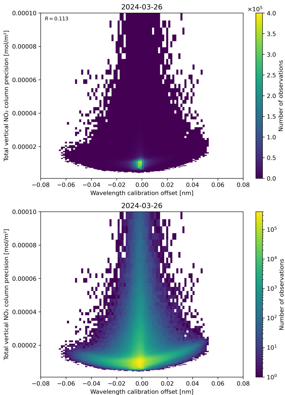
Figure 180: Scatter density plot of “Wavelength calibration offset” against “Total vertical NO 2 column precision” for 2024-03-25 to 2024-03-27.
