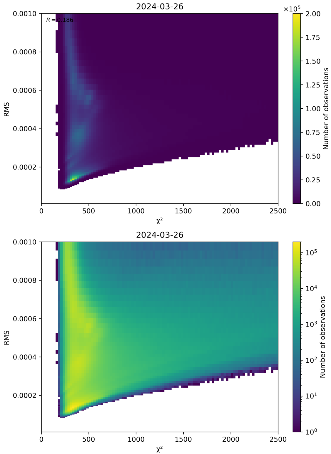
Figure 82: Scatter density plot of “ \chi^2 ” against “RMS” for 2024-03-25 to 2024-03-27.
