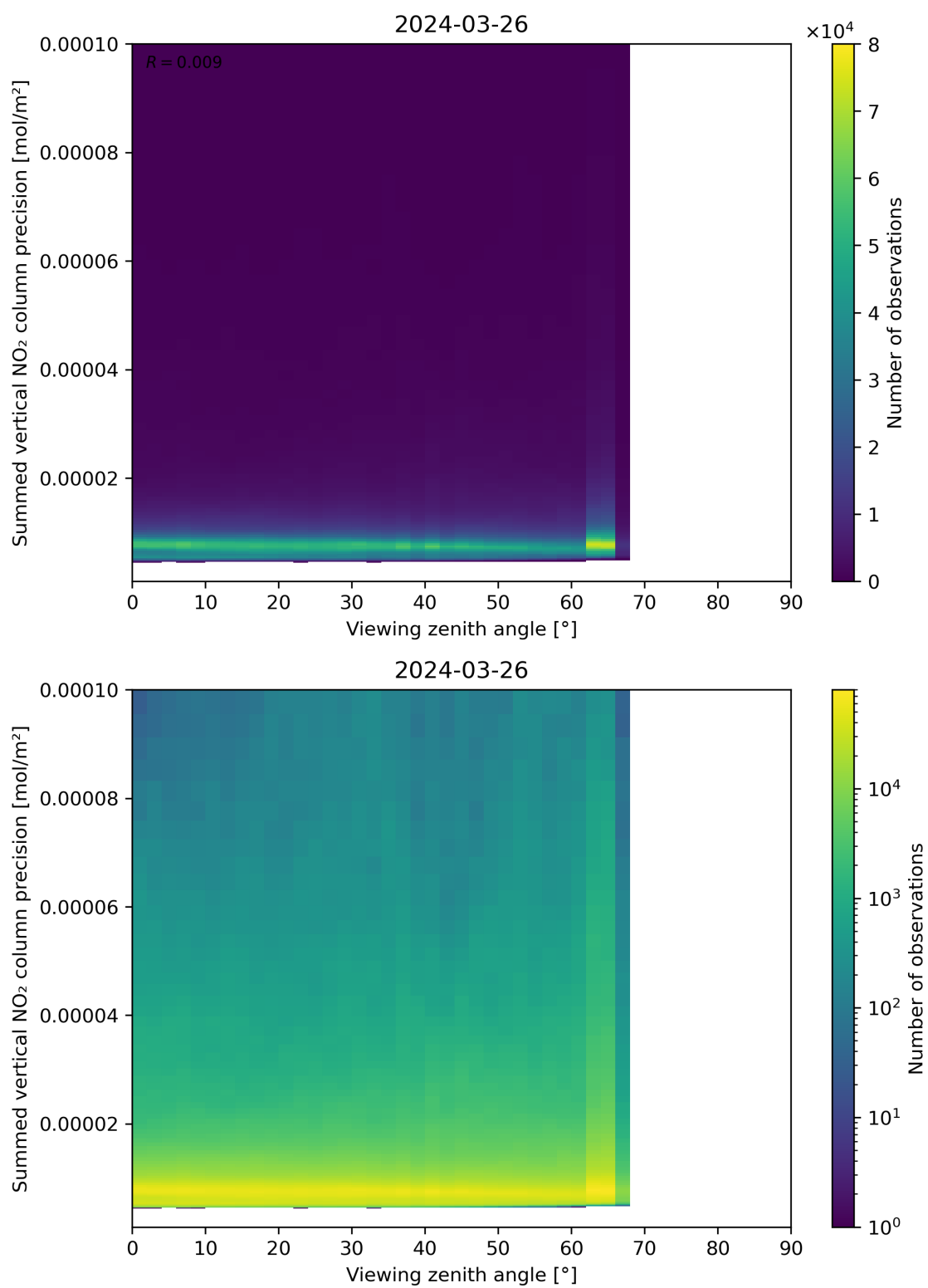
Figure 166: Scatter density plot of “Viewing zenith angle” against “Summed vertical NO 2 column precision” for 2024-03-25 to 2024-03-27.
