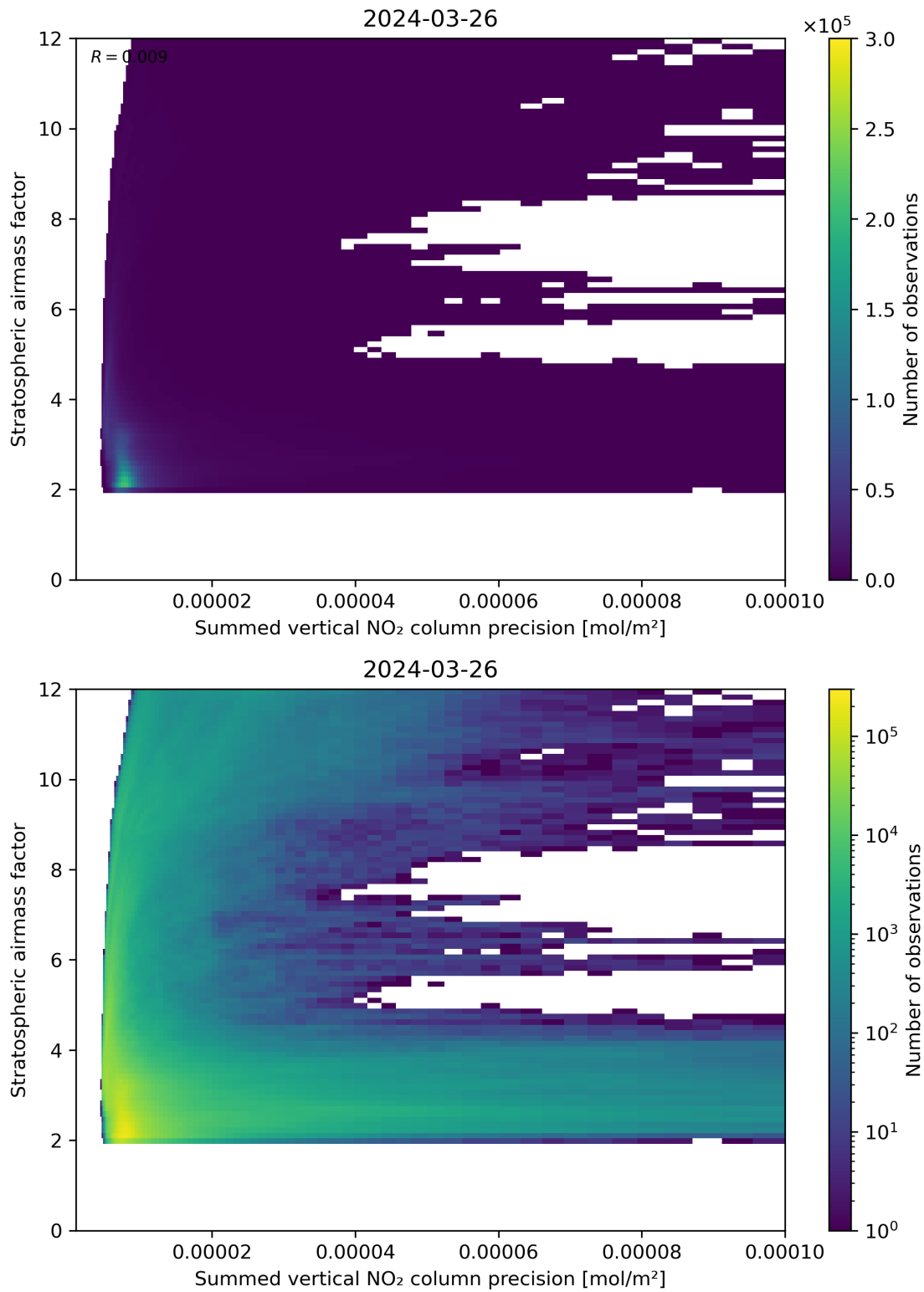
Figure 106: Scatter density plot of “Summed vertical NO 2 column precision” against “Stratospheric airmass factor” for 2024-03-25 to 2024-03-27.
