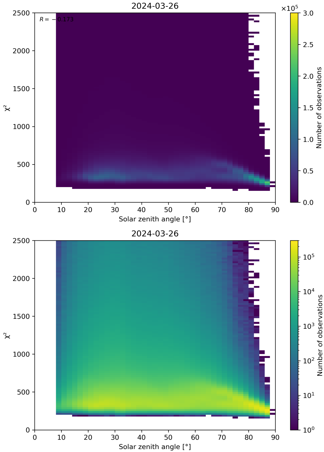
Figure 148: Scatter density plot of “Solar zenith angle” against “ \chi^2 ” for 2024-03-25 to 2024-03-27.
