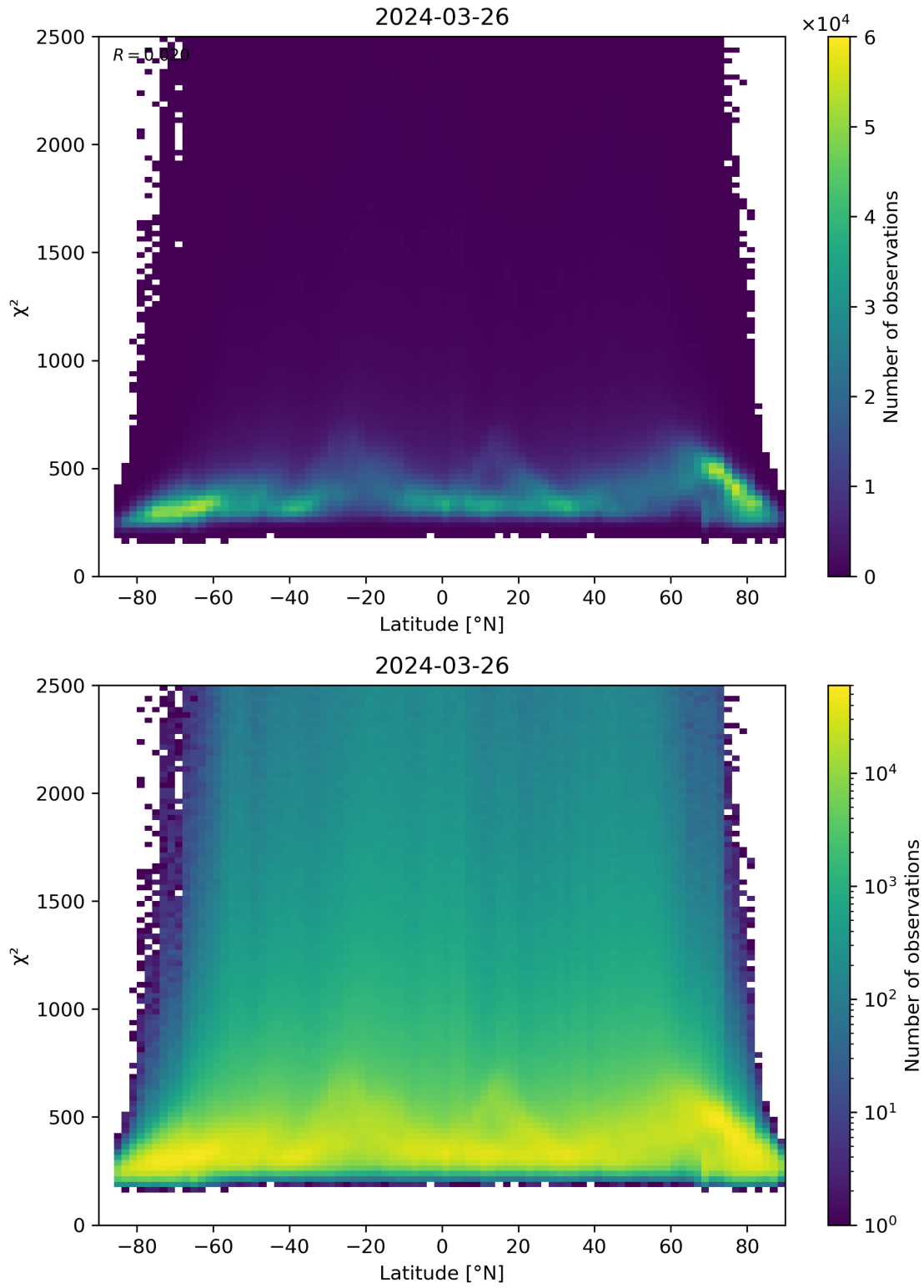
Figure 86: Scatter density plot of “Latitude” against “ \chi^2 ” for 2024-03-25 to 2024-03-27.
