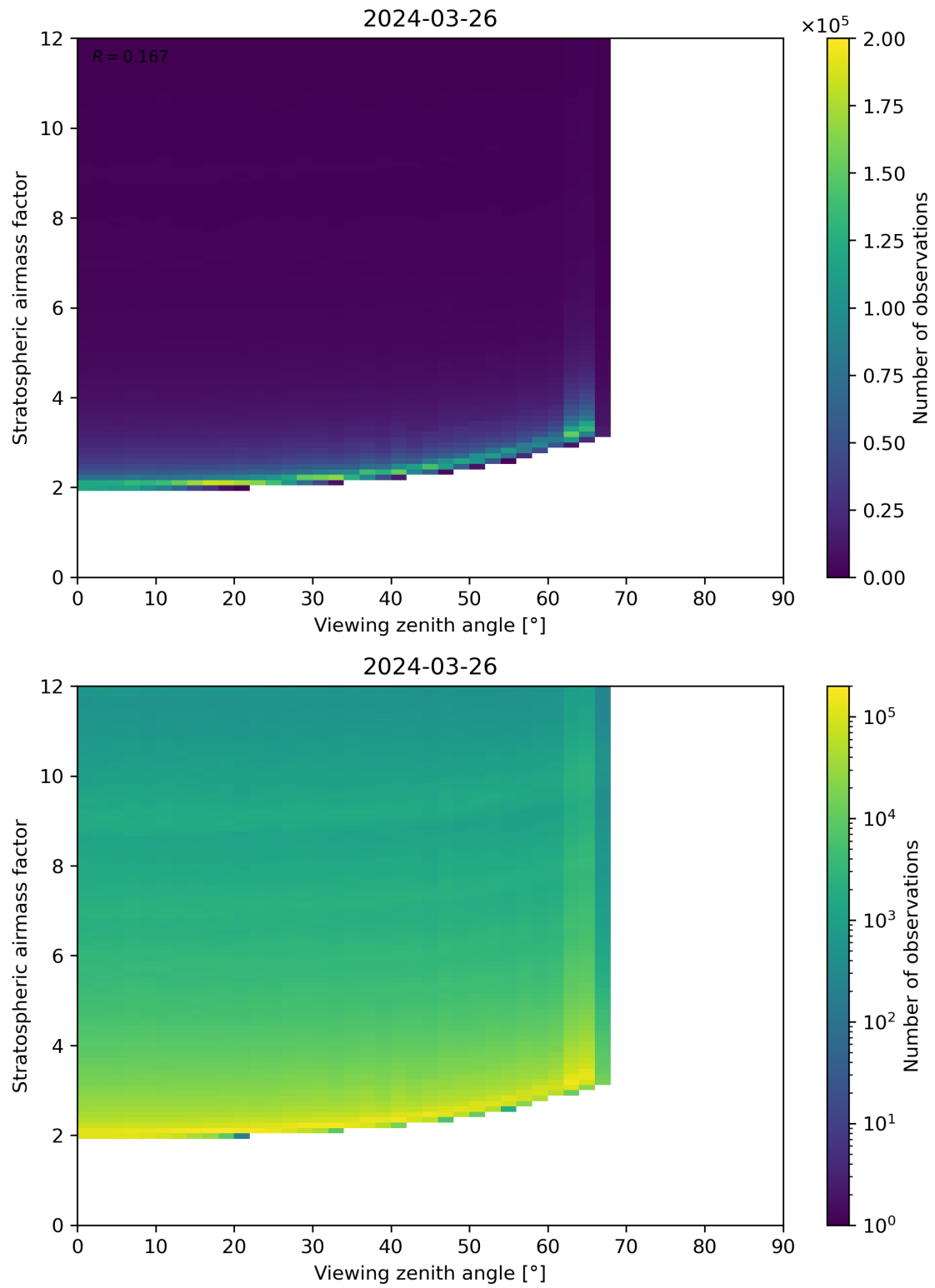
Figure 159: Scatter density plot of “Viewing zenith angle” against “Stratospheric airmass factor” for 2024-03-25 to 2024-03-27.
