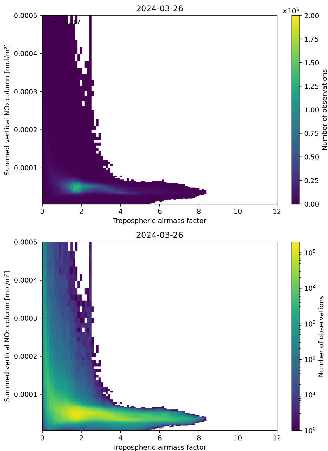
Figure 75: Scatter density plot of “Tropospheric air mass factor” against “Summed vertical NO 2 column” for 2024-03-25 to 2024-03-27.
