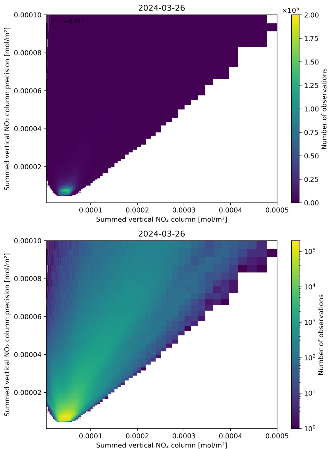
Figure 105: Scatter density plot of “Summed vertical NO 2 column” against “Summed vertical NO 2 column precision” for 2024-03-25 to 2024-03-27.
