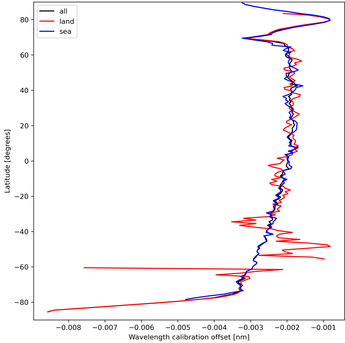
Figure 18: Zonal average of “Wavelength calibration offset” for 2024-03-25 to 2024-03-27.
