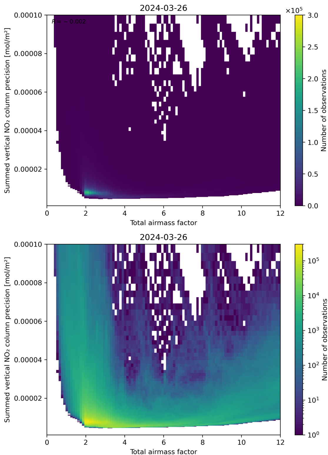
Figure 66: Scatter density plot of “Total airmass factor” against “Summed vertical NO 2 column precision” for 2024-03-25 to 2024-03-27.
