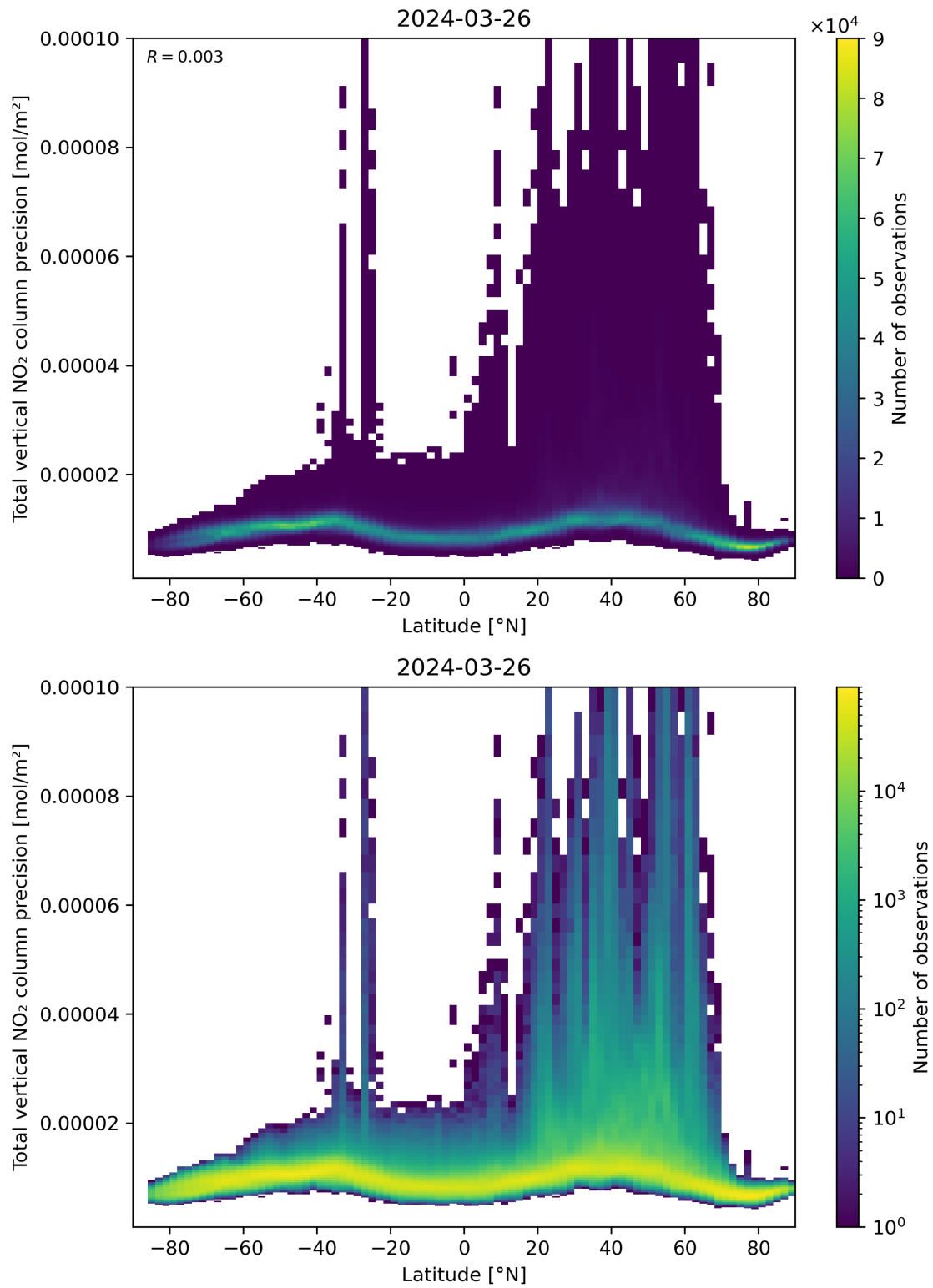
Figure 91: Scatter density plot of “Latitude” against “Total vertical NO 2 column precision” for 2024-03-25 to 2024-03-27.
