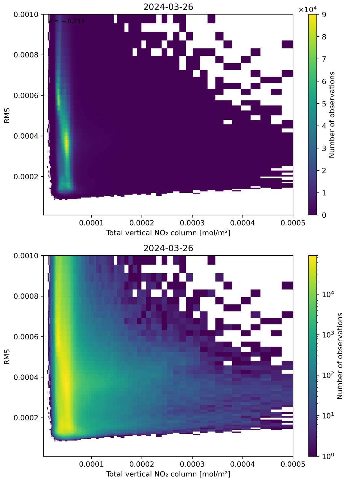
Figure 120: Scatter density plot of “Total vertical NO 2 column” against “RMS” for 2024-03-25 to 2024-03-27.
