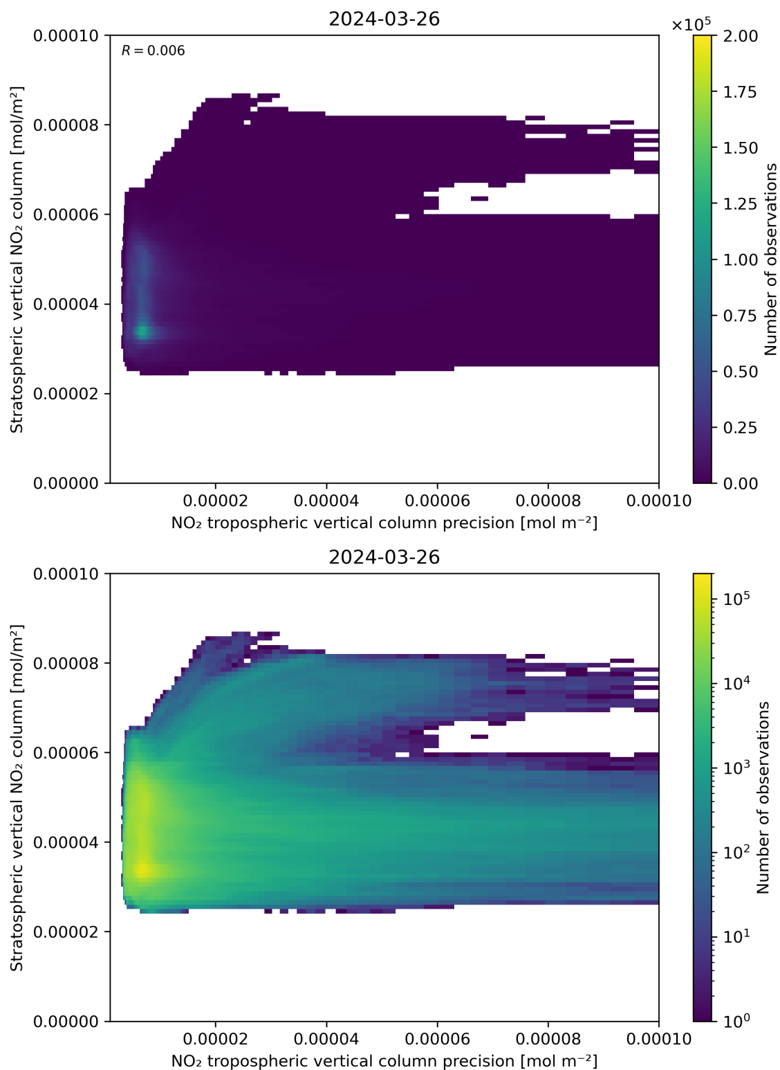
Figure 135: Scatter density plot of “NO 2 tropospheric vertical column precision” against “Stratospheric vertical NO 2 column” for 2024-03-25 to 2024-03-27.
