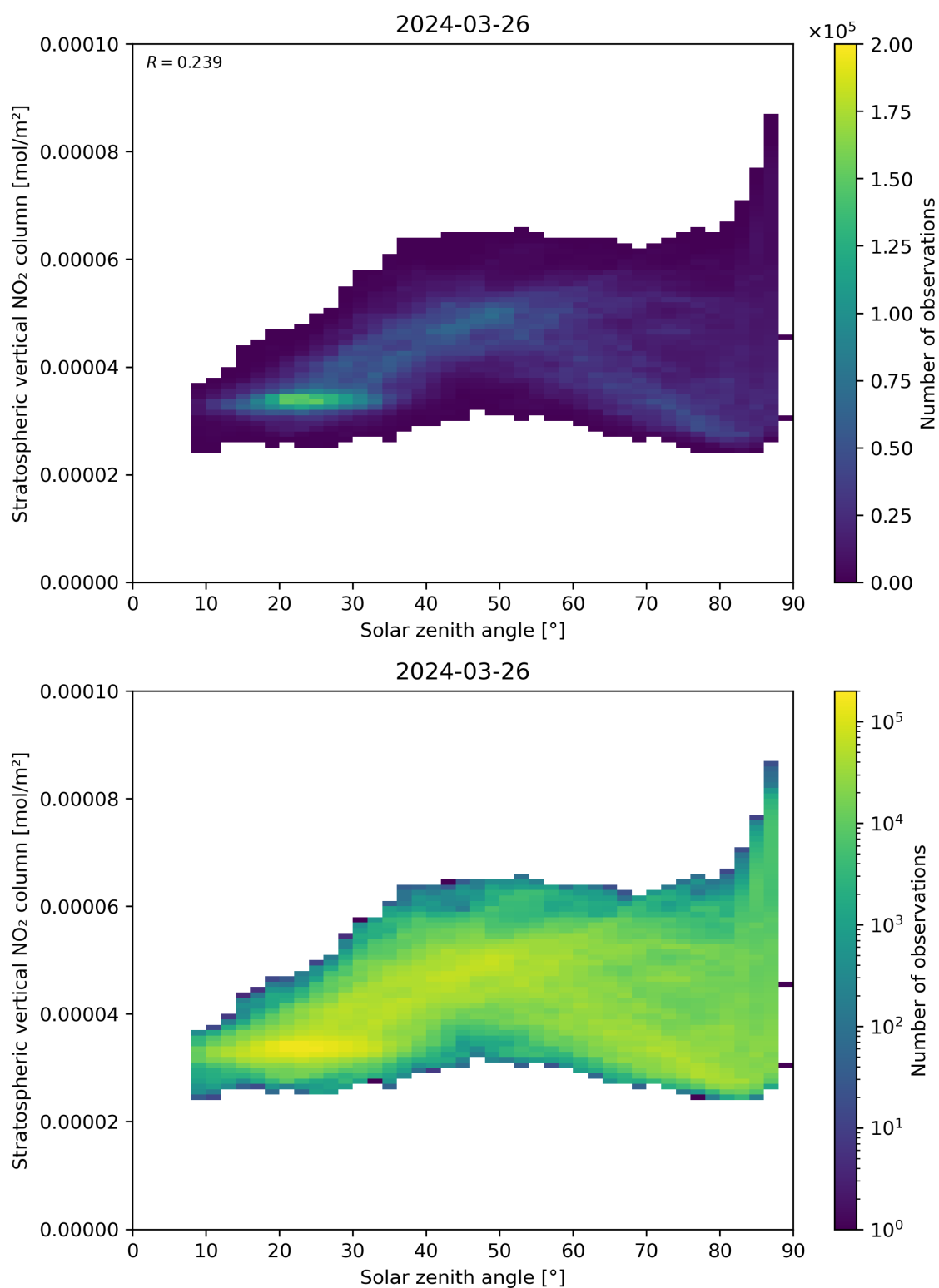
Figure 150: Scatter density plot of “Solar zenith angle” against “Stratospheric vertical NO 2 column” for 2024-03-25 to 2024-03-27.
