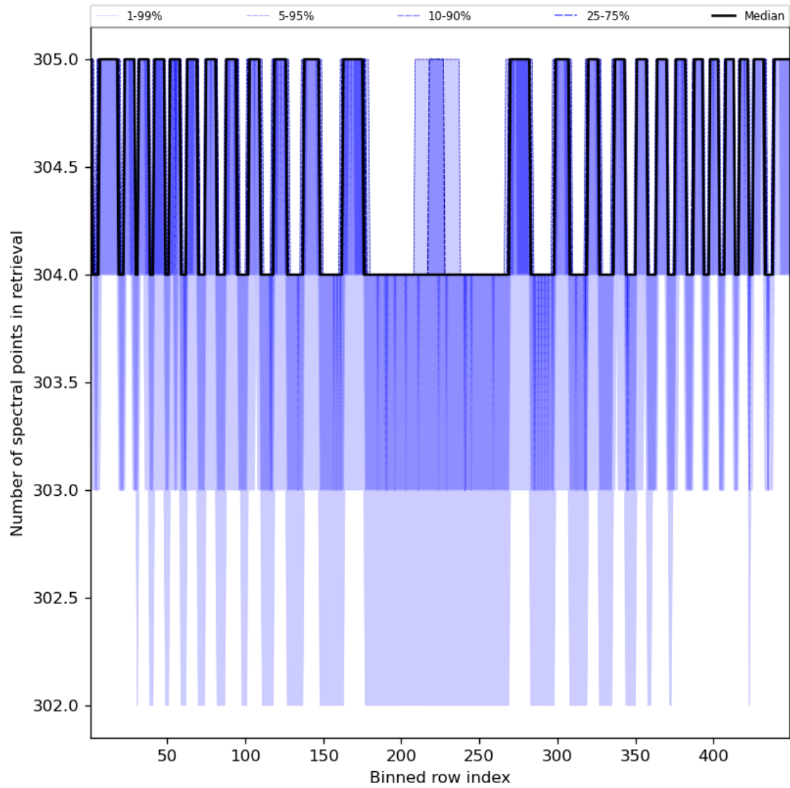
Figure 50: Along track statistics of “Number of spectral points in retrieval” for 2024-03-25 to 2024-03-27
