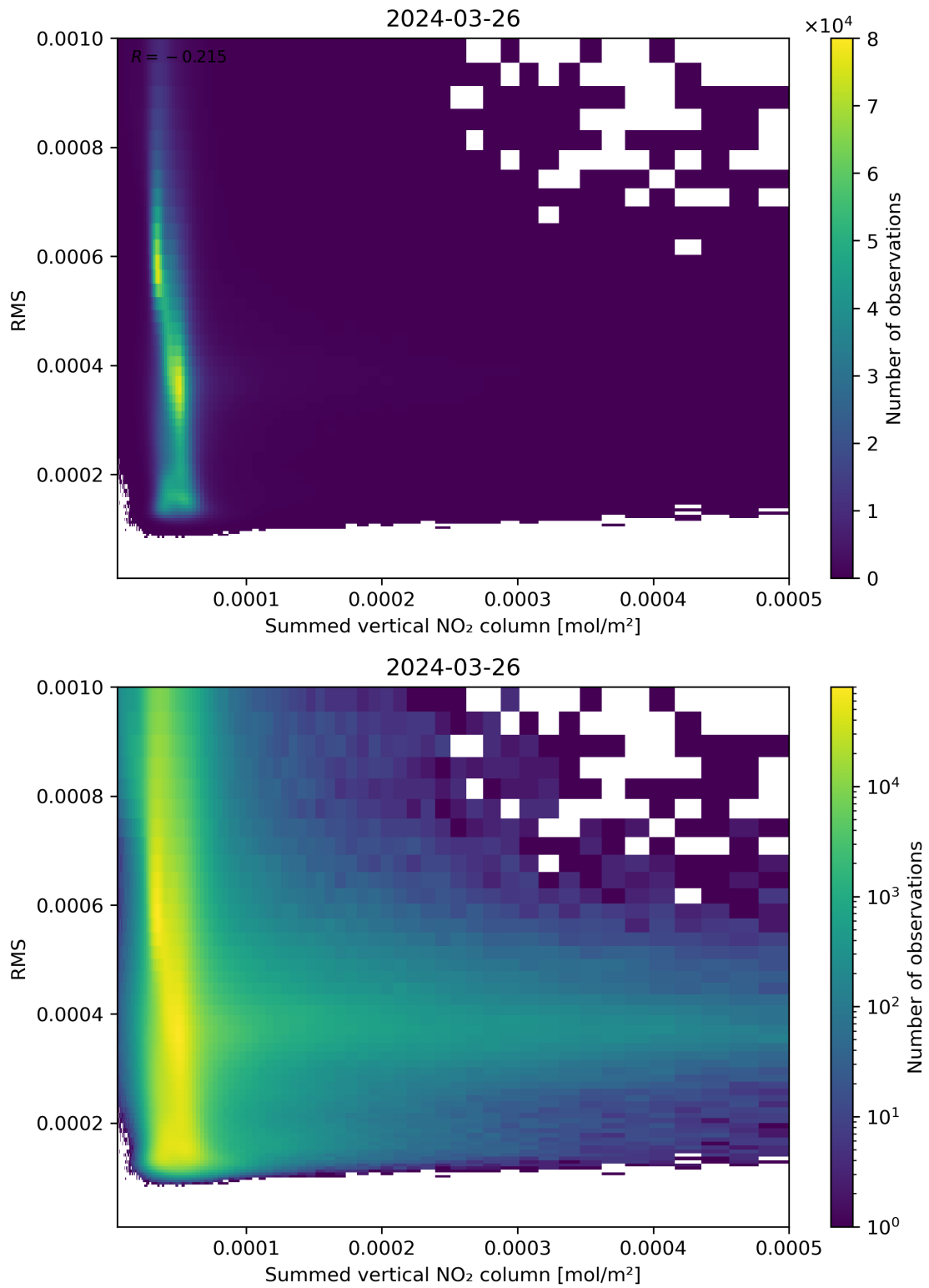
Figure 109: Scatter density plot of “Summed vertical NO 2 column” against “RMS” for 2024-03-25 to 2024-03-27.
