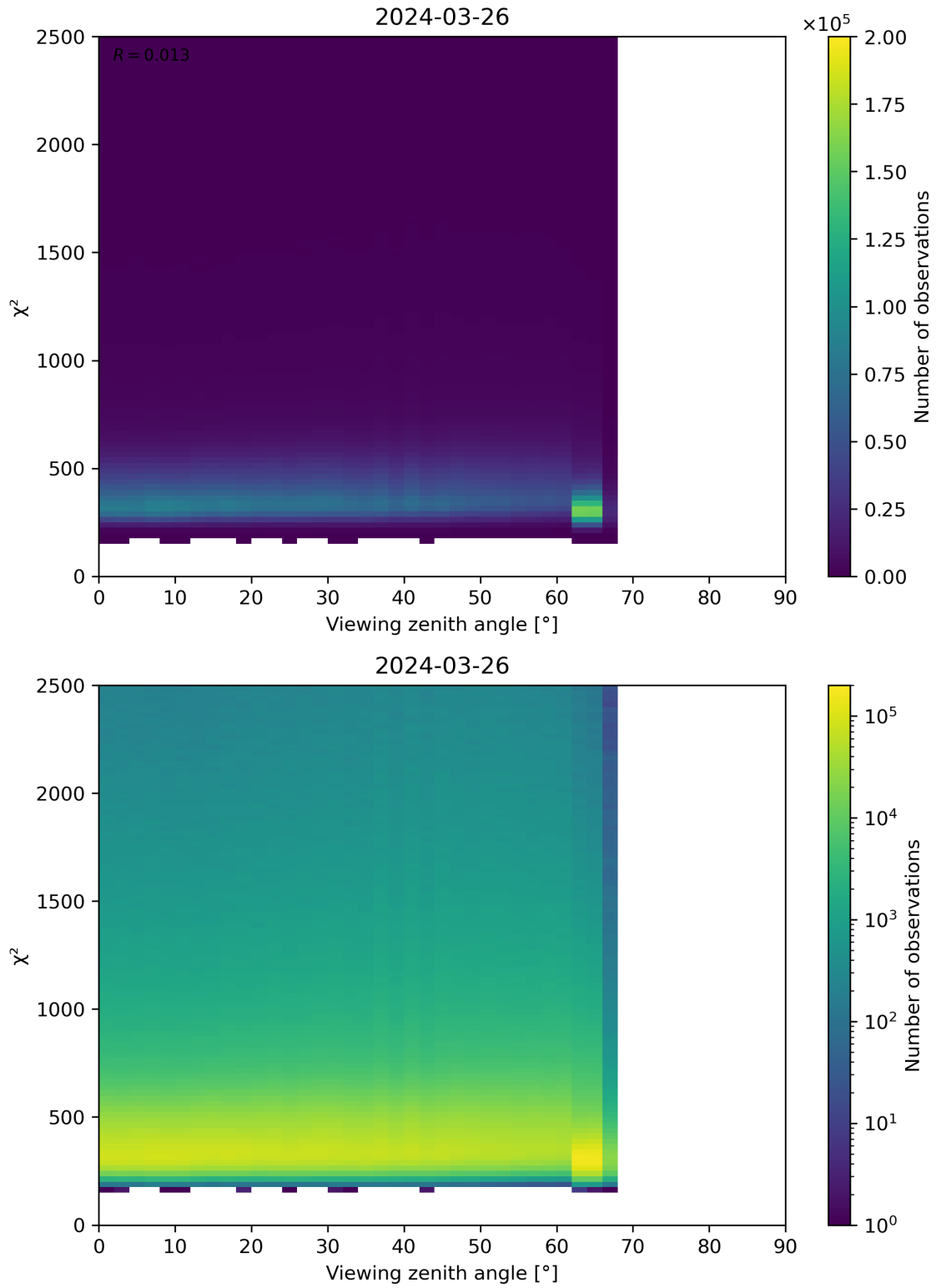
Figure 162: Scatter density plot of “Viewing zenith angle” against “ \chi^2 ” for 2024-03-25 to 2024-03-27.
