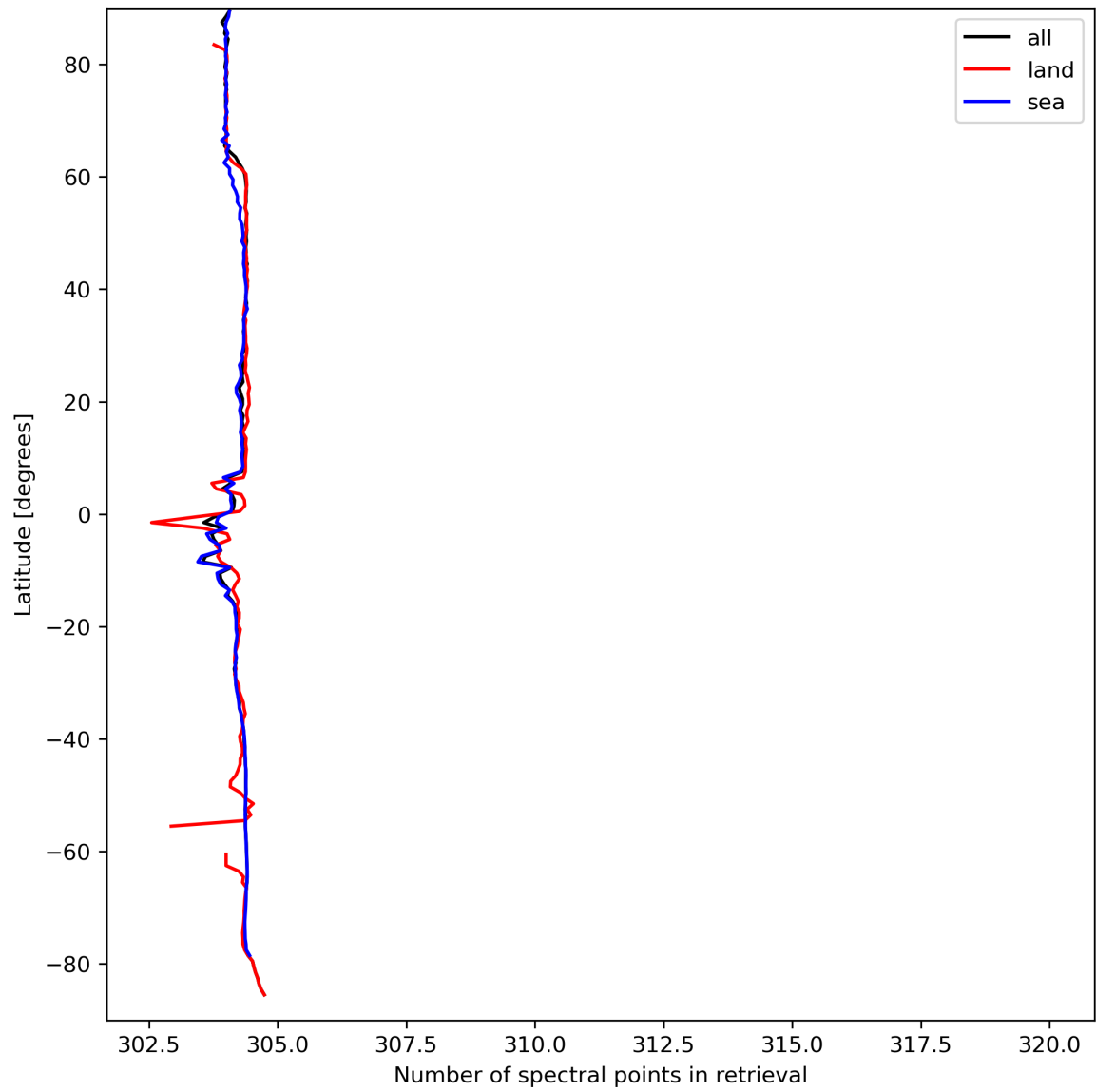
Figure 16: Zonal average of “Number of spectral points in retrieval” for 2024-03-25 to 2024-03-27.
