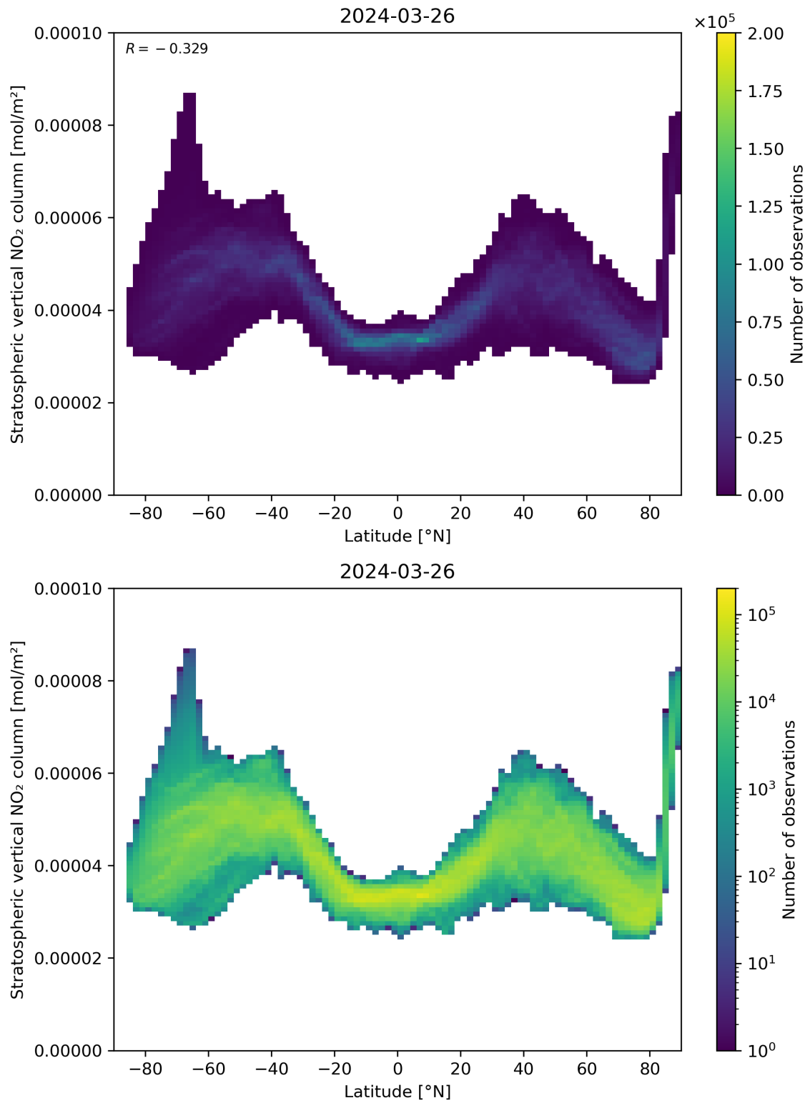
Figure 87: Scatter density plot of “Latitude” against “Stratospheric vertical NO 2 column” for 2024-03-25 to 2024-03-27.
