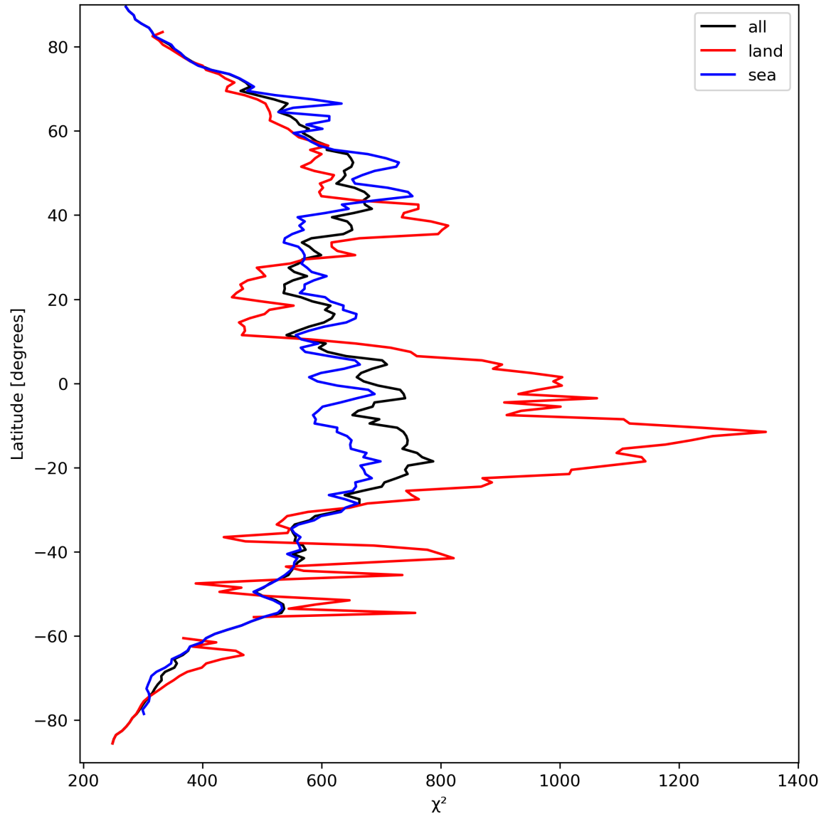
Figure 25: Zonal average of “ \chi^2 ” for 2024-03-25 to 2024-03-27.
