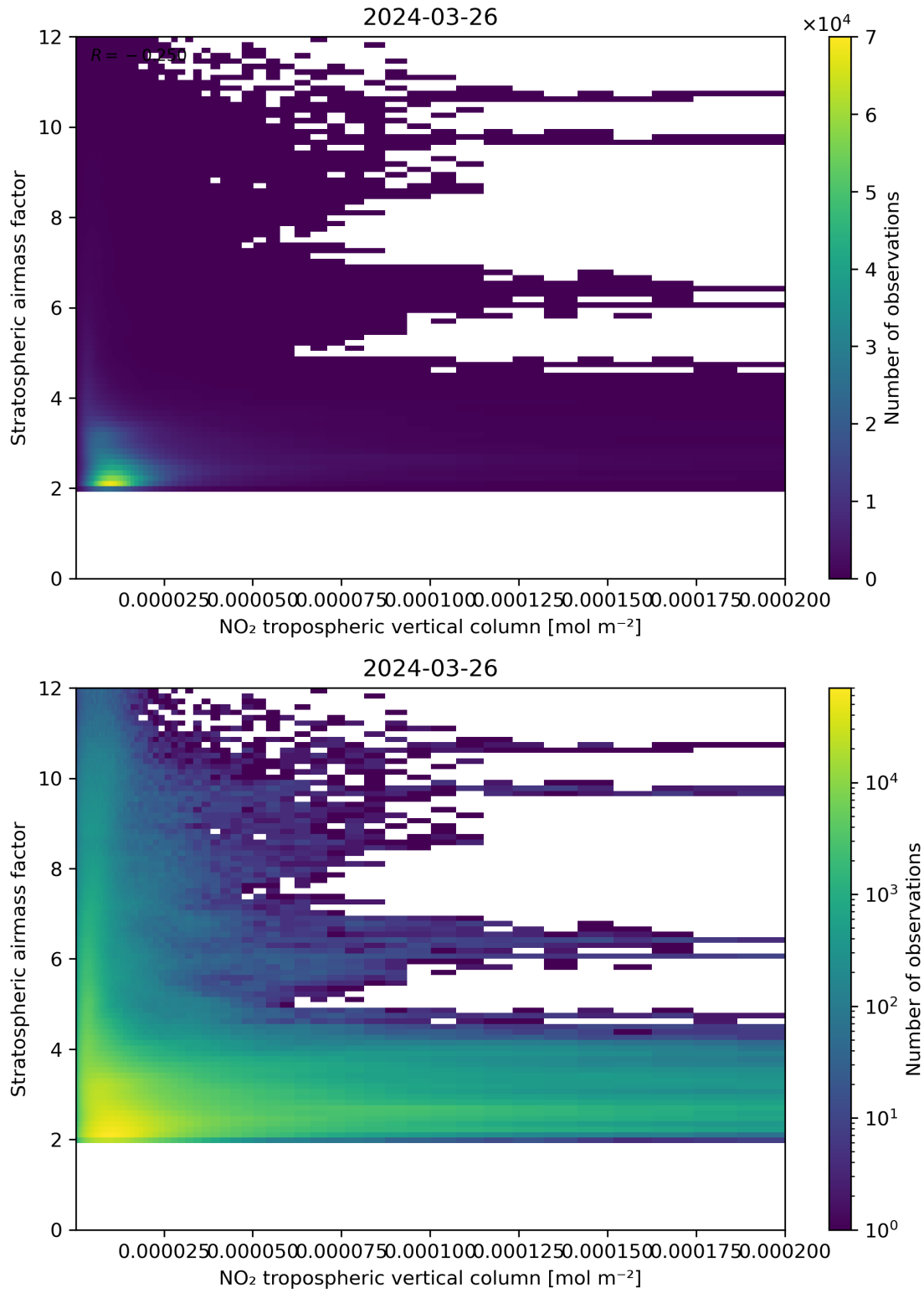
Figure 121: Scatter density plot of “NO 2 tropospheric vertical column” against “Stratospheric air mass factor” for 2024-03-25 to 2024-03-27.
