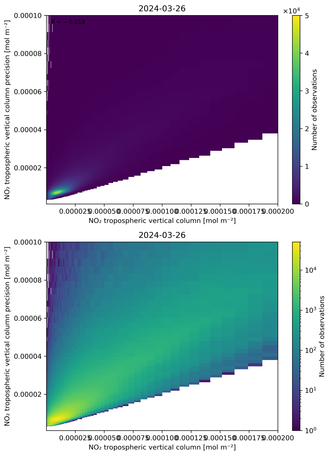
Figure 130: Scatter density plot of “NO 2 tropospheric vertical column” against “NO 2 tropospheric vertical column precision” for 2024-03-25 to 2024-03-27.
