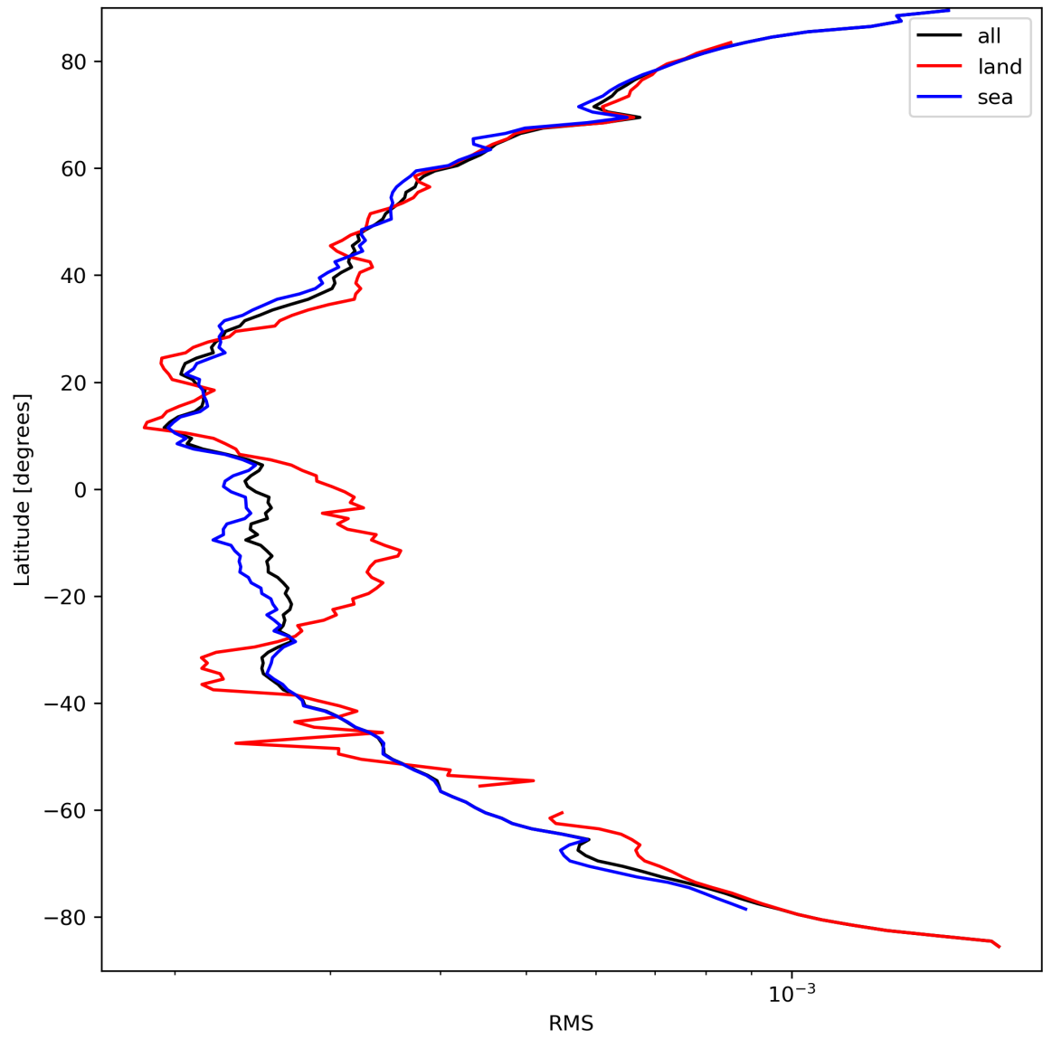
Figure 26: Zonal average of “RMS” for 2024-03-25 to 2024-03-27.
