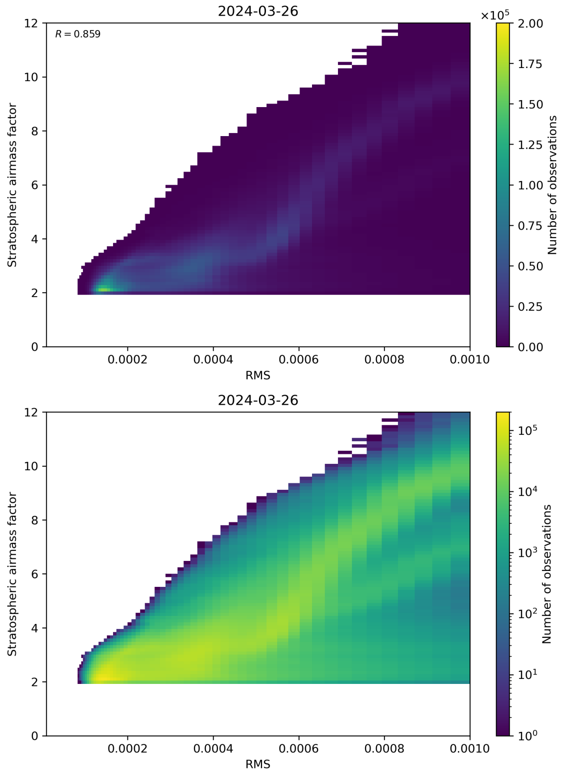
Figure 144: Scatter density plot of “RMS” against “Stratospheric airmass factor” for 2024-03-25 to 2024-03-27.
