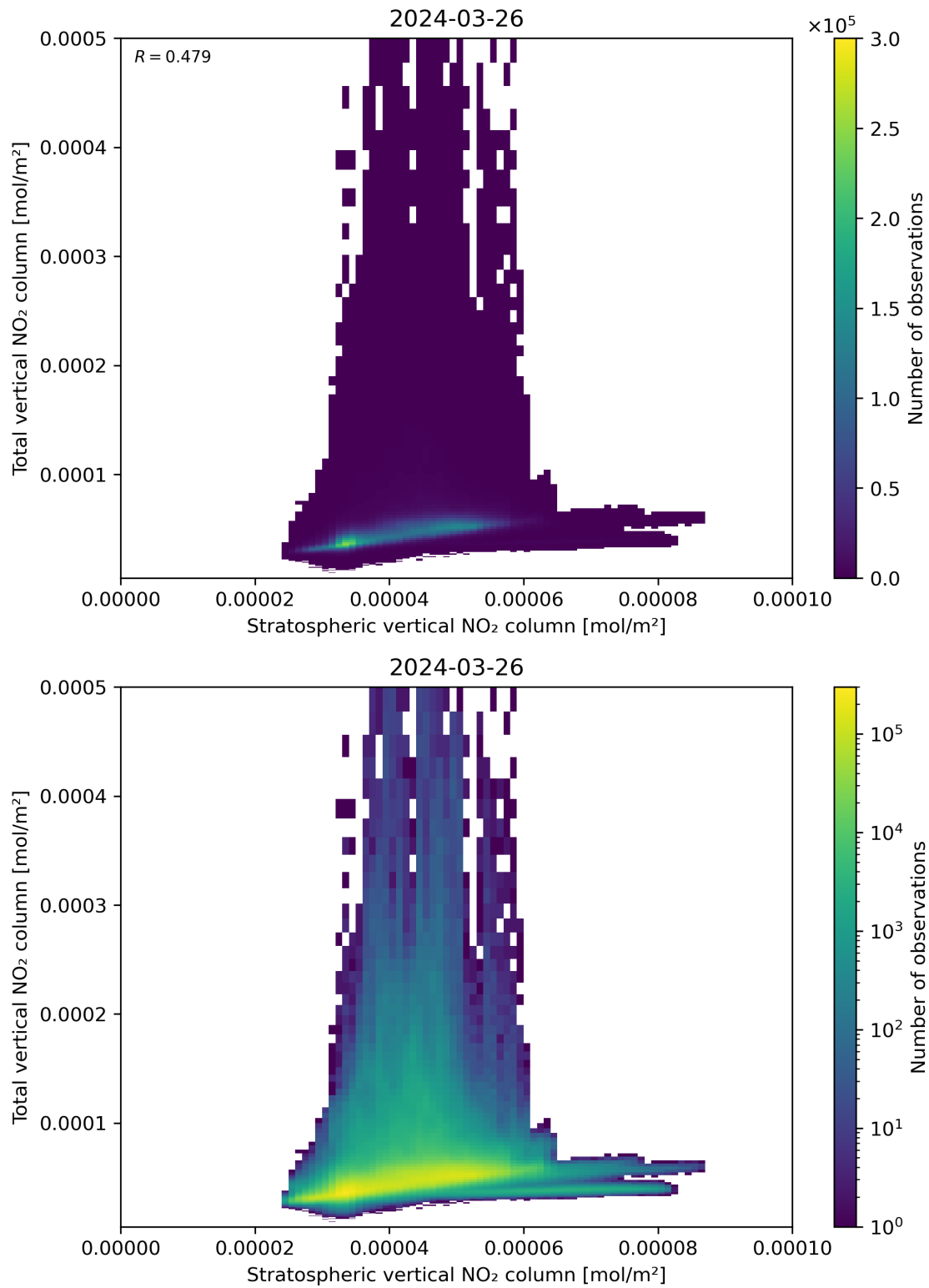
Figure 100: Scatter density plot of “Stratospheric vertical NO 2 column” against “Total vertical NO 2 column” for 2024-03-25 to 2024-03-27.
