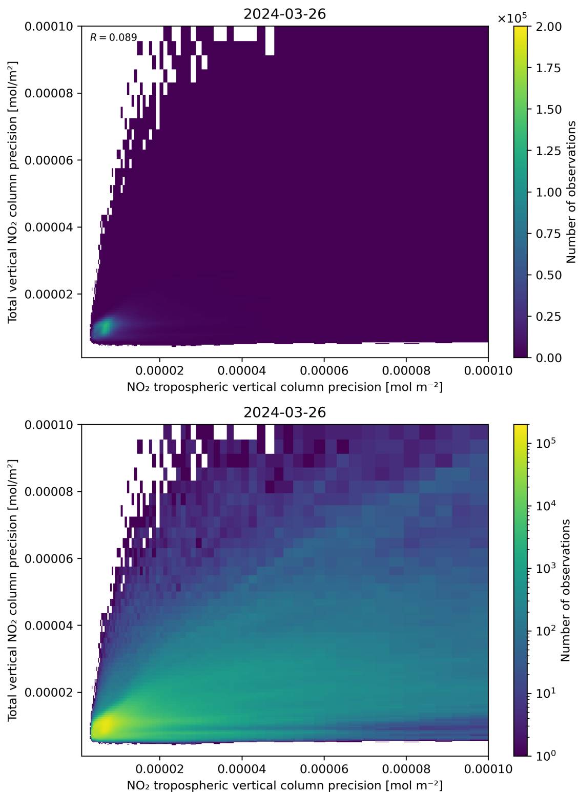
Figure 139: Scatter density plot of “NO 2 tropospheric vertical column precision” against “Total vertical NO 2 column precision” for 2024-03-25 to 2024-03-27.
