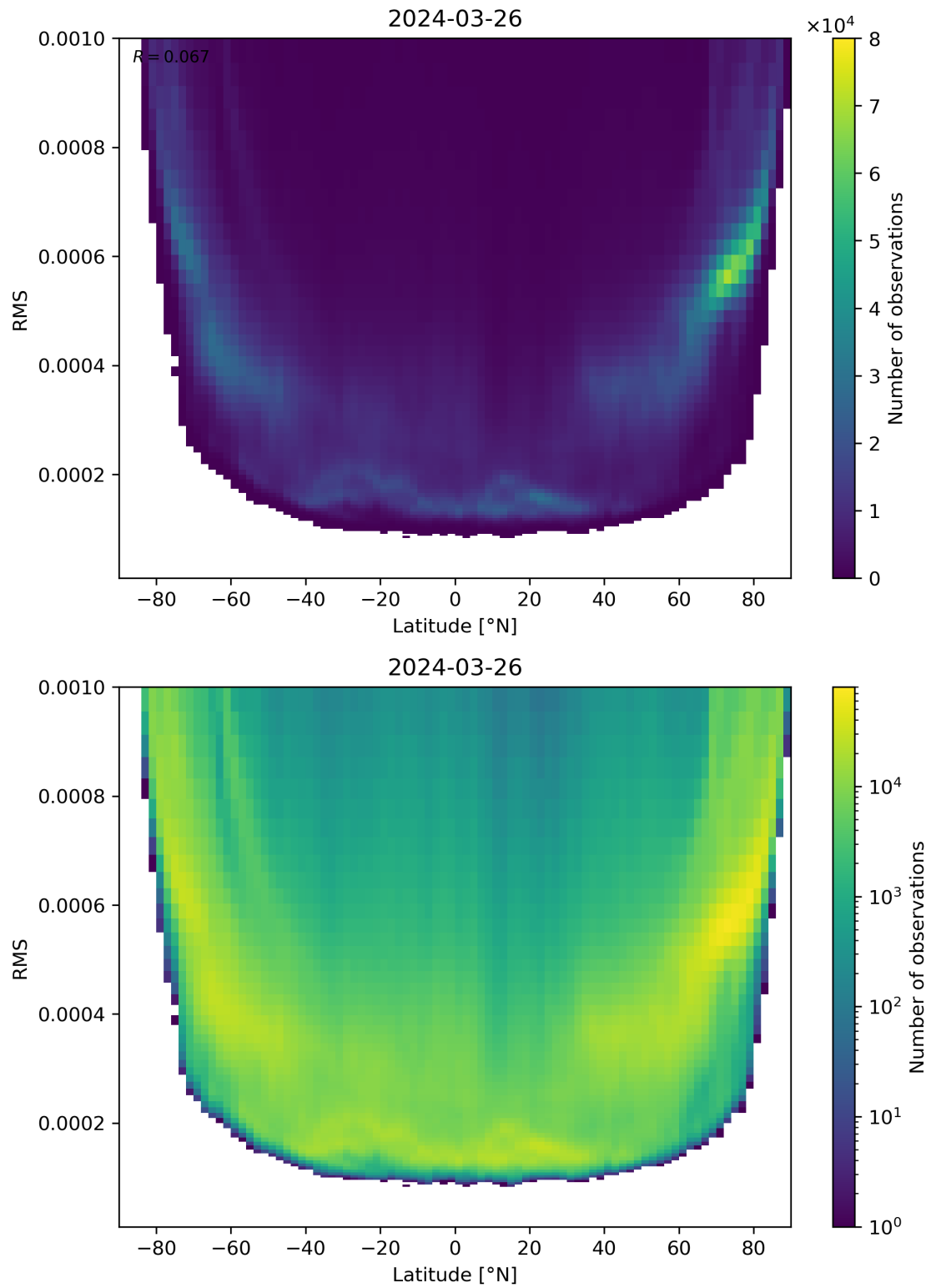
Figure 94: Scatter density plot of “Latitude” against “RMS” for 2024-03-25 to 2024-03-27.
