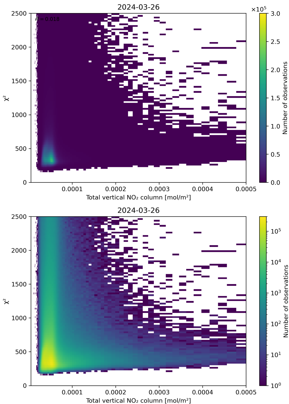
Figure 111: Scatter density plot of “Total vertical NO 2 column” against “ \chi^2 ” for 2024-03-25 to 2024-03-27.
