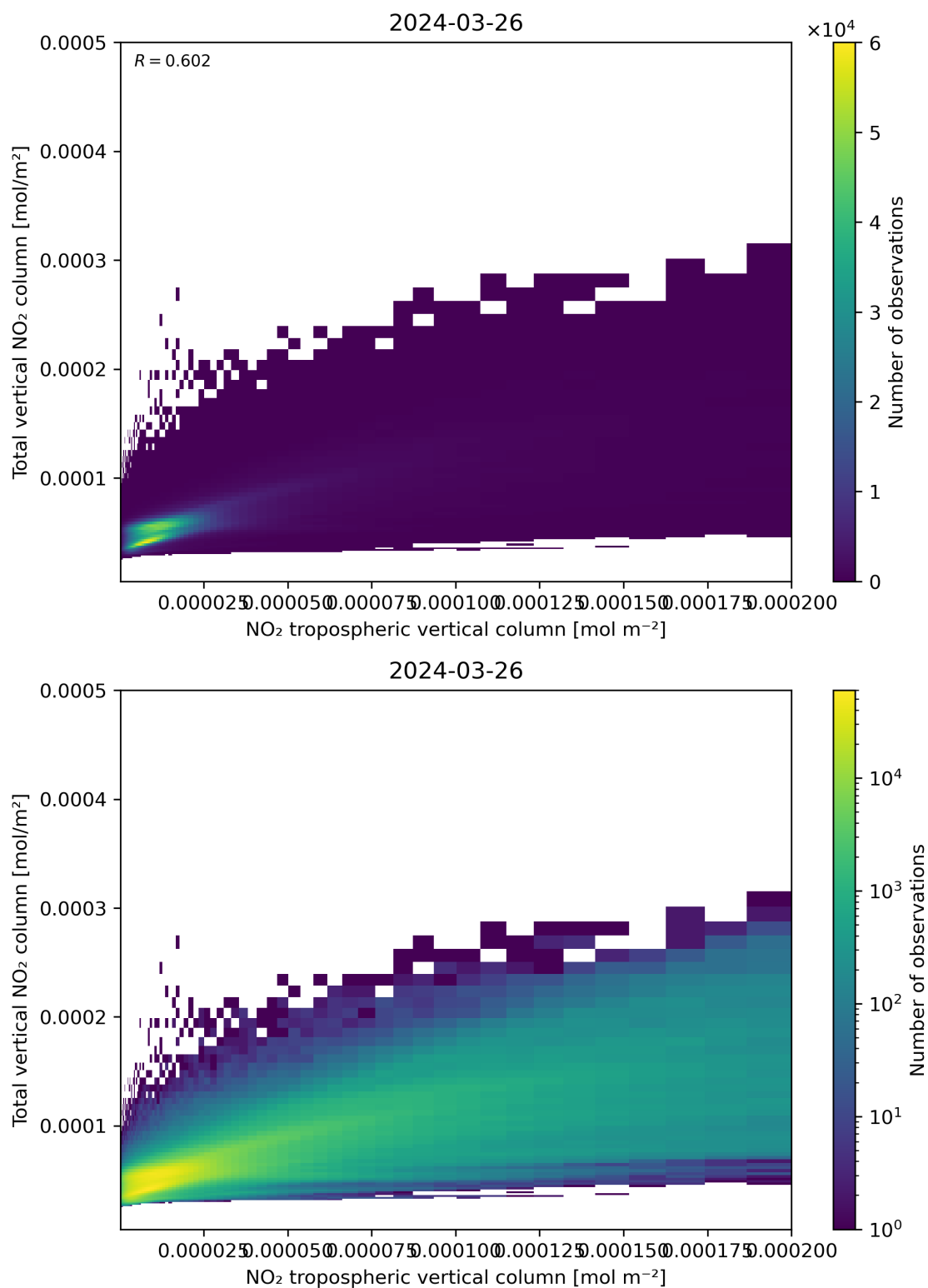
Figure 128: Scatter density plot of “NO 2 tropospheric vertical column” against “Total vertical NO 2 column” for 2024-03-25 to 2024-03-27.
