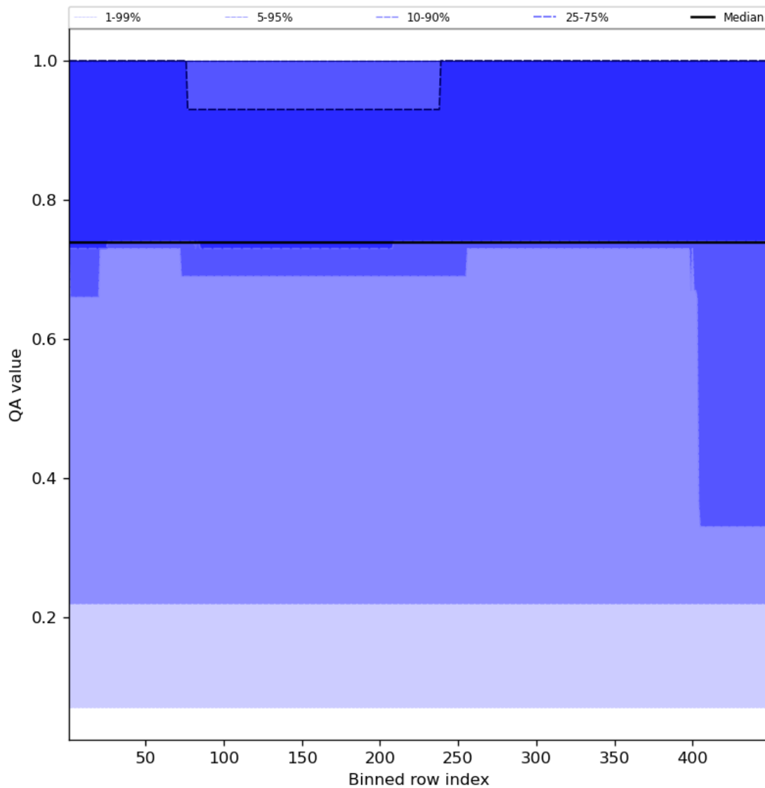
Figure 45: Along track statistics of “QA value” for 2024-03-25 to 2024-03-27
