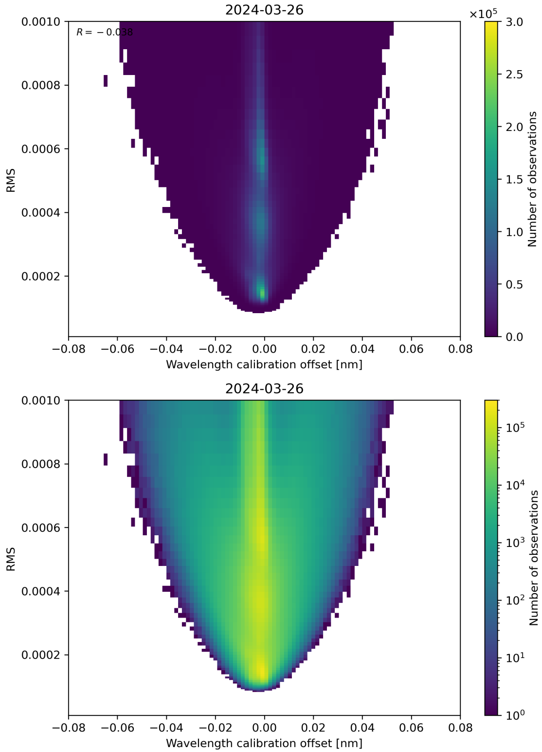
Figure 181: Scatter density plot of “Wavelength calibration offset” against “RMS” for 2024-03-25 to 2024-03-27.
