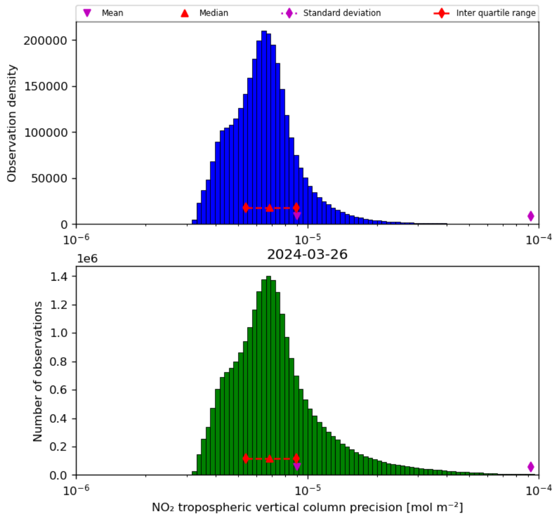
Figure 30: Histogram of “NO 2 tropospheric vertical column precision” for 2024-03-25 to 2024-03-27
