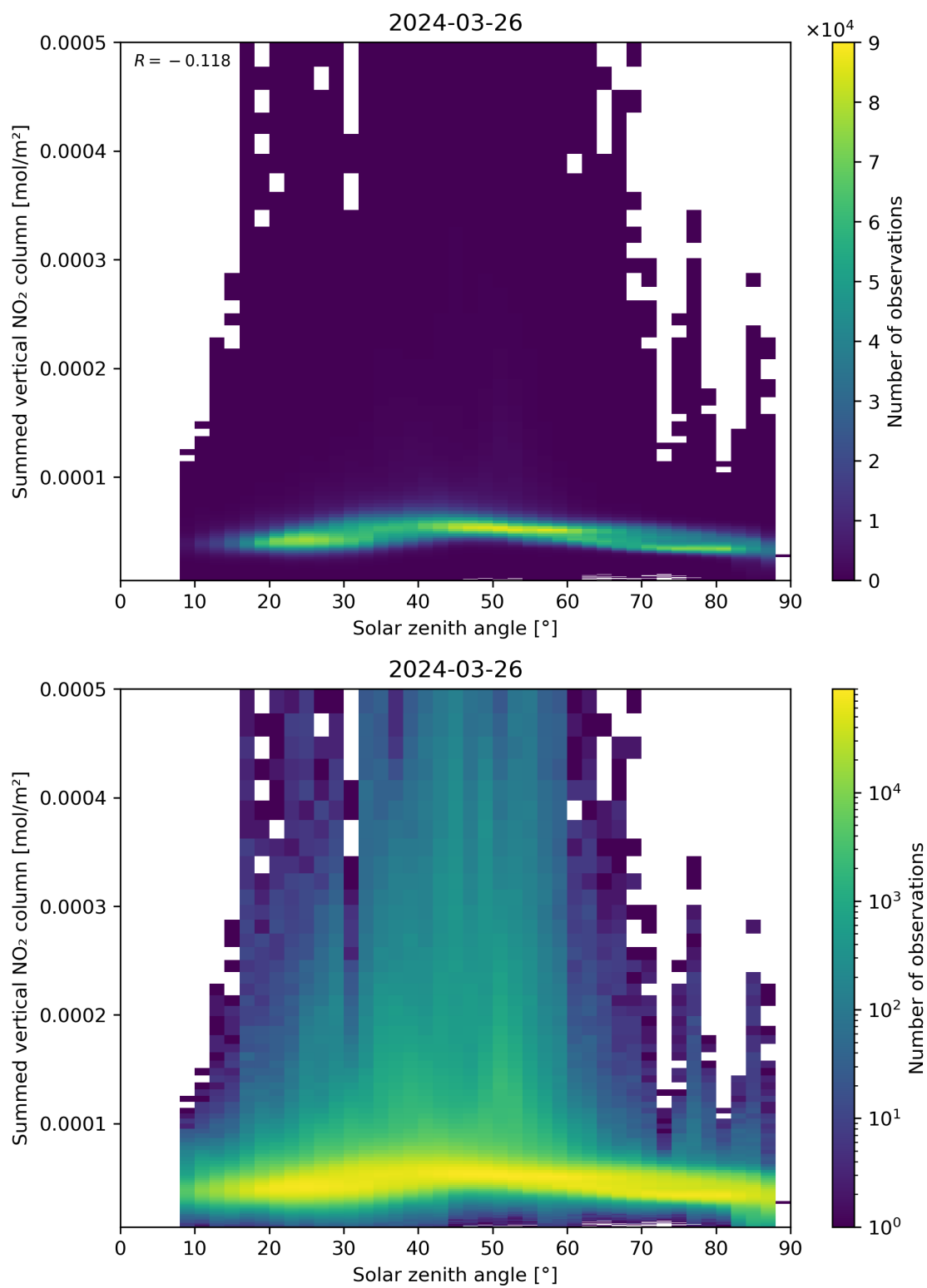
Figure 151: Scatter density plot of “Solar zenith angle” against “Summed vertical NO 2 column” for 2024-03-25 to 2024-03-27.
