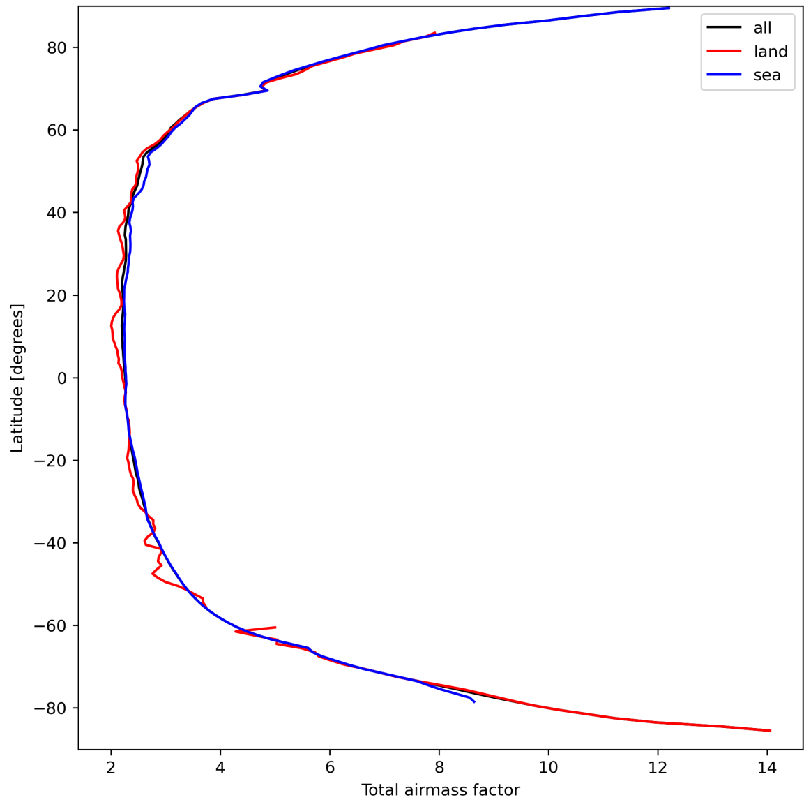
Figure 15: Zonal average of “Total airmass factor” for 2024-03-25 to 2024-03-27.
