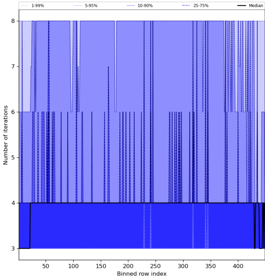
Figure 51: Along track statistics of “Number of iterations” for 2024-03-25 to 2024-03-27
