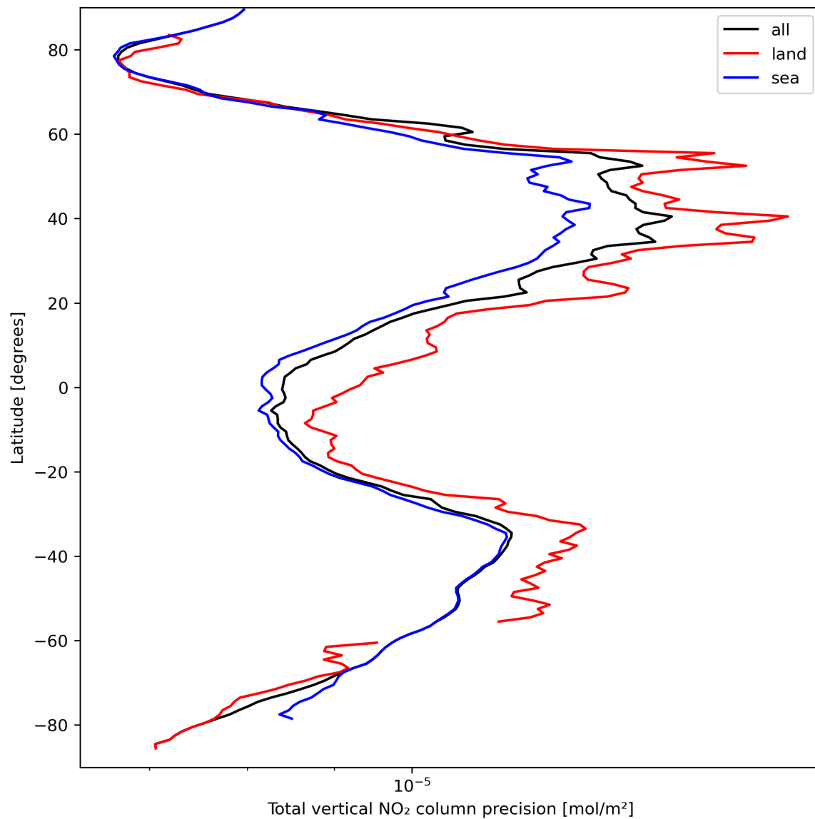
Figure 22: Zonal average of “Total vertical NO 2 column precision” for 2024-03-25 to 2024-03-27.
