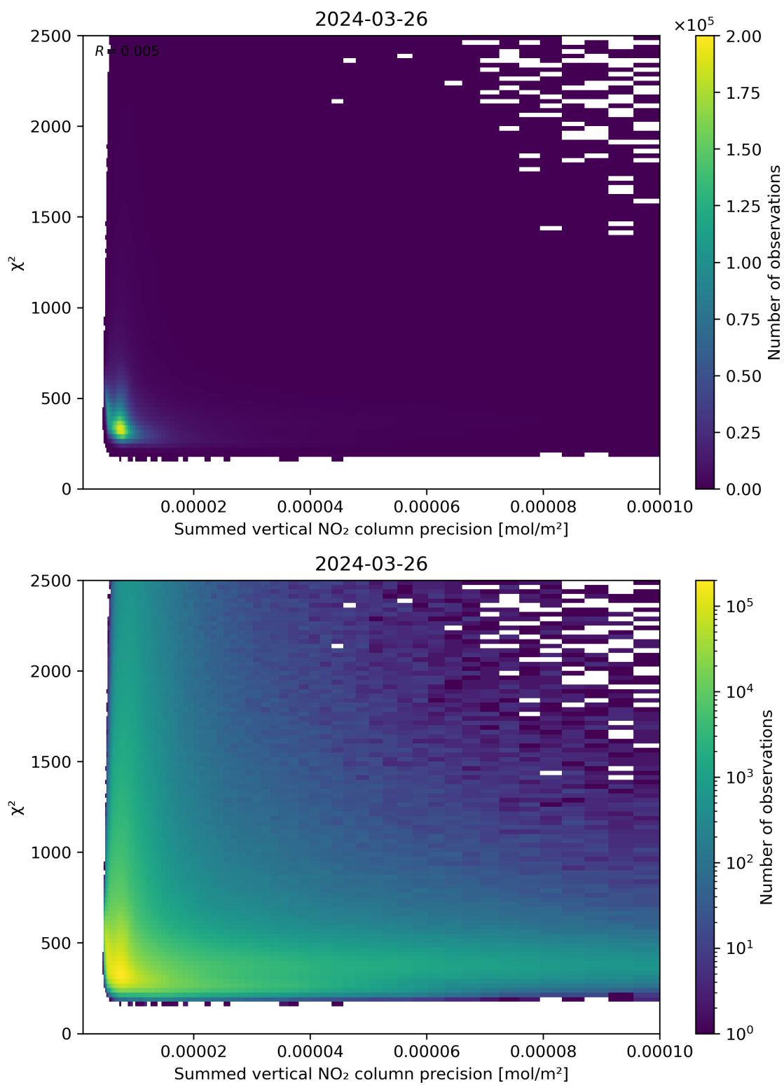
Figure 107: Scatter density plot of “Summed vertical NO 2 column precision” against “ \chi^2 ” for 2024-03-25 to 2024-03-27.
