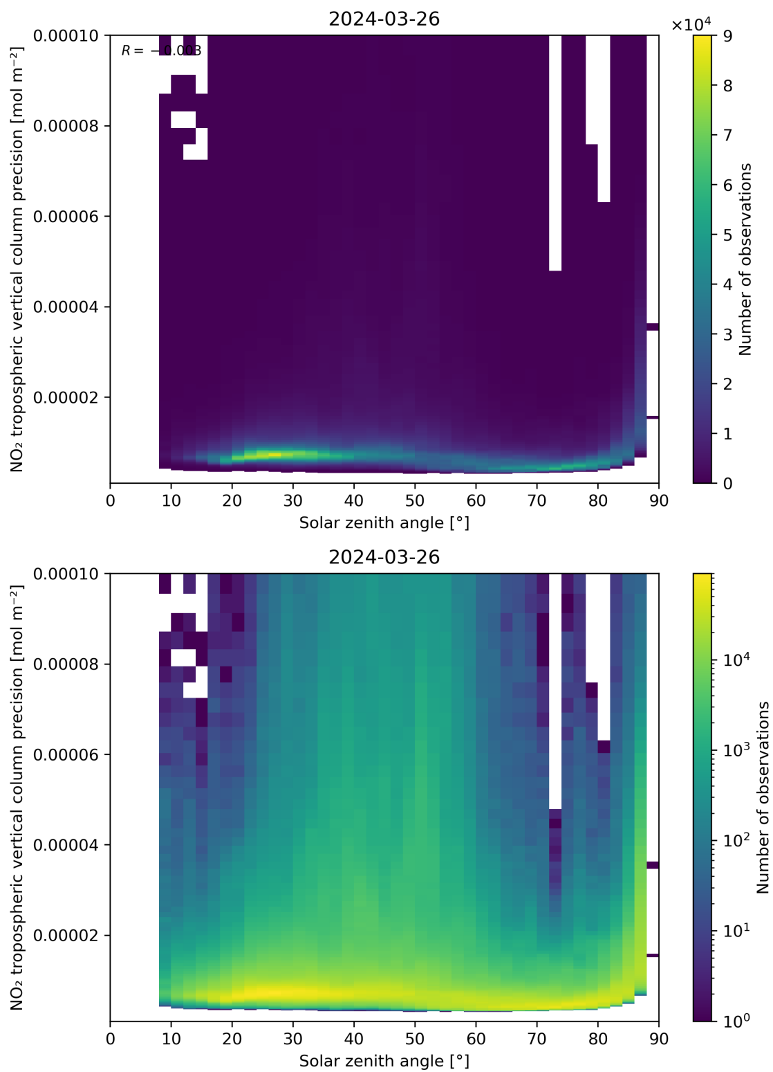
Figure 156: Scatter density plot of “Solar zenith angle” against “NO 2 tropospheric vertical column precision” for 2024-03-25 to 2024-03-27.
