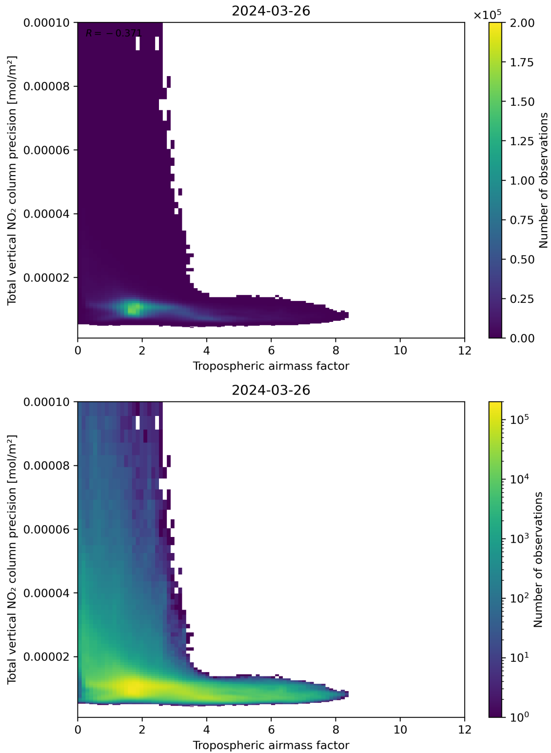
Figure 78: Scatter density plot of “Tropospheric air mass factor” against “Total vertical NO 2 column precision” for 2024-03-25 to 2024-03-27.
