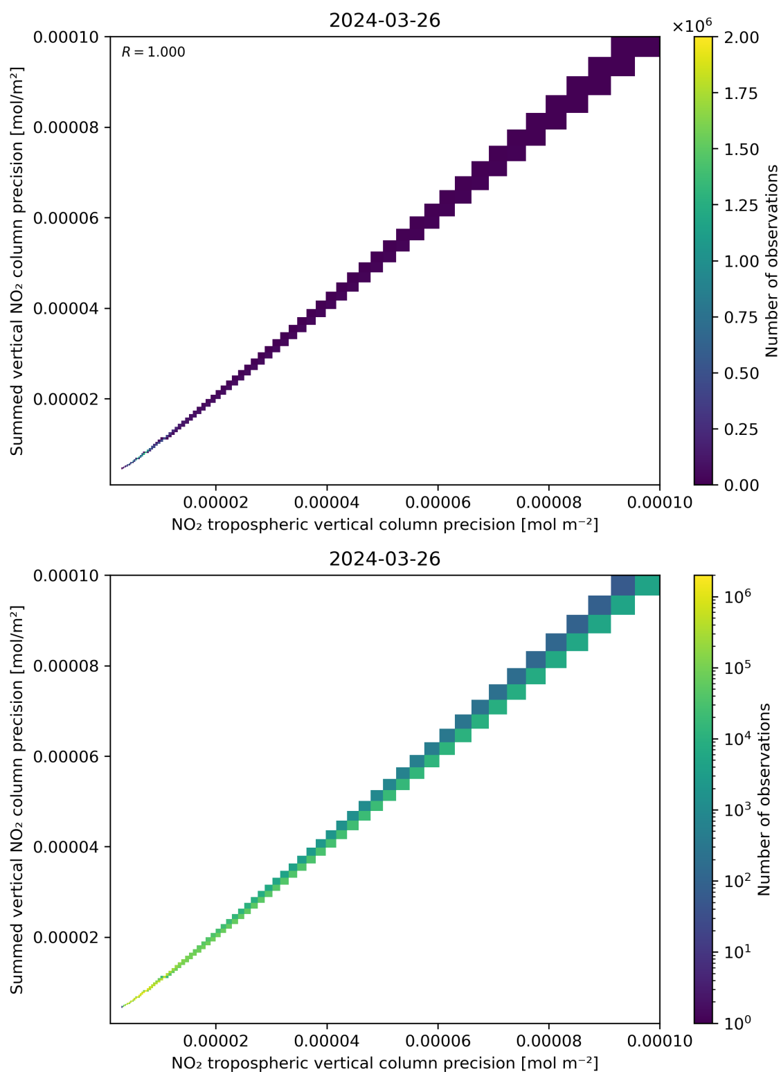
Figure 137: Scatter density plot of “NO 2 tropospheric vertical column precision” against “Summed vertical NO 2 column precision” for 2024-03-25 to 2024-03-27.
