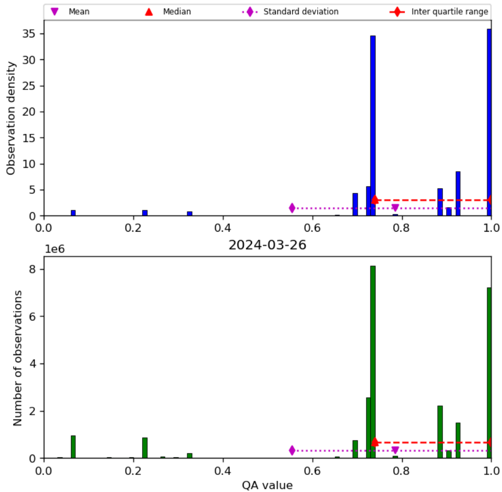
Figure 28: Histogram of “QA value” for 2024-03-25 to 2024-03-27
