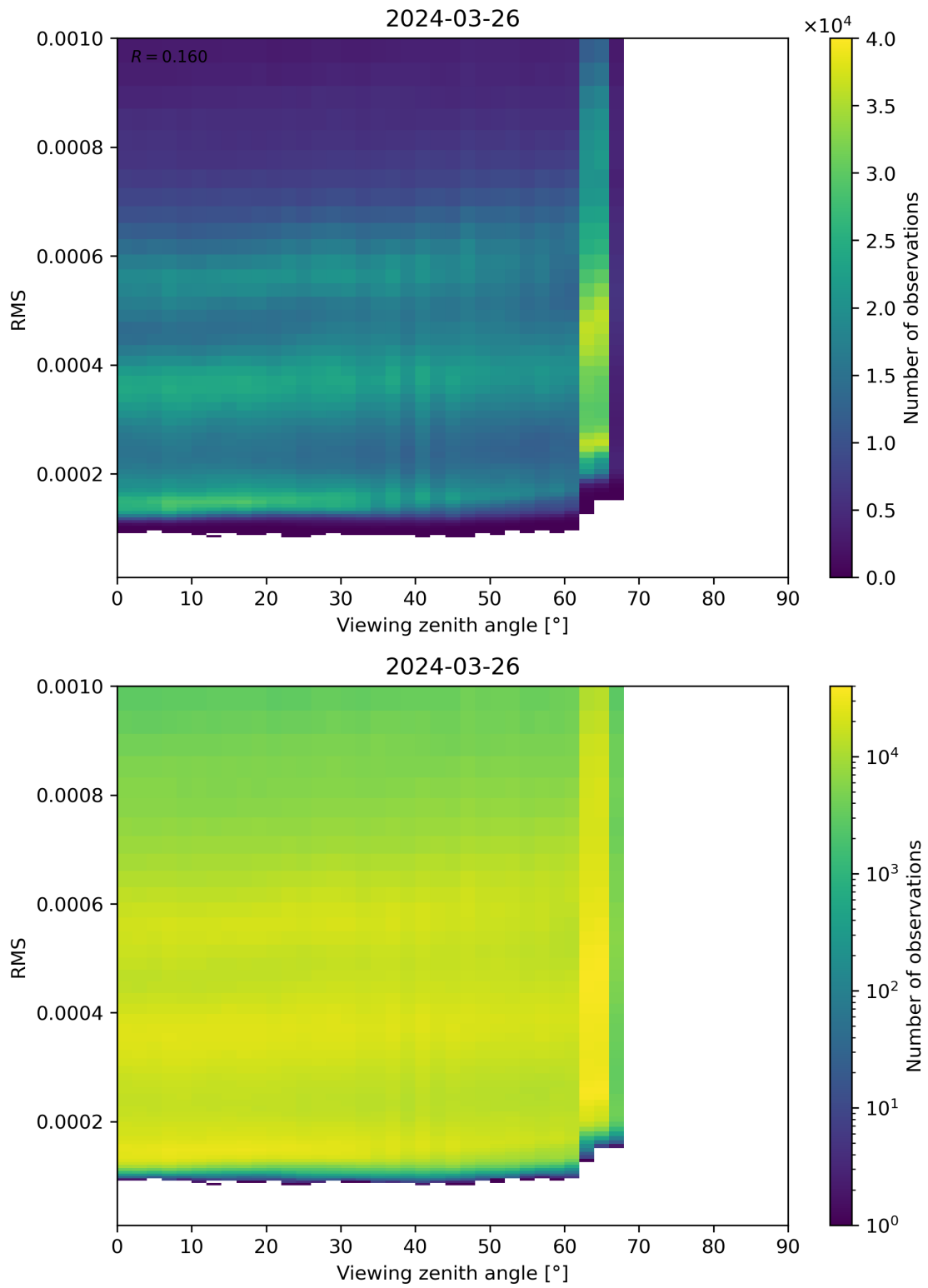
Figure 171: Scatter density plot of “Viewing zenith angle” against “RMS” for 2024-03-25 to 2024-03-27.
