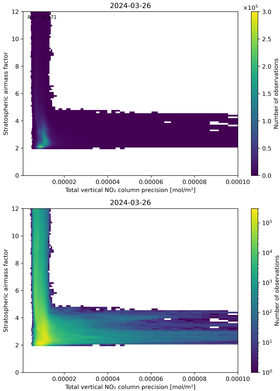
Figure 115: Scatter density plot of “Total vertical NO 2 column precision” against “Stratospheric airmass factor” for 2024-03-25 to 2024-03-27.
