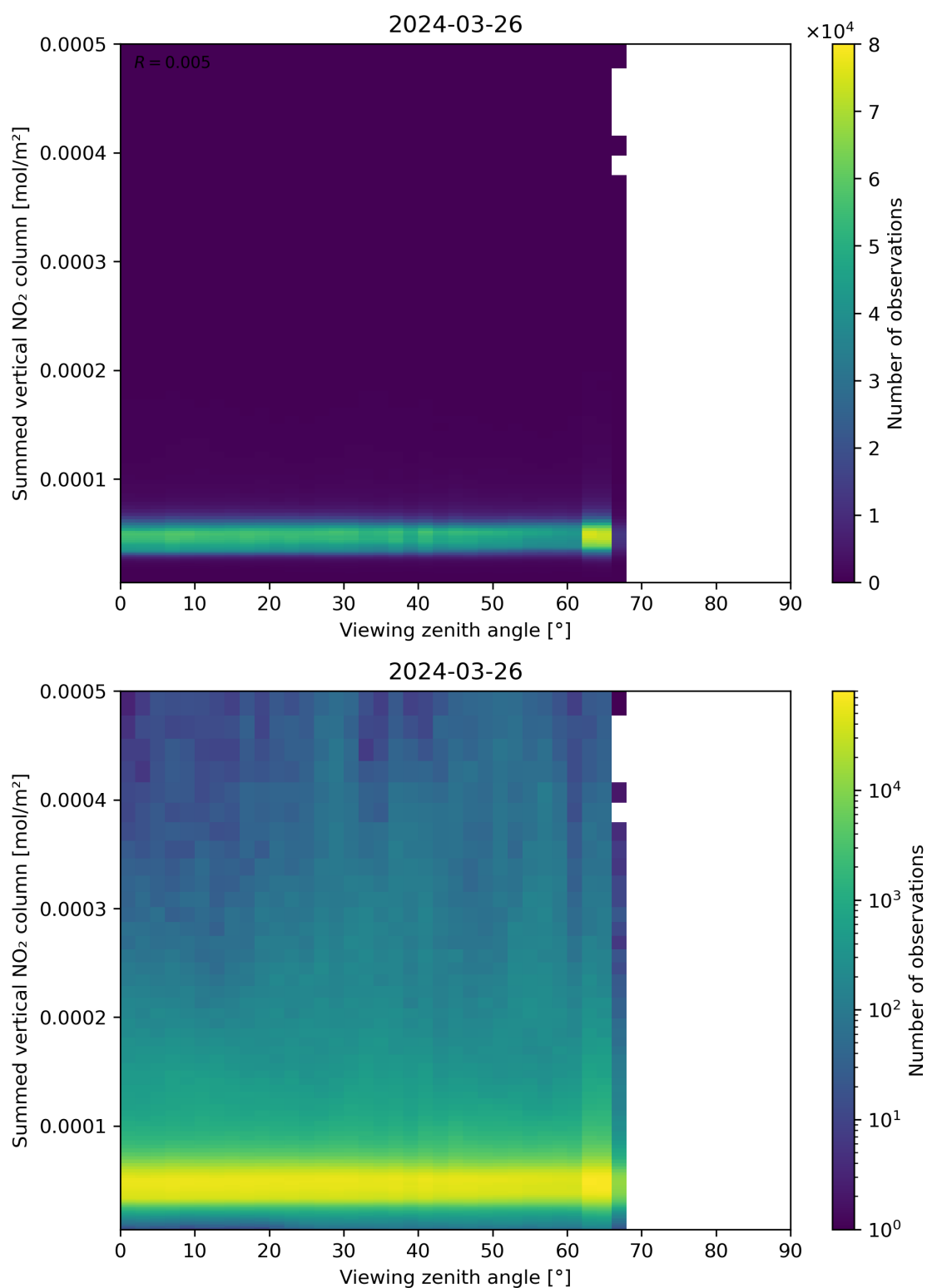
Figure 165: Scatter density plot of “Viewing zenith angle” against “Summed vertical NO 2 column” for 2024-03-25 to 2024-03-27.
