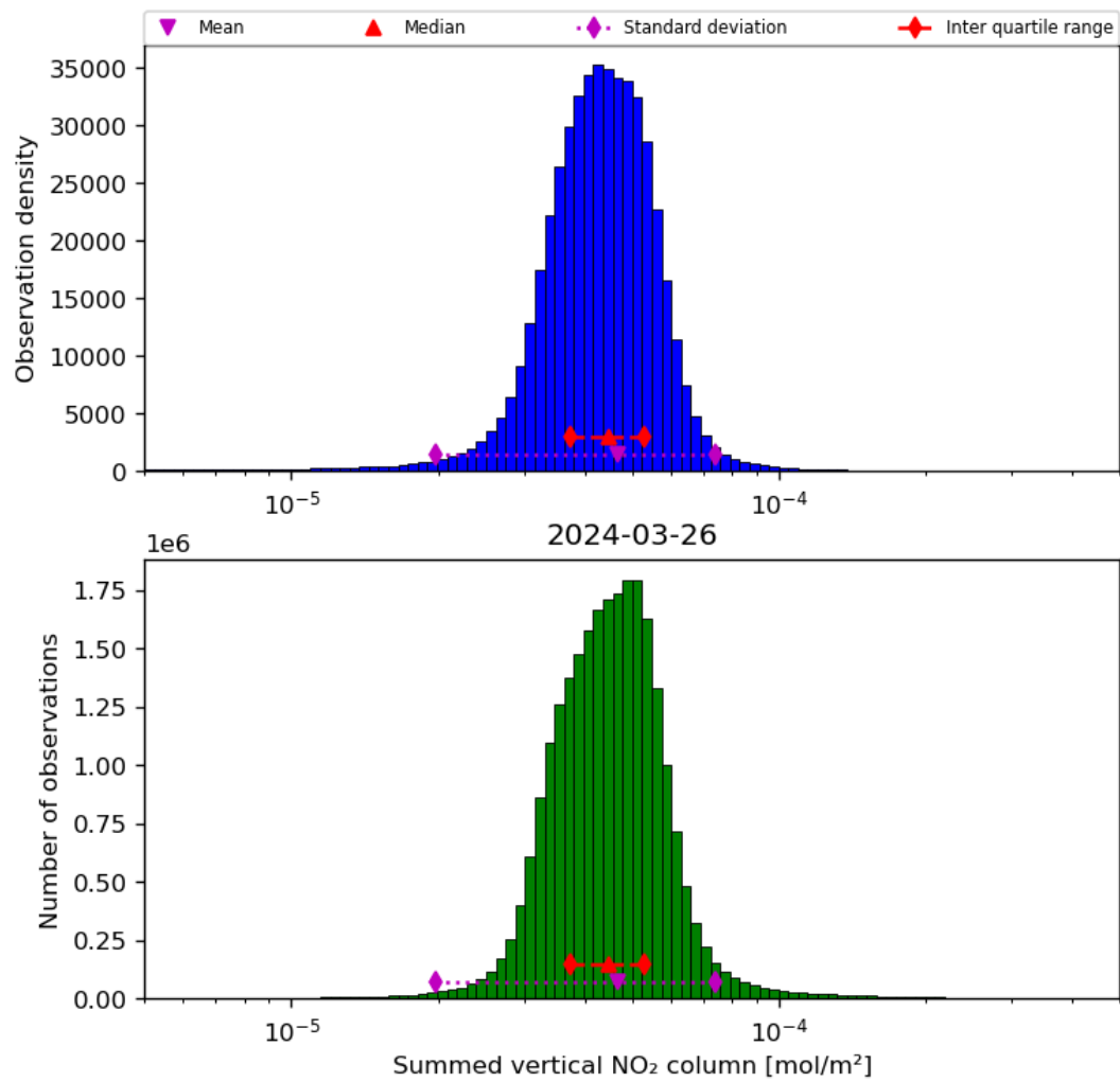
Figure 40: Histogram of “Summed vertical NO 2 column” for 2024-03-25 to 2024-03-27
