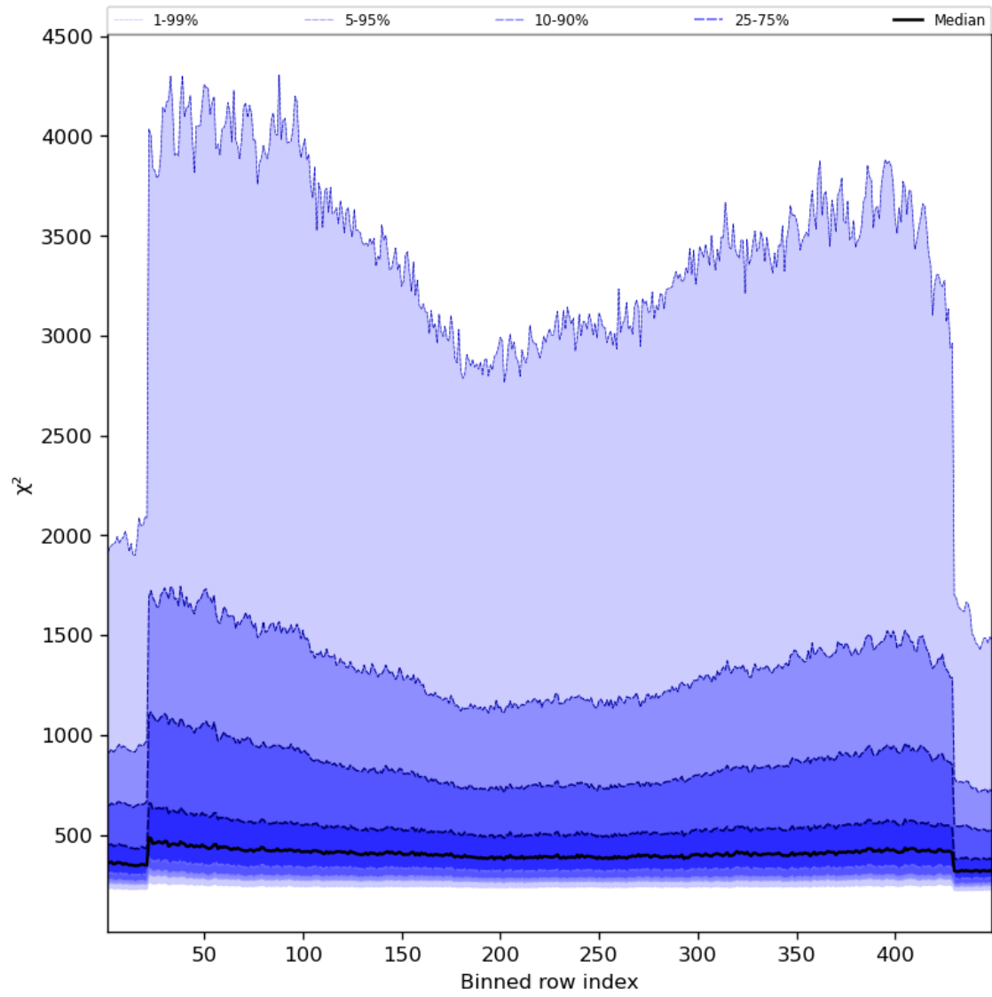
Figure 59: Along track statistics of “ \chi^2 ” for 2024-03-25 to 2024-03-27
