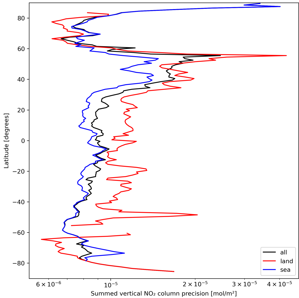
Figure 24: Zonal average of “Summed vertical NO 2 column precision” for 2024-03-25 to 2024-03-27.
