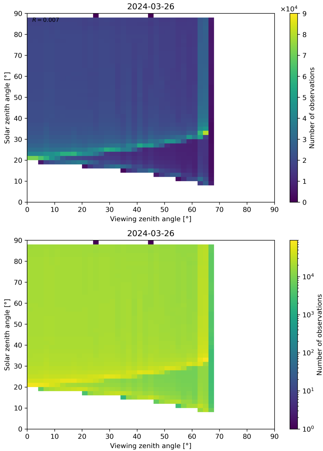
Figure 172: Scatter density plot of “Viewing zenith angle” against “Solar zenith angle” for 2024-03-25 to 2024-03-27.
