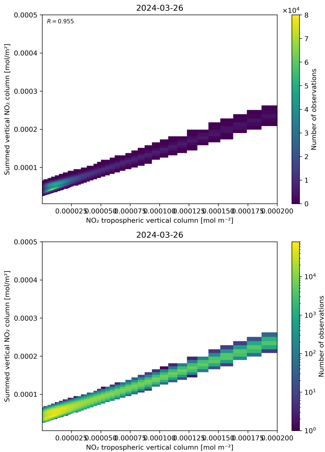
Figure 126: Scatter density plot of “NO 2 tropospheric vertical column” against “Summed vertical NO 2 column” for 2024-03-25 to 2024-03-27.
