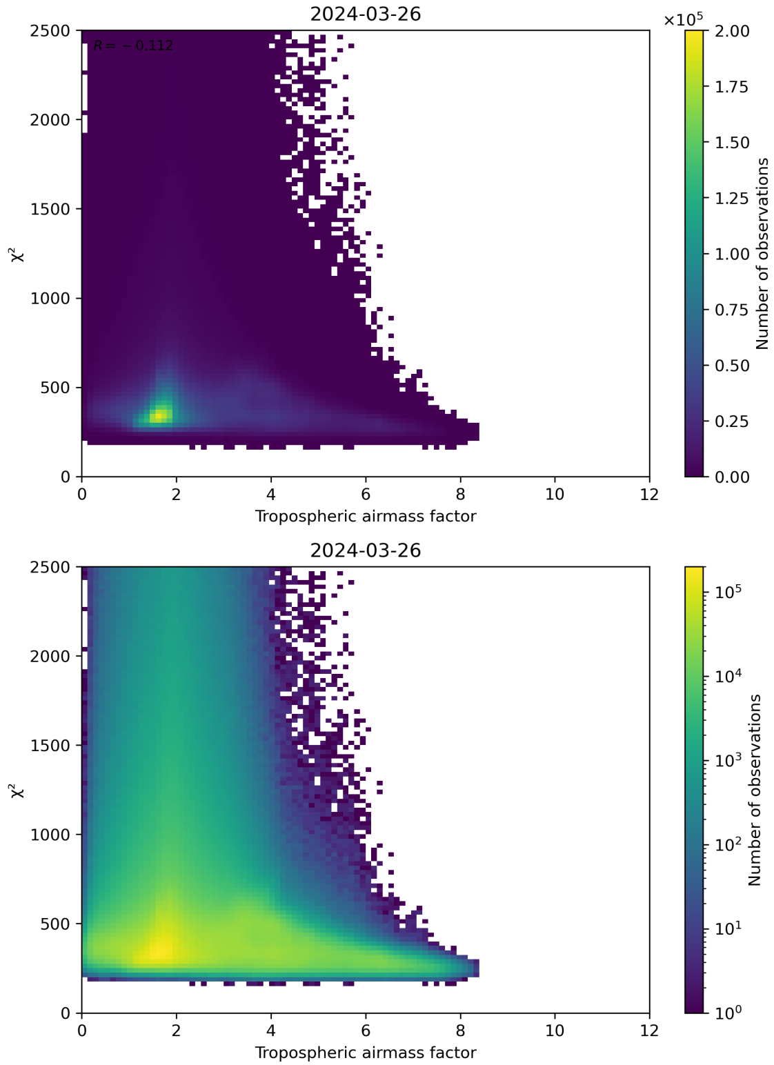
Figure 73: Scatter density plot of “Tropospheric airmass factor” against “ \chi^2 ” for 2024-03-25 to 2024-03-27.
