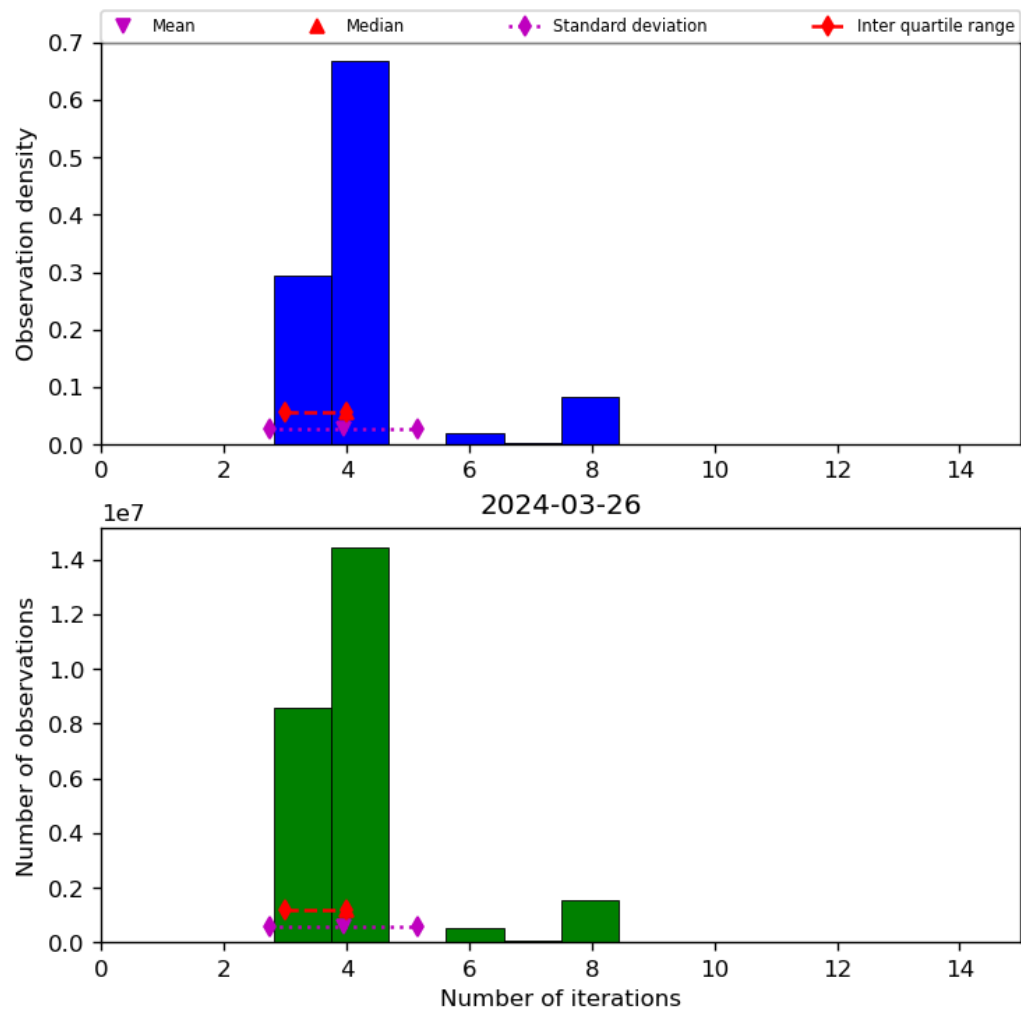
Figure 34: Histogram of “Number of iterations” for 2024-03-25 to 2024-03-27
