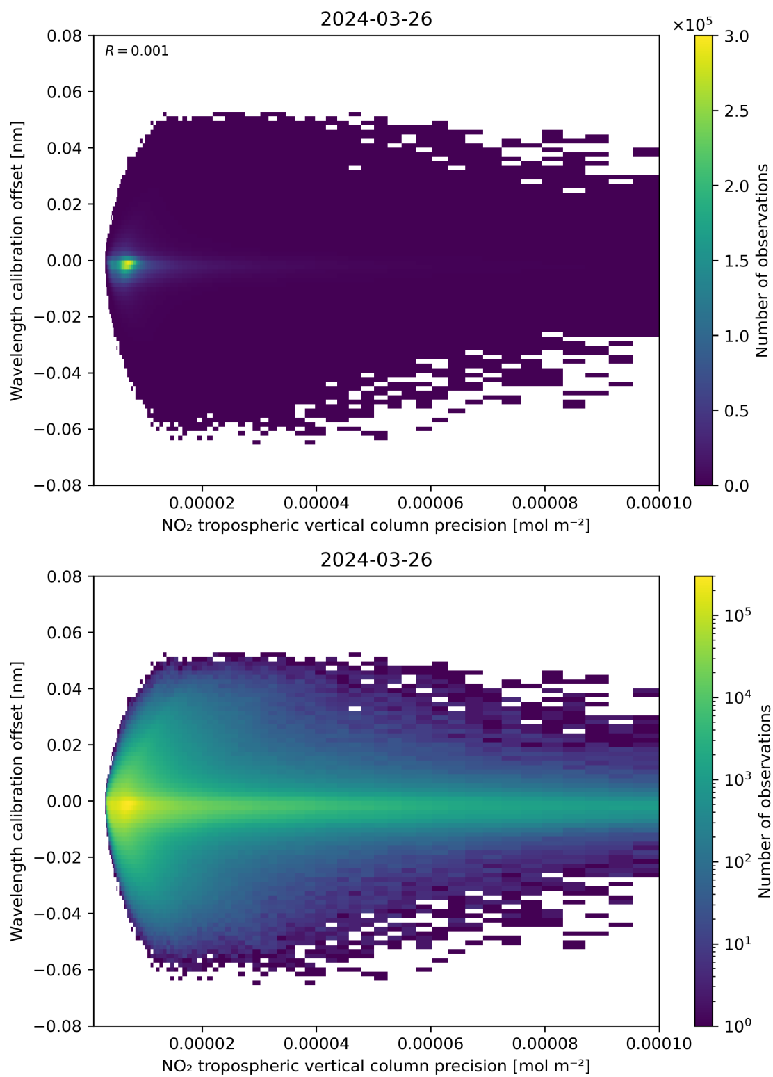
Figure 141: Scatter density plot of “NO 2 tropospheric vertical column precision” against “Wavelength calibration offset” for 2024-03-25 to 2024-03-27.
