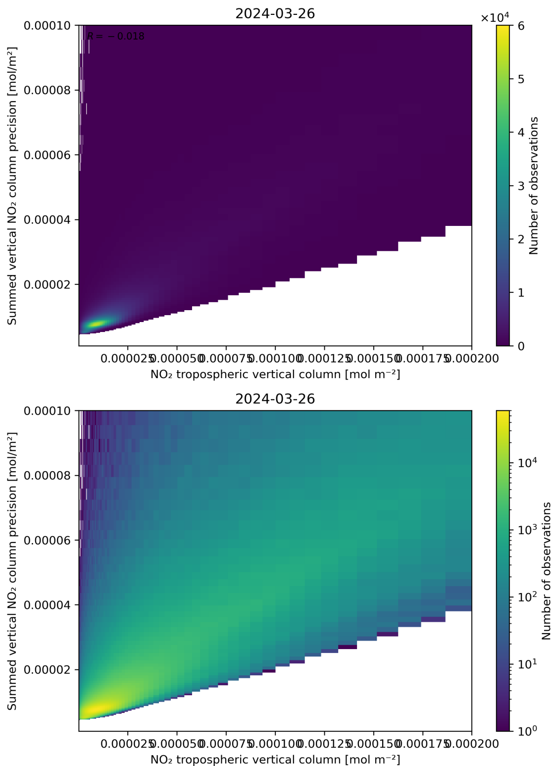
Figure 127: Scatter density plot of “NO 2 tropospheric vertical column” against “Summed vertical NO 2 column precision” for 2024-03-25 to 2024-03-27.
