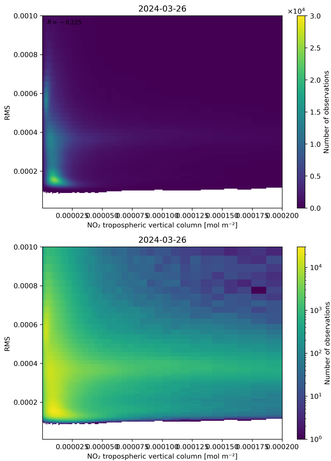
Figure 142: Scatter density plot of “NO 2 tropospheric vertical column” against “RMS” for 2024-03-25 to 2024-03-27.
