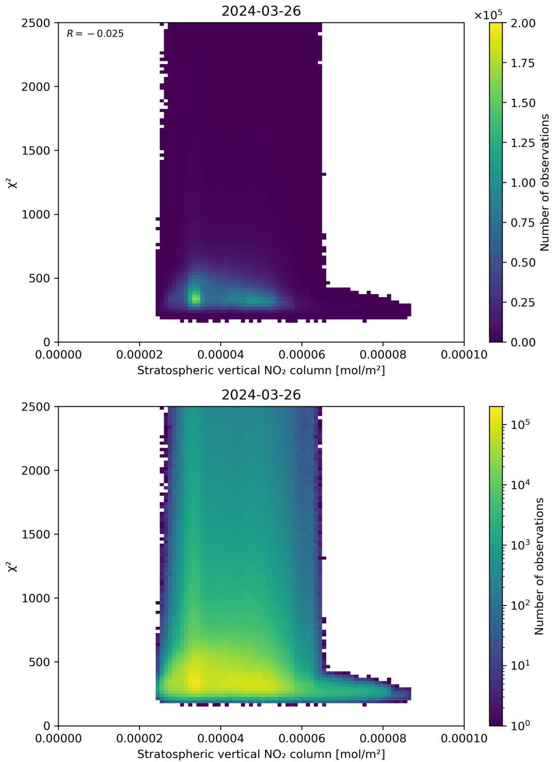
Figure 97: Scatter density plot of “Stratospheric vertical NO 2 column” against “ \chi^2 ” for 2024-03-25 to 2024-03-27.
