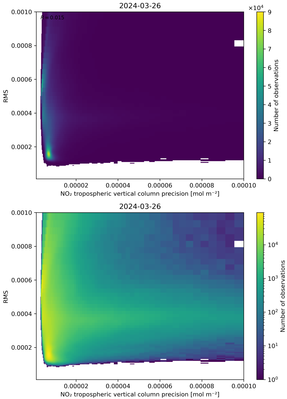
Figure 140: Scatter density plot of “NO 2 tropospheric vertical column precision” against “RMS” for 2024-03-25 to 2024-03-27.
