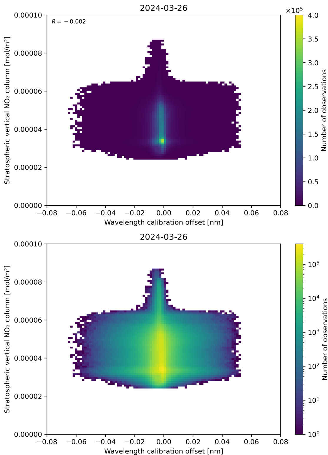
Figure 176: Scatter density plot of “Wavelength calibration offset” against “Stratospheric vertical NO 2 column” for 2024-03-25 to 2024-03-27.
