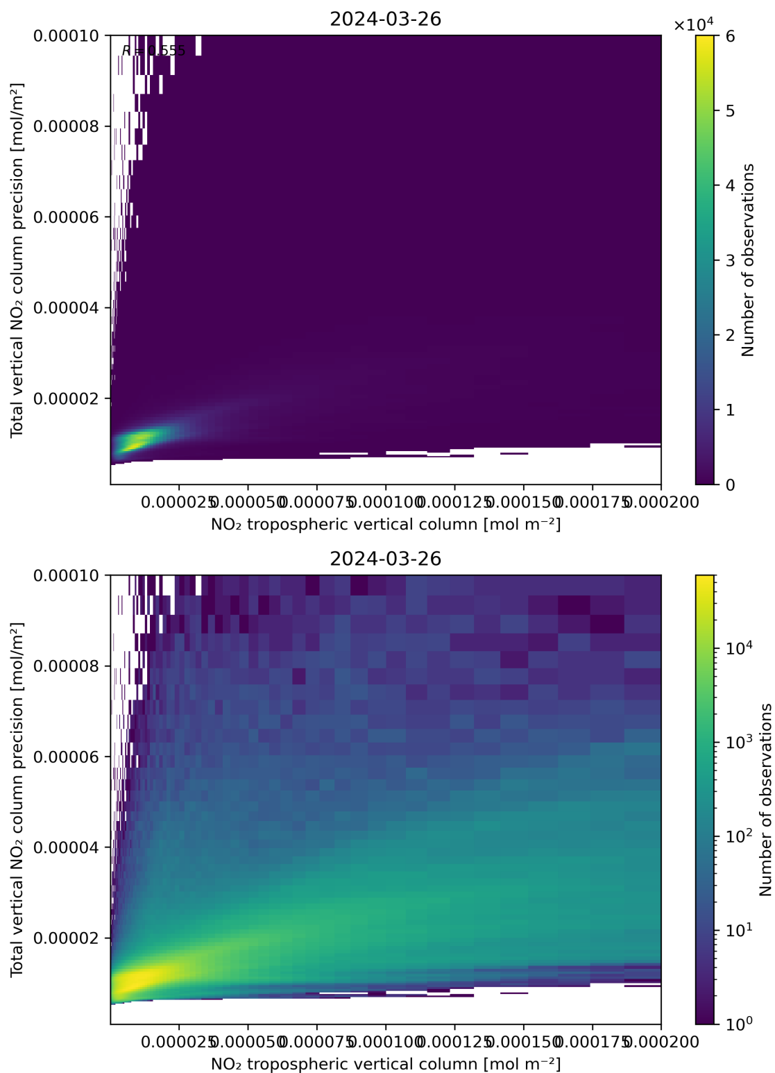
Figure 129: Scatter density plot of “NO 2 tropospheric vertical column” against “Total vertical NO 2 column precision” for 2024-03-25 to 2024-03-27.
