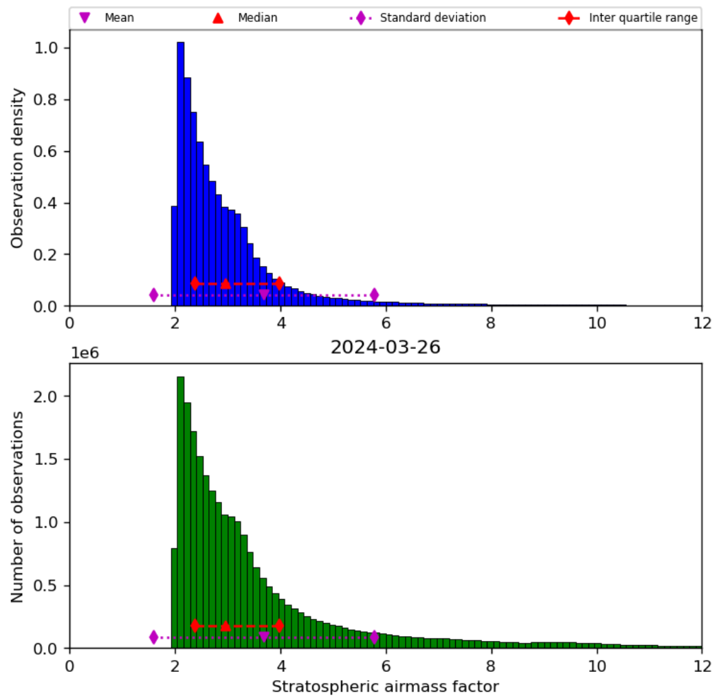
Figure 44: Histogram of “Stratospheric airmass factor” for 2024-03-25 to 2024-03-27
