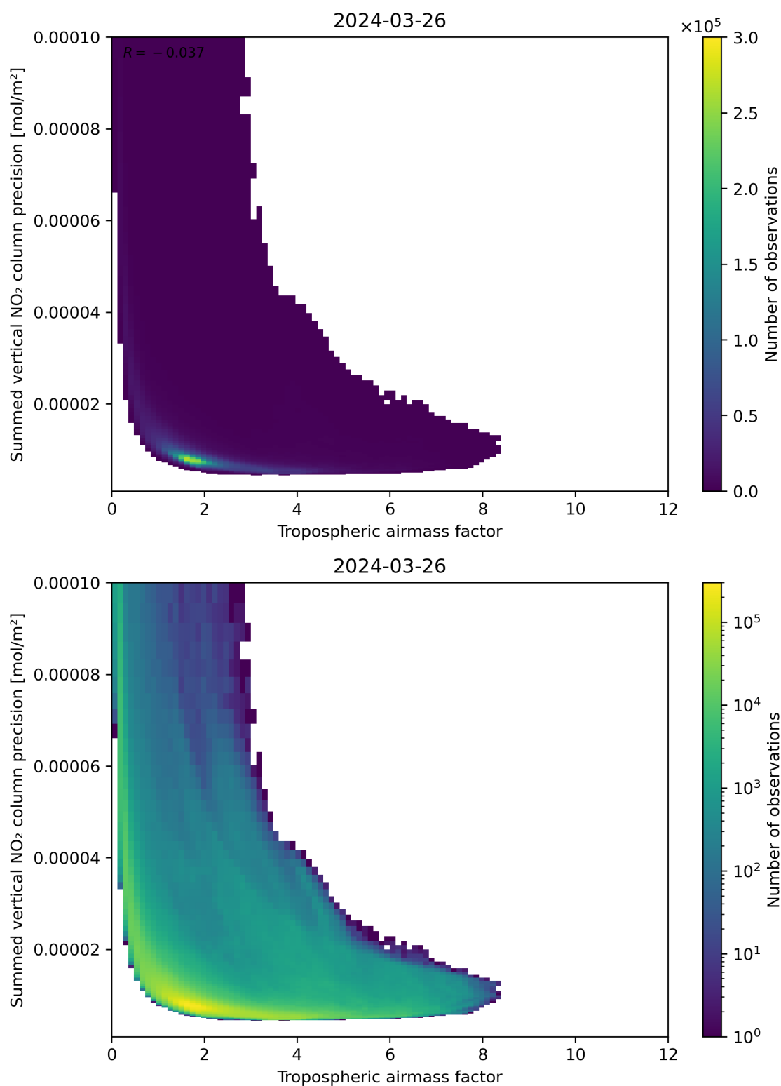
Figure 76: Scatter density plot of “Tropospheric air mass factor” against “Summed vertical NO 2 column precision” for 2024-03-25 to 2024-03-27.
