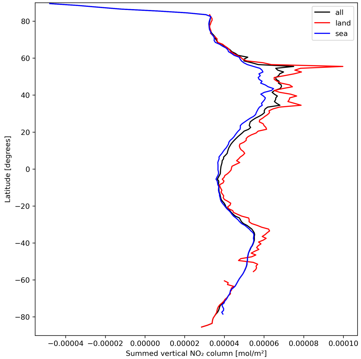
Figure 23: Zonal average of “Summed vertical NO 2 column” for 2024-03-25 to 2024-03-27.
