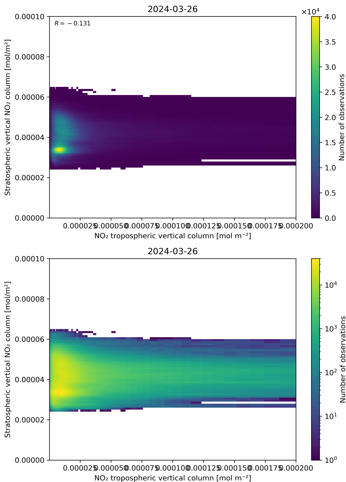
Figure 125: Scatter density plot of “NO 2 tropospheric vertical column” against “Stratospheric vertical NO 2 column” for 2024-03-25 to 2024-03-27.
