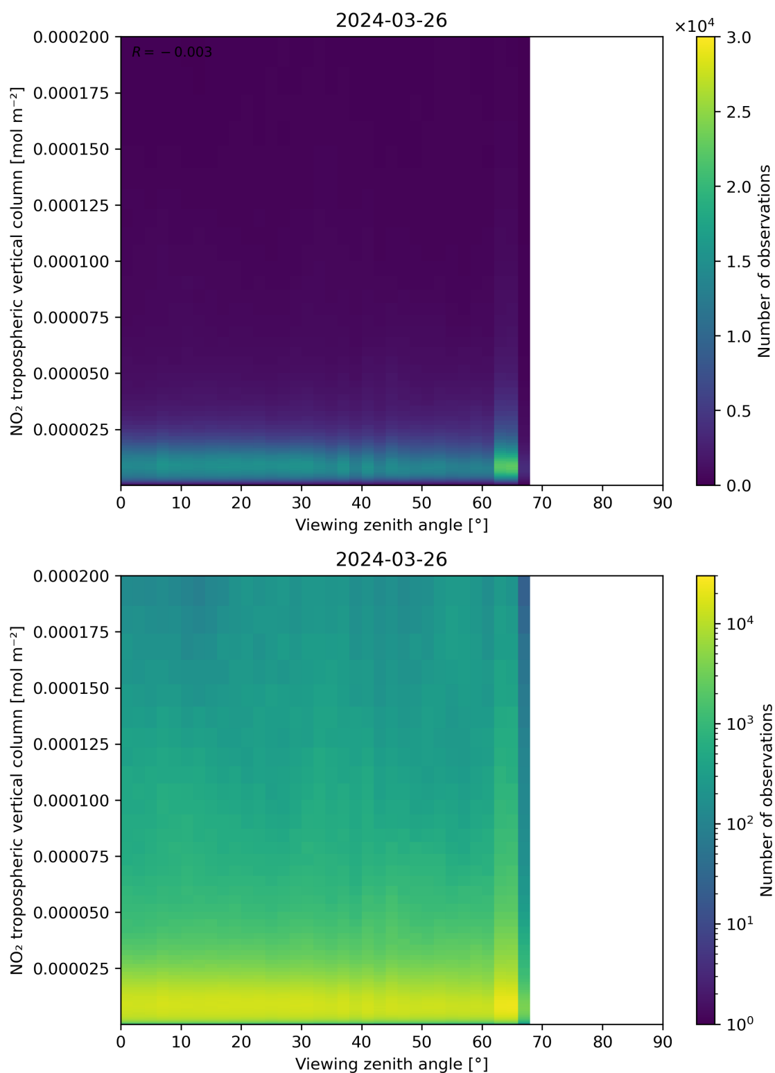
Figure 169: Scatter density plot of “Viewing zenith angle” against “NO 2 tropospheric vertical column” for 2024-03-25 to 2024-03-27.
