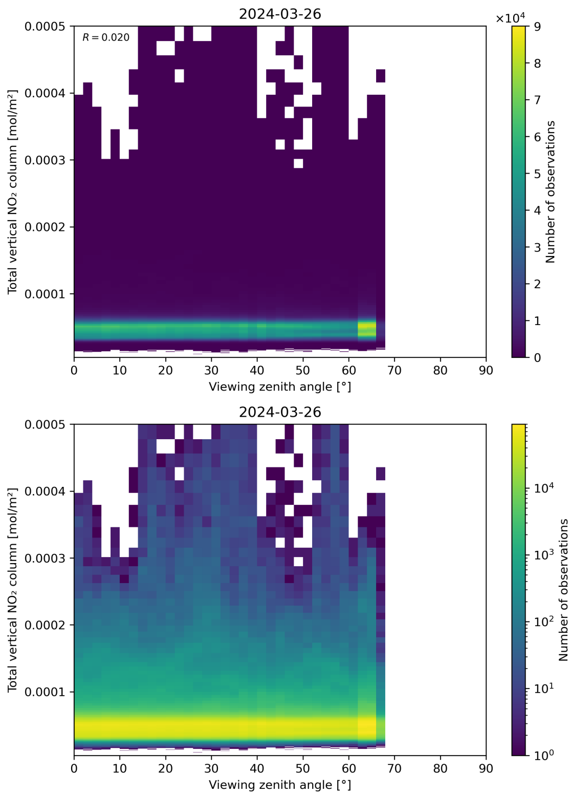
Figure 167: Scatter density plot of “Viewing zenith angle” against “Total vertical NO 2 column” for 2024-03-25 to 2024-03-27.
