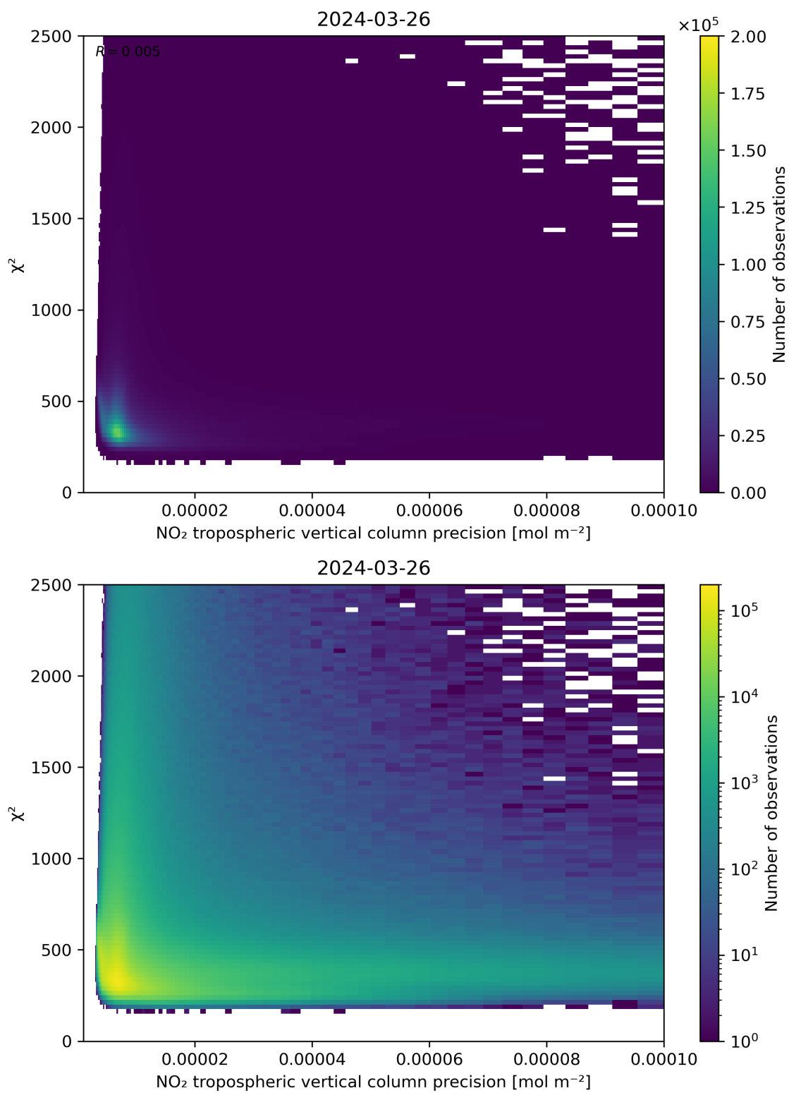
Figure 134: Scatter density plot of “NO 2 tropospheric vertical column precision” against “ \chi^2 ” for 2024-03-25 to 2024-03-27.
