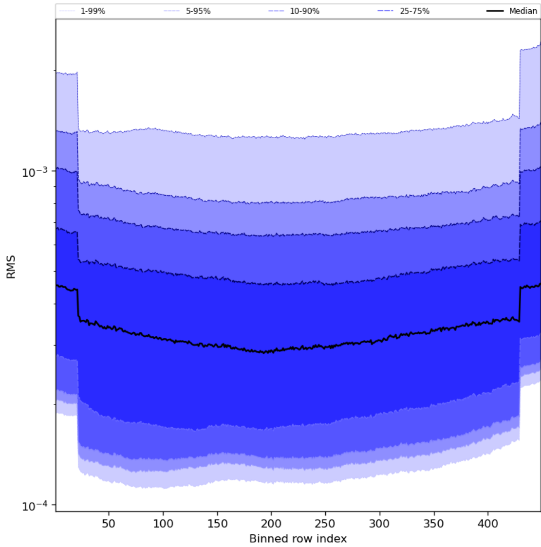
Figure 60: Along track statistics of “RMS” for 2024-03-25 to 2024-03-27
