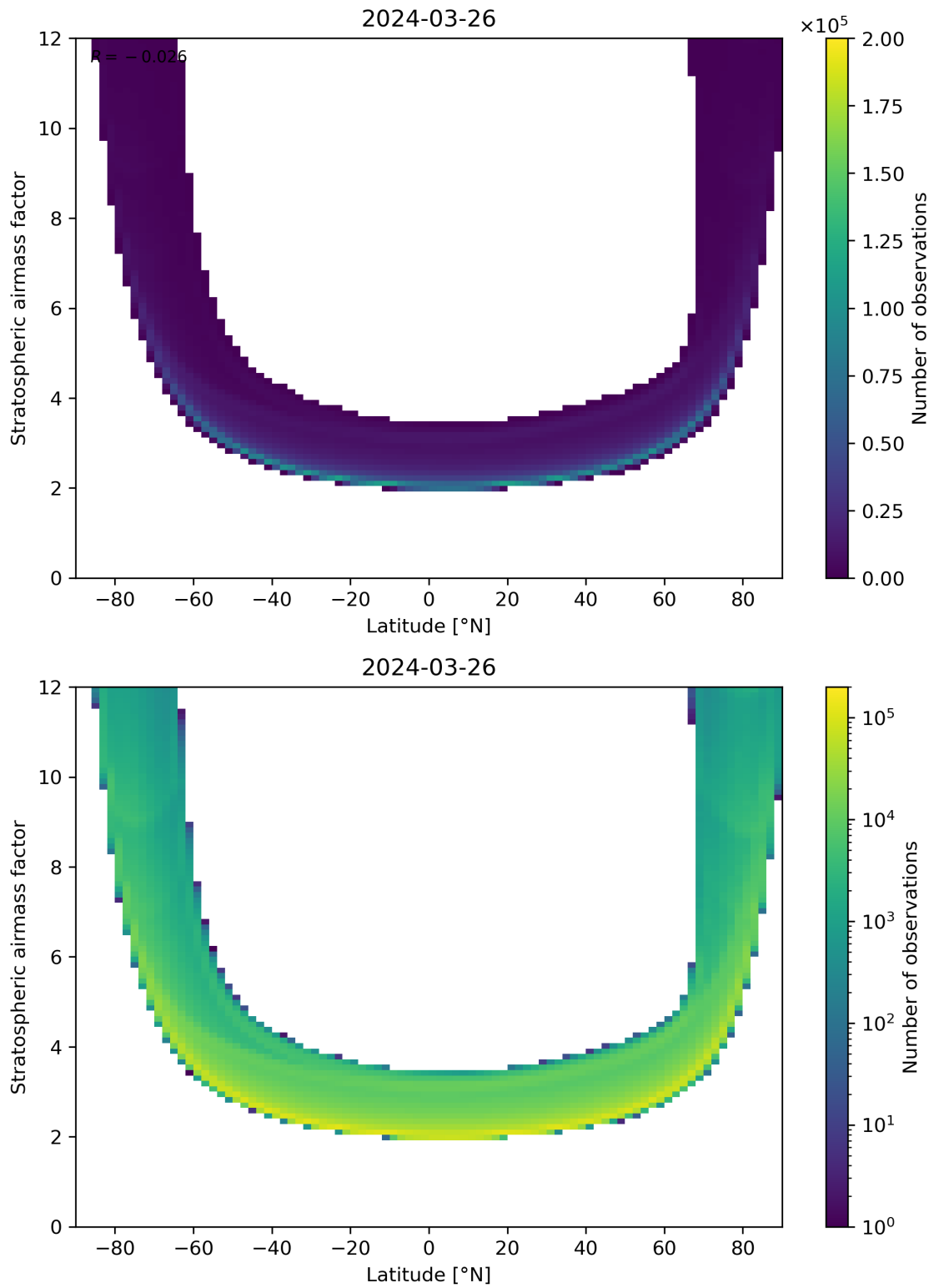
Figure 83: Scatter density plot of “Latitude” against “Stratospheric air mass factor” for 2024-03-25 to 2024-03-27.
