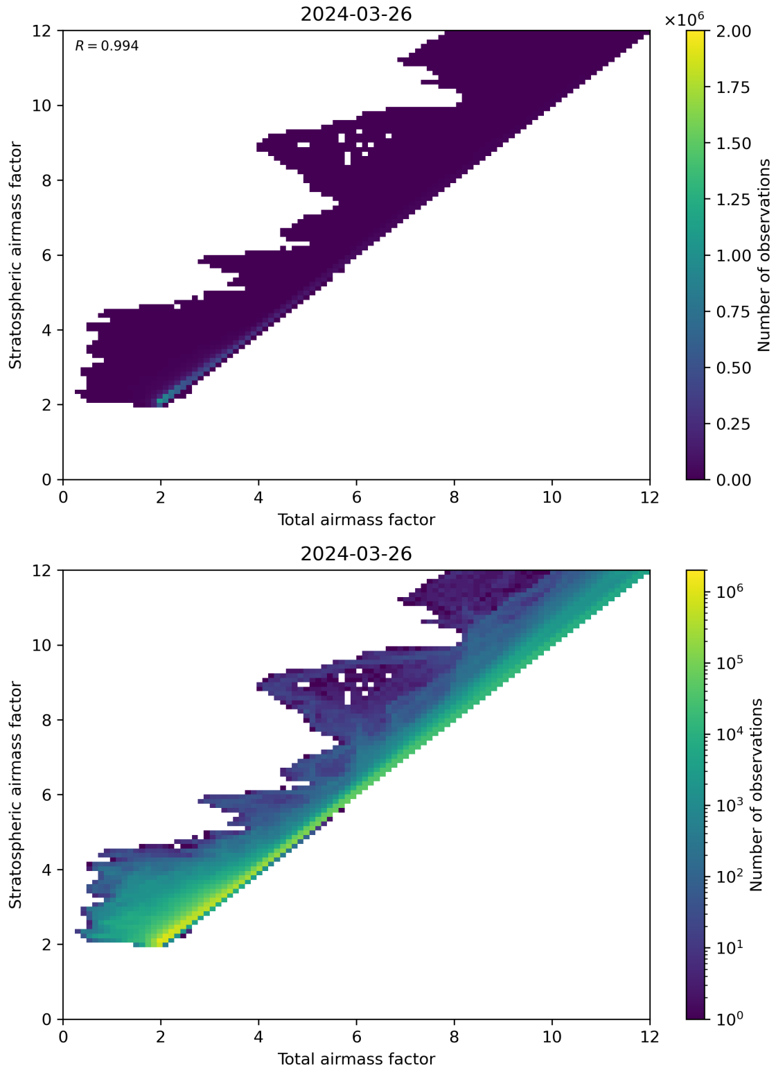
Figure 62: Scatter density plot of “Total airmass factor” against “Stratospheric airmass factor” for 2024-03-25 to 2024-03-27.
