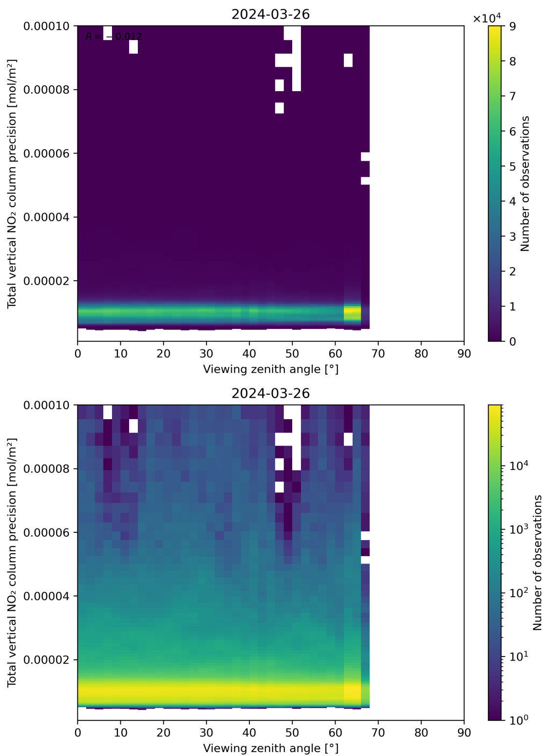
Figure 168: Scatter density plot of “Viewing zenith angle” against “Total vertical NO 2 column precision” for 2024-03-25 to 2024-03-27.
