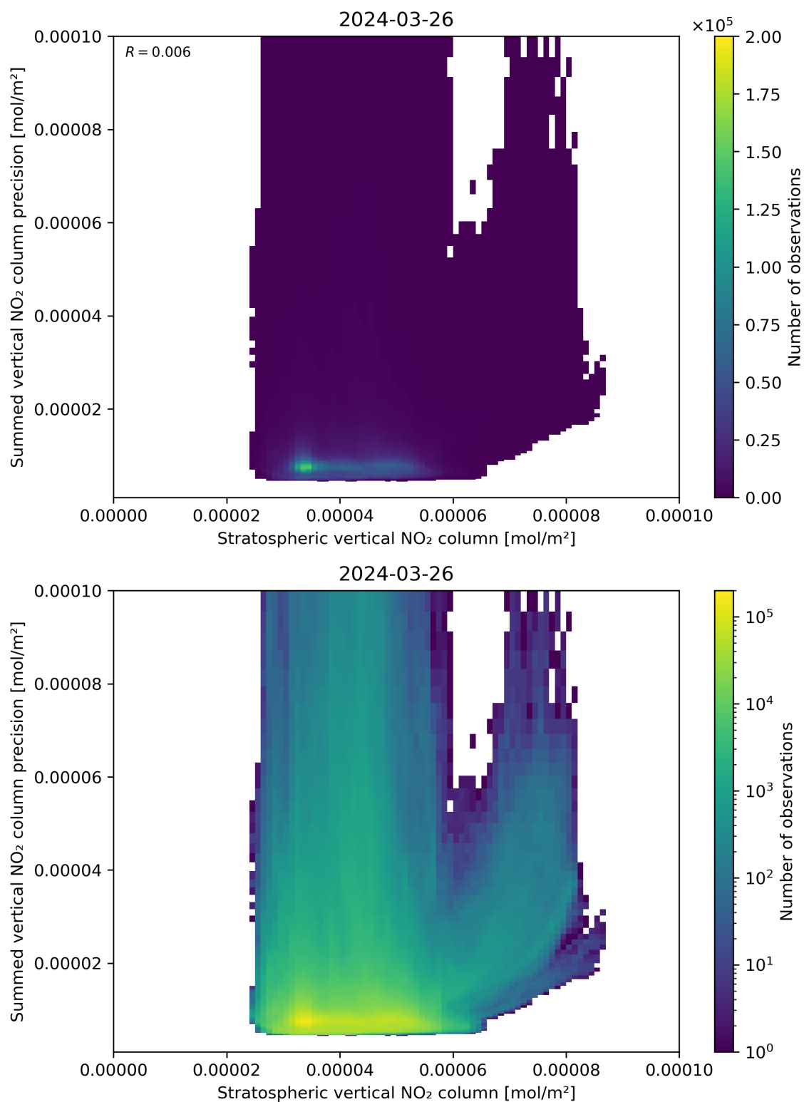
Figure 99: Scatter density plot of “Stratospheric vertical NO 2 column” against “Summed vertical NO 2 column precision” for 2024-03-25 to 2024-03-27.
