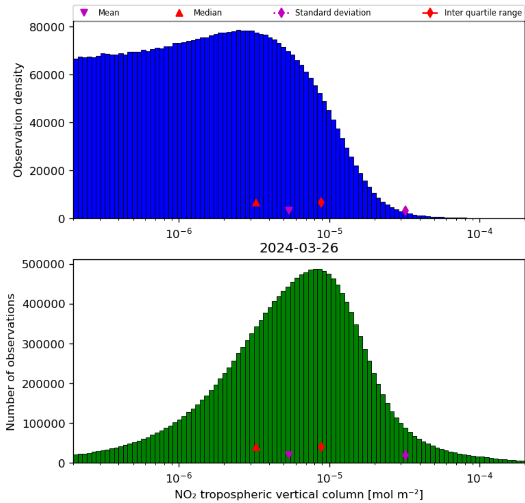
Figure 29: Histogram of “NO 2 tropospheric vertical column” for 2024-03-25 to 2024-03-27
