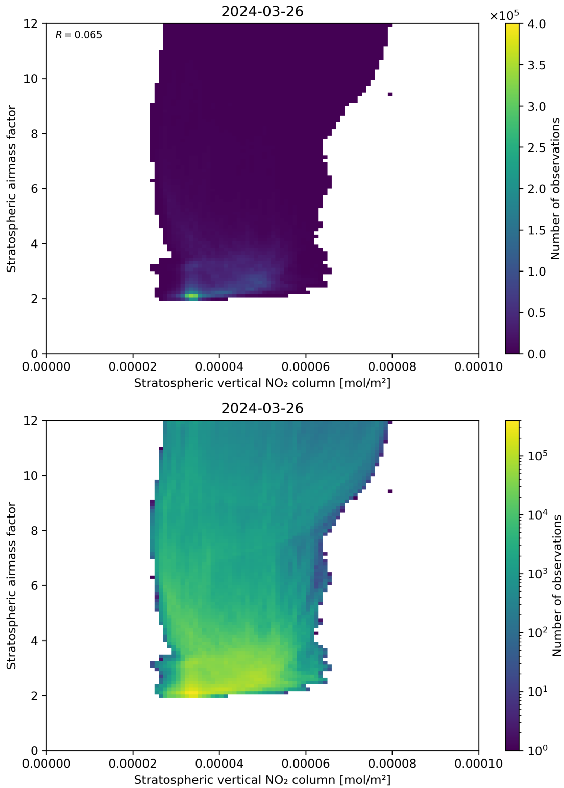
Figure 96: Scatter density plot of “Stratospheric vertical NO 2 column” against “Stratospheric airmass factor” for 2024-03-25 to 2024-03-27.
