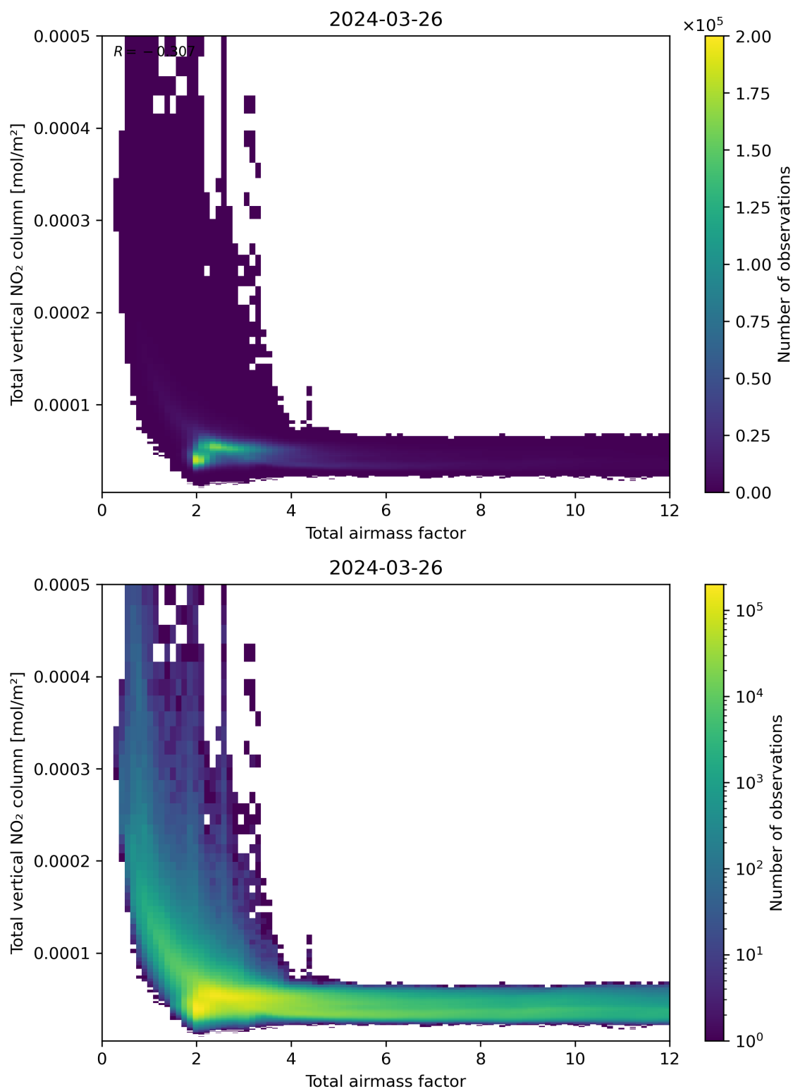
Figure 67: Scatter density plot of “Total airmass factor” against “Total vertical NO 2 column” for 2024-03-25 to 2024-03-27.
