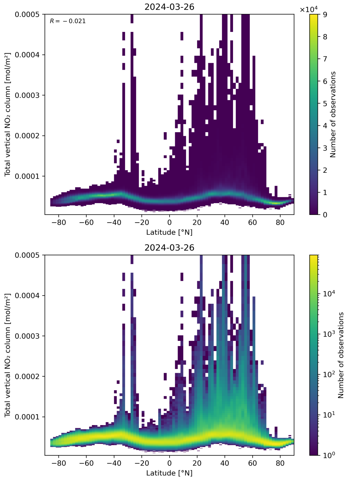
Figure 90: Scatter density plot of “Latitude” against “Total vertical NO 2 column” for 2024-03-25 to 2024-03-27.
