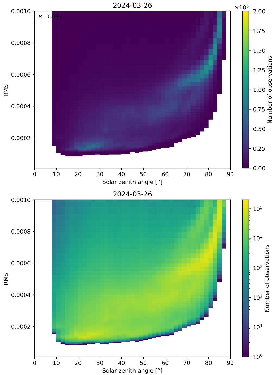
Figure 157: Scatter density plot of “Solar zenith angle” against “RMS” for 2024-03-25 to 2024-03-27.
