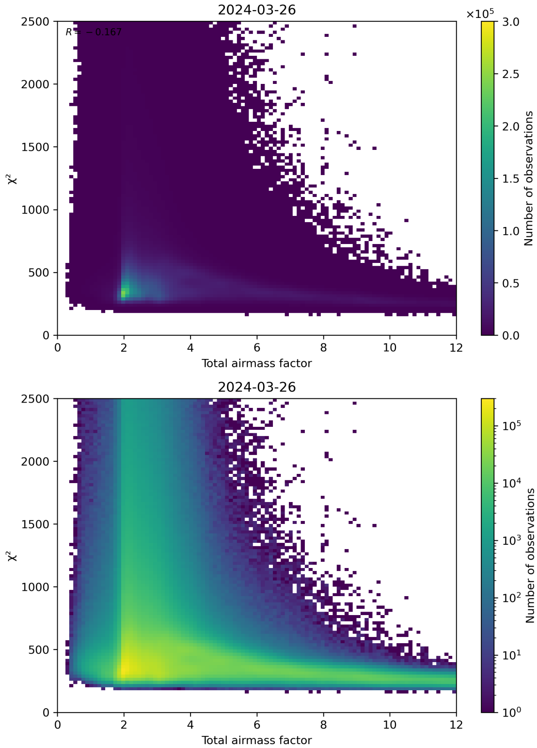
Figure 63: Scatter density plot of “Total airmass factor” against “ \chi^2 ” for 2024-03-25 to 2024-03-27.
