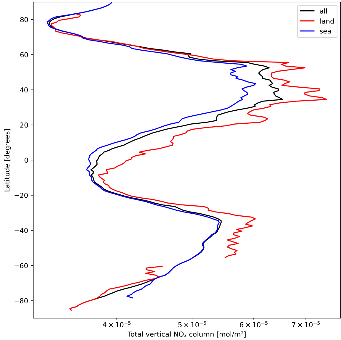
Figure 21: Zonal average of “Total vertical NO 2 column” for 2024-03-25 to 2024-03-27.
