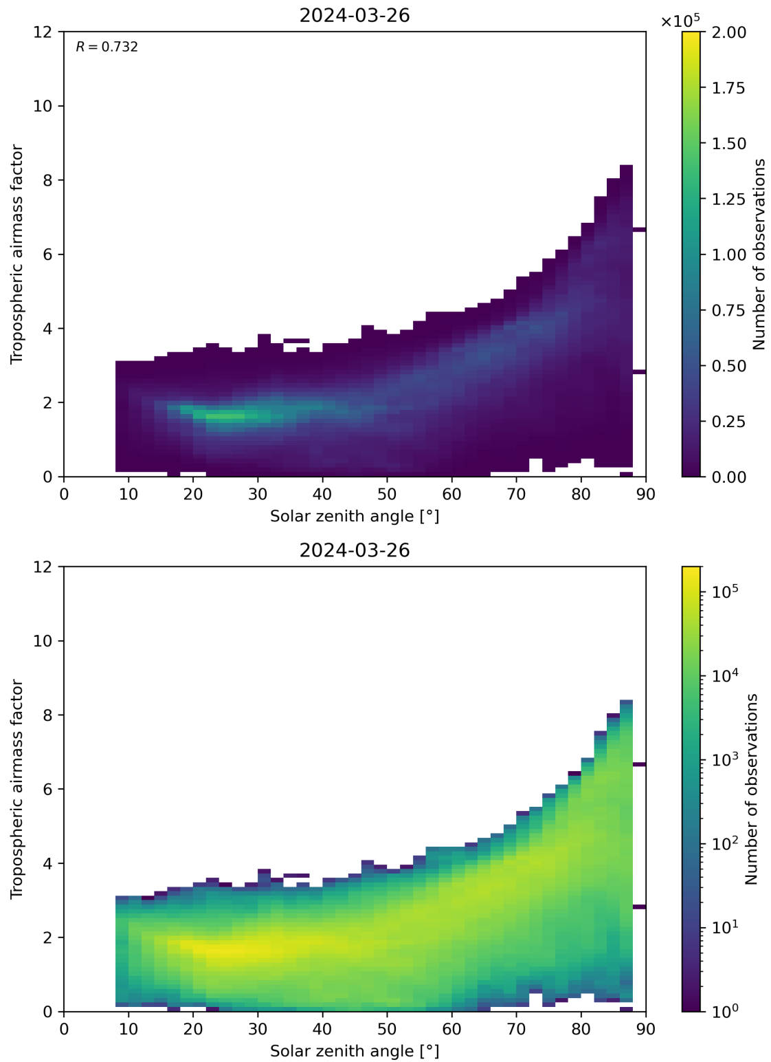
Figure 147: Scatter density plot of “Solar zenith angle” against “Tropospheric airmass factor” for 2024-03-25 to 2024-03-27.
