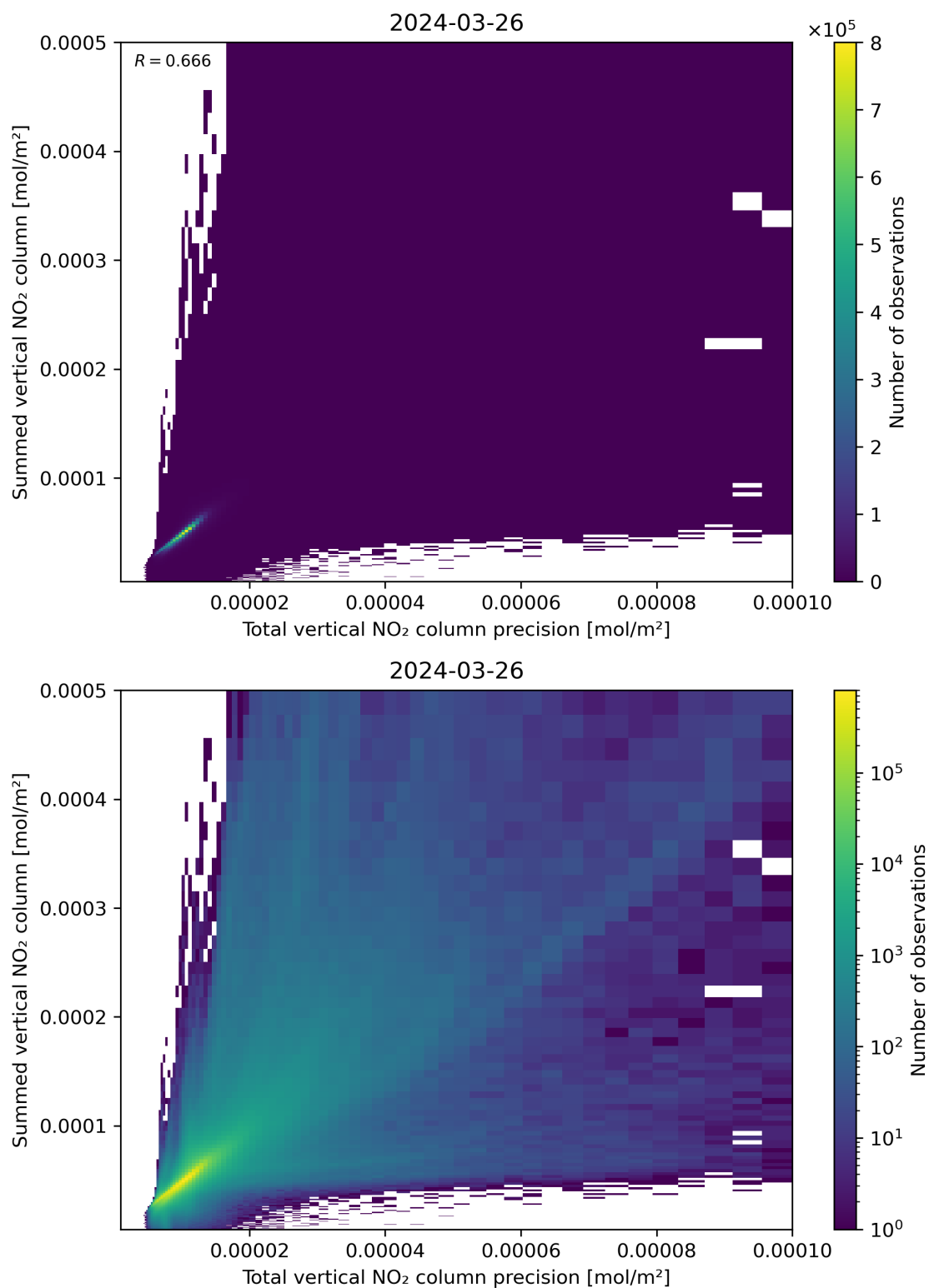
Figure 117: Scatter density plot of “Total vertical NO 2 column precision” against “Summed vertical NO 2 column” for 2024-03-25 to 2024-03-27.
