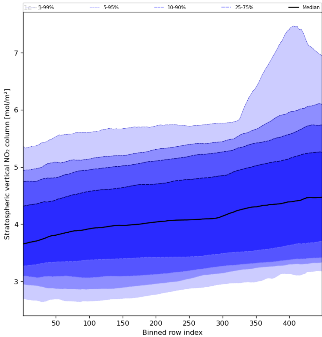
Figure 53: Along track statistics of “Stratospheric vertical NO 2 column” for 2024-03-25 to 2024-03-27
