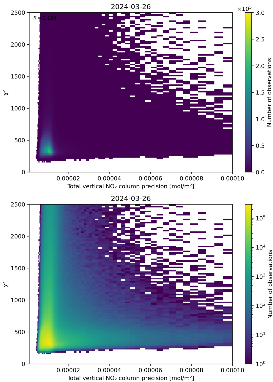
Figure 116: Scatter density plot of “Total vertical NO 2 column precision” against “ \chi^2 ” for 2024-03-25 to 2024-03-27.
