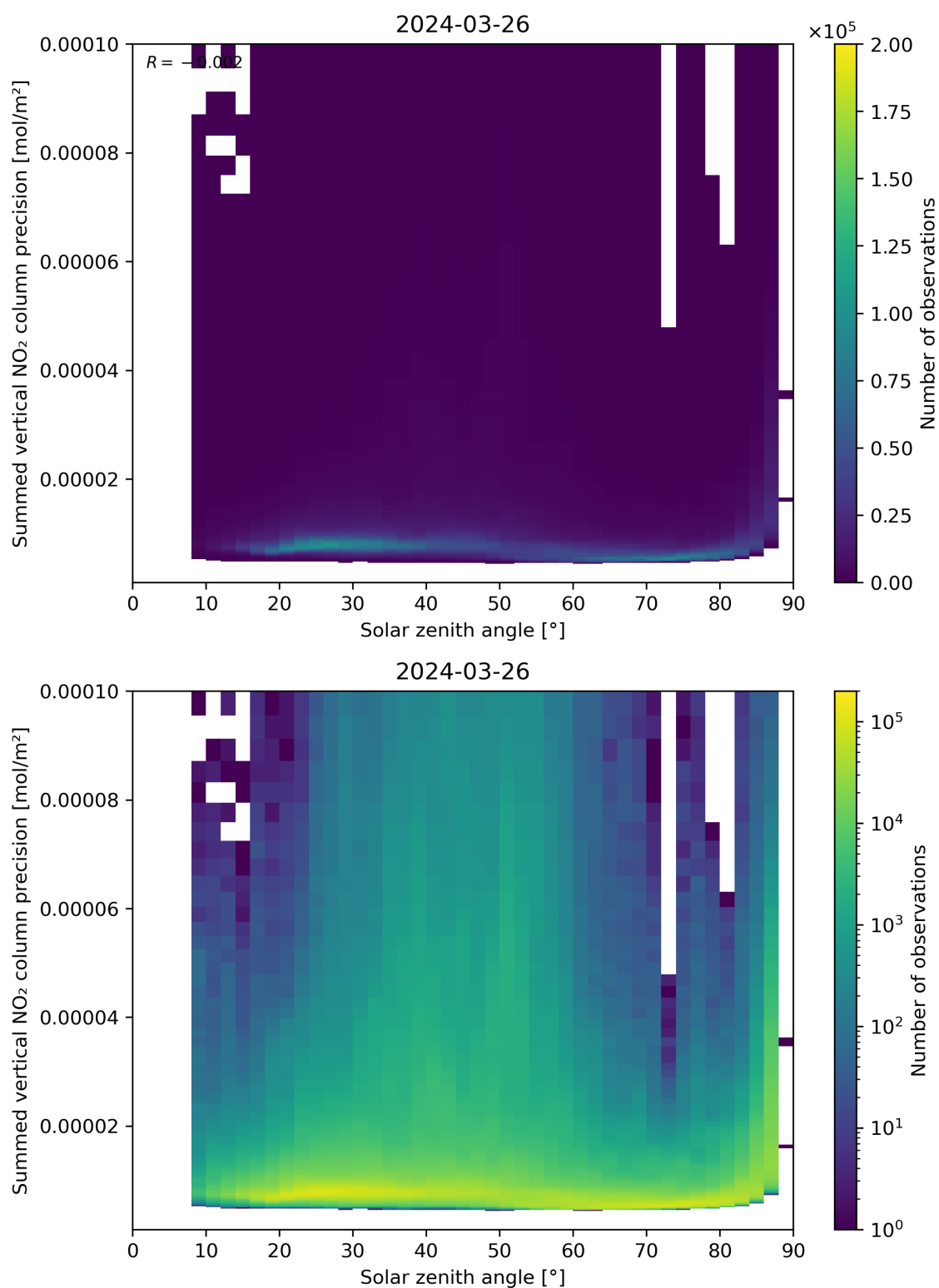
Figure 152: Scatter density plot of “Solar zenith angle” against “Summed vertical NO 2 column precision” for 2024-03-25 to 2024-03-27.
