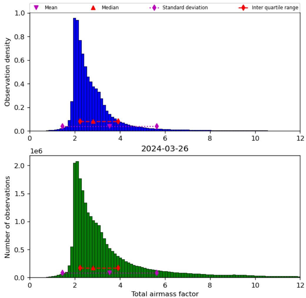
Figure 32: Histogram of “Total airmass factor” for 2024-03-25 to 2024-03-27
