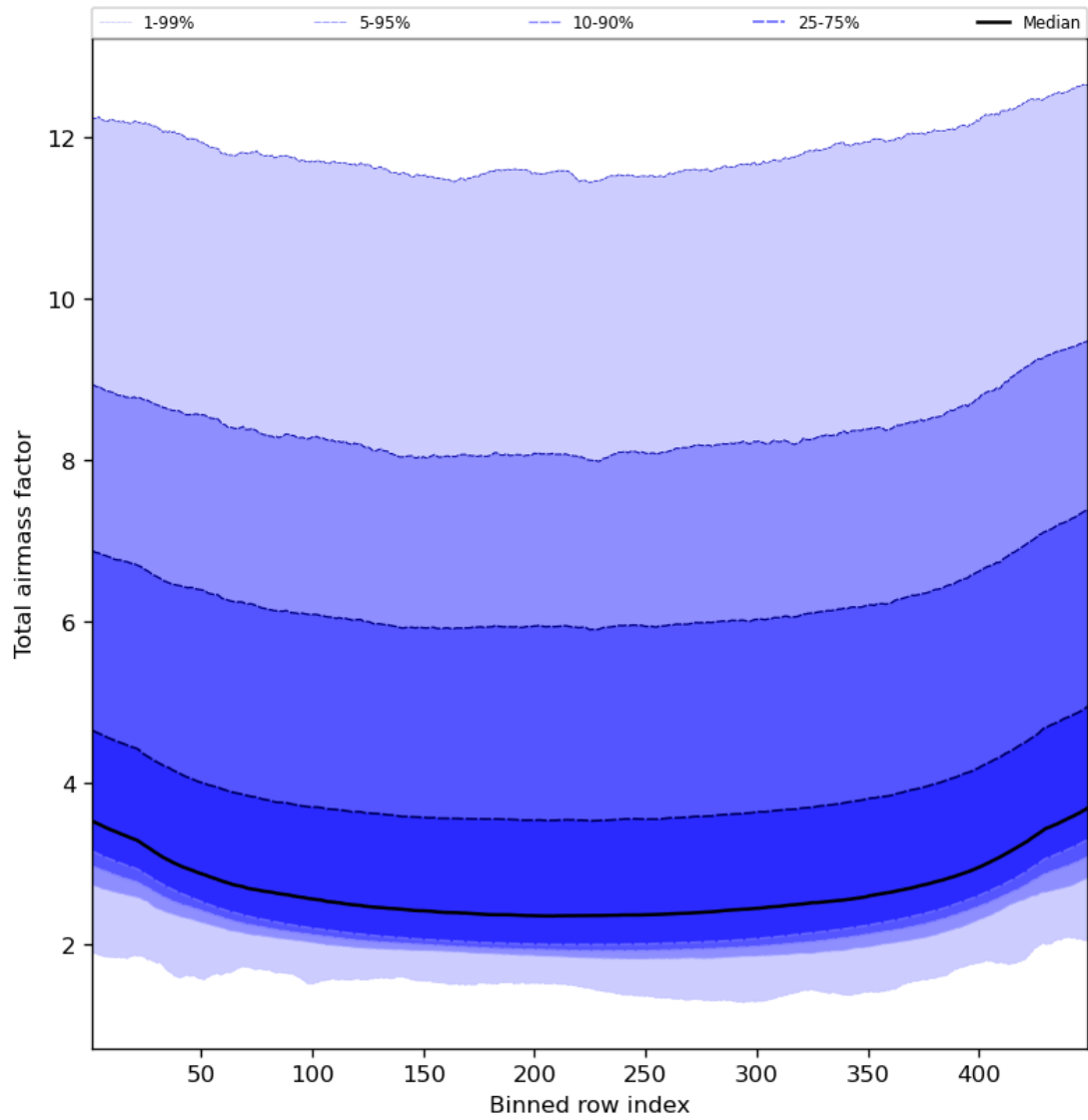
Figure 49: Along track statistics of “Total airmass factor” for 2024-03-25 to 2024-03-27
