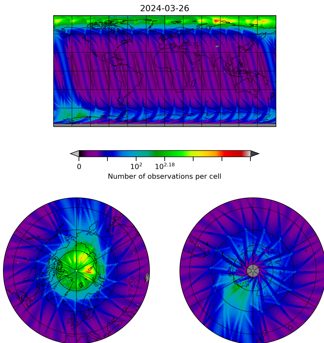
Figure 10: Map of the number of observations for 2024-03-25 to 2024-03-27
