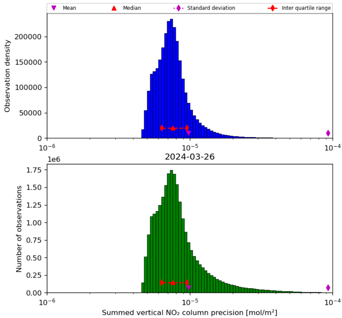
Figure 41: Histogram of "Summed vertical NO 2 column precision" for 2024-03-25 to 2024-03-27
