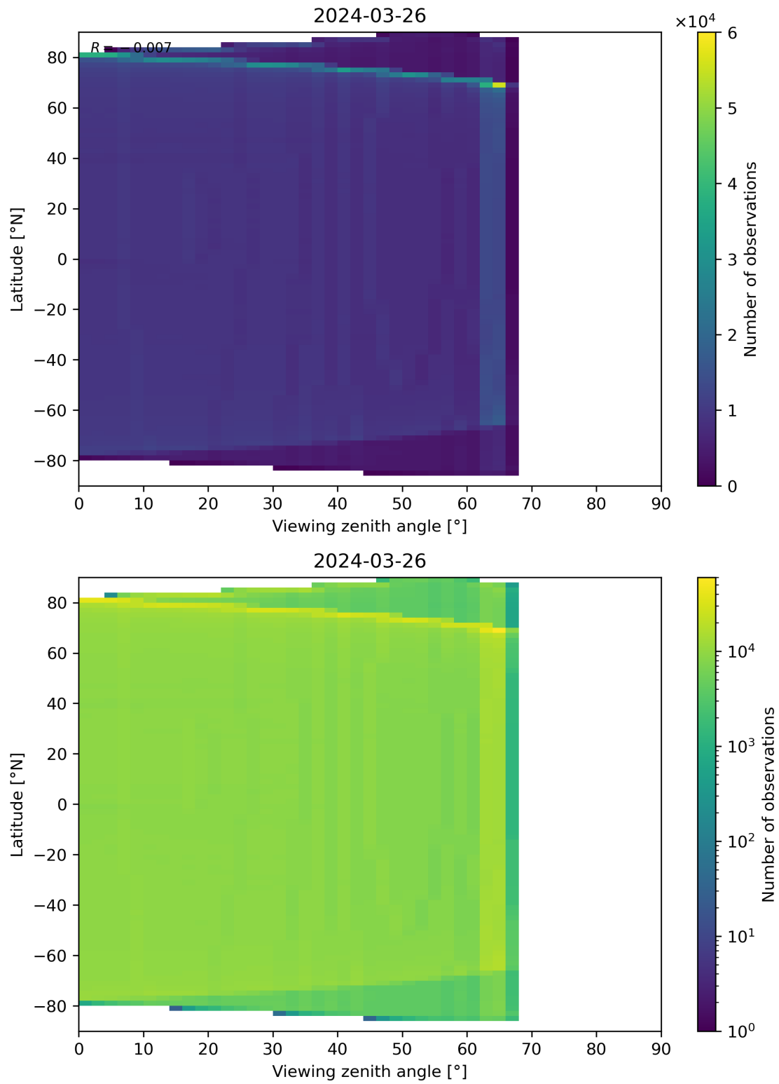
Figure 163: Scatter density plot of “Viewing zenith angle” against “Latitude” for 2024-03-25 to 2024-03-27.
