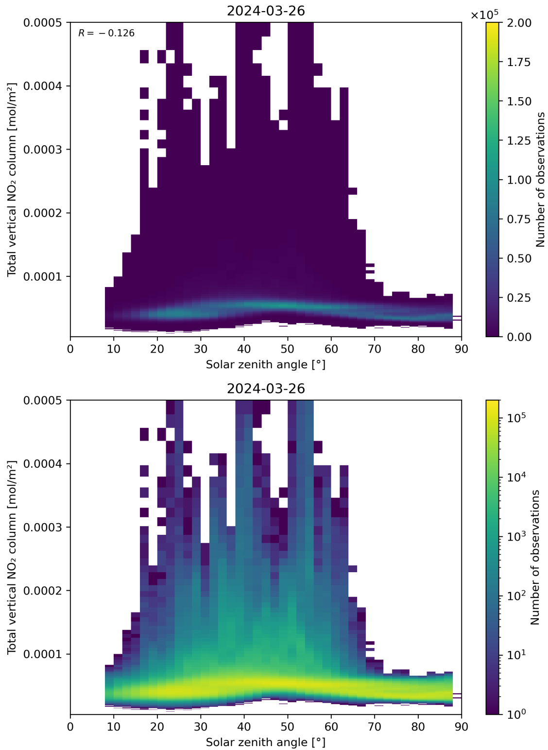
Figure 153: Scatter density plot of “Solar zenith angle” against “Total vertical NO 2 column” for 2024-03-25 to 2024-03-27.
