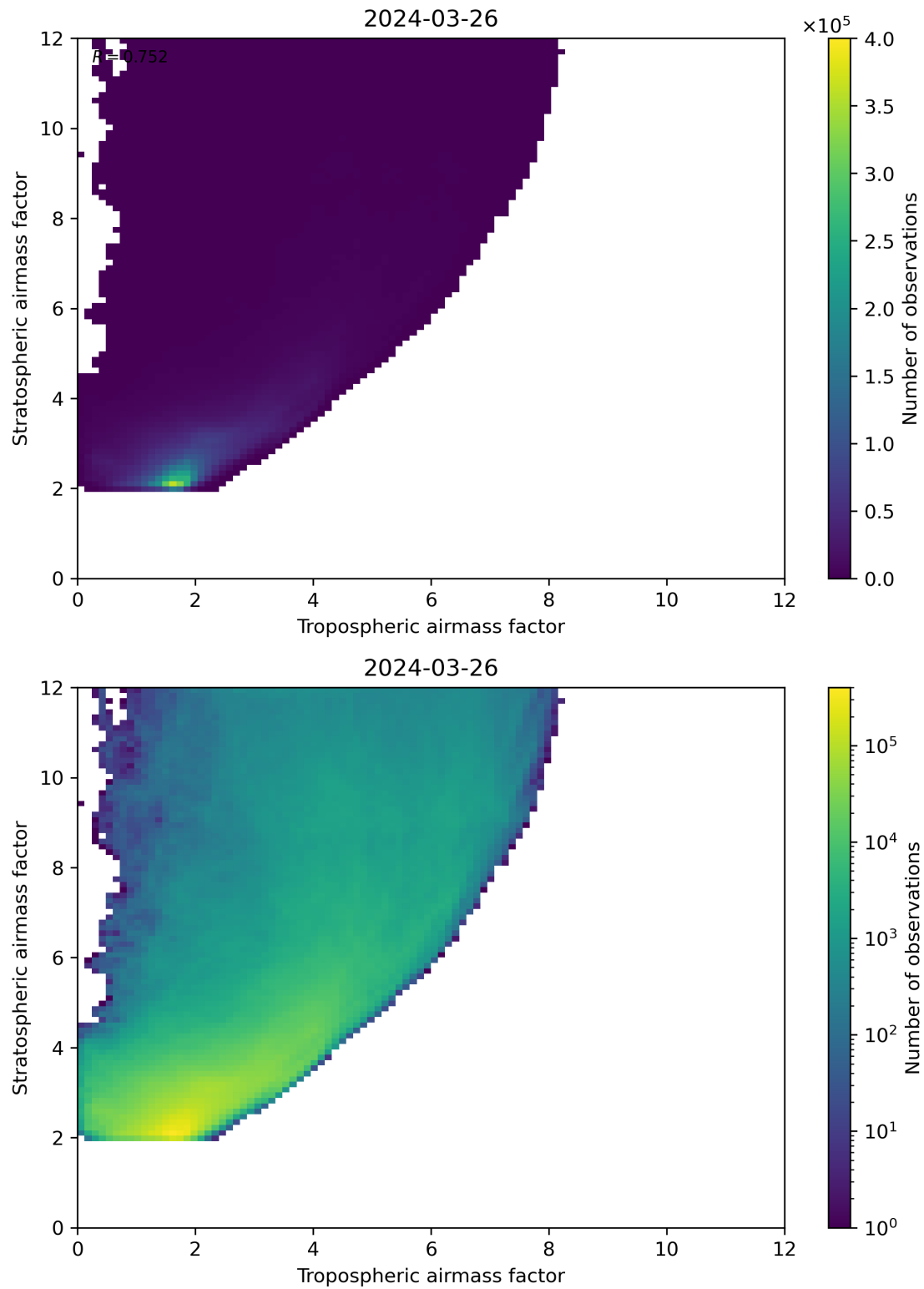
Figure 71: Scatter density plot of “Tropospheric airmass factor” against “Stratospheric airmass factor” for 2024-03-25 to 2024-03-27.
