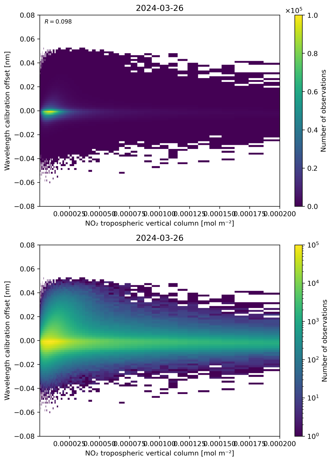
Figure 143: Scatter density plot of “NO 2 tropospheric vertical column” against “Wavelength calibration offset” for 2024-03-25 to 2024-03-27.
