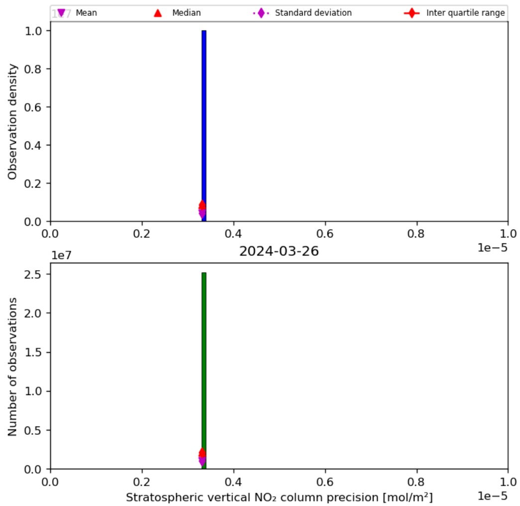
Figure 37: Histogram of “Stratospheric vertical NO 2 column precision” for 2024-03-25 to 2024-03-27
