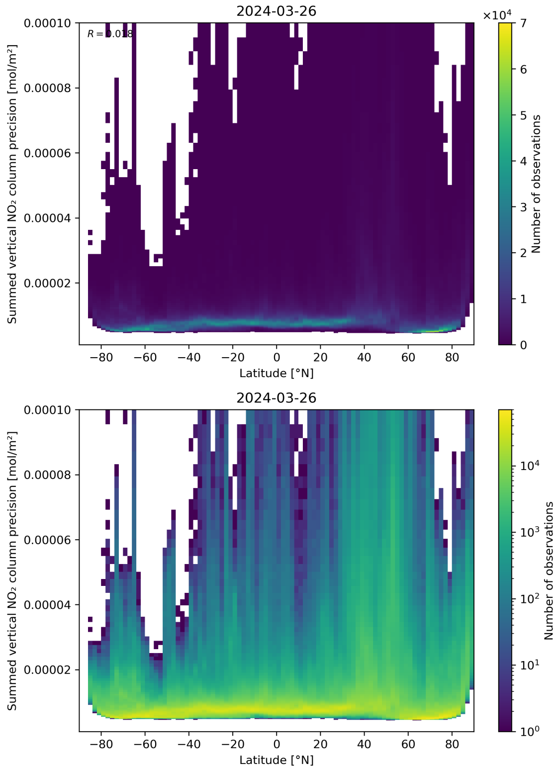
Figure 89: Scatter density plot of “Latitude” against “Summed vertical NO 2 column precision” for 2024-03-25 to 2024-03-27.
