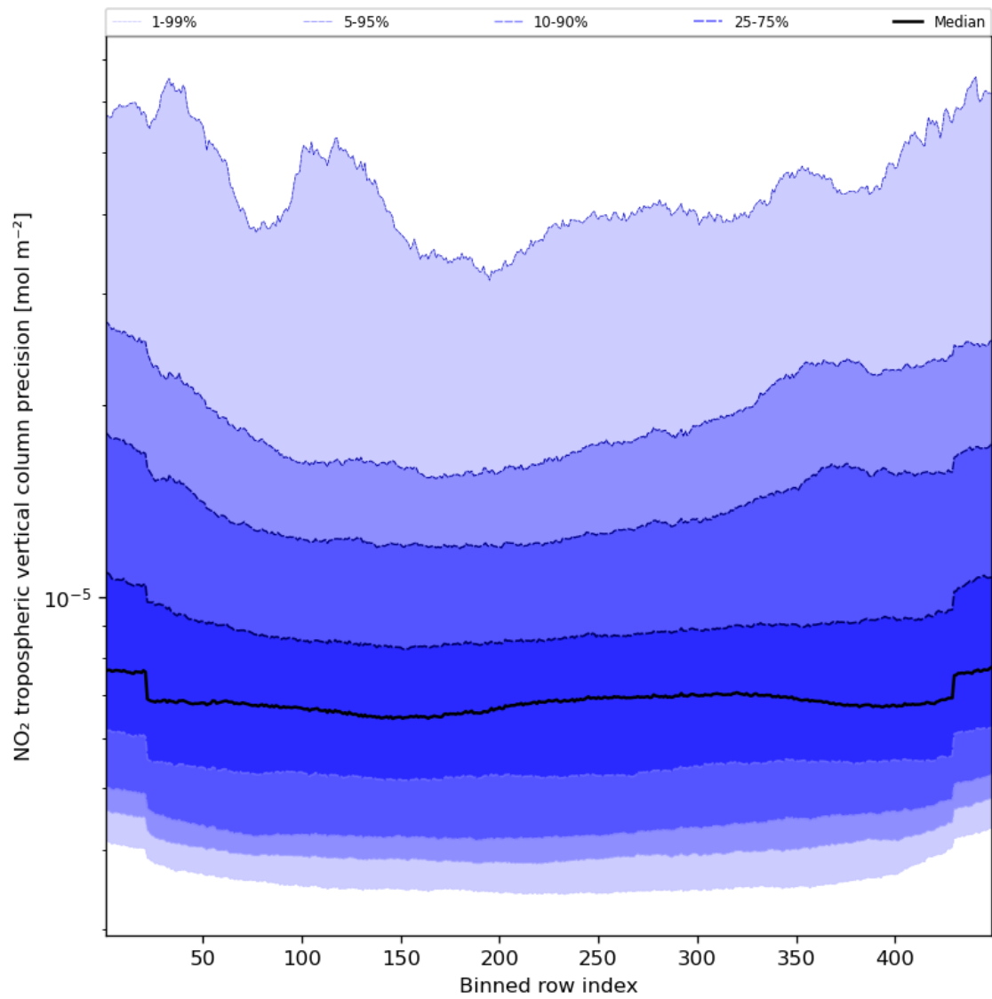
Figure 47: Along track statistics of “NO 2 tropospheric vertical column precision” for 2024-03-25 to 2024-03-27
