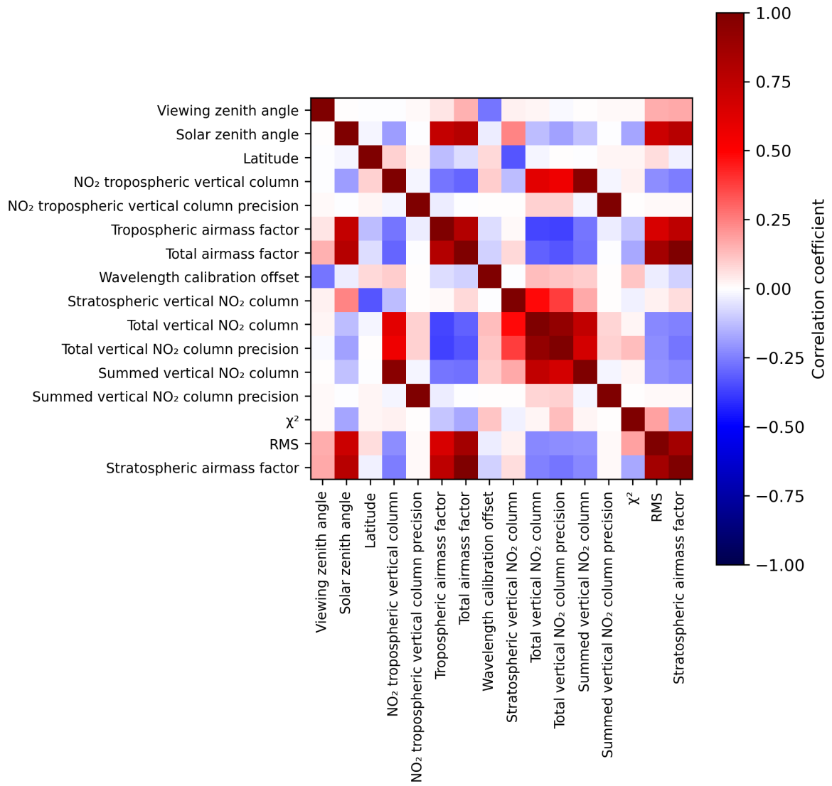
Figure 2: Map of correlation matrix for 2024-03-25 to 2024-03-27.
