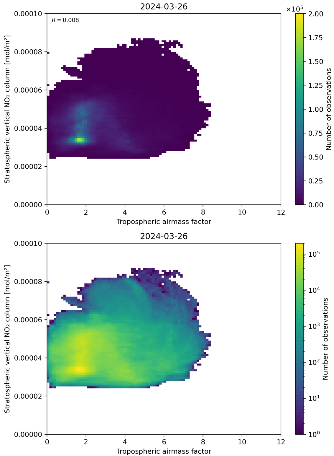
Figure 74: Scatter density plot of “Tropospheric air mass factor” against “Stratospheric vertical NO 2 column” for 2024-03-25 to 2024-03-27.
