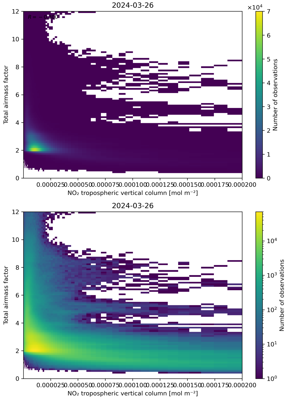
Figure 122: Scatter density plot of “NO 2 tropospheric vertical column” against “Total air mass factor” for 2024-03-25 to 2024-03-27.
