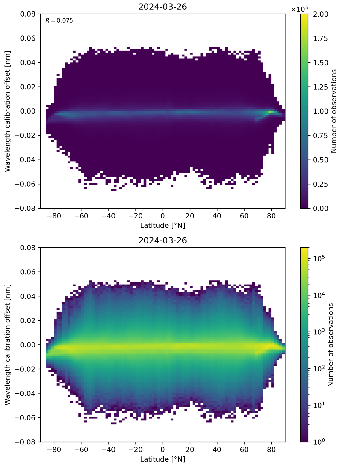
Figure 95: Scatter density plot of “Latitude” against “Wavelength calibration offset” for 2024-03-25 to 2024-03-27.
