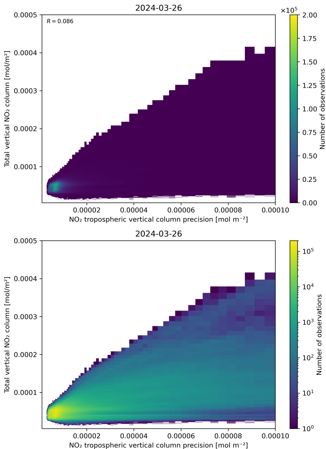
Figure 138: Scatter density plot of “NO 2 tropospheric vertical column precision” against “Total vertical NO 2 column” for 2024-03-25 to 2024-03-27.
