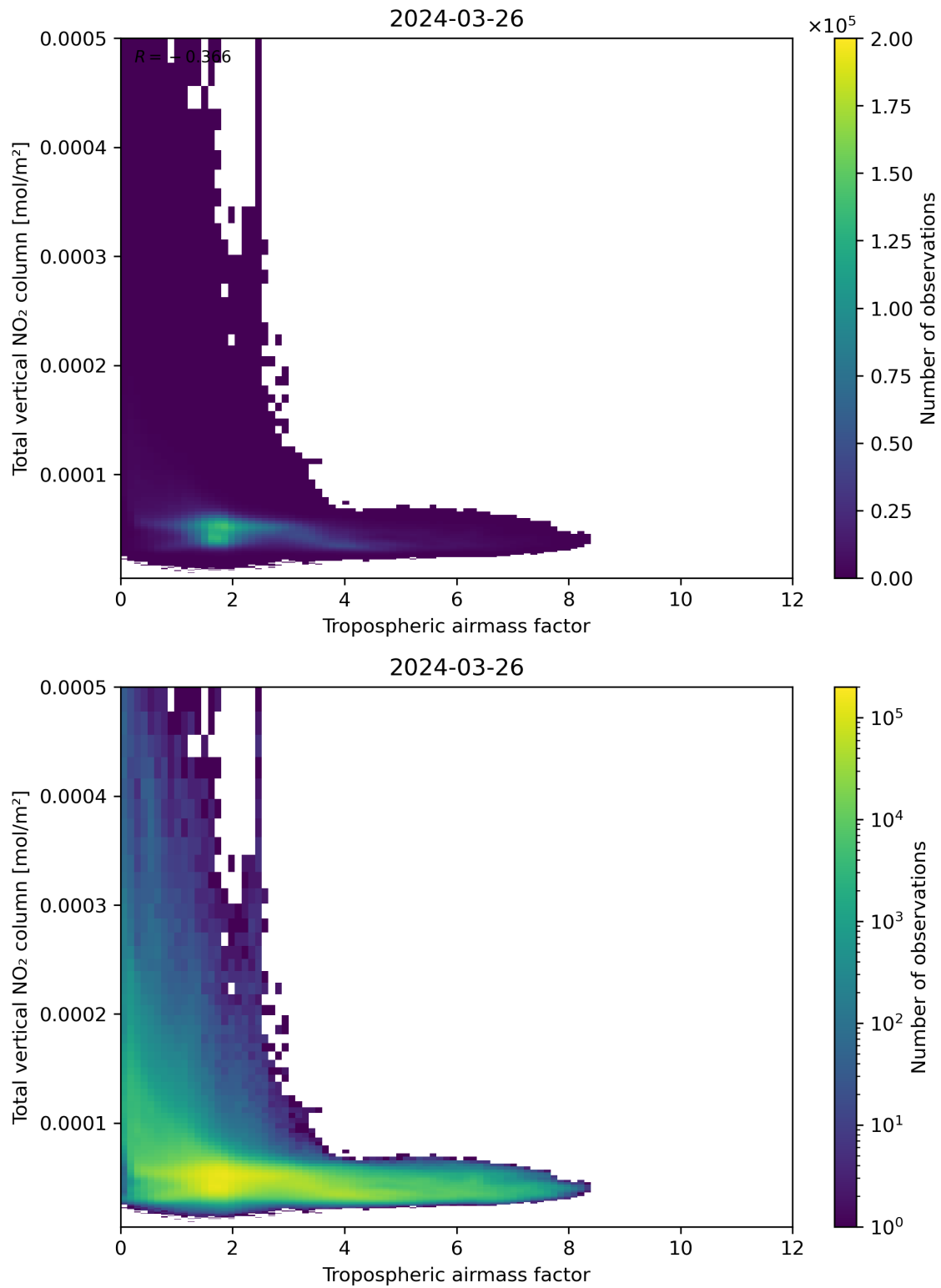
Figure 77: Scatter density plot of “Tropospheric airmass factor” against “Total vertical NO 2 column” for 2024-03-25 to 2024-03-27.
