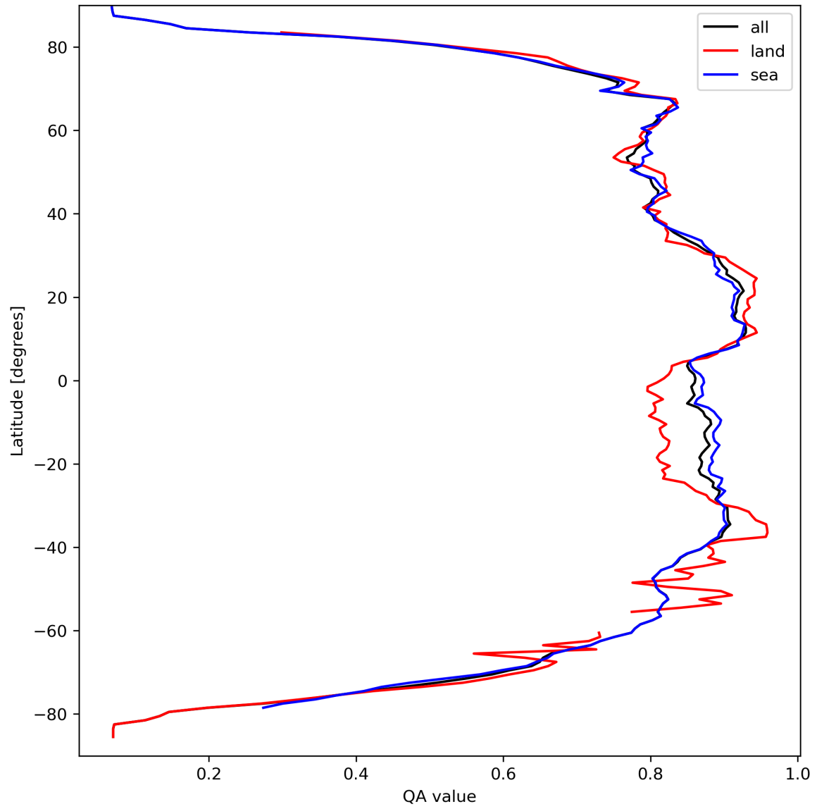
Figure 11: Zonal average of “QA value” for 2024-03-25 to 2024-03-27.
