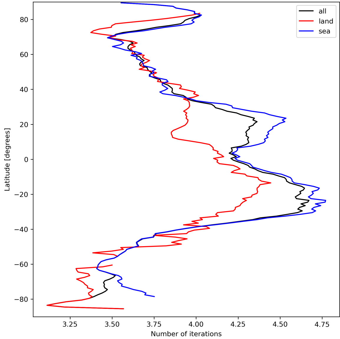
Figure 17: Zonal average of “Number of iterations” for 2024-03-25 to 2024-03-27.
