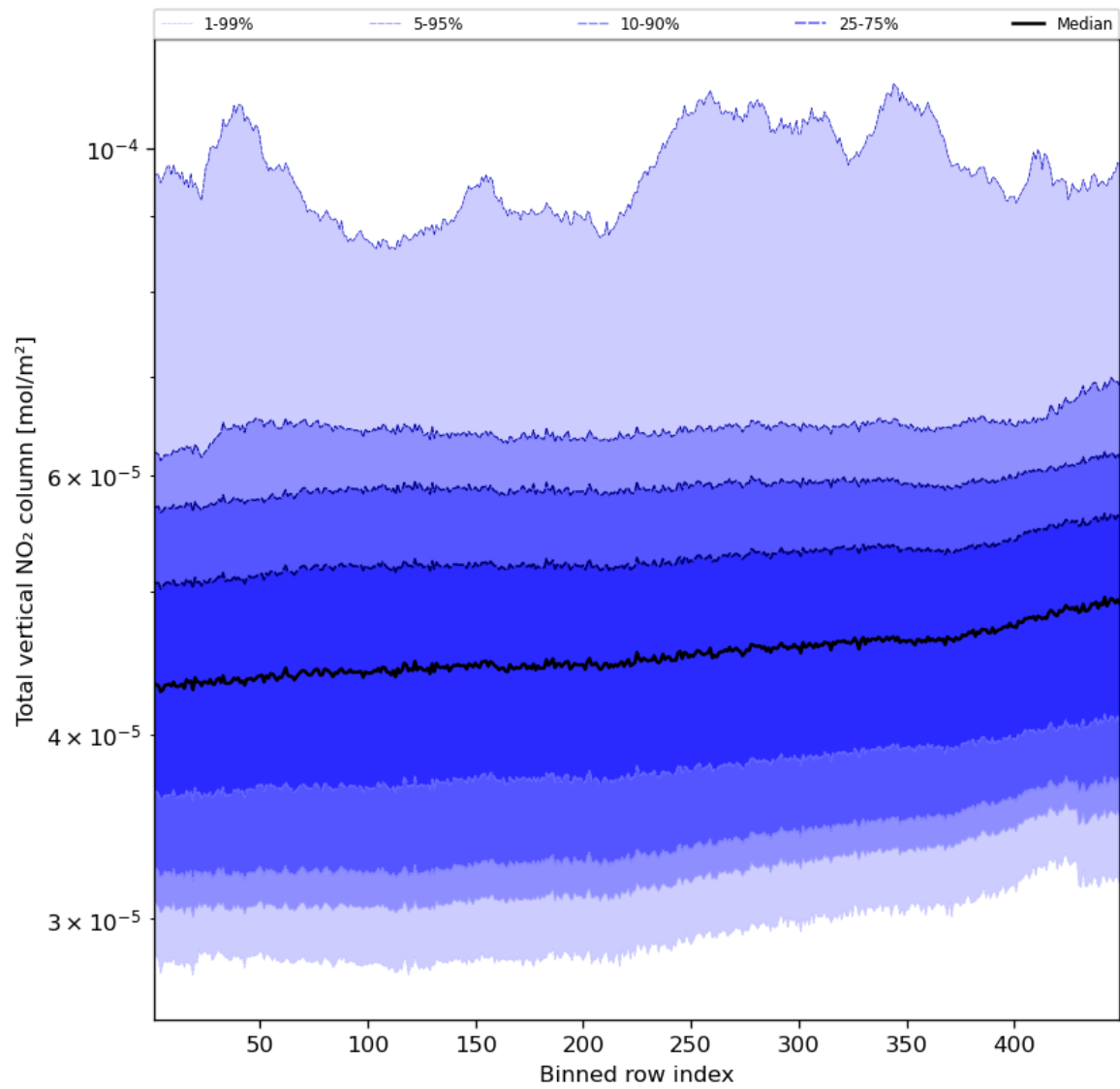
Figure 55: Along track statistics of “Total vertical NO 2 column” for 2024-03-25 to 2024-03-27
