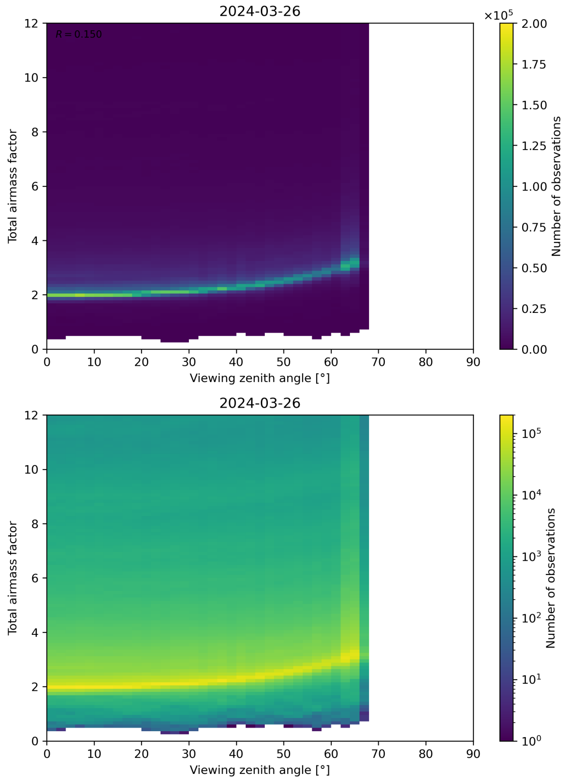
Figure 160: Scatter density plot of “Viewing zenith angle” against “Total airmass factor” for 2024-03-25 to 2024-03-27.
