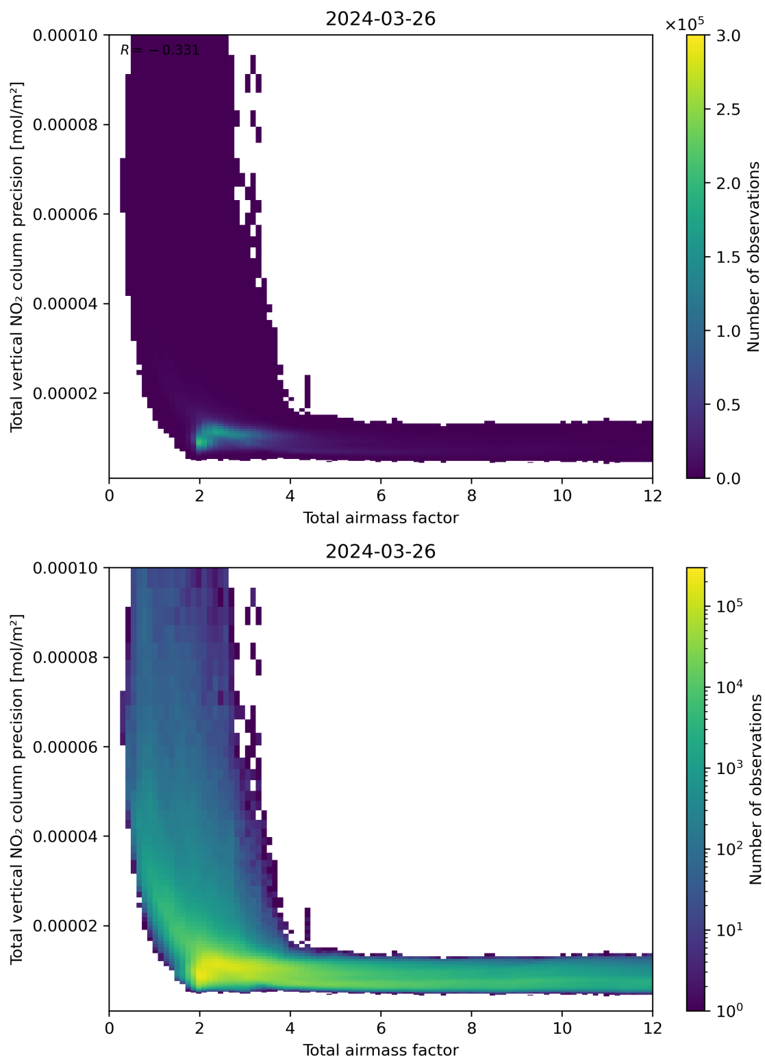
Figure 68: Scatter density plot of “Total airmass factor” against “Total vertical NO 2 column precision” for 2024-03-25 to 2024-03-27.
