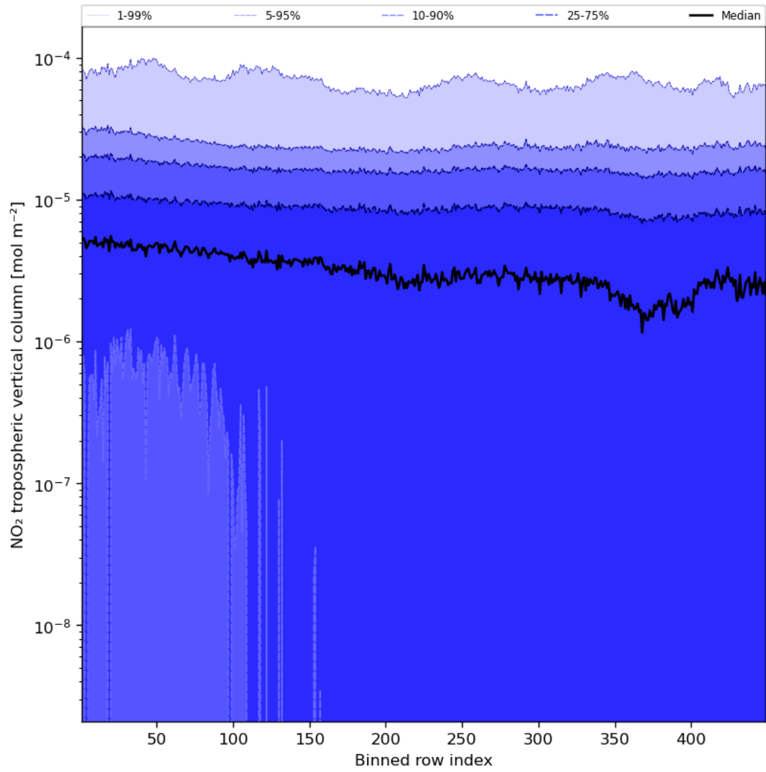
Figure 46: Along track statistics of “NO 2 tropospheric vertical column” for 2024-03-25 to 2024-03-27
