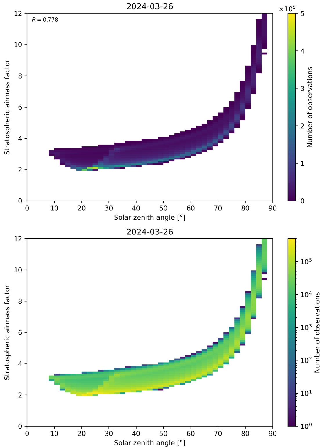
Figure 145: Scatter density plot of “Solar zenith angle” against “Stratospheric airmass factor” for 2024-03-25 to 2024-03-27.
