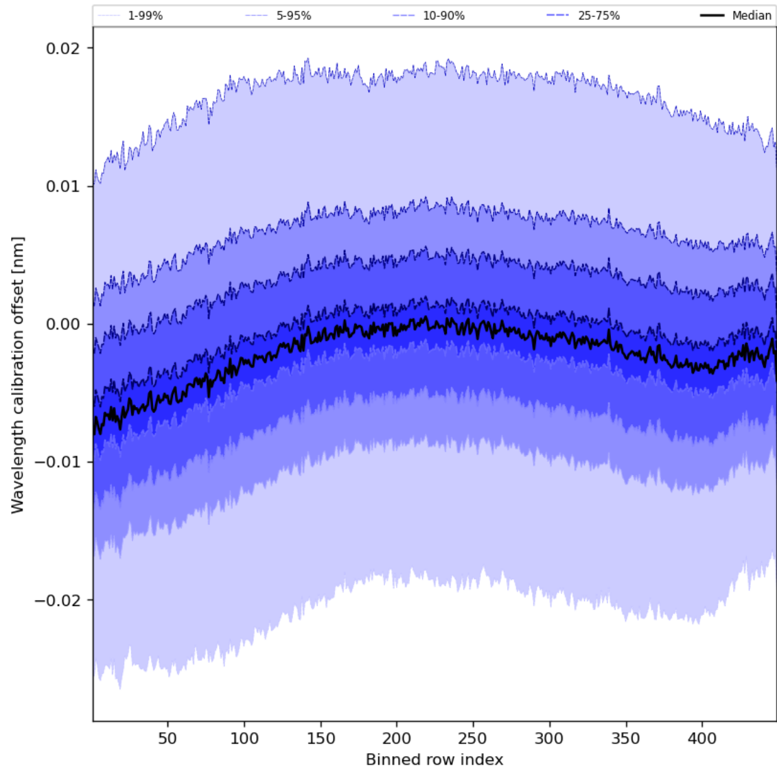
Figure 52: Along track statistics of “Wavelength calibration offset” for 2024-03-25 to 2024-03-27
