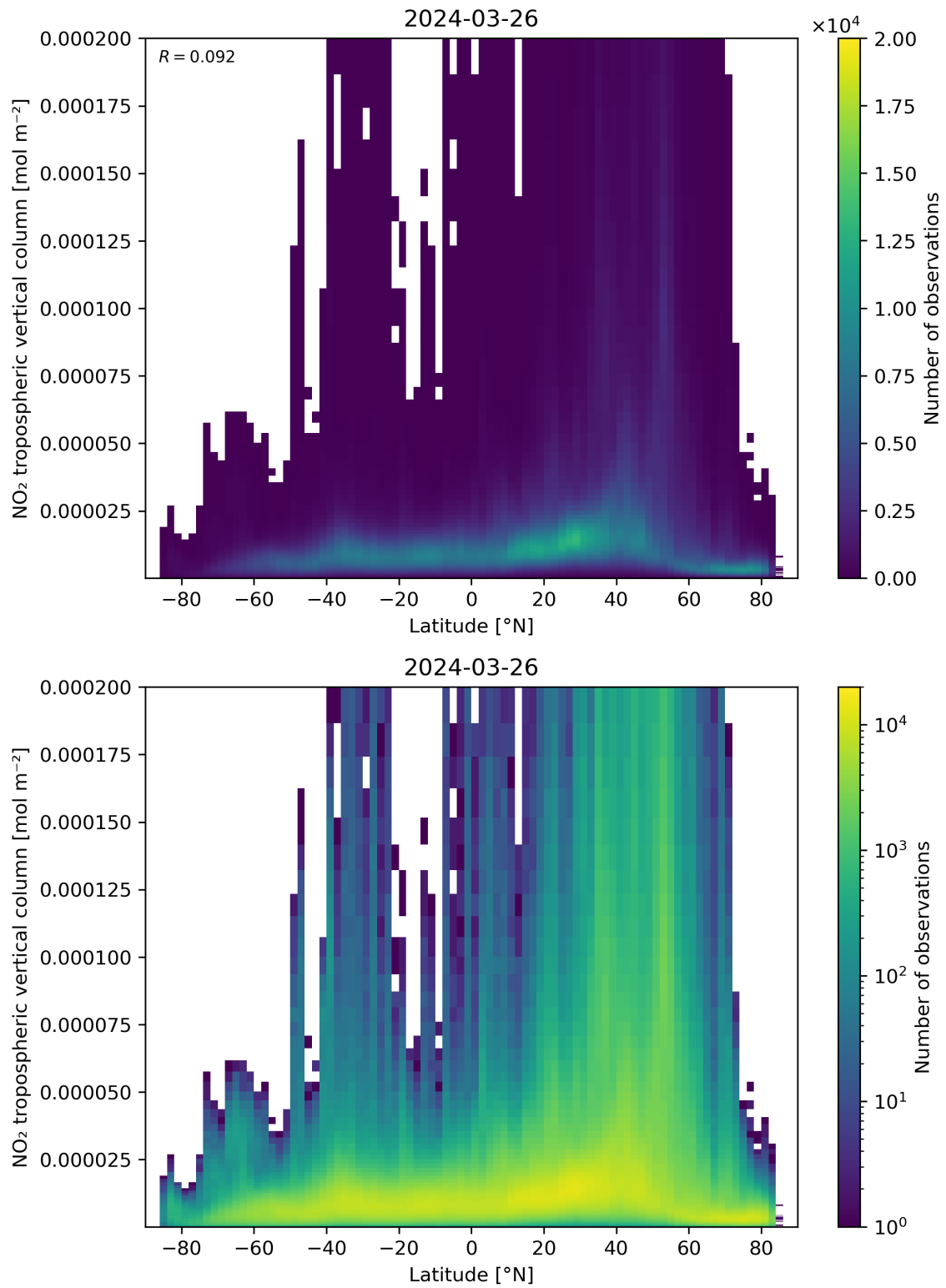
Figure 92: Scatter density plot of “Latitude” against “NO 2 tropospheric vertical column” for 2024-03-25 to 2024-03-27.
