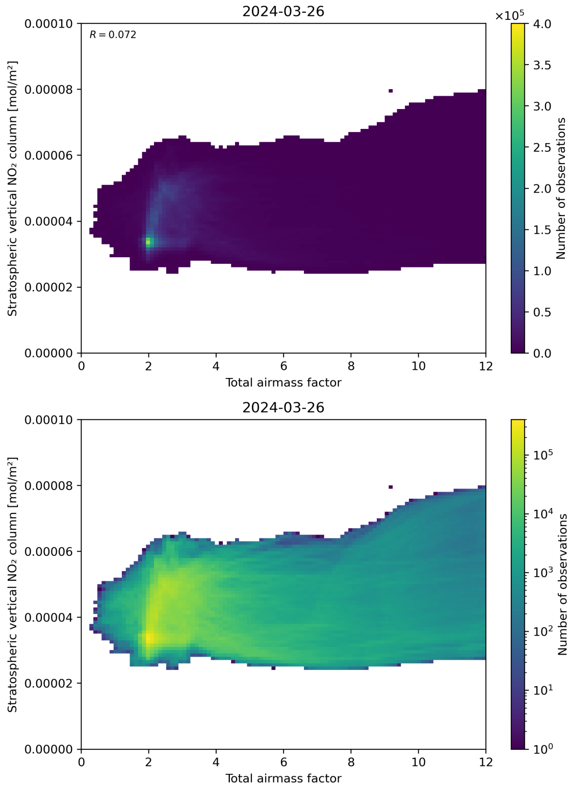
Figure 64: Scatter density plot of “Total airmass factor” against “Stratospheric vertical \text{NO}_2 column” for 2024-03-25 to 2024-03-27.
