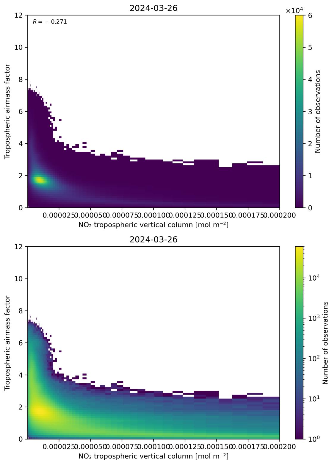
Figure 123: Scatter density plot of “NO 2 tropospheric vertical column” against “Tropospheric airmass factor” for 2024-03-25 to 2024-03-27.
