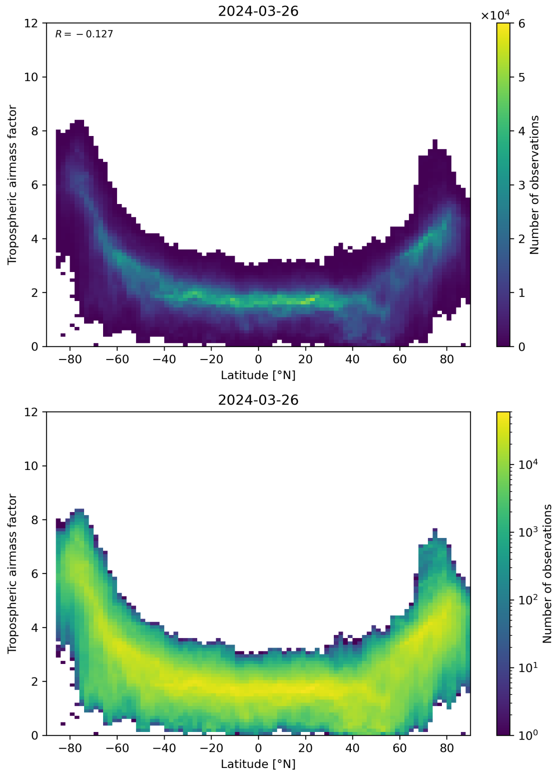
Figure 85: Scatter density plot of “Latitude” against “Tropospheric airmass factor” for 2024-03-25 to 2024-03-27.
