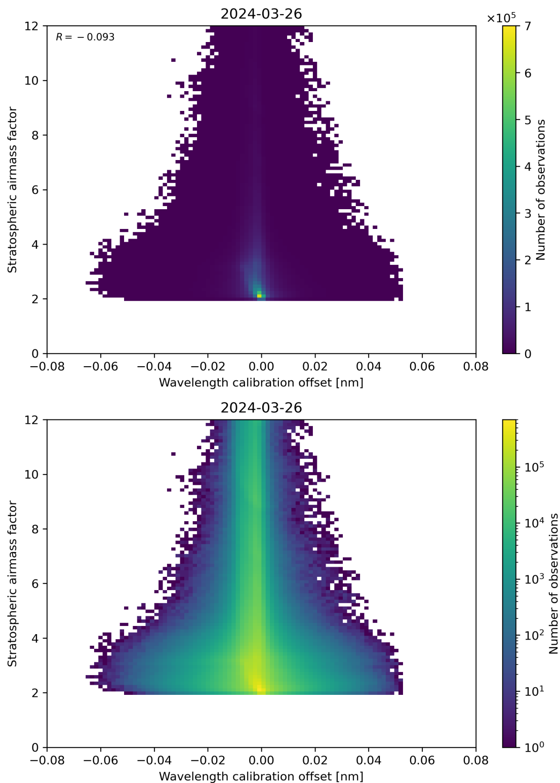
Figure 174: Scatter density plot of “Wavelength calibration offset” against “Stratospheric airmass factor” for 2024-03-25 to 2024-03-27.
