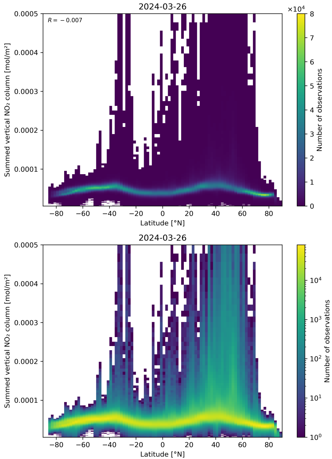
Figure 88: Scatter density plot of “Latitude” against “Summed vertical NO 2 column” for 2024-03-25 to 2024-03-27.
