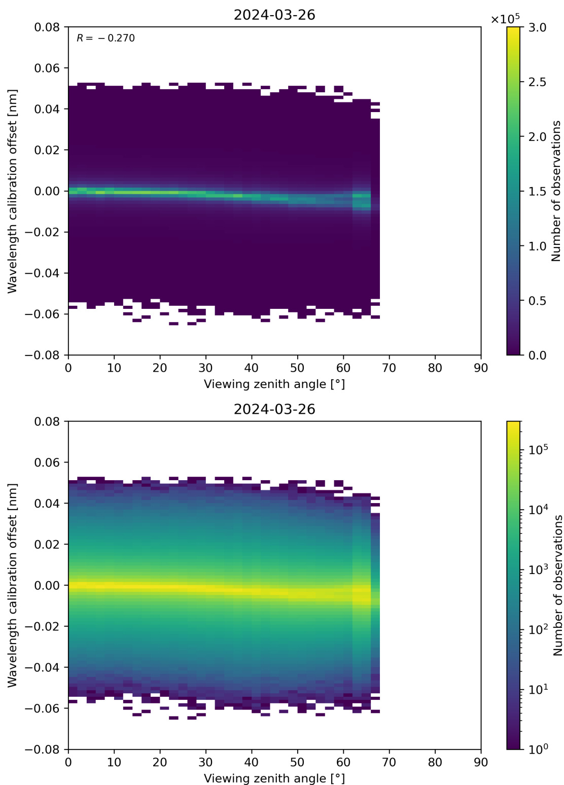
Figure 173: Scatter density plot of “Viewing zenith angle” against “Wavelength calibration offset” for 2024-03-25 to 2024-03-27.
