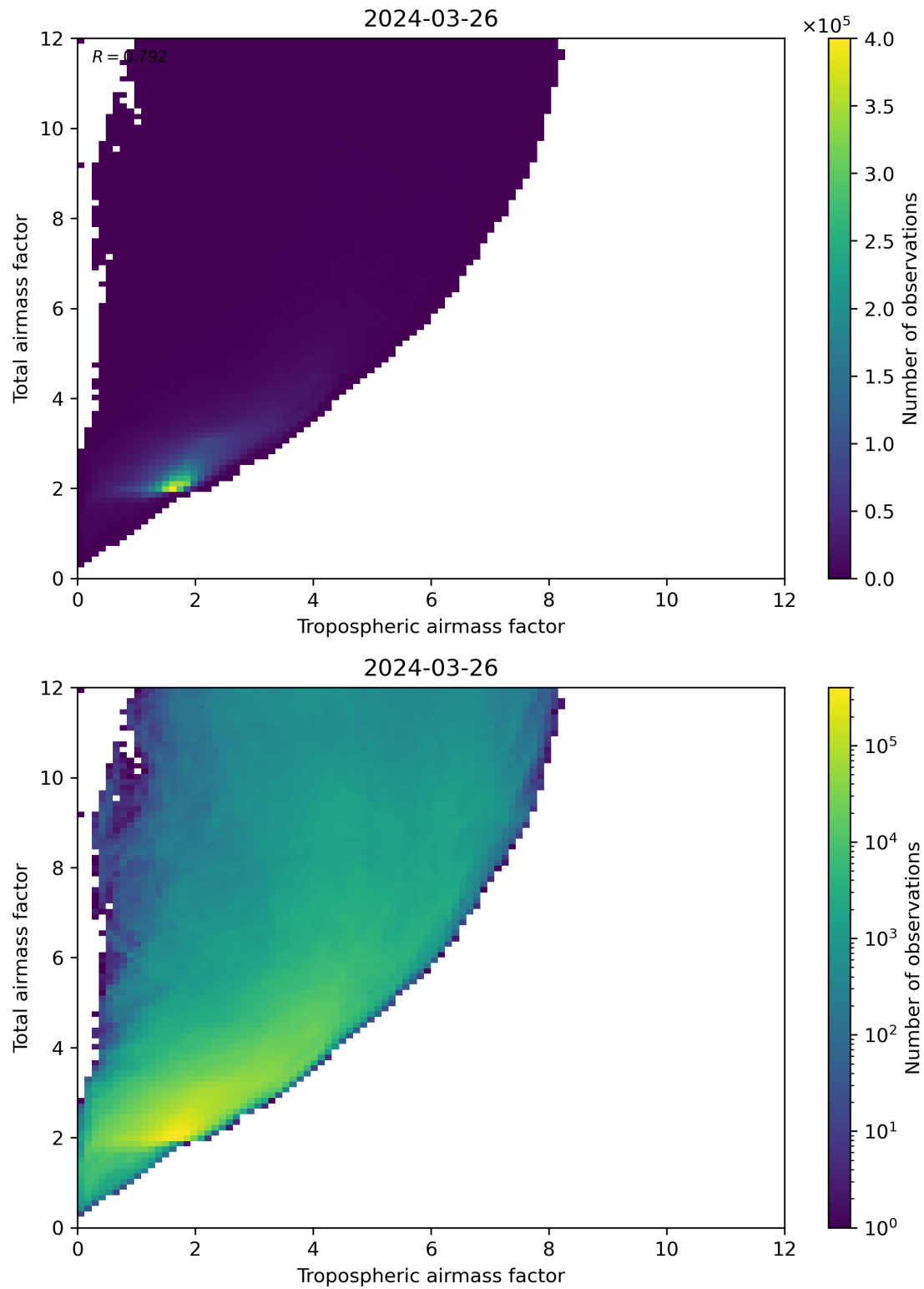
Figure 72: Scatter density plot of “Tropospheric airmass factor” against “Total airmass factor” for 2024-03-25 to 2024-03-27.
