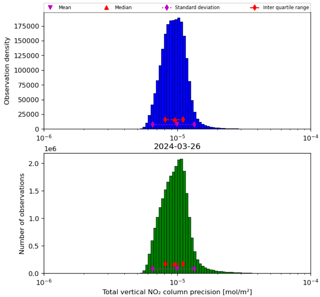
Figure 39: Histogram of “Total vertical NO 2 column precision” for 2024-03-25 to 2024-03-27
