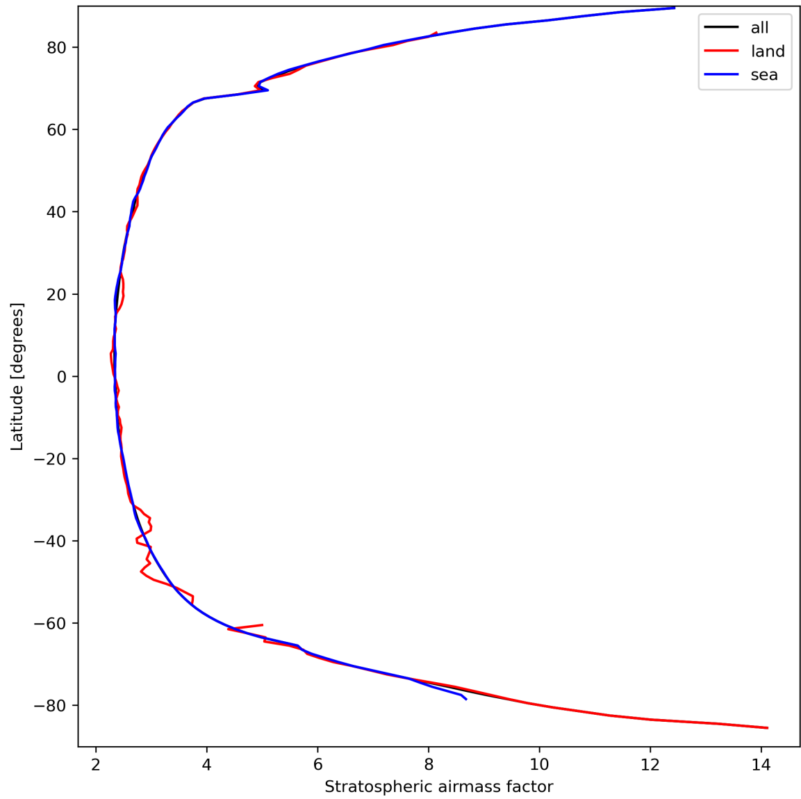
Figure 27: Zonal average of “Stratospheric airmass factor” for 2024-03-25 to 2024-03-27.
