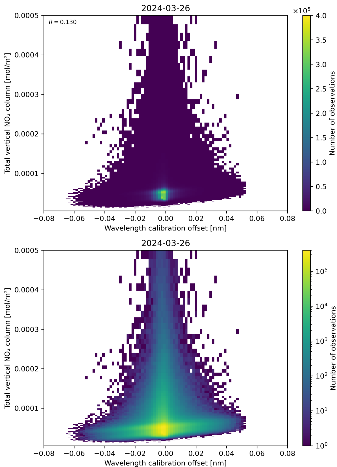
Figure 179: Scatter density plot of “Wavelength calibration offset” against “Total vertical NO 2 column” for 2024-03-25 to 2024-03-27.
