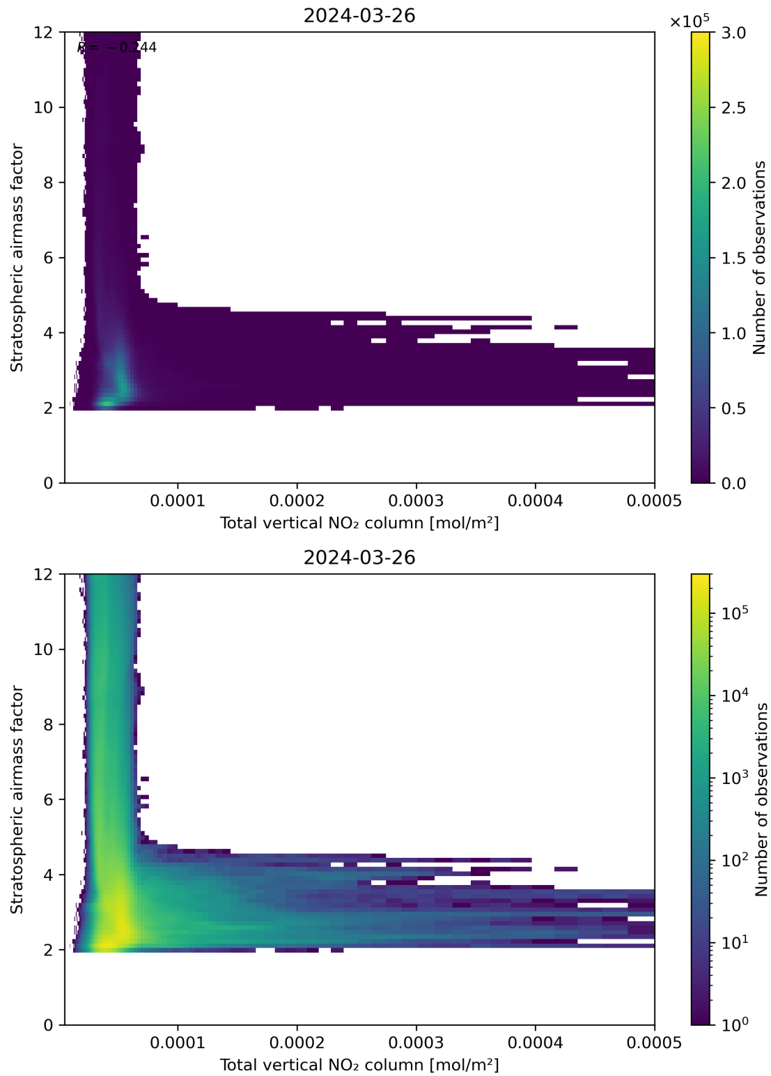
Figure 110: Scatter density plot of “Total vertical NO 2 column” against “Stratospheric airmass factor” for 2024-03-25 to 2024-03-27.
