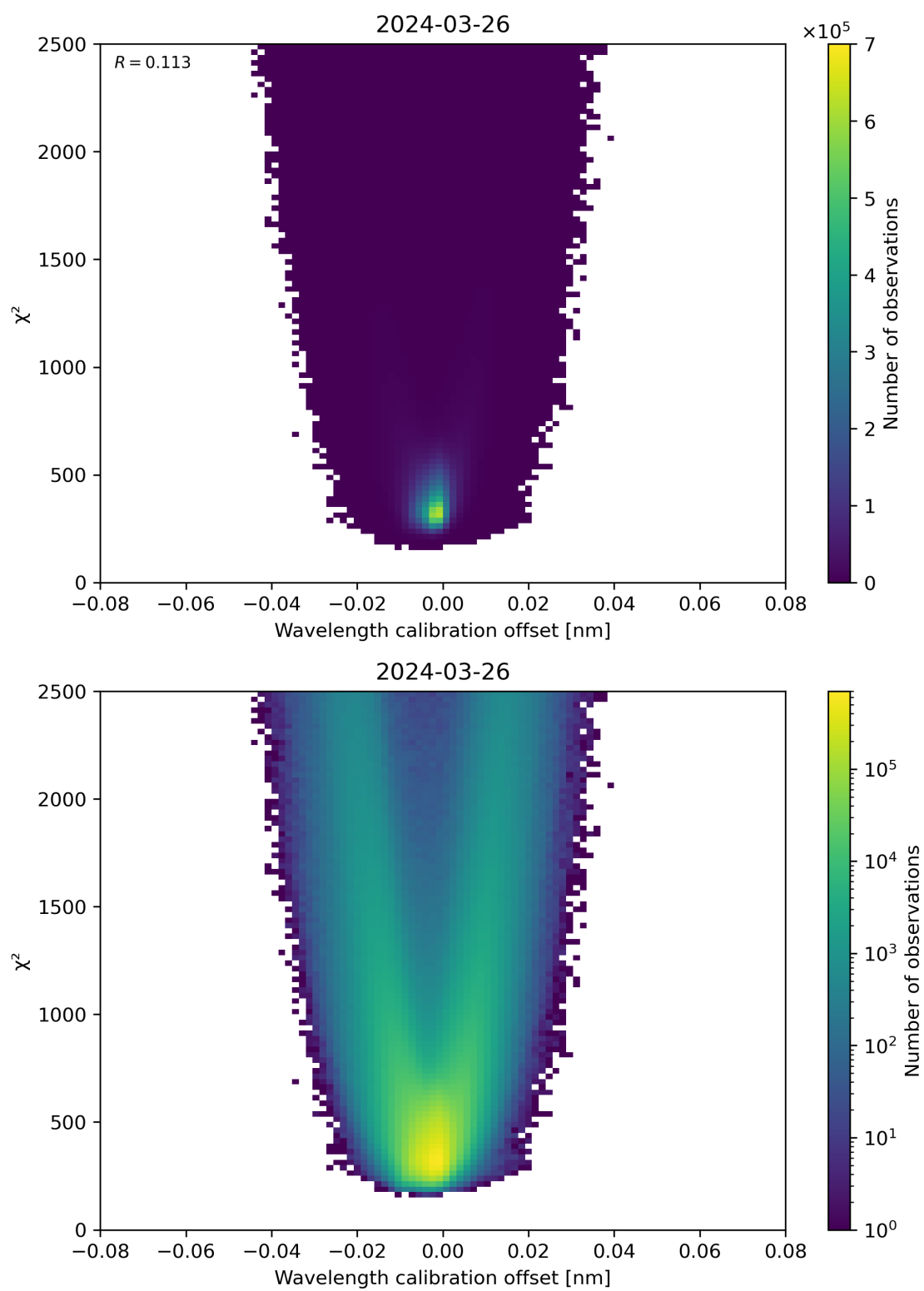
Figure 175: Scatter density plot of “Wavelength calibration offset” against “ \chi^2 ” for 2024-03-25 to 2024-03-27.
