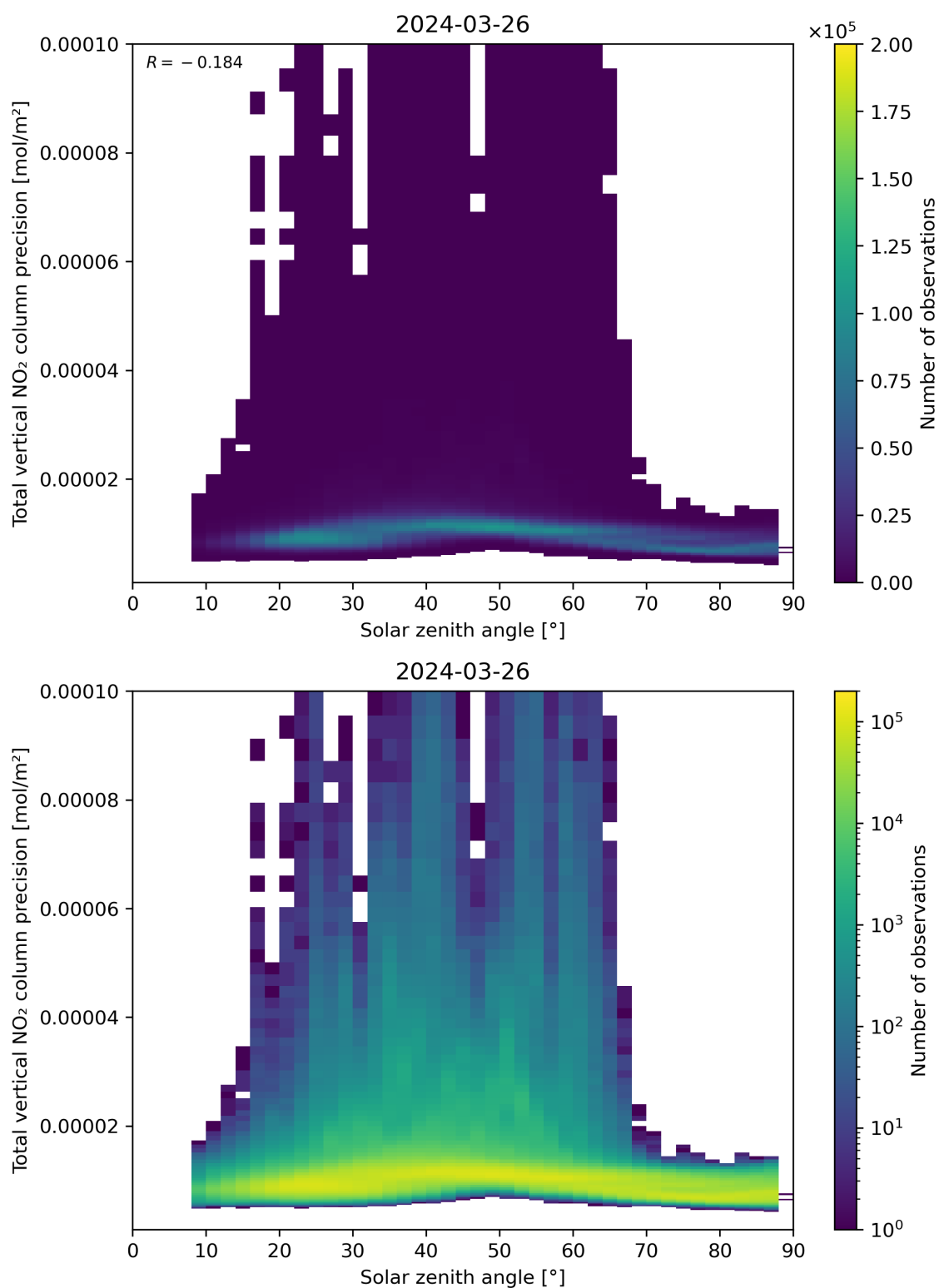
Figure 154: Scatter density plot of “Solar zenith angle” against “Total vertical NO 2 column precision” for 2024-03-25 to 2024-03-27.
