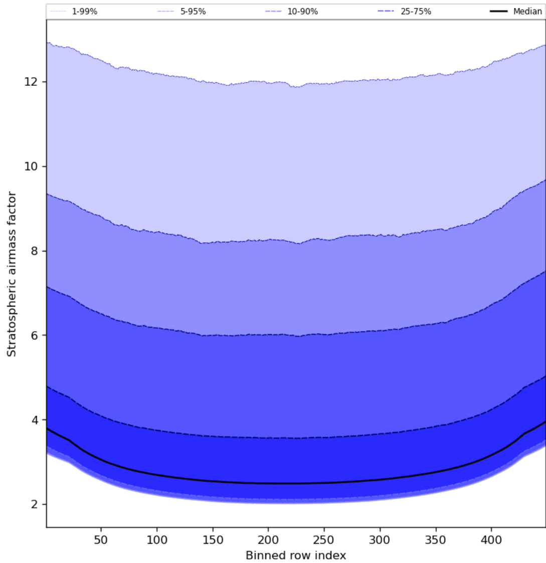
Figure 61: Along track statistics of “Stratospheric airmass factor” for 2024-03-25 to 2024-03-27
