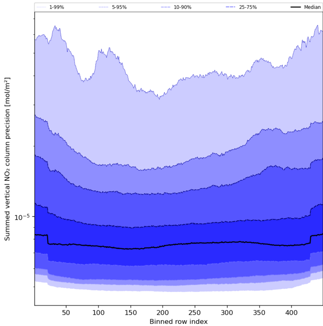
Figure 58: Along track statistics of “Summed vertical NO 2 column precision” for 2024-03-25 to 2024-03-27
