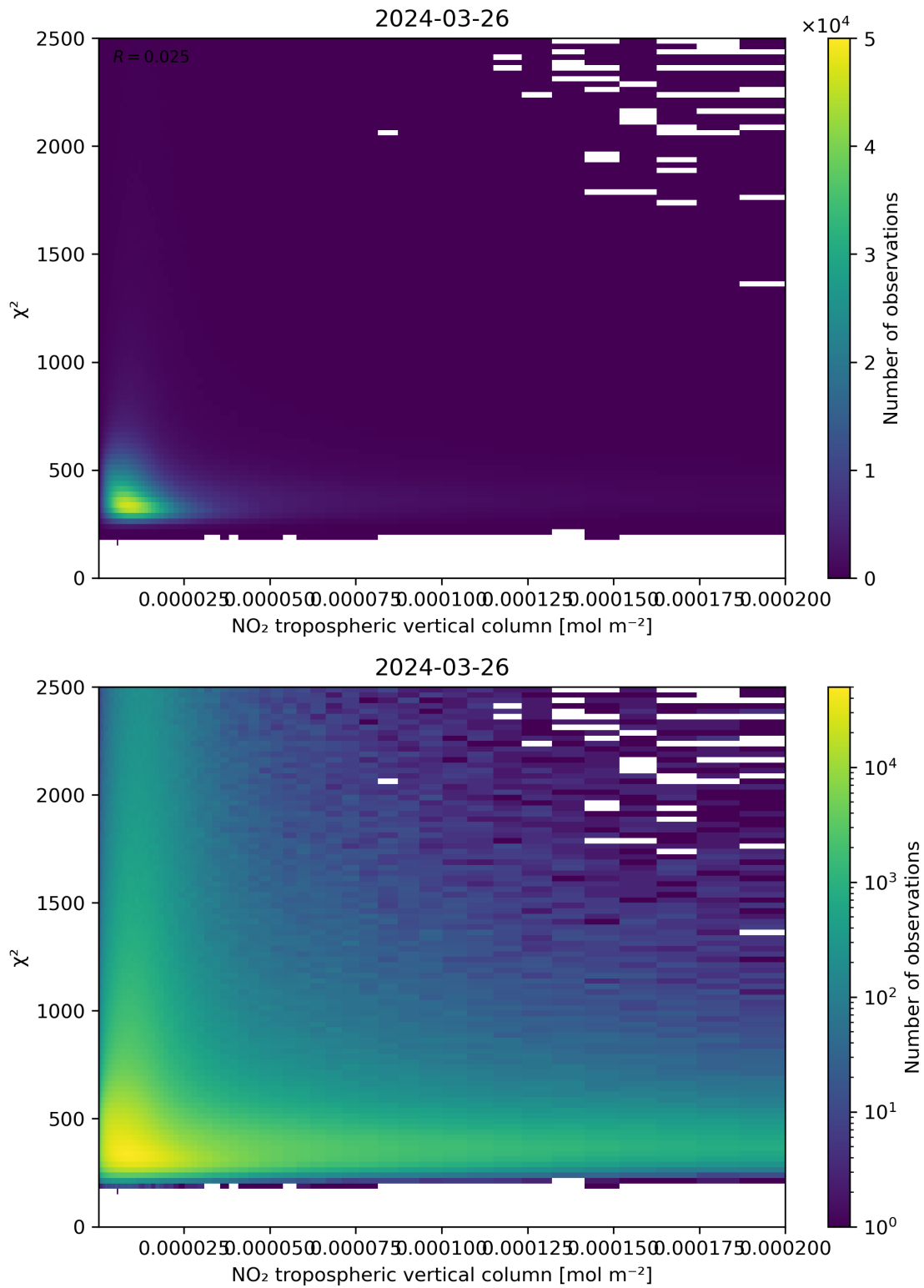
Figure 124: Scatter density plot of “NO 2 tropospheric vertical column” against “ \chi^2 ” for 2024-03-25 to 2024-03-27.
