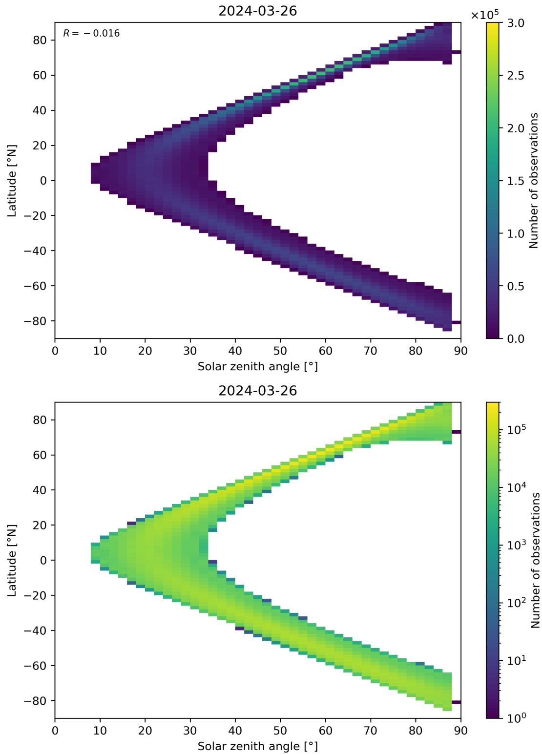
Figure 149: Scatter density plot of “Solar zenith angle” against “Latitude” for 2024-03-25 to 2024-03-27.
