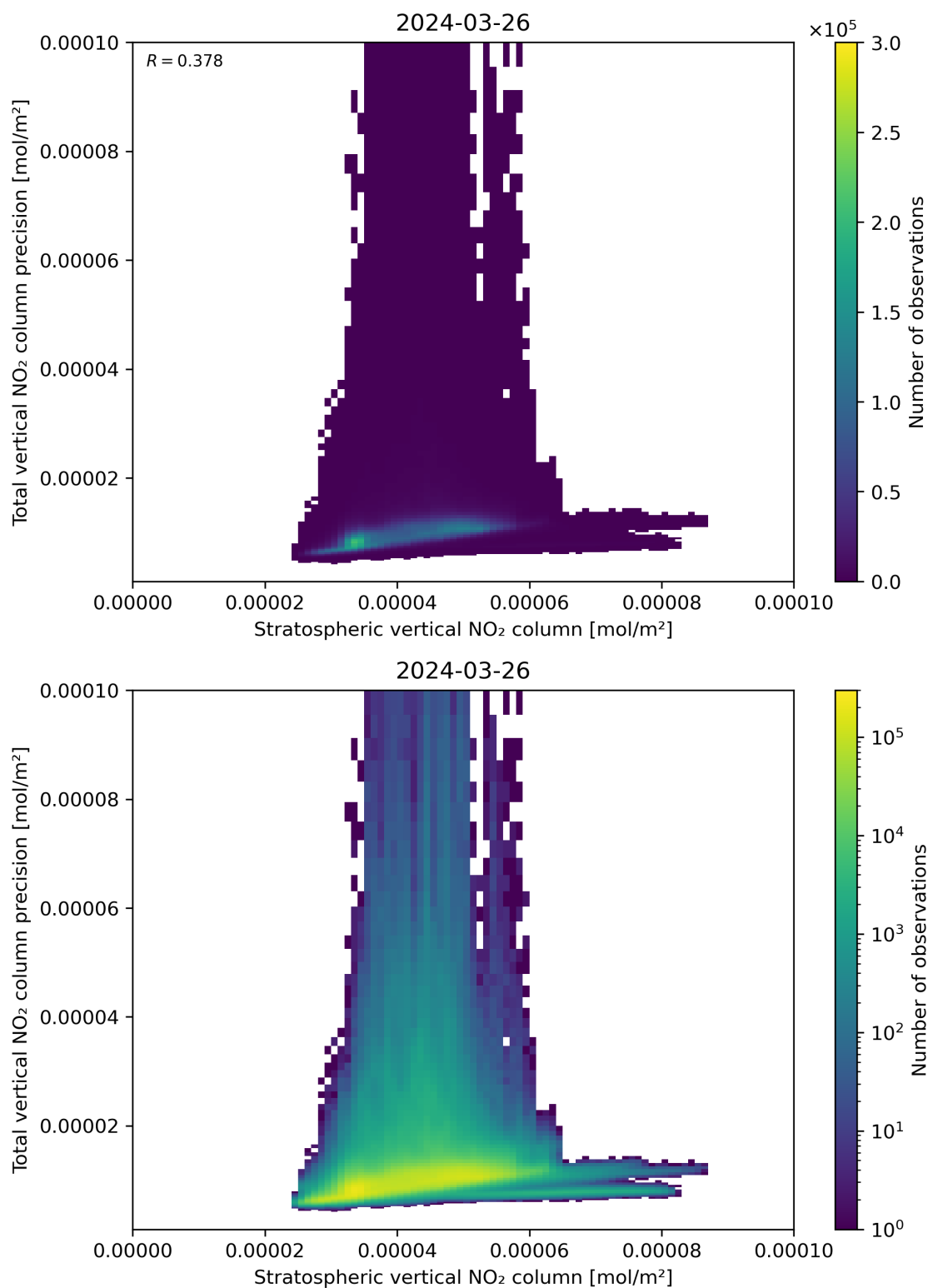
Figure 101: Scatter density plot of “Stratospheric vertical NO 2 column” against “Total vertical NO 2 column precision” for 2024-03-25 to 2024-03-27.
