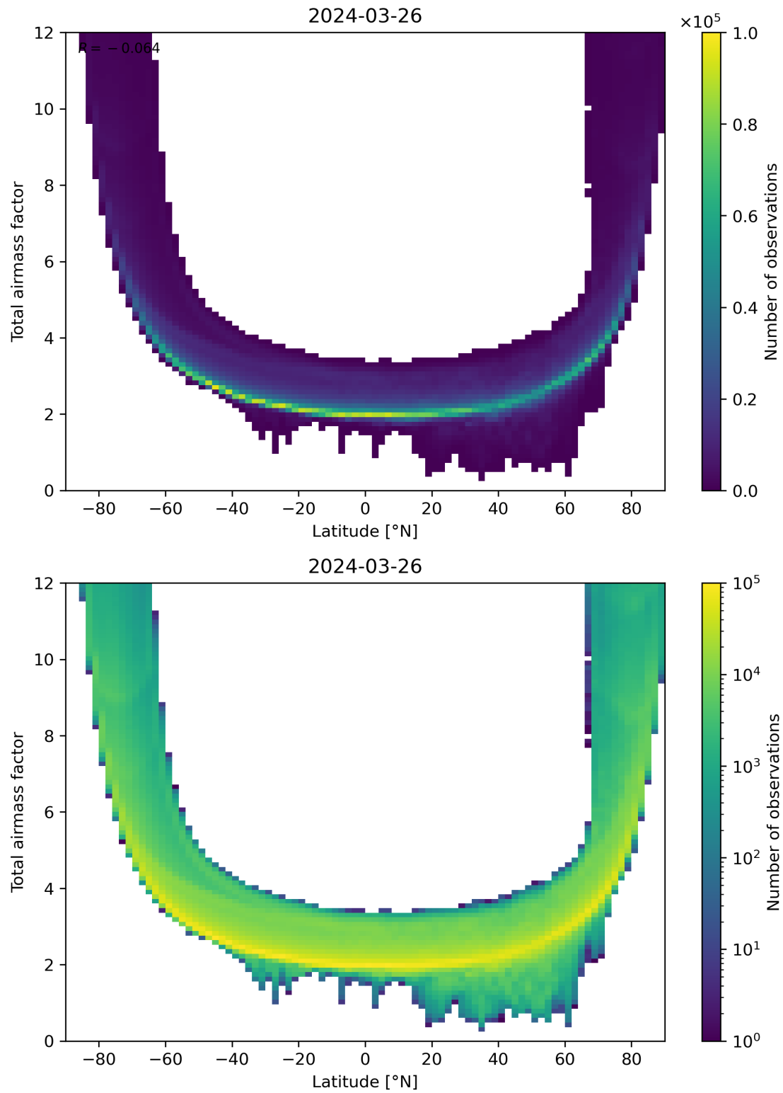
Figure 84: Scatter density plot of “Latitude” against “Total airmass factor” for 2024-03-25 to 2024-03-27.
