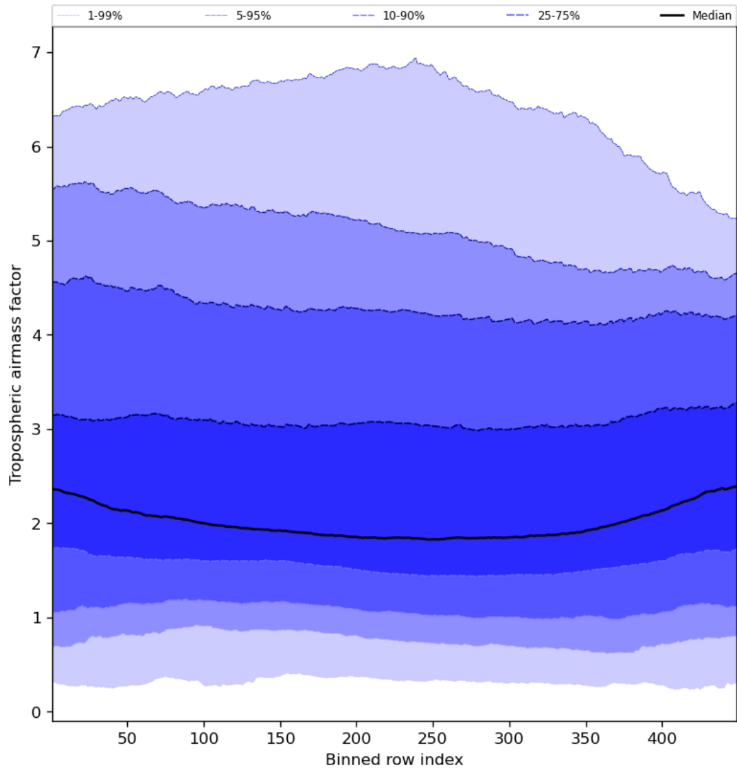
Figure 48: Along track statistics of “Tropospheric air mass factor” for 2024-03-25 to 2024-03-27
