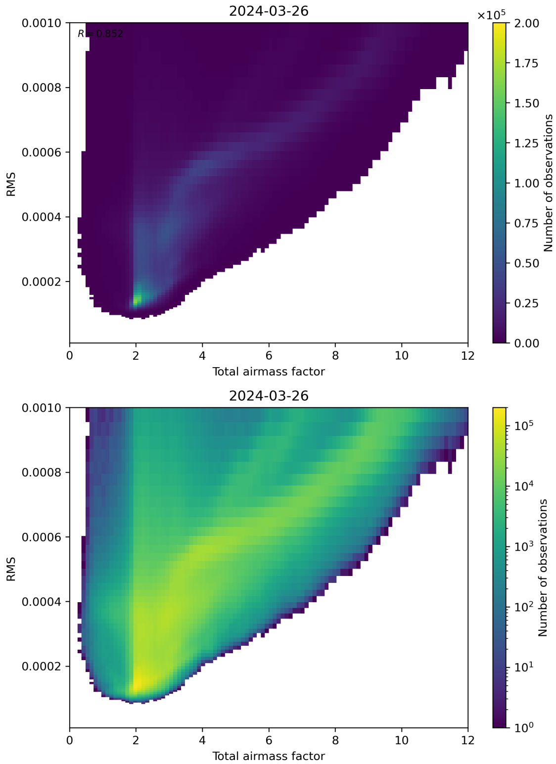
Figure 69: Scatter density plot of “Total airmass factor” against “RMS” for 2024-03-25 to 2024-03-27.
