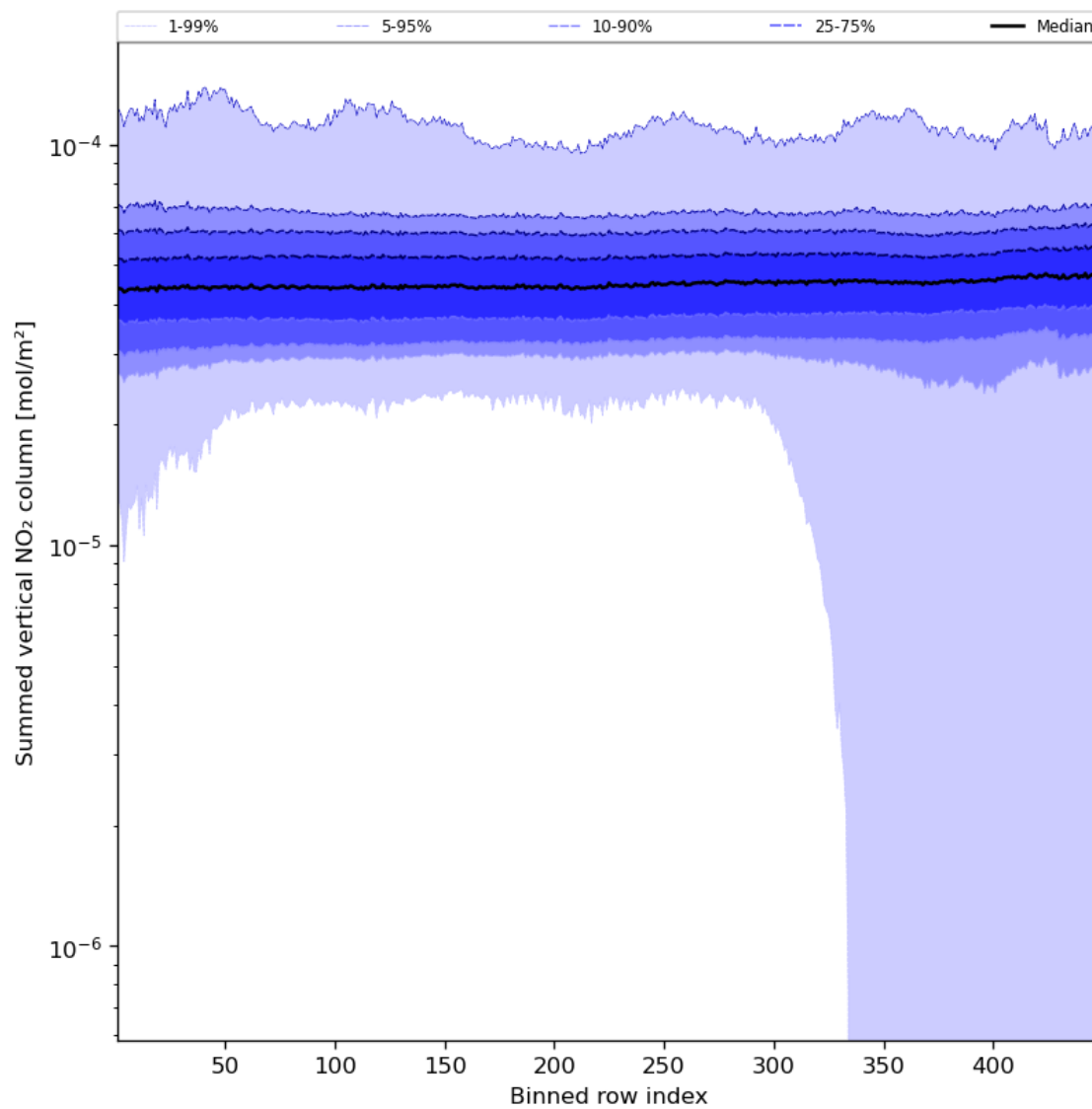
Figure 57: Along track statistics of “Summed vertical NO 2 column” for 2024-03-25 to 2024-03-27
