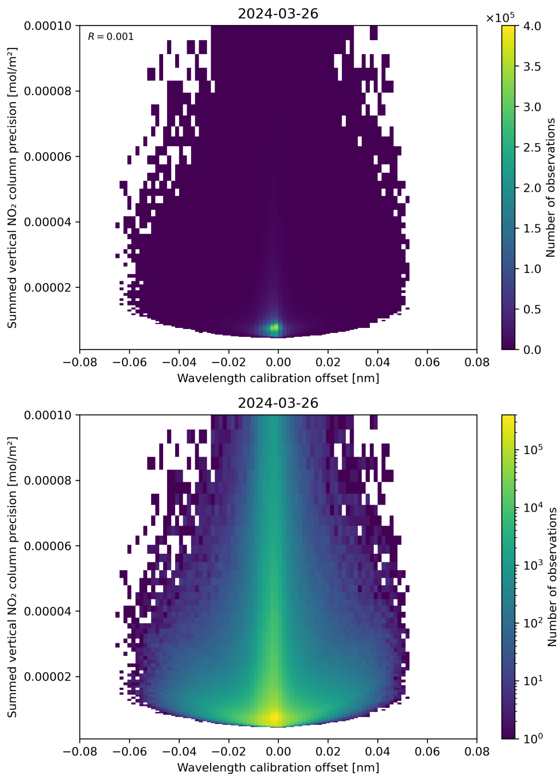
Figure 178: Scatter density plot of “Wavelength calibration offset” against “Summed vertical NO 2 column precision” for 2024-03-25 to 2024-03-27.
