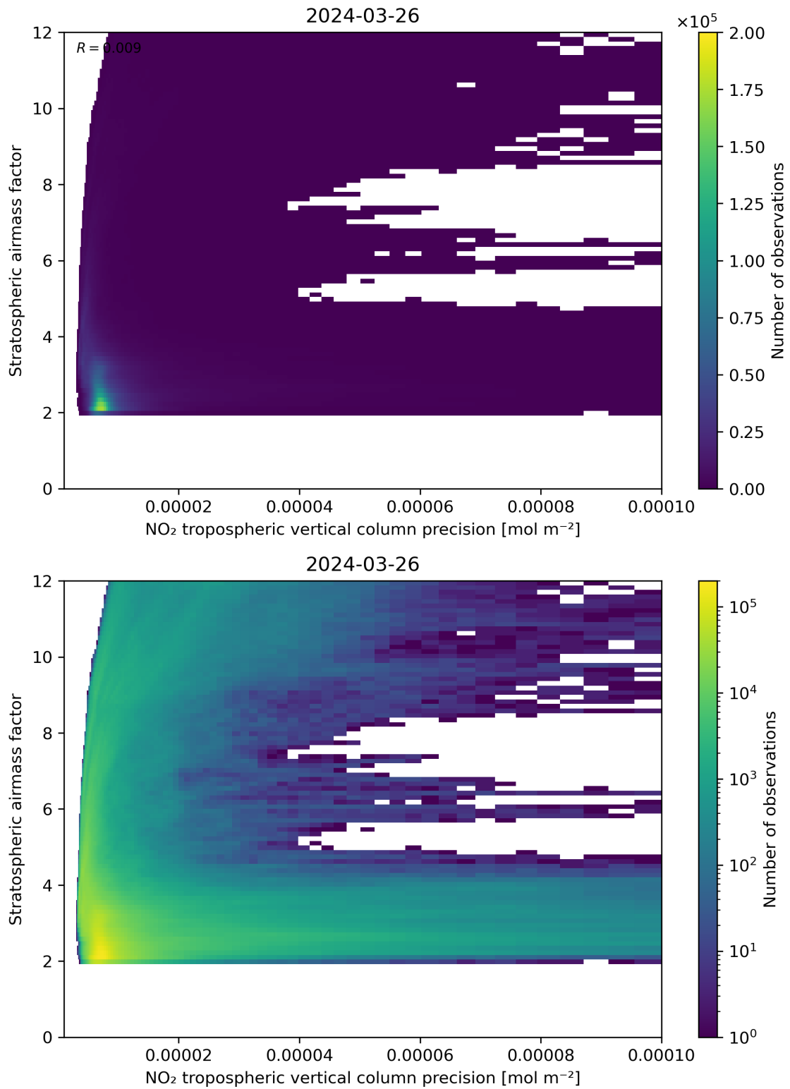
Figure 131: Scatter density plot of “NO 2 tropospheric vertical column precision” against “Stratospheric airmass factor” for 2024-03-25 to 2024-03-27.
