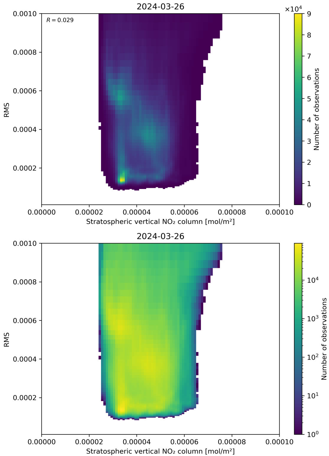
Figure 102: Scatter density plot of “Stratospheric vertical NO 2 column” against “RMS” for 2024-03-25 to 2024-03-27.
