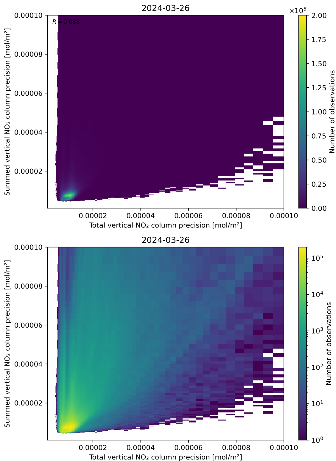
Figure 118: Scatter density plot of “Total vertical NO 2 column precision” against “Summed vertical NO 2 column precision” for 2024-03-25 to 2024-03-27.
