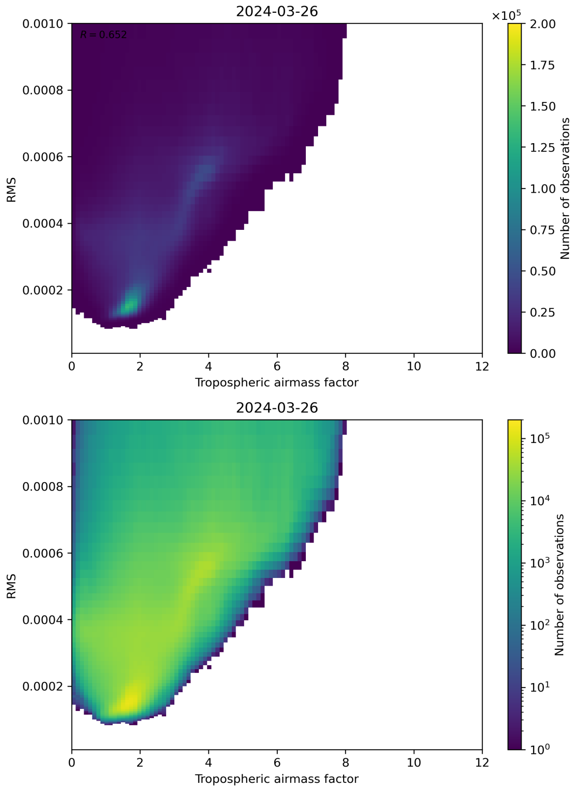
Figure 79: Scatter density plot of “Tropospheric airmass factor” against “RMS” for 2024-03-25 to 2024-03-27.
