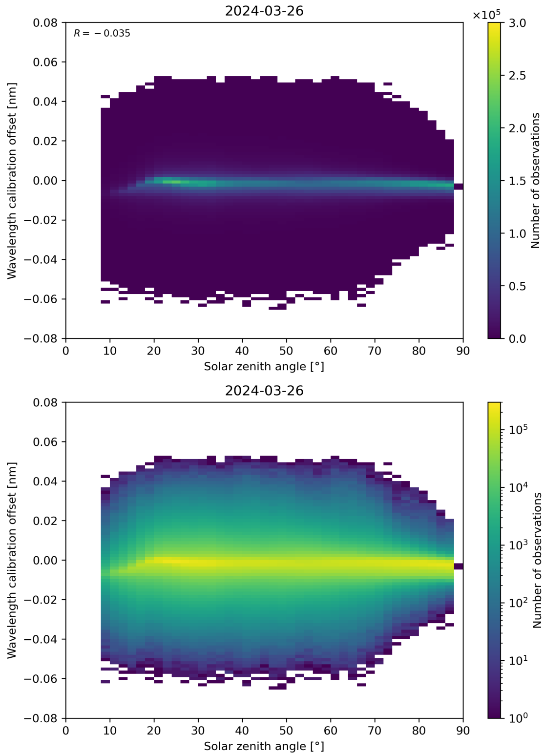
Figure 158: Scatter density plot of “Solar zenith angle” against “Wavelength calibration offset” for 2024-03-25 to 2024-03-27.
