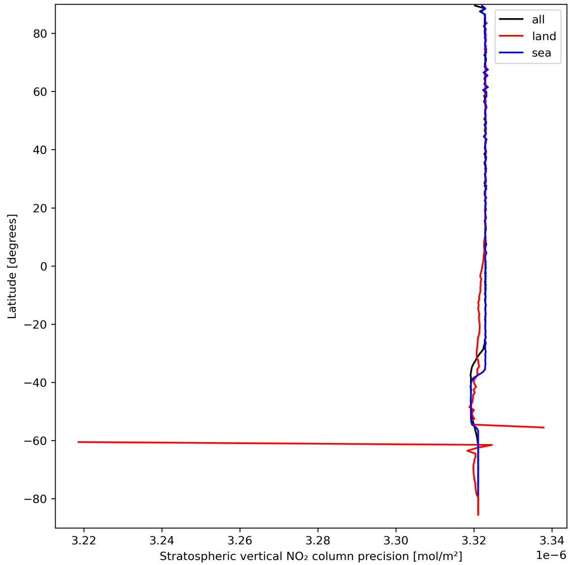
Figure 20: Zonal average of “Stratospheric vertical NO 2 column precision” for 2024-03-25 to 2024-03-27.
