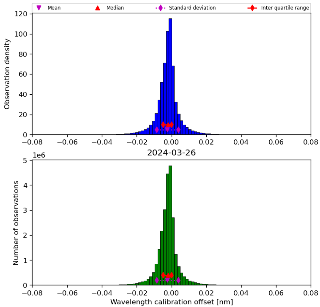
Figure 35: Histogram of “Wavelength calibration offset” for 2024-03-25 to 2024-03-27
