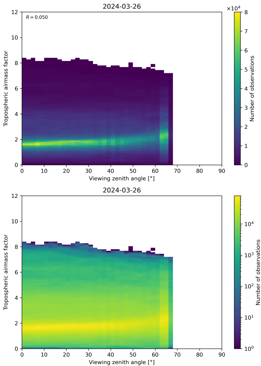
Figure 161: Scatter density plot of “Viewing zenith angle” against “Tropospheric airmass factor” for 2024-03-25 to 2024-03-27.
