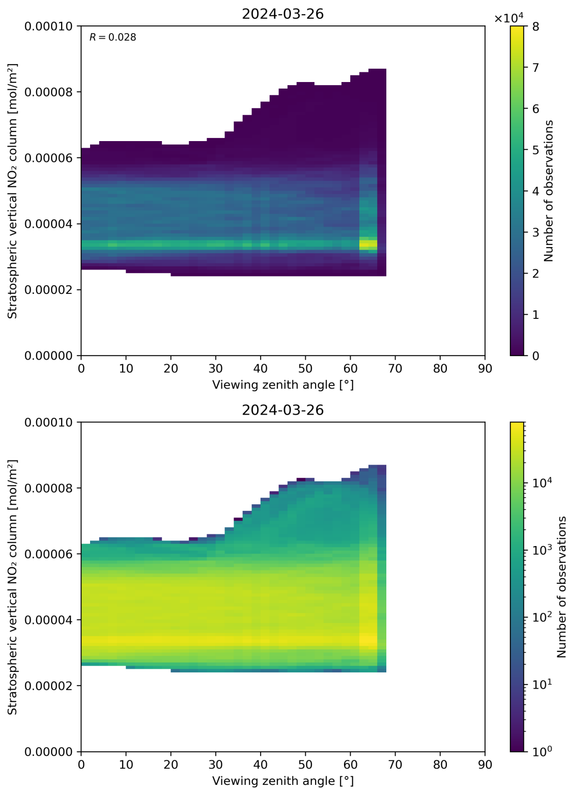
Figure 164: Scatter density plot of “Viewing zenith angle” against “Stratospheric vertical NO 2 column” for 2024-03-25 to 2024-03-27.
