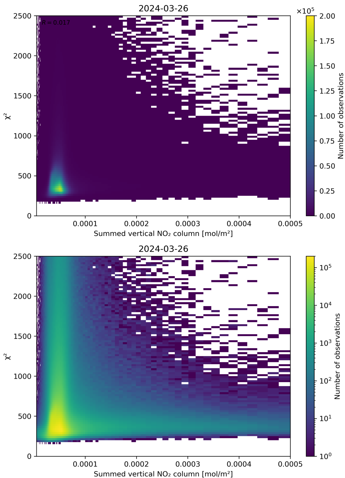
Figure 104: Scatter density plot of “Summed vertical NO 2 column” against “ \chi^2 ” for 2024-03-25 to 2024-03-27.
