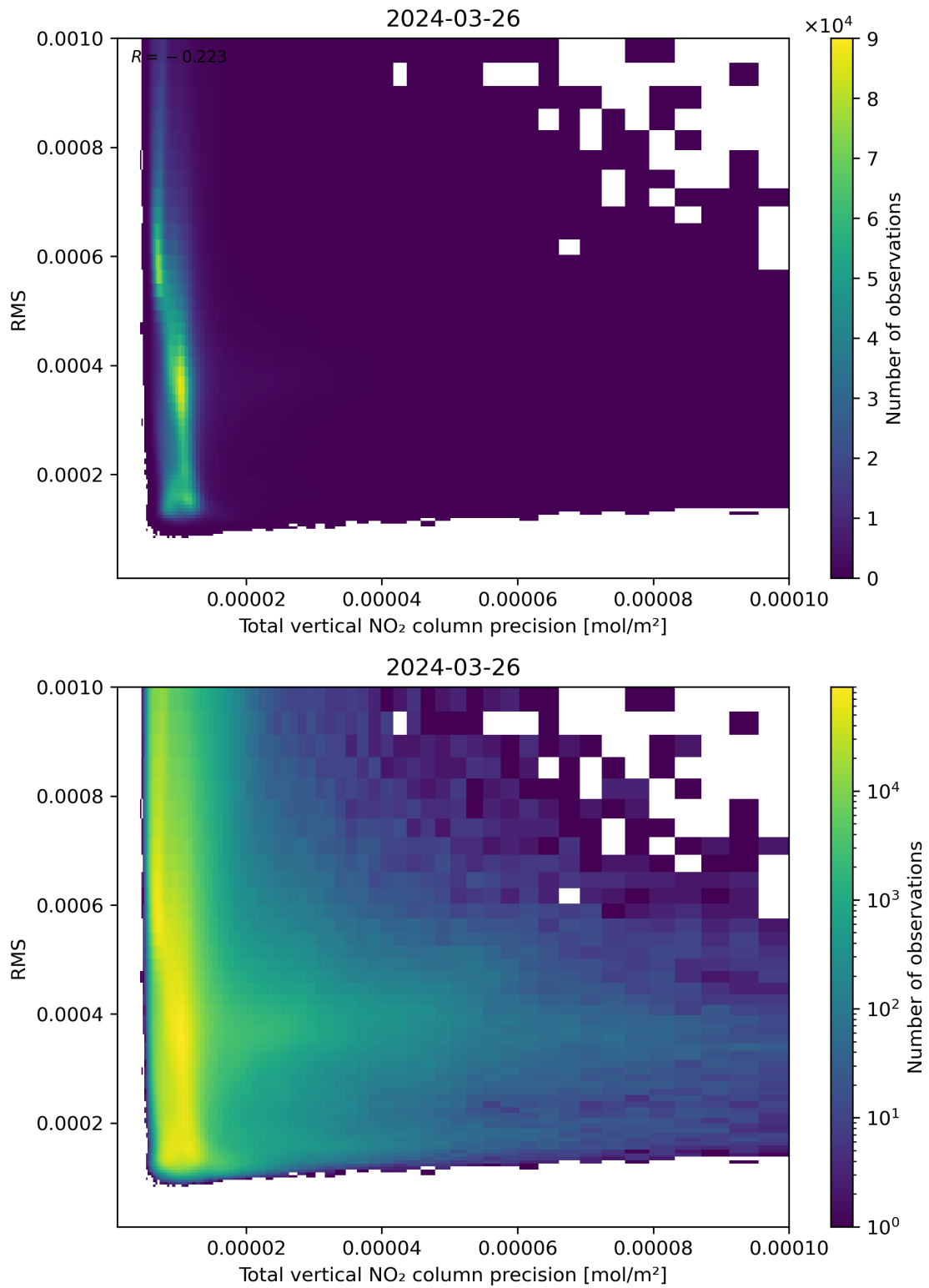
Figure 119: Scatter density plot of “Total vertical NO 2 column precision” against “RMS” for 2024-03-25 to 2024-03-27.
