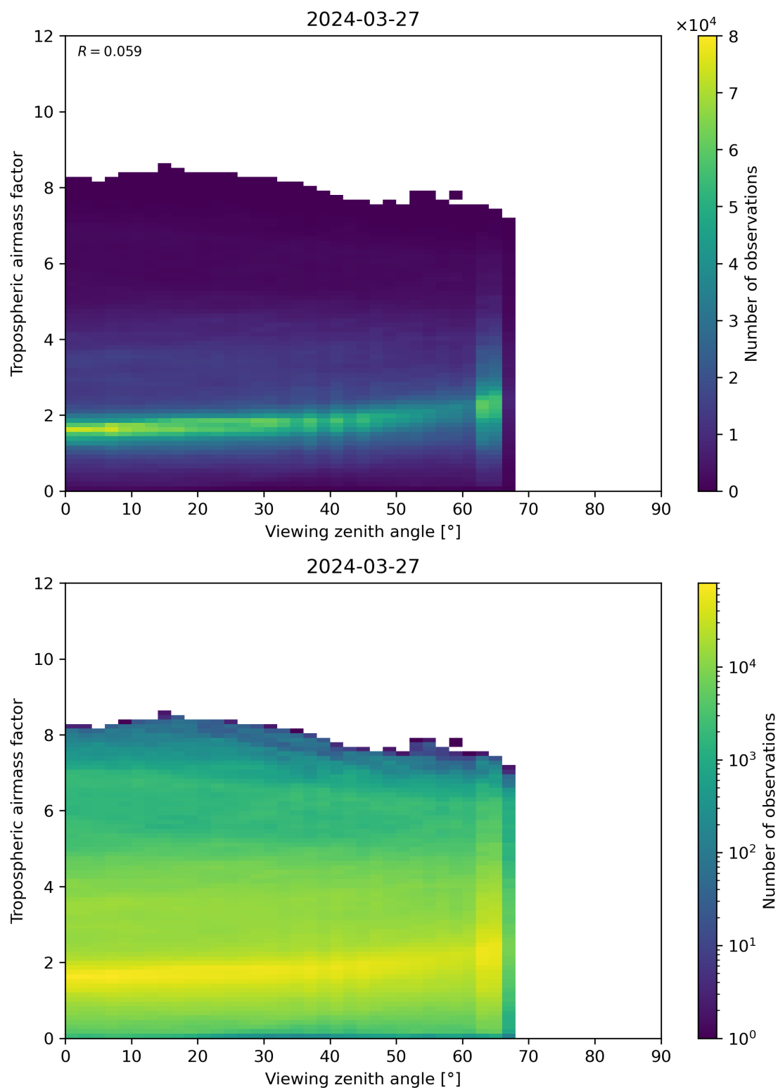
Figure 161: Scatter density plot of “Viewing zenith angle” against “Tropospheric airmass factor” for 2024-03-26 to 2024-03-28.
