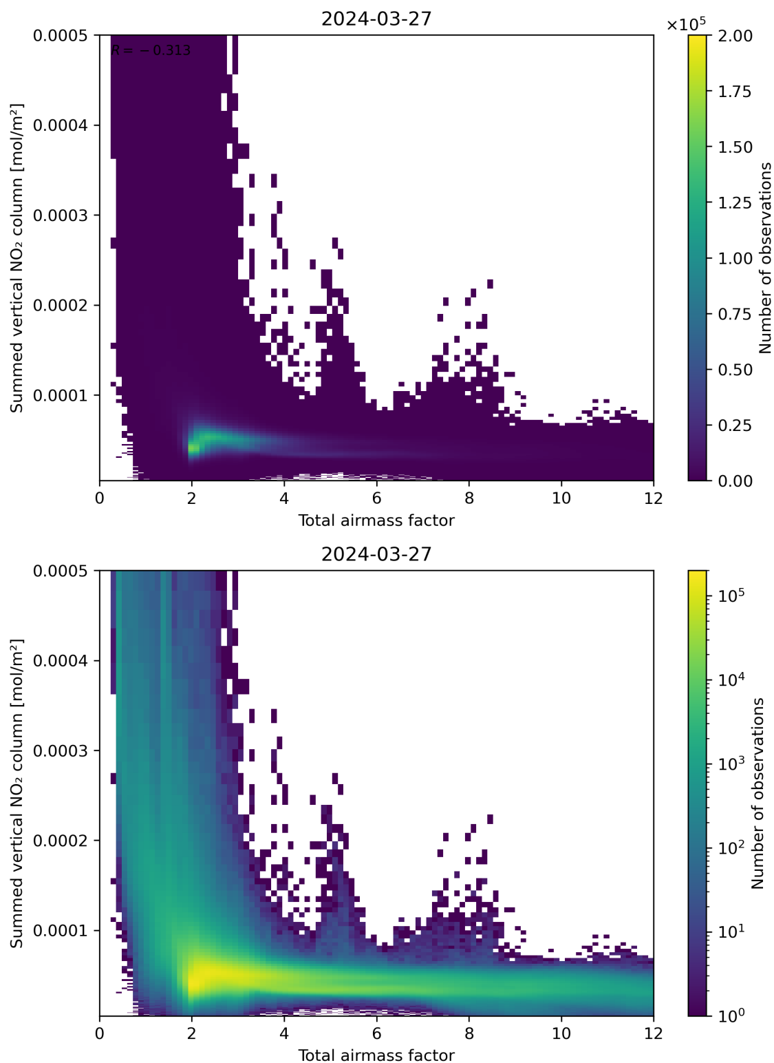
Figure 65: Scatter density plot of “Total airmass factor” against “Summed vertical NO 2 column” for 2024-03-26 to 2024-03-28.
