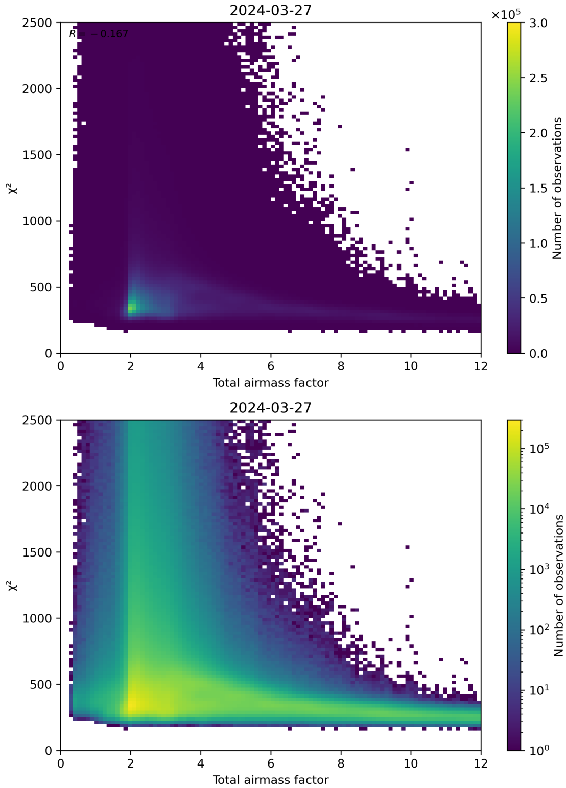
Figure 63: Scatter density plot of “Total airmass factor” against “ \chi^2 ” for 2024-03-26 to 2024-03-28.
