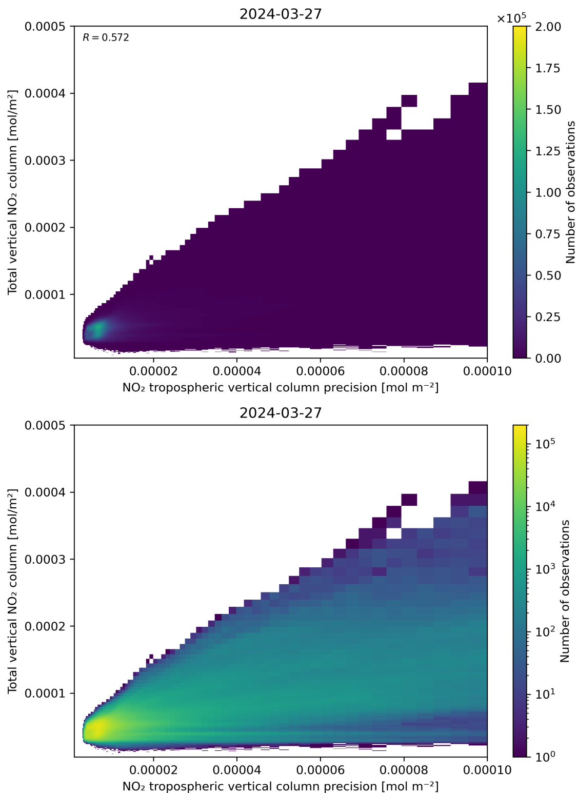
Figure 138: Scatter density plot of “NO 2 tropospheric vertical column precision” against “Total vertical NO 2 column” for 2024-03-26 to 2024-03-28.
