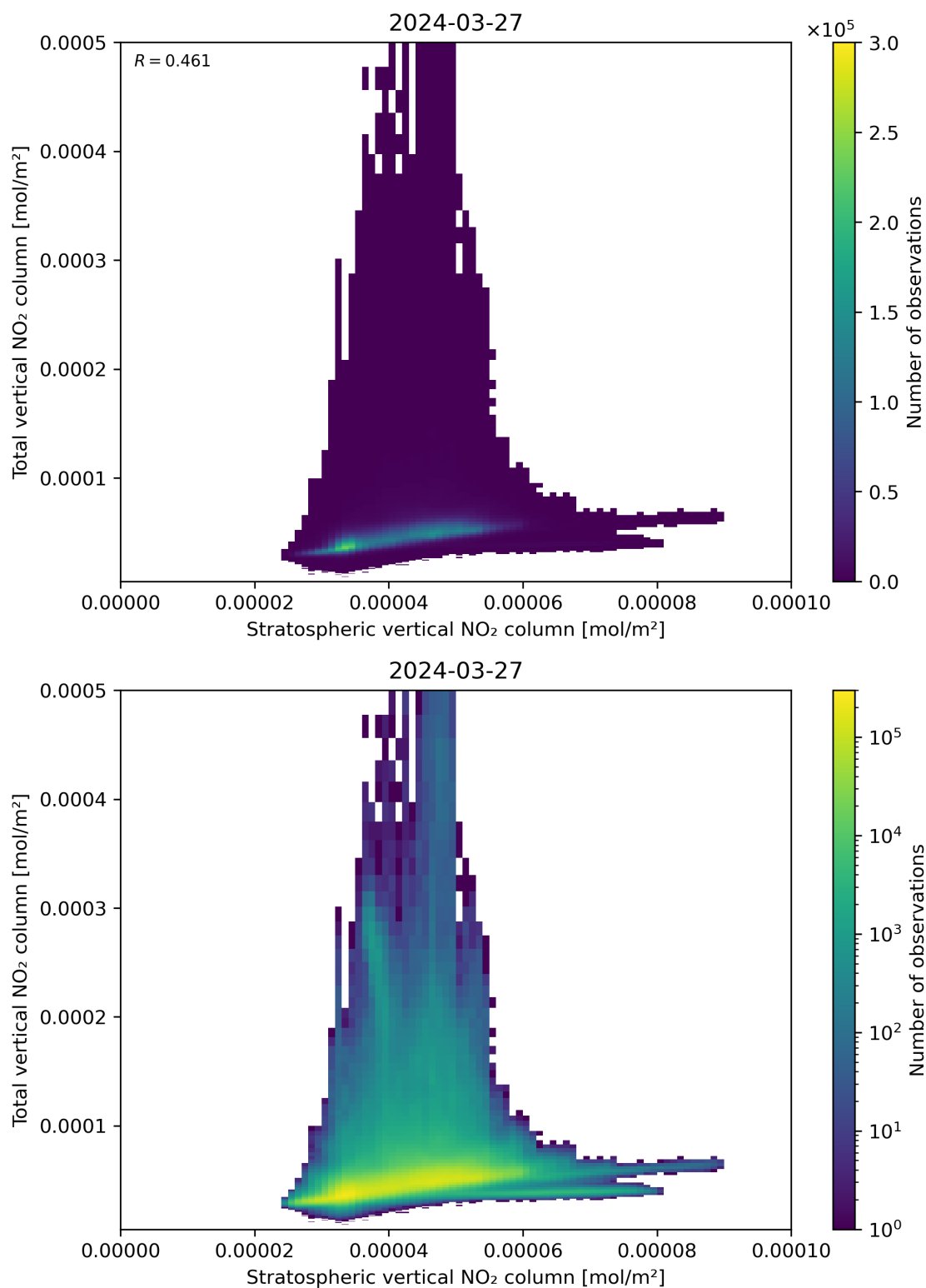
Figure 100: Scatter density plot of “Stratospheric vertical NO 2 column” against “Total vertical NO 2 column” for 2024-03-26 to 2024-03-28.
