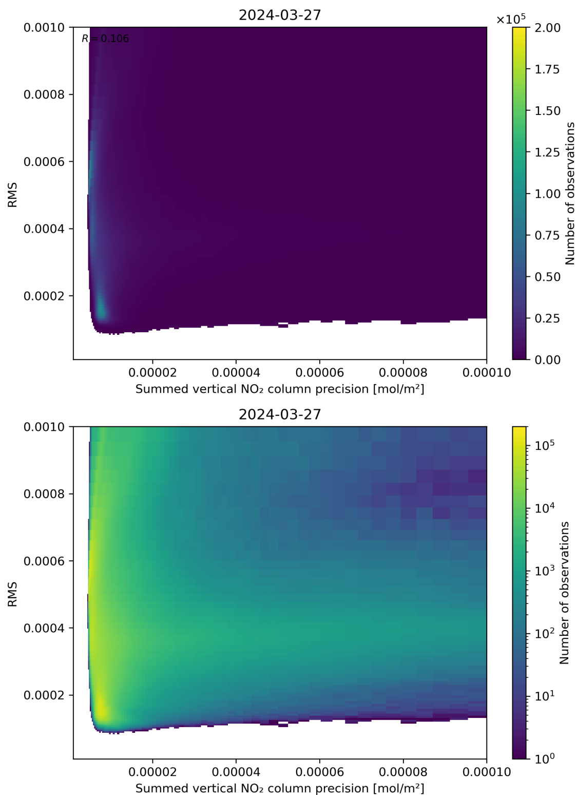
Figure 108: Scatter density plot of “Summed vertical NO 2 column precision” against “RMS” for 2024-03-26 to 2024-03-28.
