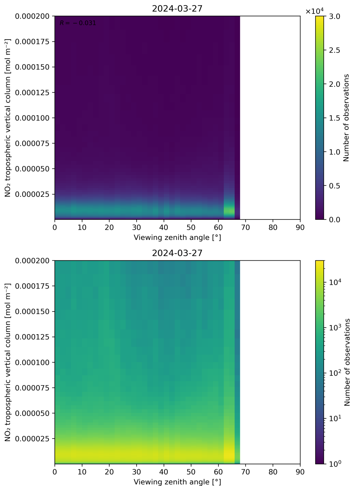
Figure 169: Scatter density plot of “Viewing zenith angle” against “NO 2 tropospheric vertical column” for 2024-03-26 to 2024-03-28.
