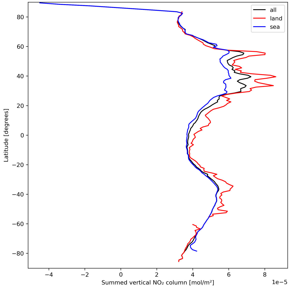
Figure 23: Zonal average of “Summed vertical NO 2 column” for 2024-03-26 to 2024-03-28.
