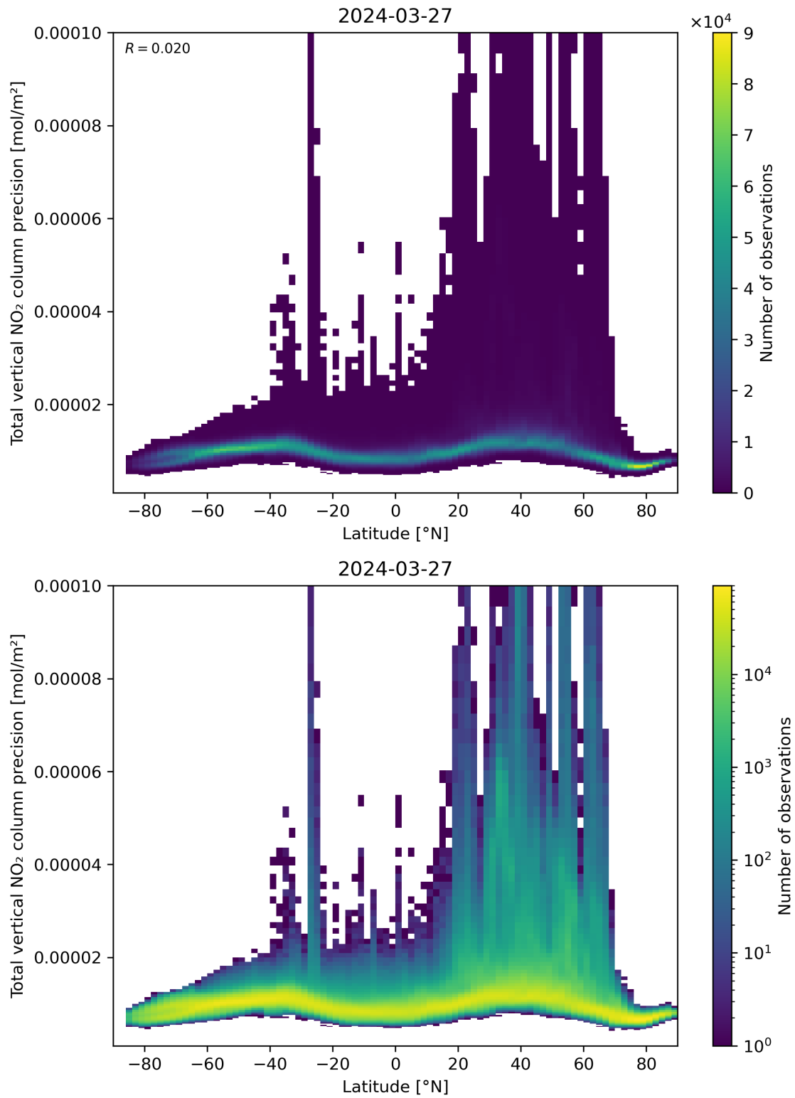
Figure 91: Scatter density plot of “Latitude” against “Total vertical NO 2 column precision” for 2024-03-26 to 2024-03-28.
