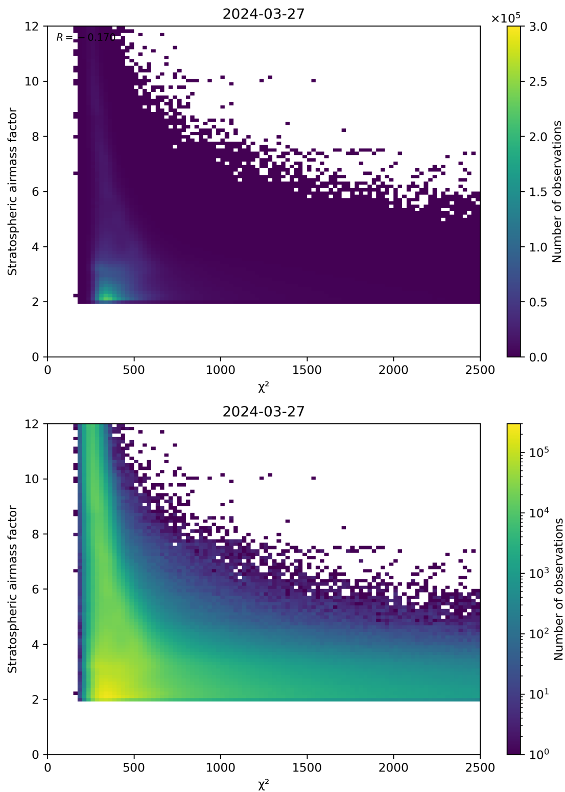
Figure 81: Scatter density plot of “ \chi^2 ” against “Stratospheric airmass factor” for 2024-03-26 to 2024-03-28.
