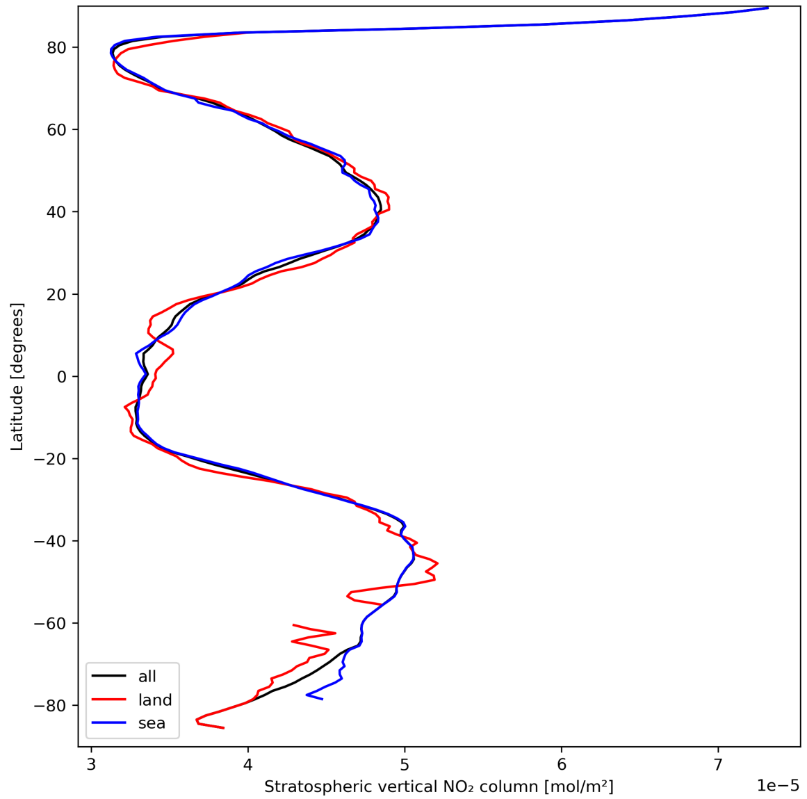
Figure 19: Zonal average of “Stratospheric vertical NO 2 column” for 2024-03-26 to 2024-03-28.
