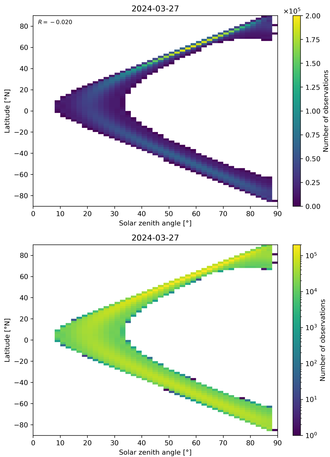
Figure 149: Scatter density plot of “Solar zenith angle” against “Latitude” for 2024-03-26 to 2024-03-28.
