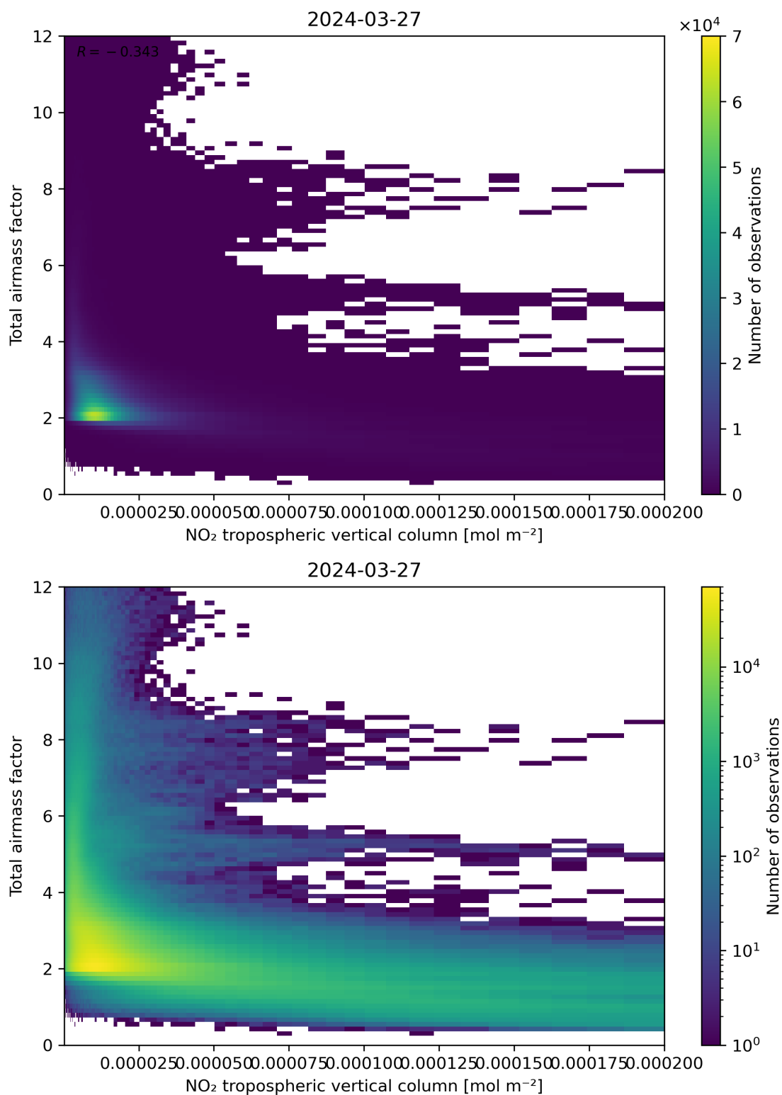
Figure 122: Scatter density plot of “NO 2 tropospheric vertical column” against “Total air mass factor” for 2024-03-26 to 2024-03-28.
