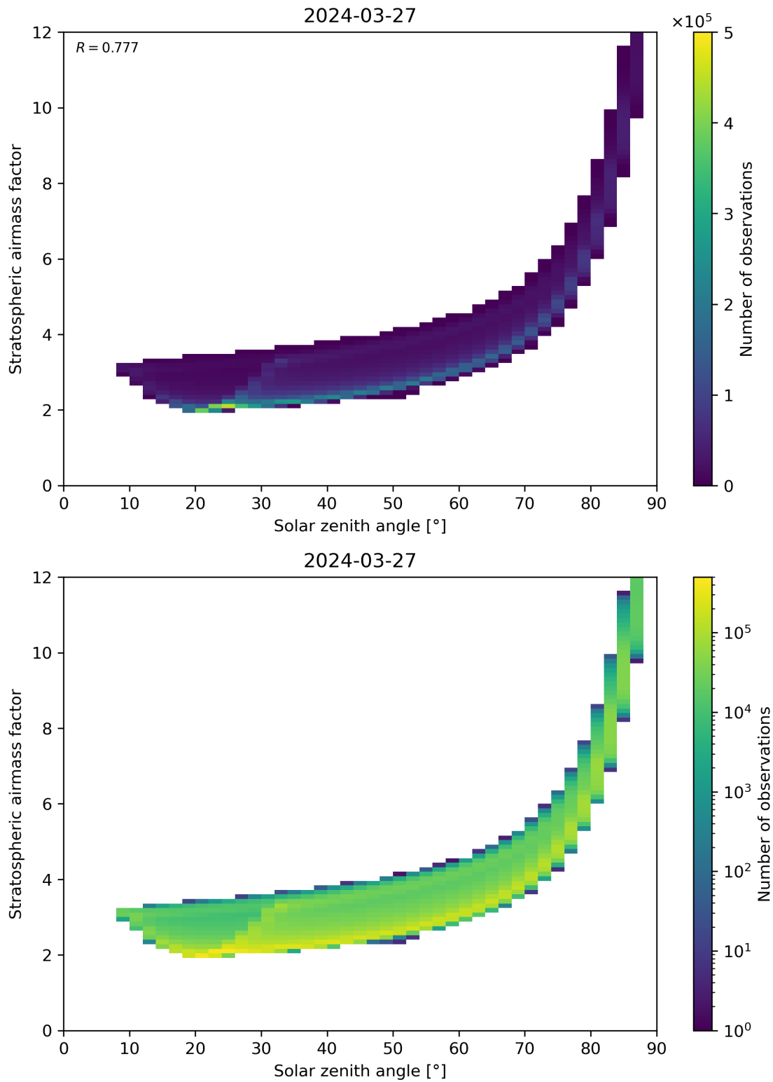
Figure 145: Scatter density plot of “Solar zenith angle” against “Stratospheric airmass factor” for 2024-03-26 to 2024-03-28.
