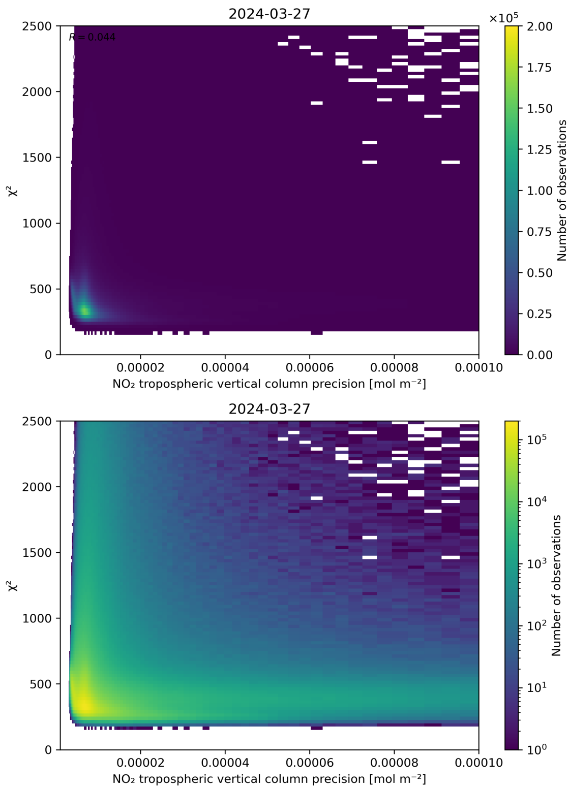
Figure 134: Scatter density plot of “NO 2 tropospheric vertical column precision” against “ \chi^2 ” for 2024-03-26 to 2024-03-28.
