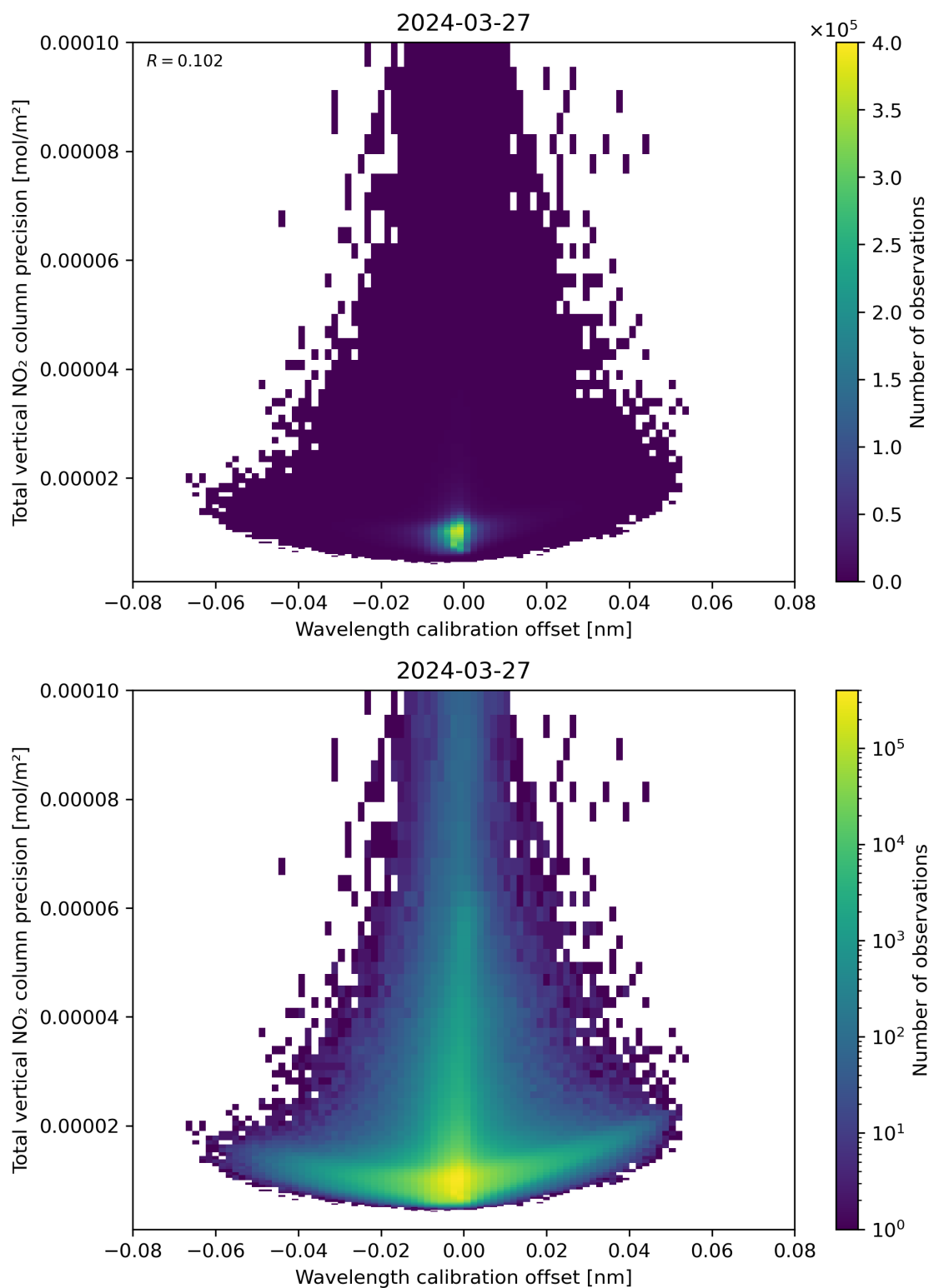
Figure 180: Scatter density plot of “Wavelength calibration offset” against “Total vertical NO 2 column precision” for 2024-03-26 to 2024-03-28.
