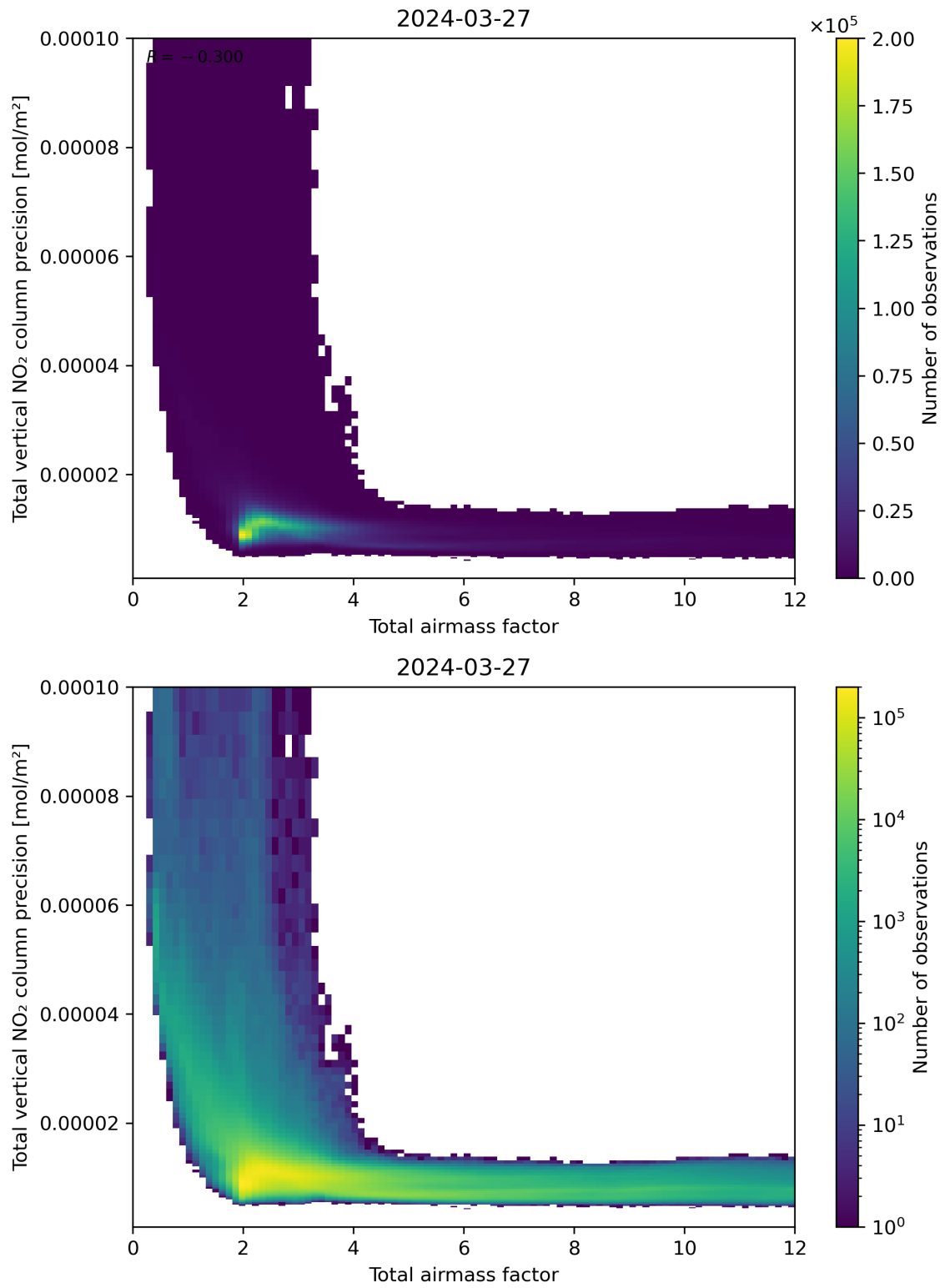
Figure 68: Scatter density plot of “Total airmass factor” against “Total vertical NO 2 column precision” for 2024-03-26 to 2024-03-28.
