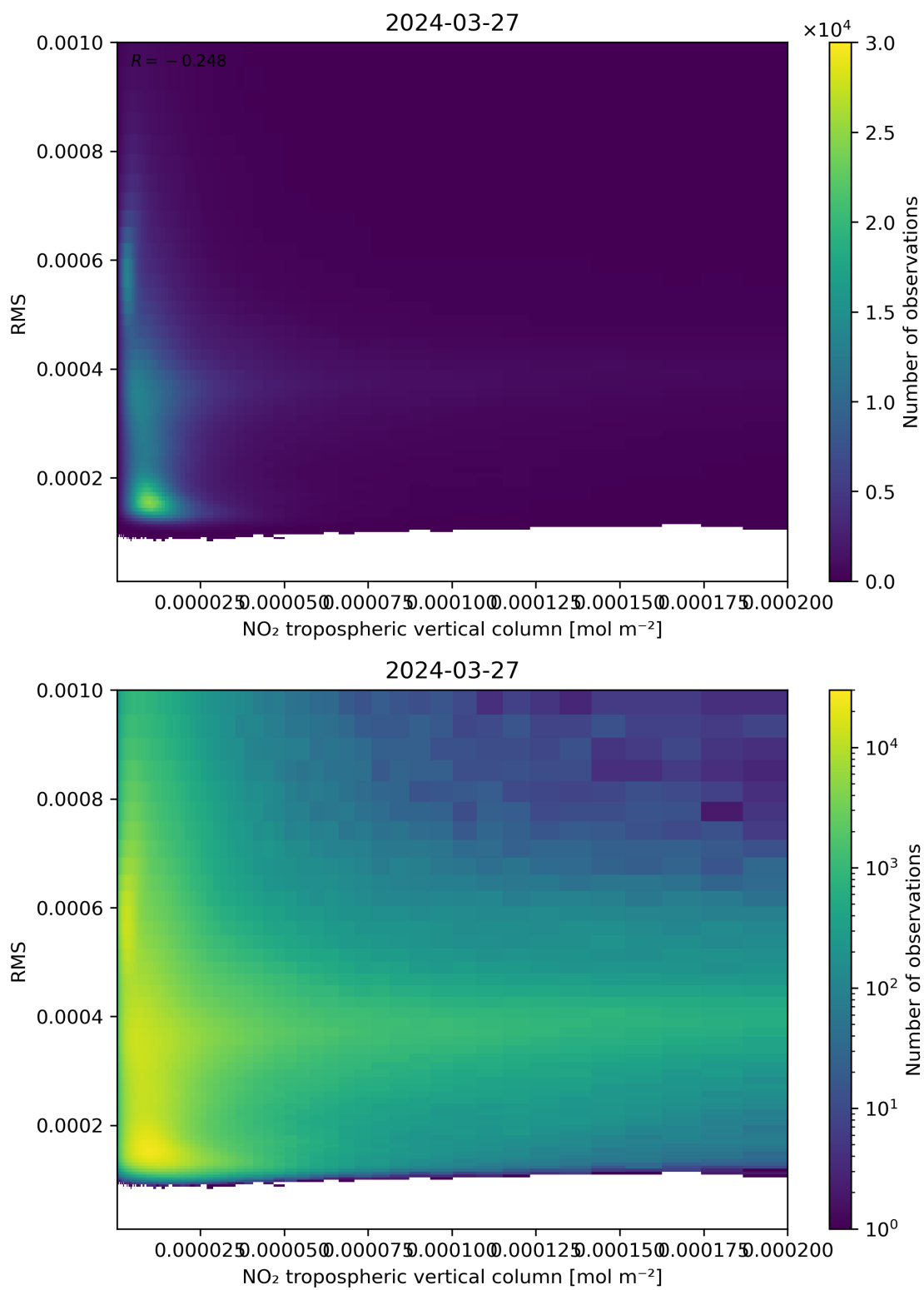
Figure 142: Scatter density plot of “NO 2 tropospheric vertical column” against “RMS” for 2024-03-26 to 2024-03-28.
