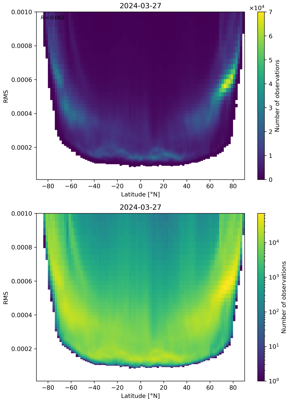
Figure 94: Scatter density plot of “Latitude” against “RMS” for 2024-03-26 to 2024-03-28.
