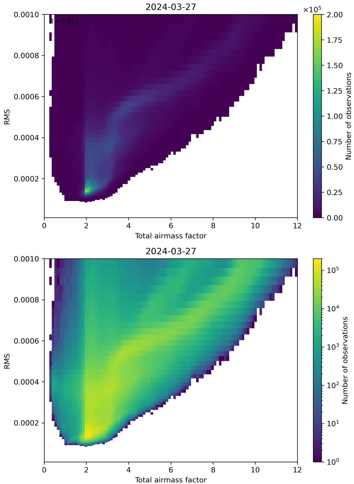
Figure 69: Scatter density plot of “Total airmass factor” against “RMS” for 2024-03-26 to 2024-03-28.
