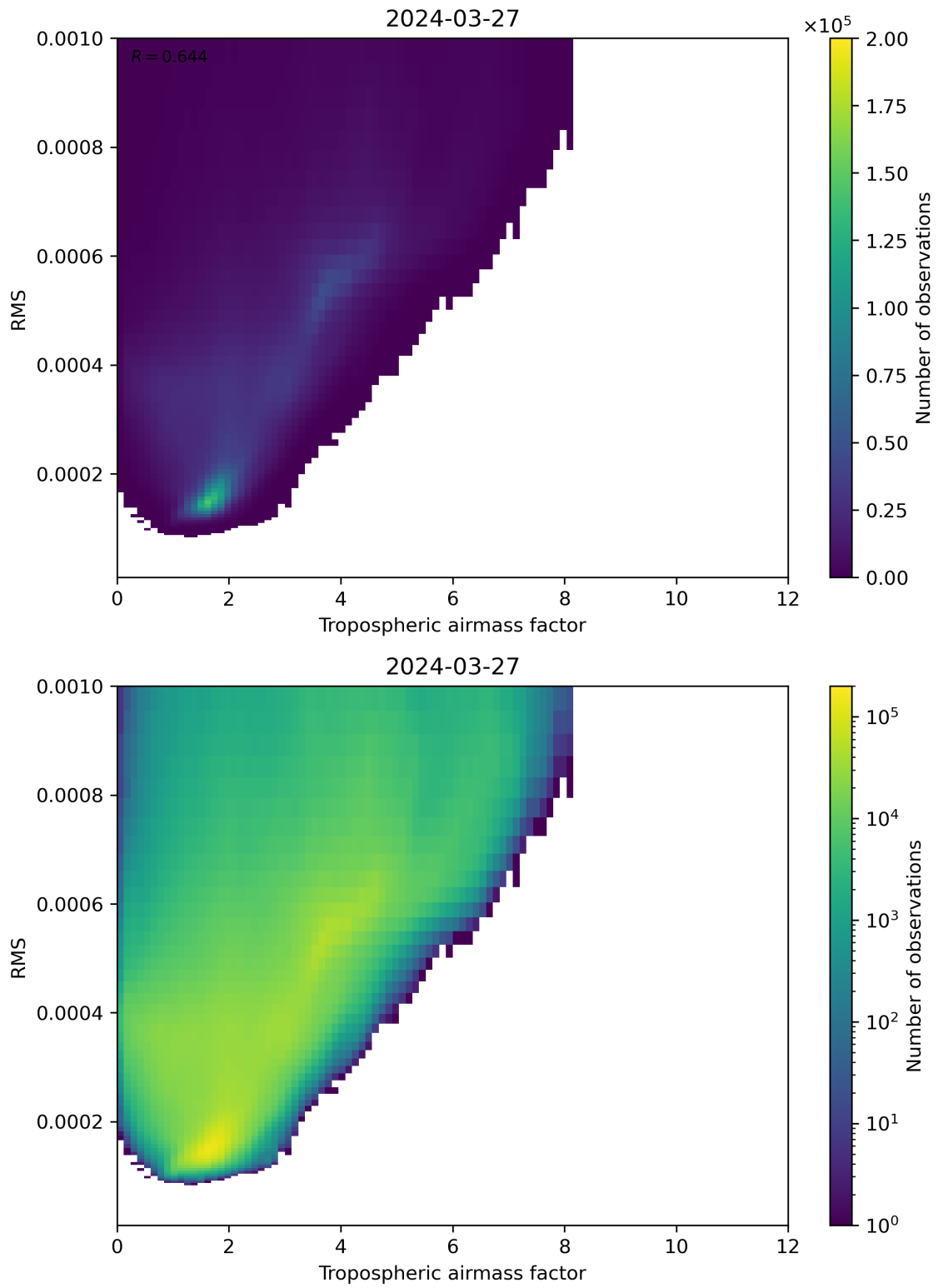
Figure 79: Scatter density plot of “Tropospheric airmass factor” against “RMS” for 2024-03-26 to 2024-03-28.
