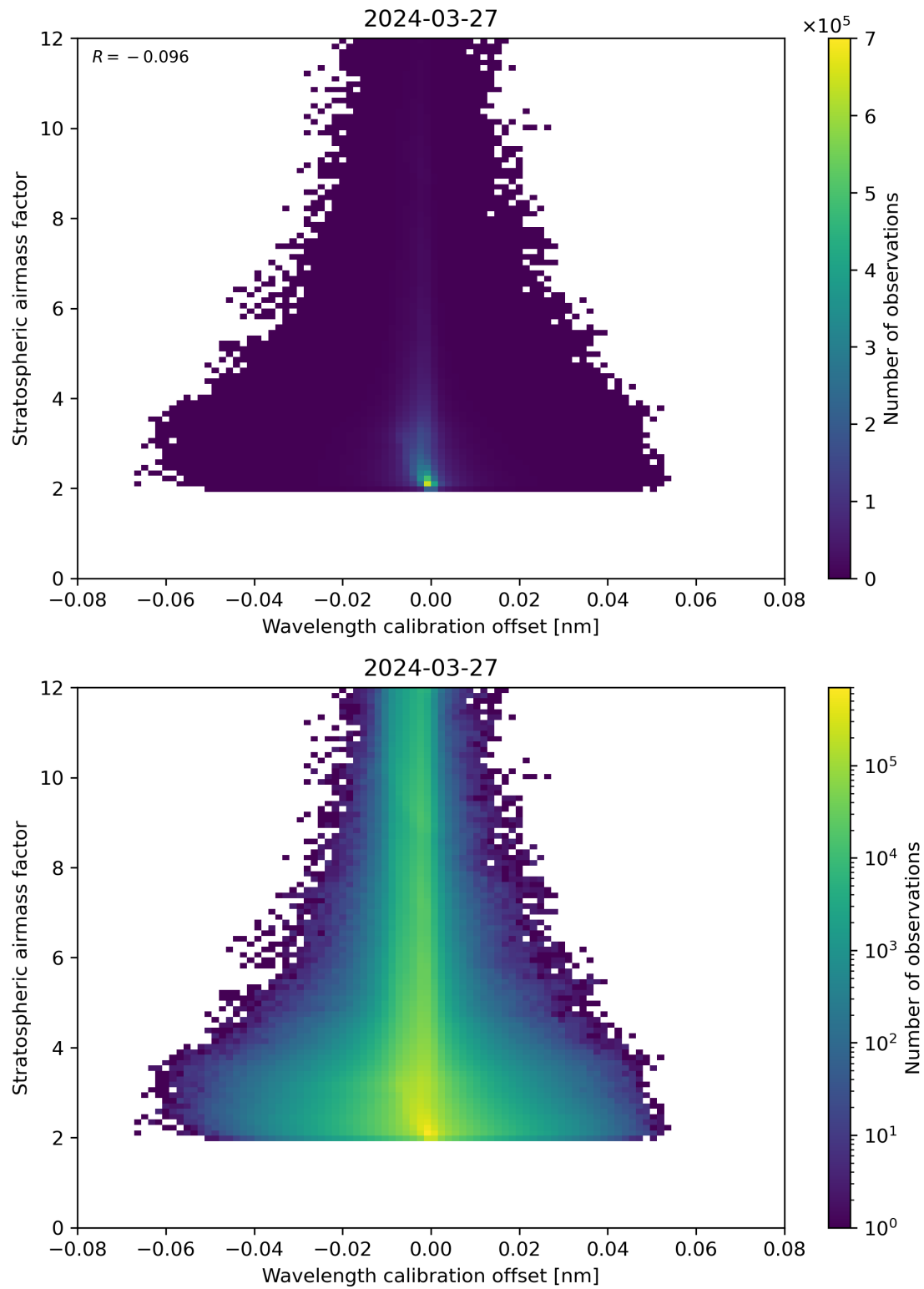
Figure 174: Scatter density plot of “Wavelength calibration offset” against “Stratospheric airmass factor” for 2024-03-26 to 2024-03-28.
