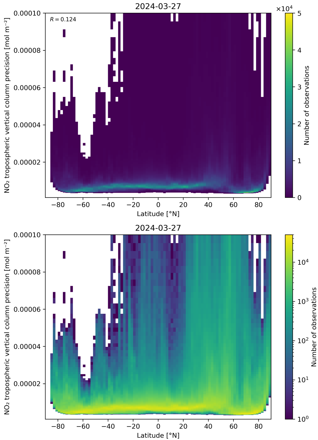
Figure 93: Scatter density plot of “Latitude” against “NO 2 tropospheric vertical column precision” for 2024-03-26 to 2024-03-28.
