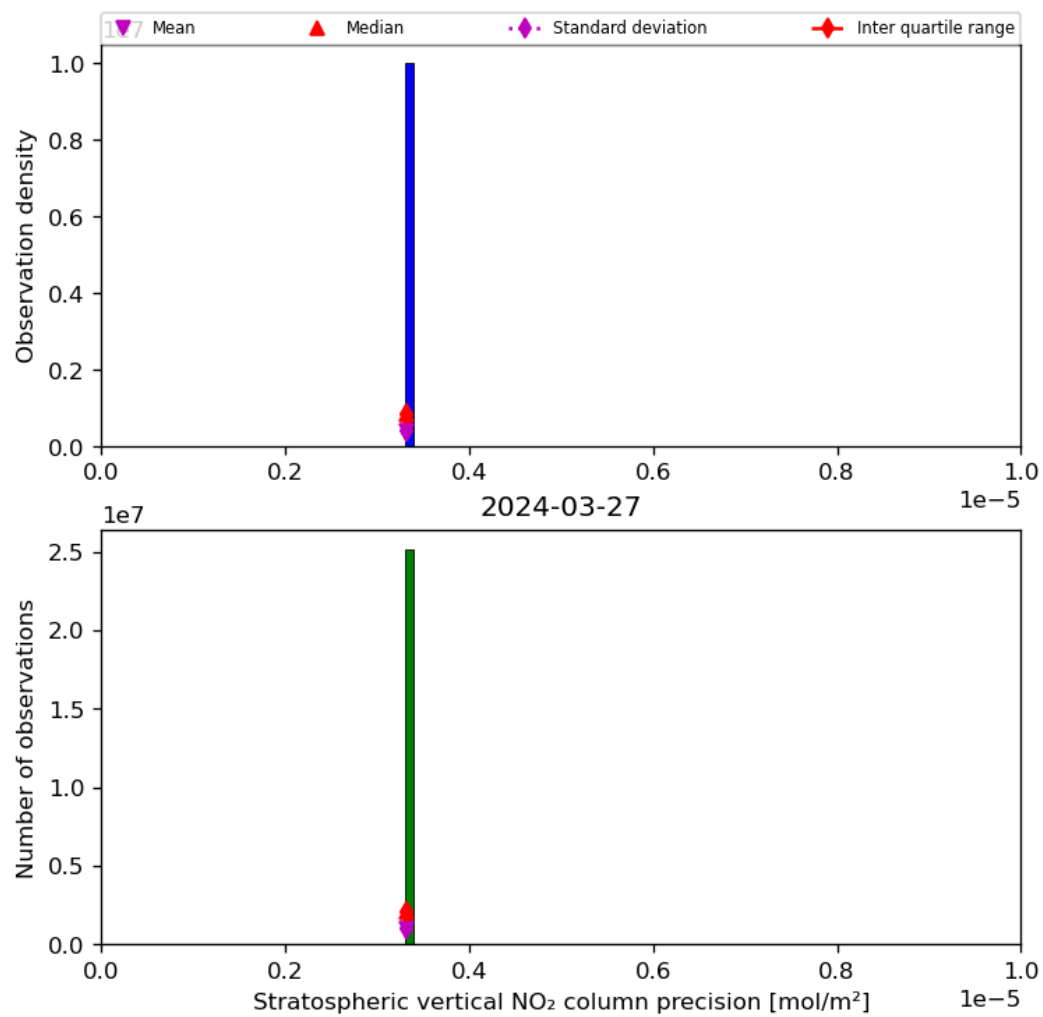
Figure 37: Histogram of “Stratospheric vertical NO 2 column precision” for 2024-03-26 to 2024-03-28
