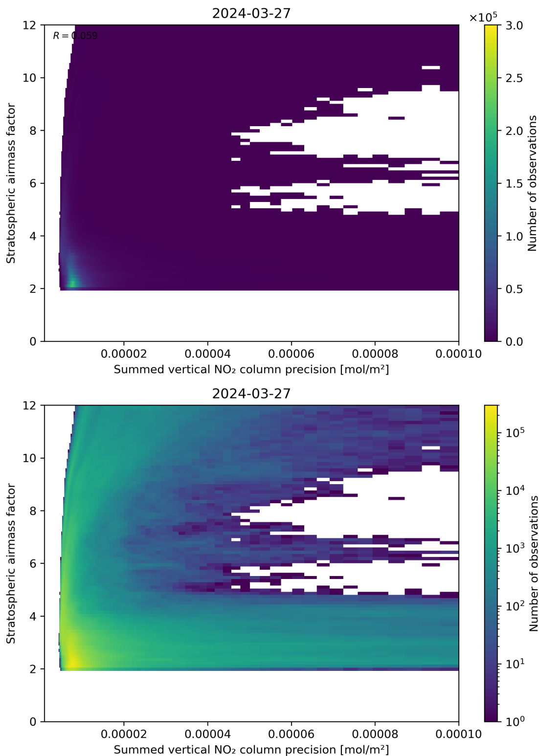
Figure 106: Scatter density plot of “Summed vertical NO 2 column precision” against “Stratospheric airmass factor” for 2024-03-26 to 2024-03-28.
