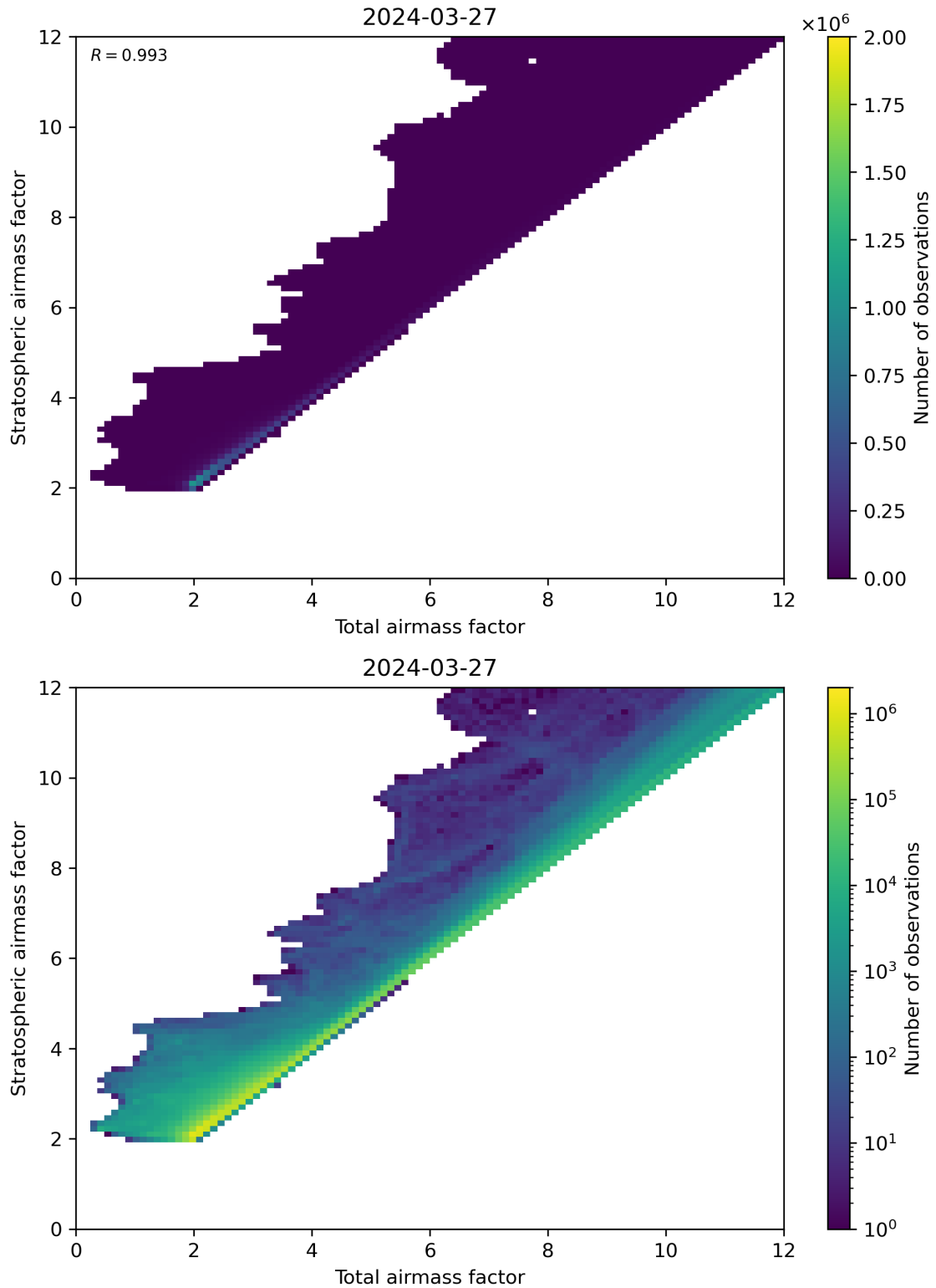
Figure 62: Scatter density plot of “Total airmass factor” against “Stratospheric airmass factor” for 2024-03-26 to 2024-03-28.
