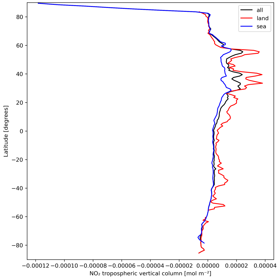
Figure 12: Zonal average of “NO 2 tropospheric vertical column” for 2024-03-26 to 2024-03-28.
