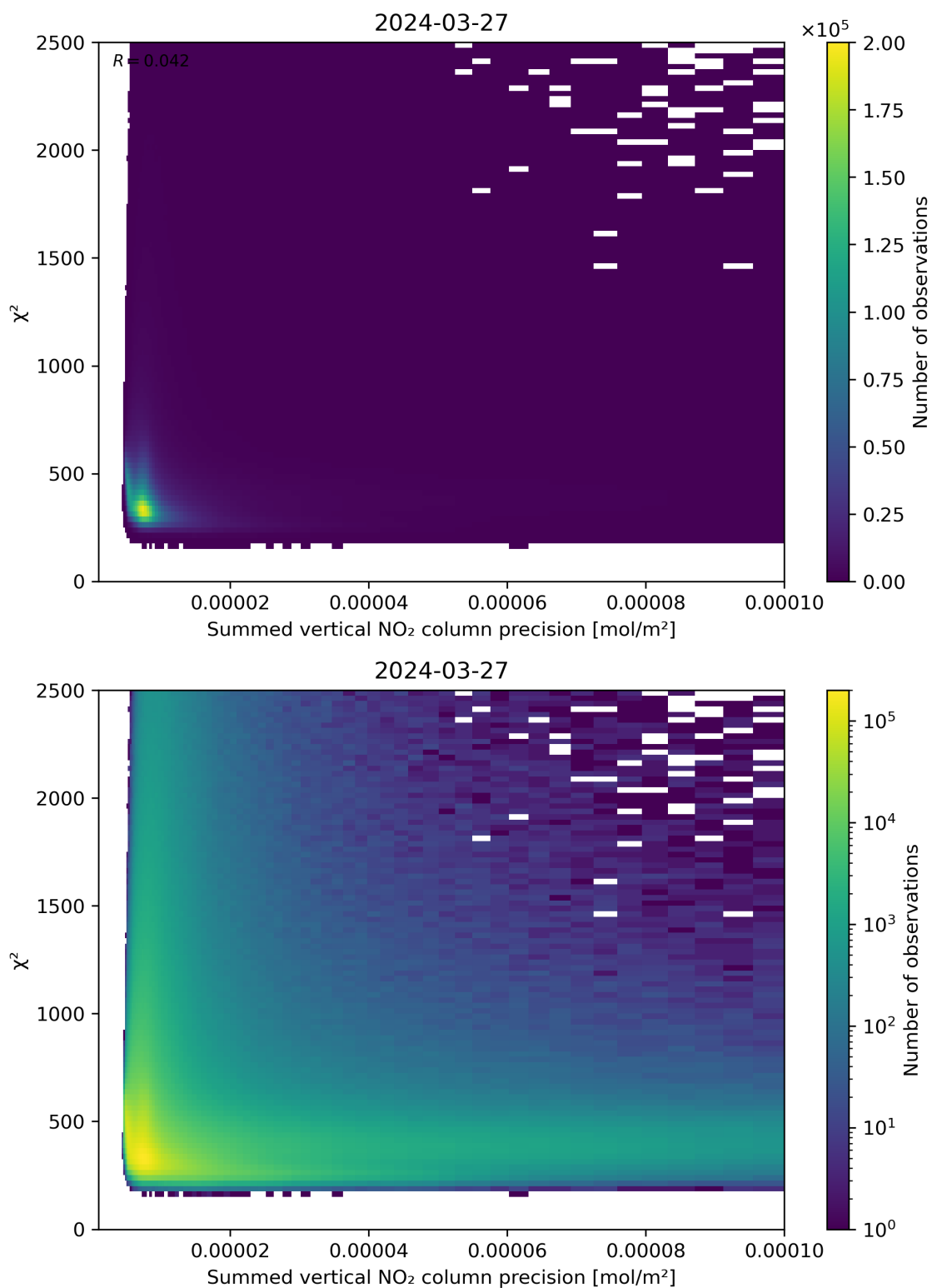
Figure 107: Scatter density plot of “Summed vertical NO 2 column precision” against “ \chi^2 ” for 2024-03-26 to 2024-03-28.
