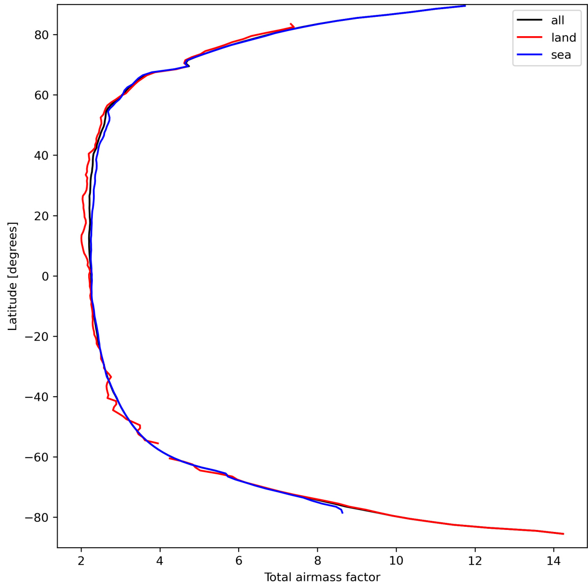
Figure 15: Zonal average of “Total airmass factor” for 2024-03-26 to 2024-03-28.
