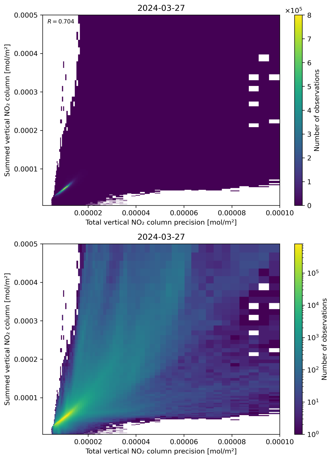
Figure 117: Scatter density plot of “Total vertical NO 2 column precision” against “Summed vertical NO 2 column” for 2024-03-26 to 2024-03-28.
