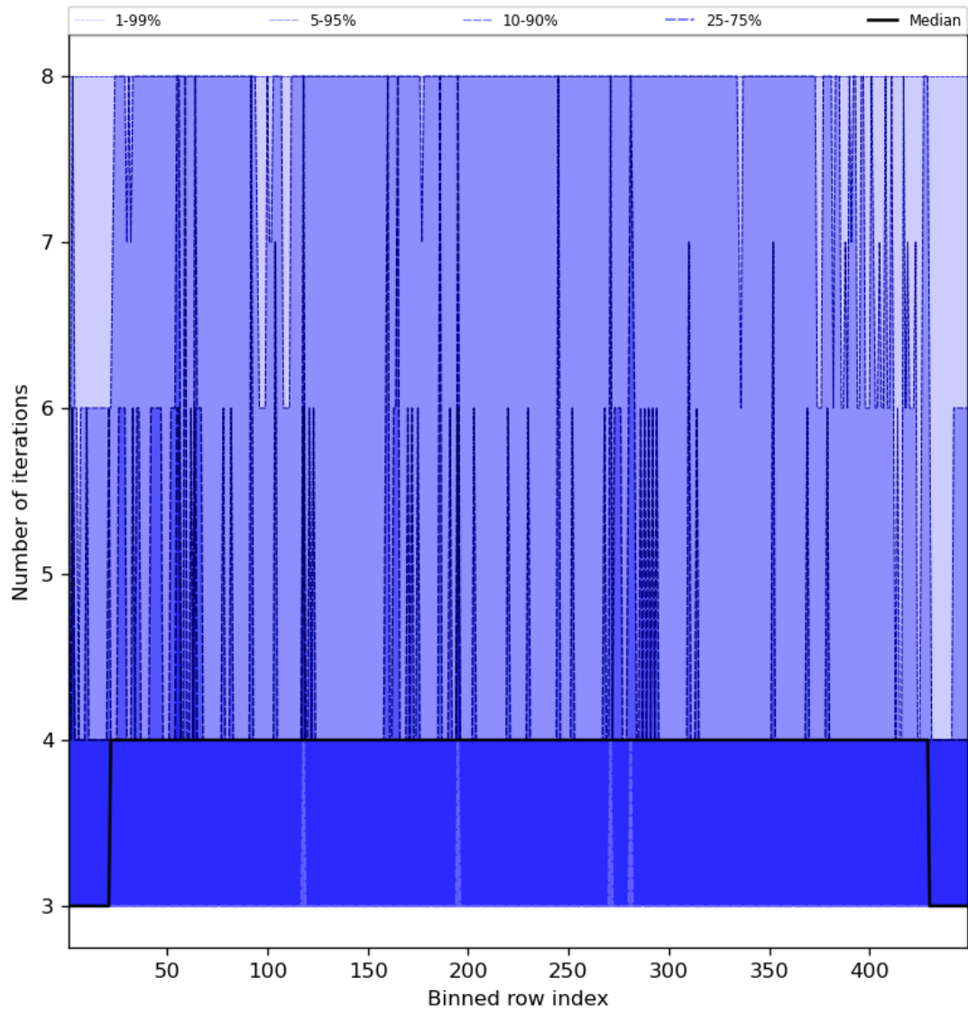
Figure 51: Along track statistics of “Number of iterations” for 2024-03-26 to 2024-03-28
