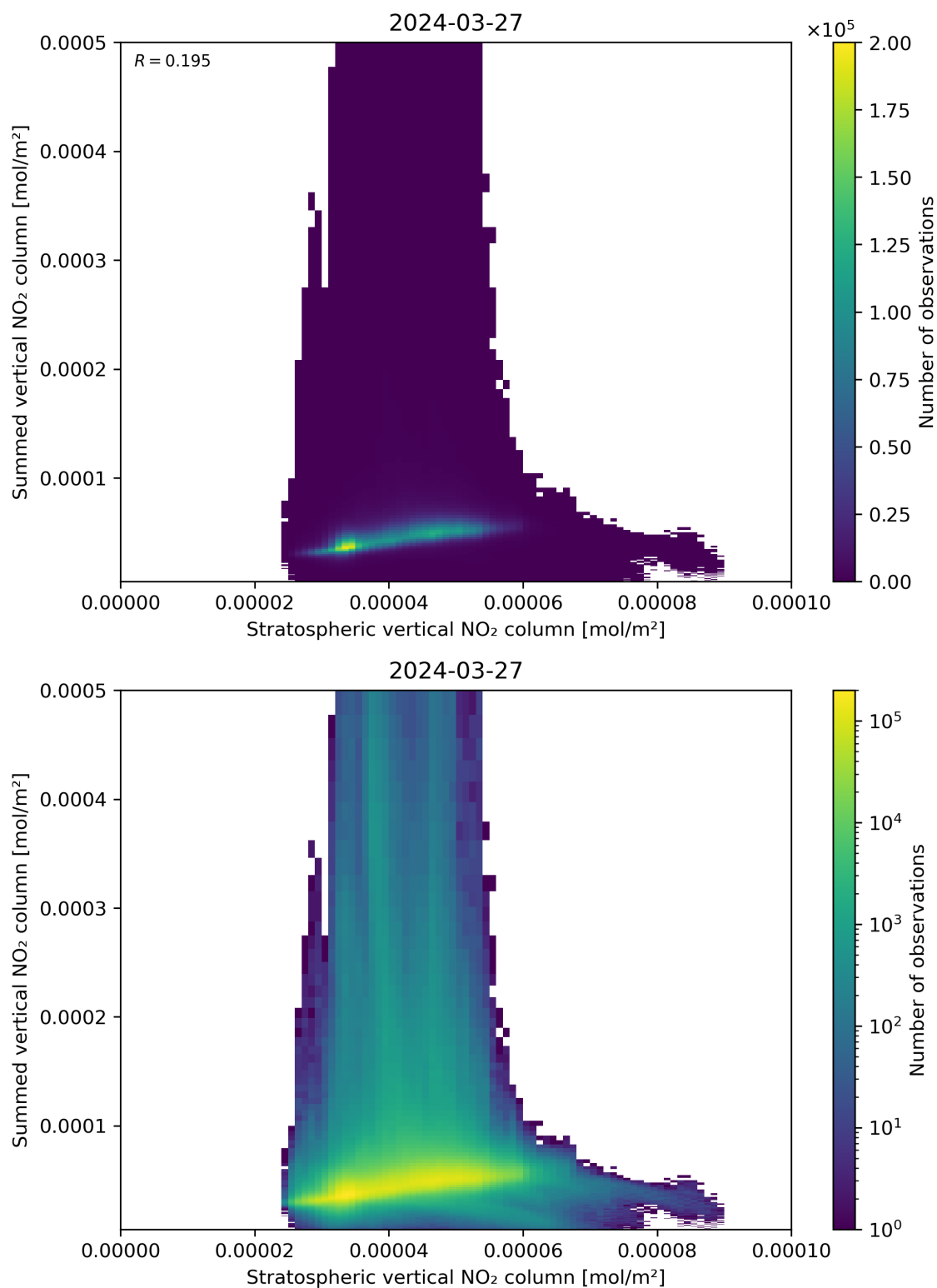
Figure 98: Scatter density plot of “Stratospheric vertical NO 2 column” against “Summed vertical NO 2 column” for 2024-03-26 to 2024-03-28.
