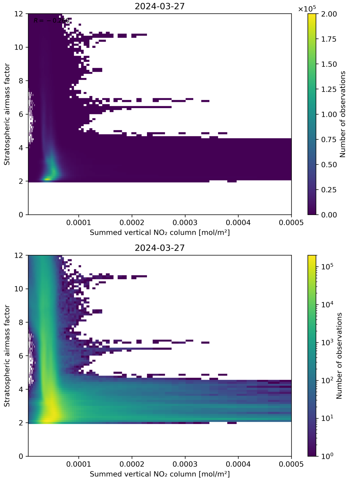
Figure 103: Scatter density plot of “Summed vertical NO 2 column” against “Stratospheric air mass factor” for 2024-03-26 to 2024-03-28.
