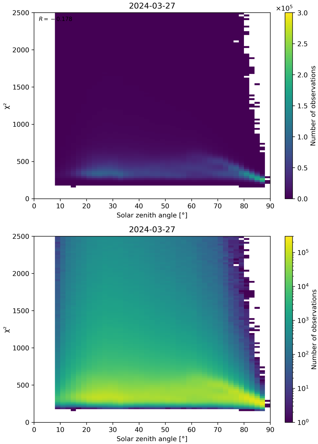
Figure 148: Scatter density plot of “Solar zenith angle” against “ \chi^2 ” for 2024-03-26 to 2024-03-28.
