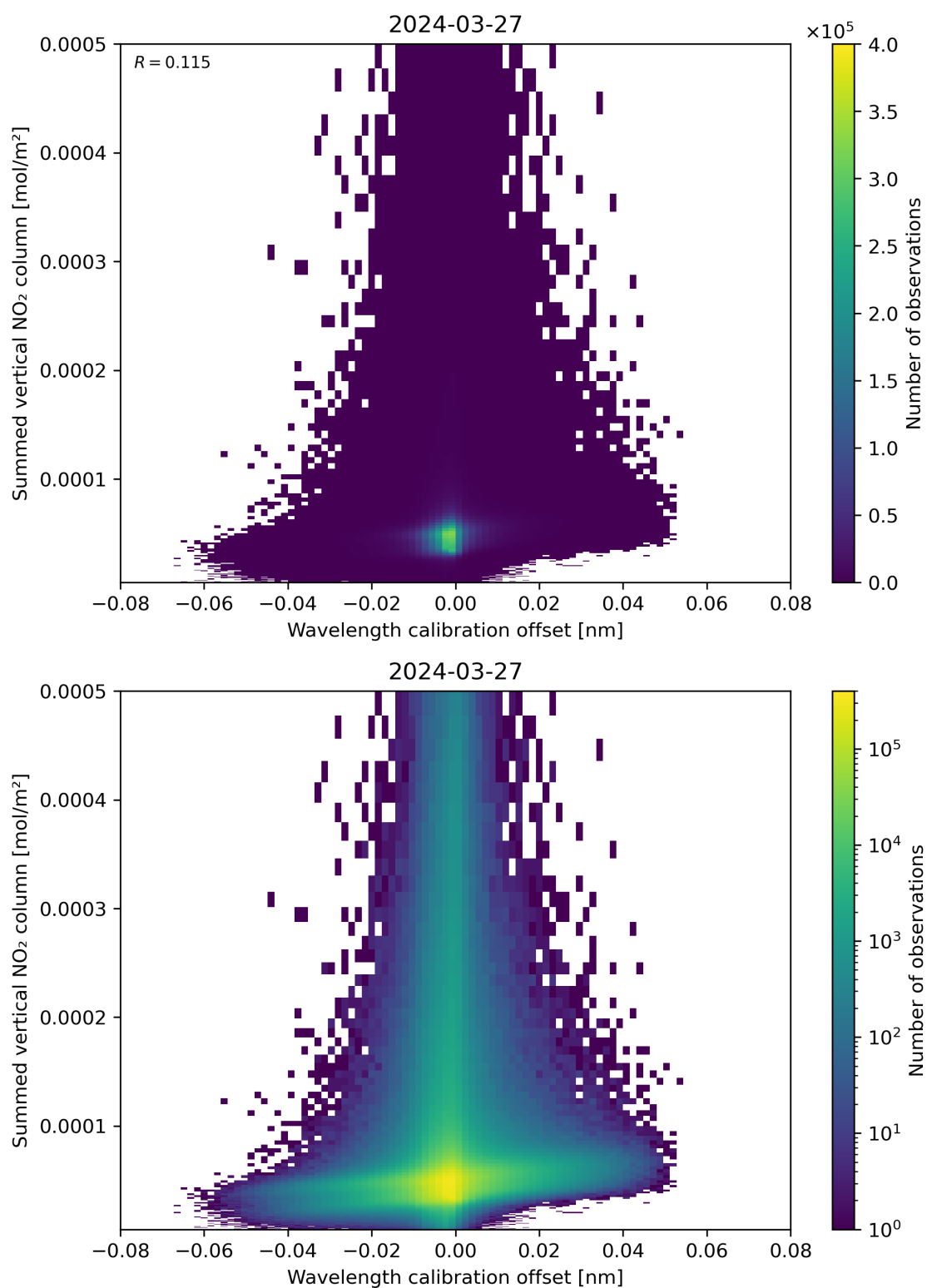
Figure 177: Scatter density plot of “Wavelength calibration offset” against “Summed vertical NO 2 column” for 2024-03-26 to 2024-03-28.
