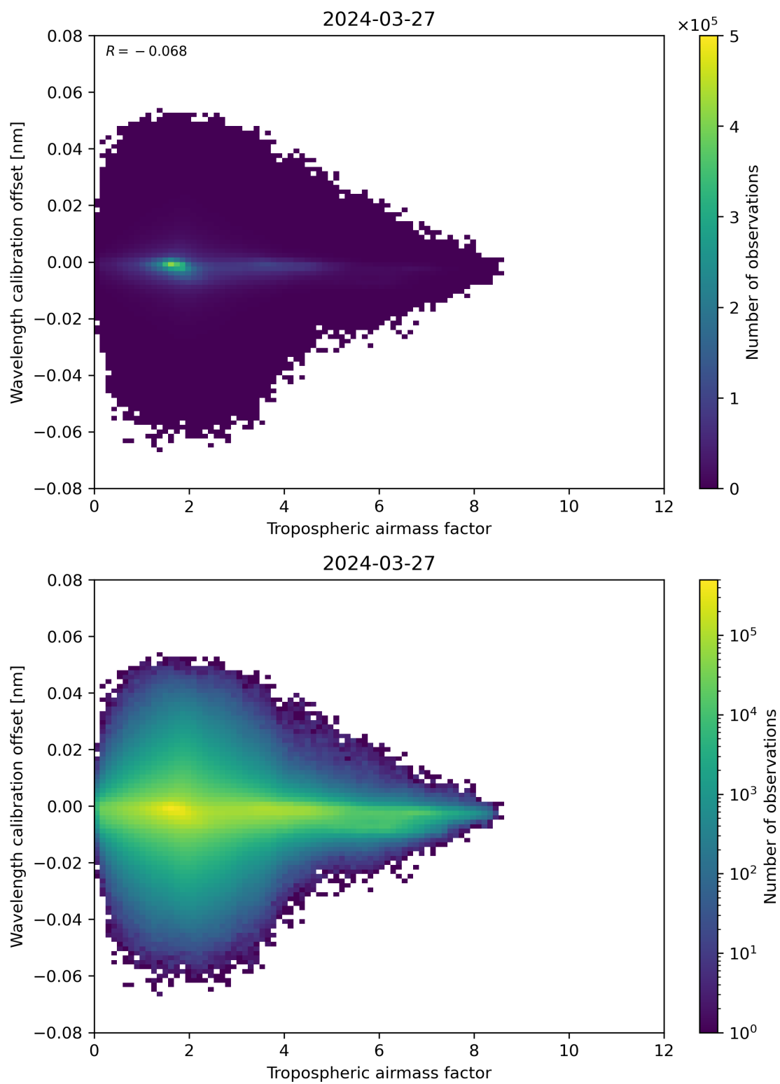
Figure 80: Scatter density plot of “Tropospheric airmass factor” against “Wavelength calibration offset” for 2024-03-26 to 2024-03-28.
