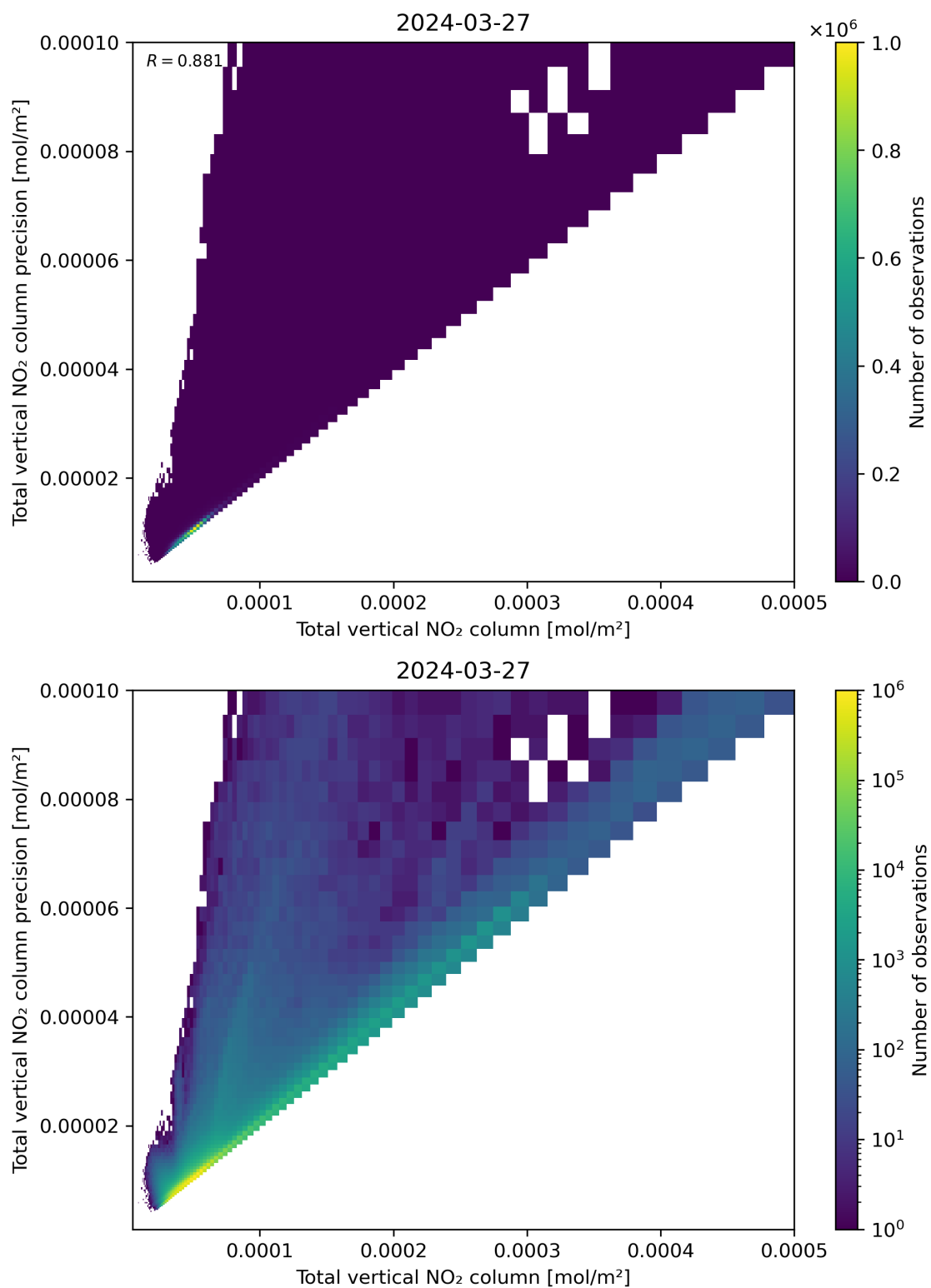
Figure 114: Scatter density plot of “Total vertical NO 2 column” against “Total vertical NO 2 column precision” for 2024-03-26 to 2024-03-28.
