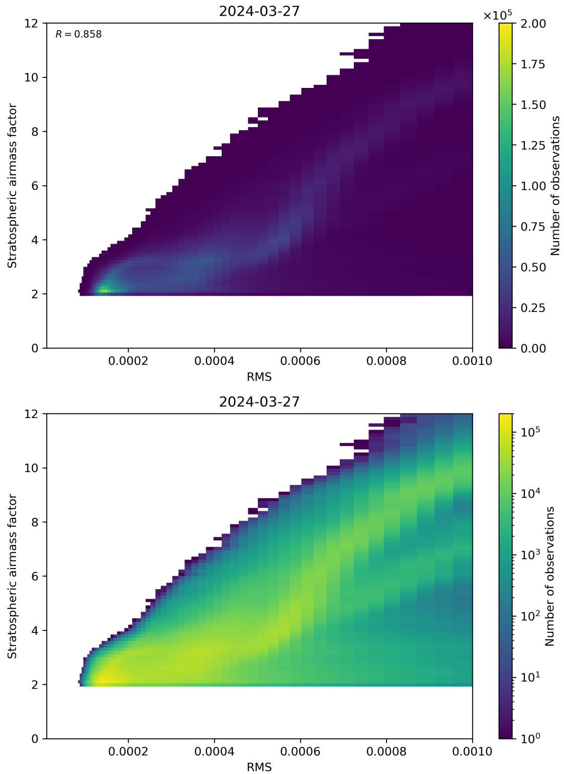
Figure 144: Scatter density plot of “RMS” against “Stratospheric airmass factor” for 2024-03-26 to 2024-03-28.
