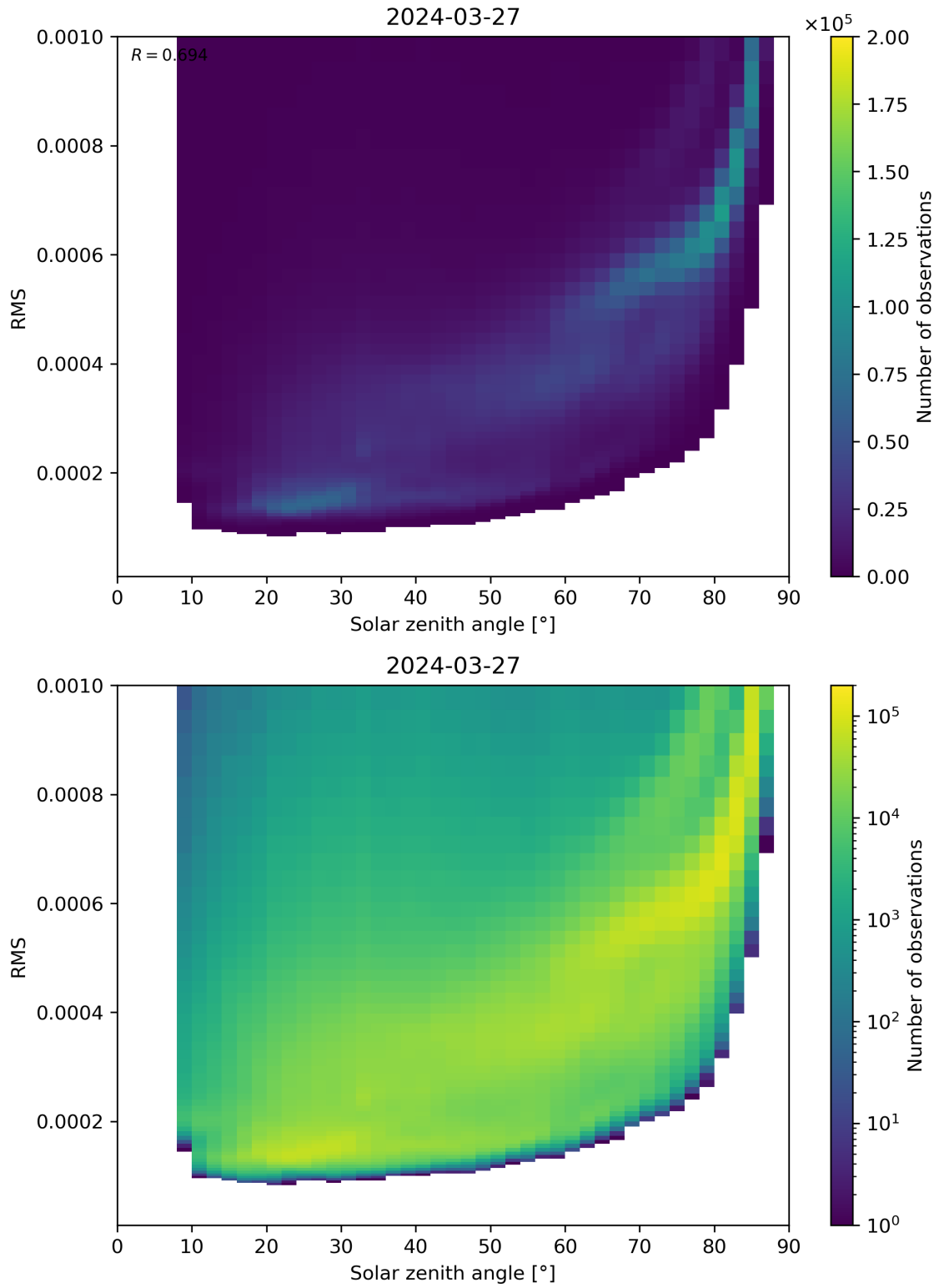
Figure 157: Scatter density plot of “Solar zenith angle” against “RMS” for 2024-03-26 to 2024-03-28.
