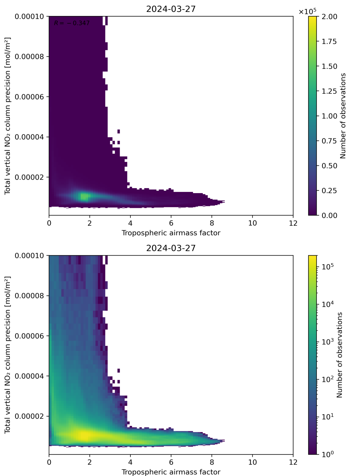
Figure 78: Scatter density plot of “Tropospheric air mass factor” against “Total vertical NO 2 column precision” for 2024-03-26 to 2024-03-28.
