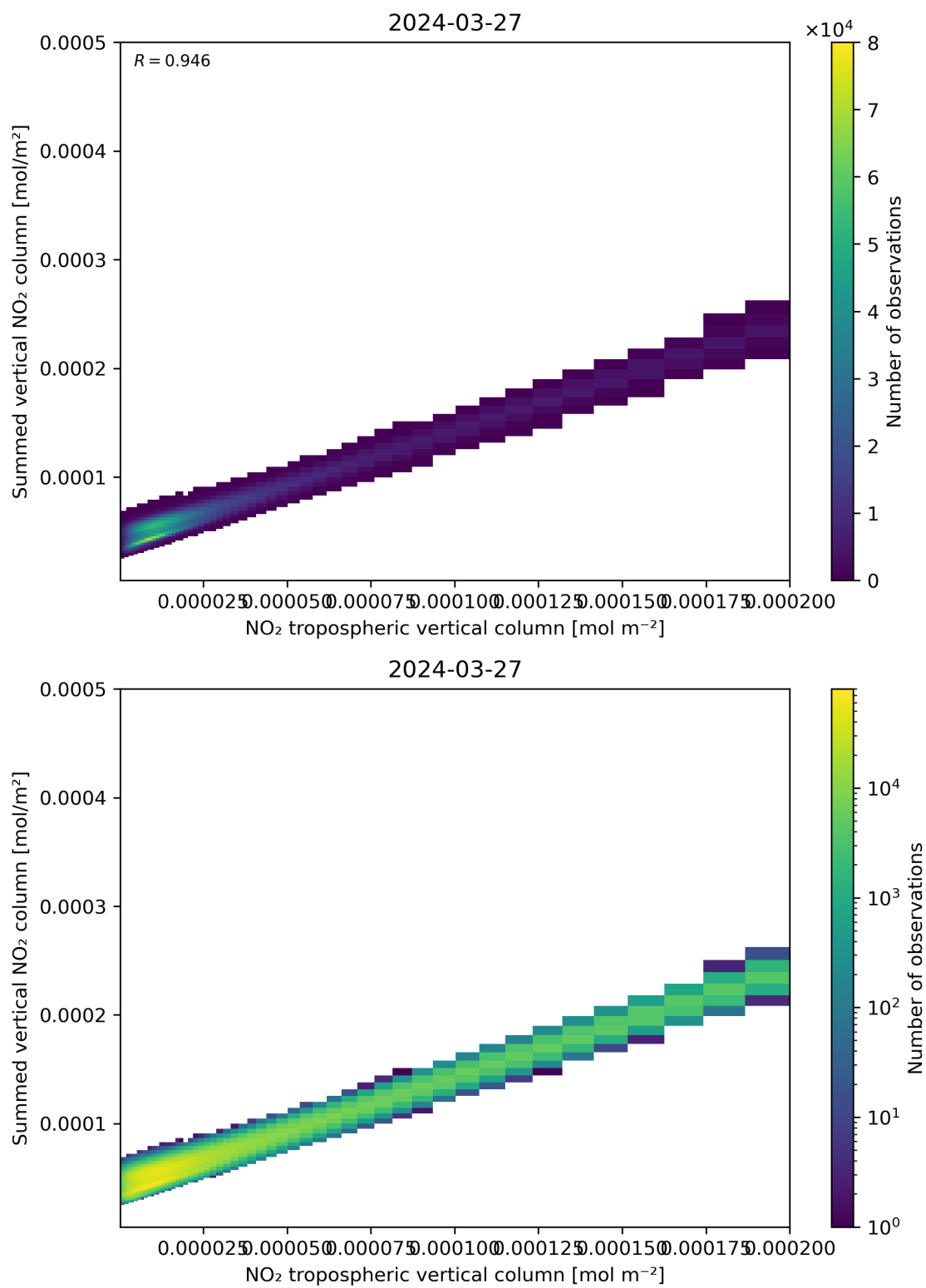
Figure 126: Scatter density plot of “NO 2 tropospheric vertical column” against “Summed vertical NO 2 column” for 2024-03-26 to 2024-03-28.
