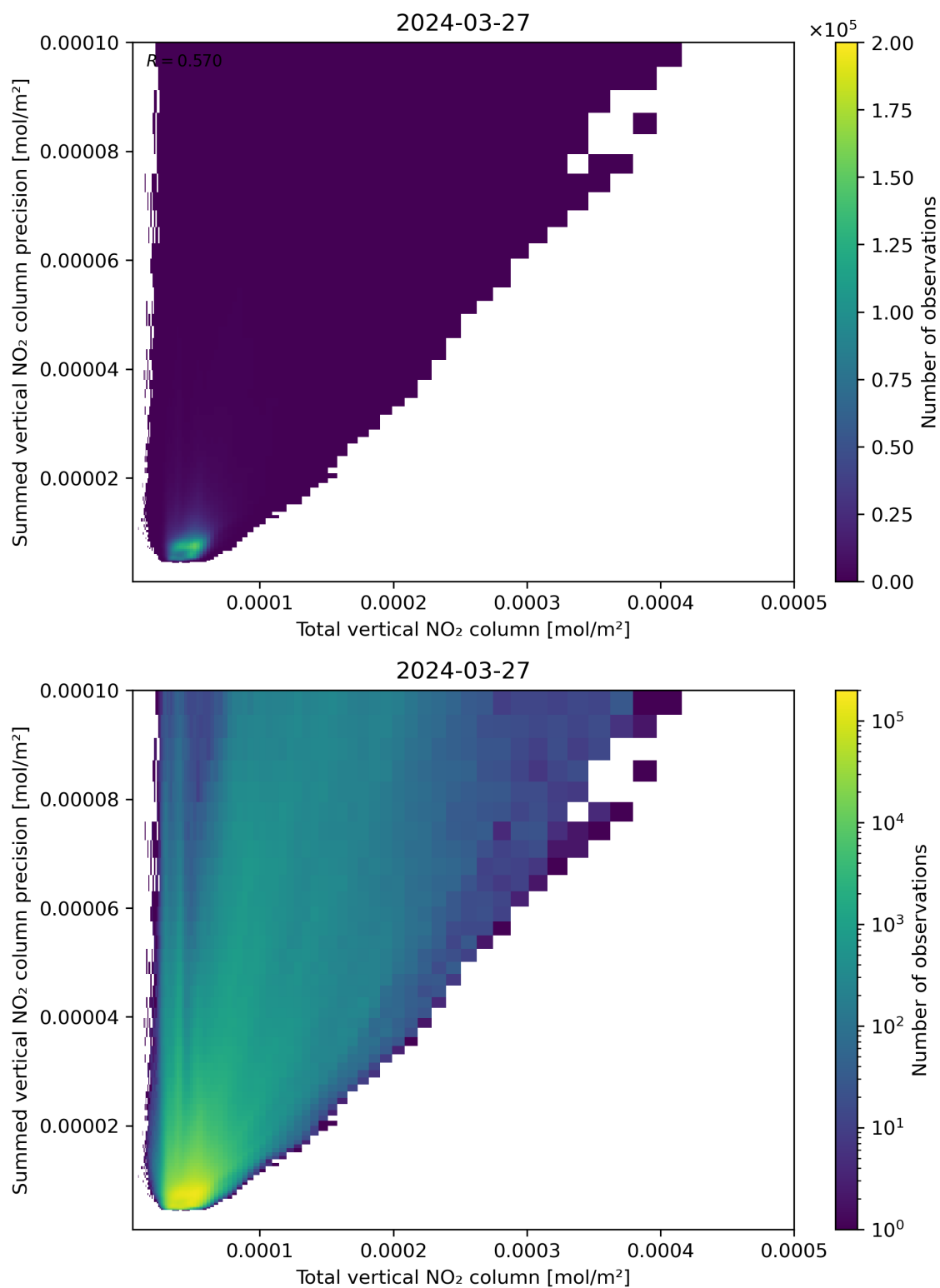
Figure 113: Scatter density plot of “Total vertical NO 2 column” against “Summed vertical NO 2 column precision” for 2024-03-26 to 2024-03-28.
