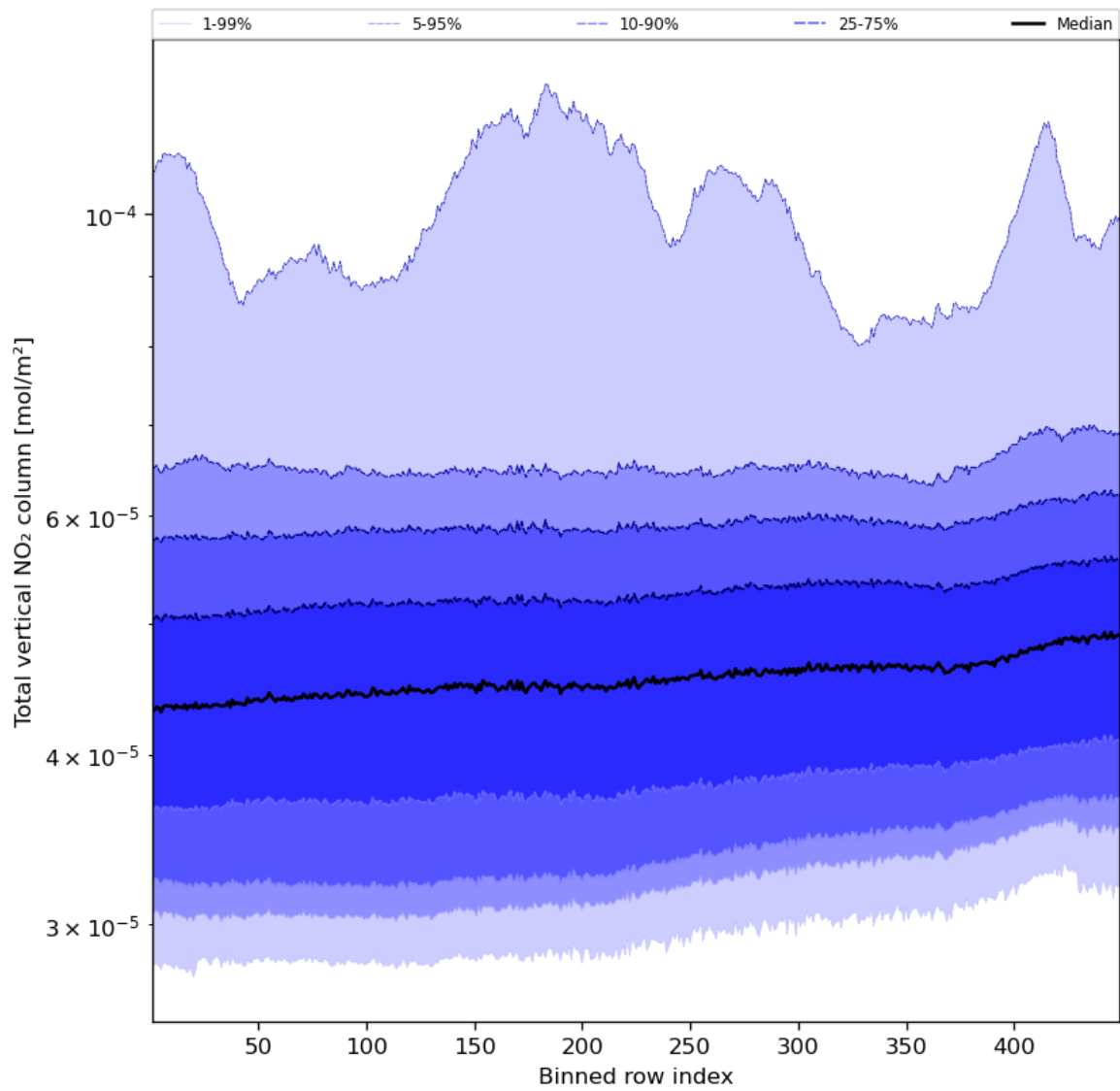
Figure 55: Along track statistics of “Total vertical NO 2 column” for 2024-03-26 to 2024-03-28
