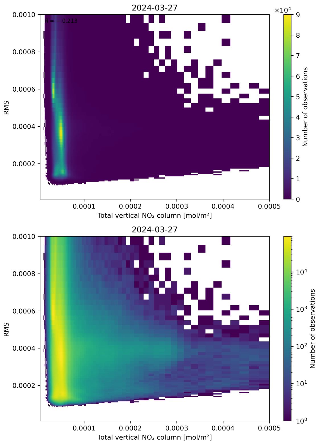
Figure 120: Scatter density plot of “Total vertical NO 2 column” against “RMS” for 2024-03-26 to 2024-03-28.
