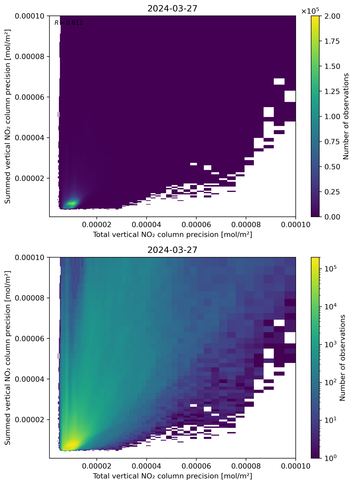
Figure 118: Scatter density plot of “Total vertical NO 2 column precision” against “Summed vertical NO 2 column precision” for 2024-03-26 to 2024-03-28.
