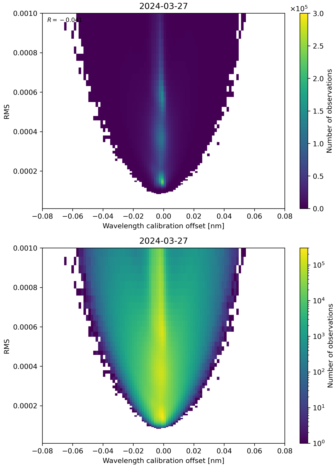
Figure 181: Scatter density plot of “Wavelength calibration offset” against “RMS” for 2024-03-26 to 2024-03-28.
