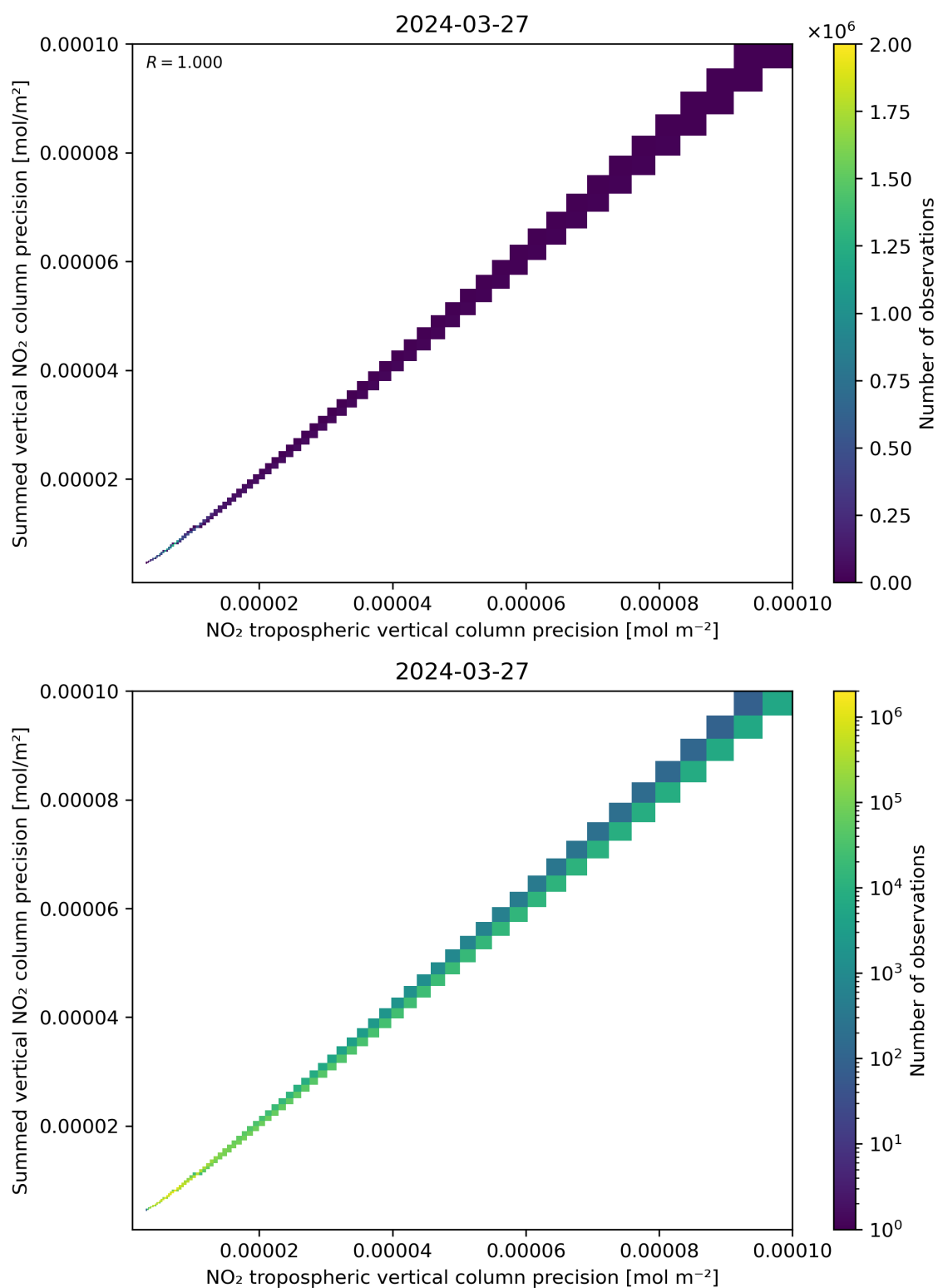
Figure 137: Scatter density plot of “NO 2 tropospheric vertical column precision” against “Summed vertical NO 2 column precision” for 2024-03-26 to 2024-03-28.
