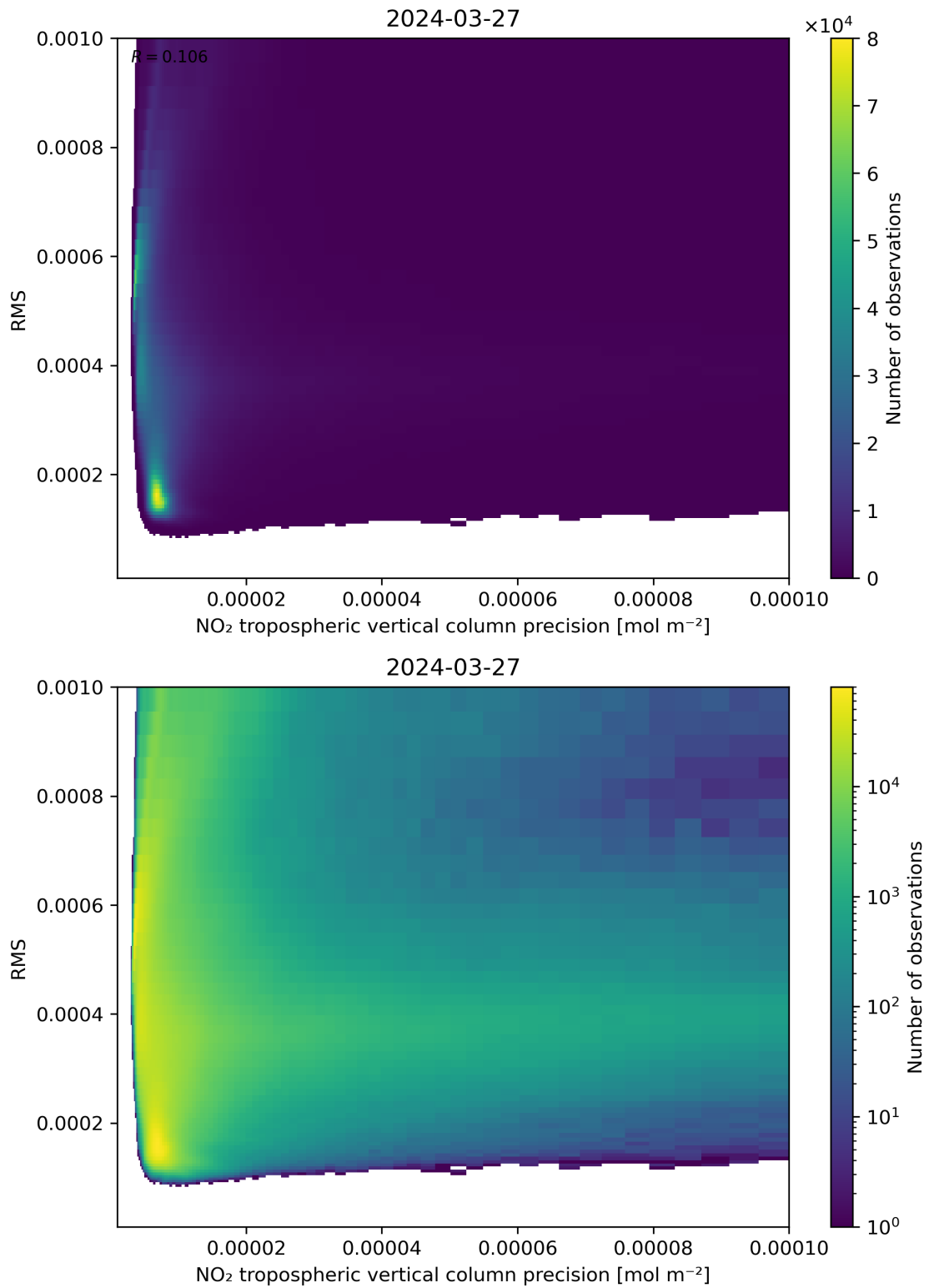
Figure 140: Scatter density plot of “NO 2 tropospheric vertical column precision” against “RMS” for 2024-03-26 to 2024-03-28.
