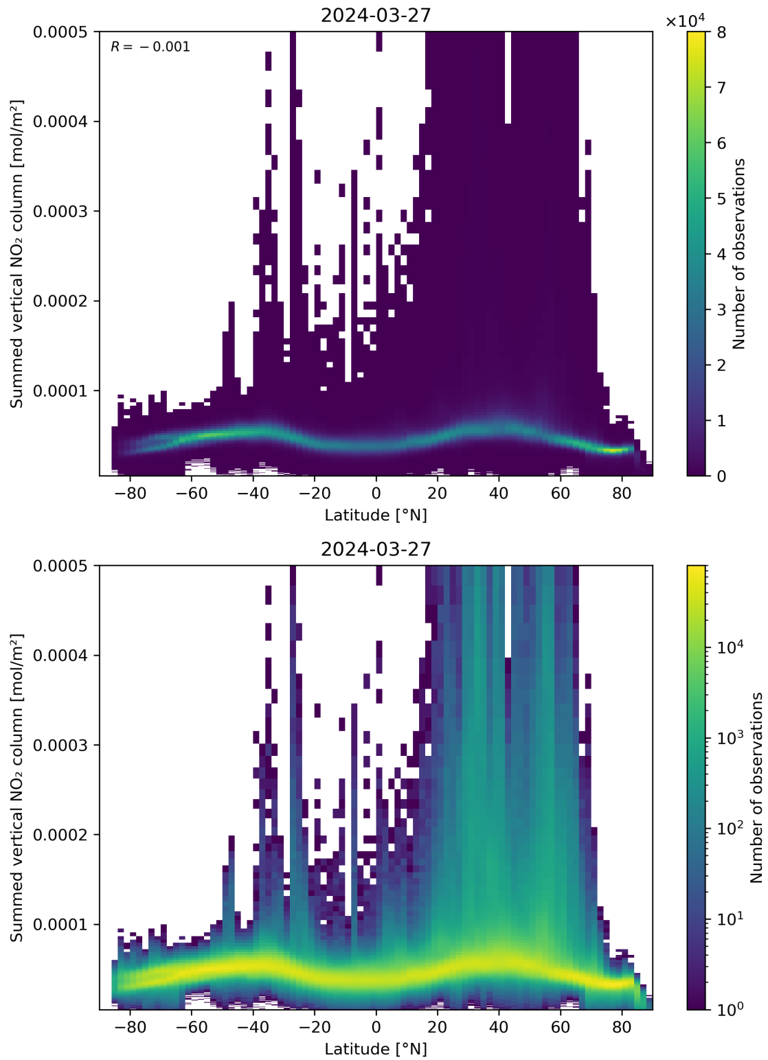
Figure 88: Scatter density plot of “Latitude” against “Summed vertical NO 2 column” for 2024-03-26 to 2024-03-28.
