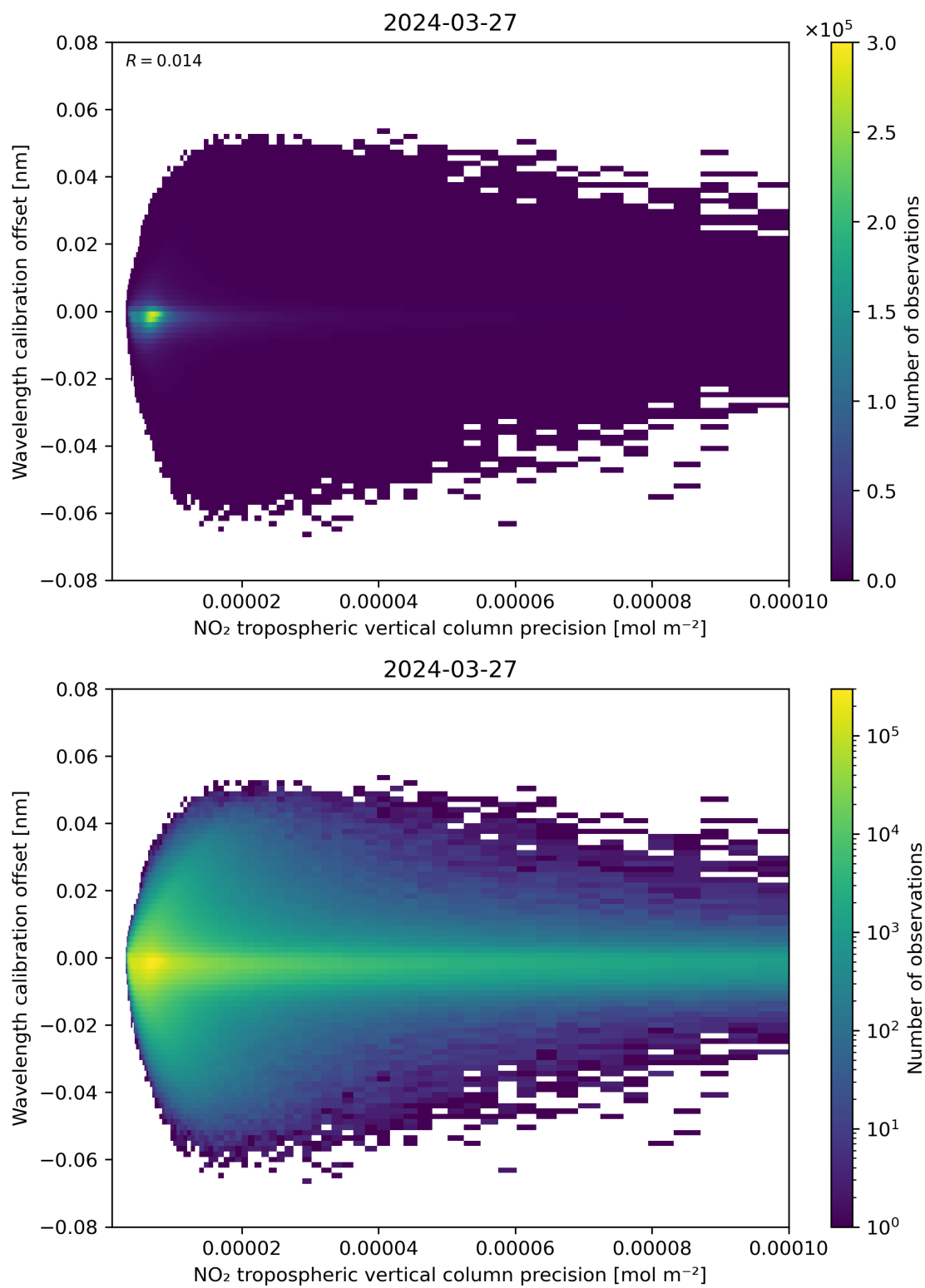
Figure 141: Scatter density plot of “NO 2 tropospheric vertical column precision” against “Wavelength calibration offset” for 2024-03-26 to 2024-03-28.
