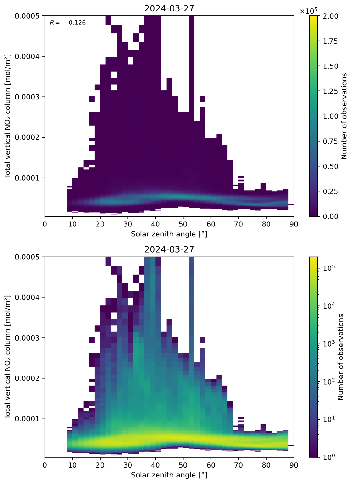
Figure 153: Scatter density plot of “Solar zenith angle” against “Total vertical NO 2 column” for 2024-03-26 to 2024-03-28.
