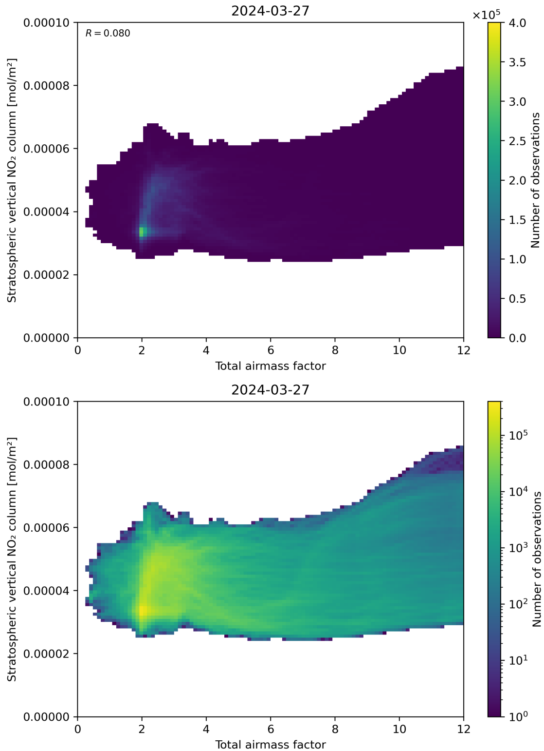
Figure 64: Scatter density plot of “Total airmass factor” against “Stratospheric vertical NO 2 column” for 2024-03-26 to 2024-03-28.
