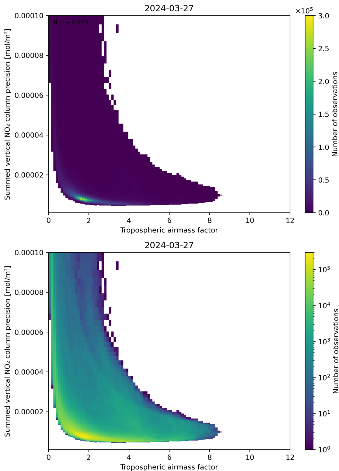
Figure 76: Scatter density plot of “Tropospheric air mass factor” against “Summed vertical NO 2 column precision” for 2024-03-26 to 2024-03-28.
