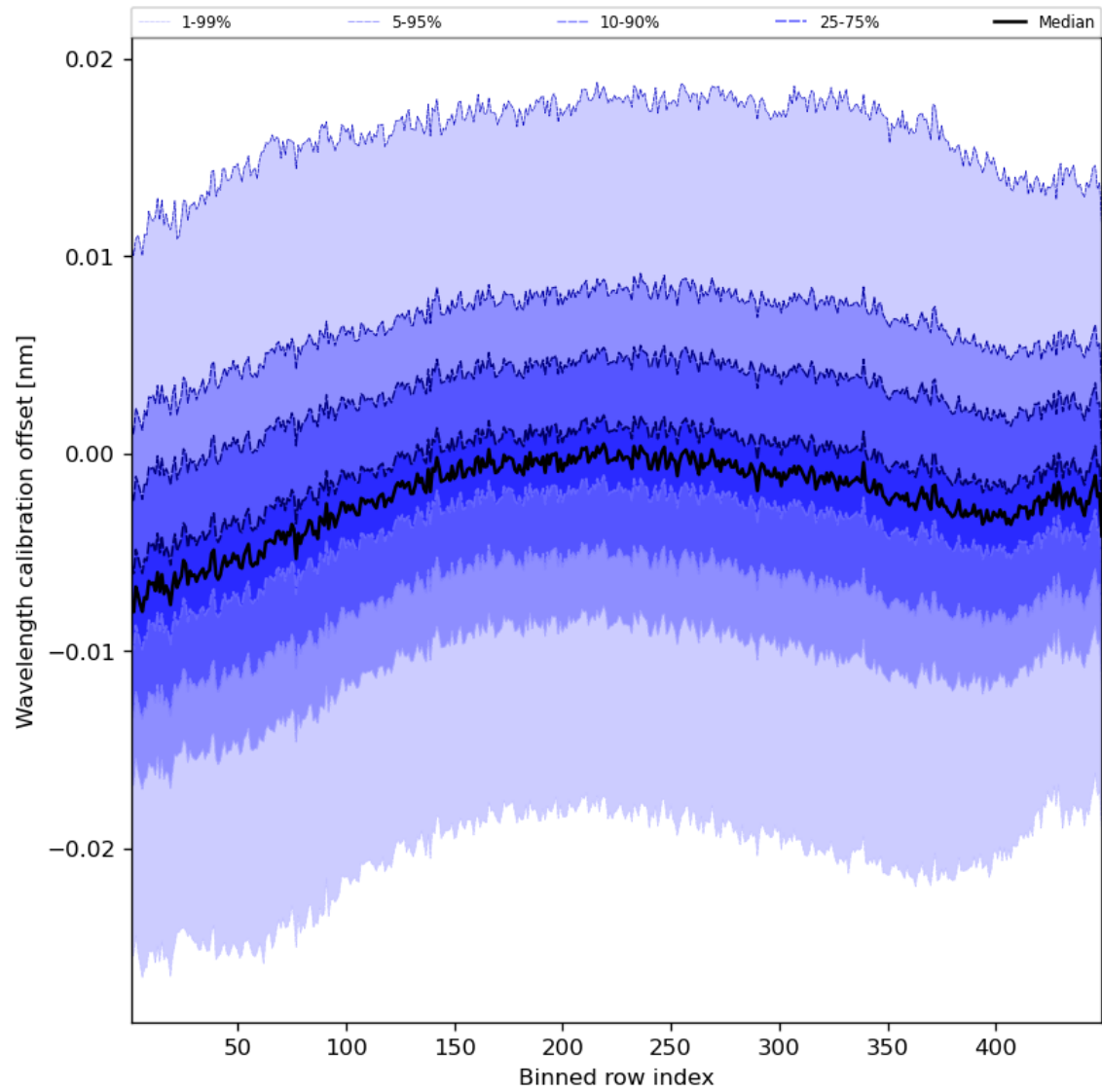
Figure 52: Along track statistics of “Wavelength calibration offset” for 2024-03-26 to 2024-03-28
