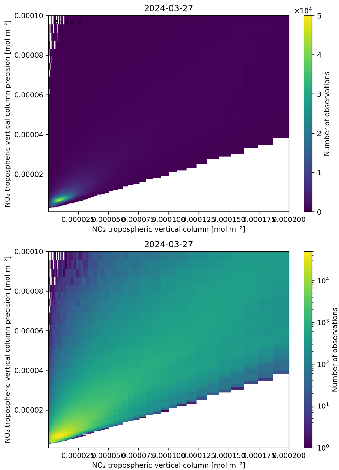
Figure 130: Scatter density plot of “NO 2 tropospheric vertical column” against “NO 2 tropospheric vertical column precision” for 2024-03-26 to 2024-03-28.
