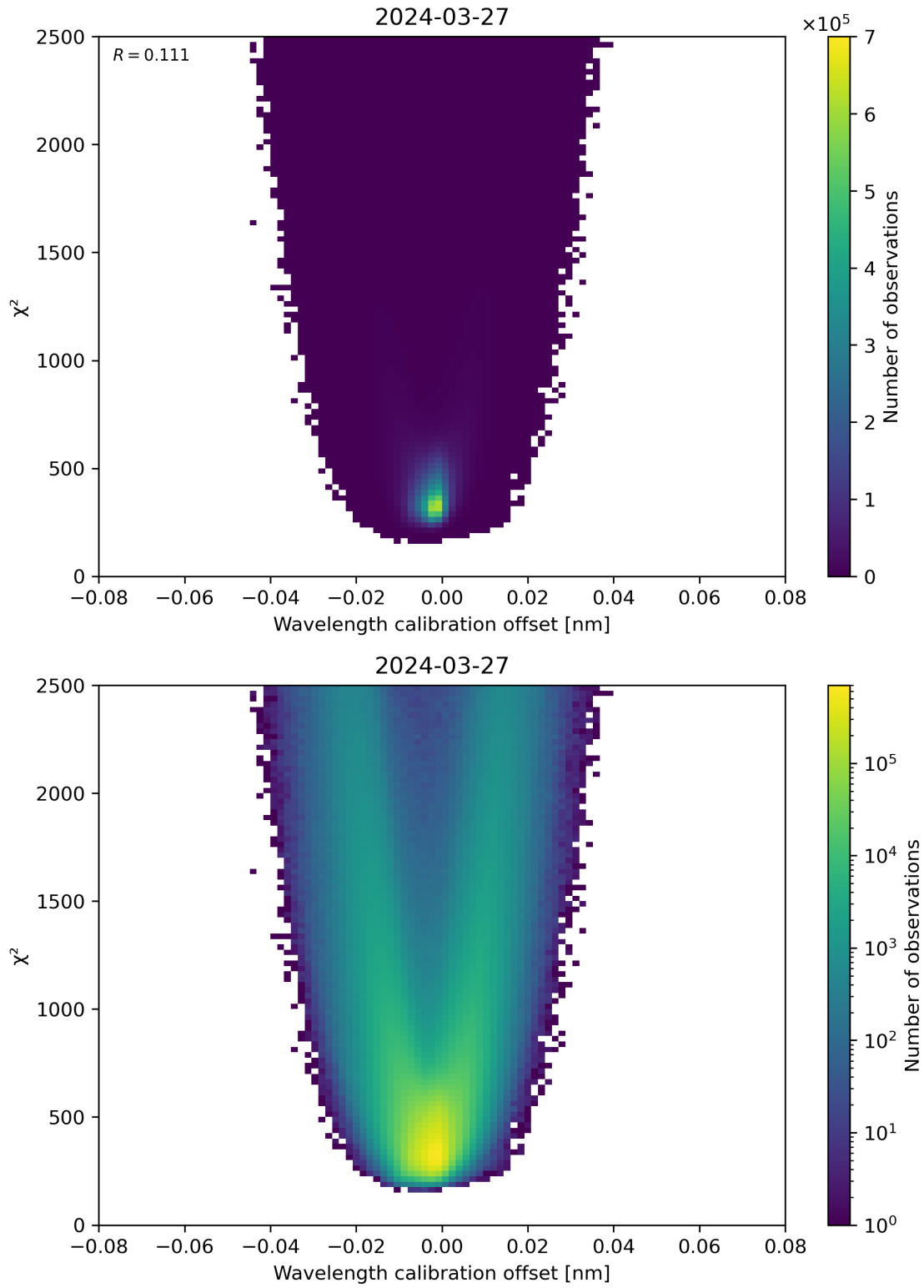
Figure 175: Scatter density plot of “Wavelength calibration offset” against “ \chi^2 ” for 2024-03-26 to 2024-03-28.
