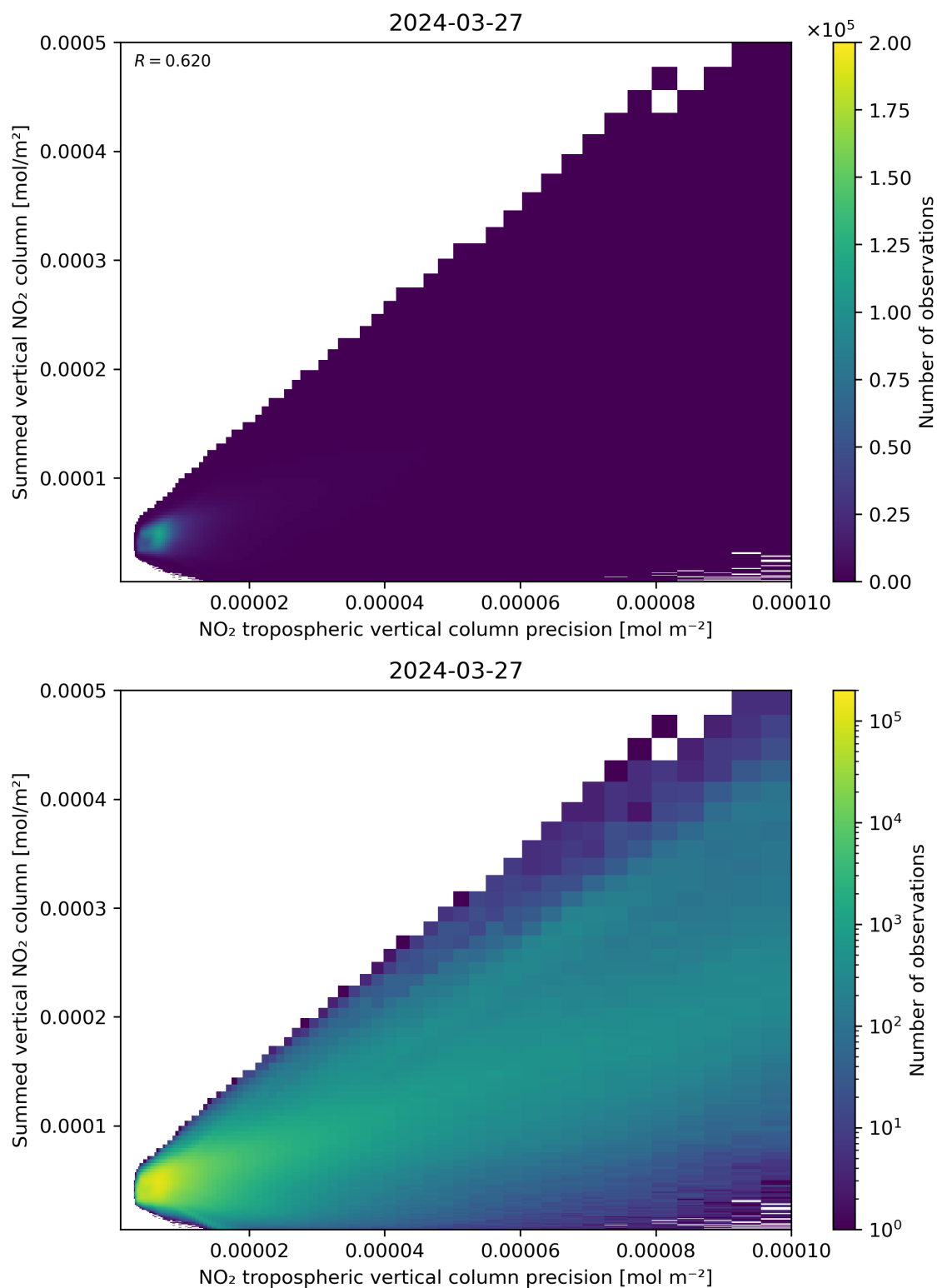
Figure 136: Scatter density plot of “NO 2 tropospheric vertical column precision” against “Summed vertical NO 2 column” for 2024-03-26 to 2024-03-28.
