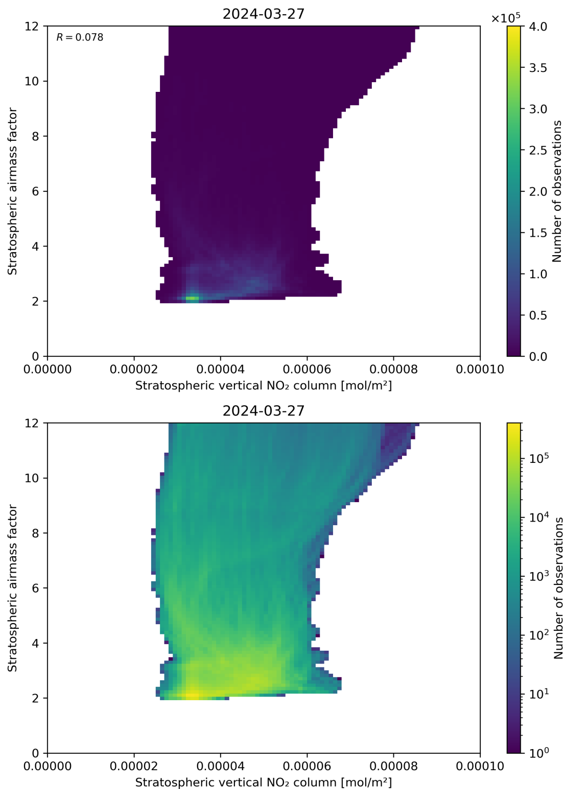
Figure 96: Scatter density plot of “Stratospheric vertical NO 2 column” against “Stratospheric airmass factor” for 2024-03-26 to 2024-03-28.
