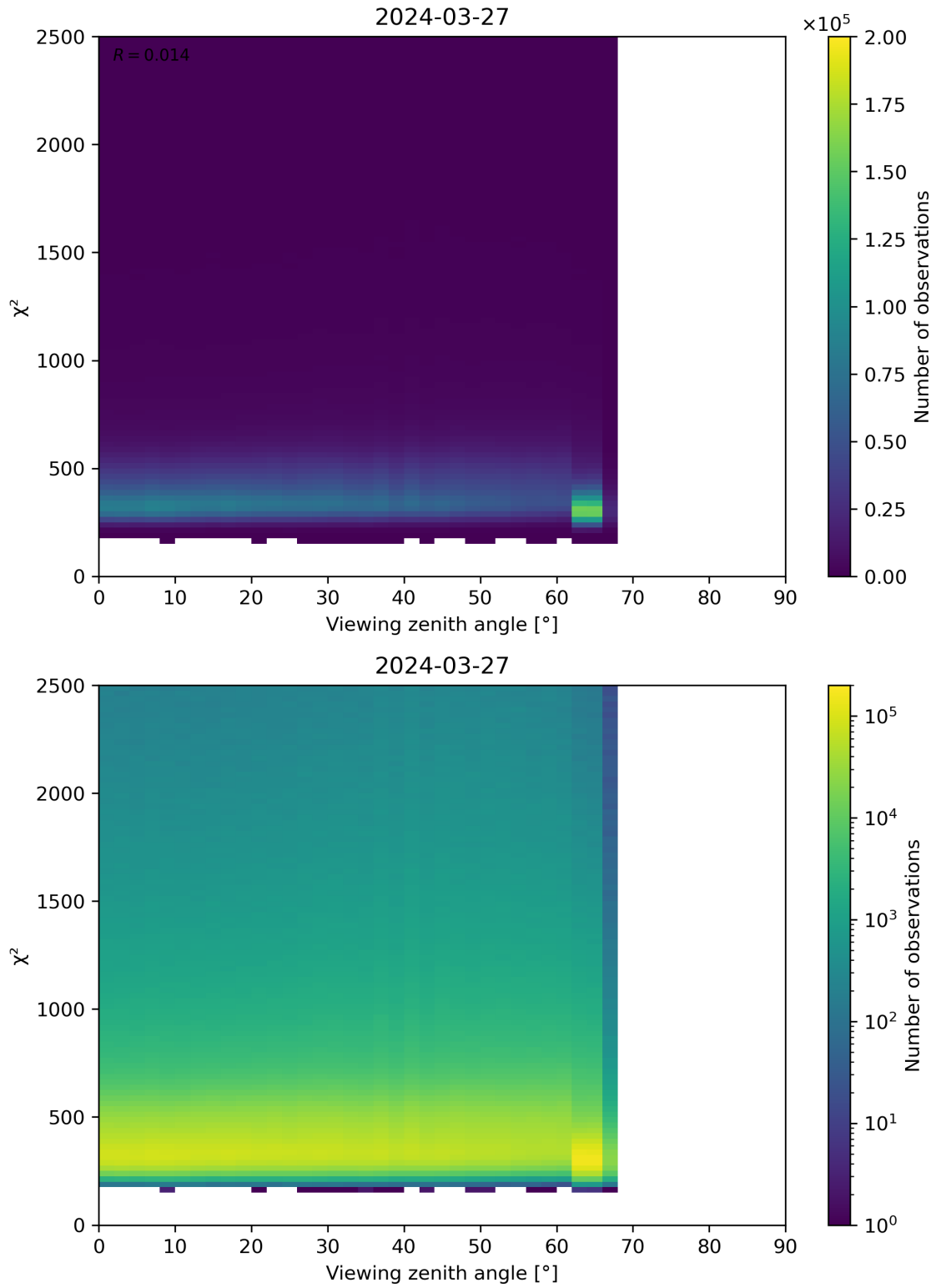
Figure 162: Scatter density plot of “Viewing zenith angle” against “ \chi^2 ” for 2024-03-26 to 2024-03-28.
