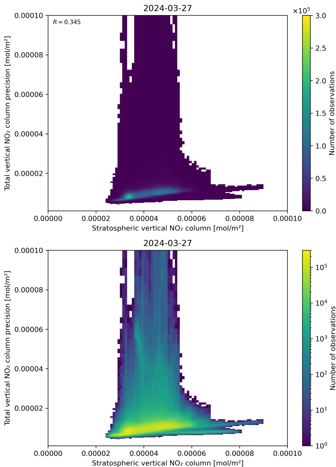
Figure 101: Scatter density plot of “Stratospheric vertical NO 2 column” against “Total vertical NO 2 column precision” for 2024-03-26 to 2024-03-28.
