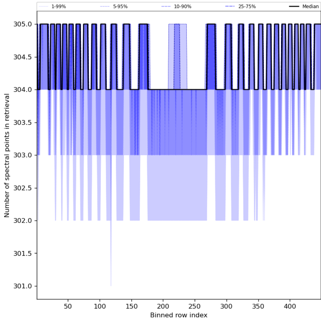
Figure 50: Along track statistics of “Number of spectral points in retrieval” for 2024-03-26 to 2024-03-28
