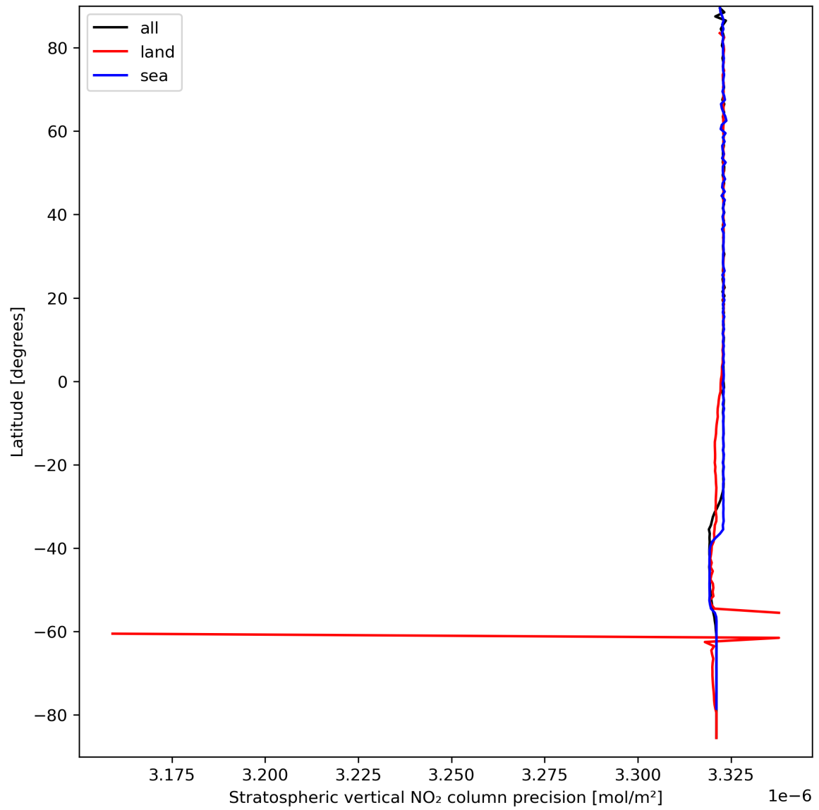
Figure 20: Zonal average of “Stratospheric vertical NO 2 column precision” for 2024-03-26 to 2024-03-28.
