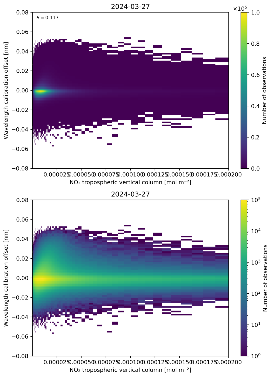
Figure 143: Scatter density plot of “NO 2 tropospheric vertical column” against “Wavelength calibration offset” for 2024-03-26 to 2024-03-28.
