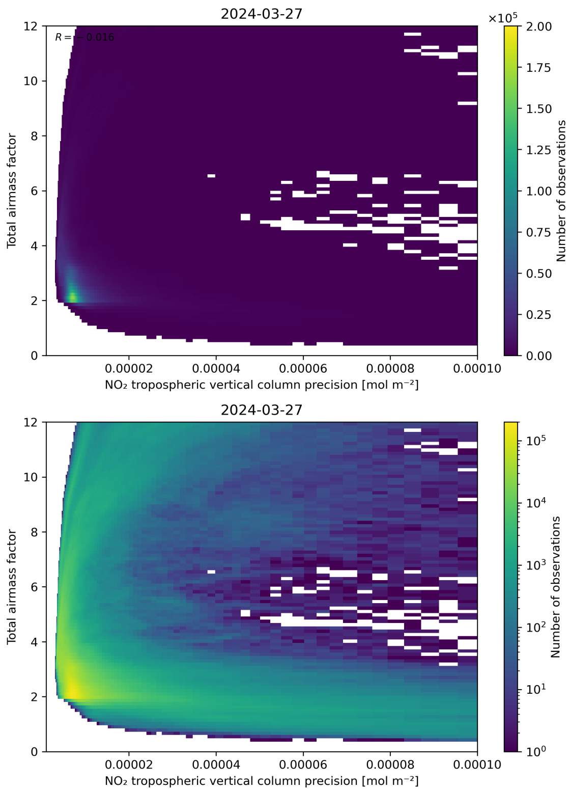
Figure 132: Scatter density plot of “NO 2 tropospheric vertical column precision” against “Total air mass factor” for 2024-03-26 to 2024-03-28.
