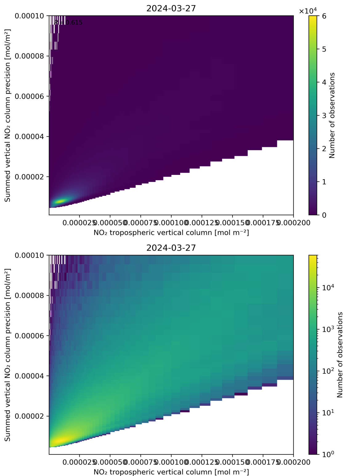
Figure 127: Scatter density plot of “NO 2 tropospheric vertical column” against “Summed vertical NO 2 column precision” for 2024-03-26 to 2024-03-28.
