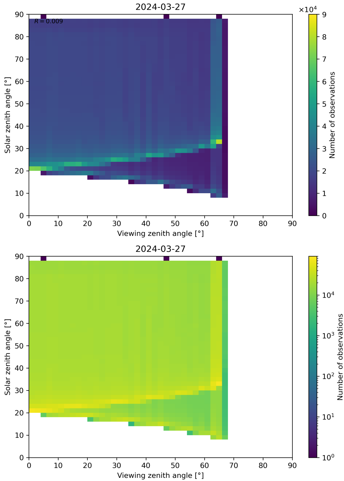
Figure 172: Scatter density plot of “Viewing zenith angle” against “Solar zenith angle” for 2024-03-26 to 2024-03-28.
