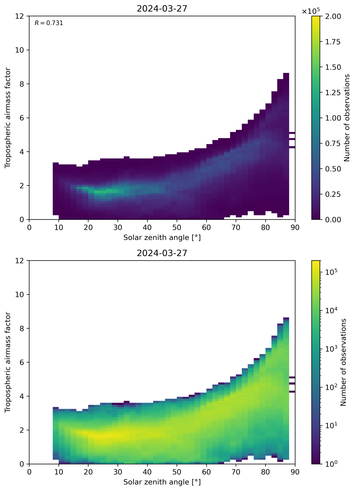
Figure 147: Scatter density plot of “Solar zenith angle” against “Tropospheric airmass factor” for 2024-03-26 to 2024-03-28.
