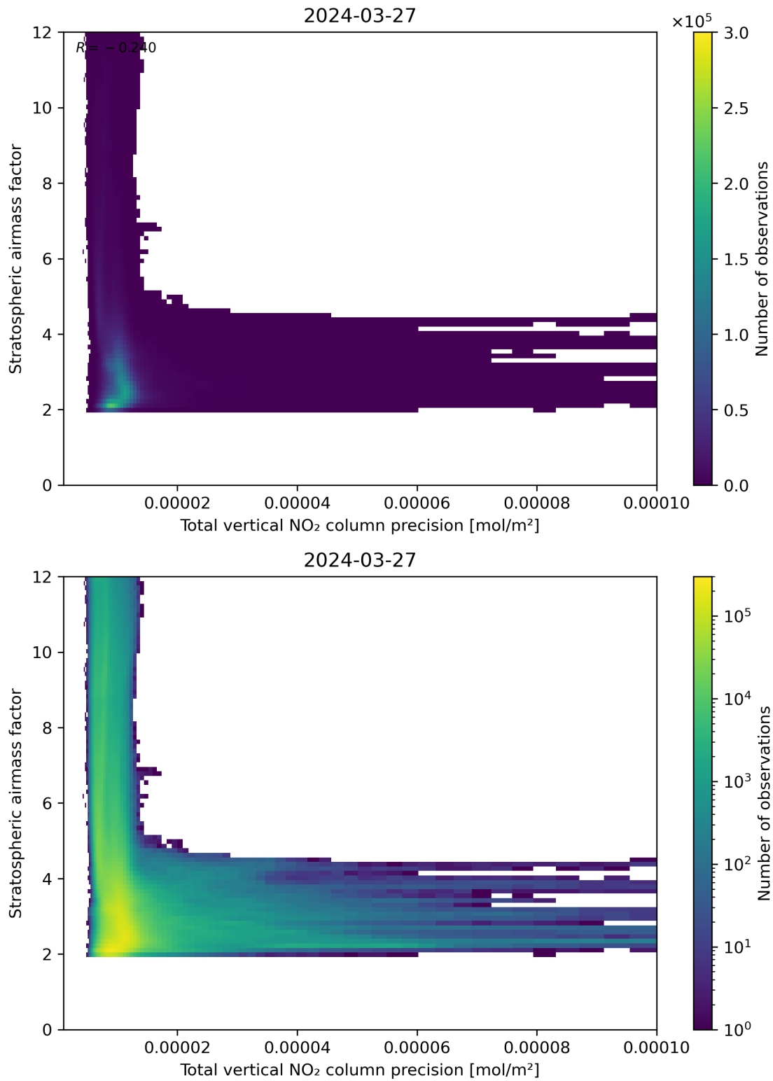
Figure 115: Scatter density plot of “Total vertical NO 2 column precision” against “Stratospheric air mass factor” for 2024-03-26 to 2024-03-28.
