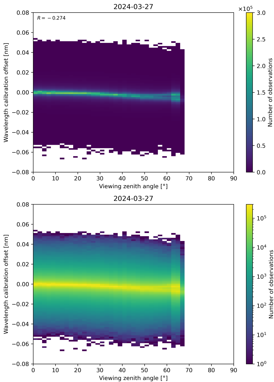
Figure 173: Scatter density plot of “Viewing zenith angle” against “Wavelength calibration offset” for 2024-03-26 to 2024-03-28.
