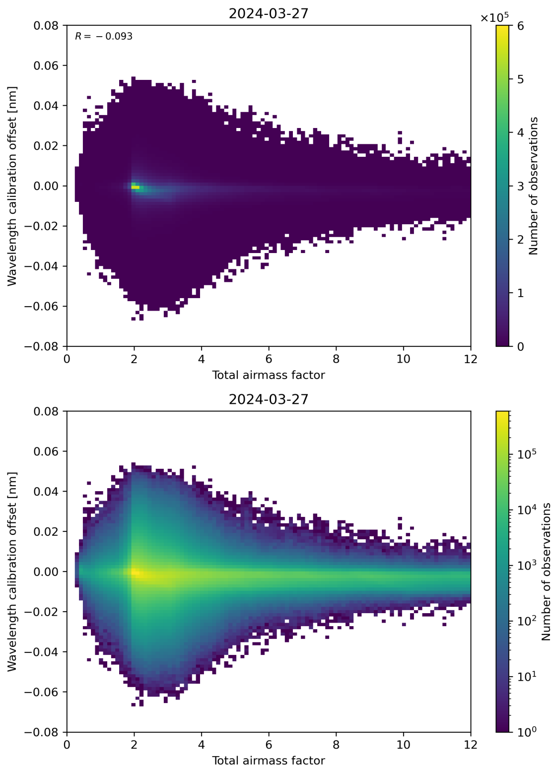
Figure 70: Scatter density plot of “Total airmass factor” against “Wavelength calibration offset” for 2024-03-26 to 2024-03-28.
