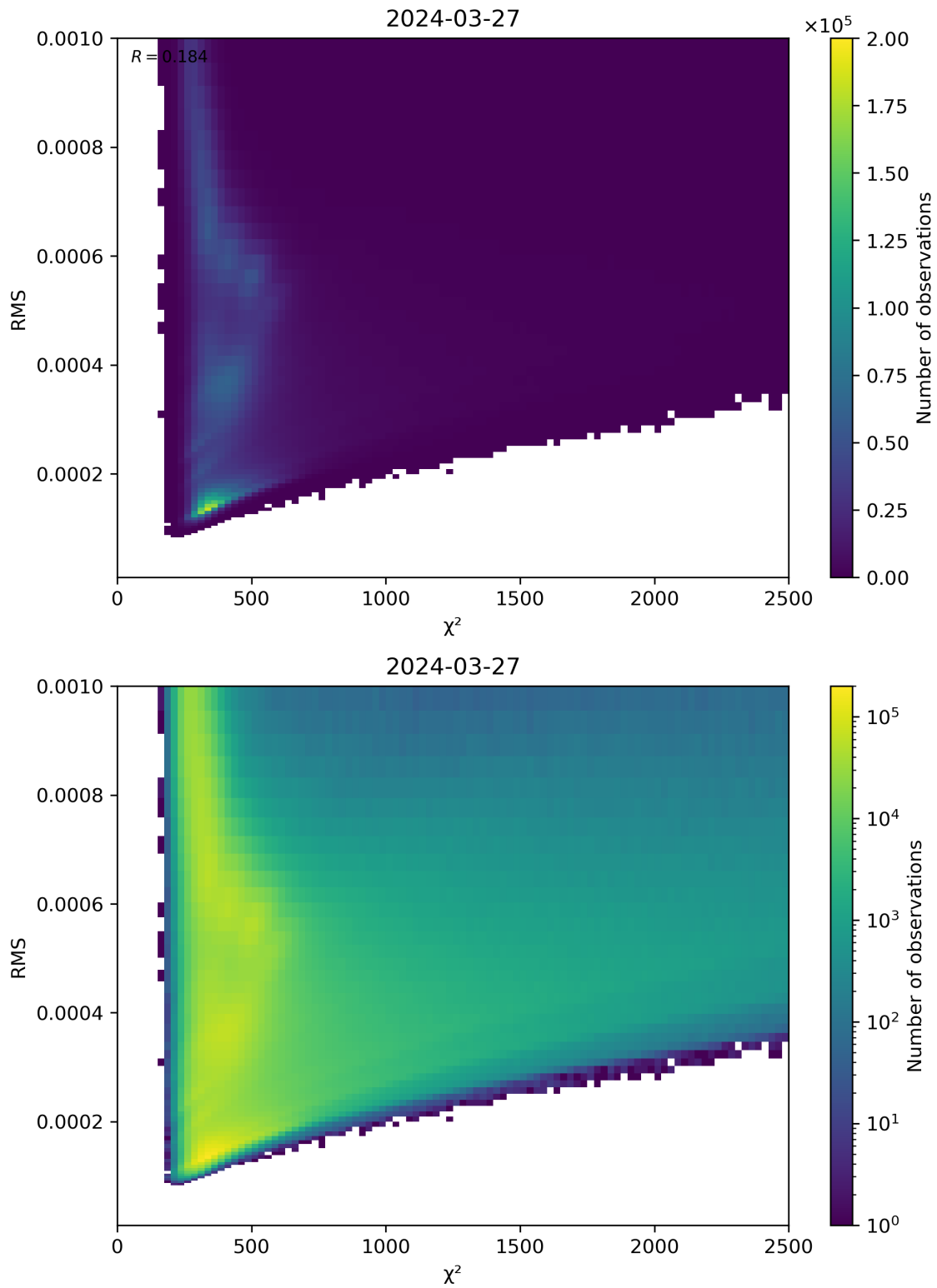
Figure 82: Scatter density plot of “ \chi^2 ” against “RMS” for 2024-03-26 to 2024-03-28.
