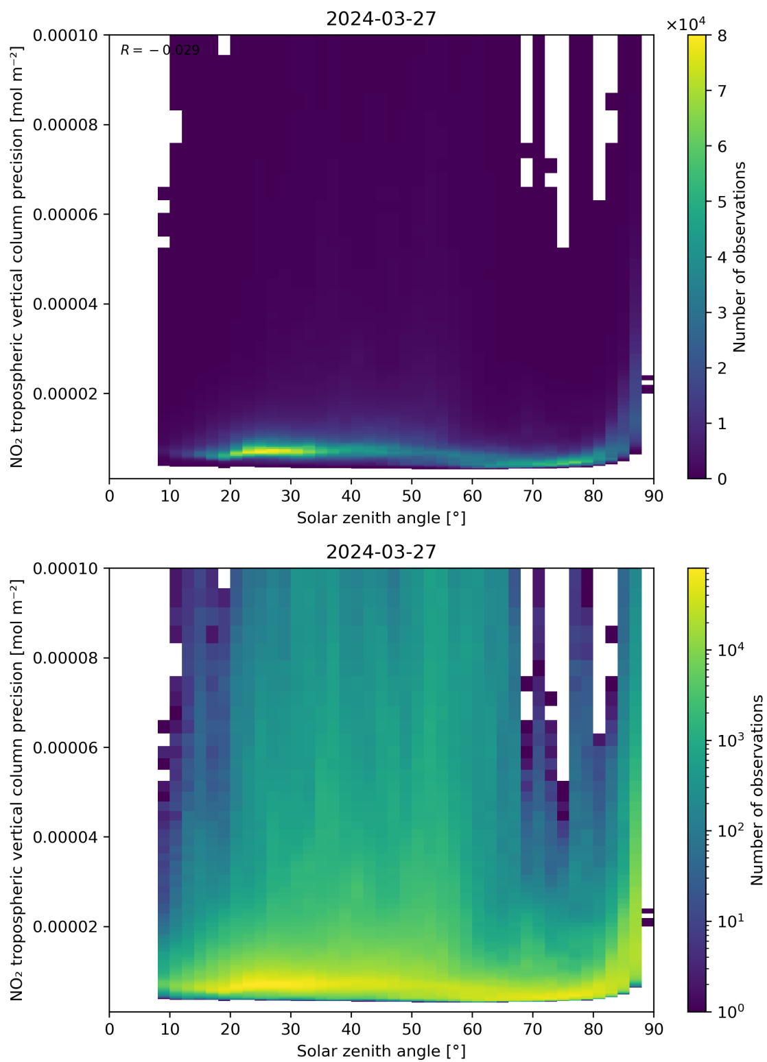
Figure 156: Scatter density plot of “Solar zenith angle” against “NO 2 tropospheric vertical column precision” for 2024-03-26 to 2024-03-28.
