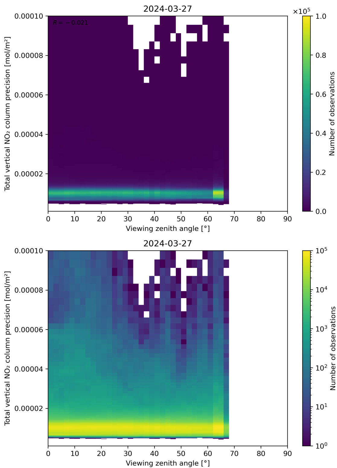
Figure 168: Scatter density plot of “Viewing zenith angle” against “Total vertical NO 2 column precision” for 2024-03-26 to 2024-03-28.
