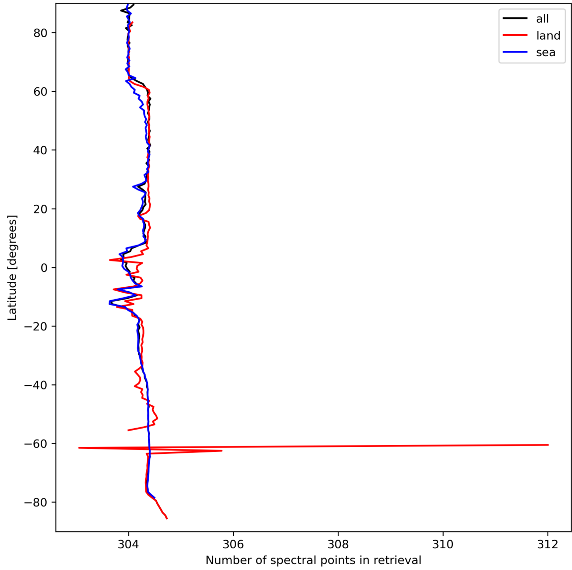
Figure 16: Zonal average of “Number of spectral points in retrieval” for 2024-03-26 to 2024-03-28.
