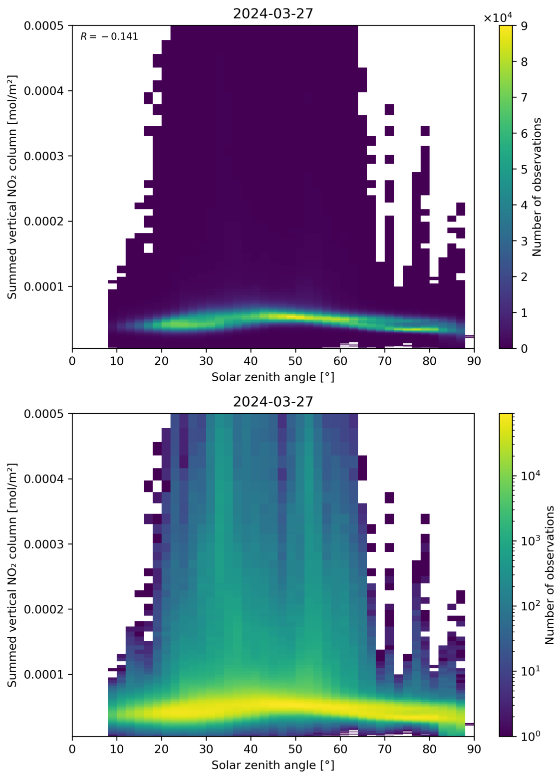
Figure 151: Scatter density plot of “Solar zenith angle” against “Summed vertical NO 2 column” for 2024-03-26 to 2024-03-28.
