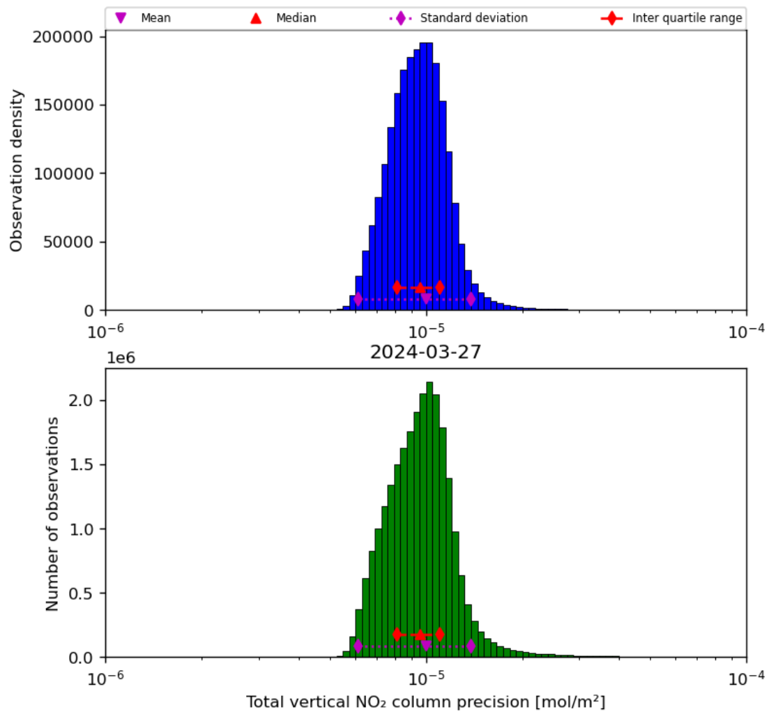
Figure 39: Histogram of "Total vertical NO 2 column precision" for 2024-03-26 to 2024-03-28
