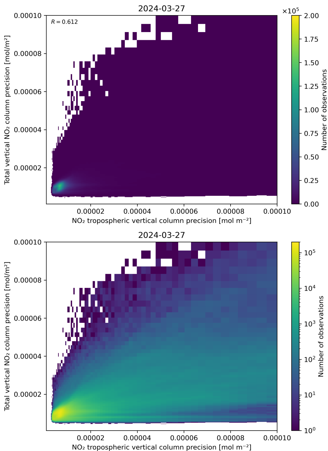
Figure 139: Scatter density plot of “NO 2 tropospheric vertical column precision” against “Total vertical NO 2 column precision” for 2024-03-26 to 2024-03-28.
