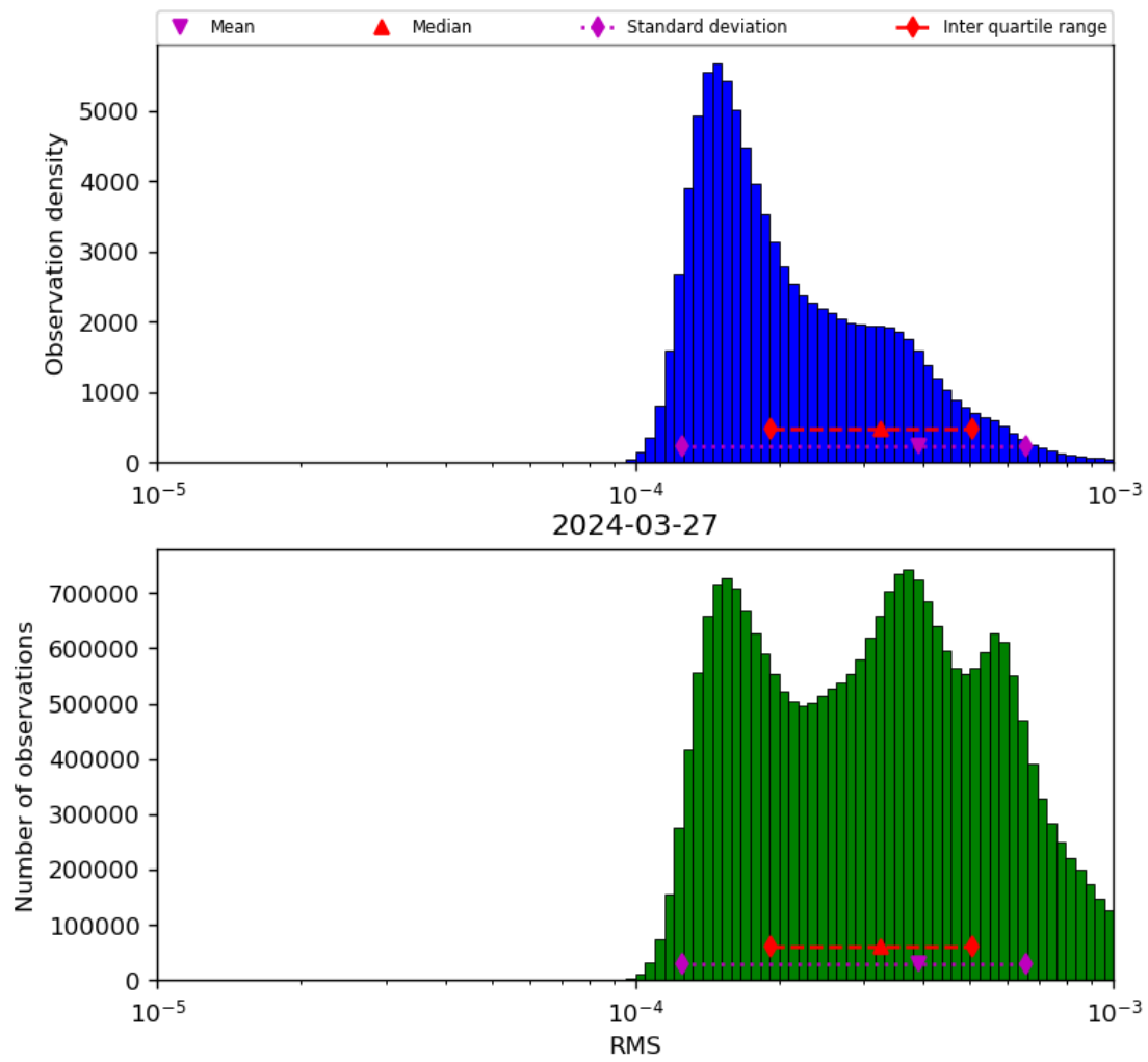
Figure 43: Histogram of “RMS” for 2024-03-26 to 2024-03-28
