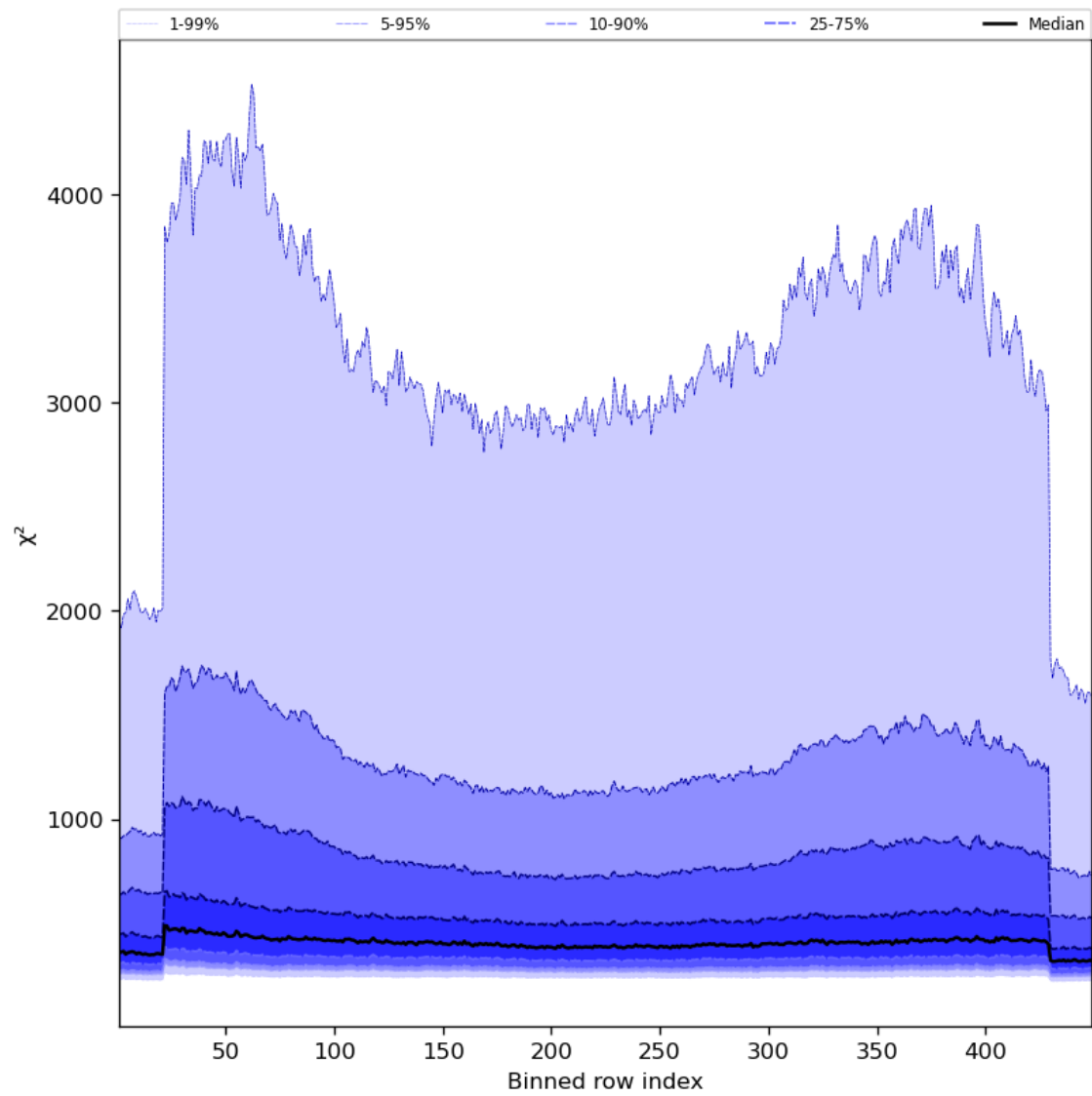
Figure 59: Along track statistics of “ \chi^2 ” for 2024-03-26 to 2024-03-28
