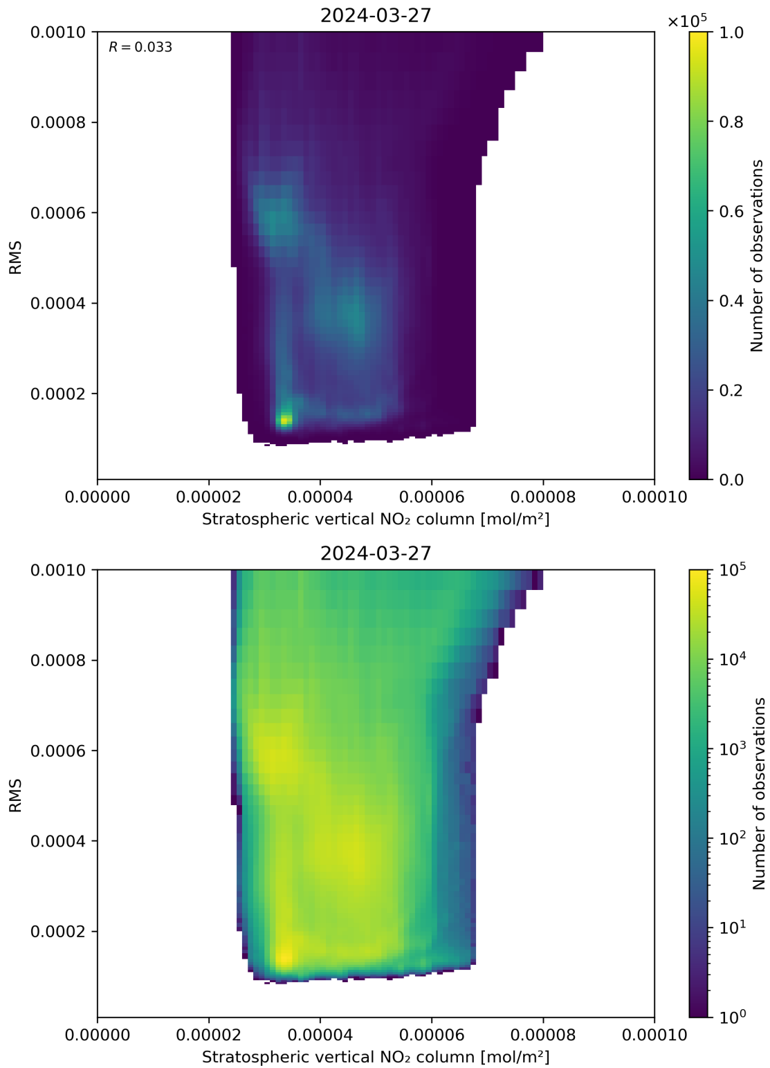
Figure 102: Scatter density plot of “Stratospheric vertical NO 2 column” against “RMS” for 2024-03-26 to 2024-03-28.
