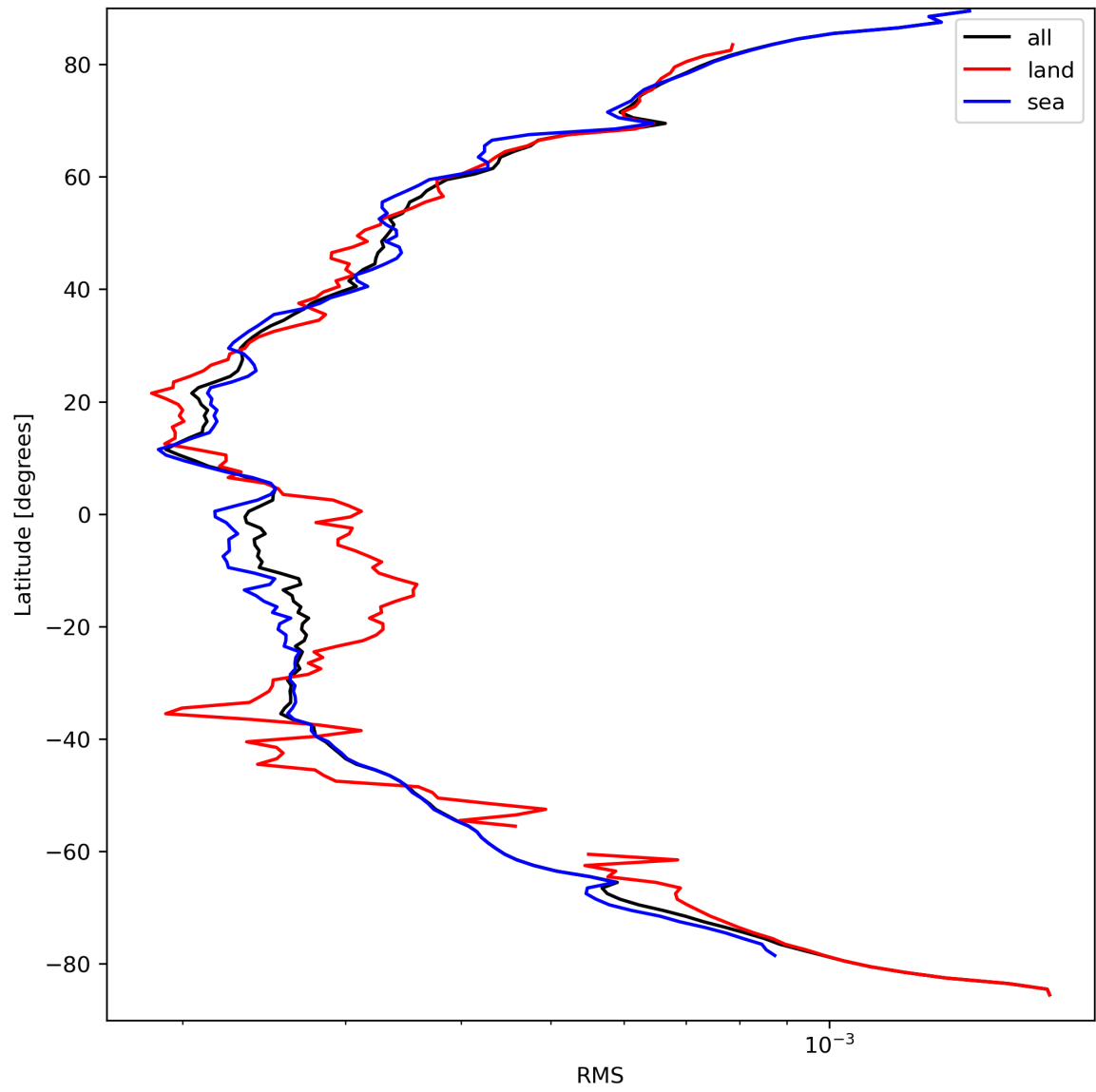
Figure 26: Zonal average of “RMS” for 2024-03-26 to 2024-03-28.
