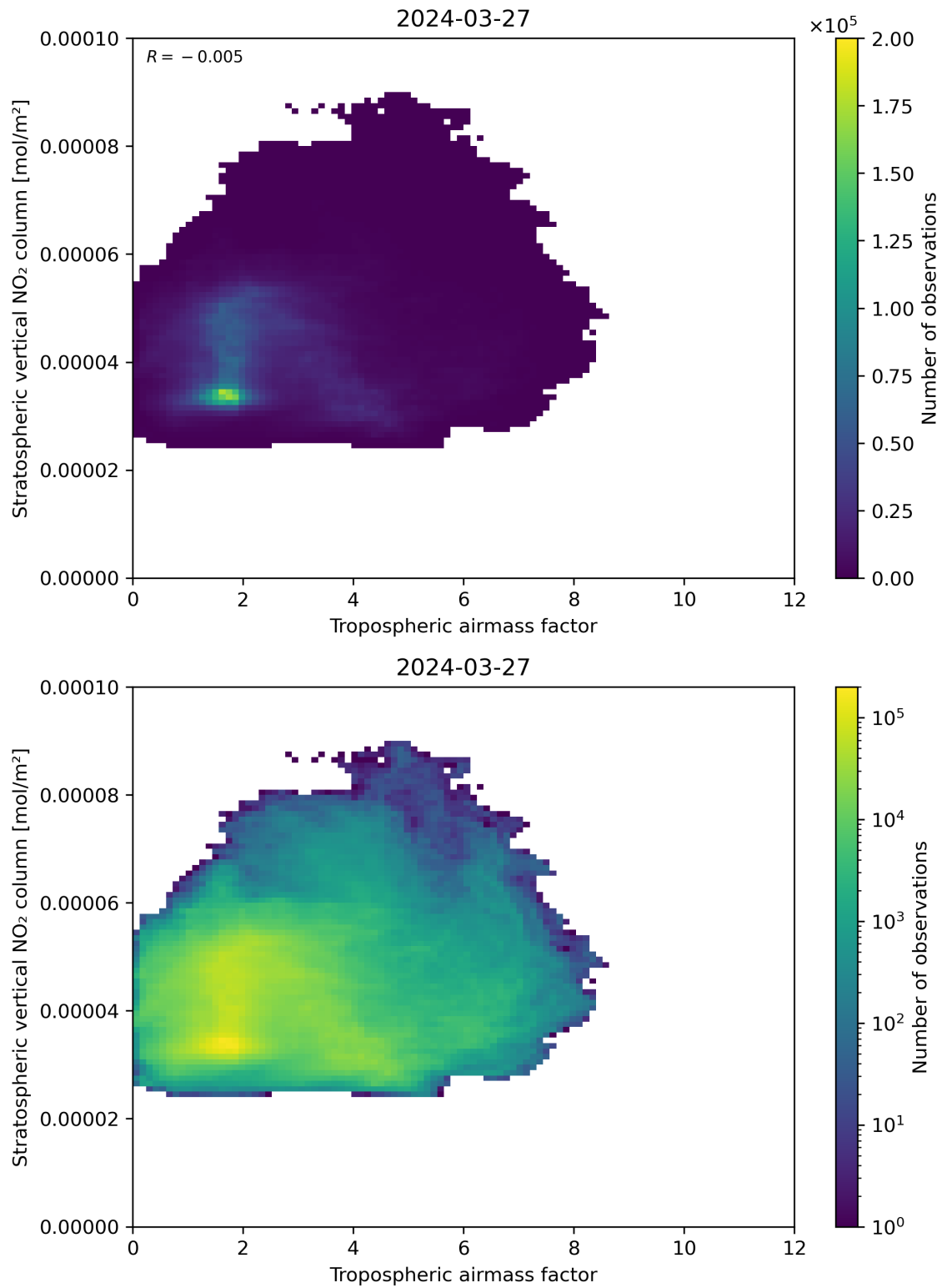
Figure 74: Scatter density plot of “Tropospheric air mass factor” against “Stratospheric vertical NO 2 column” for 2024-03-26 to 2024-03-28.
