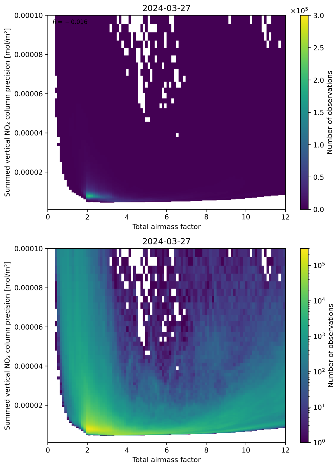
Figure 66: Scatter density plot of “Total airmass factor” against “Summed vertical NO 2 column precision” for 2024-03-26 to 2024-03-28.
