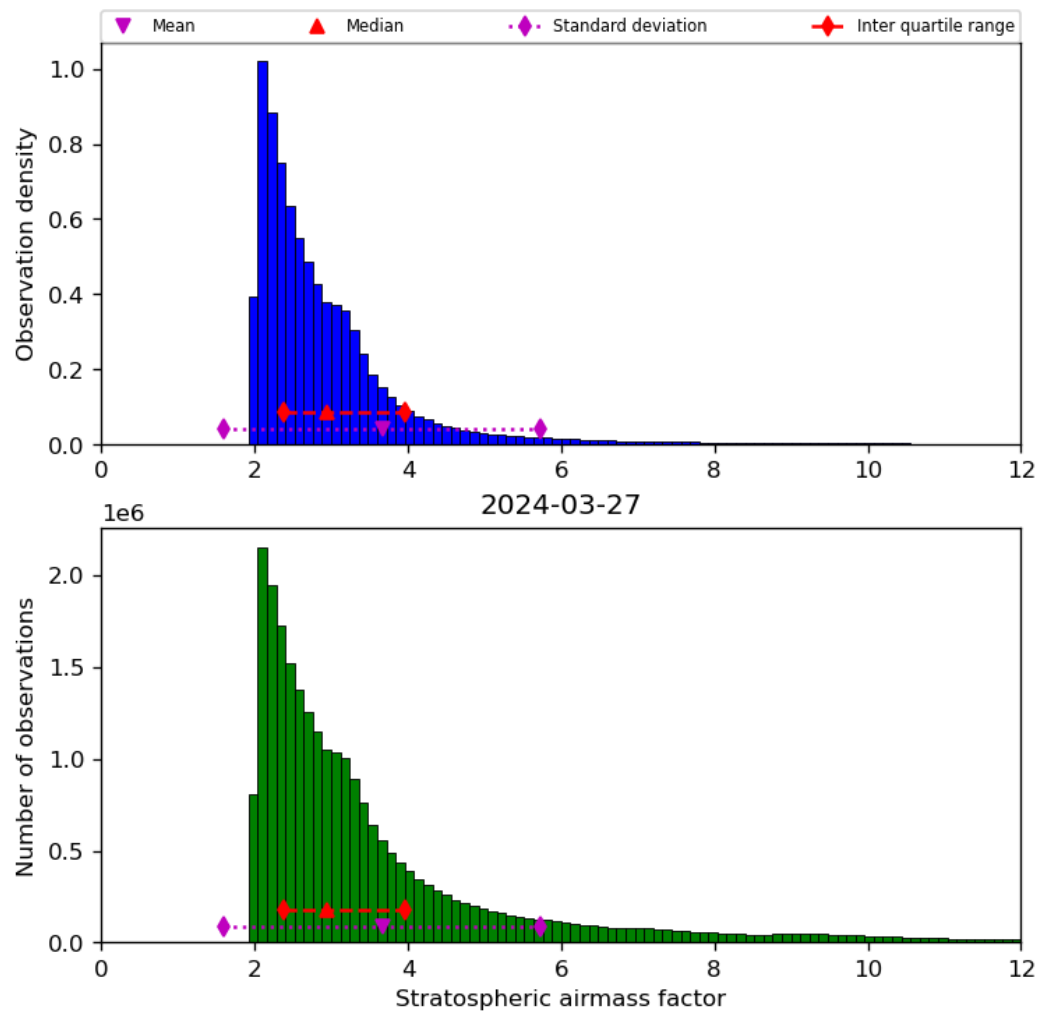
Figure 44: Histogram of “Stratospheric airmass factor” for 2024-03-26 to 2024-03-28
