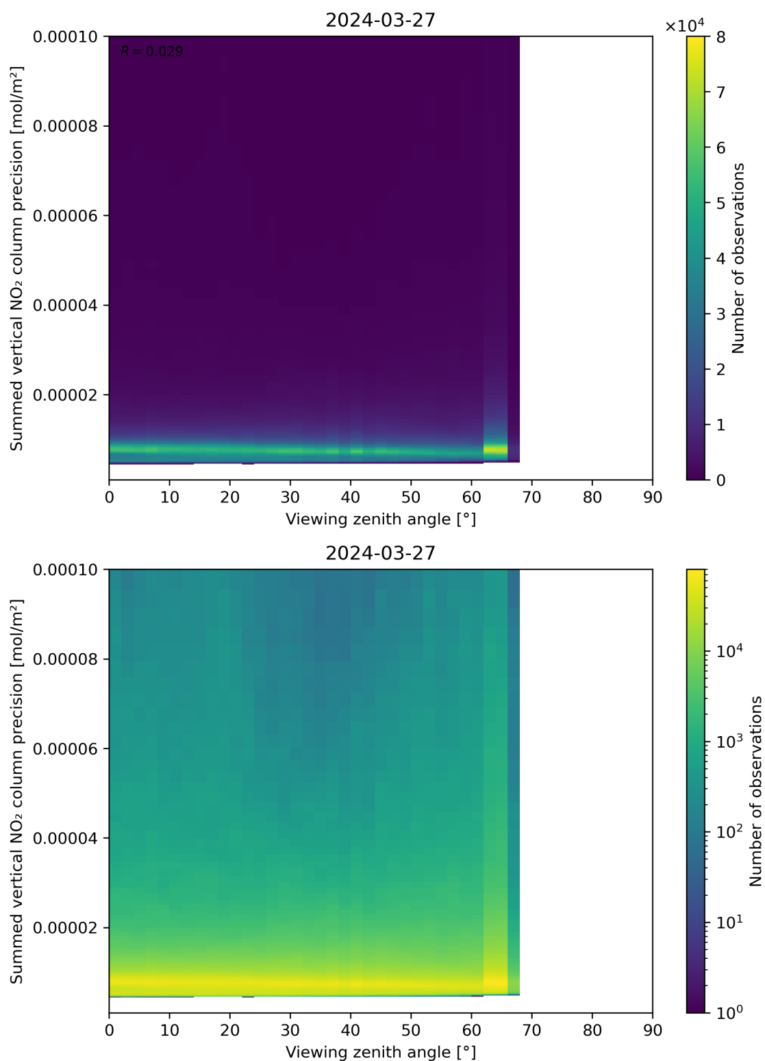
Figure 166: Scatter density plot of “Viewing zenith angle” against “Summed vertical NO 2 column precision” for 2024-03-26 to 2024-03-28.
