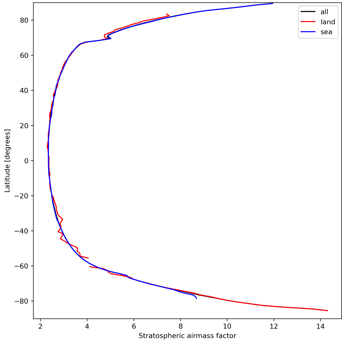
Figure 27: Zonal average of “Stratospheric airmass factor” for 2024-03-26 to 2024-03-28.
