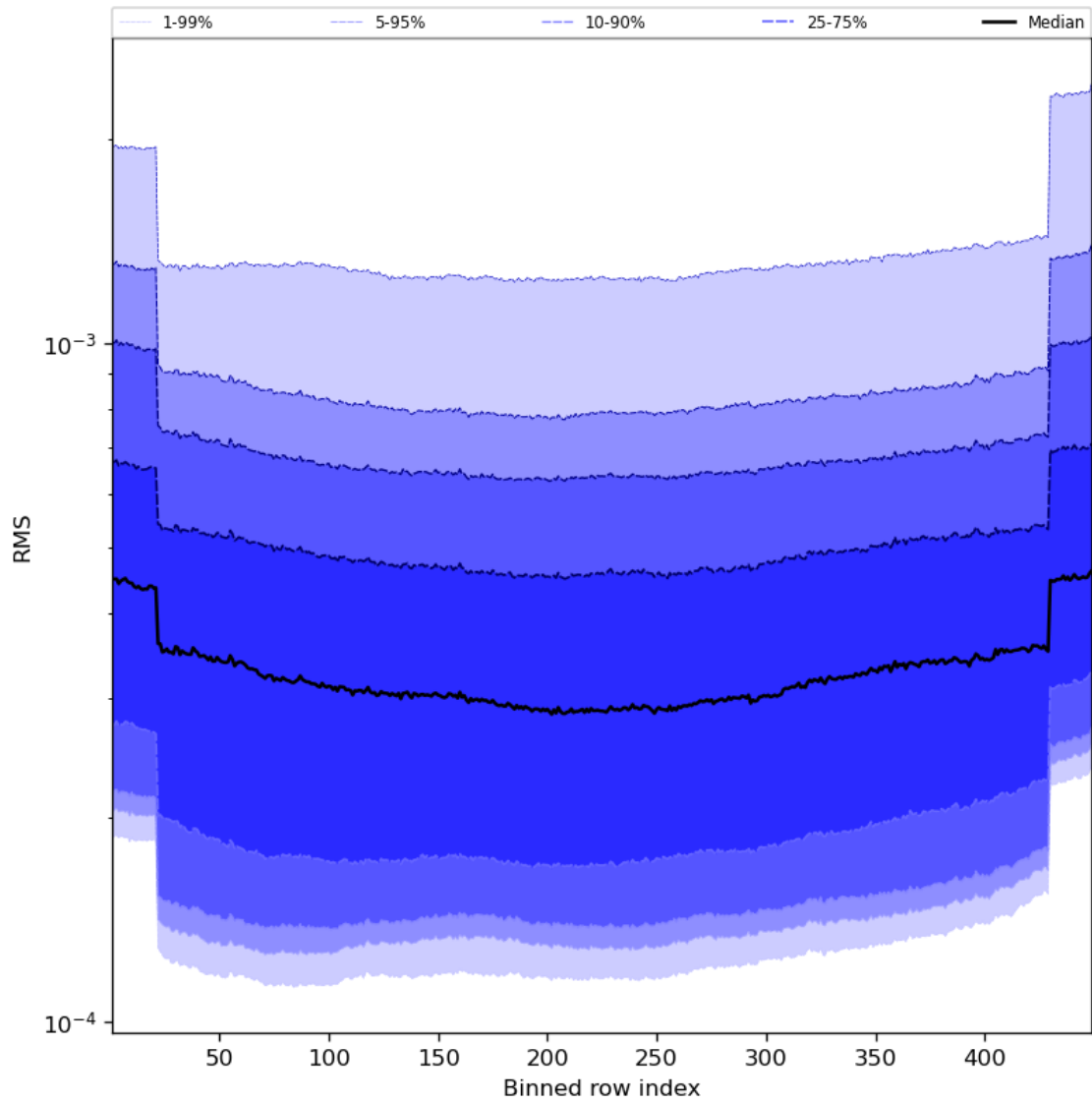
Figure 60: Along track statistics of “RMS” for 2024-03-26 to 2024-03-28
