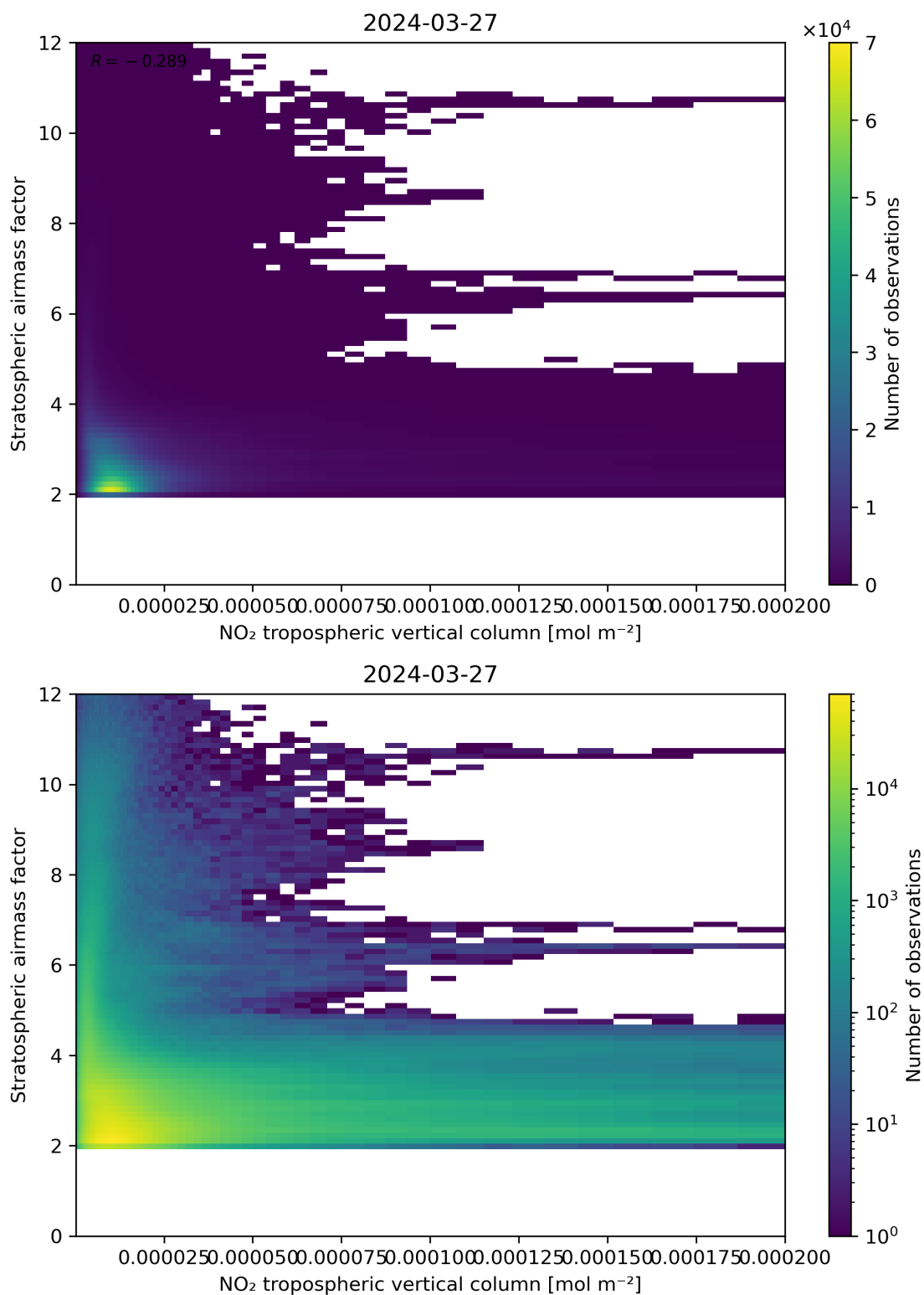
Figure 121: Scatter density plot of “NO 2 tropospheric vertical column” against “Stratospheric air mass factor” for 2024-03-26 to 2024-03-28.
