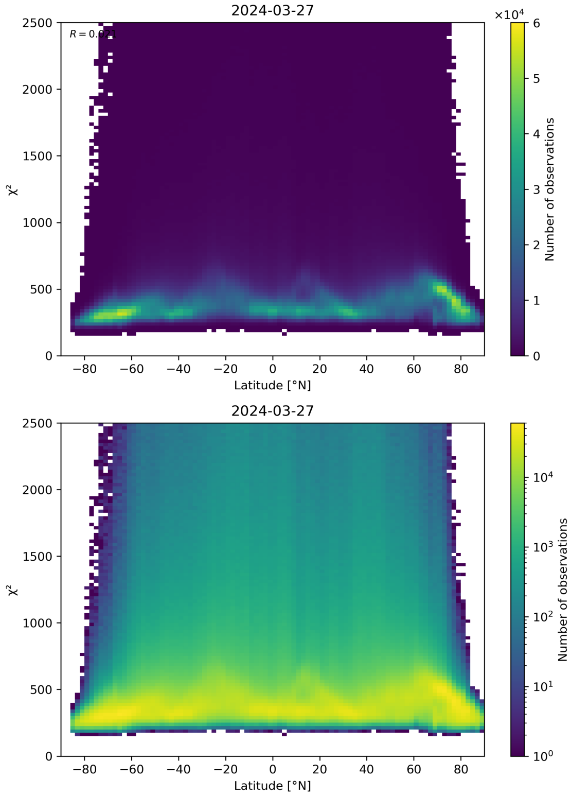
Figure 86: Scatter density plot of “Latitude” against “ \chi^2 ” for 2024-03-26 to 2024-03-28.
