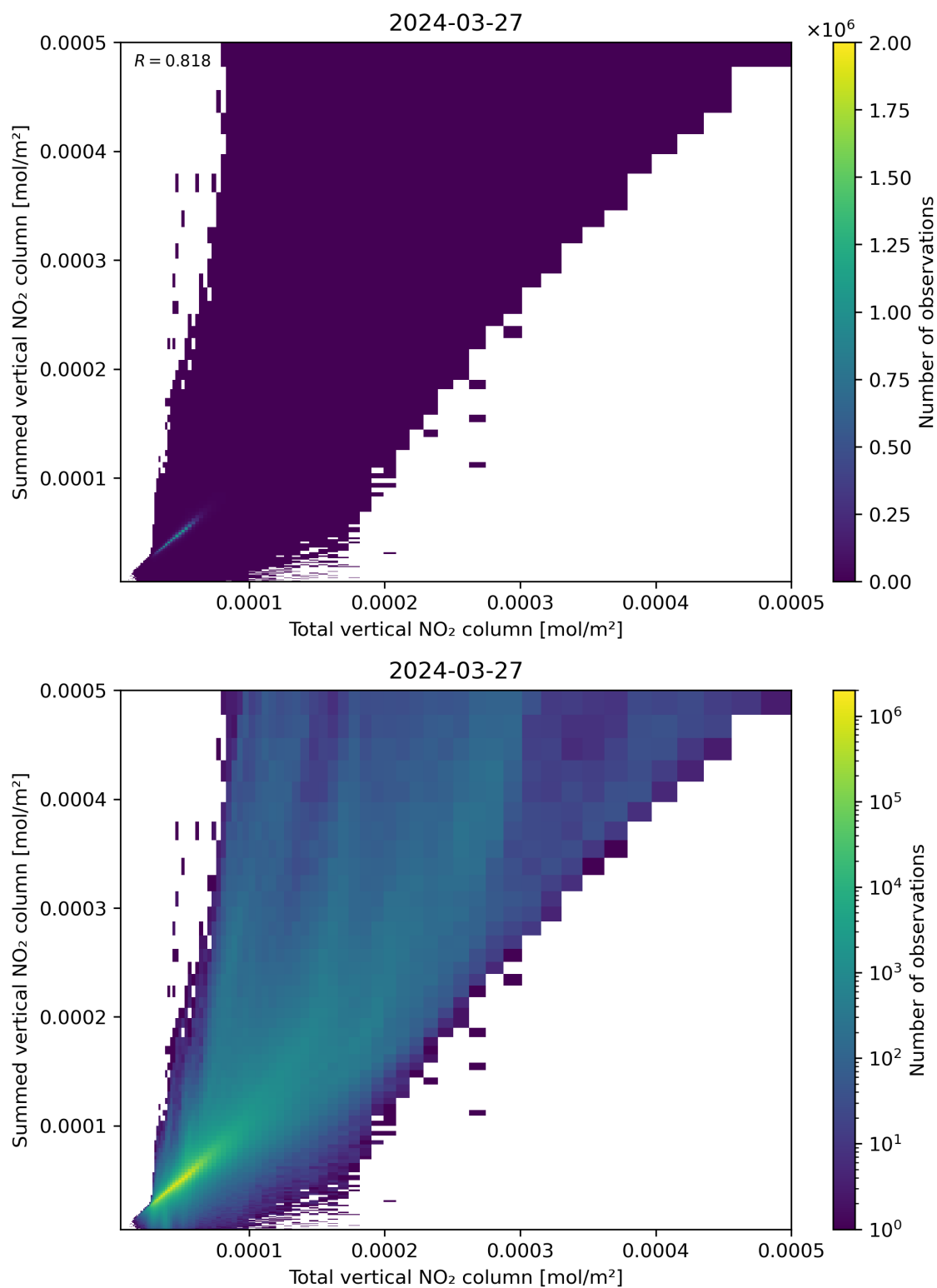
Figure 112: Scatter density plot of “Total vertical NO 2 column” against “Summed vertical NO 2 column” for 2024-03-26 to 2024-03-28.
