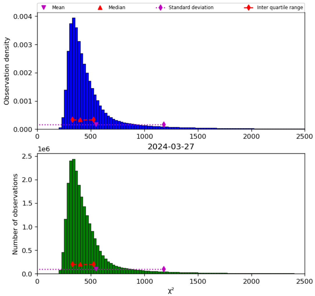
Figure 42: Histogram of “ \chi^2 ” for 2024-03-26 to 2024-03-28
