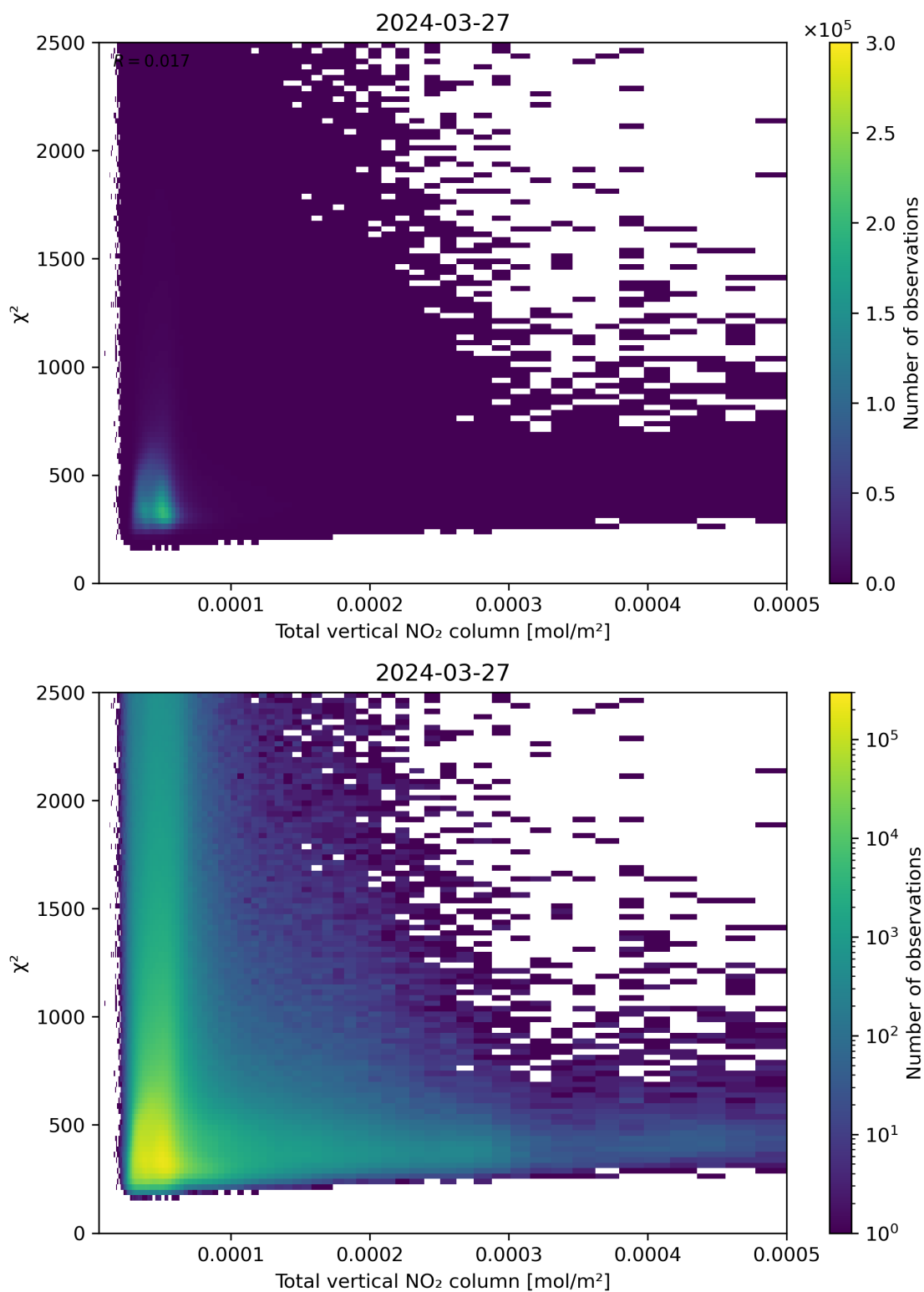
Figure 111: Scatter density plot of “Total vertical NO 2 column” against “ \chi^2 ” for 2024-03-26 to 2024-03-28.
