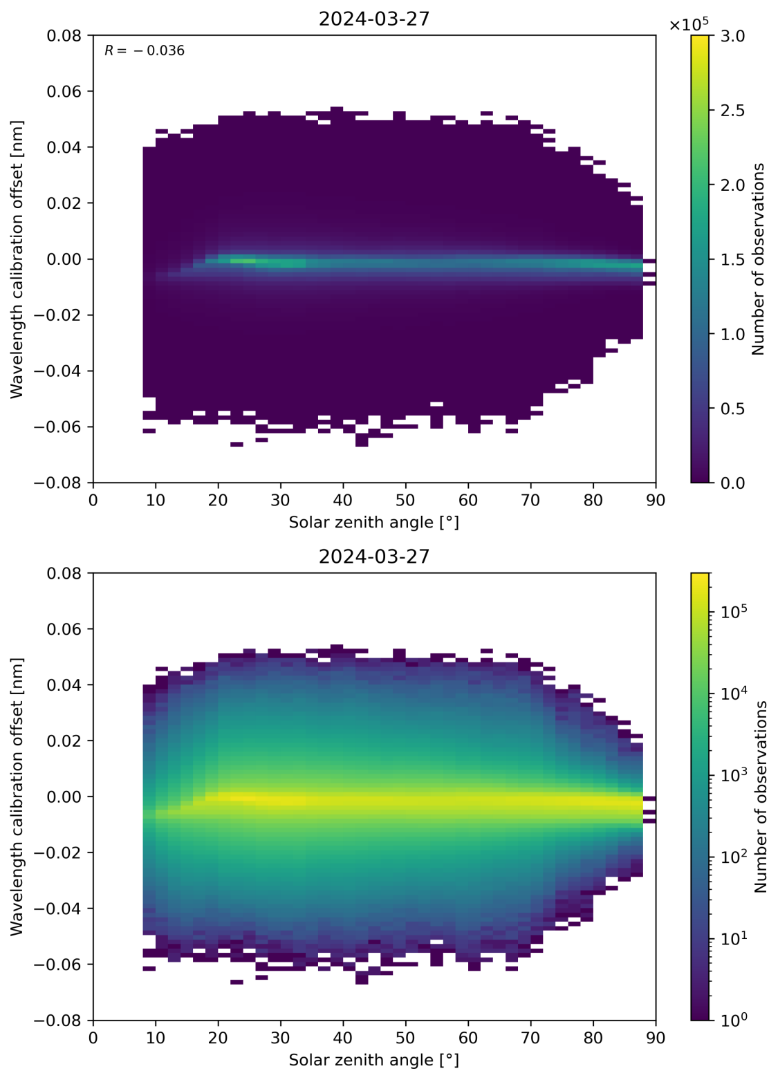
Figure 158: Scatter density plot of “Solar zenith angle” against “Wavelength calibration offset” for 2024-03-26 to 2024-03-28.
