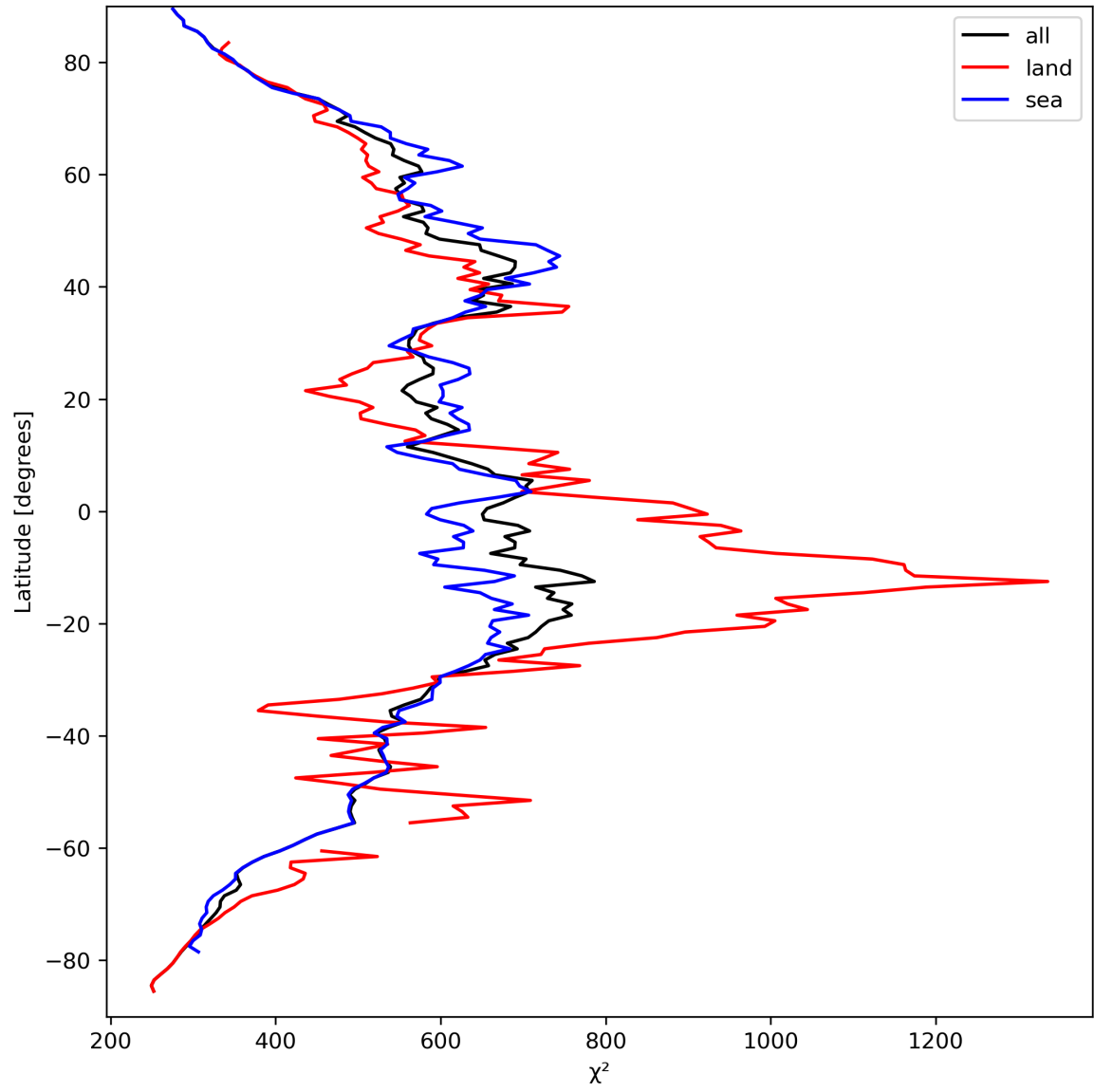
Figure 25: Zonal average of “ \chi^2 ” for 2024-03-26 to 2024-03-28.
