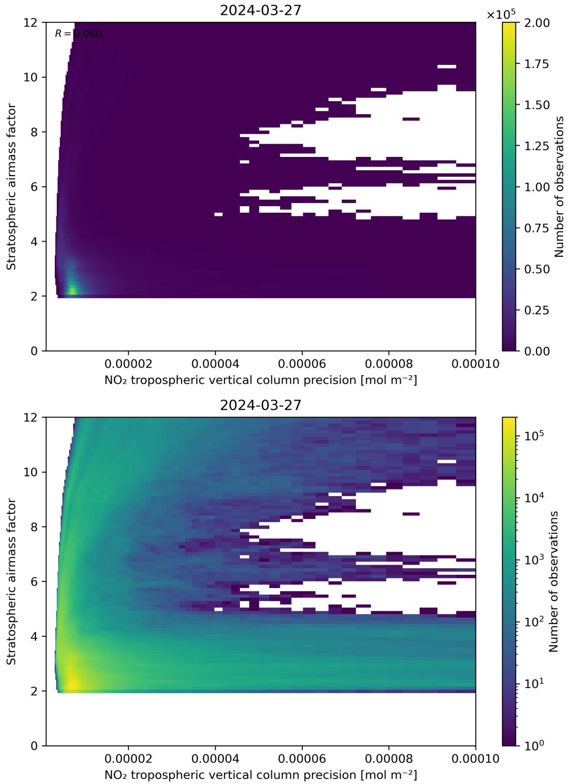
Figure 131: Scatter density plot of “NO 2 tropospheric vertical column precision” against “Stratospheric airmass factor” for 2024-03-26 to 2024-03-28.
