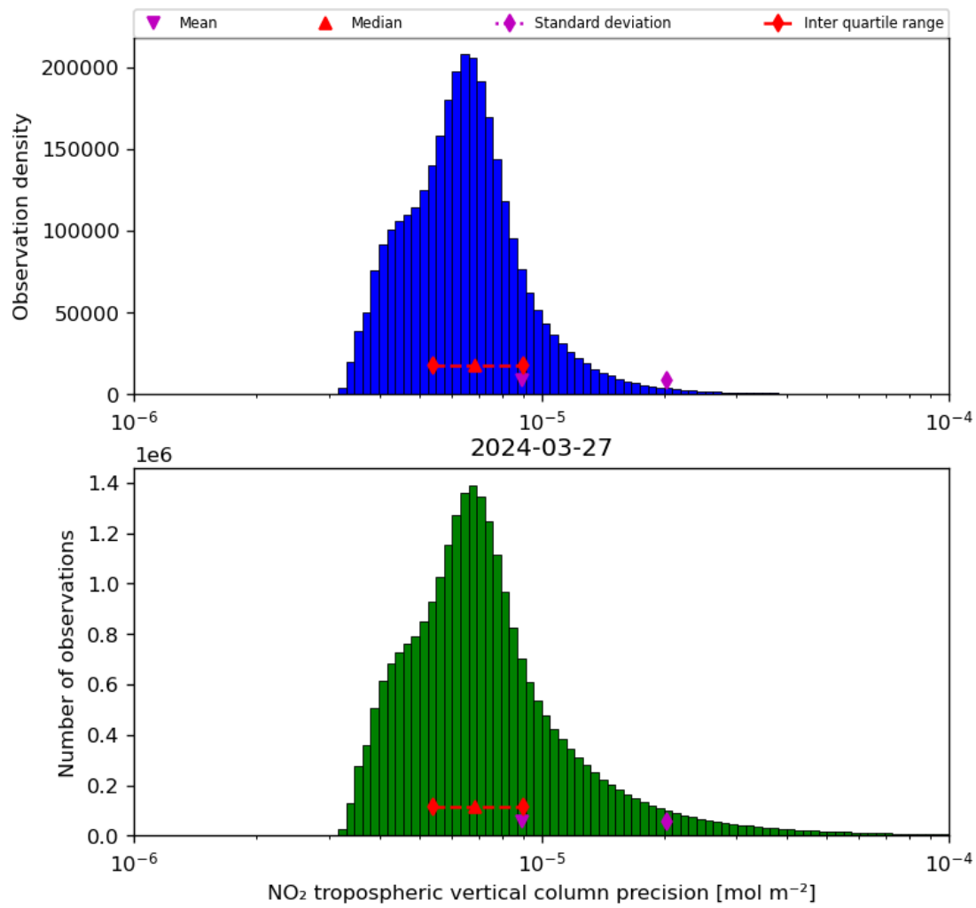
Figure 30: Histogram of “NO 2 tropospheric vertical column precision” for 2024-03-26 to 2024-03-28
