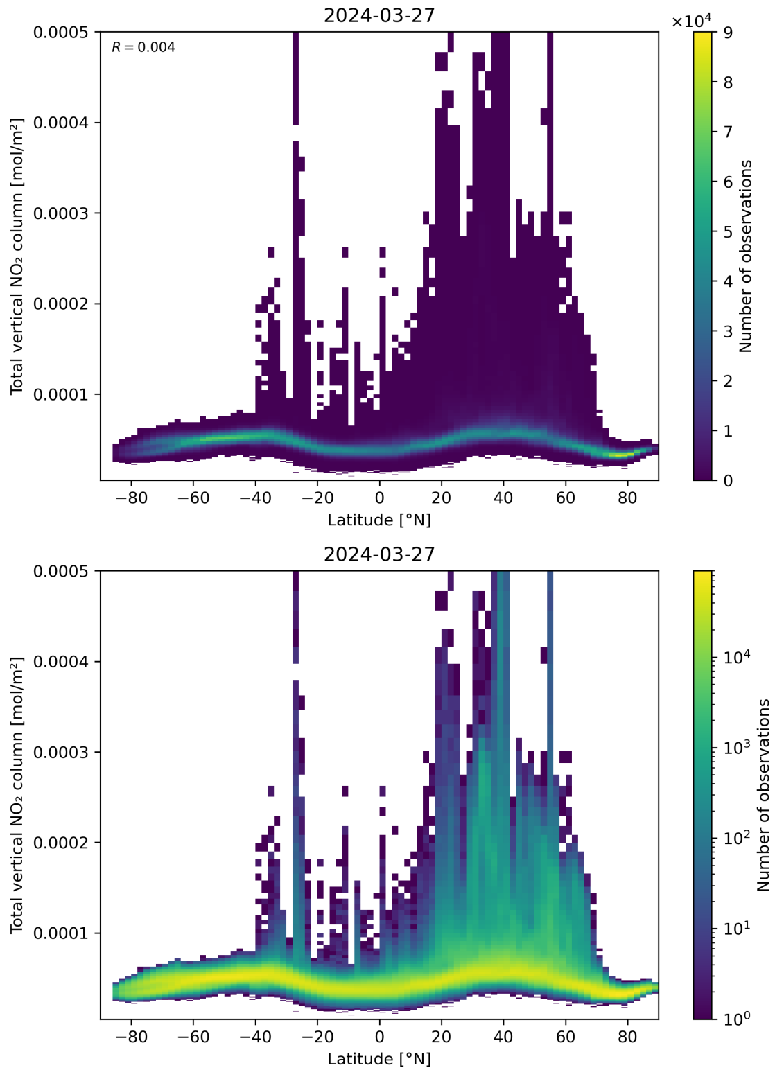
Figure 90: Scatter density plot of “Latitude” against “Total vertical NO 2 column” for 2024-03-26 to 2024-03-28.
