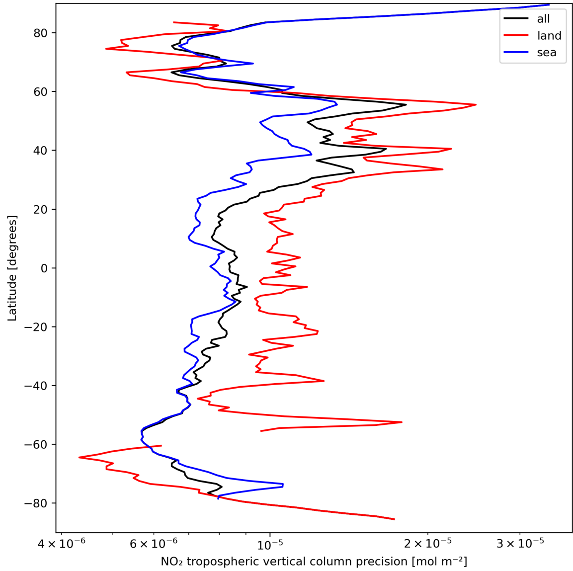
Figure 13: Zonal average of “NO 2 tropospheric vertical column precision” for 2024-03-26 to 2024-03-28.
