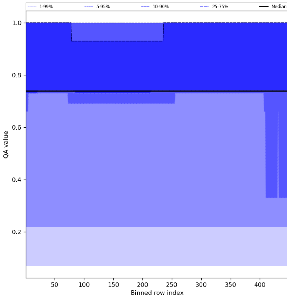
Figure 45: Along track statistics of “QA value” for 2024-03-26 to 2024-03-28
