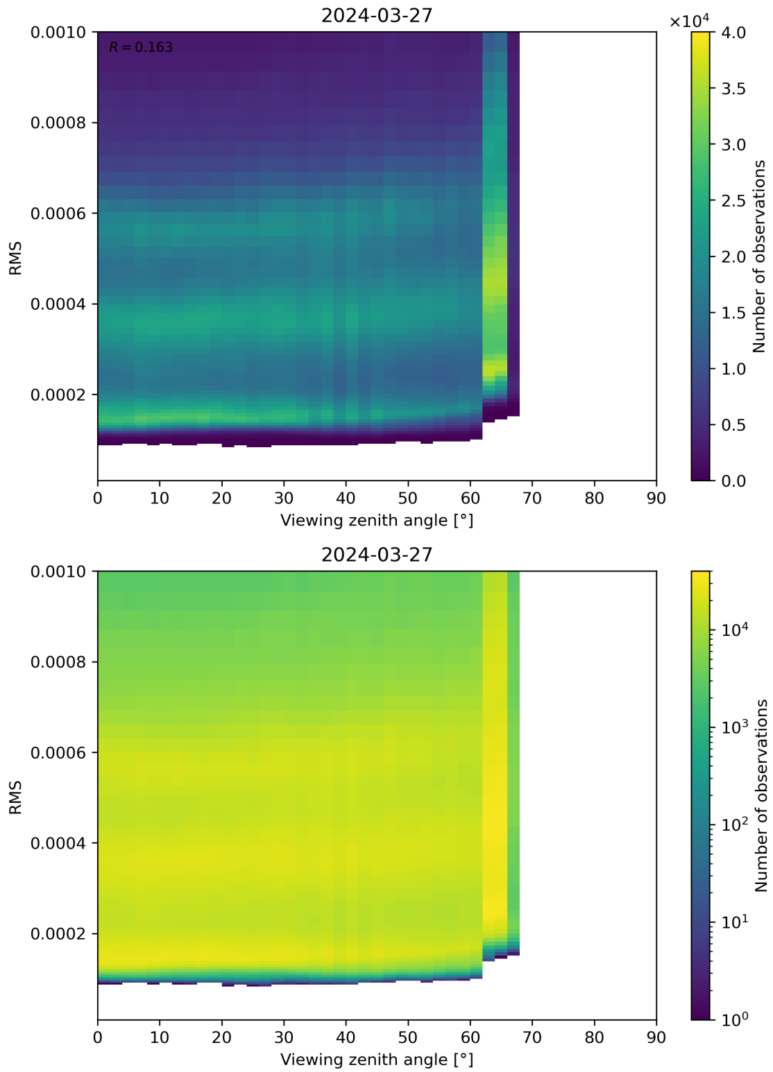
Figure 171: Scatter density plot of “Viewing zenith angle” against “RMS” for 2024-03-26 to 2024-03-28.
