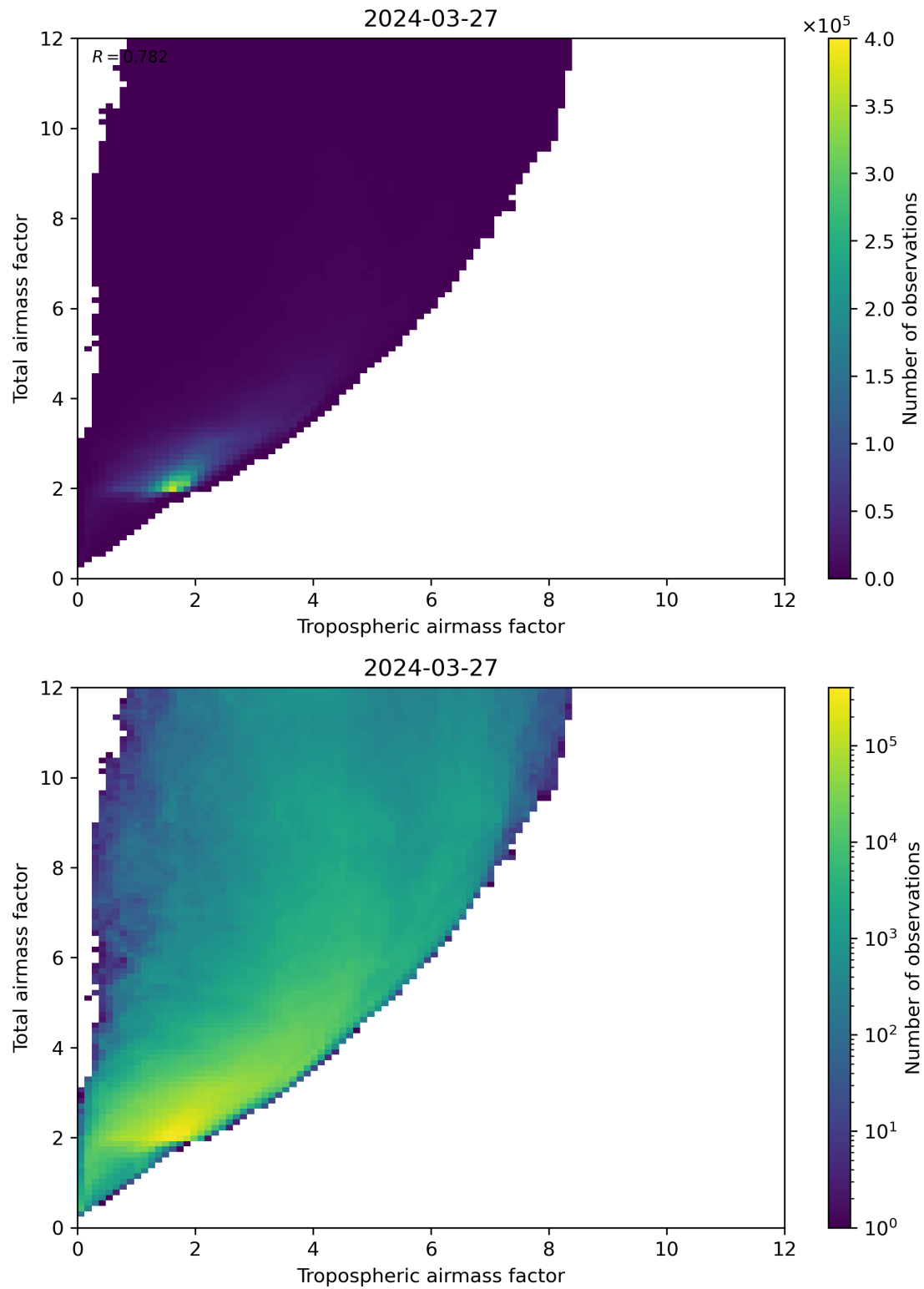
Figure 72: Scatter density plot of “Tropospheric airmass factor” against “Total airmass factor” for 2024-03-26 to 2024-03-28.
