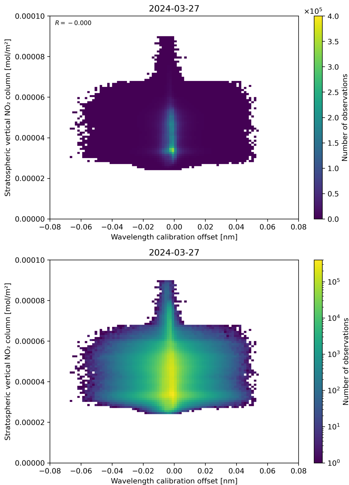
Figure 176: Scatter density plot of “Wavelength calibration offset” against “Stratospheric vertical NO 2 column” for 2024-03-26 to 2024-03-28.
