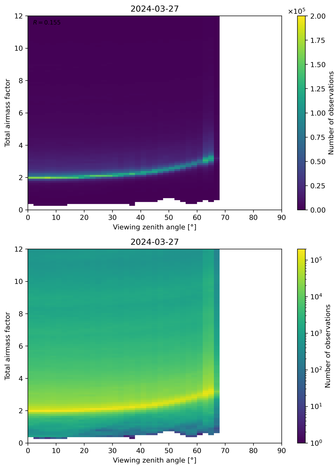
Figure 160: Scatter density plot of “Viewing zenith angle” against “Total airmass factor” for 2024-03-26 to 2024-03-28.
