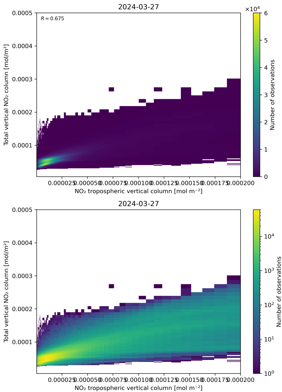
Figure 128: Scatter density plot of “NO 2 tropospheric vertical column” against “Total vertical NO 2 column” for 2024-03-26 to 2024-03-28.
