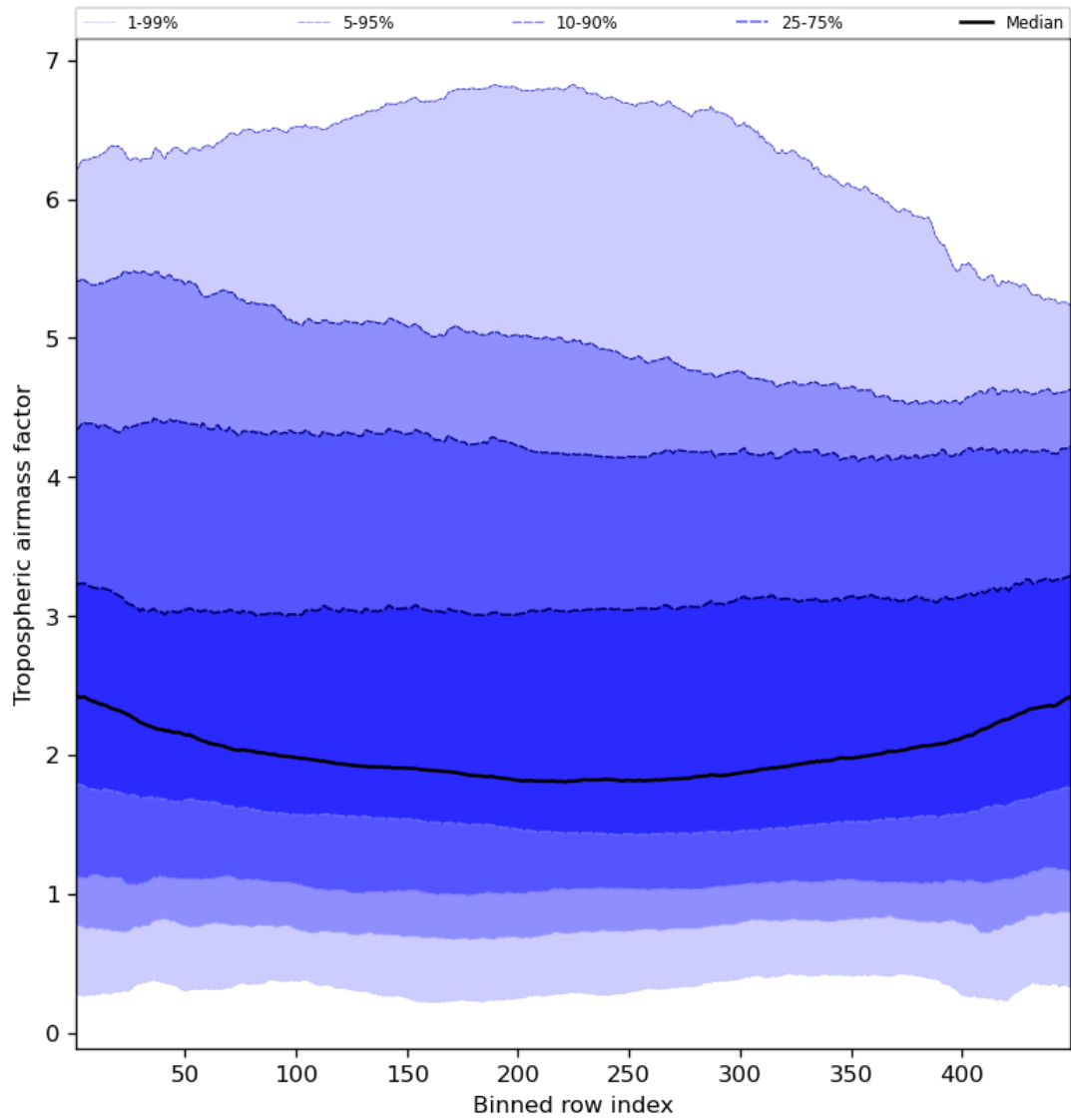
Figure 48: Along track statistics of “Tropospheric airmass factor” for 2024-03-26 to 2024-03-28
