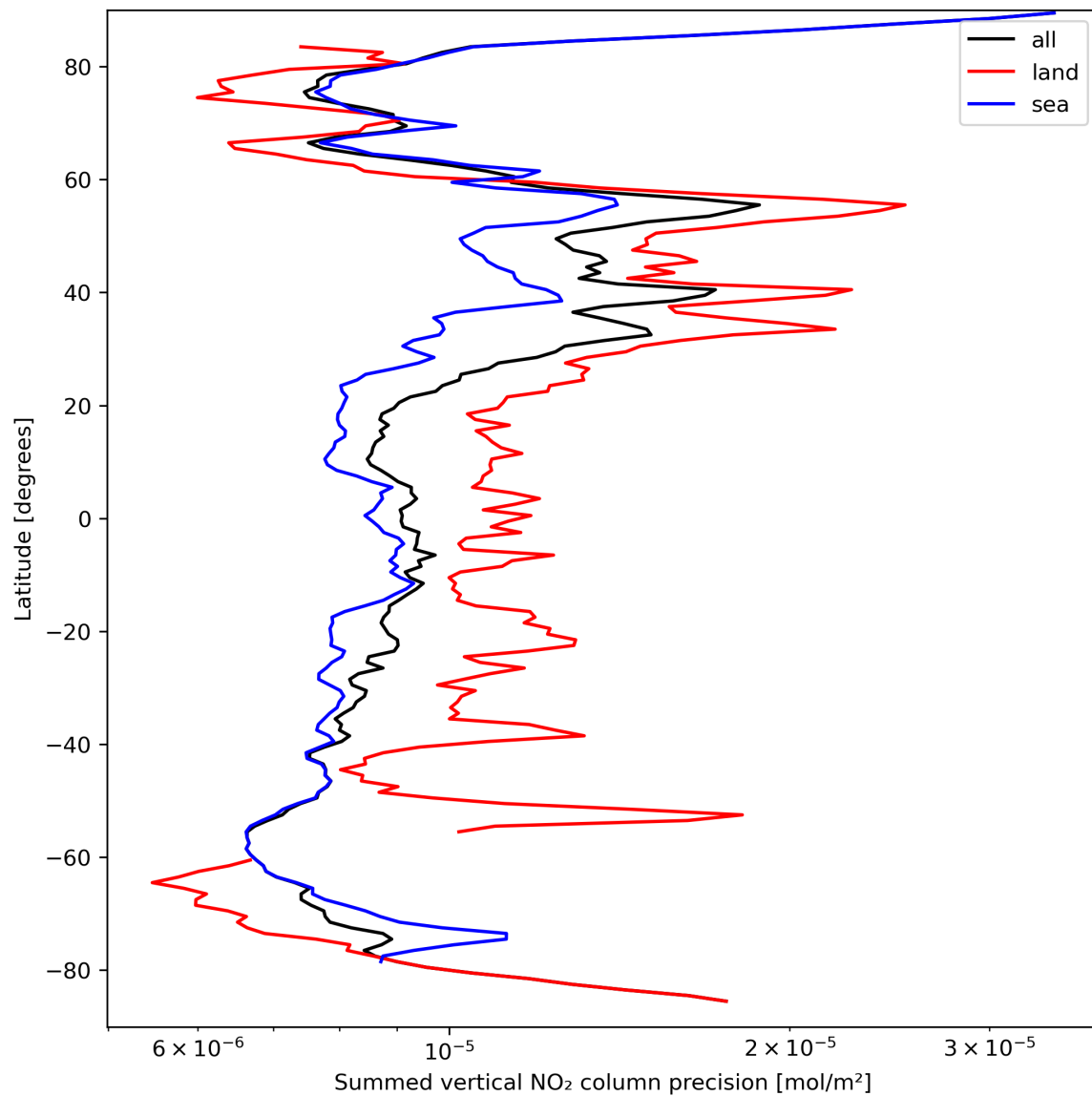
Figure 24: Zonal average of “Summed vertical NO 2 column precision” for 2024-03-26 to 2024-03-28.
