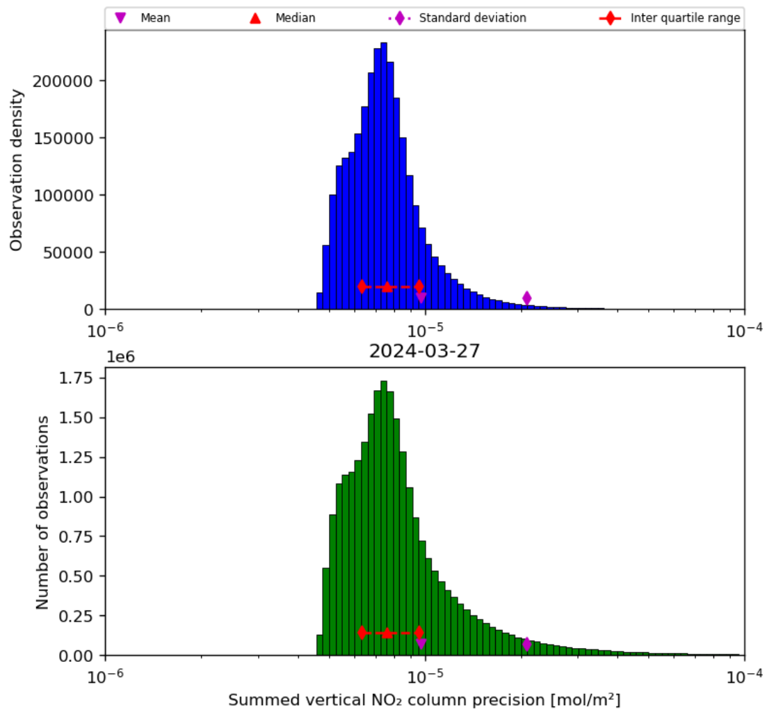
Figure 41: Histogram of “Summed vertical NO 2 column precision” for 2024-03-26 to 2024-03-28
