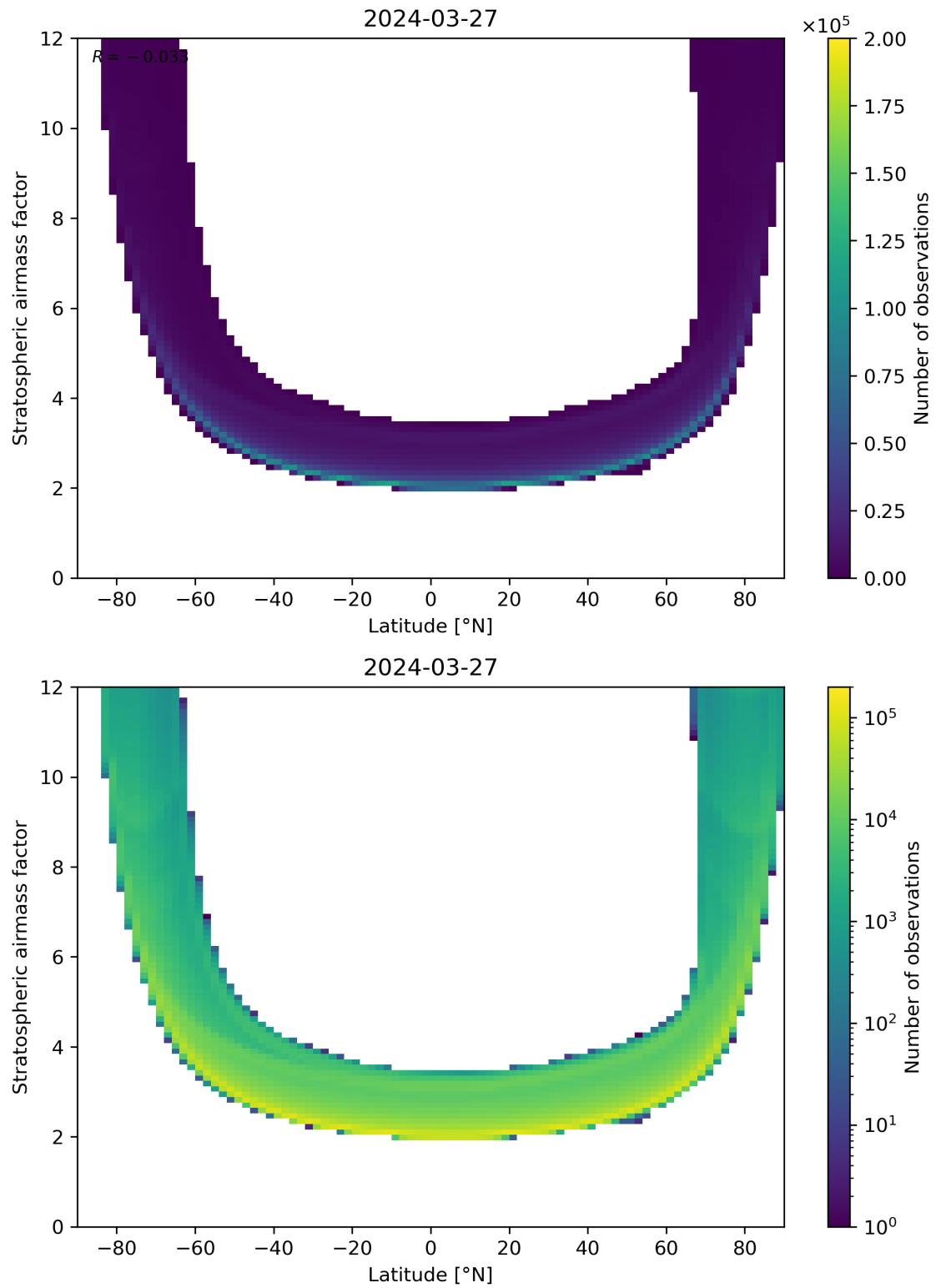
Figure 83: Scatter density plot of “Latitude” against “Stratospheric air mass factor” for 2024-03-26 to 2024-03-28.
