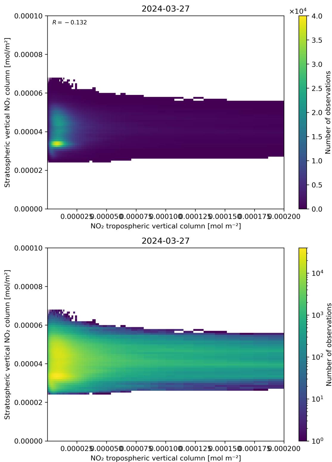
Figure 125: Scatter density plot of “NO 2 tropospheric vertical column” against “Stratospheric vertical NO 2 column” for 2024-03-26 to 2024-03-28.
