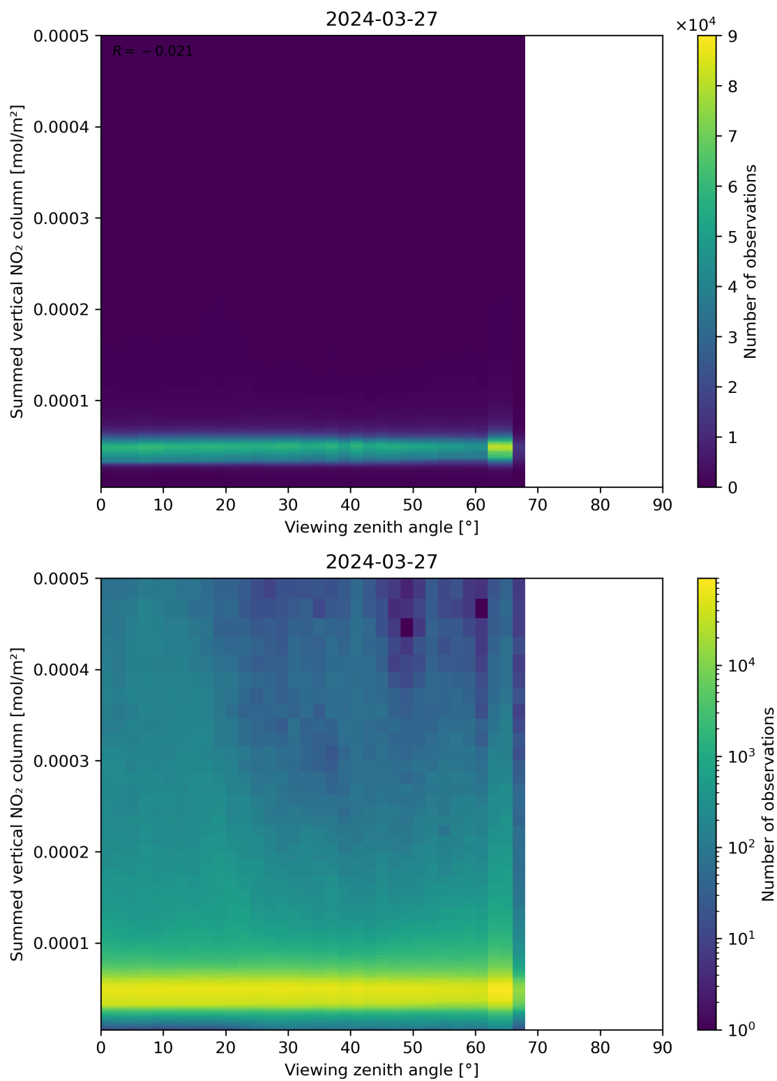
Figure 165: Scatter density plot of “Viewing zenith angle” against “Summed vertical NO 2 column” for 2024-03-26 to 2024-03-28.
