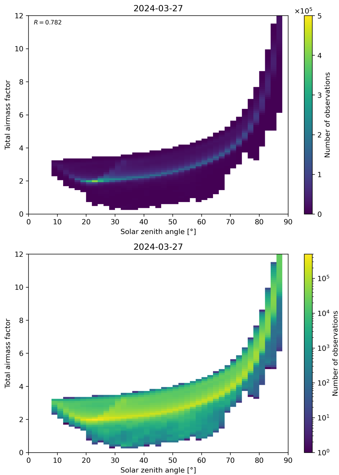
Figure 146: Scatter density plot of “Solar zenith angle” against “Total airmass factor” for 2024-03-26 to 2024-03-28.
