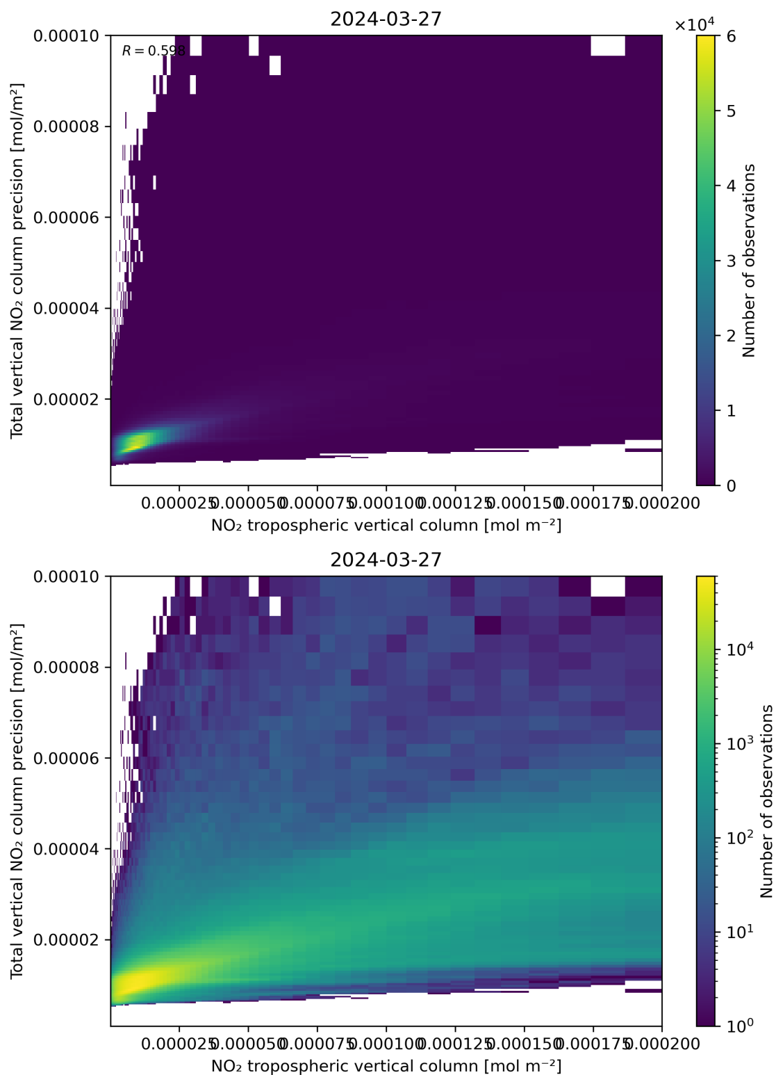
Figure 129: Scatter density plot of “NO 2 tropospheric vertical column” against “Total vertical NO 2 column precision” for 2024-03-26 to 2024-03-28.
