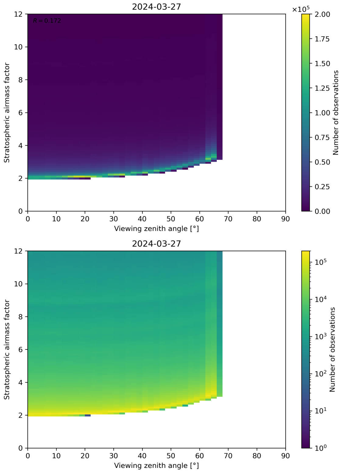
Figure 159: Scatter density plot of “Viewing zenith angle” against “Stratospheric airmass factor” for 2024-03-26 to 2024-03-28.
