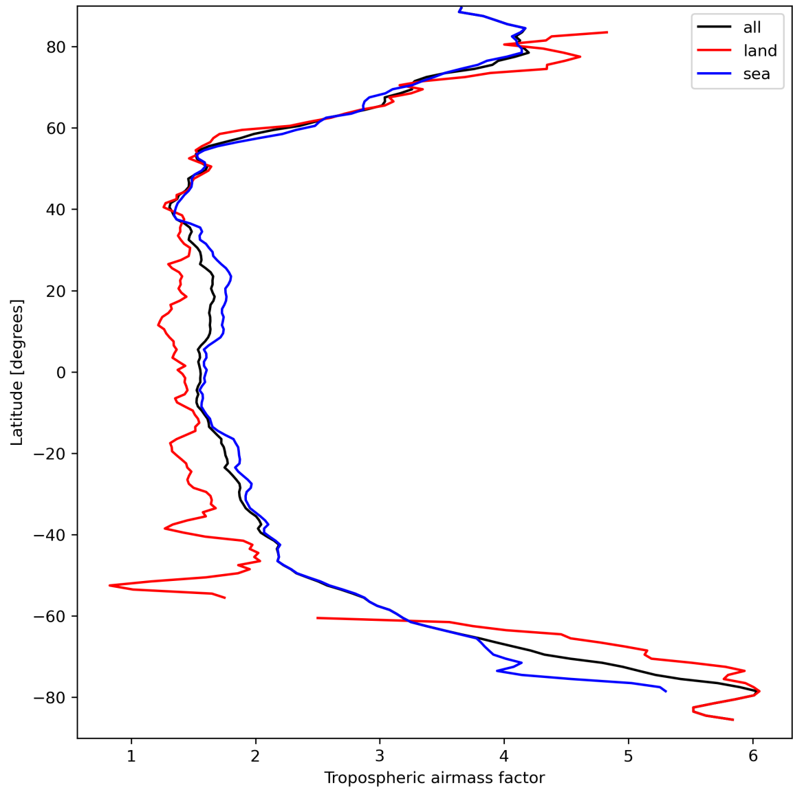
Figure 14: Zonal average of “Tropospheric airmass factor” for 2024-03-26 to 2024-03-28.
