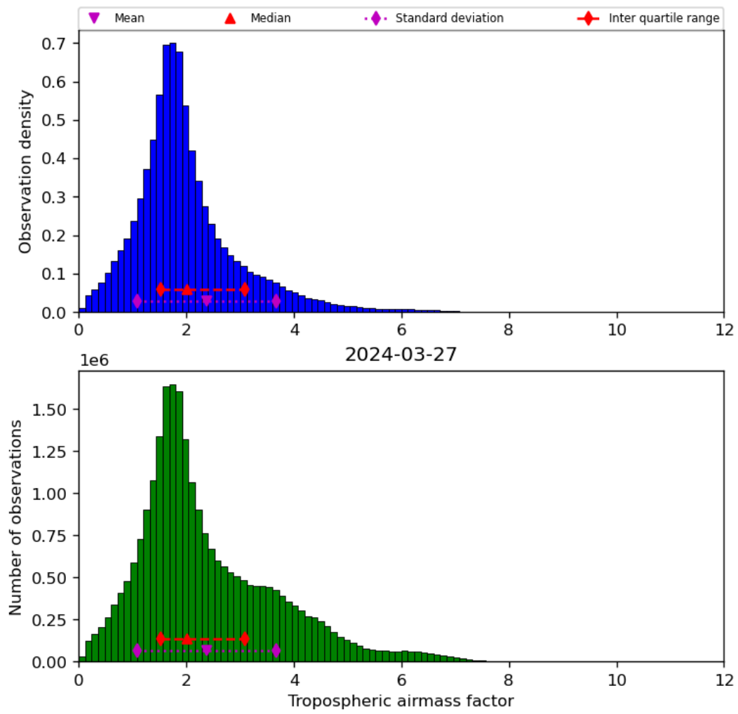
Figure 31: Histogram of “Tropospheric airmass factor” for 2024-03-26 to 2024-03-28
