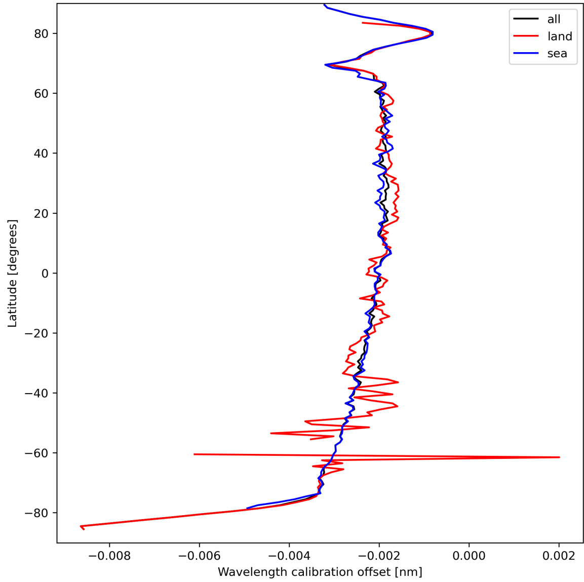
Figure 18: Zonal average of “Wavelength calibration offset” for 2024-03-26 to 2024-03-28.
