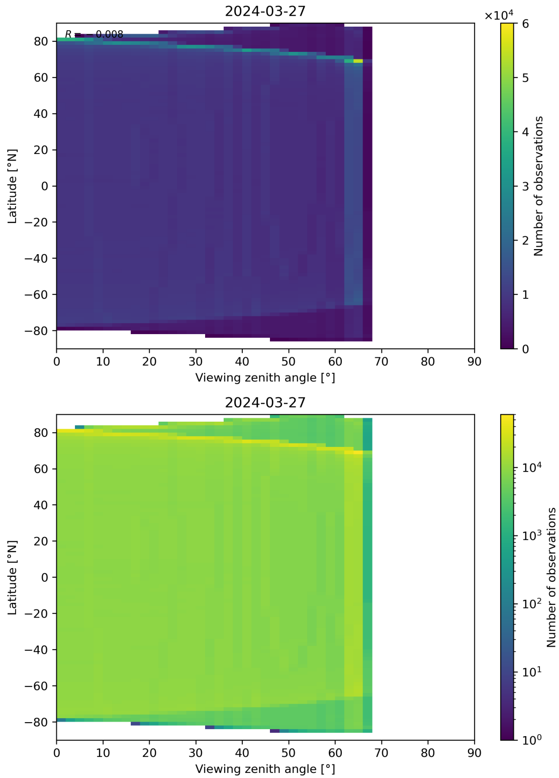
Figure 163: Scatter density plot of “Viewing zenith angle” against “Latitude” for 2024-03-26 to 2024-03-28.
