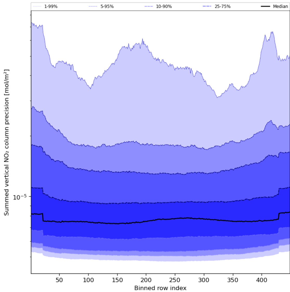
Figure 58: Along track statistics of “Summed vertical NO 2 column precision” for 2024-03-26 to 2024-03-28
