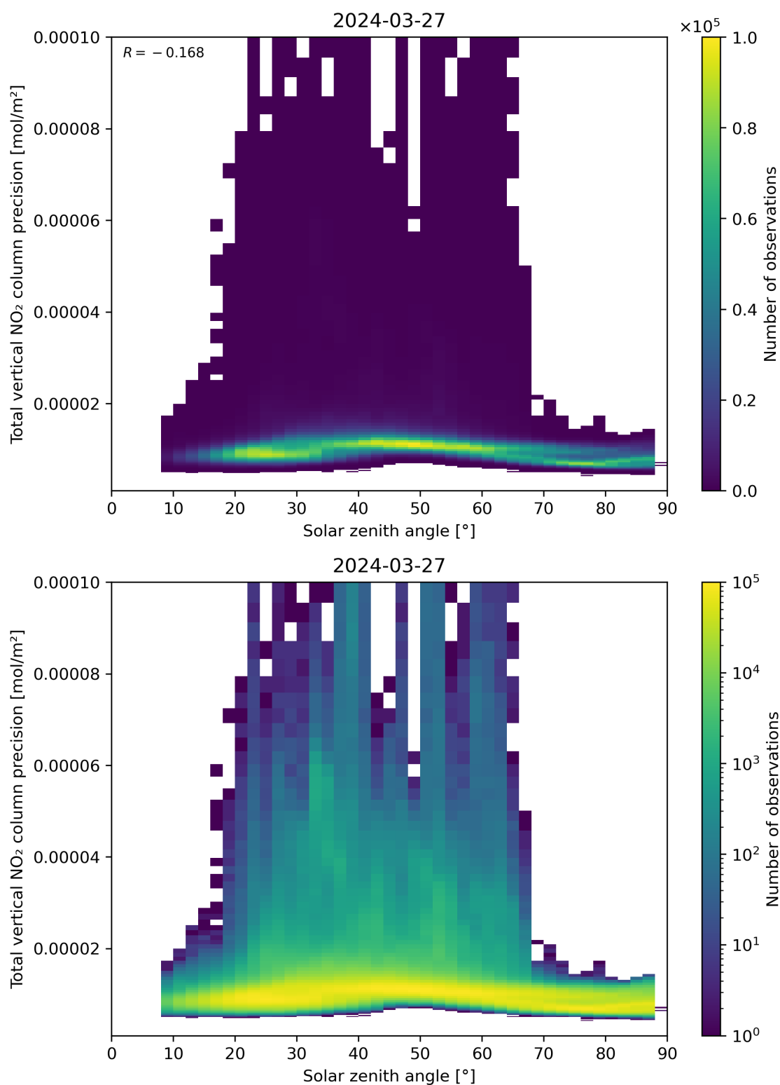
Figure 154: Scatter density plot of “Solar zenith angle” against “Total vertical NO 2 column precision” for 2024-03-26 to 2024-03-28.
