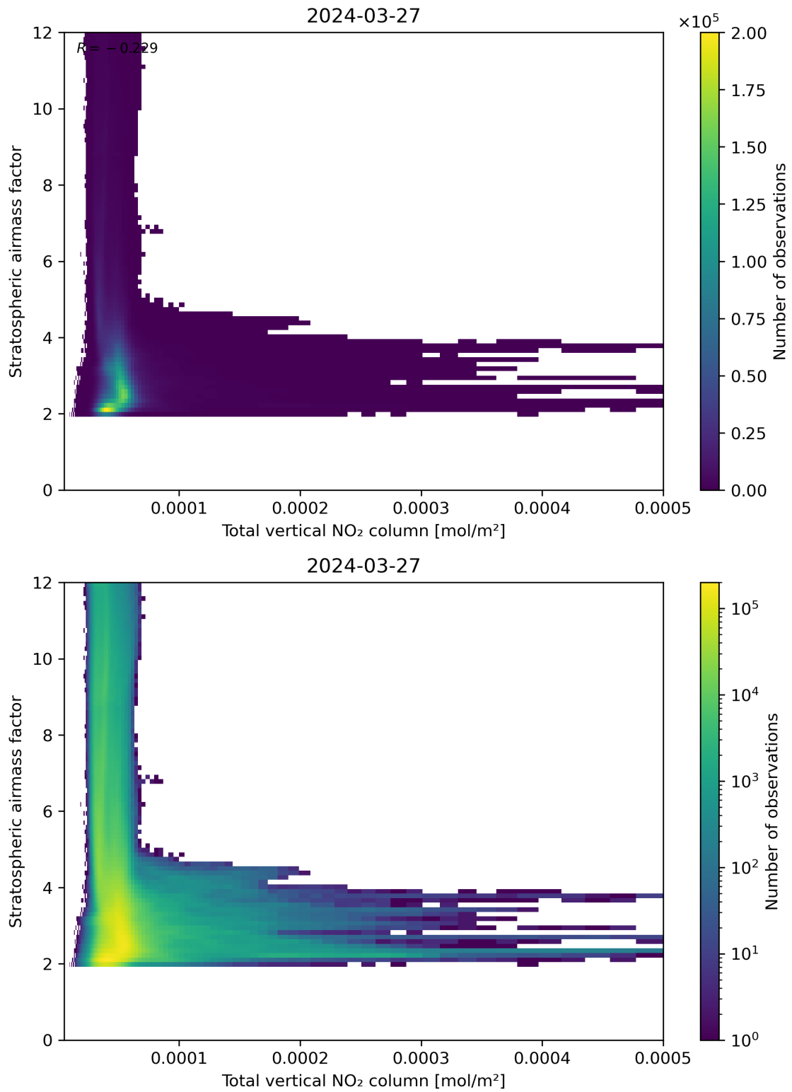
Figure 110: Scatter density plot of “Total vertical NO 2 column” against “Stratospheric airmass factor” for 2024-03-26 to 2024-03-28.
