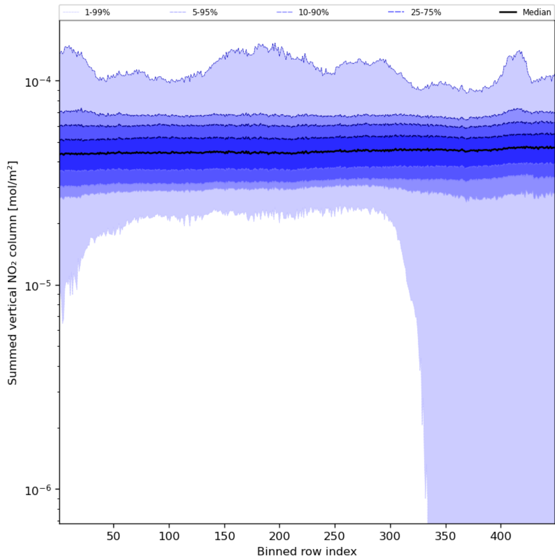
Figure 57: Along track statistics of “Summed vertical NO 2 column” for 2024-03-26 to 2024-03-28
