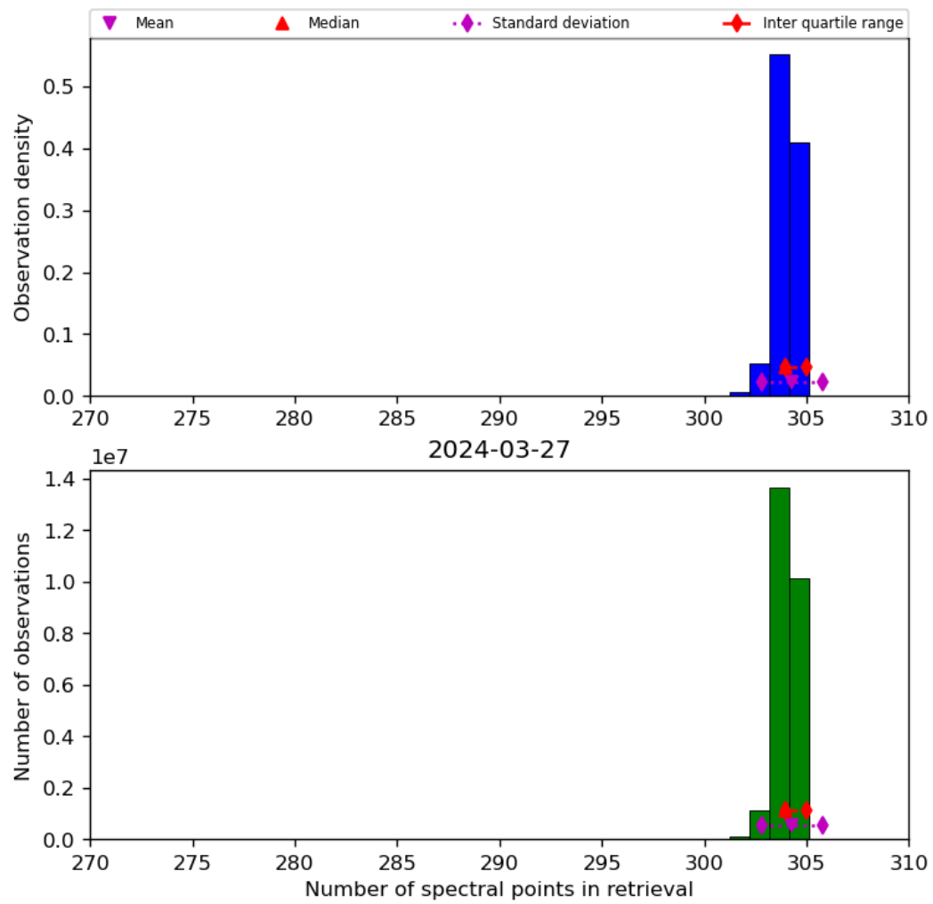
Figure 33: Histogram of “Number of spectral points in retrieval” for 2024-03-26 to 2024-03-28
