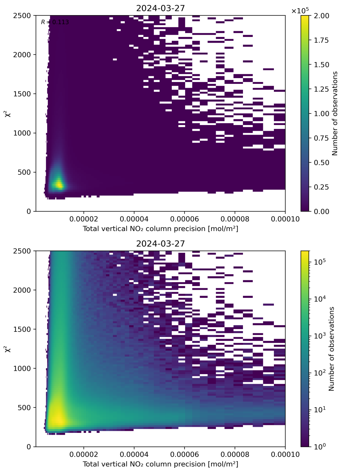
Figure 116: Scatter density plot of “Total vertical NO 2 column precision” against “ \chi^2 ” for 2024-03-26 to 2024-03-28.
