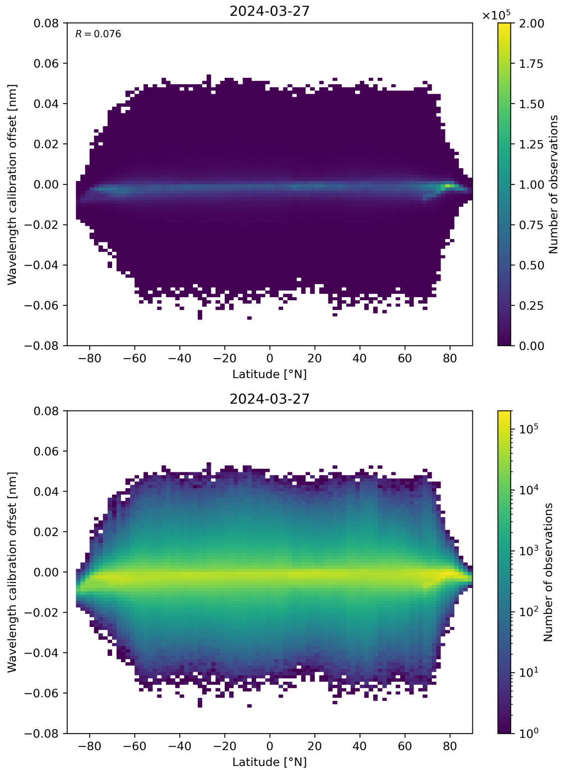
Figure 95: Scatter density plot of “Latitude” against “Wavelength calibration offset” for 2024-03-26 to 2024-03-28.
