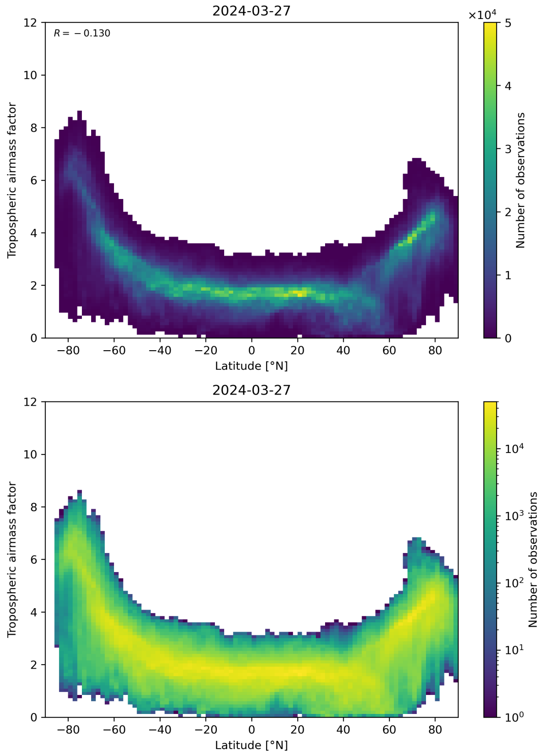
Figure 85: Scatter density plot of “Latitude” against “Tropospheric airmass factor” for 2024-03-26 to 2024-03-28.
