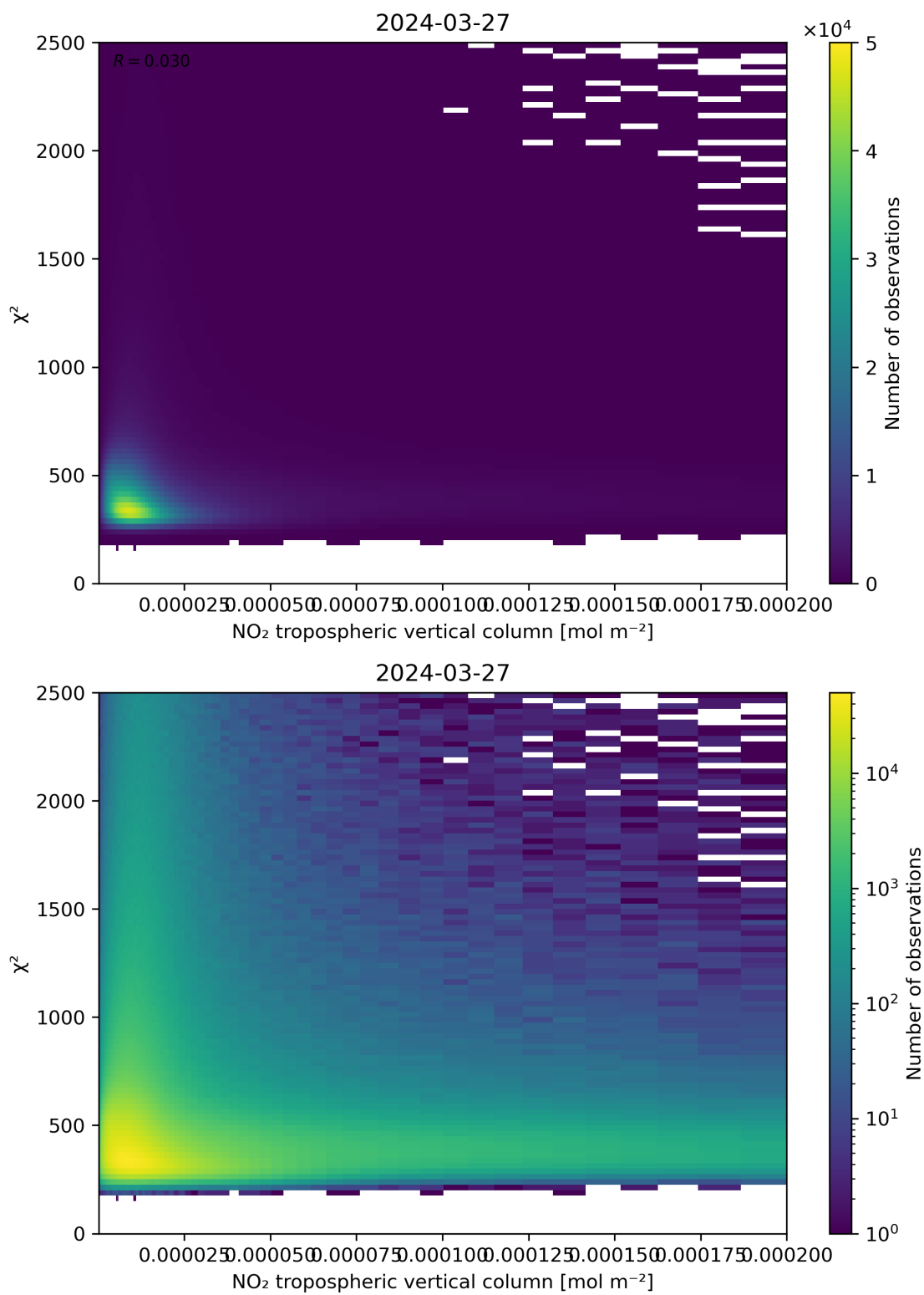
Figure 124: Scatter density plot of “NO 2 tropospheric vertical column” against “ \chi^2 ” for 2024-03-26 to 2024-03-28.
