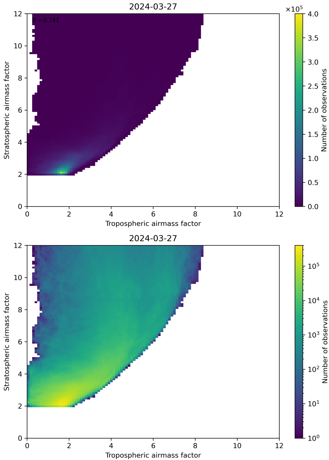
Figure 71: Scatter density plot of “Tropospheric airmass factor” against “Stratospheric airmass factor” for 2024-03-26 to 2024-03-28.
