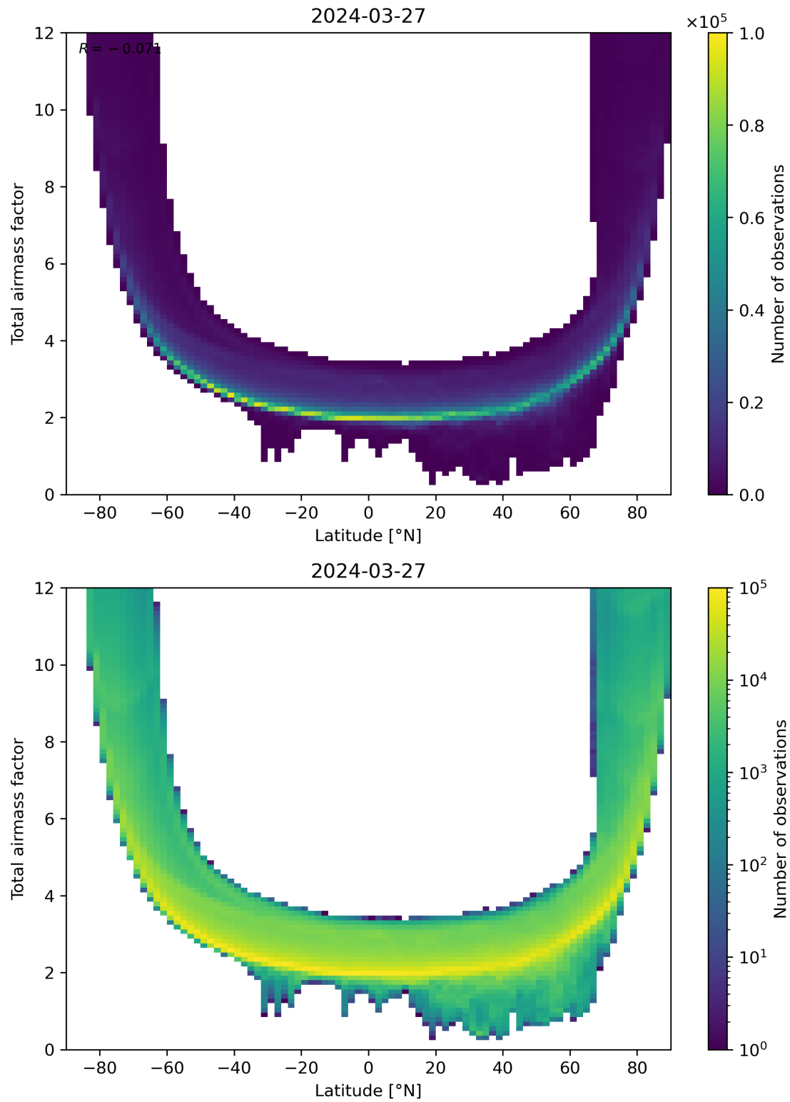
Figure 84: Scatter density plot of “Latitude” against “Total airmass factor” for 2024-03-26 to 2024-03-28.
