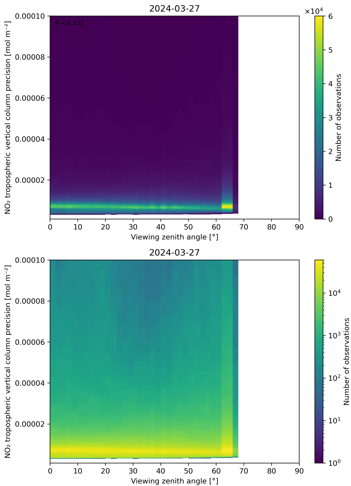
Figure 170: Scatter density plot of “Viewing zenith angle” against “NO 2 tropospheric vertical column precision” for 2024-03-26 to 2024-03-28.
