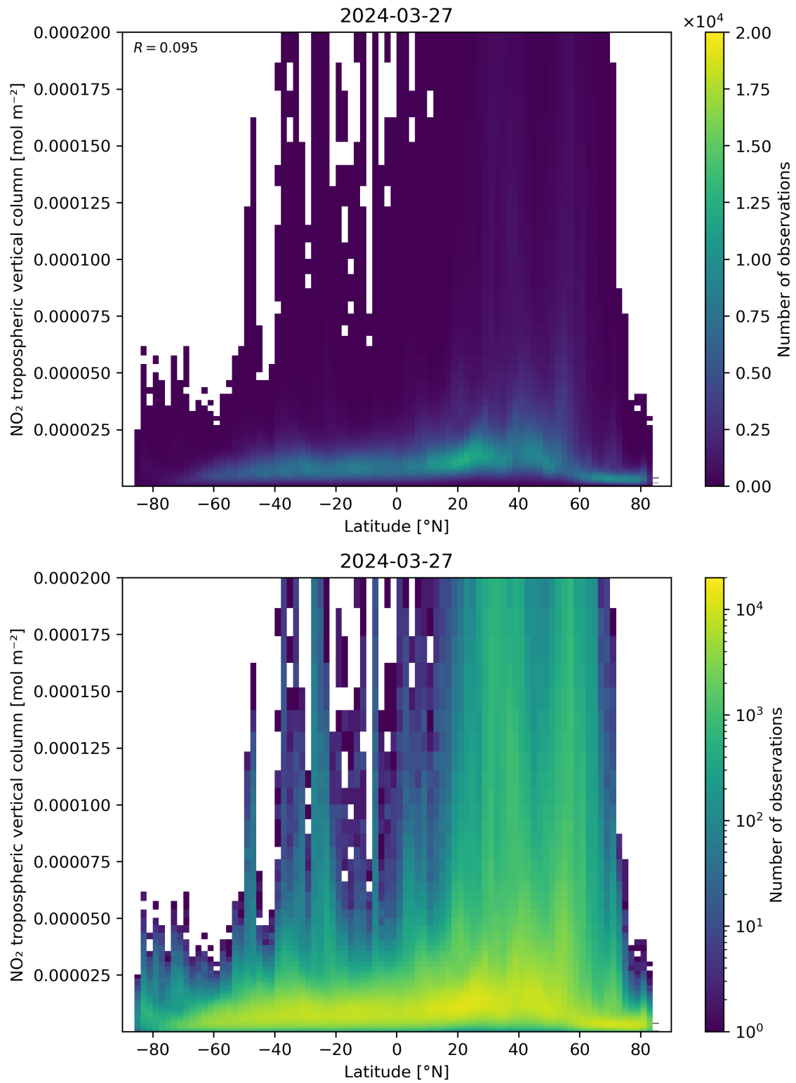
Figure 92: Scatter density plot of “Latitude” against “NO 2 tropospheric vertical column” for 2024-03-26 to 2024-03-28.
