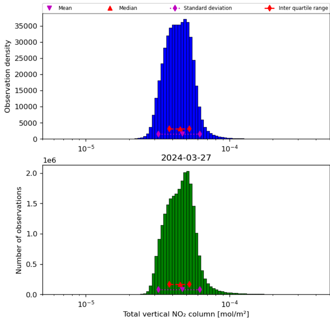
Figure 38: Histogram of “Total vertical NO 2 column” for 2024-03-26 to 2024-03-28
