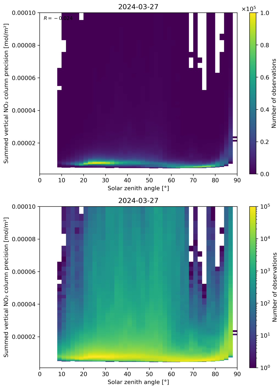
Figure 152: Scatter density plot of “Solar zenith angle” against “Summed vertical NO 2 column precision” for 2024-03-26 to 2024-03-28.
