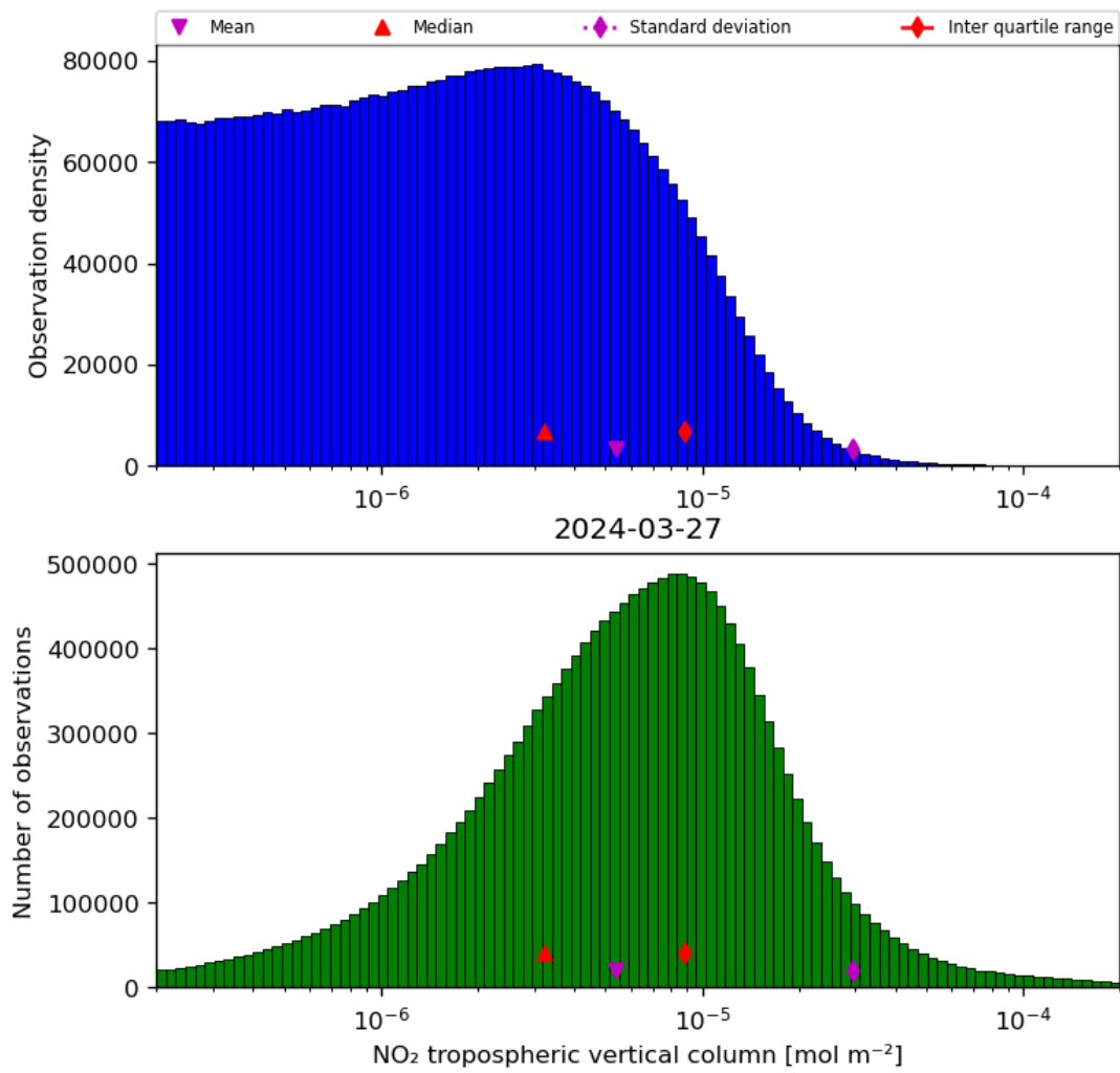
Figure 29: Histogram of “NO 2 tropospheric vertical column” for 2024-03-26 to 2024-03-28
