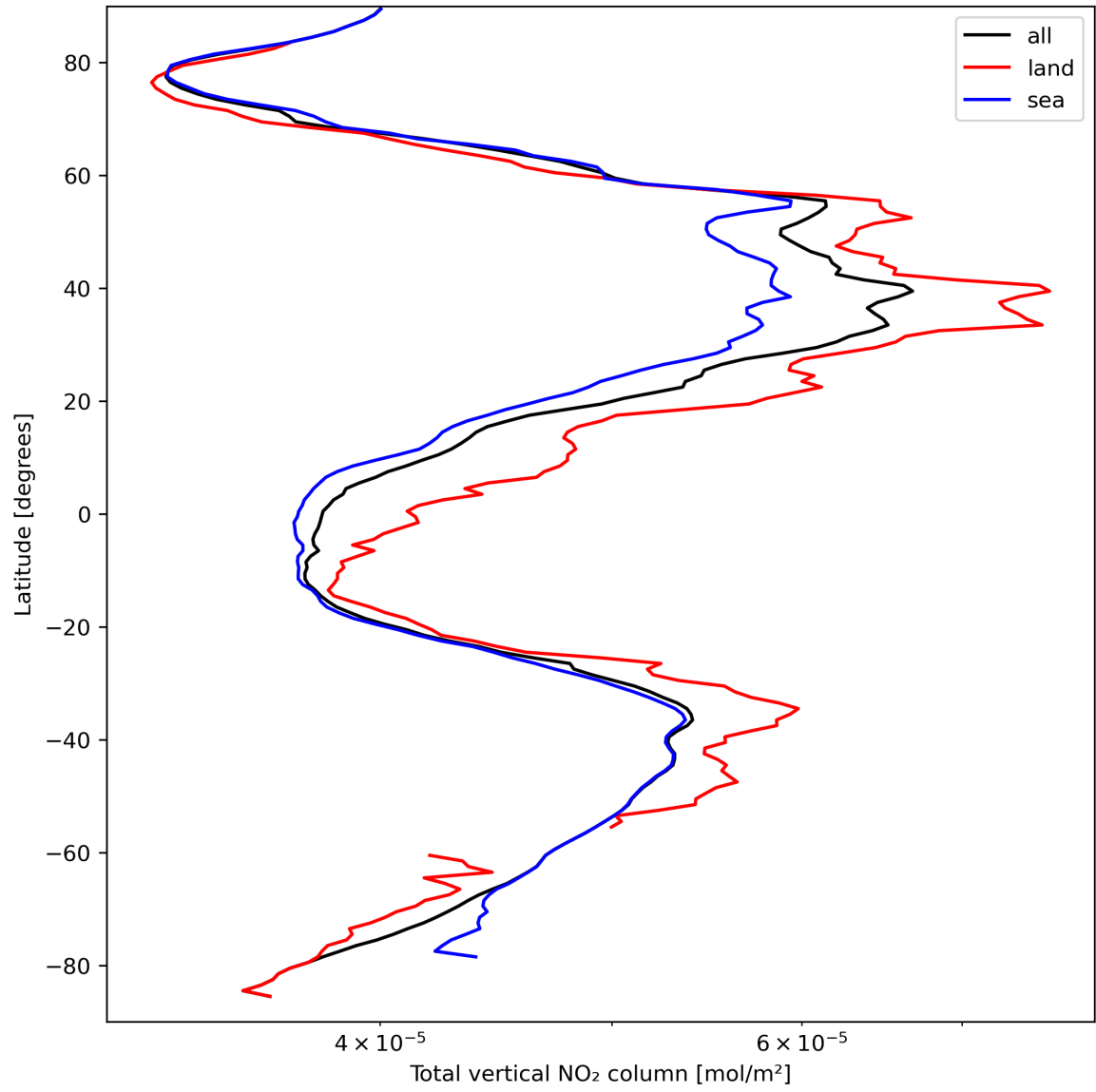
Figure 21: Zonal average of “Total vertical NO 2 column” for 2024-03-26 to 2024-03-28.
