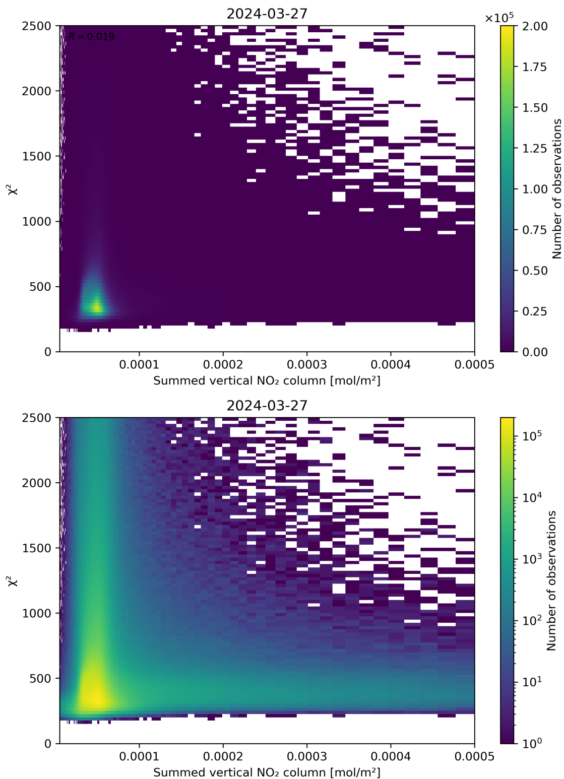
Figure 104: Scatter density plot of “Summed vertical NO 2 column” against “ \chi^2 ” for 2024-03-26 to 2024-03-28.
