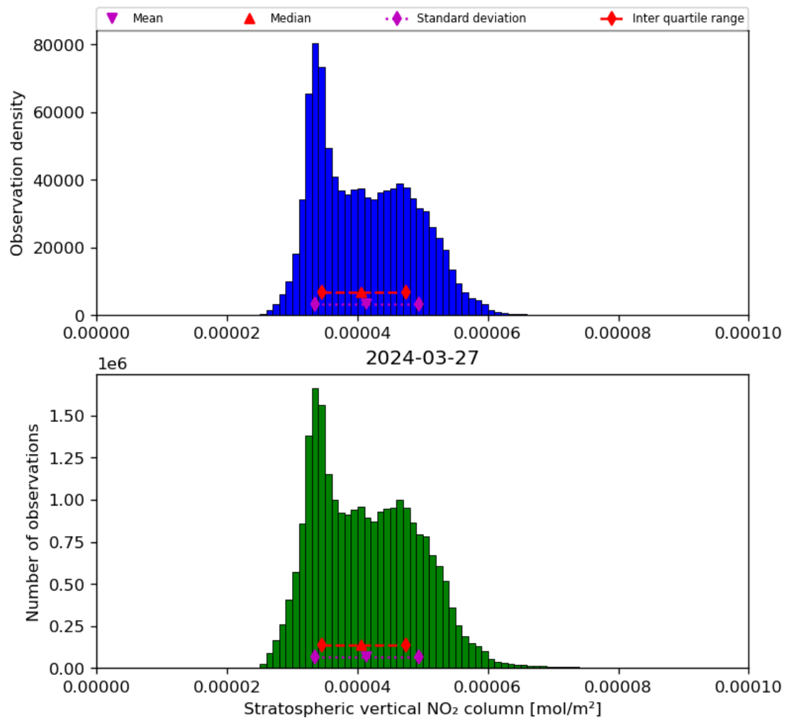
Figure 36: Histogram of “Stratospheric vertical NO 2 column” for 2024-03-26 to 2024-03-28
