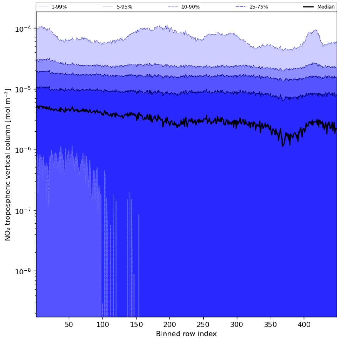
Figure 46: Along track statistics of “NO 2 tropospheric vertical column” for 2024-03-26 to 2024-03-28
