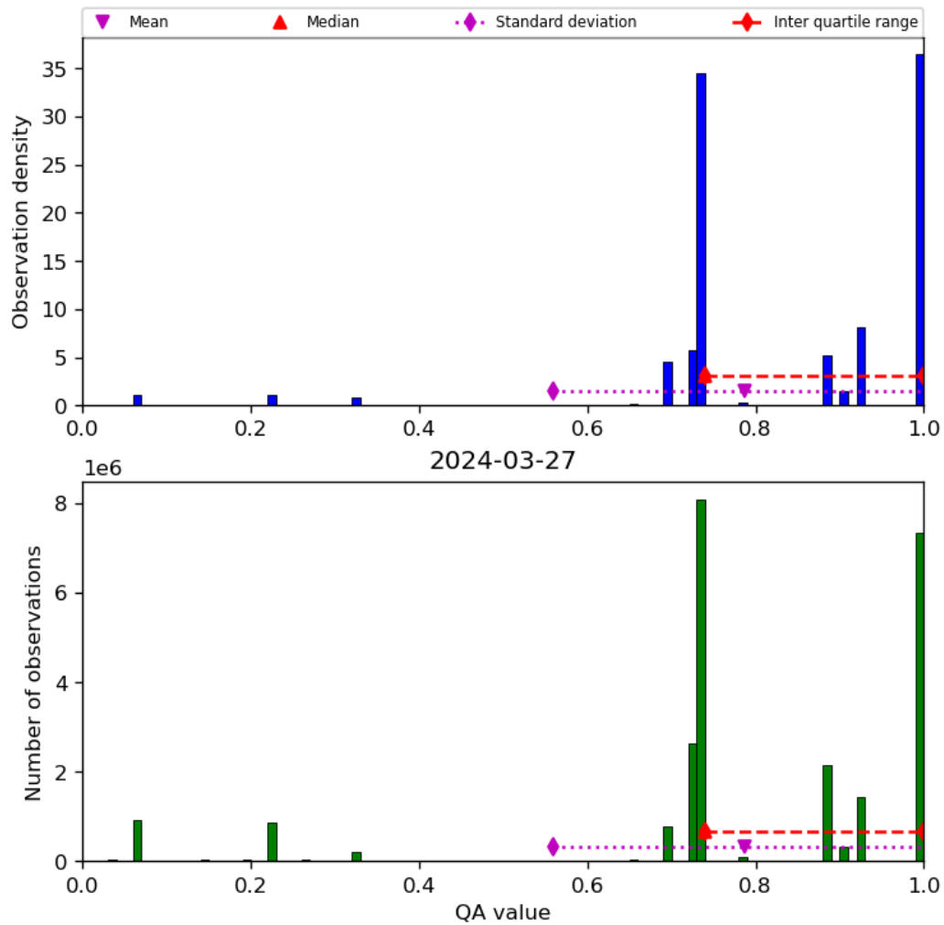
Figure 28: Histogram of “QA value” for 2024-03-26 to 2024-03-28
