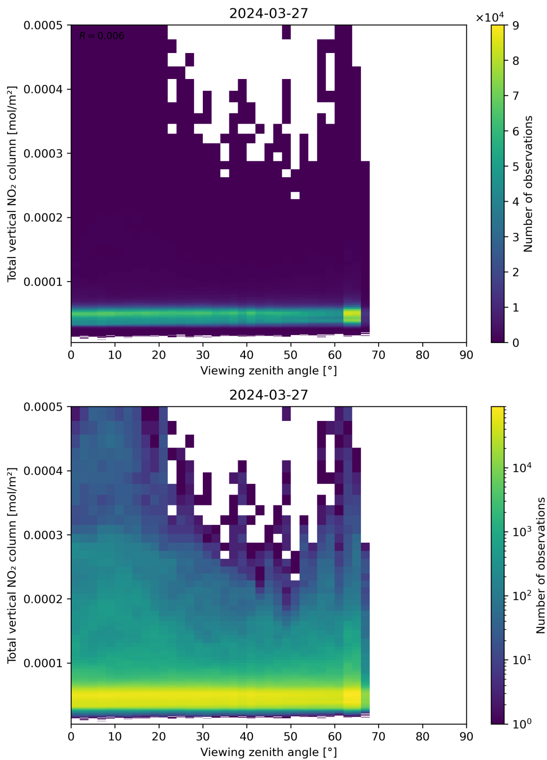
Figure 167: Scatter density plot of “Viewing zenith angle” against “Total vertical NO 2 column” for 2024-03-26 to 2024-03-28.
