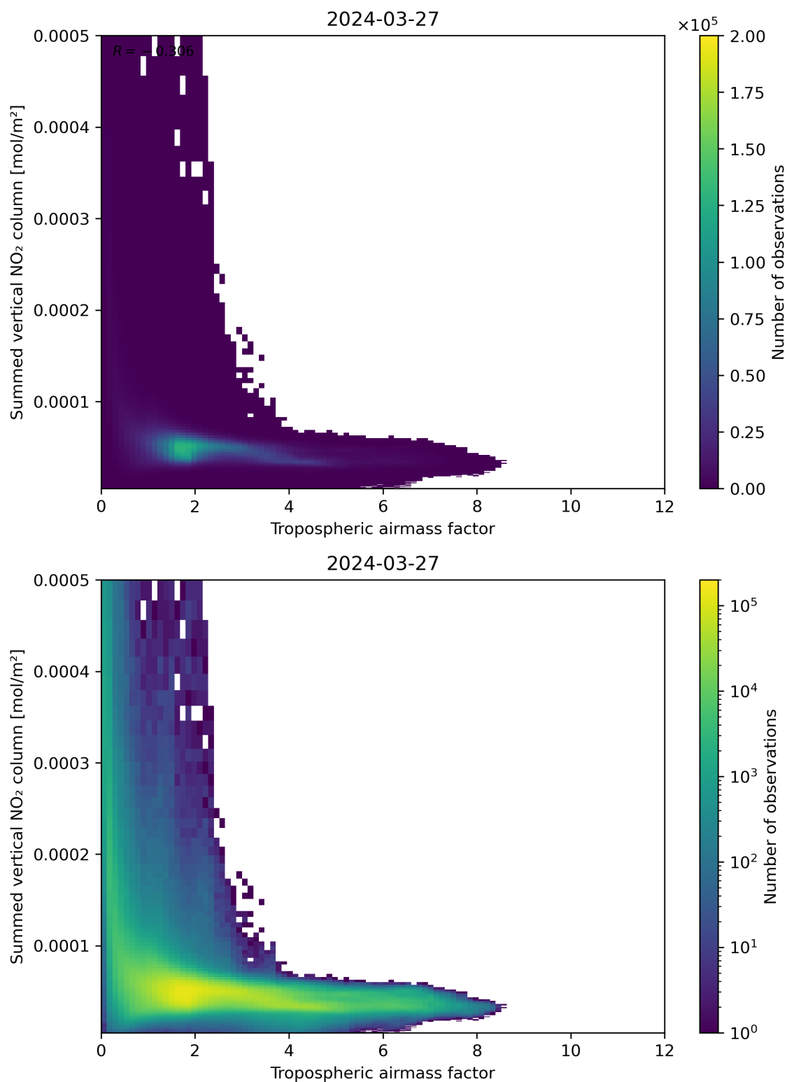
Figure 75: Scatter density plot of “Tropospheric air mass factor” against “Summed vertical NO 2 column” for 2024-03-26 to 2024-03-28.
