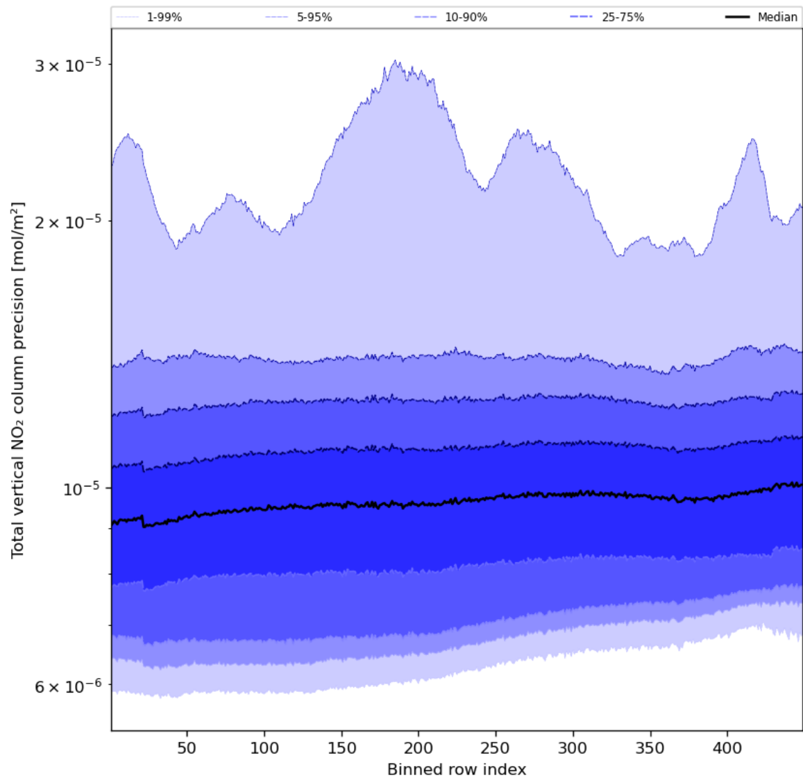
Figure 56: Along track statistics of “Total vertical NO 2 column precision” for 2024-03-26 to 2024-03-28
