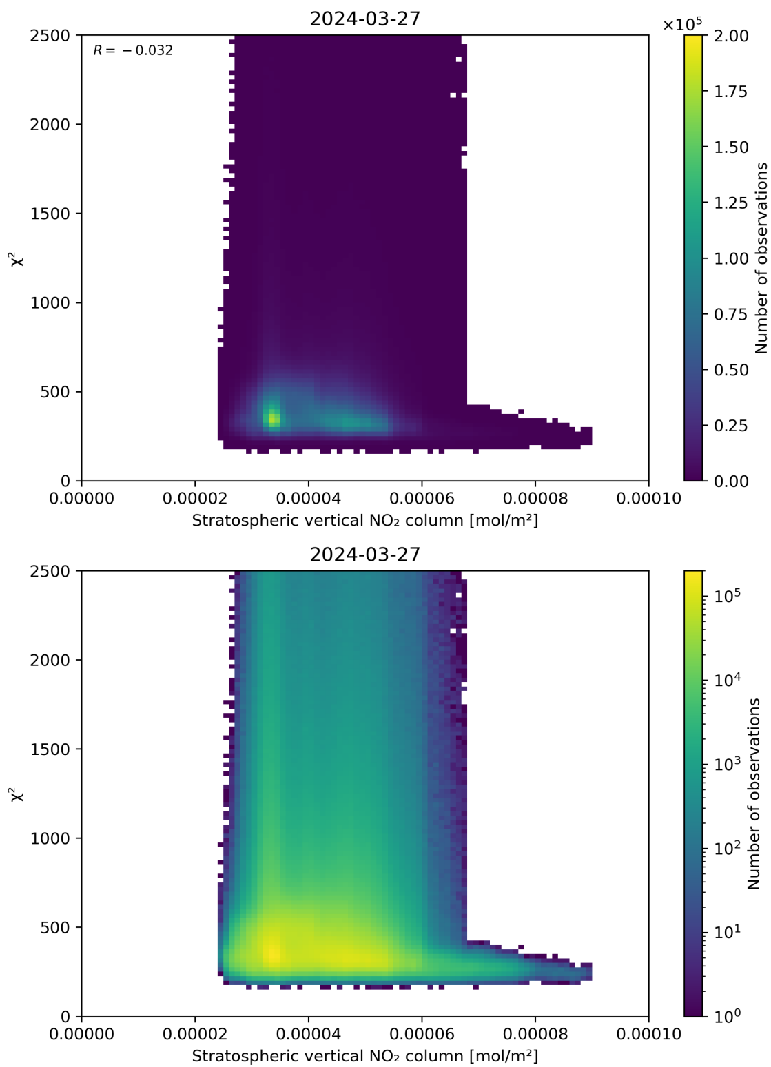
Figure 97: Scatter density plot of “Stratospheric vertical NO 2 column” against “ \chi^2 ” for 2024-03-26 to 2024-03-28.
