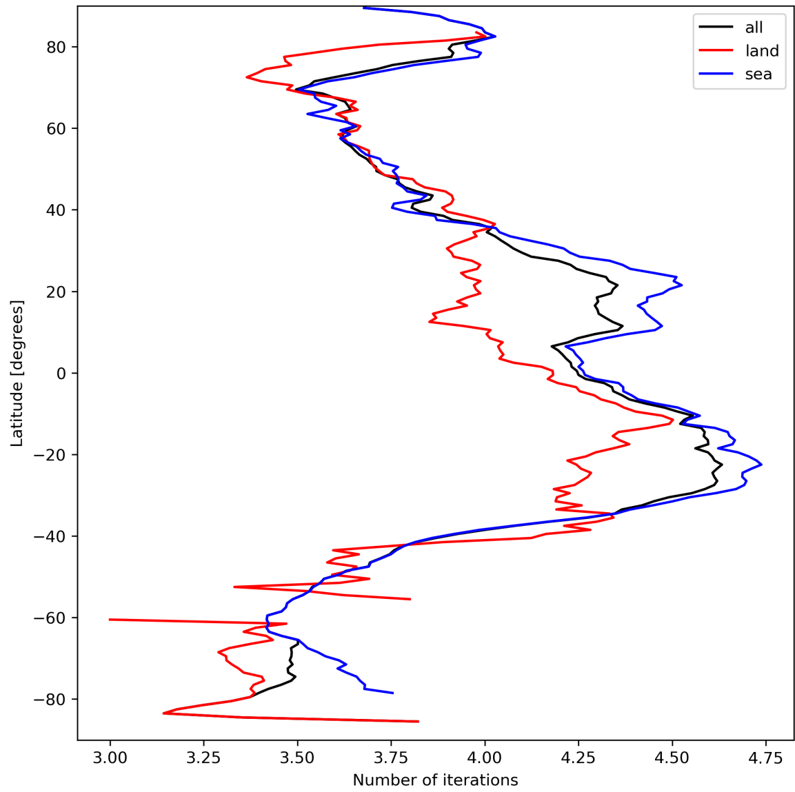
Figure 17: Zonal average of “Number of iterations” for 2024-03-26 to 2024-03-28.
