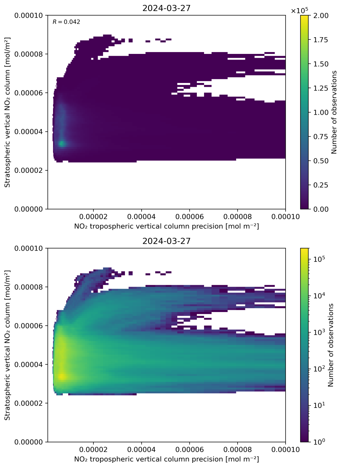
Figure 135: Scatter density plot of “NO 2 tropospheric vertical column precision” against “Stratospheric vertical NO 2 column” for 2024-03-26 to 2024-03-28.
