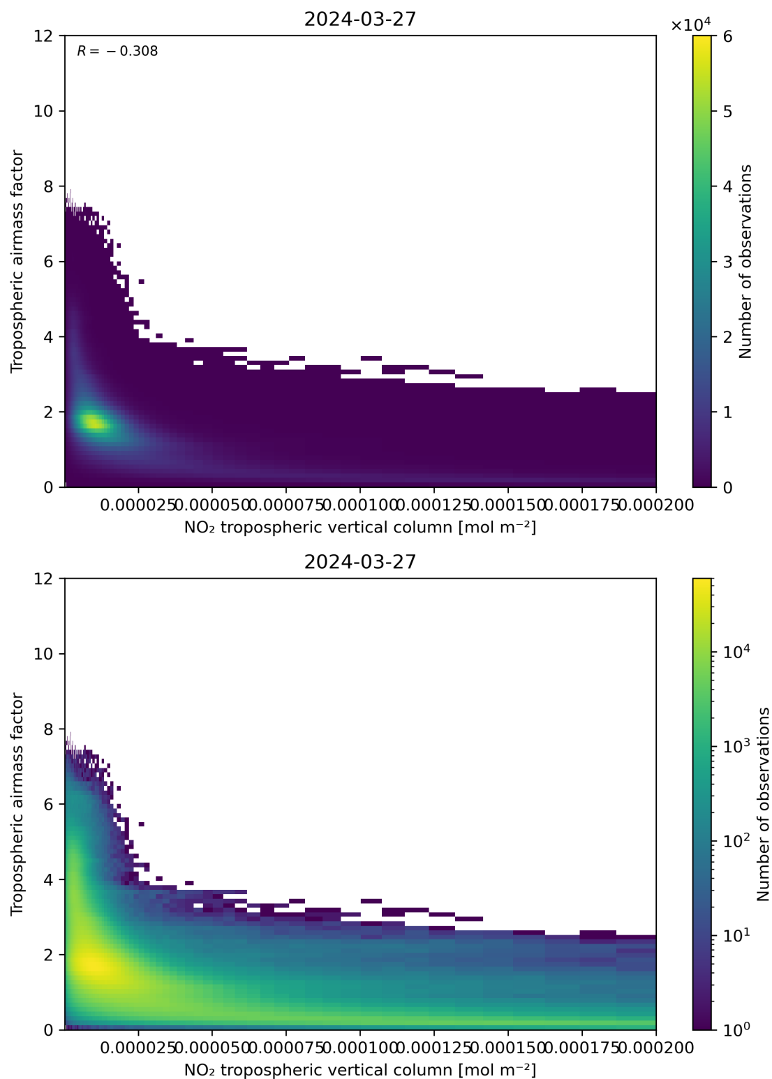
Figure 123: Scatter density plot of “NO 2 tropospheric vertical column” against “Tropospheric airmass factor” for 2024-03-26 to 2024-03-28.
