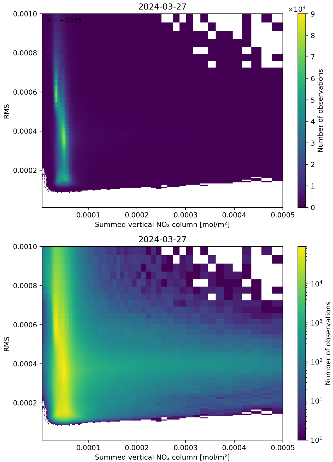
Figure 109: Scatter density plot of “Summed vertical NO 2 column” against “RMS” for 2024-03-26 to 2024-03-28.
