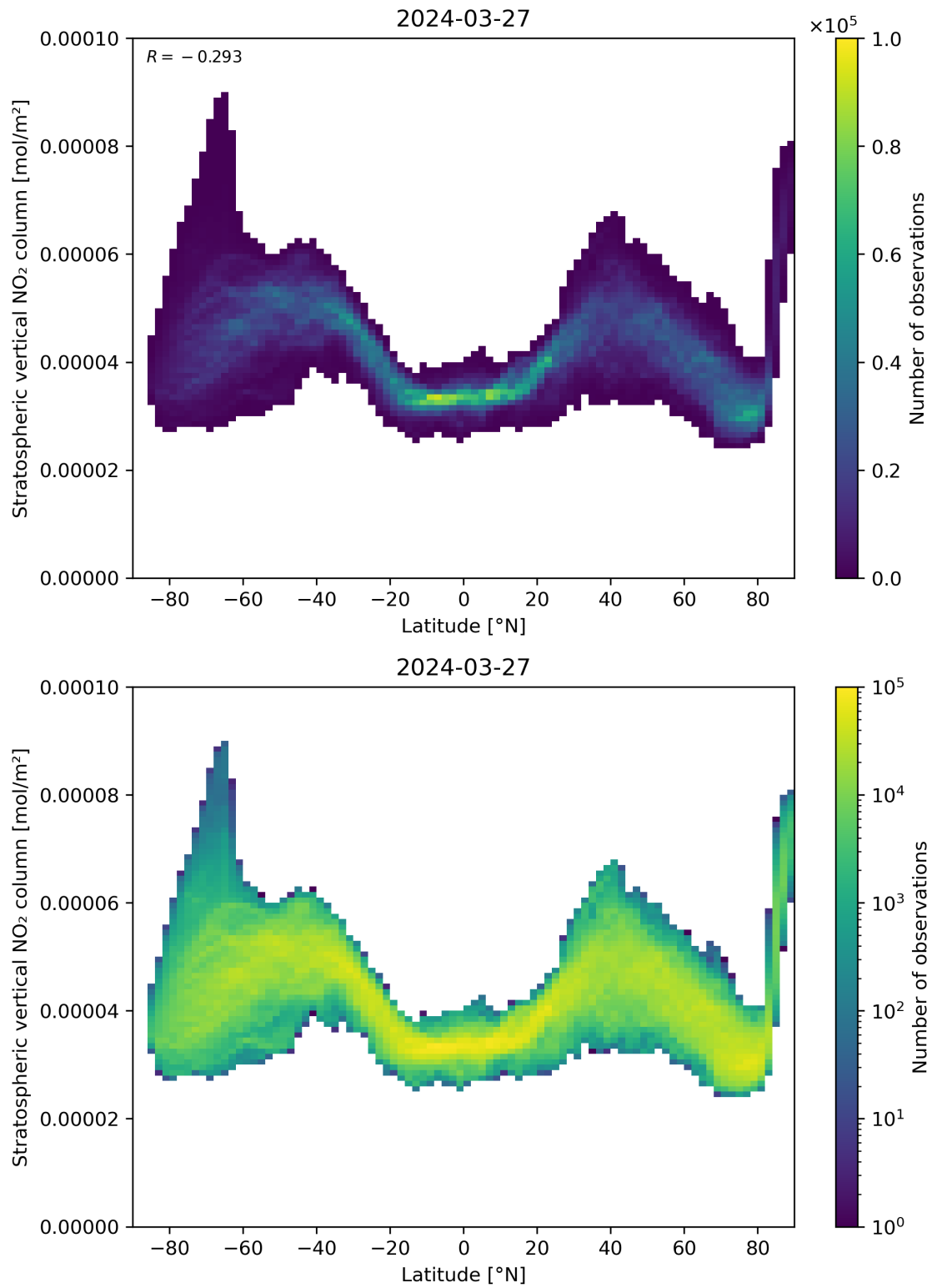
Figure 87: Scatter density plot of “Latitude” against “Stratospheric vertical NO 2 column” for 2024-03-26 to 2024-03-28.
