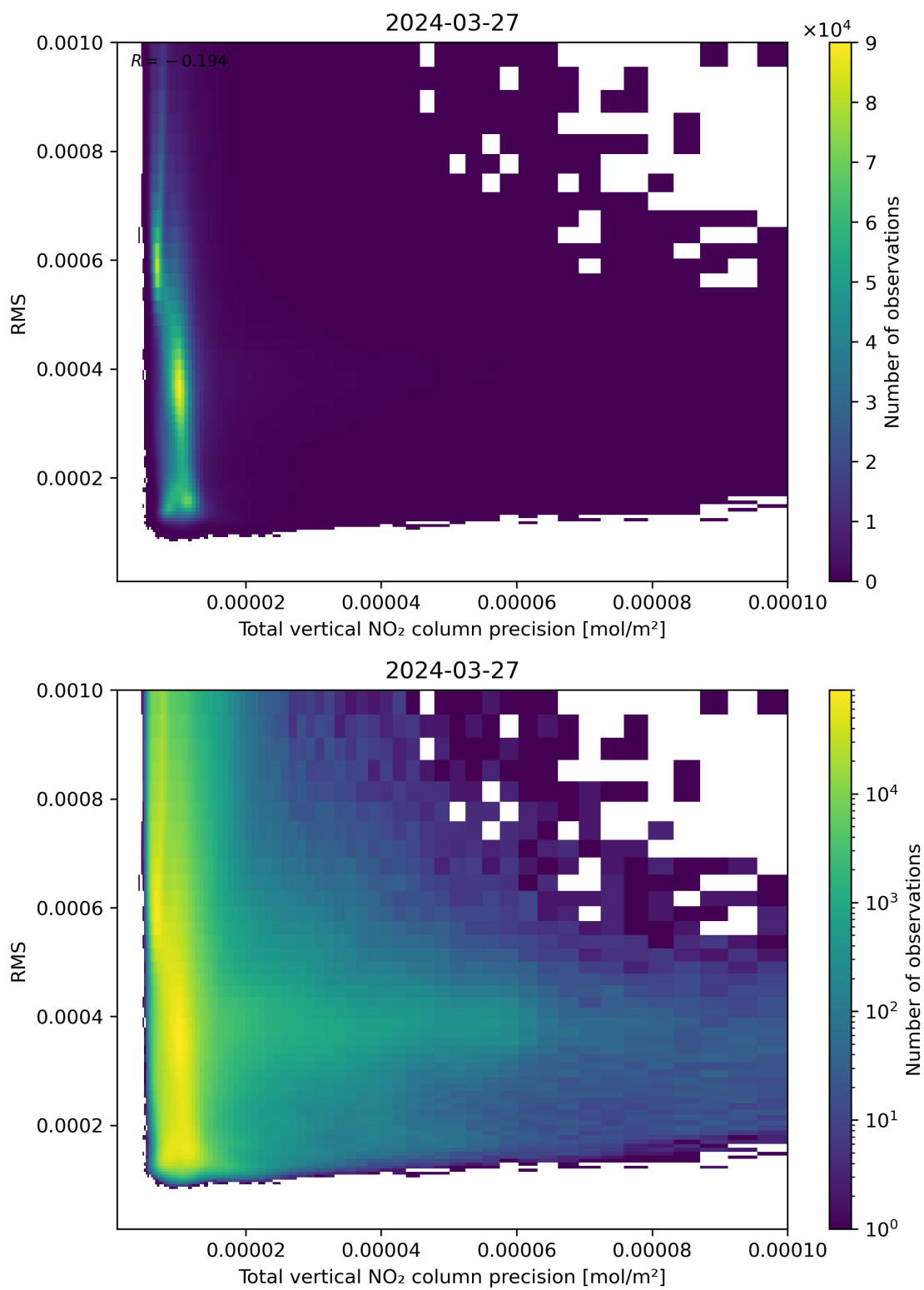
Figure 119: Scatter density plot of “Total vertical NO 2 column precision” against “RMS” for 2024-03-26 to 2024-03-28.
