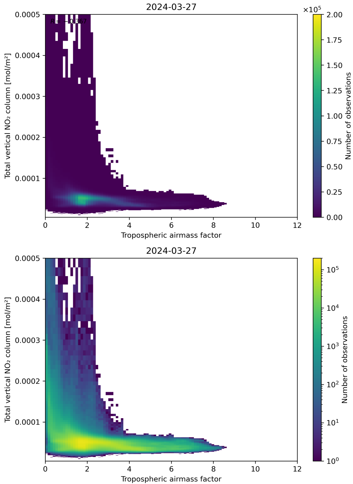
Figure 77: Scatter density plot of “Tropospheric airmass factor” against “Total vertical NO 2 column” for 2024-03-26 to 2024-03-28.
