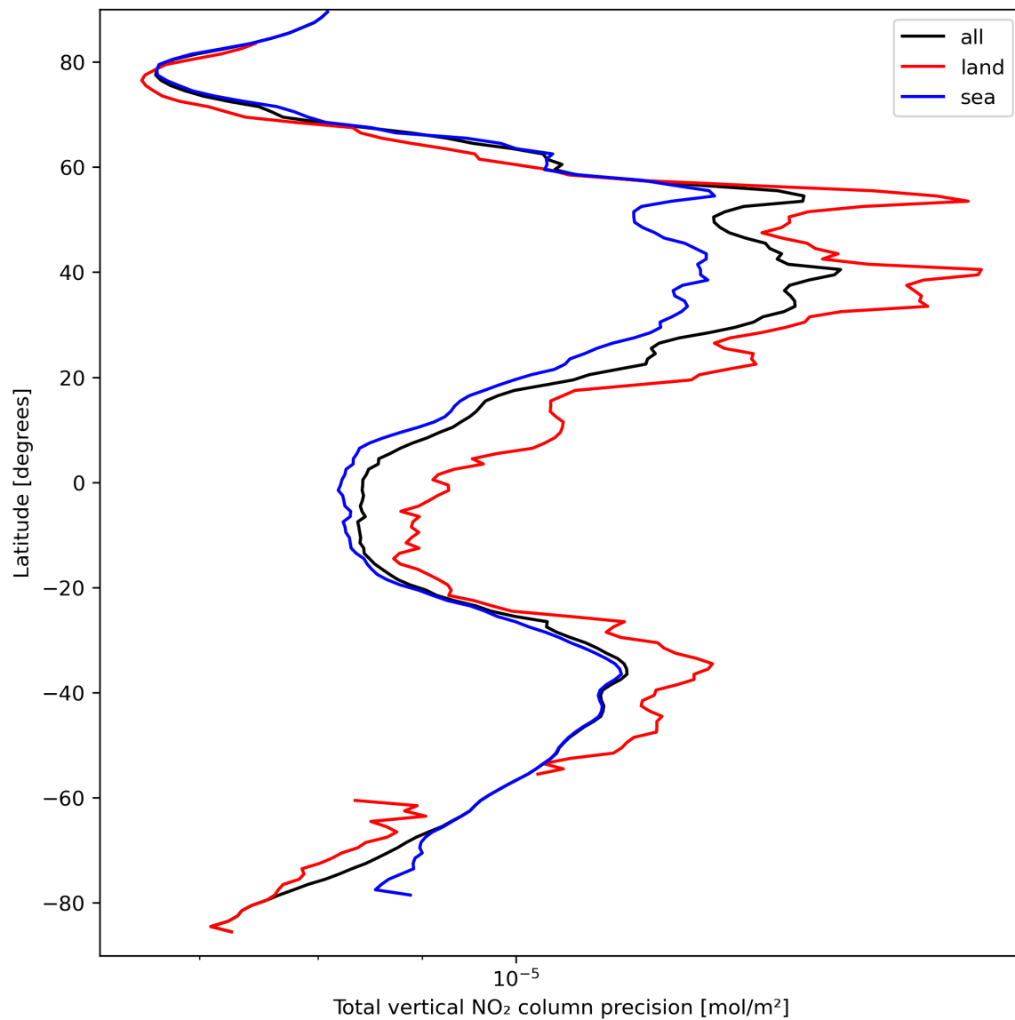
Figure 22: Zonal average of "Total vertical NO 2 column precision" for 2024-03-26 to 2024-03-28.
