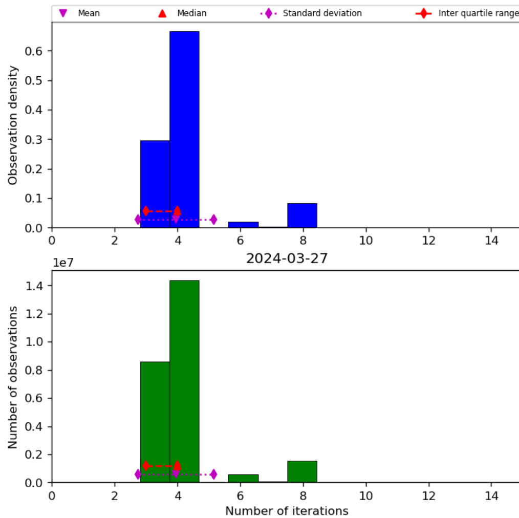
Figure 34: Histogram of “Number of iterations” for 2024-03-26 to 2024-03-28
