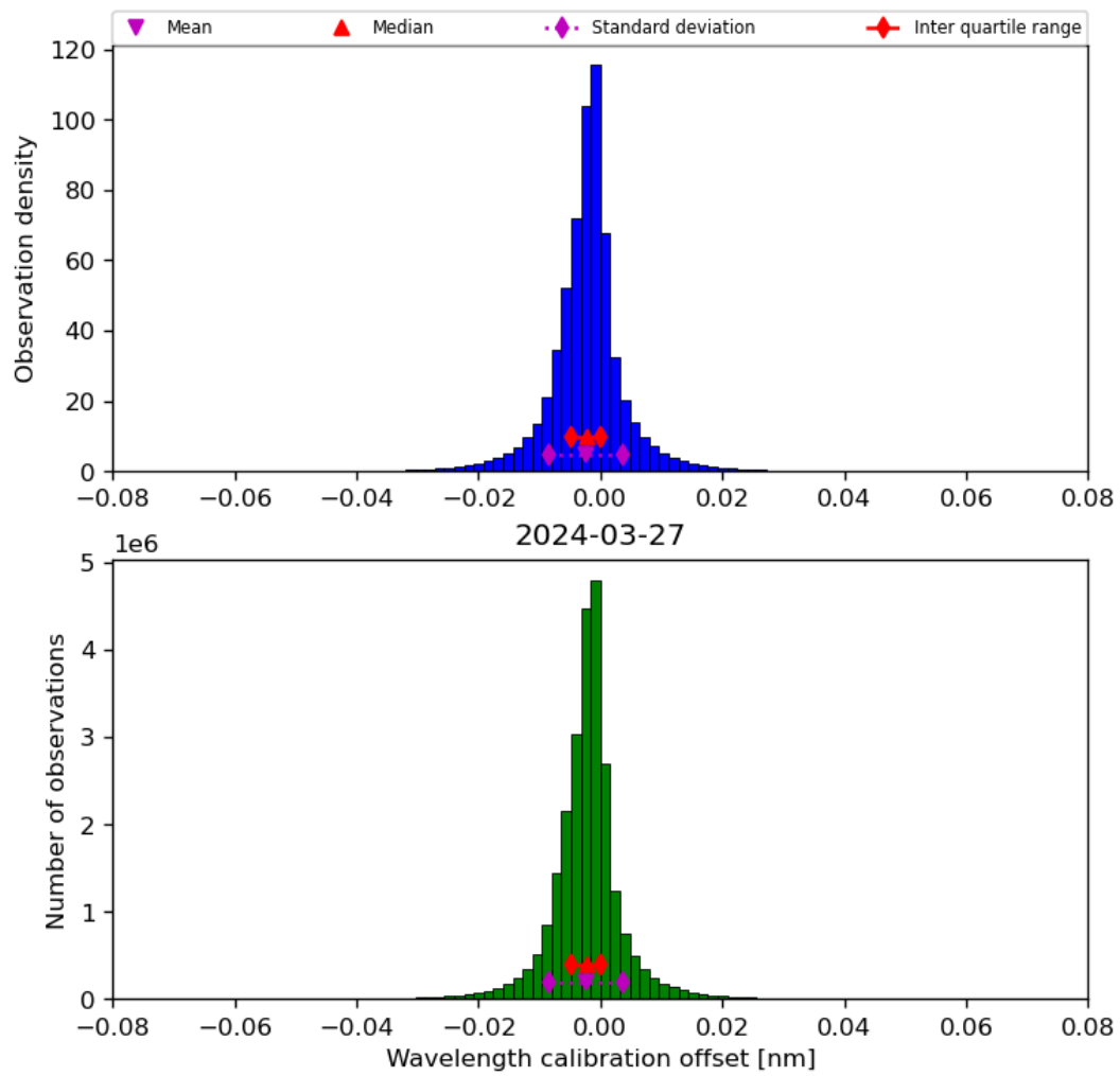
Figure 35: Histogram of “Wavelength calibration offset” for 2024-03-26 to 2024-03-28
