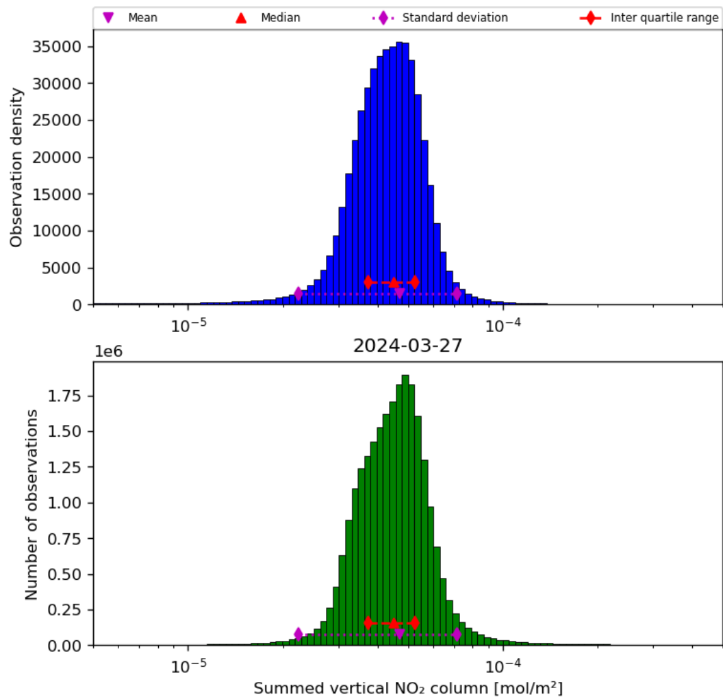
Figure 40: Histogram of “Summed vertical NO 2 column” for 2024-03-26 to 2024-03-28
