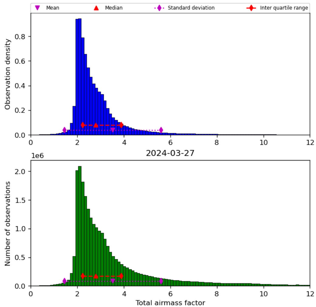
Figure 32: Histogram of “Total airmass factor” for 2024-03-26 to 2024-03-28
