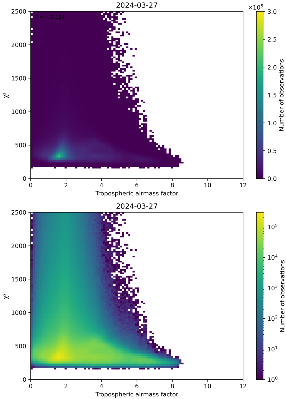
Figure 73: Scatter density plot of “Tropospheric airmass factor” against “ \chi^2 ” for 2024-03-26 to 2024-03-28.
