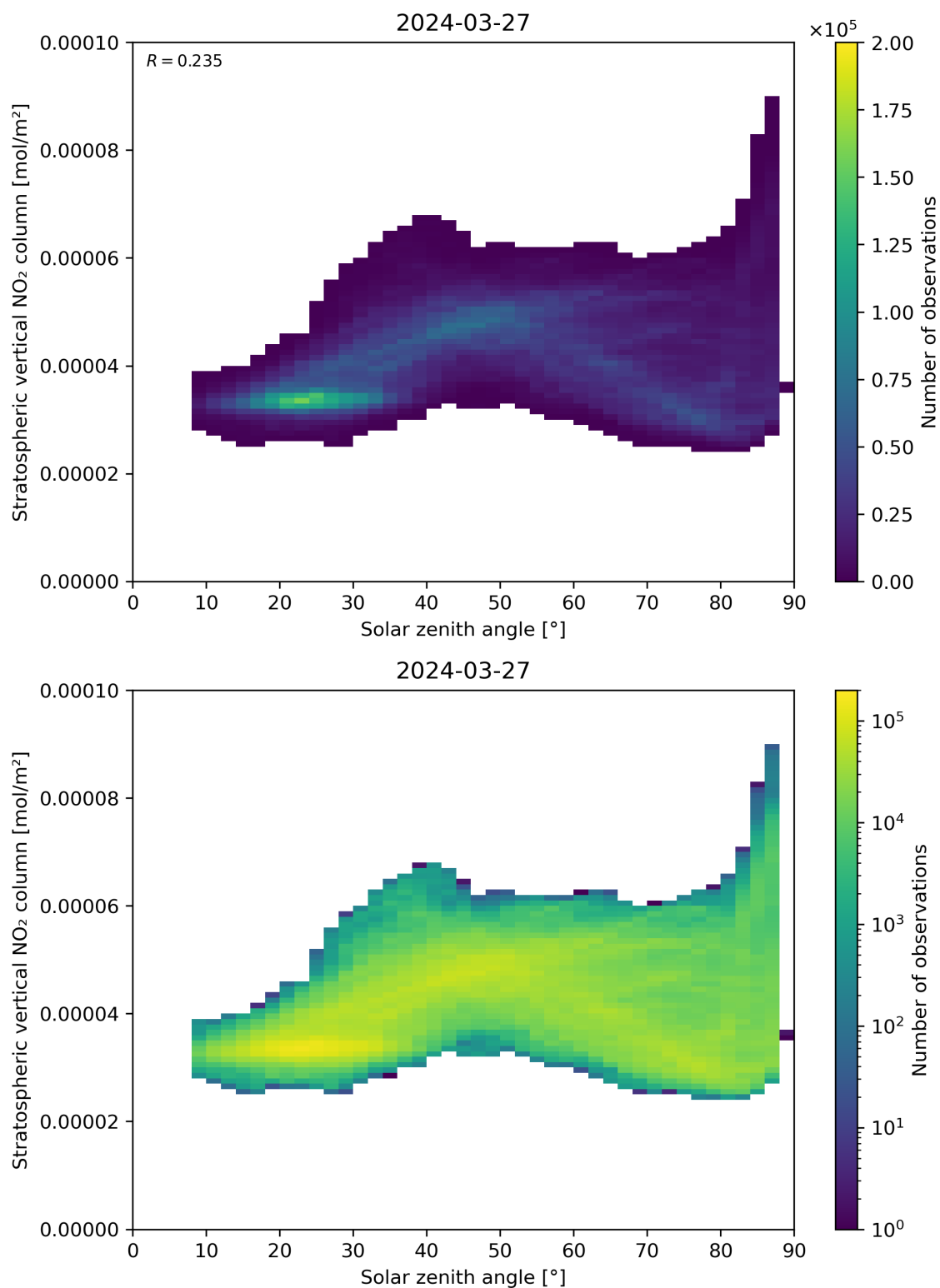
Figure 150: Scatter density plot of “Solar zenith angle” against “Stratospheric vertical NO 2 column” for 2024-03-26 to 2024-03-28.
