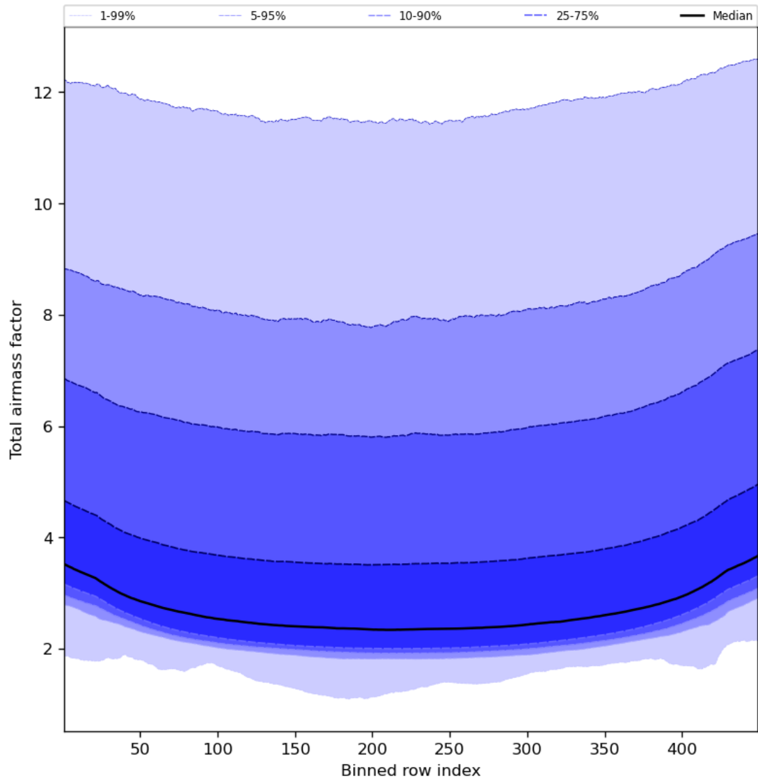
Figure 49: Along track statistics of “Total airmass factor” for 2024-03-26 to 2024-03-28
