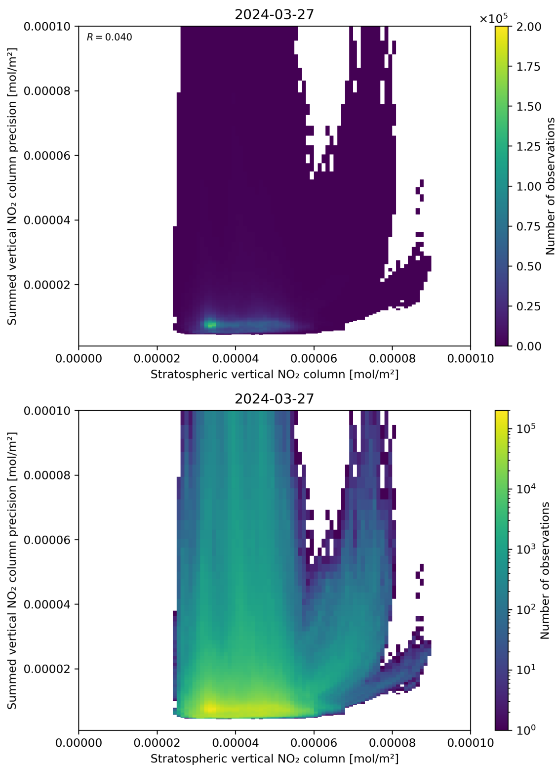
Figure 99: Scatter density plot of “Stratospheric vertical NO 2 column” against “Summed vertical NO 2 column precision” for 2024-03-26 to 2024-03-28.
