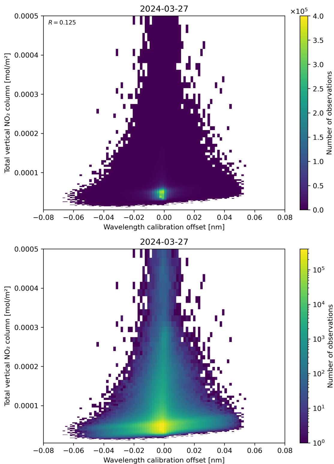
Figure 179: Scatter density plot of “Wavelength calibration offset” against “Total vertical NO 2 column” for 2024-03-26 to 2024-03-28.
