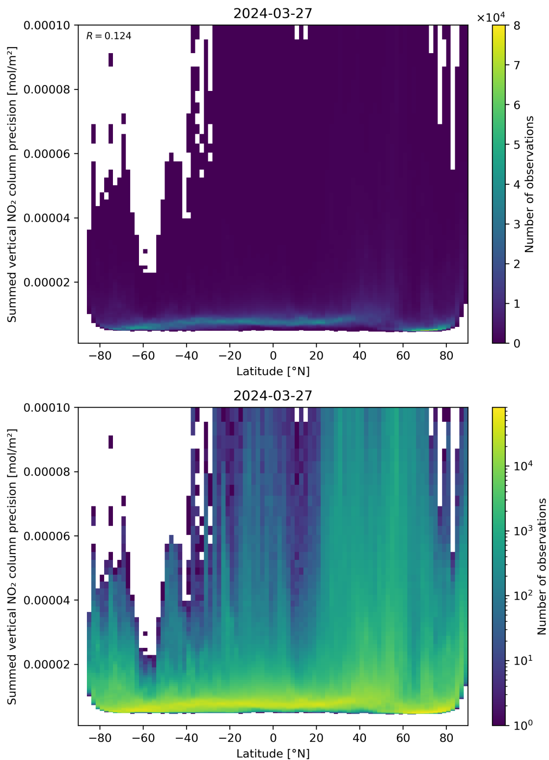
Figure 89: Scatter density plot of “Latitude” against “Summed vertical NO 2 column precision” for 2024-03-26 to 2024-03-28.
