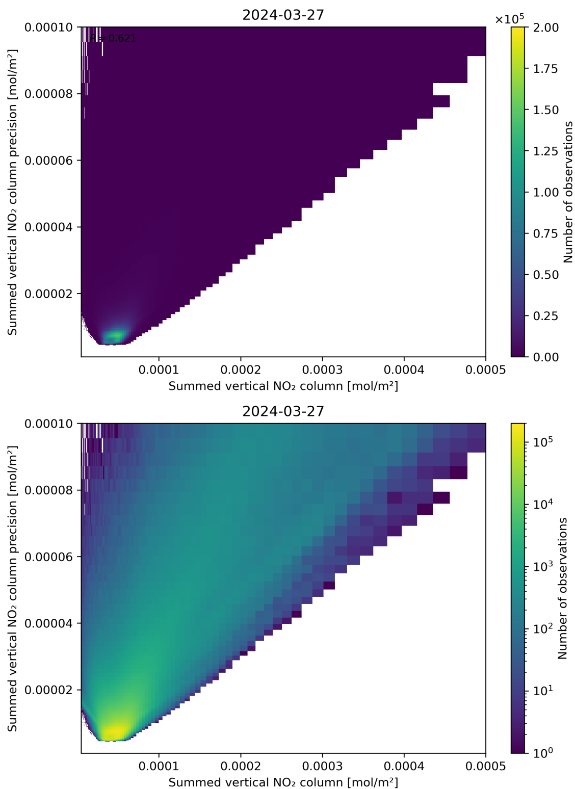
Figure 105: Scatter density plot of “Summed vertical NO 2 column” against “Summed vertical NO 2 column precision” for 2024-03-26 to 2024-03-28.
