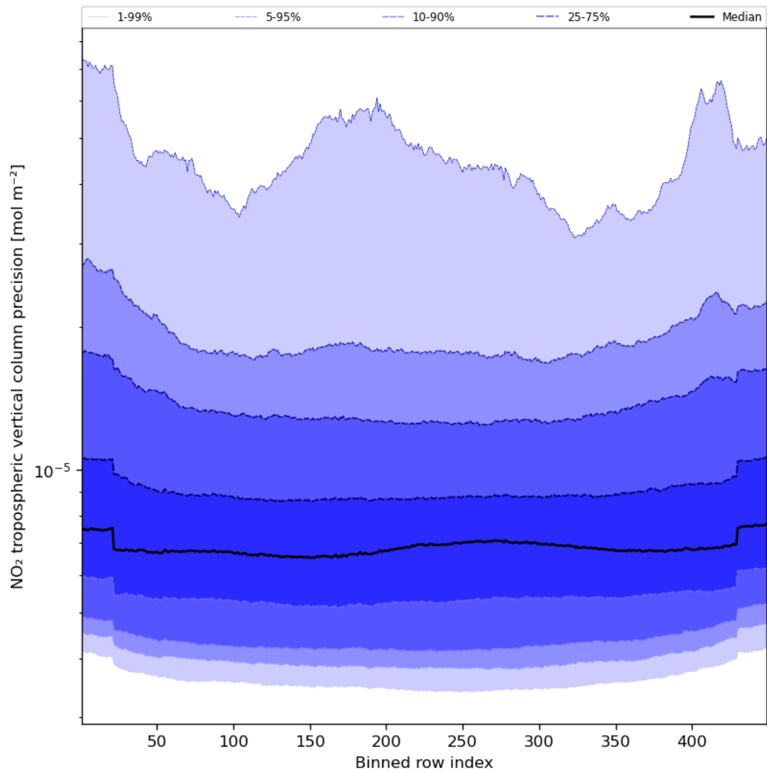
Figure 47: Along track statistics of “NO 2 tropospheric vertical column precision” for 2024-03-26 to 2024-03-28
