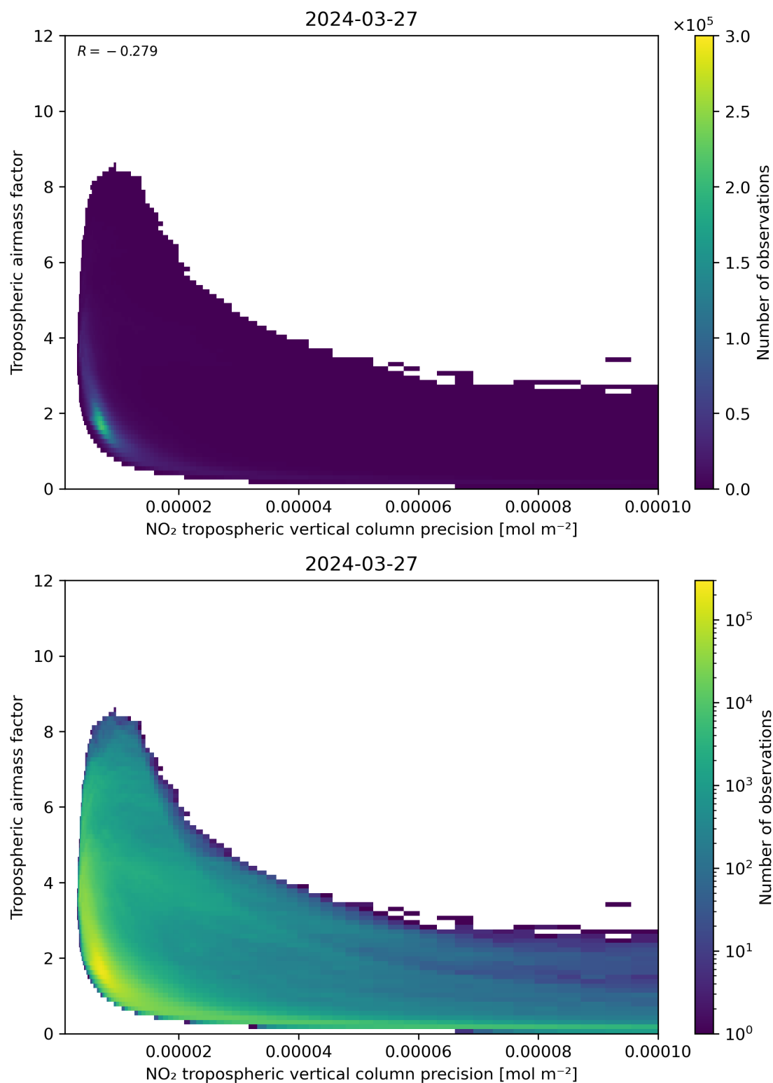
Figure 133: Scatter density plot of “NO 2 tropospheric vertical column precision” against “Tropospheric airmass factor” for 2024-03-26 to 2024-03-28.
