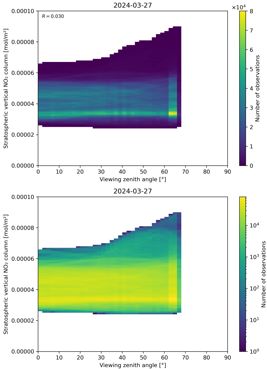
Figure 164: Scatter density plot of “Viewing zenith angle” against “Stratospheric vertical NO 2 column” for 2024-03-26 to 2024-03-28.
