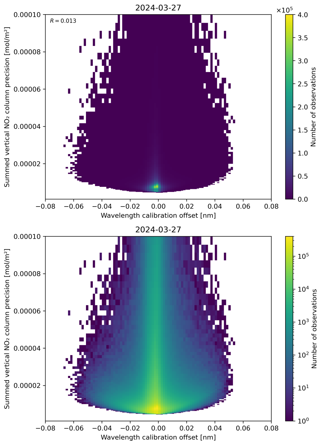
Figure 178: Scatter density plot of “Wavelength calibration offset” against “Summed vertical NO 2 column precision” for 2024-03-26 to 2024-03-28.
