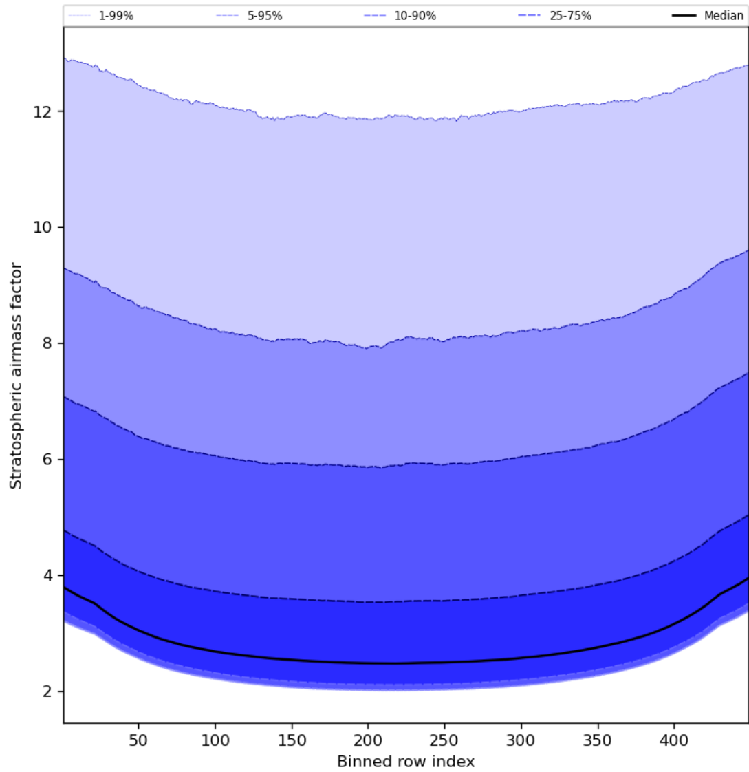
Figure 61: Along track statistics of “Stratospheric airmass factor” for 2024-03-26 to 2024-03-28
