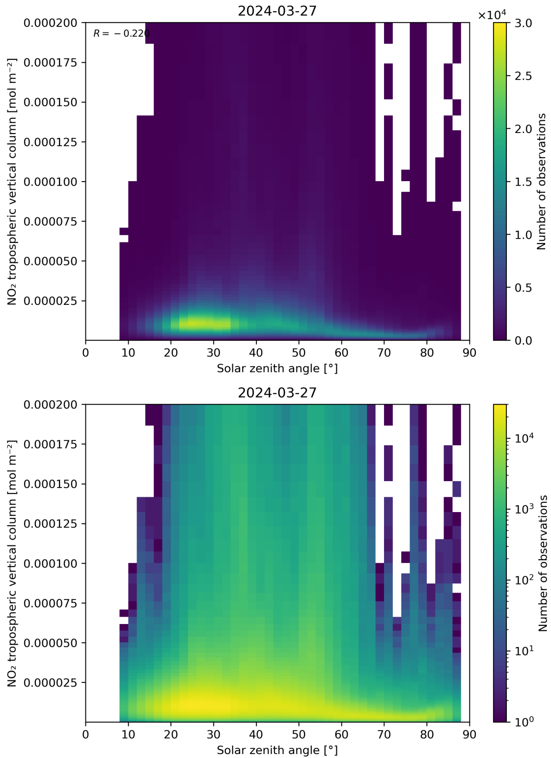
Figure 155: Scatter density plot of “Solar zenith angle” against “NO 2 tropospheric vertical column” for 2024-03-26 to 2024-03-28.
