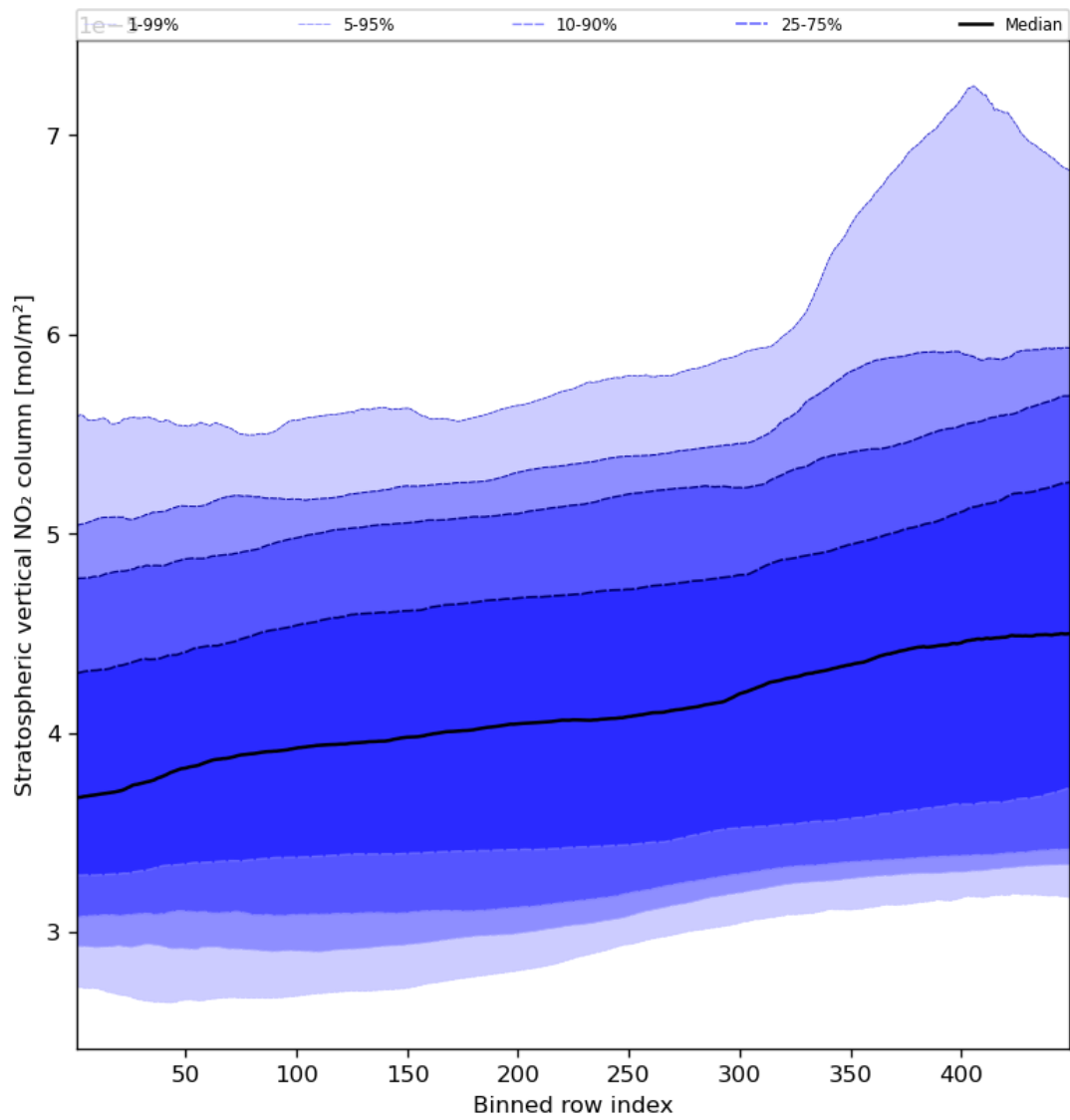
Figure 53: Along track statistics of “Stratospheric vertical NO 2 column” for 2024-03-26 to 2024-03-28
