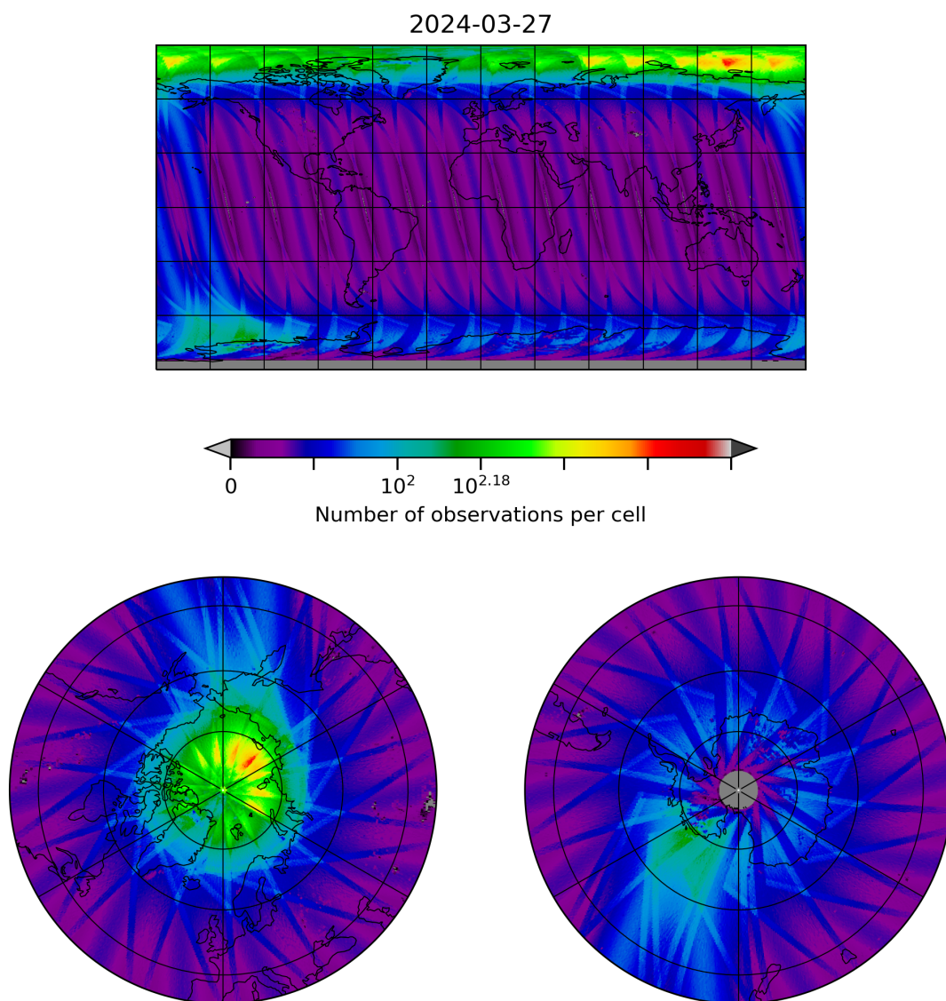
Figure 10: Map of the number of observations for 2024-03-26 to 2024-03-28
