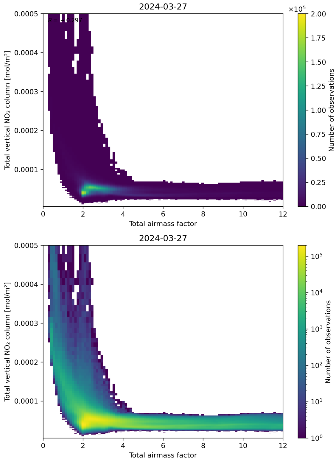
Figure 67: Scatter density plot of “Total airmass factor” against “Total vertical NO 2 column” for 2024-03-26 to 2024-03-28.
