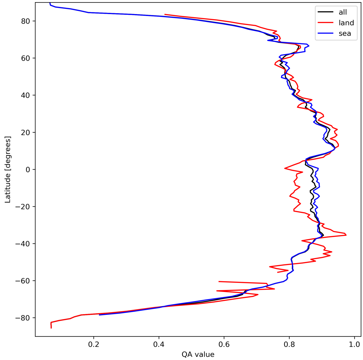
Figure 11: Zonal average of “QA value” for 2024-03-26 to 2024-03-28.
