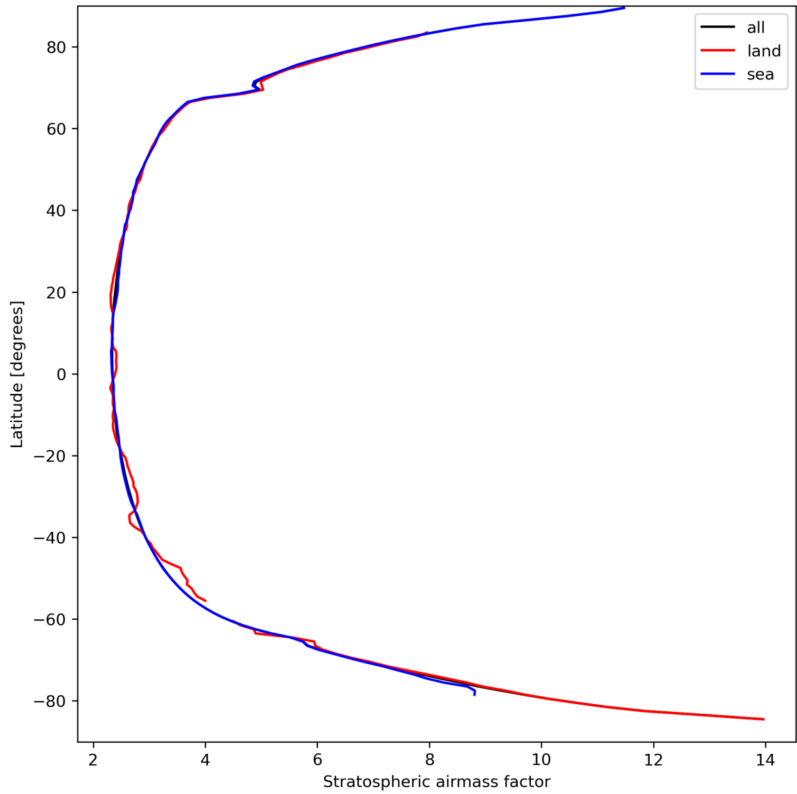
Figure 27: Zonal average of “Stratospheric air mass factor” for 2024-03-27 to 2024-03-29.
