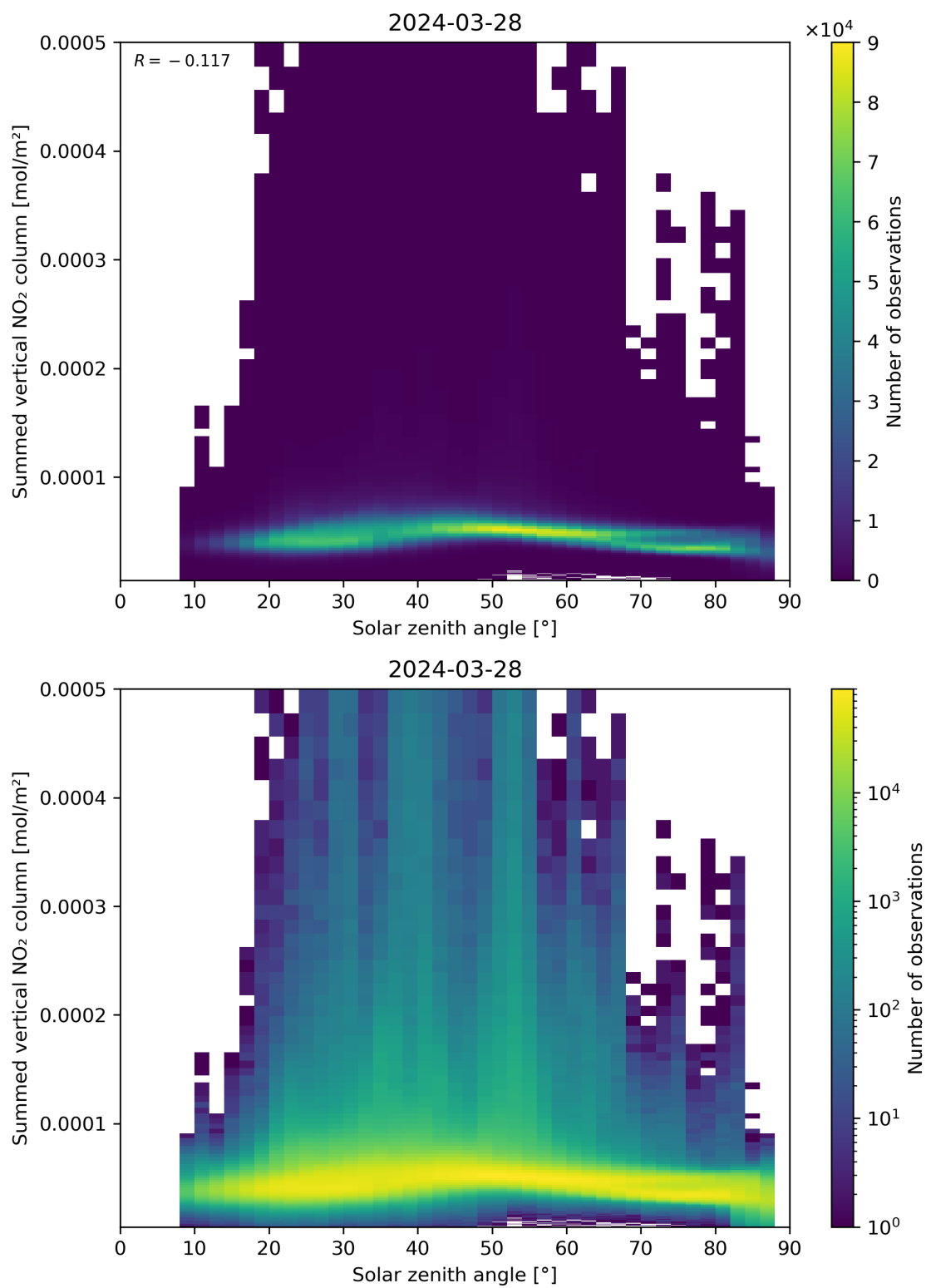
Figure 151: Scatter density plot of “Solar zenith angle” against “Summed vertical NO 2 column” for 2024-03-27 to 2024-03-29.
