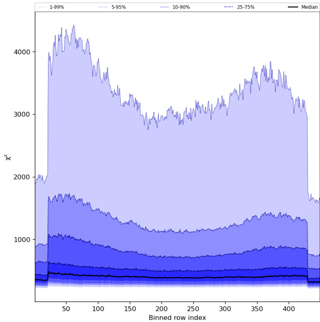
Figure 59: Along track statistics of “ \chi^2 ” for 2024-03-27 to 2024-03-29
