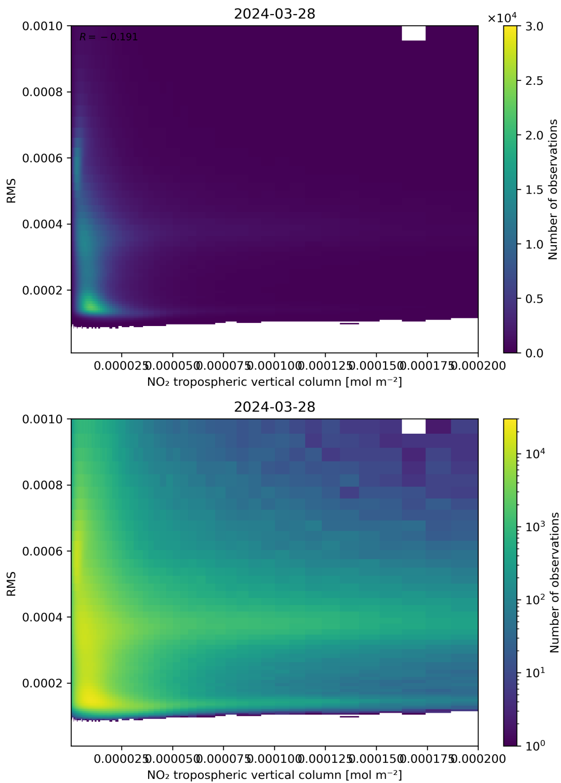
Figure 142: Scatter density plot of “NO 2 tropospheric vertical column” against “RMS” for 2024-03-27 to 2024-03-29.
