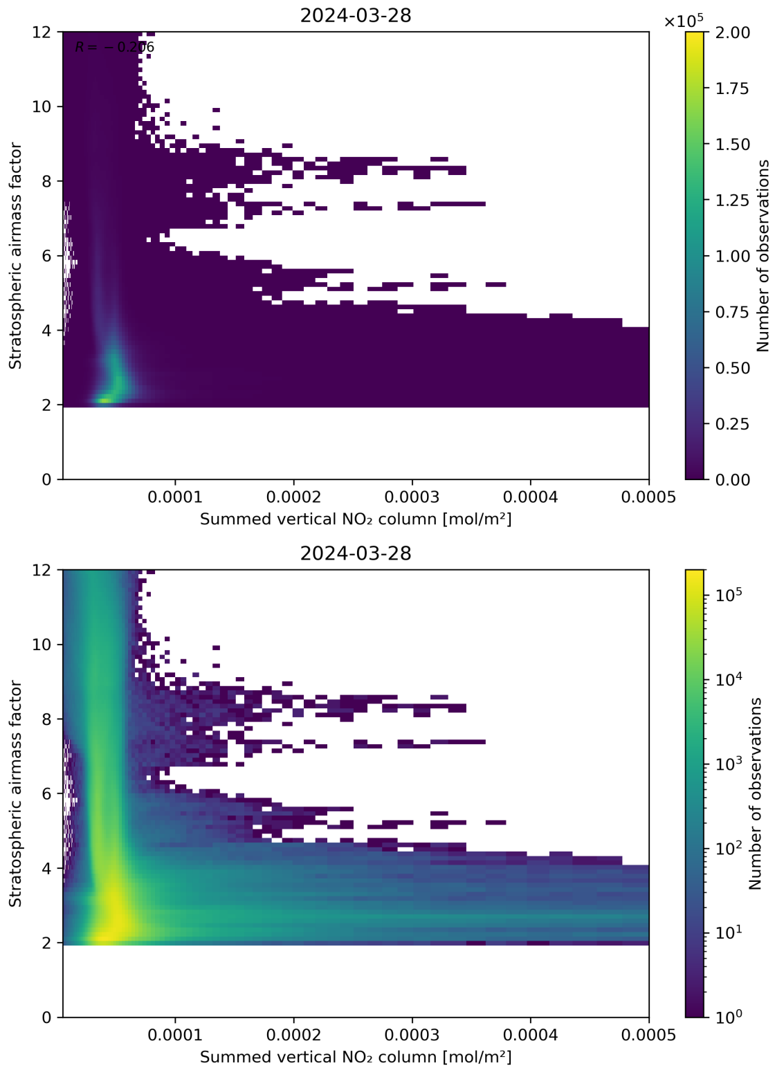
Figure 103: Scatter density plot of “Summed vertical NO 2 column” against “Stratospheric air mass factor” for 2024-03-27 to 2024-03-29.
