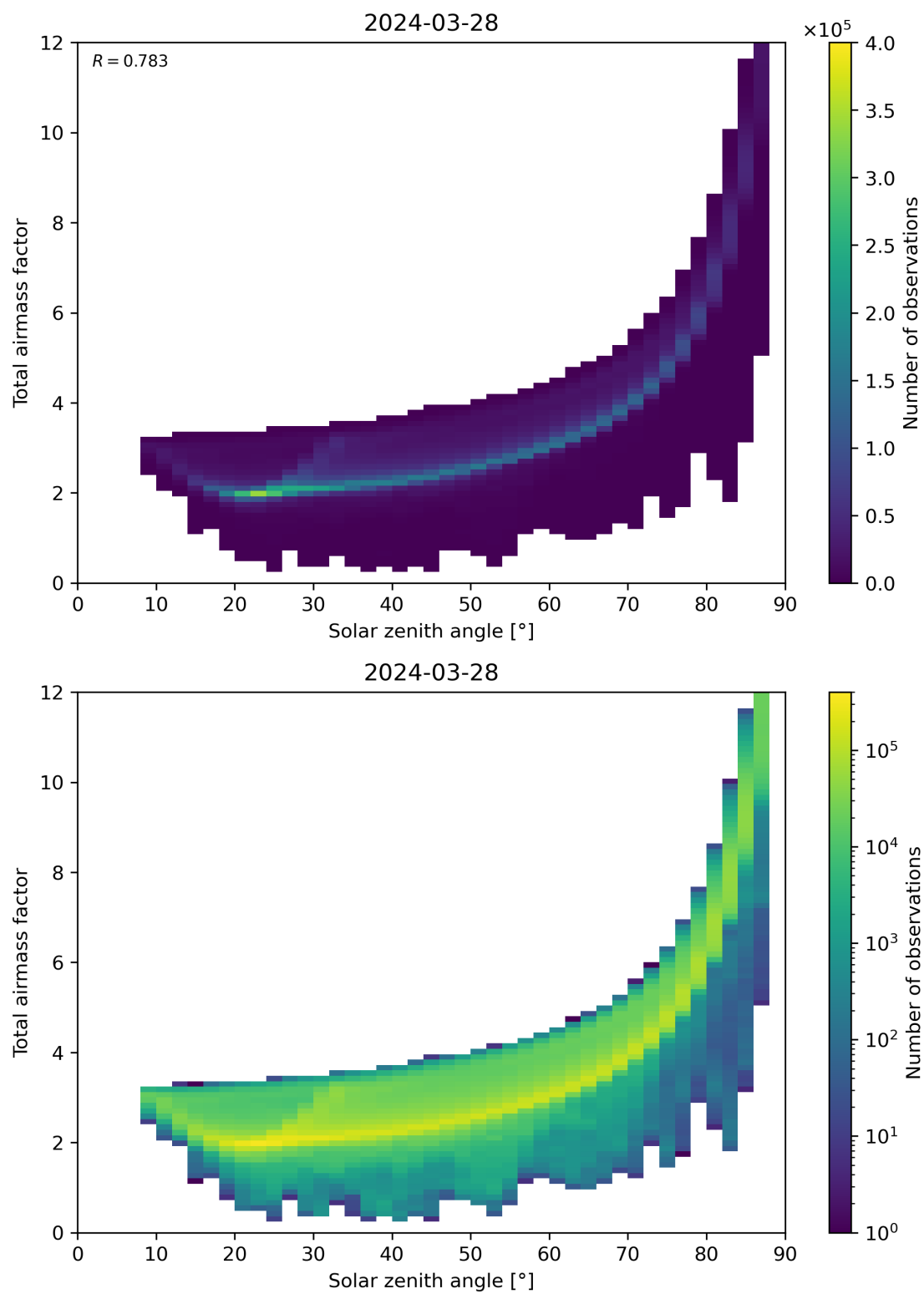
Figure 146: Scatter density plot of “Solar zenith angle” against “Total air mass factor” for 2024-03-27 to 2024-03-29.
