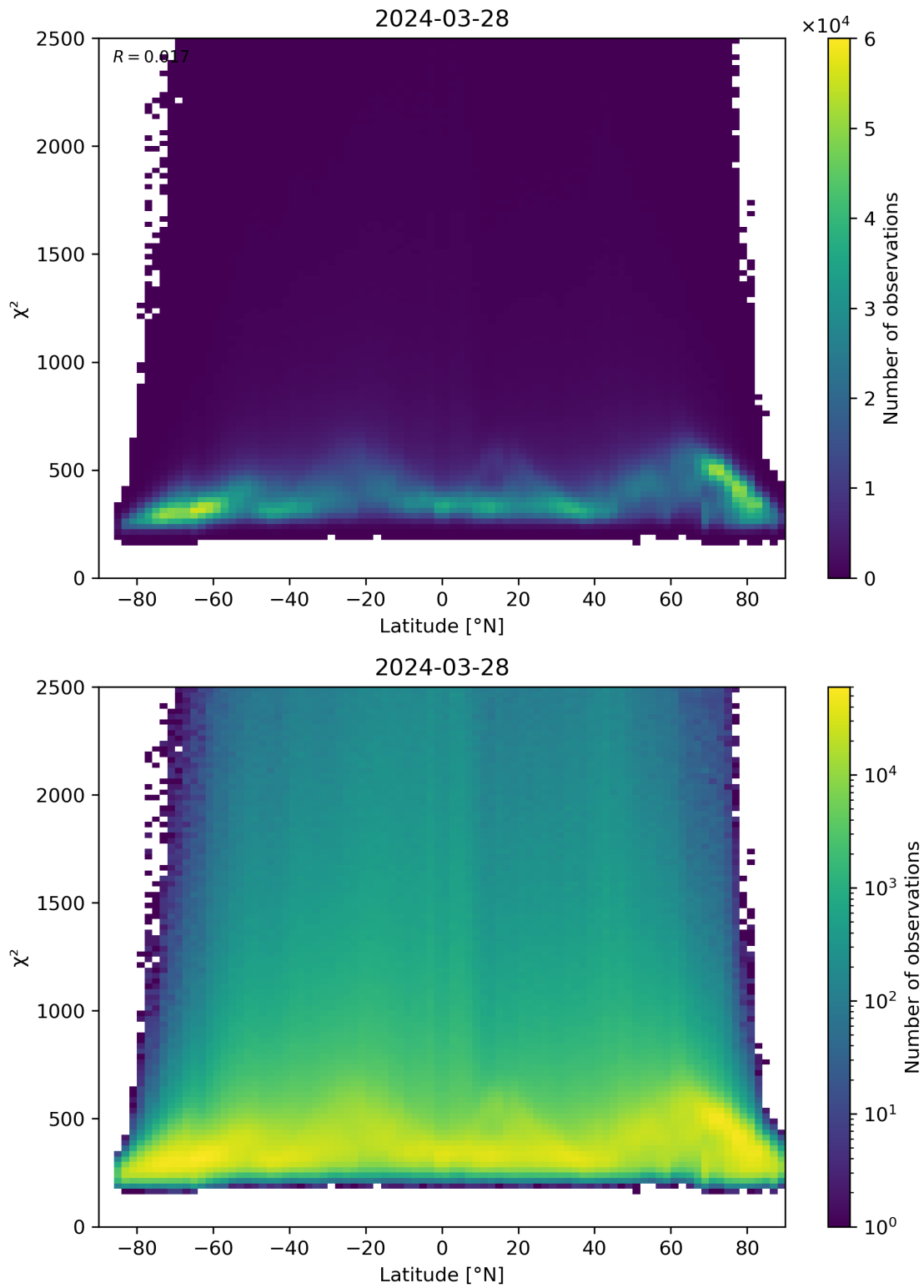
Figure 86: Scatter density plot of “Latitude” against “ \chi^2 ” for 2024-03-27 to 2024-03-29.
