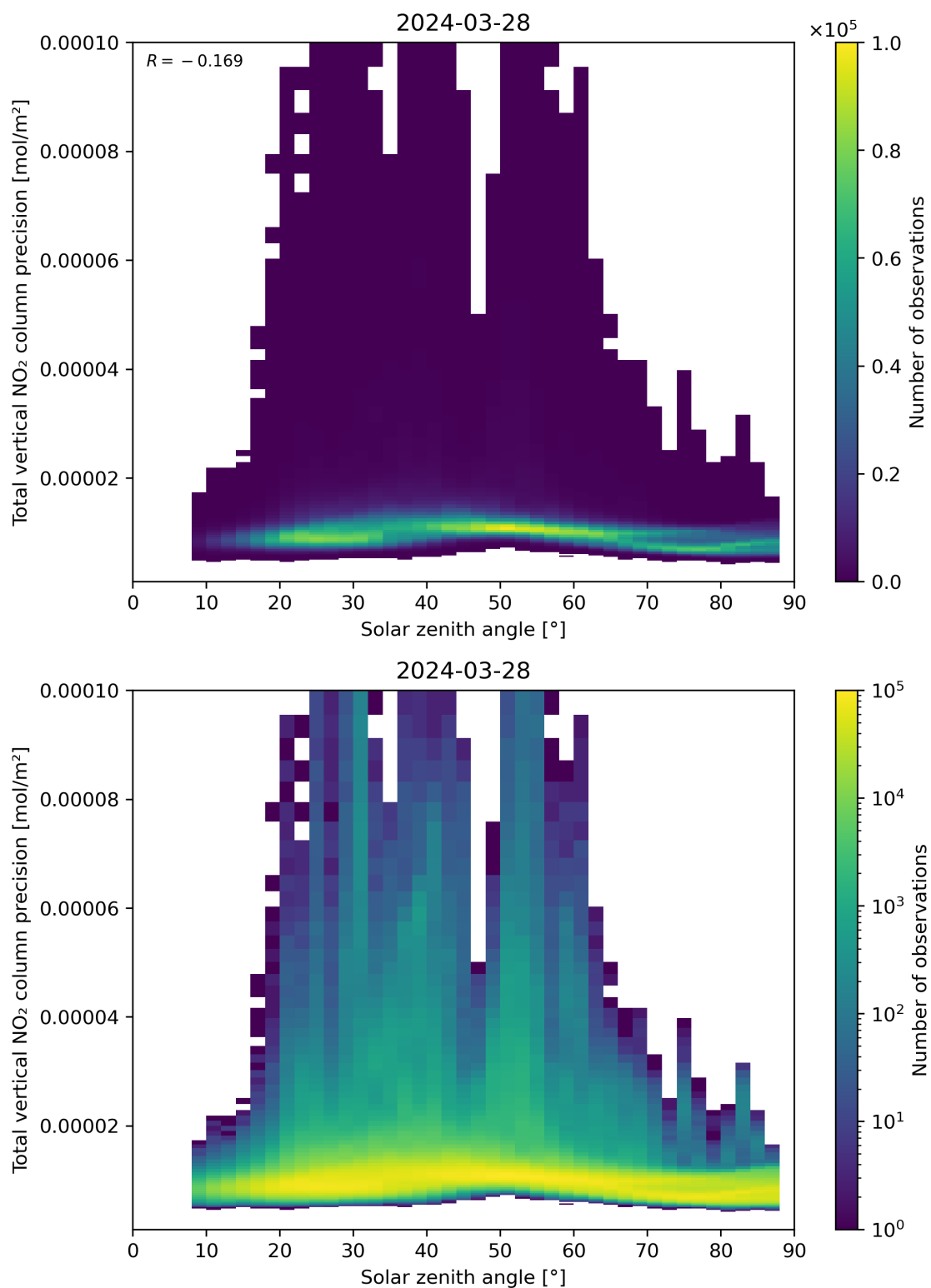
Figure 154: Scatter density plot of “Solar zenith angle” against “Total vertical NO 2 column precision” for 2024-03-27 to 2024-03-29.
