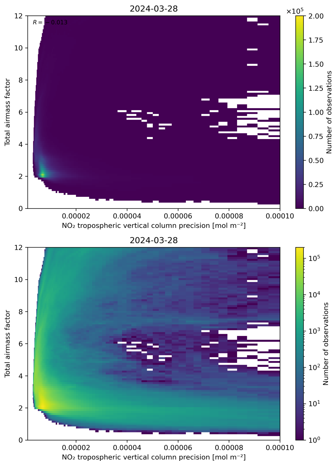
Figure 132: Scatter density plot of “NO 2 tropospheric vertical column precision” against “Total air mass factor” for 2024-03-27 to 2024-03-29.
