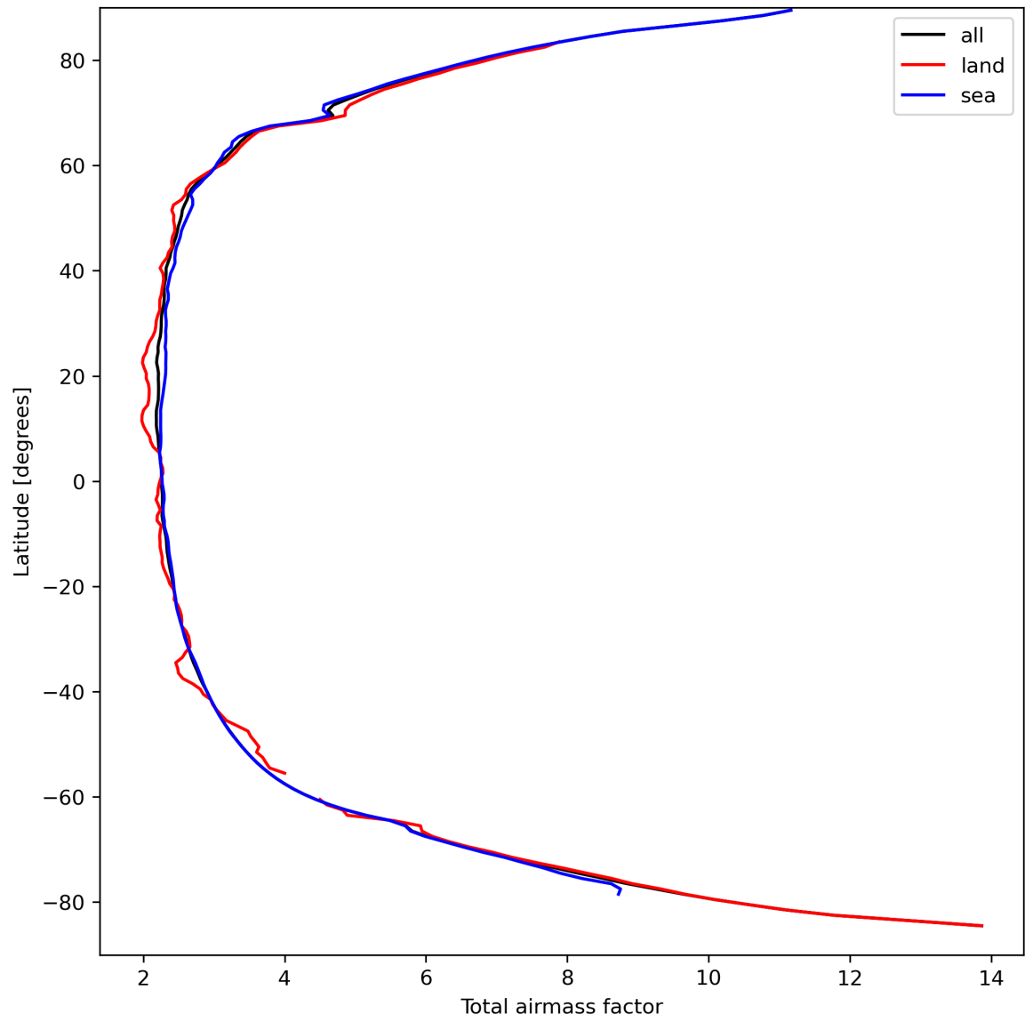
Figure 15: Zonal average of “Total airmass factor” for 2024-03-27 to 2024-03-29.
