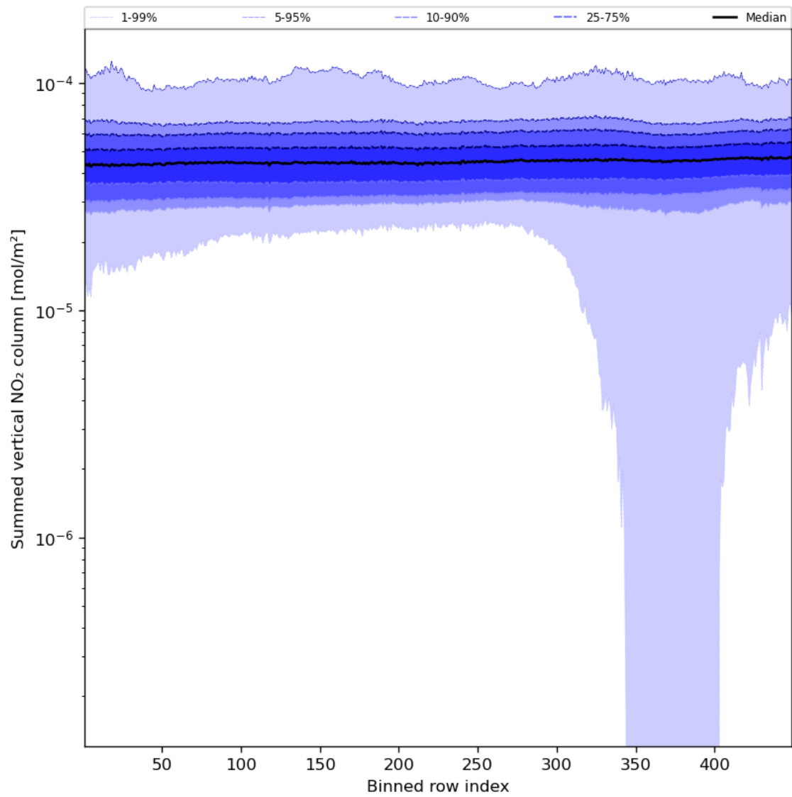
Figure 57: Along track statistics of “Summed vertical NO 2 column” for 2024-03-27 to 2024-03-29
