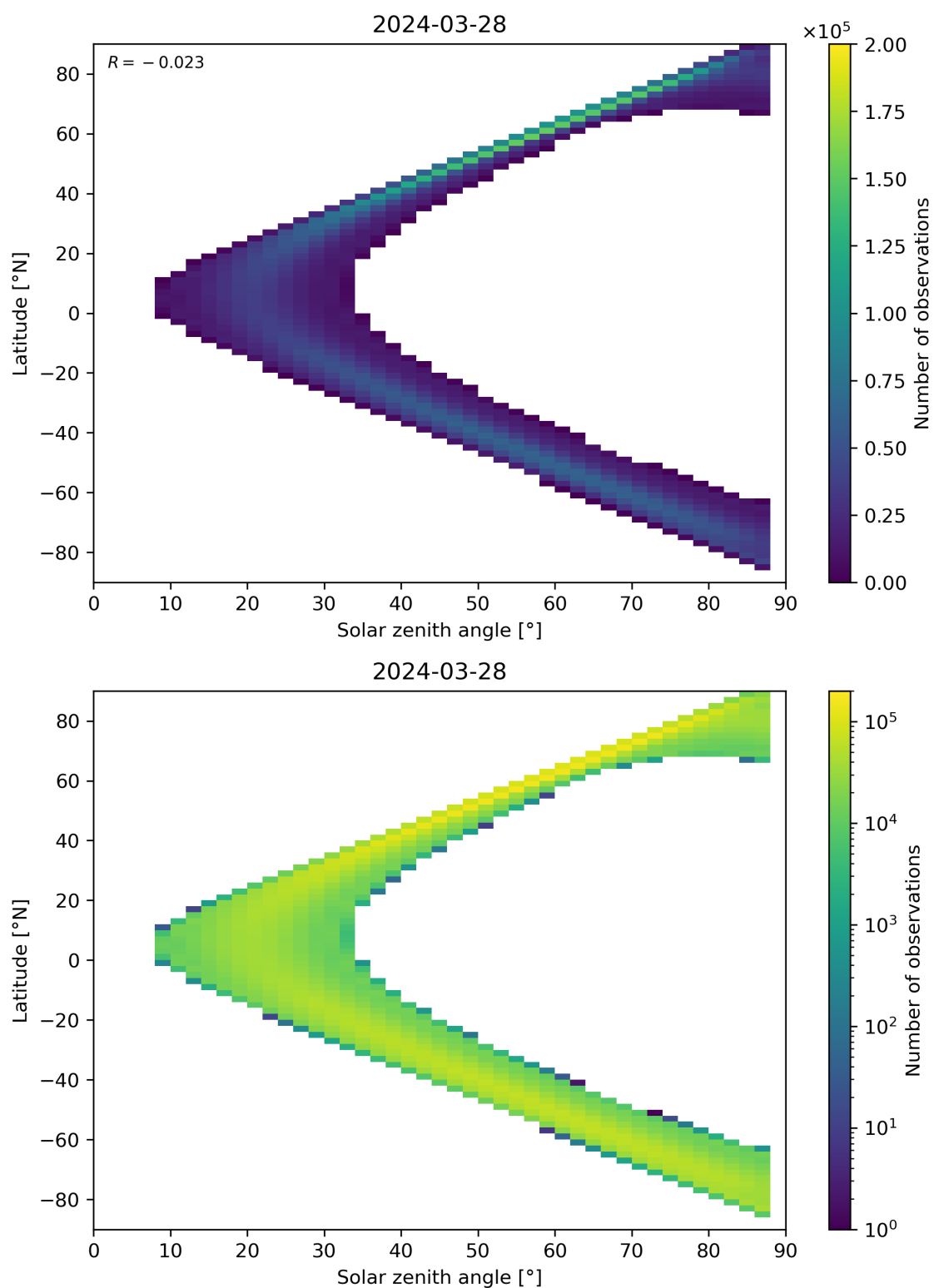
Figure 149: Scatter density plot of “Solar zenith angle” against “Latitude” for 2024-03-27 to 2024-03-29.
