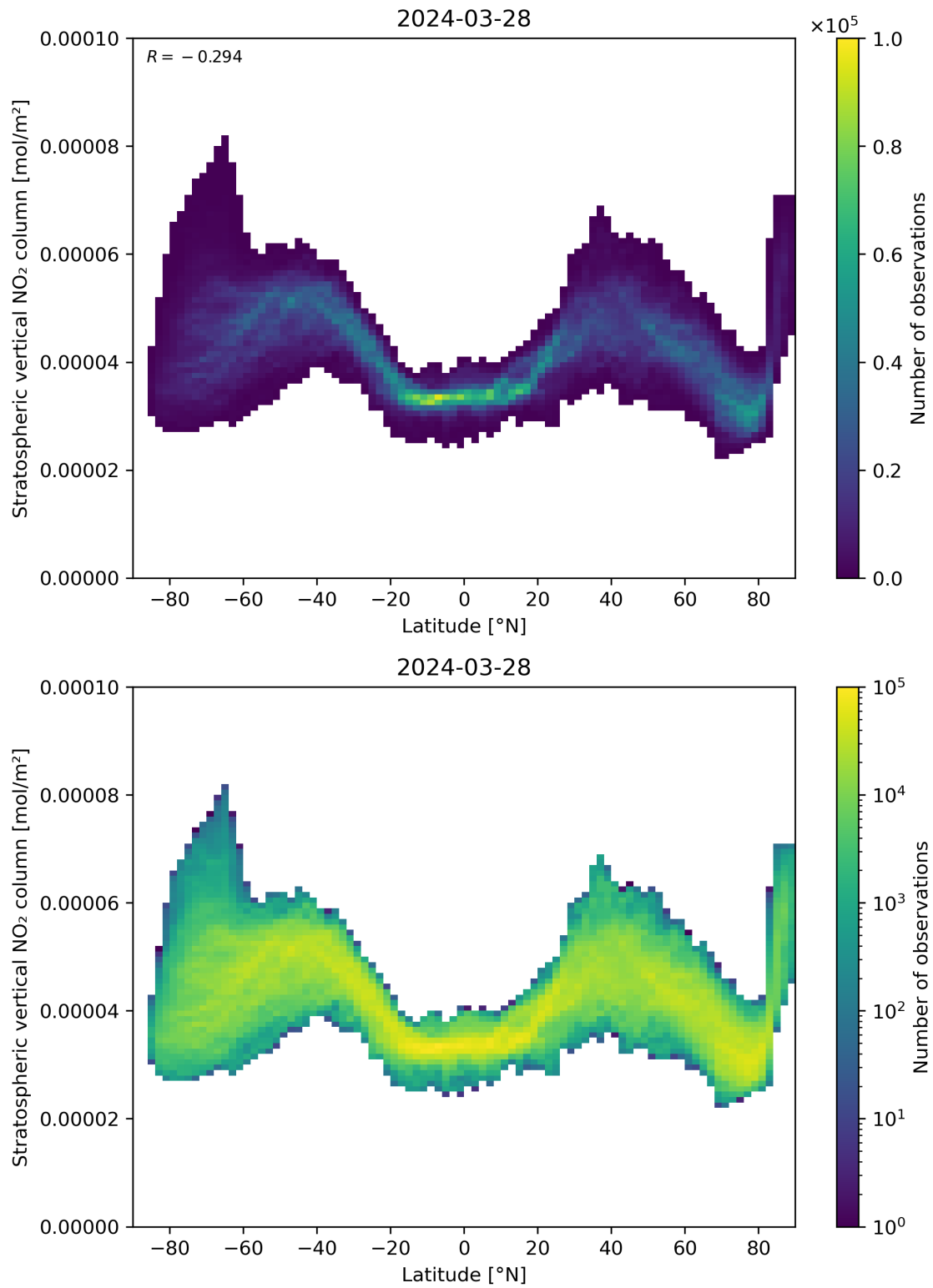
Figure 87: Scatter density plot of “Latitude” against “Stratospheric vertical NO 2 column” for 2024-03-27 to 2024-03-29.
