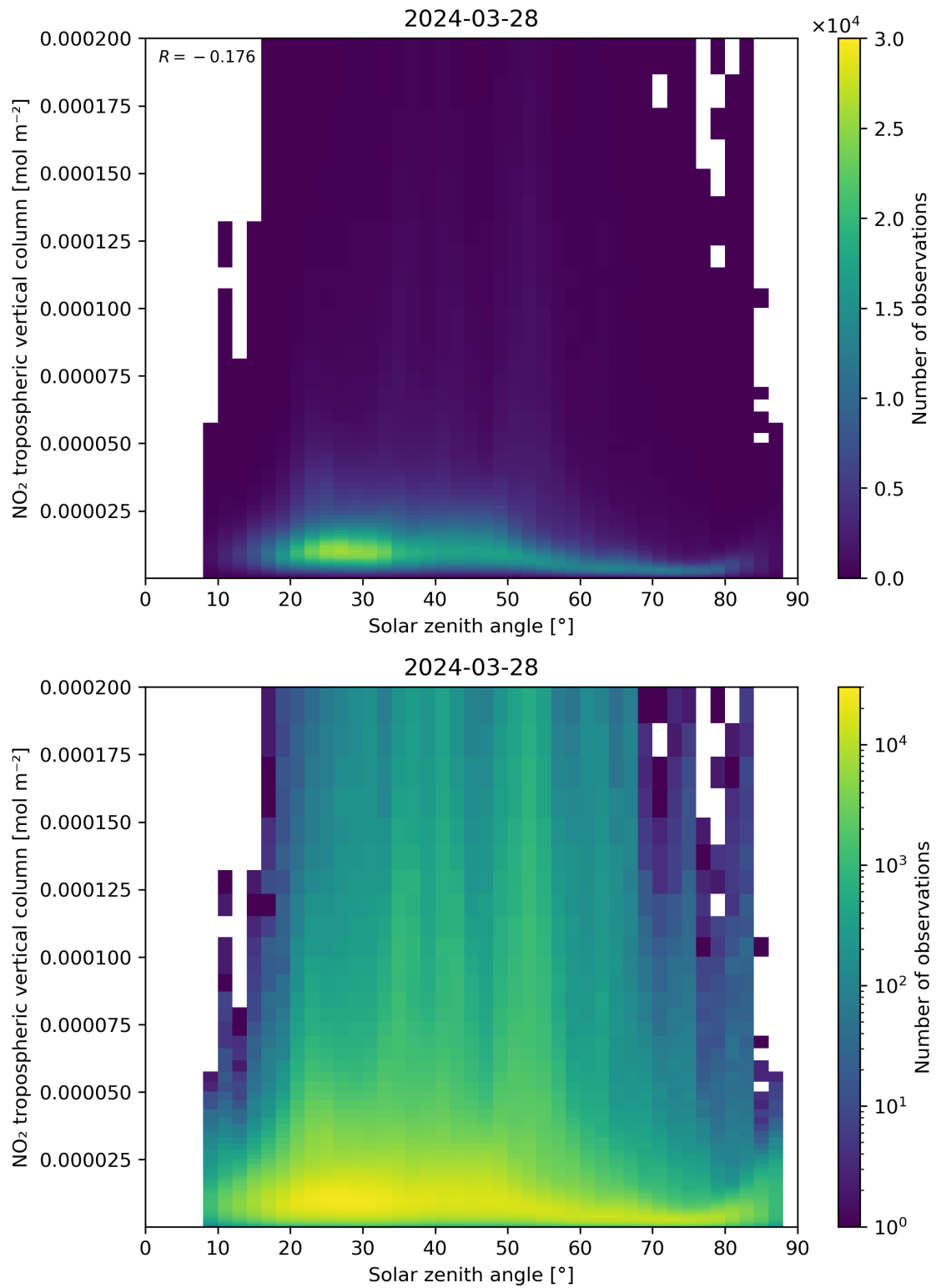
Figure 155: Scatter density plot of “Solar zenith angle” against “NO 2 tropospheric vertical column” for 2024-03-27 to 2024-03-29.
