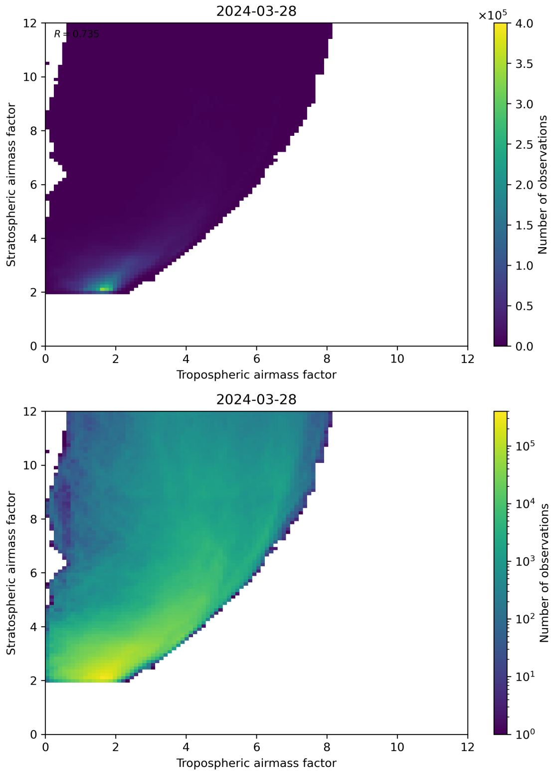
Figure 71: Scatter density plot of “Tropospheric airmass factor” against “Stratospheric airmass factor” for 2024-03-27 to 2024-03-29.
