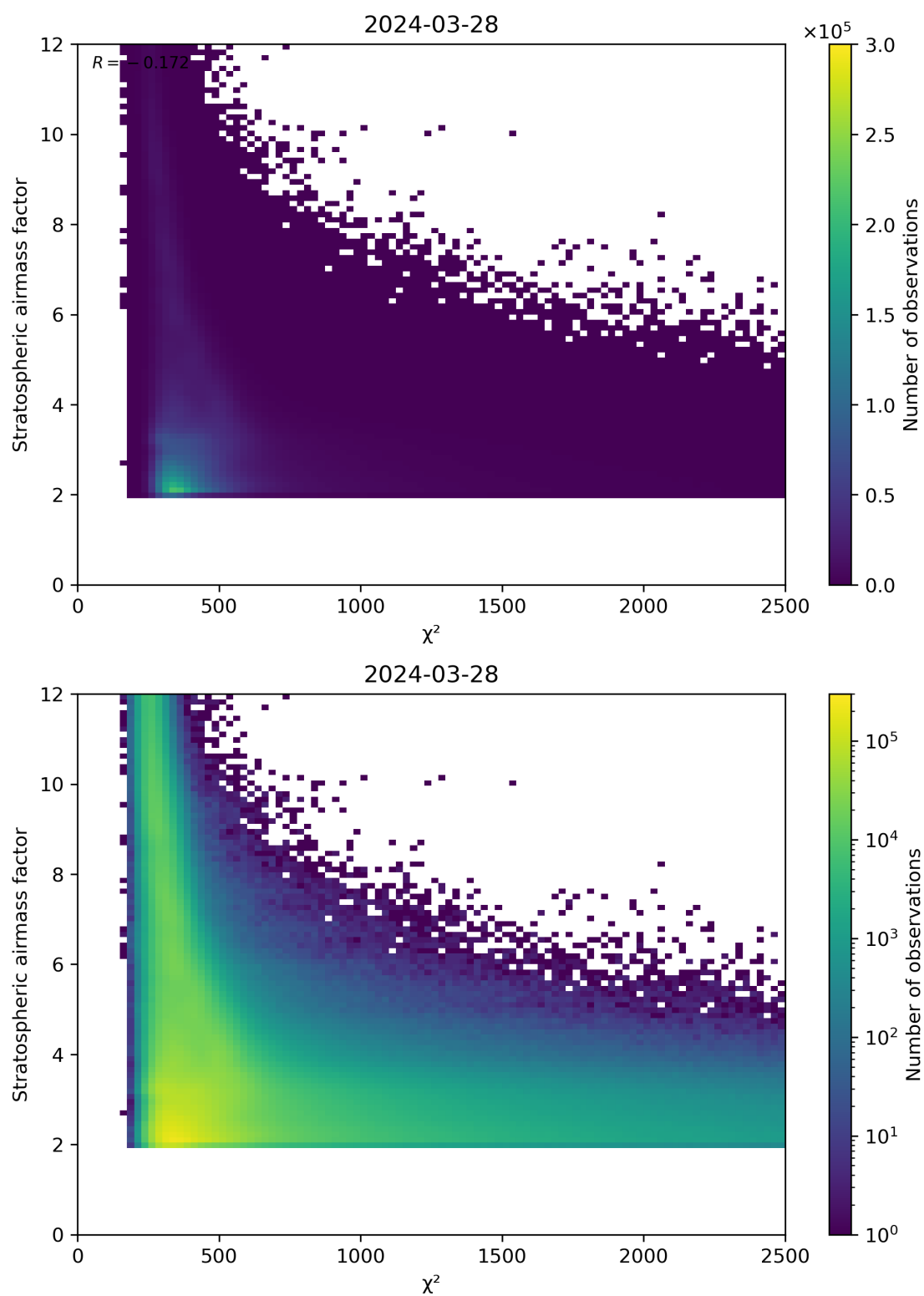
Figure 81: Scatter density plot of “ \chi^2 ” against “Stratospheric airmass factor” for 2024-03-27 to 2024-03-29.
