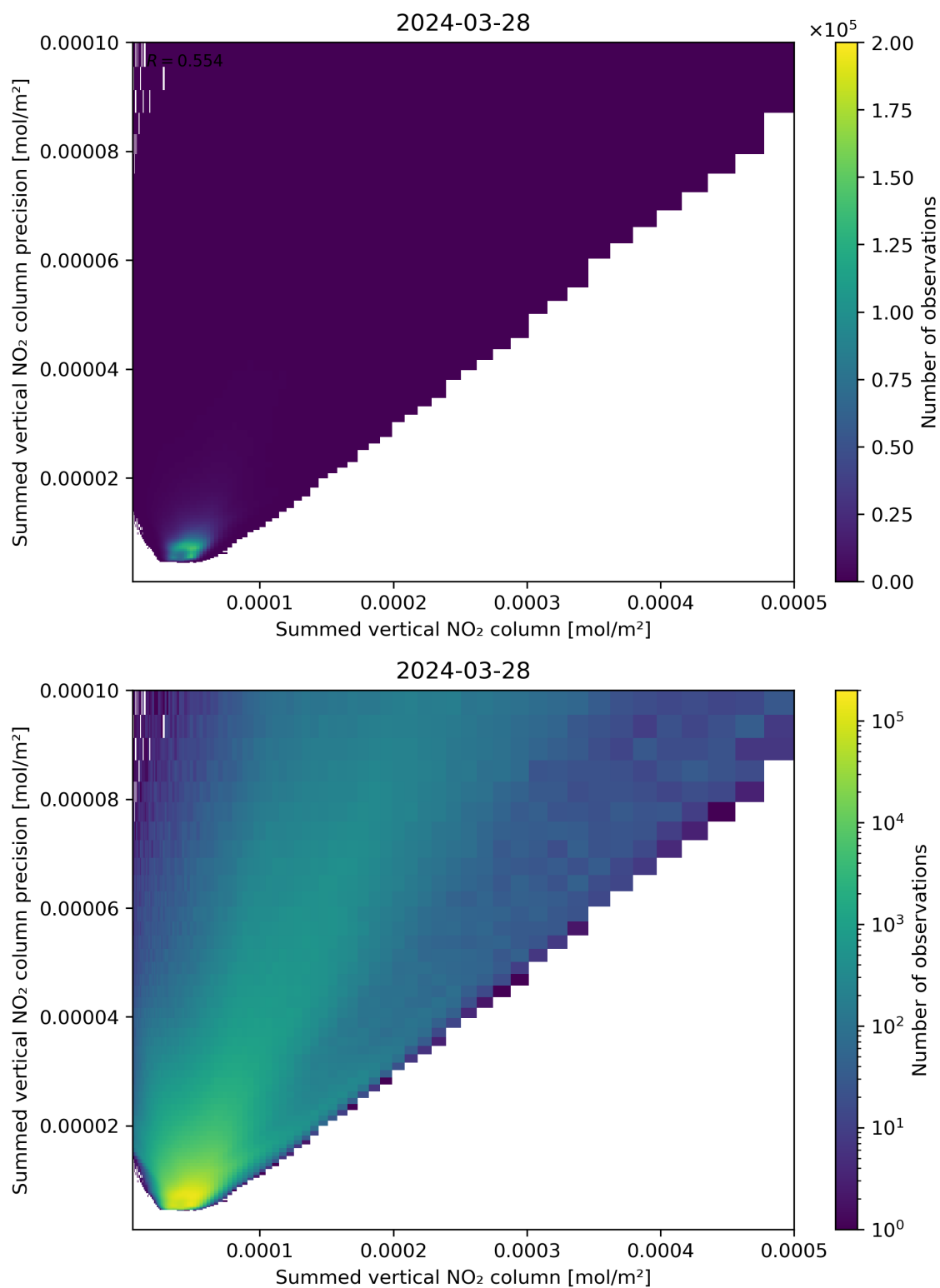
Figure 105: Scatter density plot of “Summed vertical NO 2 column” against “Summed vertical NO 2 column precision” for 2024-03-27 to 2024-03-29.
