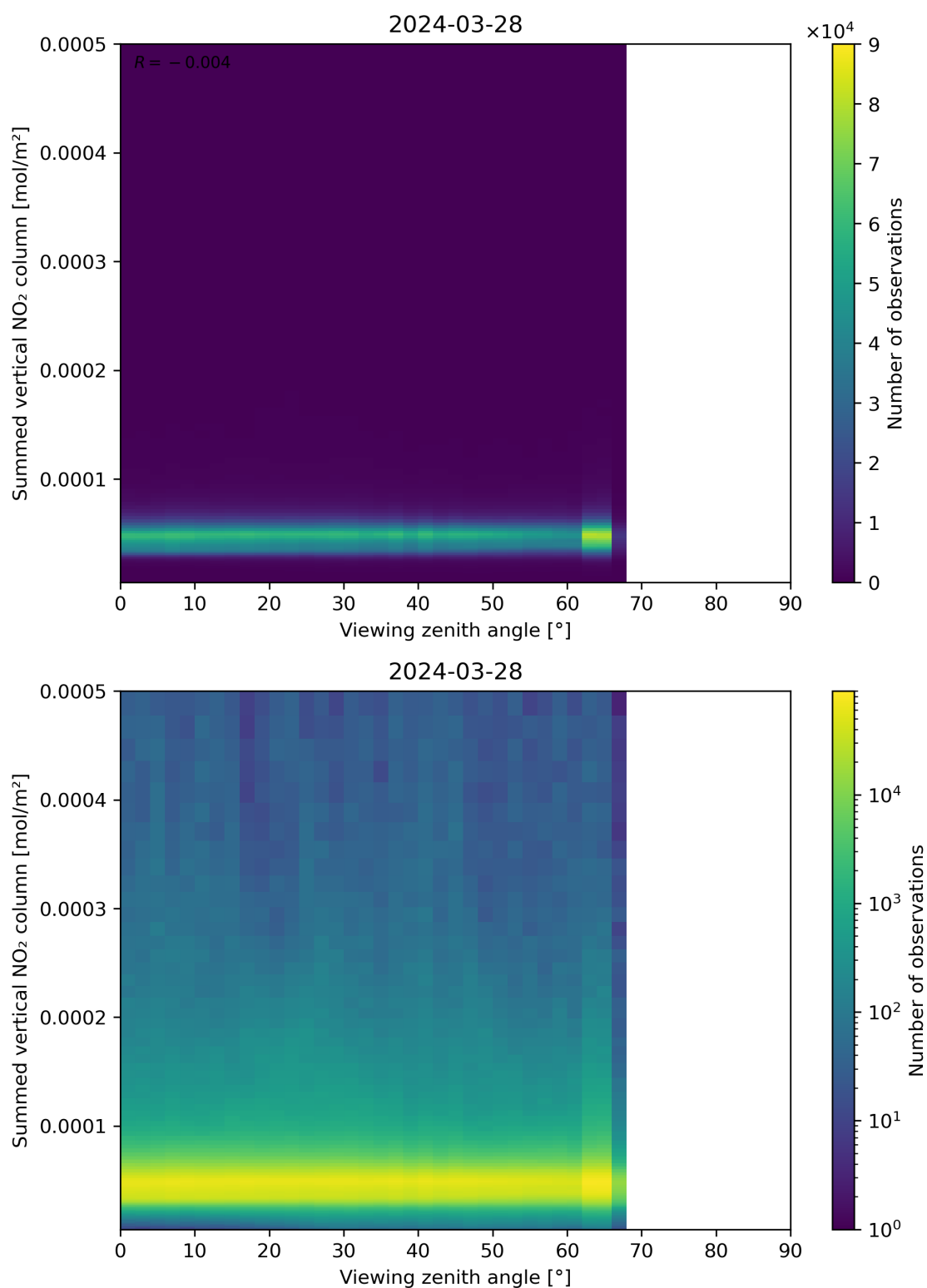
Figure 165: Scatter density plot of “Viewing zenith angle” against “Summed vertical NO 2 column” for 2024-03-27 to 2024-03-29.
