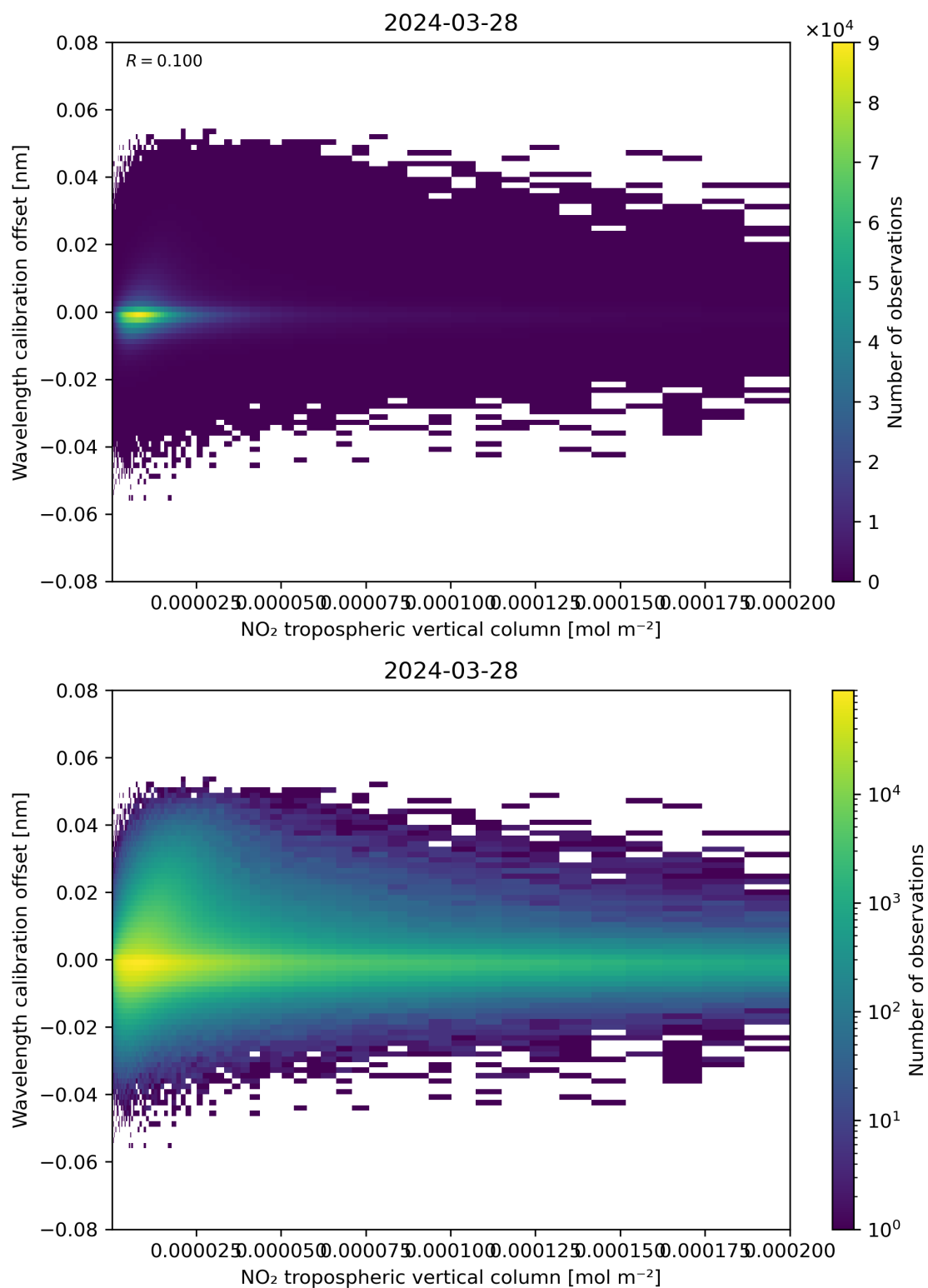
Figure 143: Scatter density plot of “NO 2 tropospheric vertical column” against “Wavelength calibration offset” for 2024-03-27 to 2024-03-29.
