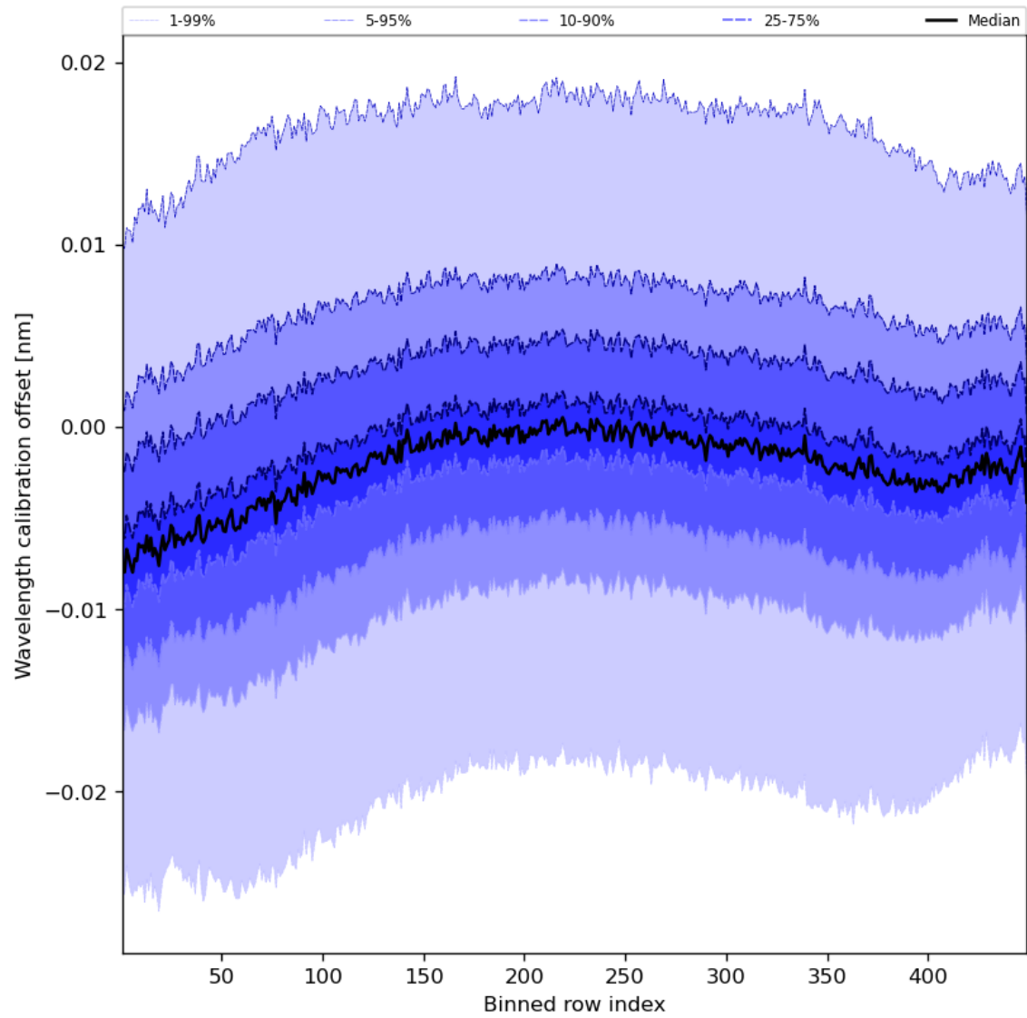
Figure 52: Along track statistics of “Wavelength calibration offset” for 2024-03-27 to 2024-03-29
