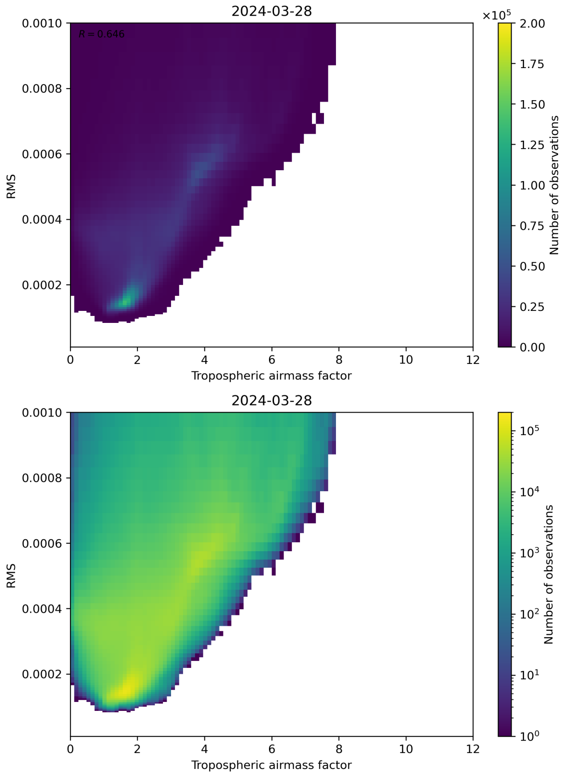
Figure 79: Scatter density plot of “Tropospheric airmass factor” against “RMS” for 2024-03-27 to 2024-03-29.
