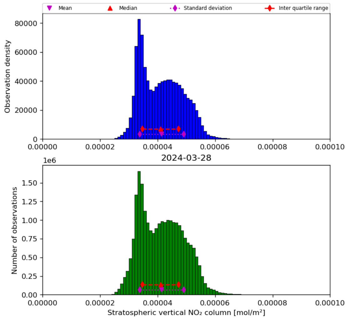
Figure 36: Histogram of “Stratospheric vertical NO 2 column” for 2024-03-27 to 2024-03-29
