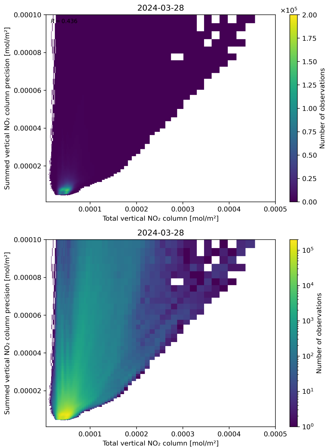
Figure 113: Scatter density plot of “Total vertical NO 2 column” against “Summed vertical NO 2 column precision” for 2024-03-27 to 2024-03-29.
