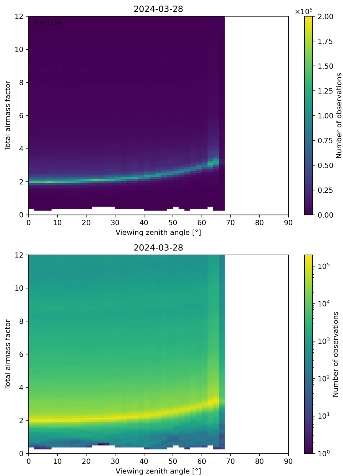
Figure 160: Scatter density plot of “Viewing zenith angle” against “Total airmass factor” for 2024-03-27 to 2024-03-29.
