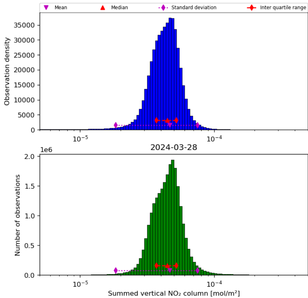
Figure 40: Histogram of “Summed vertical NO 2 column” for 2024-03-27 to 2024-03-29
