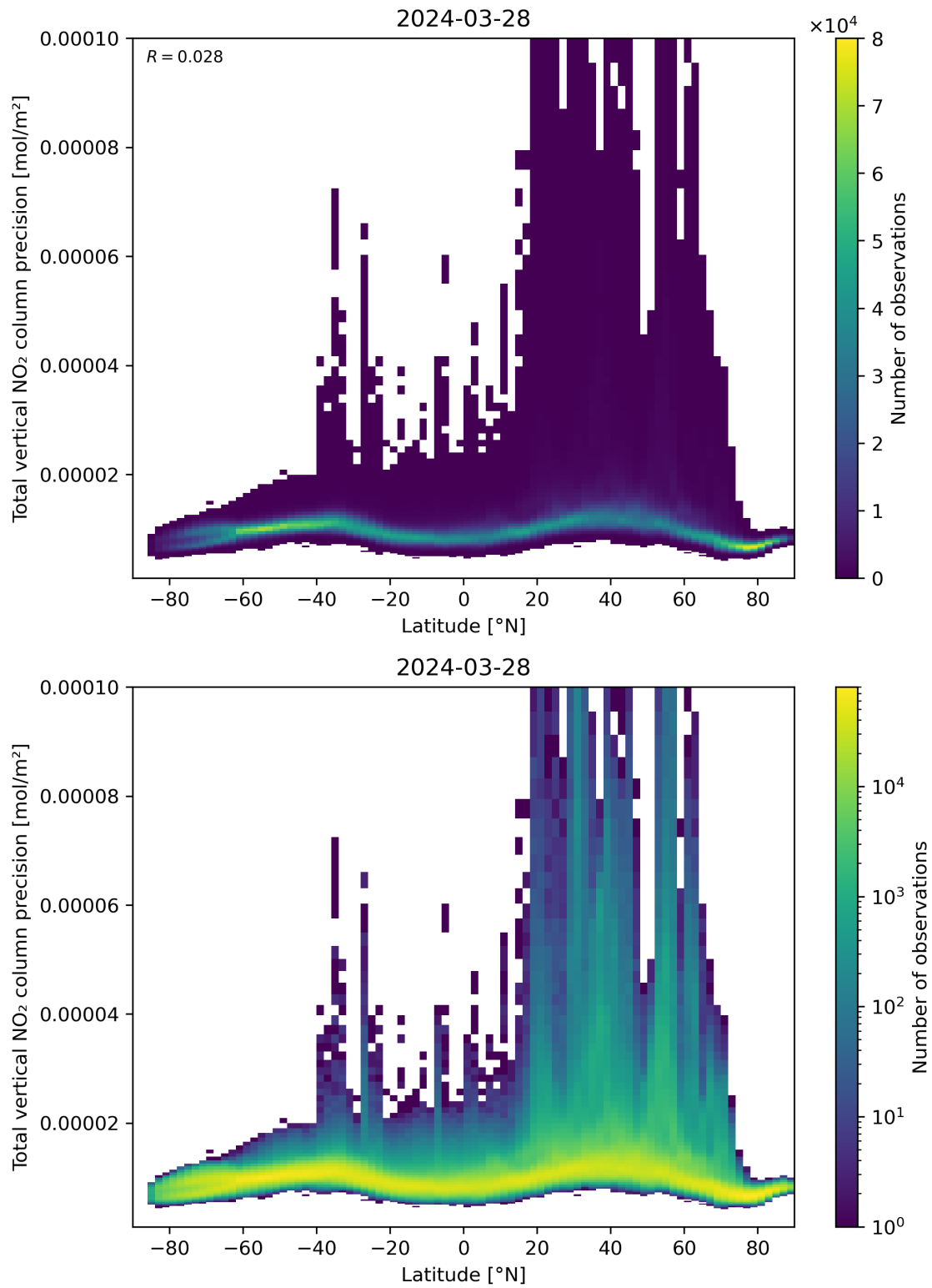
Figure 91: Scatter density plot of “Latitude” against “Total vertical NO 2 column precision” for 2024-03-27 to 2024-03-29.
