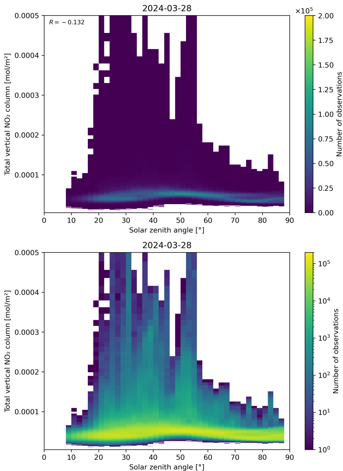
Figure 153: Scatter density plot of “Solar zenith angle” against “Total vertical NO 2 column” for 2024-03-27 to 2024-03-29.
