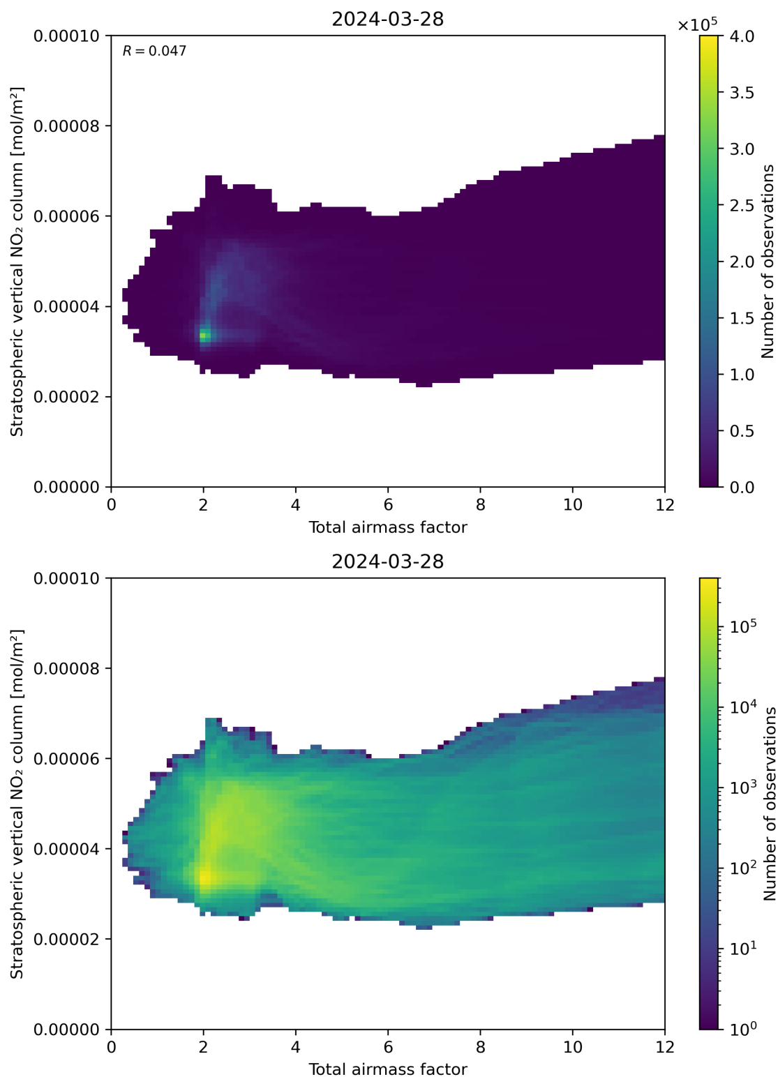
Figure 64: Scatter density plot of “Total airmass factor” against “Stratospheric vertical NO 2 column” for 2024-03-27 to 2024-03-29.
