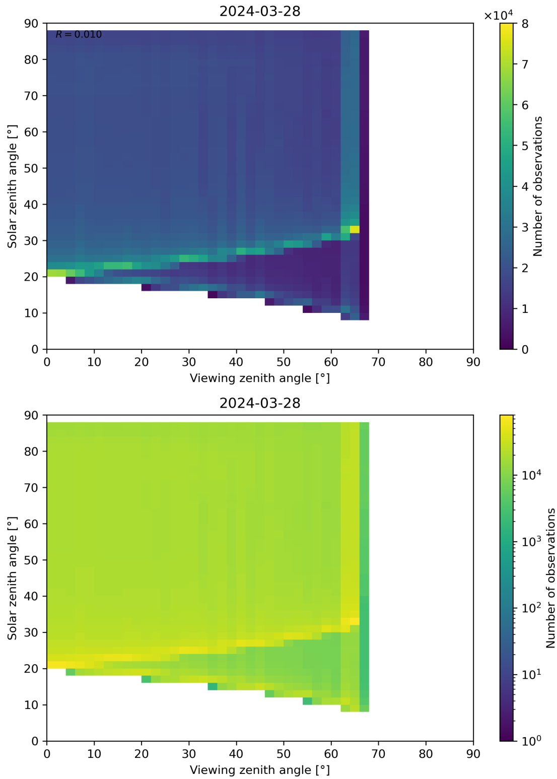
Figure 172: Scatter density plot of “Viewing zenith angle” against “Solar zenith angle” for 2024-03-27 to 2024-03-29.
