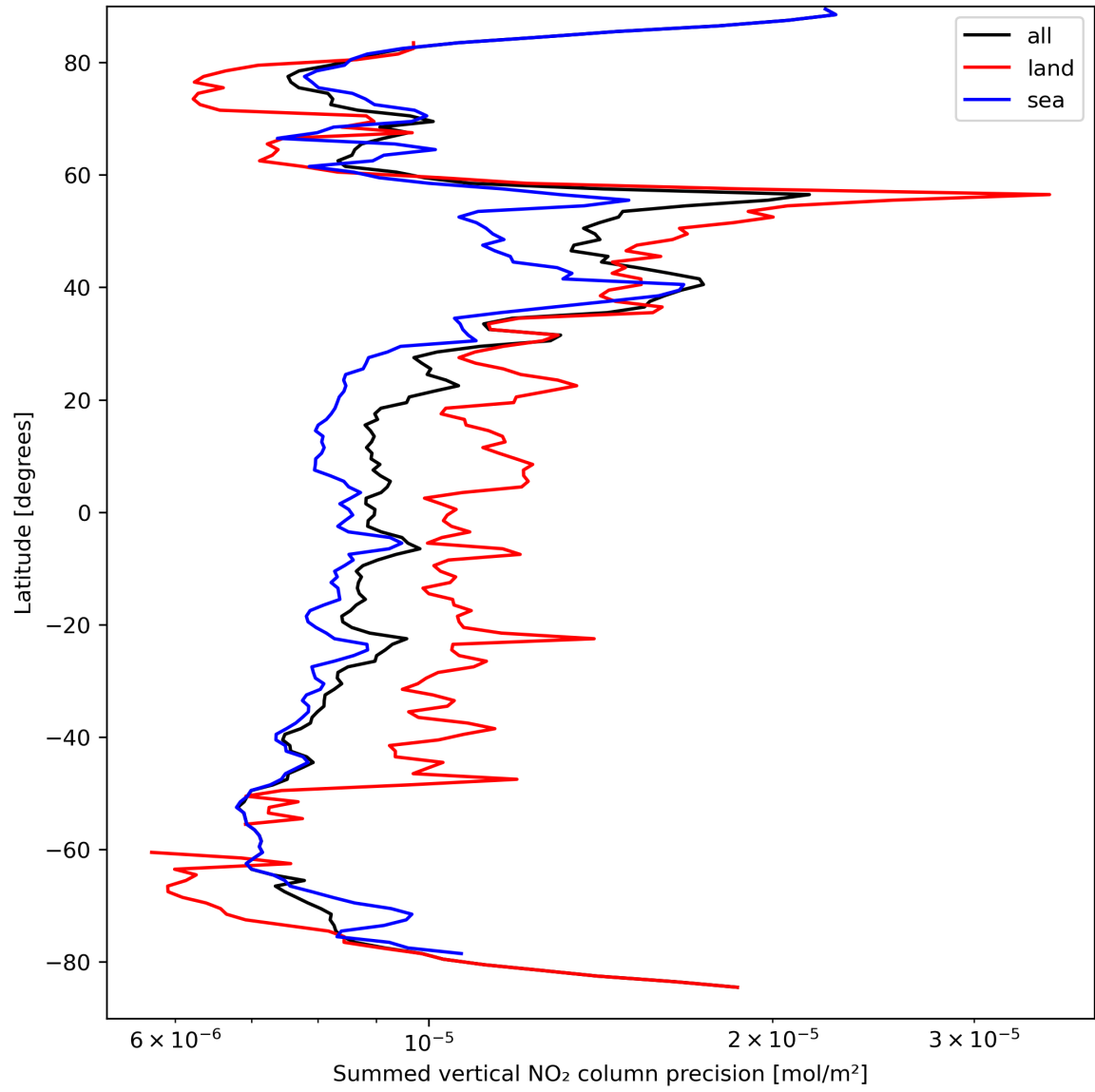
Figure 24: Zonal average of “Summed vertical NO 2 column precision” for 2024-03-27 to 2024-03-29.
