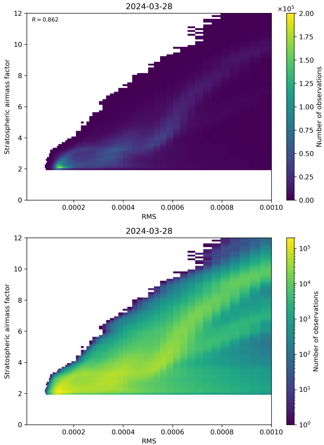
Figure 144: Scatter density plot of “RMS” against “Stratospheric airmass factor” for 2024-03-27 to 2024-03-29.
