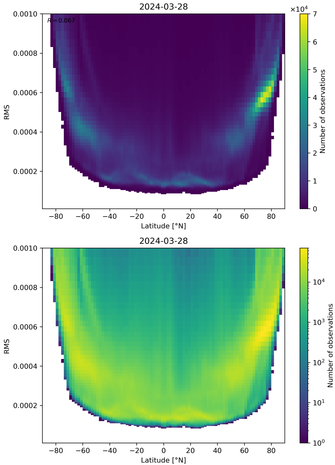
Figure 94: Scatter density plot of “Latitude” against “RMS” for 2024-03-27 to 2024-03-29.
