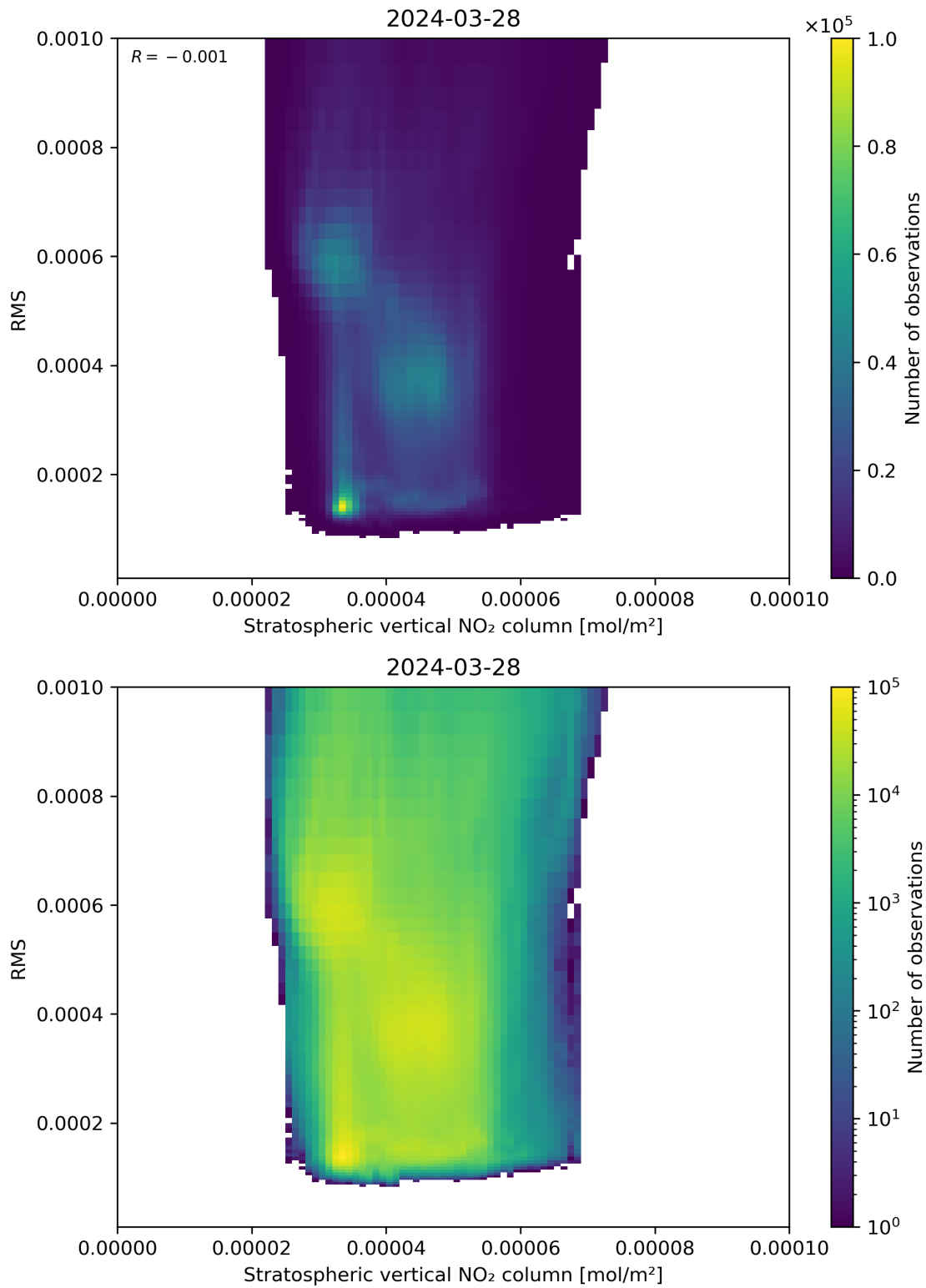
Figure 102: Scatter density plot of “Stratospheric vertical NO 2 column” against “RMS” for 2024-03-27 to 2024-03-29.
