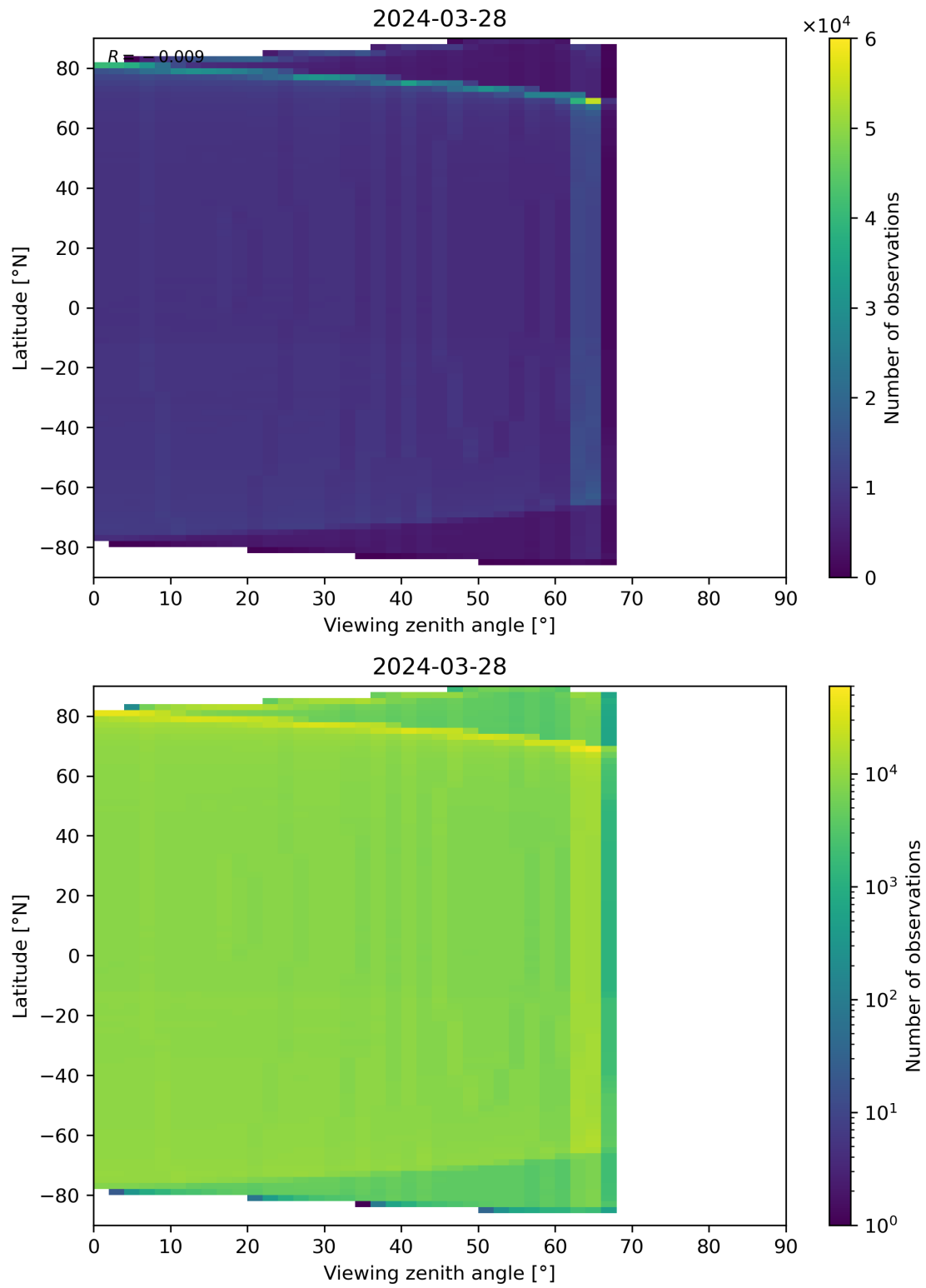
Figure 163: Scatter density plot of “Viewing zenith angle” against “Latitude” for 2024-03-27 to 2024-03-29.
