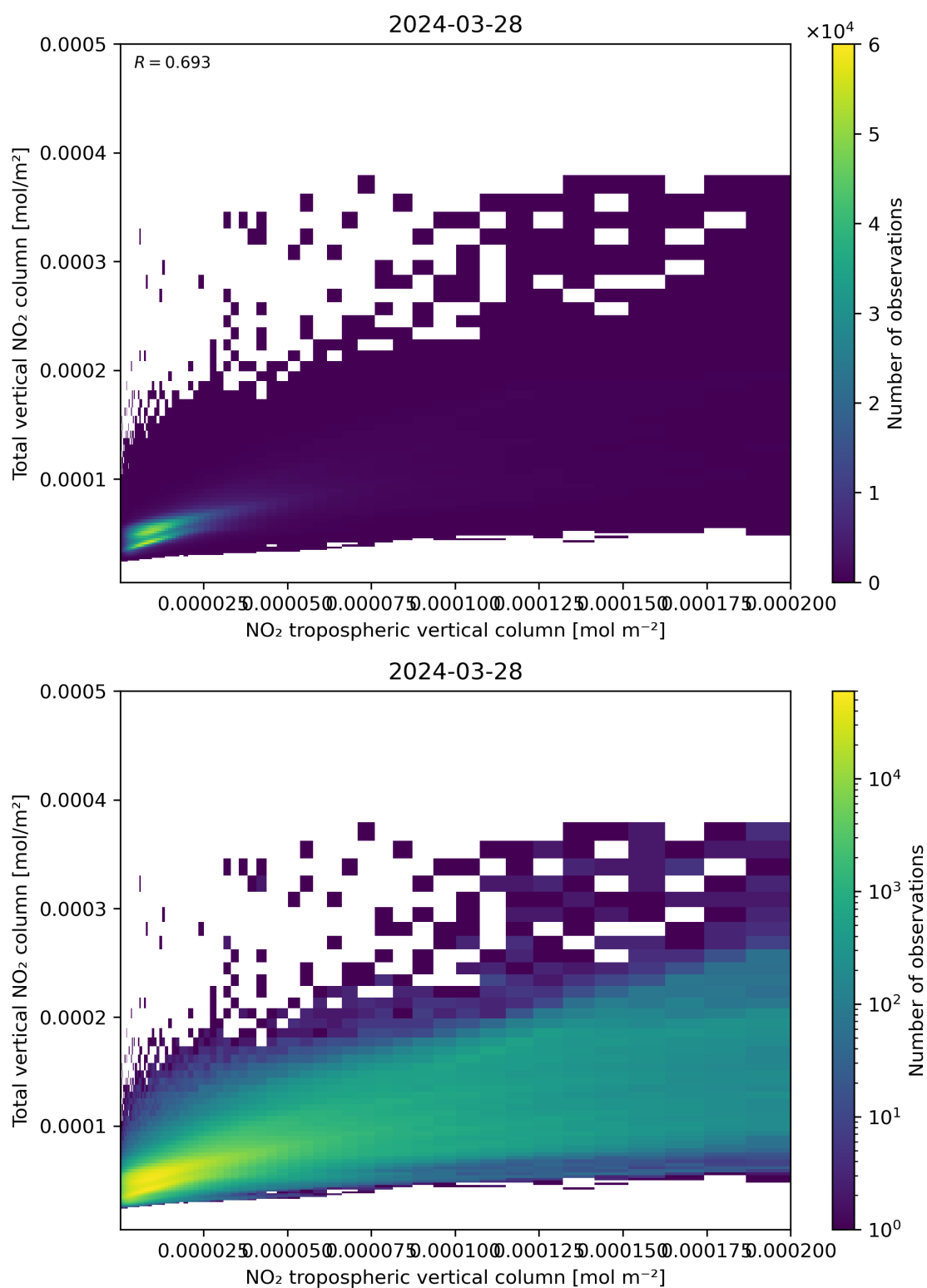
Figure 128: Scatter density plot of “NO 2 tropospheric vertical column” against “Total vertical NO 2 column” for 2024-03-27 to 2024-03-29.
