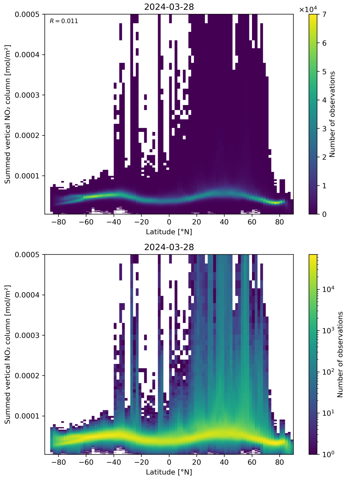
Figure 88: Scatter density plot of “Latitude” against “Summed vertical NO 2 column” for 2024-03-27 to 2024-03-29.
