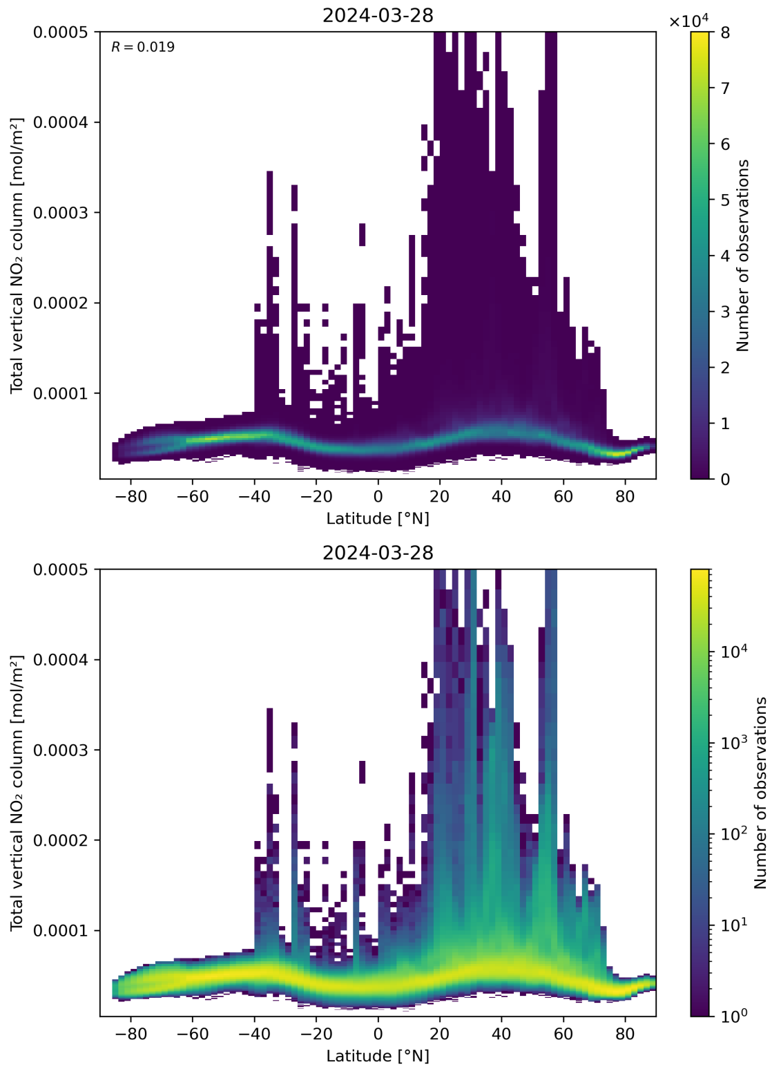
Figure 90: Scatter density plot of “Latitude” against “Total vertical NO 2 column” for 2024-03-27 to 2024-03-29.
