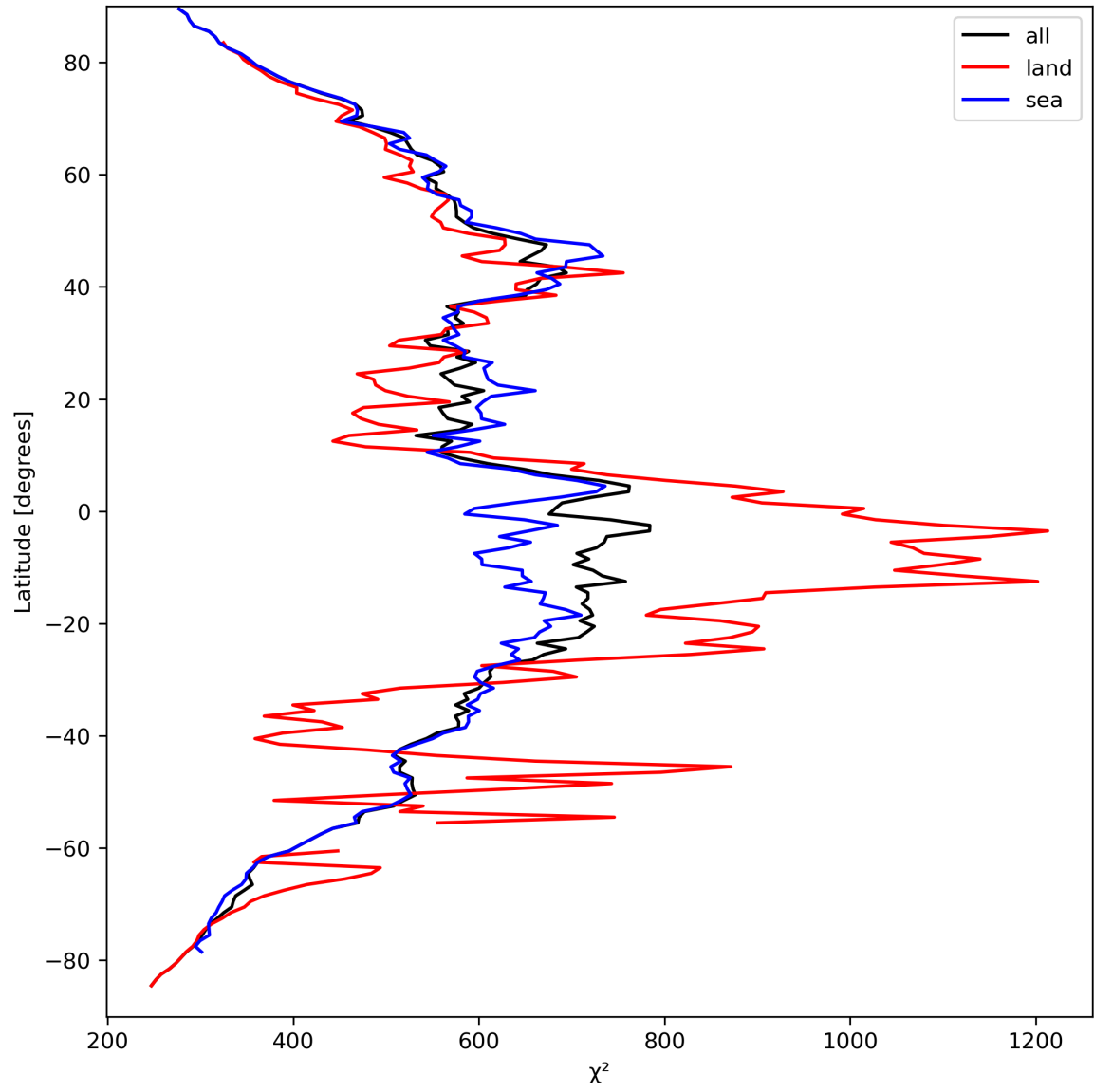
Figure 25: Zonal average of “ \chi^2 ” for 2024-03-27 to 2024-03-29.
