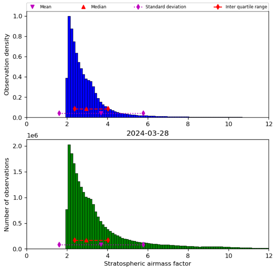
Figure 44: Histogram of “Stratospheric airmass factor” for 2024-03-27 to 2024-03-29
