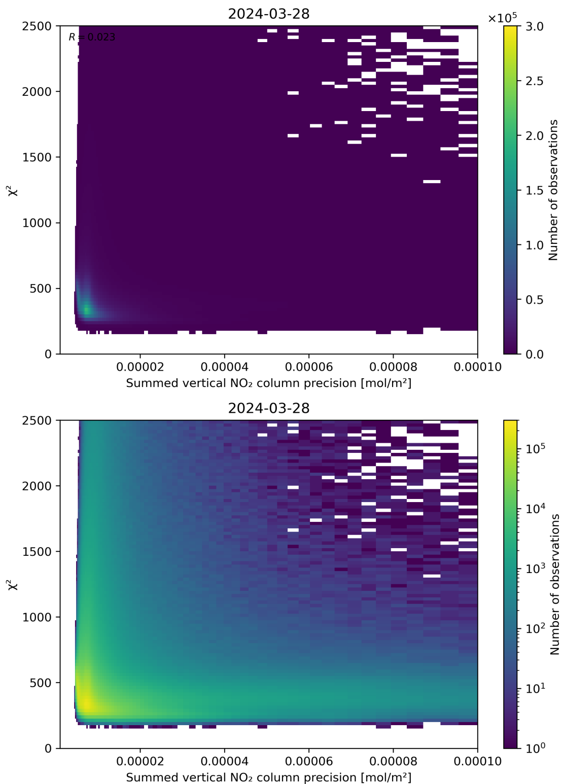
Figure 107: Scatter density plot of “Summed vertical NO 2 column precision” against “ \chi^2 ” for 2024-03-27 to 2024-03-29.
