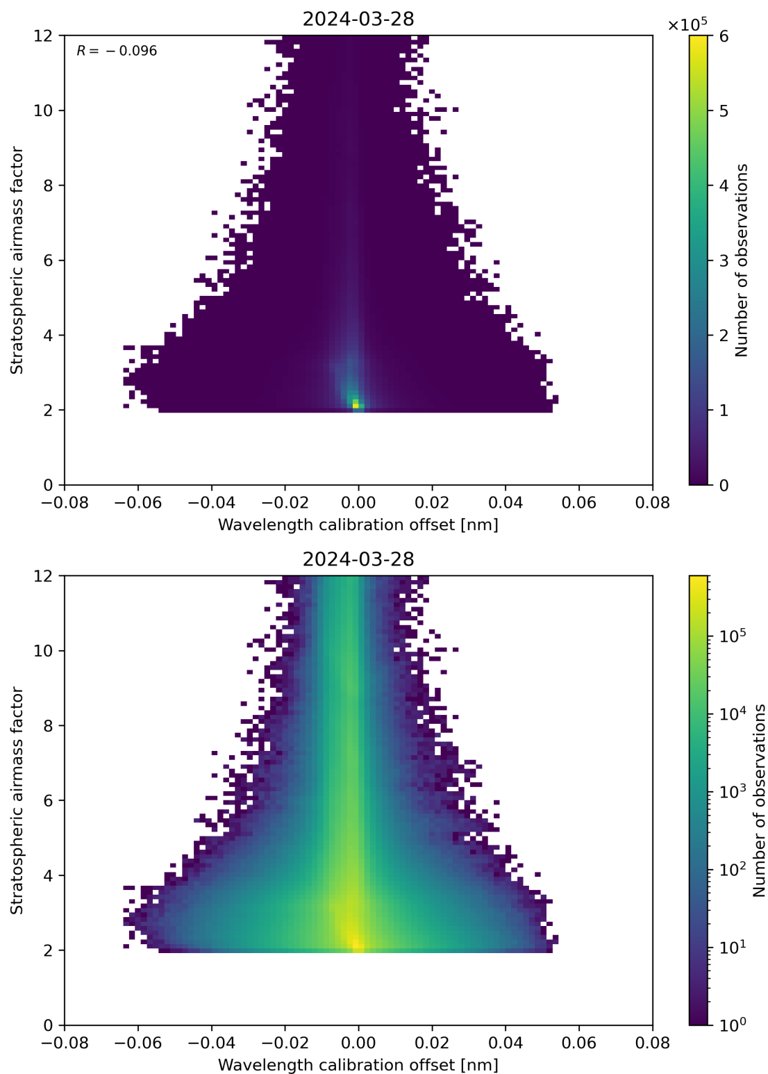
Figure 174: Scatter density plot of “Wavelength calibration offset” against “Stratospheric air mass factor” for 2024-03-27 to 2024-03-29.
