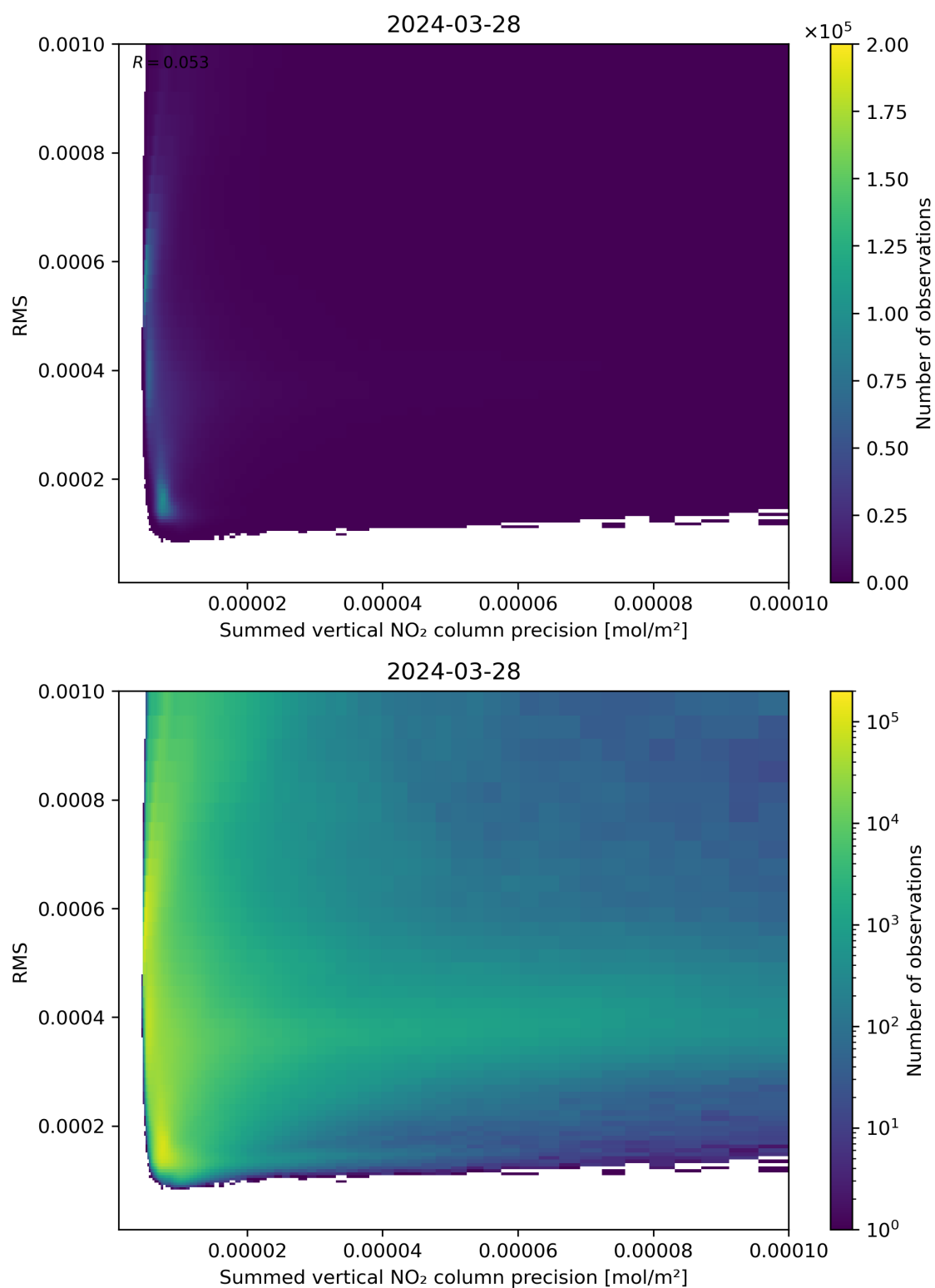
Figure 108: Scatter density plot of “Summed vertical NO 2 column precision” against “RMS” for 2024-03-27 to 2024-03-29.
