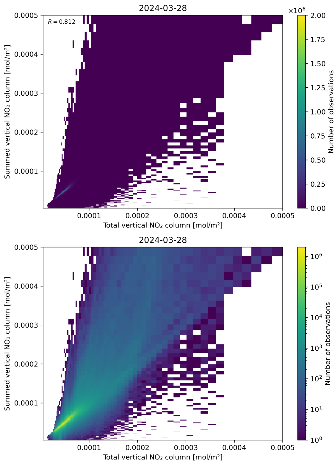
Figure 112: Scatter density plot of “Total vertical NO 2 column” against “Summed vertical NO 2 column” for 2024-03-27 to 2024-03-29.
