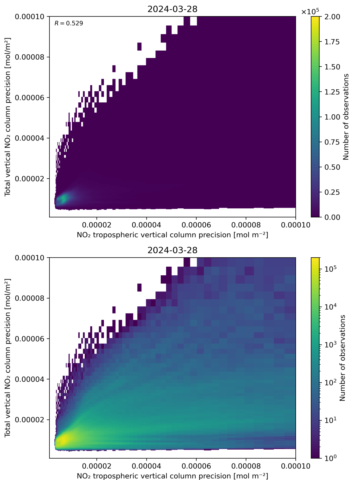
Figure 139: Scatter density plot of “NO 2 tropospheric vertical column precision” against “Total vertical NO 2 column precision” for 2024-03-27 to 2024-03-29.
