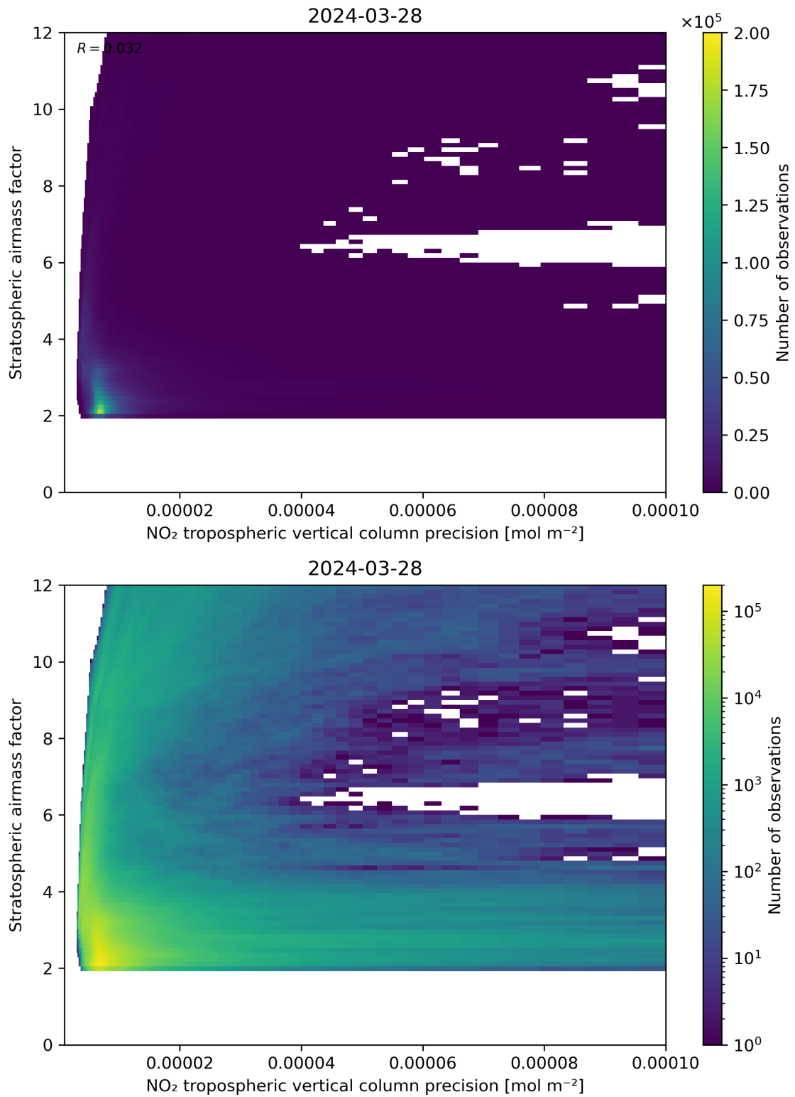
Figure 131: Scatter density plot of “NO 2 tropospheric vertical column precision” against “Stratospheric airmass factor” for 2024-03-27 to 2024-03-29.
