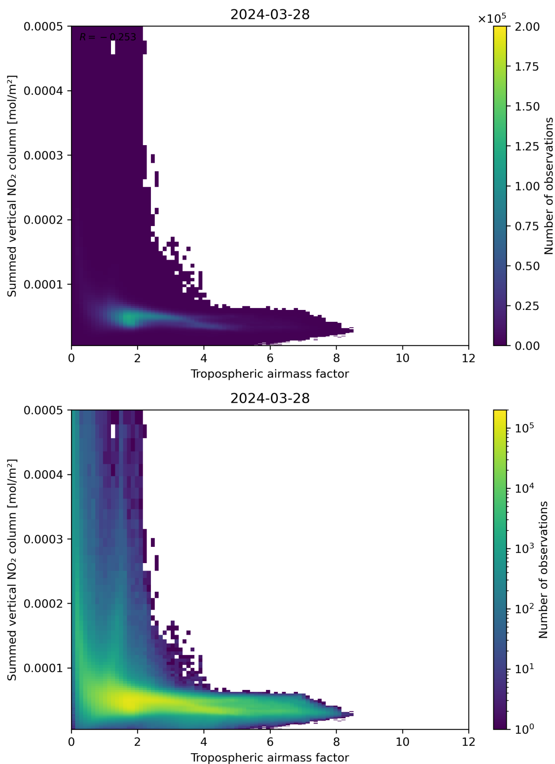
Figure 75: Scatter density plot of “Tropospheric air mass factor” against “Summed vertical NO 2 column” for 2024-03-27 to 2024-03-29.
