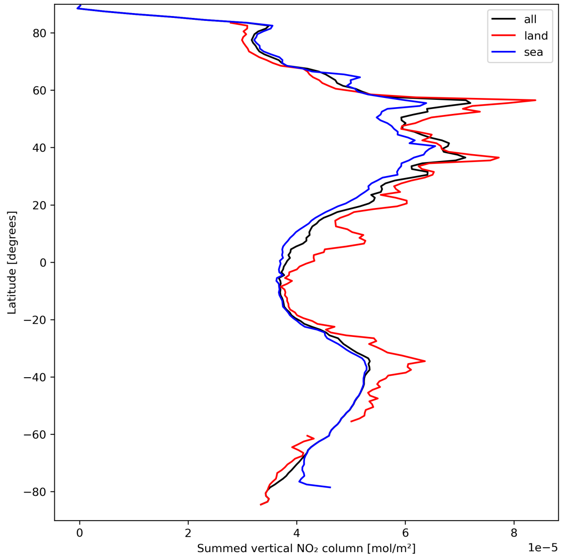
Figure 23: Zonal average of “Summed vertical NO 2 column” for 2024-03-27 to 2024-03-29.
