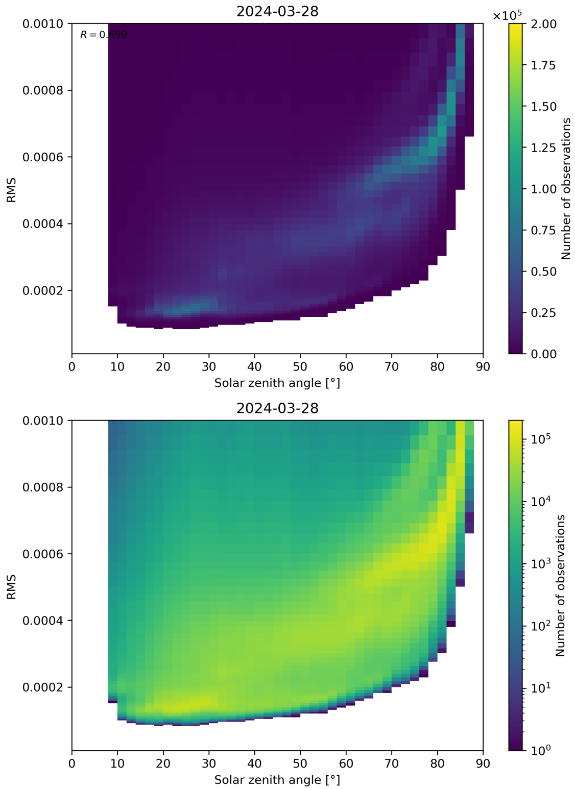
Figure 157: Scatter density plot of “Solar zenith angle” against “RMS” for 2024-03-27 to 2024-03-29.
