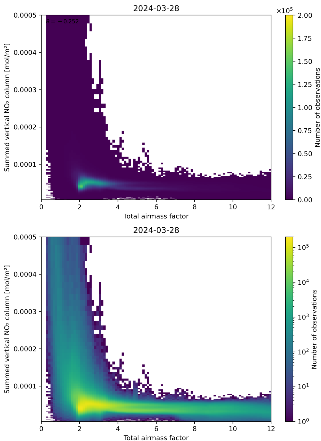
Figure 65: Scatter density plot of “Total airmass factor” against “Summed vertical NO 2 column” for 2024-03-27 to 2024-03-29.
