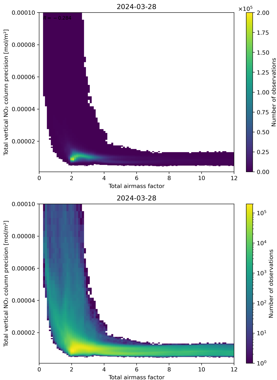
Figure 68: Scatter density plot of “Total airmass factor” against “Total vertical NO 2 column precision” for 2024-03-27 to 2024-03-29.
