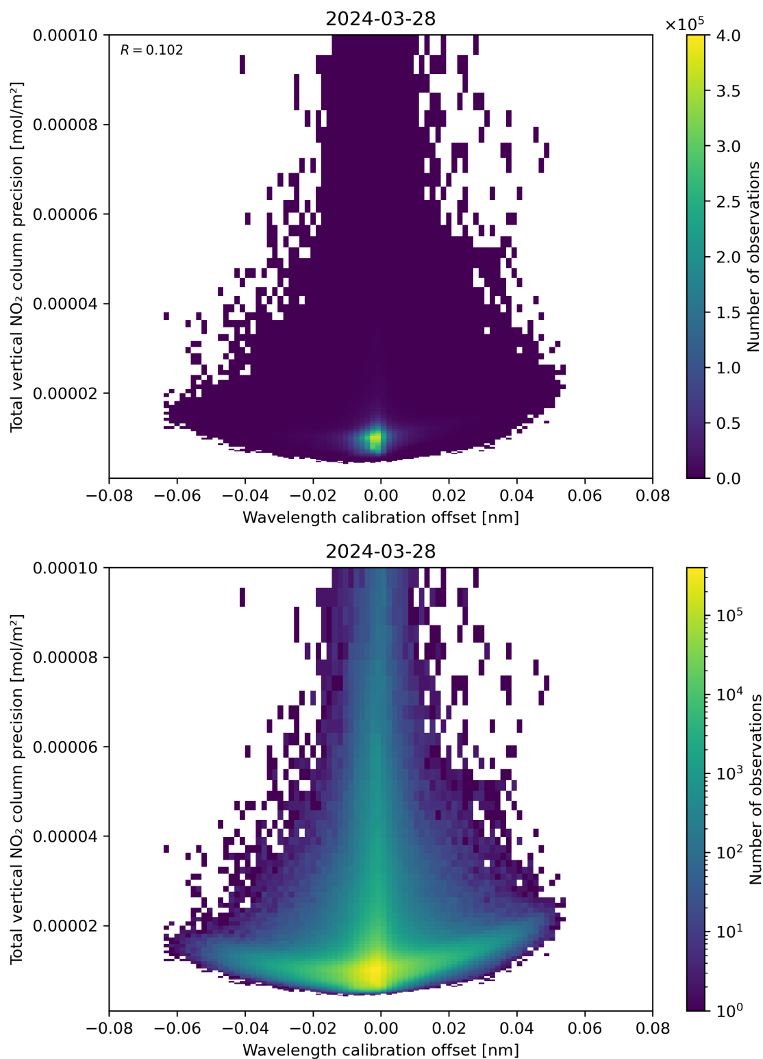
Figure 180: Scatter density plot of “Wavelength calibration offset” against “Total vertical NO 2 column precision” for 2024-03-27 to 2024-03-29.
