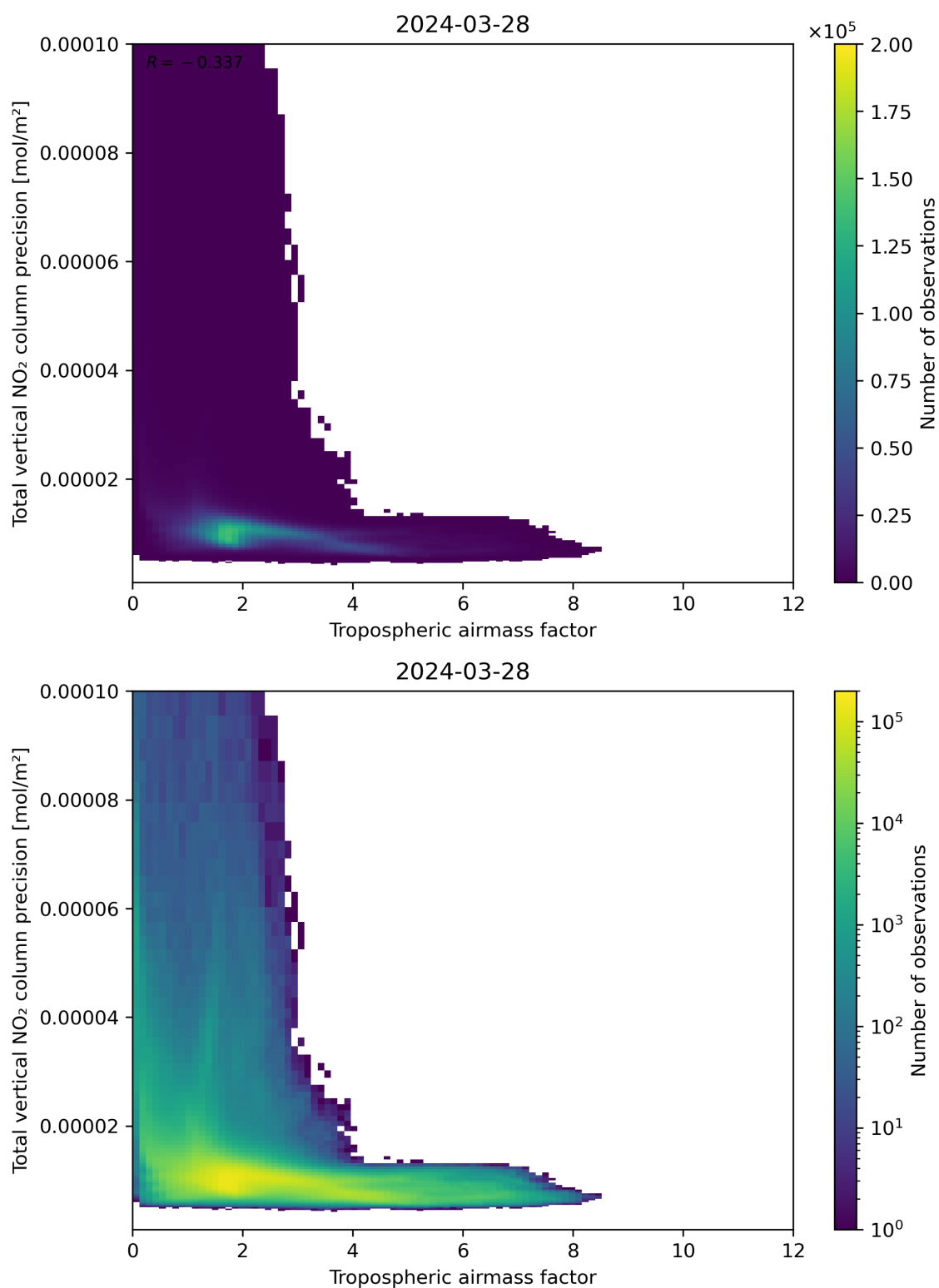
Figure 78: Scatter density plot of “Tropospheric air mass factor” against “Total vertical NO 2 column precision” for 2024-03-27 to 2024-03-29.
