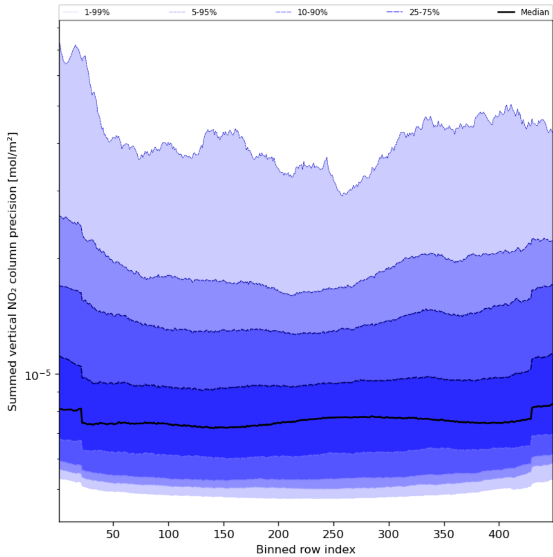
Figure 58: Along track statistics of “Summed vertical NO 2 column precision” for 2024-03-27 to 2024-03-29
