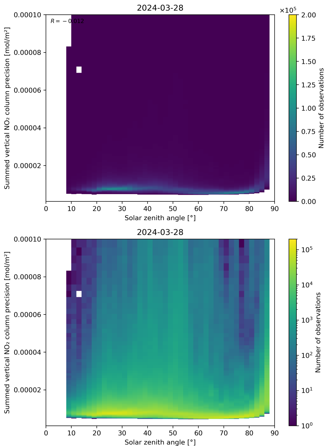
Figure 152: Scatter density plot of “Solar zenith angle” against “Summed vertical NO 2 column precision” for 2024-03-27 to 2024-03-29.
