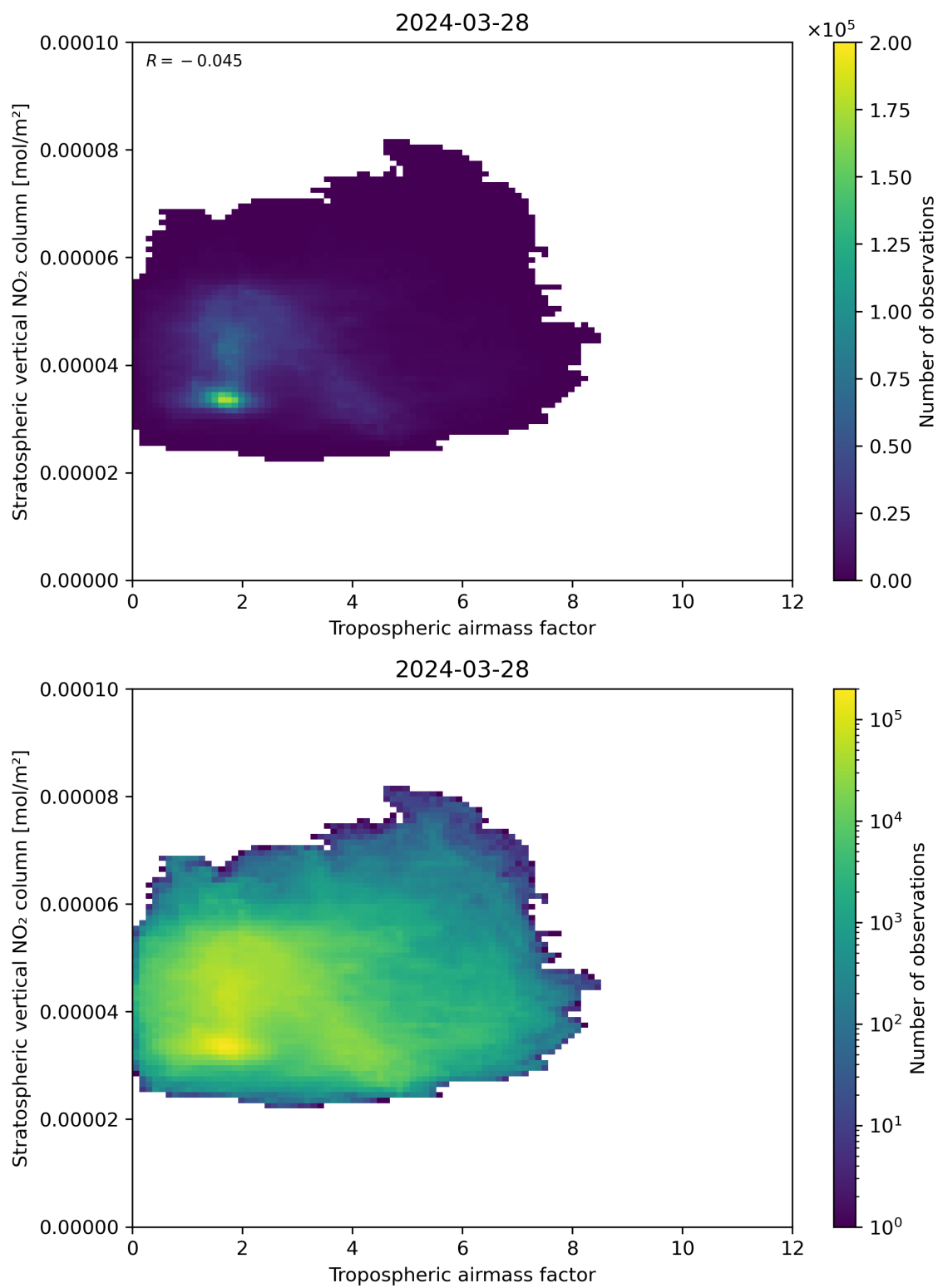
Figure 74: Scatter density plot of “Tropospheric air mass factor” against “Stratospheric vertical NO 2 column” for 2024-03-27 to 2024-03-29.
