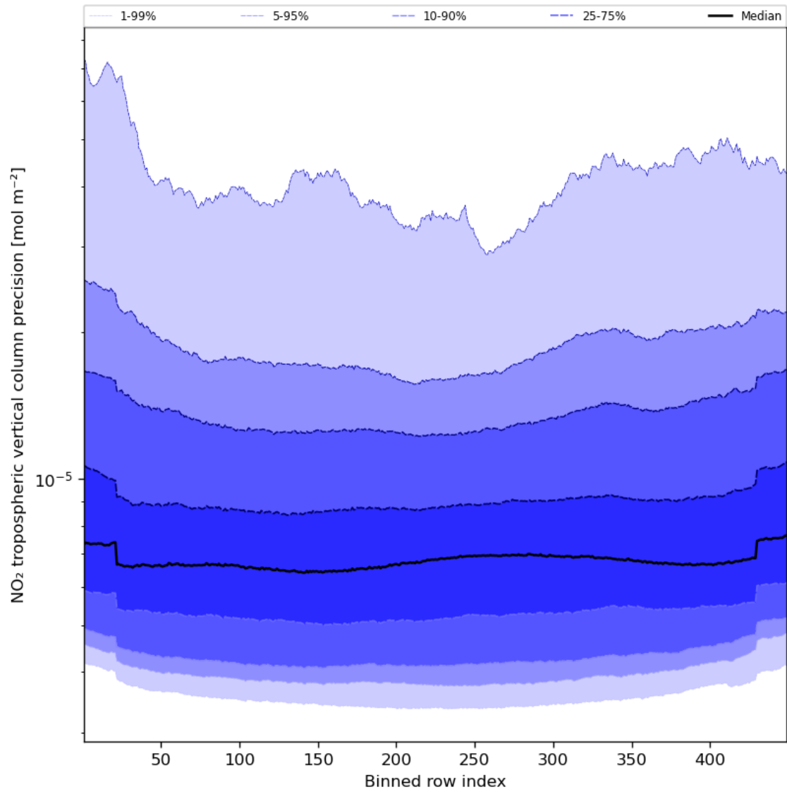
Figure 47: Along track statistics of “NO 2 tropospheric vertical column precision” for 2024-03-27 to 2024-03-29
