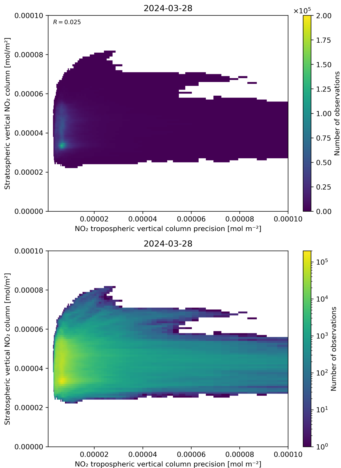
Figure 135: Scatter density plot of “NO 2 tropospheric vertical column precision” against “Stratospheric vertical NO 2 column” for 2024-03-27 to 2024-03-29.
