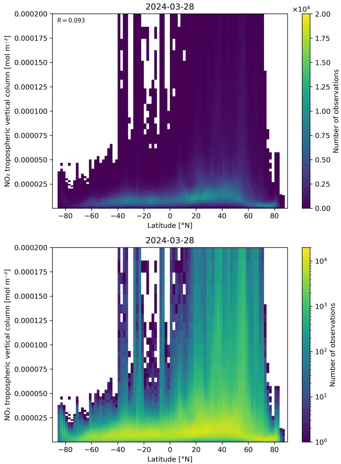
Figure 92: Scatter density plot of “Latitude” against “NO 2 tropospheric vertical column” for 2024-03-27 to 2024-03-29.
