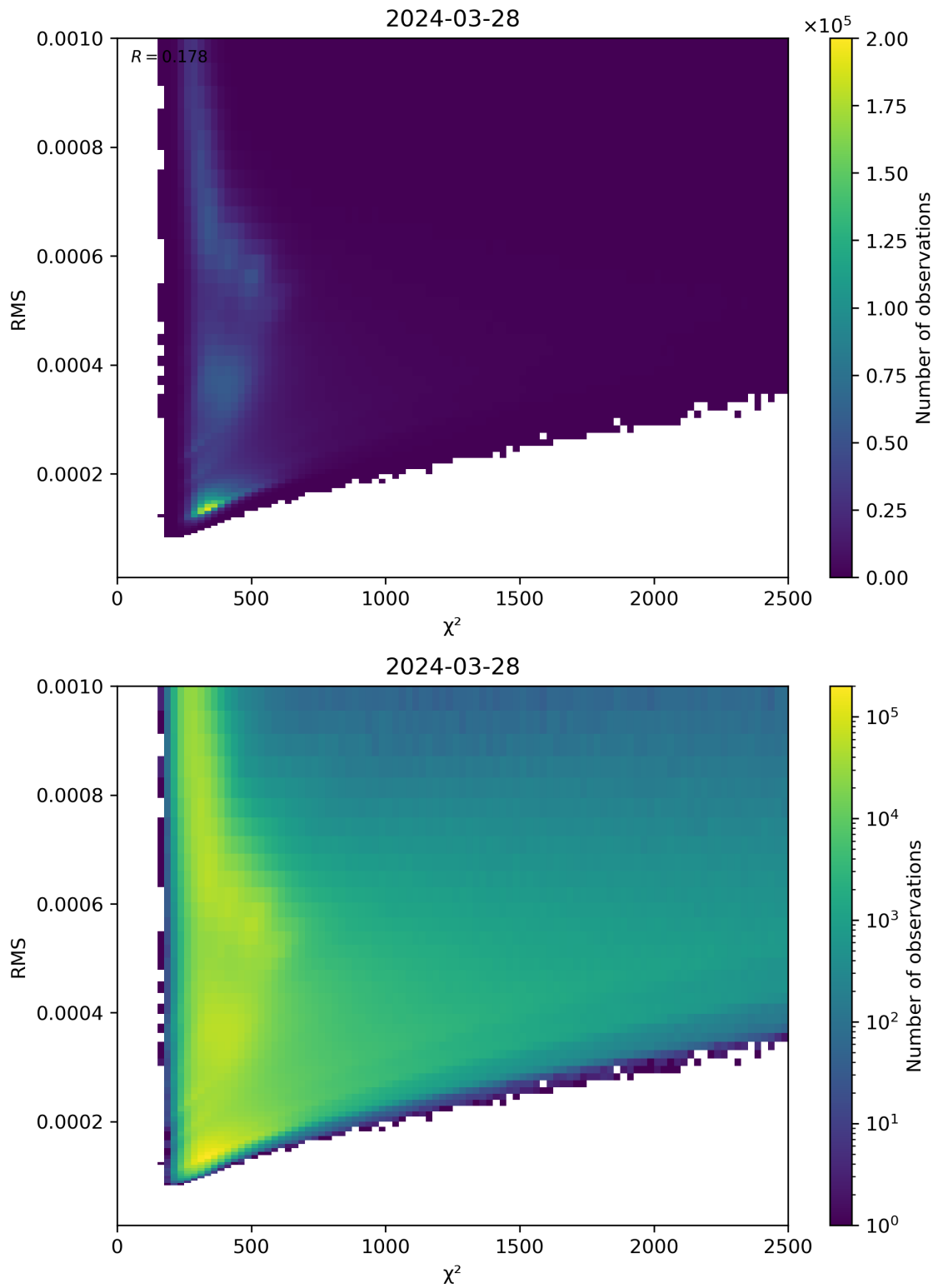
Figure 82: Scatter density plot of “ \chi^2 ” against “RMS” for 2024-03-27 to 2024-03-29.
