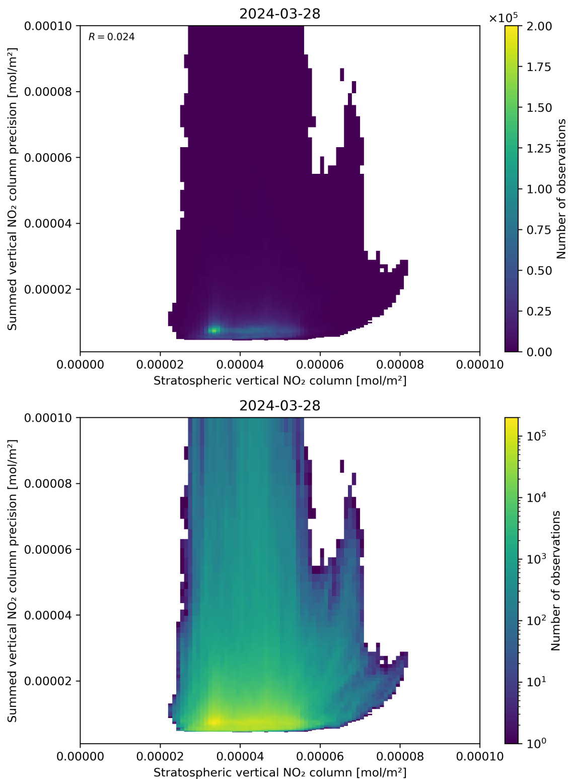
Figure 99: Scatter density plot of “Stratospheric vertical NO 2 column” against “Summed vertical NO 2 column precision” for 2024-03-27 to 2024-03-29.
