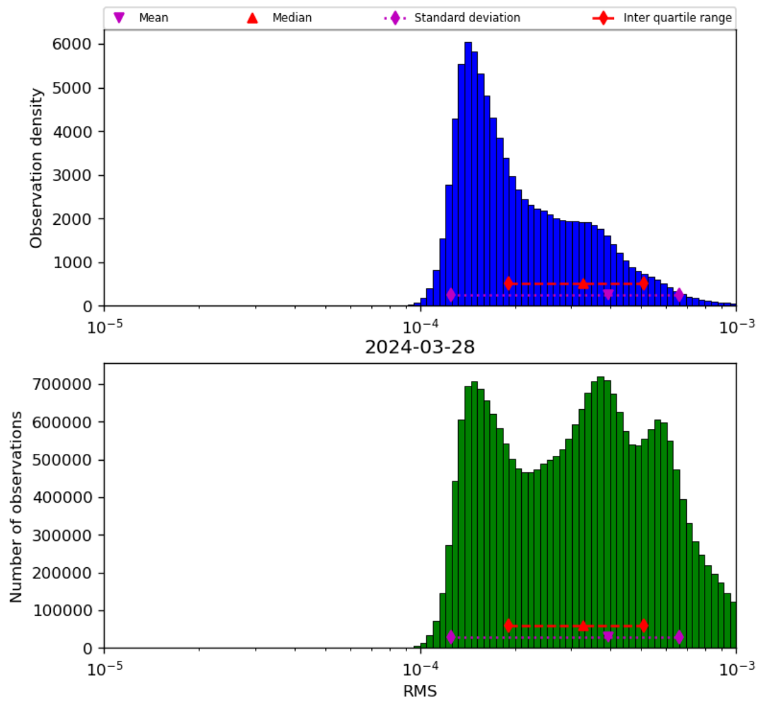
Figure 43: Histogram of “RMS” for 2024-03-27 to 2024-03-29
