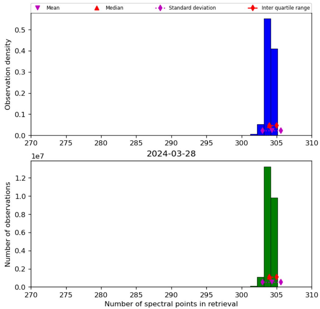
Figure 33: Histogram of “Number of spectral points in retrieval” for 2024-03-27 to 2024-03-29
