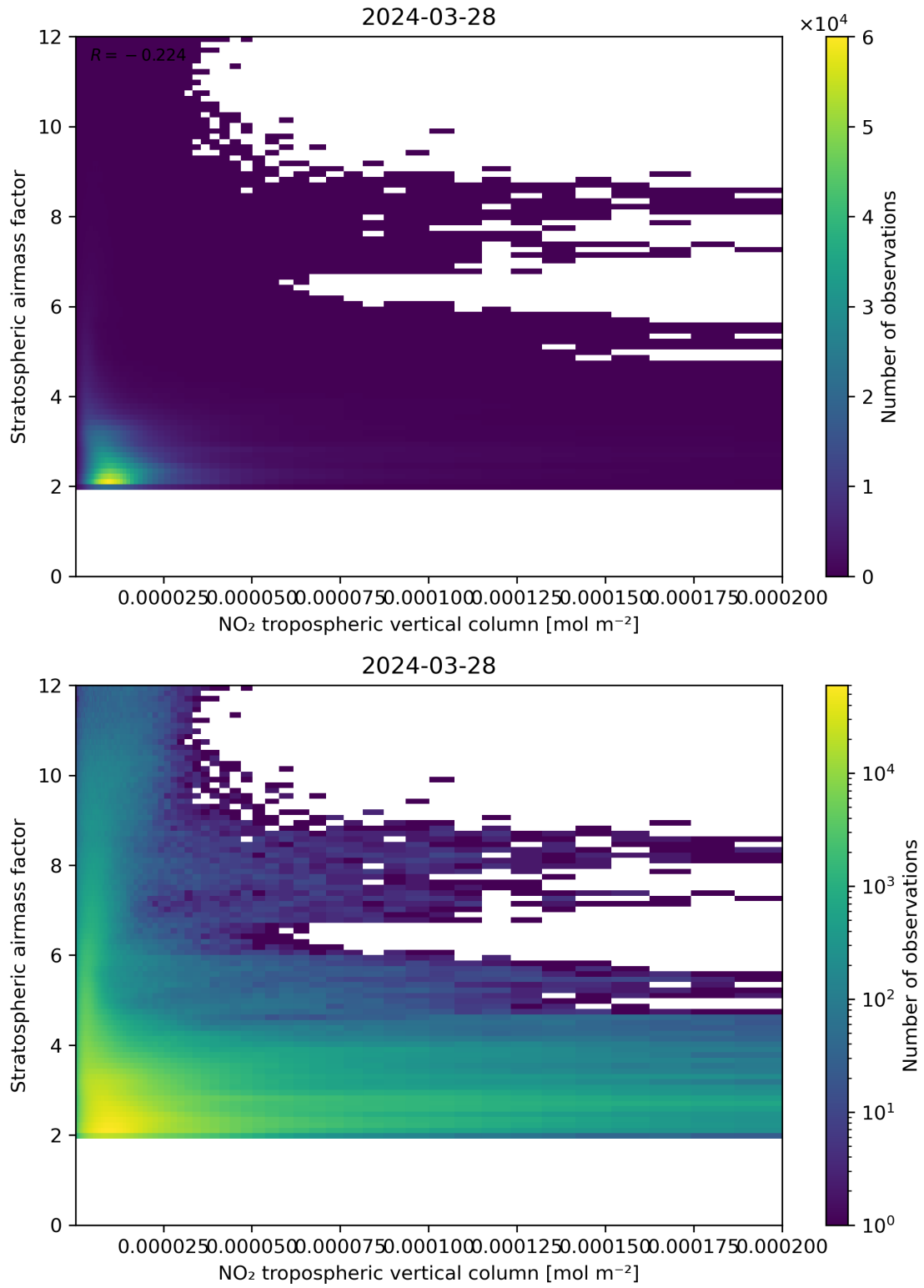
Figure 121: Scatter density plot of “NO 2 tropospheric vertical column” against “Stratospheric air mass factor” for 2024-03-27 to 2024-03-29.
