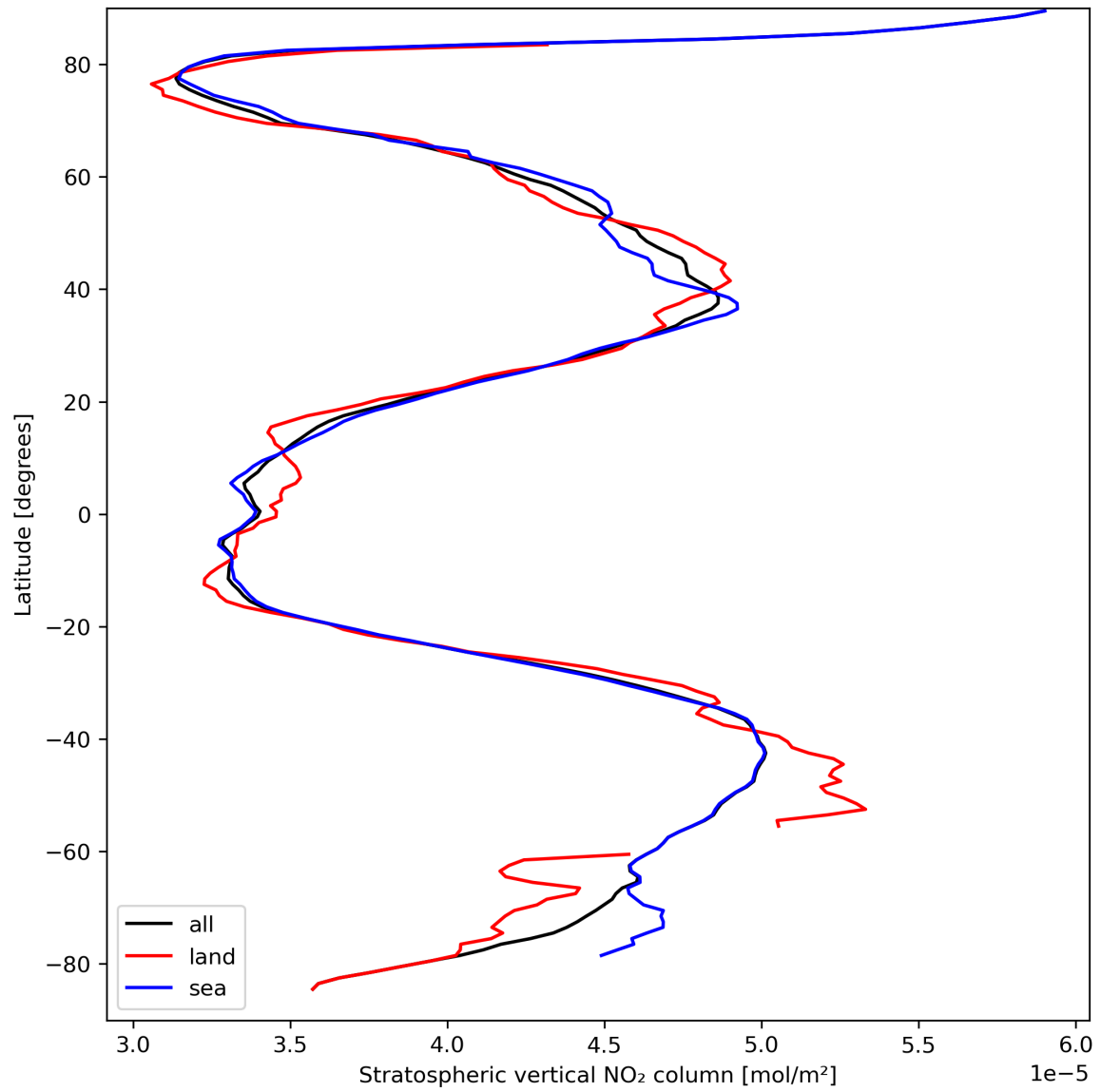
Figure 19: Zonal average of “Stratospheric vertical NO 2 column” for 2024-03-27 to 2024-03-29.
