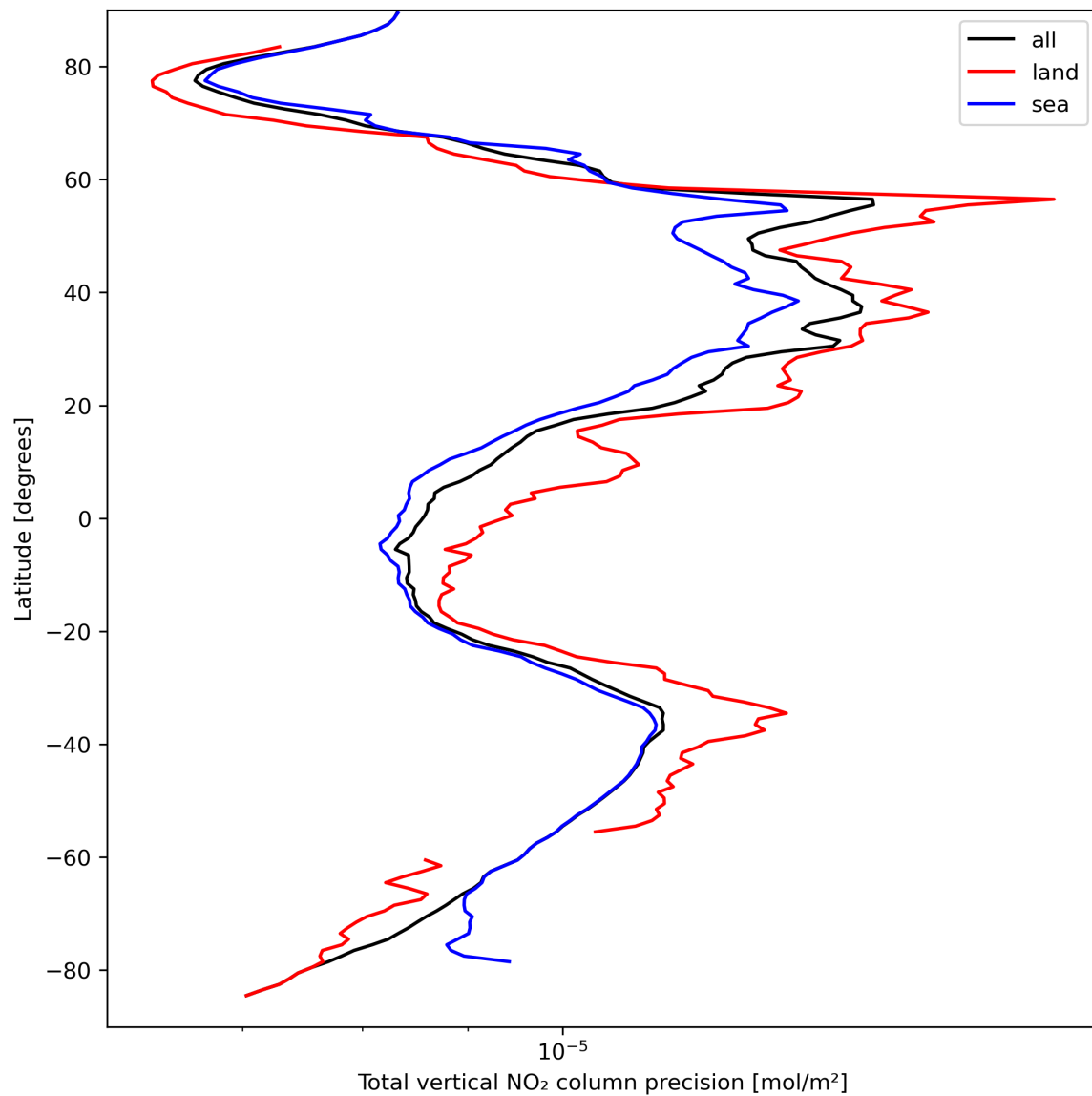
Figure 22: Zonal average of “Total vertical NO 2 column precision” for 2024-03-27 to 2024-03-29.
