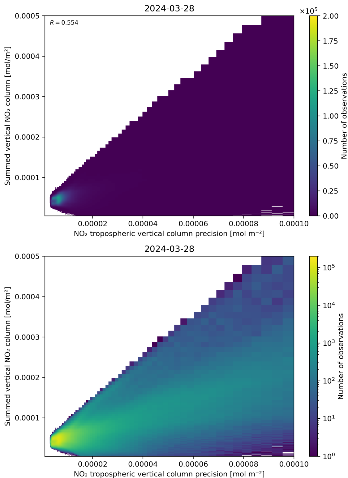
Figure 136: Scatter density plot of “NO 2 tropospheric vertical column precision” against “Summed vertical NO 2 column” for 2024-03-27 to 2024-03-29.
