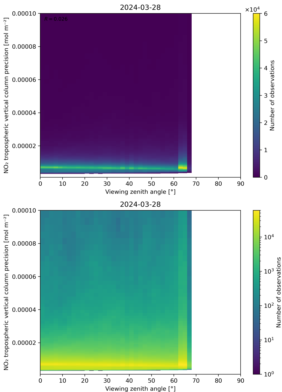
Figure 170: Scatter density plot of “Viewing zenith angle” against “NO 2 tropospheric vertical column precision” for 2024-03-27 to 2024-03-29.
