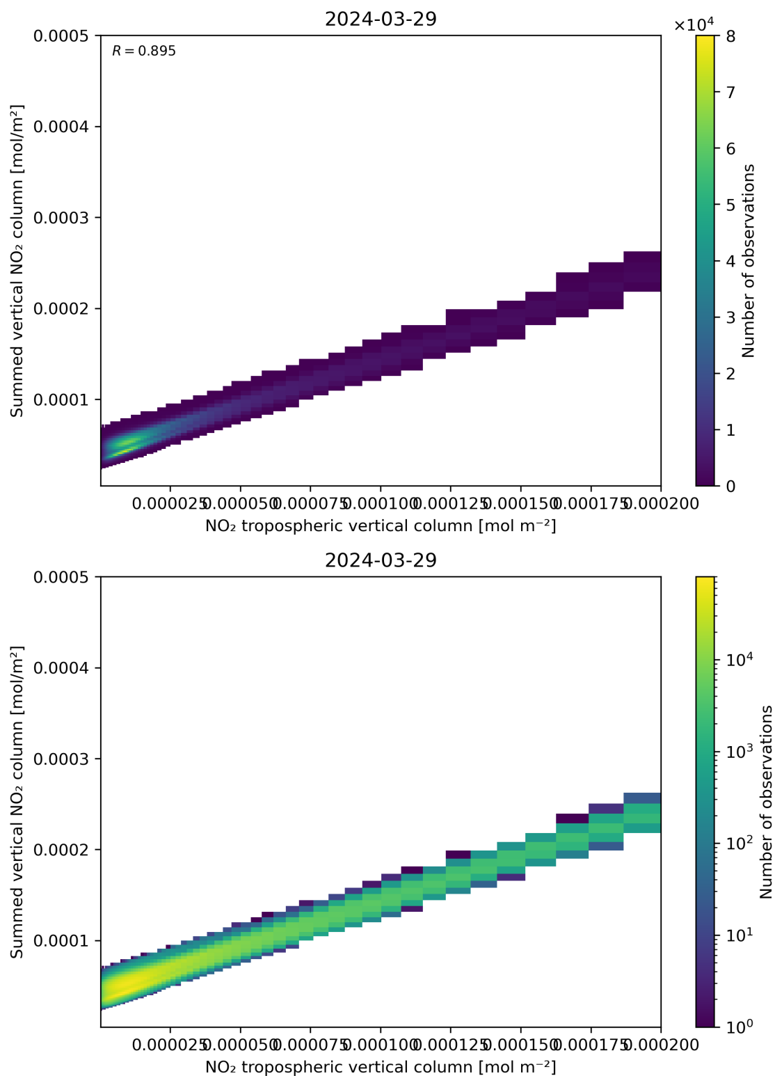
Figure 126: Scatter density plot of “NO 2 tropospheric vertical column” against “Summed vertical NO 2 column” for 2024-03-28 to 2024-03-30.
