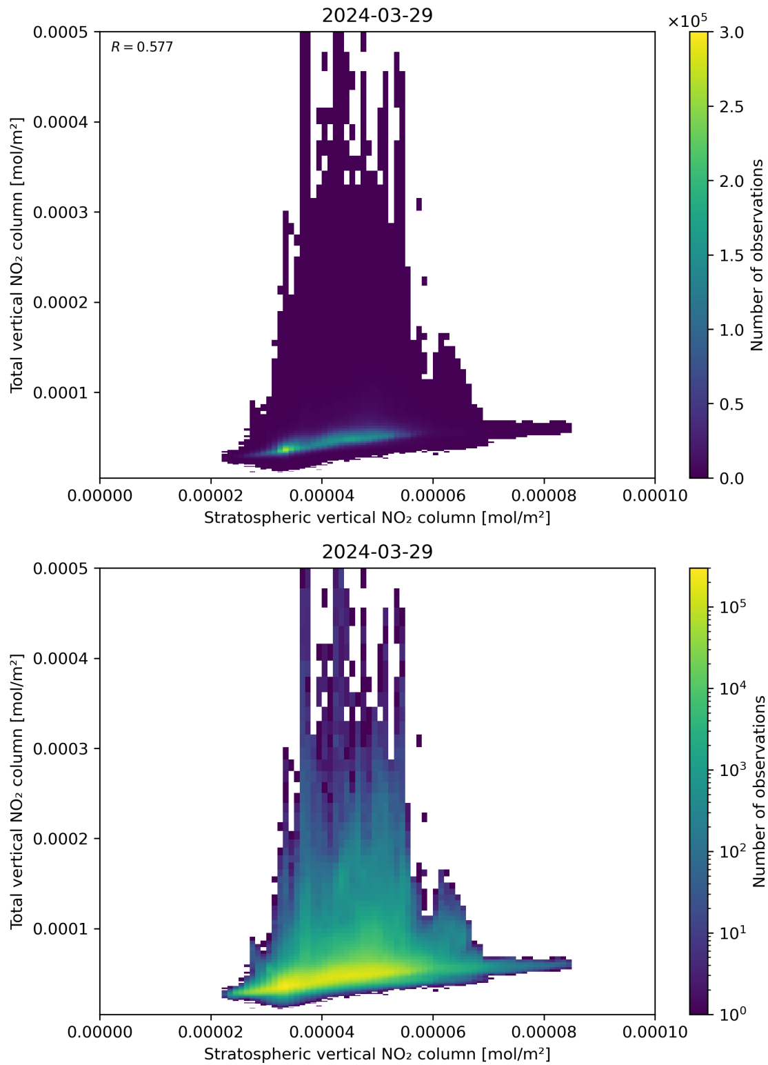
Figure 100: Scatter density plot of “Stratospheric vertical NO 2 column” against “Total vertical NO 2 column” for 2024-03-28 to 2024-03-30.
