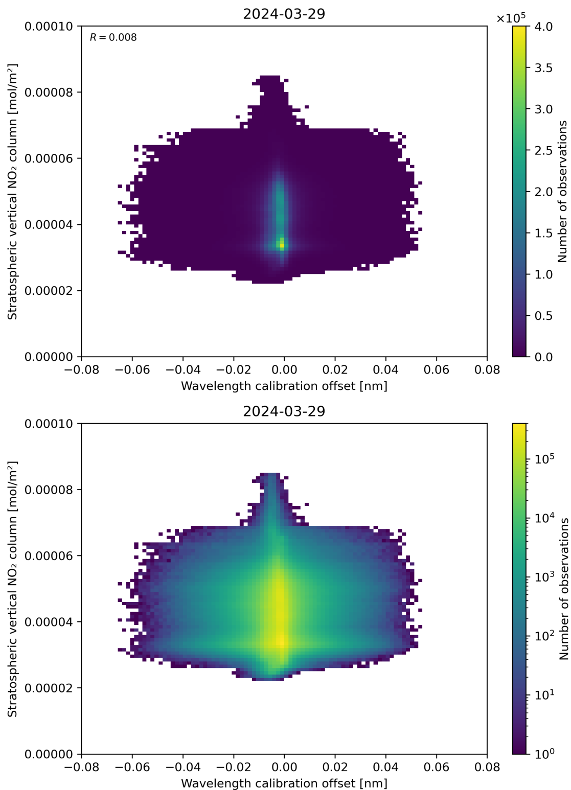
Figure 176: Scatter density plot of “Wavelength calibration offset” against “Stratospheric vertical NO 2 column” for 2024-03-28 to 2024-03-30.
