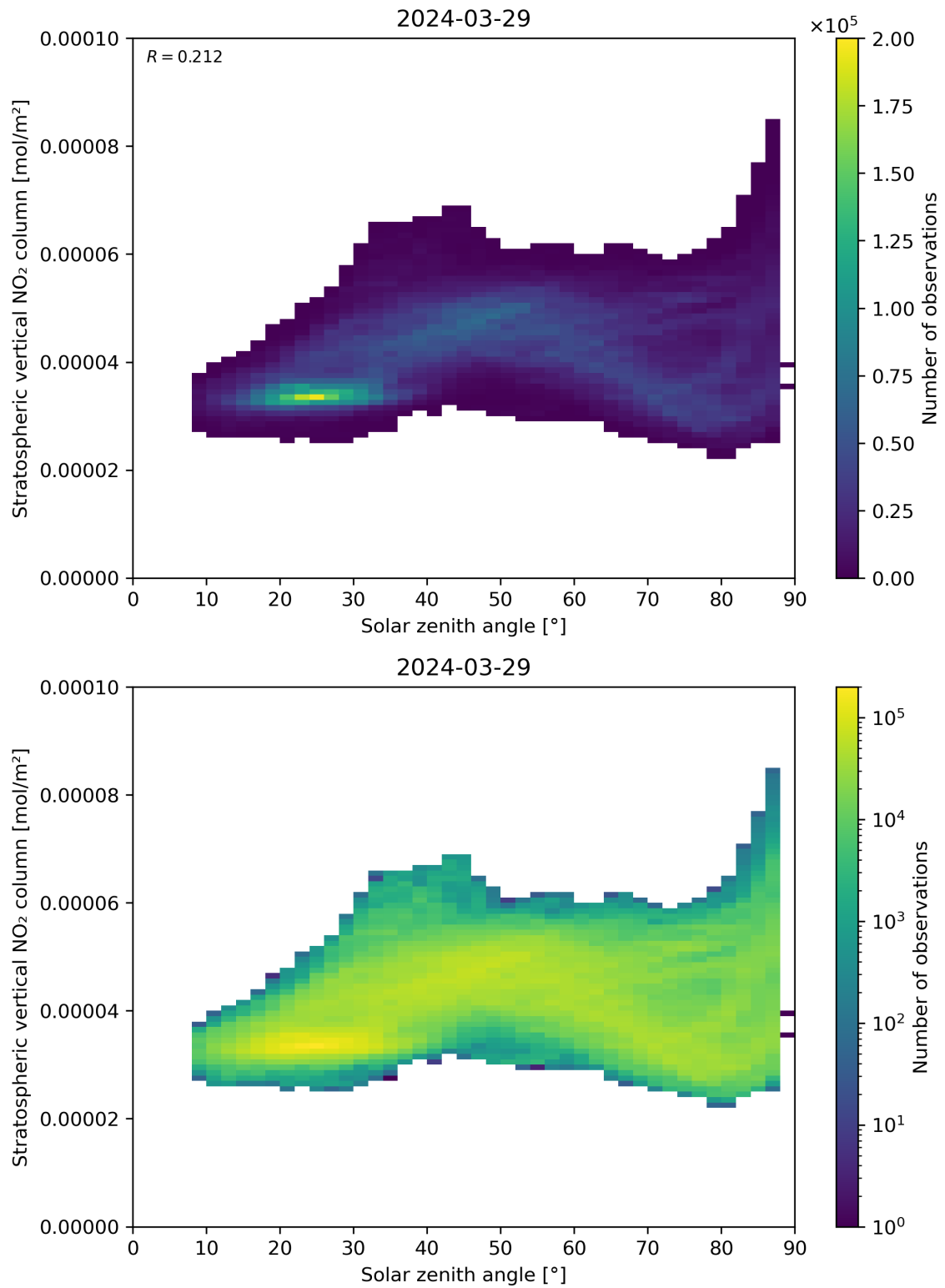
Figure 150: Scatter density plot of “Solar zenith angle” against “Stratospheric vertical NO 2 column” for 2024-03-28 to 2024-03-30.
