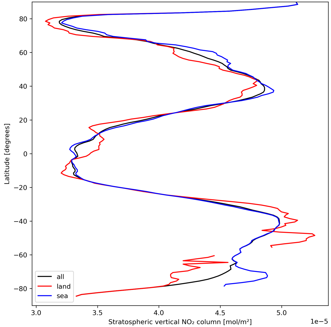
Figure 19: Zonal average of “Stratospheric vertical NO 2 column” for 2024-03-28 to 2024-03-30.
