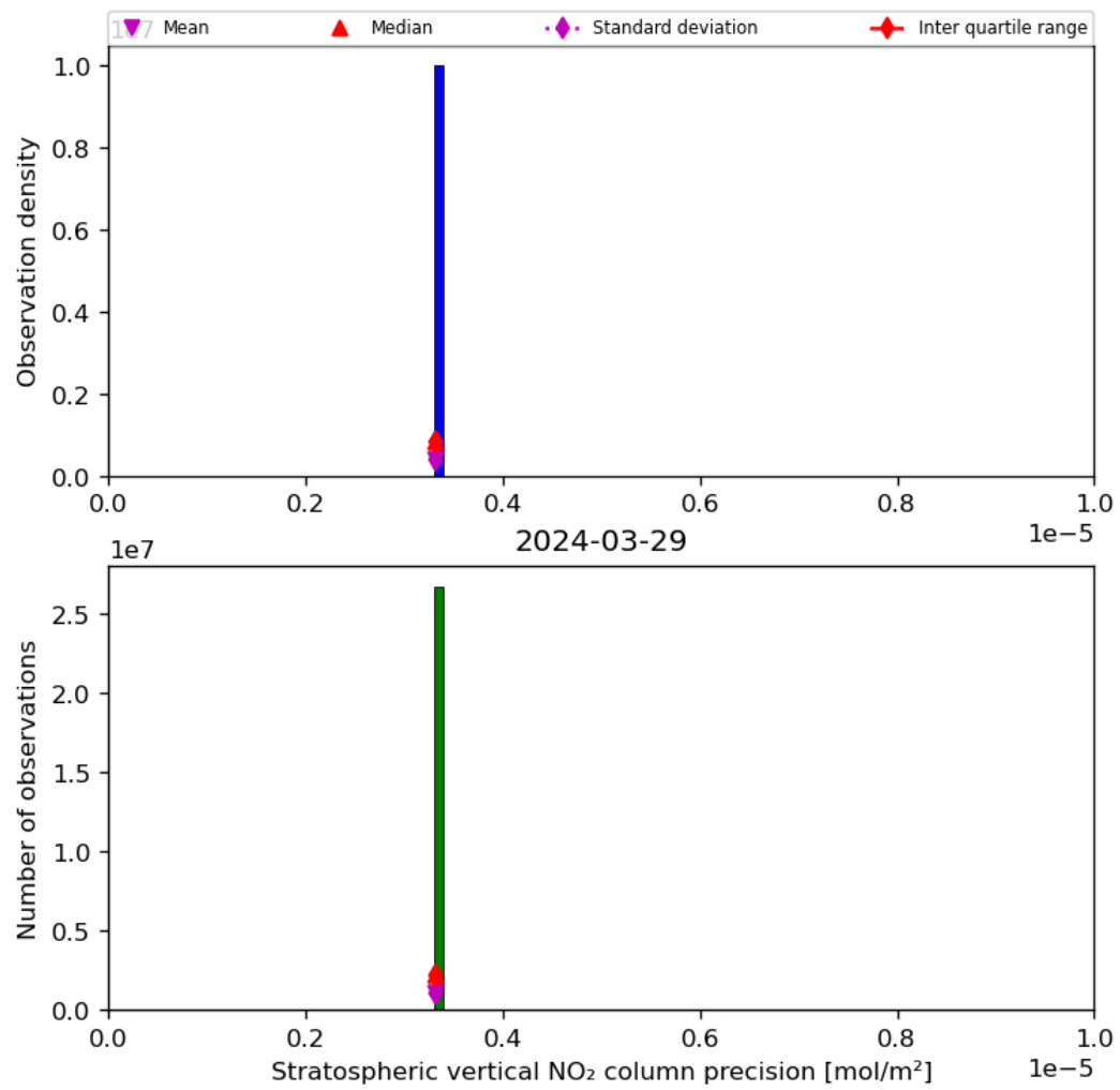
Figure 37: Histogram of “Stratospheric vertical NO 2 column precision” for 2024-03-28 to 2024-03-30
