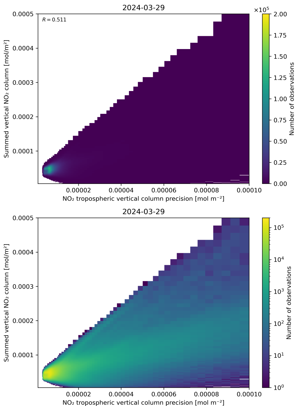
Figure 136: Scatter density plot of “NO 2 tropospheric vertical column precision” against “Summed vertical NO 2 column” for 2024-03-28 to 2024-03-30.
