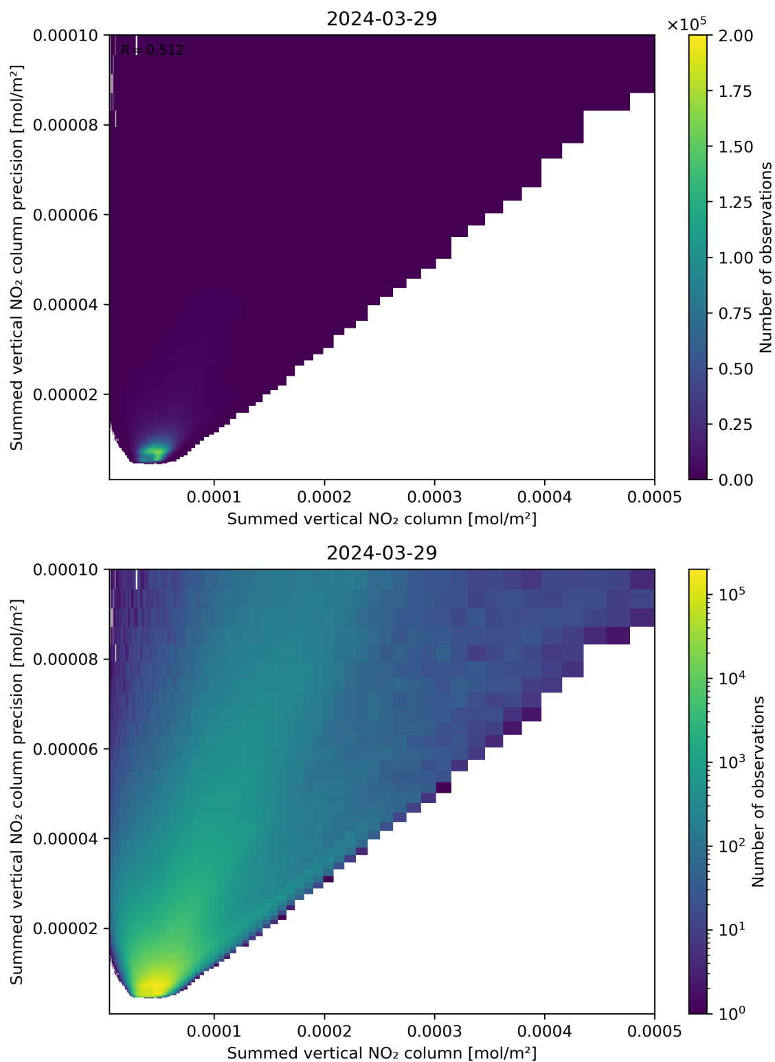
Figure 105: Scatter density plot of “Summed vertical NO 2 column” against “Summed vertical NO 2 column precision” for 2024-03-28 to 2024-03-30.
