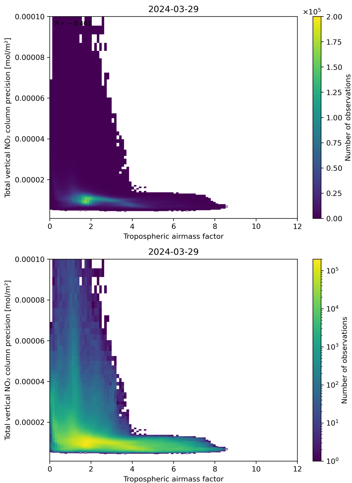
Figure 78: Scatter density plot of “Tropospheric air mass factor” against “Total vertical NO 2 column precision” for 2024-03-28 to 2024-03-30.
