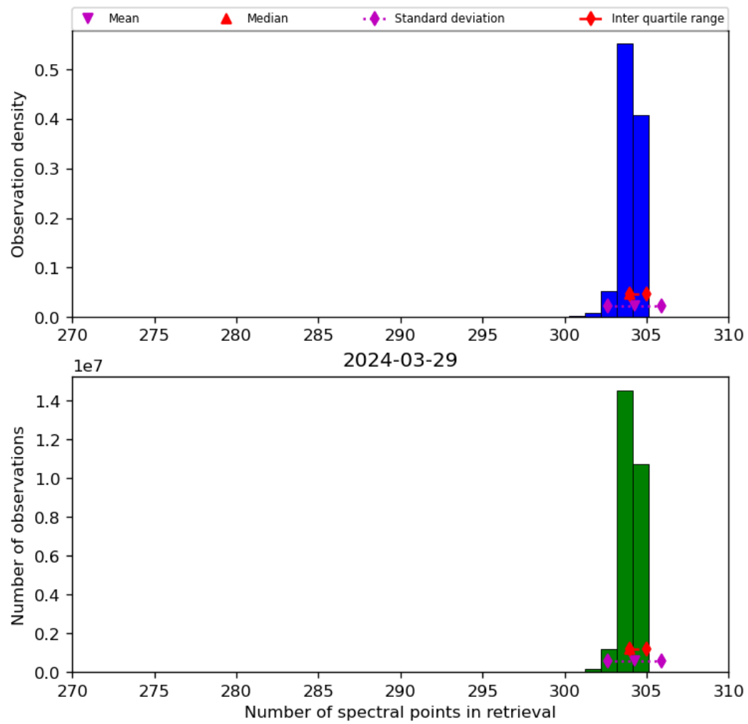
Figure 33: Histogram of “Number of spectral points in retrieval” for 2024-03-28 to 2024-03-30
