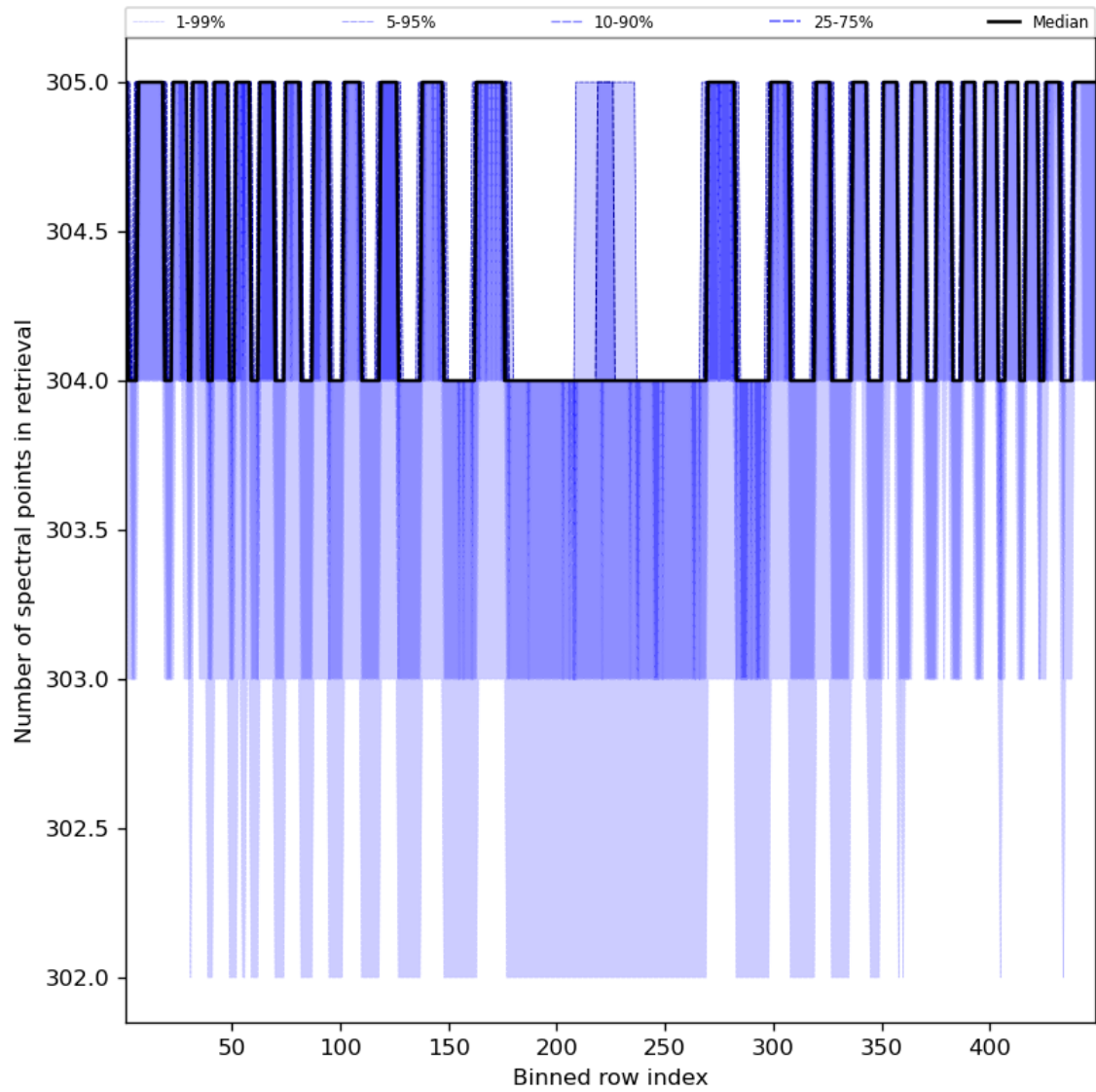
Figure 50: Along track statistics of “Number of spectral points in retrieval” for 2024-03-28 to 2024-03-30
