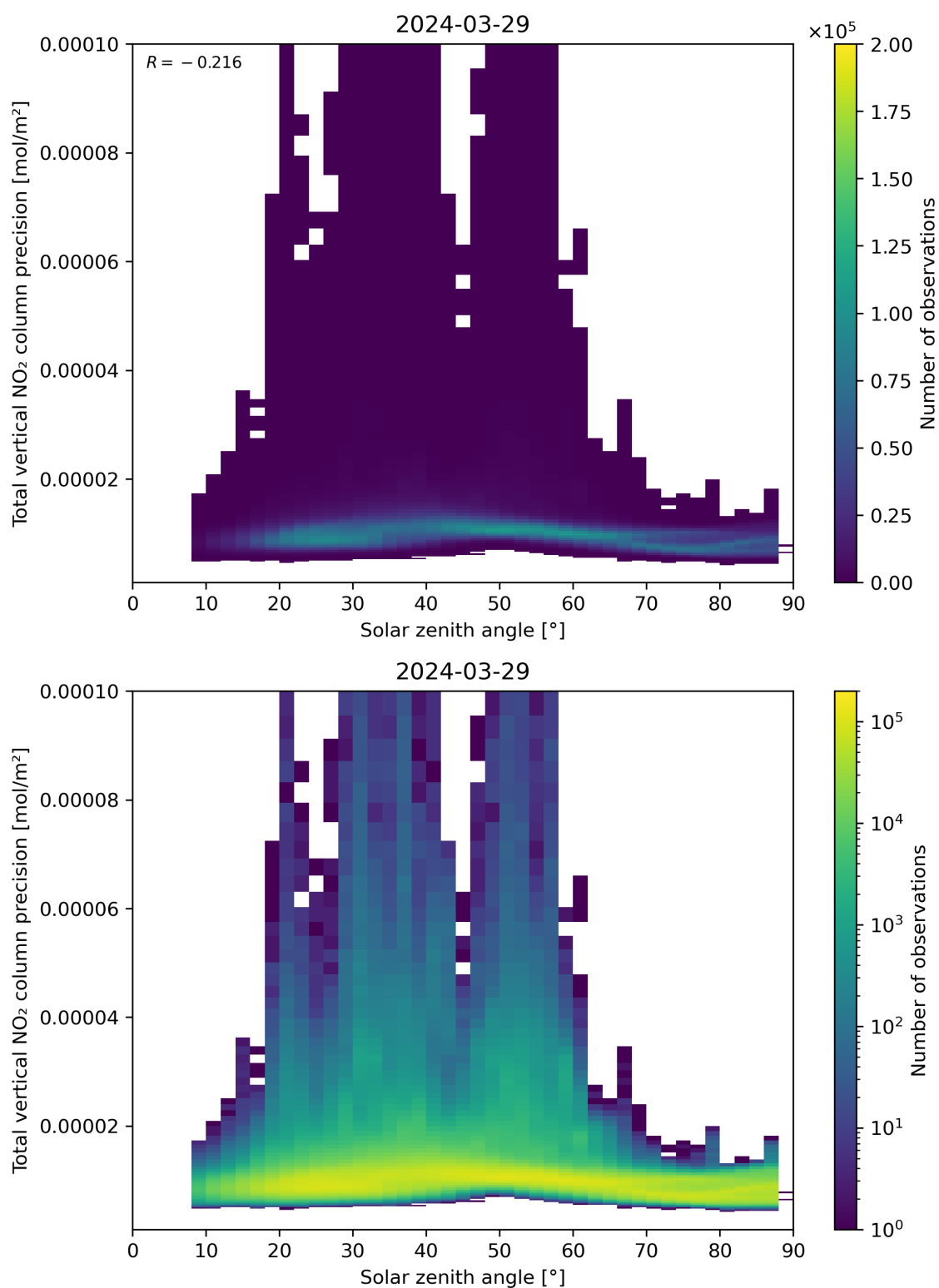
Figure 154: Scatter density plot of “Solar zenith angle” against “Total vertical NO 2 column precision” for 2024-03-28 to 2024-03-30.
