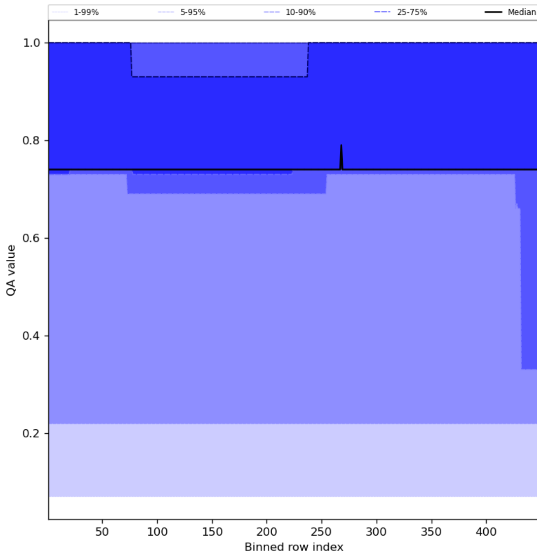
Figure 45: Along track statistics of “QA value” for 2024-03-28 to 2024-03-30
