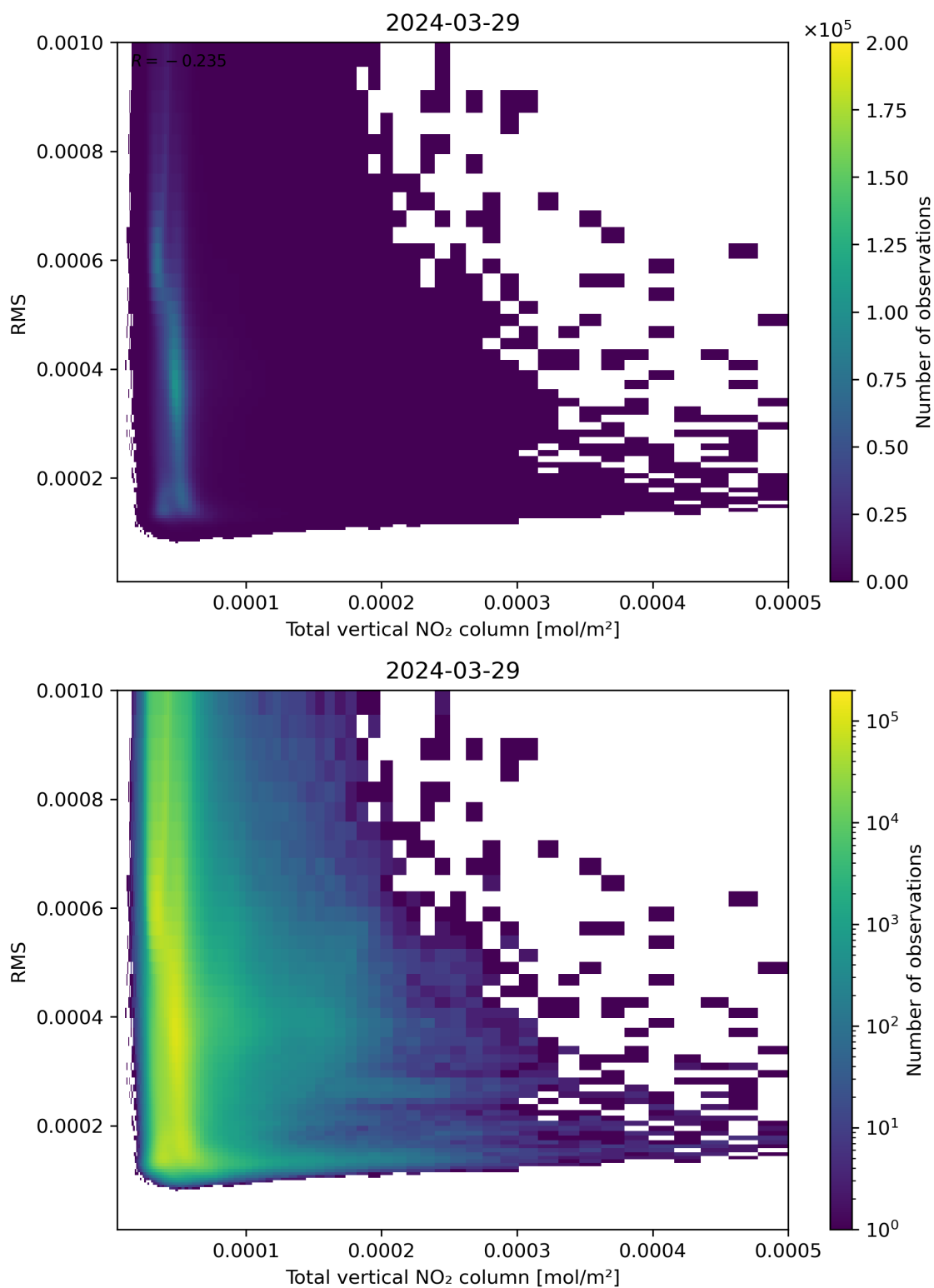
Figure 120: Scatter density plot of “Total vertical NO 2 column” against “RMS” for 2024-03-28 to 2024-03-30.
