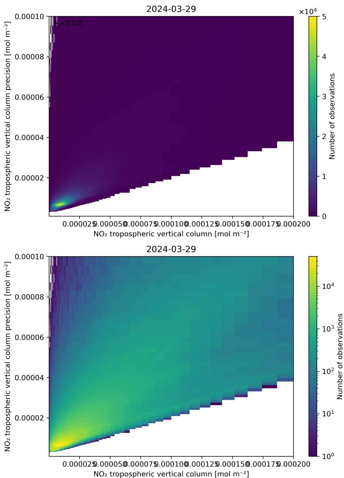
Figure 130: Scatter density plot of “NO 2 tropospheric vertical column” against “NO 2 tropospheric vertical column precision” for 2024-03-28 to 2024-03-30.
