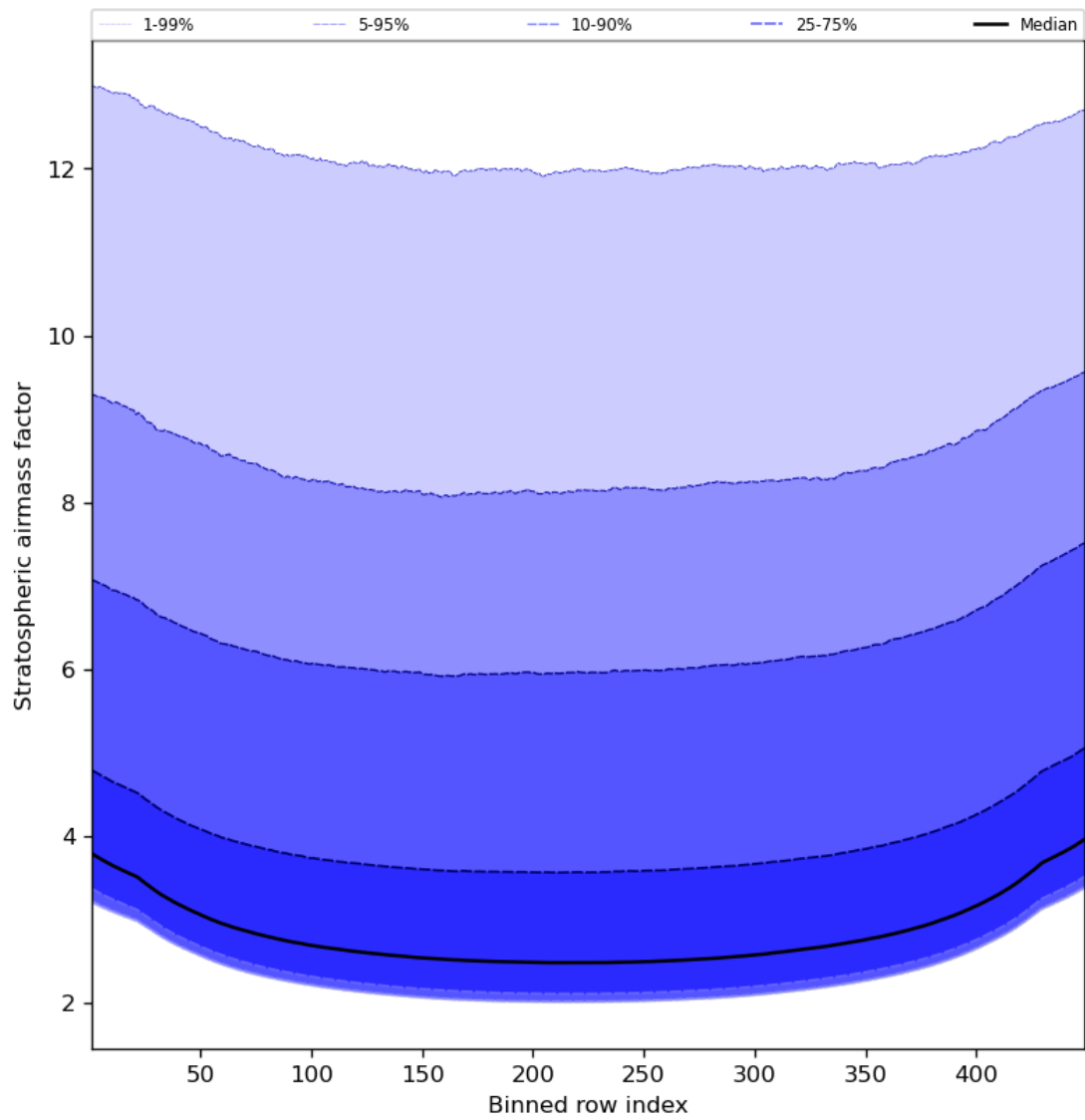
Figure 61: Along track statistics of “Stratospheric airmass factor” for 2024-03-28 to 2024-03-30
