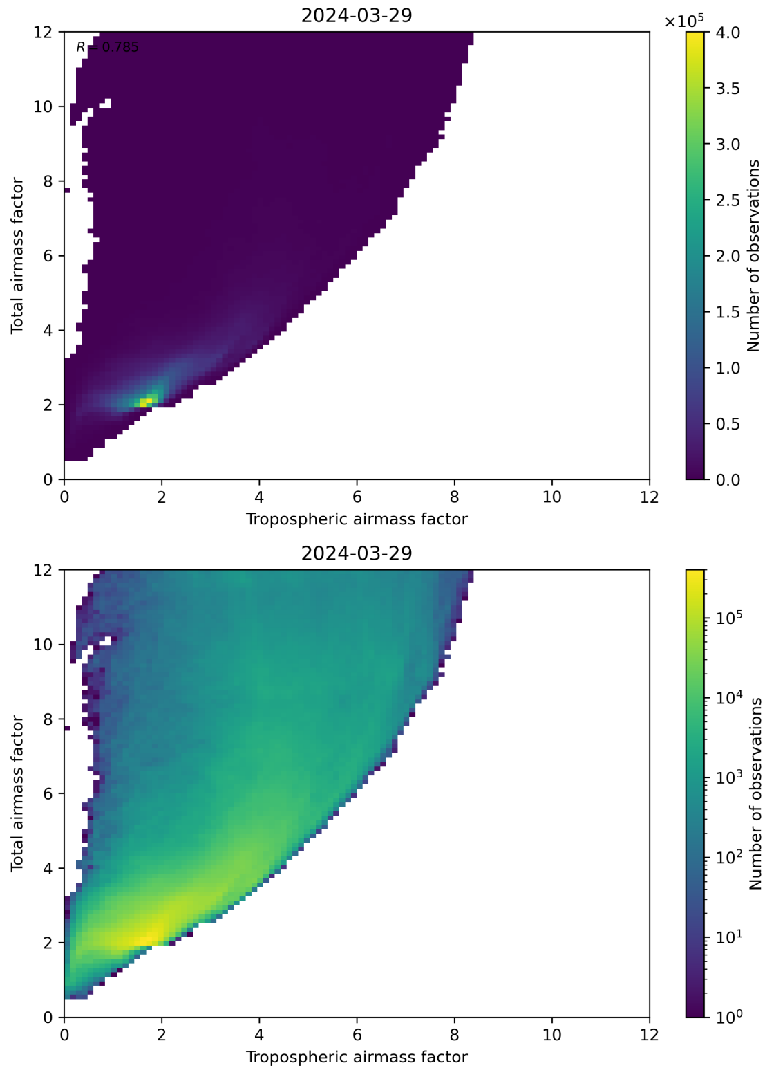
Figure 72: Scatter density plot of “Tropospheric airmass factor” against “Total airmass factor” for 2024-03-28 to 2024-03-30.
