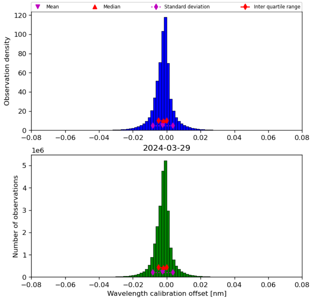
Figure 35: Histogram of “Wavelength calibration offset” for 2024-03-28 to 2024-03-30
