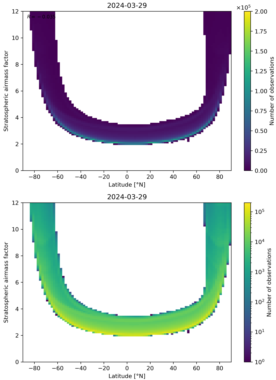
Figure 83: Scatter density plot of “Latitude” against “Stratospheric airmass factor” for 2024-03-28 to 2024-03-30.
