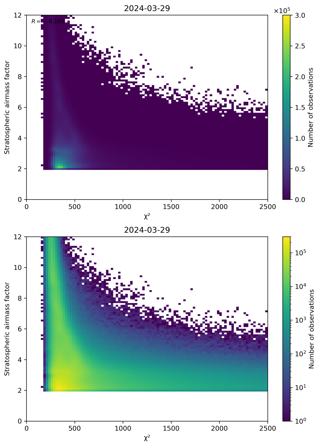
Figure 81: Scatter density plot of “ \chi^2 ” against “Stratospheric airmass factor” for 2024-03-28 to 2024-03-30.
