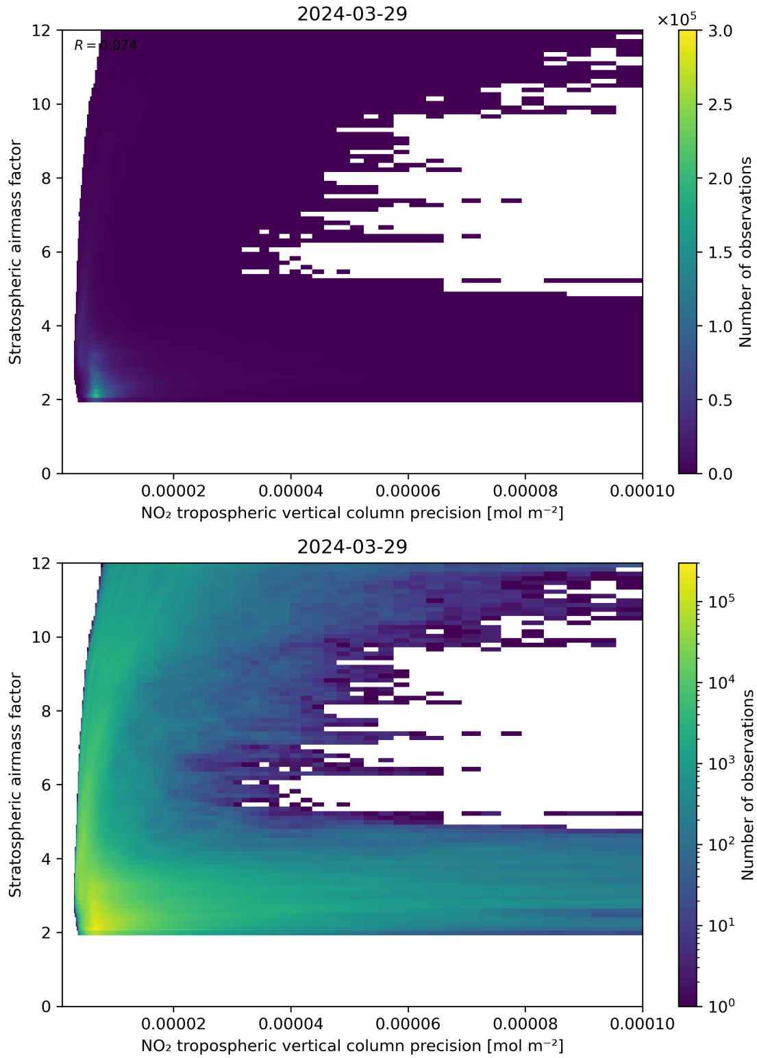
Figure 131: Scatter density plot of “NO 2 tropospheric vertical column precision” against “Stratospheric airmass factor” for 2024-03-28 to 2024-03-30.
