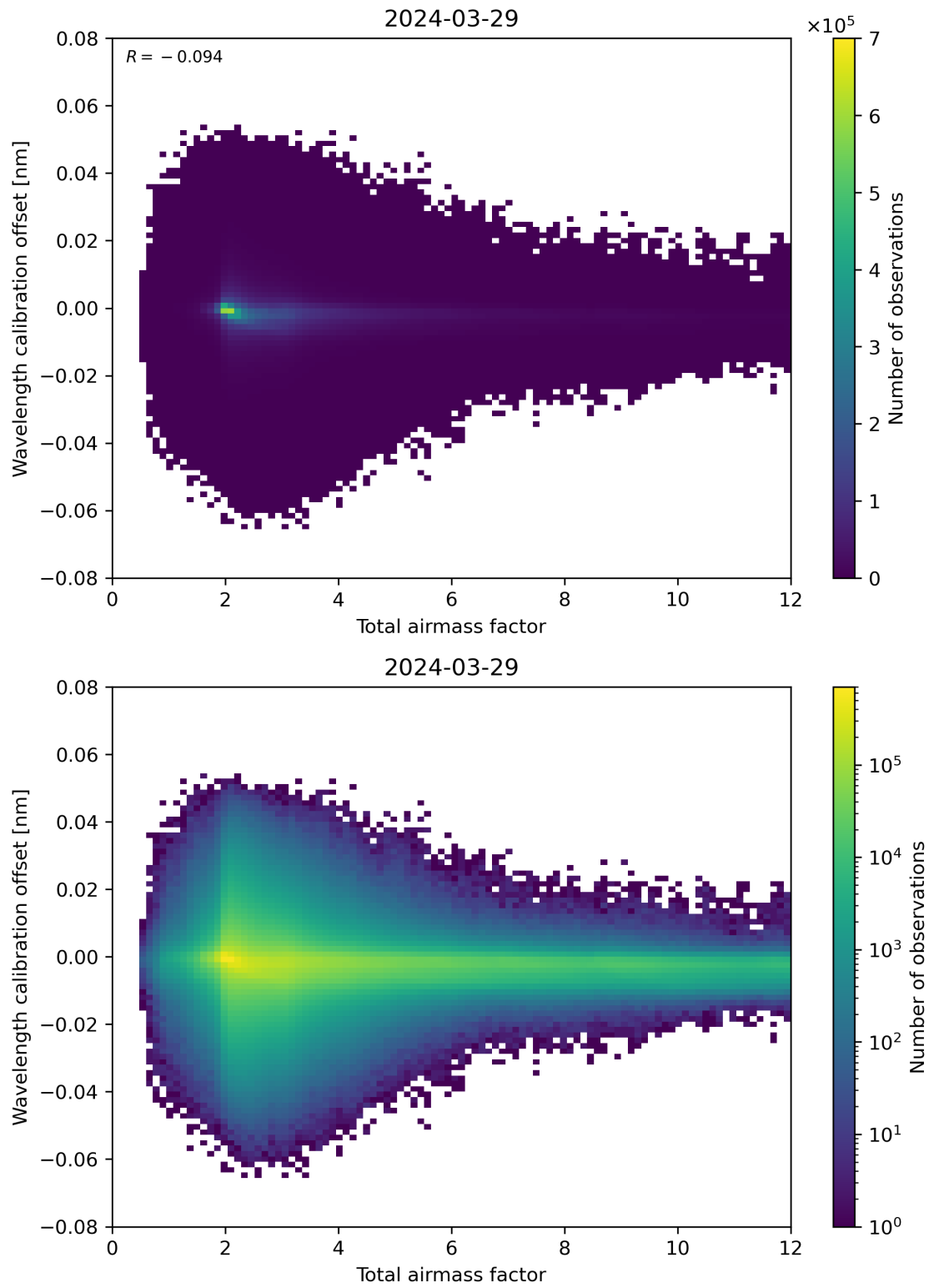
Figure 70: Scatter density plot of “Total airmass factor” against “Wavelength calibration offset” for 2024-03-28 to 2024-03-30.
