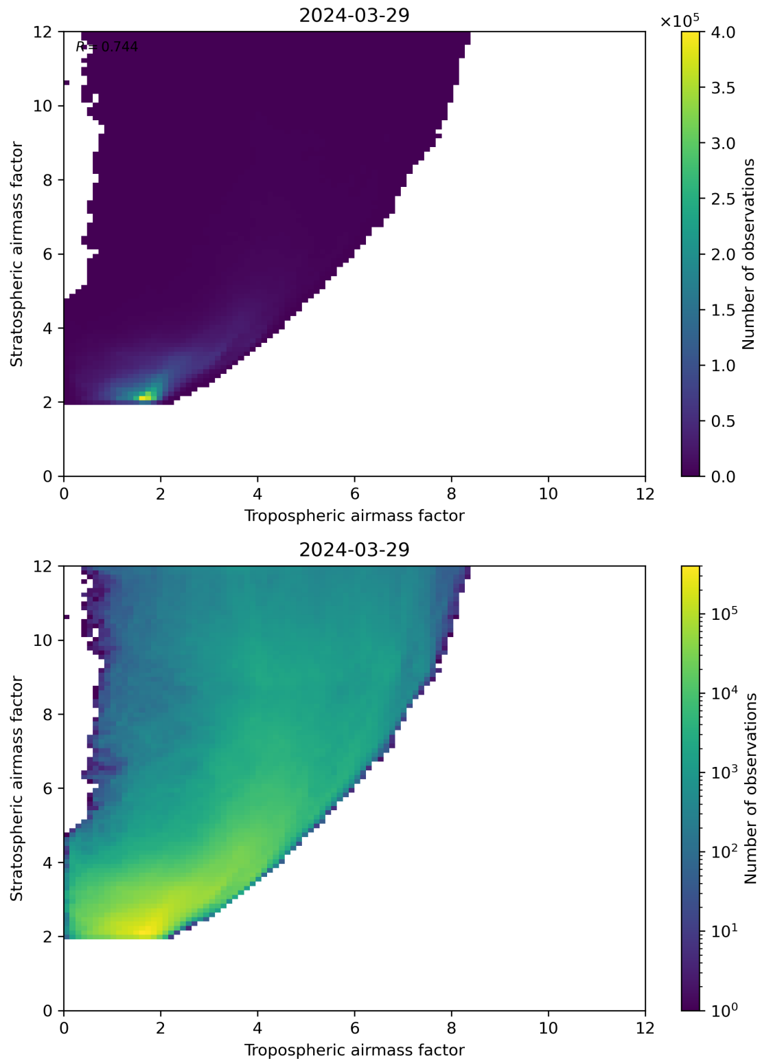
Figure 71: Scatter density plot of “Tropospheric airmass factor” against “Stratospheric airmass factor” for 2024-03-28 to 2024-03-30.
