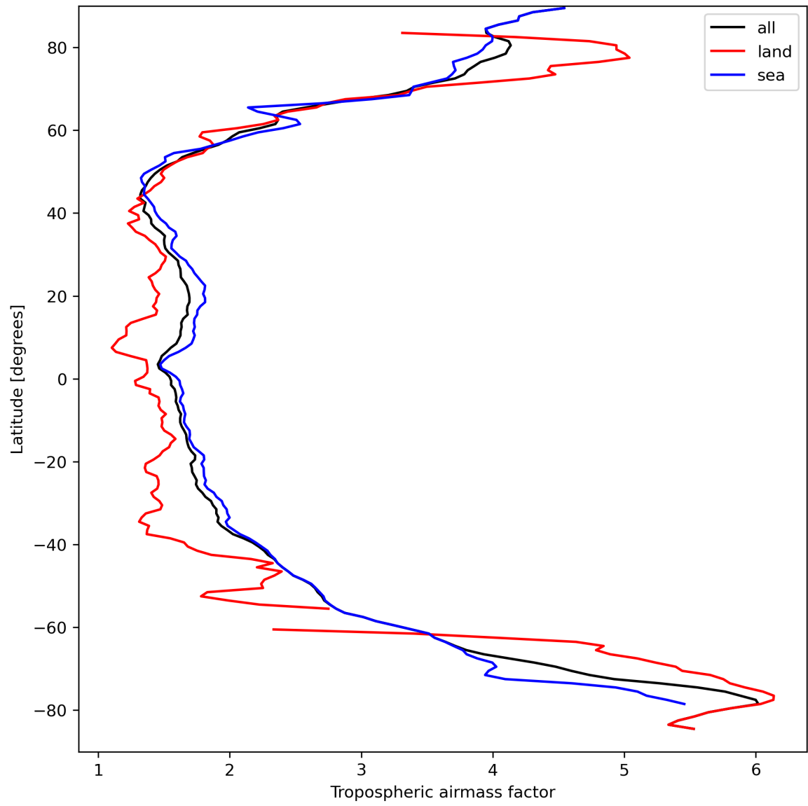
Figure 14: Zonal average of “Tropospheric airmass factor” for 2024-03-28 to 2024-03-30.
