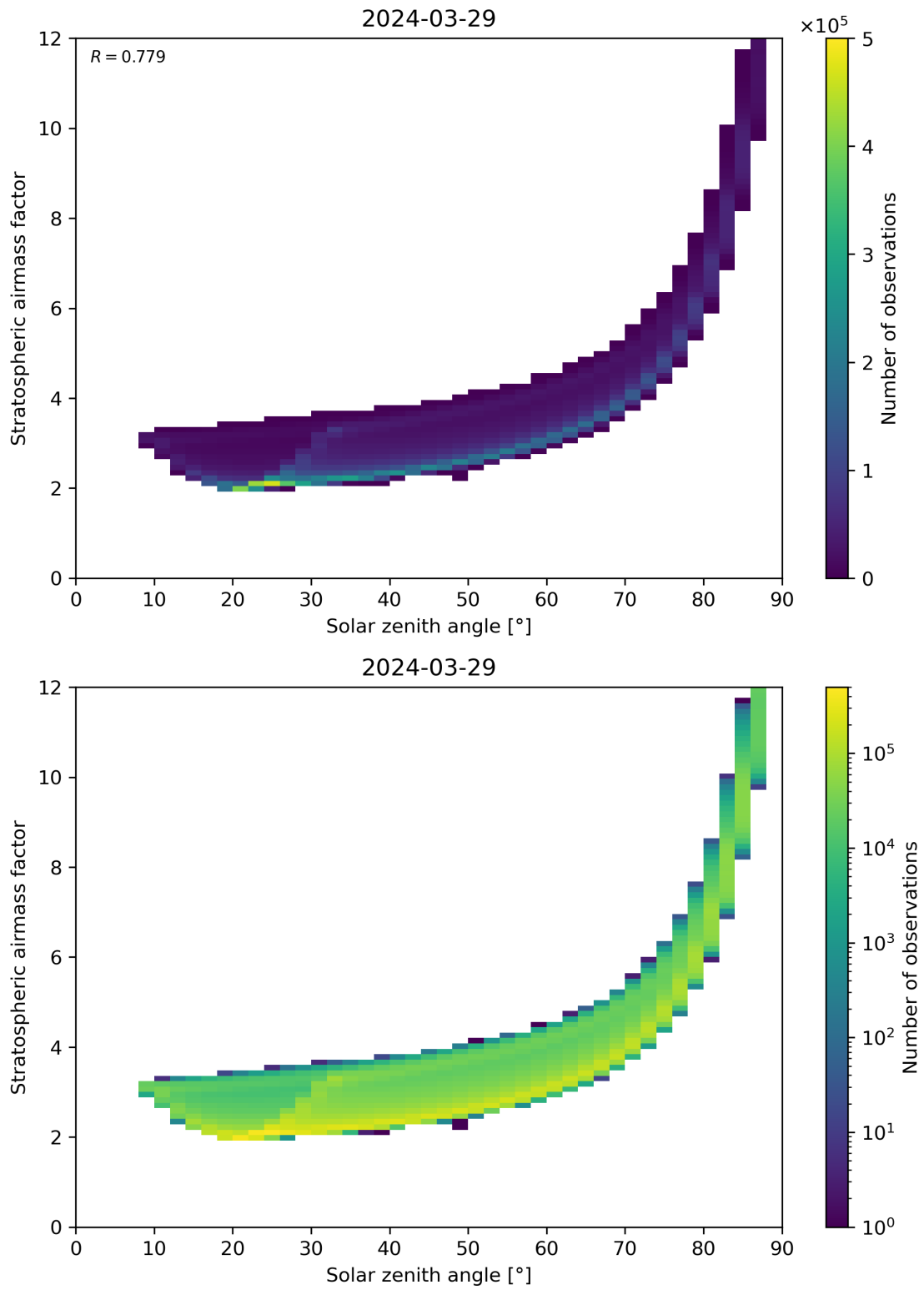
Figure 145: Scatter density plot of “Solar zenith angle” against “Stratospheric airmass factor” for 2024-03-28 to 2024-03-30.
