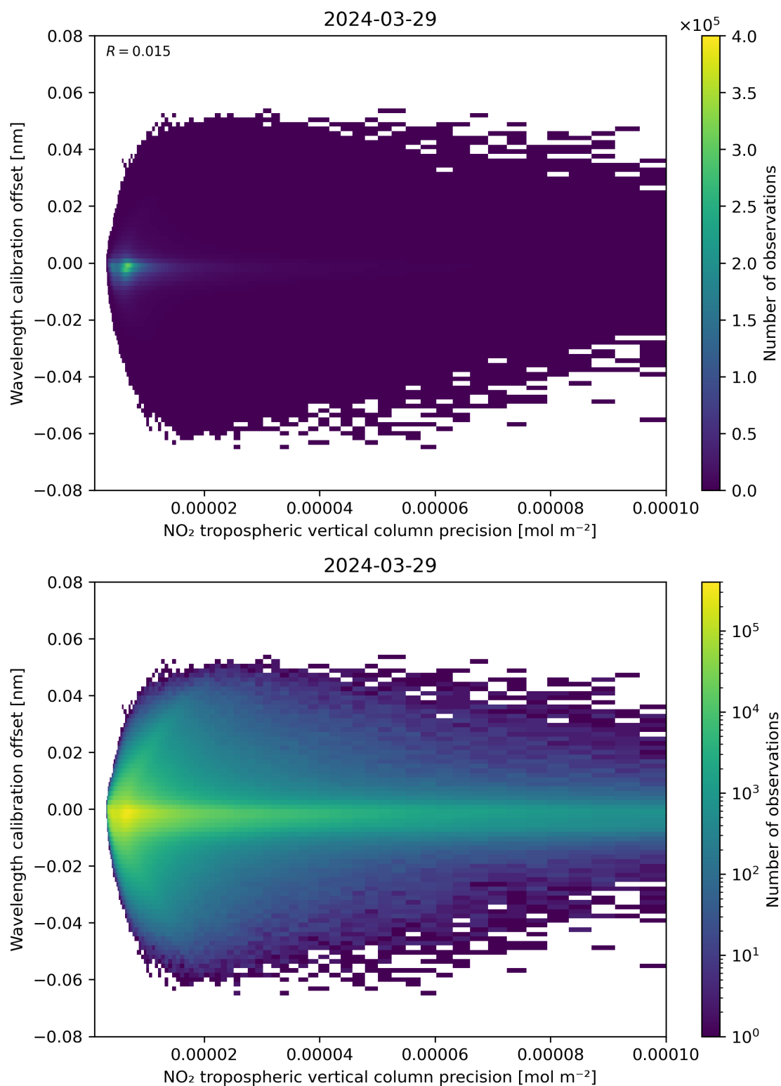
Figure 141: Scatter density plot of “NO 2 tropospheric vertical column precision” against “Wavelength calibration offset” for 2024-03-28 to 2024-03-30.
