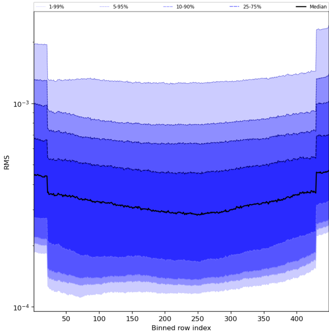
Figure 60: Along track statistics of “RMS” for 2024-03-28 to 2024-03-30
