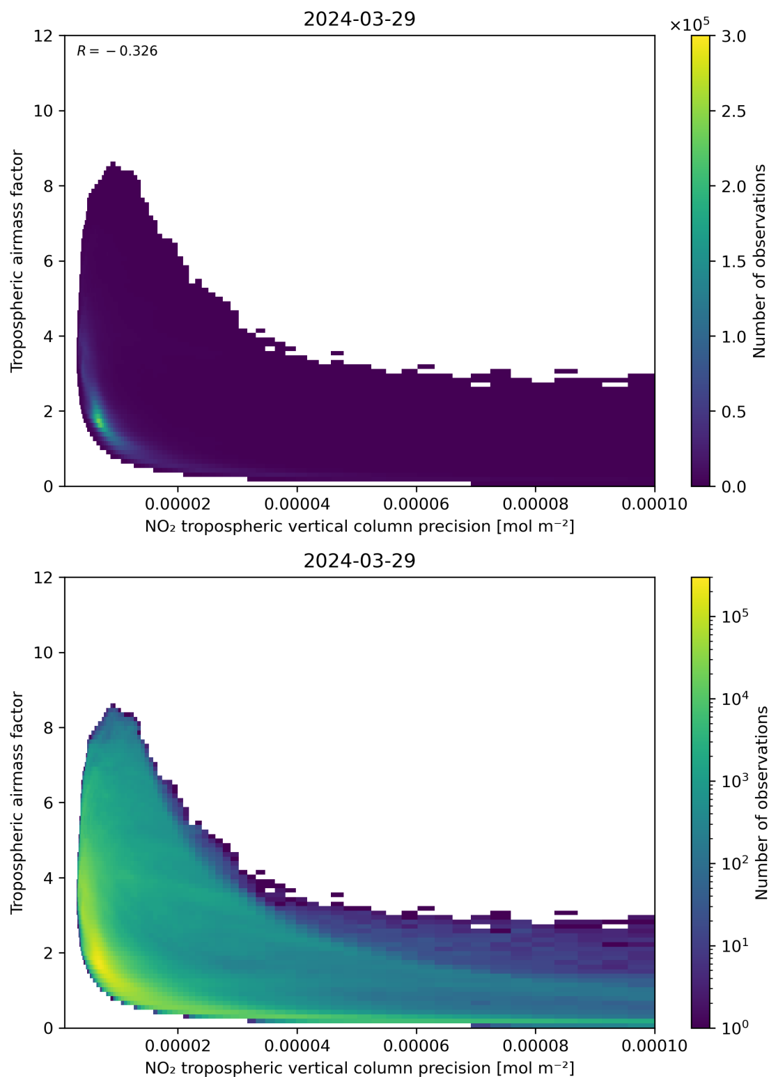
Figure 133: Scatter density plot of “NO 2 tropospheric vertical column precision” against “Tropospheric airmass factor” for 2024-03-28 to 2024-03-30.
