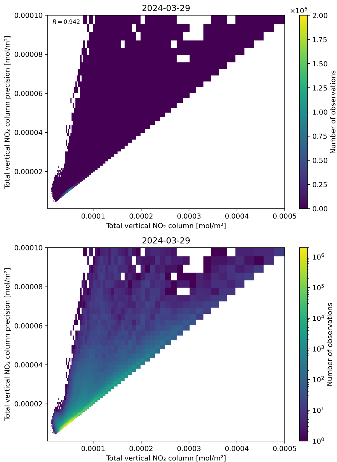
Figure 114: Scatter density plot of “Total vertical NO 2 column” against “Total vertical NO 2 column precision” for 2024-03-28 to 2024-03-30.
