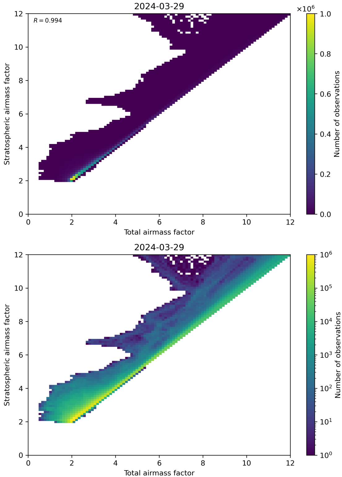
Figure 62: Scatter density plot of “Total airmass factor” against “Stratospheric airmass factor” for 2024-03-28 to 2024-03-30.
