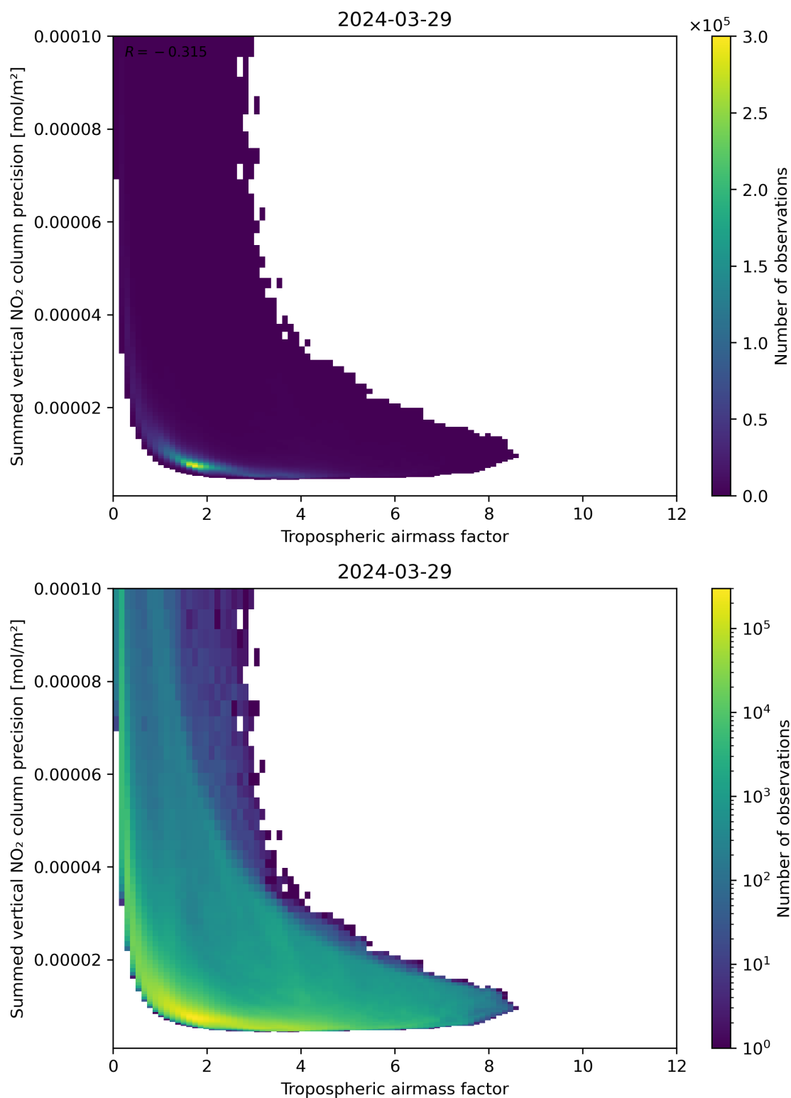
Figure 76: Scatter density plot of “Tropospheric air mass factor” against “Summed vertical NO 2 column precision” for 2024-03-28 to 2024-03-30.
