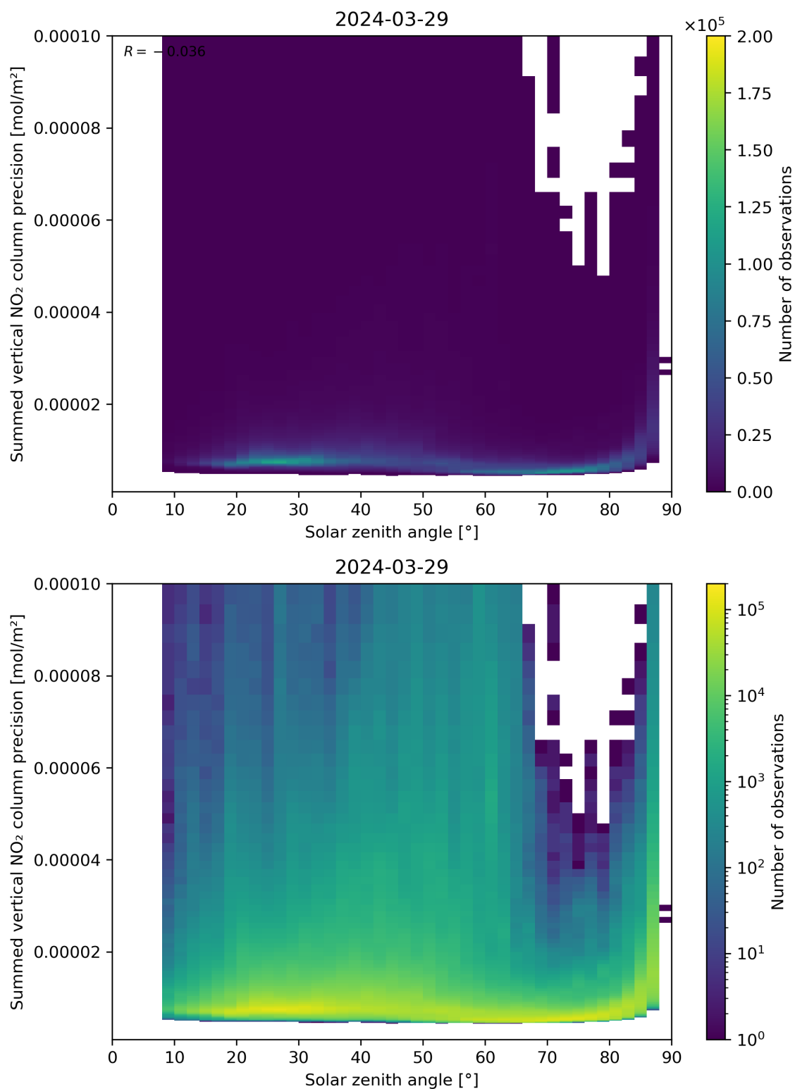
Figure 152: Scatter density plot of “Solar zenith angle” against “Summed vertical NO 2 column precision” for 2024-03-28 to 2024-03-30.
