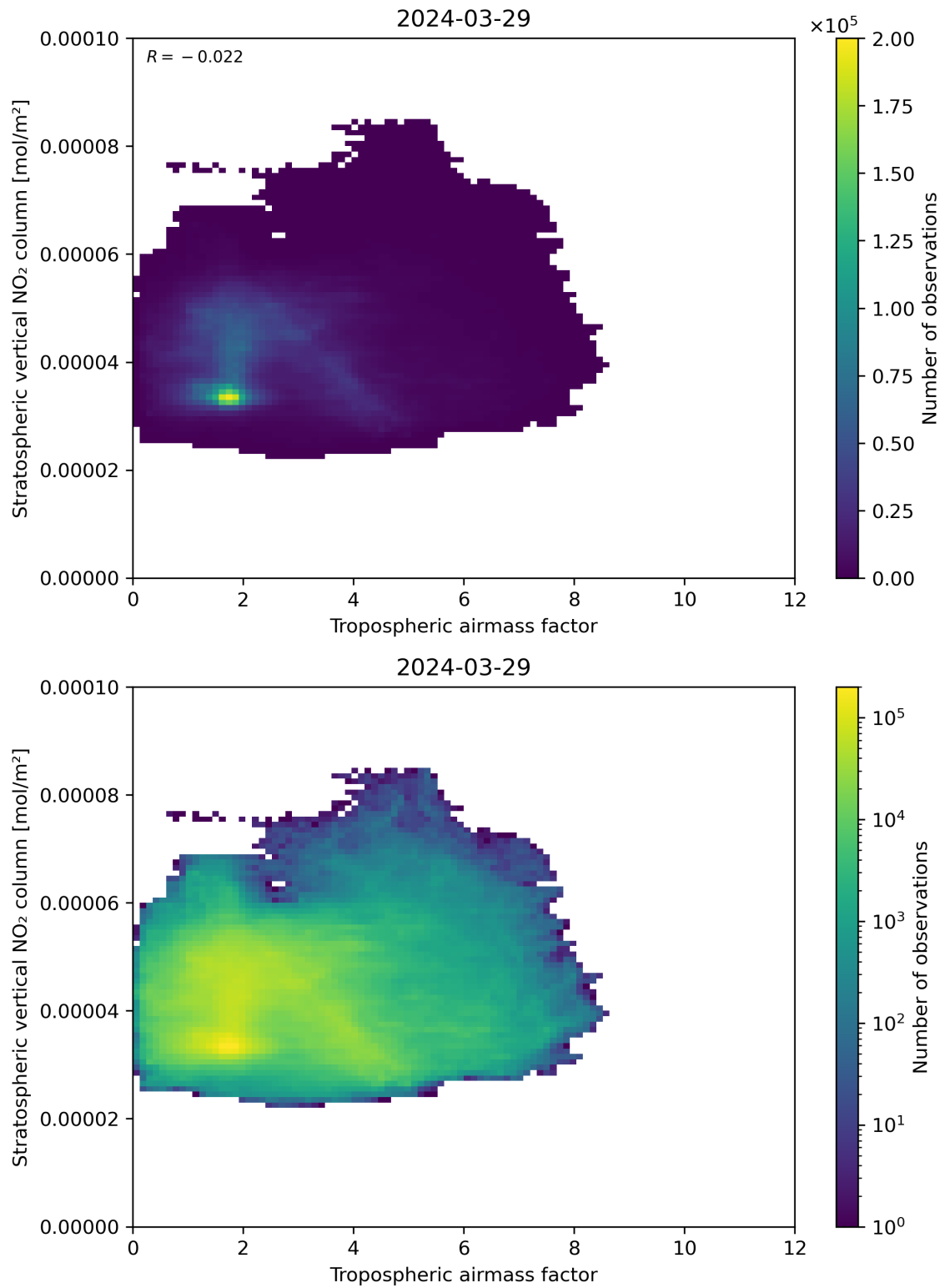
Figure 74: Scatter density plot of “Tropospheric air mass factor” against “Stratospheric vertical NO 2 column” for 2024-03-28 to 2024-03-30.
