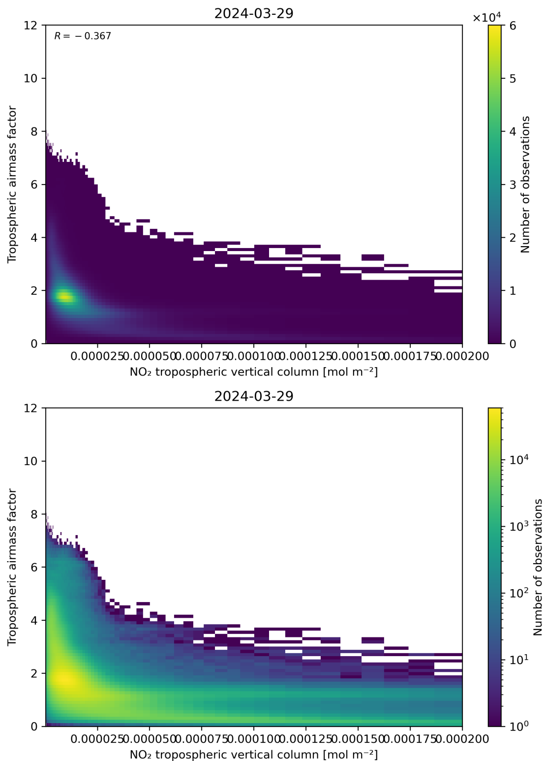
Figure 123: Scatter density plot of “NO 2 tropospheric vertical column” against “Tropospheric airmass factor” for 2024-03-28 to 2024-03-30.
