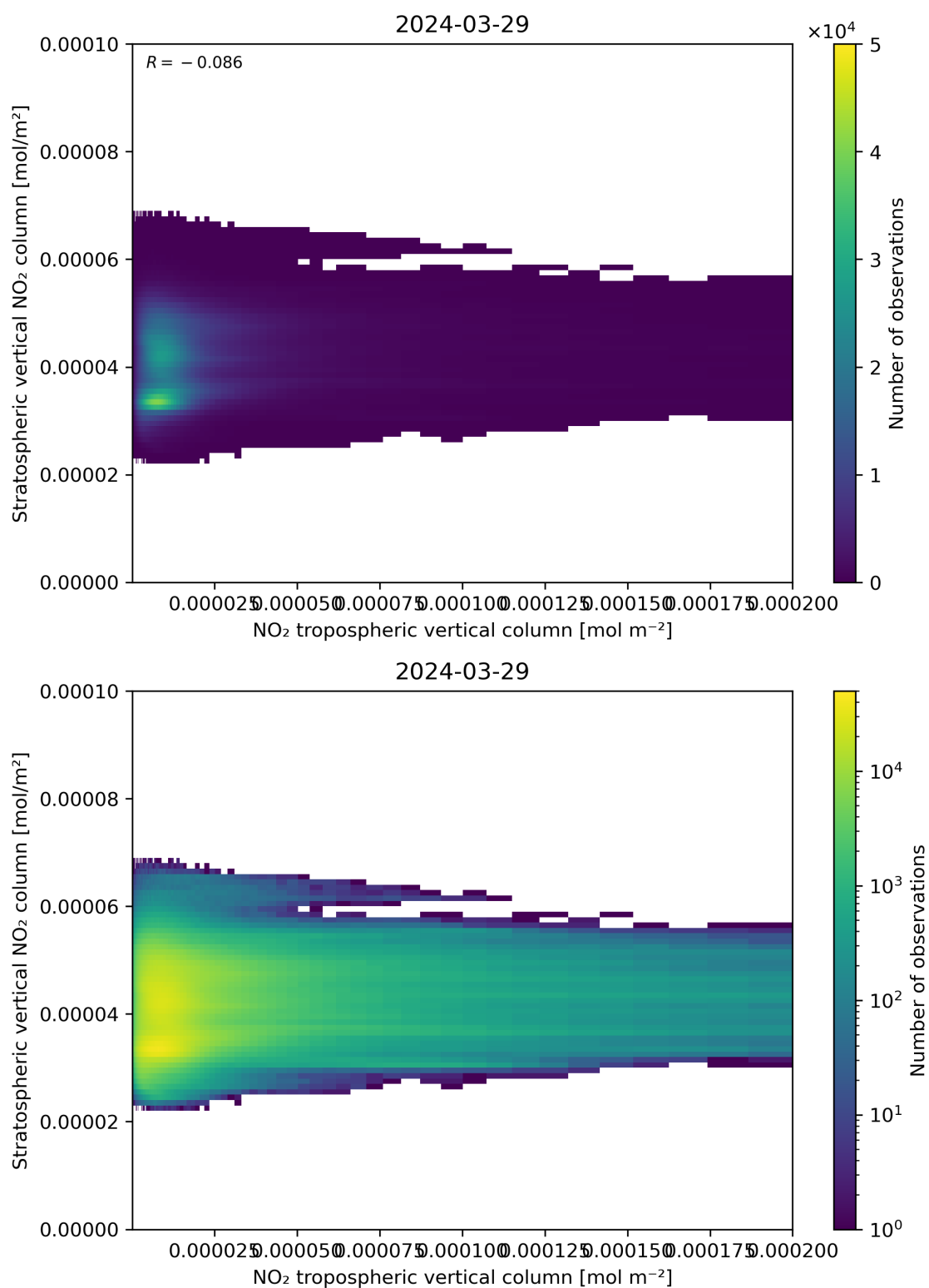
Figure 125: Scatter density plot of “NO 2 tropospheric vertical column” against “Stratospheric vertical NO 2 column” for 2024-03-28 to 2024-03-30.
