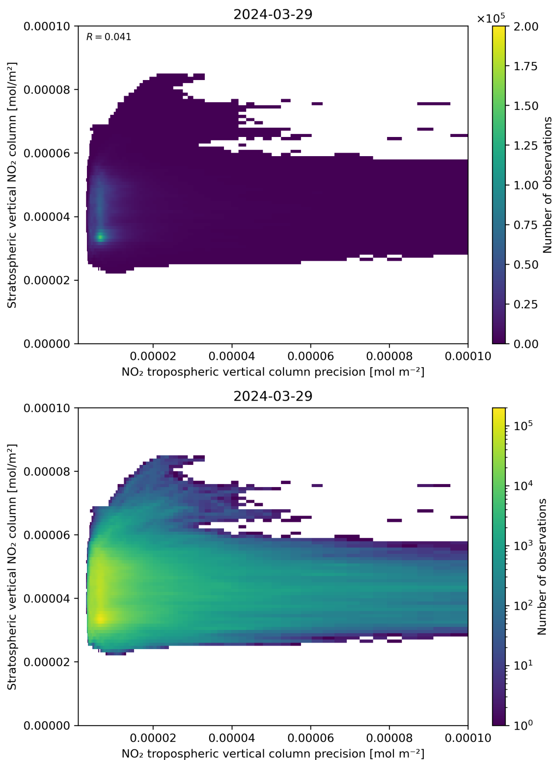
Figure 135: Scatter density plot of “NO 2 tropospheric vertical column precision” against “Stratospheric vertical NO 2 column” for 2024-03-28 to 2024-03-30.
