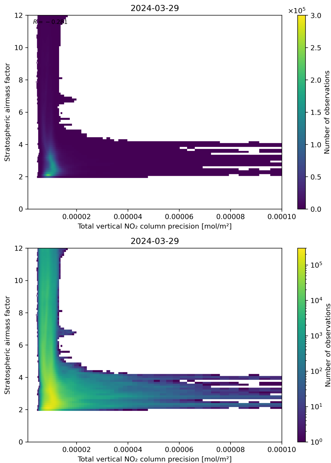
Figure 115: Scatter density plot of “Total vertical NO 2 column precision” against “Stratospheric air mass factor” for 2024-03-28 to 2024-03-30.
