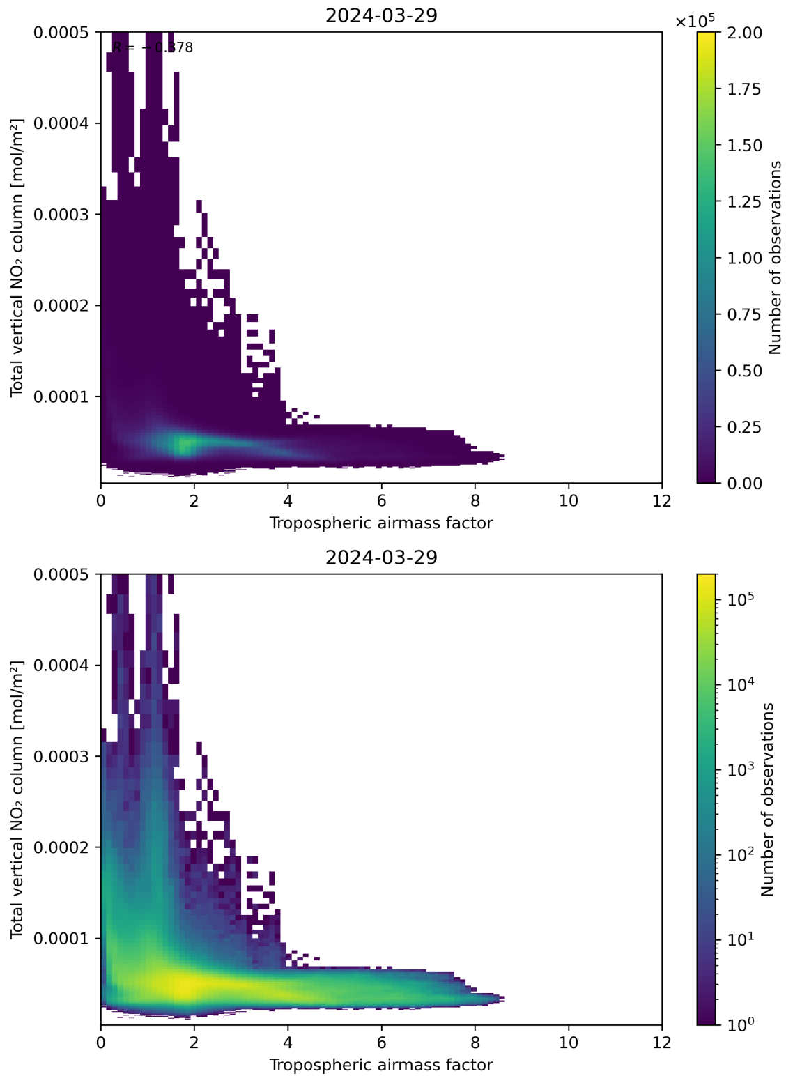
Figure 77: Scatter density plot of “Tropospheric airmass factor” against “Total vertical NO 2 column” for 2024-03-28 to 2024-03-30.
