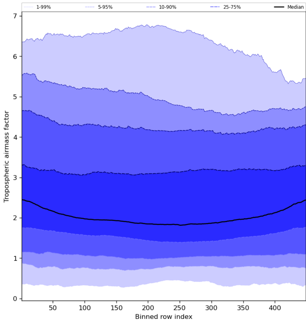
Figure 48: Along track statistics of “Tropospheric air mass factor” for 2024-03-28 to 2024-03-30
