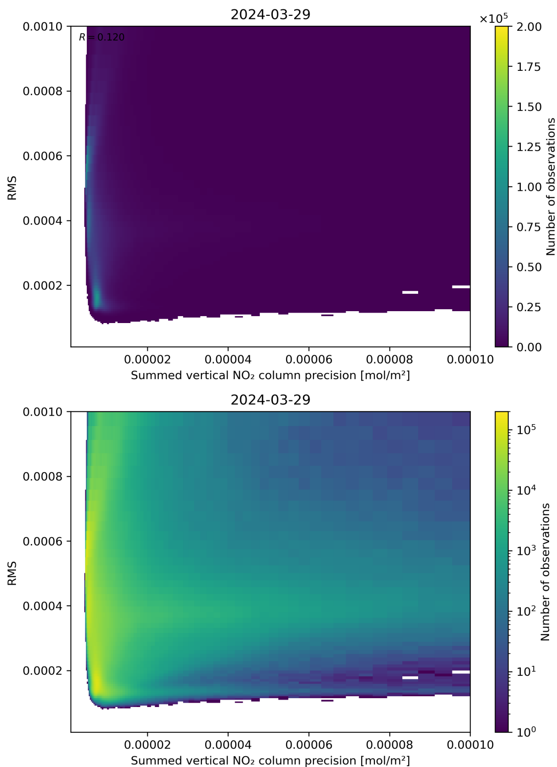
Figure 108: Scatter density plot of “Summed vertical NO 2 column precision” against “RMS” for 2024-03-28 to 2024-03-30.
