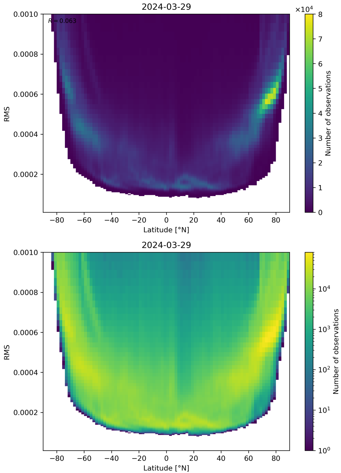
Figure 94: Scatter density plot of “Latitude” against “RMS” for 2024-03-28 to 2024-03-30.
