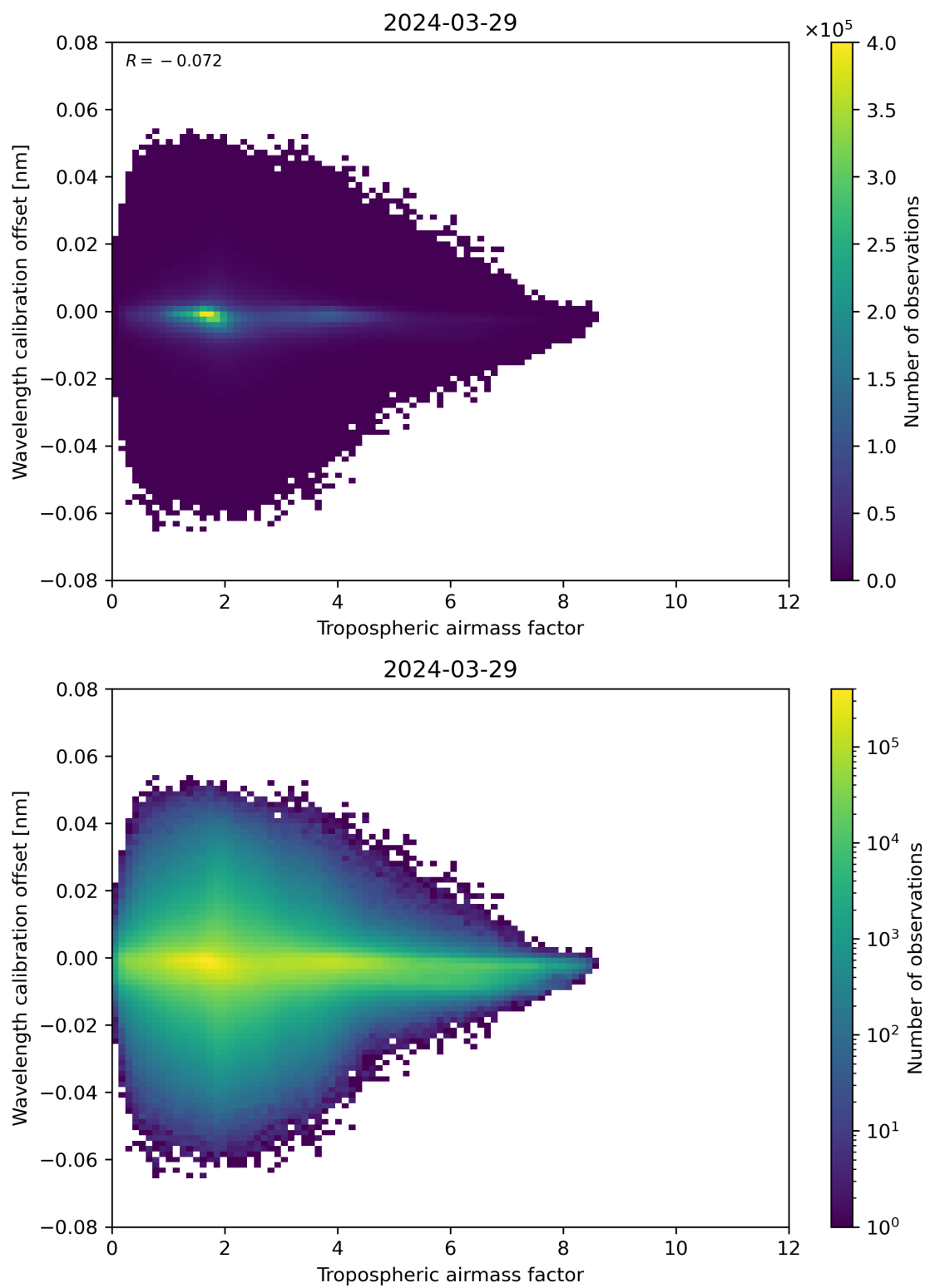
Figure 80: Scatter density plot of “Tropospheric airmass factor” against “Wavelength calibration offset” for 2024-03-28 to 2024-03-30.
