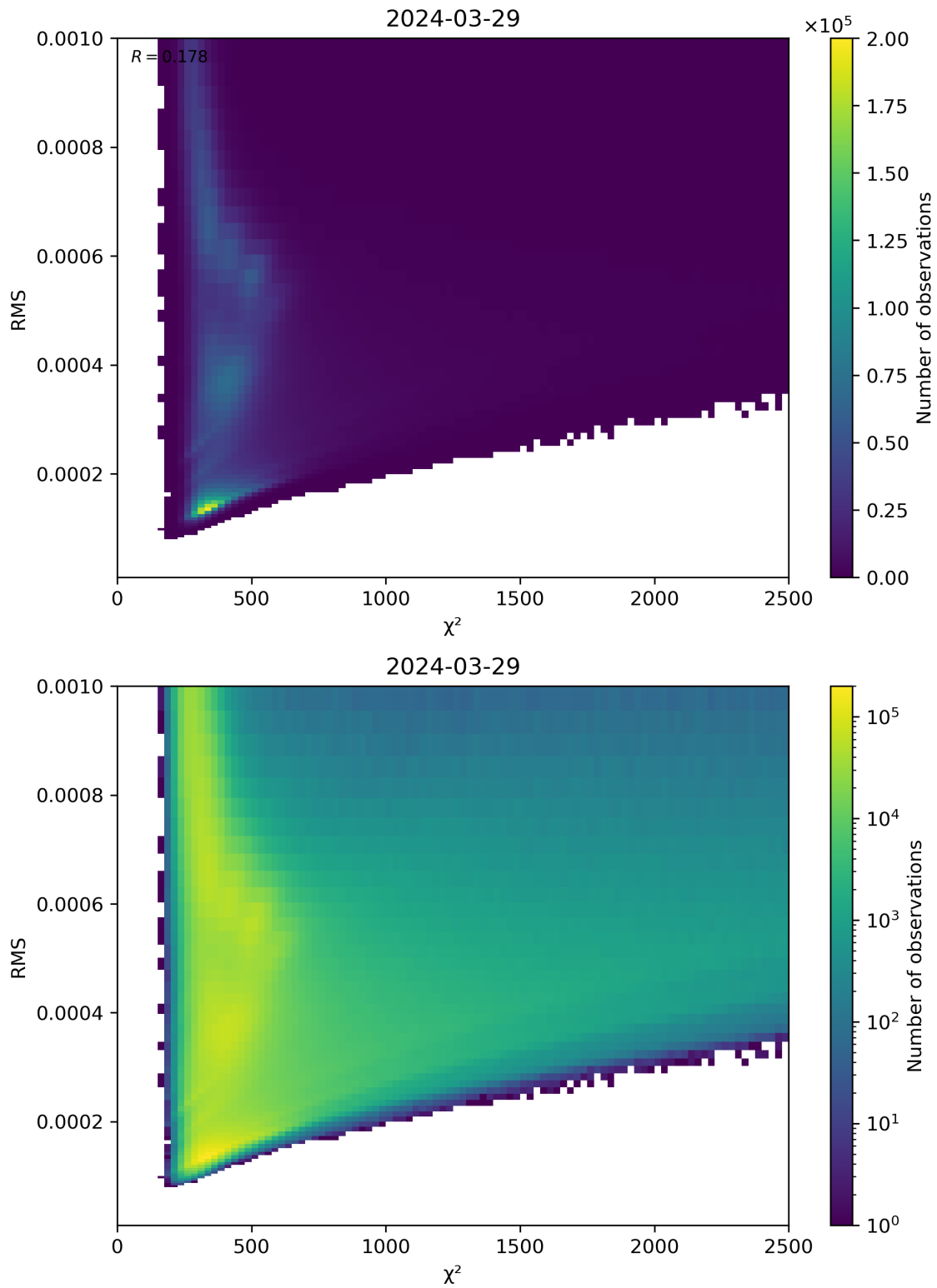
Figure 82: Scatter density plot of “ \chi^2 ” against “RMS” for 2024-03-28 to 2024-03-30.
