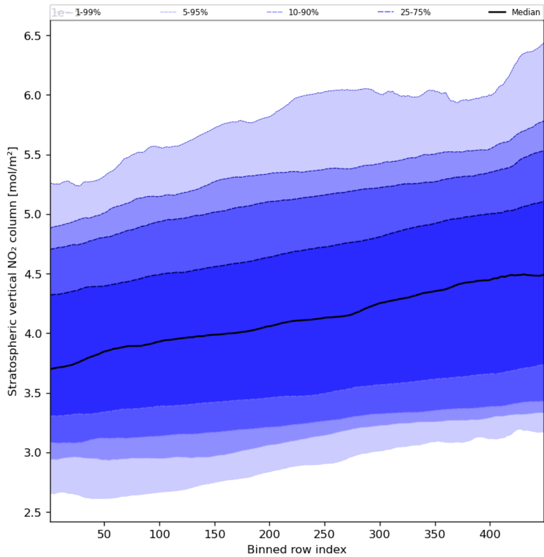
Figure 53: Along track statistics of “Stratospheric vertical NO 2 column” for 2024-03-28 to 2024-03-30
