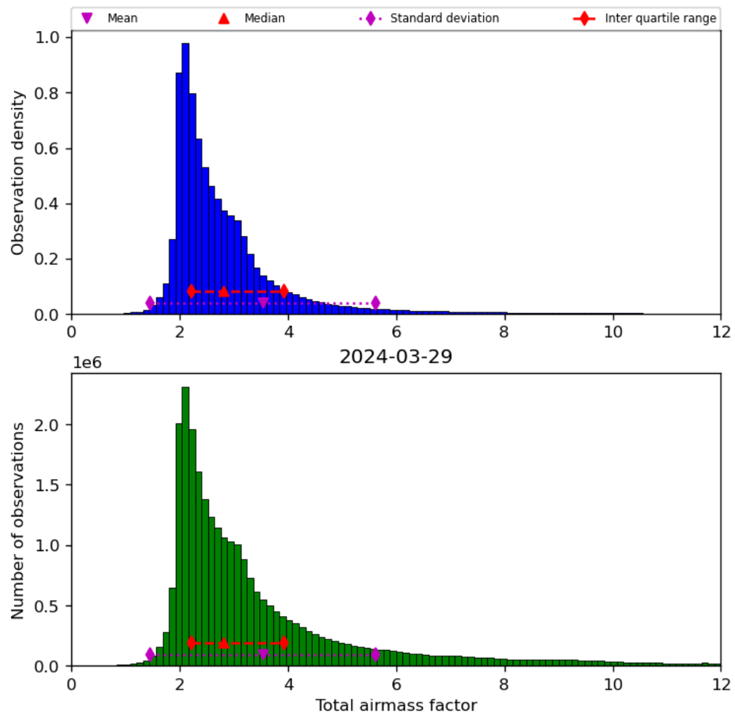
Figure 32: Histogram of “Total airmass factor” for 2024-03-28 to 2024-03-30
