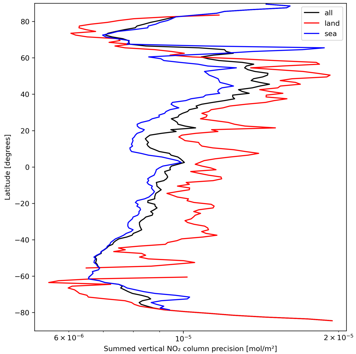
Figure 24: Zonal average of “Summed vertical NO 2 column precision” for 2024-03-28 to 2024-03-30.
