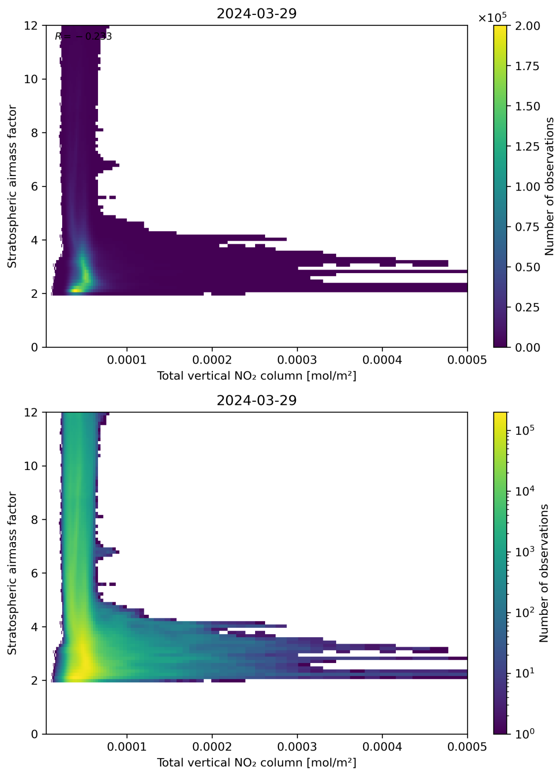
Figure 110: Scatter density plot of “Total vertical NO 2 column” against “Stratospheric airmass factor” for 2024-03-28 to 2024-03-30.
