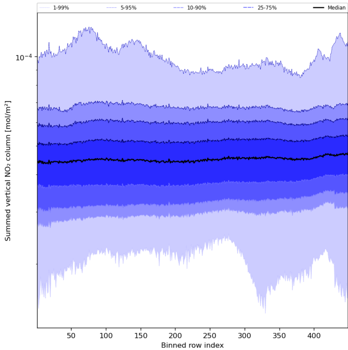
Figure 57: Along track statistics of “Summed vertical NO 2 column” for 2024-03-28 to 2024-03-30
