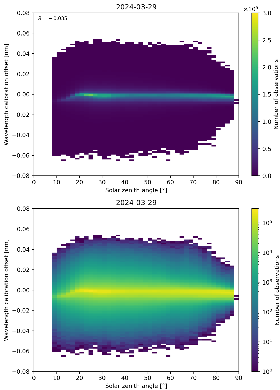
Figure 158: Scatter density plot of “Solar zenith angle” against “Wavelength calibration offset” for 2024-03-28 to 2024-03-30.
