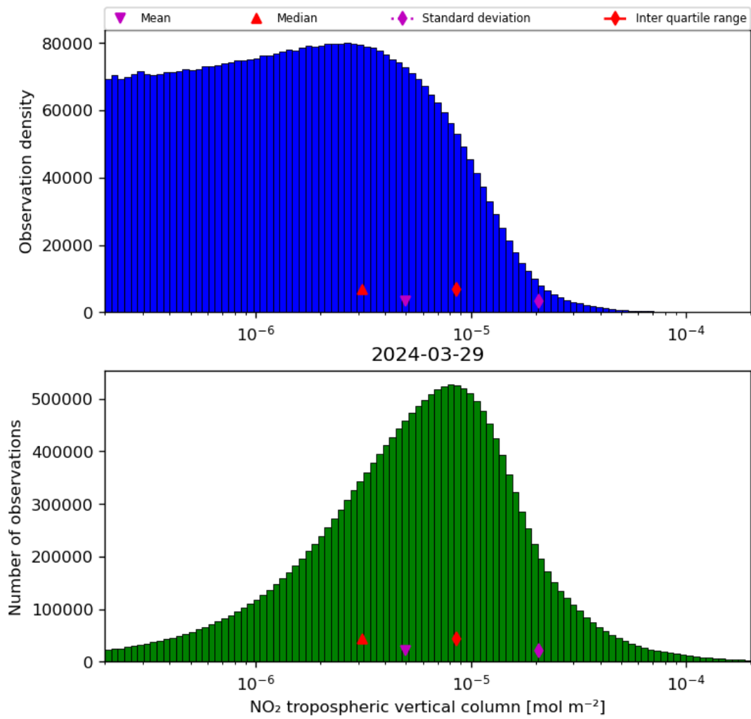
Figure 29: Histogram of “ \text{NO}_2 tropospheric vertical column” for 2024-03-28 to 2024-03-30
