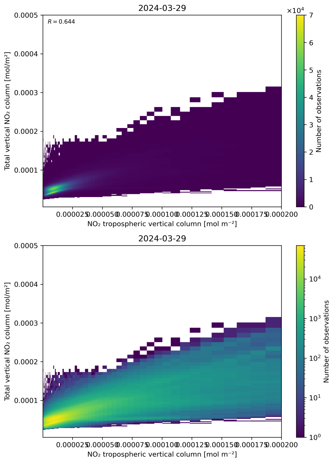
Figure 128: Scatter density plot of “NO 2 tropospheric vertical column” against “Total vertical NO 2 column” for 2024-03-28 to 2024-03-30.
