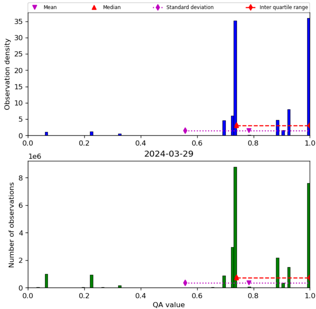
Figure 28: Histogram of “QA value” for 2024-03-28 to 2024-03-30
