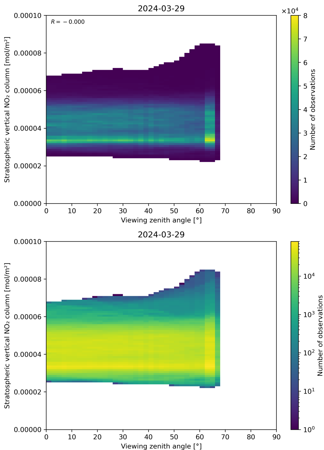
Figure 164: Scatter density plot of “Viewing zenith angle” against “Stratospheric vertical NO 2 column” for 2024-03-28 to 2024-03-30.
