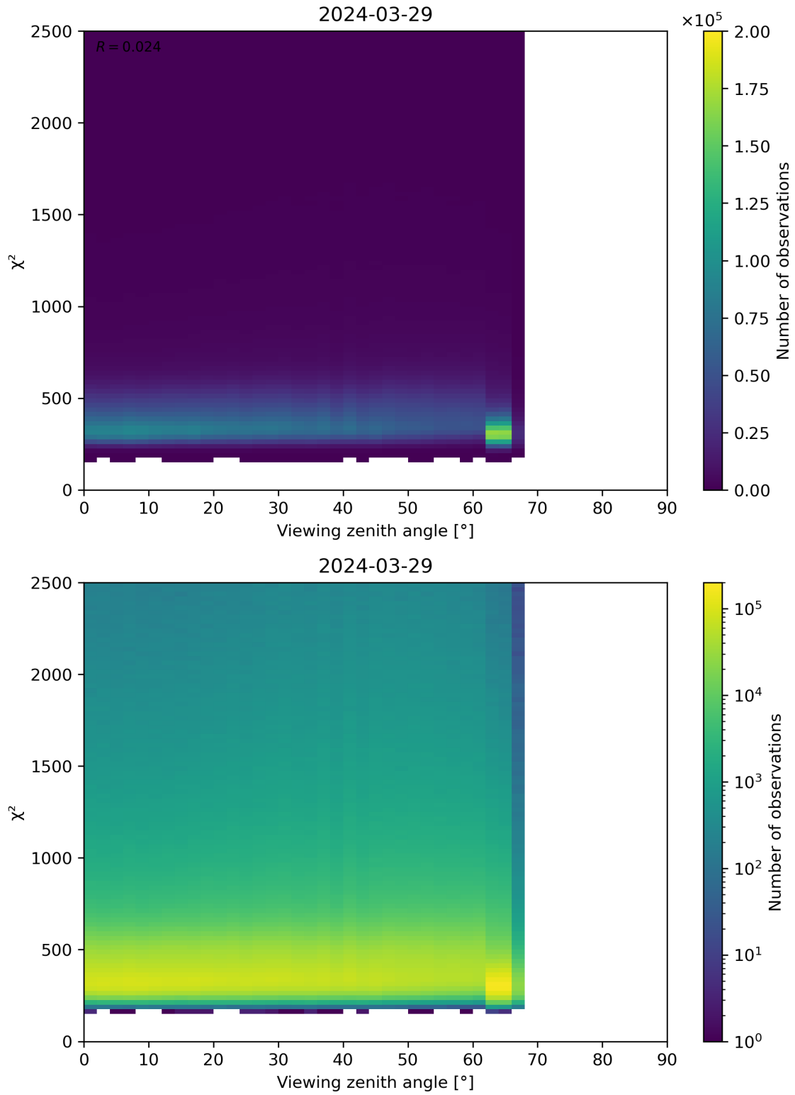
Figure 162: Scatter density plot of “Viewing zenith angle” against “ \chi^2 ” for 2024-03-28 to 2024-03-30.
