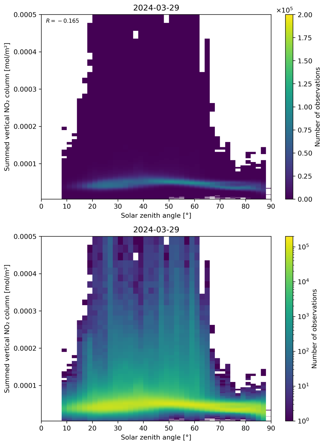
Figure 151: Scatter density plot of “Solar zenith angle” against “Summed vertical NO 2 column” for 2024-03-28 to 2024-03-30.
