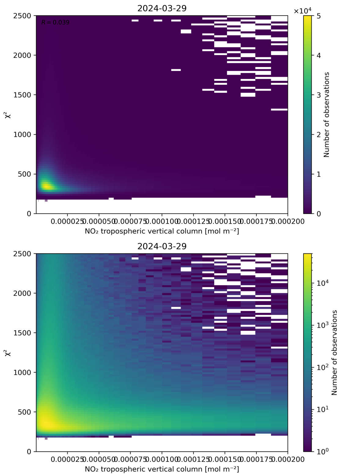
Figure 124: Scatter density plot of “NO 2 tropospheric vertical column” against “ \chi^2 ” for 2024-03-28 to 2024-03-30.
