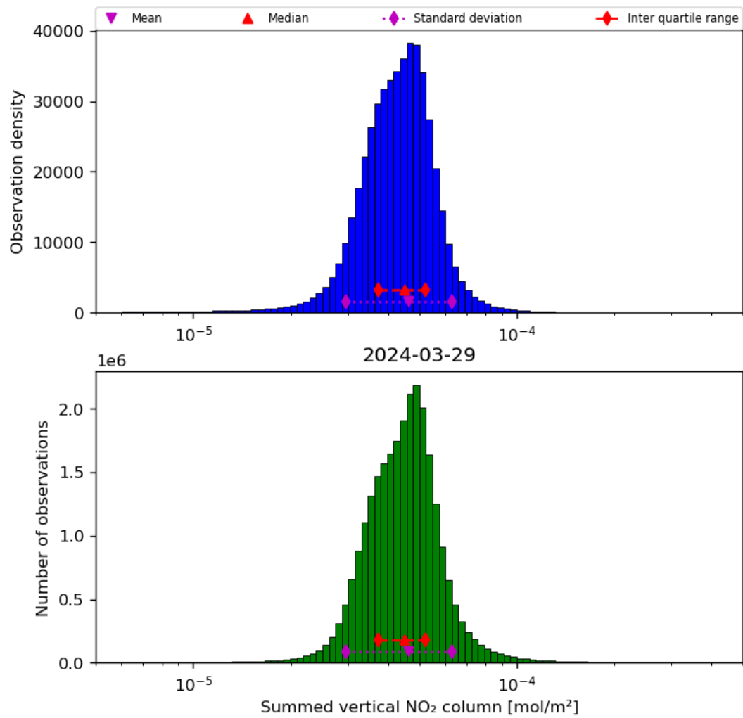
Figure 40: Histogram of “Summed vertical NO 2 column” for 2024-03-28 to 2024-03-30
