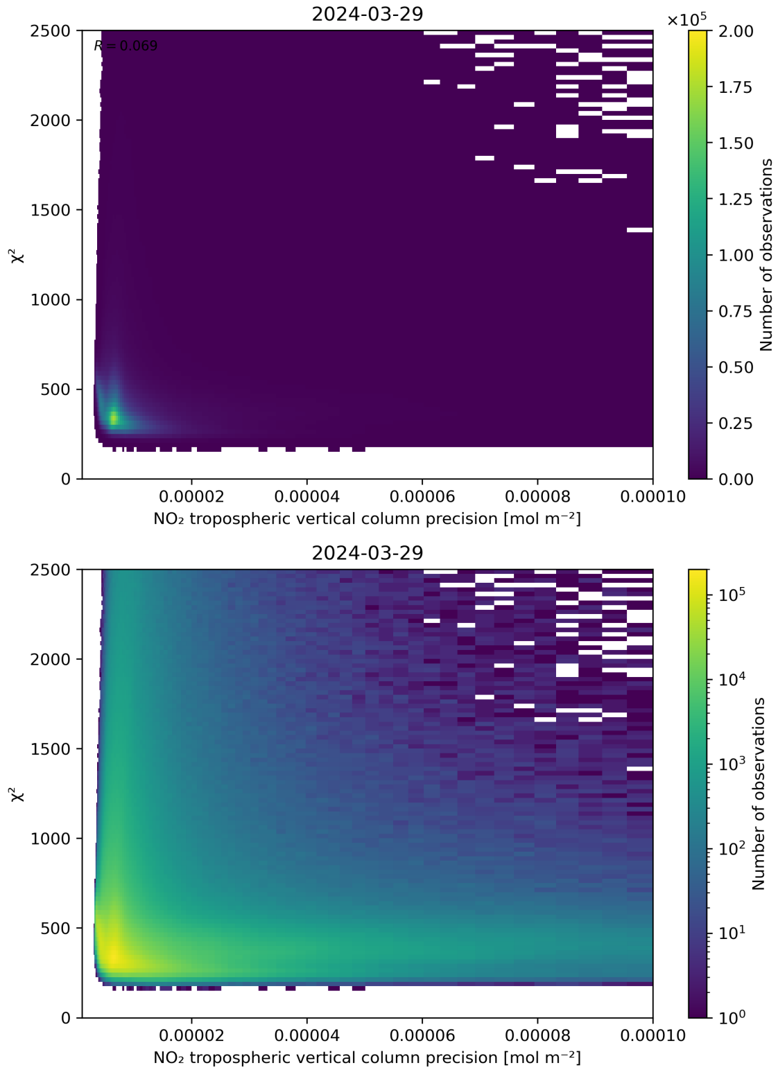
Figure 134: Scatter density plot of “NO 2 tropospheric vertical column precision” against “ \chi^2 ” for 2024-03-28 to 2024-03-30.
