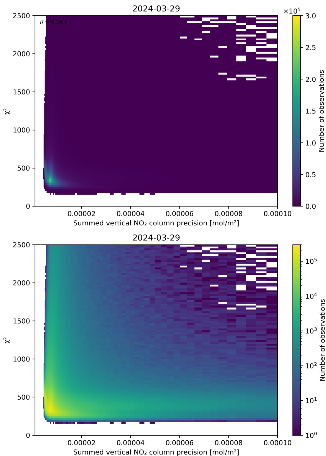
Figure 107: Scatter density plot of “Summed vertical NO 2 column precision” against “ \chi^2 ” for 2024-03-28 to 2024-03-30.
