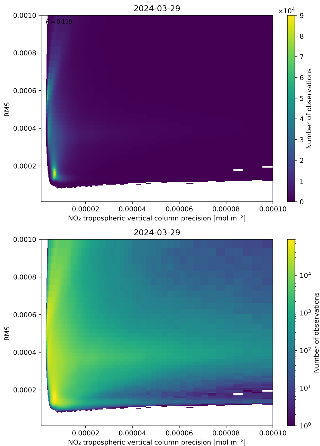
Figure 140: Scatter density plot of “NO 2 tropospheric vertical column precision” against “RMS” for 2024-03-28 to 2024-03-30.
