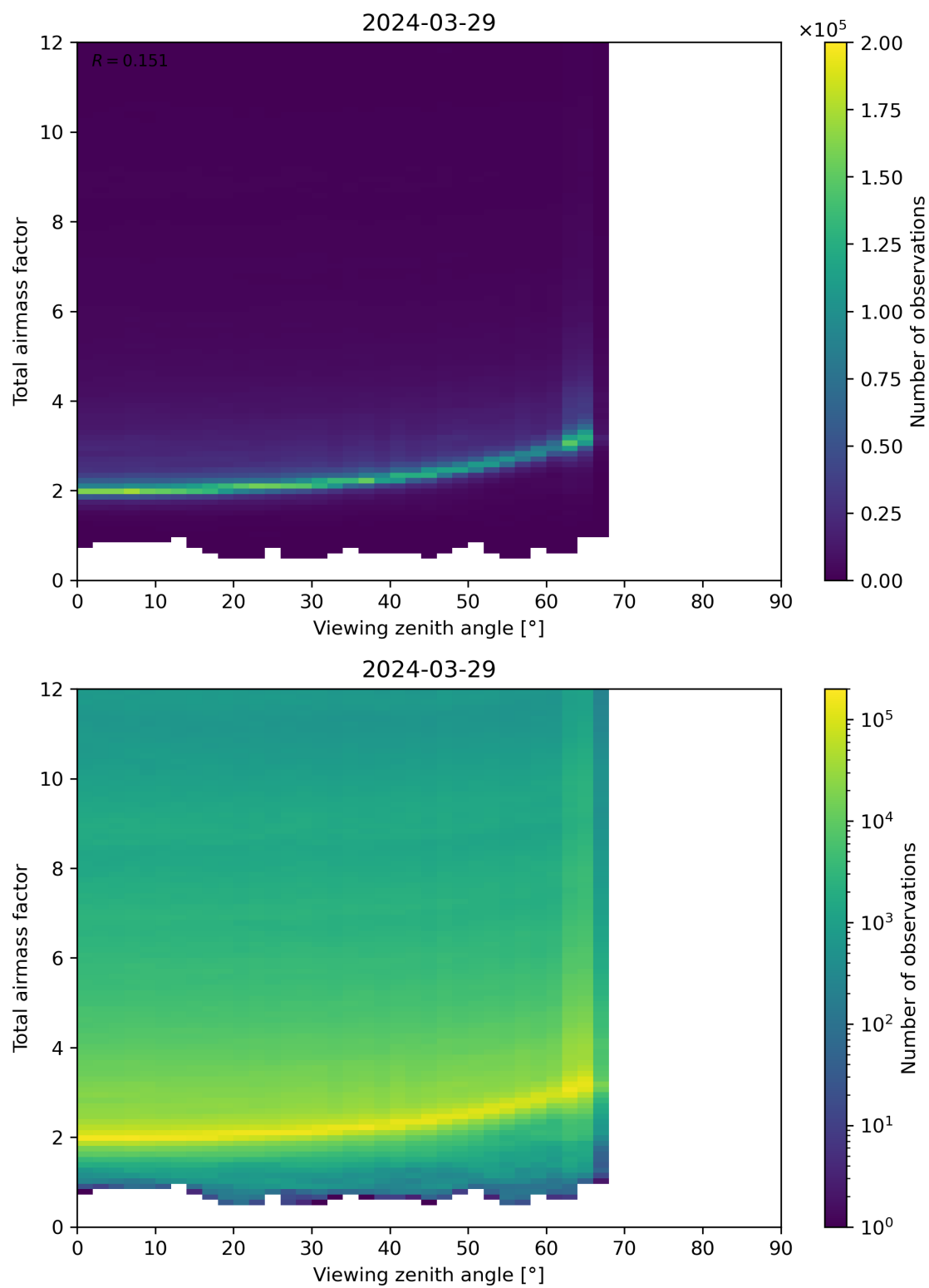
Figure 160: Scatter density plot of “Viewing zenith angle” against “Total airmass factor” for 2024-03-28 to 2024-03-30.
