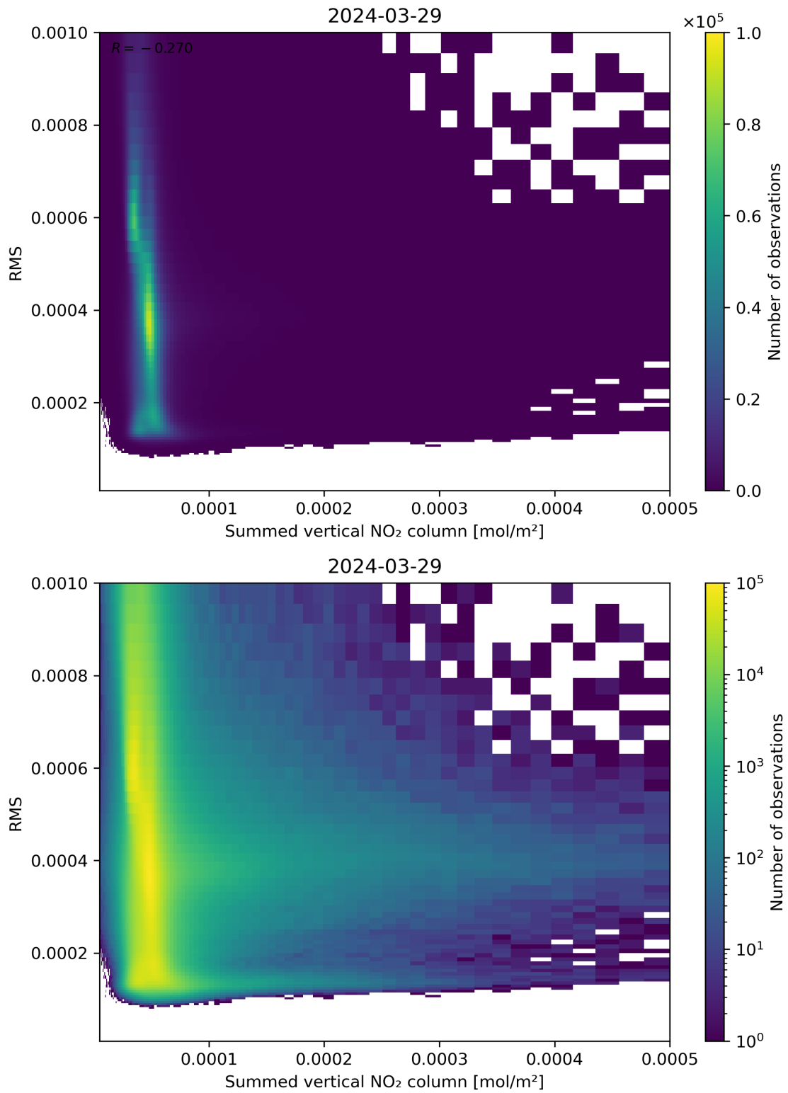
Figure 109: Scatter density plot of “Summed vertical NO 2 column” against “RMS” for 2024-03-28 to 2024-03-30.
