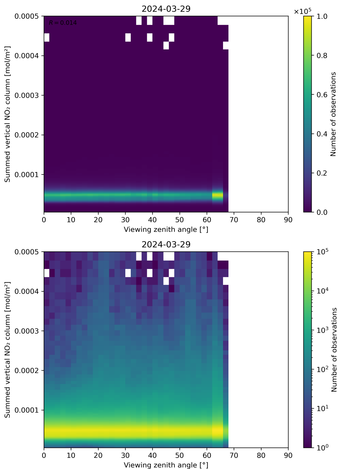
Figure 165: Scatter density plot of “Viewing zenith angle” against “Summed vertical NO 2 column” for 2024-03-28 to 2024-03-30.
