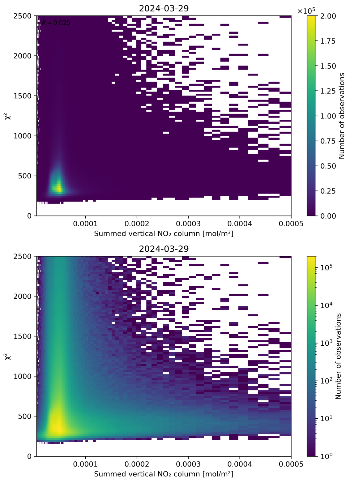
Figure 104: Scatter density plot of “Summed vertical NO 2 column” against “ \chi^2 ” for 2024-03-28 to 2024-03-30.
