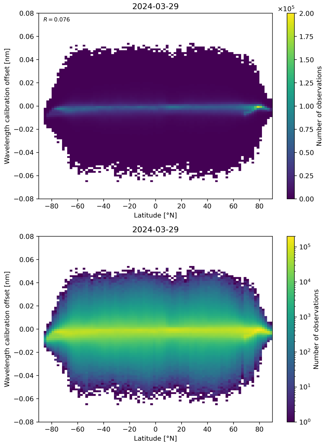
Figure 95: Scatter density plot of “Latitude” against “Wavelength calibration offset” for 2024-03-28 to 2024-03-30.
