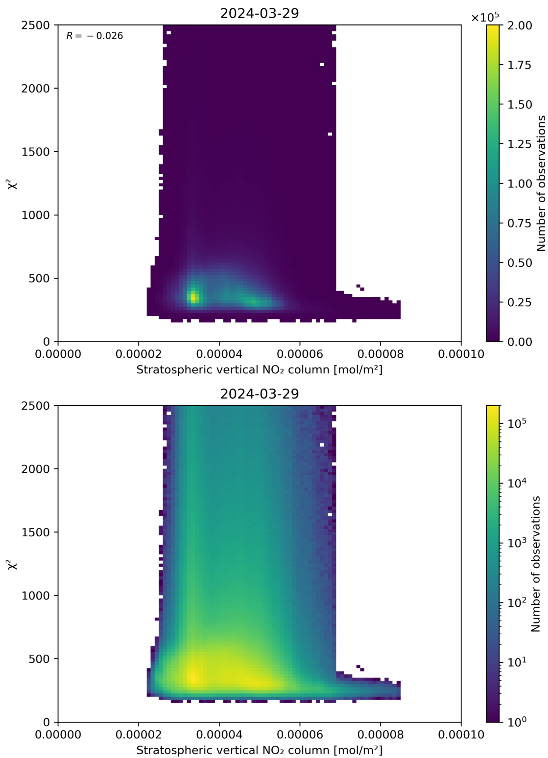
Figure 97: Scatter density plot of “Stratospheric vertical NO 2 column” against “ \chi^2 ” for 2024-03-28 to 2024-03-30.
