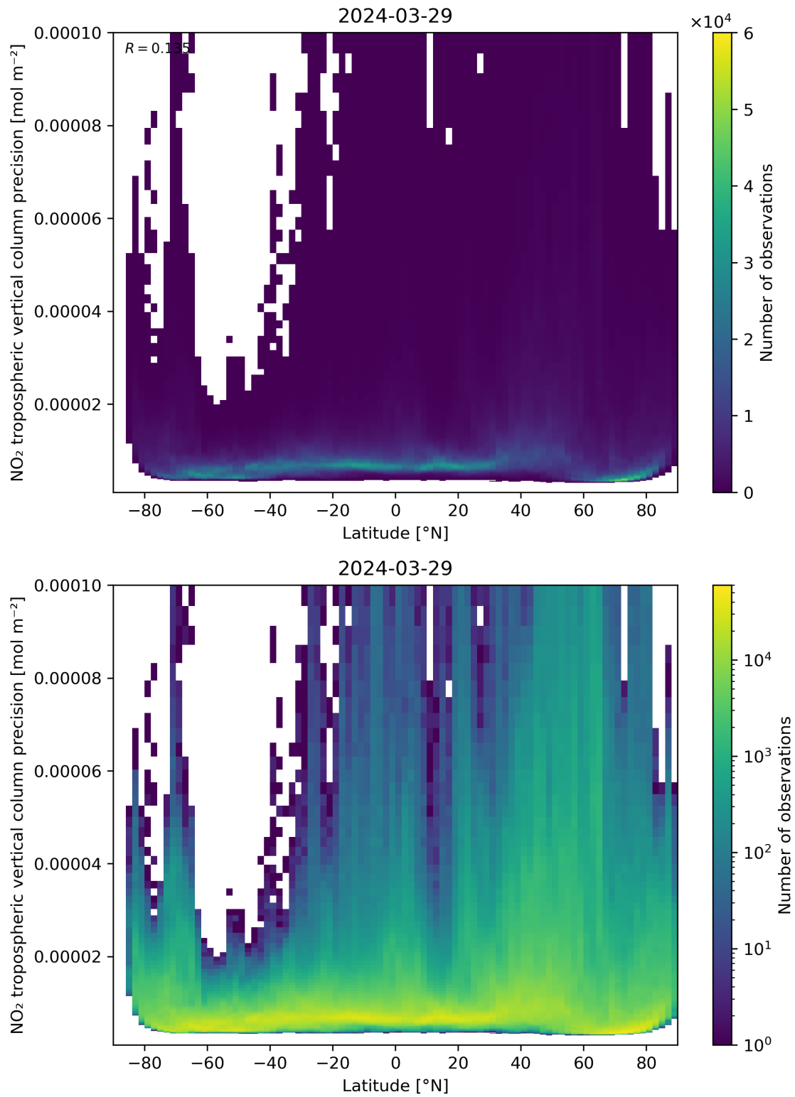
Figure 93: Scatter density plot of “Latitude” against “NO 2 tropospheric vertical column precision” for 2024-03-28 to 2024-03-30.
