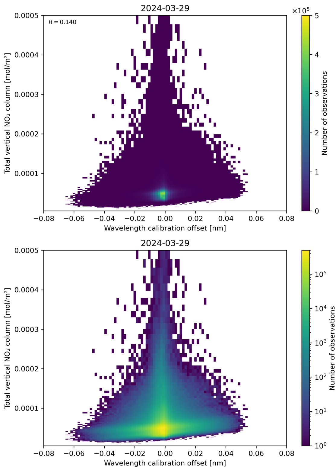
Figure 179: Scatter density plot of “Wavelength calibration offset” against “Total vertical NO 2 column” for 2024-03-28 to 2024-03-30.
