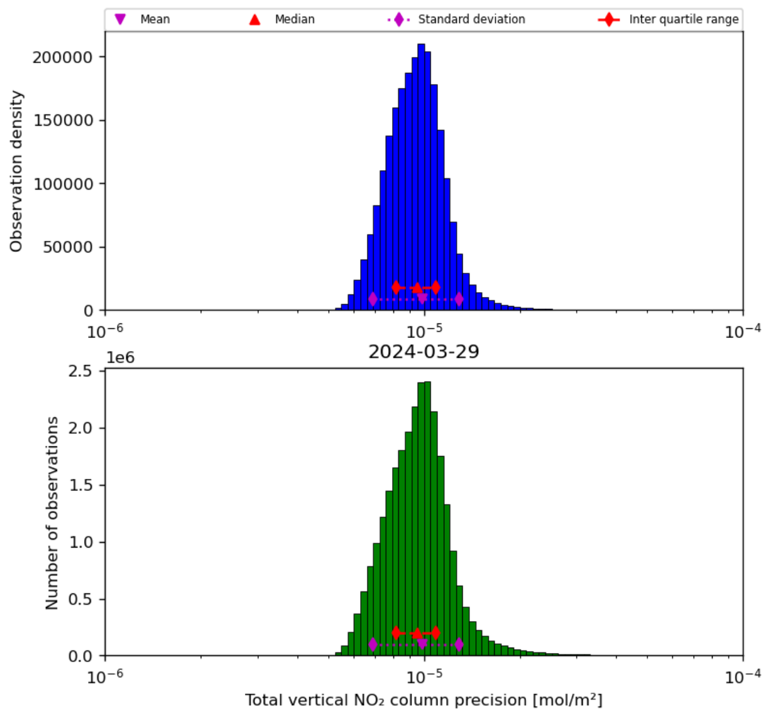
Figure 39: Histogram of "Total vertical NO 2 column precision" for 2024-03-28 to 2024-03-30
