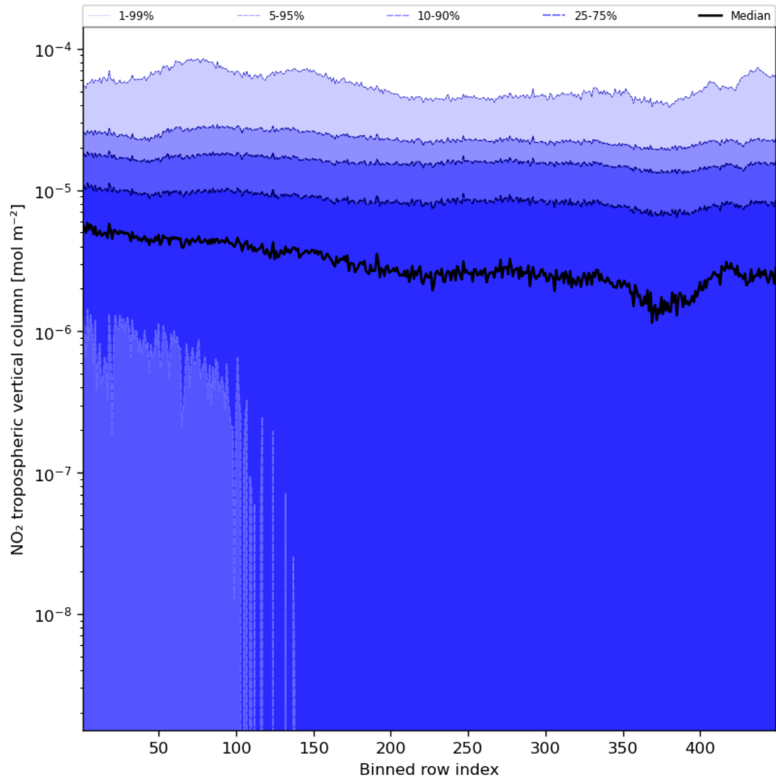
Figure 46: Along track statistics of “NO 2 tropospheric vertical column” for 2024-03-28 to 2024-03-30
