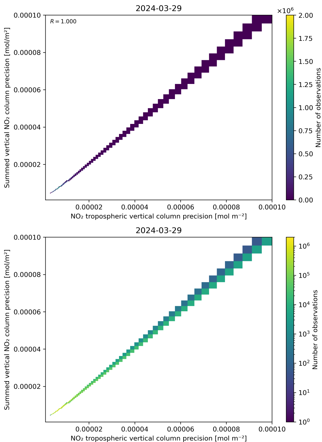
Figure 137: Scatter density plot of “NO 2 tropospheric vertical column precision” against “Summed vertical NO 2 column precision” for 2024-03-28 to 2024-03-30.
