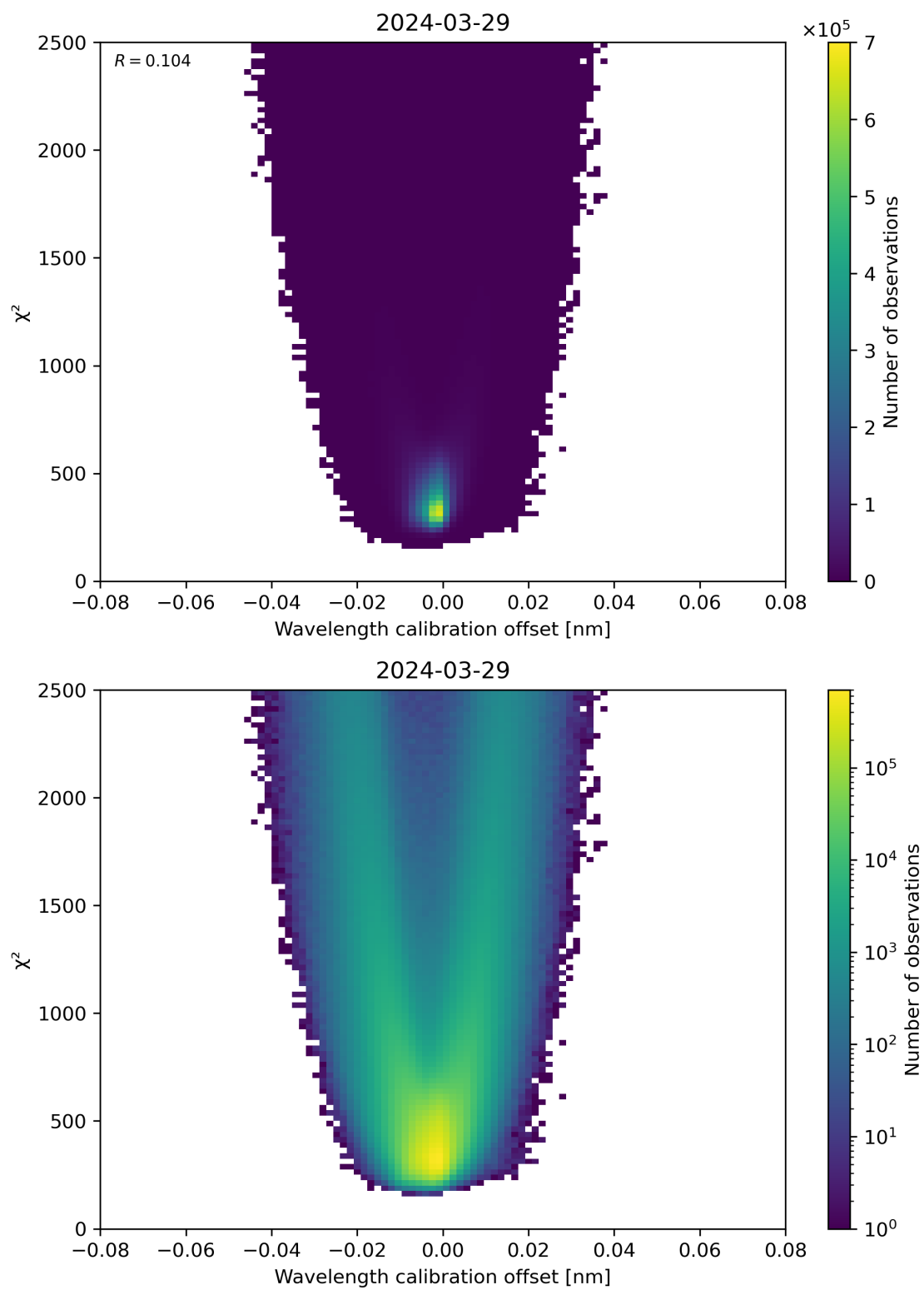
Figure 175: Scatter density plot of “Wavelength calibration offset” against “ \chi^2 ” for 2024-03-28 to 2024-03-30.
