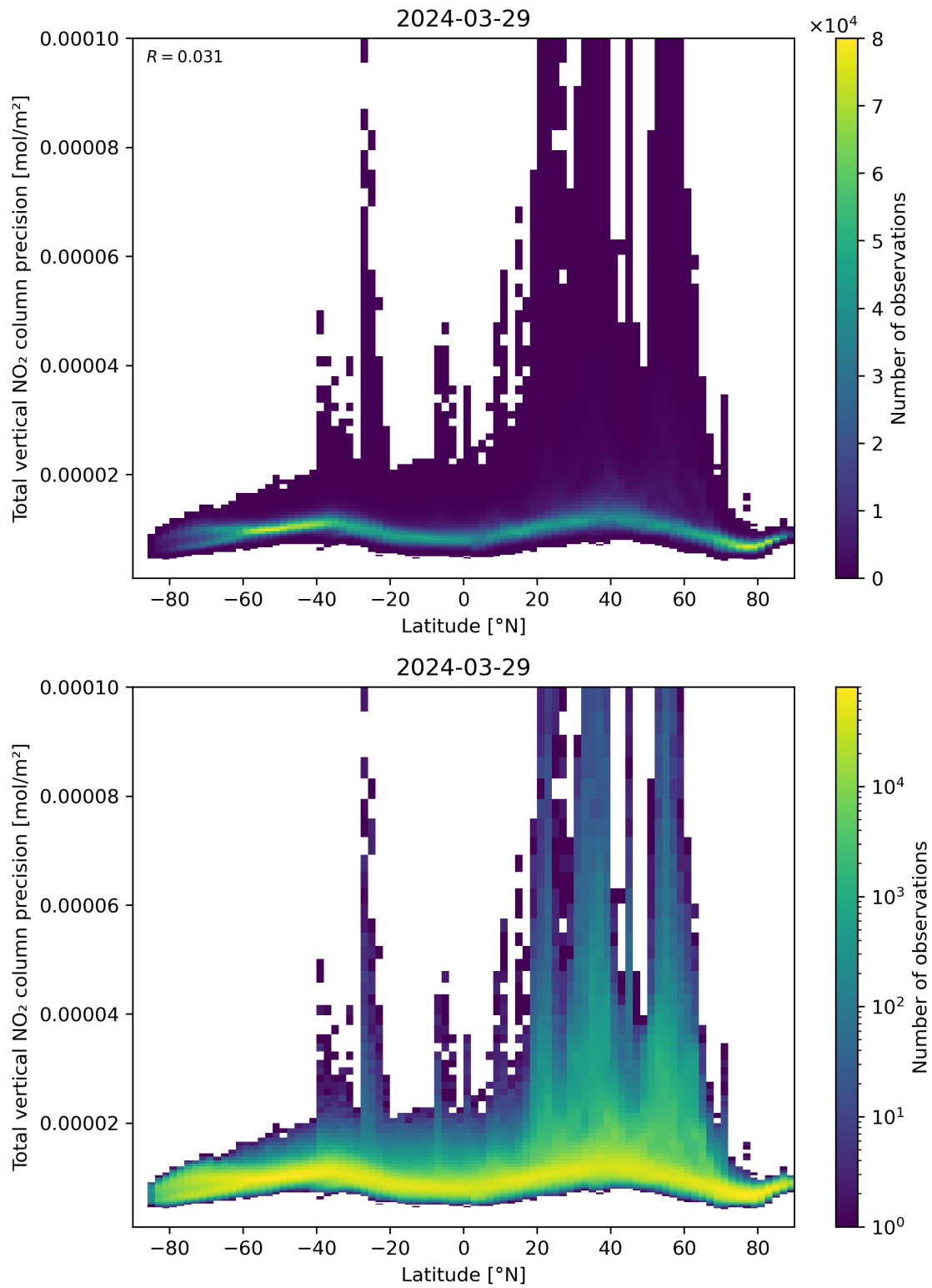
Figure 91: Scatter density plot of “Latitude” against “Total vertical NO 2 column precision” for 2024-03-28 to 2024-03-30.
