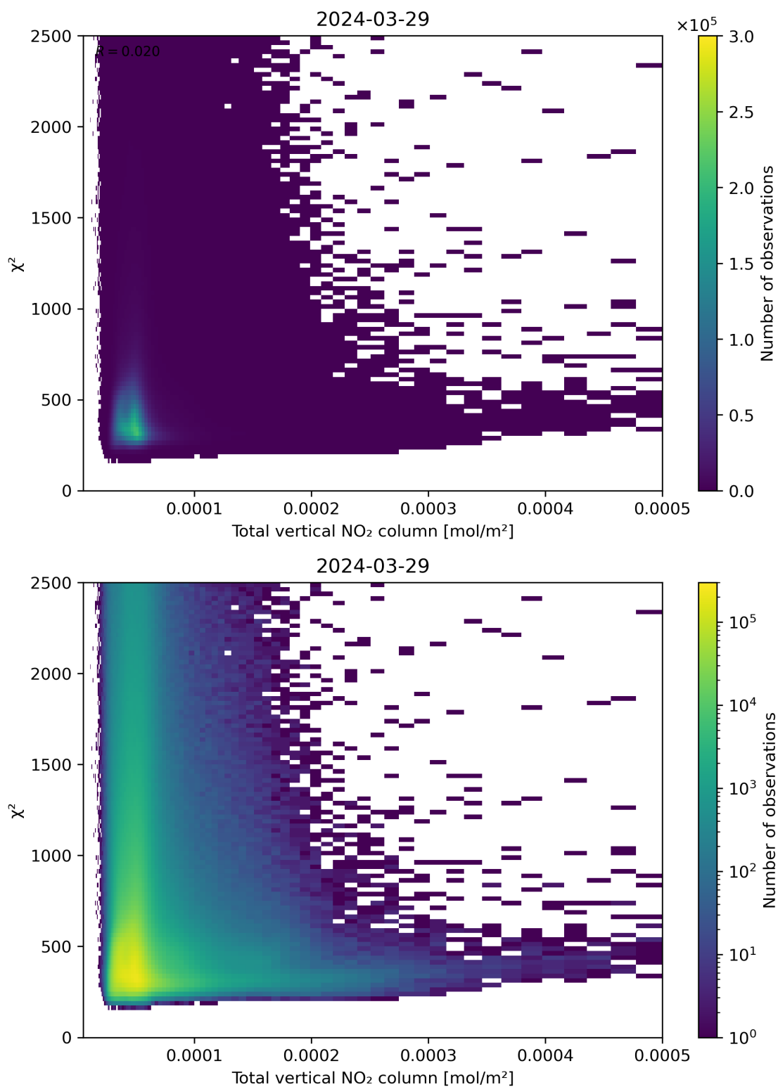
Figure 111: Scatter density plot of “Total vertical NO 2 column” against “ \chi^2 ” for 2024-03-28 to 2024-03-30.
