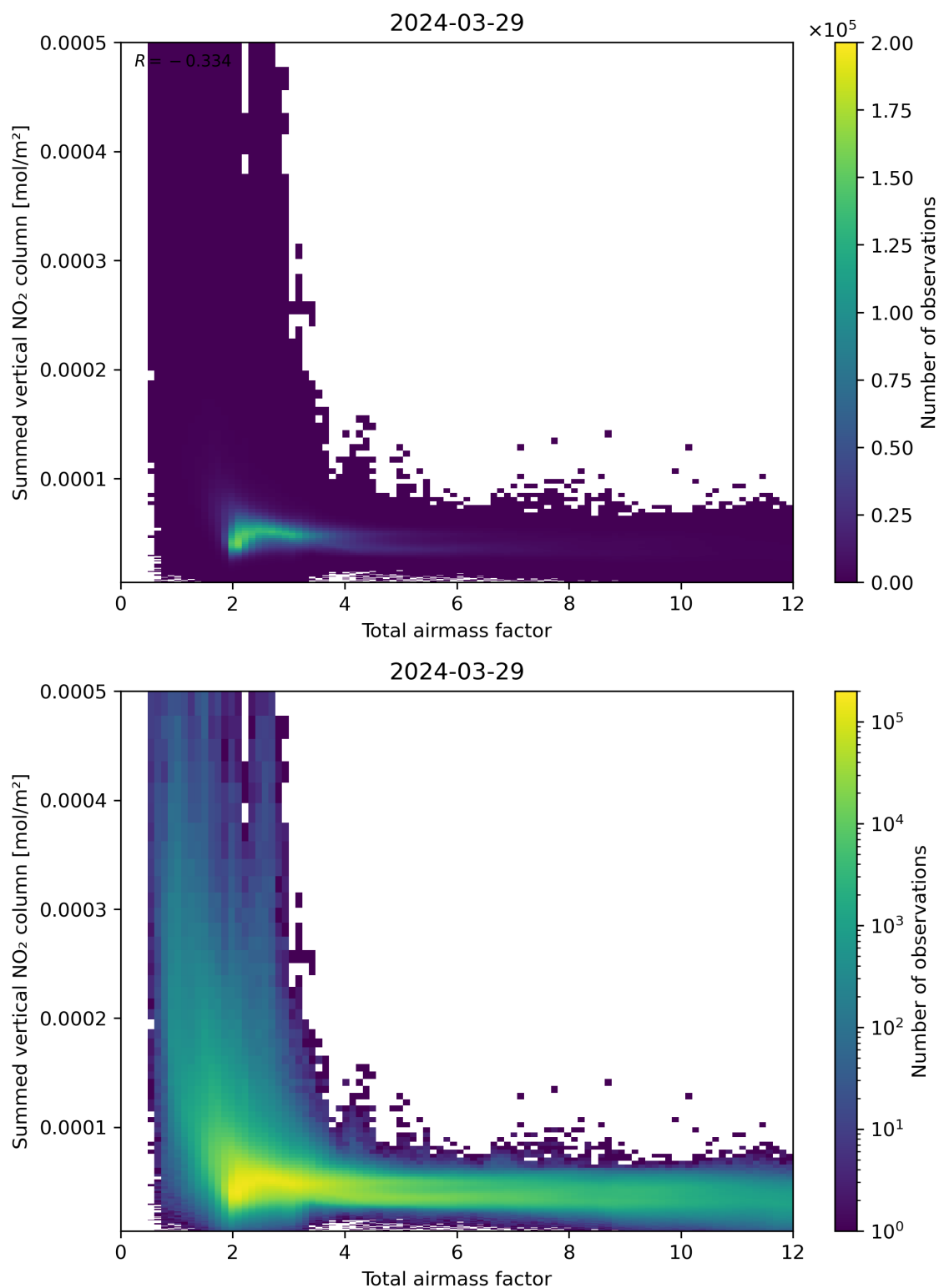
Figure 65: Scatter density plot of “Total airmass factor” against “Summed vertical NO 2 column” for 2024-03-28 to 2024-03-30.
