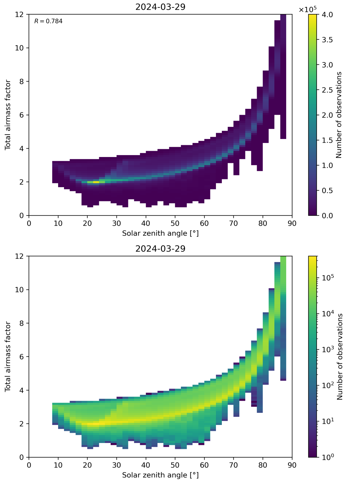
Figure 146: Scatter density plot of “Solar zenith angle” against “Total air mass factor” for 2024-03-28 to 2024-03-30.
