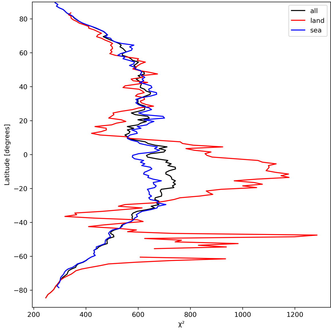
Figure 25: Zonal average of “ \chi^2 ” for 2024-03-28 to 2024-03-30.
