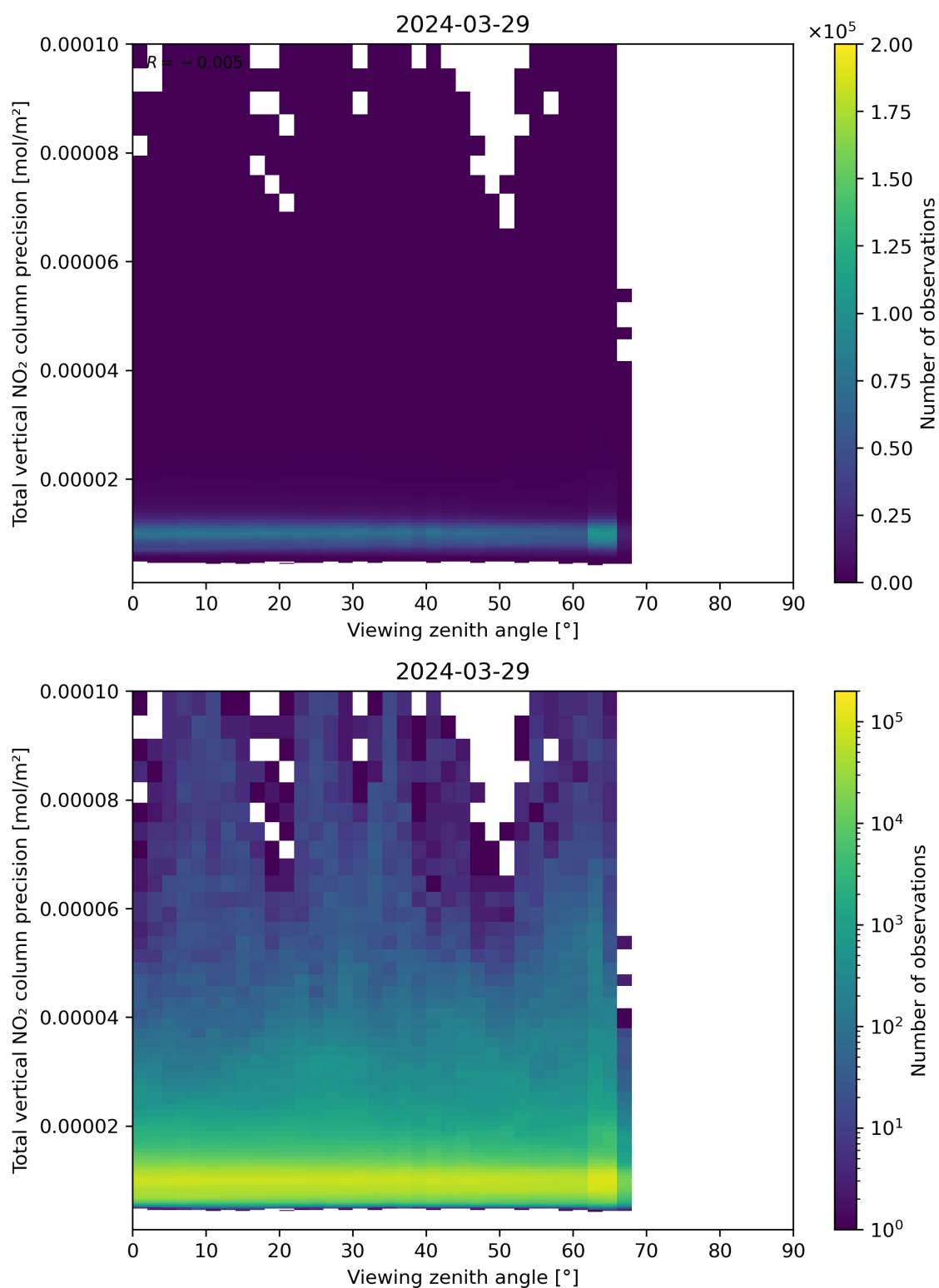
Figure 168: Scatter density plot of “Viewing zenith angle” against “Total vertical NO 2 column precision” for 2024-03-28 to 2024-03-30.
