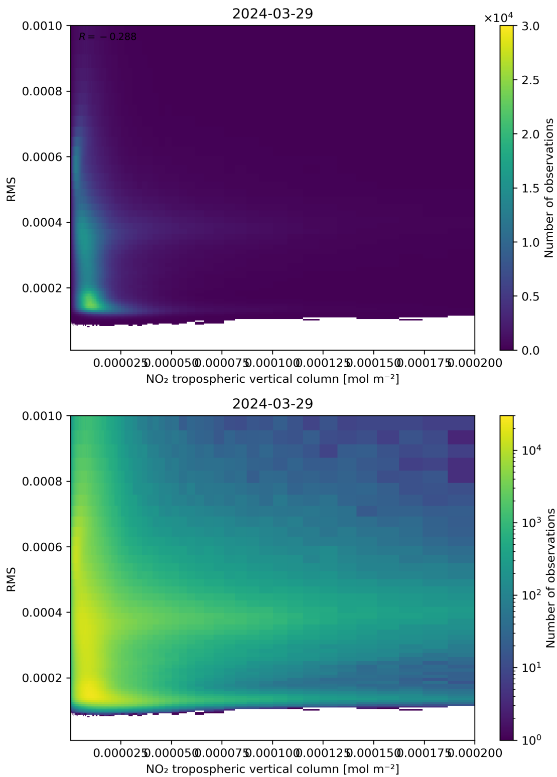
Figure 142: Scatter density plot of “NO 2 tropospheric vertical column” against “RMS” for 2024-03-28 to 2024-03-30.
