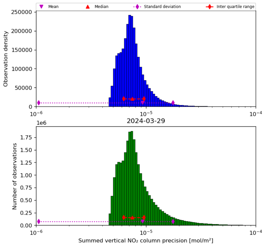
Figure 41: Histogram of “Summed vertical NO 2 column precision” for 2024-03-28 to 2024-03-30
