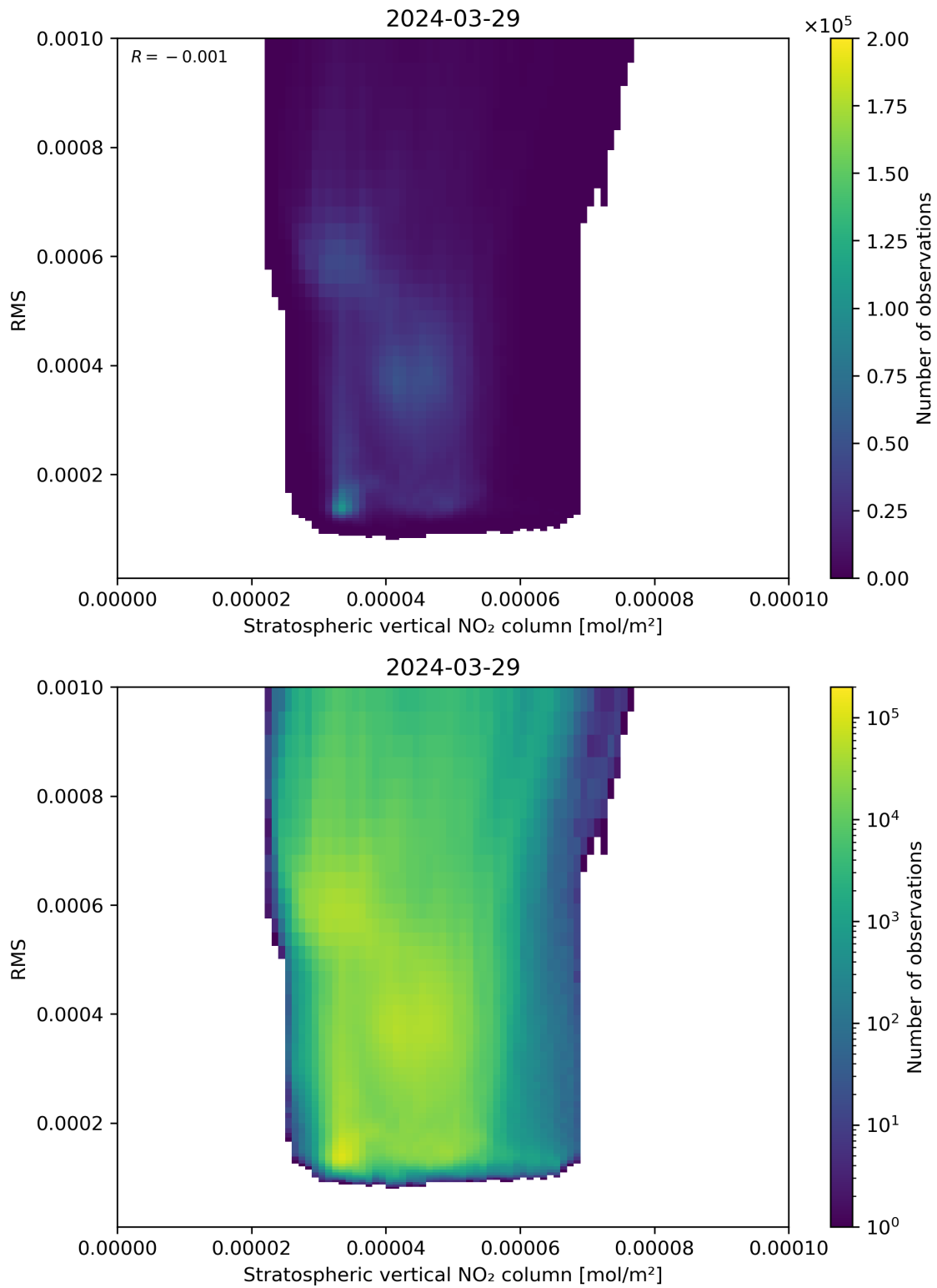
Figure 102: Scatter density plot of “Stratospheric vertical NO 2 column” against “RMS” for 2024-03-28 to 2024-03-30.
