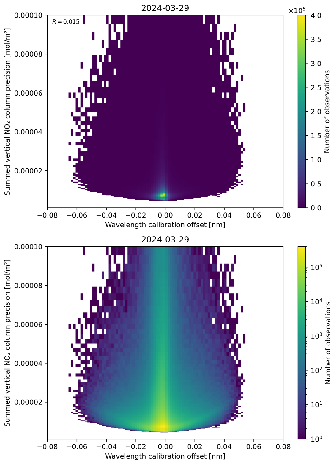
Figure 178: Scatter density plot of “Wavelength calibration offset” against “Summed vertical NO 2 column precision” for 2024-03-28 to 2024-03-30.
