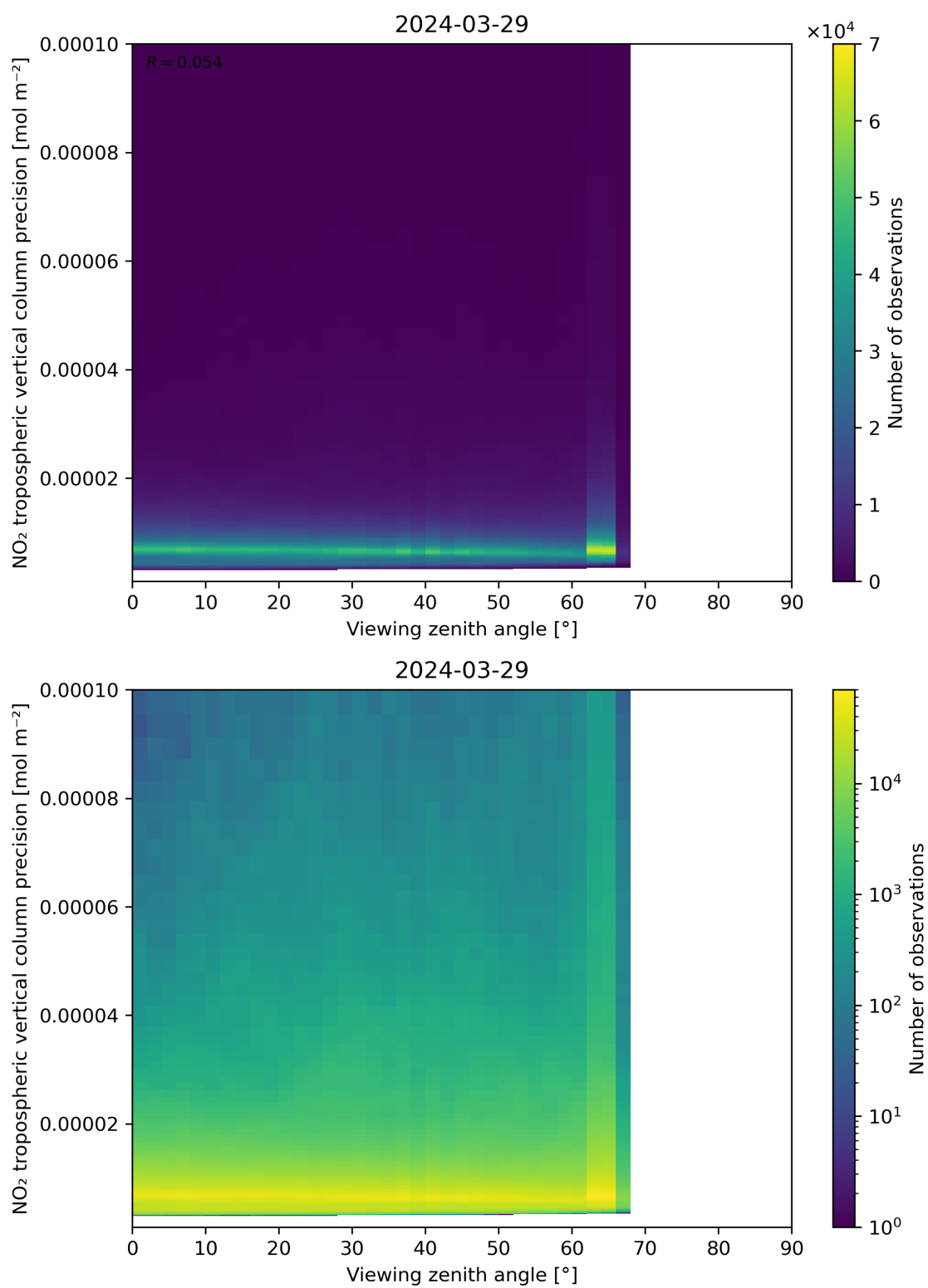
Figure 170: Scatter density plot of “Viewing zenith angle” against “NO 2 tropospheric vertical column precision” for 2024-03-28 to 2024-03-30.
