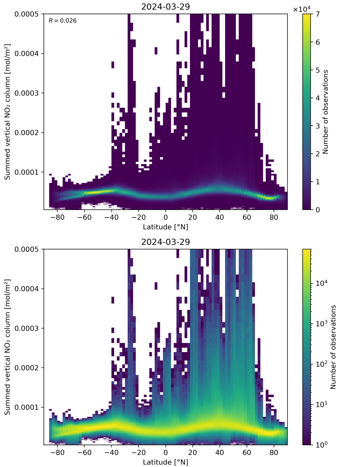
Figure 88: Scatter density plot of “Latitude” against “Summed vertical NO 2 column” for 2024-03-28 to 2024-03-30.
