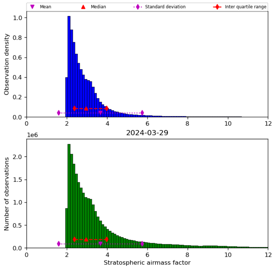
Figure 44: Histogram of “Stratospheric airmass factor” for 2024-03-28 to 2024-03-30
