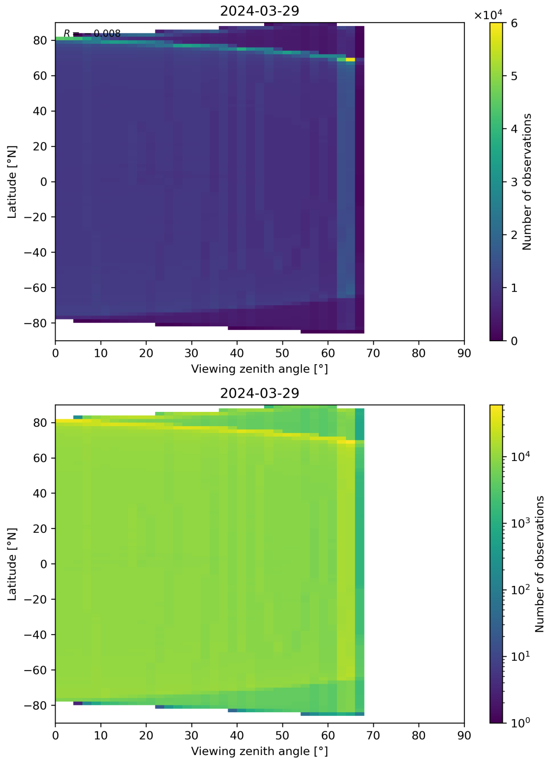
Figure 163: Scatter density plot of “Viewing zenith angle” against “Latitude” for 2024-03-28 to 2024-03-30.
