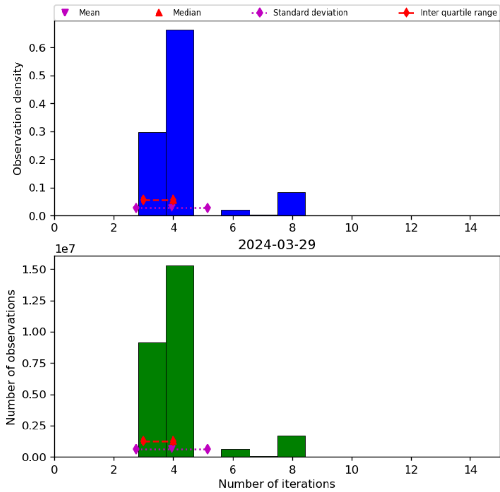
Figure 34: Histogram of “Number of iterations” for 2024-03-28 to 2024-03-30
