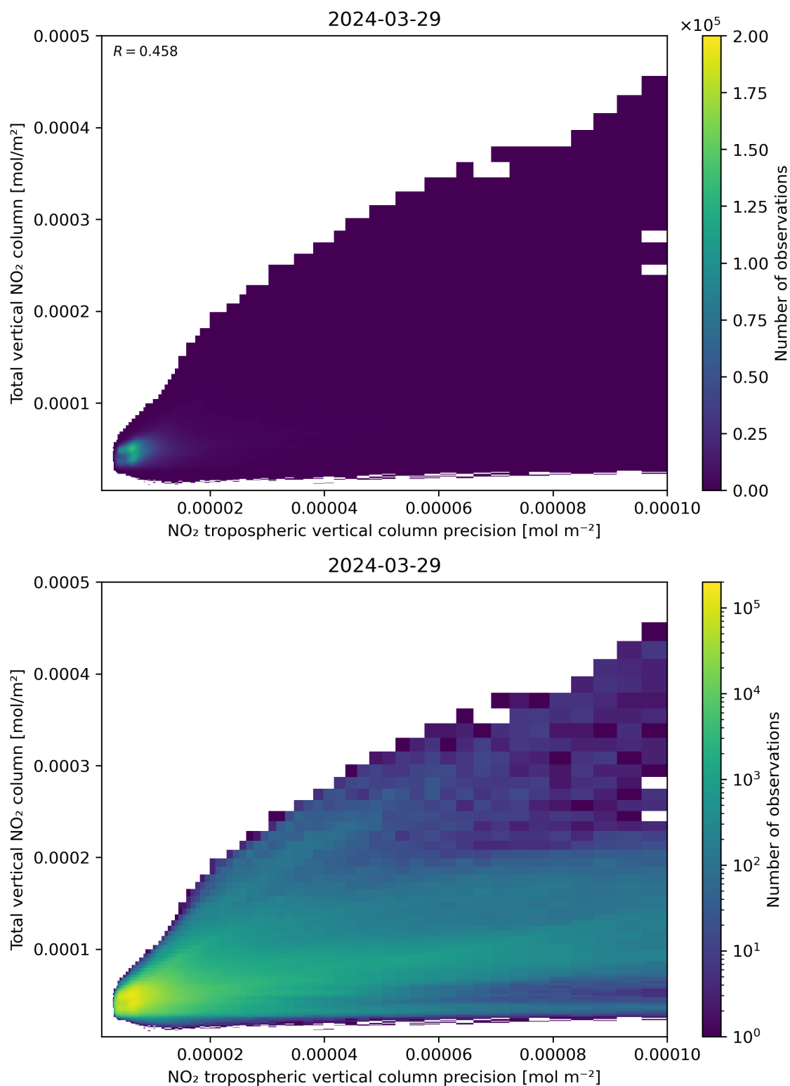
Figure 138: Scatter density plot of “NO 2 tropospheric vertical column precision” against “Total vertical NO 2 column” for 2024-03-28 to 2024-03-30.
