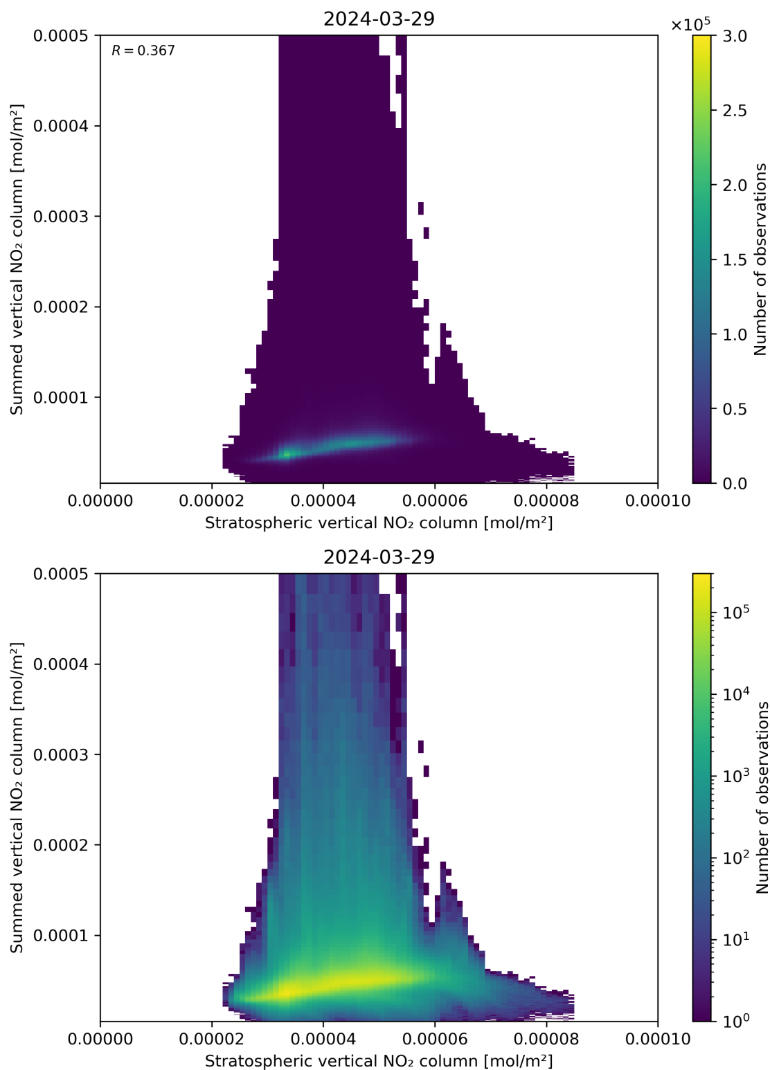
Figure 98: Scatter density plot of “Stratospheric vertical NO 2 column” against “Summed vertical NO 2 column” for 2024-03-28 to 2024-03-30.
