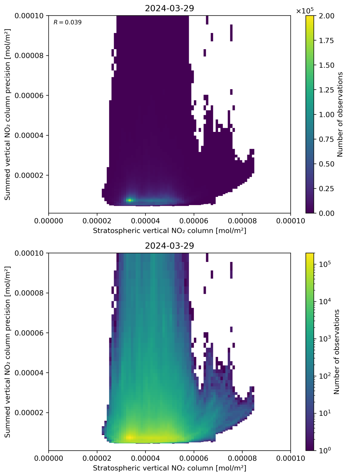
Figure 99: Scatter density plot of “Stratospheric vertical NO 2 column” against “Summed vertical NO 2 column precision” for 2024-03-28 to 2024-03-30.
