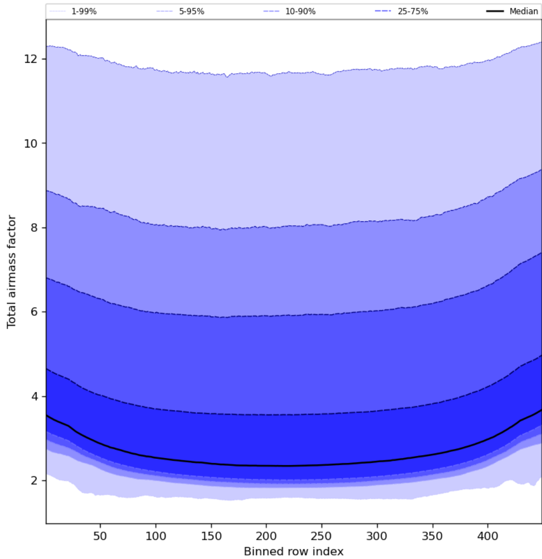
Figure 49: Along track statistics of “Total airmass factor” for 2024-03-28 to 2024-03-30
