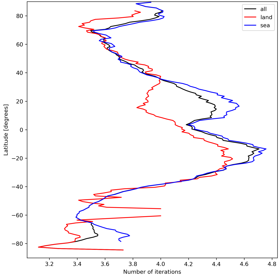
Figure 17: Zonal average of “Number of iterations” for 2024-03-28 to 2024-03-30.
