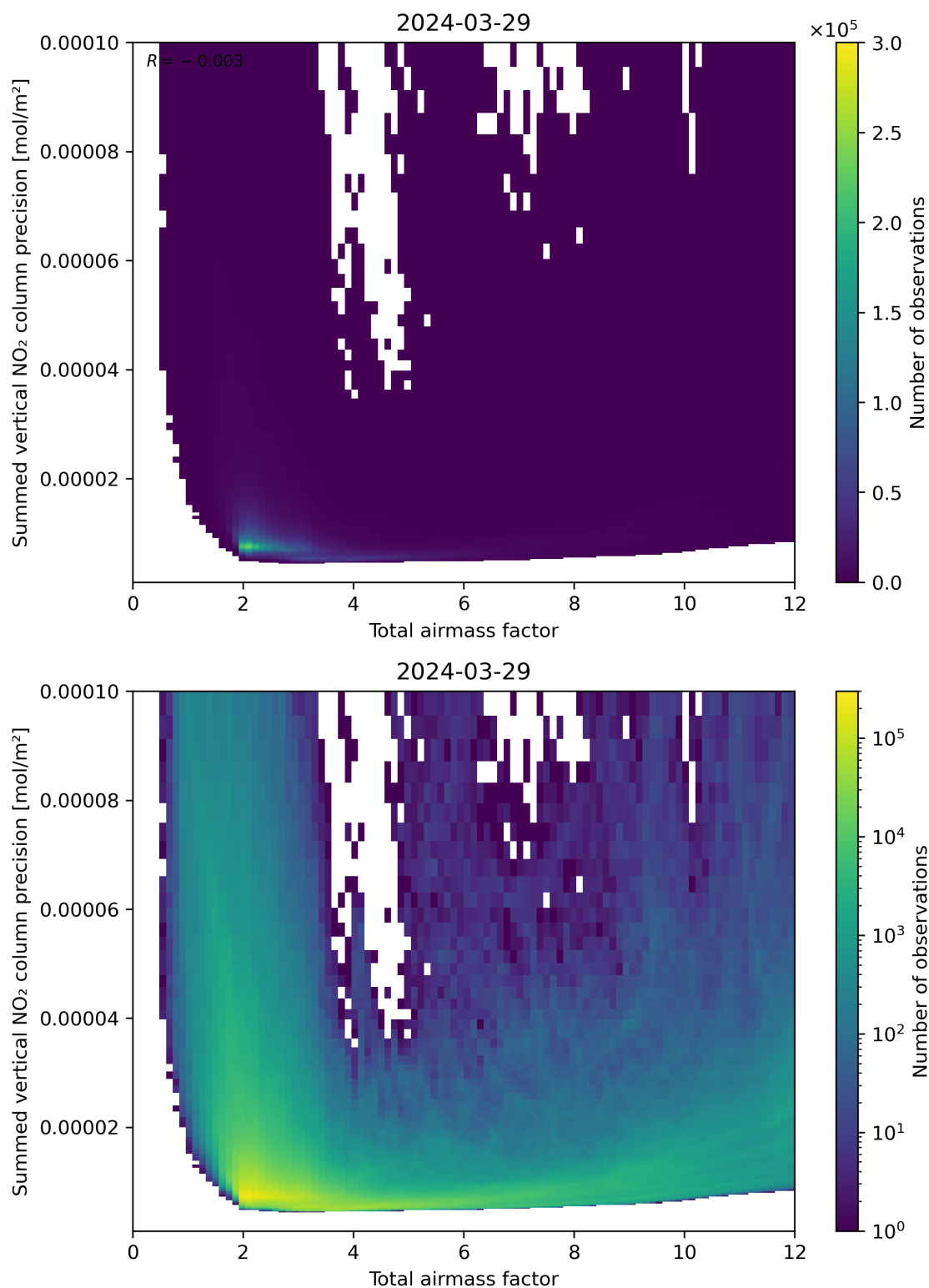
Figure 66: Scatter density plot of “Total airmass factor” against “Summed vertical NO 2 column precision” for 2024-03-28 to 2024-03-30.
