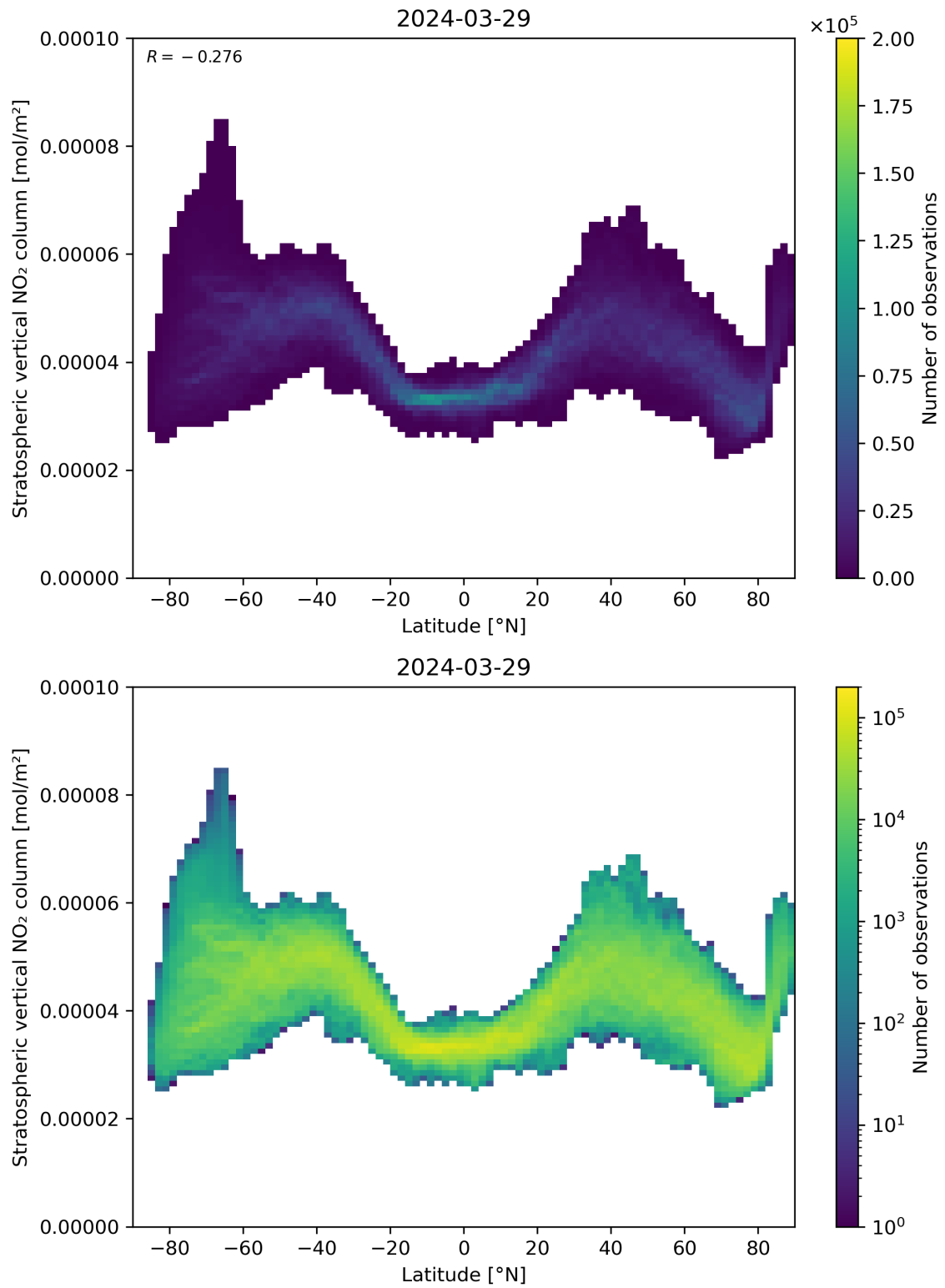
Figure 87: Scatter density plot of “Latitude” against “Stratospheric vertical NO 2 column” for 2024-03-28 to 2024-03-30.
