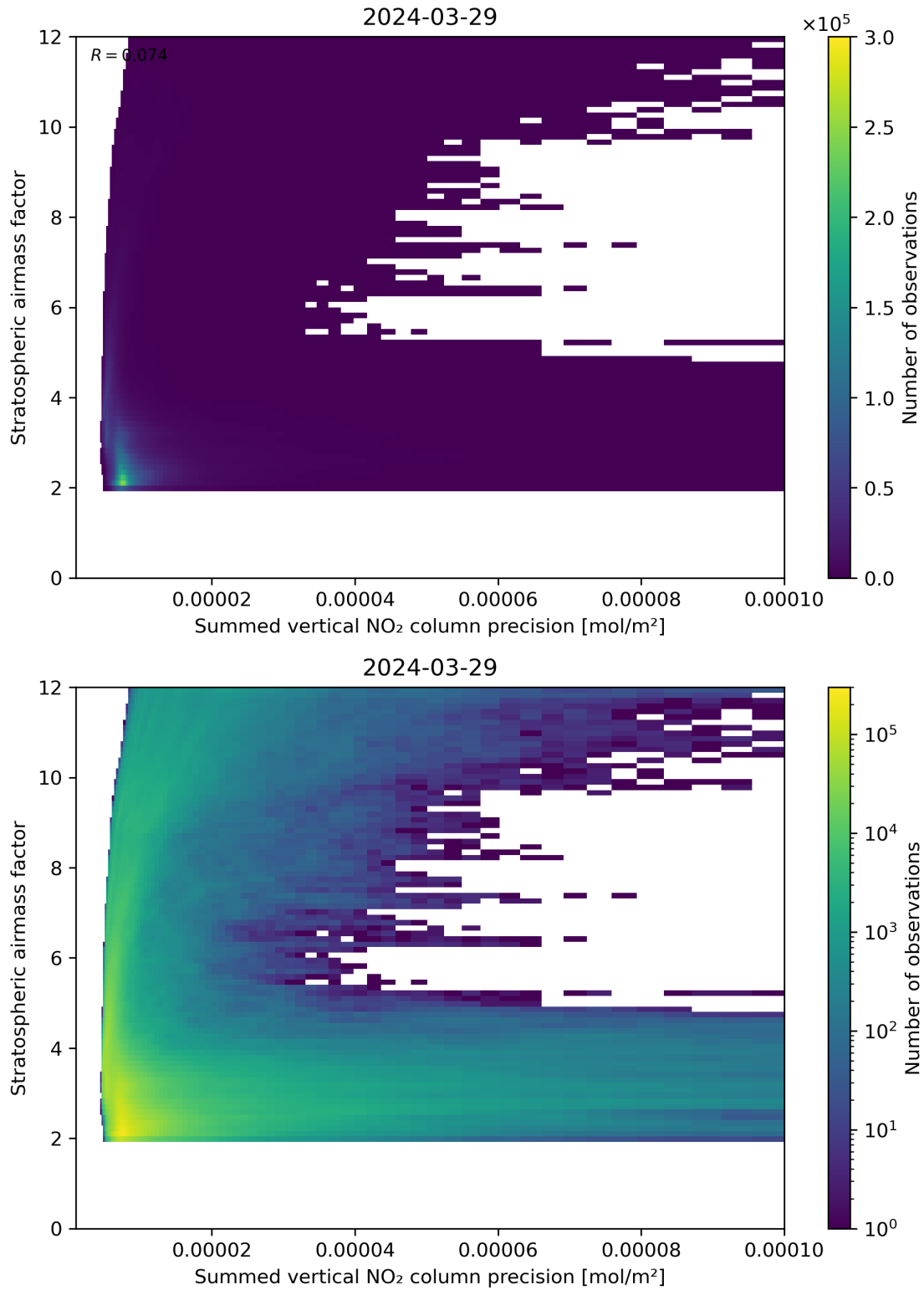
Figure 106: Scatter density plot of “Summed vertical NO 2 column precision” against “Stratospheric airmass factor” for 2024-03-28 to 2024-03-30.
