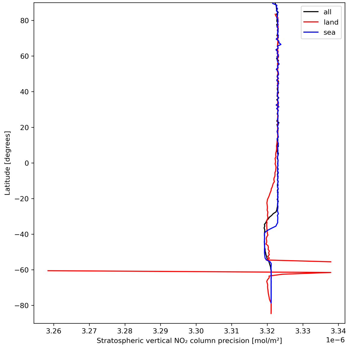
Figure 20: Zonal average of “Stratospheric vertical NO 2 column precision” for 2024-03-28 to 2024-03-30.
