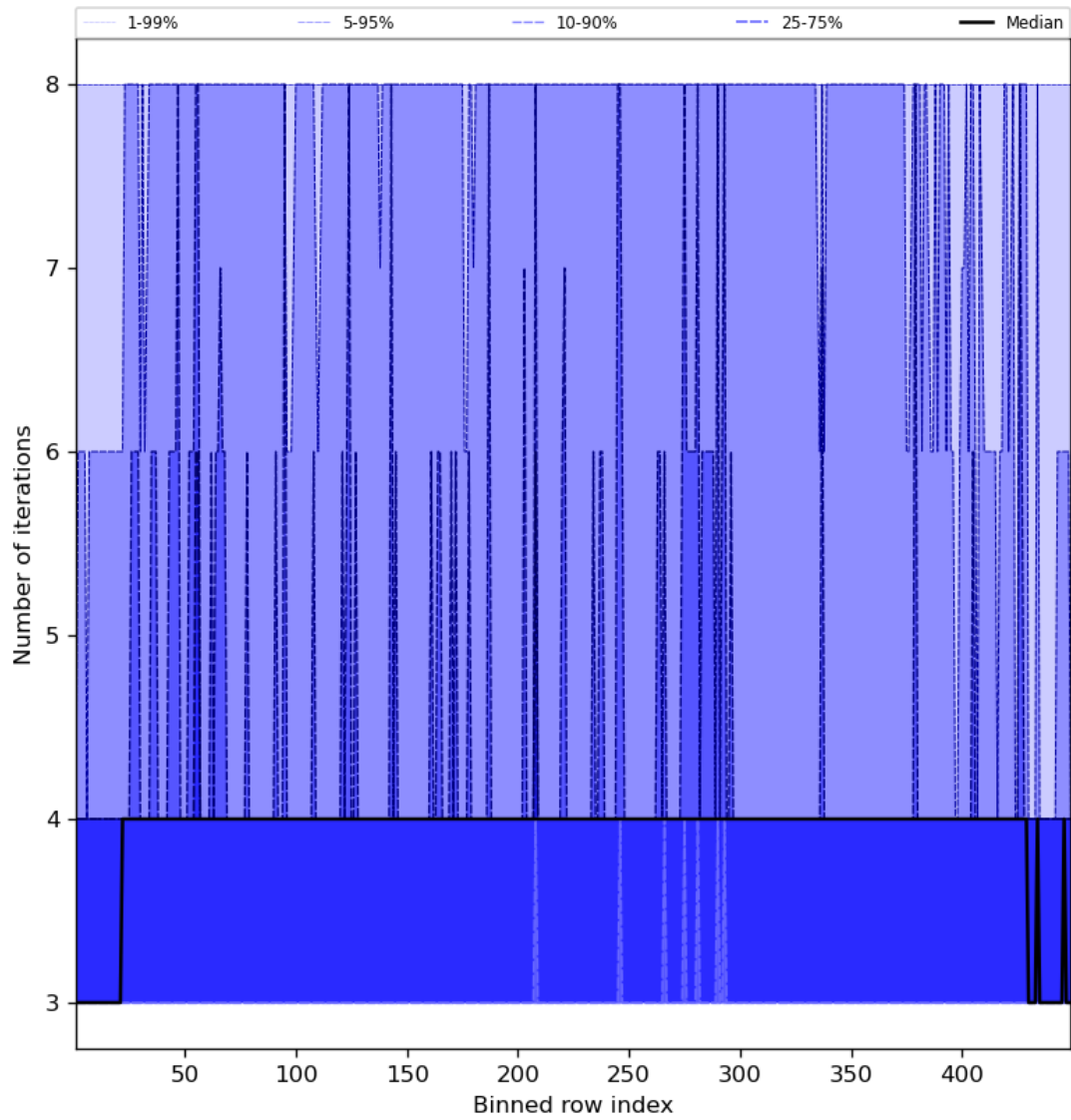
Figure 51: Along track statistics of “Number of iterations” for 2024-03-28 to 2024-03-30
