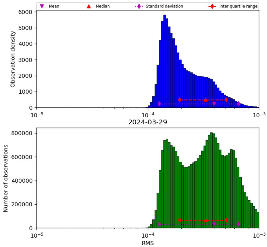
Figure 43: Histogram of “RMS” for 2024-03-28 to 2024-03-30
