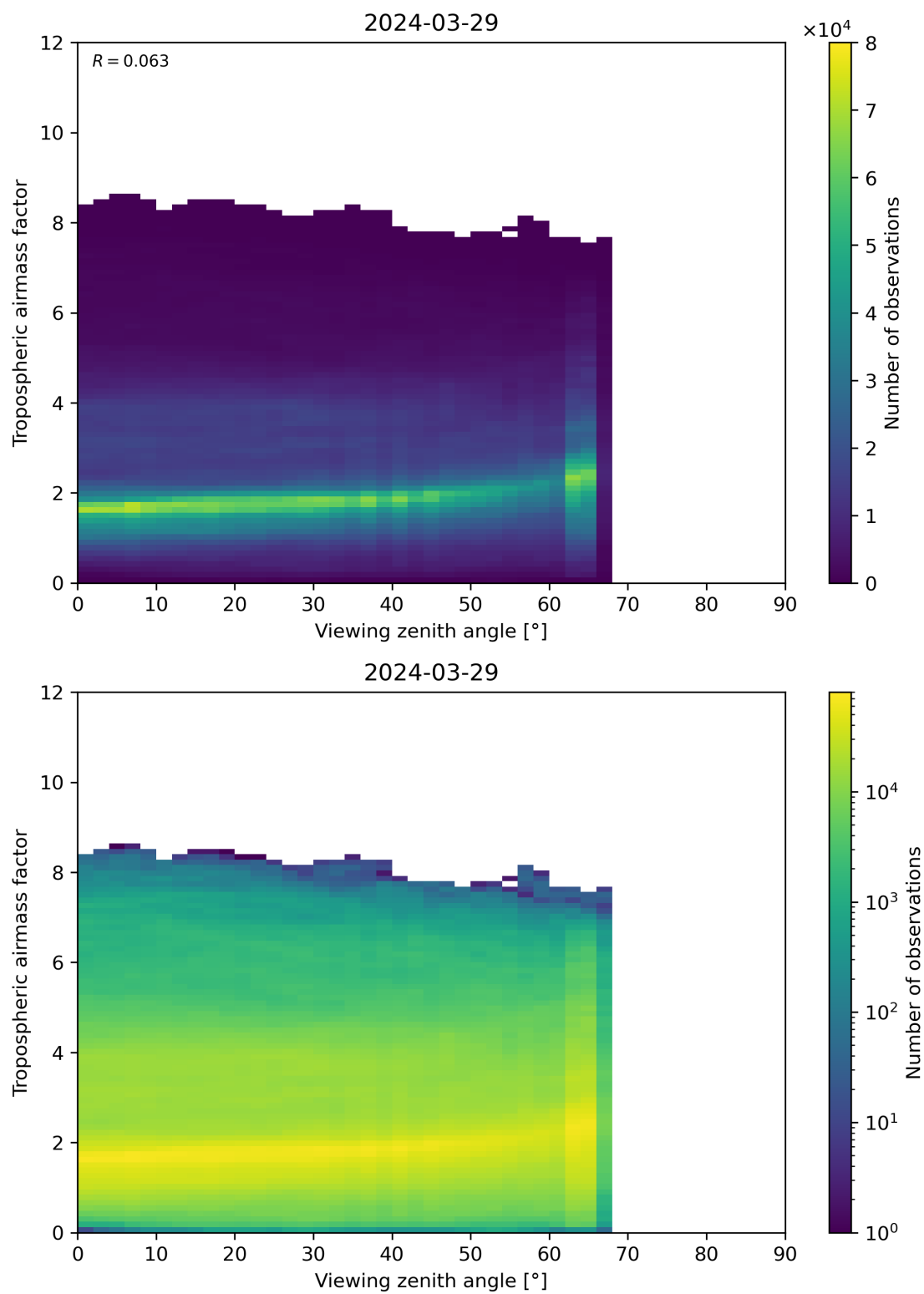
Figure 161: Scatter density plot of “Viewing zenith angle” against “Tropospheric airmass factor” for 2024-03-28 to 2024-03-30.
