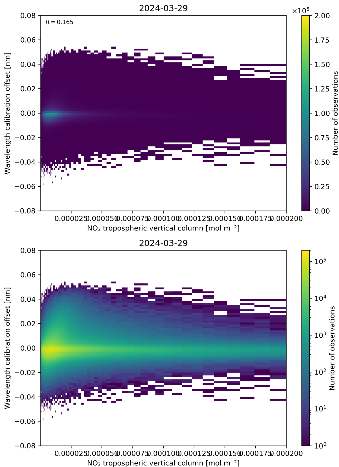
Figure 143: Scatter density plot of “NO 2 tropospheric vertical column” against “Wavelength calibration offset” for 2024-03-28 to 2024-03-30.
