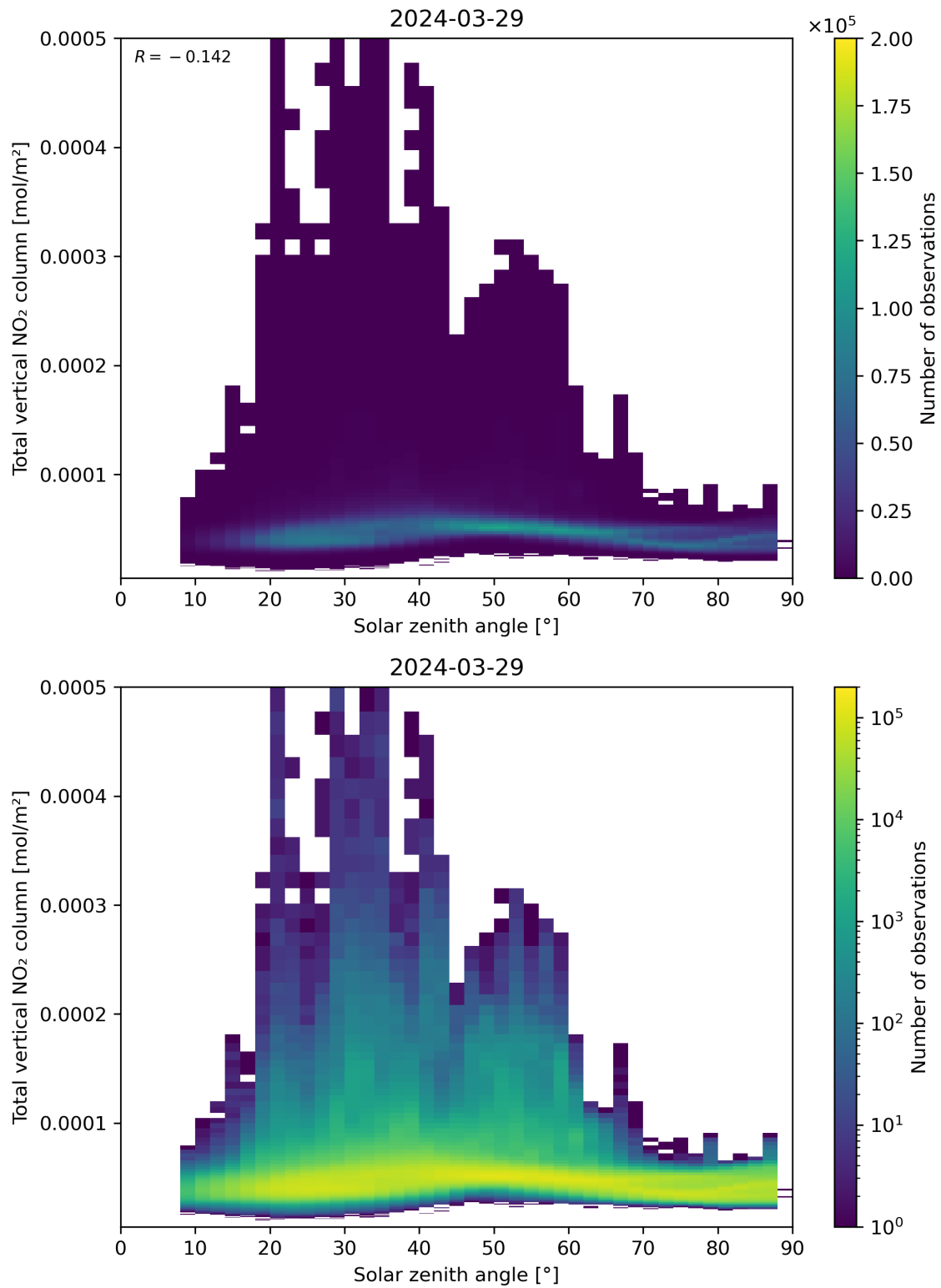
Figure 153: Scatter density plot of “Solar zenith angle” against “Total vertical NO 2 column” for 2024-03-28 to 2024-03-30.
