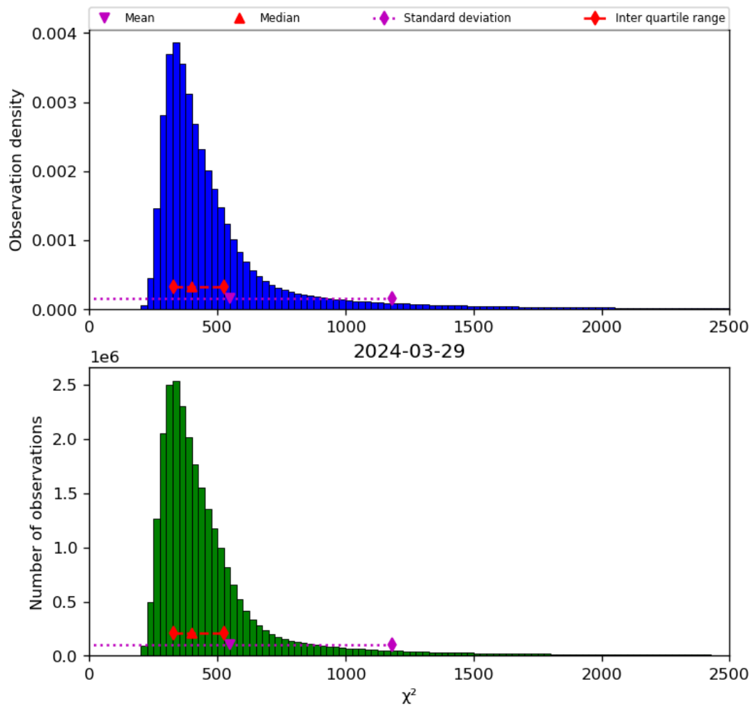
Figure 42: Histogram of " \chi^2 " for 2024-03-28 to 2024-03-30
