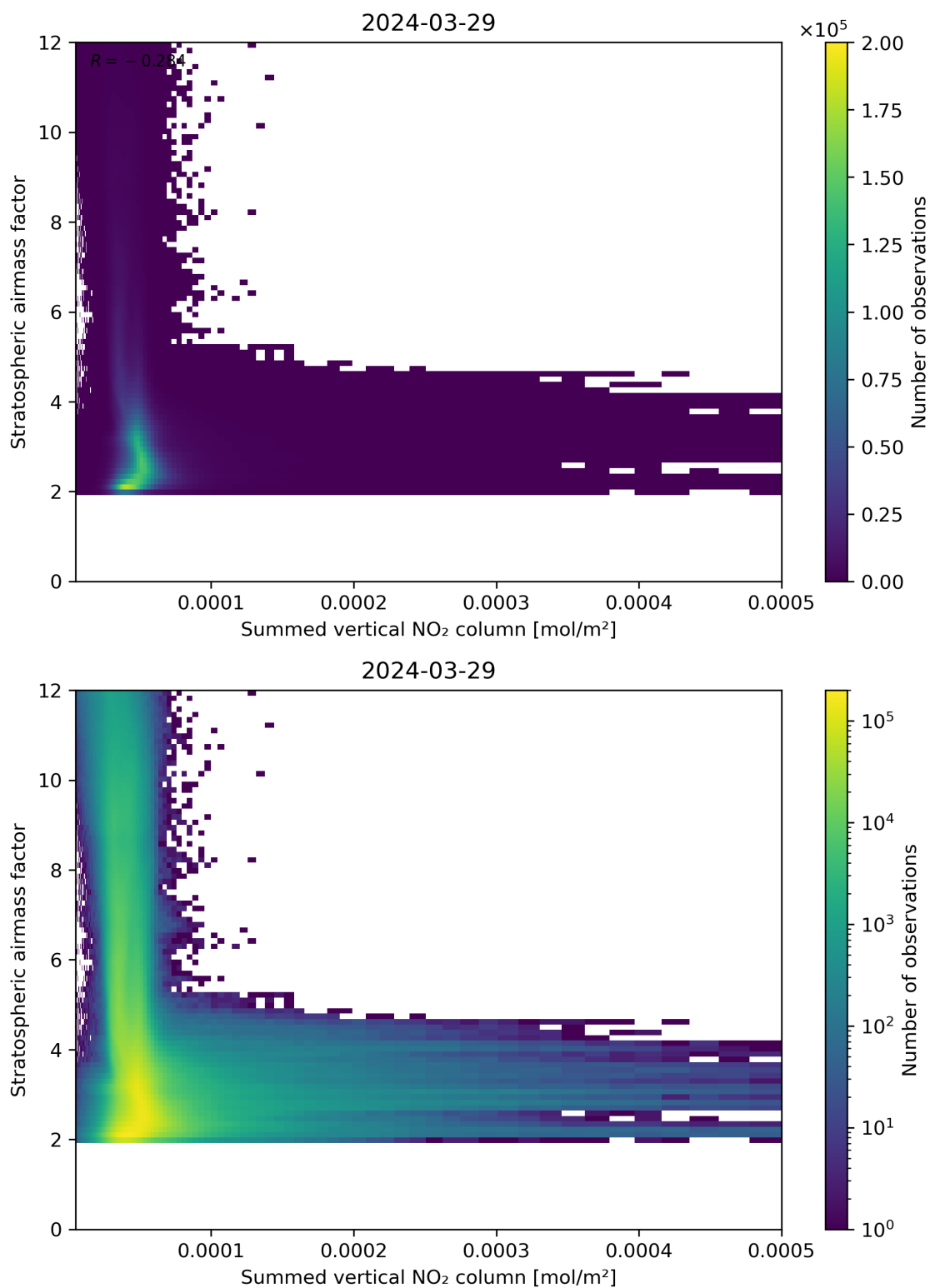
Figure 103: Scatter density plot of “Summed vertical NO 2 column” against “Stratospheric air mass factor” for 2024-03-28 to 2024-03-30.
