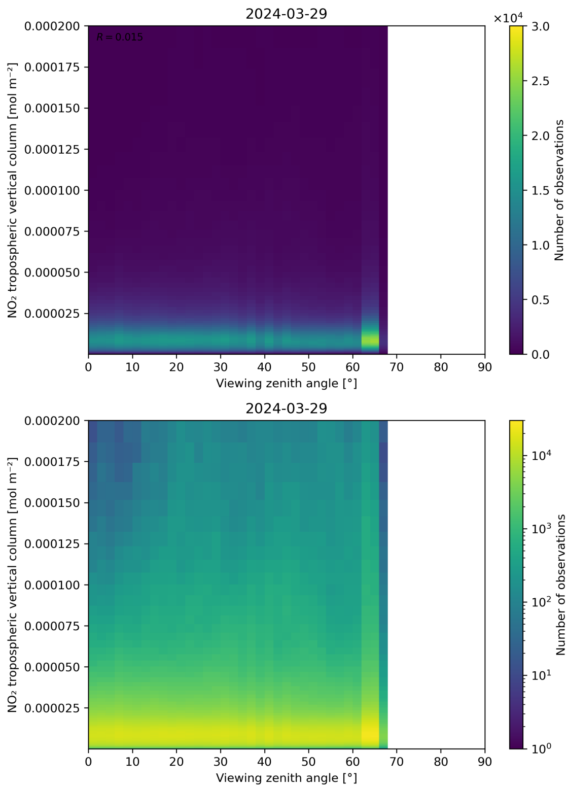
Figure 169: Scatter density plot of “Viewing zenith angle” against “NO 2 tropospheric vertical column” for 2024-03-28 to 2024-03-30.
