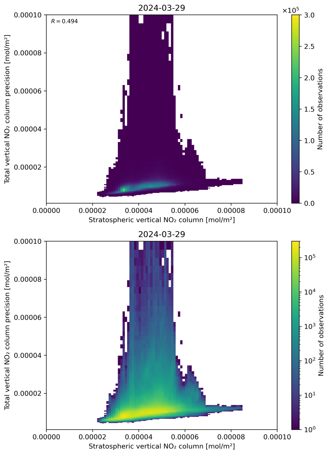
Figure 101: Scatter density plot of “Stratospheric vertical NO 2 column” against “Total vertical NO 2 column precision” for 2024-03-28 to 2024-03-30.
