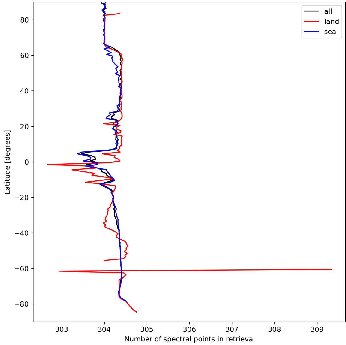
Figure 16: Zonal average of “Number of spectral points in retrieval” for 2024-03-28 to 2024-03-30.
