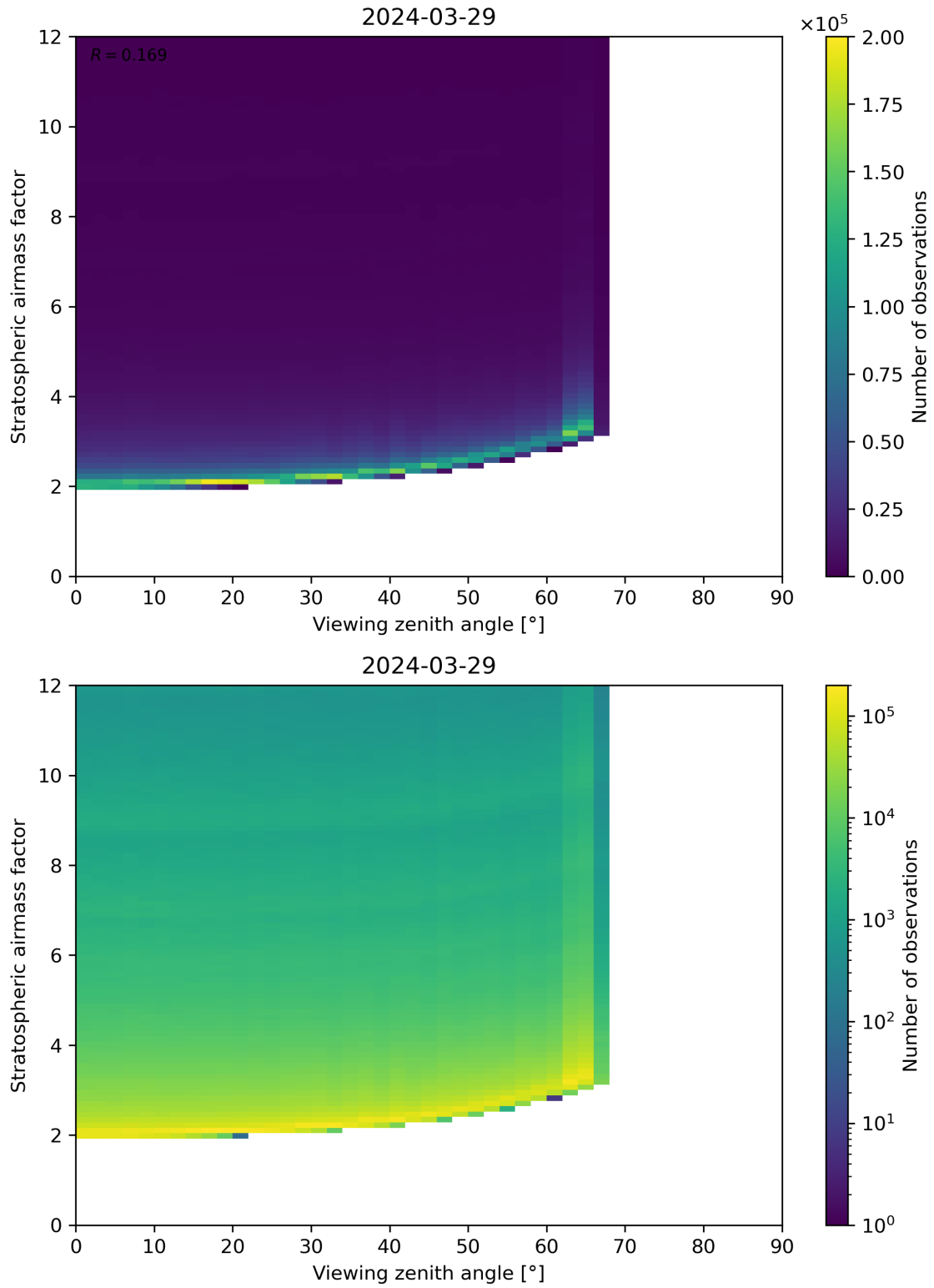
Figure 159: Scatter density plot of “Viewing zenith angle” against “Stratospheric airmass factor” for 2024-03-28 to 2024-03-30.
