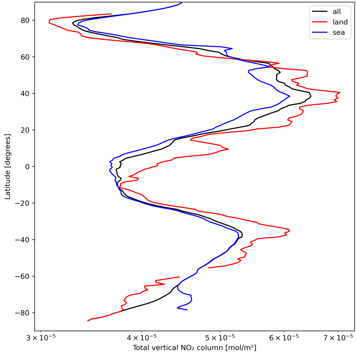
Figure 21: Zonal average of “Total vertical NO 2 column” for 2024-03-28 to 2024-03-30.
