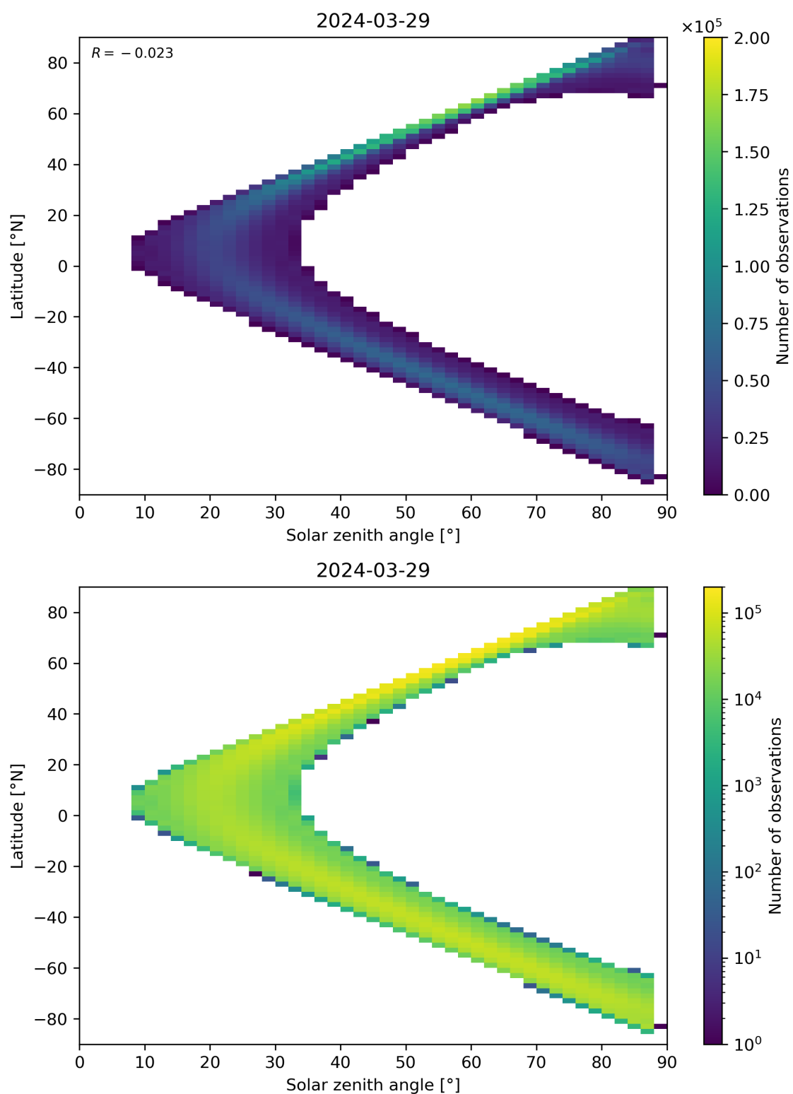
Figure 149: Scatter density plot of “Solar zenith angle” against “Latitude” for 2024-03-28 to 2024-03-30.
