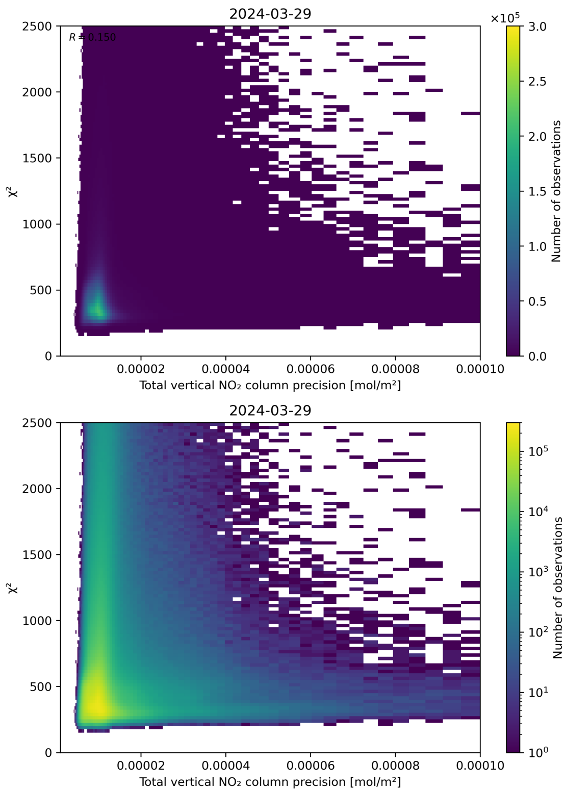
Figure 116: Scatter density plot of “Total vertical NO 2 column precision” against “ \chi^2 ” for 2024-03-28 to 2024-03-30.
