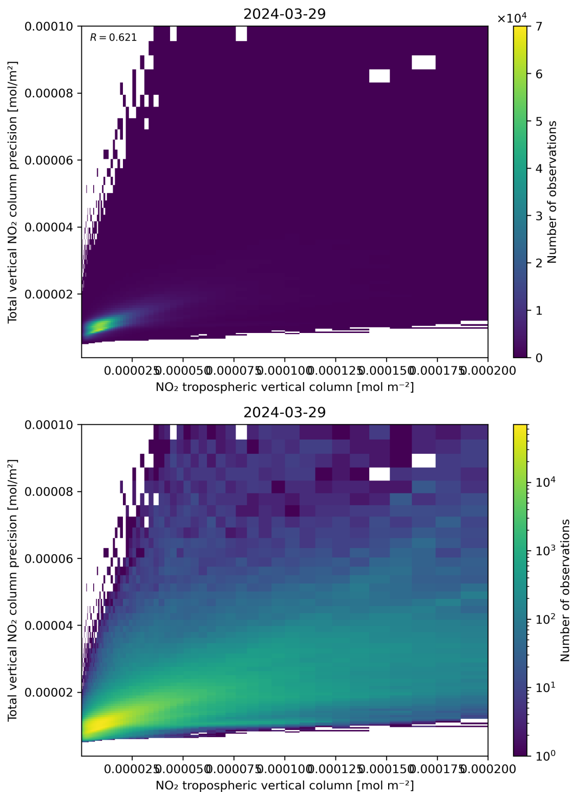
Figure 129: Scatter density plot of “NO 2 tropospheric vertical column” against “Total vertical NO 2 column precision” for 2024-03-28 to 2024-03-30.
