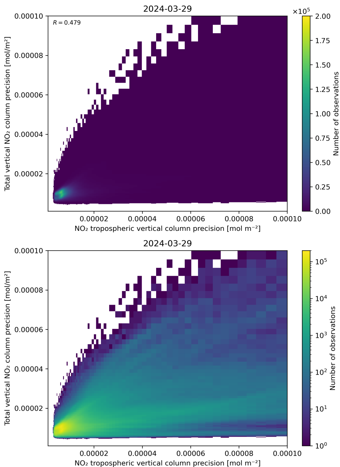
Figure 139: Scatter density plot of “NO 2 tropospheric vertical column precision” against “Total vertical NO 2 column precision” for 2024-03-28 to 2024-03-30.
