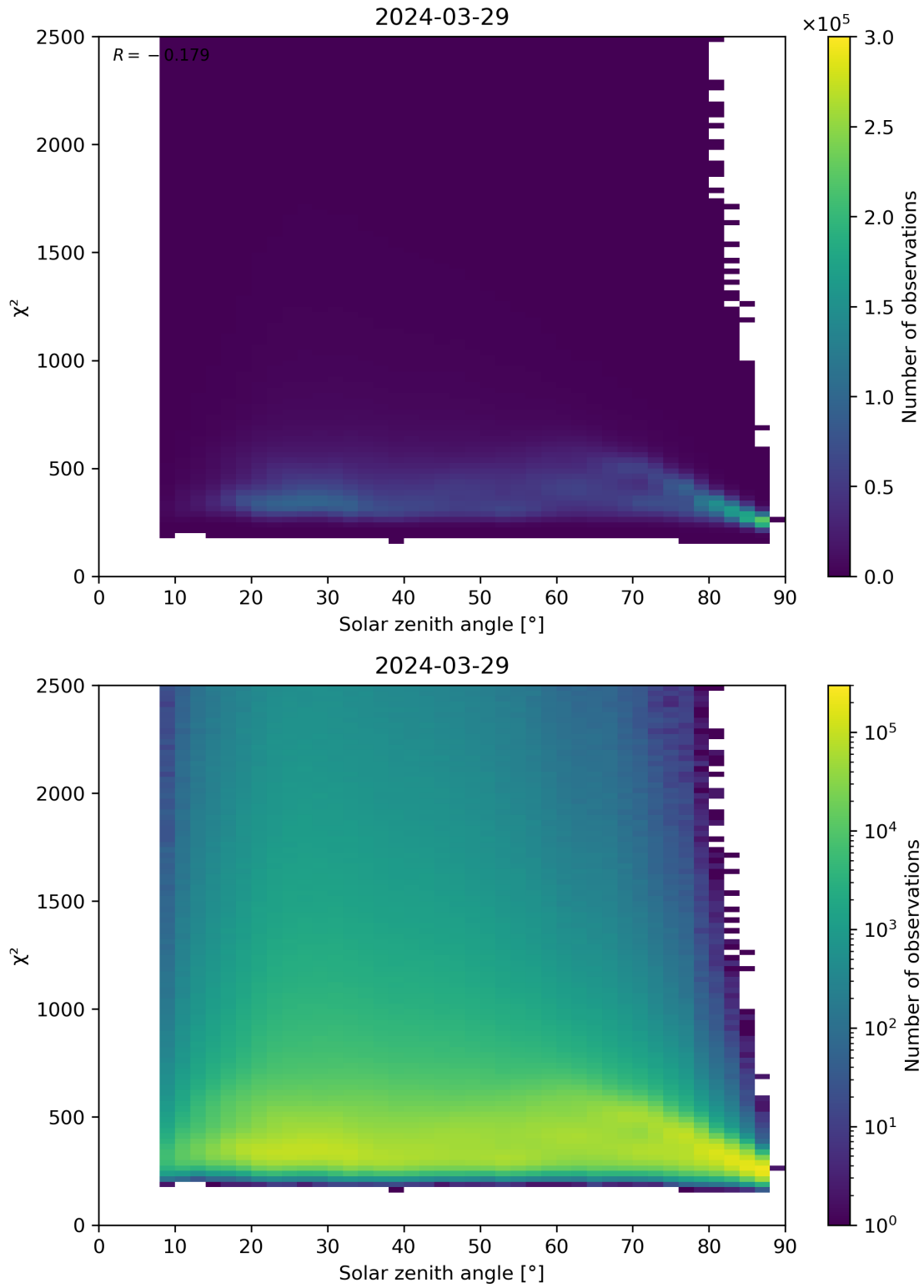
Figure 148: Scatter density plot of “Solar zenith angle” against “ \chi^2 ” for 2024-03-28 to 2024-03-30.
