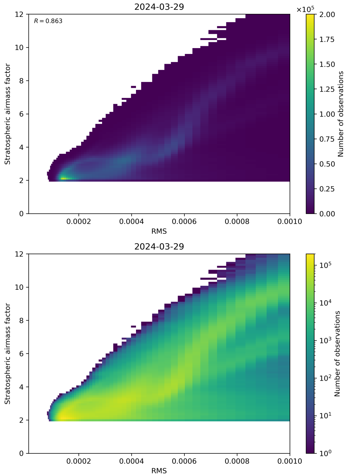
Figure 144: Scatter density plot of “RMS” against “Stratospheric airmass factor” for 2024-03-28 to 2024-03-30.
