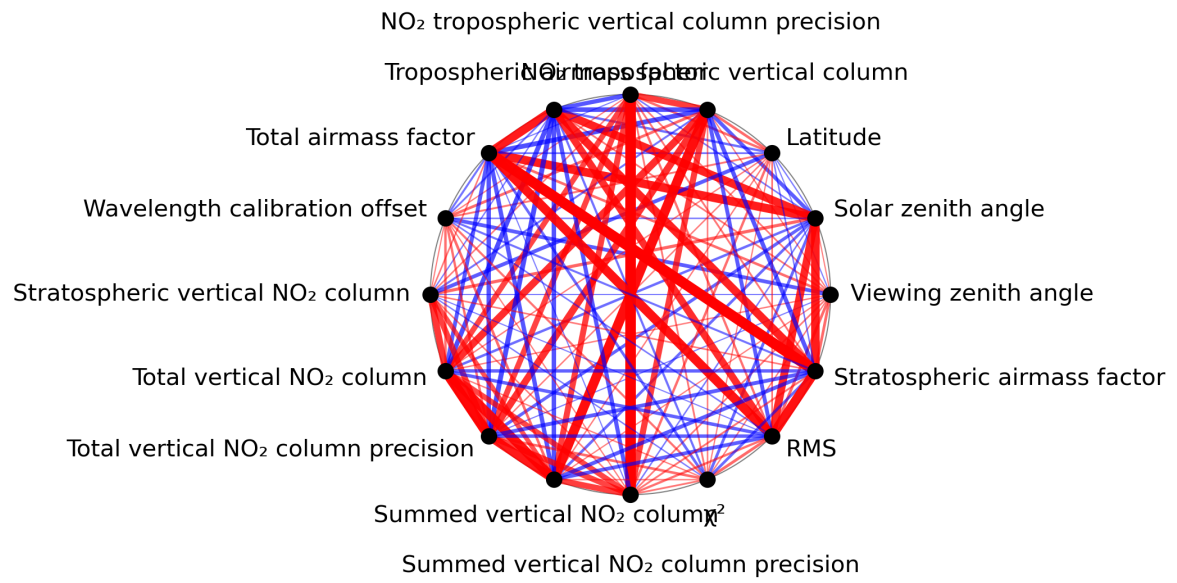
Figure 1: Map of correlation graph for 2024-03-28 to 2024-03-30.
