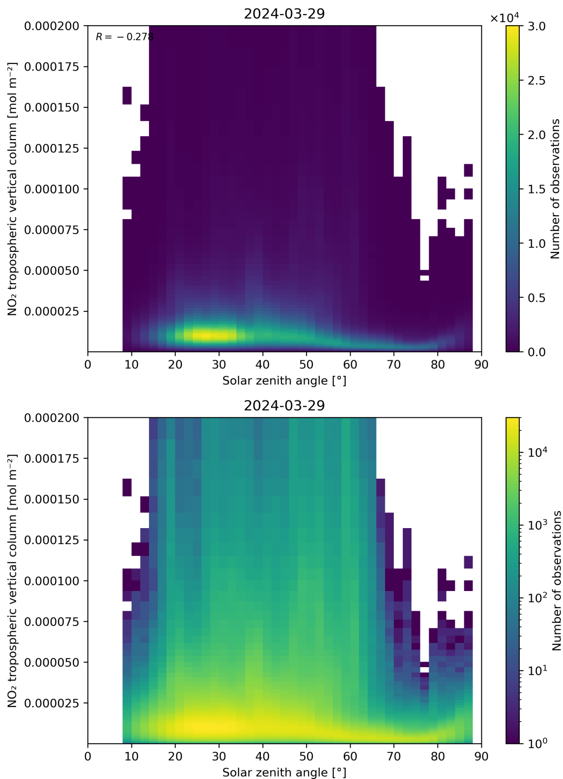
Figure 155: Scatter density plot of “Solar zenith angle” against “NO 2 tropospheric vertical column” for 2024-03-28 to 2024-03-30.
