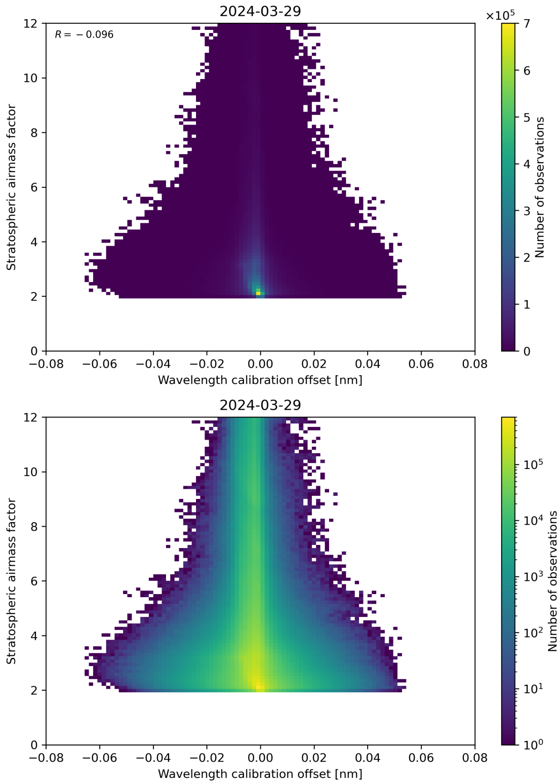
Figure 174: Scatter density plot of “Wavelength calibration offset” against “Stratospheric air mass factor” for 2024-03-28 to 2024-03-30.
