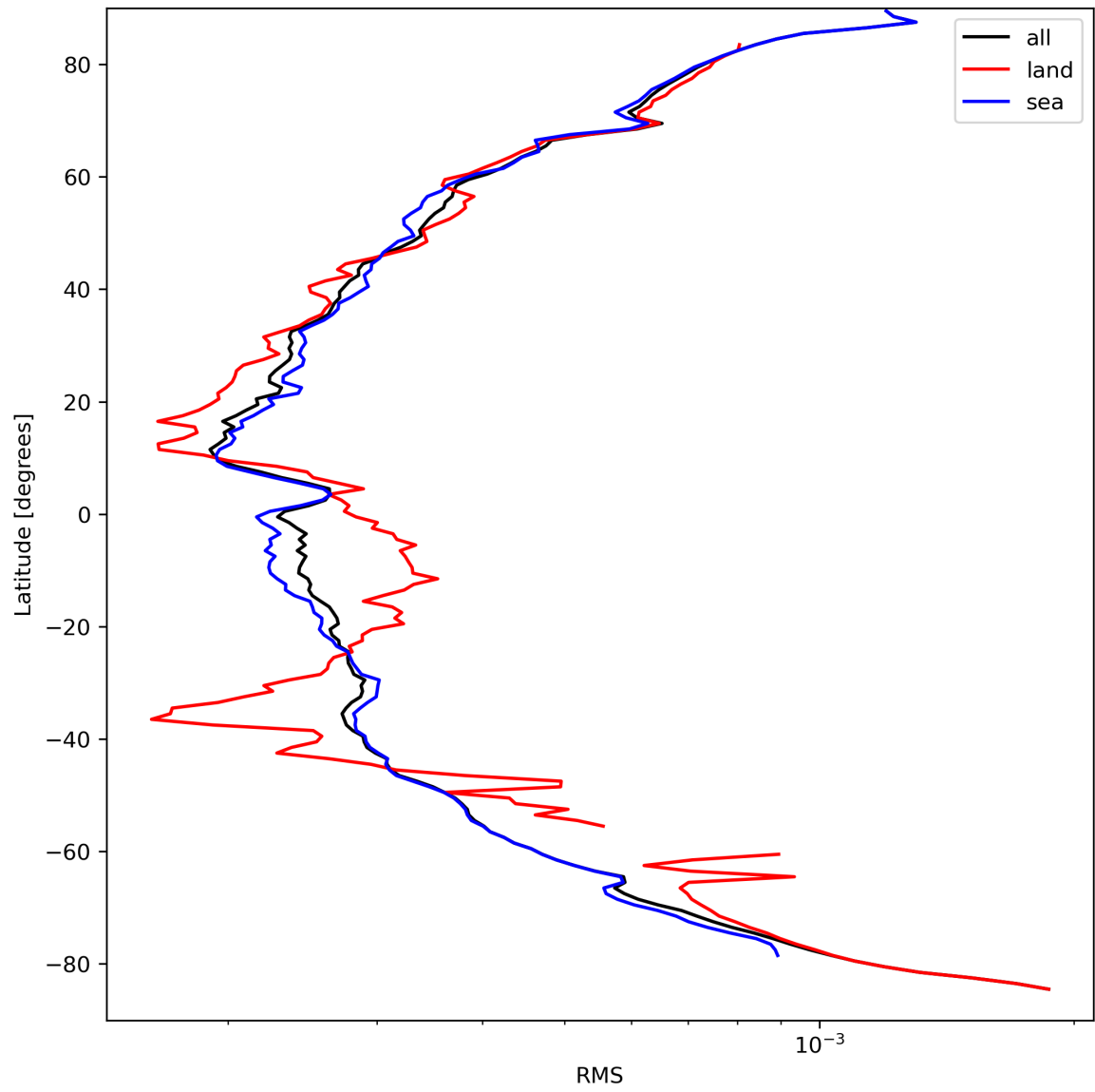
Figure 26: Zonal average of “RMS” for 2024-03-28 to 2024-03-30.
