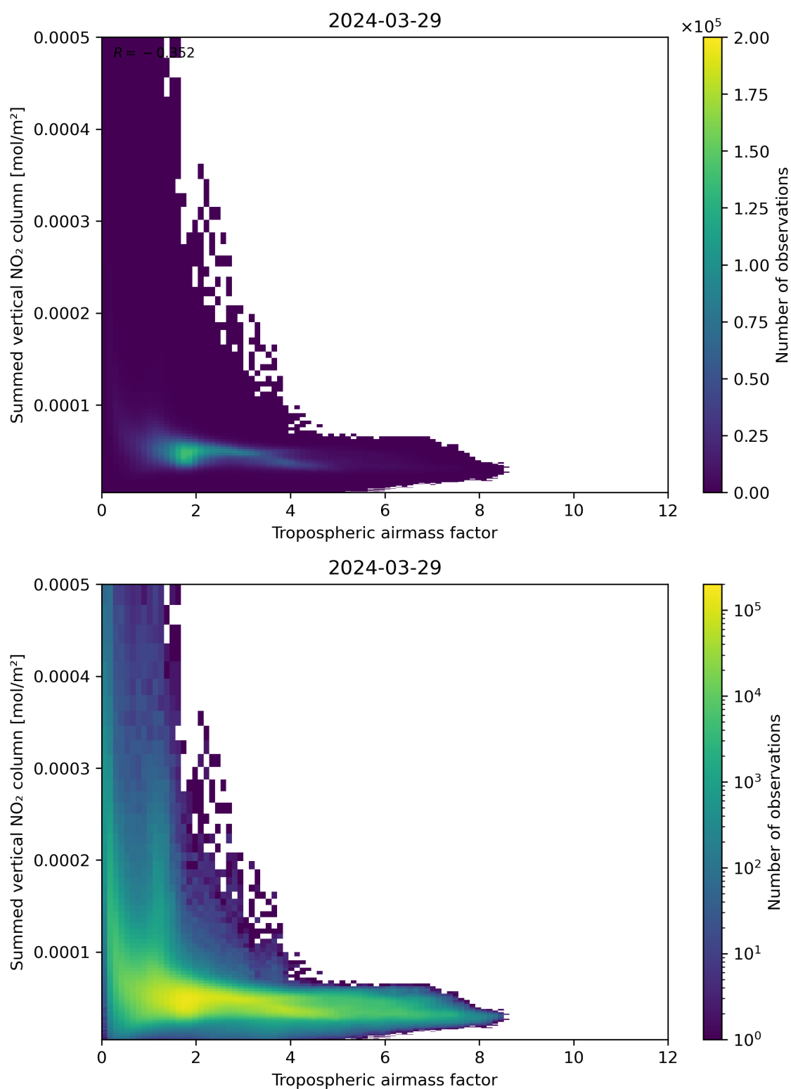
Figure 75: Scatter density plot of “Tropospheric airmass factor” against “Summed vertical NO 2 column” for 2024-03-28 to 2024-03-30.
