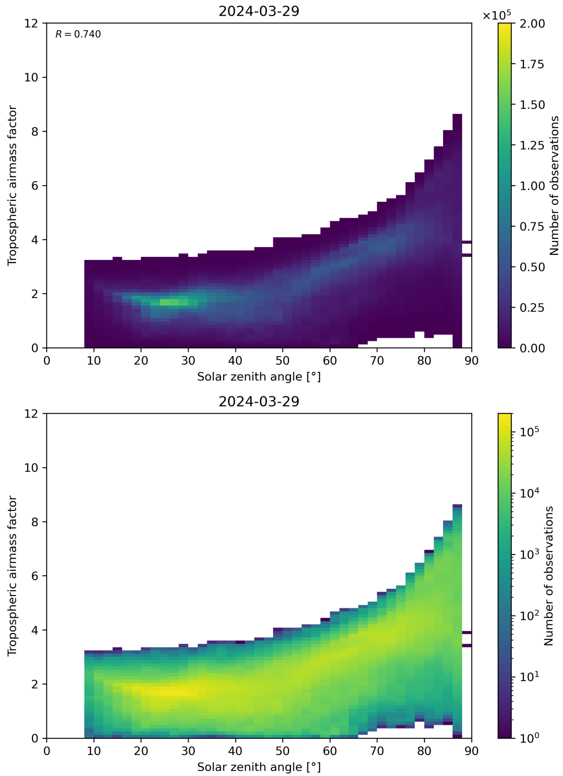
Figure 147: Scatter density plot of “Solar zenith angle” against “Tropospheric airmass factor” for 2024-03-28 to 2024-03-30.
