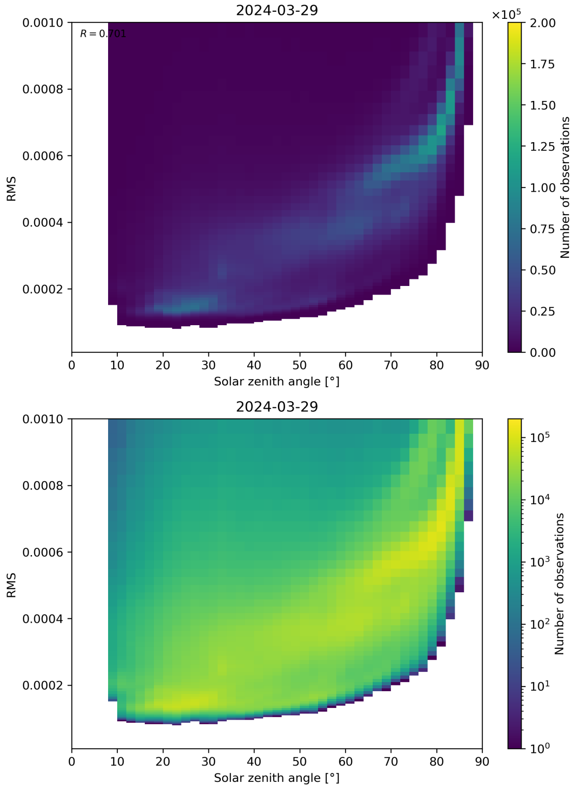
Figure 157: Scatter density plot of “Solar zenith angle” against “RMS” for 2024-03-28 to 2024-03-30.
