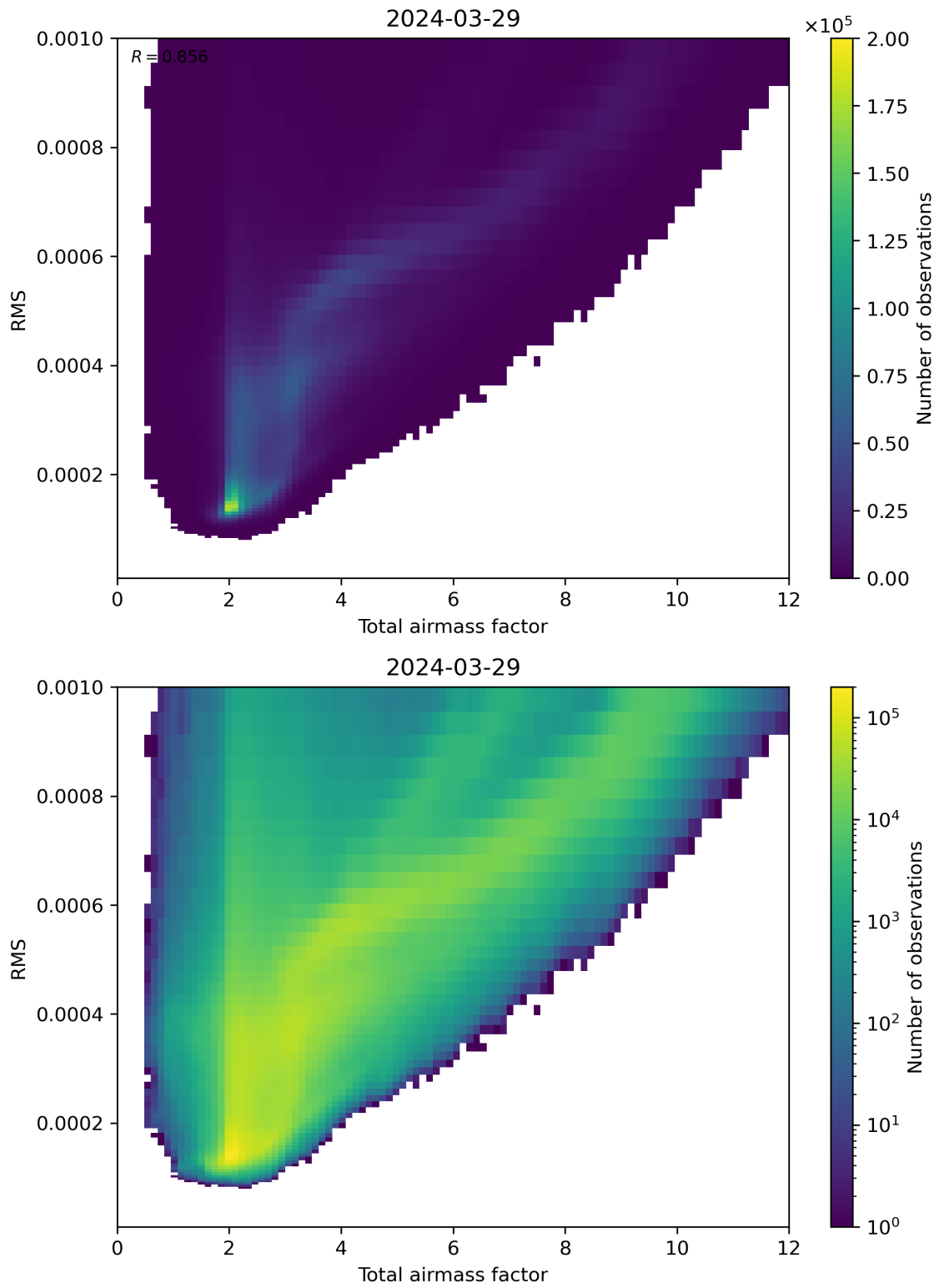
Figure 69: Scatter density plot of “Total airmass factor” against “RMS” for 2024-03-28 to 2024-03-30.
