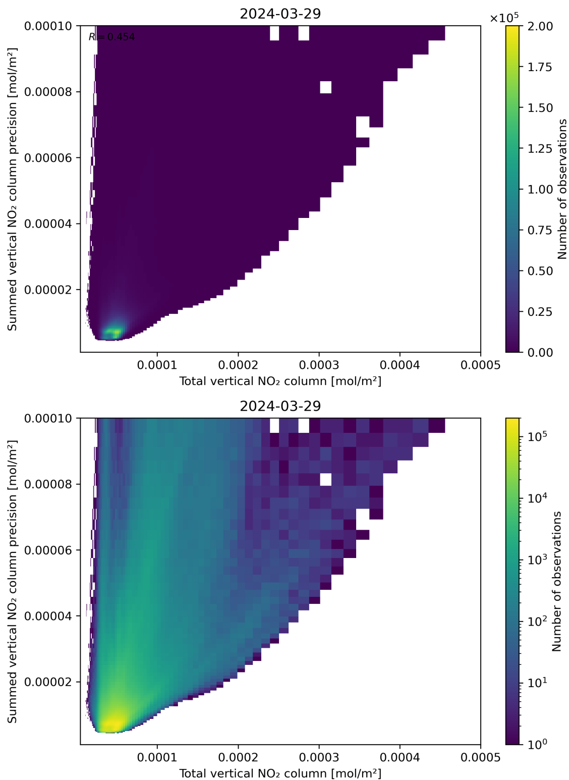
Figure 113: Scatter density plot of “Total vertical NO 2 column” against “Summed vertical NO 2 column precision” for 2024-03-28 to 2024-03-30.
