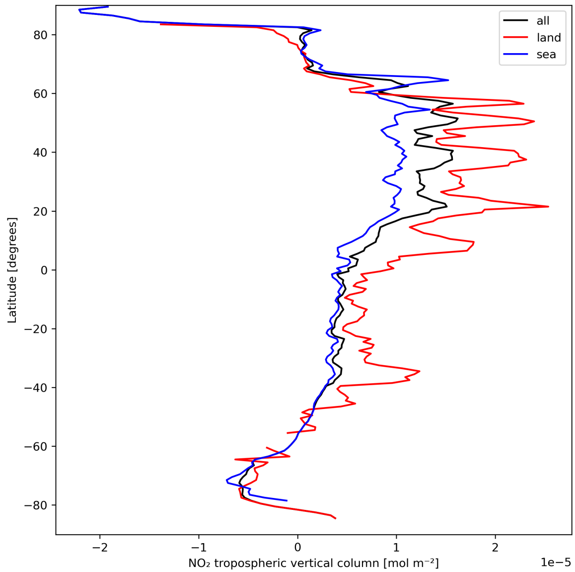
Figure 12: Zonal average of “NO 2 tropospheric vertical column” for 2024-03-28 to 2024-03-30.
