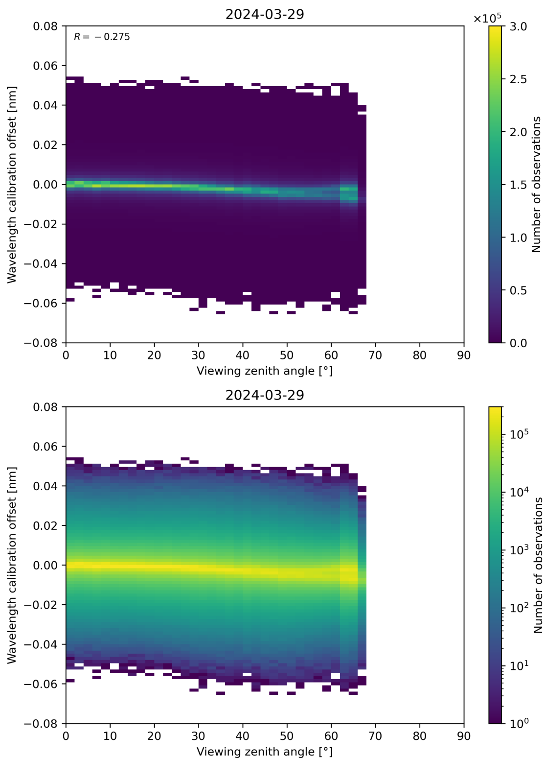
Figure 173: Scatter density plot of “Viewing zenith angle” against “Wavelength calibration offset” for 2024-03-28 to 2024-03-30.
