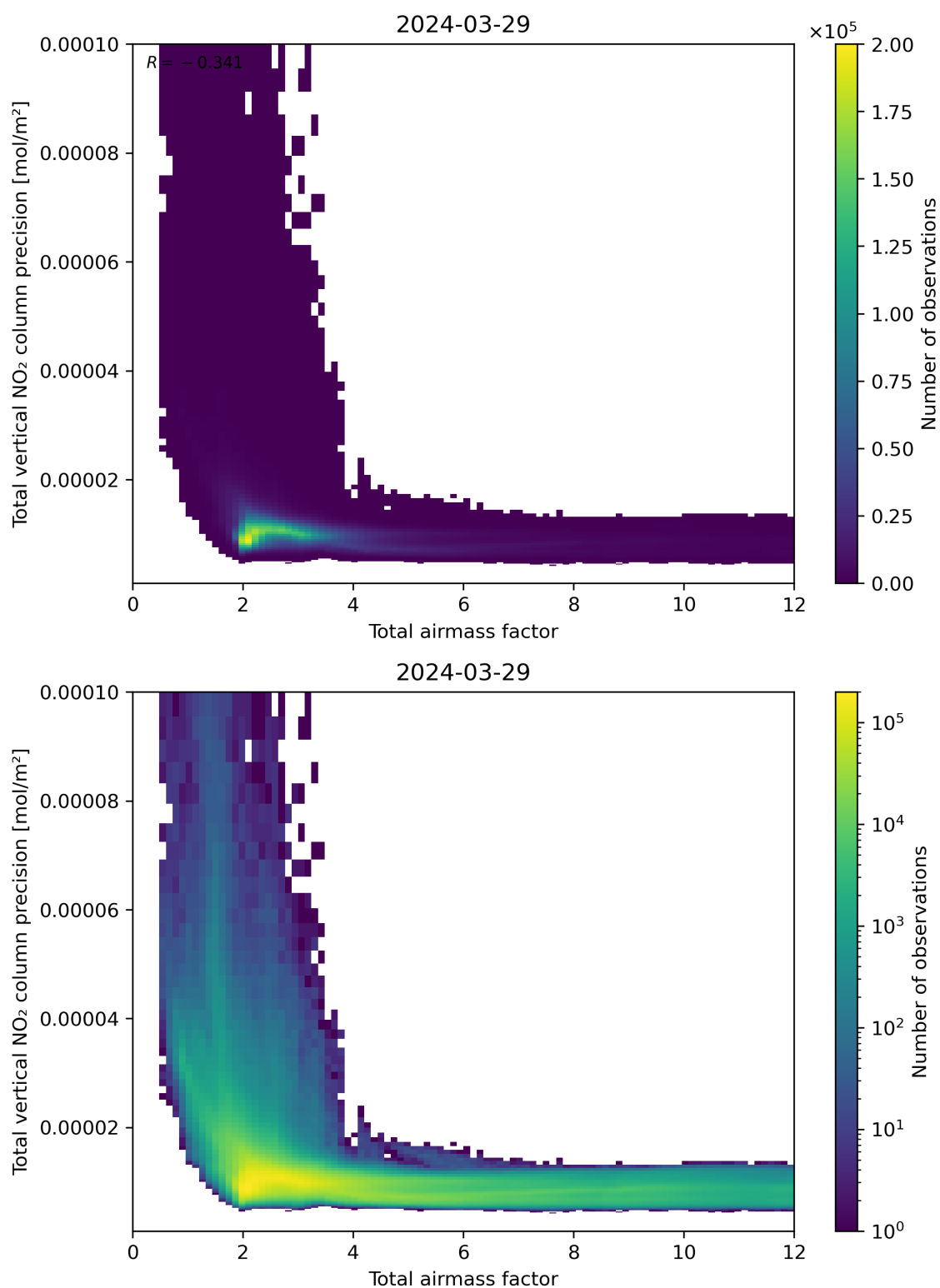
Figure 68: Scatter density plot of “Total airmass factor” against “Total vertical NO 2 column precision” for 2024-03-28 to 2024-03-30.
