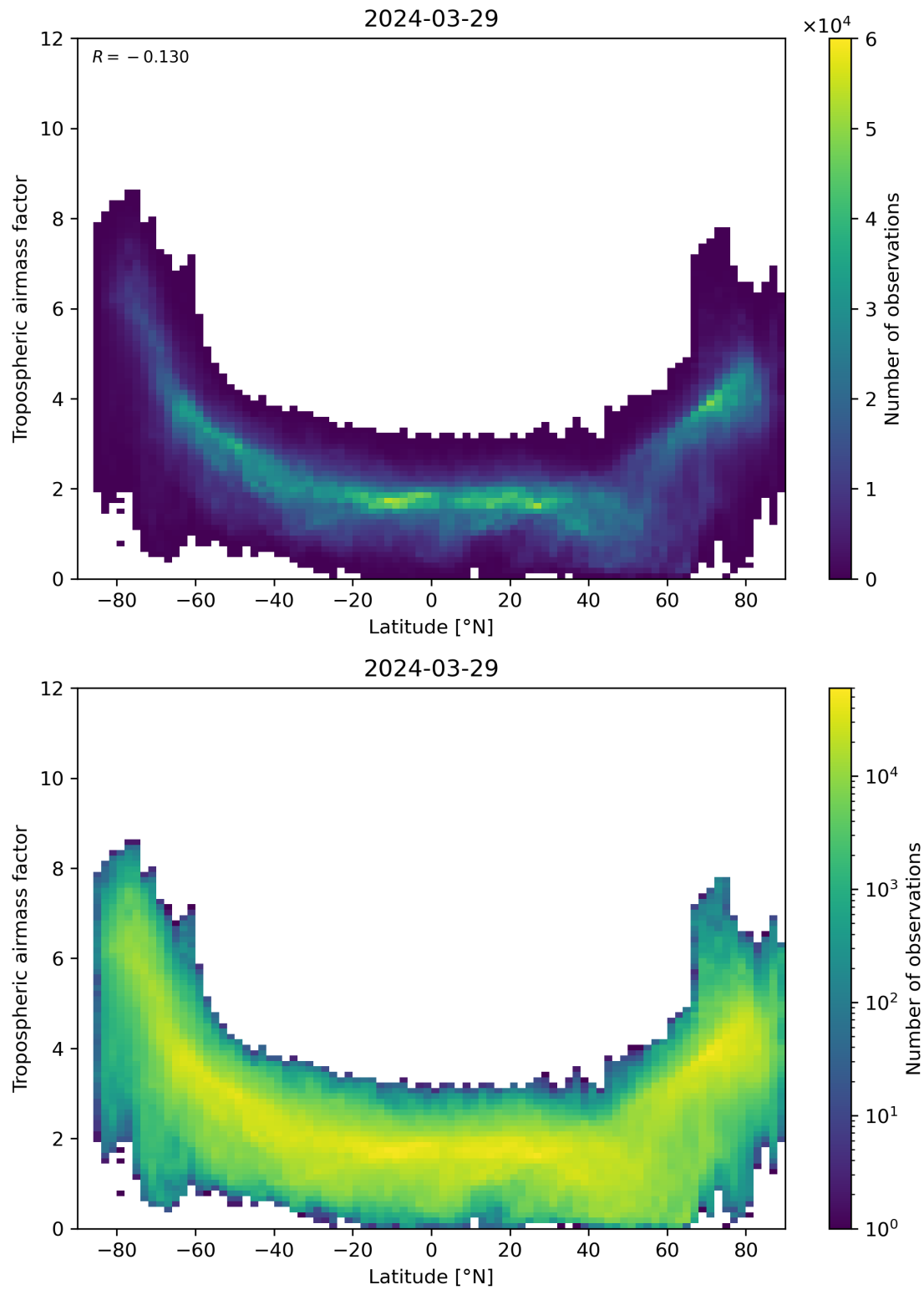
Figure 85: Scatter density plot of “Latitude” against “Tropospheric airmass factor” for 2024-03-28 to 2024-03-30.
