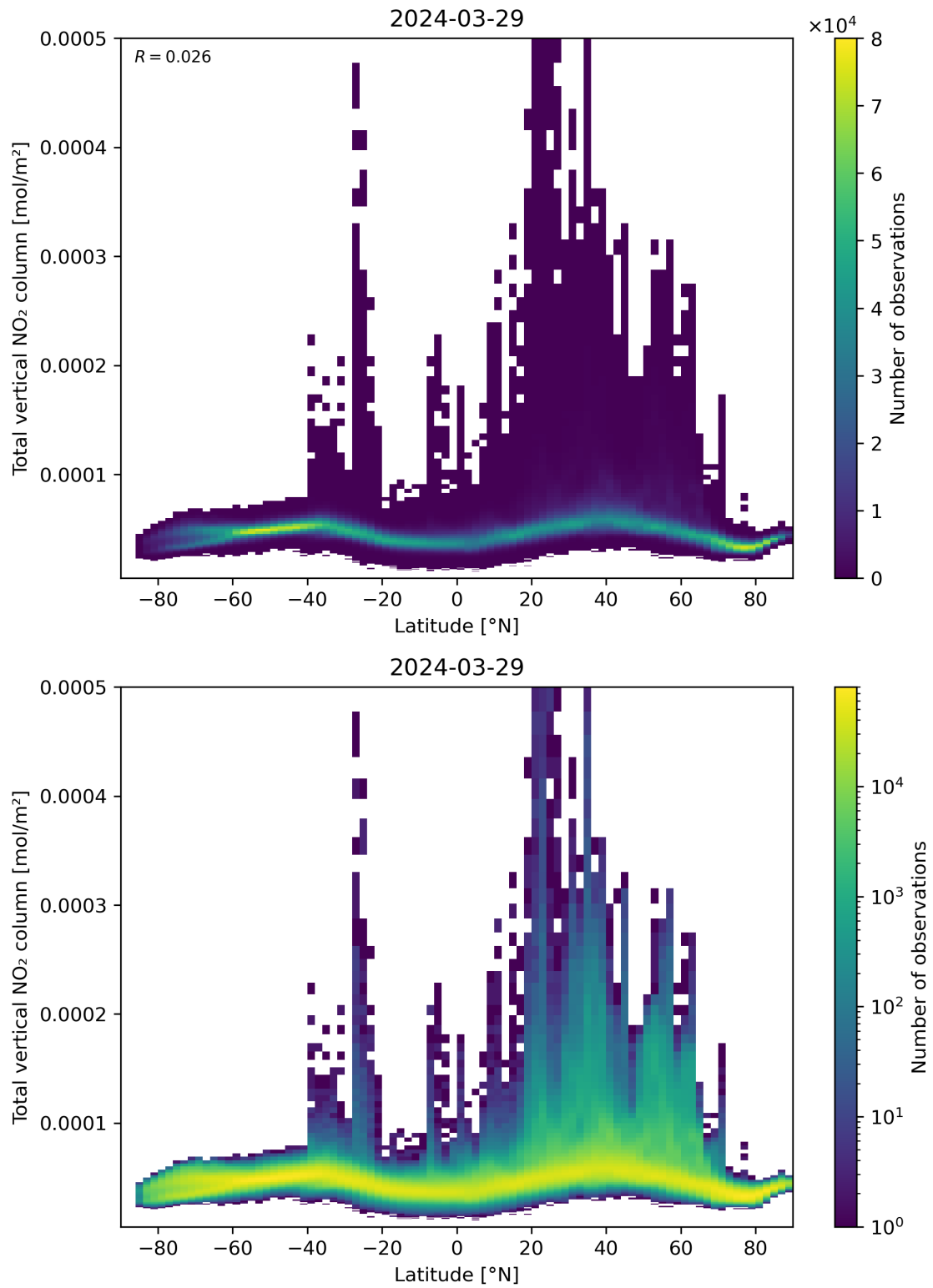
Figure 90: Scatter density plot of “Latitude” against “Total vertical NO 2 column” for 2024-03-28 to 2024-03-30.
