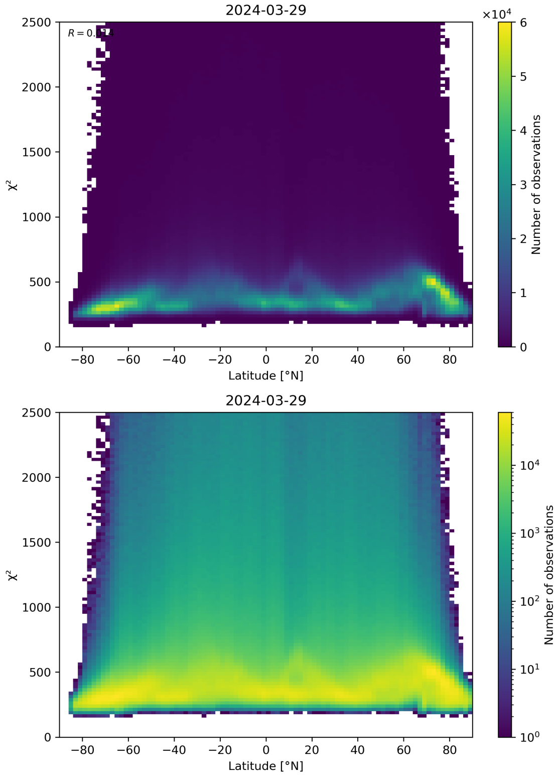
Figure 86: Scatter density plot of “Latitude” against “ \chi^2 ” for 2024-03-28 to 2024-03-30.
