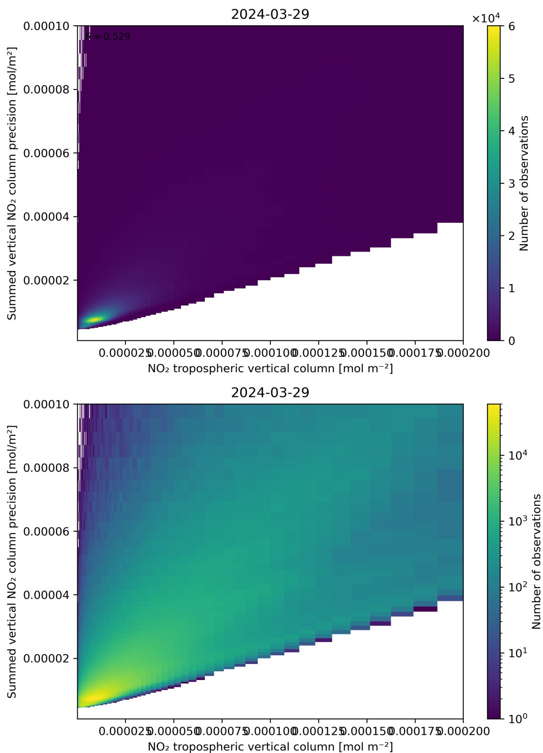
Figure 127: Scatter density plot of “NO 2 tropospheric vertical column” against “Summed vertical NO 2 column precision” for 2024-03-28 to 2024-03-30.
