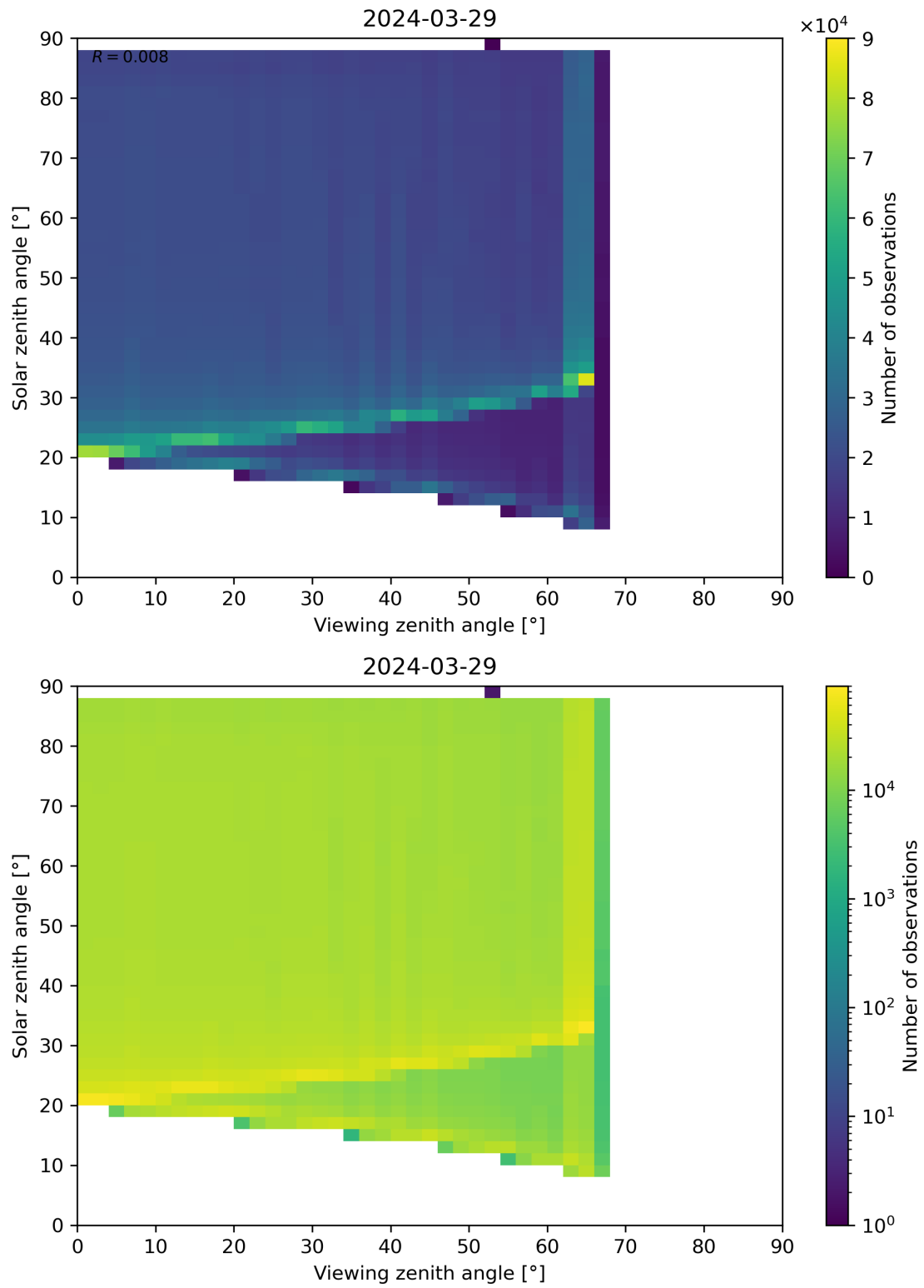
Figure 172: Scatter density plot of “Viewing zenith angle” against “Solar zenith angle” for 2024-03-28 to 2024-03-30.
