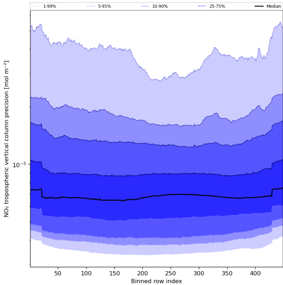
Figure 47: Along track statistics of “NO 2 tropospheric vertical column precision” for 2024-03-28 to 2024-03-30
