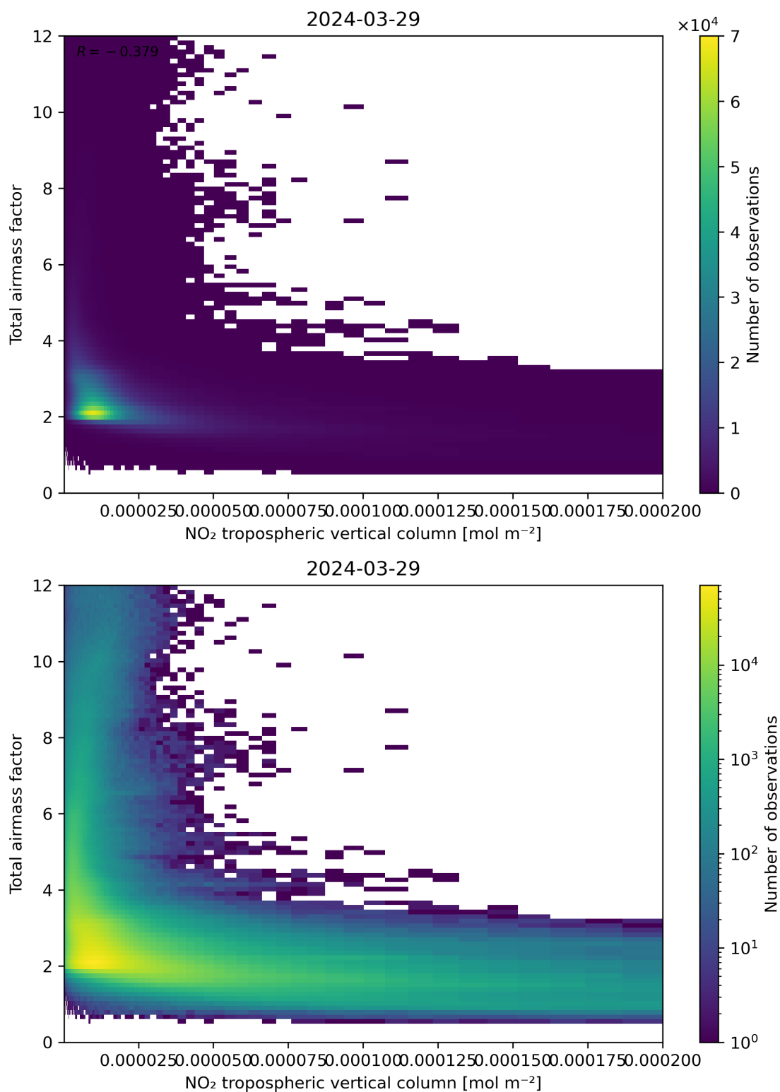
Figure 122: Scatter density plot of “NO 2 tropospheric vertical column” against “Total airmass factor” for 2024-03-28 to 2024-03-30.
