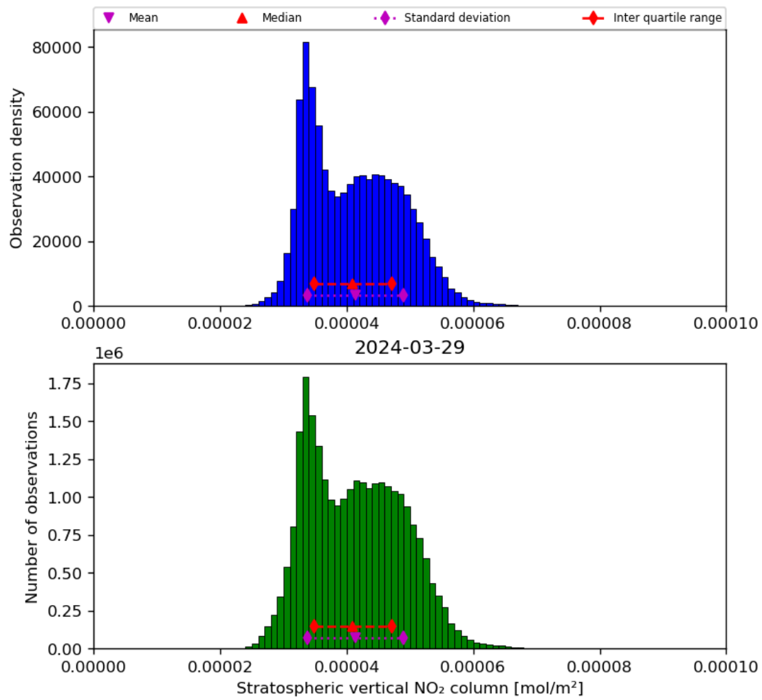
Figure 36: Histogram of “Stratospheric vertical NO 2 column” for 2024-03-28 to 2024-03-30
