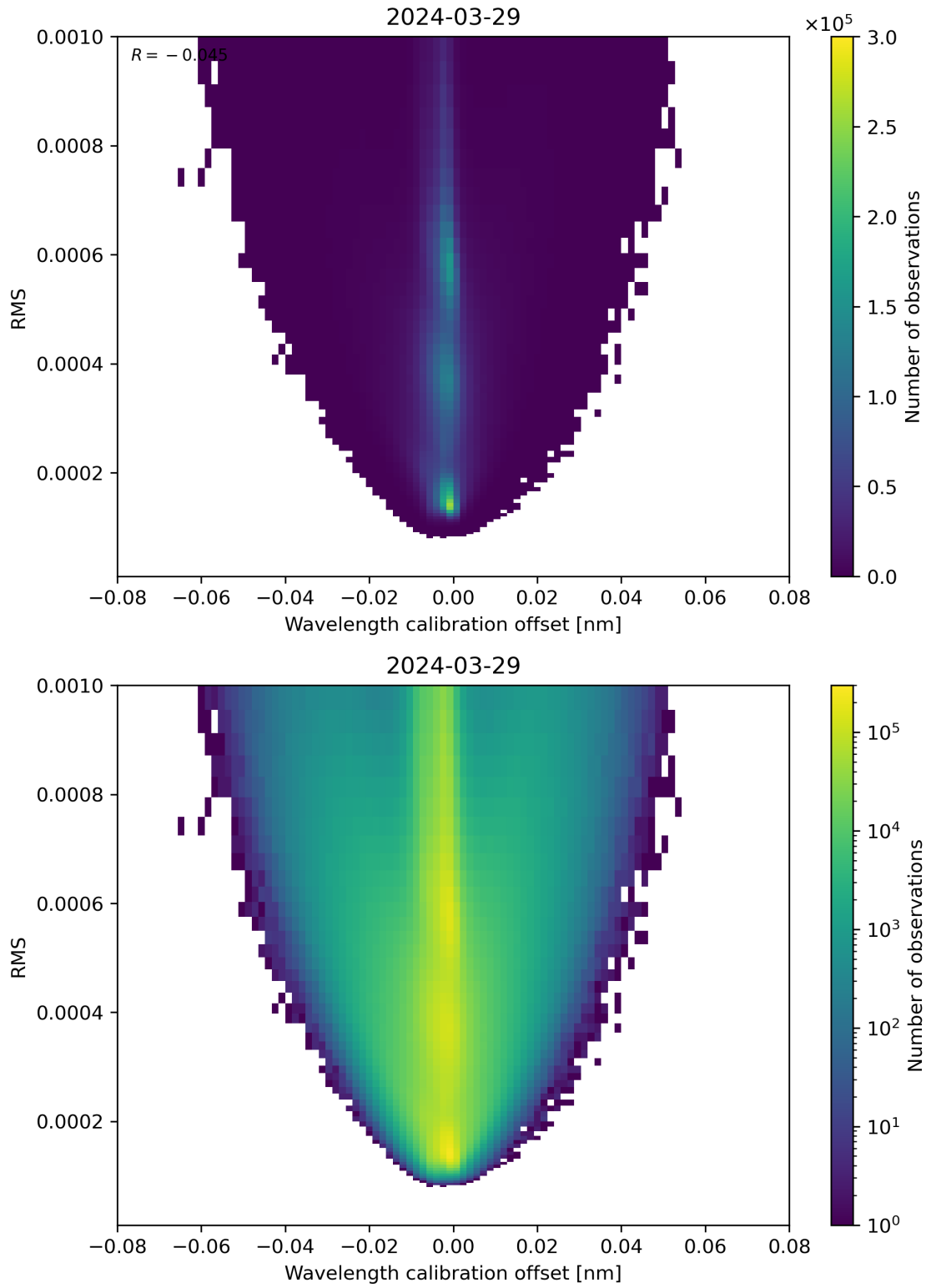
Figure 181: Scatter density plot of “Wavelength calibration offset” against “RMS” for 2024-03-28 to 2024-03-30.
