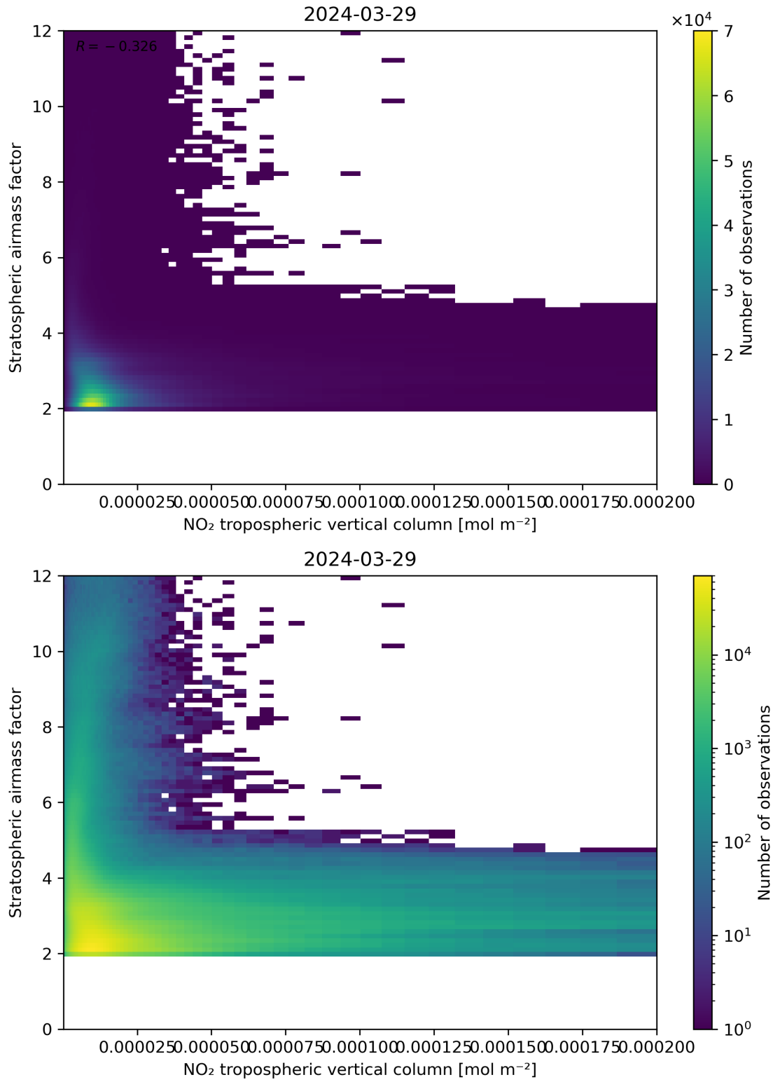
Figure 121: Scatter density plot of “NO 2 tropospheric vertical column” against “Stratospheric air mass factor” for 2024-03-28 to 2024-03-30.
