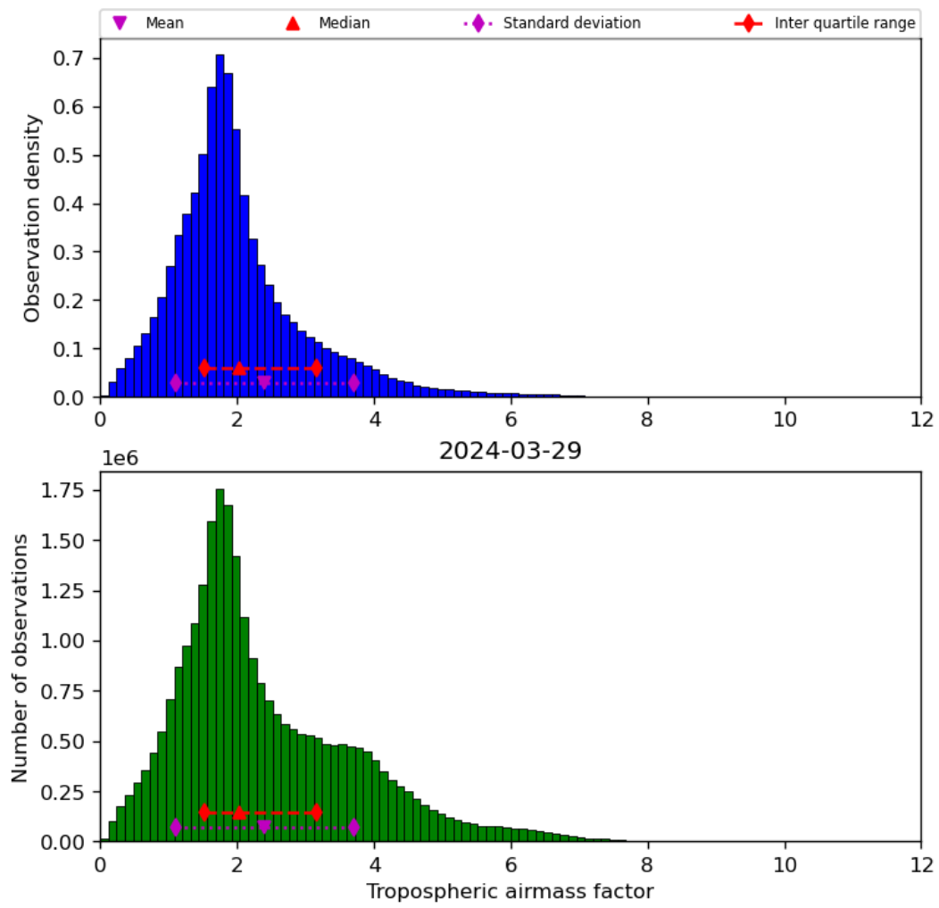
Figure 31: Histogram of “Tropospheric airmass factor” for 2024-03-28 to 2024-03-30
