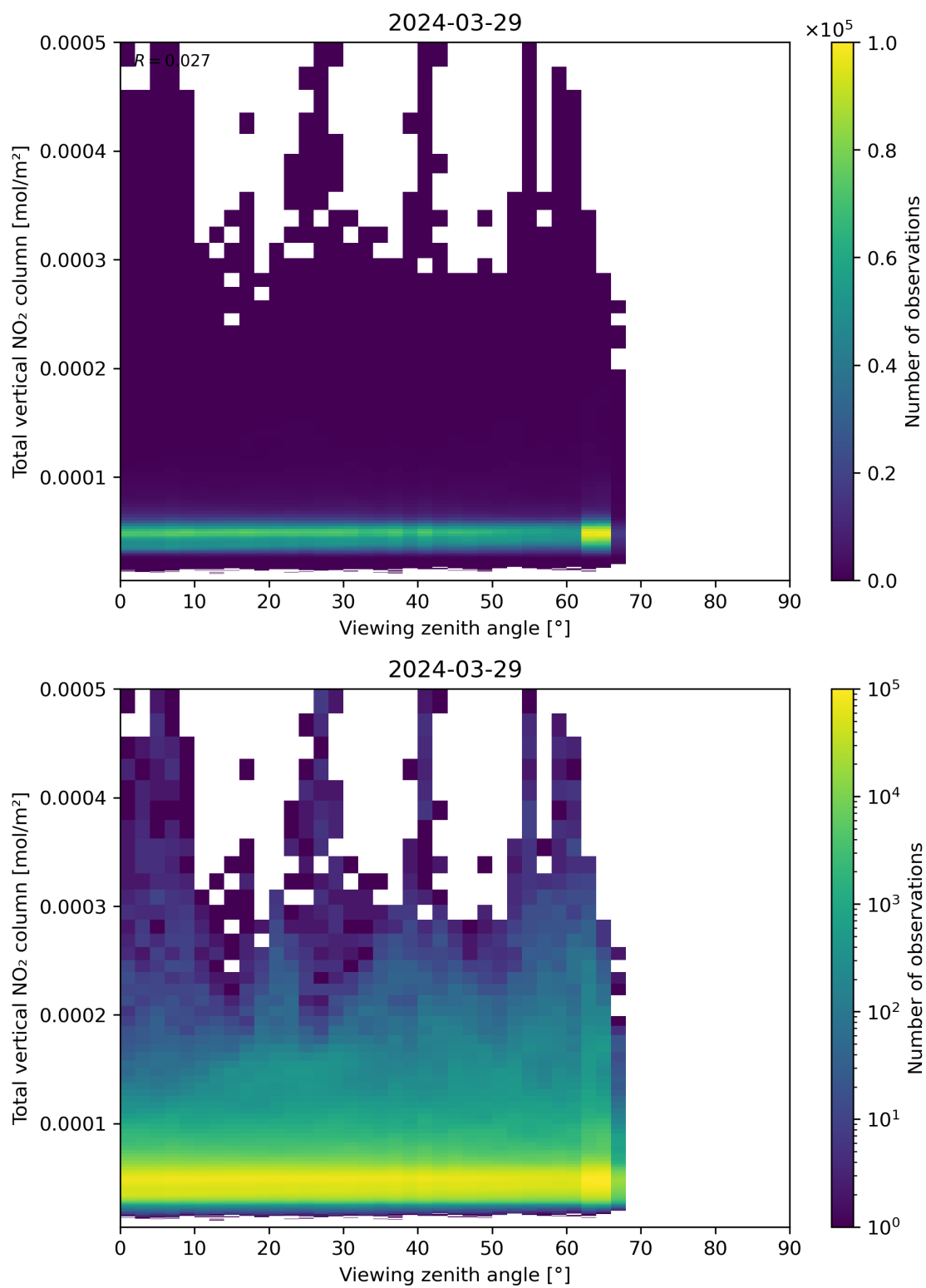
Figure 167: Scatter density plot of “Viewing zenith angle” against “Total vertical NO 2 column” for 2024-03-28 to 2024-03-30.
