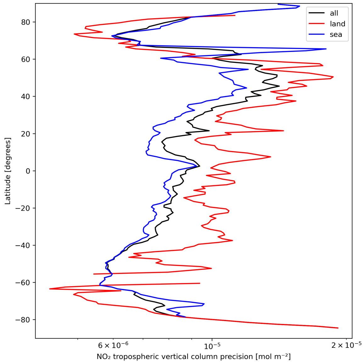
Figure 13: Zonal average of “NO 2 tropospheric vertical column precision” for 2024-03-28 to 2024-03-30.
