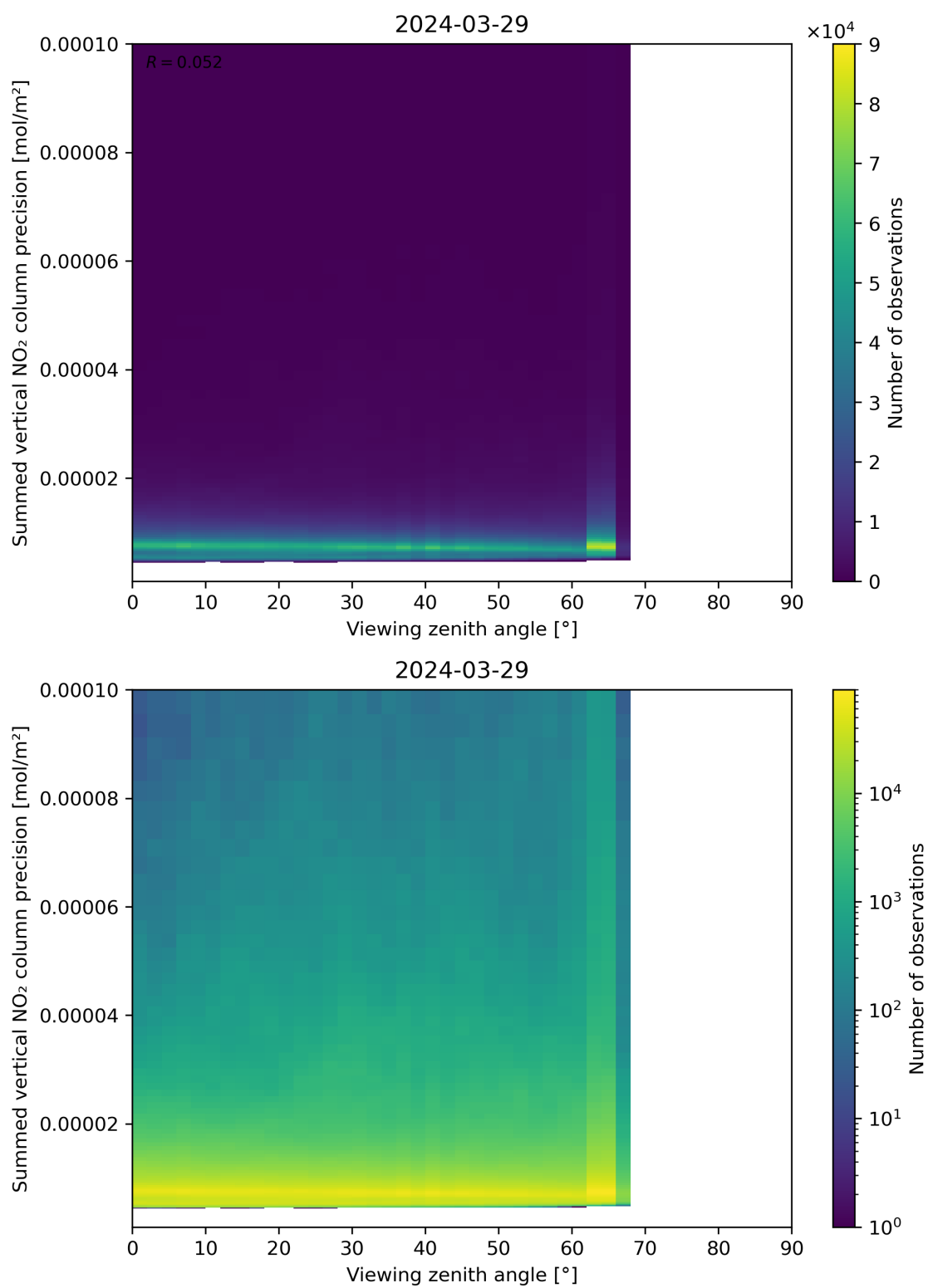
Figure 166: Scatter density plot of “Viewing zenith angle” against “Summed vertical NO 2 column precision” for 2024-03-28 to 2024-03-30.
