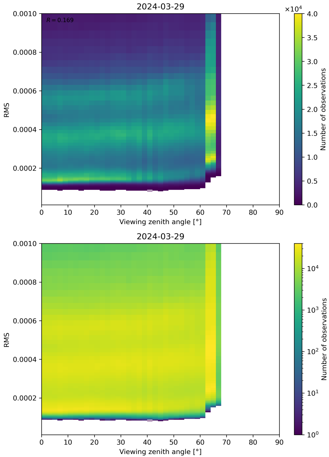
Figure 171: Scatter density plot of “Viewing zenith angle” against “RMS” for 2024-03-28 to 2024-03-30.
