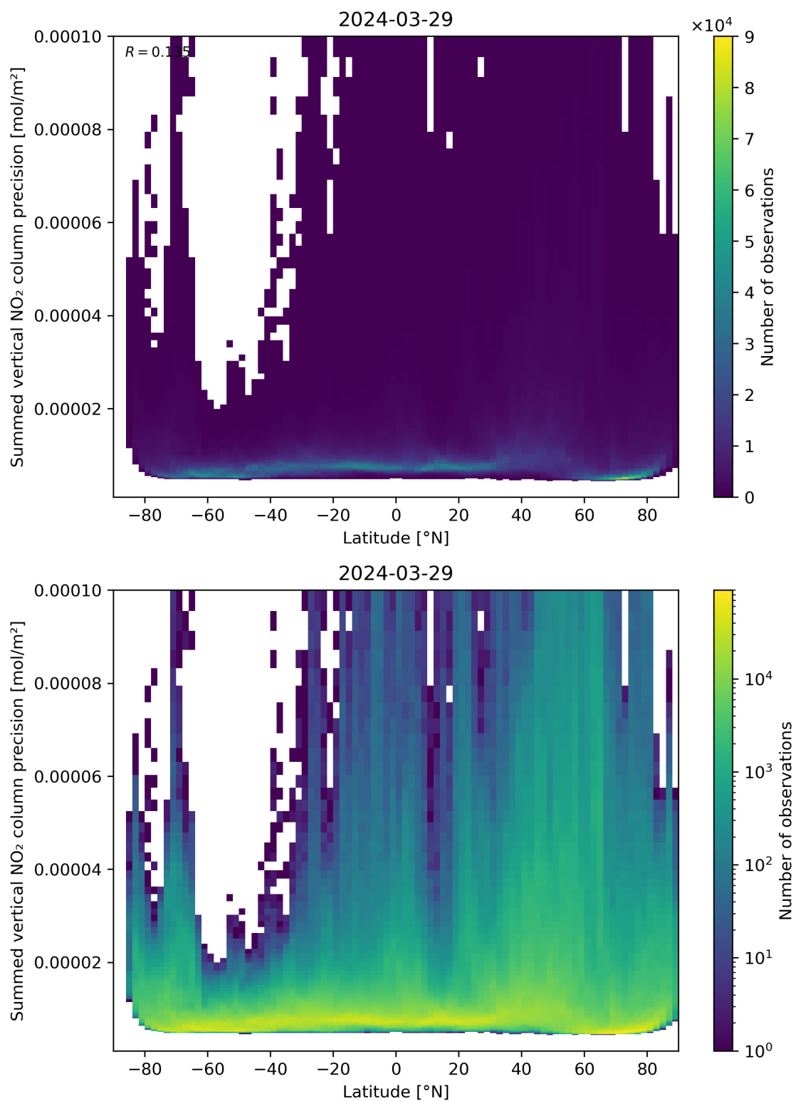
Figure 89: Scatter density plot of “Latitude” against “Summed vertical NO 2 column precision” for 2024-03-28 to 2024-03-30.
