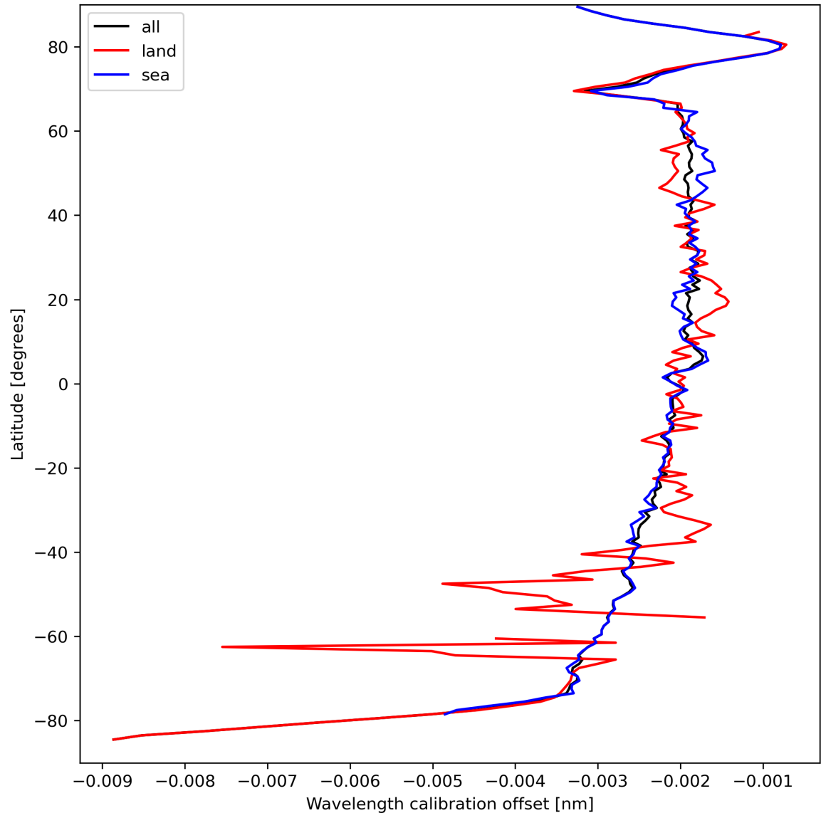
Figure 18: Zonal average of “Wavelength calibration offset” for 2024-03-28 to 2024-03-30.
