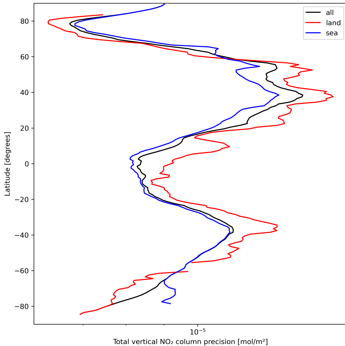
Figure 22: Zonal average of “Total vertical NO 2 column precision” for 2024-03-28 to 2024-03-30.
