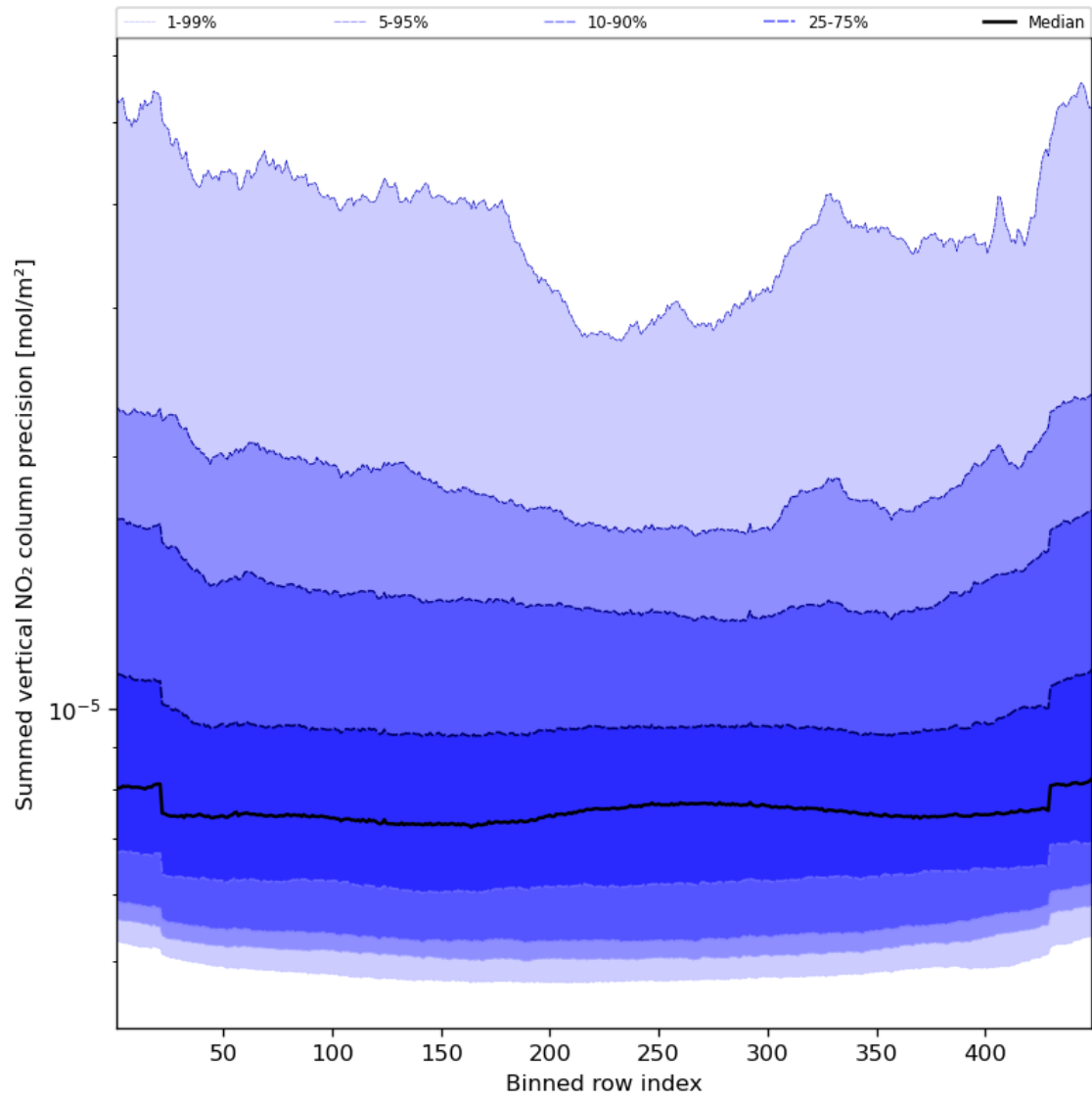
Figure 58: Along track statistics of “Summed vertical NO 2 column precision” for 2024-03-28 to 2024-03-30
