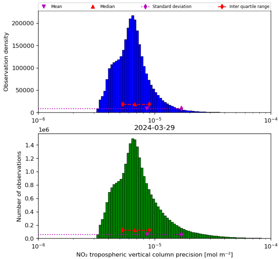
Figure 30: Histogram of “NO 2 tropospheric vertical column precision” for 2024-03-28 to 2024-03-30
