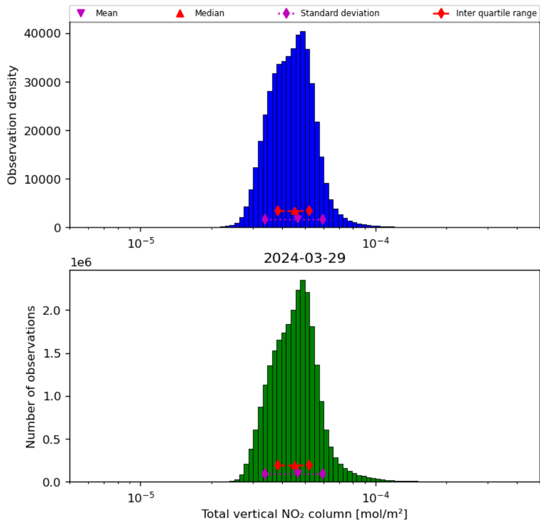
Figure 38: Histogram of "Total vertical NO 2 column" for 2024-03-28 to 2024-03-30
