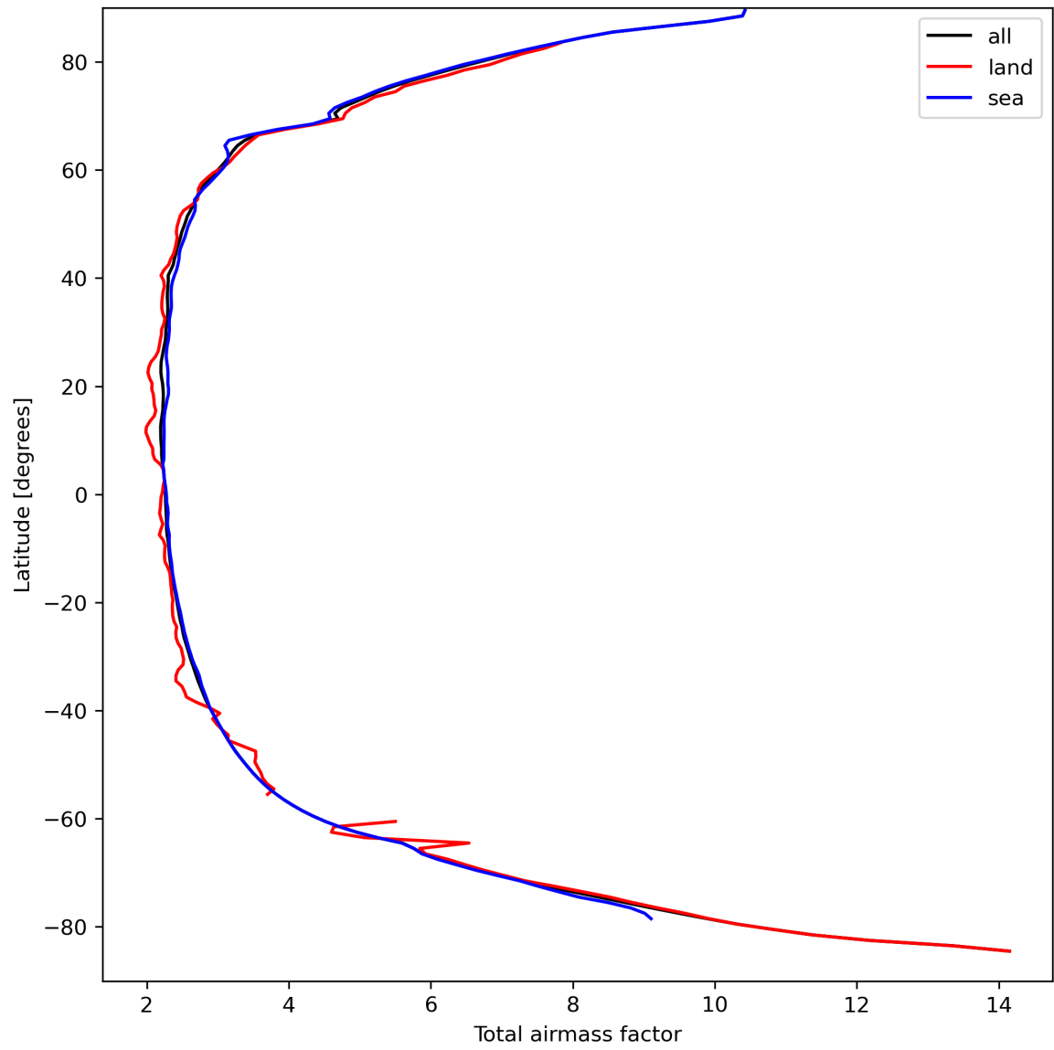
Figure 15: Zonal average of “Total airmass factor” for 2024-03-28 to 2024-03-30.
