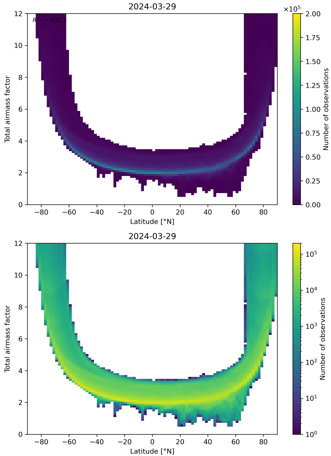
Figure 84: Scatter density plot of “Latitude” against “Total airmass factor” for 2024-03-28 to 2024-03-30.
