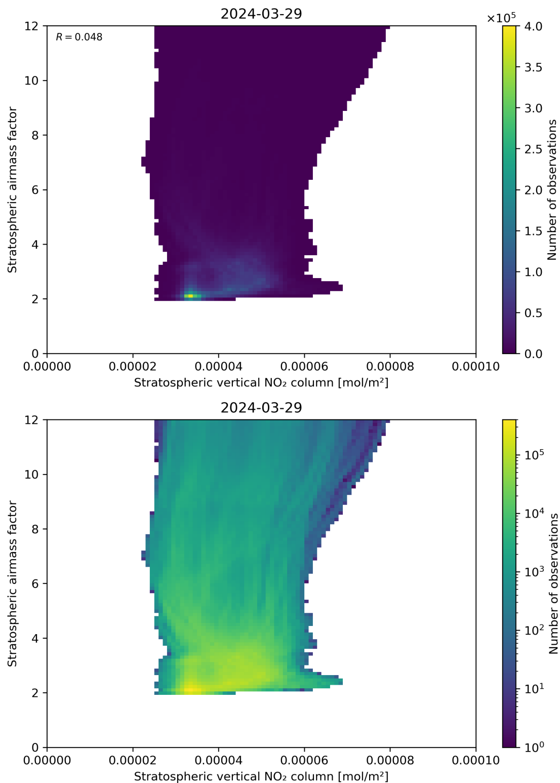
Figure 96: Scatter density plot of “Stratospheric vertical NO 2 column” against “Stratospheric airmass factor” for 2024-03-28 to 2024-03-30.
