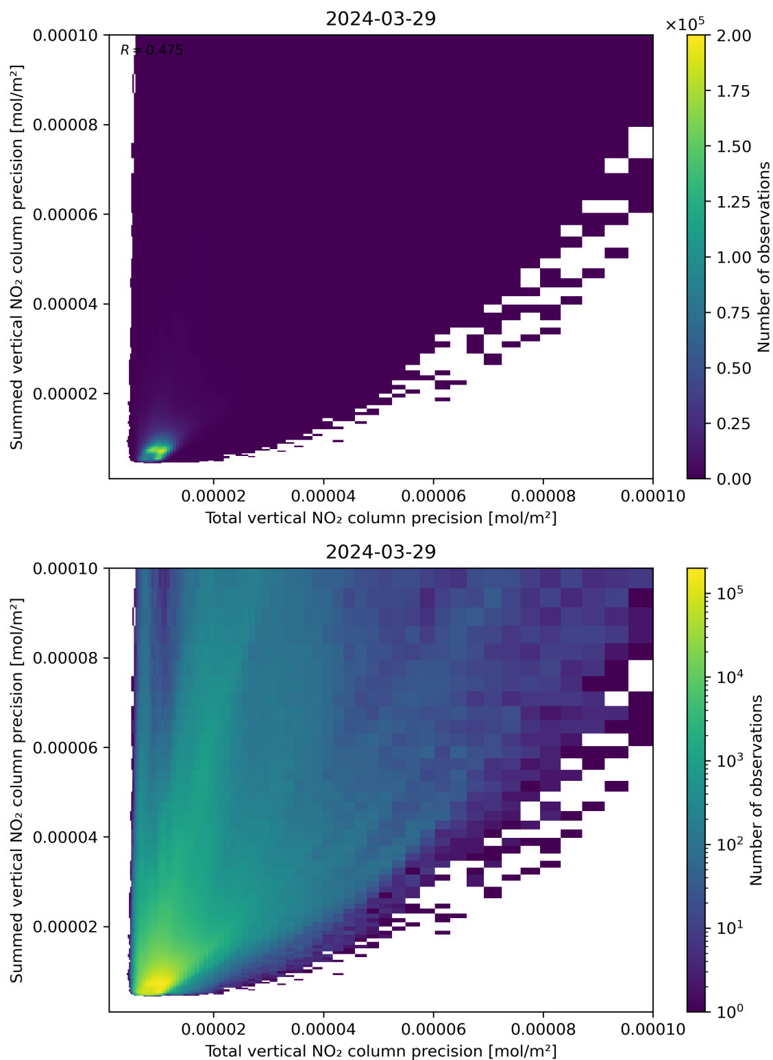
Figure 118: Scatter density plot of “Total vertical NO 2 column precision” against “Summed vertical NO 2 column precision” for 2024-03-28 to 2024-03-30.
