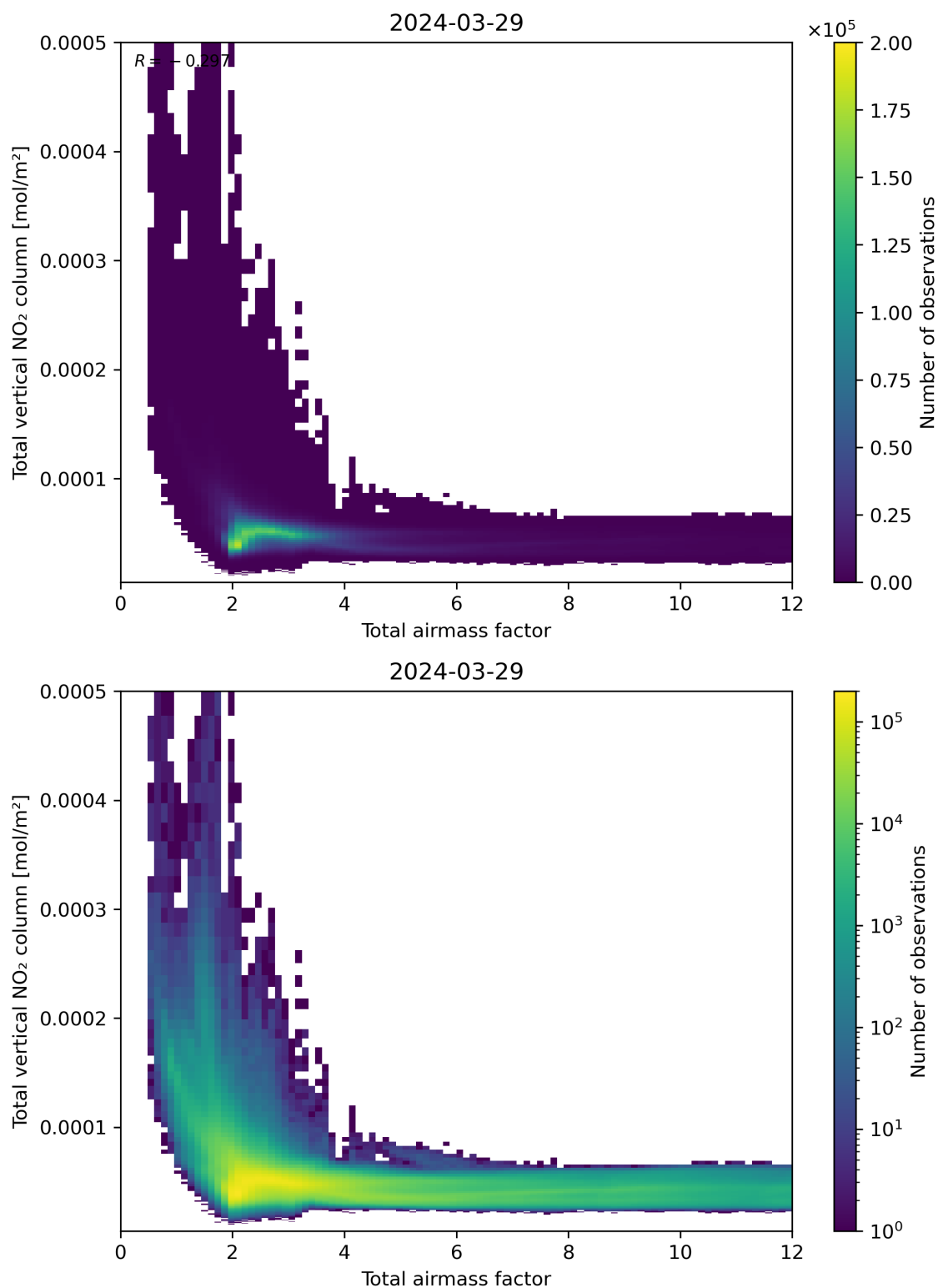
Figure 67: Scatter density plot of “Total airmass factor” against “Total vertical NO 2 column” for 2024-03-28 to 2024-03-30.
