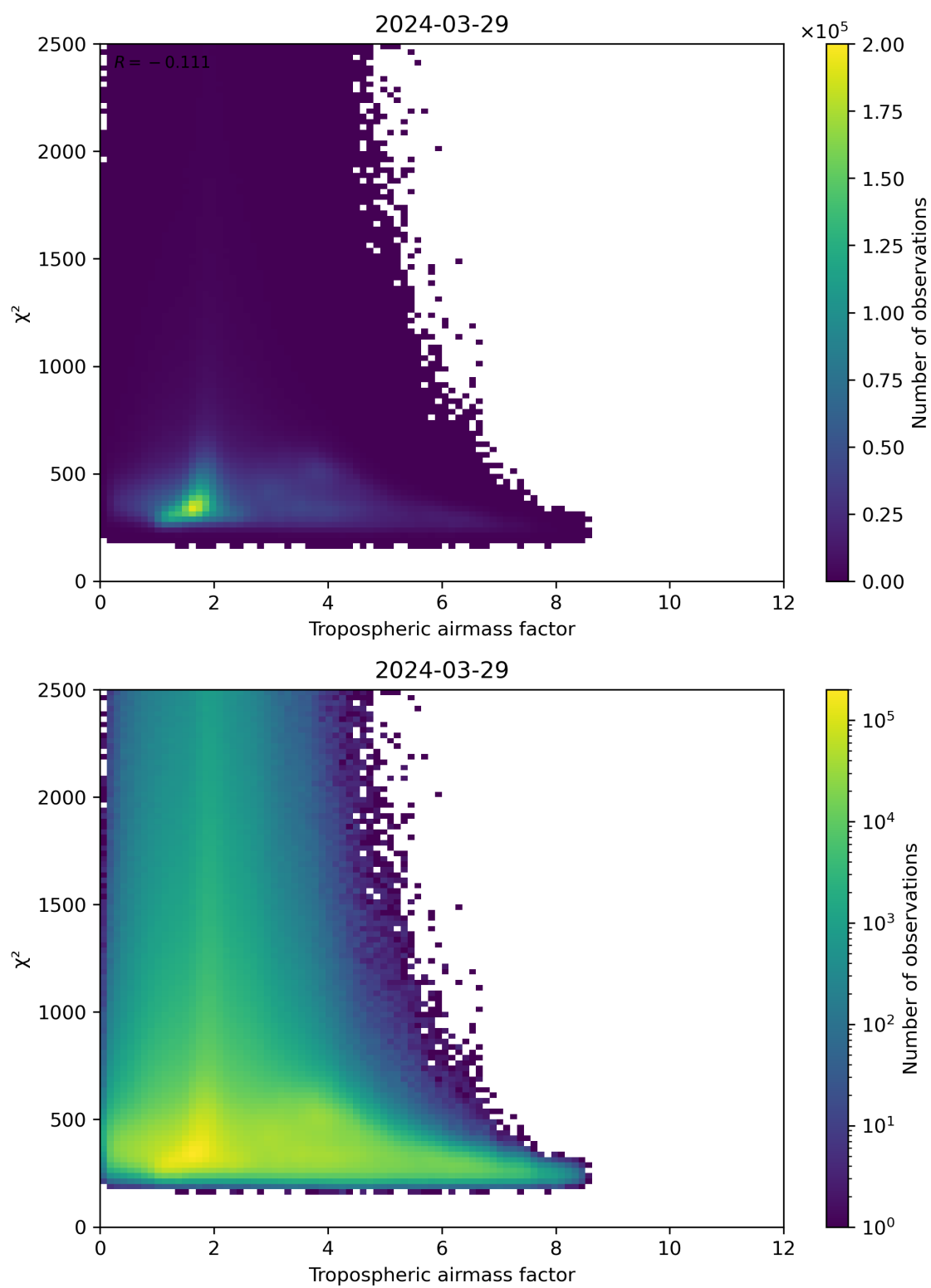
Figure 73: Scatter density plot of “Tropospheric airmass factor” against “ \chi^2 ” for 2024-03-28 to 2024-03-30.
