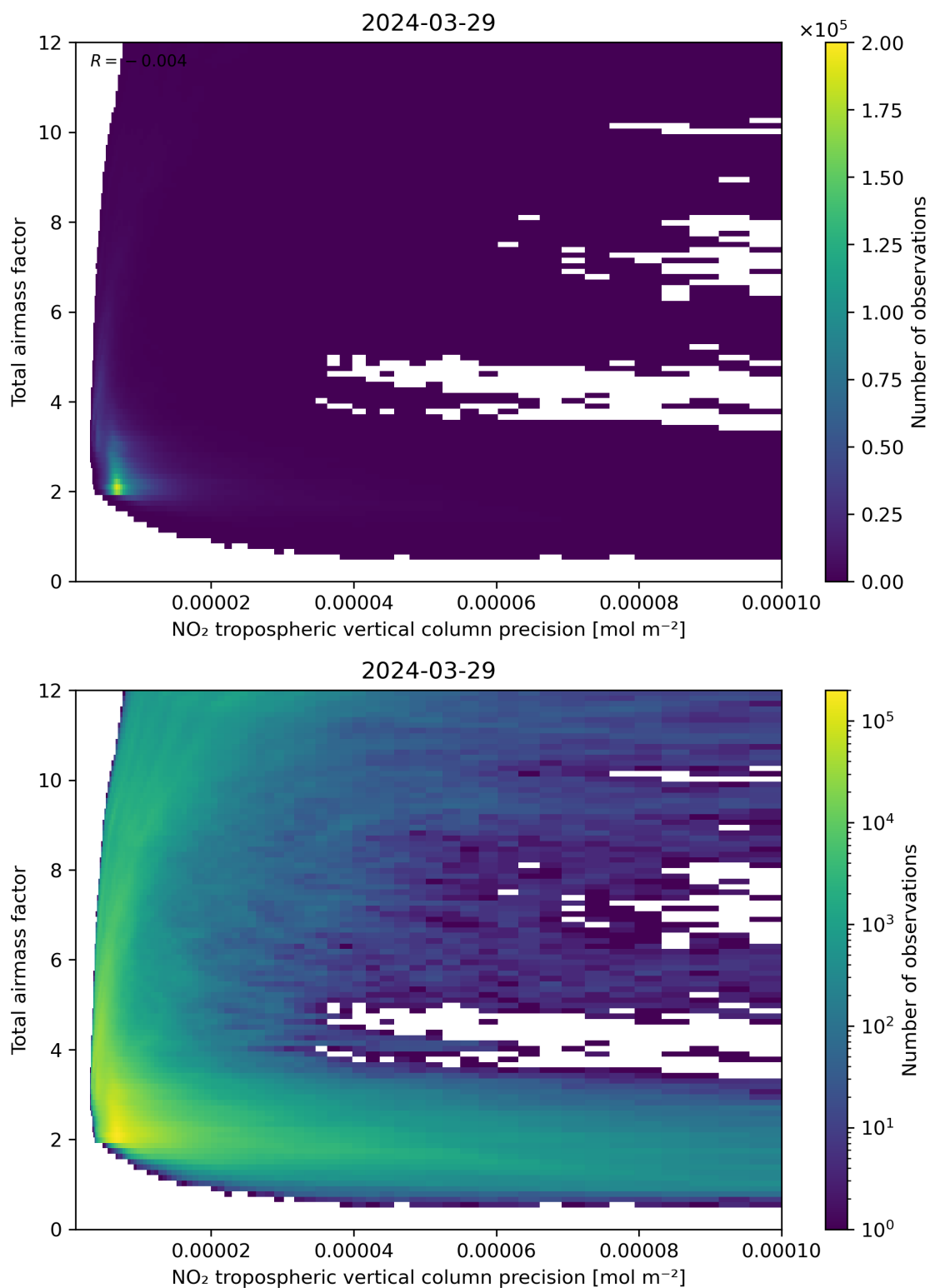
Figure 132: Scatter density plot of “NO 2 tropospheric vertical column precision” against “Total air mass factor” for 2024-03-28 to 2024-03-30.
