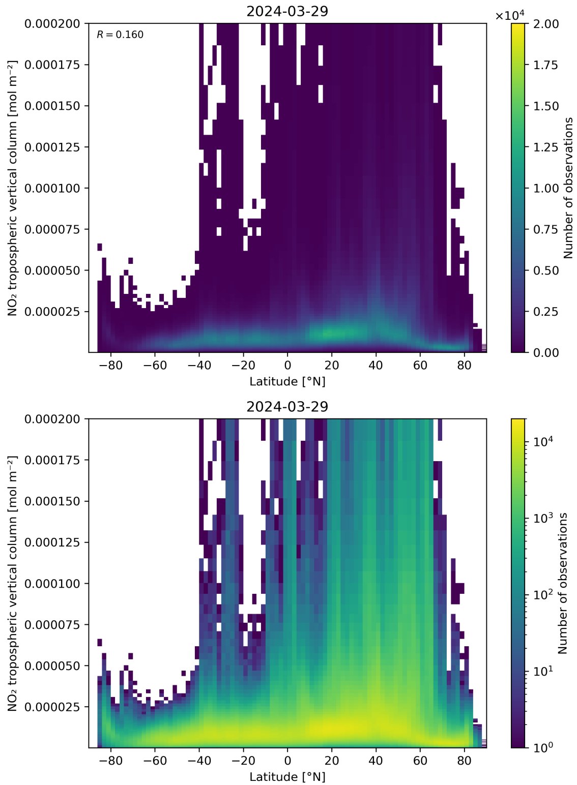
Figure 92: Scatter density plot of “Latitude” against “NO 2 tropospheric vertical column” for 2024-03-28 to 2024-03-30.
