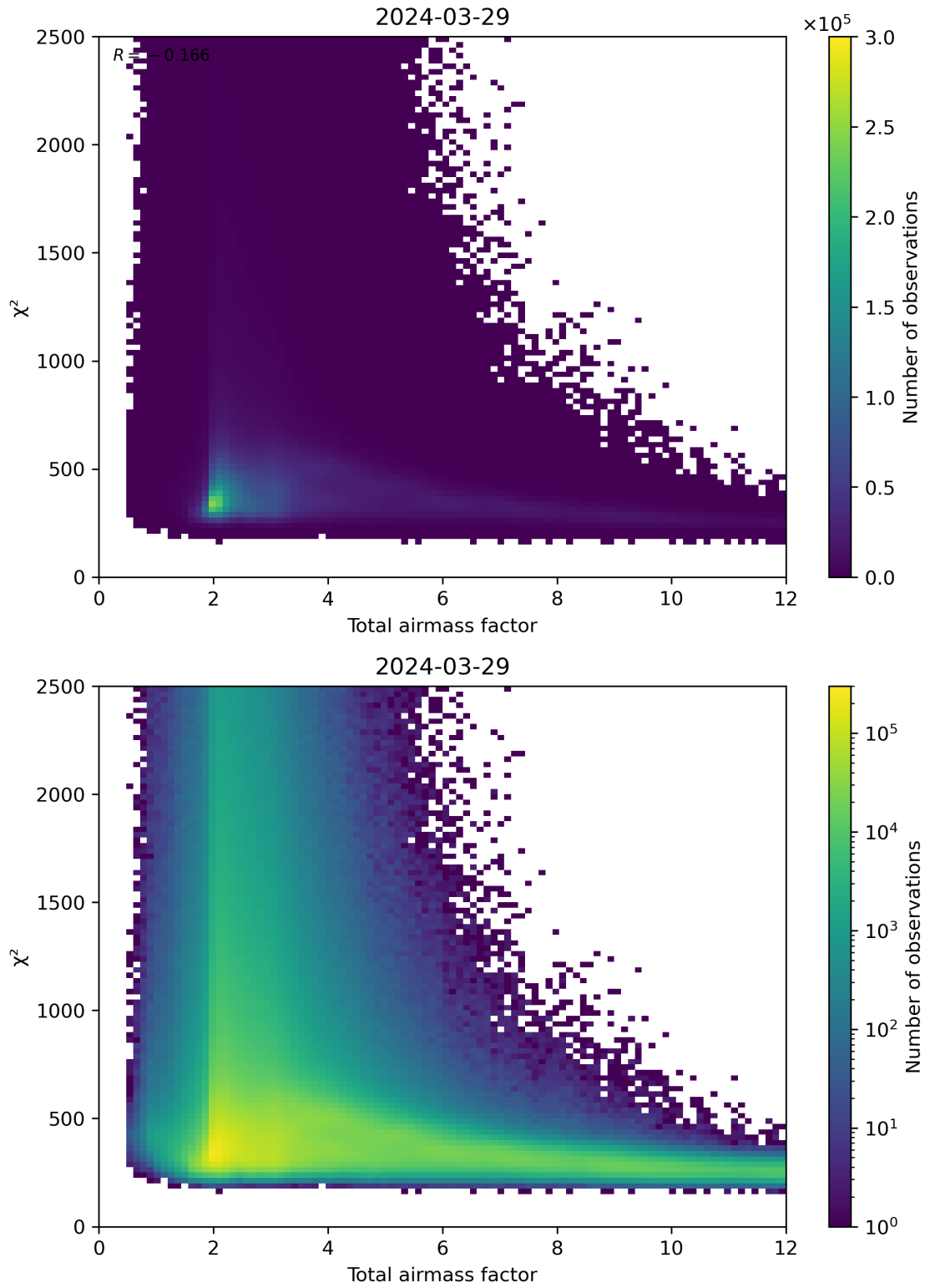
Figure 63: Scatter density plot of “Total airmass factor” against “ \chi^2 ” for 2024-03-28 to 2024-03-30.
