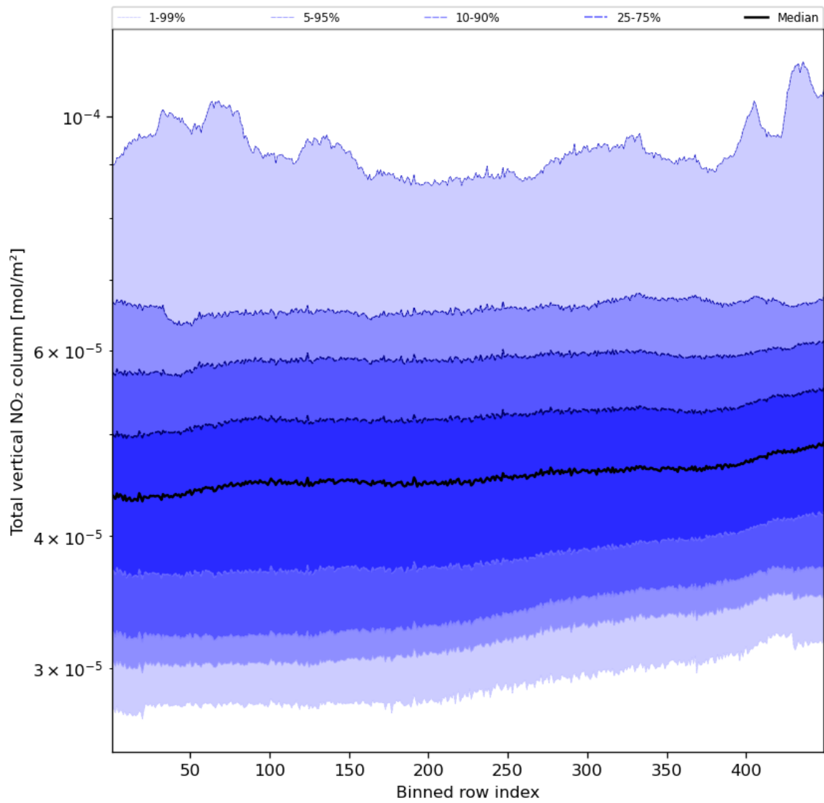
Figure 55: Along track statistics of “Total vertical NO 2 column” for 2024-03-28 to 2024-03-30
