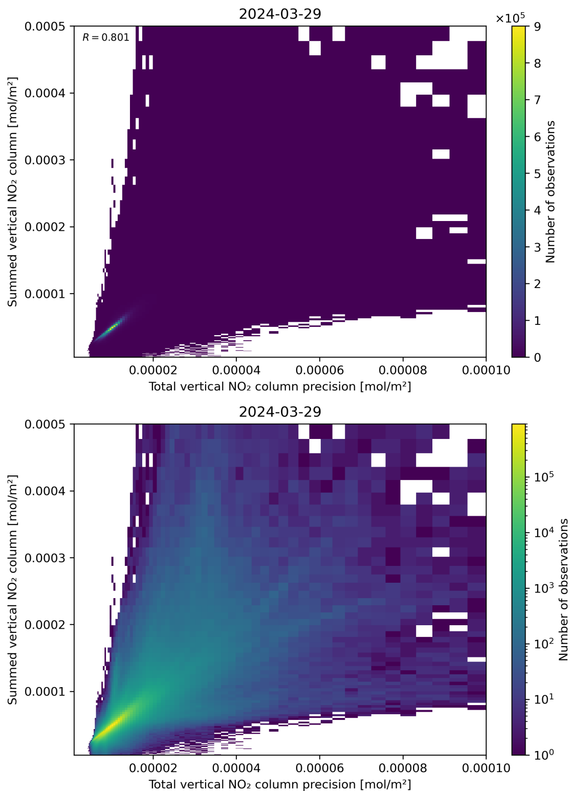
Figure 117: Scatter density plot of “Total vertical NO 2 column precision” against “Summed vertical NO 2 column” for 2024-03-28 to 2024-03-30.
