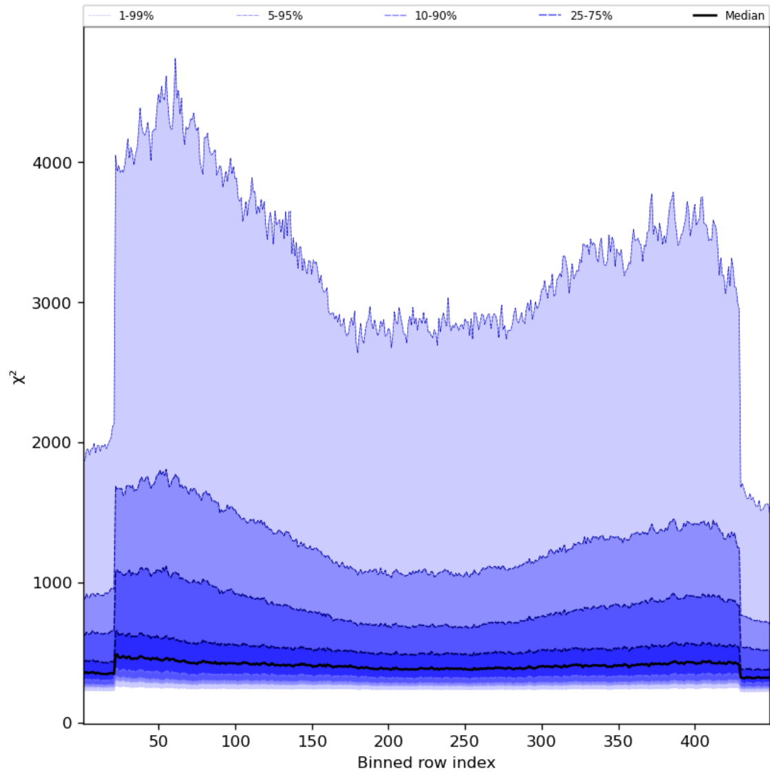
Figure 59: Along track statistics of “ \chi^2 ” for 2024-03-28 to 2024-03-30
