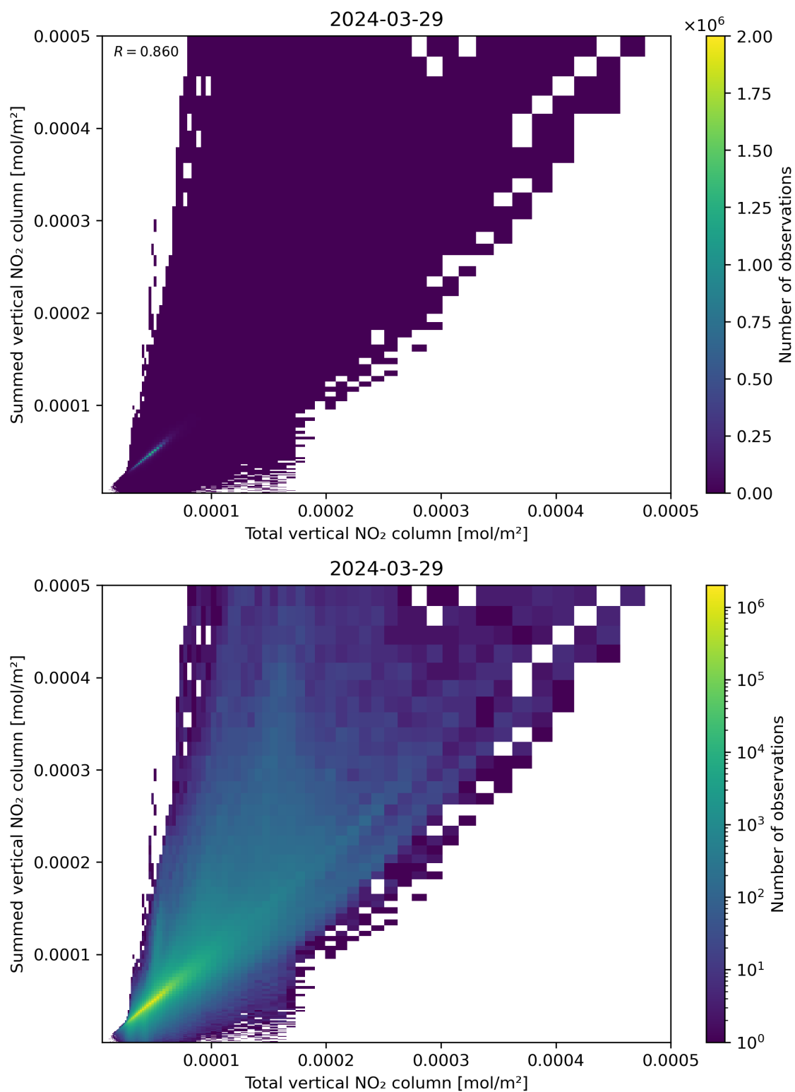
Figure 112: Scatter density plot of “Total vertical NO 2 column” against “Summed vertical NO 2 column” for 2024-03-28 to 2024-03-30.
