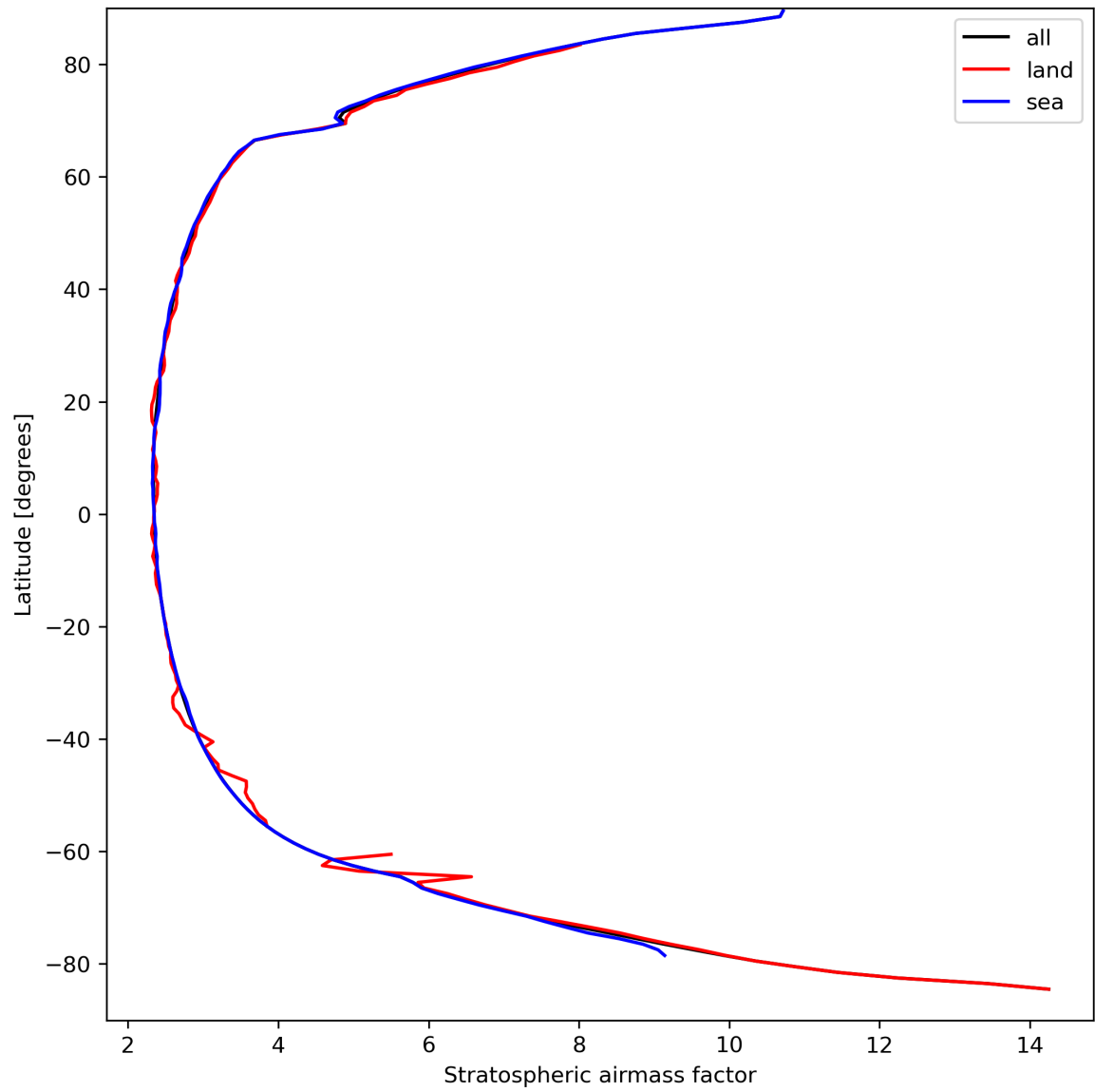
Figure 27: Zonal average of “Stratospheric air mass factor” for 2024-03-28 to 2024-03-30.
