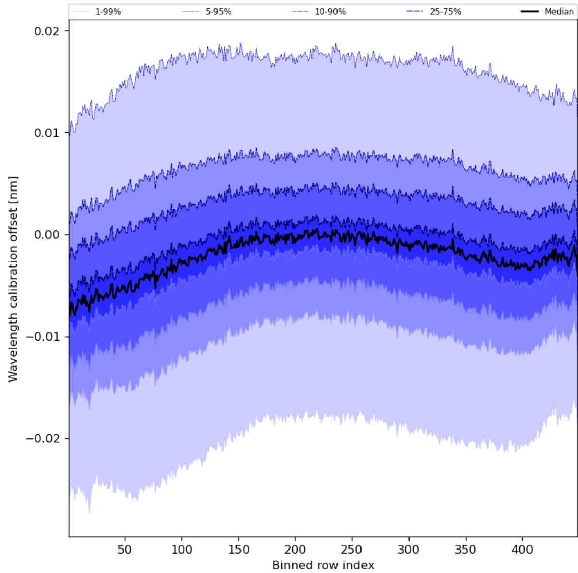
Figure 52: Along track statistics of “Wavelength calibration offset” for 2024-03-28 to 2024-03-30
