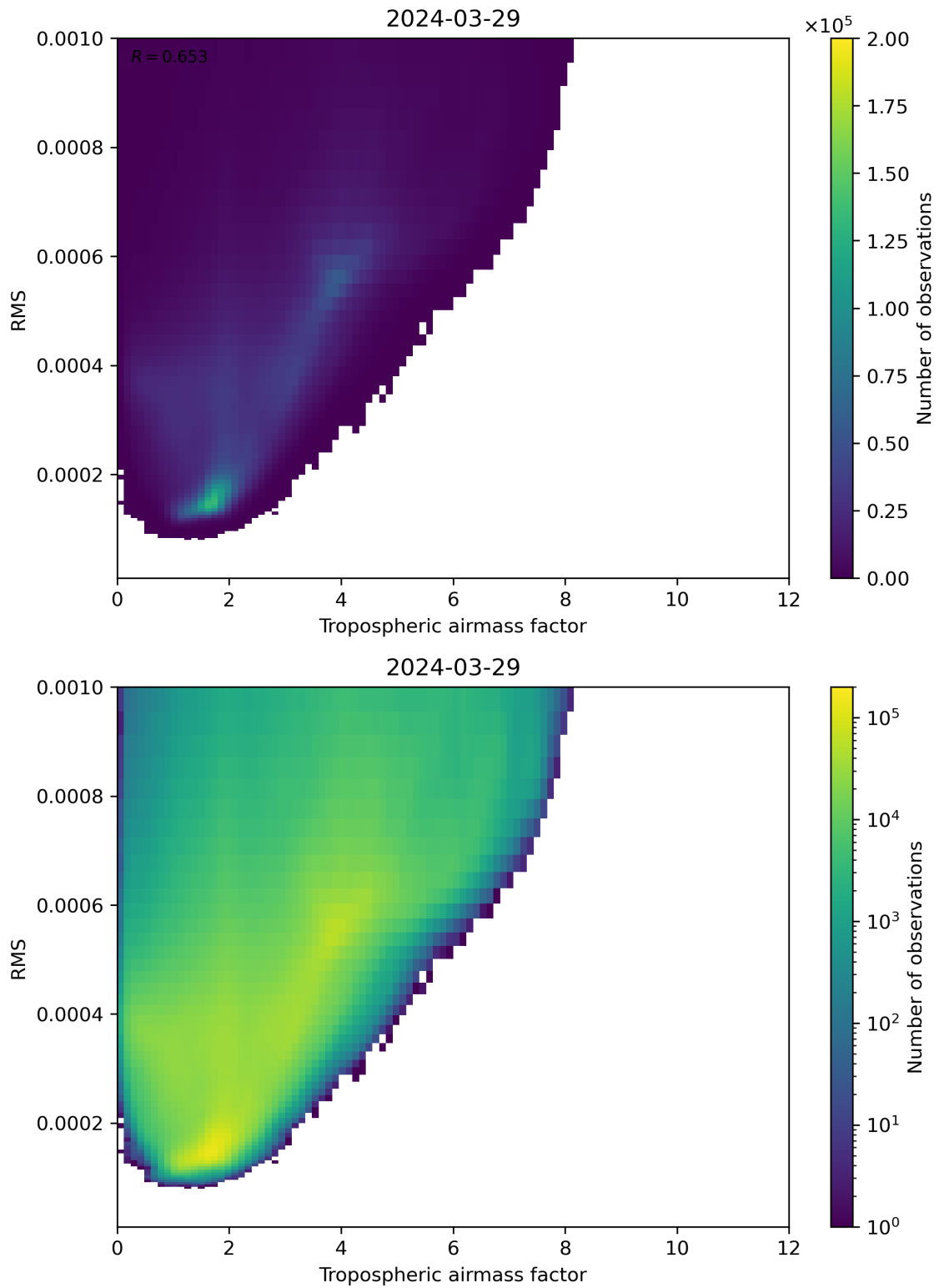
Figure 79: Scatter density plot of “Tropospheric airmass factor” against “RMS” for 2024-03-28 to 2024-03-30.
