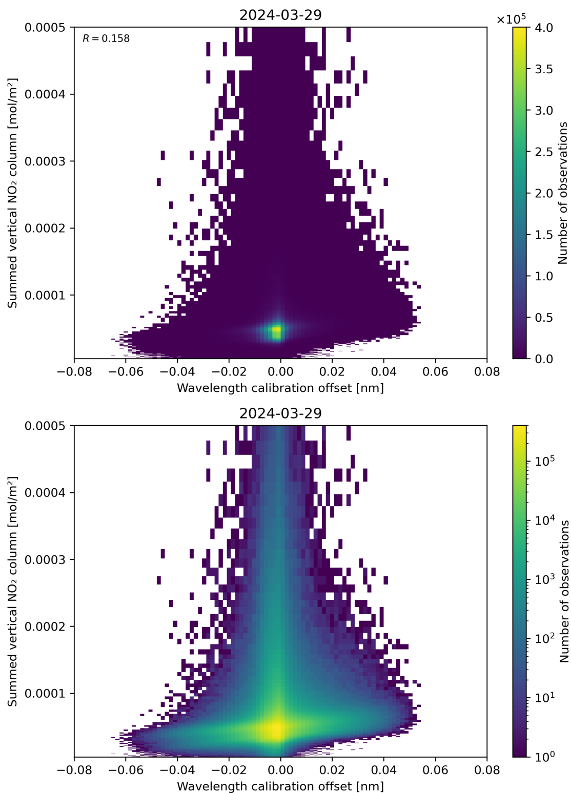
Figure 177: Scatter density plot of “Wavelength calibration offset” against “Summed vertical NO 2 column” for 2024-03-28 to 2024-03-30.
