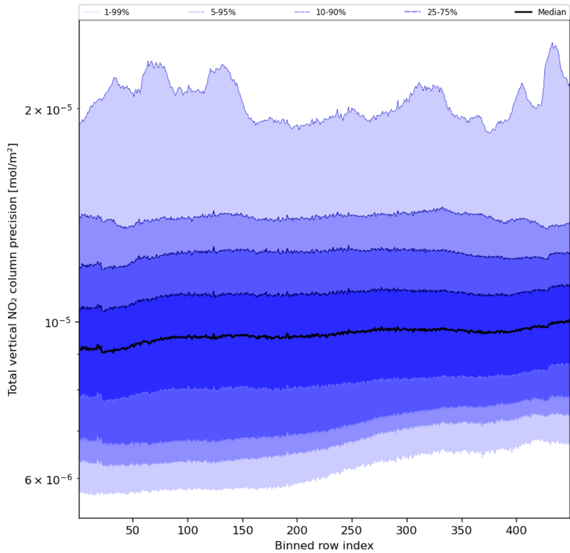
Figure 56: Along track statistics of “Total vertical NO 2 column precision” for 2024-03-28 to 2024-03-30
