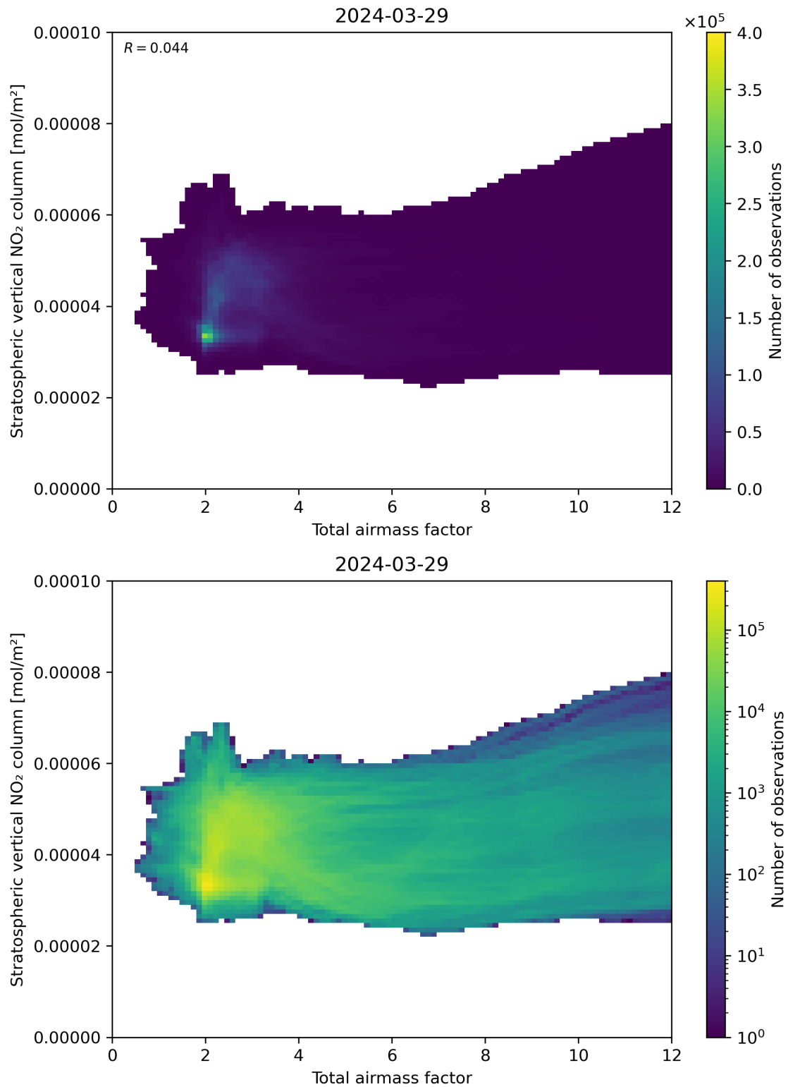
Figure 64: Scatter density plot of “Total airmass factor” against “Stratospheric vertical NO 2 column” for 2024-03-28 to 2024-03-30.
