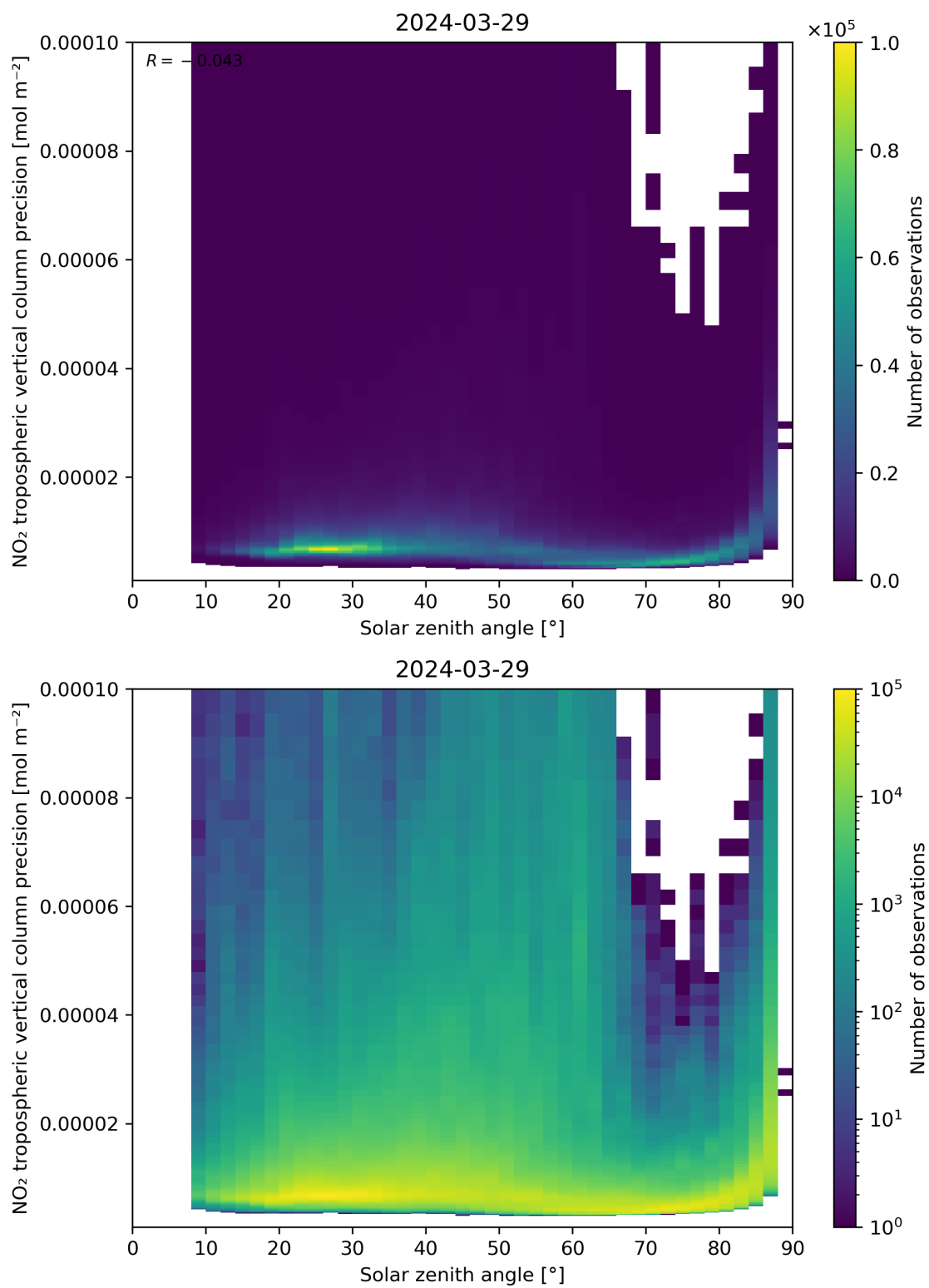
Figure 156: Scatter density plot of “Solar zenith angle” against “NO 2 tropospheric vertical column precision” for 2024-03-28 to 2024-03-30.
