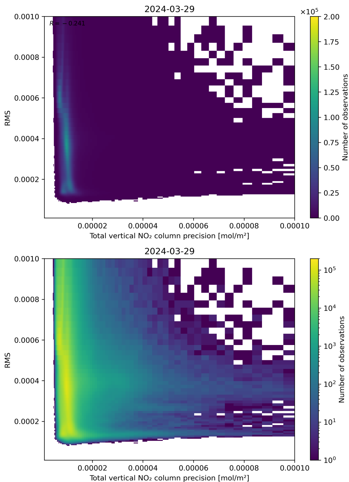
Figure 119: Scatter density plot of “Total vertical NO 2 column precision” against “RMS” for 2024-03-28 to 2024-03-30.
