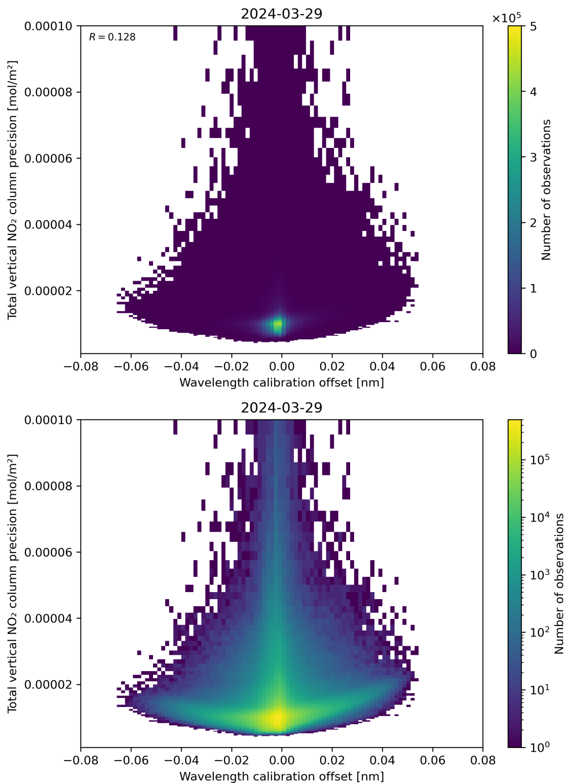
Figure 180: Scatter density plot of “Wavelength calibration offset” against “Total vertical NO 2 column precision” for 2024-03-28 to 2024-03-30.
