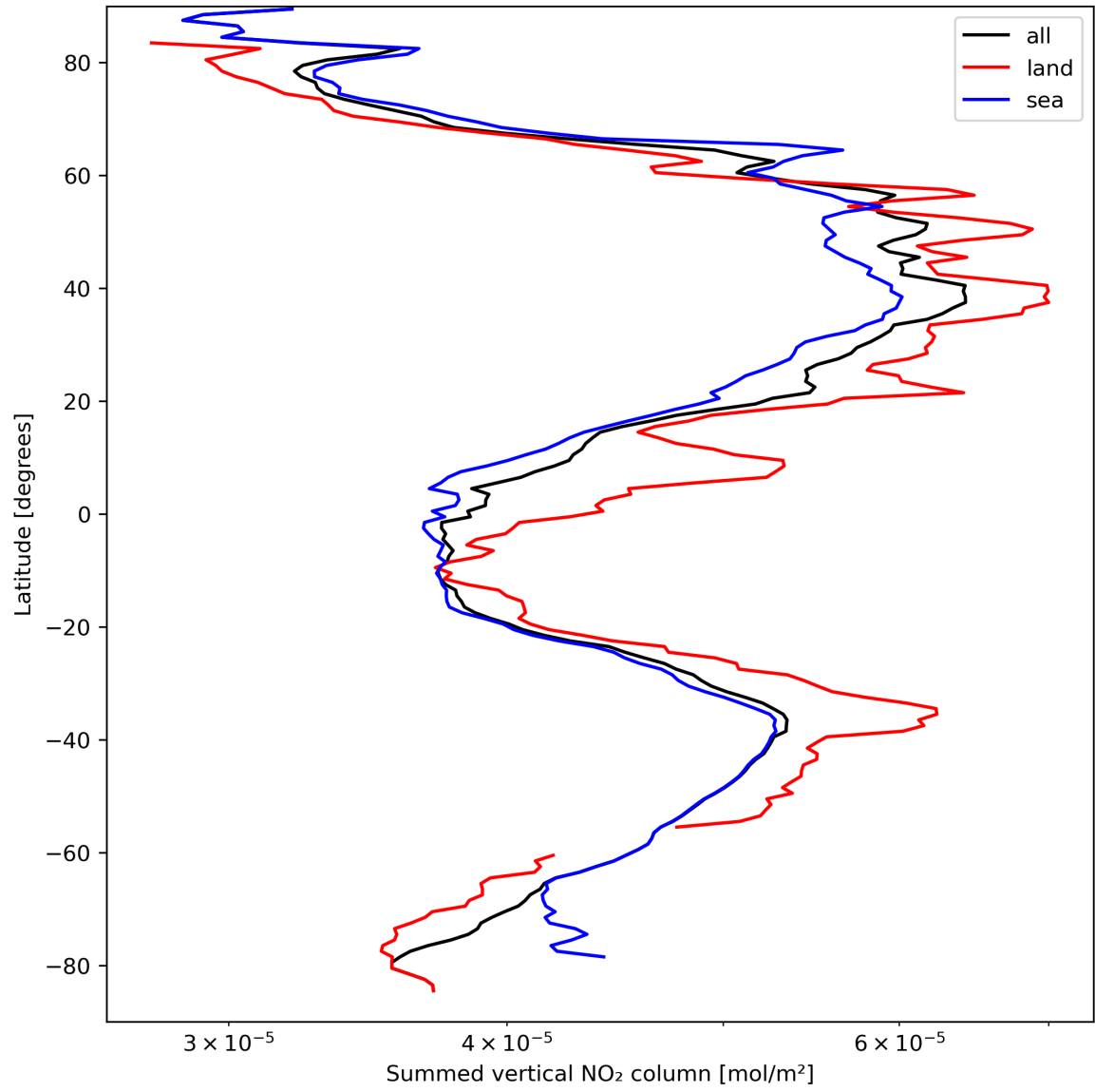
Figure 23: Zonal average of “Summed vertical NO 2 column” for 2024-03-28 to 2024-03-30.
