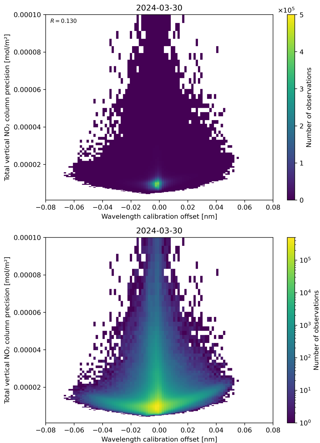
Figure 180: Scatter density plot of “Wavelength calibration offset” against “Total vertical NO 2 column precision” for 2024-03-30 to 2024-03-31.
