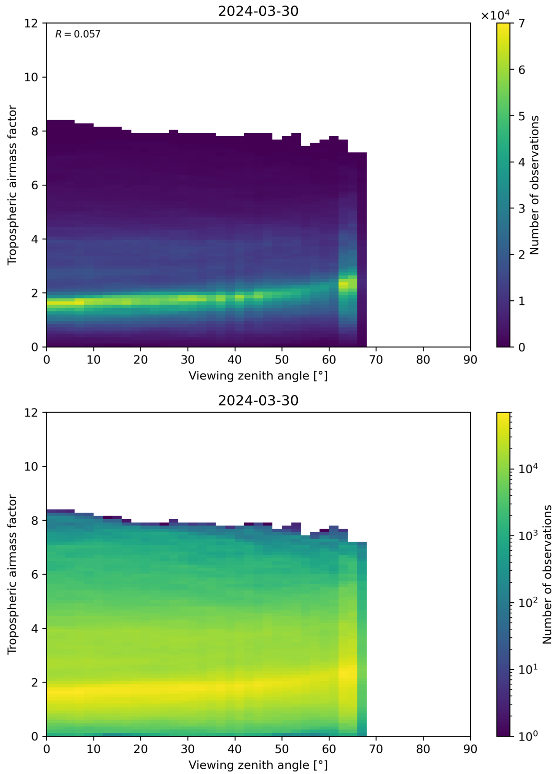
Figure 161: Scatter density plot of “Viewing zenith angle” against “Tropospheric airmass factor” for 2024-03-30 to 2024-03-31.
