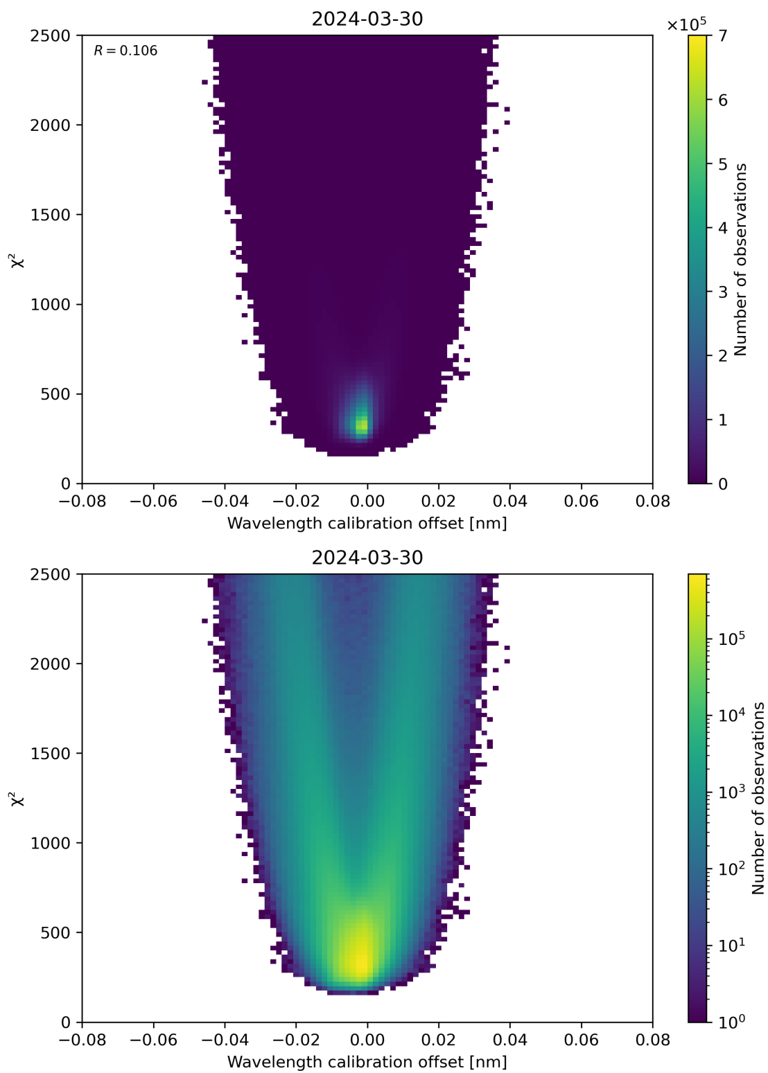
Figure 175: Scatter density plot of “Wavelength calibration offset” against “ \chi^2 ” for 2024-03-30 to 2024-03-31.
