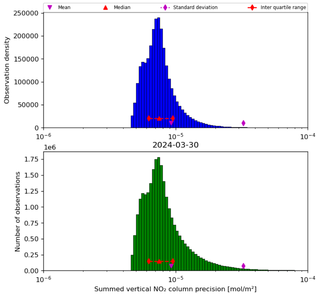
Figure 41: Histogram of “Summed vertical NO 2 column precision” for 2024-03-30 to 2024-03-31
