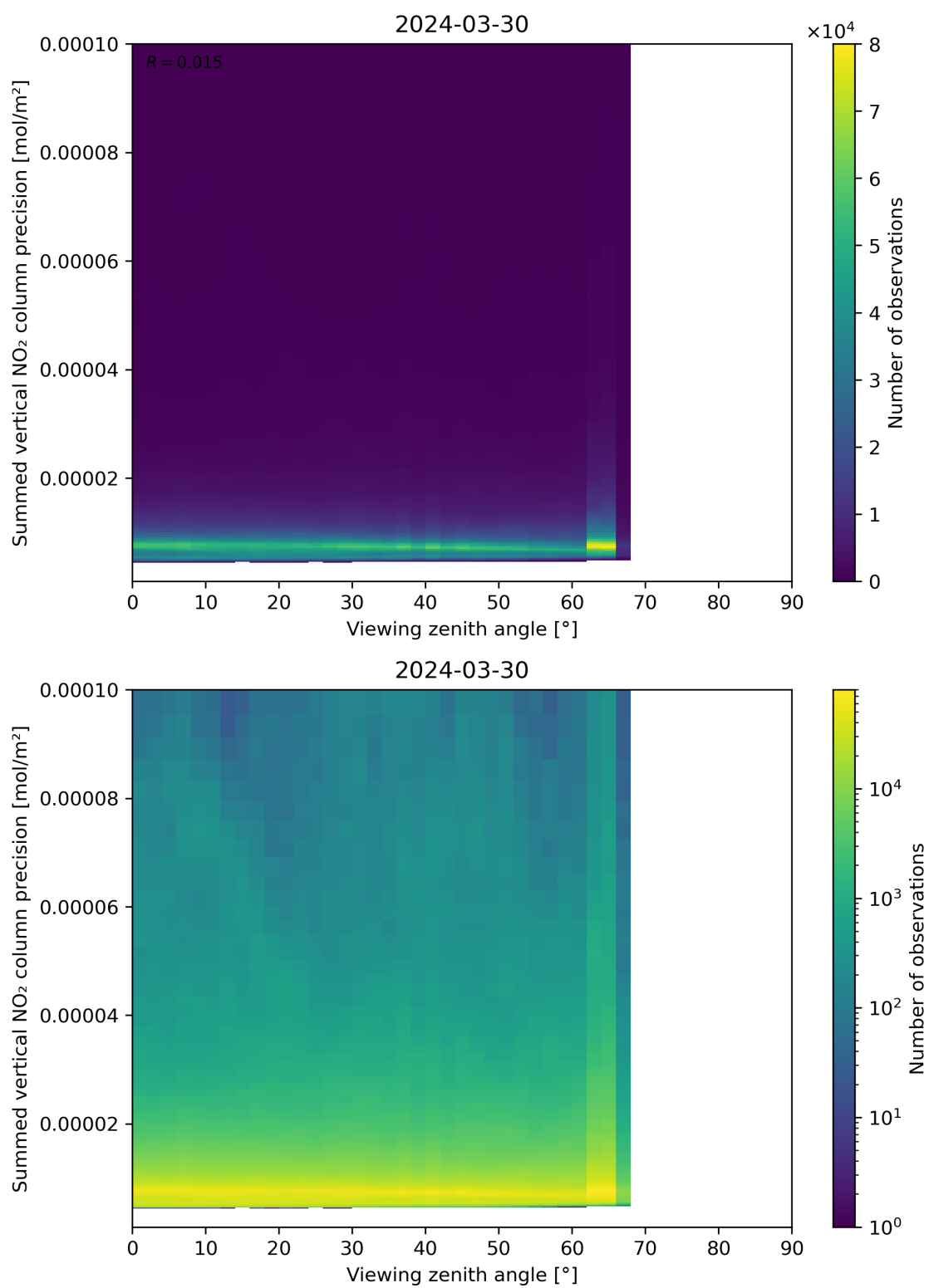
Figure 166: Scatter density plot of “Viewing zenith angle” against “Summed vertical NO 2 column precision” for 2024-03-30 to 2024-03-31.
