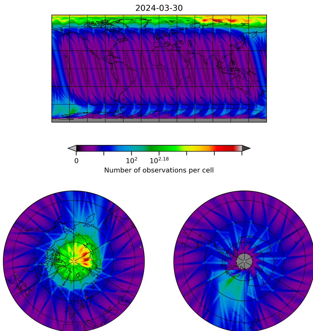
Figure 10: Map of the number of observations for 2024-03-30 to 2024-03-31
