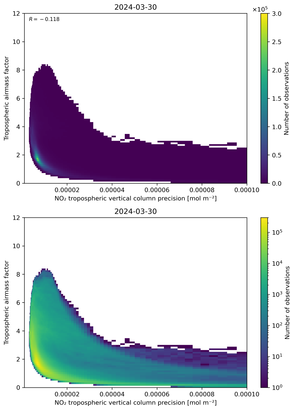
Figure 133: Scatter density plot of “NO 2 tropospheric vertical column precision” against “Tropospheric airmass factor” for 2024-03-30 to 2024-03-31.
