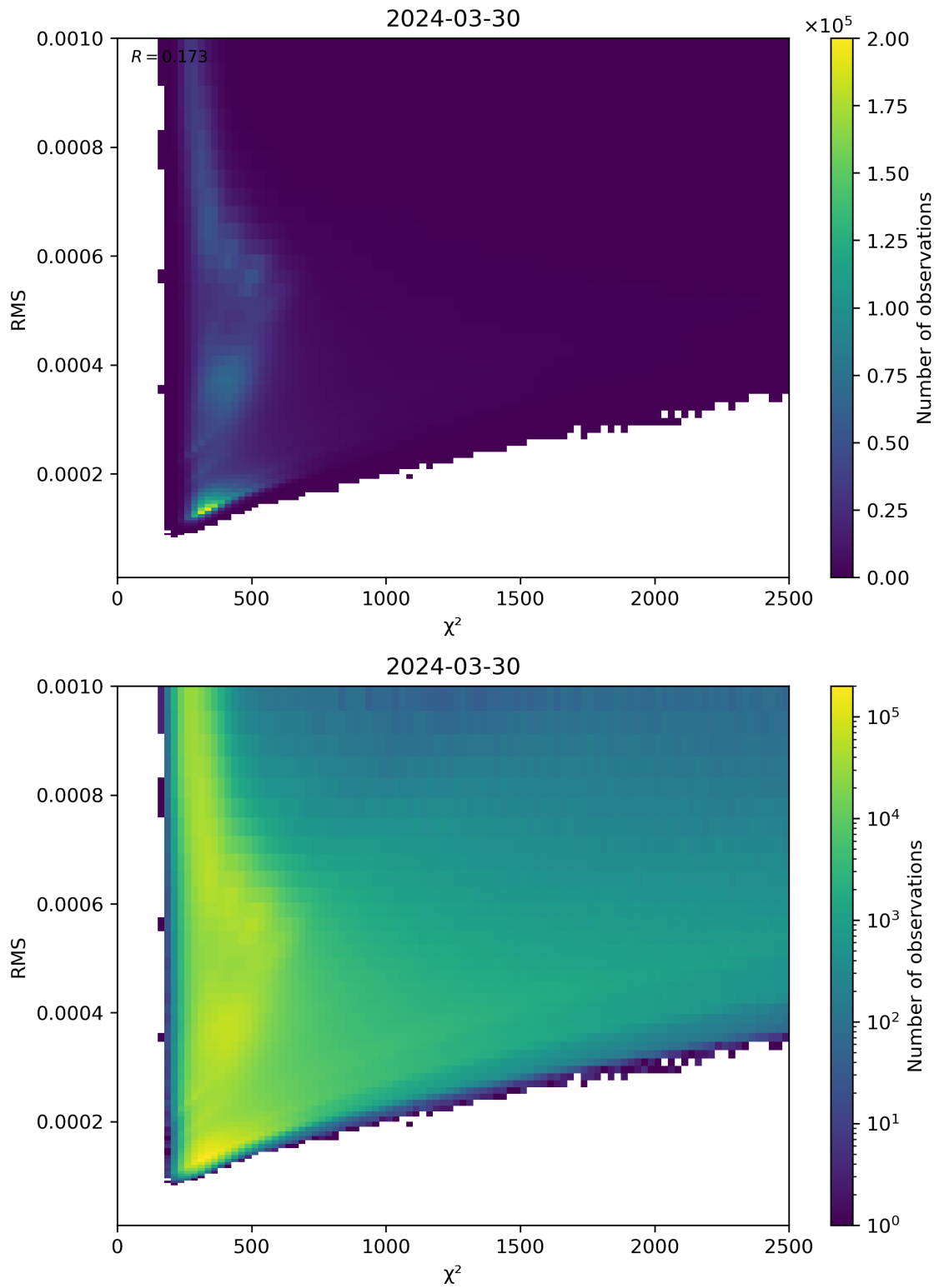
Figure 82: Scatter density plot of “ \chi^2 ” against “RMS” for 2024-03-30 to 2024-03-31.
