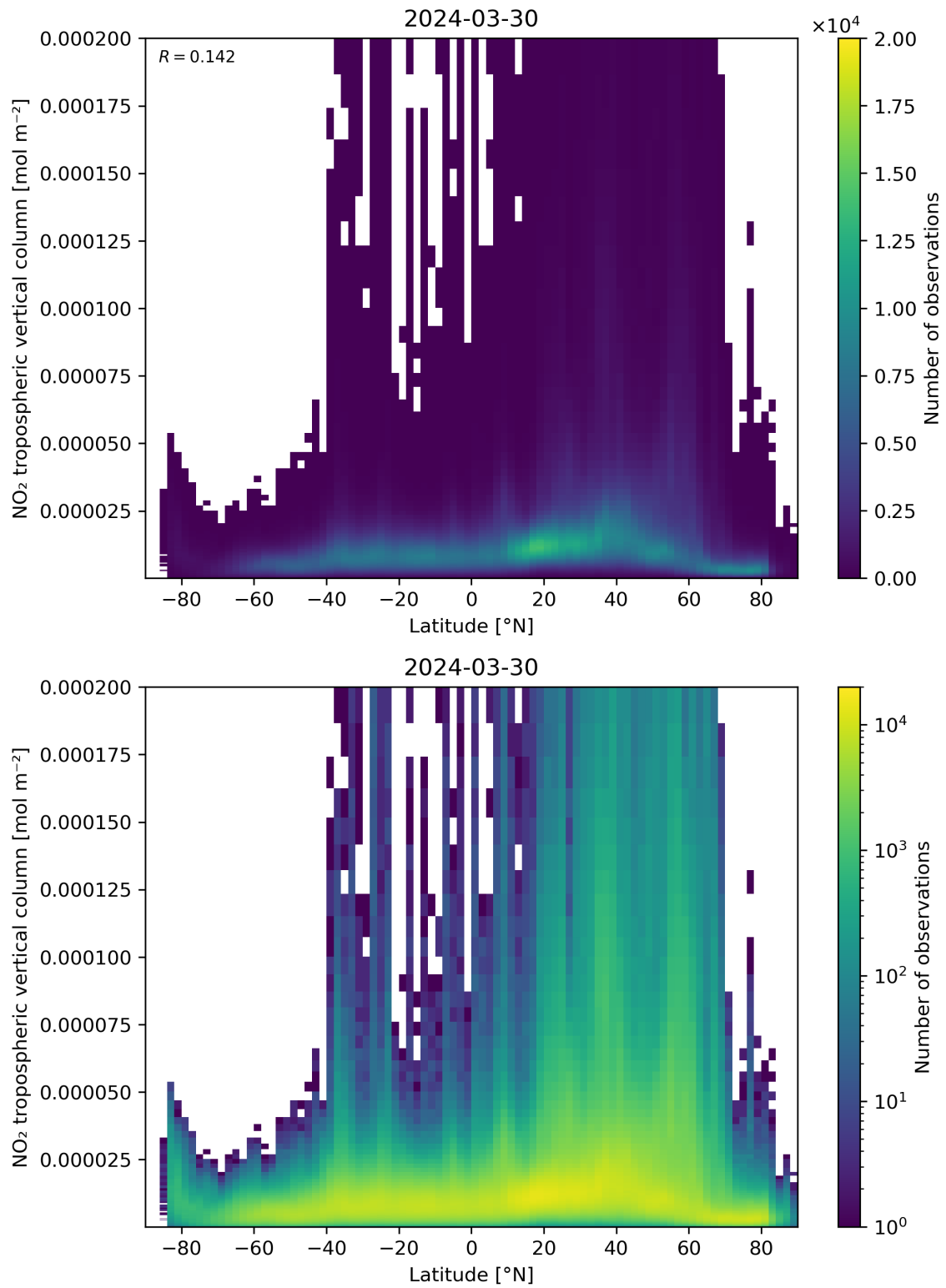
Figure 92: Scatter density plot of “Latitude” against “NO 2 tropospheric vertical column” for 2024-03-30 to 2024-03-31.
