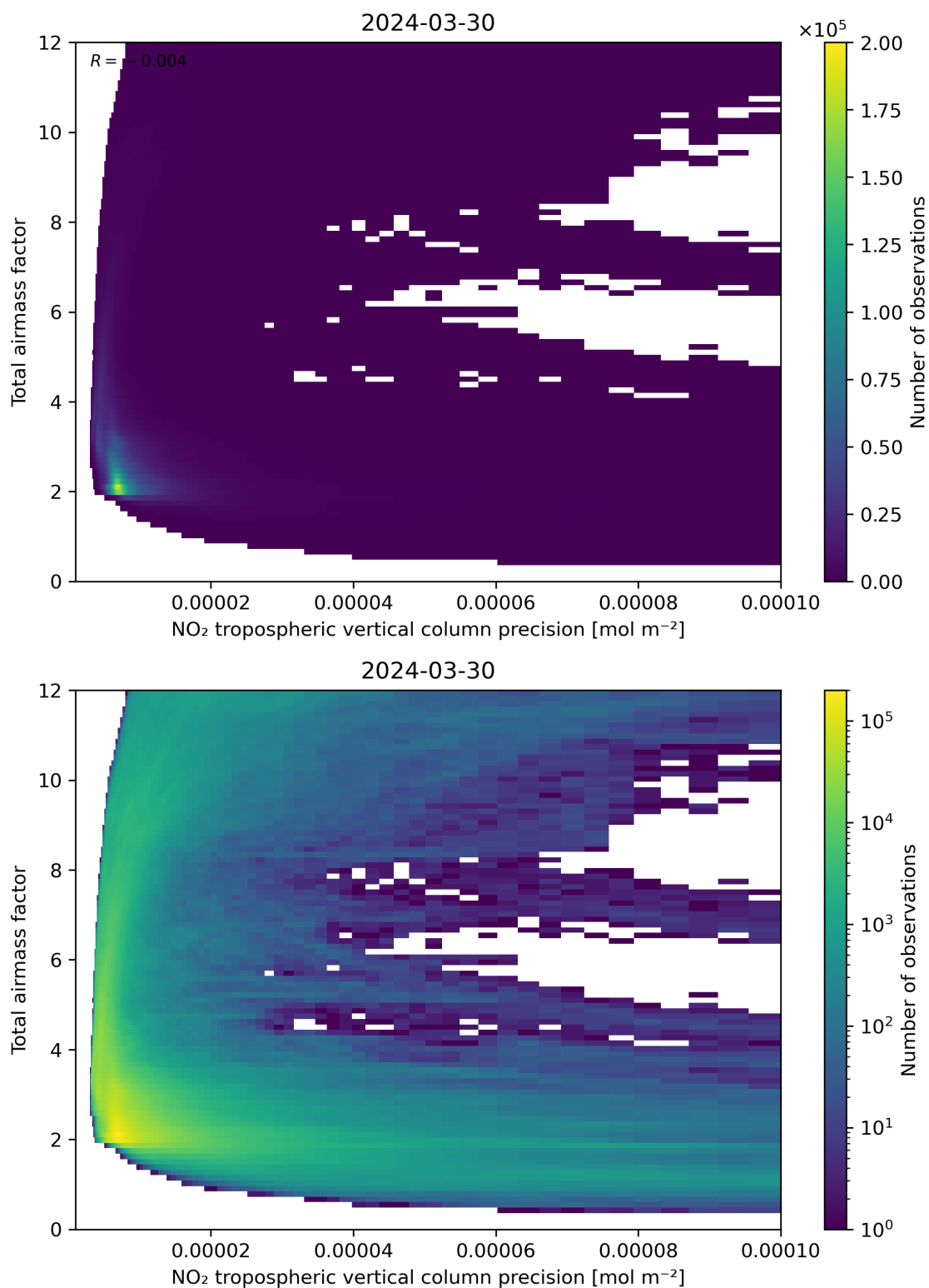
Figure 132: Scatter density plot of “NO 2 tropospheric vertical column precision” against “Total air mass factor” for 2024-03-30 to 2024-03-31.
