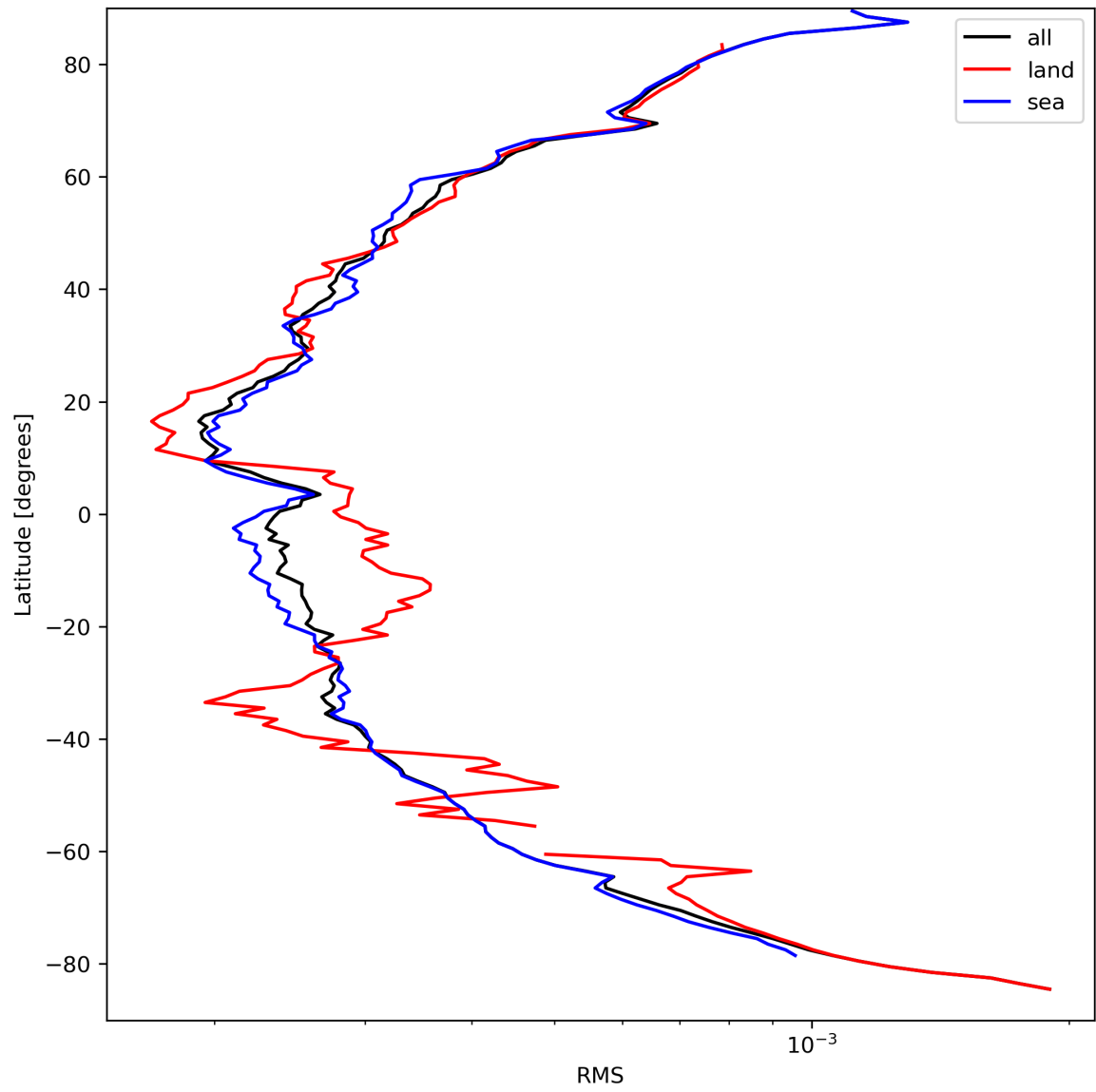
Figure 26: Zonal average of “RMS” for 2024-03-30 to 2024-03-31.
