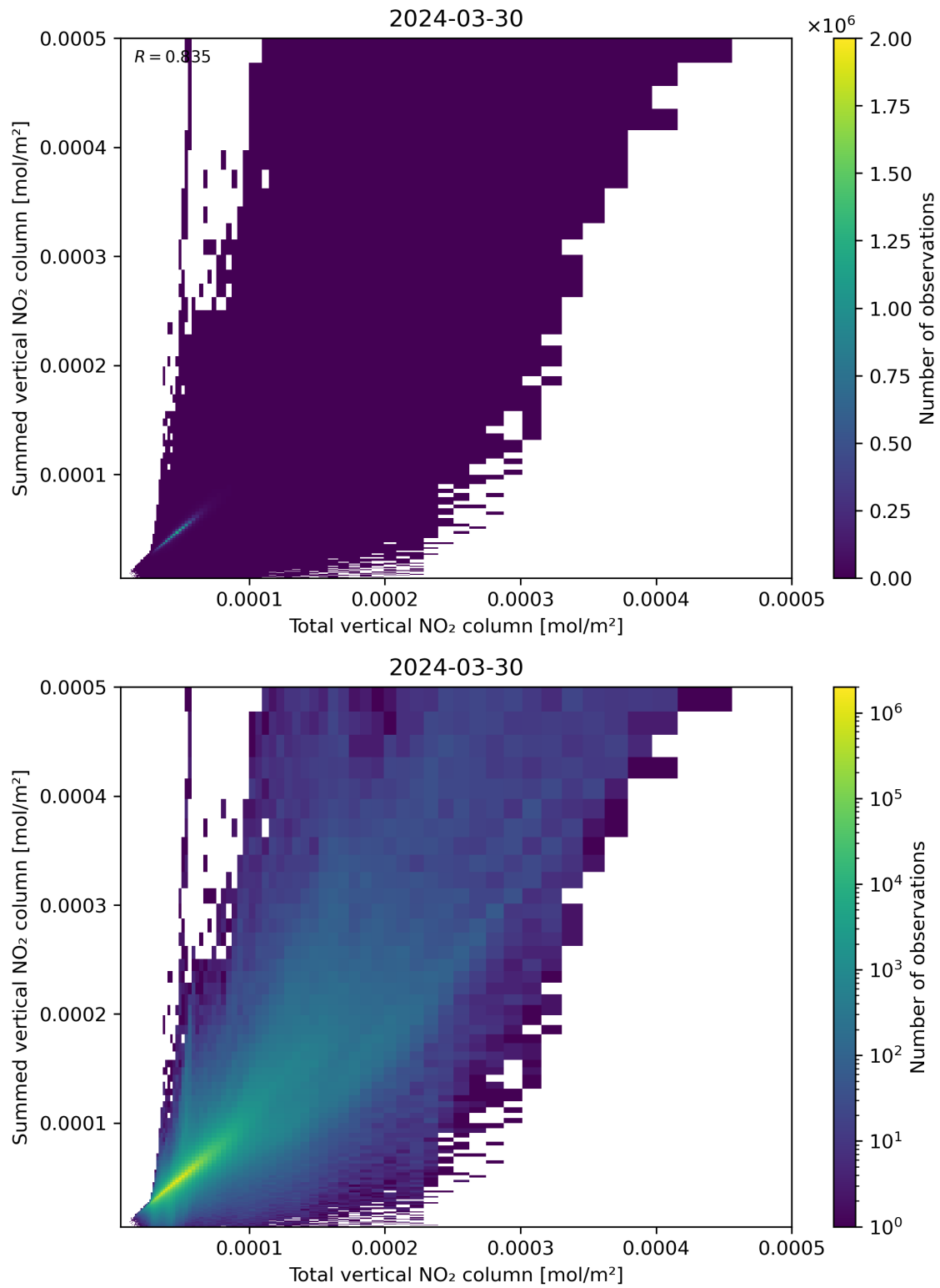
Figure 112: Scatter density plot of “Total vertical NO 2 column” against “Summed vertical NO 2 column” for 2024-03-30 to 2024-03-31.
