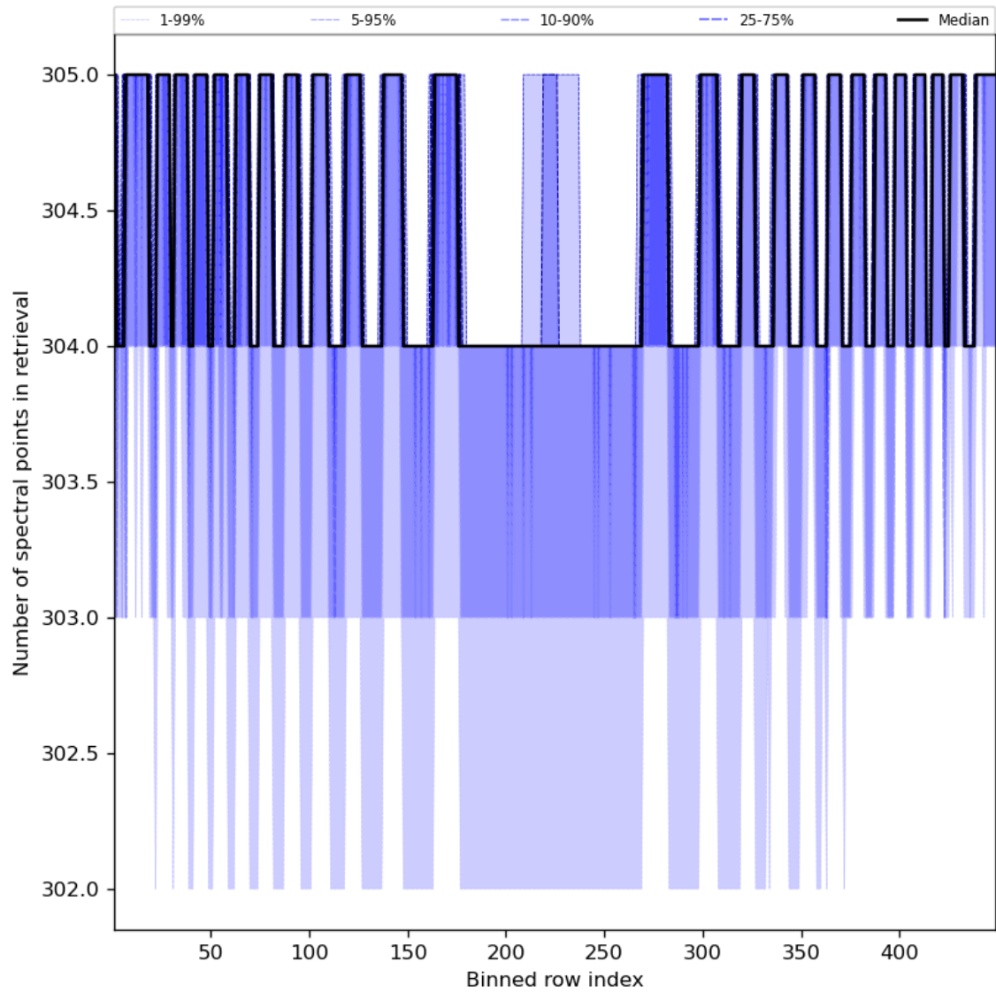
Figure 50: Along track statistics of “Number of spectral points in retrieval” for 2024-03-30 to 2024-03-31
