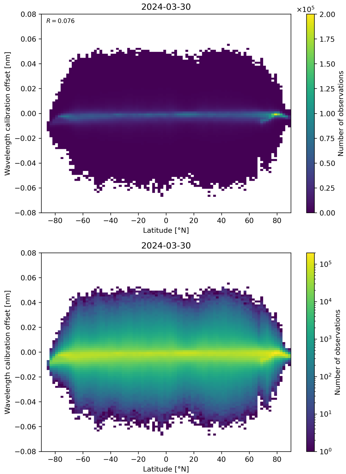
Figure 95: Scatter density plot of “Latitude” against “Wavelength calibration offset” for 2024-03-30 to 2024-03-31.
