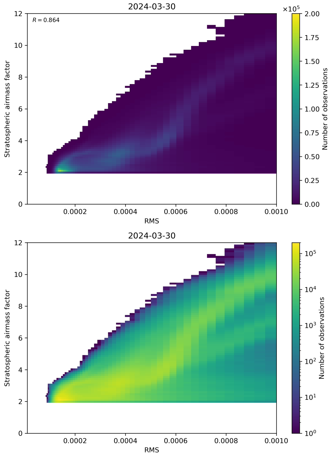
Figure 144: Scatter density plot of “RMS” against “Stratospheric airmass factor” for 2024-03-30 to 2024-03-31.
