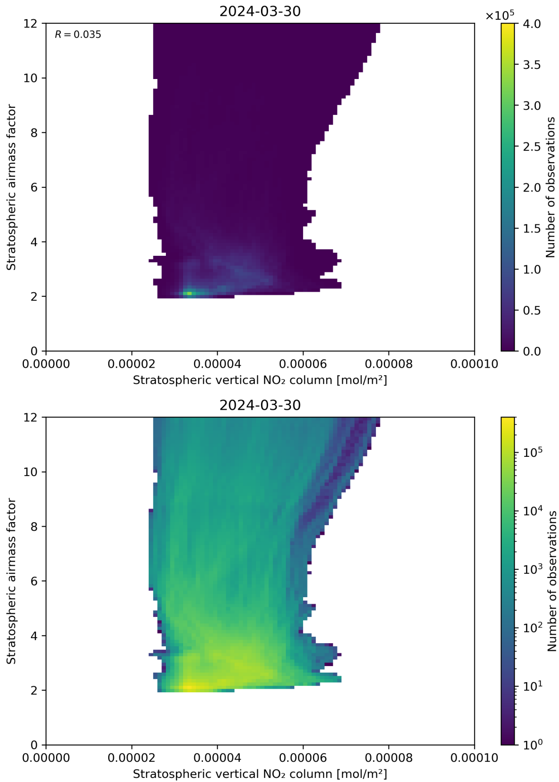
Figure 96: Scatter density plot of “Stratospheric vertical NO 2 column” against “Stratospheric airmass factor” for 2024-03-30 to 2024-03-31.
