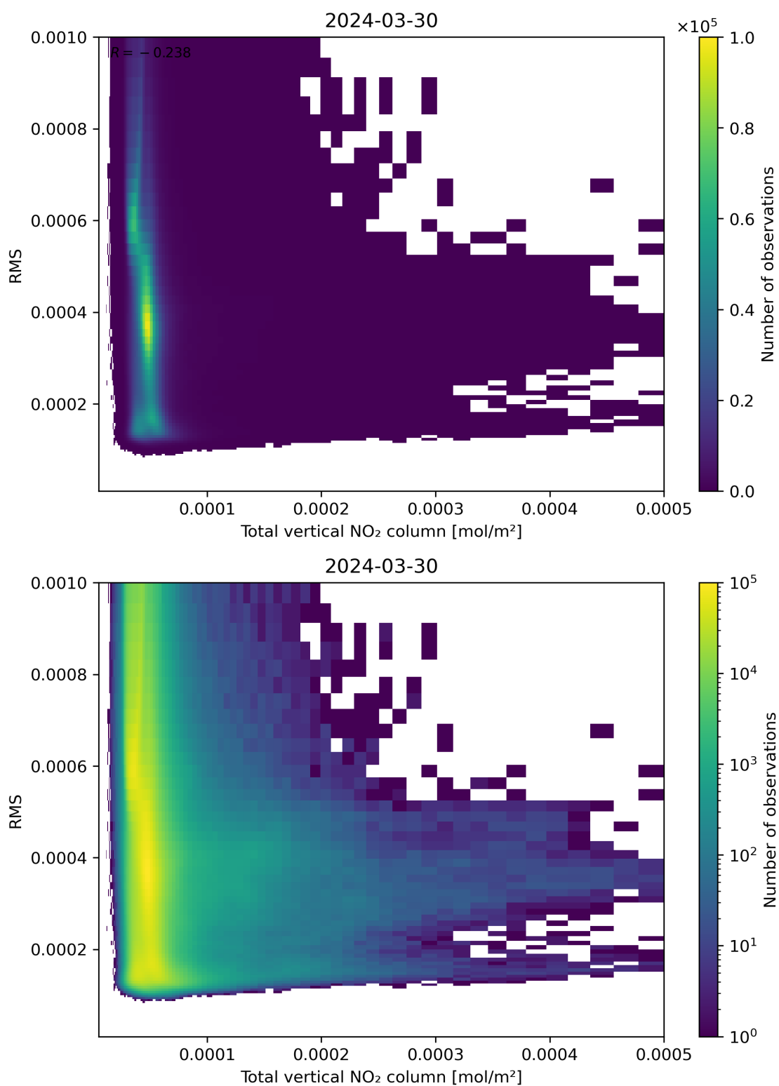
Figure 120: Scatter density plot of “Total vertical NO 2 column” against “RMS” for 2024-03-30 to 2024-03-31.
