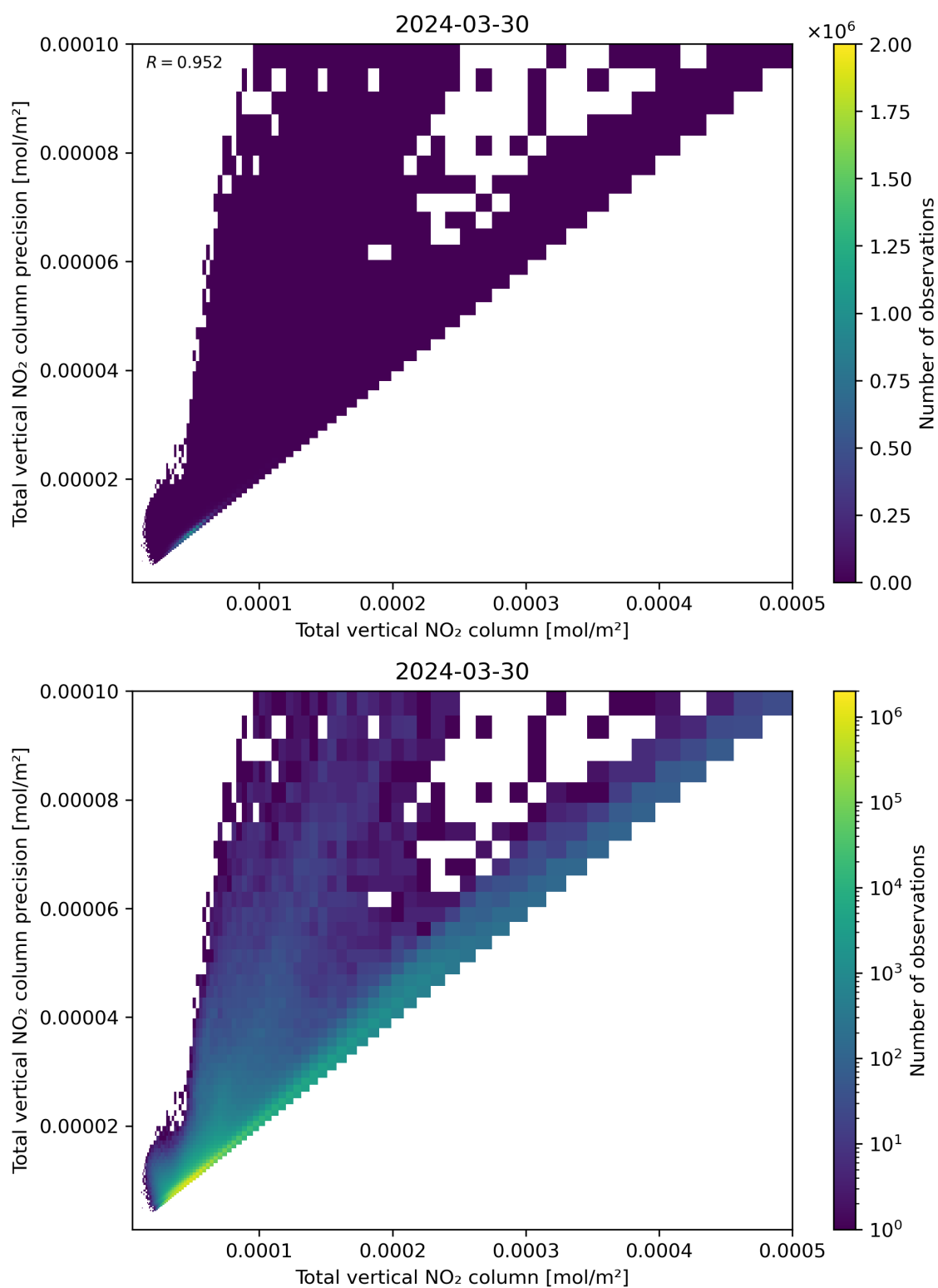
Figure 114: Scatter density plot of “Total vertical NO 2 column” against “Total vertical NO 2 column precision” for 2024-03-30 to 2024-03-31.
