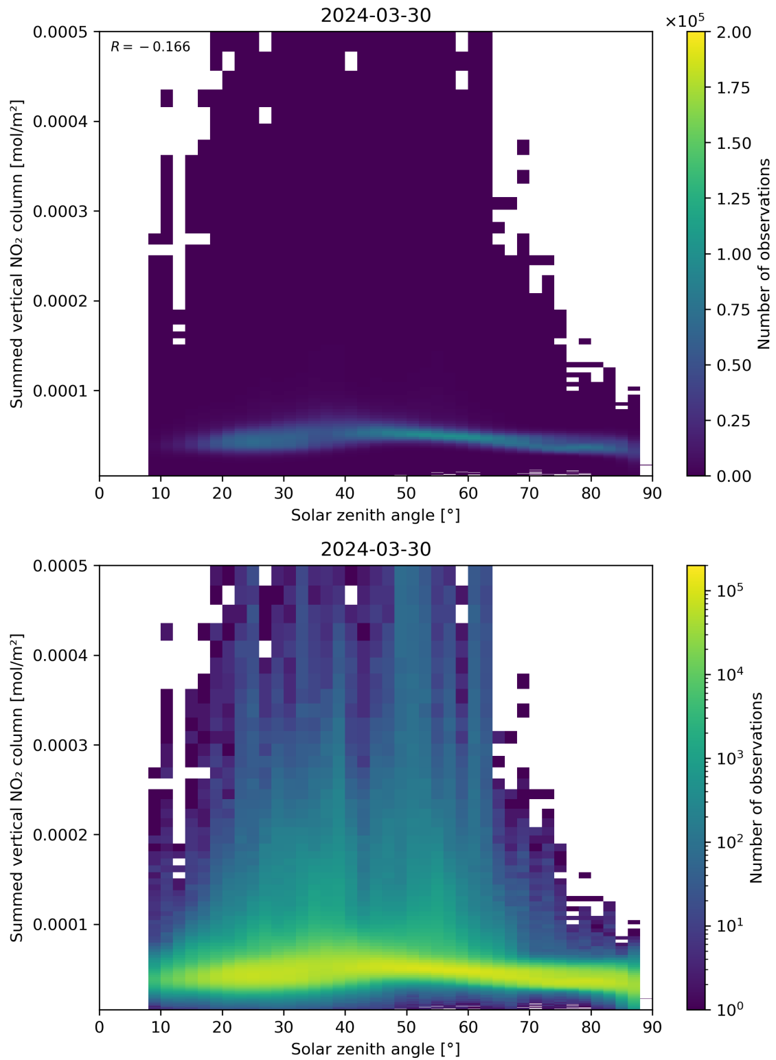
Figure 151: Scatter density plot of “Solar zenith angle” against “Summed vertical NO 2 column” for 2024-03-30 to 2024-03-31.
