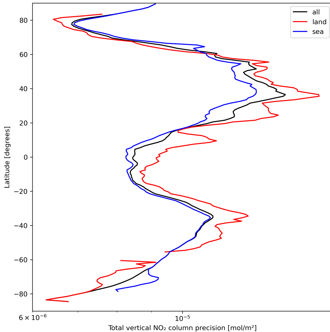
Figure 22: Zonal average of “Total vertical NO 2 column precision” for 2024-03-30 to 2024-03-31.
