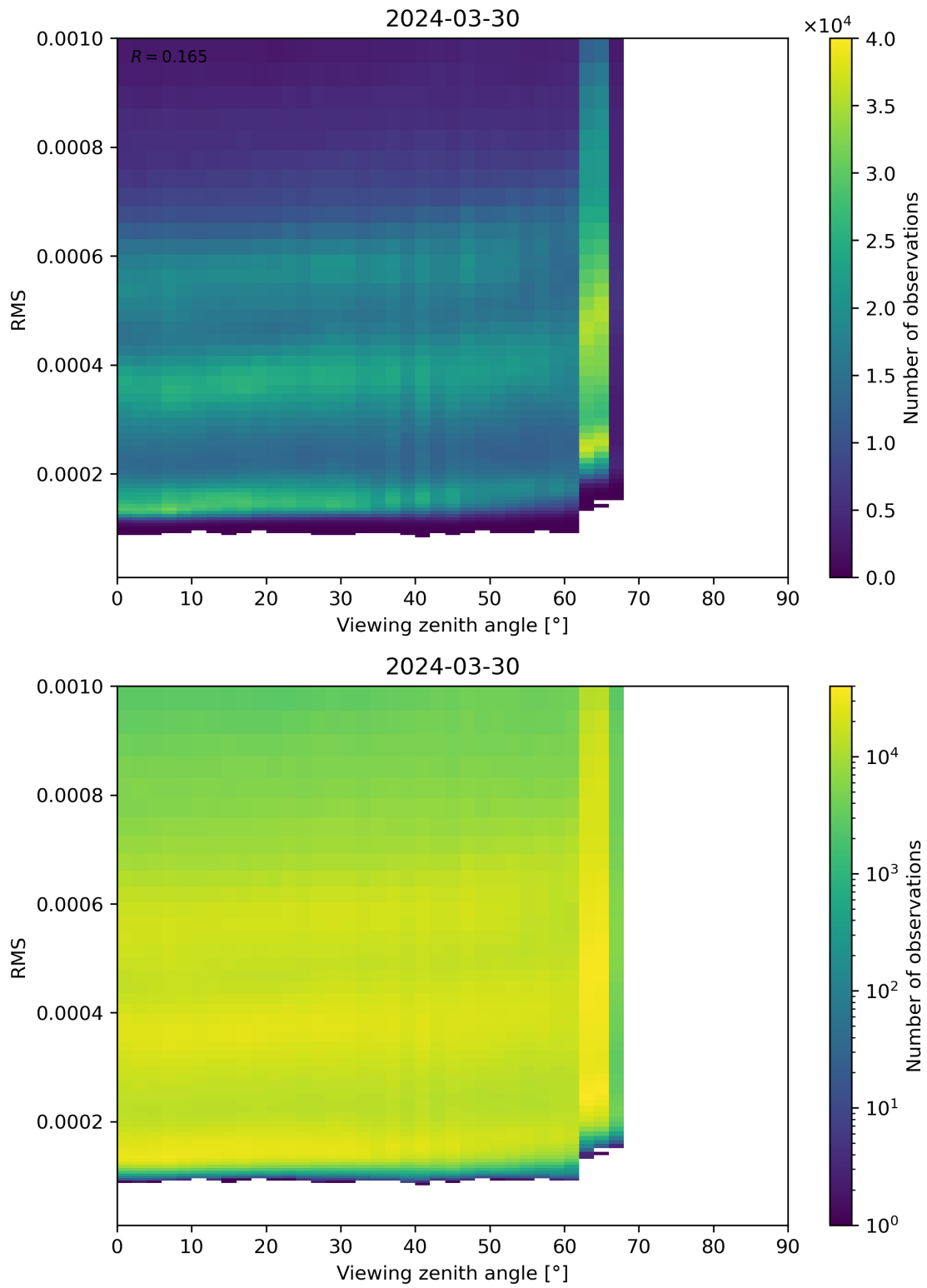
Figure 171: Scatter density plot of “Viewing zenith angle” against “RMS” for 2024-03-30 to 2024-03-31.
