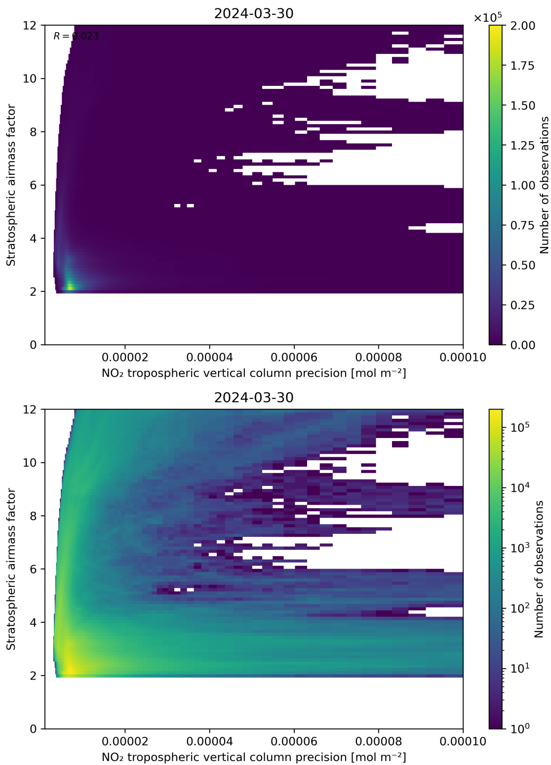
Figure 131: Scatter density plot of “NO 2 tropospheric vertical column precision” against “Stratospheric airmass factor” for 2024-03-30 to 2024-03-31.
