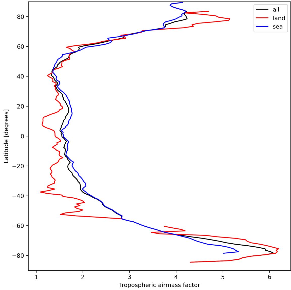
Figure 14: Zonal average of “Tropospheric airmass factor” for 2024-03-30 to 2024-03-31.
