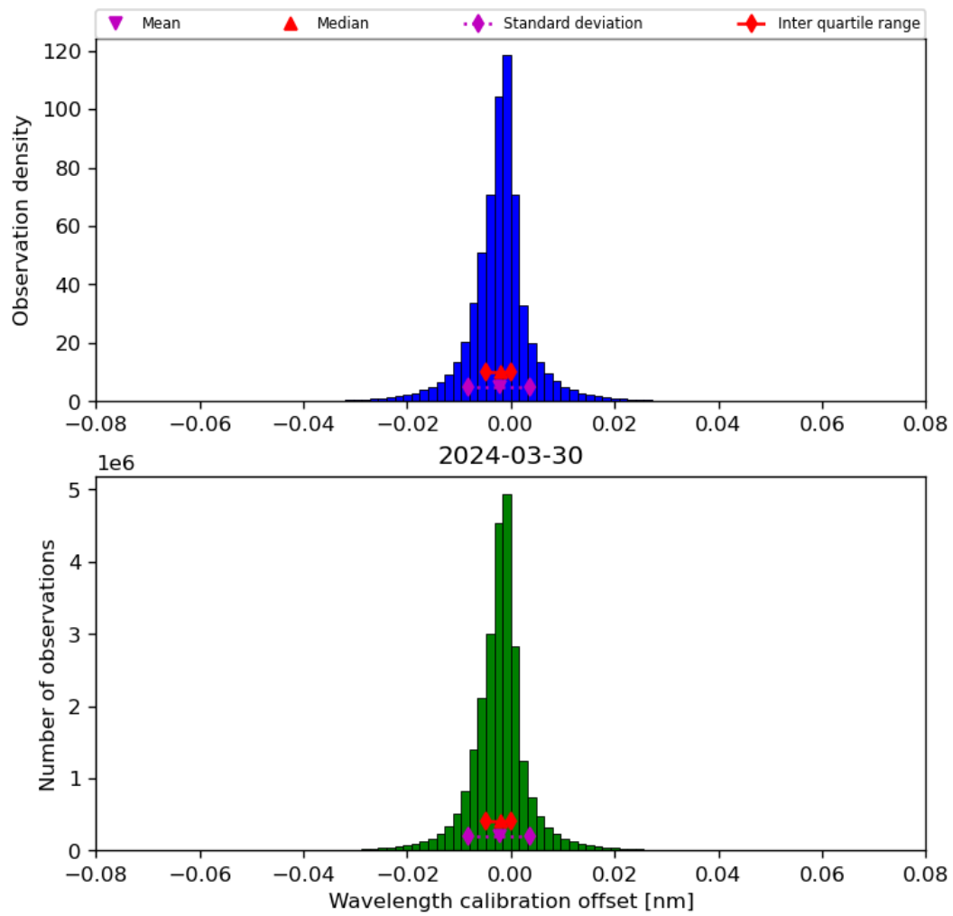
Figure 35: Histogram of “Wavelength calibration offset” for 2024-03-30 to 2024-03-31
