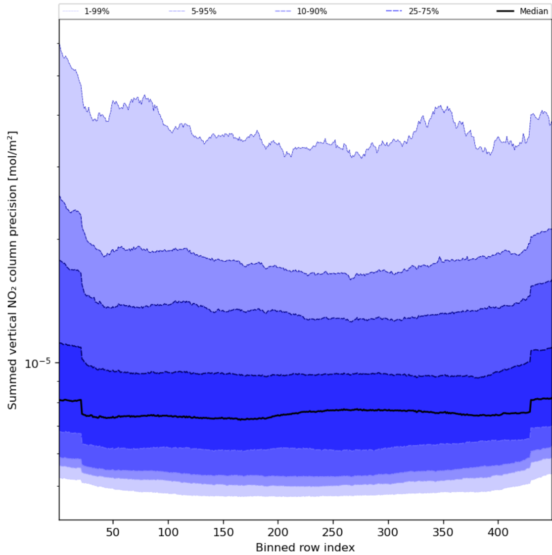
Figure 58: Along track statistics of “Summed vertical NO 2 column precision” for 2024-03-30 to 2024-03-31
