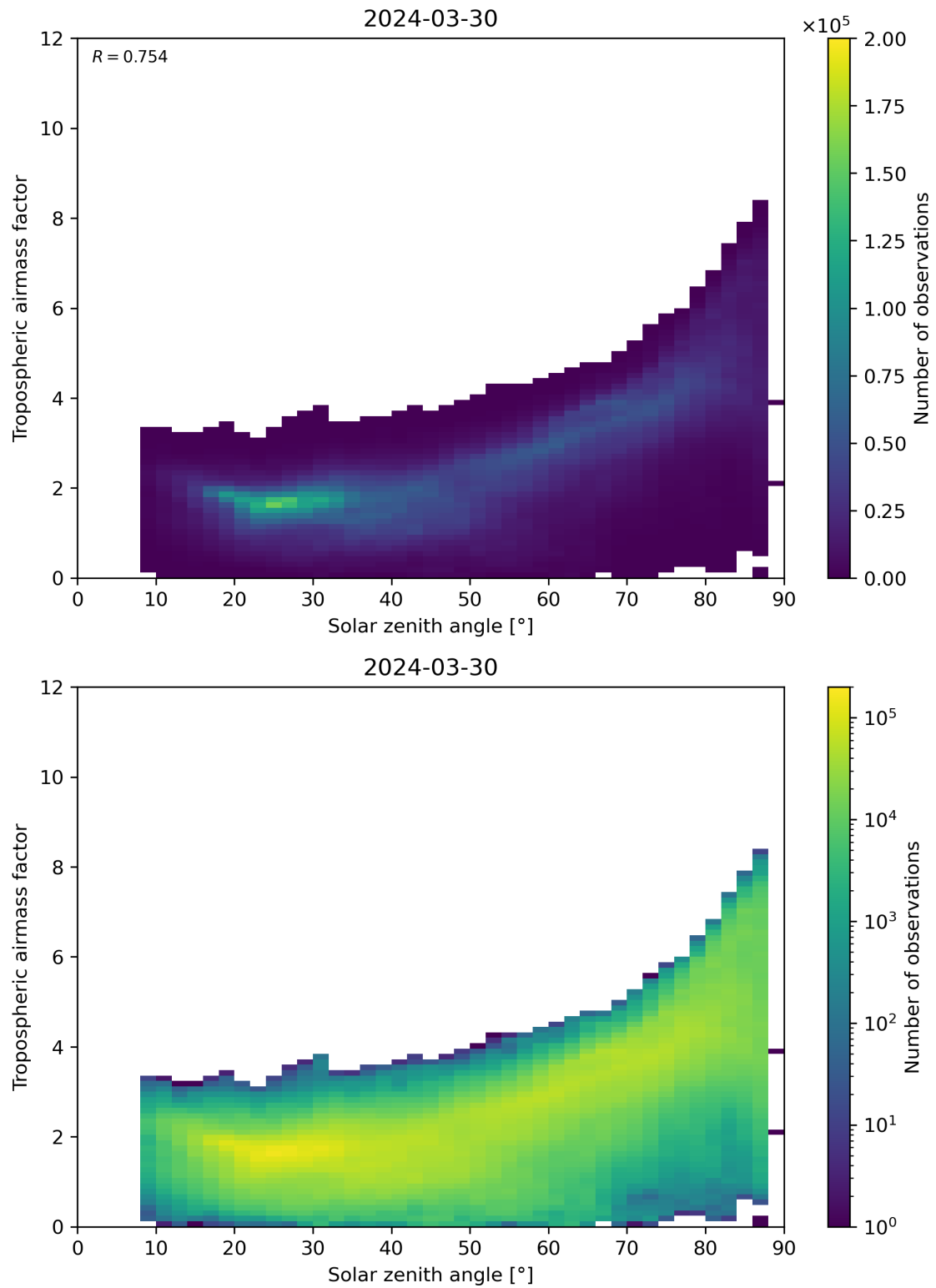
Figure 147: Scatter density plot of “Solar zenith angle” against “Tropospheric airmass factor” for 2024-03-30 to 2024-03-31.
