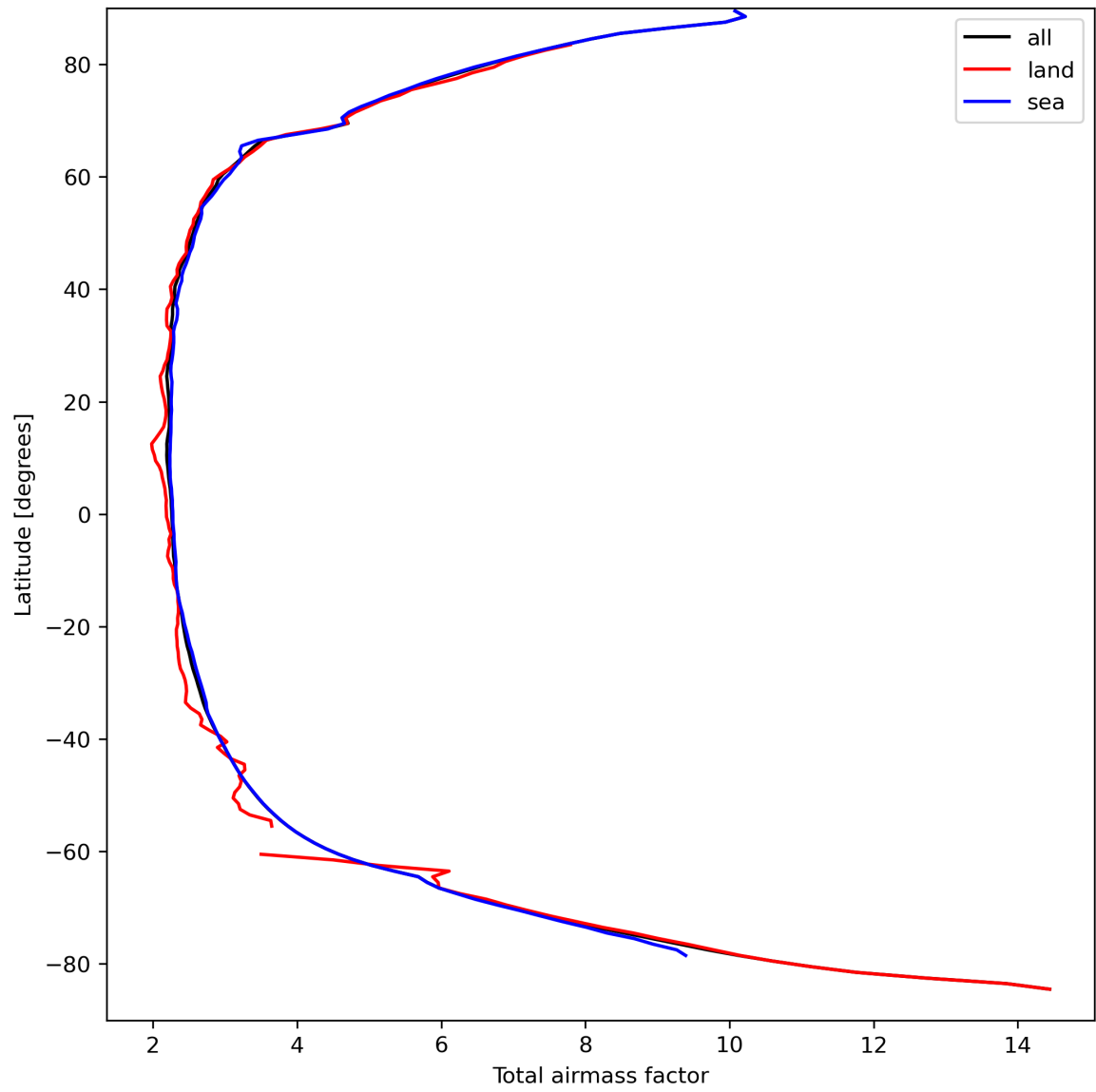
Figure 15: Zonal average of “Total airmass factor” for 2024-03-30 to 2024-03-31.
