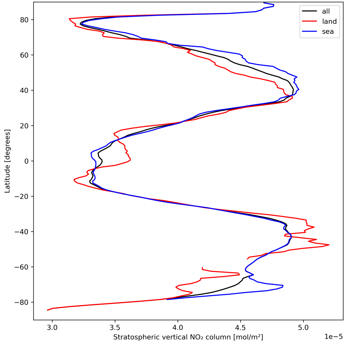
Figure 19: Zonal average of “Stratospheric vertical NO 2 column” for 2024-03-30 to 2024-03-31.
