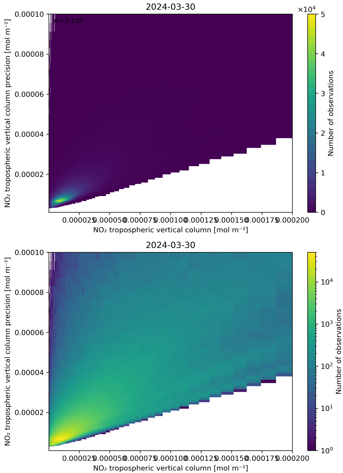
Figure 130: Scatter density plot of “NO 2 tropospheric vertical column” against “NO 2 tropospheric vertical column precision” for 2024-03-30 to 2024-03-31.
