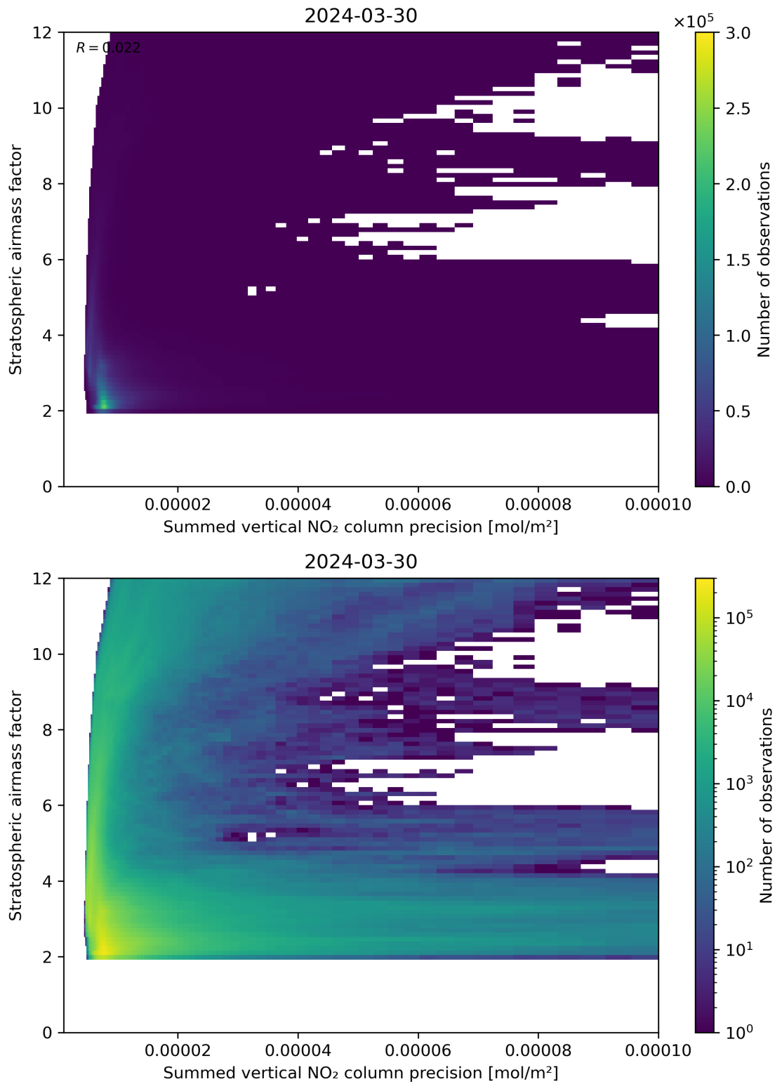
Figure 106: Scatter density plot of “Summed vertical NO 2 column precision” against “Stratospheric airmass factor” for 2024-03-30 to 2024-03-31.
