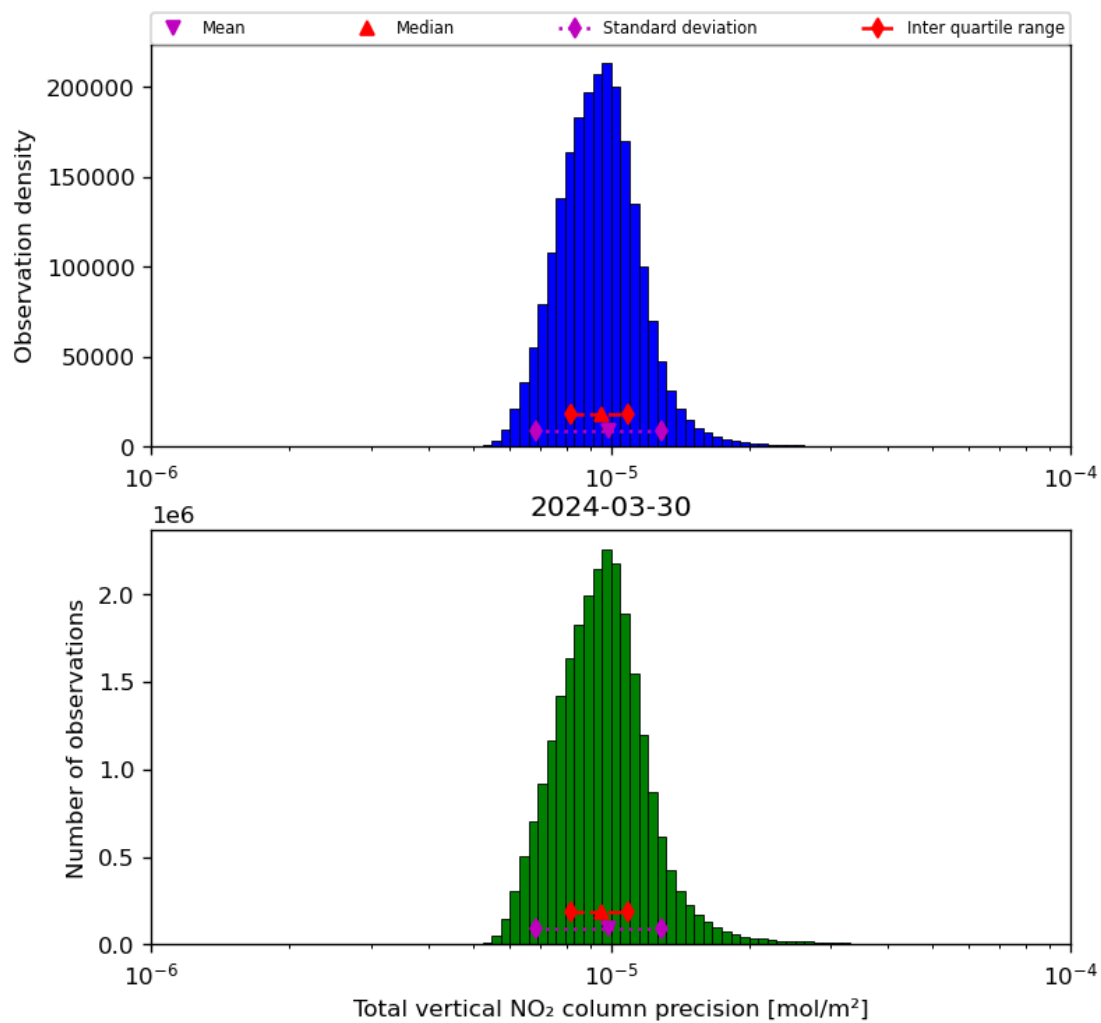
Figure 39: Histogram of "Total vertical NO 2 column precision" for 2024-03-30 to 2024-03-31
