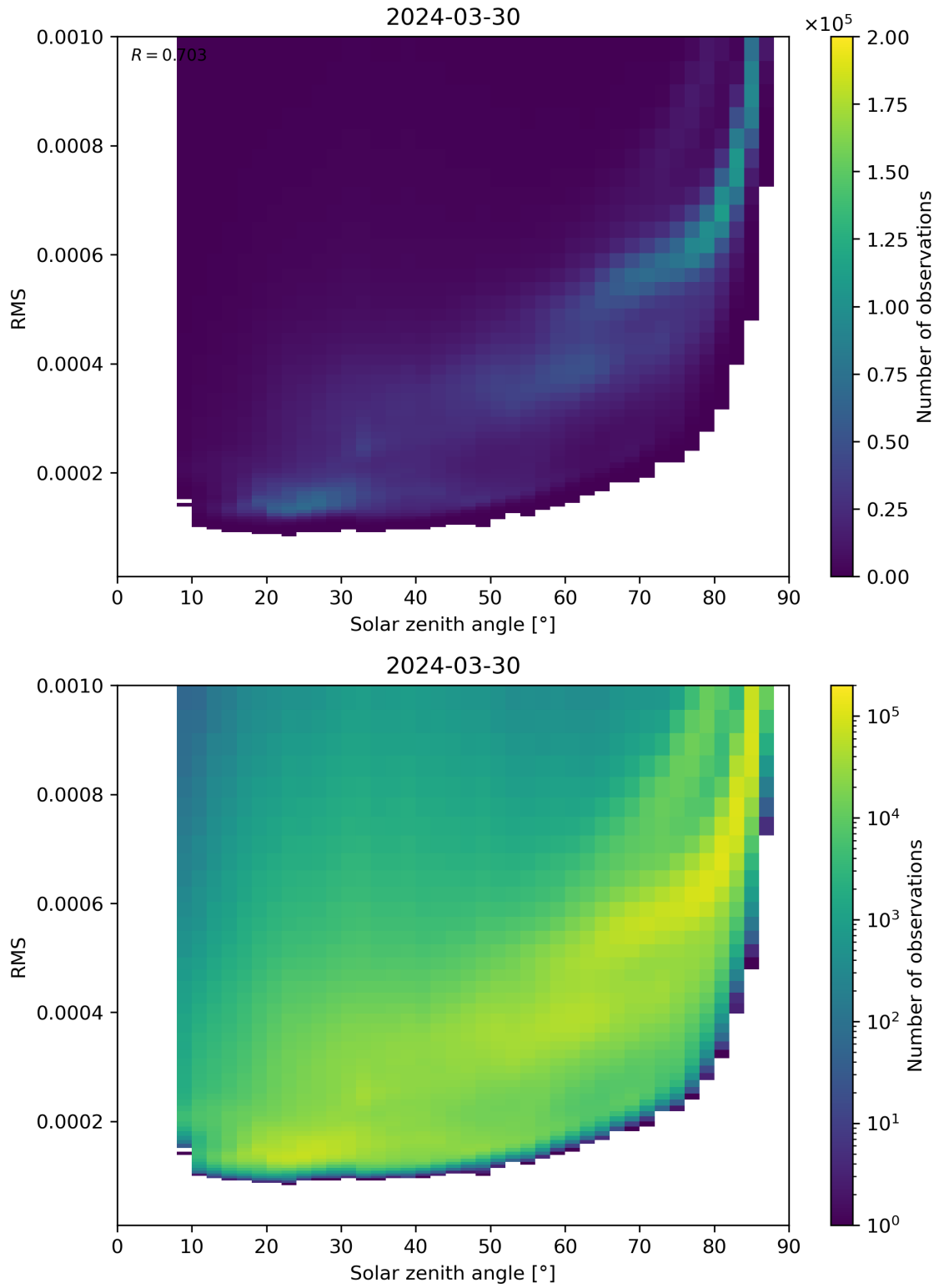
Figure 157: Scatter density plot of “Solar zenith angle” against “RMS” for 2024-03-30 to 2024-03-31.
