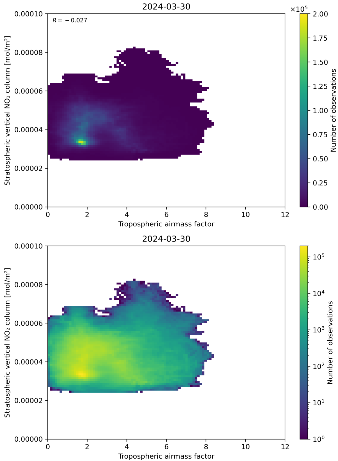
Figure 74: Scatter density plot of “Tropospheric airmass factor” against “Stratospheric vertical NO 2 column” for 2024-03-30 to 2024-03-31.
