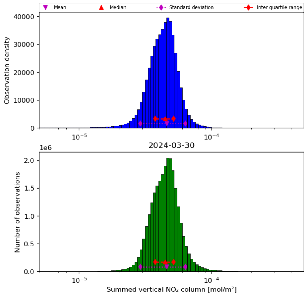
Figure 40: Histogram of “Summed vertical NO 2 column” for 2024-03-30 to 2024-03-31
