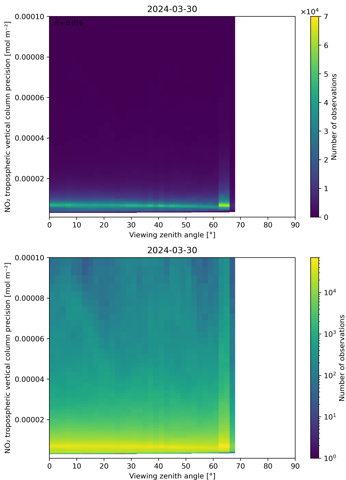
Figure 170: Scatter density plot of “Viewing zenith angle” against “NO 2 tropospheric vertical column precision” for 2024-03-30 to 2024-03-31.
