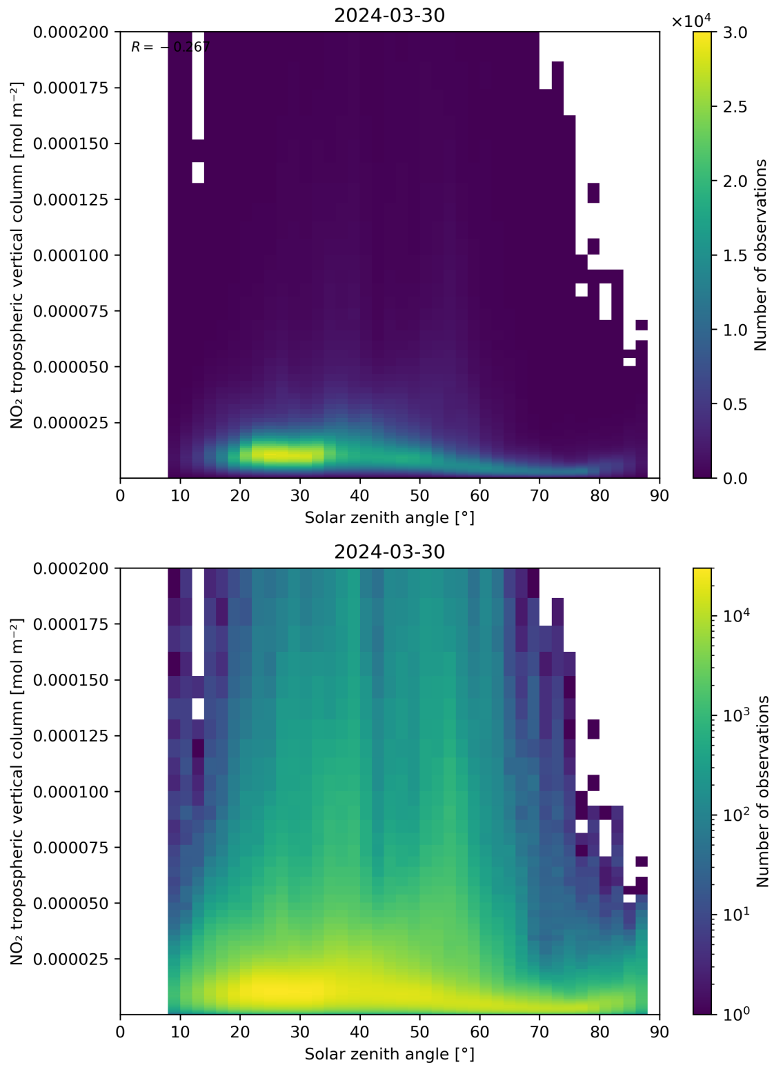
Figure 155: Scatter density plot of “Solar zenith angle” against “NO 2 tropospheric vertical column” for 2024-03-30 to 2024-03-31.
