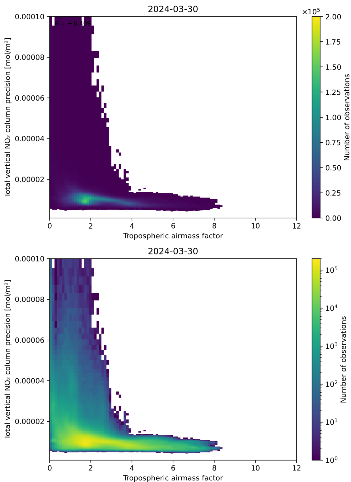
Figure 78: Scatter density plot of “Tropospheric air mass factor” against “Total vertical NO 2 column precision” for 2024-03-30 to 2024-03-31.
