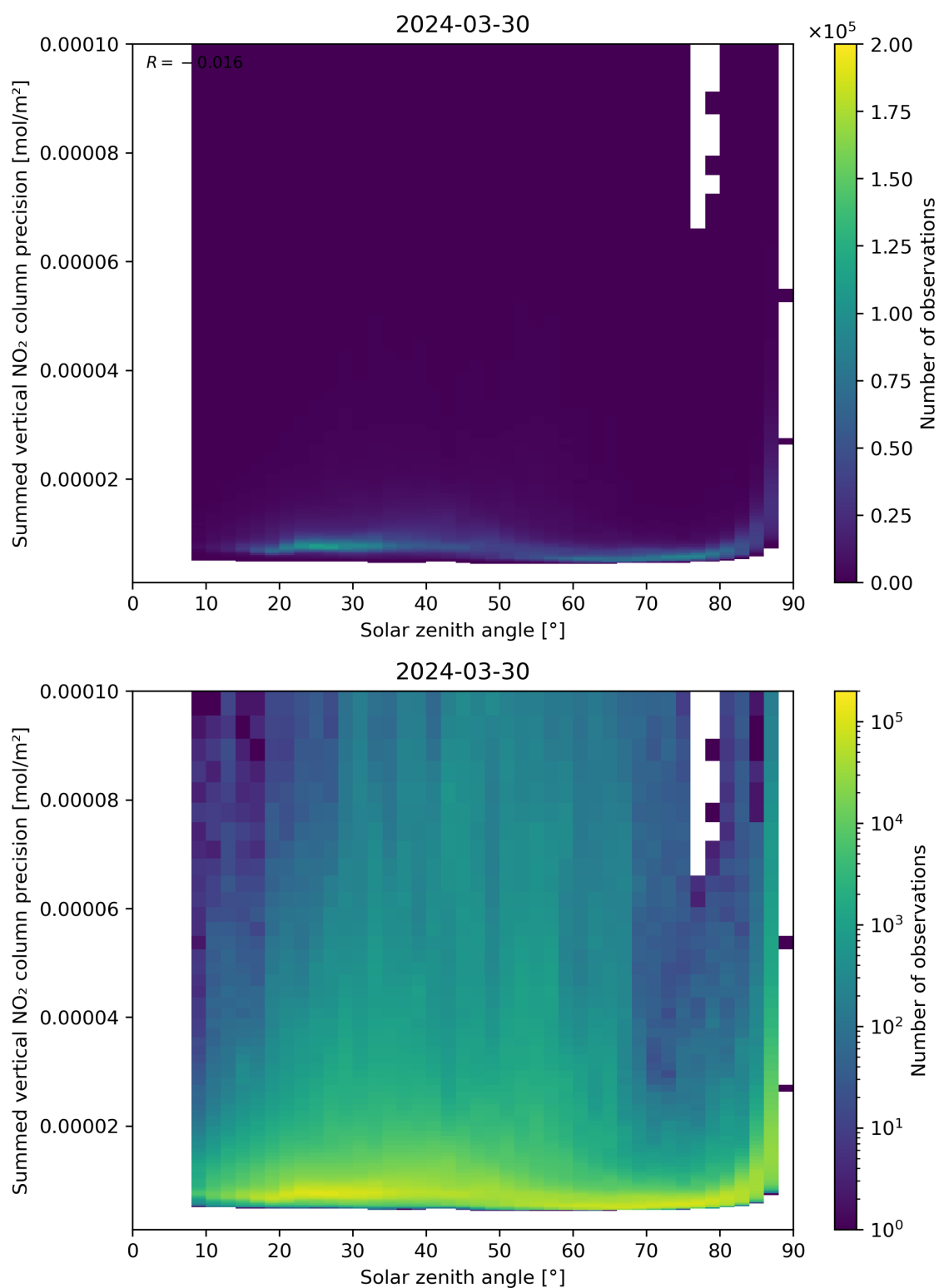
Figure 152: Scatter density plot of “Solar zenith angle” against “Summed vertical NO 2 column precision” for 2024-03-30 to 2024-03-31.
