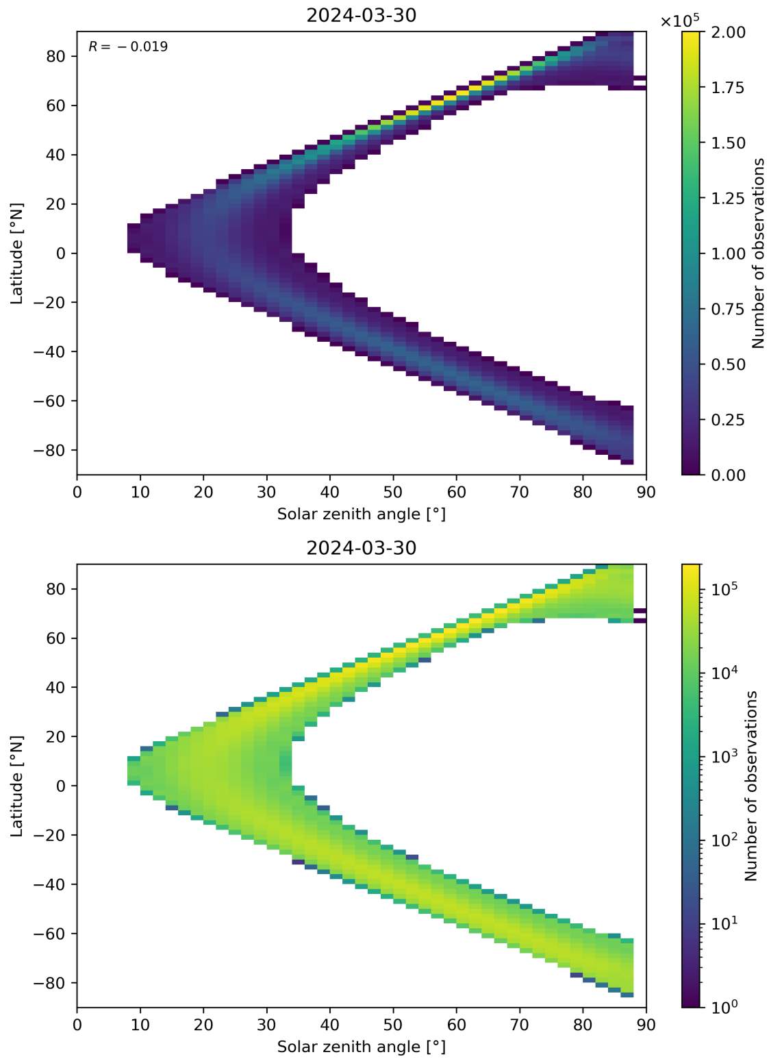
Figure 149: Scatter density plot of “Solar zenith angle” against “Latitude” for 2024-03-30 to 2024-03-31.
