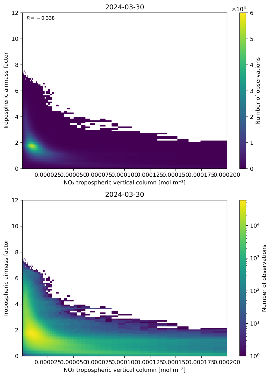
Figure 123: Scatter density plot of “NO 2 tropospheric vertical column” against “Tropospheric air mass factor” for 2024-03-30 to 2024-03-31.
