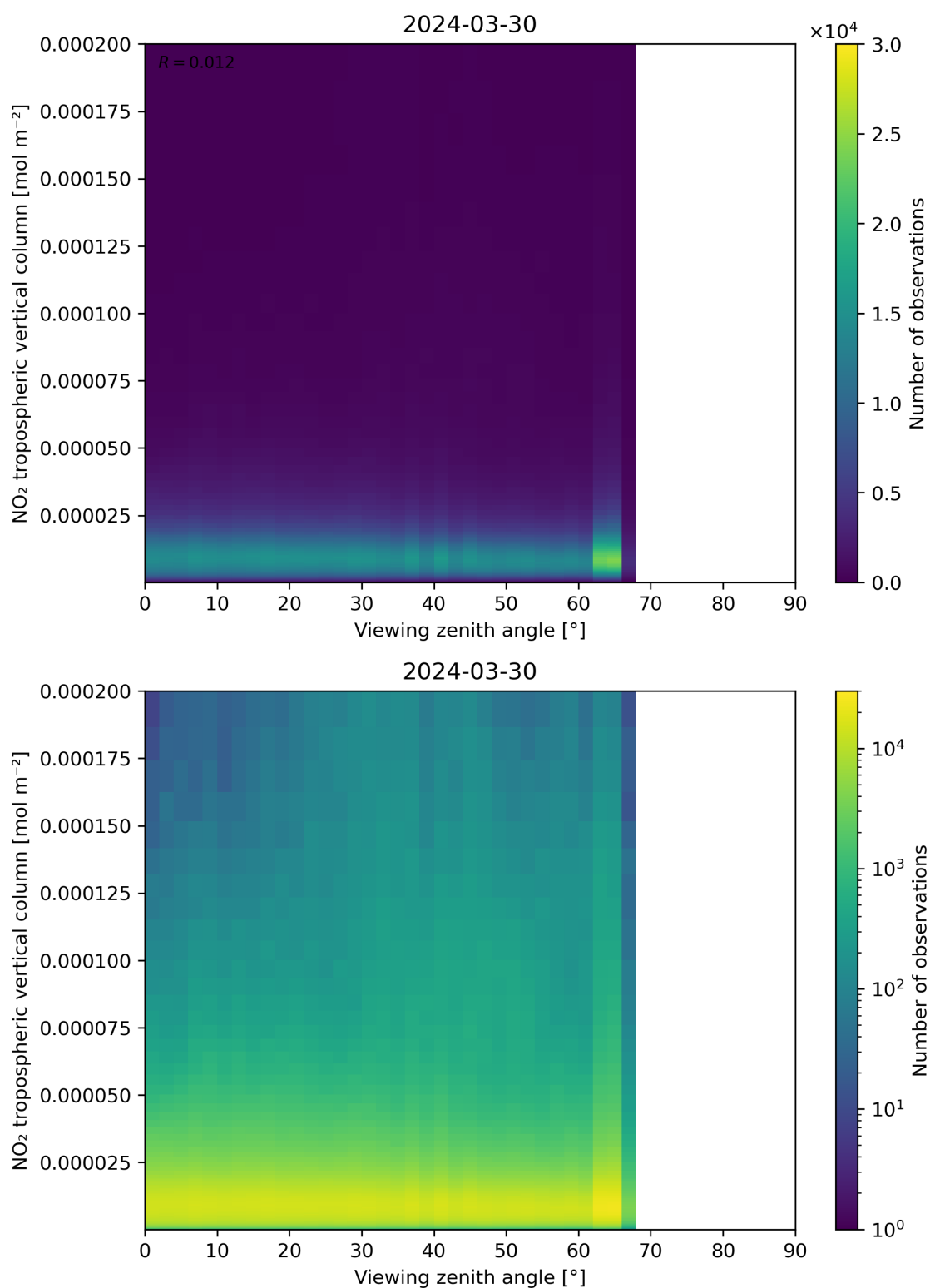
Figure 169: Scatter density plot of “Viewing zenith angle” against “NO 2 tropospheric vertical column” for 2024-03-30 to 2024-03-31.
