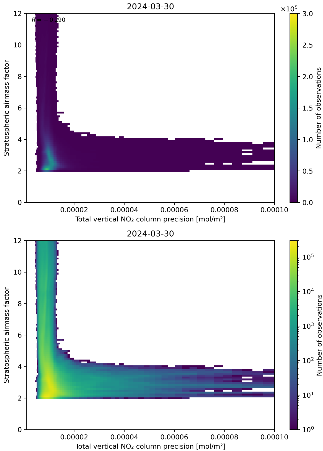
Figure 115: Scatter density plot of “Total vertical NO 2 column precision” against “Stratospheric air mass factor” for 2024-03-30 to 2024-03-31.
