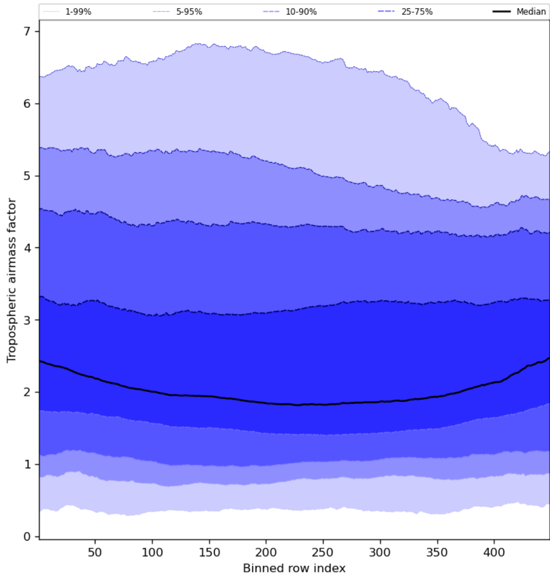
Figure 48: Along track statistics of “Tropospheric air mass factor” for 2024-03-30 to 2024-03-31
