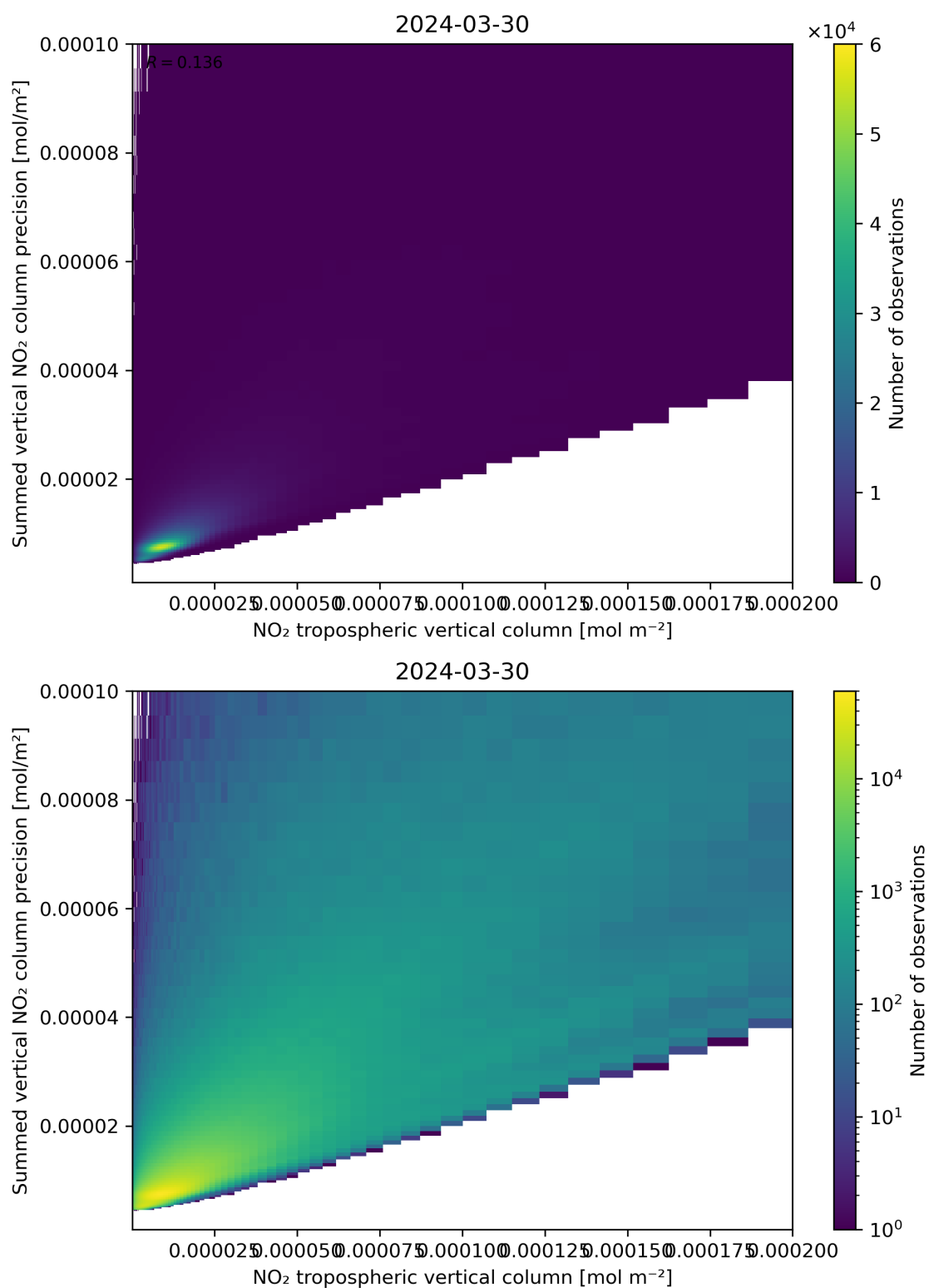
Figure 127: Scatter density plot of “NO 2 tropospheric vertical column” against “Summed vertical NO 2 column precision” for 2024-03-30 to 2024-03-31.
