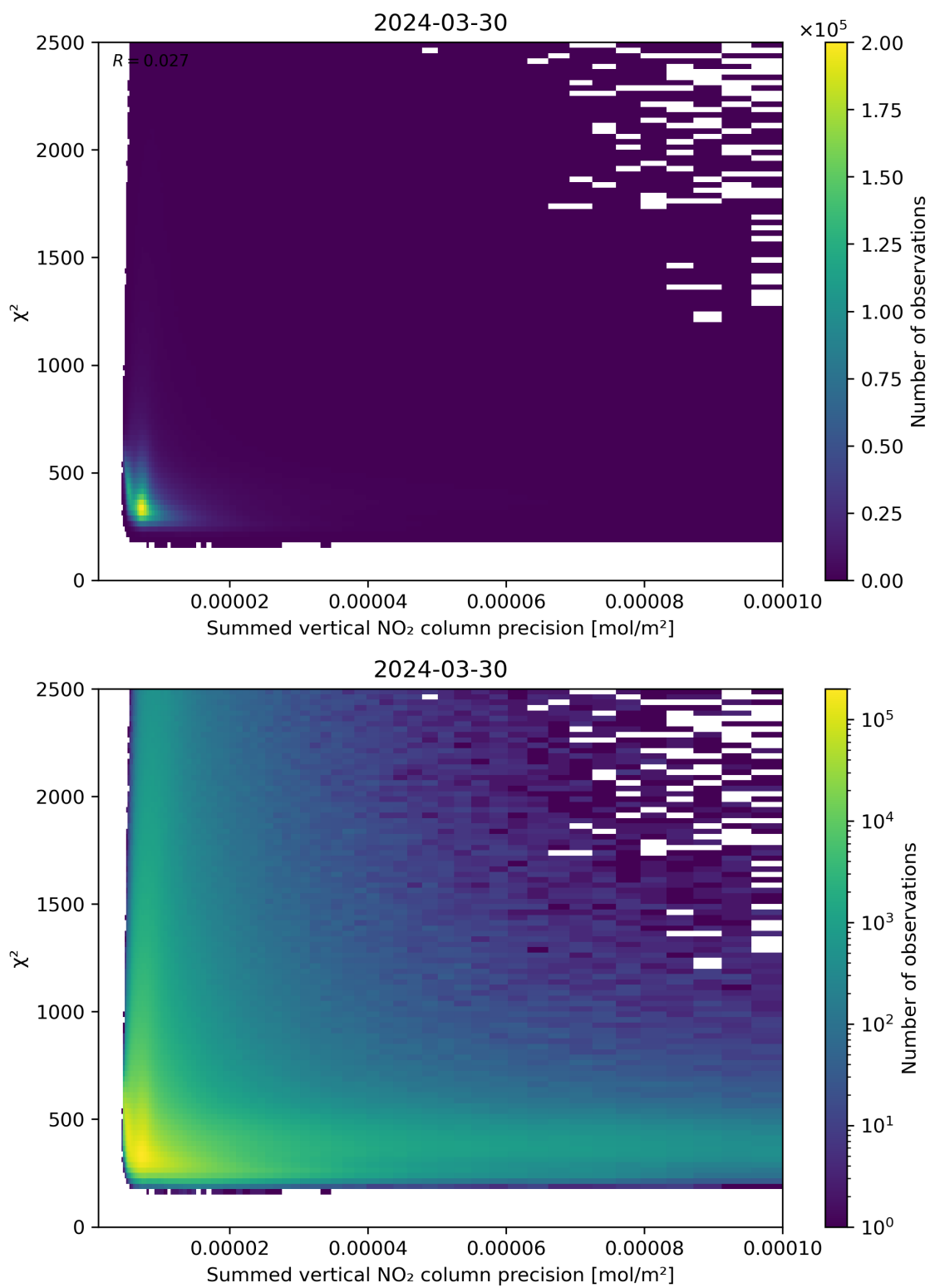
Figure 107: Scatter density plot of “Summed vertical NO 2 column precision” against “ \chi^2 ” for 2024-03-30 to 2024-03-31.
