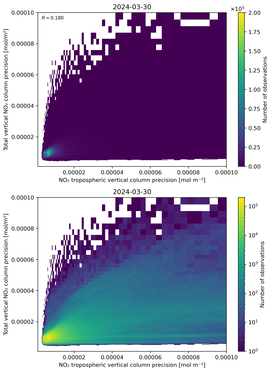
Figure 139: Scatter density plot of “NO 2 tropospheric vertical column precision” against “Total vertical NO 2 column precision” for 2024-03-30 to 2024-03-31.
