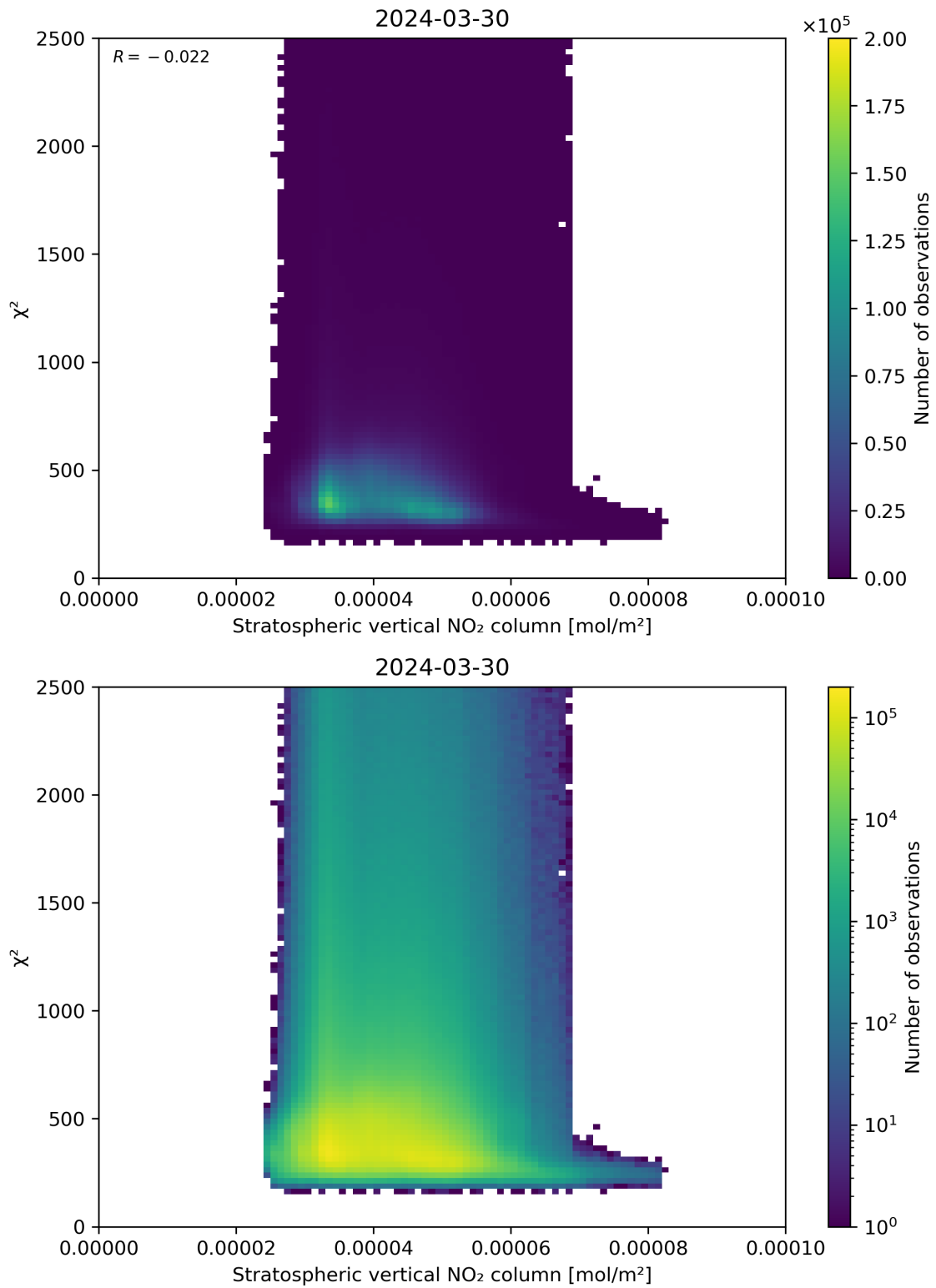
Figure 97: Scatter density plot of “Stratospheric vertical NO 2 column” against “ \chi^2 ” for 2024-03-30 to 2024-03-31.
