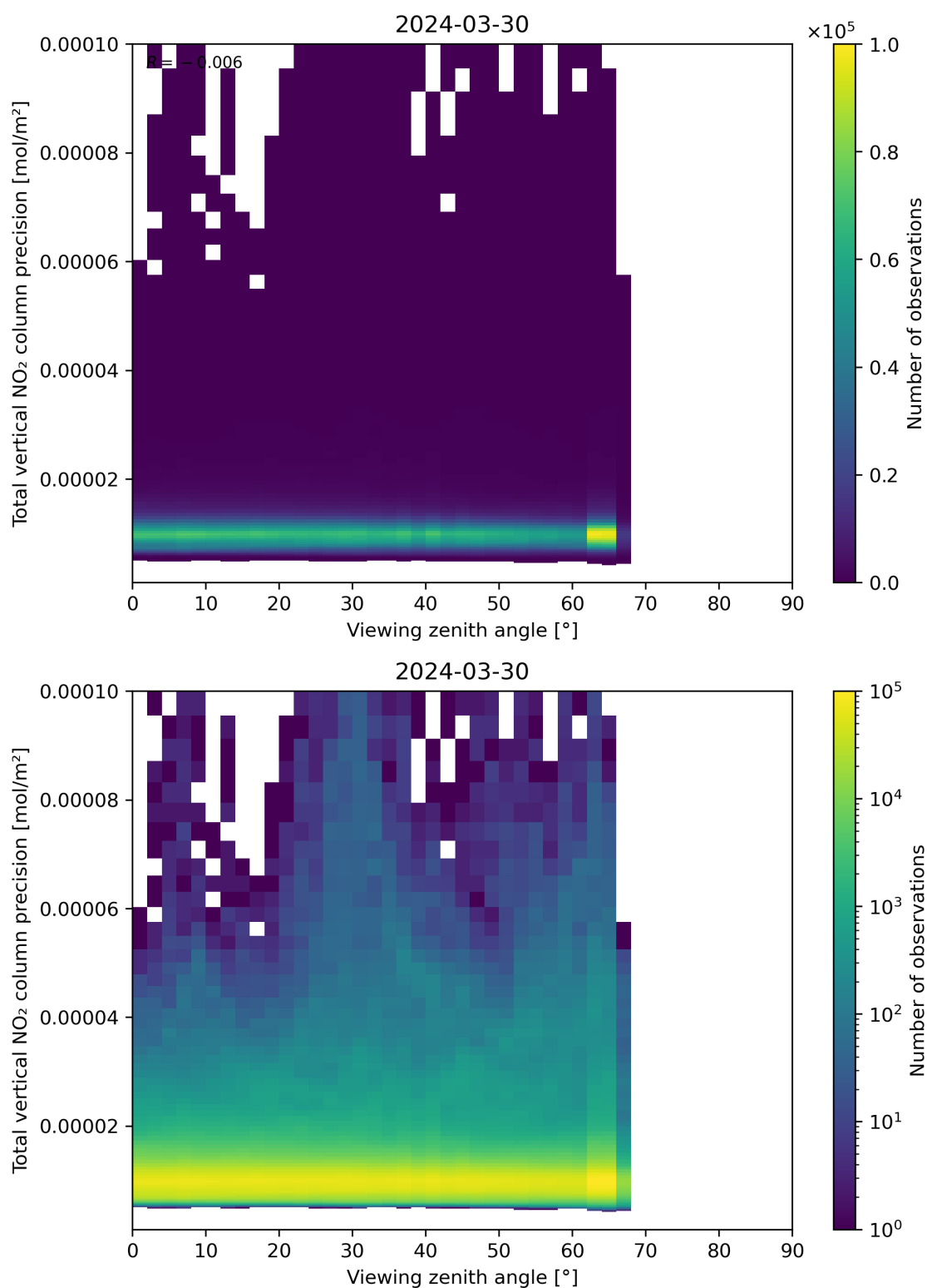
Figure 168: Scatter density plot of “Viewing zenith angle” against “Total vertical NO 2 column precision” for 2024-03-30 to 2024-03-31.
