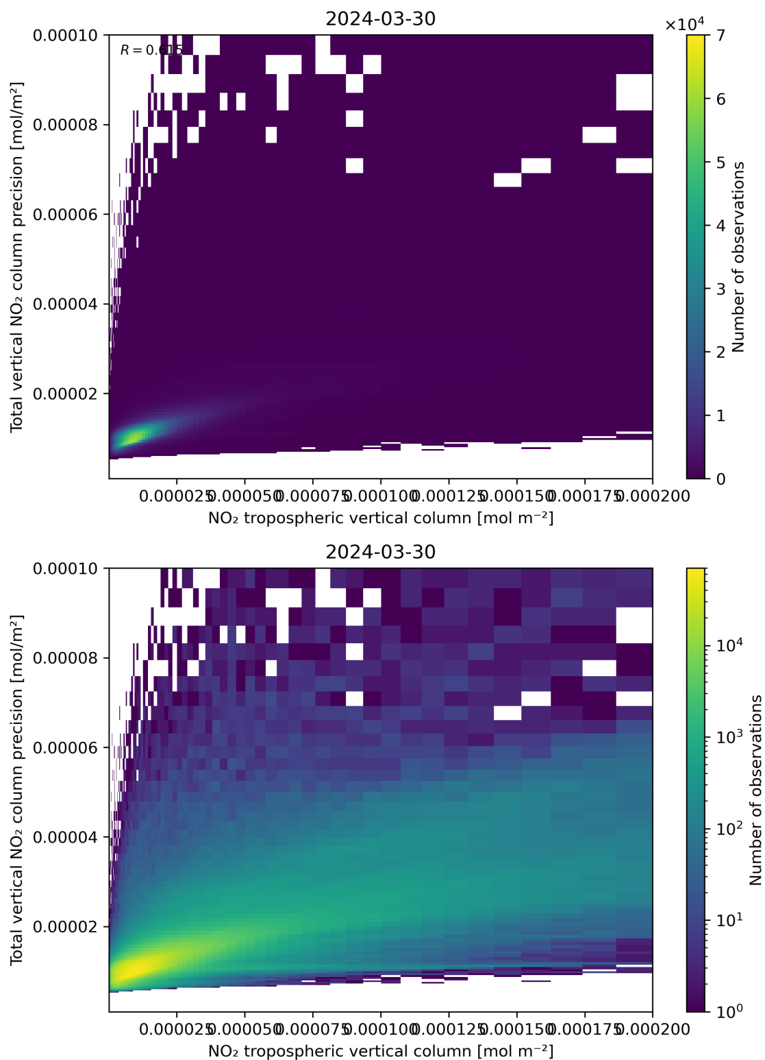
Figure 129: Scatter density plot of “NO 2 tropospheric vertical column” against “Total vertical NO 2 column precision” for 2024-03-30 to 2024-03-31.
