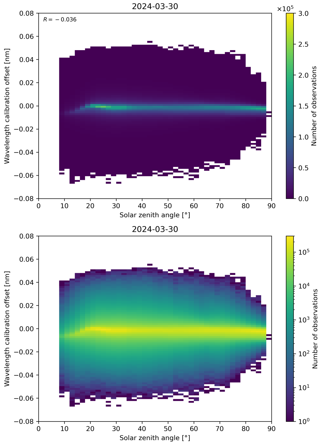
Figure 158: Scatter density plot of “Solar zenith angle” against “Wavelength calibration offset” for 2024-03-30 to 2024-03-31.
