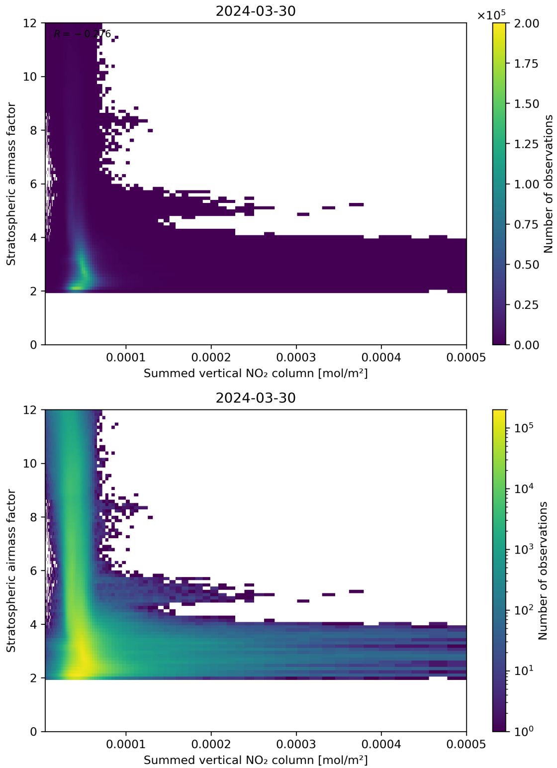
Figure 103: Scatter density plot of “Summed vertical NO 2 column” against “Stratospheric airmass factor” for 2024-03-30 to 2024-03-31.
