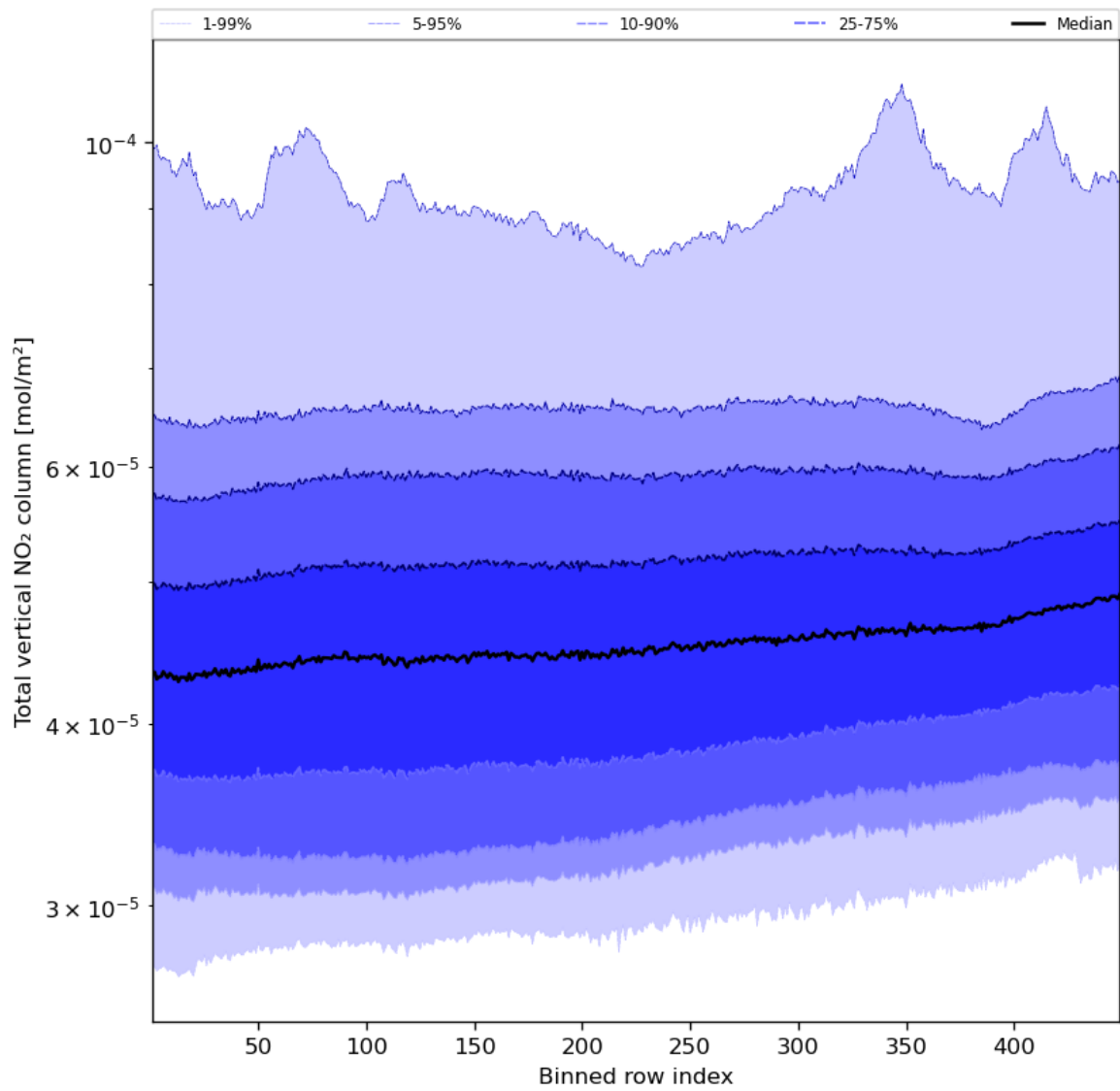
Figure 55: Along track statistics of “Total vertical NO 2 column” for 2024-03-30 to 2024-03-31
