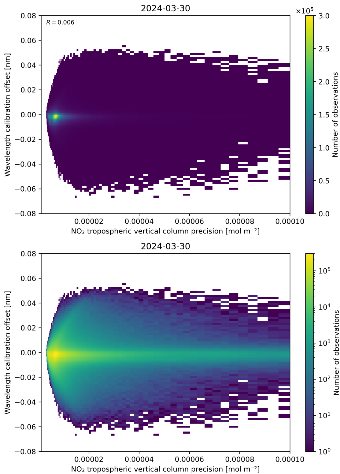
Figure 141: Scatter density plot of “NO 2 tropospheric vertical column precision” against “Wavelength calibration offset” for 2024-03-30 to 2024-03-31.
