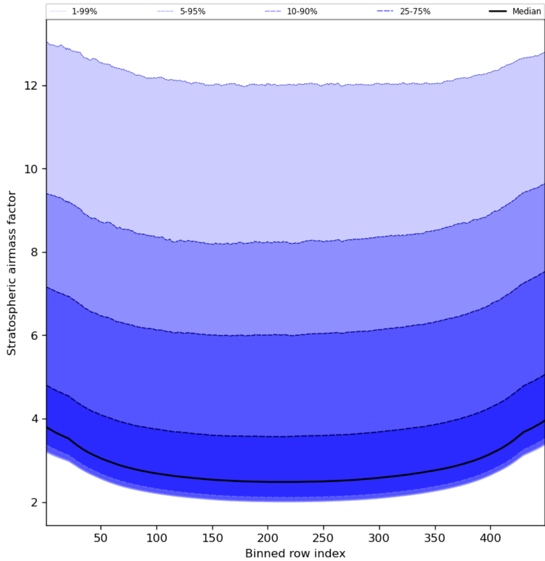
Figure 61: Along track statistics of “Stratospheric airmass factor” for 2024-03-30 to 2024-03-31
