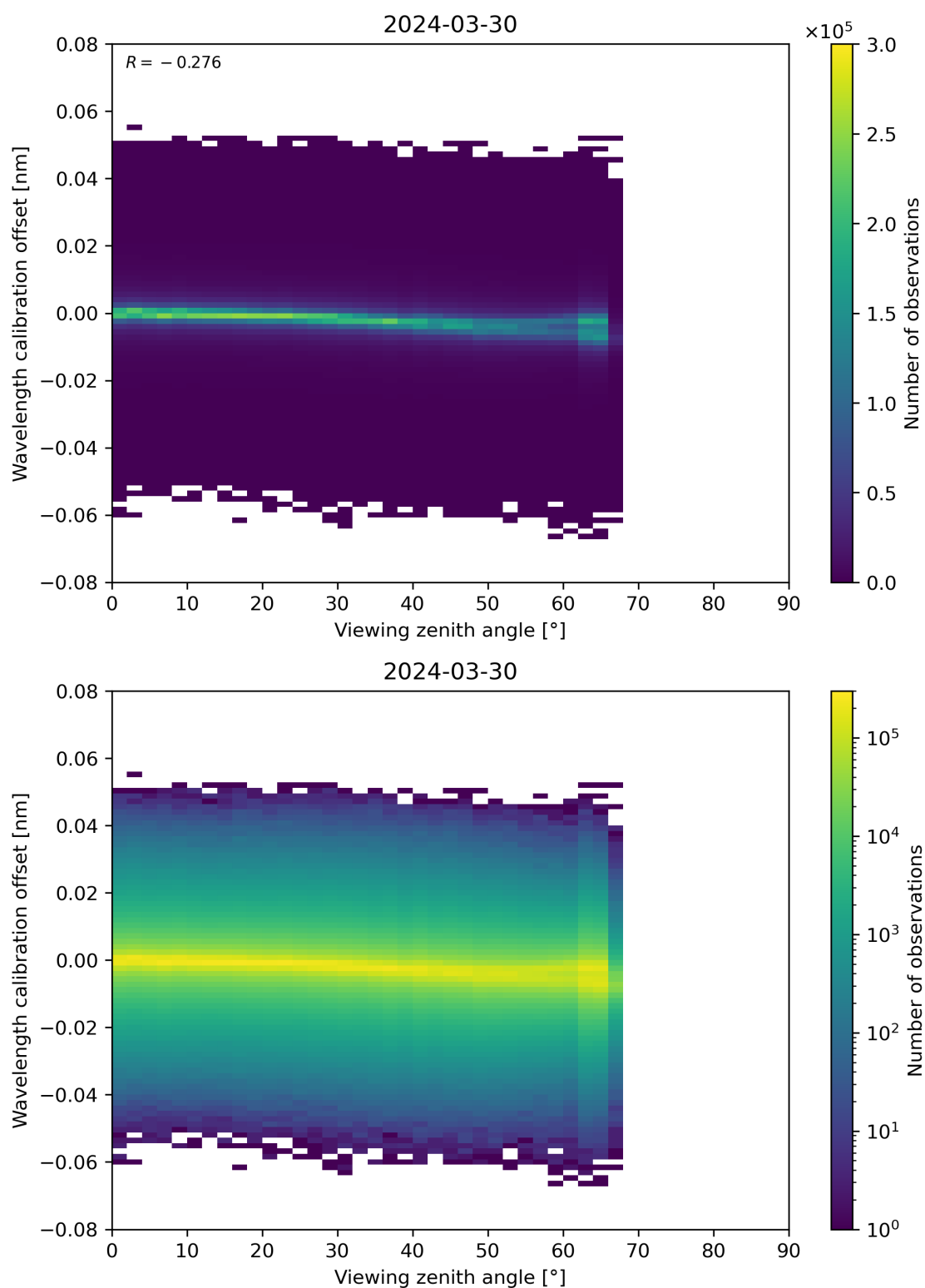
Figure 173: Scatter density plot of “Viewing zenith angle” against “Wavelength calibration offset” for 2024-03-30 to 2024-03-31.
