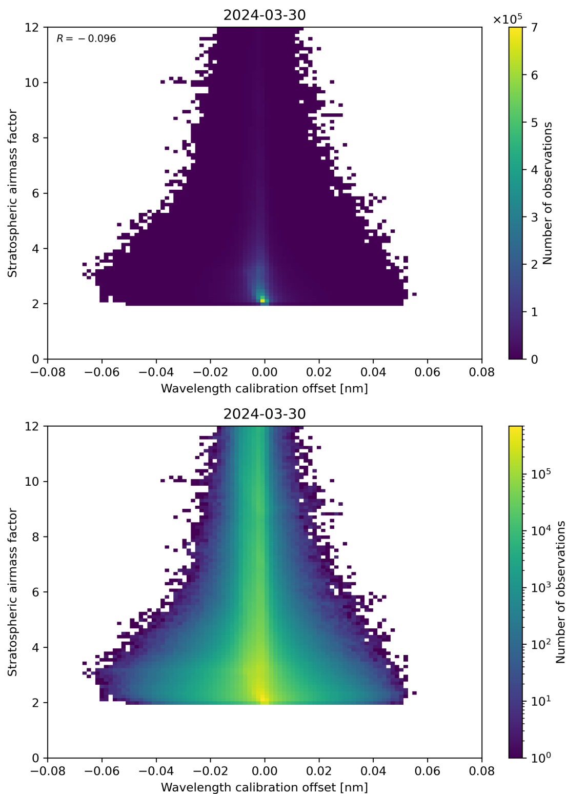
Figure 174: Scatter density plot of “Wavelength calibration offset” against “Stratospheric airmass factor” for 2024-03-30 to 2024-03-31.
