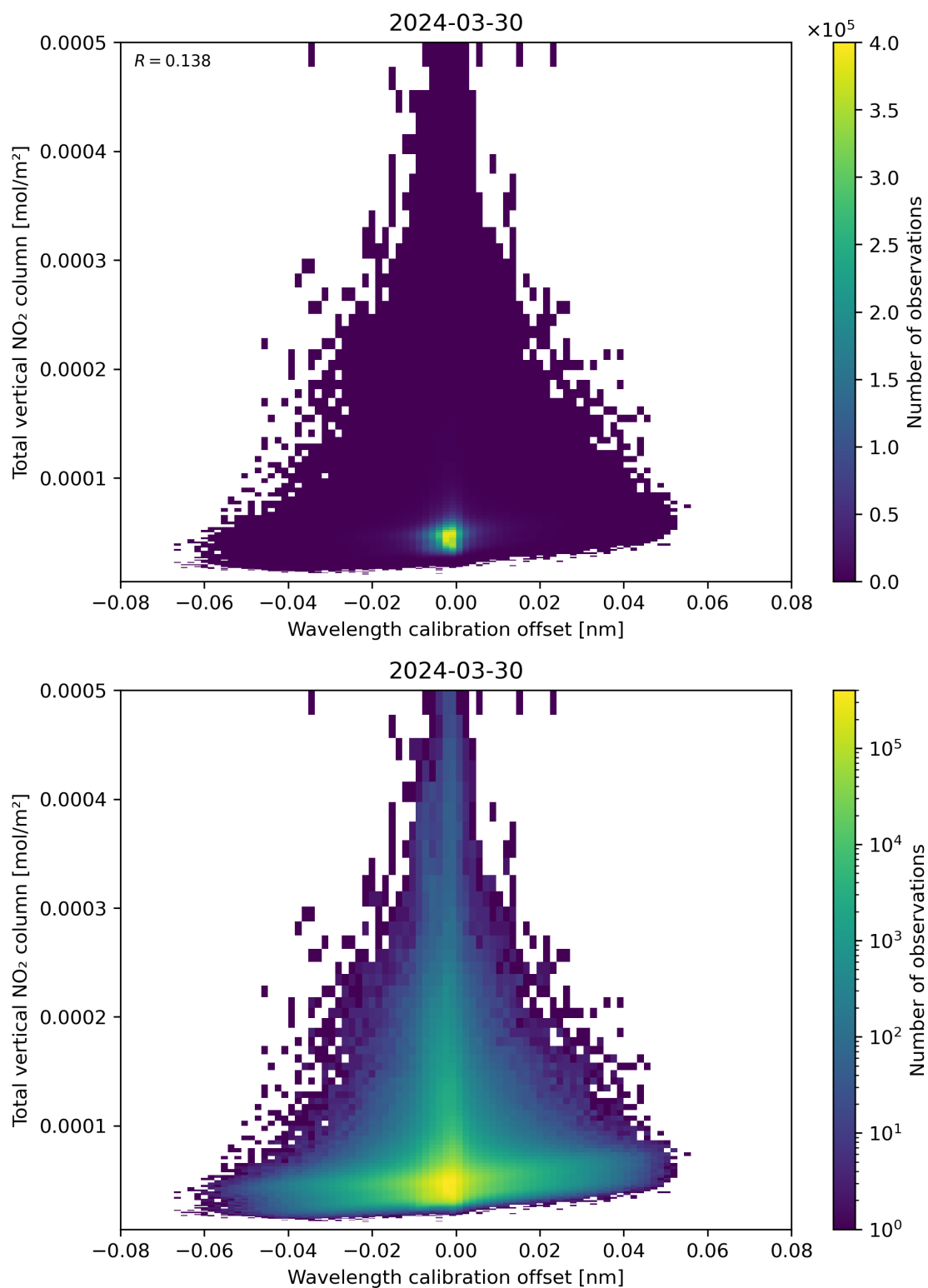
Figure 179: Scatter density plot of “Wavelength calibration offset” against “Total vertical NO 2 column” for 2024-03-30 to 2024-03-31.
