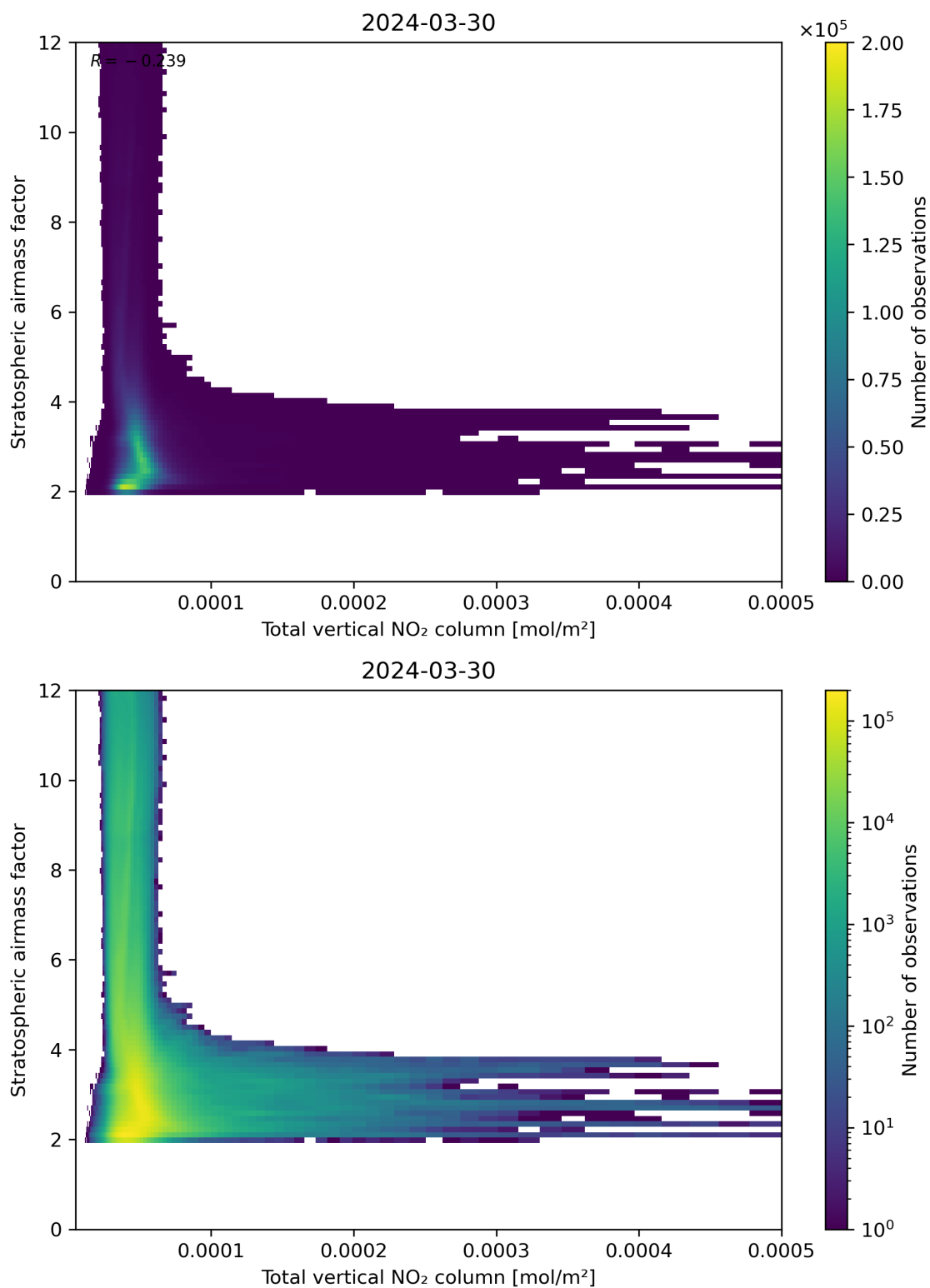
Figure 110: Scatter density plot of “Total vertical NO 2 column” against “Stratospheric airmass factor” for 2024-03-30 to 2024-03-31.
