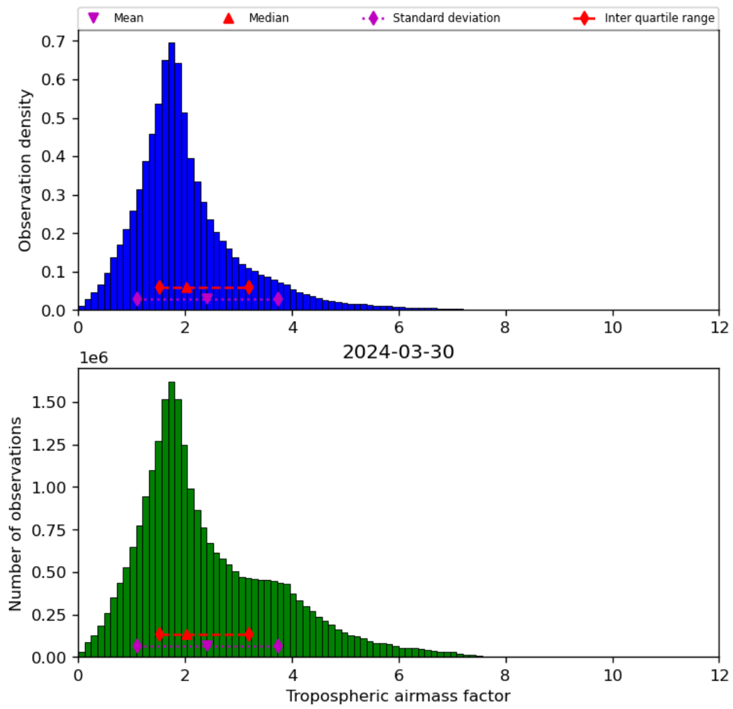
Figure 31: Histogram of “Tropospheric airmass factor” for 2024-03-30 to 2024-03-31
