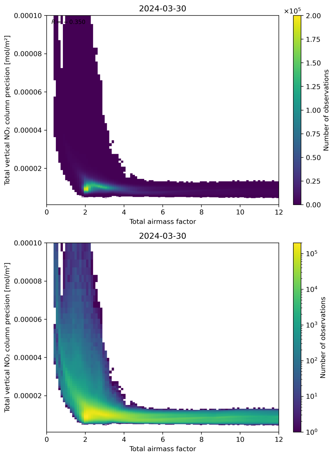
Figure 68: Scatter density plot of “Total airmass factor” against “Total vertical NO 2 column precision” for 2024-03-30 to 2024-03-31.
