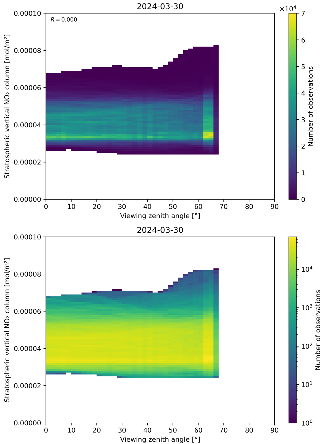
Figure 164: Scatter density plot of “Viewing zenith angle” against “Stratospheric vertical NO 2 column” for 2024-03-30 to 2024-03-31.
