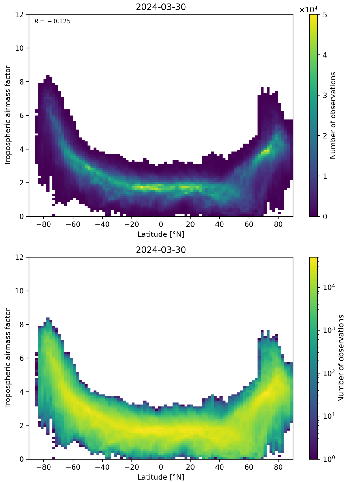
Figure 85: Scatter density plot of “Latitude” against “Tropospheric airmass factor” for 2024-03-30 to 2024-03-31.
