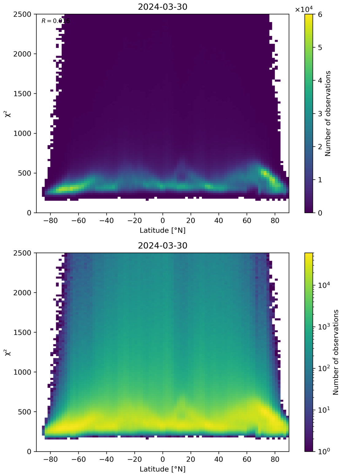
Figure 86: Scatter density plot of “Latitude” against “ \chi^2 ” for 2024-03-30 to 2024-03-31.
