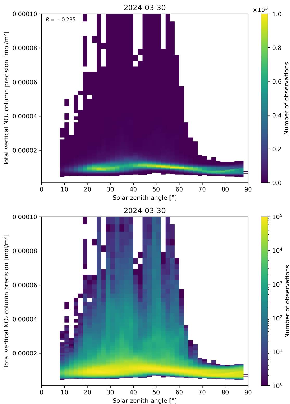
Figure 154: Scatter density plot of “Solar zenith angle” against “Total vertical NO 2 column precision” for 2024-03-30 to 2024-03-31.
