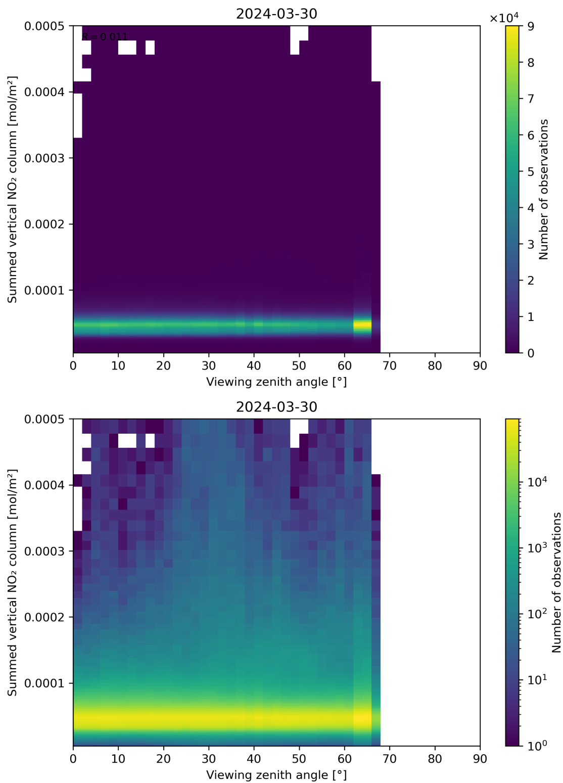
Figure 165: Scatter density plot of “Viewing zenith angle” against “Summed vertical NO 2 column” for 2024-03-30 to 2024-03-31.
