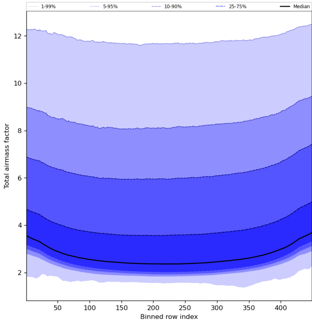
Figure 49: Along track statistics of “Total airmass factor” for 2024-03-30 to 2024-03-31
