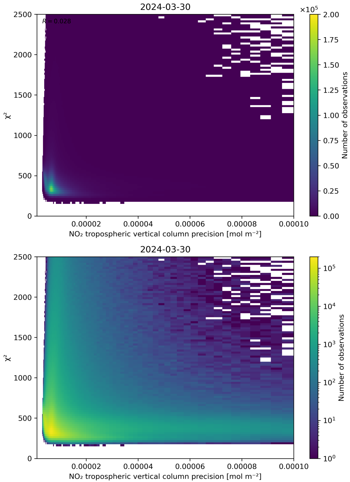
Figure 134: Scatter density plot of “NO 2 tropospheric vertical column precision” against “ \chi^2 ” for 2024-03-30 to 2024-03-31.
