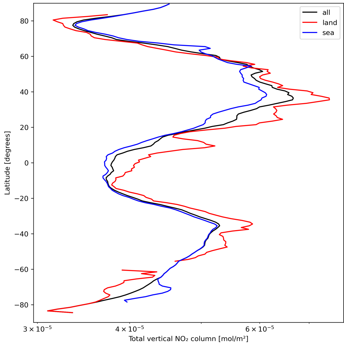
Figure 21: Zonal average of “Total vertical NO 2 column” for 2024-03-30 to 2024-03-31.
