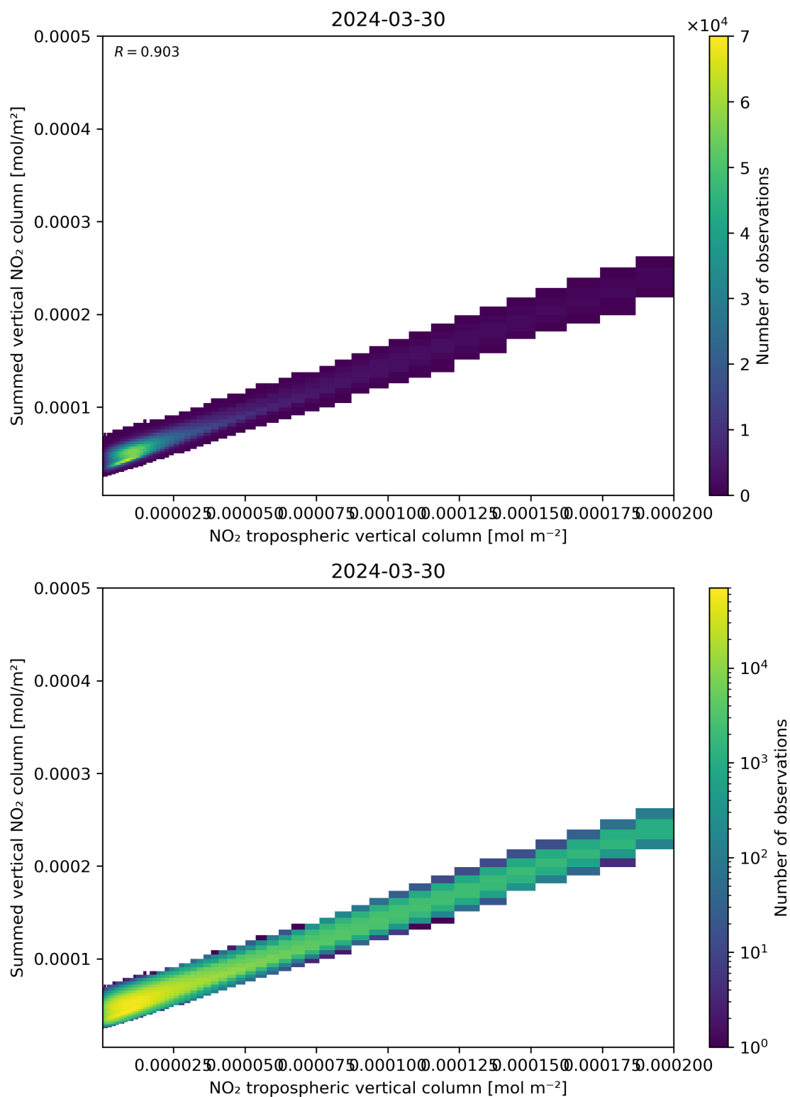
Figure 126: Scatter density plot of “NO 2 tropospheric vertical column” against “Summed vertical NO 2 column” for 2024-03-30 to 2024-03-31.
