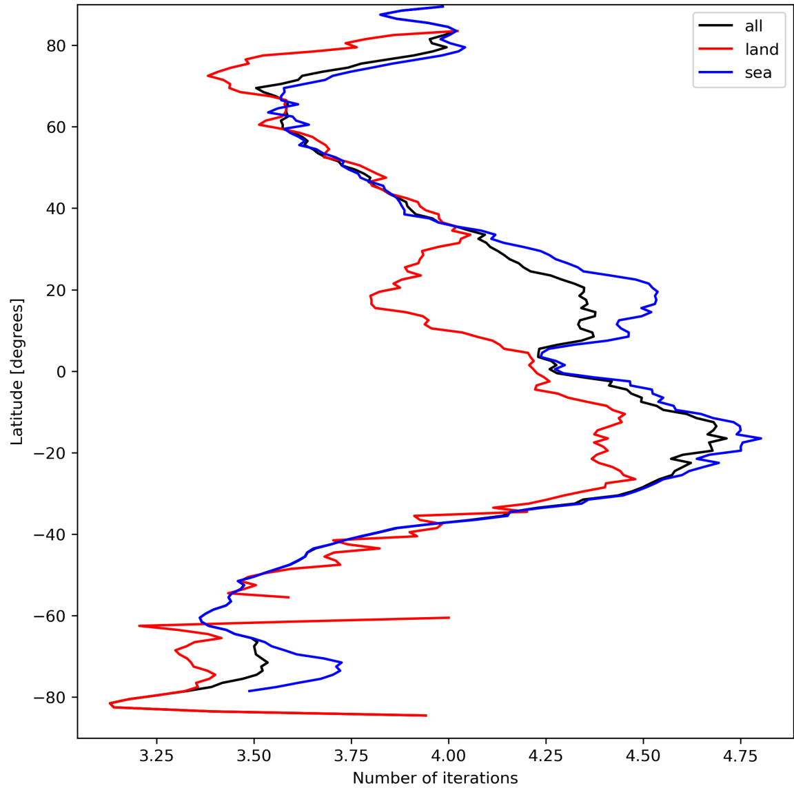
Figure 17: Zonal average of “Number of iterations” for 2024-03-30 to 2024-03-31.
