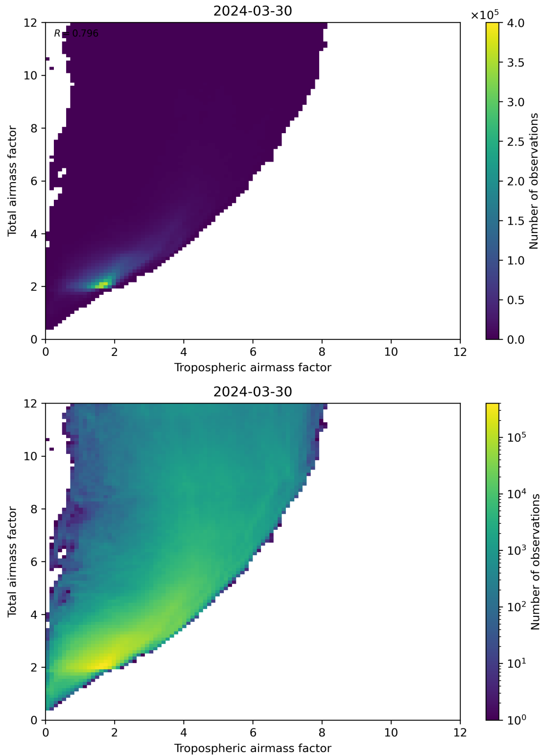
Figure 72: Scatter density plot of “Tropospheric airmass factor” against “Total airmass factor” for 2024-03-30 to 2024-03-31.
