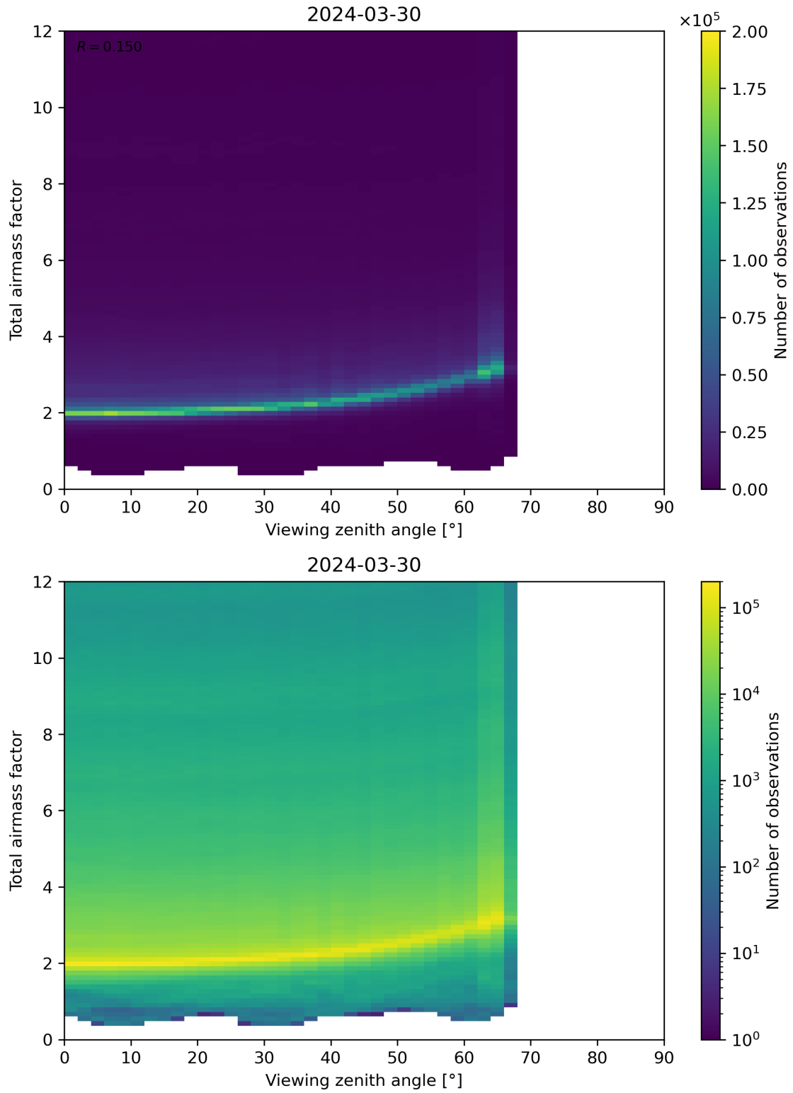
Figure 160: Scatter density plot of “Viewing zenith angle” against “Total airmass factor” for 2024-03-30 to 2024-03-31.
