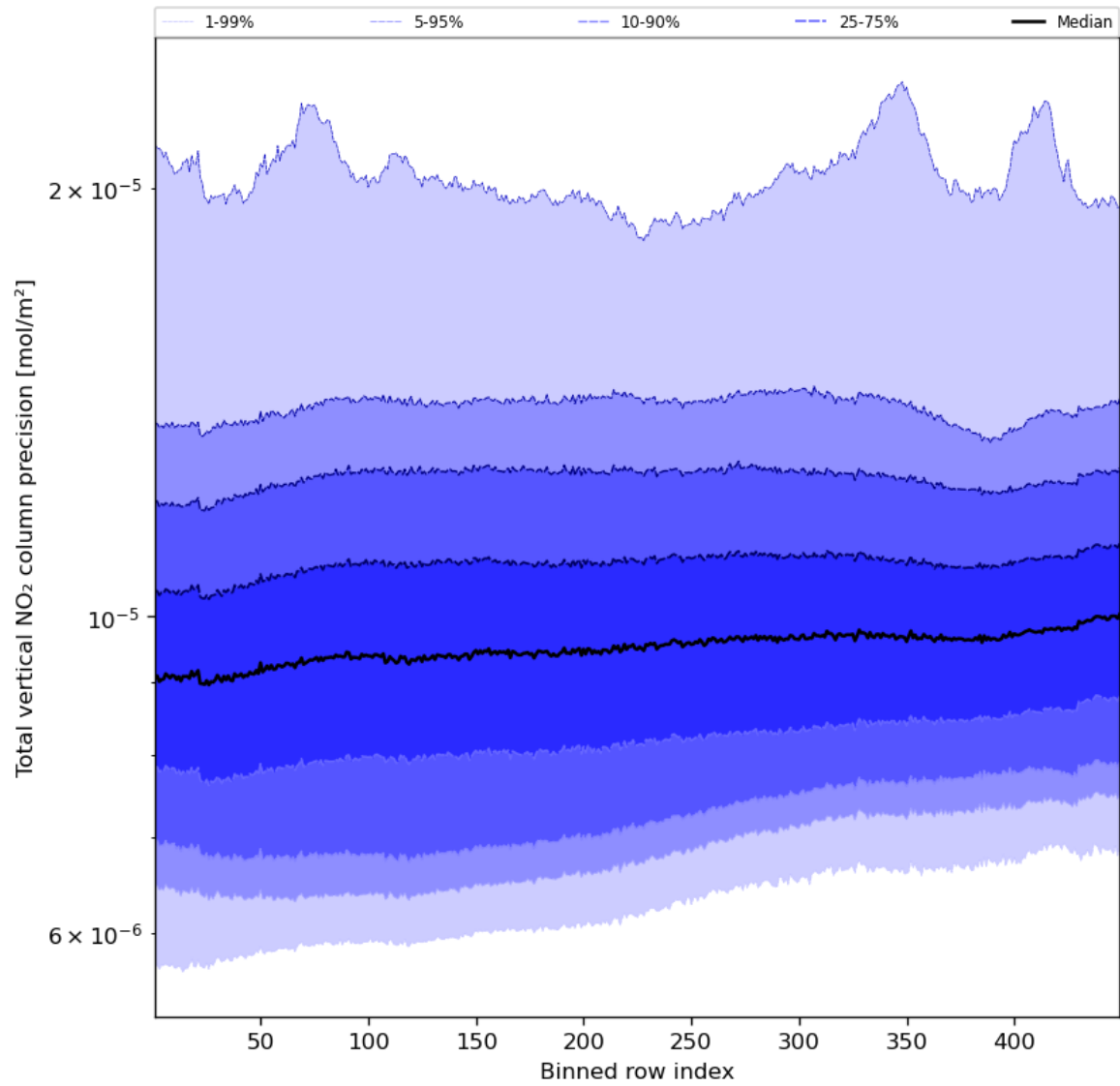
Figure 56: Along track statistics of “Total vertical NO 2 column precision” for 2024-03-30 to 2024-03-31
