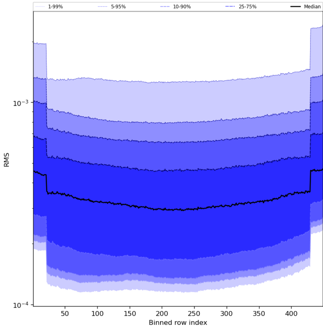
Figure 60: Along track statistics of “RMS” for 2024-03-30 to 2024-03-31
