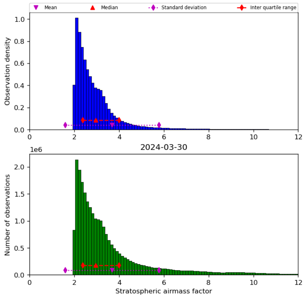
Figure 44: Histogram of "Stratospheric airmass factor" for 2024-03-30 to 2024-03-31
