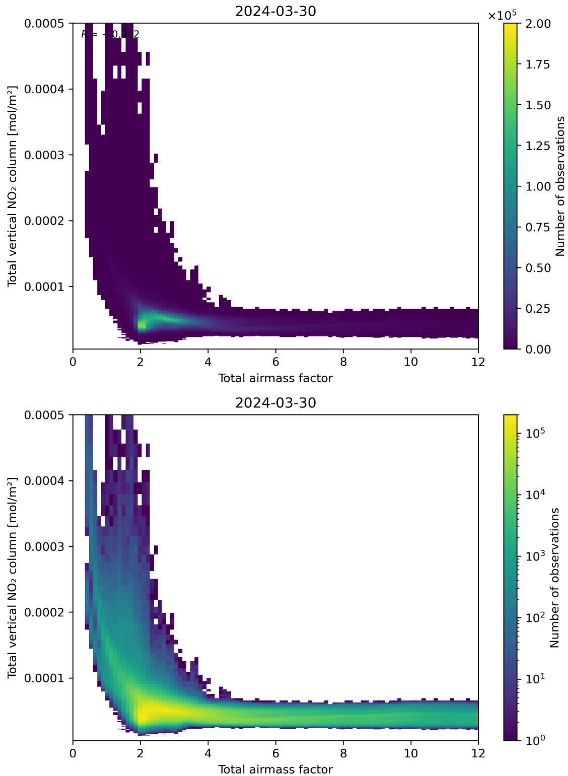
Figure 67: Scatter density plot of “Total airmass factor” against “Total vertical NO 2 column” for 2024-03-30 to 2024-03-31.
