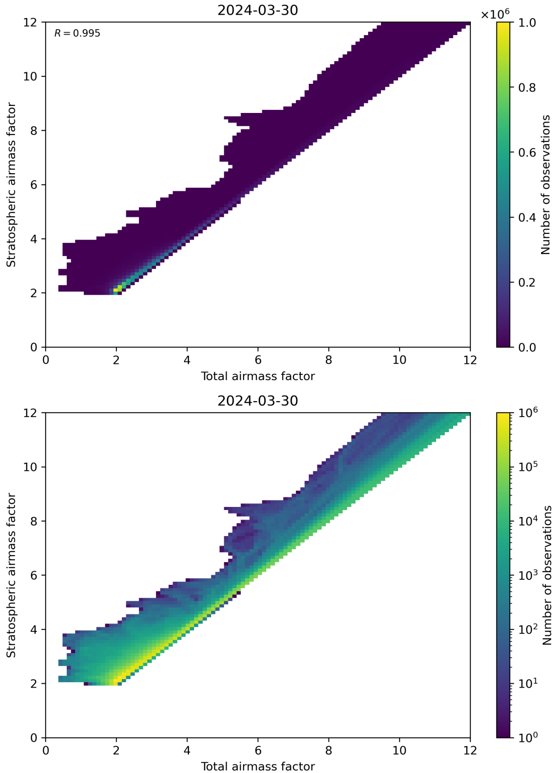
Figure 62: Scatter density plot of “Total airmass factor” against “Stratospheric airmass factor” for 2024-03-30 to 2024-03-31.
