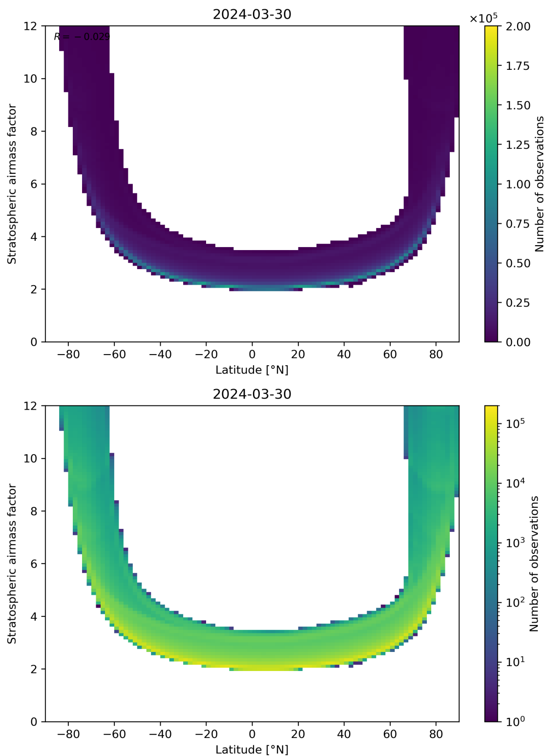
Figure 83: Scatter density plot of “Latitude” against “Stratospheric air mass factor” for 2024-03-30 to 2024-03-31.
