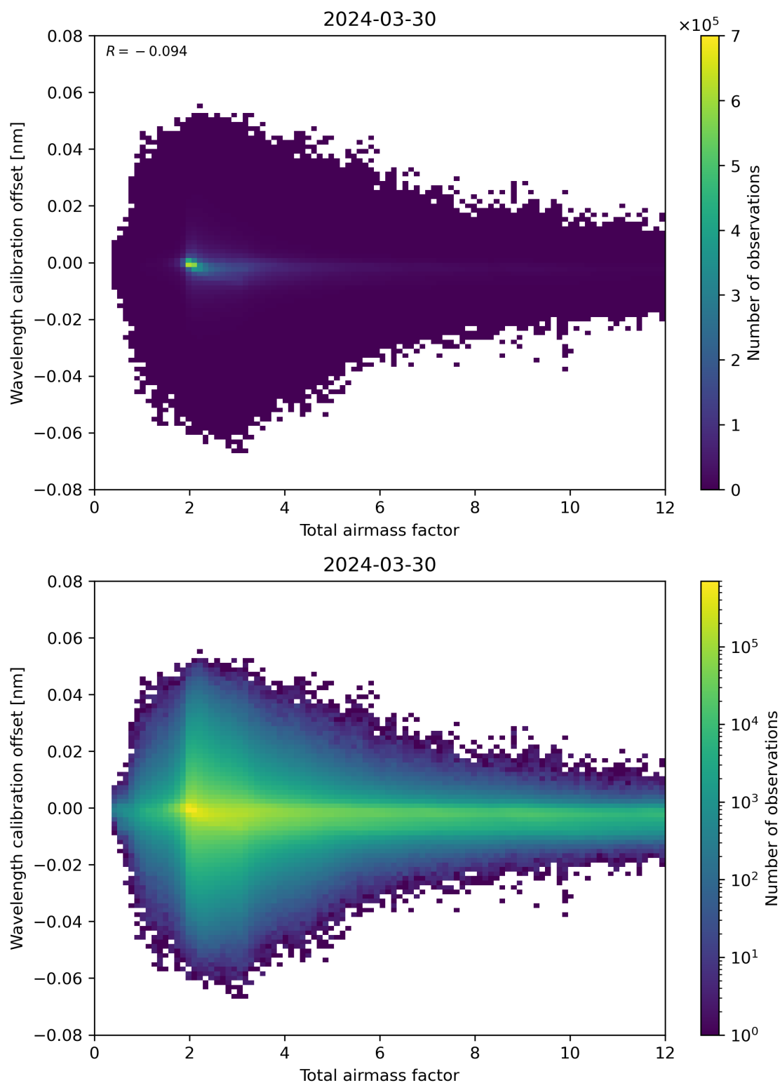
Figure 70: Scatter density plot of “Total airmass factor” against “Wavelength calibration offset” for 2024-03-30 to 2024-03-31.
