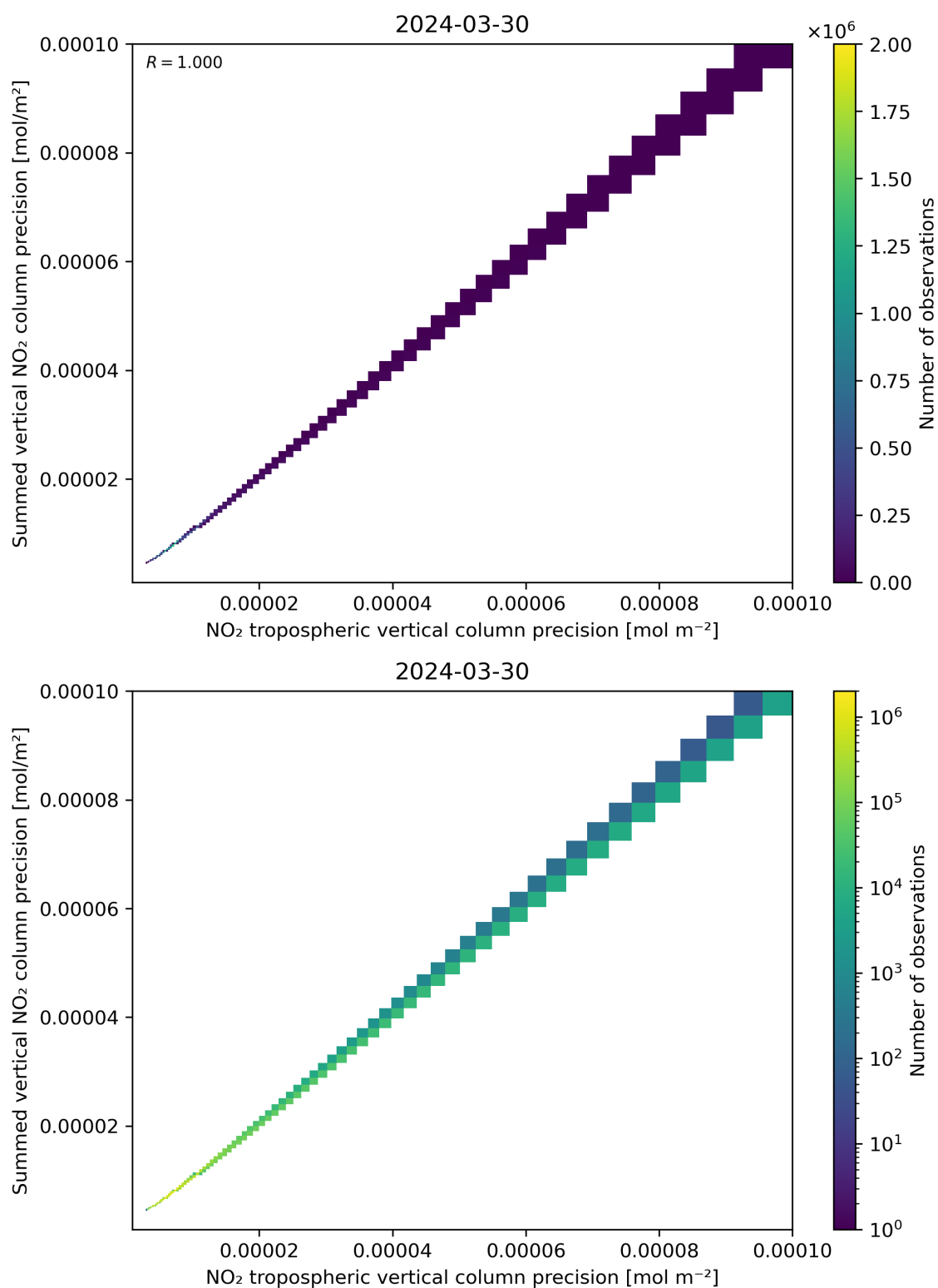
Figure 137: Scatter density plot of “NO 2 tropospheric vertical column precision” against “Summed vertical NO 2 column precision” for 2024-03-30 to 2024-03-31.
