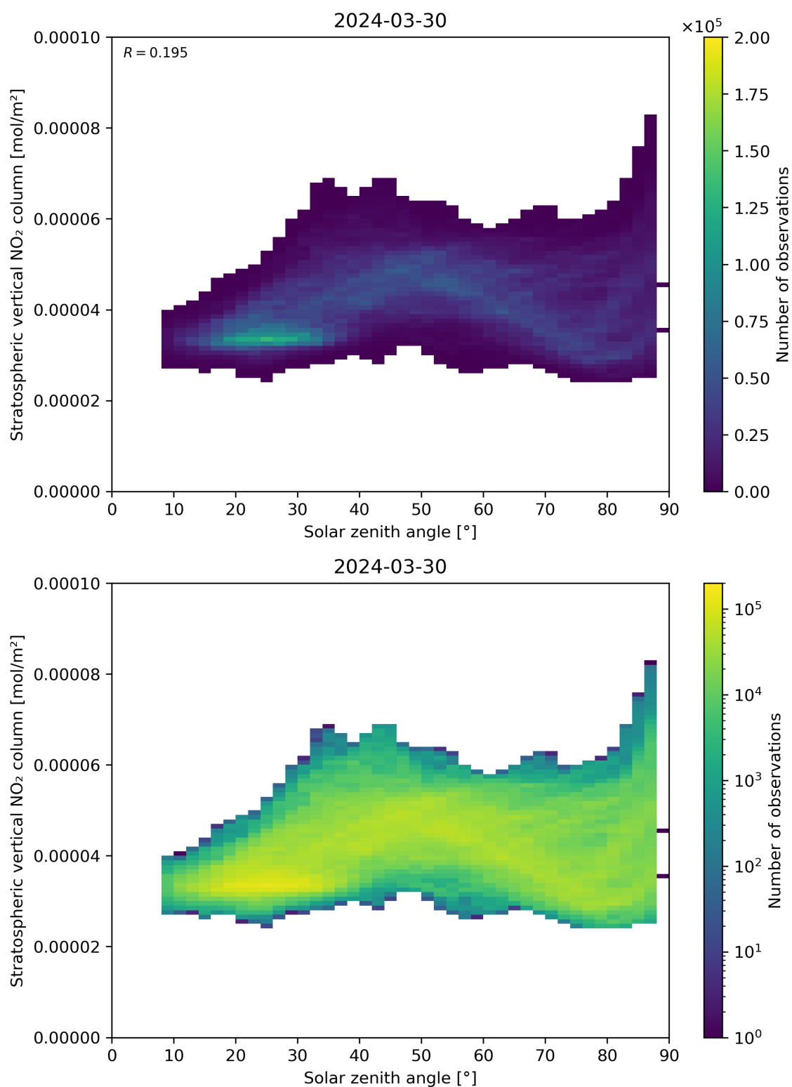
Figure 150: Scatter density plot of “Solar zenith angle” against “Stratospheric vertical NO 2 column” for 2024-03-30 to 2024-03-31.
