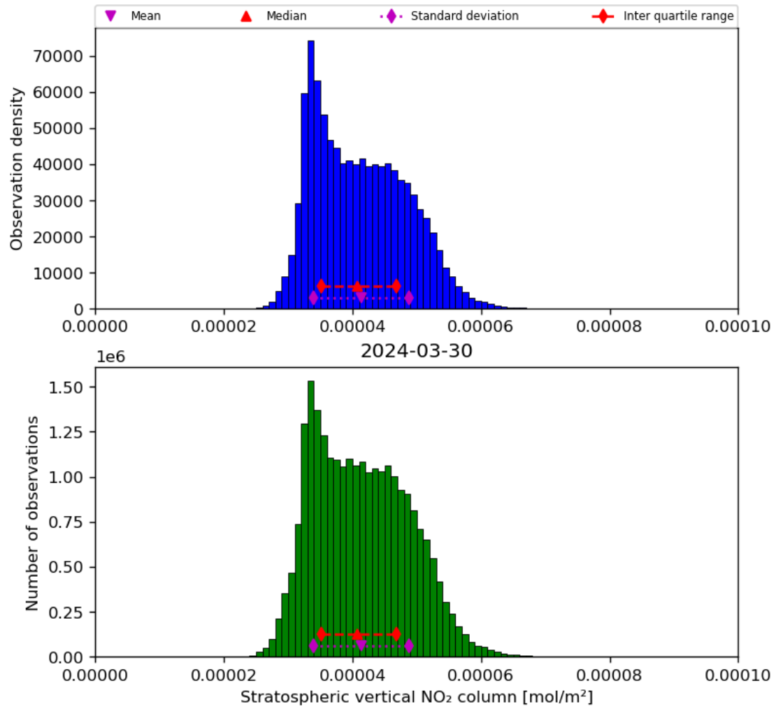
Figure 36: Histogram of “Stratospheric vertical NO 2 column” for 2024-03-30 to 2024-03-31
