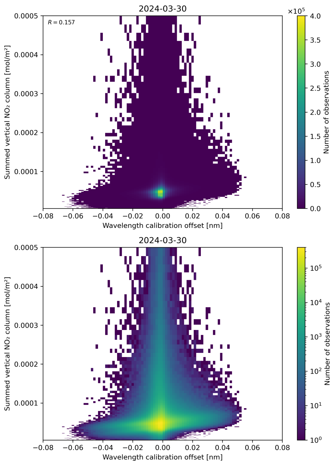
Figure 177: Scatter density plot of “Wavelength calibration offset” against “Summed vertical NO 2 column” for 2024-03-30 to 2024-03-31.
