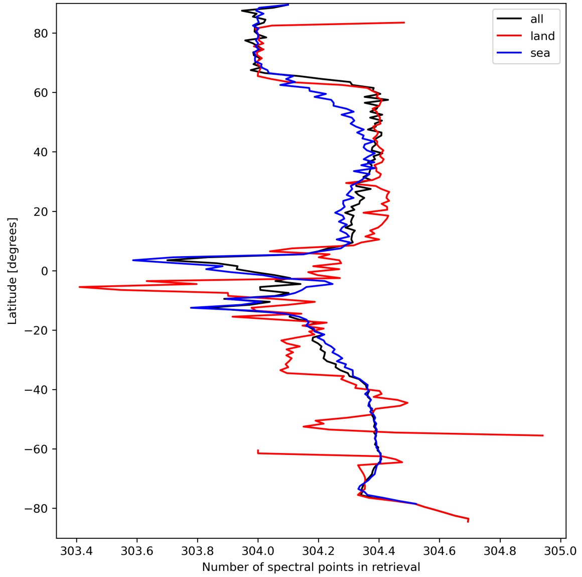
Figure 16: Zonal average of “Number of spectral points in retrieval” for 2024-03-30 to 2024-03-31.
