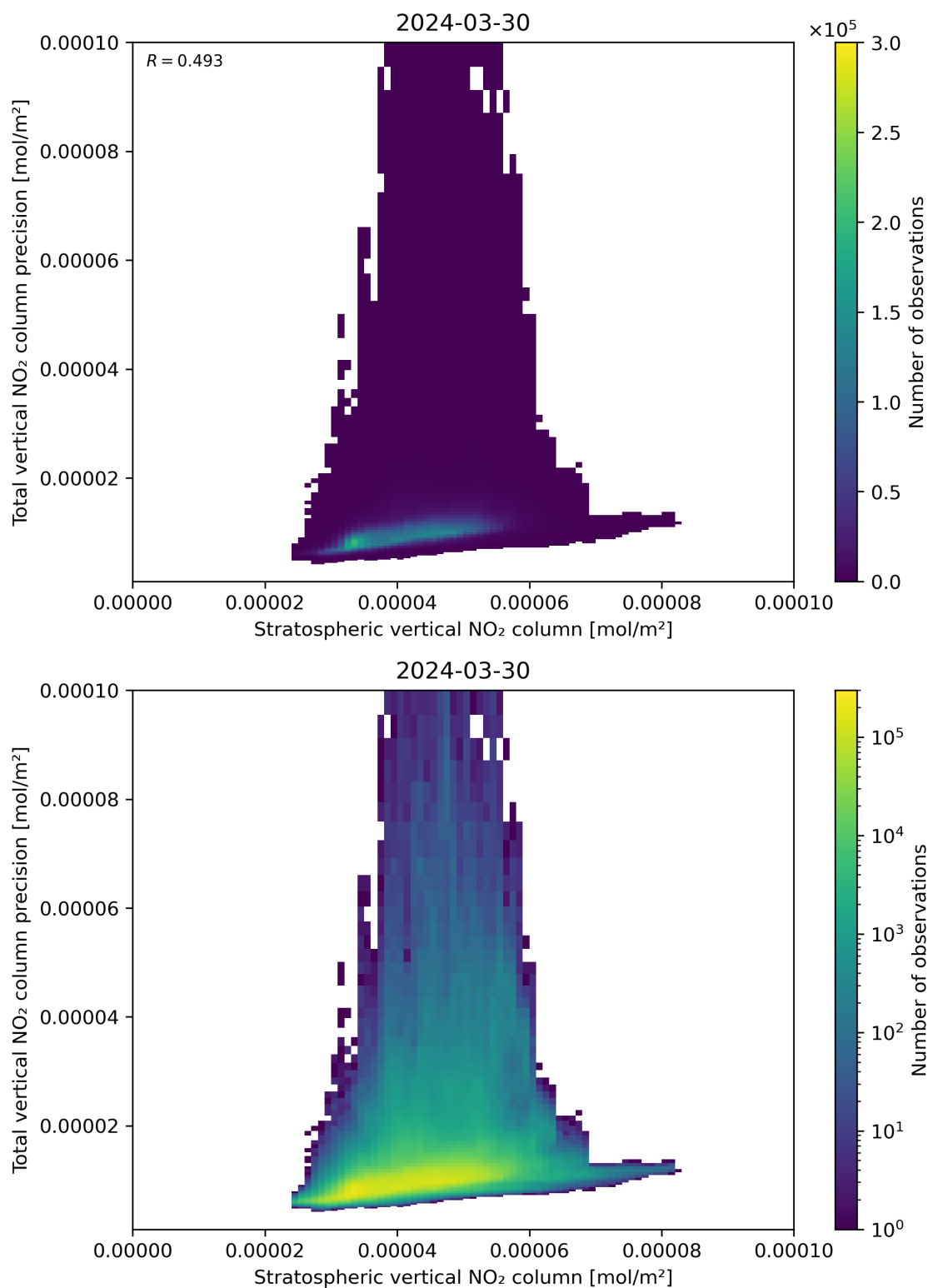
Figure 101: Scatter density plot of “Stratospheric vertical NO 2 column” against “Total vertical NO 2 column precision” for 2024-03-30 to 2024-03-31.
