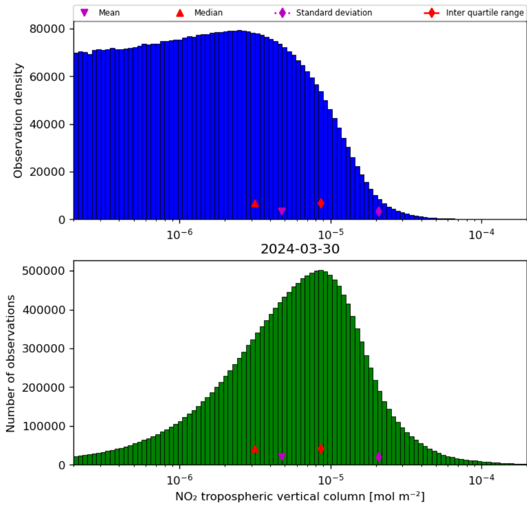
Figure 29: Histogram of “NO 2 tropospheric vertical column” for 2024-03-30 to 2024-03-31
