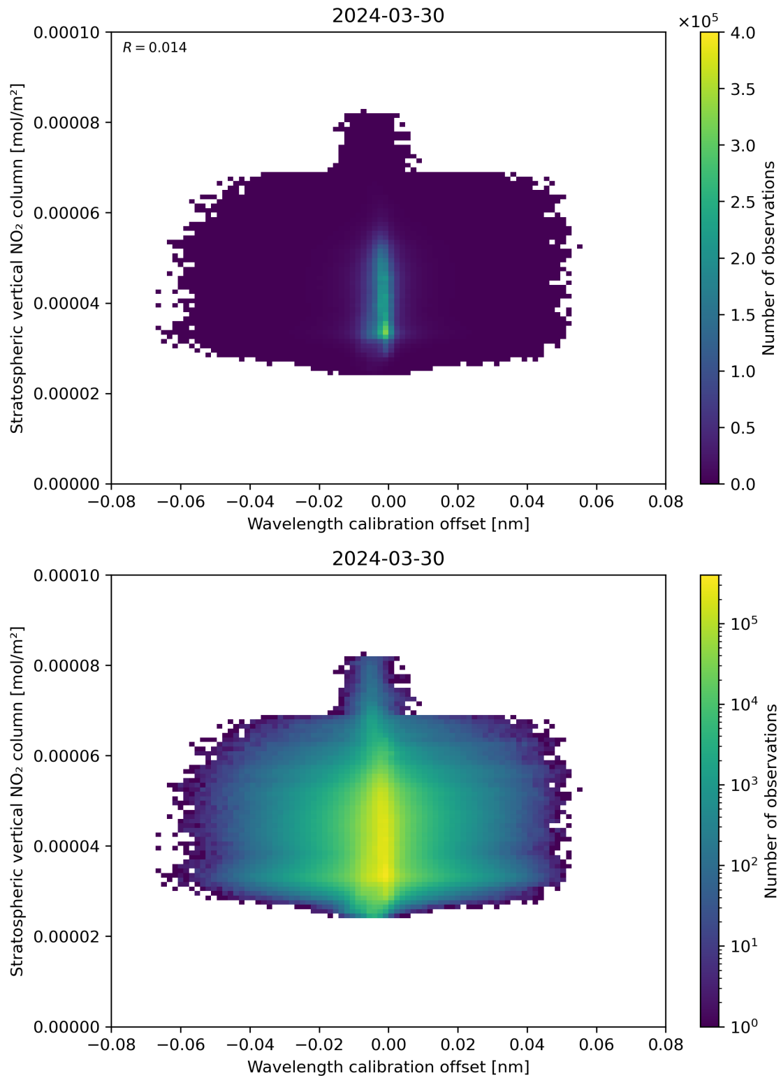
Figure 176: Scatter density plot of “Wavelength calibration offset” against “Stratospheric vertical NO 2 column” for 2024-03-30 to 2024-03-31.
