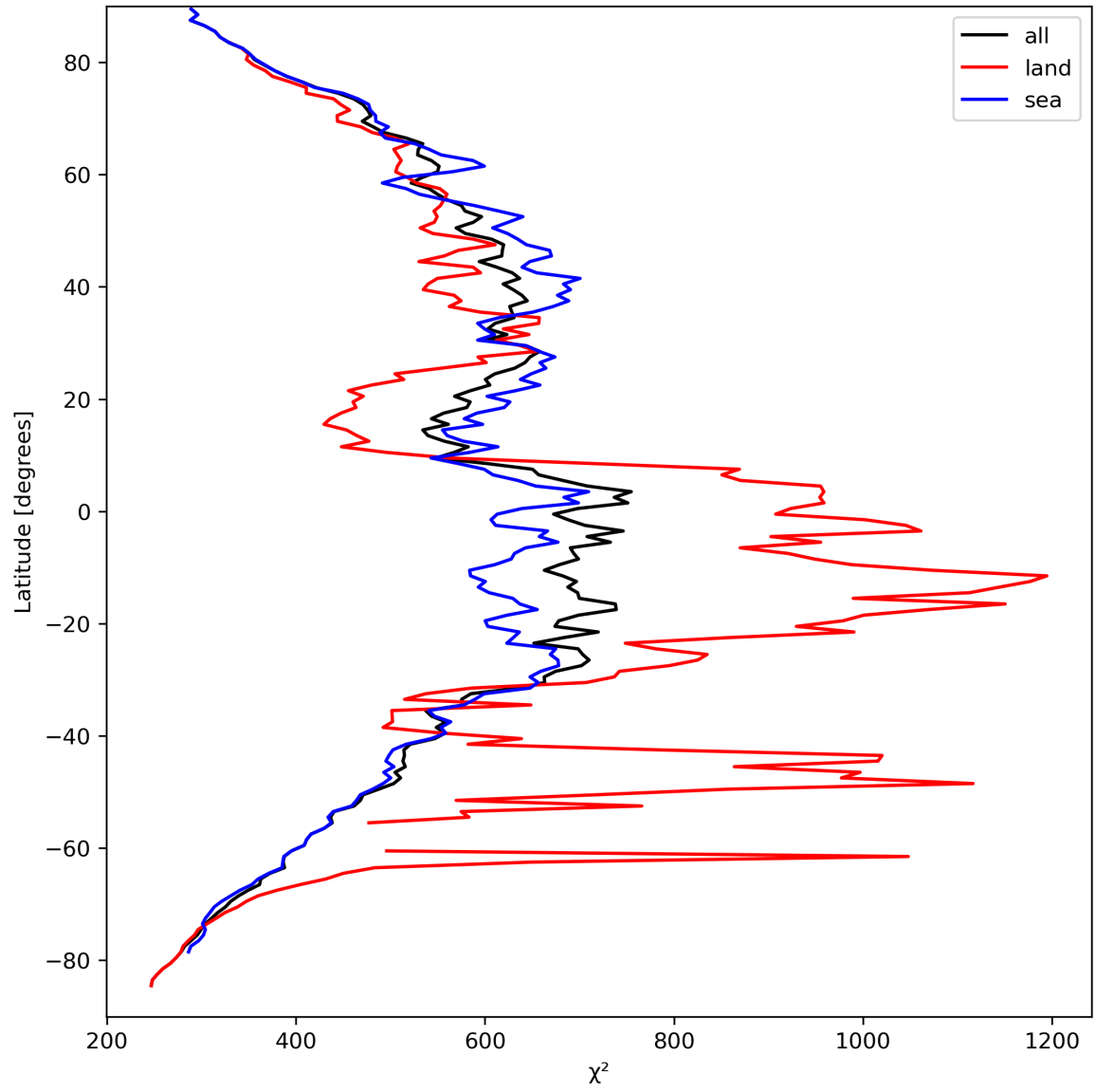
Figure 25: Zonal average of “ \chi^2 ” for 2024-03-30 to 2024-03-31.
