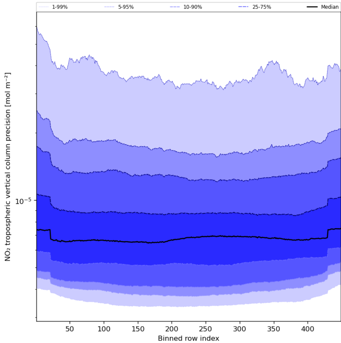
Figure 47: Along track statistics of “NO 2 tropospheric vertical column precision” for 2024-03-30 to 2024-03-31
