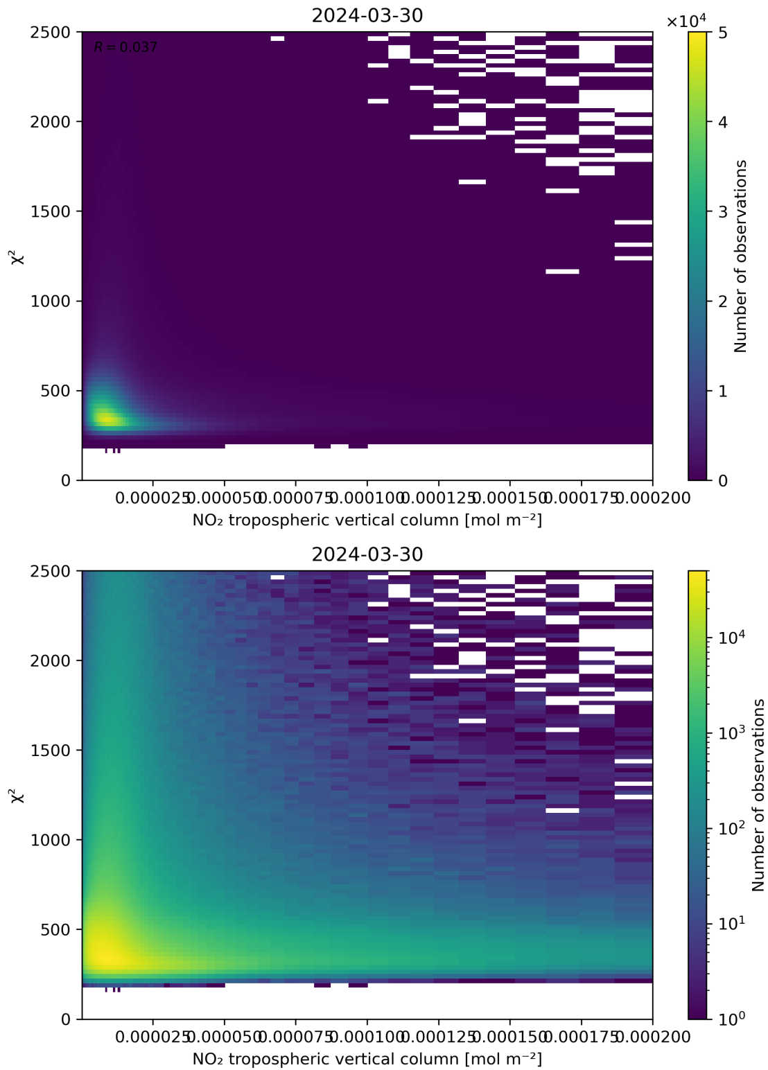
Figure 124: Scatter density plot of “NO 2 tropospheric vertical column” against “ \chi^2 ” for 2024-03-30 to 2024-03-31.
