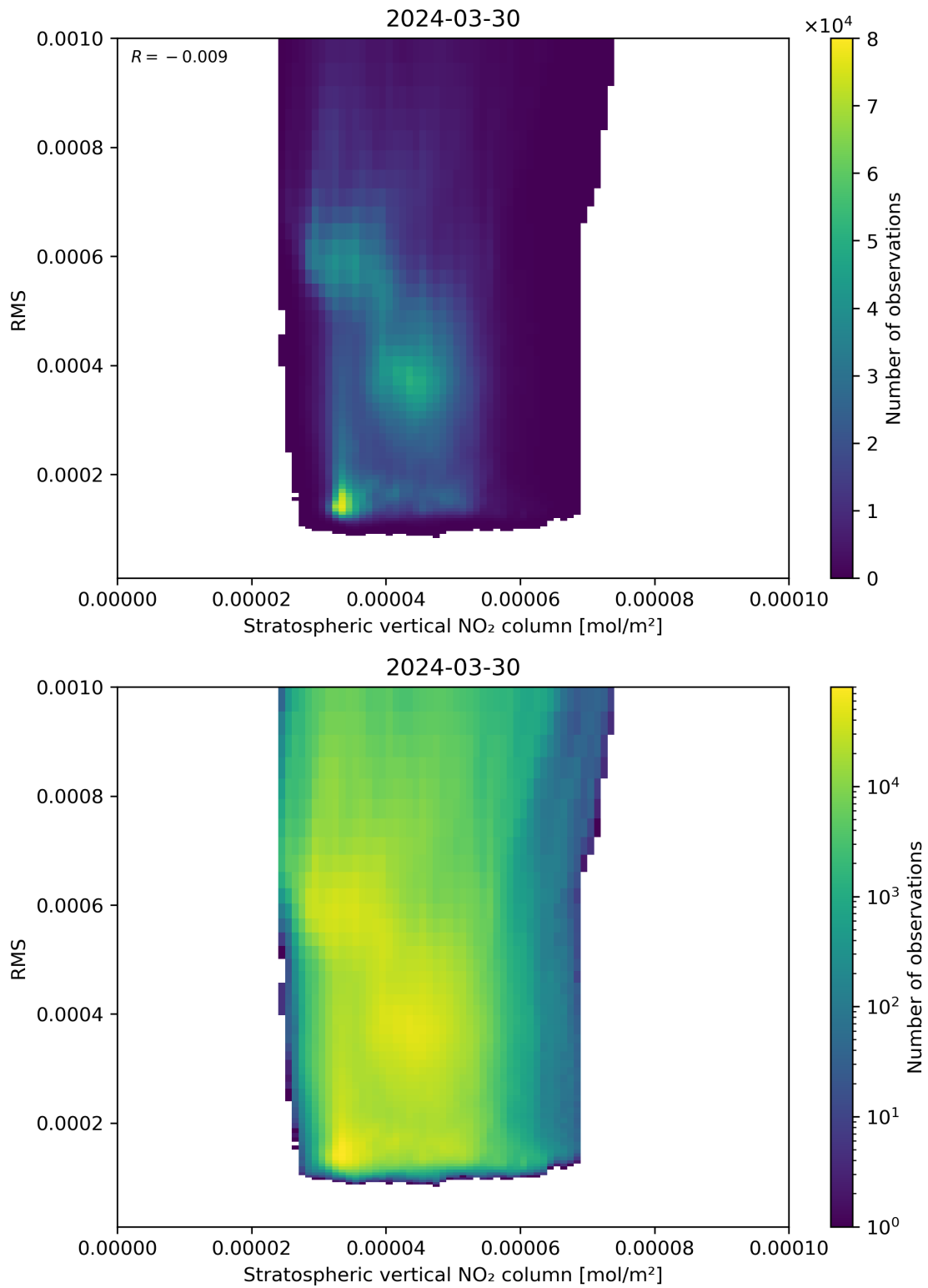
Figure 102: Scatter density plot of “Stratospheric vertical NO 2 column” against “RMS” for 2024-03-30 to 2024-03-31.
