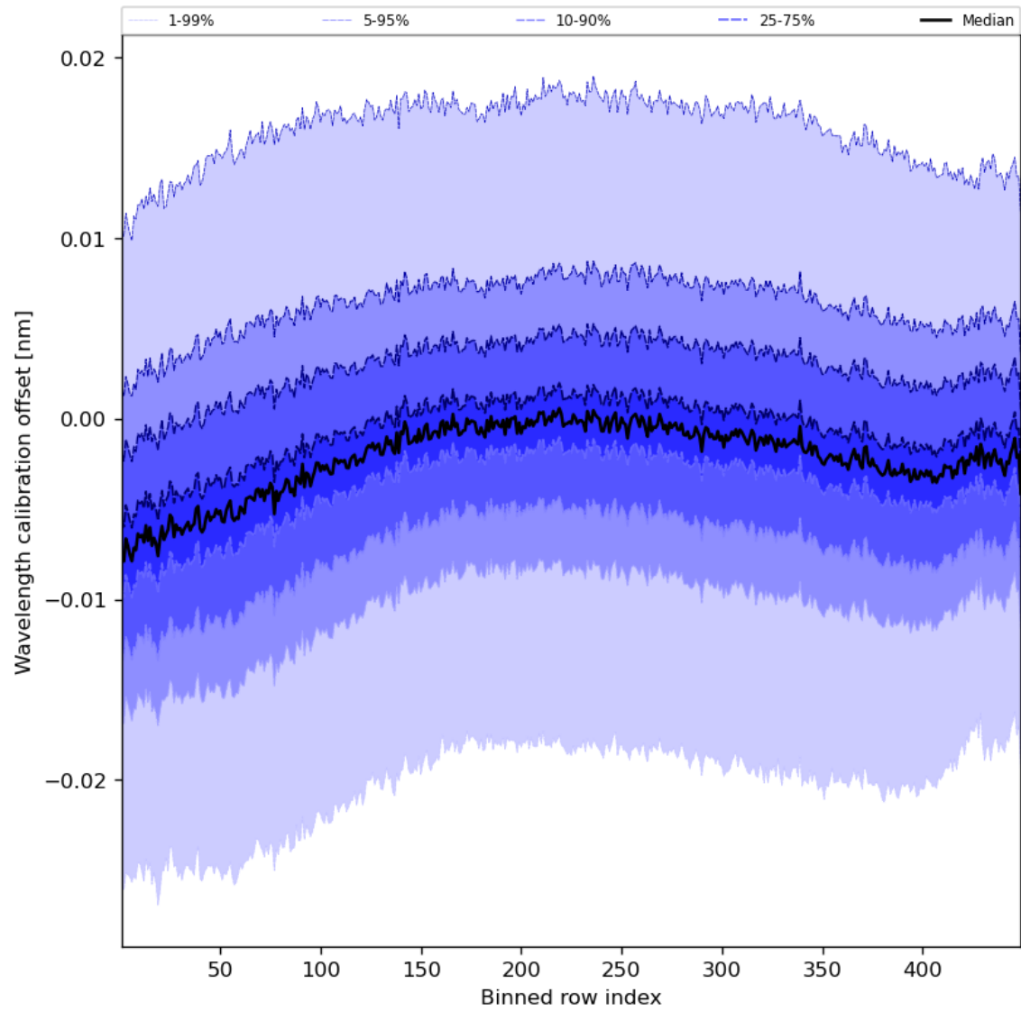
Figure 52: Along track statistics of “Wavelength calibration offset” for 2024-03-30 to 2024-03-31
