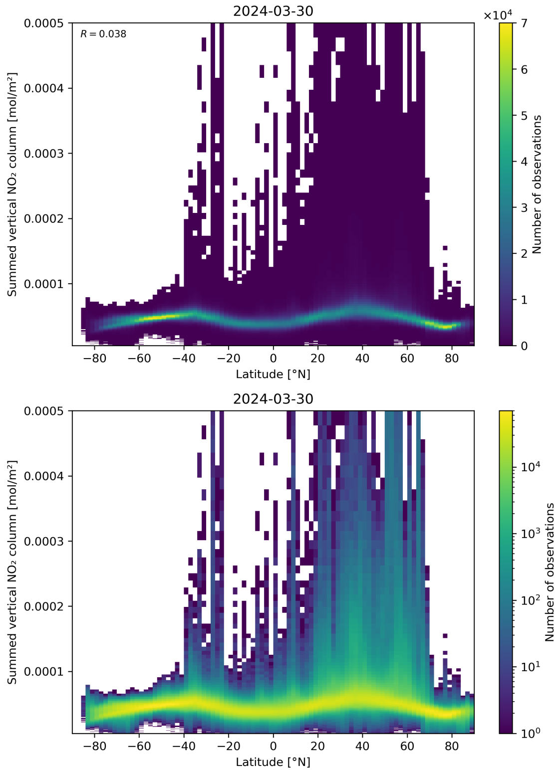
Figure 88: Scatter density plot of “Latitude” against “Summed vertical NO 2 column” for 2024-03-30 to 2024-03-31.
