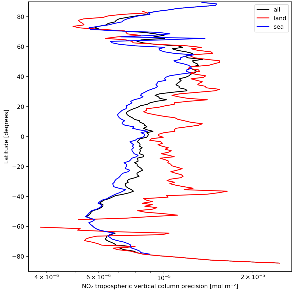
Figure 13: Zonal average of “NO 2 tropospheric vertical column precision” for 2024-03-30 to 2024-03-31.
