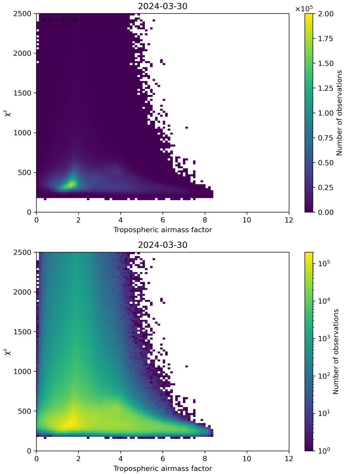
Figure 73: Scatter density plot of “Tropospheric airmass factor” against “ \chi^2 ” for 2024-03-30 to 2024-03-31.
