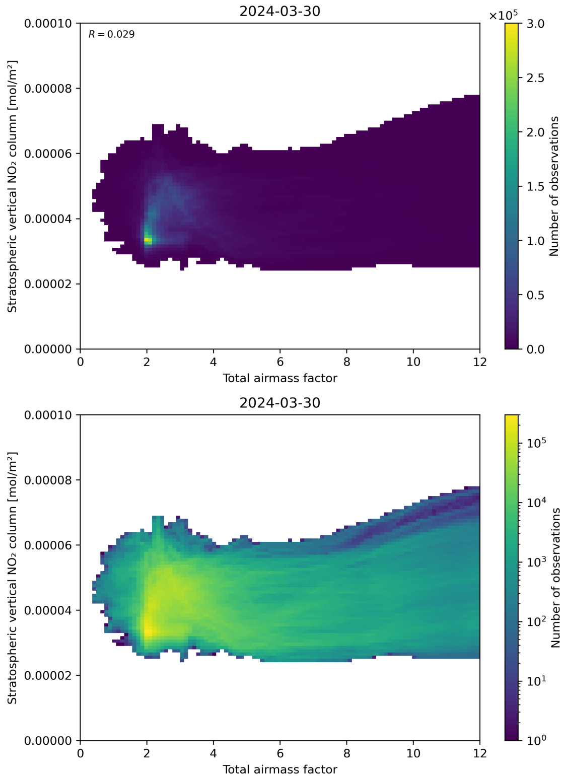
Figure 64: Scatter density plot of “Total airmass factor” against “Stratospheric vertical \text{NO}_2 column” for 2024-03-30 to 2024-03-31.
