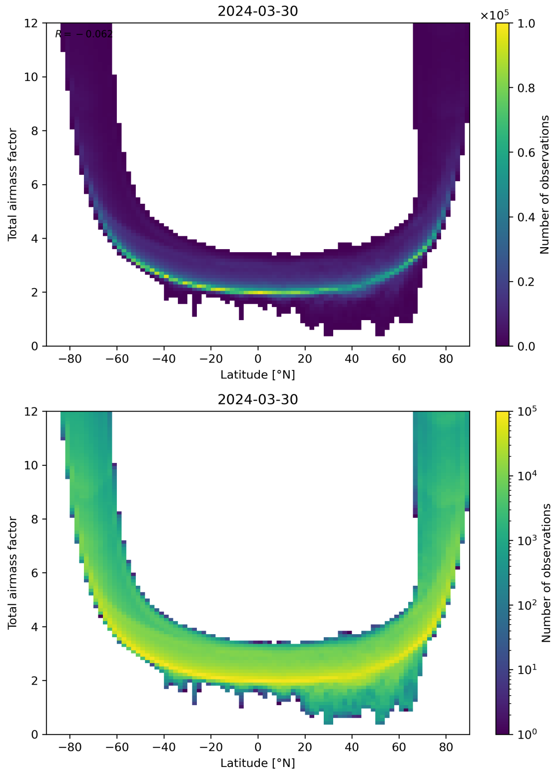
Figure 84: Scatter density plot of “Latitude” against “Total airmass factor” for 2024-03-30 to 2024-03-31.
