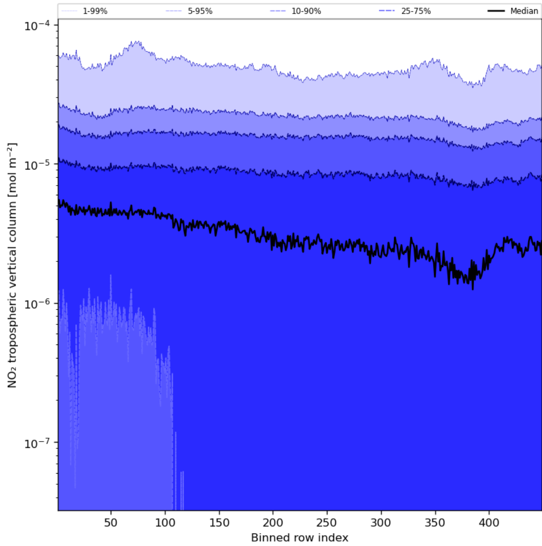
Figure 46: Along track statistics of “NO 2 tropospheric vertical column” for 2024-03-30 to 2024-03-31
