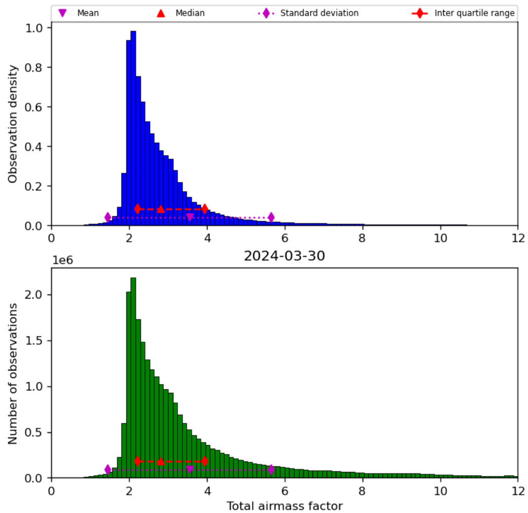
Figure 32: Histogram of “Total airmass factor” for 2024-03-30 to 2024-03-31
