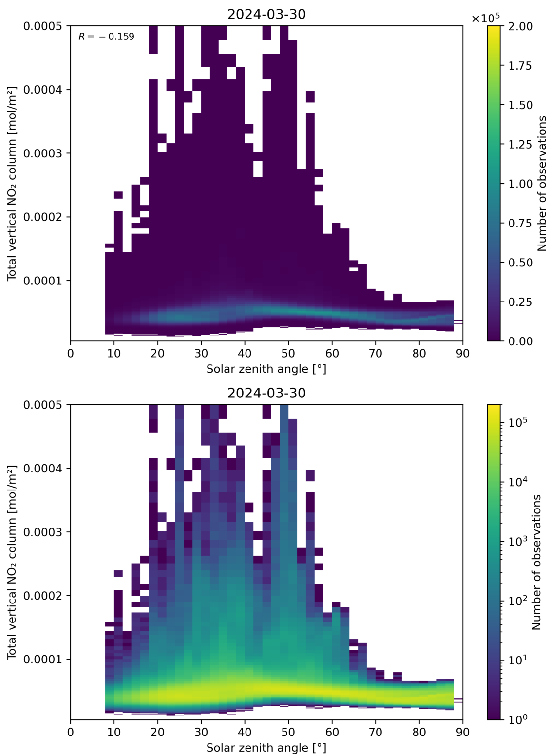
Figure 153: Scatter density plot of “Solar zenith angle” against “Total vertical NO 2 column” for 2024-03-30 to 2024-03-31.
