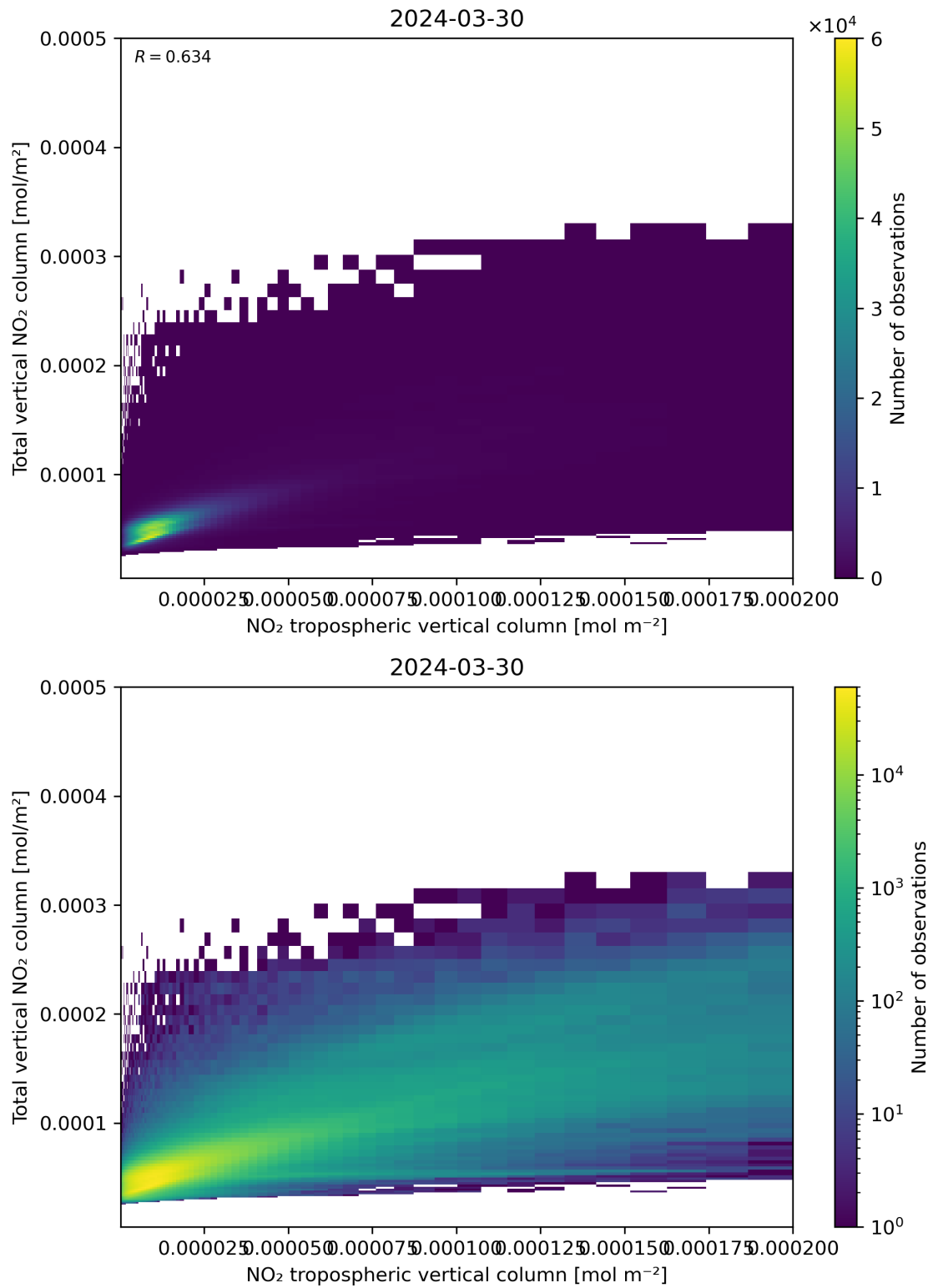
Figure 128: Scatter density plot of “NO 2 tropospheric vertical column” against “Total vertical NO 2 column” for 2024-03-30 to 2024-03-31.
