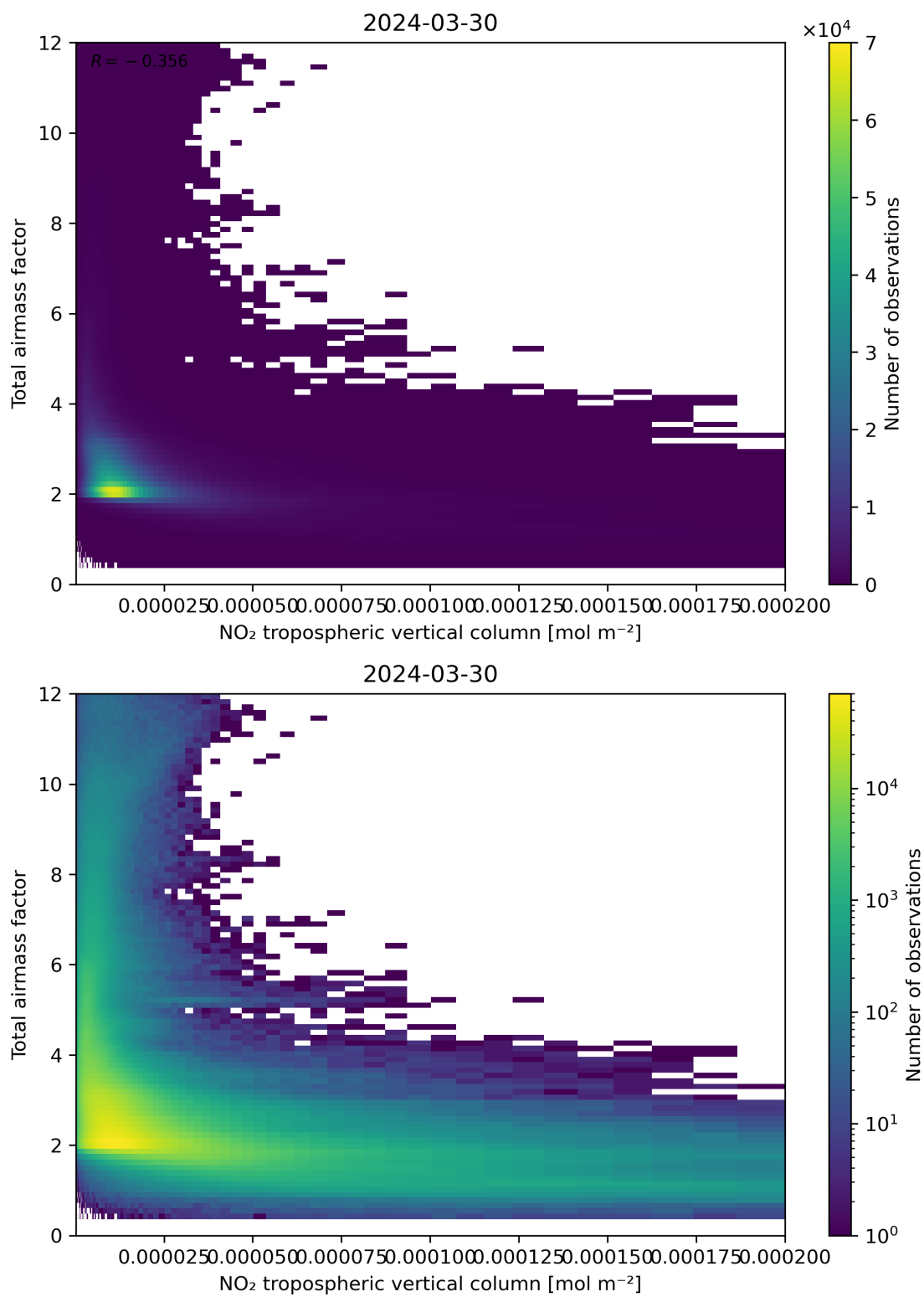
Figure 122: Scatter density plot of “NO 2 tropospheric vertical column” against “Total air mass factor” for 2024-03-30 to 2024-03-31.
