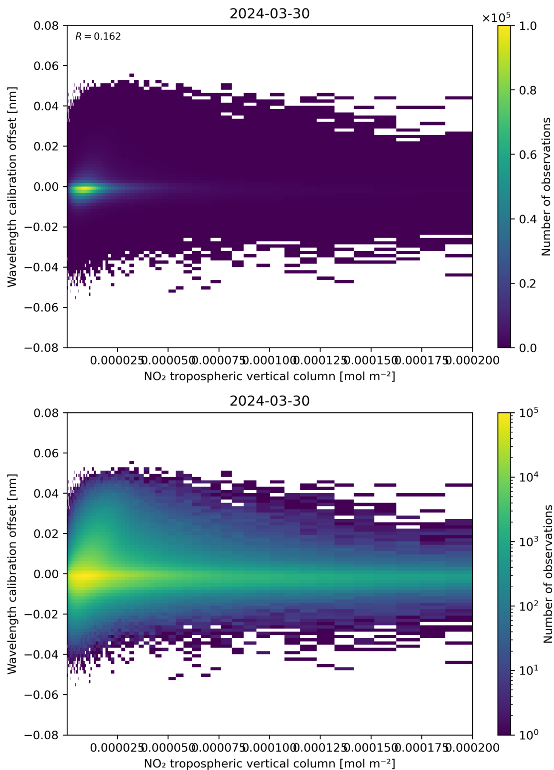
Figure 143: Scatter density plot of “NO 2 tropospheric vertical column” against “Wavelength calibration offset” for 2024-03-30 to 2024-03-31.
