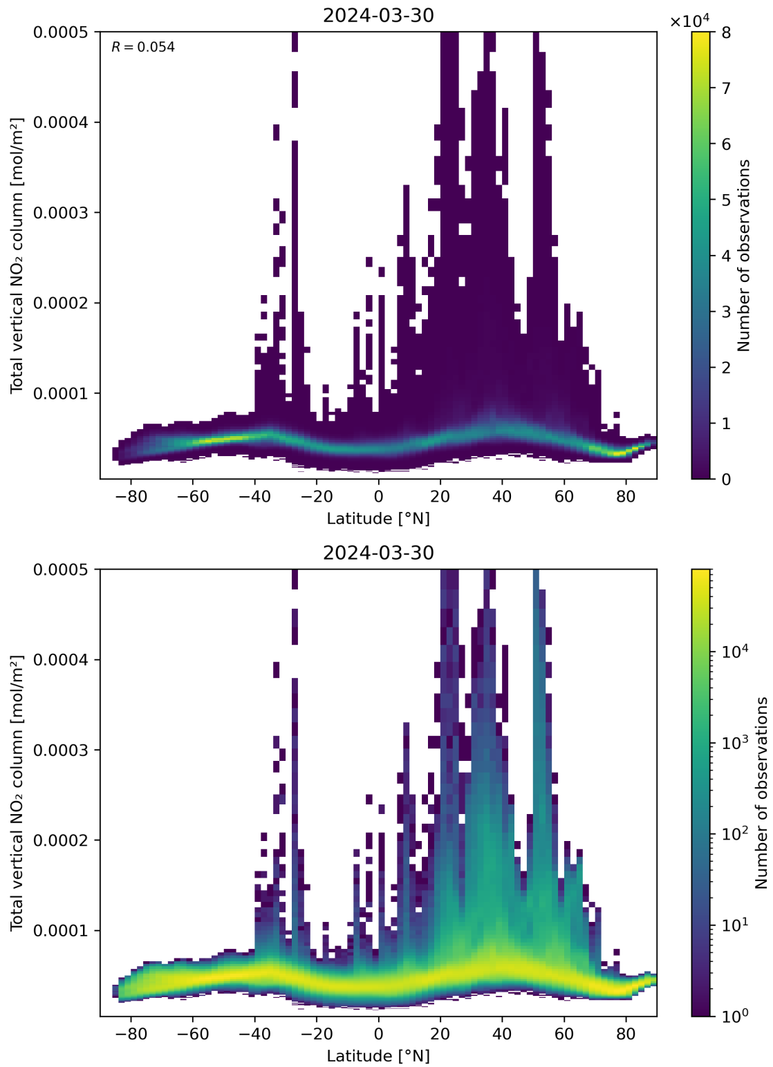
Figure 90: Scatter density plot of “Latitude” against “Total vertical NO 2 column” for 2024-03-30 to 2024-03-31.
