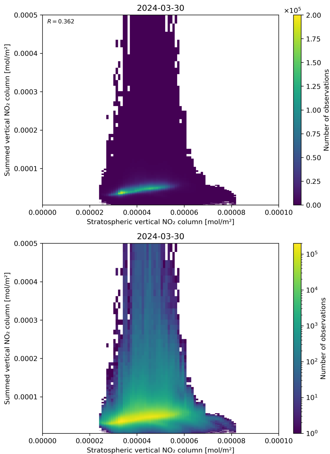
Figure 98: Scatter density plot of “Stratospheric vertical NO 2 column” against “Summed vertical NO 2 column” for 2024-03-30 to 2024-03-31.
