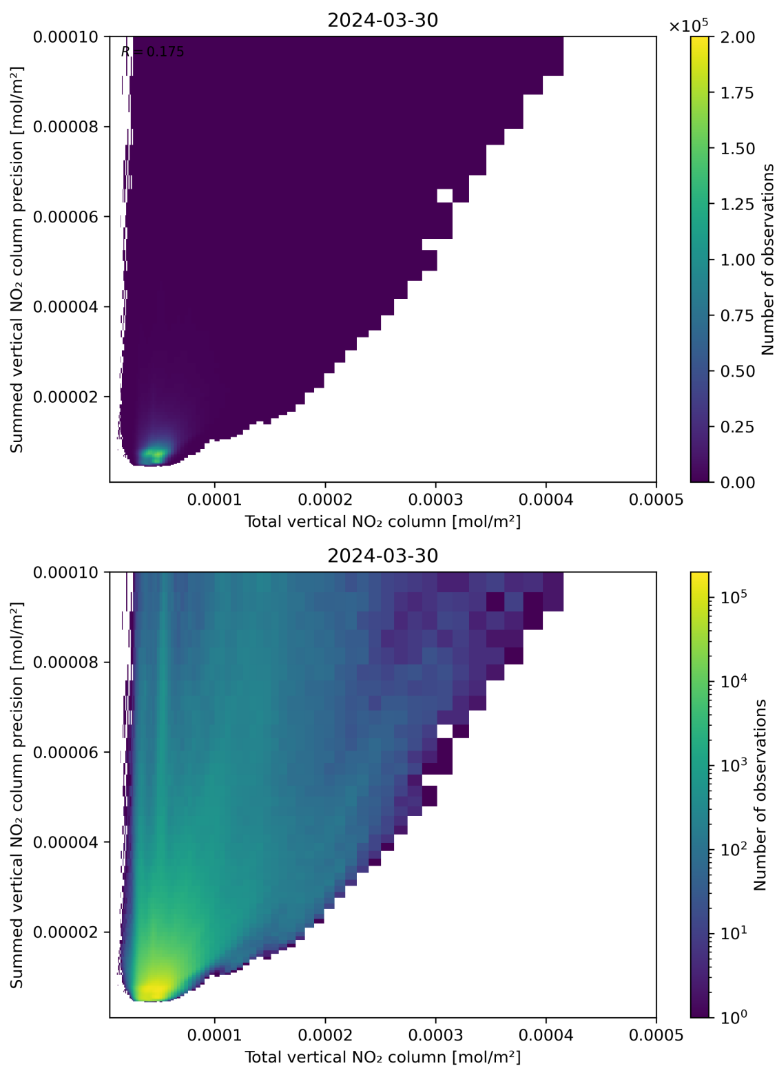
Figure 113: Scatter density plot of “Total vertical NO 2 column” against “Summed vertical NO 2 column precision” for 2024-03-30 to 2024-03-31.
