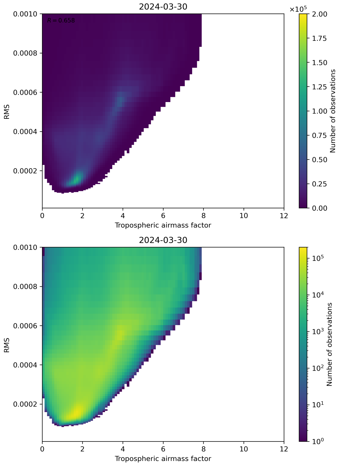
Figure 79: Scatter density plot of “Tropospheric airmass factor” against “RMS” for 2024-03-30 to 2024-03-31.
