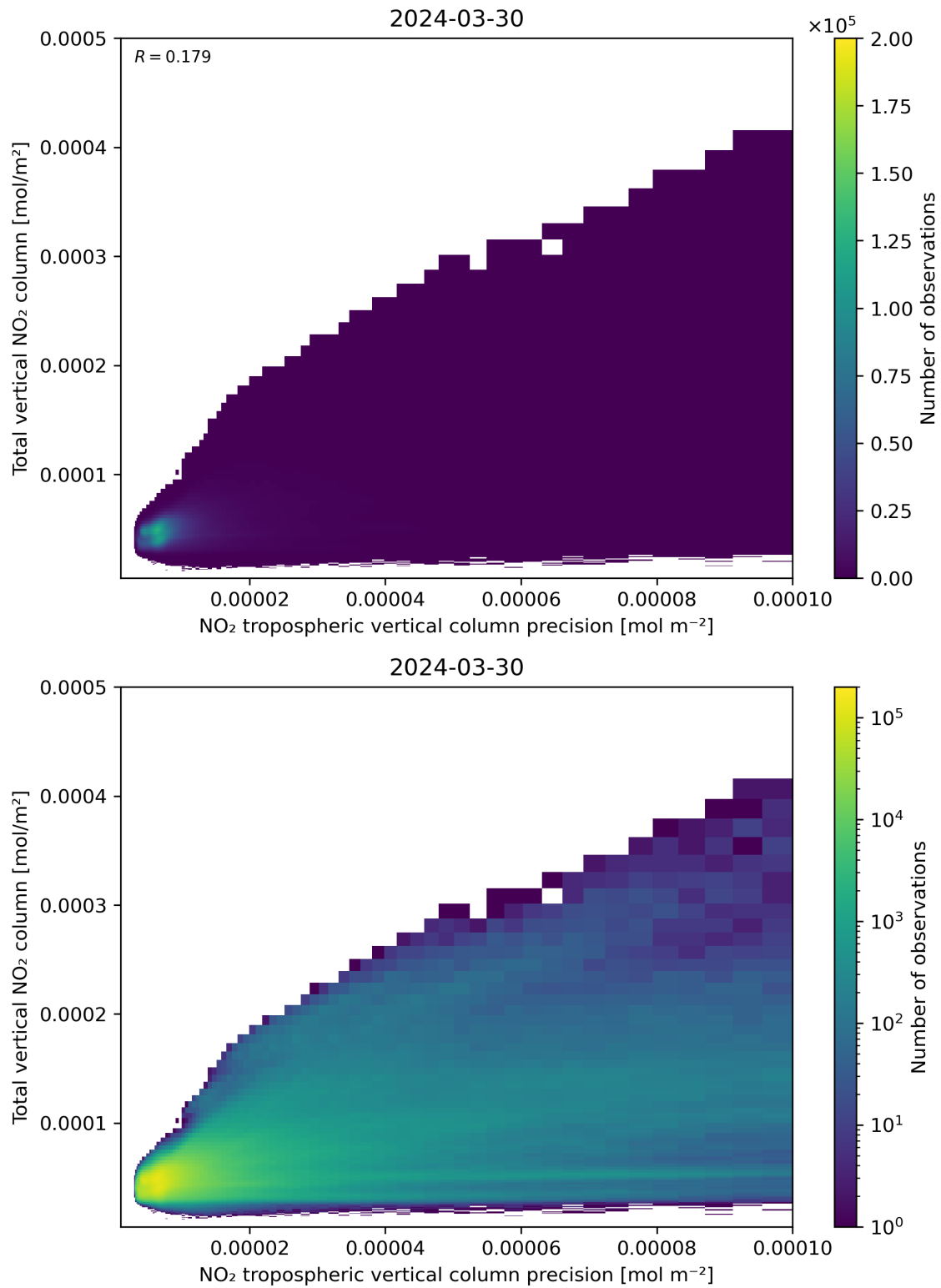
Figure 138: Scatter density plot of “NO 2 tropospheric vertical column precision” against “Total vertical NO 2 column” for 2024-03-30 to 2024-03-31.
