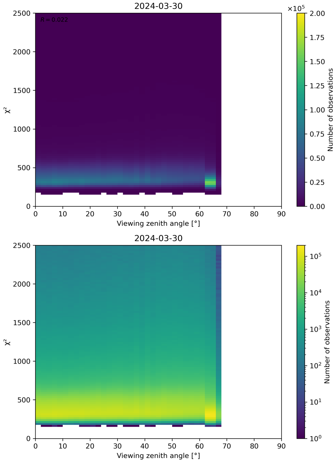
Figure 162: Scatter density plot of “Viewing zenith angle” against “ \chi^2 ” for 2024-03-30 to 2024-03-31.
