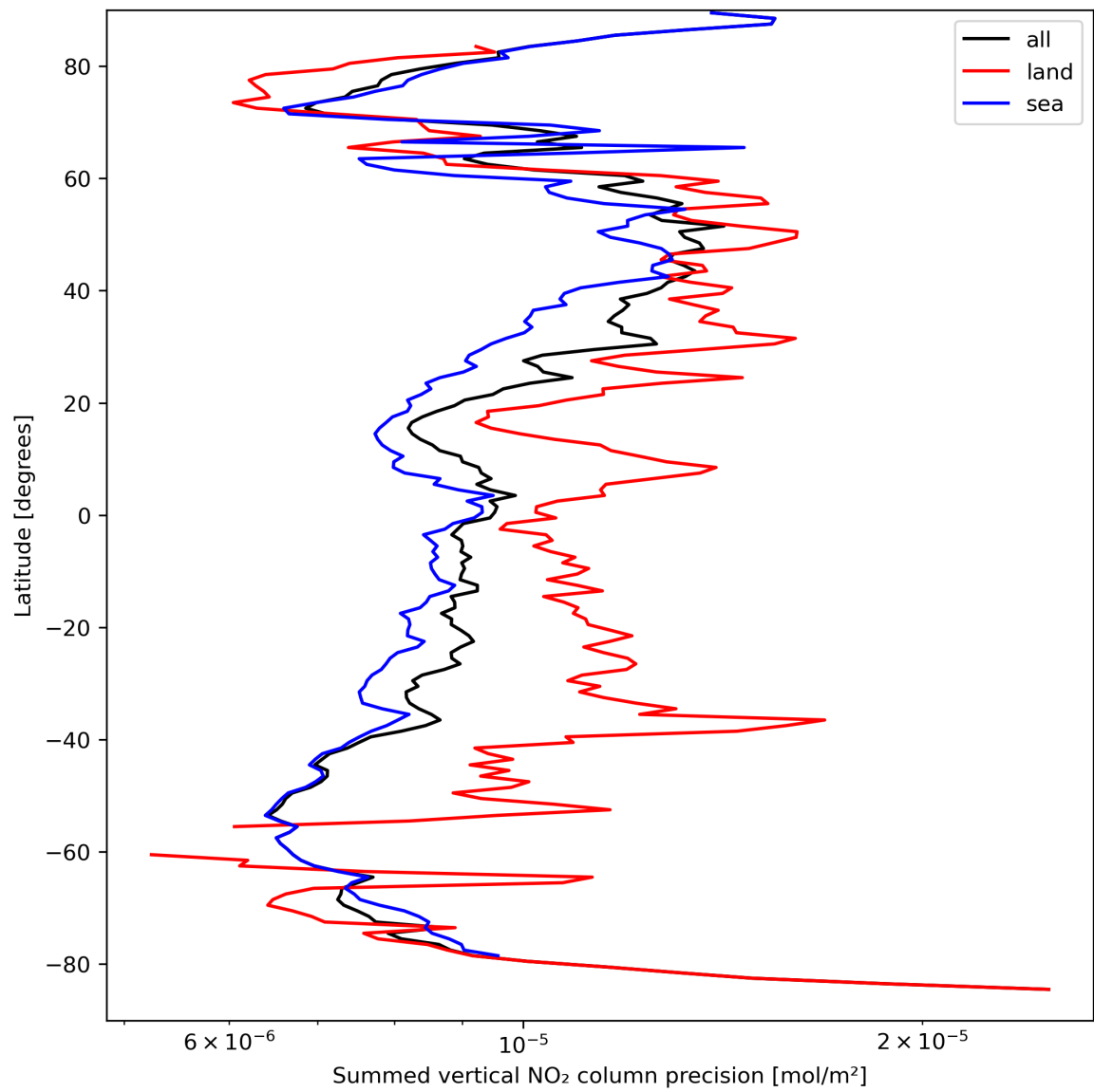
Figure 24: Zonal average of “Summed vertical NO 2 column precision” for 2024-03-30 to 2024-03-31.
