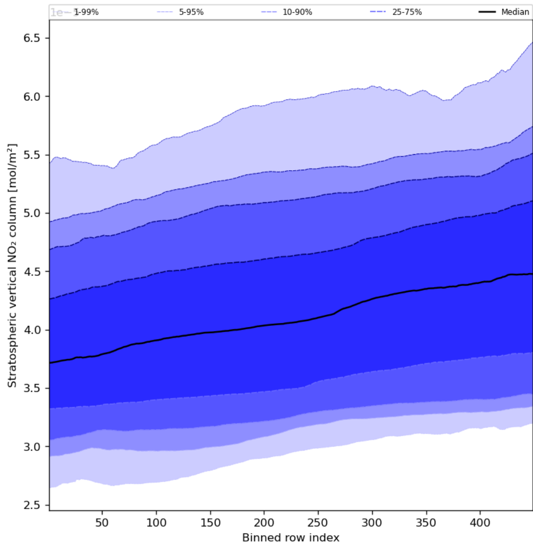
Figure 53: Along track statistics of “Stratospheric vertical NO 2 column” for 2024-03-30 to 2024-03-31
