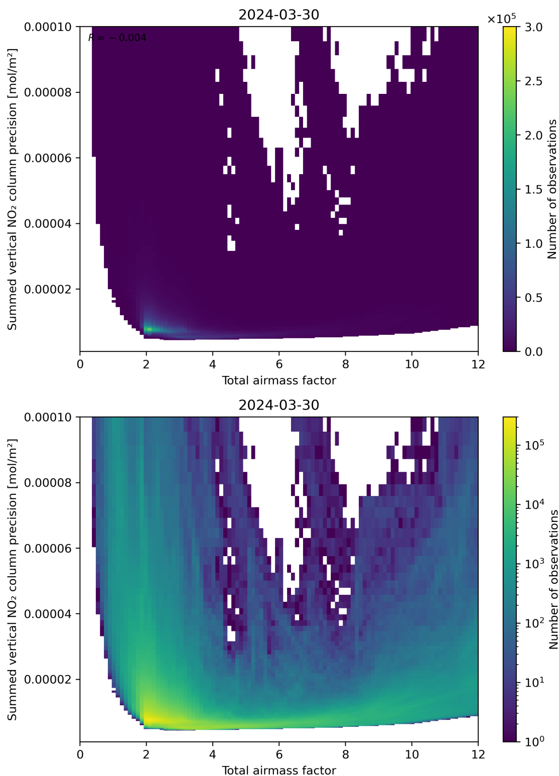
Figure 66: Scatter density plot of “Total airmass factor” against “Summed vertical NO 2 column precision” for 2024-03-30 to 2024-03-31.
