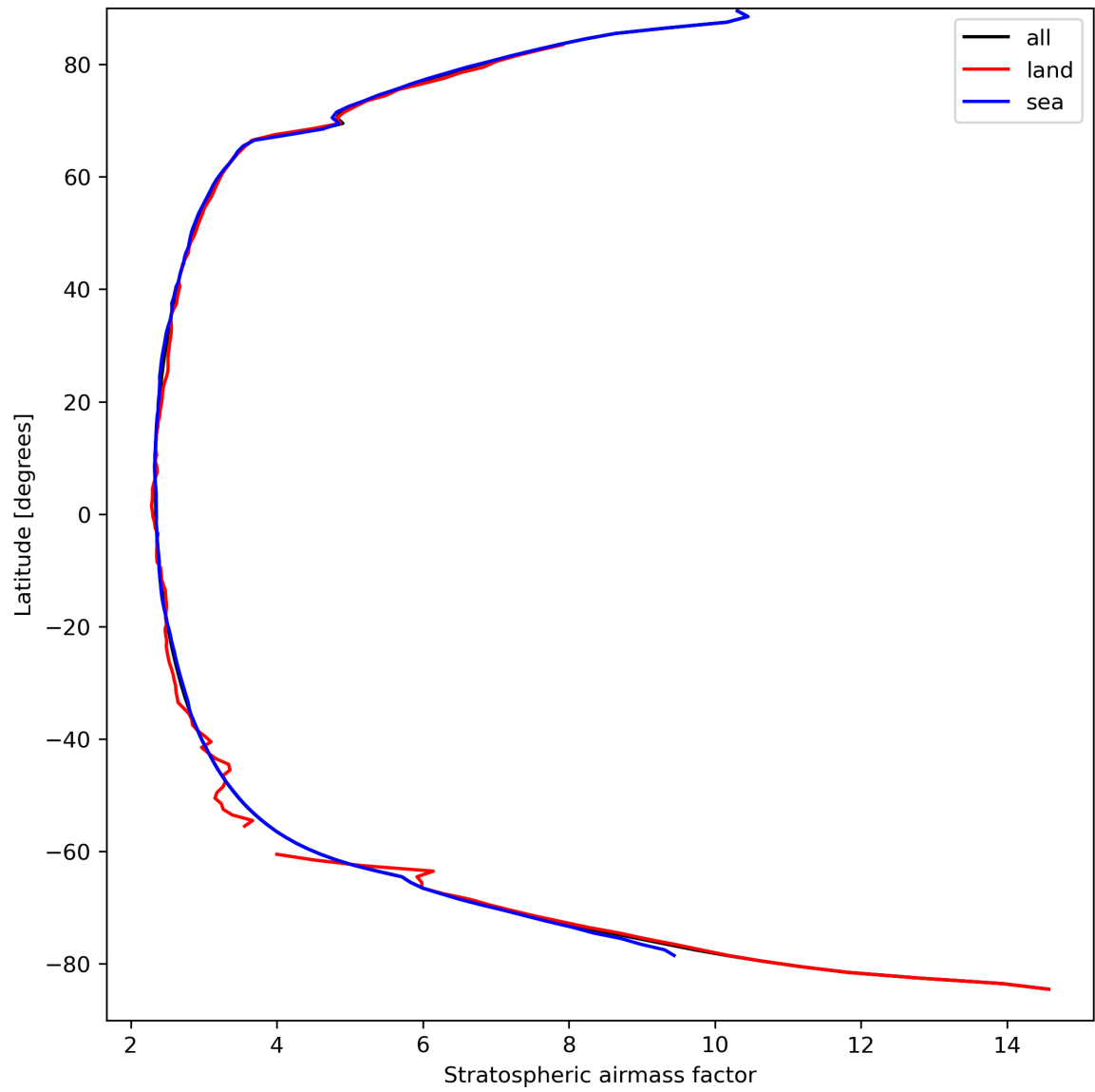
Figure 27: Zonal average of “Stratospheric airmass factor” for 2024-03-30 to 2024-03-31.
