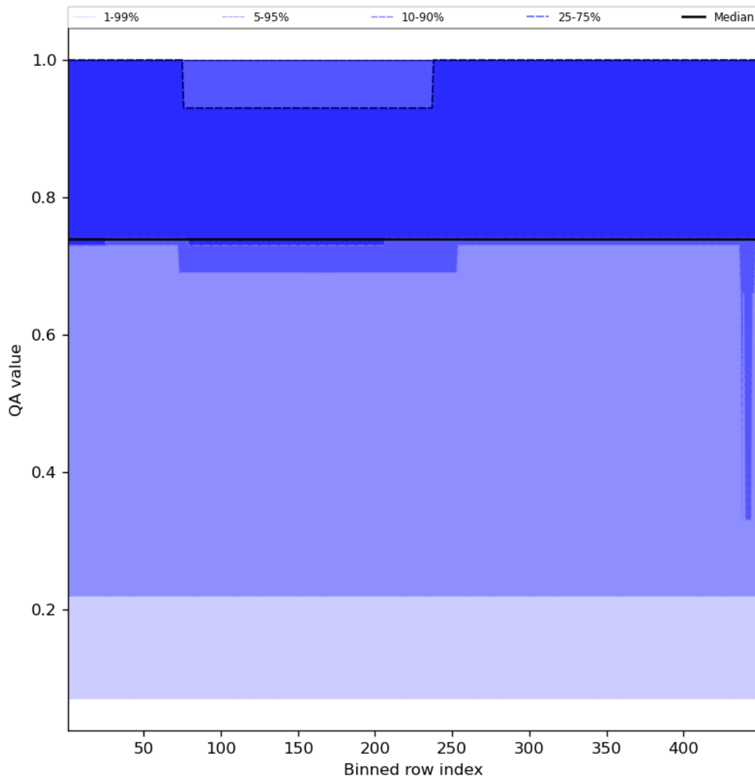
Figure 45: Along track statistics of “QA value” for 2024-03-30 to 2024-03-31
