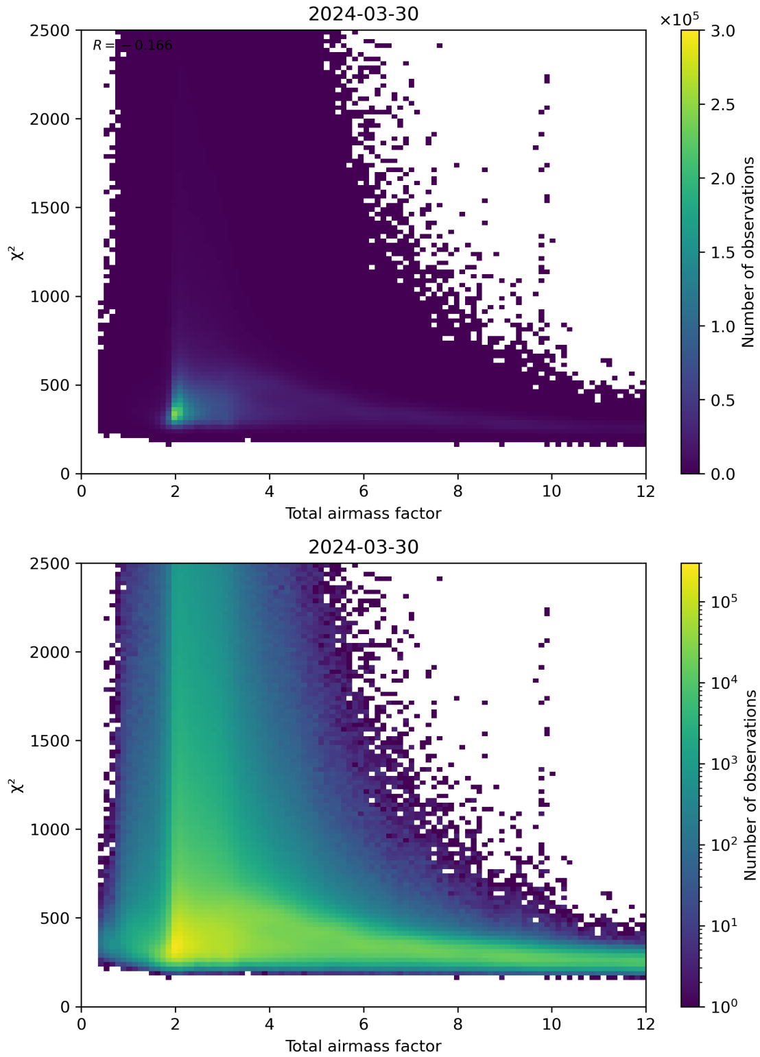
Figure 63: Scatter density plot of “Total airmass factor” against “ \chi^2 ” for 2024-03-30 to 2024-03-31.
