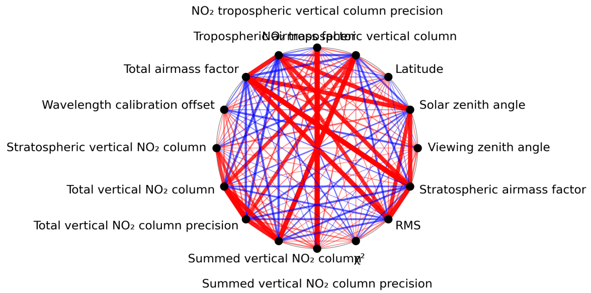
Figure 1: Map of correlation graph for 2024-03-30 to 2024-03-31.
