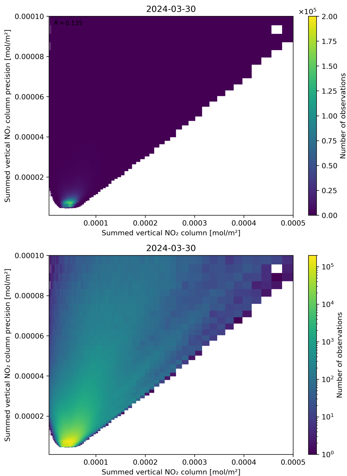
Figure 105: Scatter density plot of “Summed vertical NO 2 column” against “Summed vertical NO 2 column precision” for 2024-03-30 to 2024-03-31.
