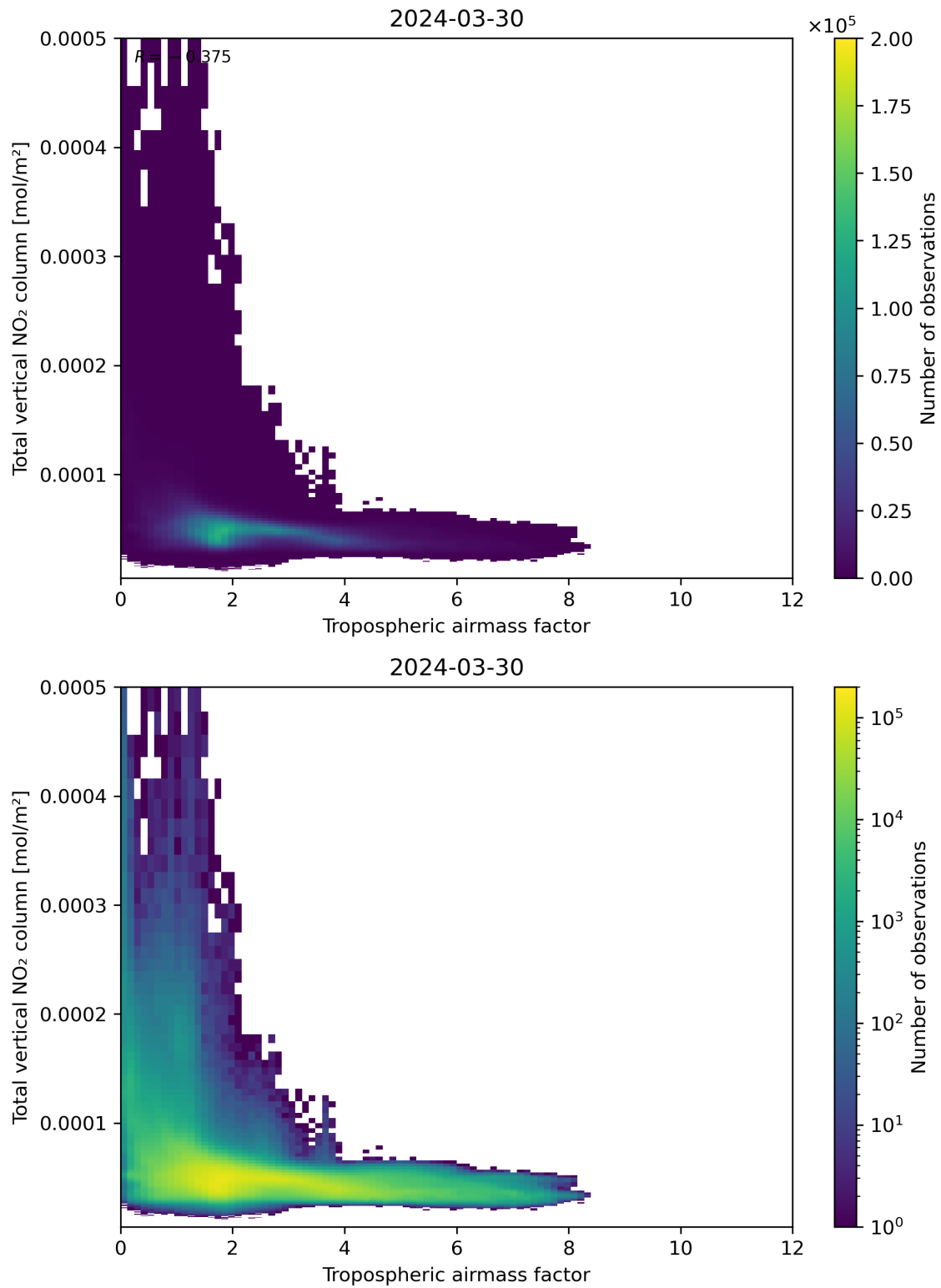
Figure 77: Scatter density plot of “Tropospheric airmass factor” against “Total vertical NO 2 column” for 2024-03-30 to 2024-03-31.
