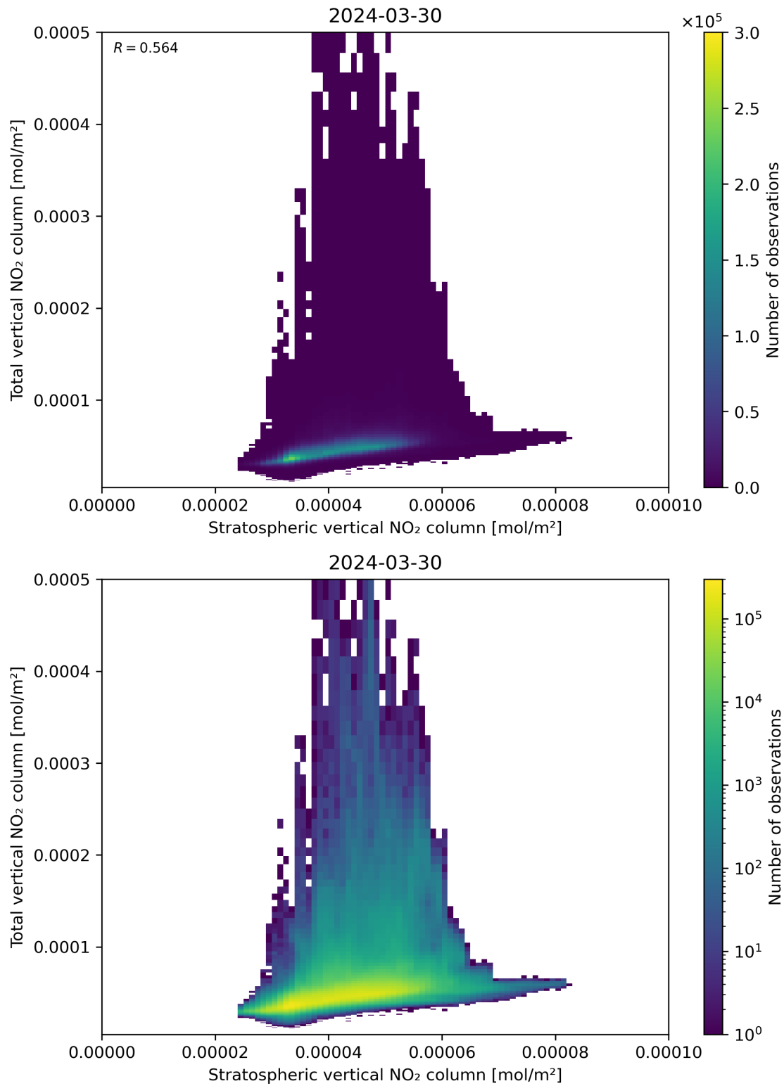
Figure 100: Scatter density plot of “Stratospheric vertical NO 2 column” against “Total vertical NO 2 column” for 2024-03-30 to 2024-03-31.
