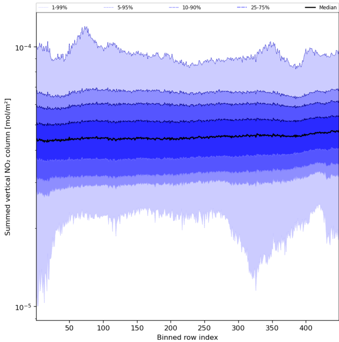
Figure 57: Along track statistics of “Summed vertical NO 2 column” for 2024-03-30 to 2024-03-31
