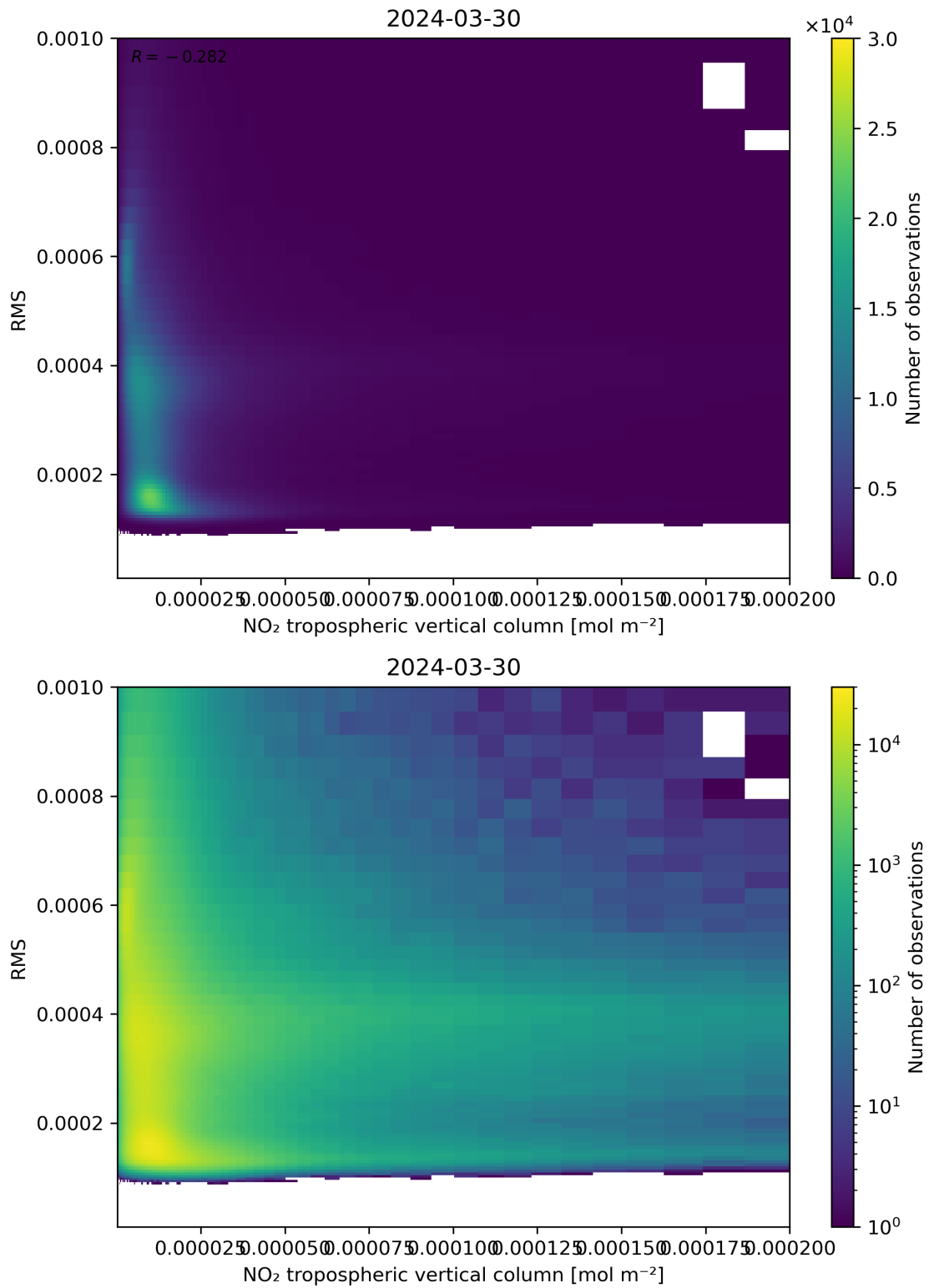
Figure 142: Scatter density plot of “NO 2 tropospheric vertical column” against “RMS” for 2024-03-30 to 2024-03-31.
