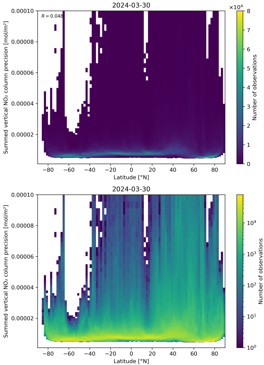
Figure 89: Scatter density plot of “Latitude” against “Summed vertical NO 2 column precision” for 2024-03-30 to 2024-03-31.
