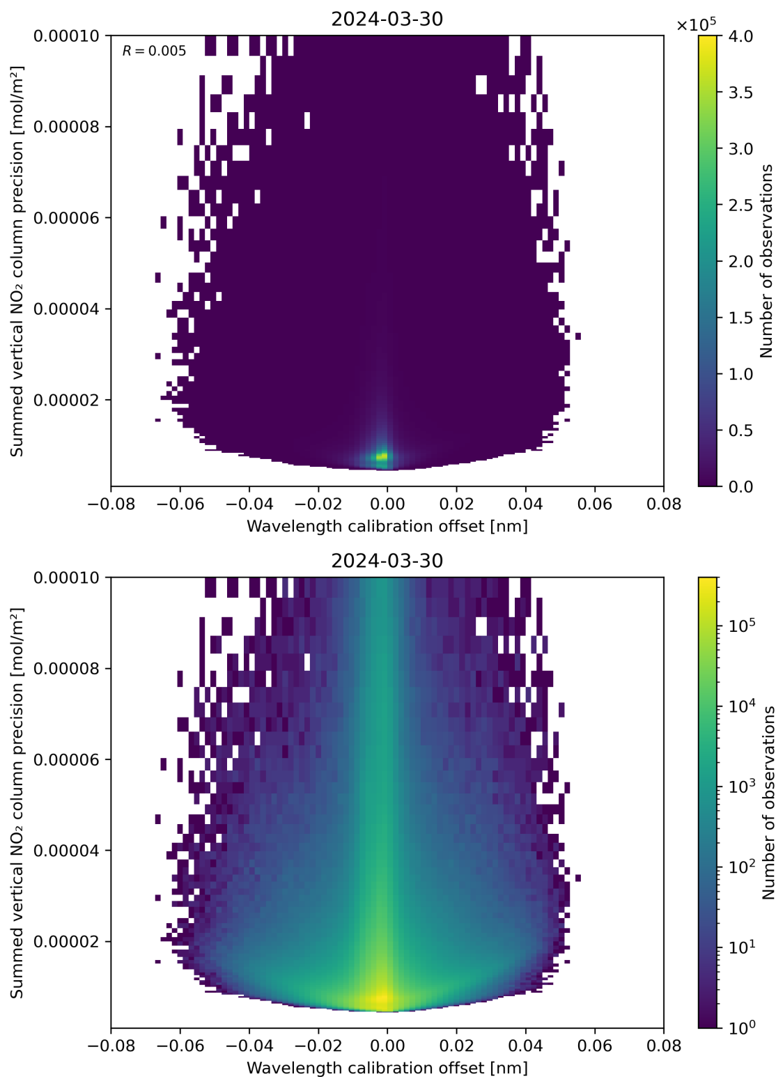
Figure 178: Scatter density plot of “Wavelength calibration offset” against “Summed vertical NO 2 column precision” for 2024-03-30 to 2024-03-31.
