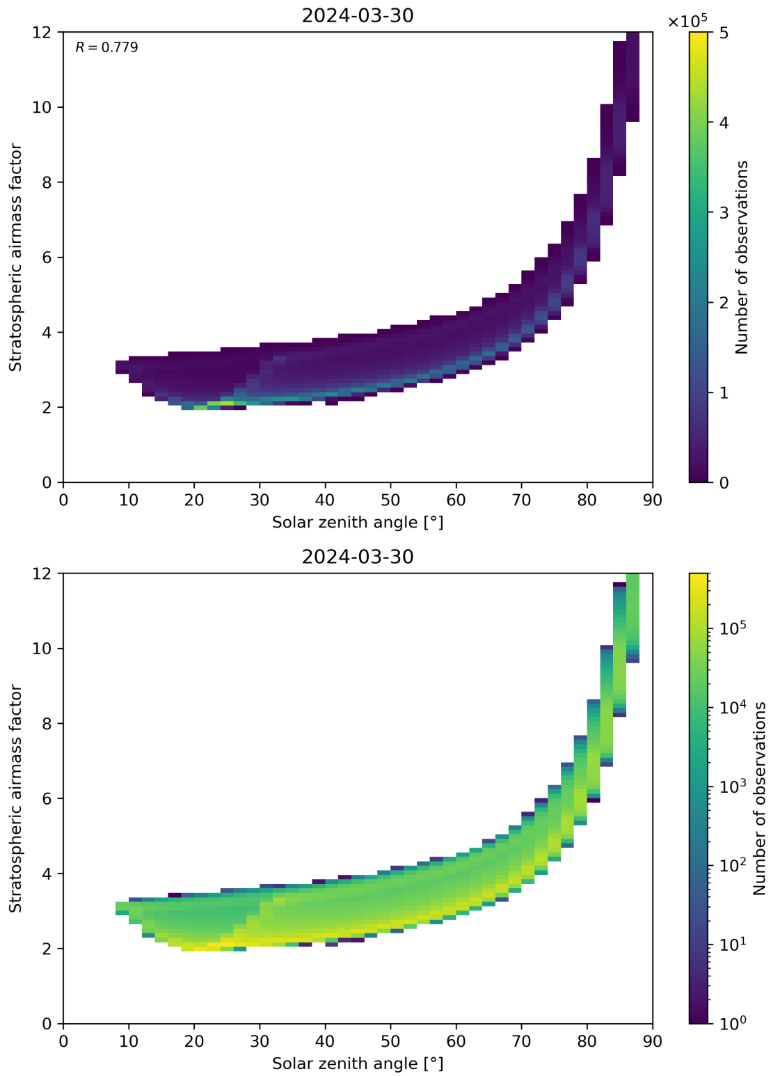
Figure 145: Scatter density plot of “Solar zenith angle” against “Stratospheric airmass factor” for 2024-03-30 to 2024-03-31.
