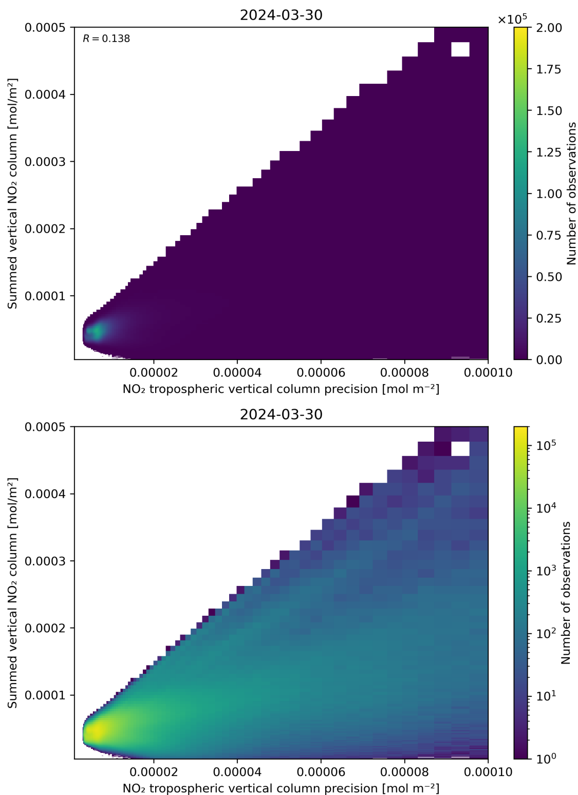
Figure 136: Scatter density plot of “NO 2 tropospheric vertical column precision” against “Summed vertical NO 2 column” for 2024-03-30 to 2024-03-31.
