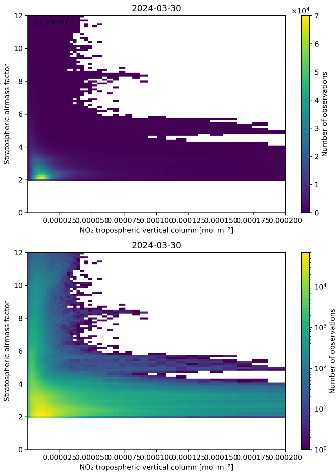
Figure 121: Scatter density plot of “NO 2 tropospheric vertical column” against “Stratospheric air mass factor” for 2024-03-30 to 2024-03-31.
