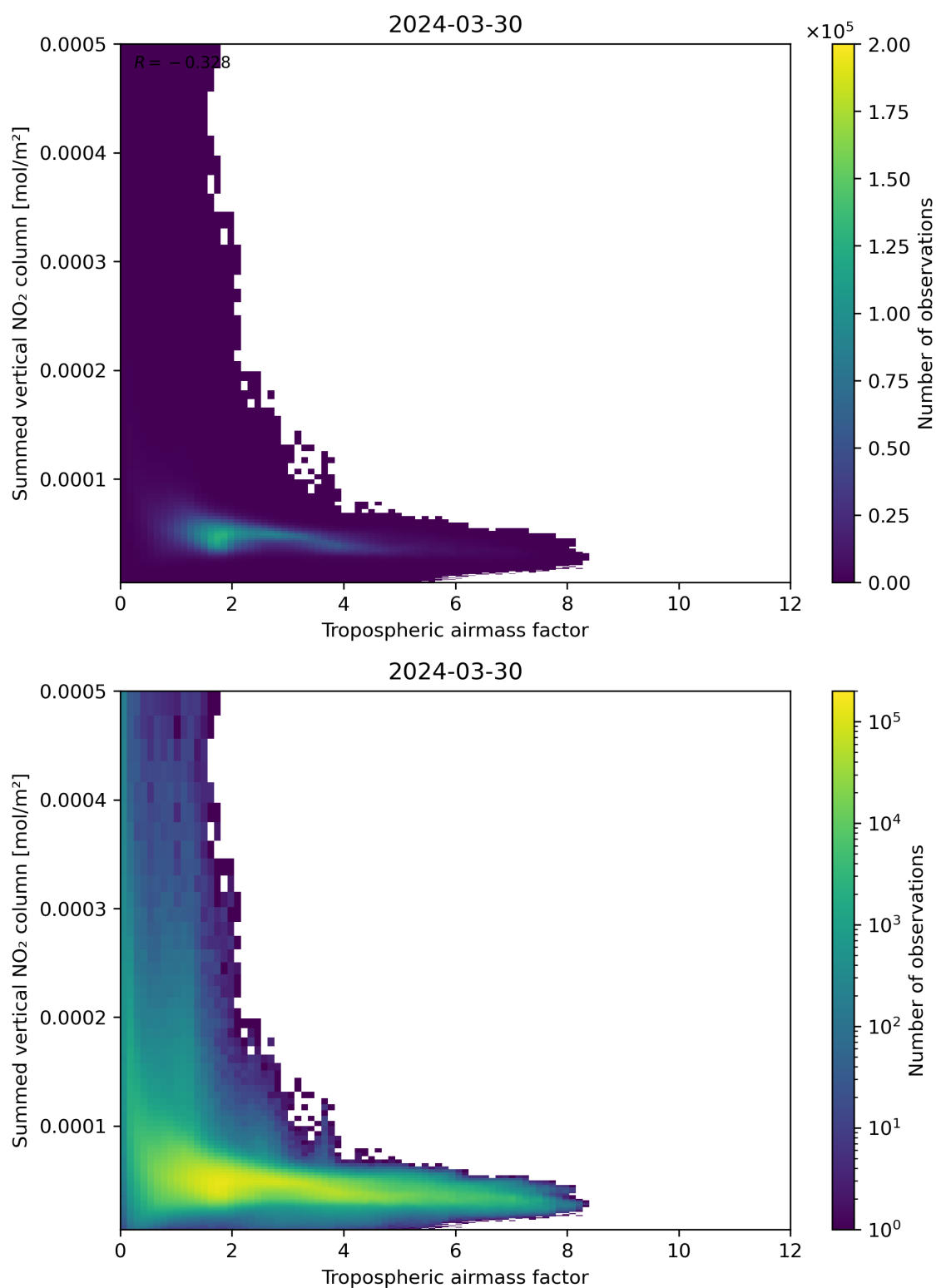
Figure 75: Scatter density plot of “Tropospheric air mass factor” against “Summed vertical NO 2 column” for 2024-03-30 to 2024-03-31.
