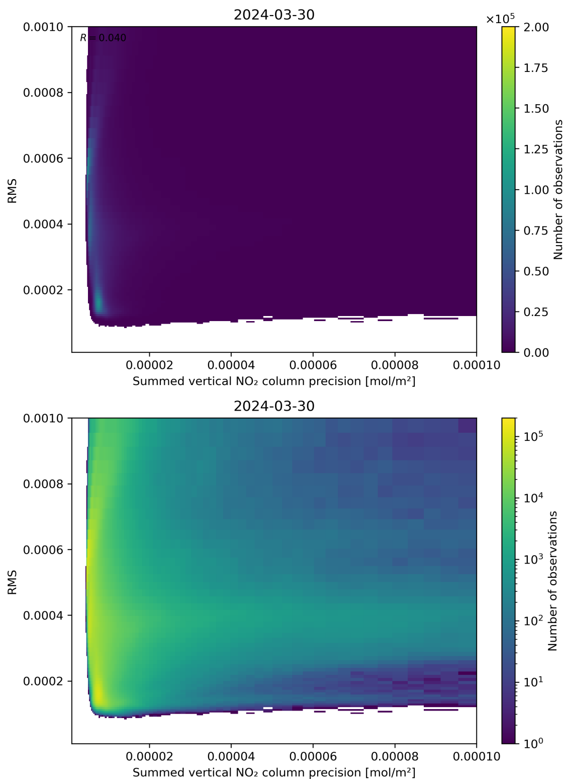
Figure 108: Scatter density plot of “Summed vertical NO 2 column precision” against “RMS” for 2024-03-30 to 2024-03-31.
