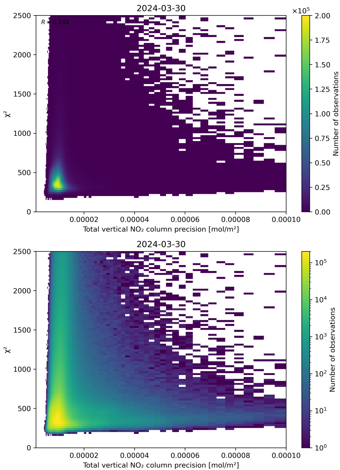
Figure 116: Scatter density plot of “Total vertical NO 2 column precision” against “ \chi^2 ” for 2024-03-30 to 2024-03-31.
