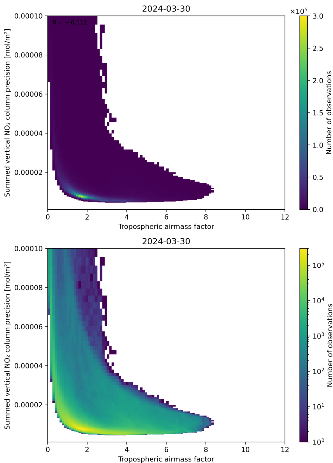
Figure 76: Scatter density plot of “Tropospheric air mass factor” against “Summed vertical NO 2 column precision” for 2024-03-30 to 2024-03-31.
