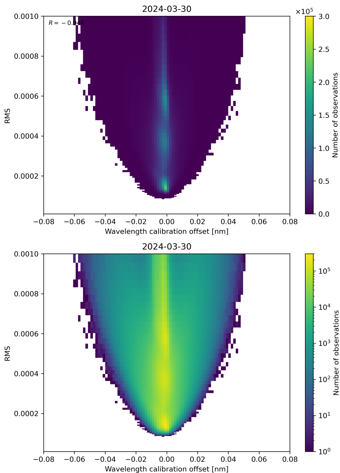
Figure 181: Scatter density plot of “Wavelength calibration offset” against “RMS” for 2024-03-30 to 2024-03-31.
