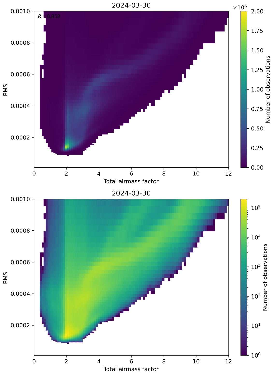
Figure 69: Scatter density plot of “Total airmass factor” against “RMS” for 2024-03-30 to 2024-03-31.
