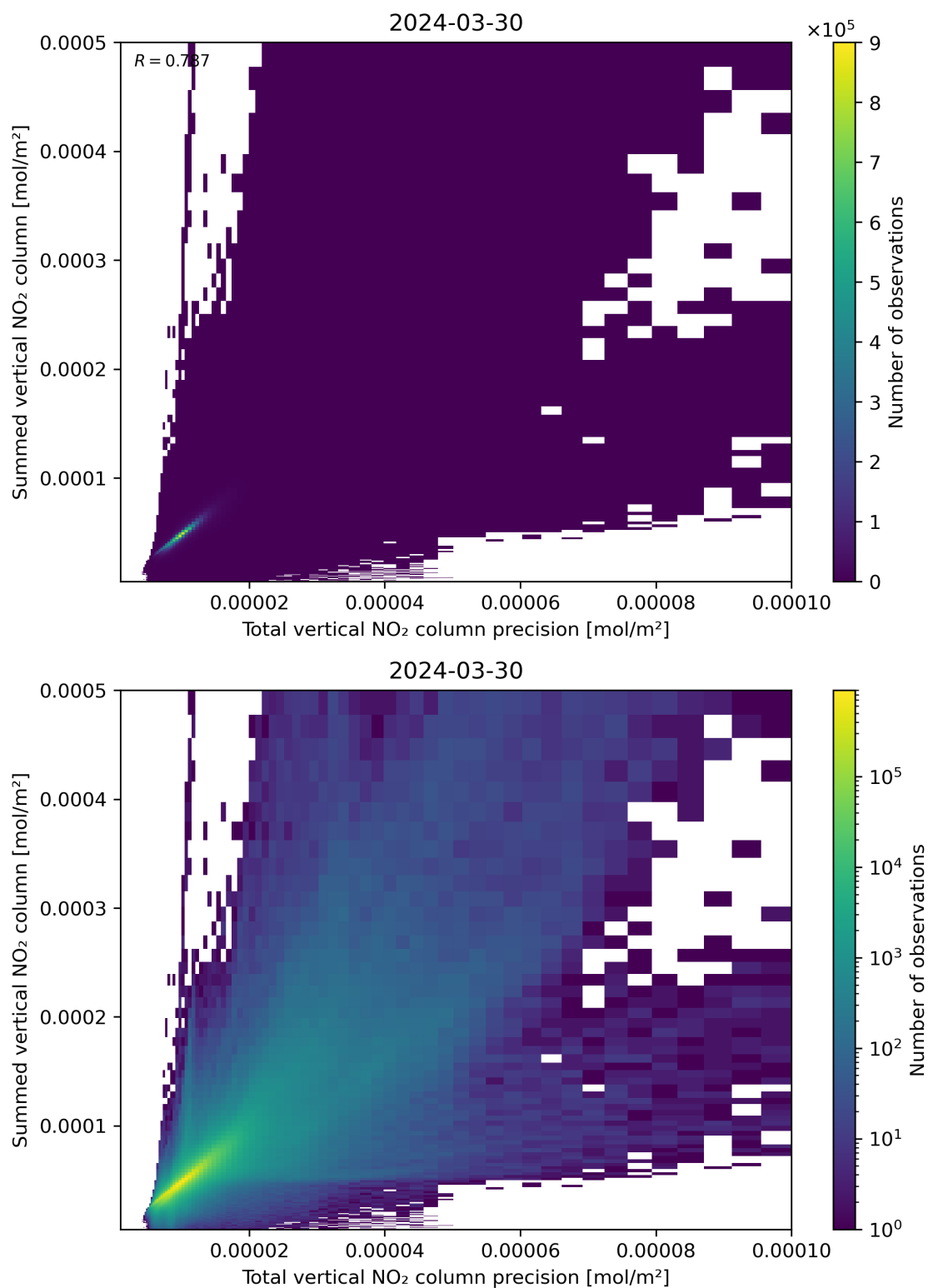
Figure 117: Scatter density plot of “Total vertical NO 2 column precision” against “Summed vertical NO 2 column” for 2024-03-30 to 2024-03-31.
