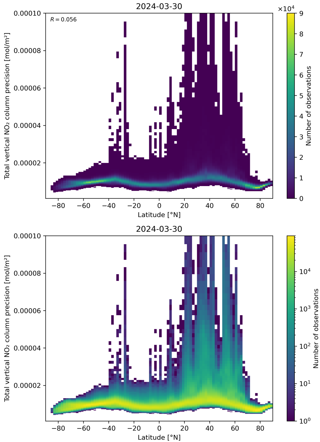
Figure 91: Scatter density plot of “Latitude” against “Total vertical NO 2 column precision” for 2024-03-30 to 2024-03-31.
