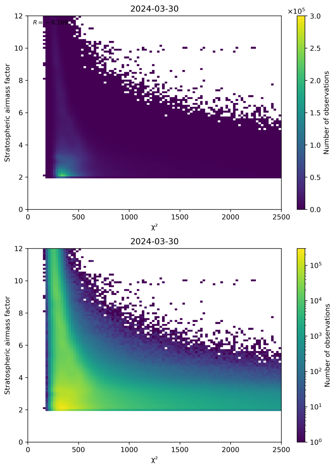
Figure 81: Scatter density plot of “ \chi^2 ” against “Stratospheric airmass factor” for 2024-03-30 to 2024-03-31.
