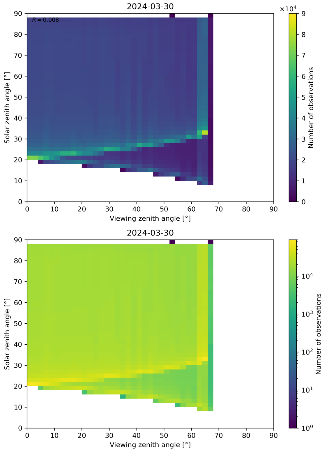
Figure 172: Scatter density plot of “Viewing zenith angle” against “Solar zenith angle” for 2024-03-30 to 2024-03-31.
