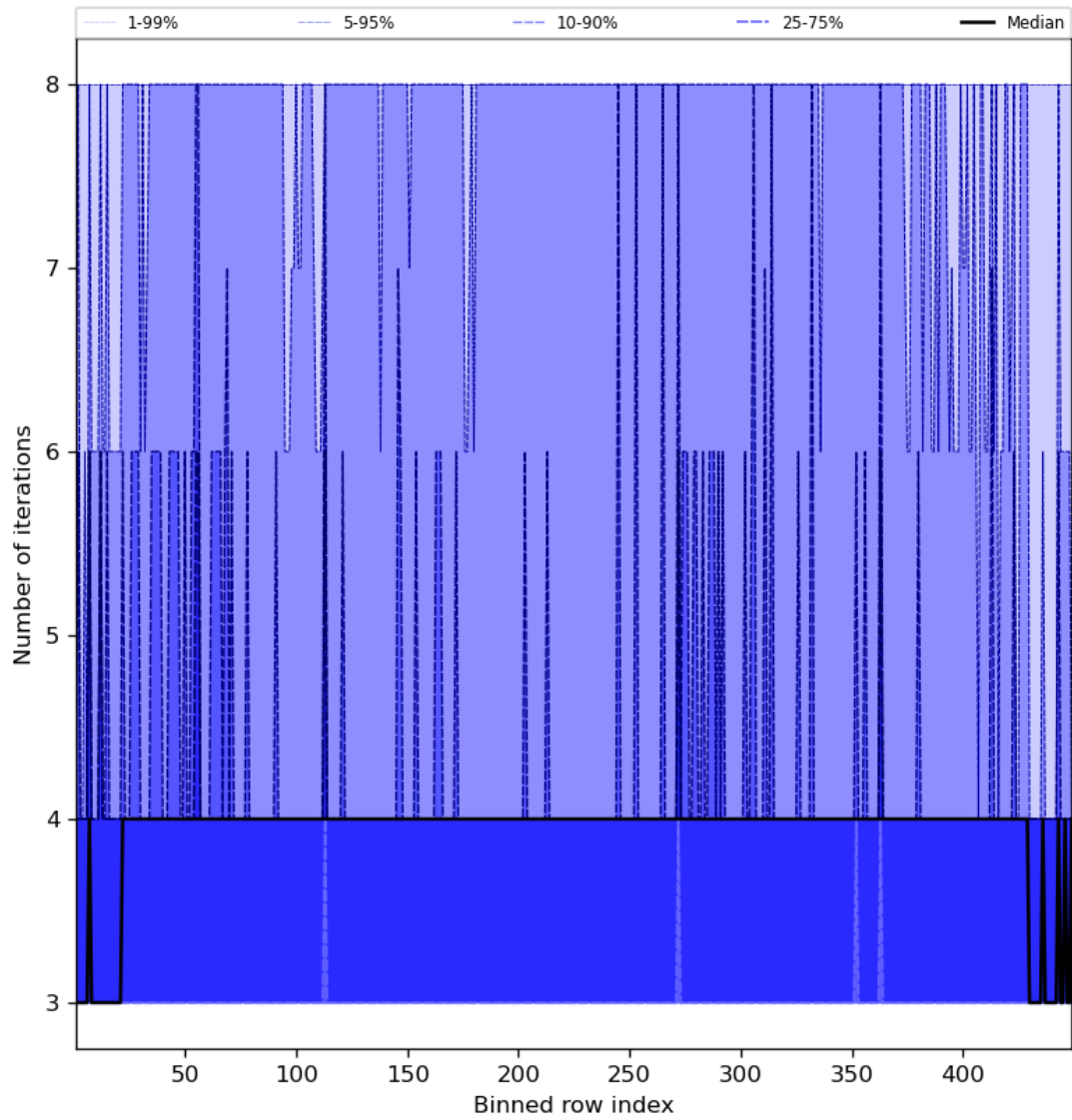
Figure 51: Along track statistics of “Number of iterations” for 2024-03-30 to 2024-03-31
