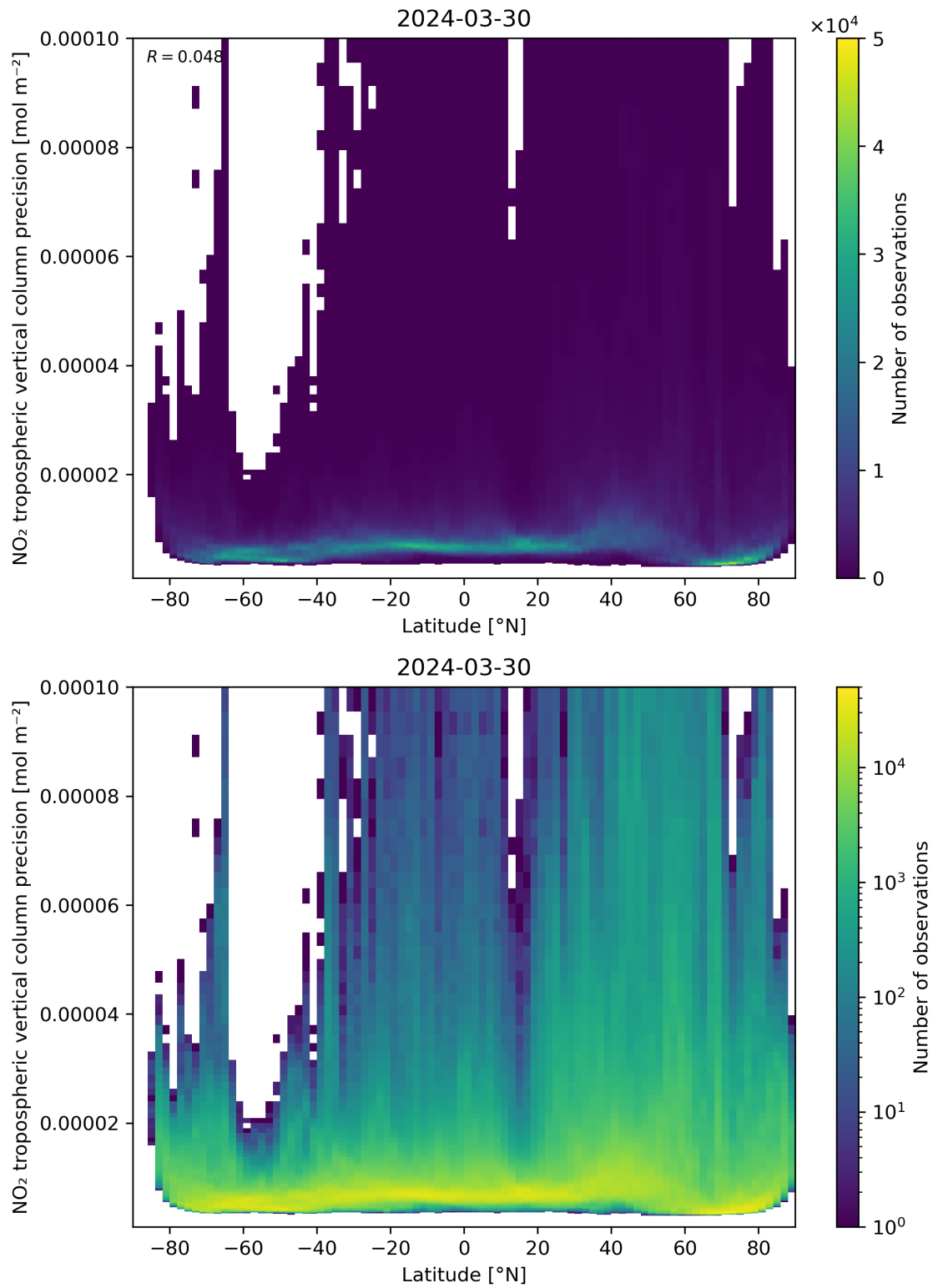
Figure 93: Scatter density plot of “Latitude” against “NO 2 tropospheric vertical column precision” for 2024-03-30 to 2024-03-31.
