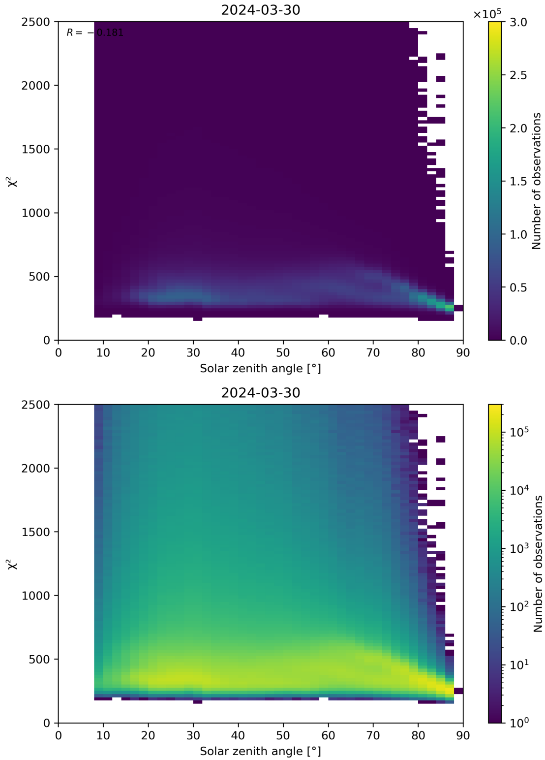
Figure 148: Scatter density plot of “Solar zenith angle” against “ \chi^2 ” for 2024-03-30 to 2024-03-31.
