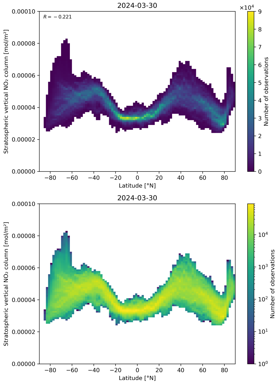
Figure 87: Scatter density plot of “Latitude” against “Stratospheric vertical NO 2 column” for 2024-03-30 to 2024-03-31.
