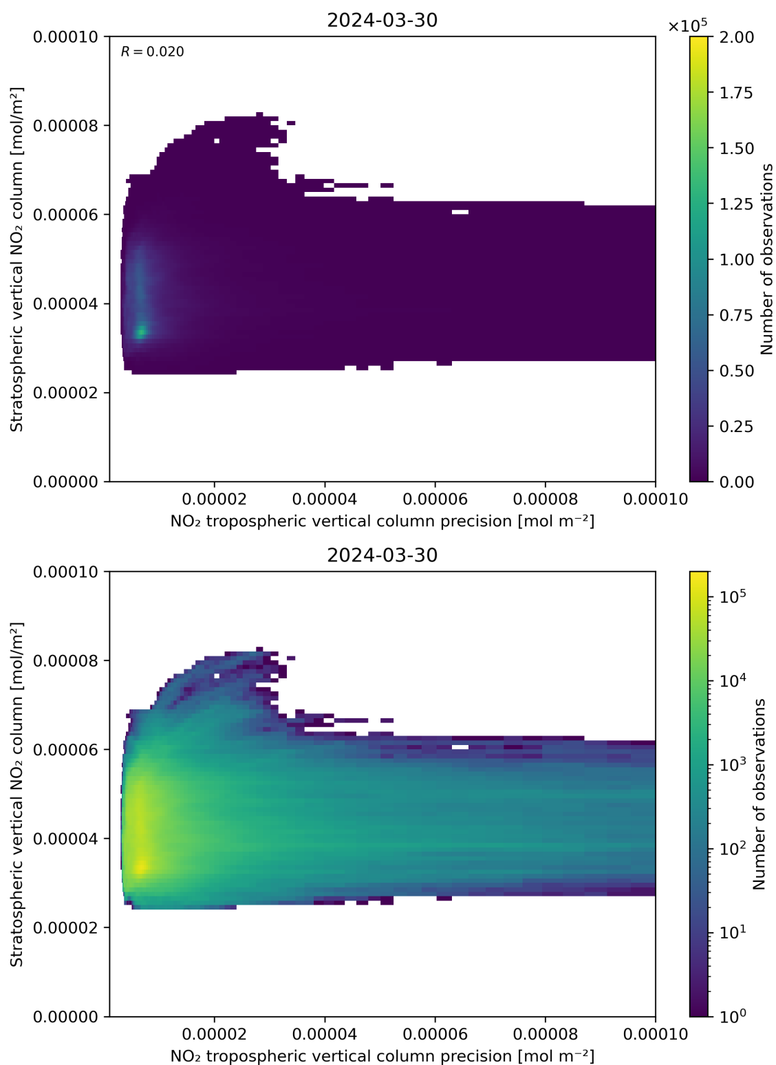
Figure 135: Scatter density plot of “NO 2 tropospheric vertical column precision” against “Stratospheric vertical NO 2 column” for 2024-03-30 to 2024-03-31.
