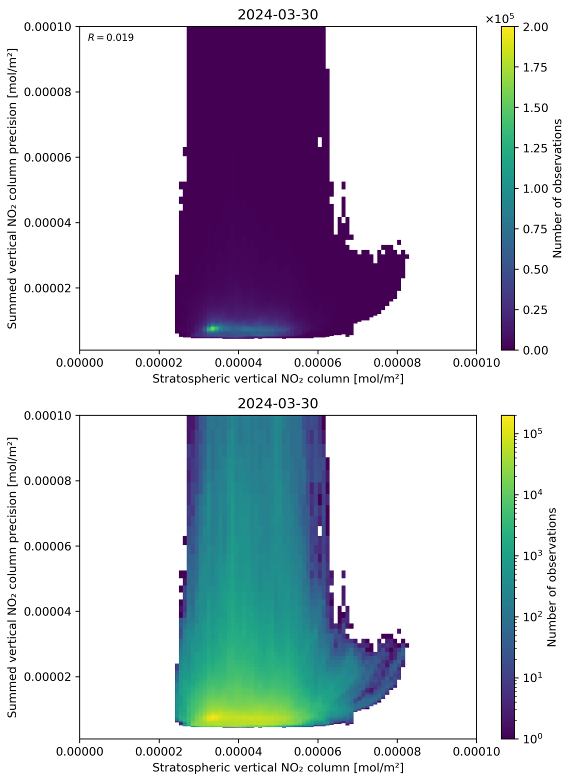
Figure 99: Scatter density plot of “Stratospheric vertical NO 2 column” against “Summed vertical NO 2 column precision” for 2024-03-30 to 2024-03-31.
