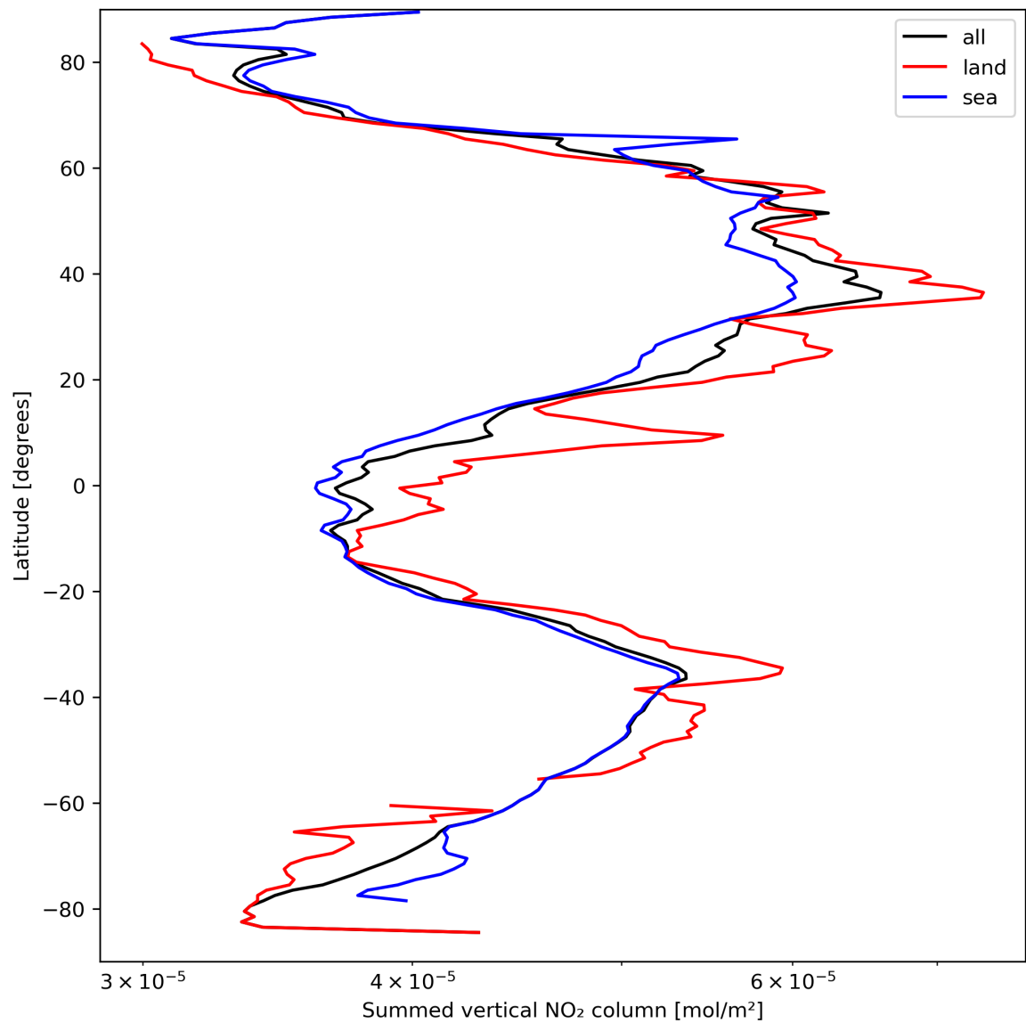
Figure 23: Zonal average of “Summed vertical NO 2 column” for 2024-03-30 to 2024-03-31.
