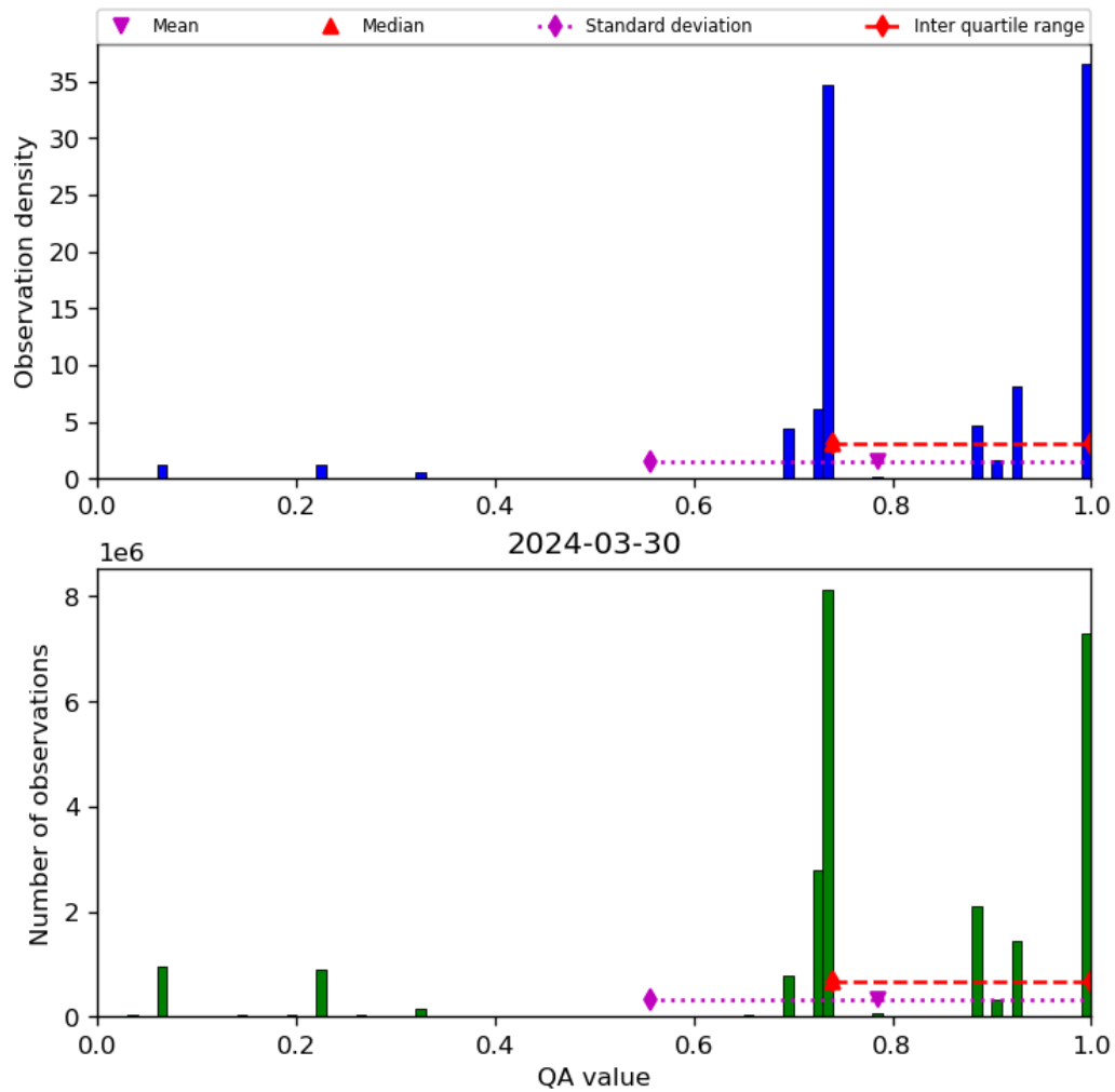
Figure 28: Histogram of “QA value” for 2024-03-30 to 2024-03-31
