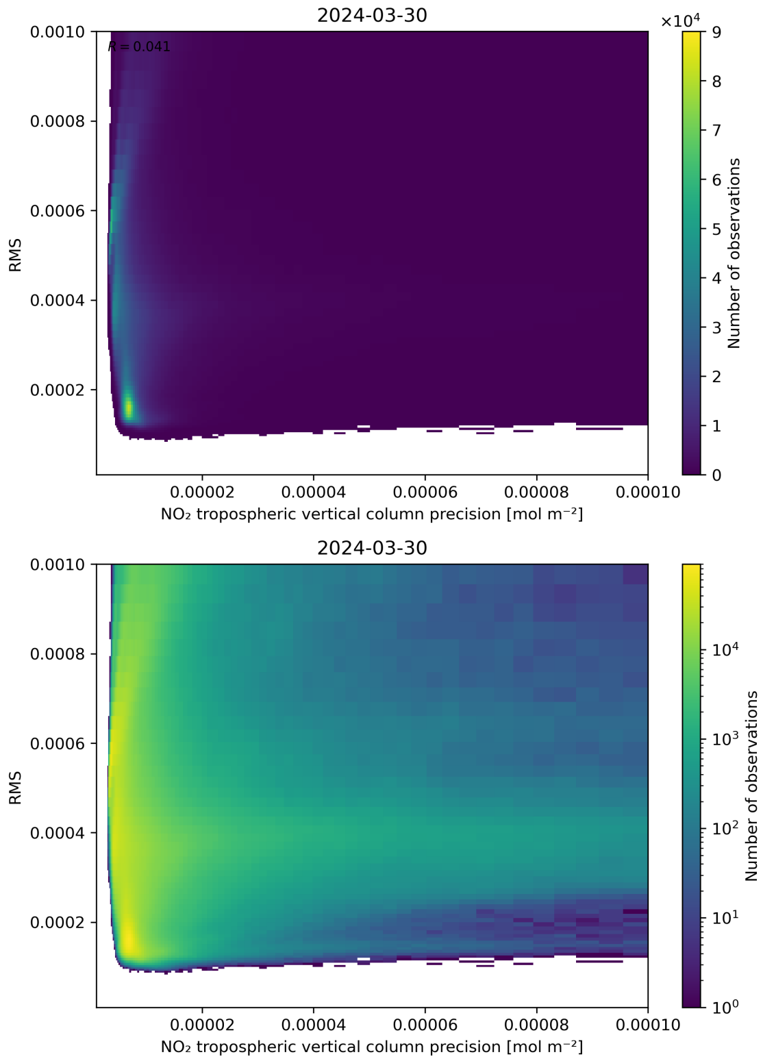
Figure 140: Scatter density plot of “NO 2 tropospheric vertical column precision” against “RMS” for 2024-03-30 to 2024-03-31.
