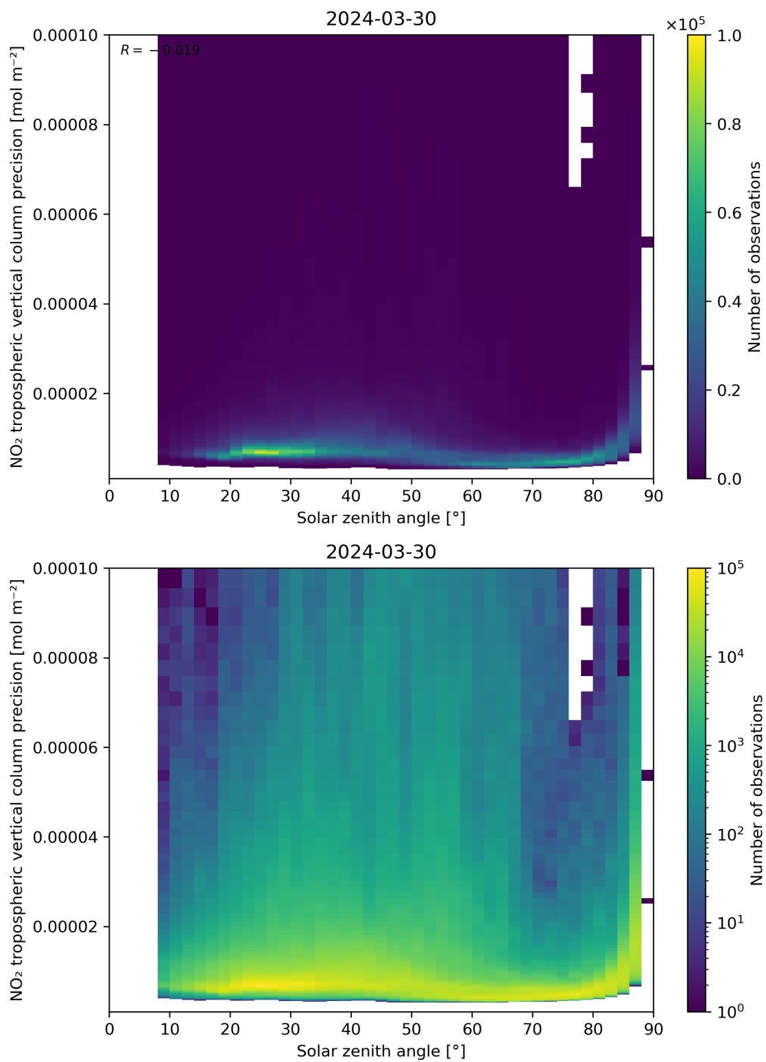
Figure 156: Scatter density plot of “Solar zenith angle” against “NO 2 tropospheric vertical column precision” for 2024-03-30 to 2024-03-31.
