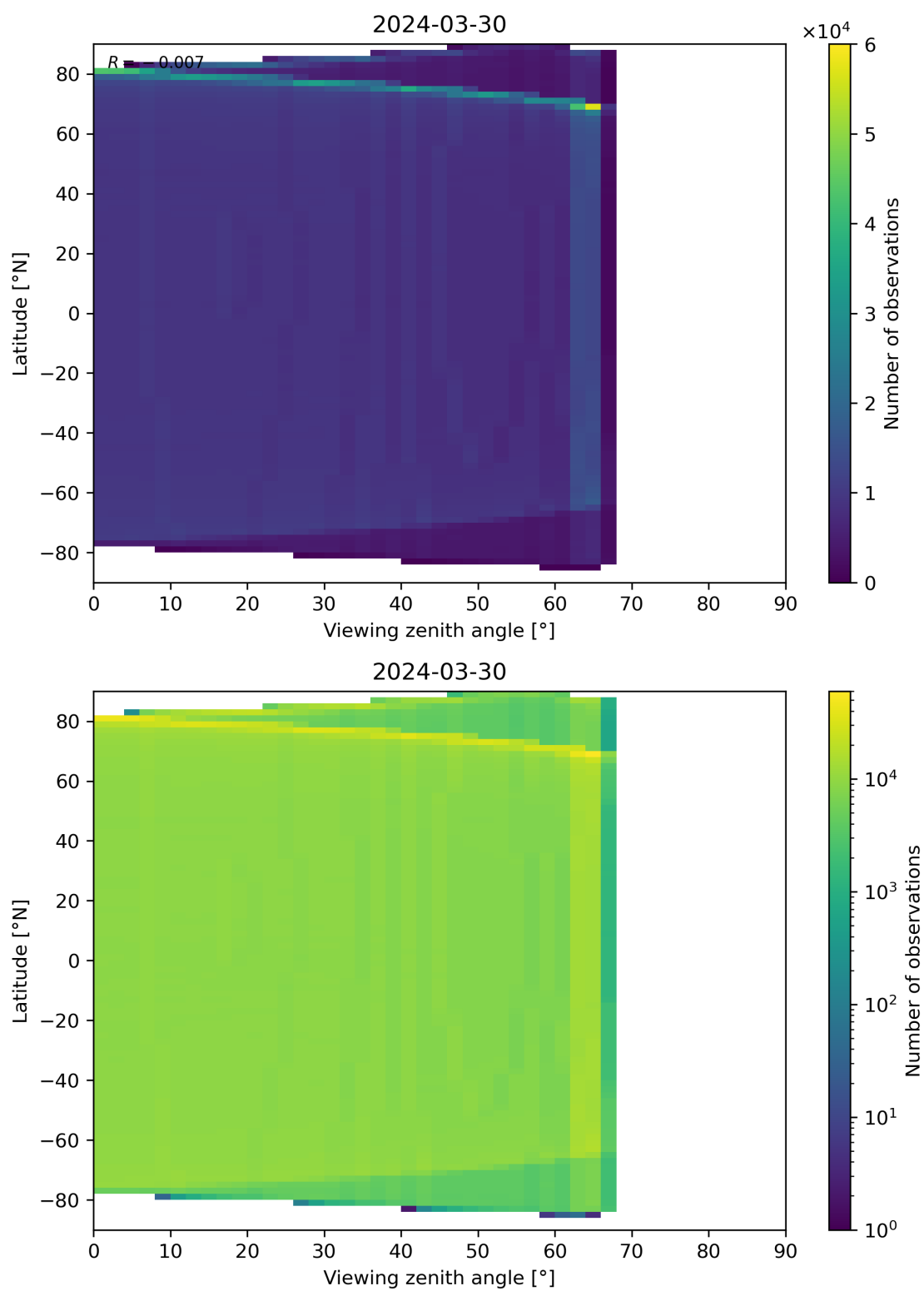
Figure 163: Scatter density plot of “Viewing zenith angle” against “Latitude” for 2024-03-30 to 2024-03-31.
