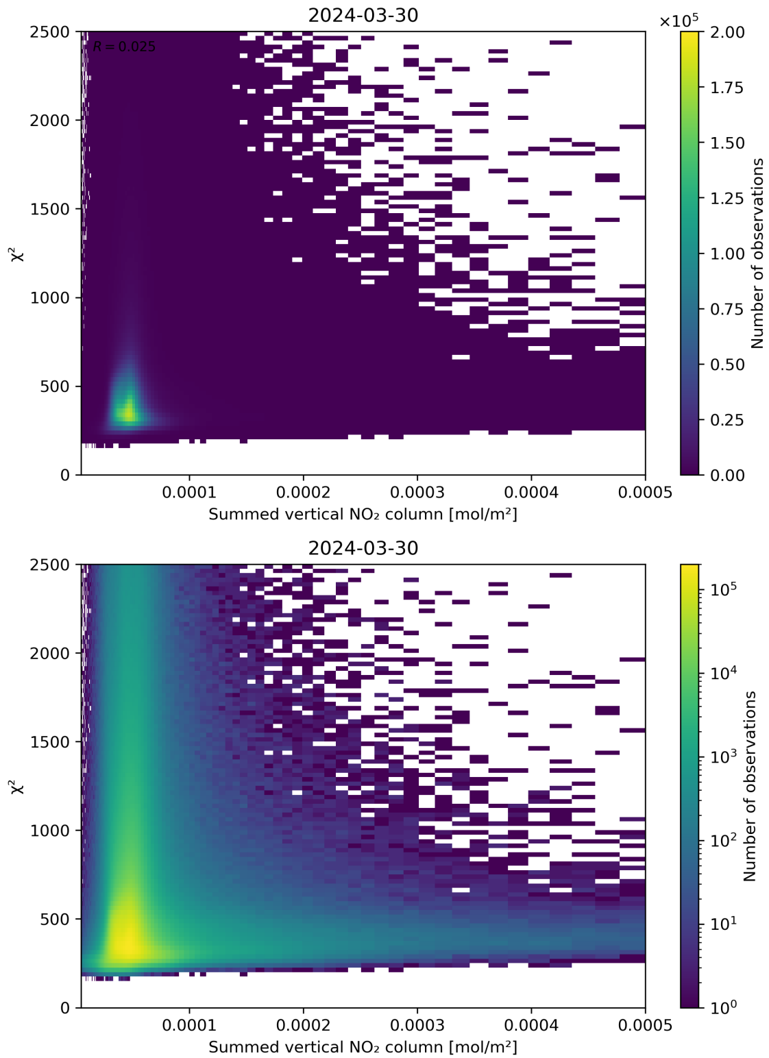
Figure 104: Scatter density plot of “Summed vertical NO 2 column” against “ \chi^2 ” for 2024-03-30 to 2024-03-31.
