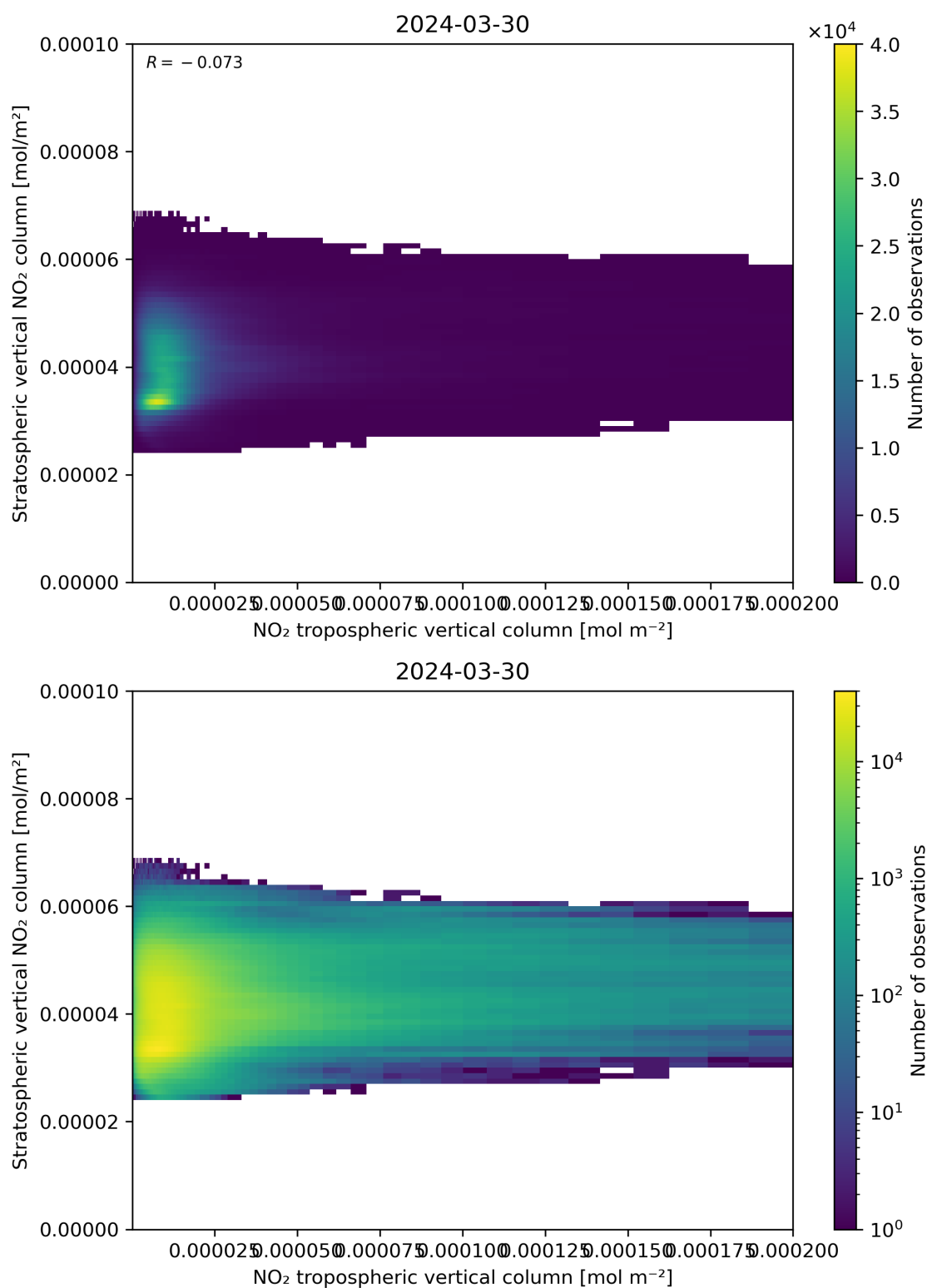
Figure 125: Scatter density plot of “NO 2 tropospheric vertical column” against “Stratospheric vertical NO 2 column” for 2024-03-30 to 2024-03-31.
