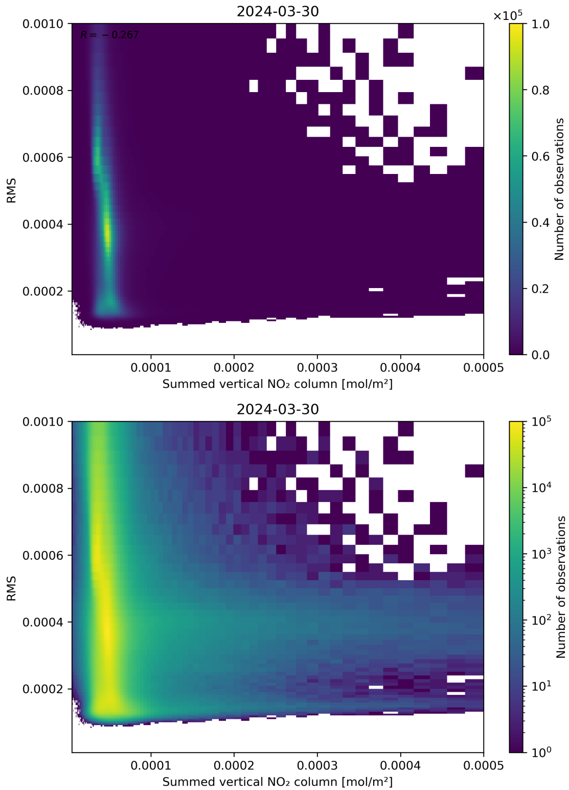
Figure 109: Scatter density plot of “Summed vertical NO 2 column” against “RMS” for 2024-03-30 to 2024-03-31.
