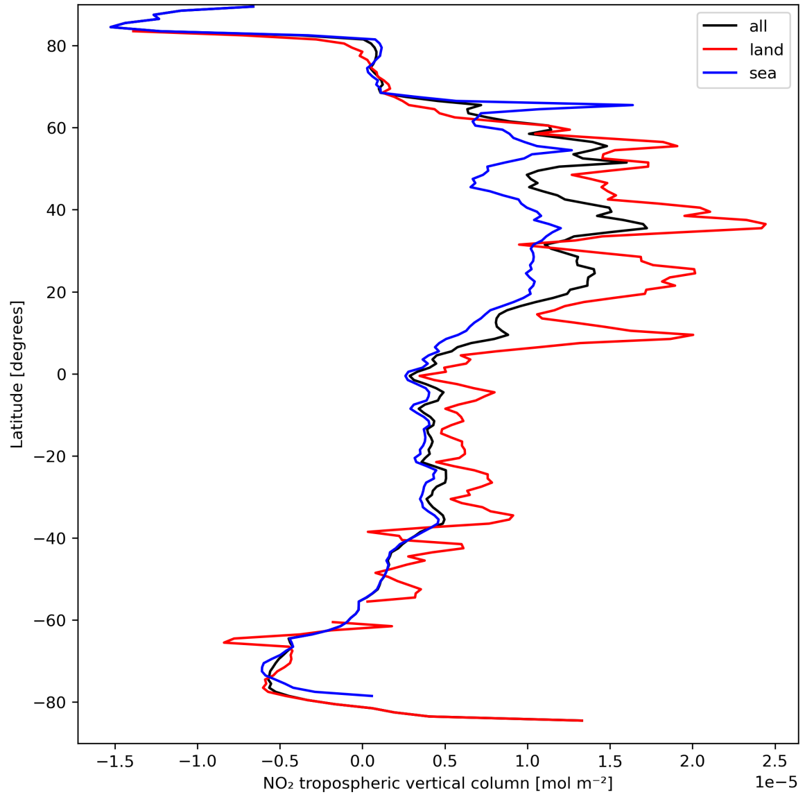
Figure 12: Zonal average of “NO 2 tropospheric vertical column” for 2024-03-30 to 2024-03-31.
