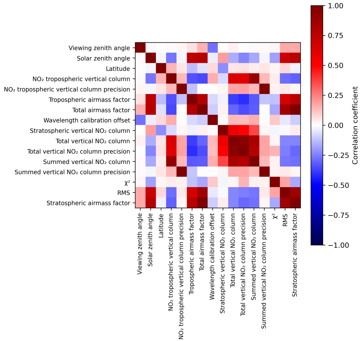
Figure 2: Map of correlation matrix for 2024-03-30 to 2024-03-31.
