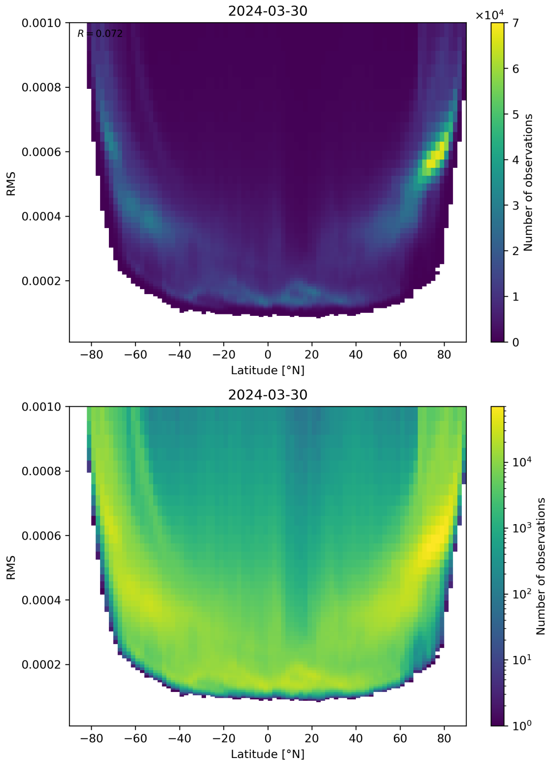
Figure 94: Scatter density plot of “Latitude” against “RMS” for 2024-03-30 to 2024-03-31.
