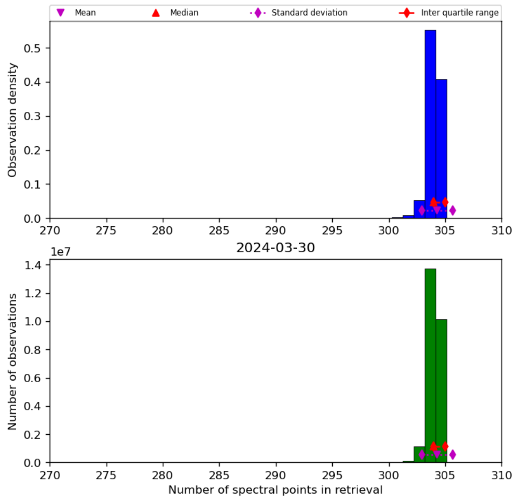
Figure 33: Histogram of “Number of spectral points in retrieval” for 2024-03-30 to 2024-03-31
