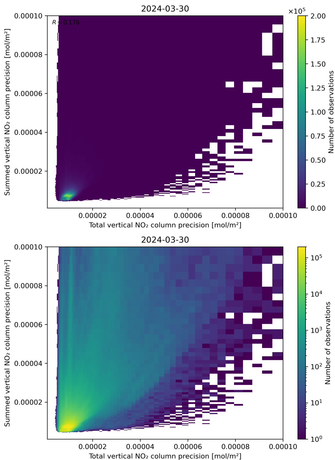
Figure 118: Scatter density plot of “Total vertical NO 2 column precision” against “Summed vertical NO 2 column precision” for 2024-03-30 to 2024-03-31.
