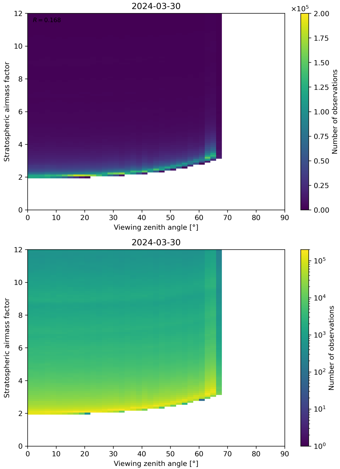
Figure 159: Scatter density plot of “Viewing zenith angle” against “Stratospheric airmass factor” for 2024-03-30 to 2024-03-31.
