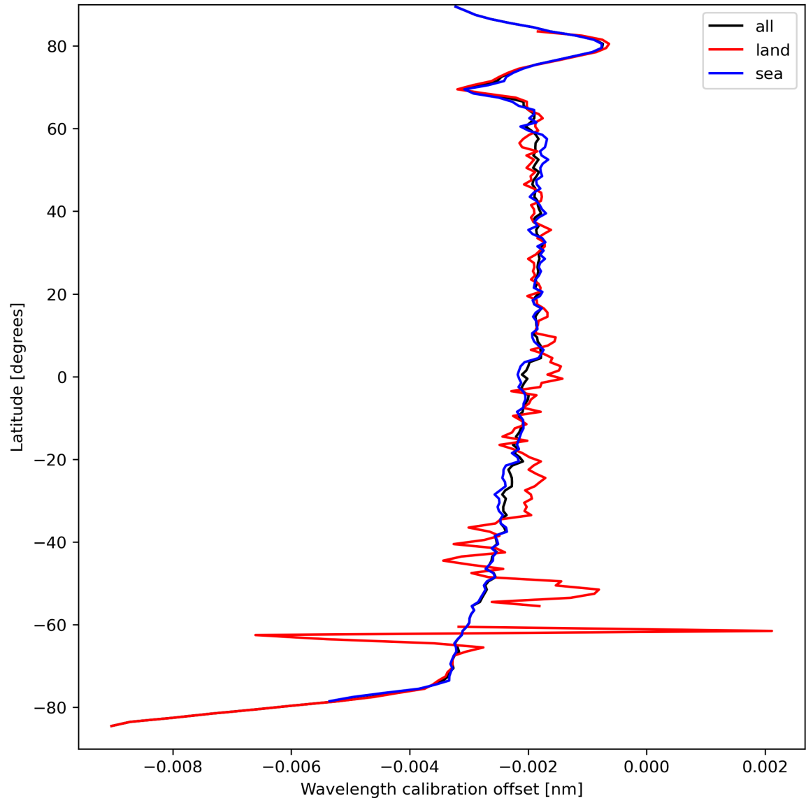
Figure 18: Zonal average of “Wavelength calibration offset” for 2024-03-30 to 2024-03-31.
