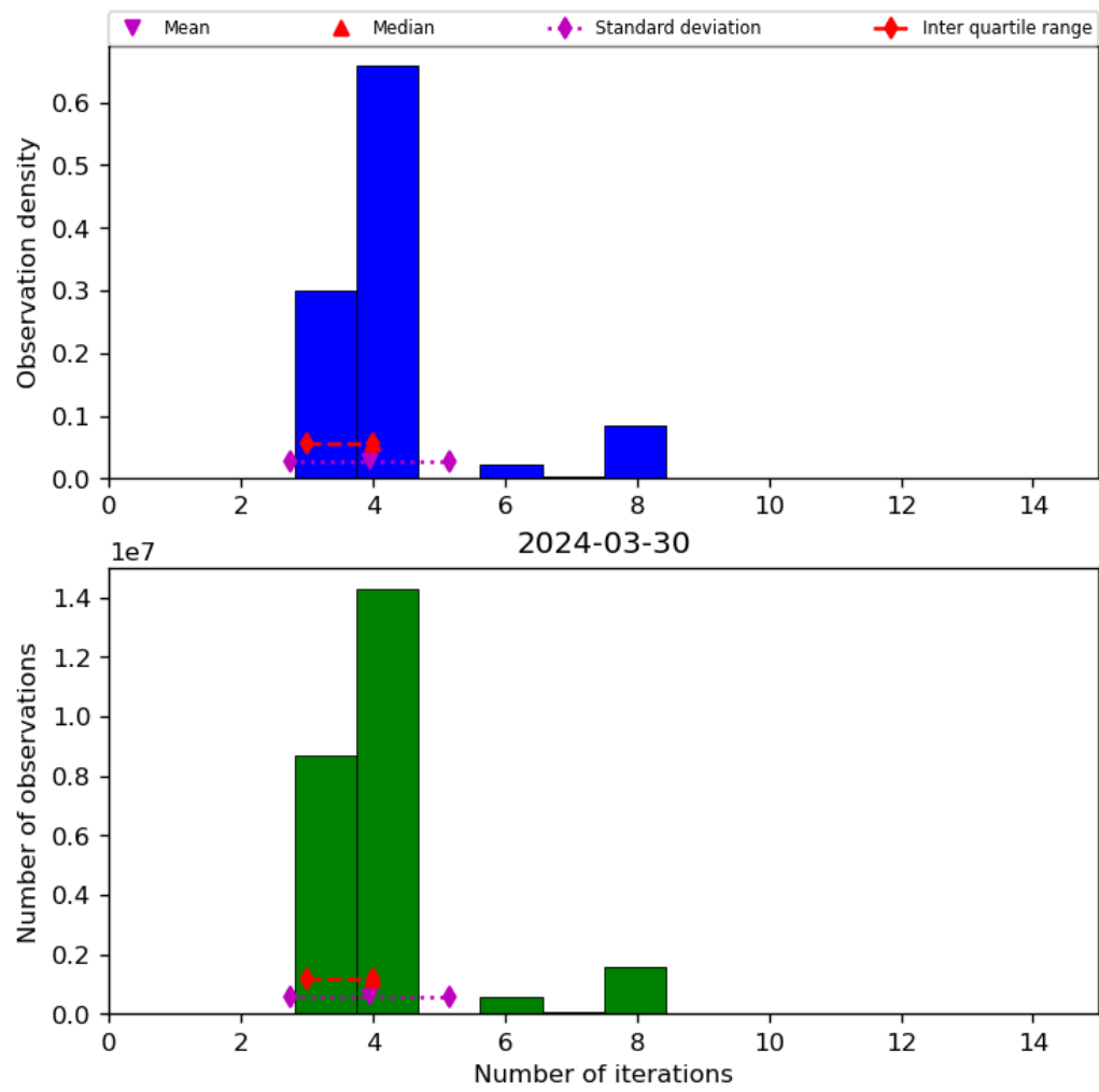
Figure 34: Histogram of “Number of iterations” for 2024-03-30 to 2024-03-31
