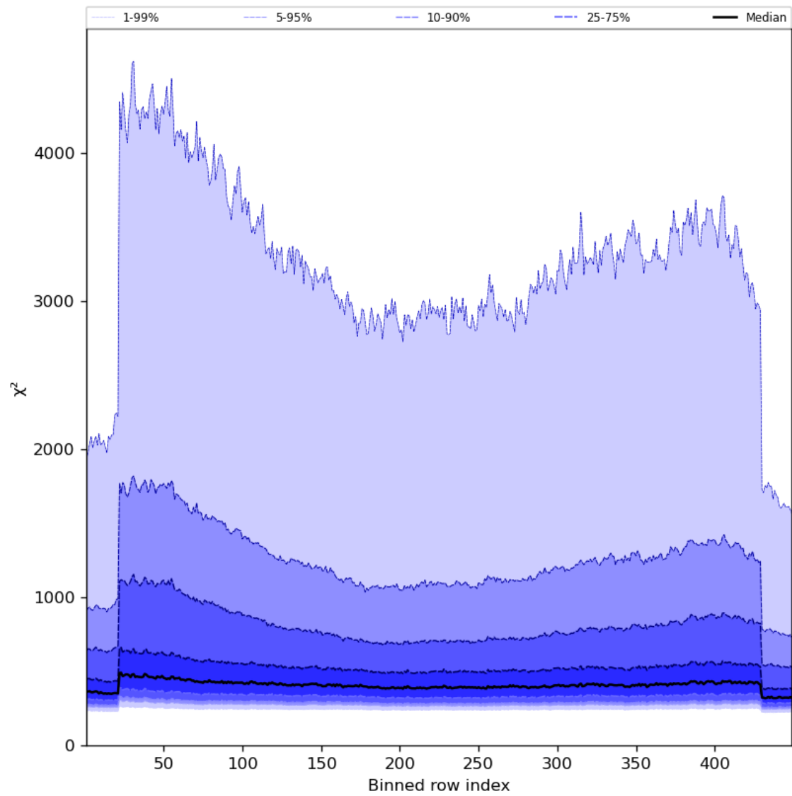
Figure 59: Along track statistics of “ \chi^2 ” for 2024-03-30 to 2024-03-31
