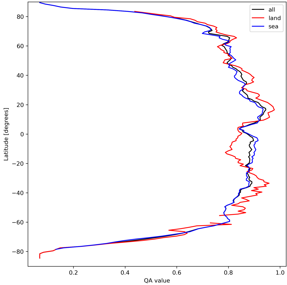
Figure 11: Zonal average of “QA value” for 2024-03-30 to 2024-03-31.
