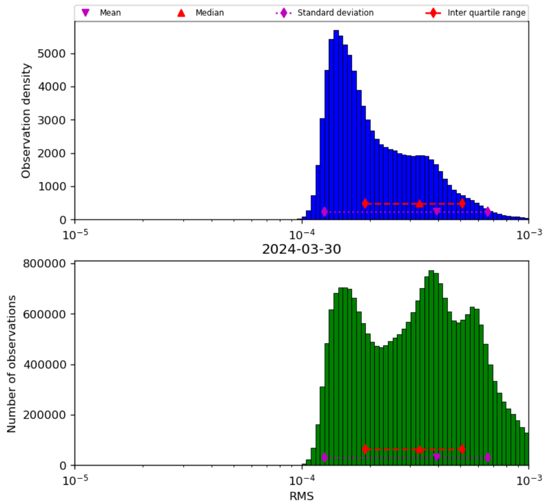
Figure 43: Histogram of “RMS” for 2024-03-30 to 2024-03-31
