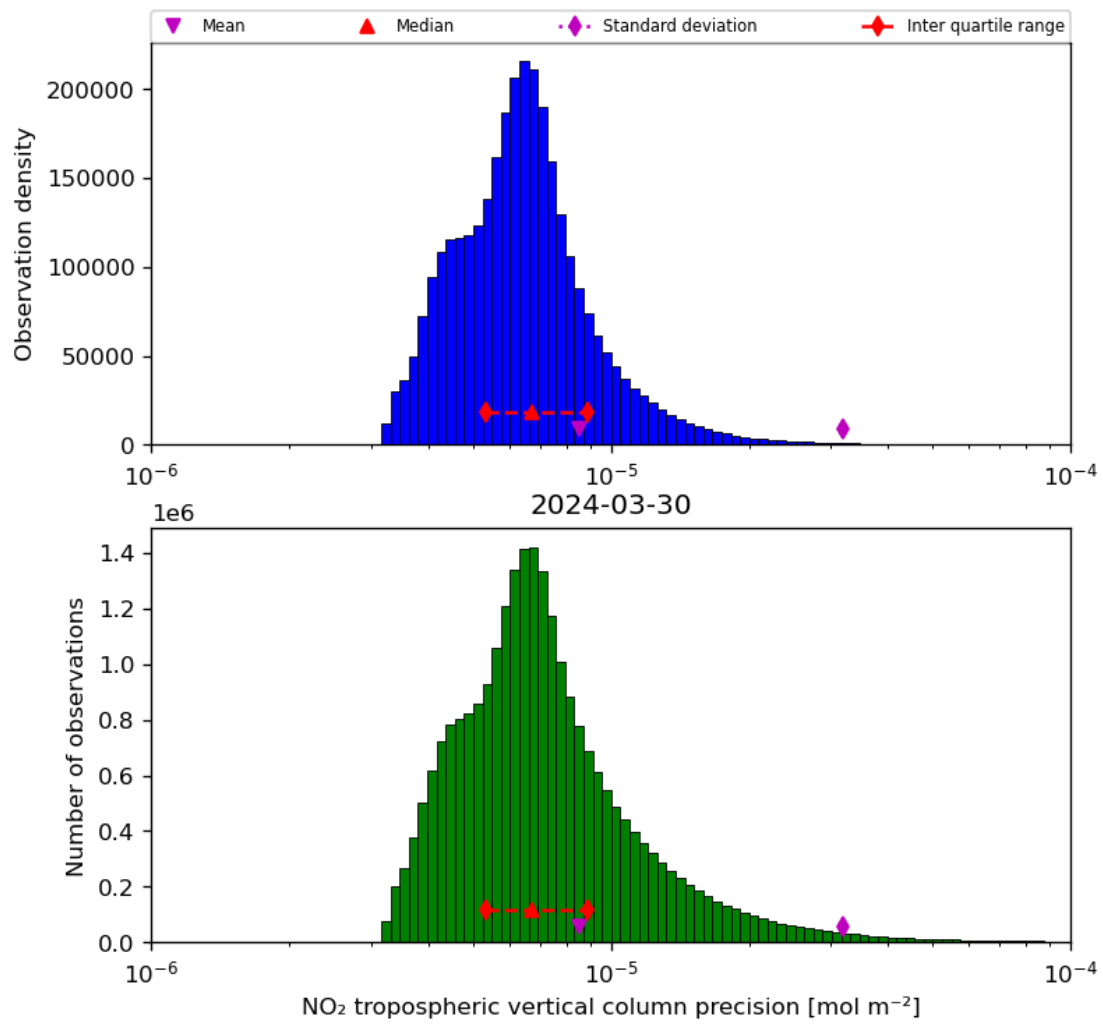
Figure 30: Histogram of “NO 2 tropospheric vertical column precision” for 2024-03-30 to 2024-03-31
