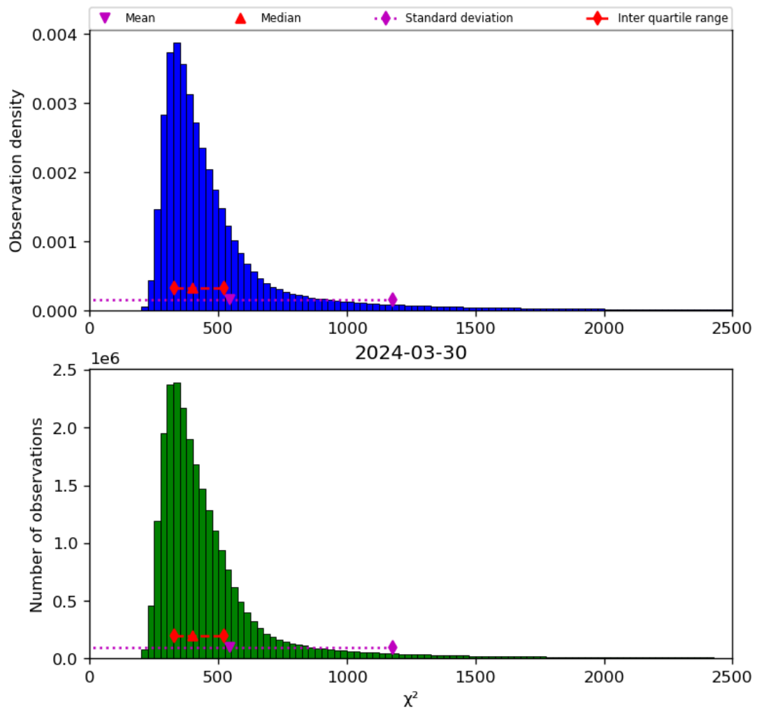
Figure 42: Histogram of “ \chi^2 ” for 2024-03-30 to 2024-03-31
