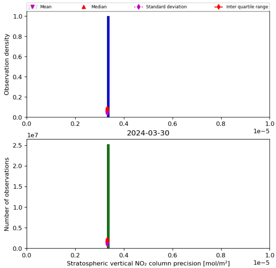
Figure 37: Histogram of “Stratospheric vertical NO 2 column precision” for 2024-03-30 to 2024-03-31
