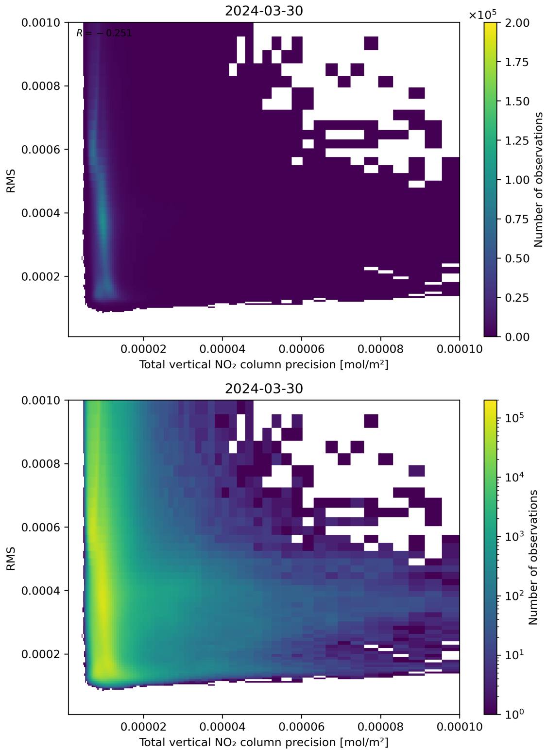
Figure 119: Scatter density plot of “Total vertical NO 2 column precision” against “RMS” for 2024-03-30 to 2024-03-31.
