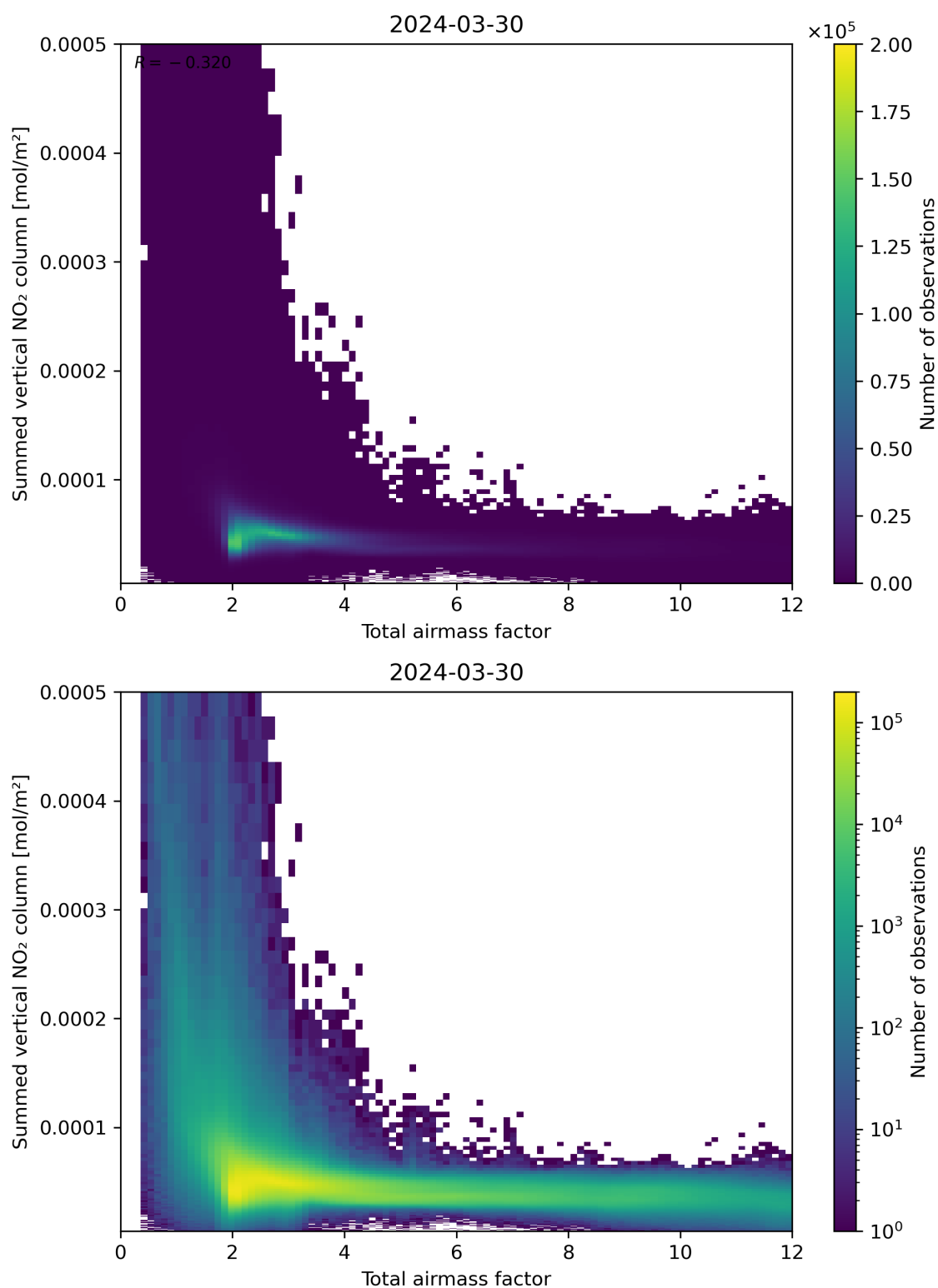
Figure 65: Scatter density plot of “Total airmass factor” against “Summed vertical NO 2 column” for 2024-03-30 to 2024-03-31.
