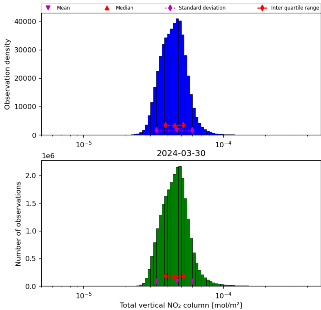
Figure 38: Histogram of “Total vertical NO 2 column” for 2024-03-30 to 2024-03-31
