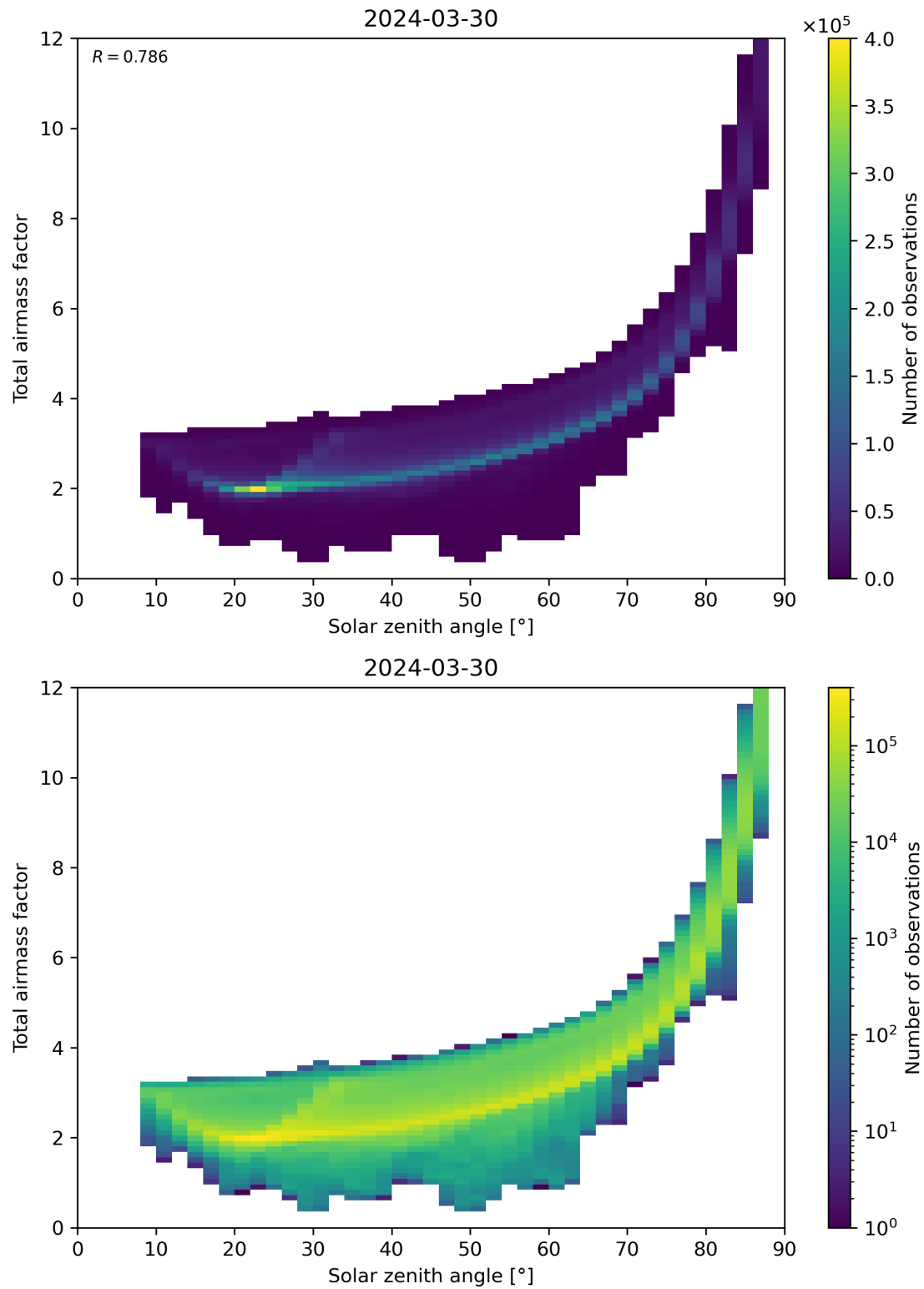
Figure 146: Scatter density plot of “Solar zenith angle” against “Total air mass factor” for 2024-03-30 to 2024-03-31.
