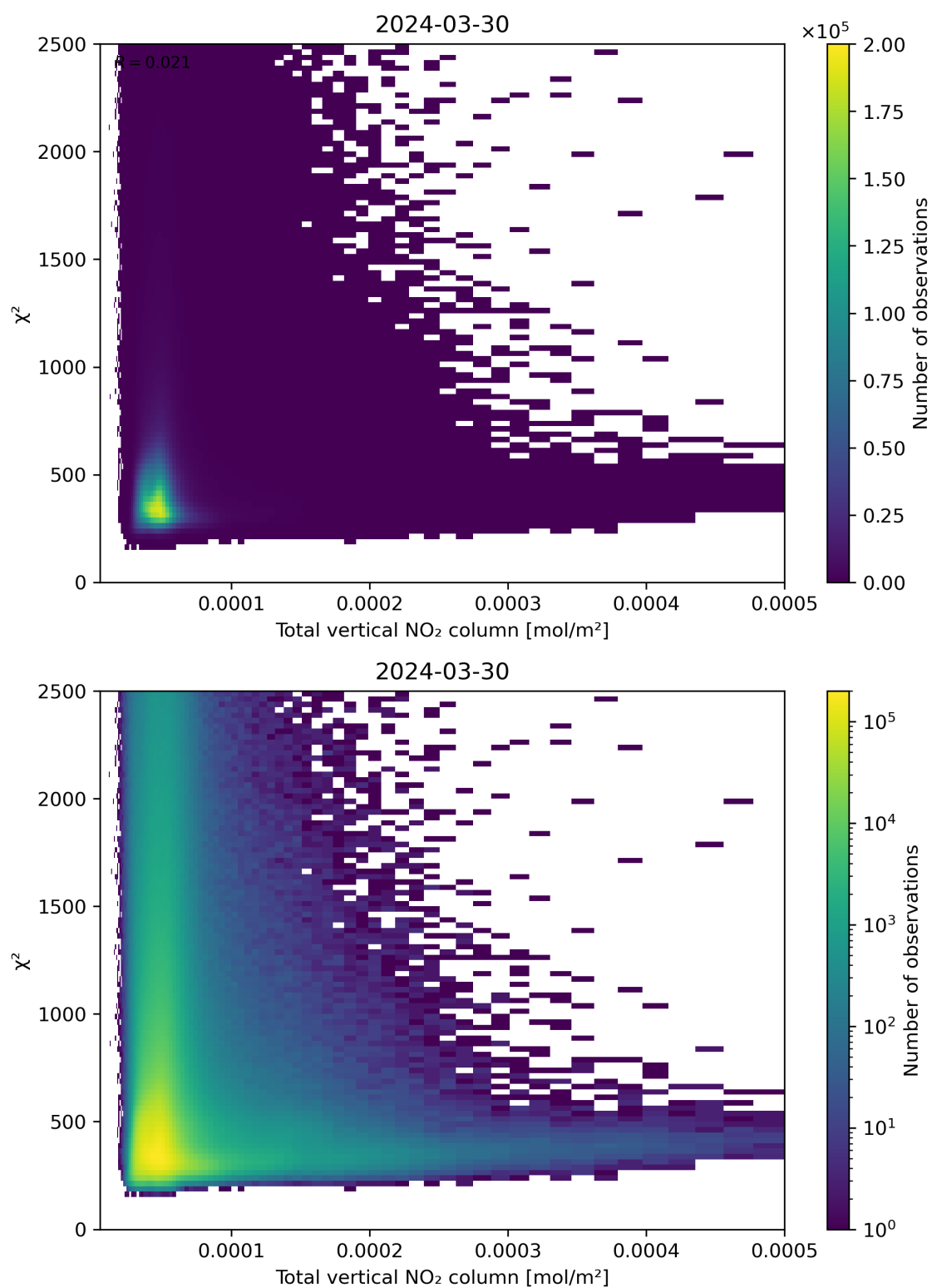
Figure 111: Scatter density plot of “Total vertical NO 2 column” against “ \chi^2 ” for 2024-03-30 to 2024-03-31.
