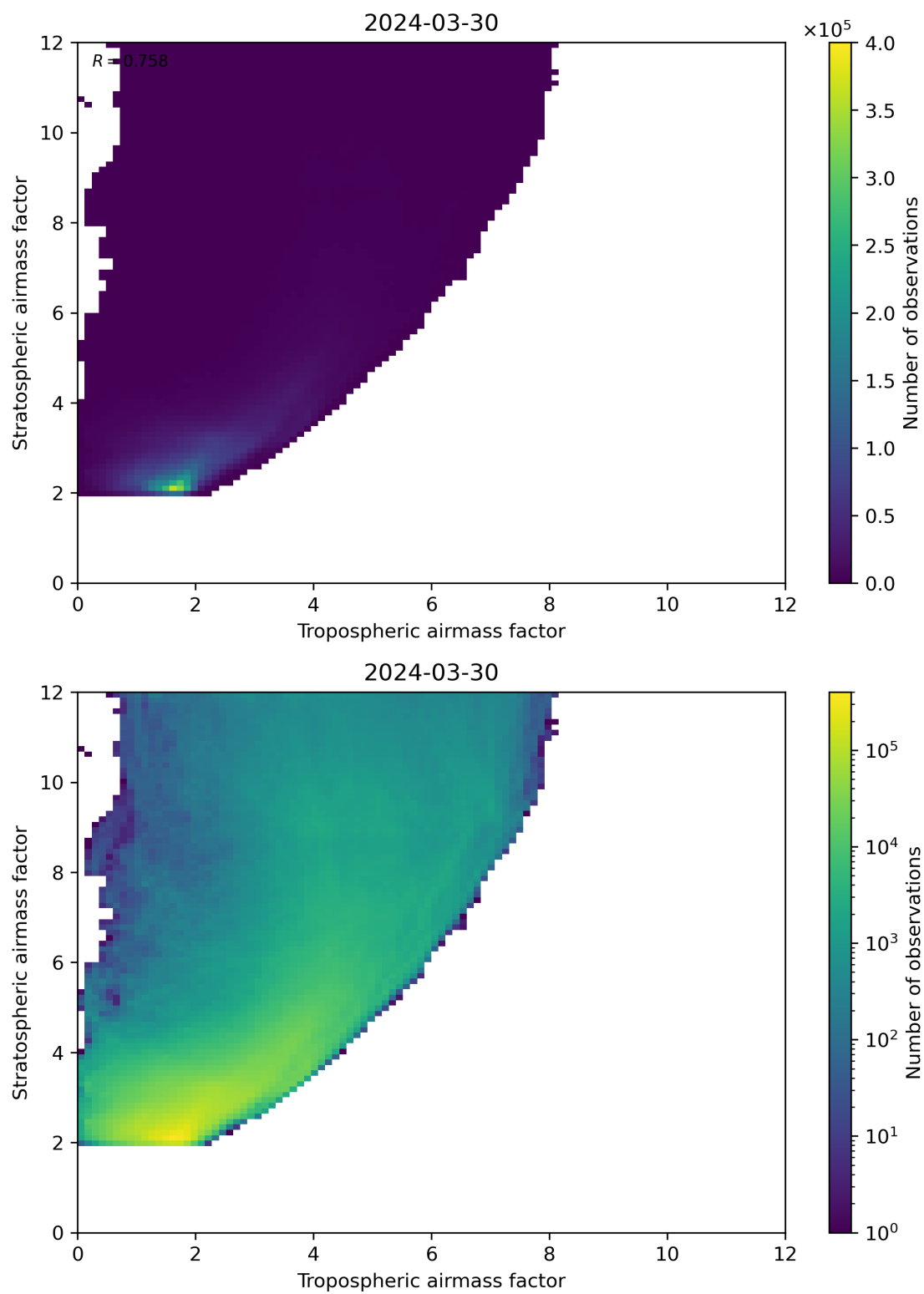
Figure 71: Scatter density plot of “Tropospheric airmass factor” against “Stratospheric airmass factor” for 2024-03-30 to 2024-03-31.
