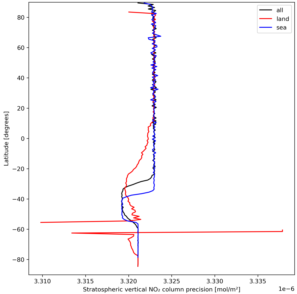
Figure 20: Zonal average of “Stratospheric vertical NO 2 column precision” for 2024-03-30 to 2024-03-31.
