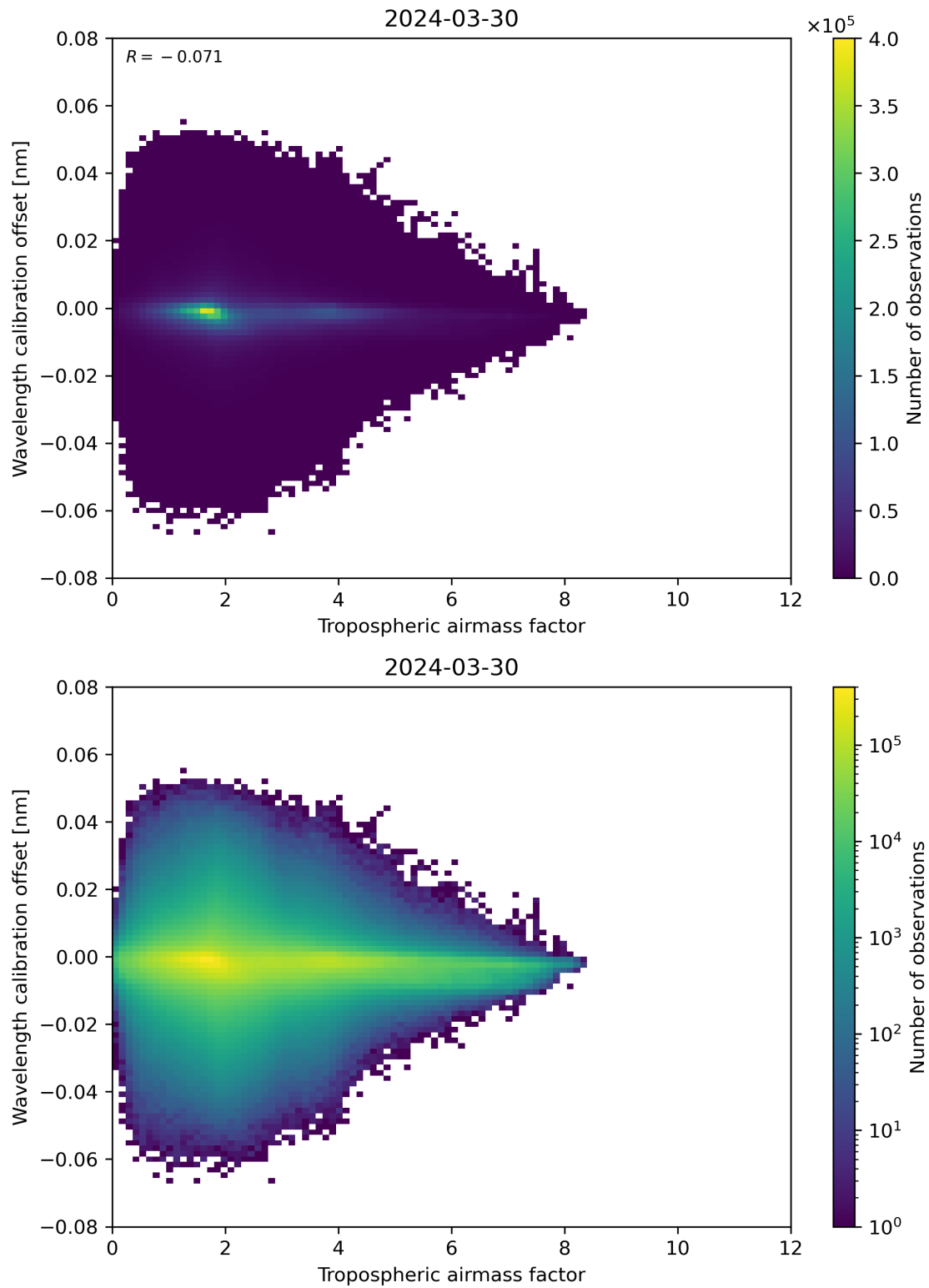
Figure 80: Scatter density plot of “Tropospheric airmass factor” against “Wavelength calibration offset” for 2024-03-30 to 2024-03-31.
