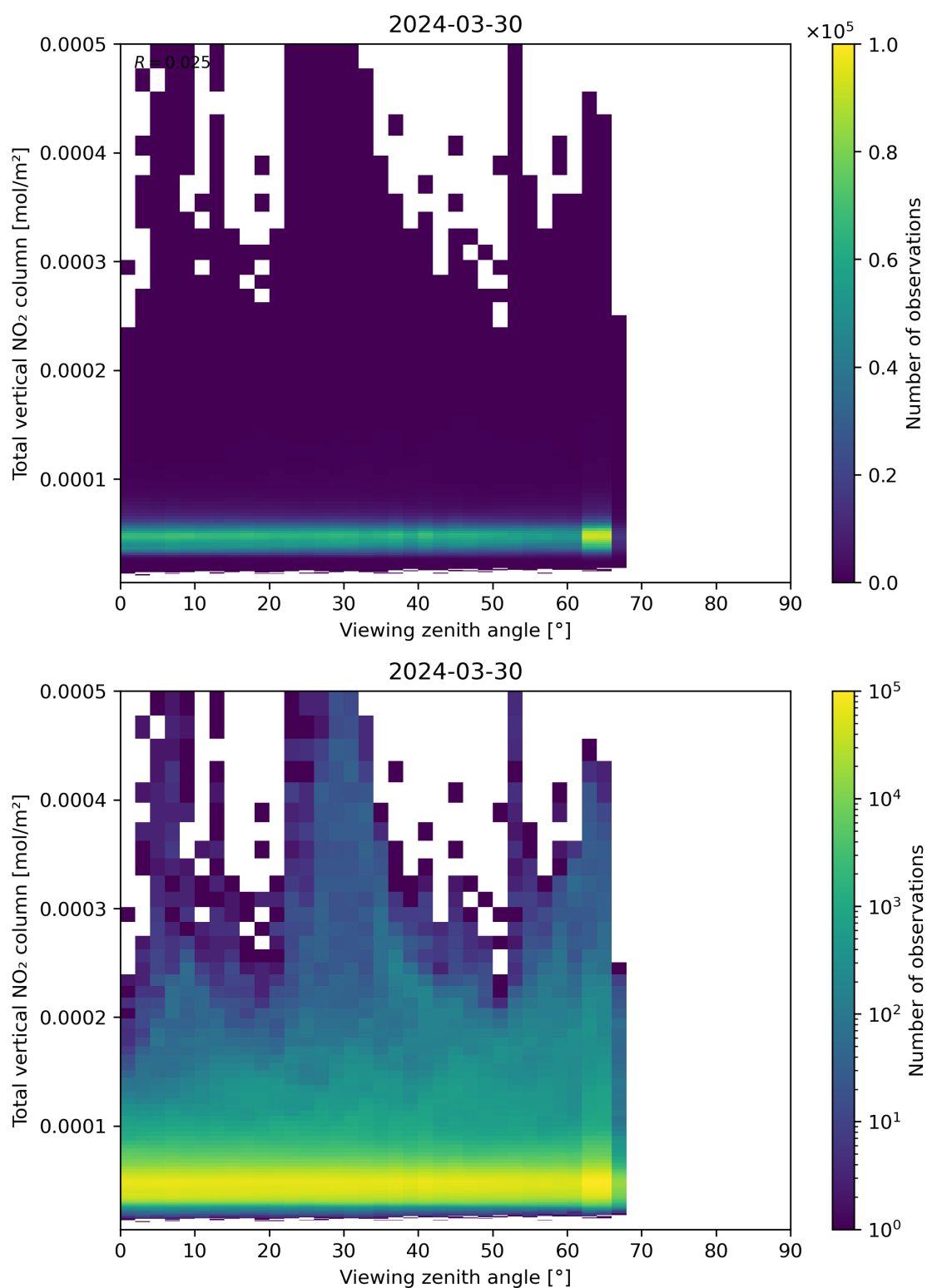
Figure 167: Scatter density plot of “Viewing zenith angle” against “Total vertical NO 2 column” for 2024-03-30 to 2024-03-31.
