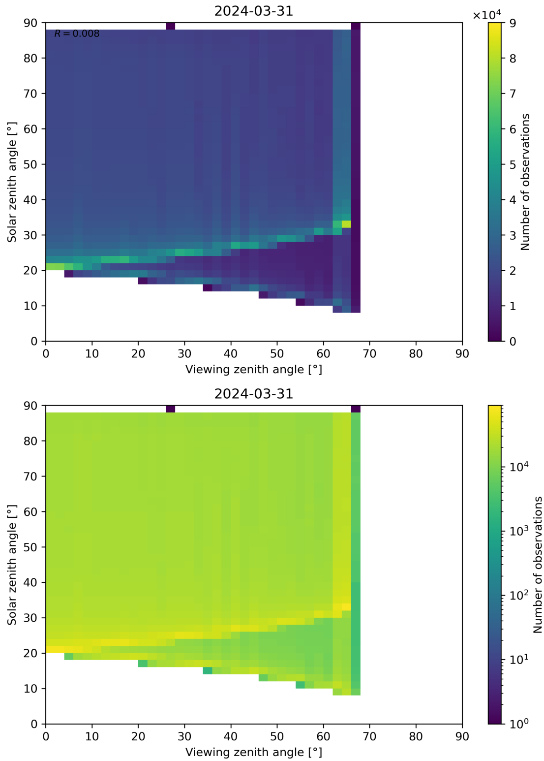
Figure 172: Scatter density plot of “Viewing zenith angle” against “Solar zenith angle” for 2024-03-31 to 2024-04-01.
