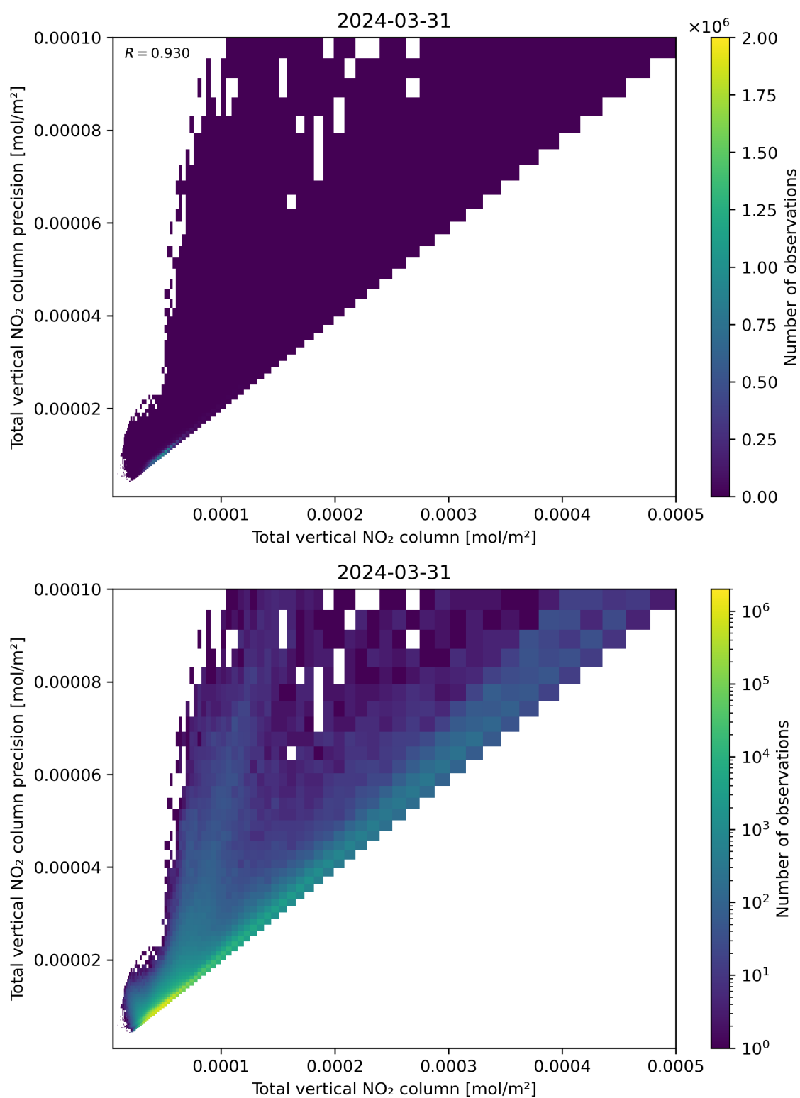
Figure 114: Scatter density plot of “Total vertical NO 2 column” against “Total vertical NO 2 column precision” for 2024-03-31 to 2024-04-01.
