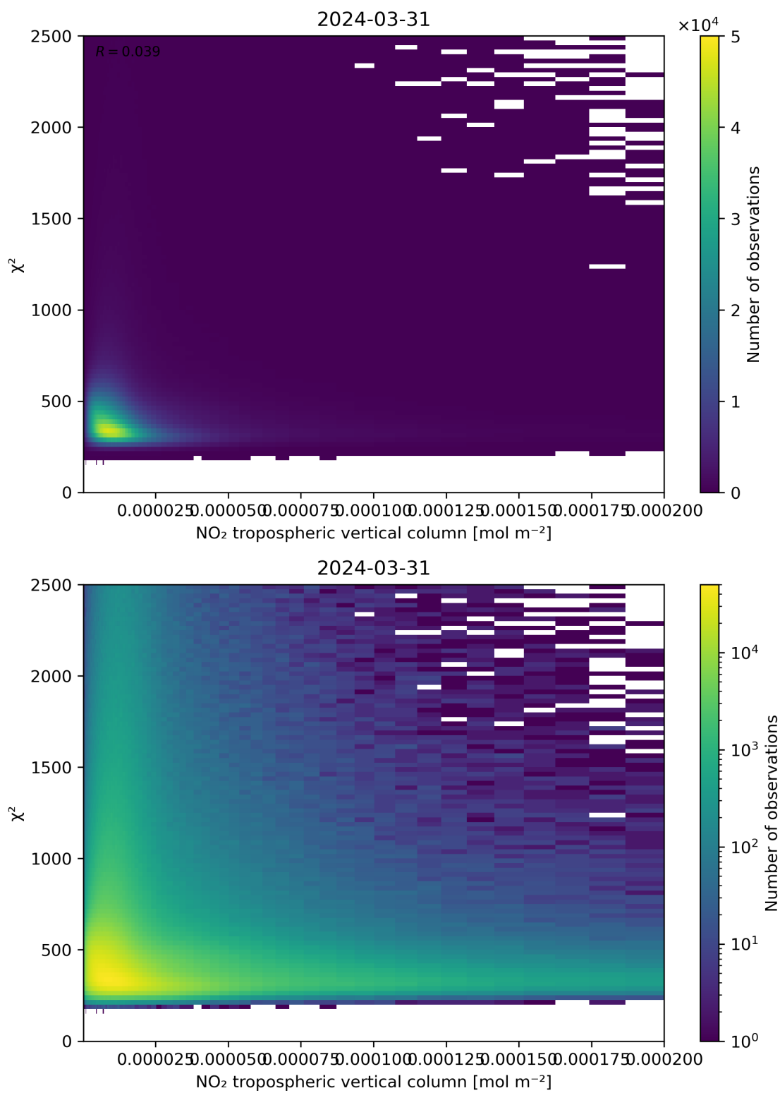
Figure 124: Scatter density plot of “NO 2 tropospheric vertical column” against “ \chi^2 ” for 2024-03-31 to 2024-04-01.
