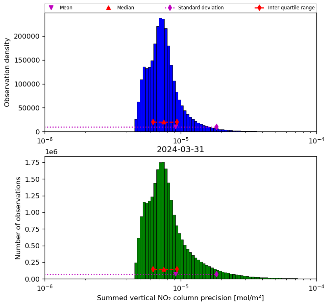
Figure 41: Histogram of “Summed vertical NO 2 column precision” for 2024-03-31 to 2024-04-01
