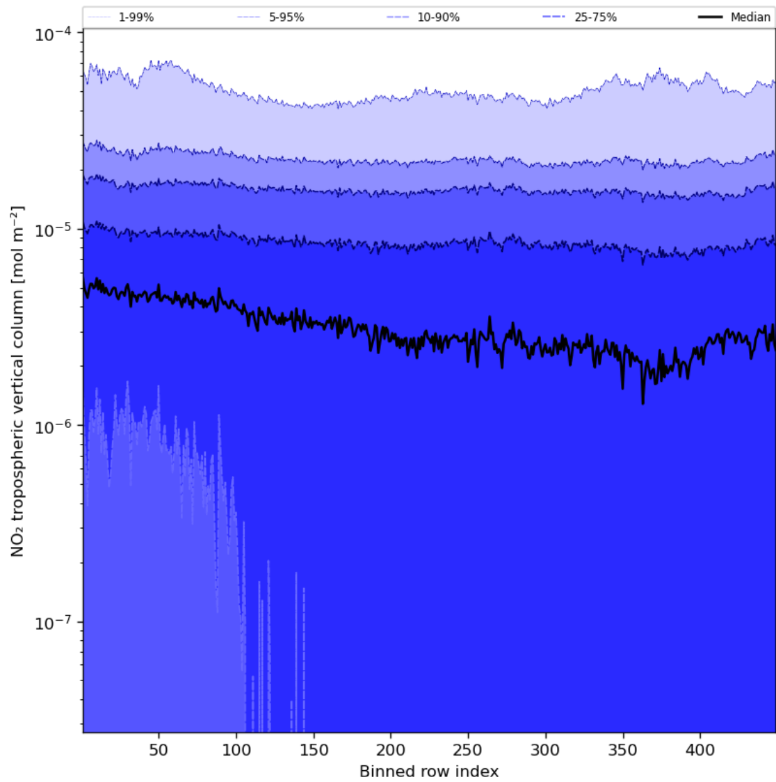
Figure 46: Along track statistics of “NO 2 tropospheric vertical column” for 2024-03-31 to 2024-04-01
