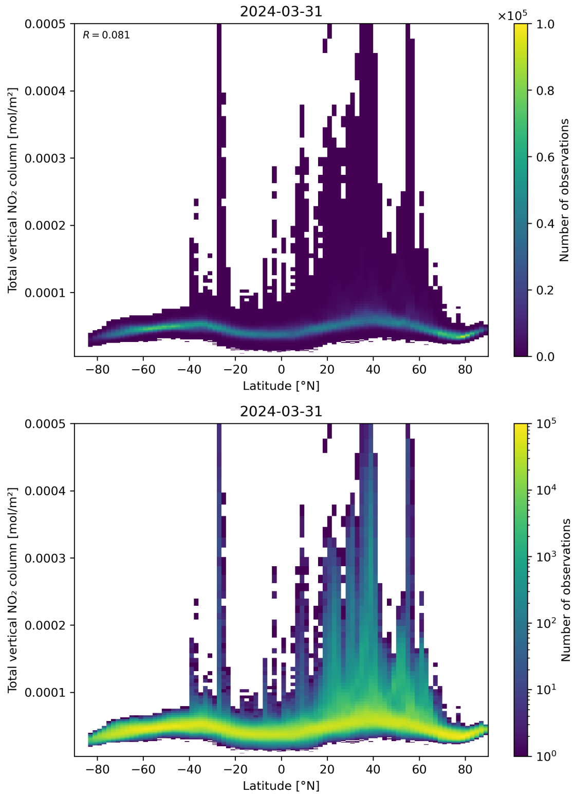
Figure 90: Scatter density plot of “Latitude” against “Total vertical NO 2 column” for 2024-03-31 to 2024-04-01.
