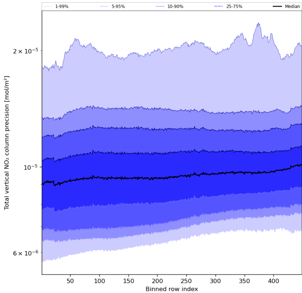
Figure 56: Along track statistics of “Total vertical NO 2 column precision” for 2024-03-31 to 2024-04-01
