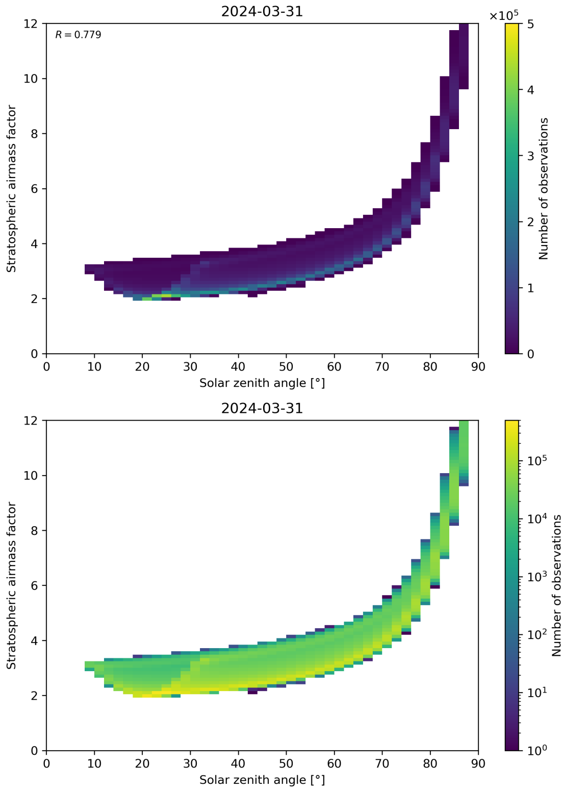
Figure 145: Scatter density plot of “Solar zenith angle” against “Stratospheric airmass factor” for 2024-03-31 to 2024-04-01.
