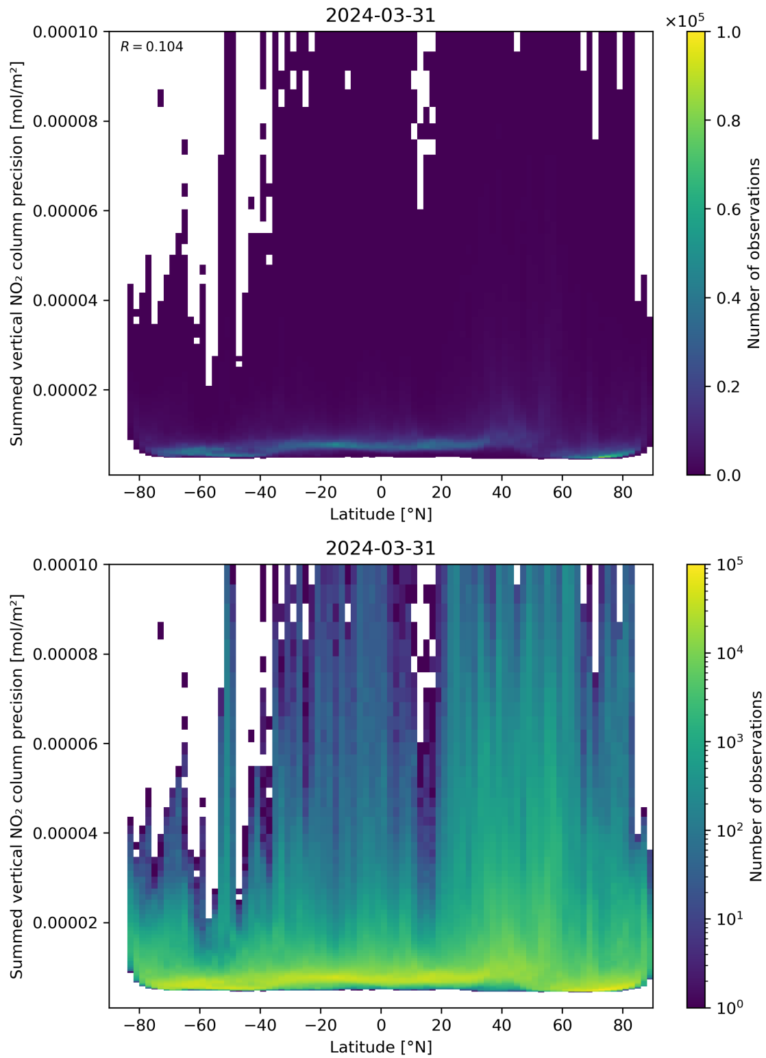
Figure 89: Scatter density plot of “Latitude” against “Summed vertical NO 2 column precision” for 2024-03-31 to 2024-04-01.
