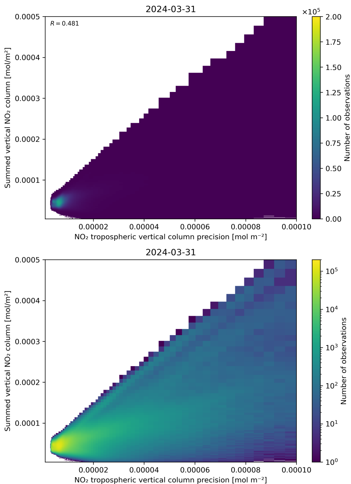
Figure 136: Scatter density plot of “NO 2 tropospheric vertical column precision” against “Summed vertical NO 2 column” for 2024-03-31 to 2024-04-01.
