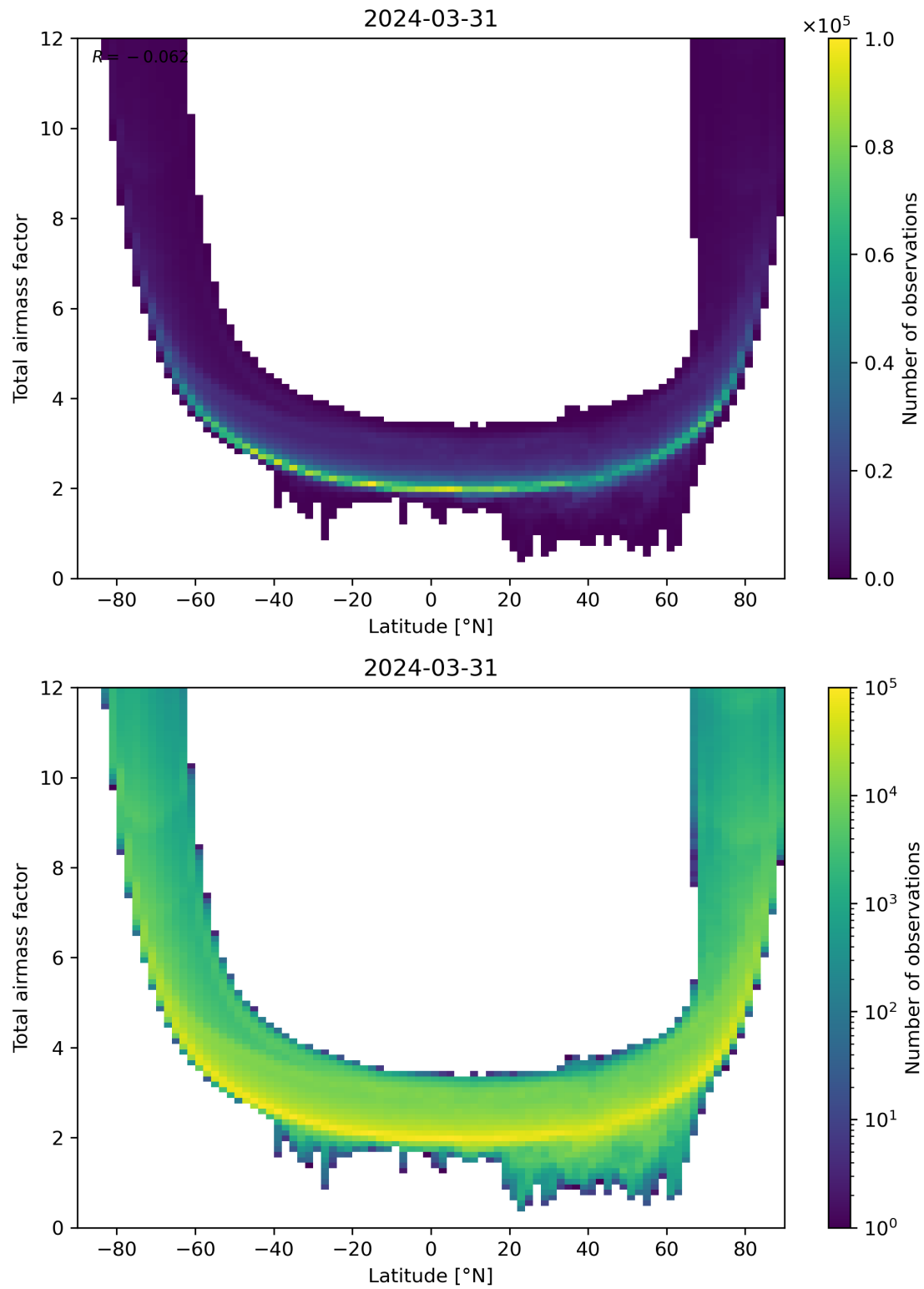
Figure 84: Scatter density plot of “Latitude” against “Total airmass factor” for 2024-03-31 to 2024-04-01.
