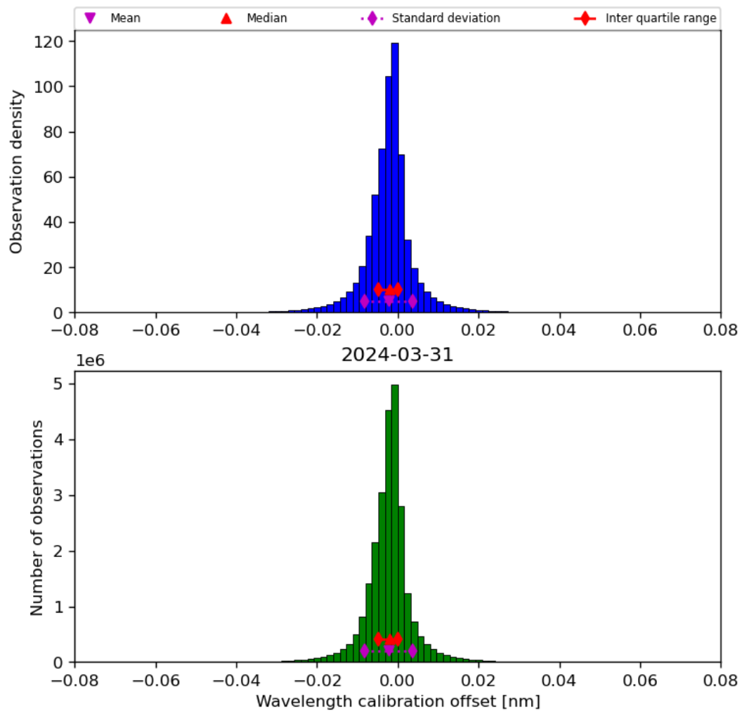
Figure 35: Histogram of “Wavelength calibration offset” for 2024-03-31 to 2024-04-01
