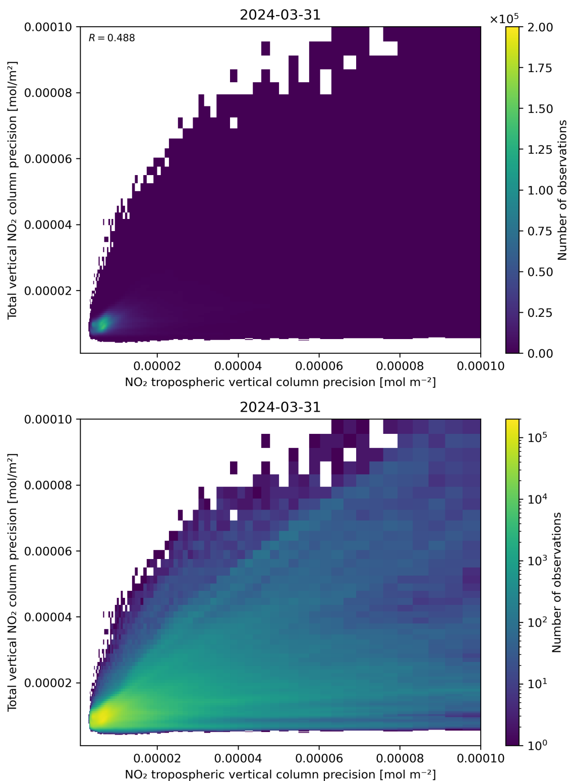
Figure 139: Scatter density plot of “NO 2 tropospheric vertical column precision” against “Total vertical NO 2 column precision” for 2024-03-31 to 2024-04-01.
