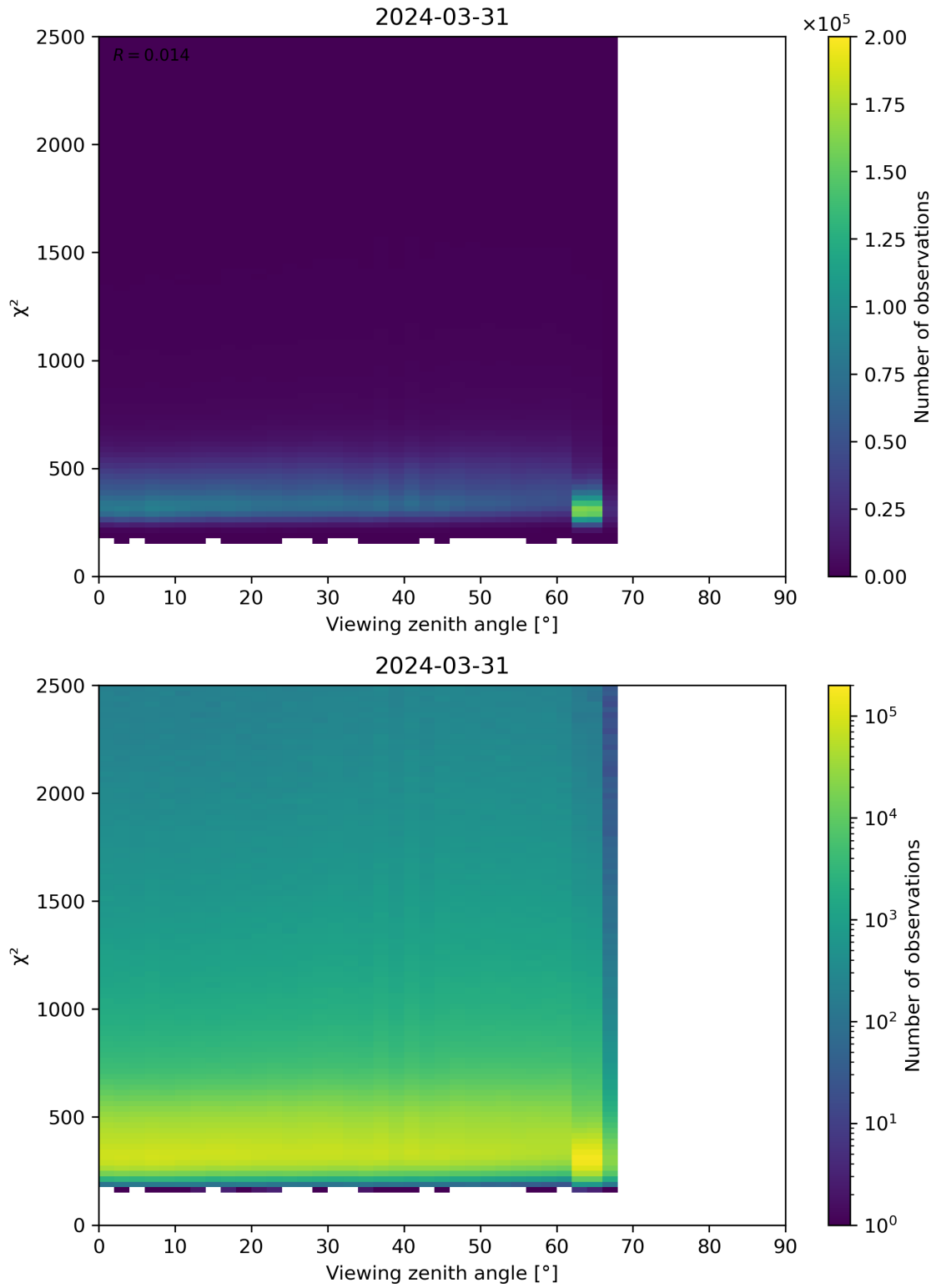
Figure 162: Scatter density plot of “Viewing zenith angle” against “ \chi^2 ” for 2024-03-31 to 2024-04-01.
