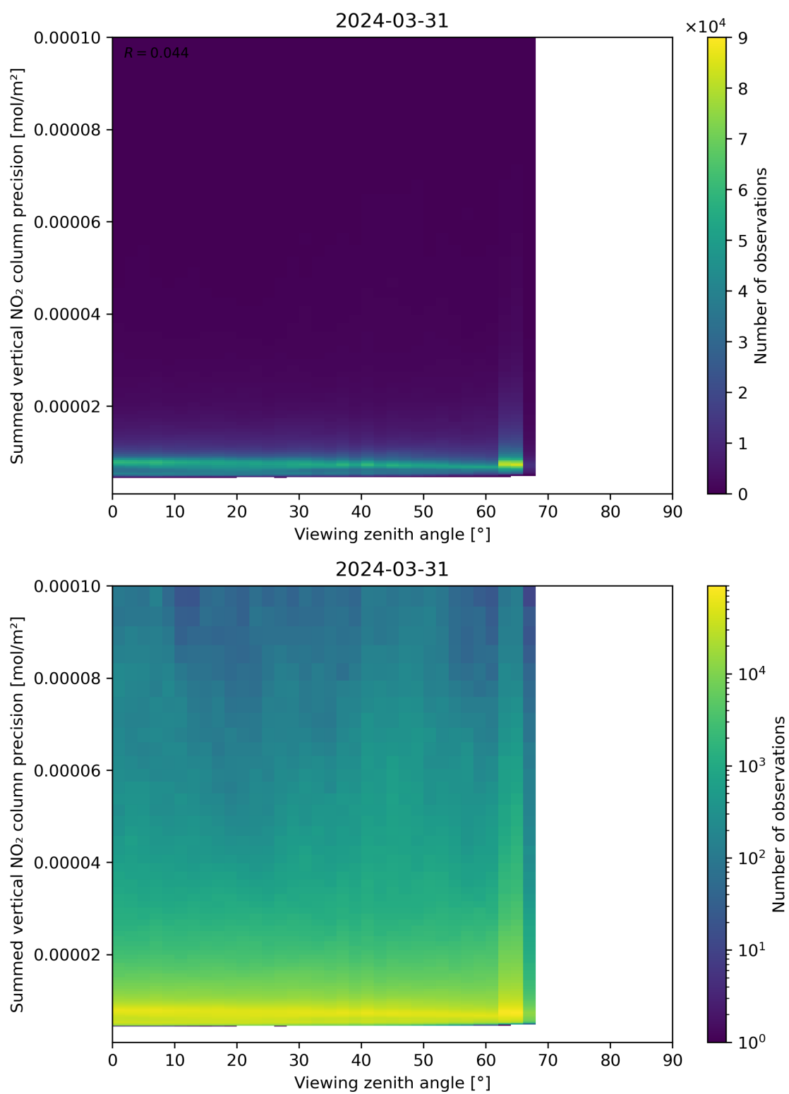
Figure 166: Scatter density plot of “Viewing zenith angle” against “Summed vertical NO 2 column precision” for 2024-03-31 to 2024-04-01.
