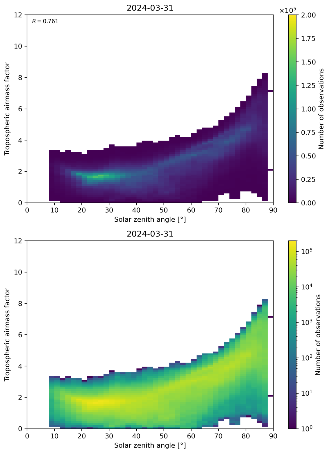
Figure 147: Scatter density plot of “Solar zenith angle” against “Tropospheric airmass factor” for 2024-03-31 to 2024-04-01.
