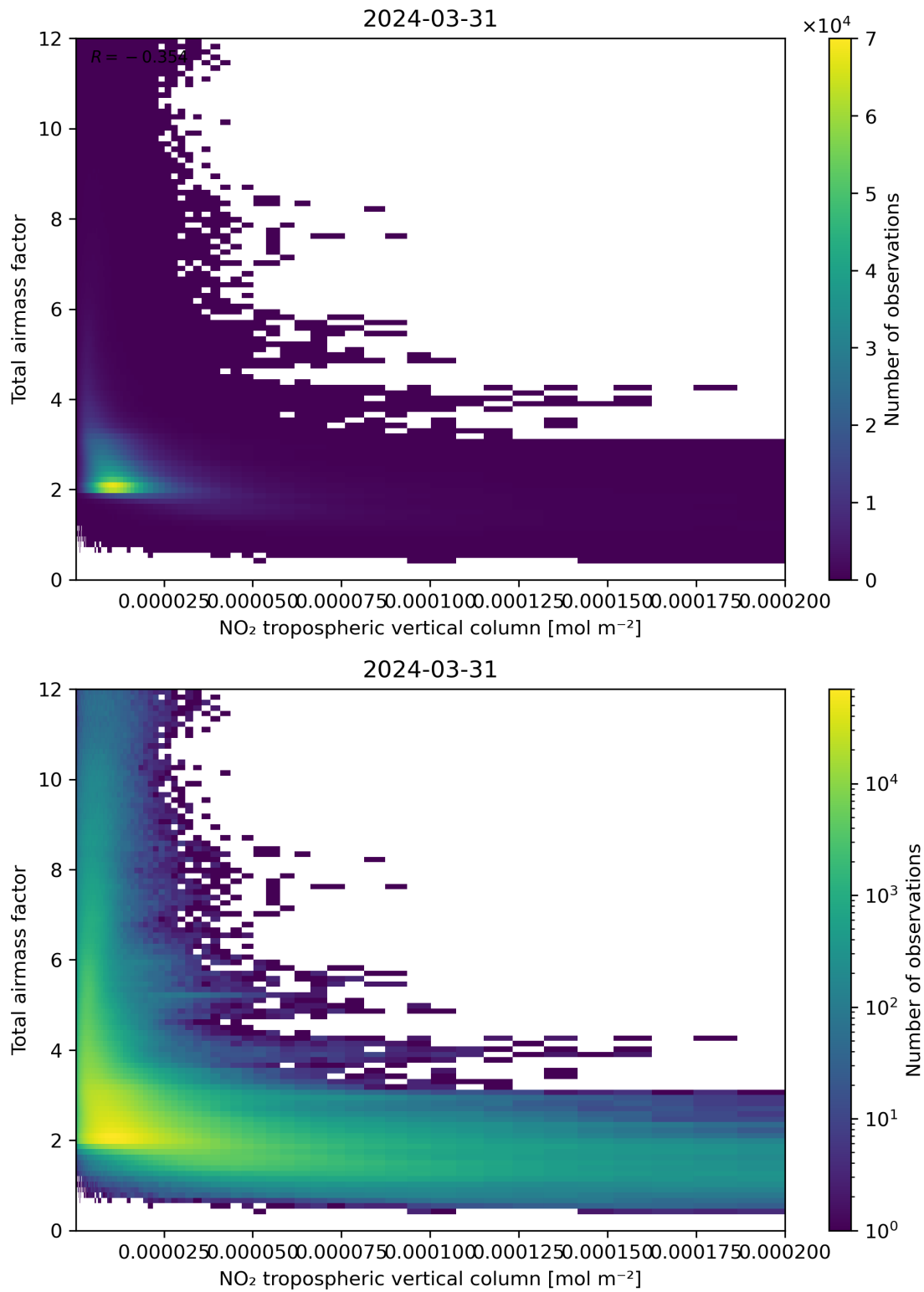
Figure 122: Scatter density plot of “NO 2 tropospheric vertical column” against “Total air mass factor” for 2024-03-31 to 2024-04-01.
