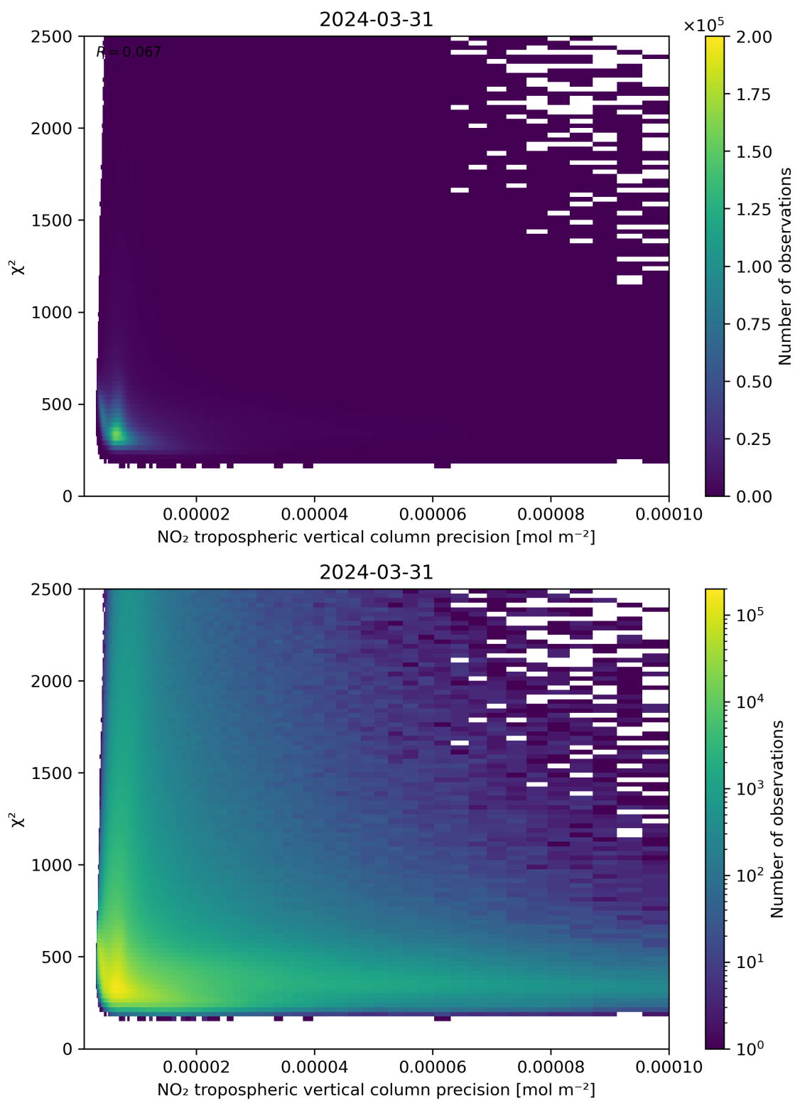
Figure 134: Scatter density plot of “NO 2 tropospheric vertical column precision” against “ \chi^2 ” for 2024-03-31 to 2024-04-01.
