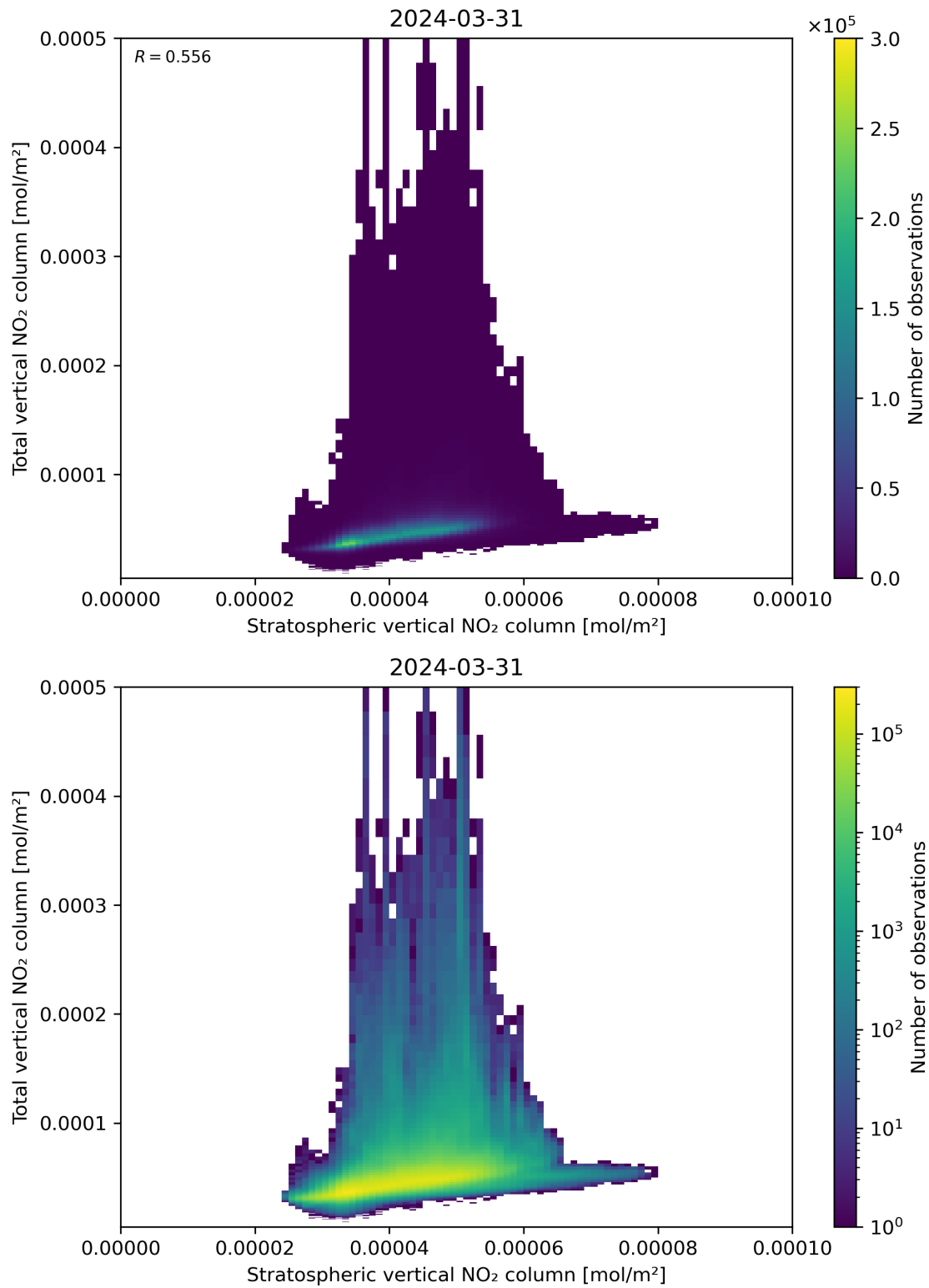
Figure 100: Scatter density plot of “Stratospheric vertical NO 2 column” against “Total vertical NO 2 column” for 2024-03-31 to 2024-04-01.
