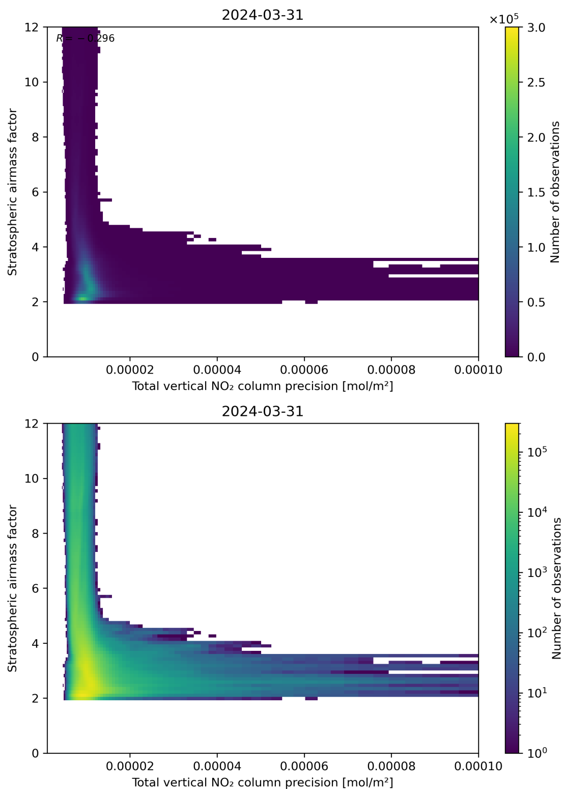
Figure 115: Scatter density plot of “Total vertical NO 2 column precision” against “Stratospheric air mass factor” for 2024-03-31 to 2024-04-01.
