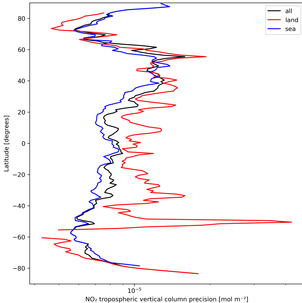
Figure 13: Zonal average of “NO 2 tropospheric vertical column precision” for 2024-03-31 to 2024-04-01.
