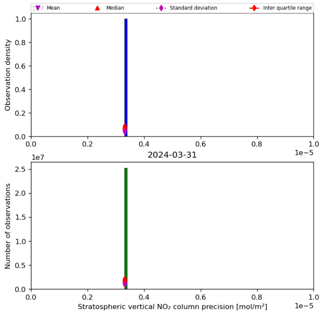
Figure 37: Histogram of “Stratospheric vertical NO 2 column precision” for 2024-03-31 to 2024-04-01
