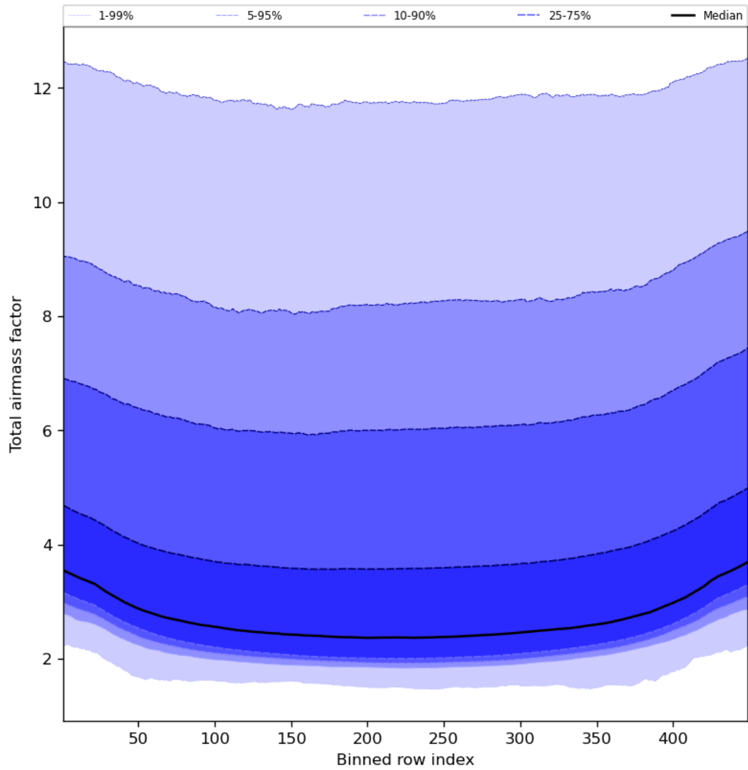
Figure 49: Along track statistics of “Total airmass factor” for 2024-03-31 to 2024-04-01
