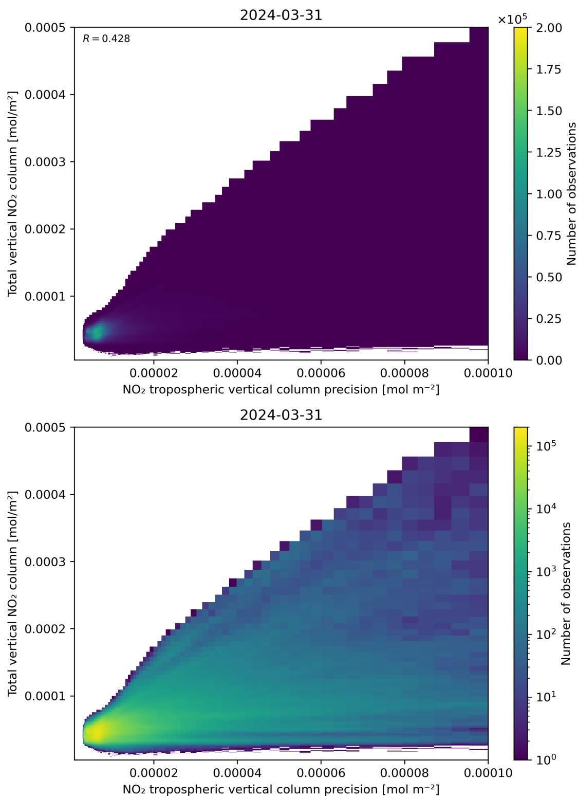
Figure 138: Scatter density plot of “NO 2 tropospheric vertical column precision” against “Total vertical NO 2 column” for 2024-03-31 to 2024-04-01.
