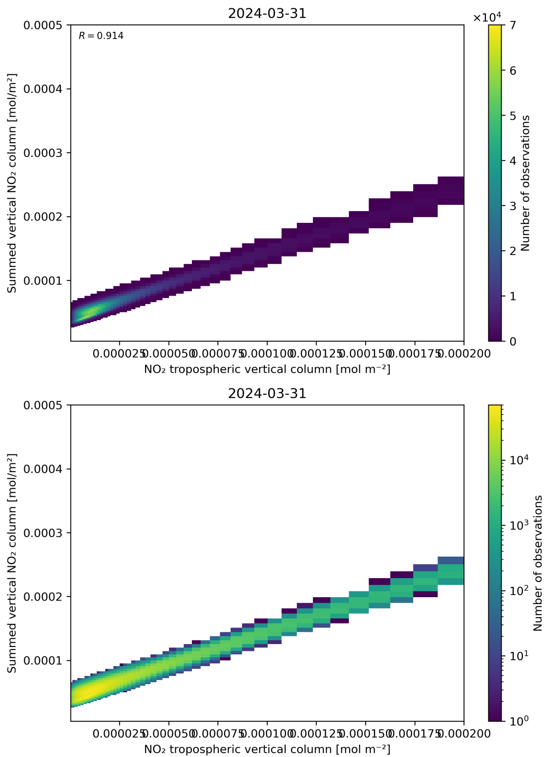
Figure 126: Scatter density plot of “NO 2 tropospheric vertical column” against “Summed vertical NO 2 column” for 2024-03-31 to 2024-04-01.
