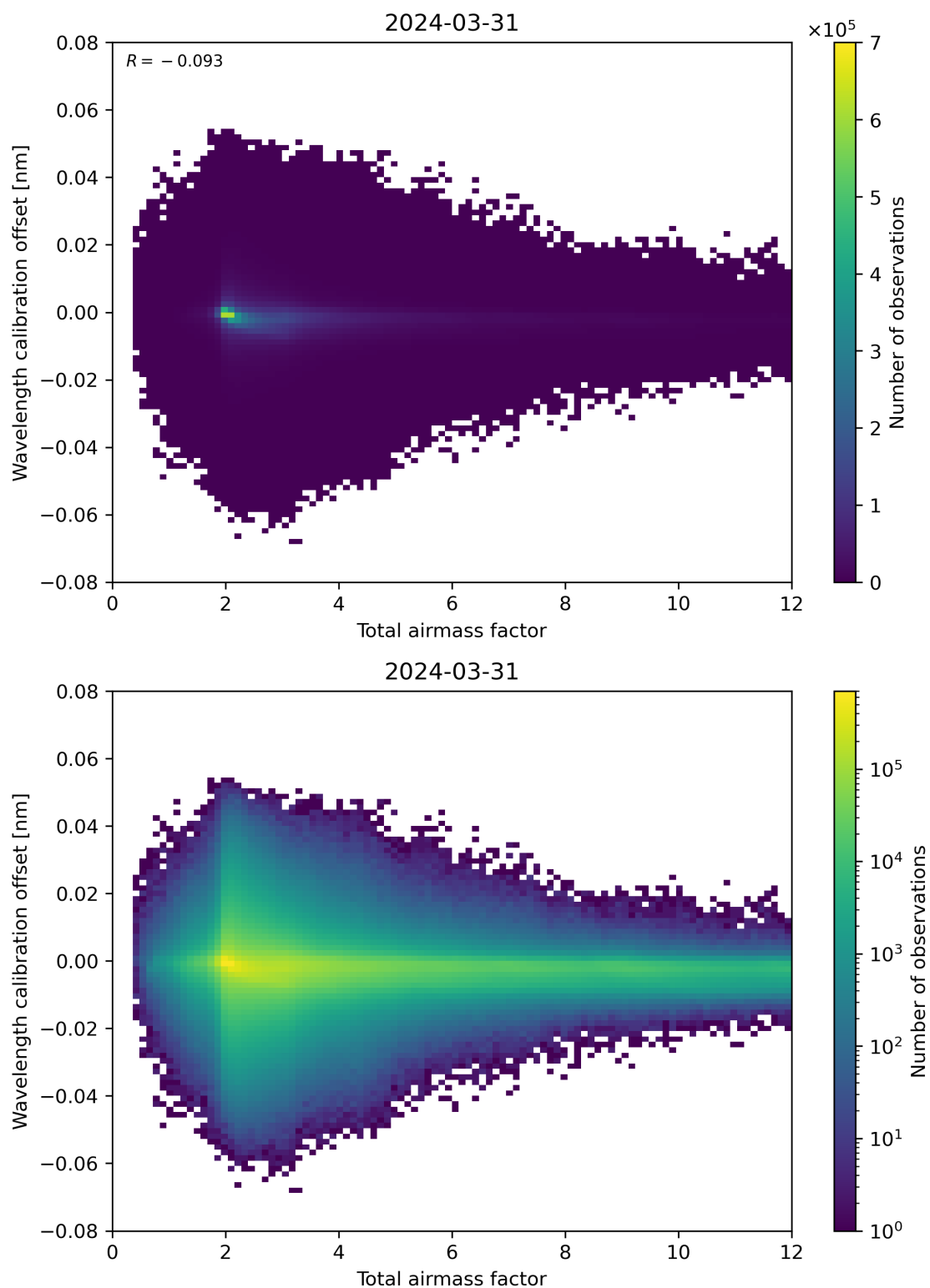
Figure 70: Scatter density plot of “Total airmass factor” against “Wavelength calibration offset” for 2024-03-31 to 2024-04-01.
