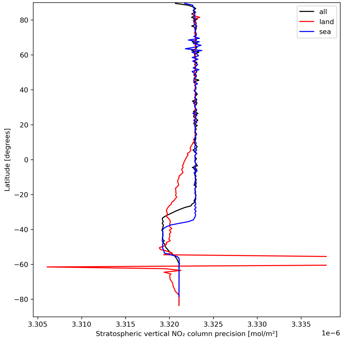
Figure 20: Zonal average of “Stratospheric vertical NO 2 column precision” for 2024-03-31 to 2024-04-01.
