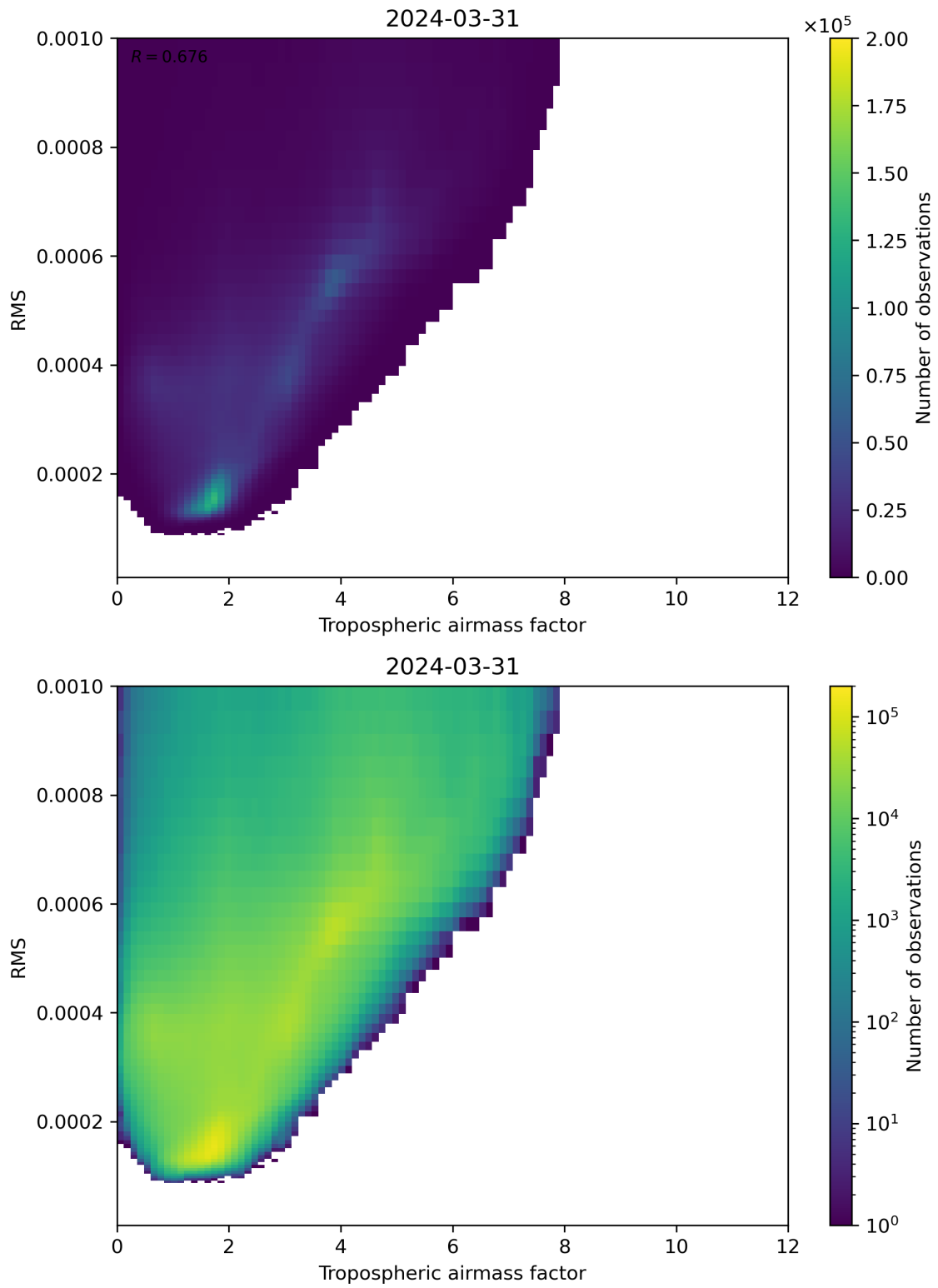
Figure 79: Scatter density plot of “Tropospheric airmass factor” against “RMS” for 2024-03-31 to 2024-04-01.
