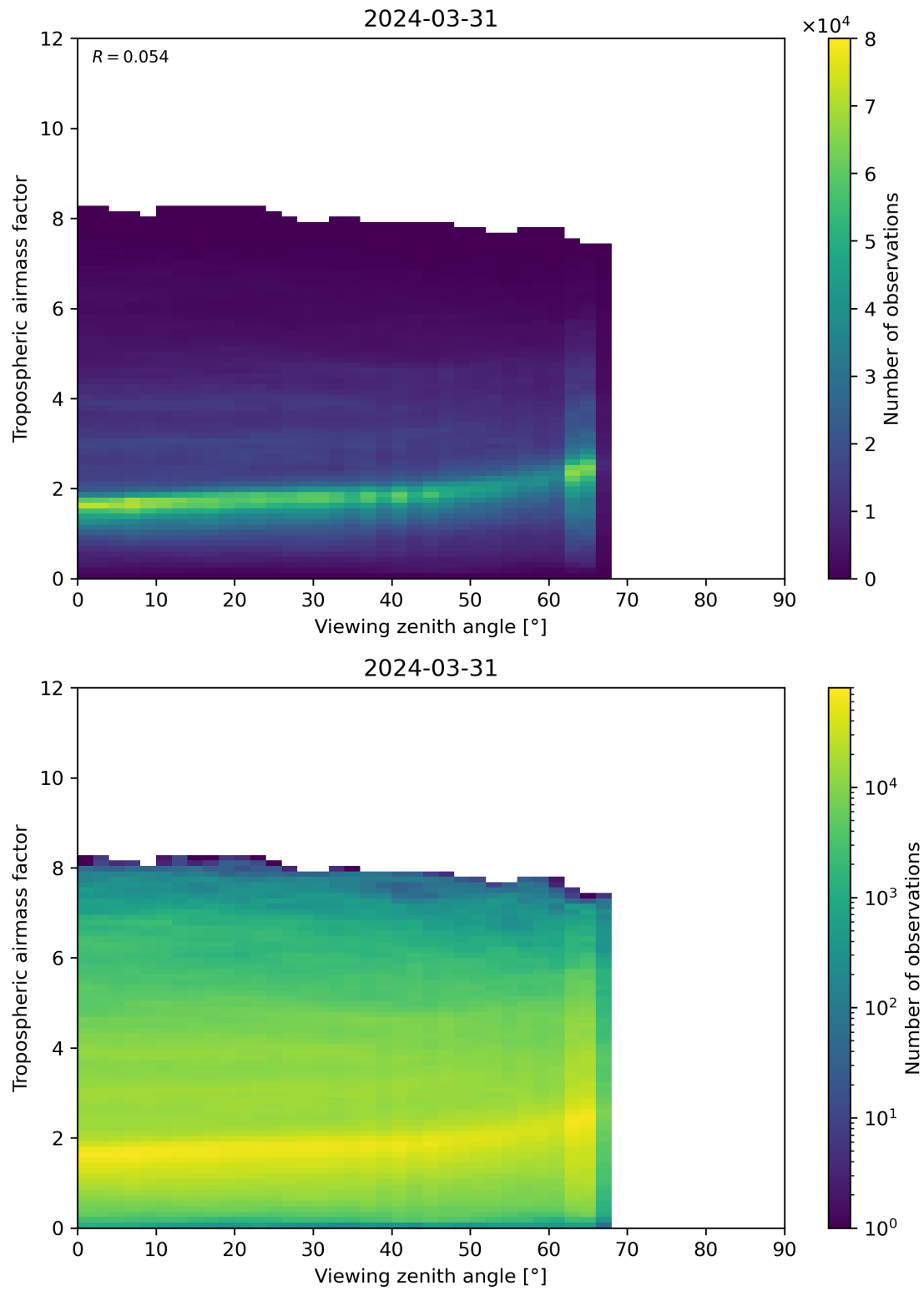
Figure 161: Scatter density plot of “Viewing zenith angle” against “Tropospheric airmass factor” for 2024-03-31 to 2024-04-01.
