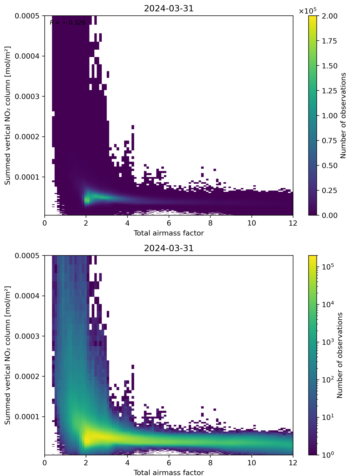
Figure 65: Scatter density plot of “Total airmass factor” against “Summed vertical NO 2 column” for 2024-03-31 to 2024-04-01.
