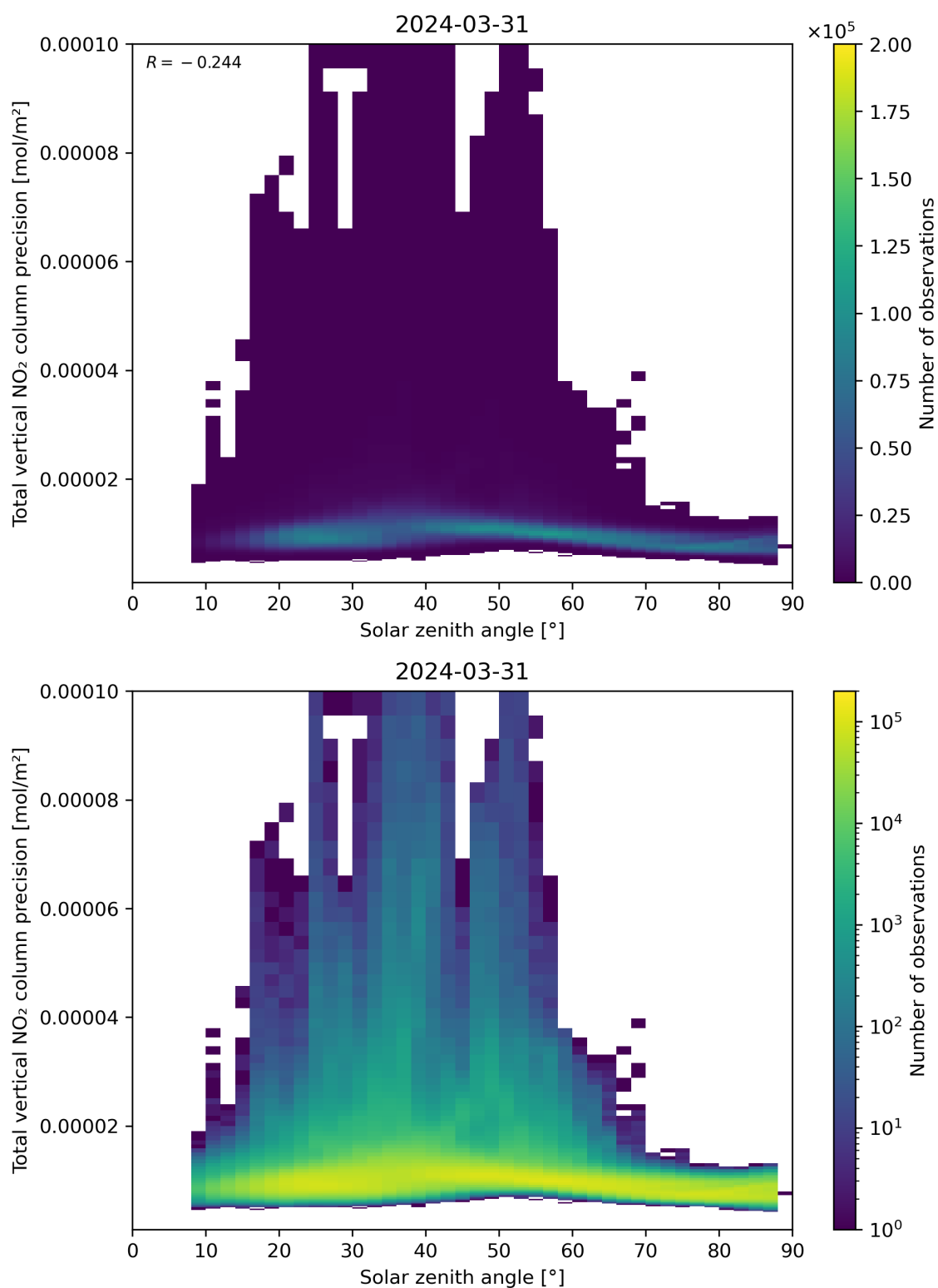
Figure 154: Scatter density plot of “Solar zenith angle” against “Total vertical NO 2 column precision” for 2024-03-31 to 2024-04-01.
