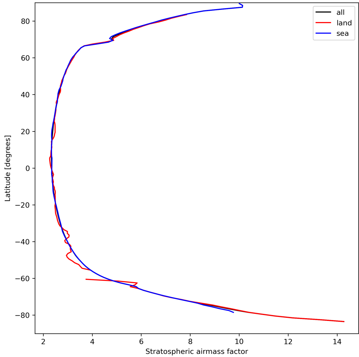
Figure 27: Zonal average of “Stratospheric airmass factor” for 2024-03-31 to 2024-04-01.
