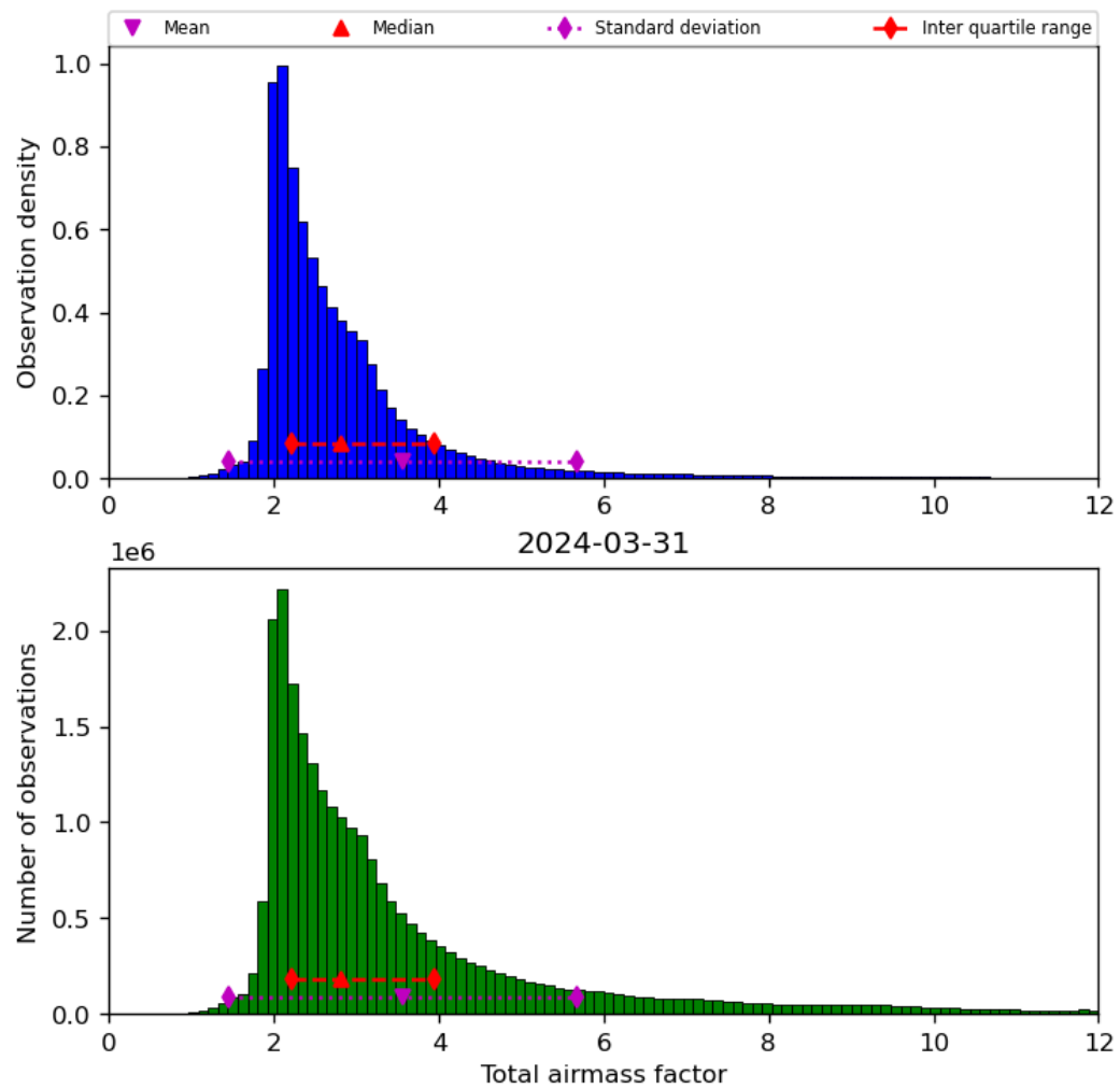
Figure 32: Histogram of “Total airmass factor” for 2024-03-31 to 2024-04-01
