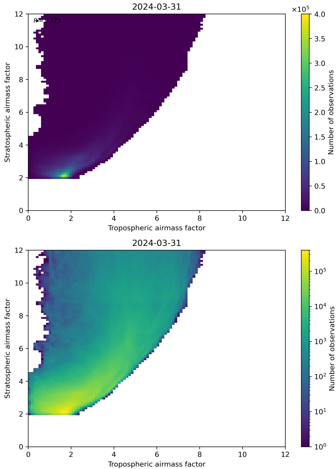
Figure 71: Scatter density plot of “Tropospheric airmass factor” against “Stratospheric airmass factor” for 2024-03-31 to 2024-04-01.
