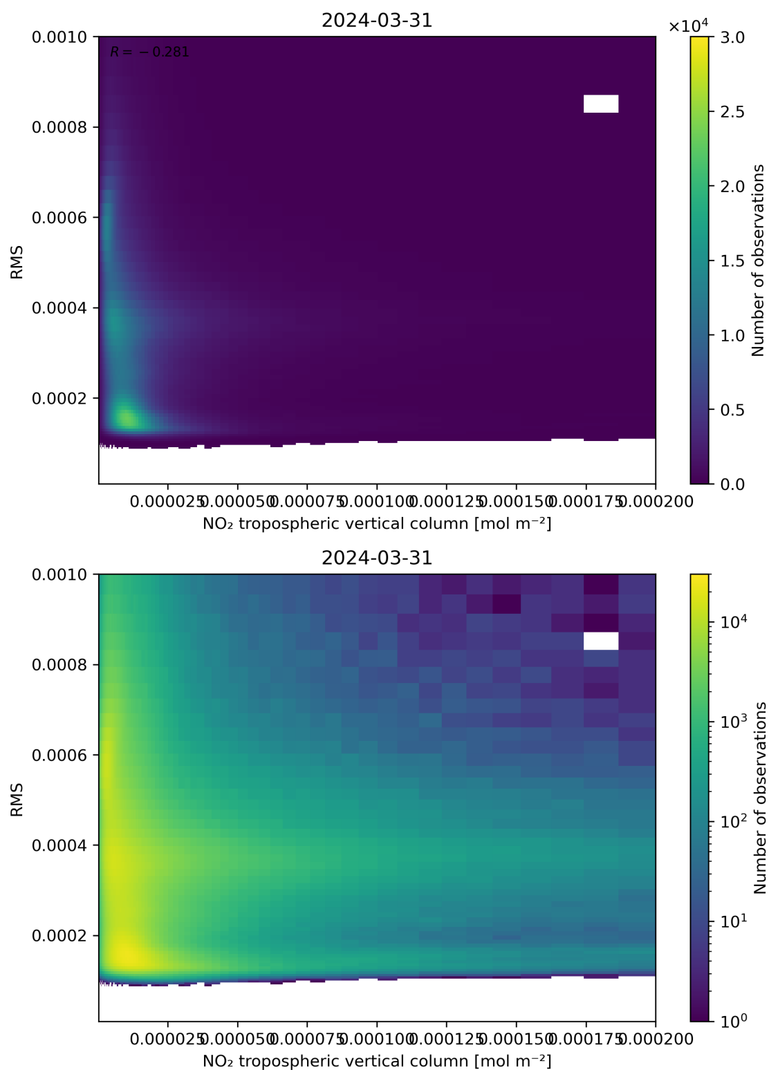
Figure 142: Scatter density plot of “NO 2 tropospheric vertical column” against “RMS” for 2024-03-31 to 2024-04-01.
