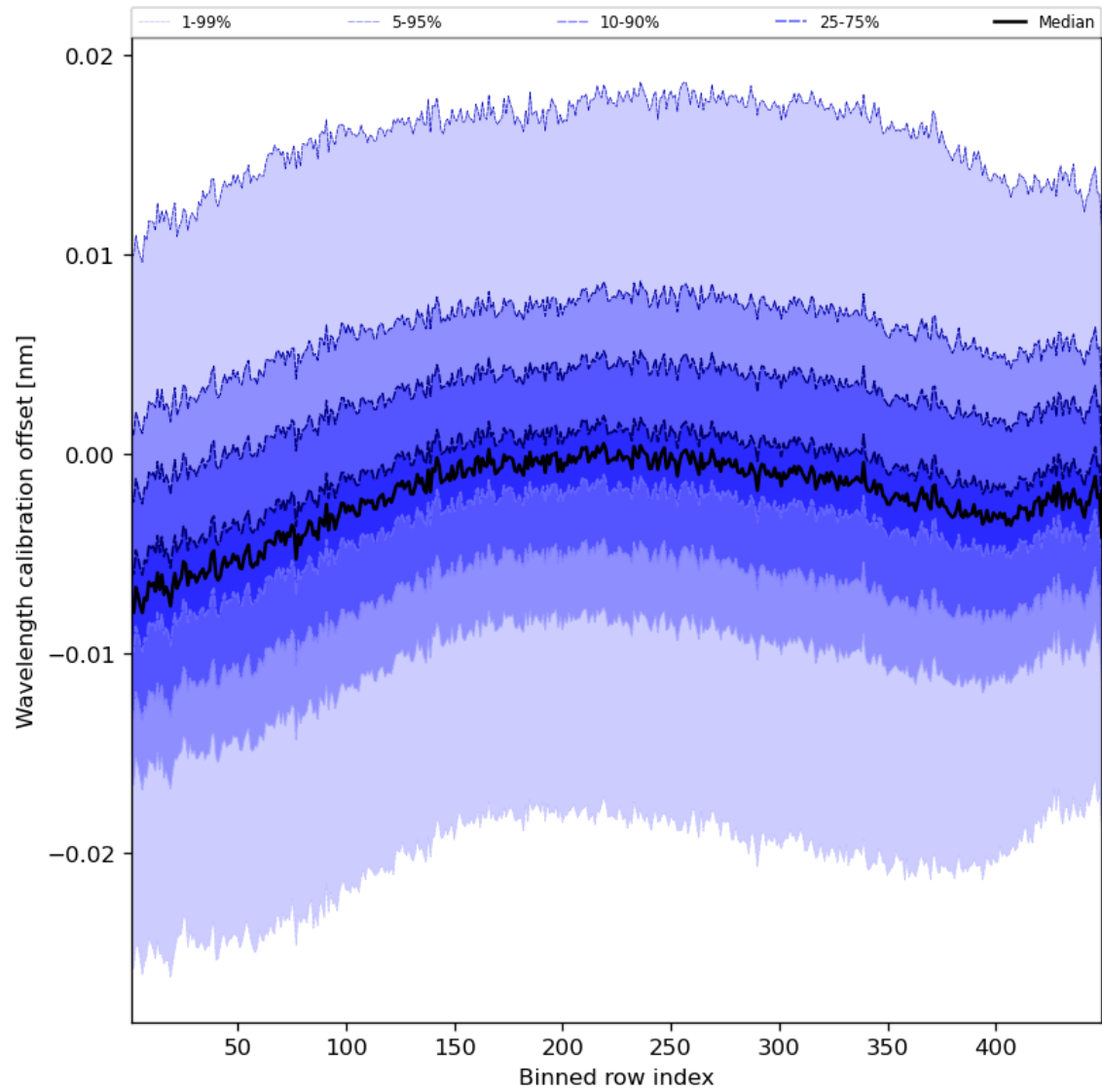
Figure 52: Along track statistics of “Wavelength calibration offset” for 2024-03-31 to 2024-04-01
