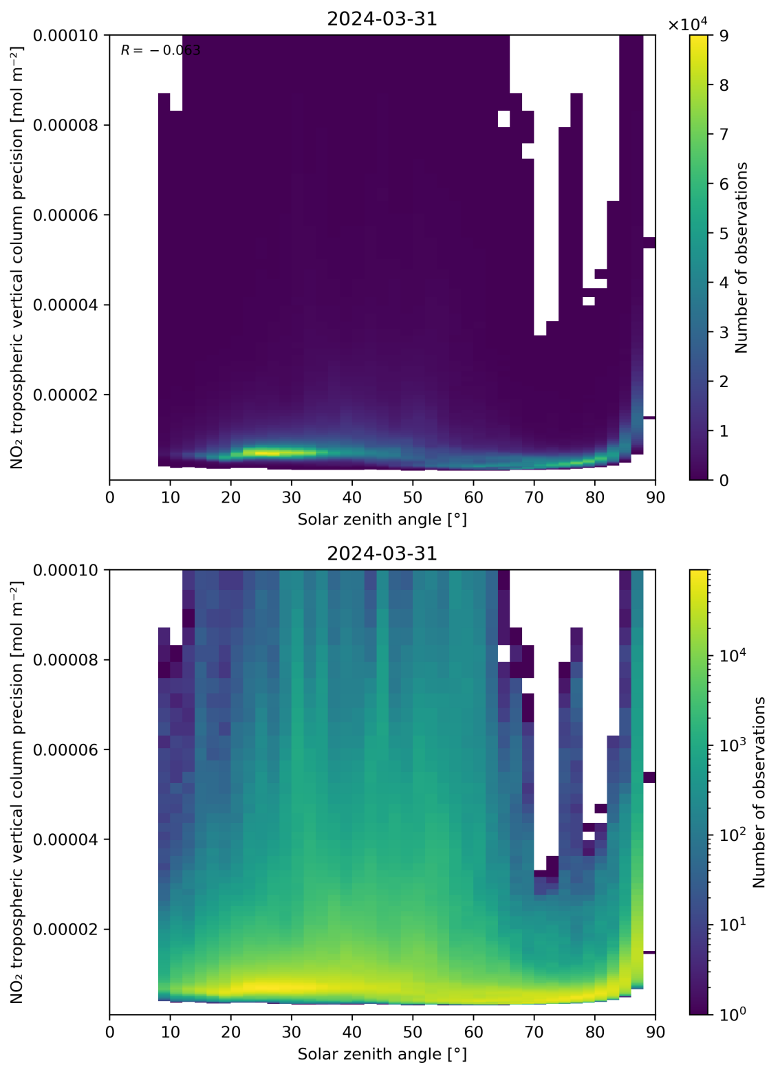
Figure 156: Scatter density plot of “Solar zenith angle” against “NO 2 tropospheric vertical column precision” for 2024-03-31 to 2024-04-01.
