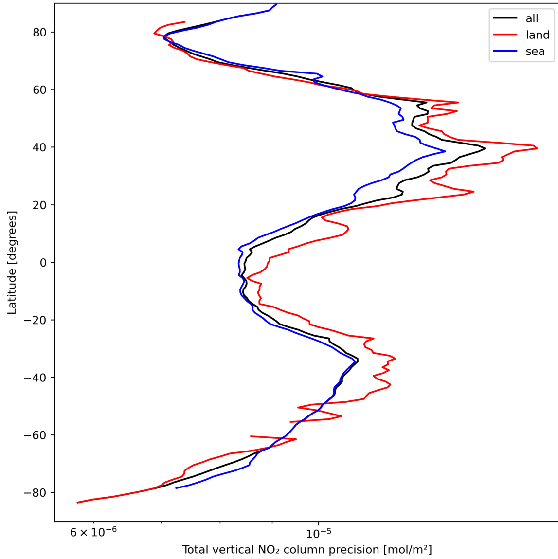
Figure 22: Zonal average of “Total vertical NO 2 column precision” for 2024-03-31 to 2024-04-01.
