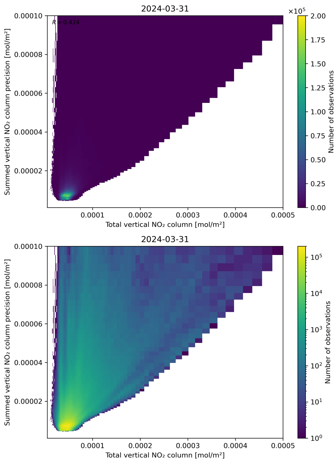
Figure 113: Scatter density plot of “Total vertical NO 2 column” against “Summed vertical NO 2 column precision” for 2024-03-31 to 2024-04-01.
