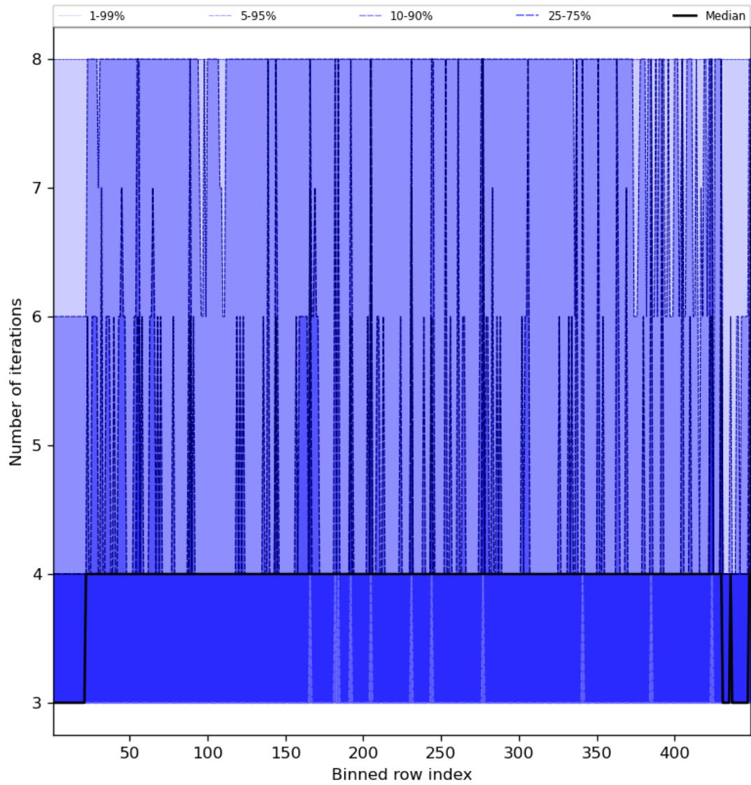
Figure 51: Along track statistics of “Number of iterations” for 2024-03-31 to 2024-04-01
