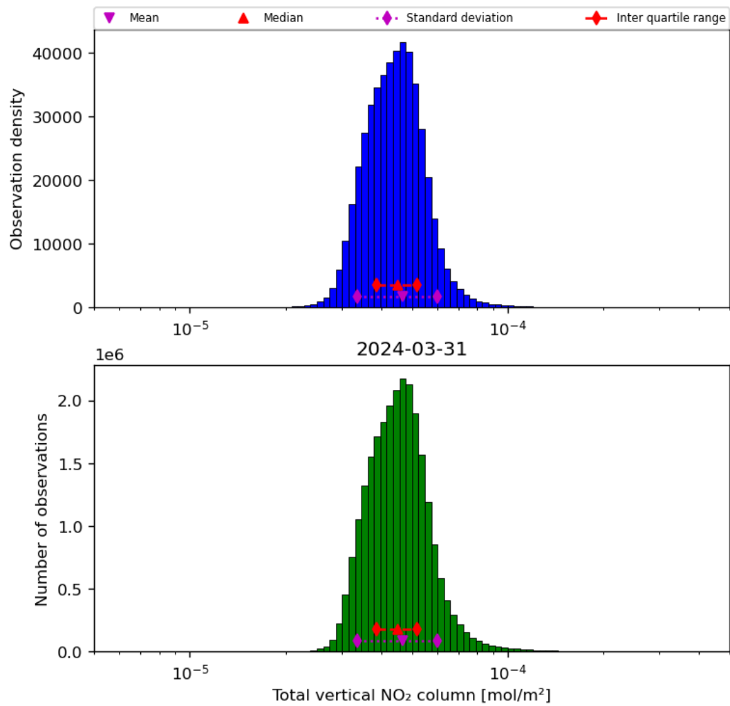
Figure 38: Histogram of “Total vertical NO 2 column” for 2024-03-31 to 2024-04-01
