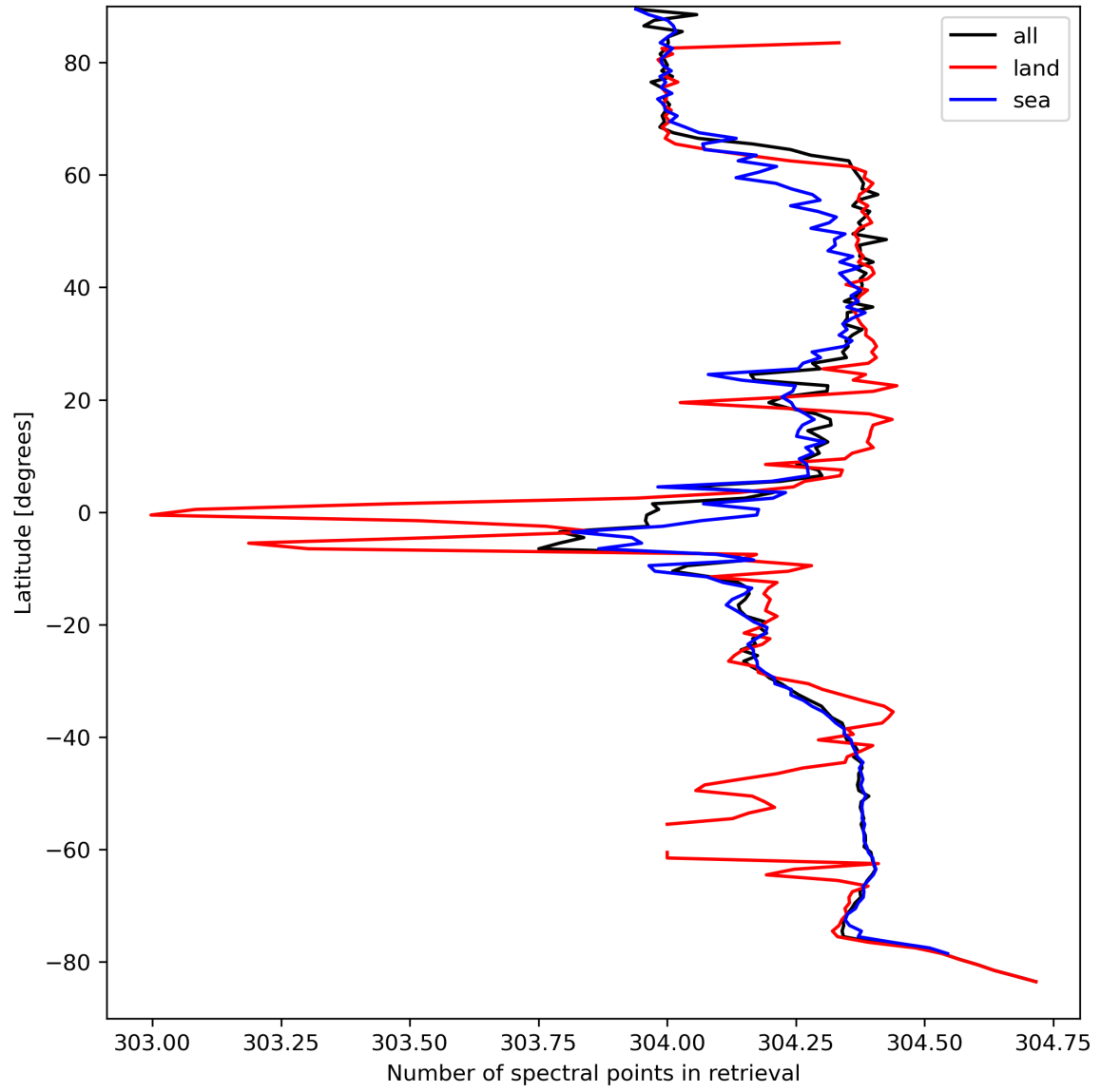
Figure 16: Zonal average of “Number of spectral points in retrieval” for 2024-03-31 to 2024-04-01.
