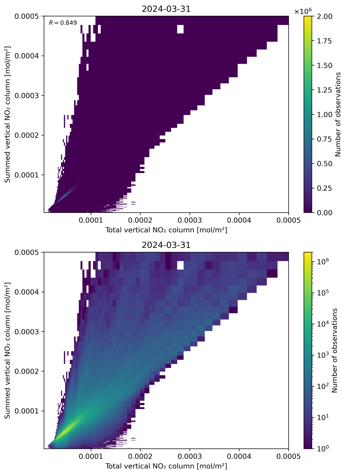
Figure 112: Scatter density plot of “Total vertical NO 2 column” against “Summed vertical NO 2 column” for 2024-03-31 to 2024-04-01.
