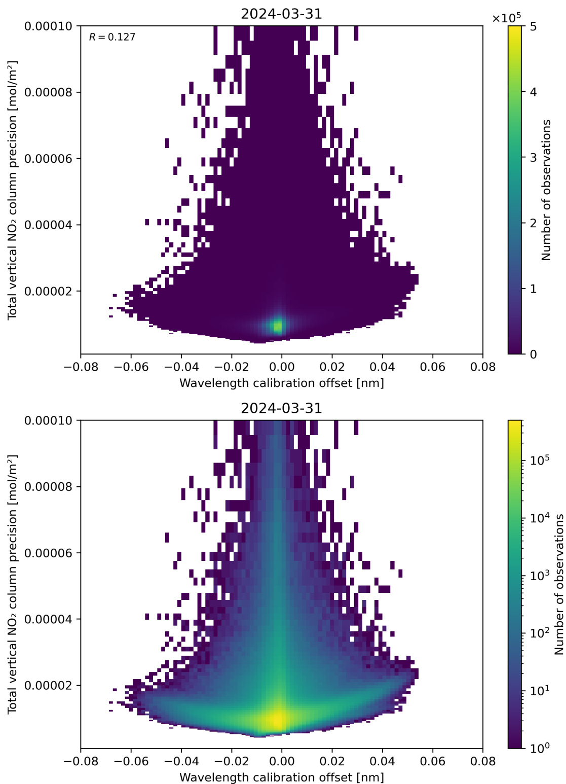
Figure 180: Scatter density plot of “Wavelength calibration offset” against “Total vertical NO 2 column precision” for 2024-03-31 to 2024-04-01.
