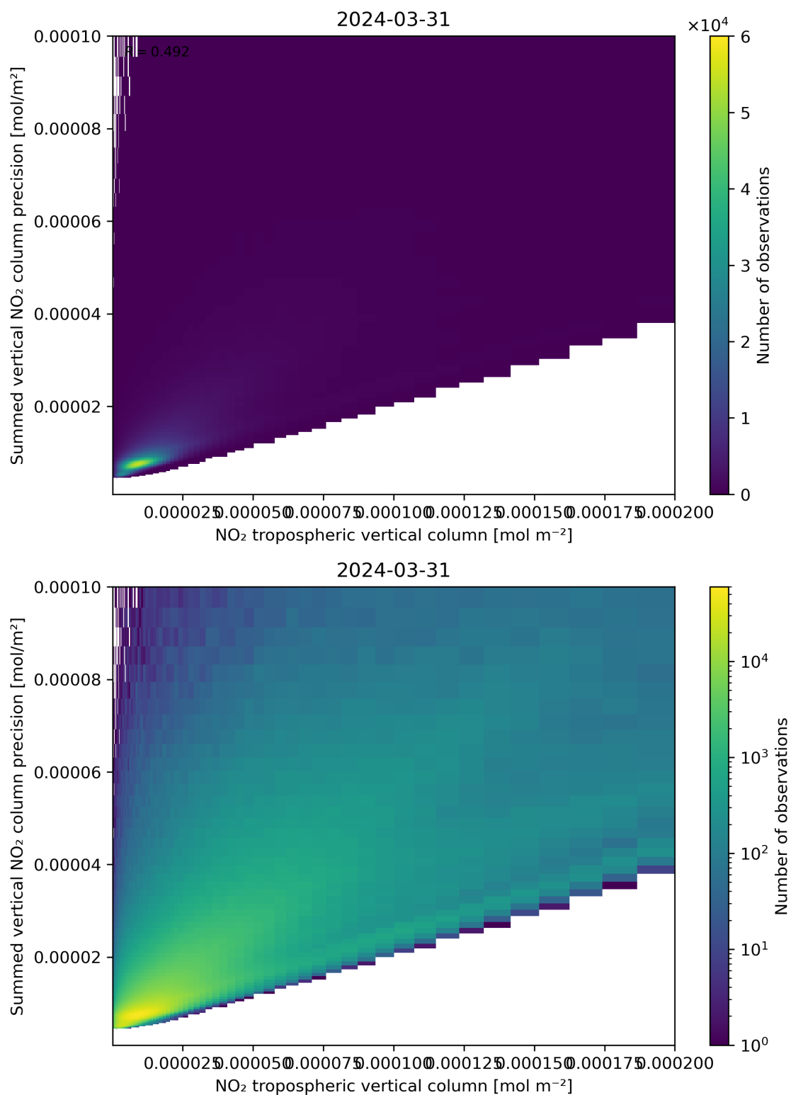
Figure 127: Scatter density plot of “NO 2 tropospheric vertical column” against “Summed vertical NO 2 column precision” for 2024-03-31 to 2024-04-01.
