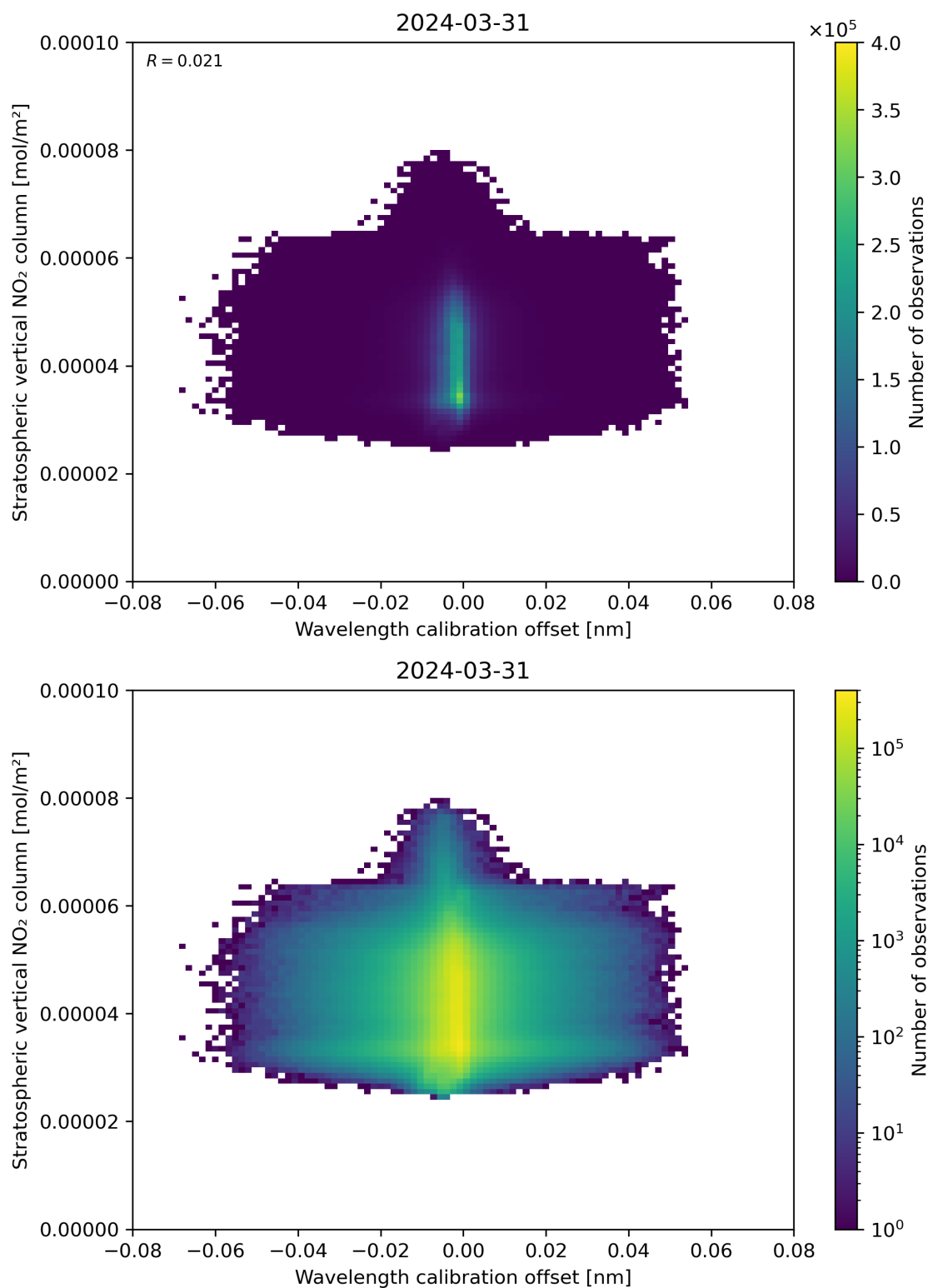
Figure 176: Scatter density plot of “Wavelength calibration offset” against “Stratospheric vertical NO 2 column” for 2024-03-31 to 2024-04-01.
