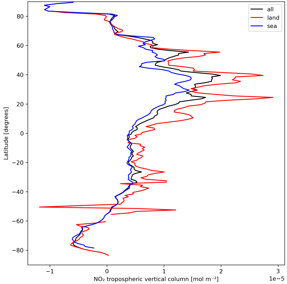
Figure 12: Zonal average of “NO 2 tropospheric vertical column” for 2024-03-31 to 2024-04-01.
