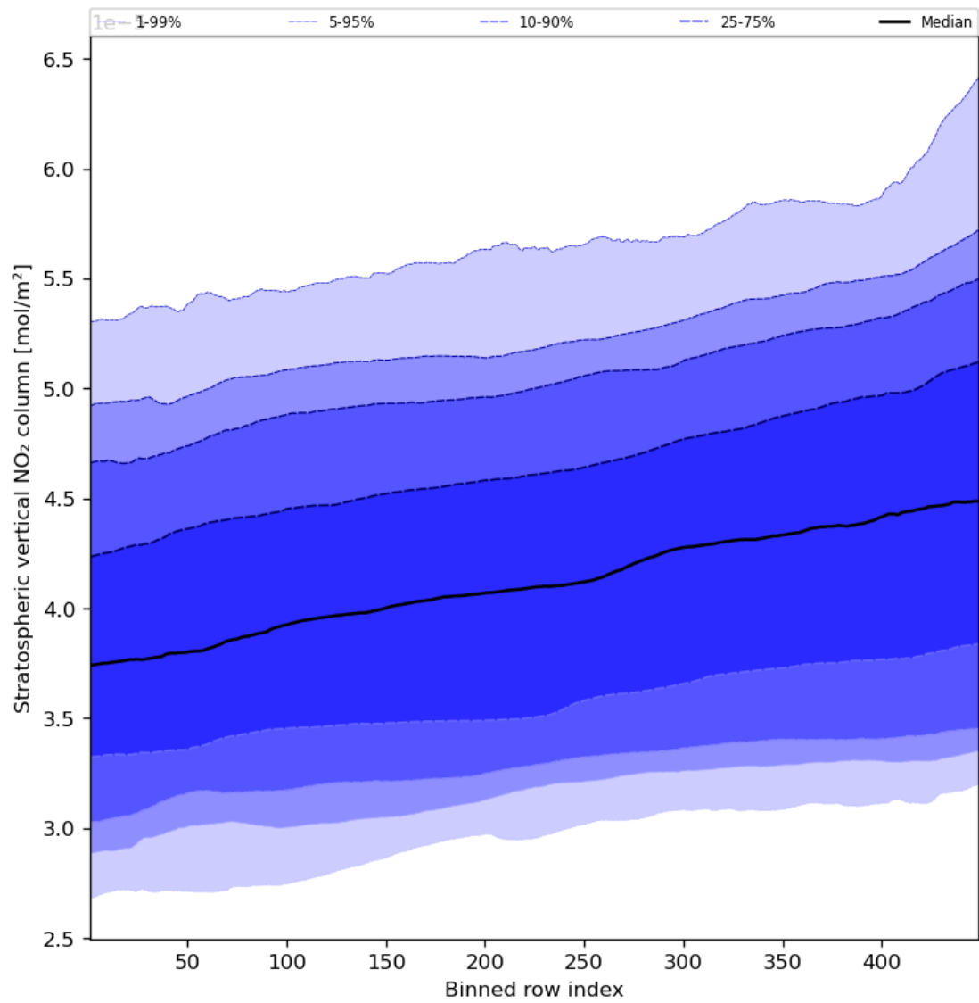
Figure 53: Along track statistics of “Stratospheric vertical NO 2 column” for 2024-03-31 to 2024-04-01
