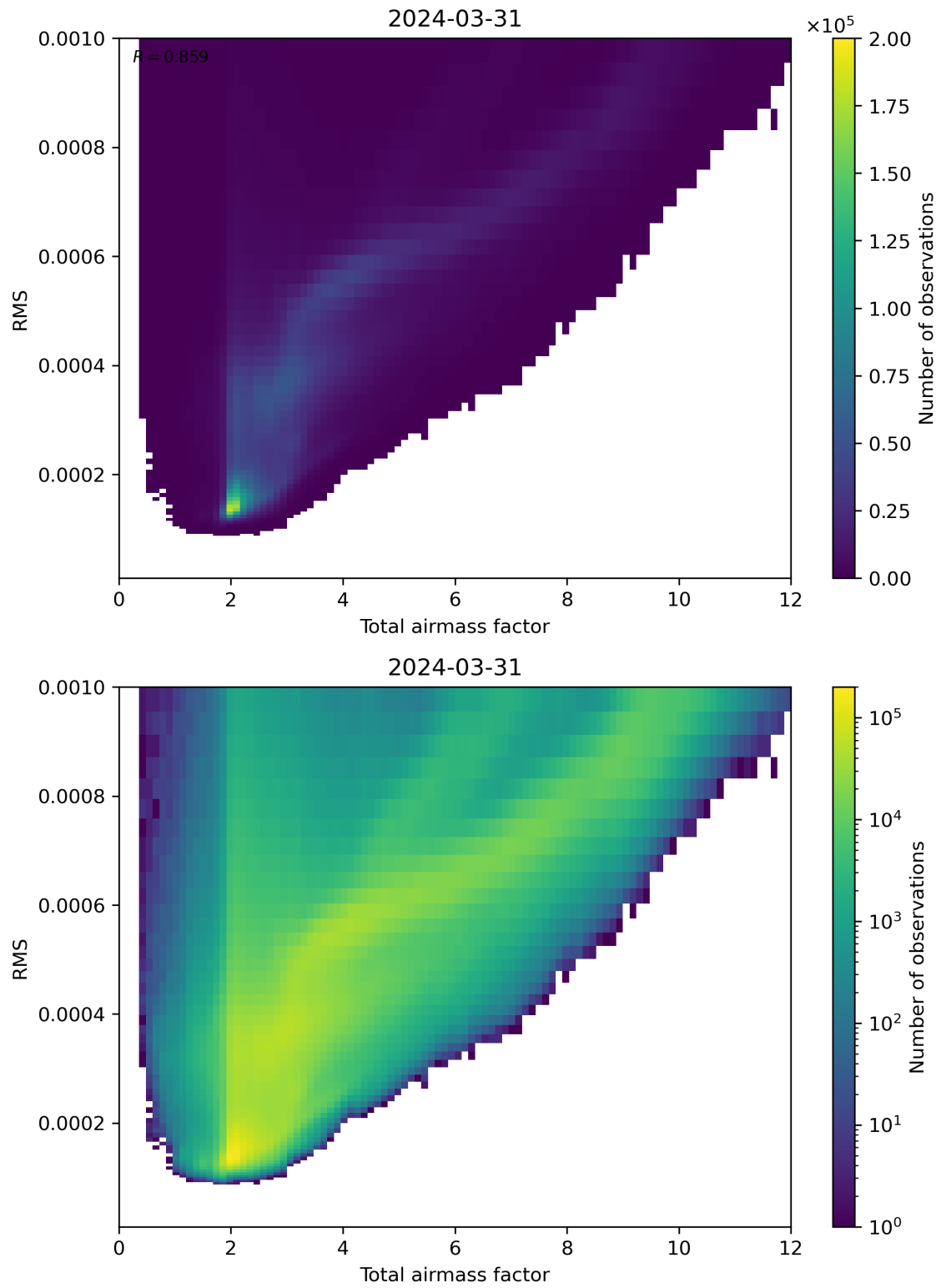
Figure 69: Scatter density plot of “Total airmass factor” against “RMS” for 2024-03-31 to 2024-04-01.
