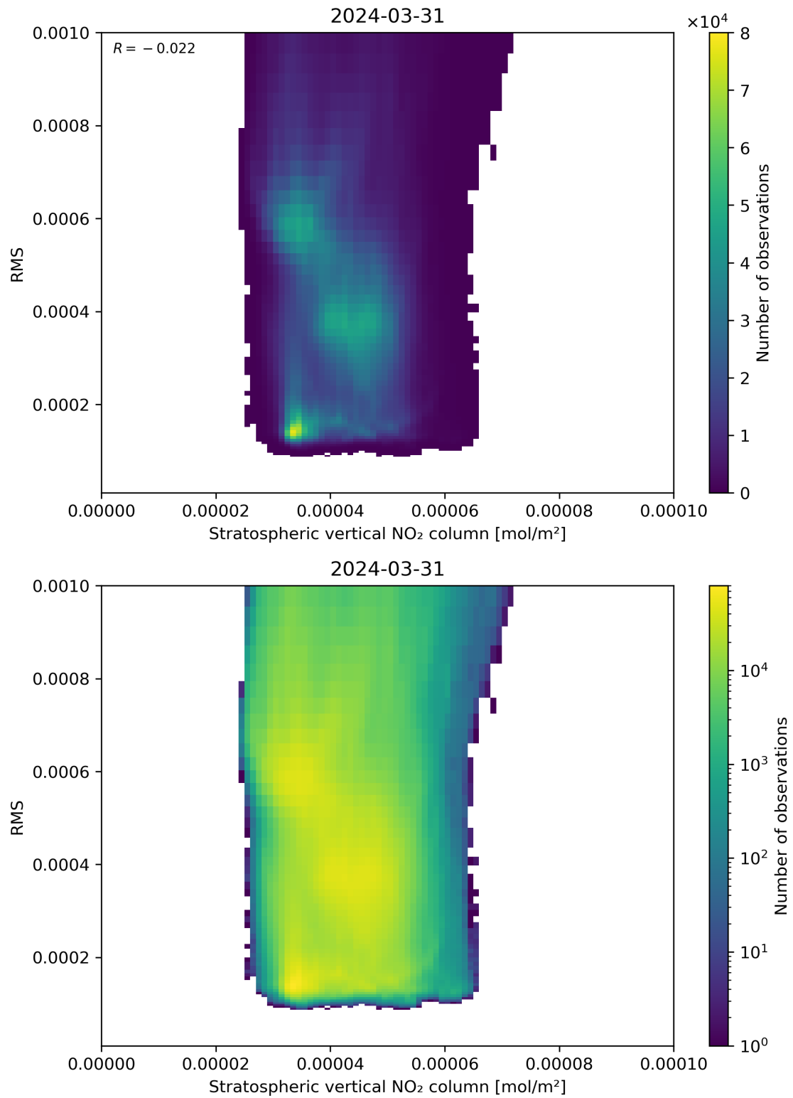
Figure 102: Scatter density plot of “Stratospheric vertical NO 2 column” against “RMS” for 2024-03-31 to 2024-04-01.
