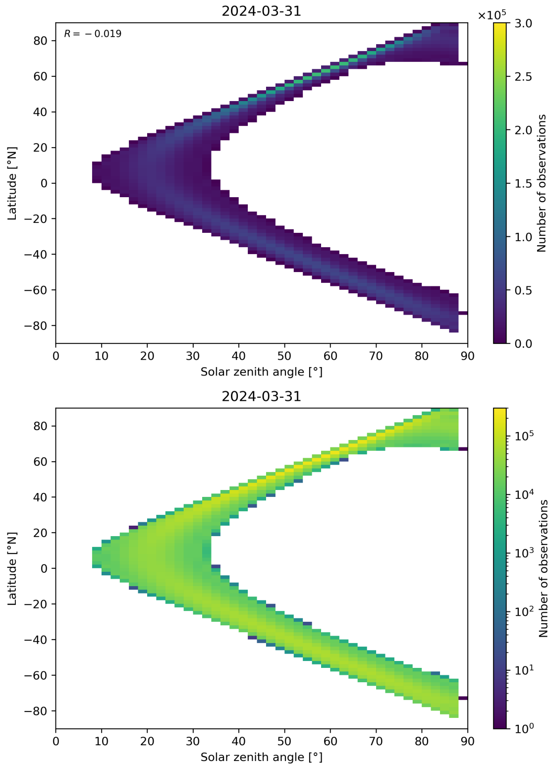
Figure 149: Scatter density plot of “Solar zenith angle” against “Latitude” for 2024-03-31 to 2024-04-01.
