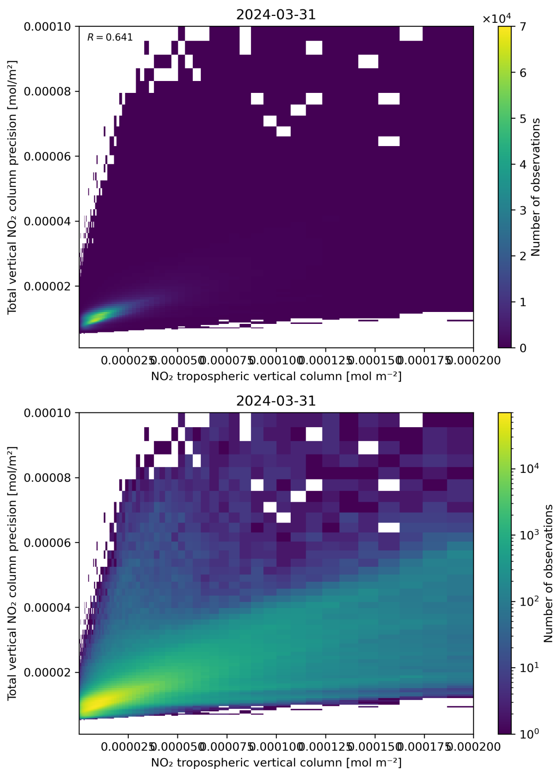
Figure 129: Scatter density plot of “NO 2 tropospheric vertical column” against “Total vertical NO 2 column precision” for 2024-03-31 to 2024-04-01.
