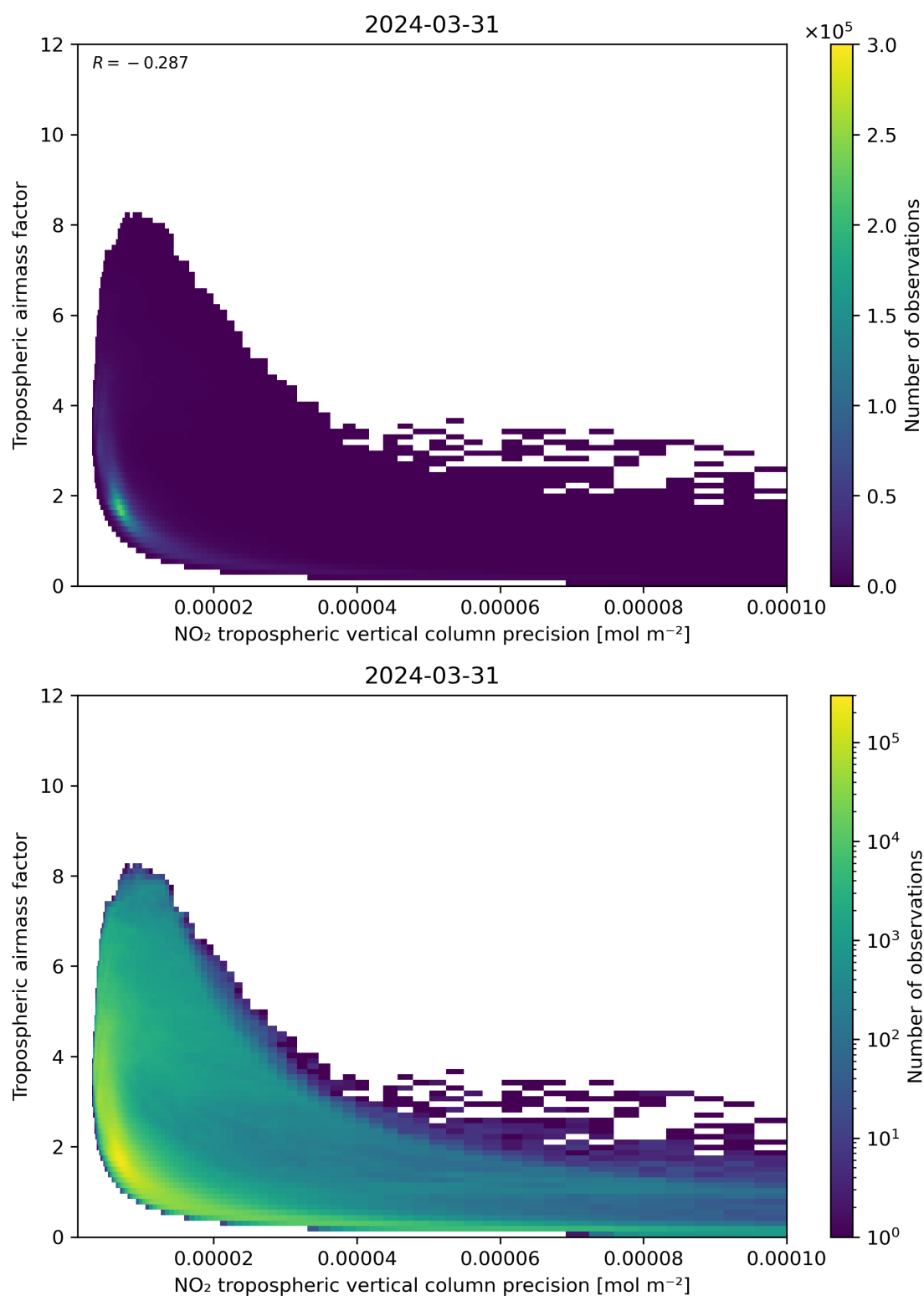
Figure 133: Scatter density plot of “NO 2 tropospheric vertical column precision” against “Tropospheric airmass factor” for 2024-03-31 to 2024-04-01.
