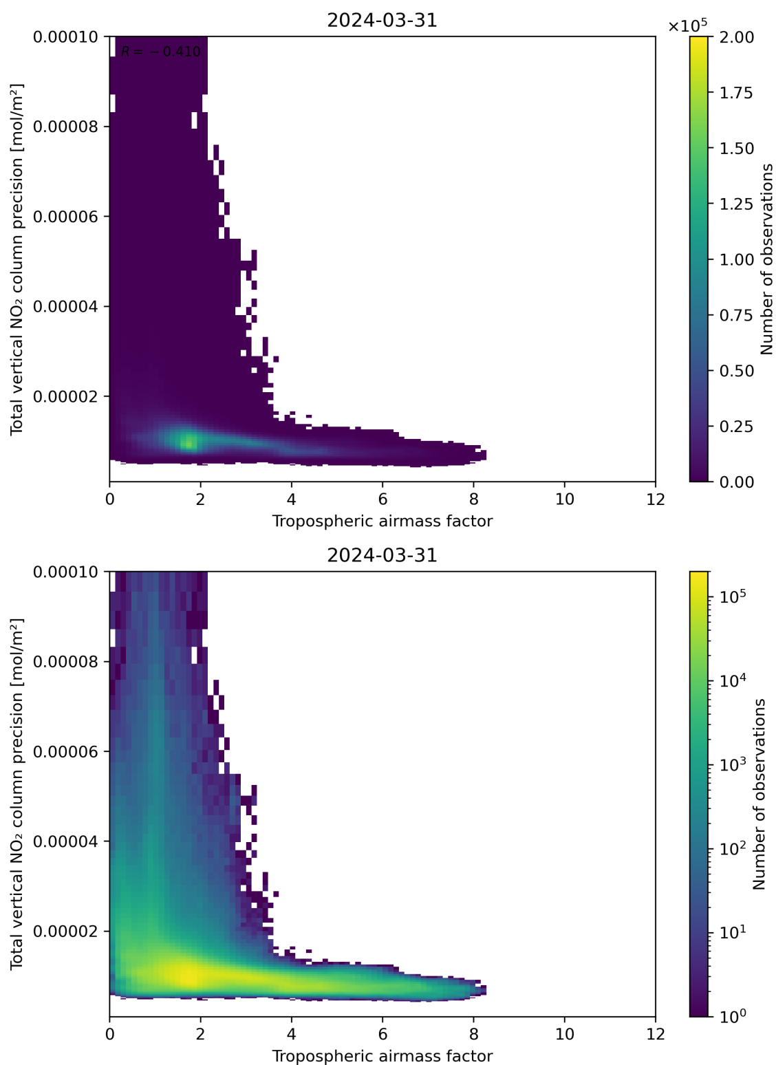
Figure 78: Scatter density plot of “Tropospheric air mass factor” against “Total vertical NO 2 column precision” for 2024-03-31 to 2024-04-01.
