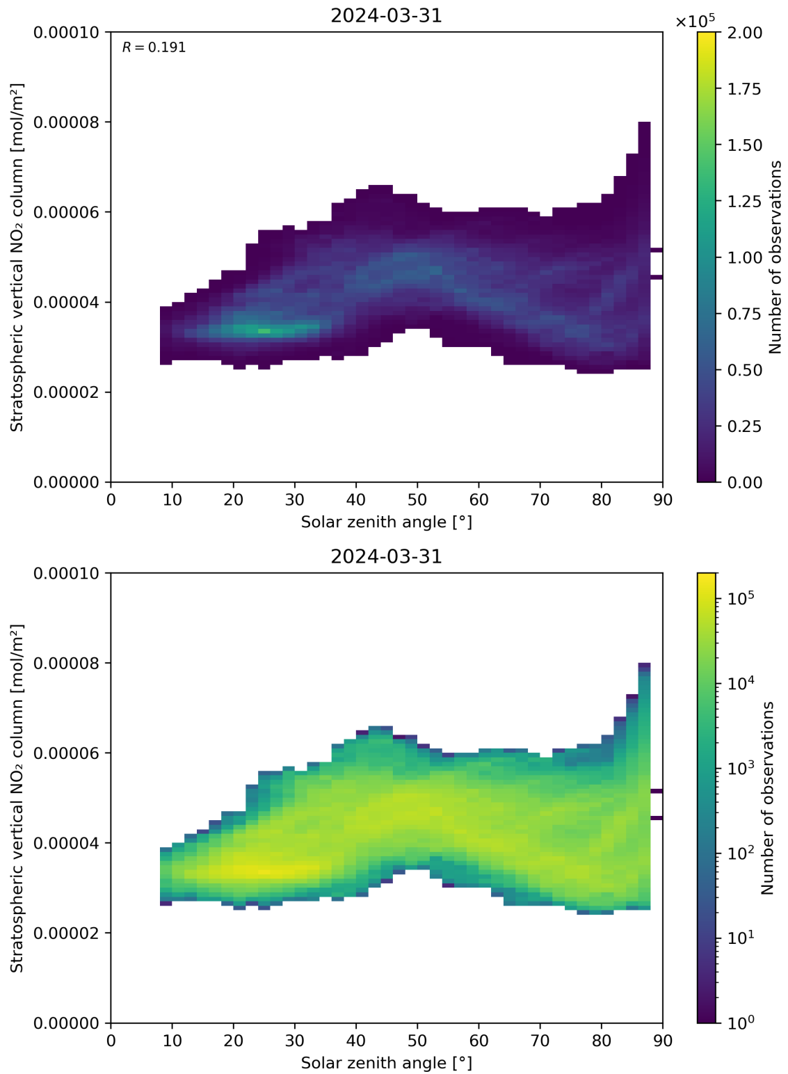
Figure 150: Scatter density plot of “Solar zenith angle” against “Stratospheric vertical NO 2 column” for 2024-03-31 to 2024-04-01.
