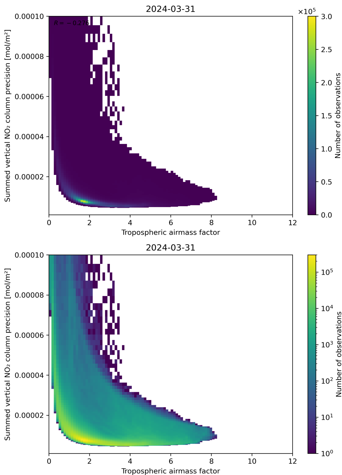
Figure 76: Scatter density plot of “Tropospheric air mass factor” against “Summed vertical NO 2 column precision” for 2024-03-31 to 2024-04-01.
