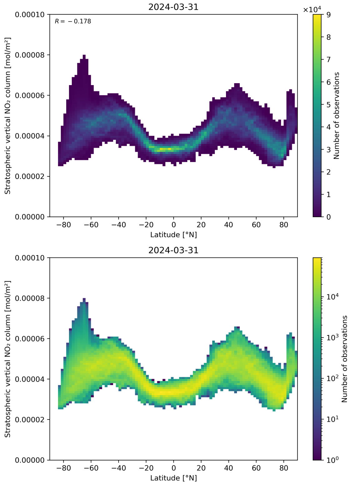
Figure 87: Scatter density plot of “Latitude” against “Stratospheric vertical NO 2 column” for 2024-03-31 to 2024-04-01.
