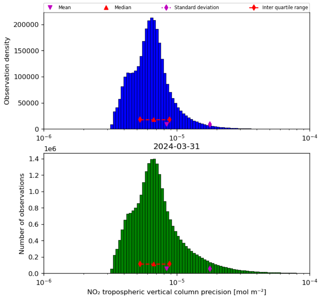
Figure 30: Histogram of “NO 2 tropospheric vertical column precision” for 2024-03-31 to 2024-04-01
