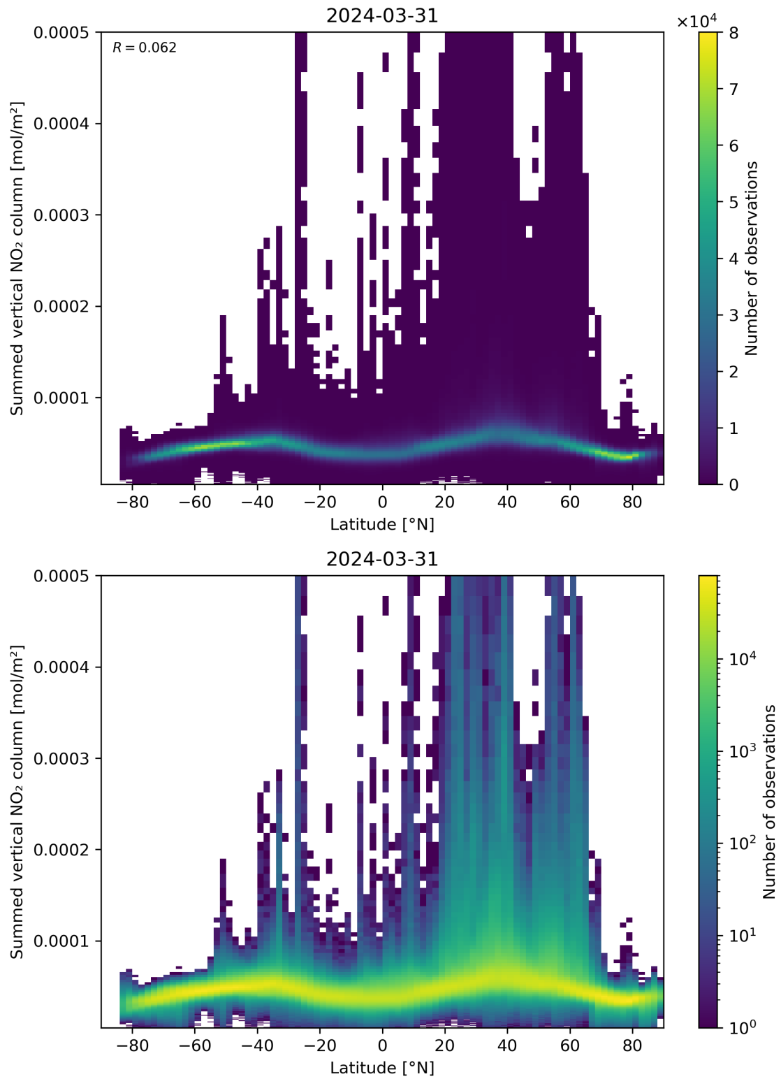
Figure 88: Scatter density plot of “Latitude” against “Summed vertical NO 2 column” for 2024-03-31 to 2024-04-01.
