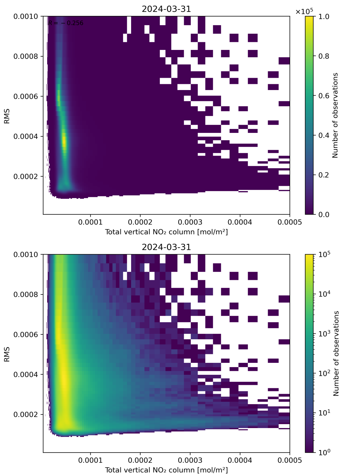
Figure 120: Scatter density plot of “Total vertical NO 2 column” against “RMS” for 2024-03-31 to 2024-04-01.
