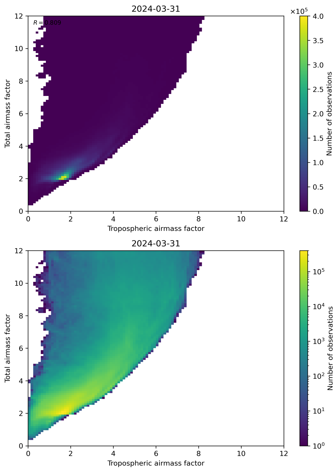
Figure 72: Scatter density plot of “Tropospheric airmass factor” against “Total airmass factor” for 2024-03-31 to 2024-04-01.
