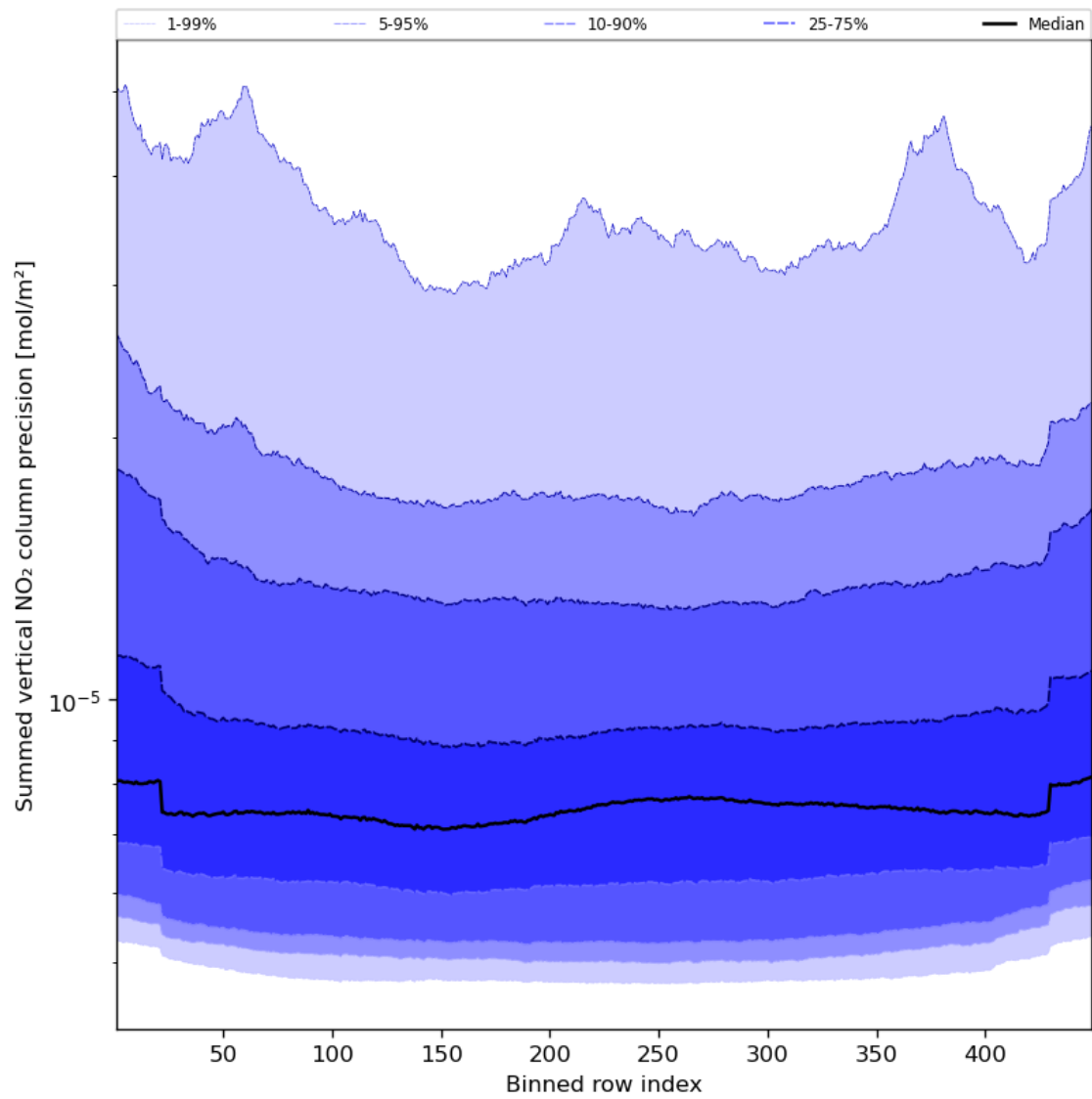
Figure 58: Along track statistics of “Summed vertical NO 2 column precision” for 2024-03-31 to 2024-04-01
