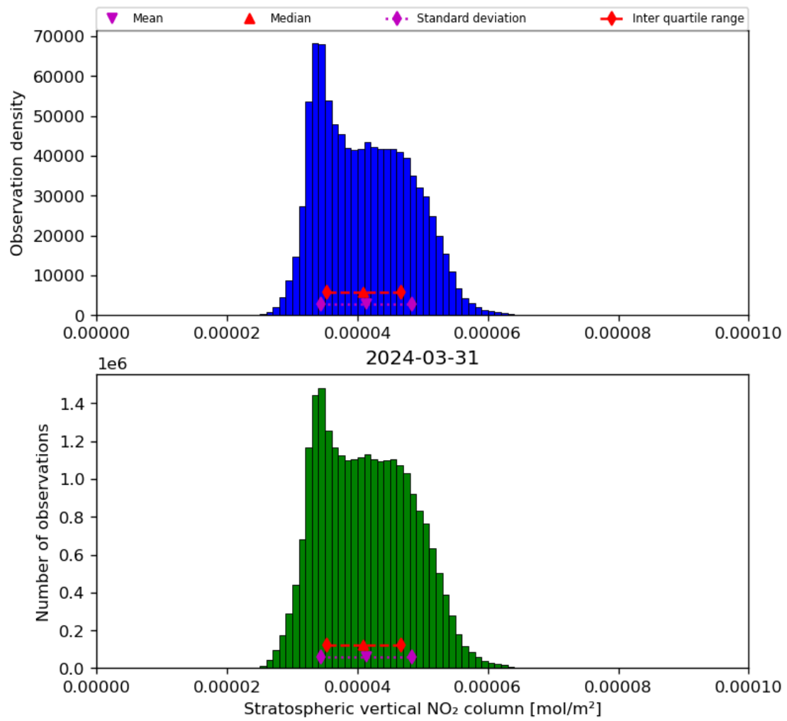
Figure 36: Histogram of “Stratospheric vertical NO 2 column” for 2024-03-31 to 2024-04-01
