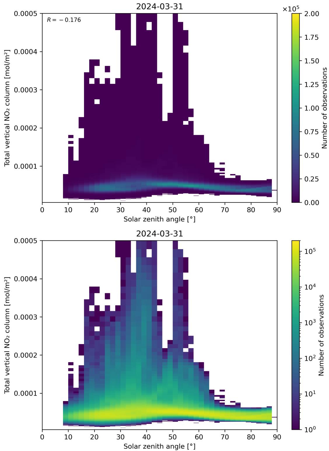
Figure 153: Scatter density plot of “Solar zenith angle” against “Total vertical NO 2 column” for 2024-03-31 to 2024-04-01.
