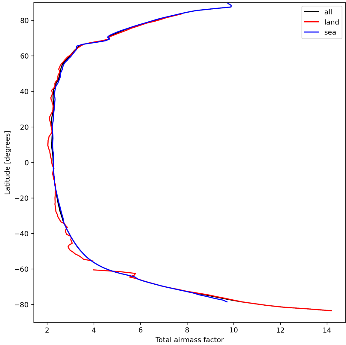
Figure 15: Zonal average of “Total airmass factor” for 2024-03-31 to 2024-04-01.
