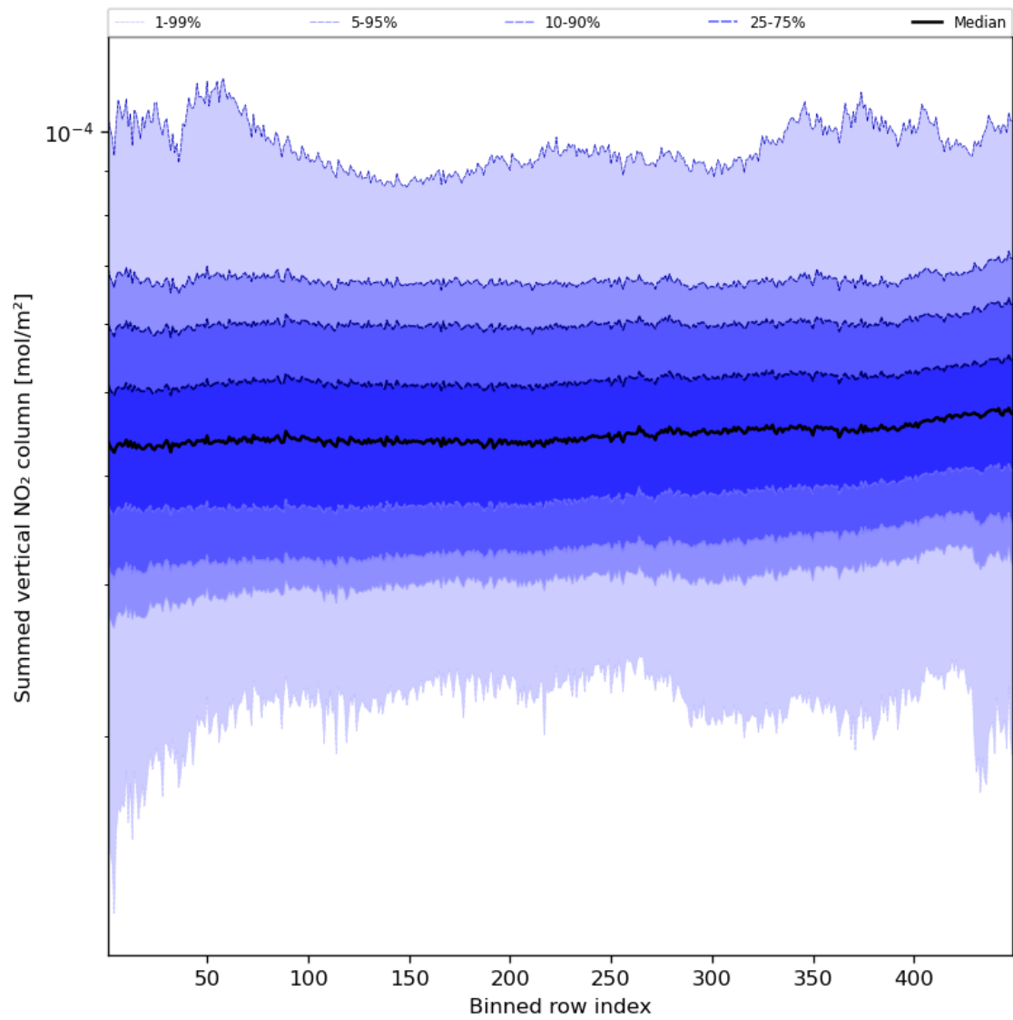
Figure 57: Along track statistics of “Summed vertical NO 2 column” for 2024-03-31 to 2024-04-01
