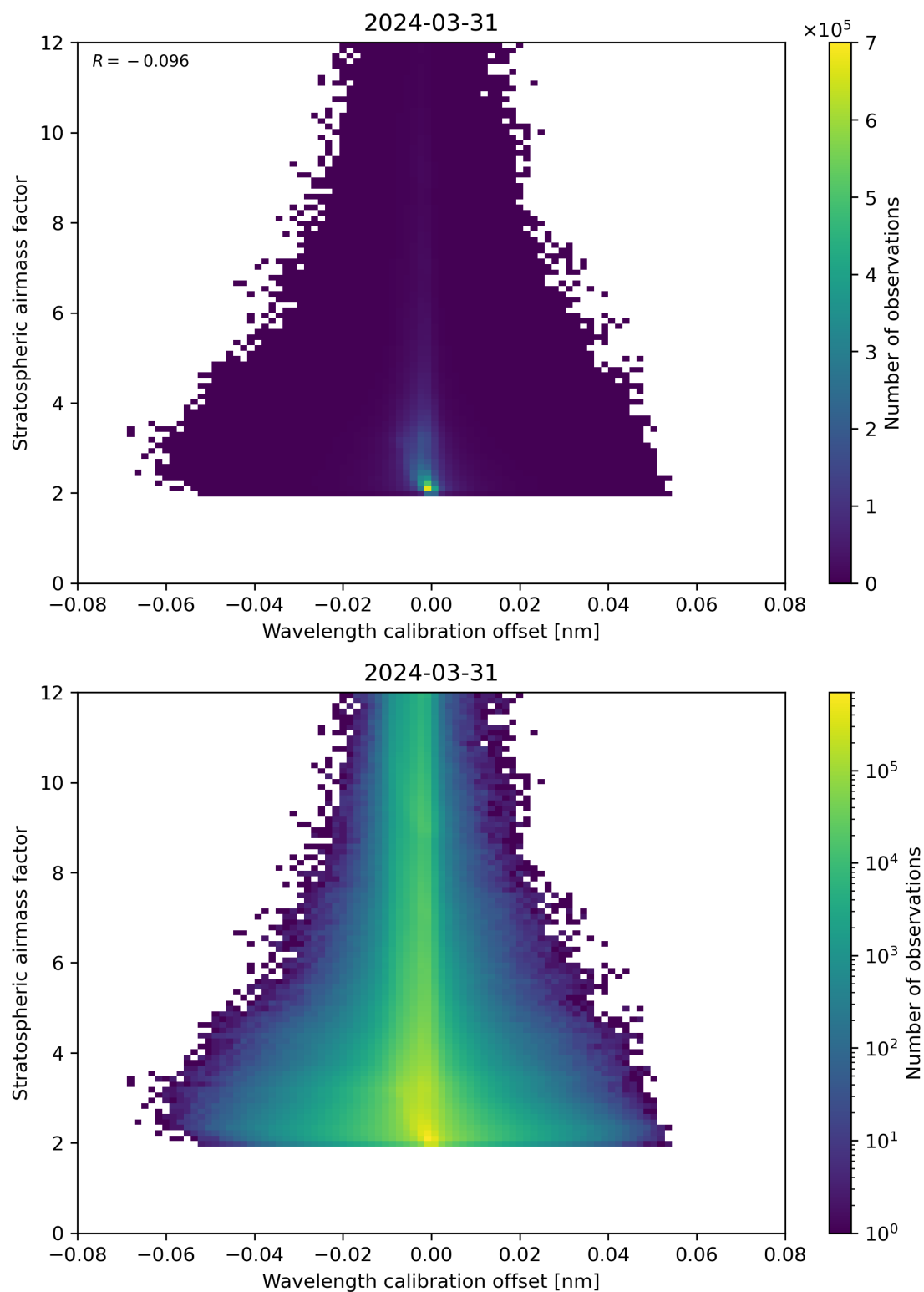
Figure 174: Scatter density plot of “Wavelength calibration offset” against “Stratospheric air mass factor” for 2024-03-31 to 2024-04-01.
