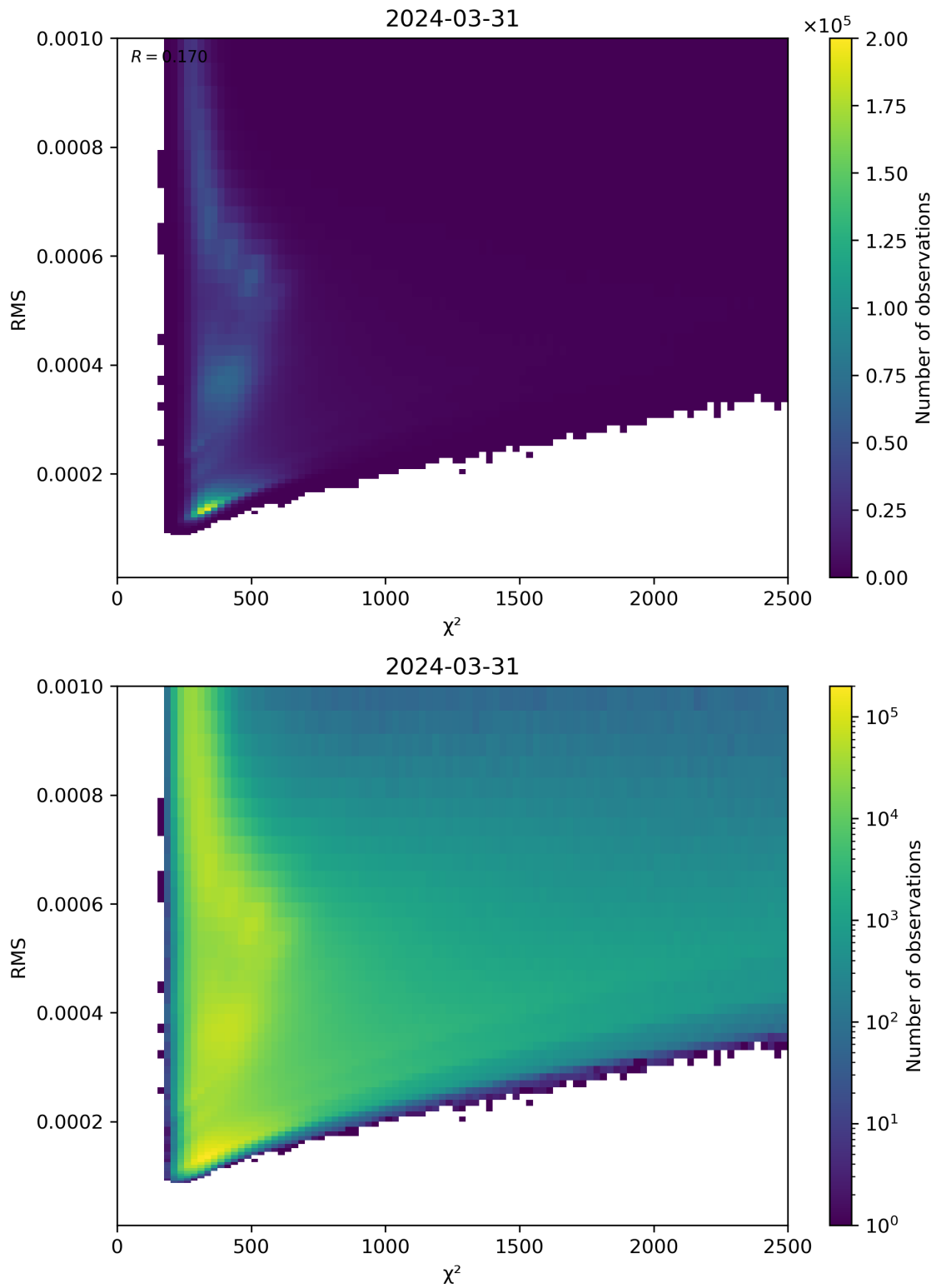
Figure 82: Scatter density plot of “ \chi^2 ” against “RMS” for 2024-03-31 to 2024-04-01.
