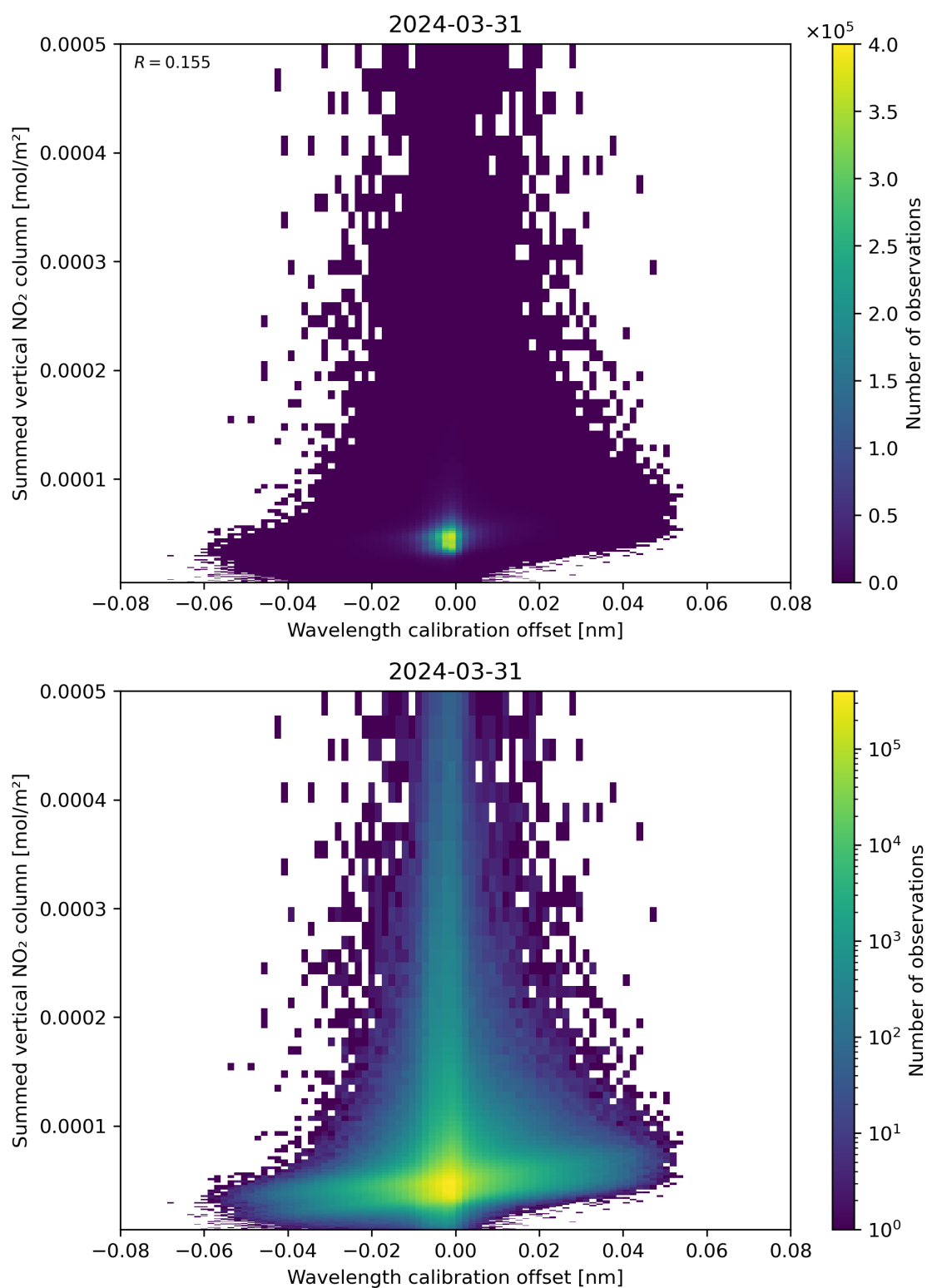
Figure 177: Scatter density plot of “Wavelength calibration offset” against “Summed vertical NO 2 column” for 2024-03-31 to 2024-04-01.
