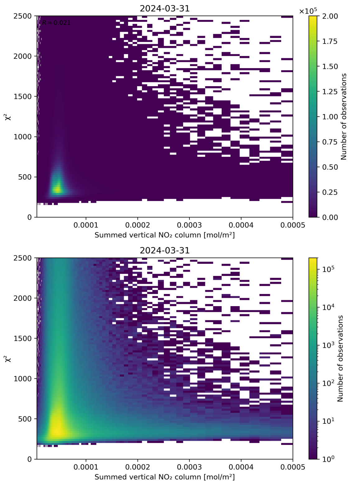
Figure 104: Scatter density plot of “Summed vertical NO 2 column” against “ \chi^2 ” for 2024-03-31 to 2024-04-01.
