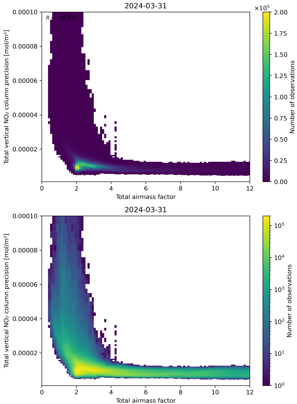
Figure 68: Scatter density plot of “Total airmass factor” against “Total vertical NO 2 column precision” for 2024-03-31 to 2024-04-01.
