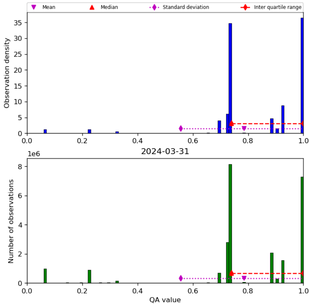
Figure 28: Histogram of “QA value” for 2024-03-31 to 2024-04-01
