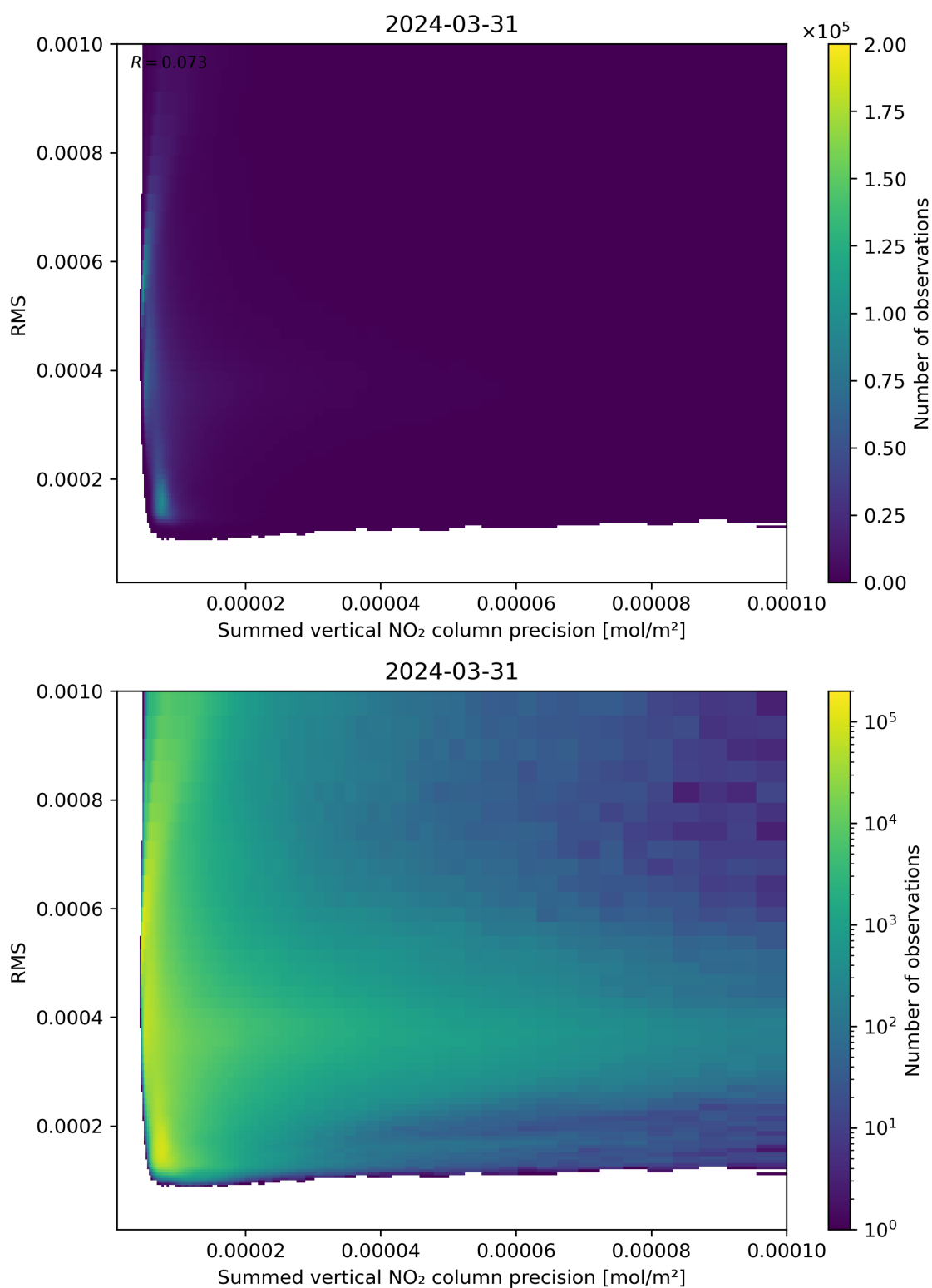
Figure 108: Scatter density plot of “Summed vertical NO 2 column precision” against “RMS” for 2024-03-31 to 2024-04-01.
