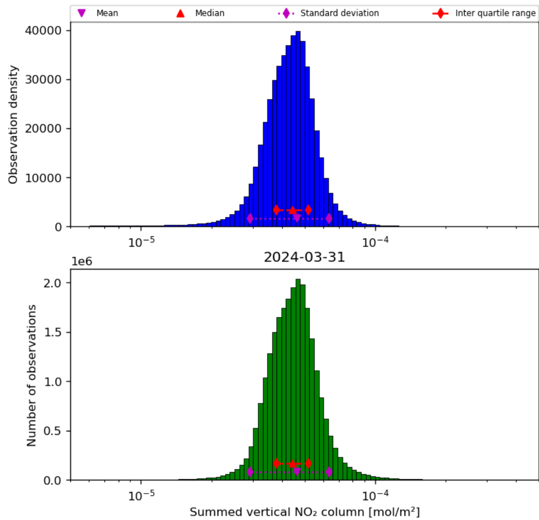
Figure 40: Histogram of “Summed vertical NO 2 column” for 2024-03-31 to 2024-04-01
