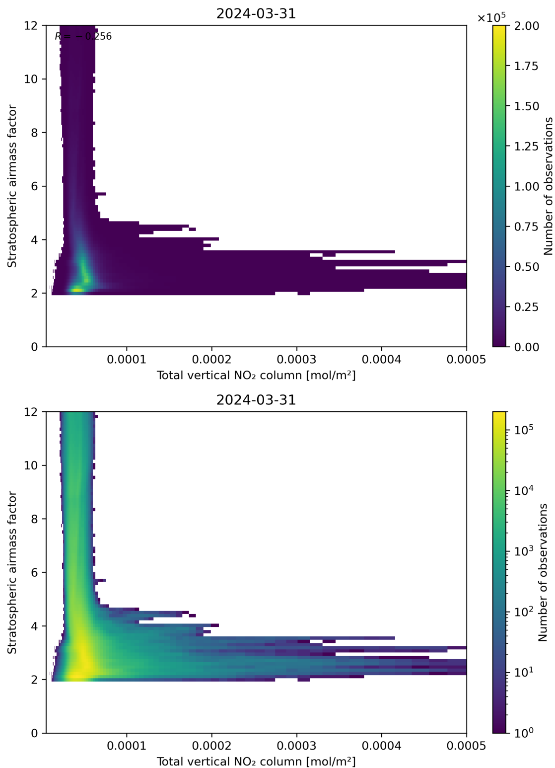
Figure 110: Scatter density plot of “Total vertical NO 2 column” against “Stratospheric airmass factor” for 2024-03-31 to 2024-04-01.
