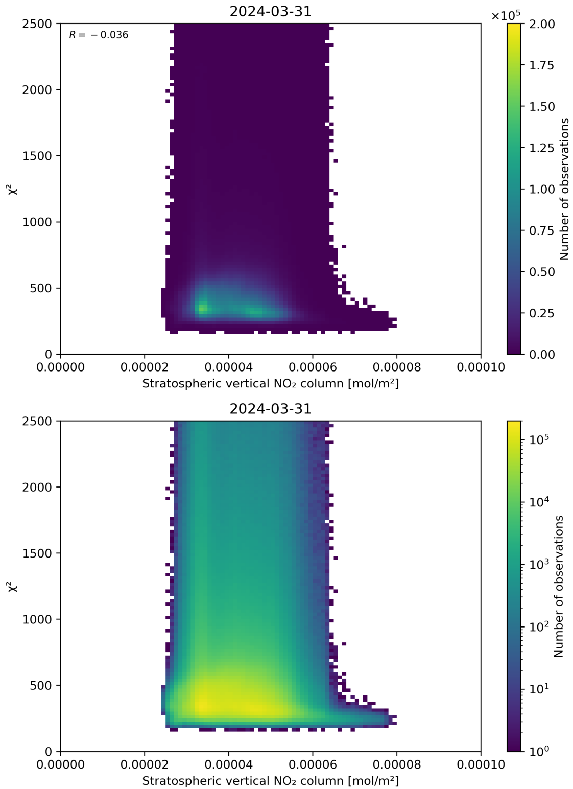
Figure 97: Scatter density plot of “Stratospheric vertical NO 2 column” against “ \chi^2 ” for 2024-03-31 to 2024-04-01.
