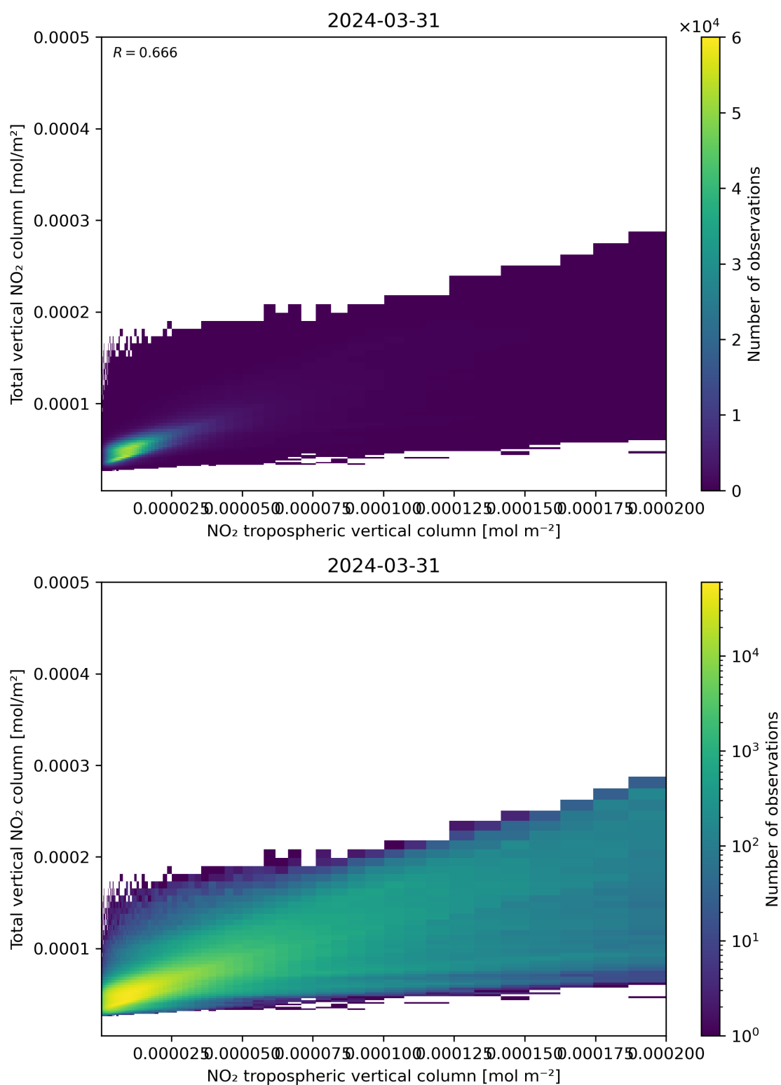
Figure 128: Scatter density plot of “NO 2 tropospheric vertical column” against “Total vertical NO 2 column” for 2024-03-31 to 2024-04-01.
