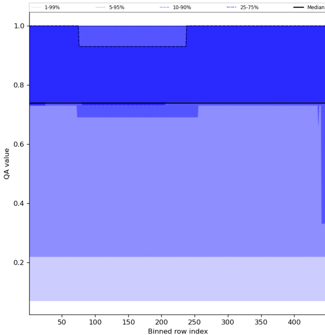
Figure 45: Along track statistics of “QA value” for 2024-03-31 to 2024-04-01
