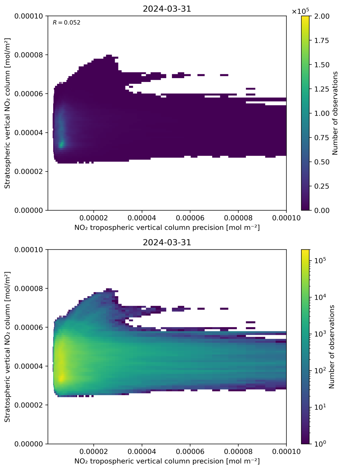
Figure 135: Scatter density plot of “NO 2 tropospheric vertical column precision” against “Stratospheric vertical NO 2 column” for 2024-03-31 to 2024-04-01.
