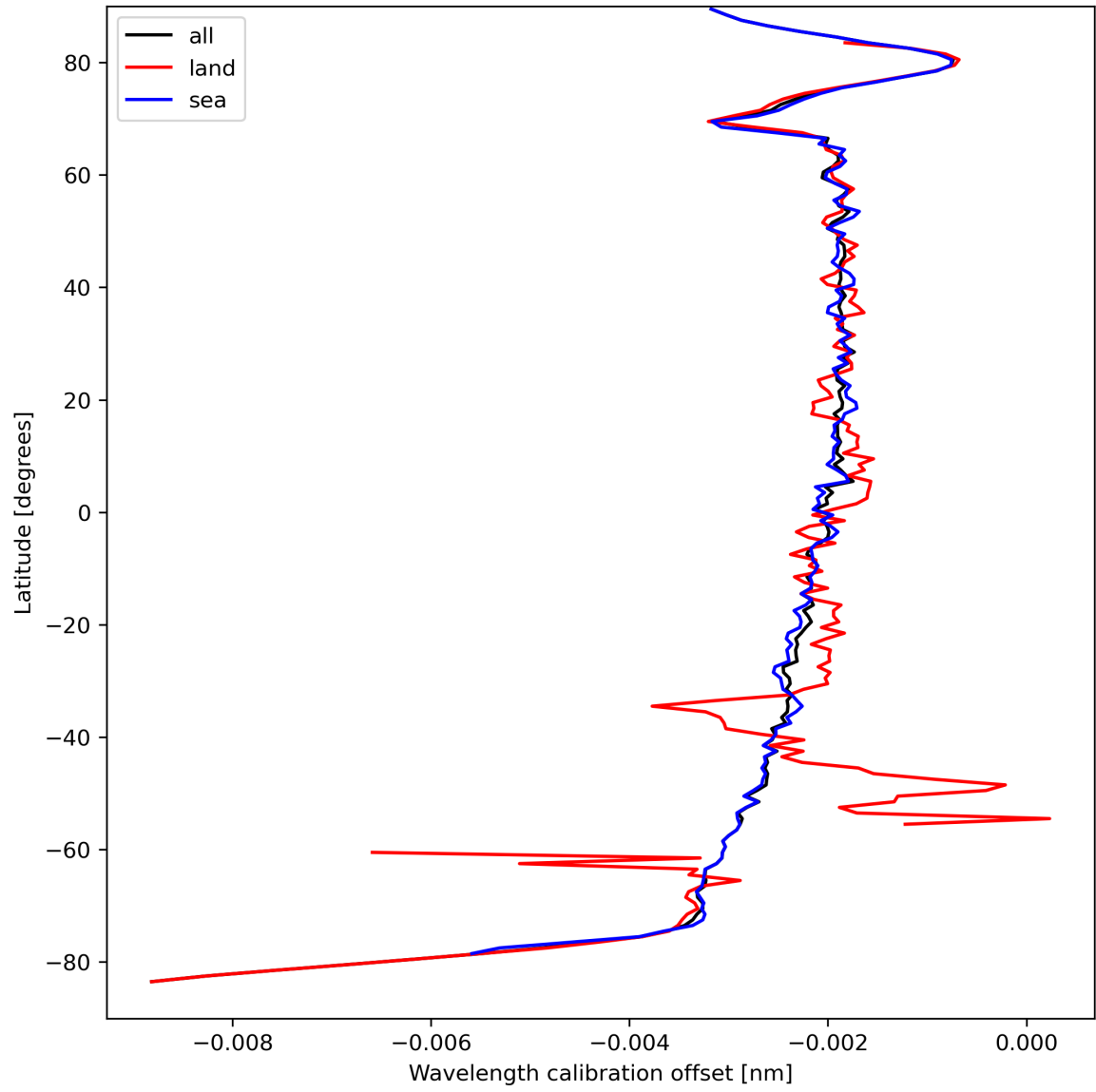
Figure 18: Zonal average of “Wavelength calibration offset” for 2024-03-31 to 2024-04-01.
