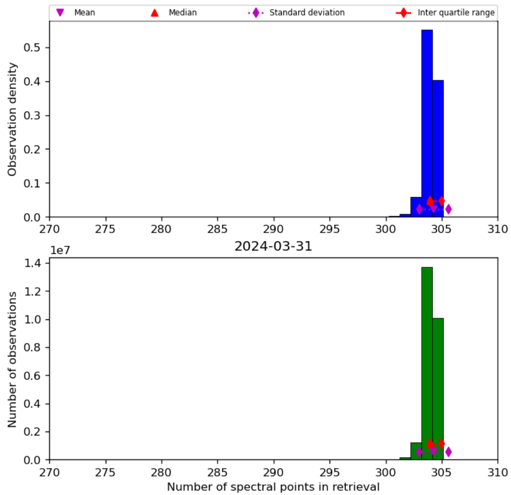
Figure 33: Histogram of “Number of spectral points in retrieval” for 2024-03-31 to 2024-04-01
