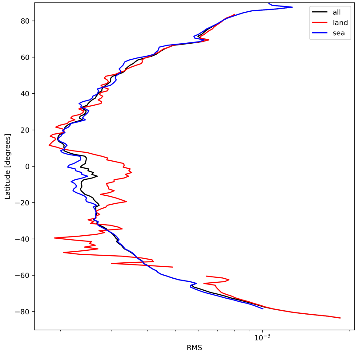
Figure 26: Zonal average of “RMS” for 2024-03-31 to 2024-04-01.
