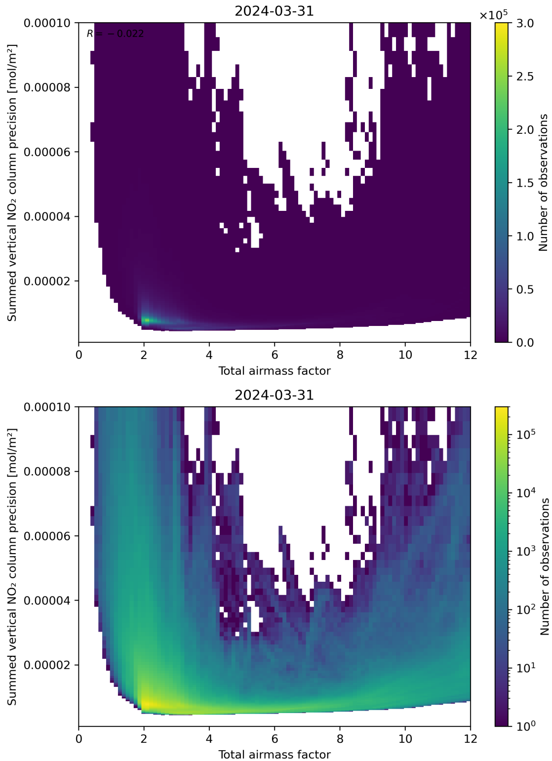
Figure 66: Scatter density plot of “Total airmass factor” against “Summed vertical NO 2 column precision” for 2024-03-31 to 2024-04-01.
