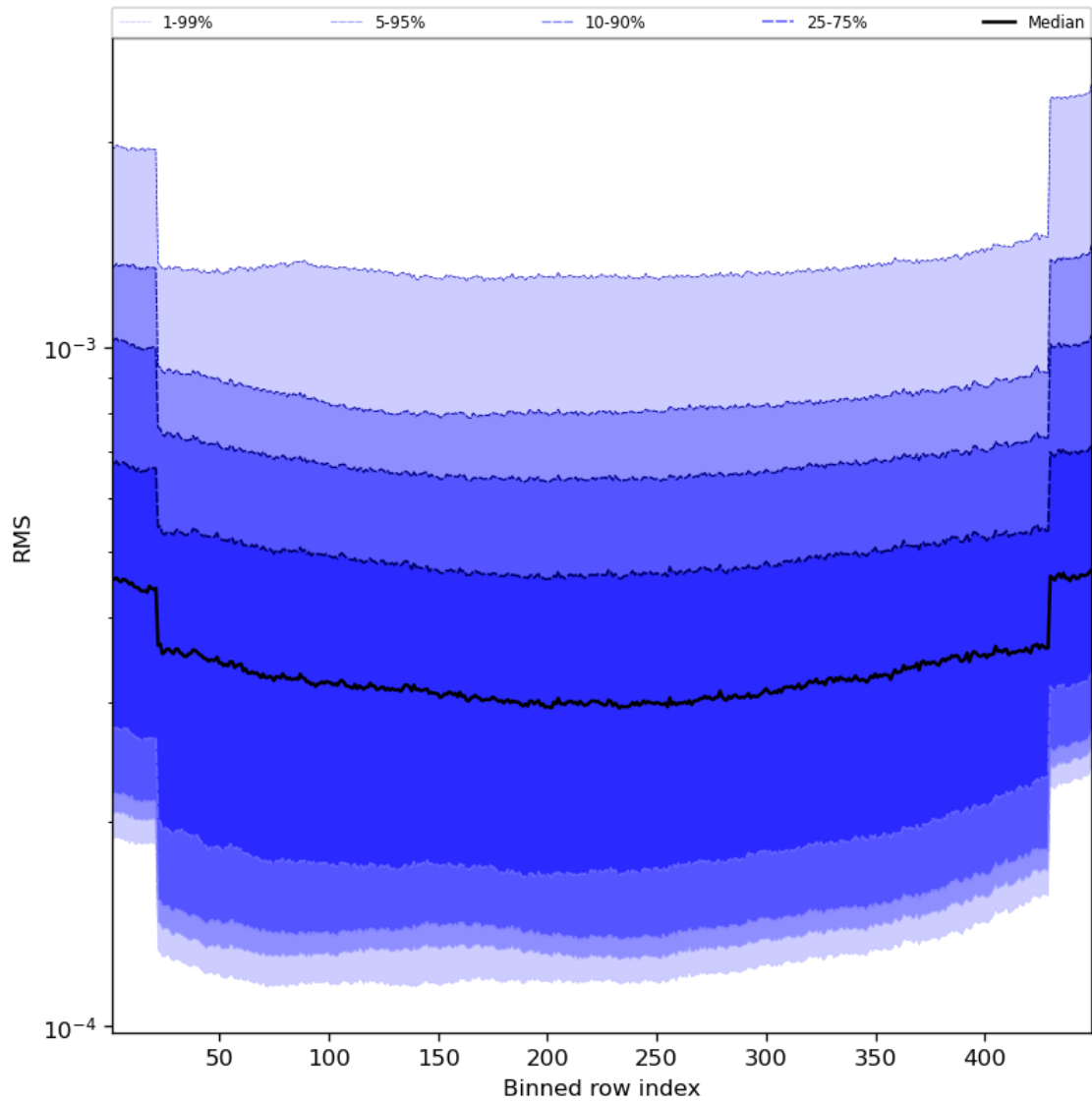
Figure 60: Along track statistics of “RMS” for 2024-03-31 to 2024-04-01
