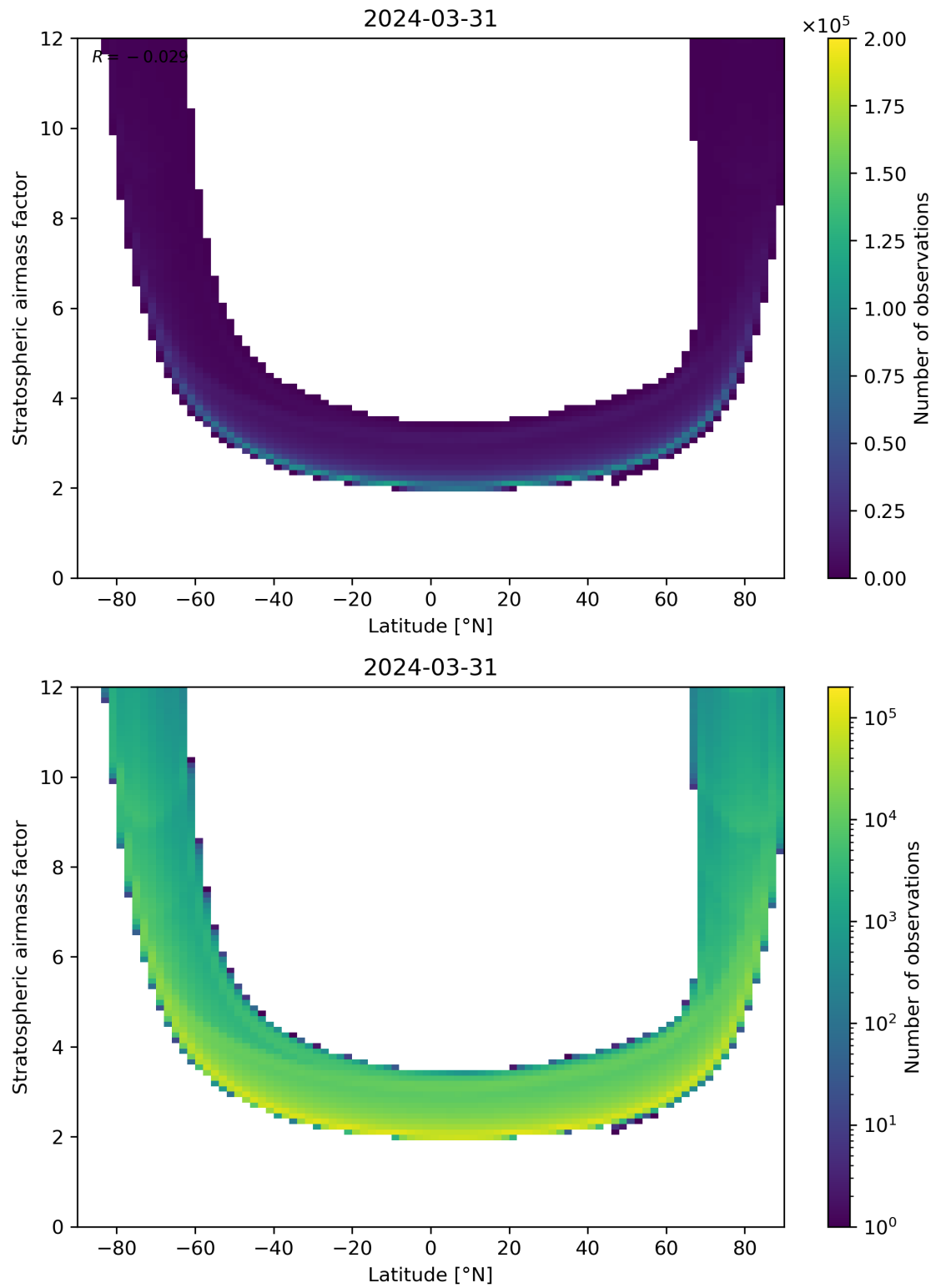
Figure 83: Scatter density plot of “Latitude” against “Stratospheric air mass factor” for 2024-03-31 to 2024-04-01.
