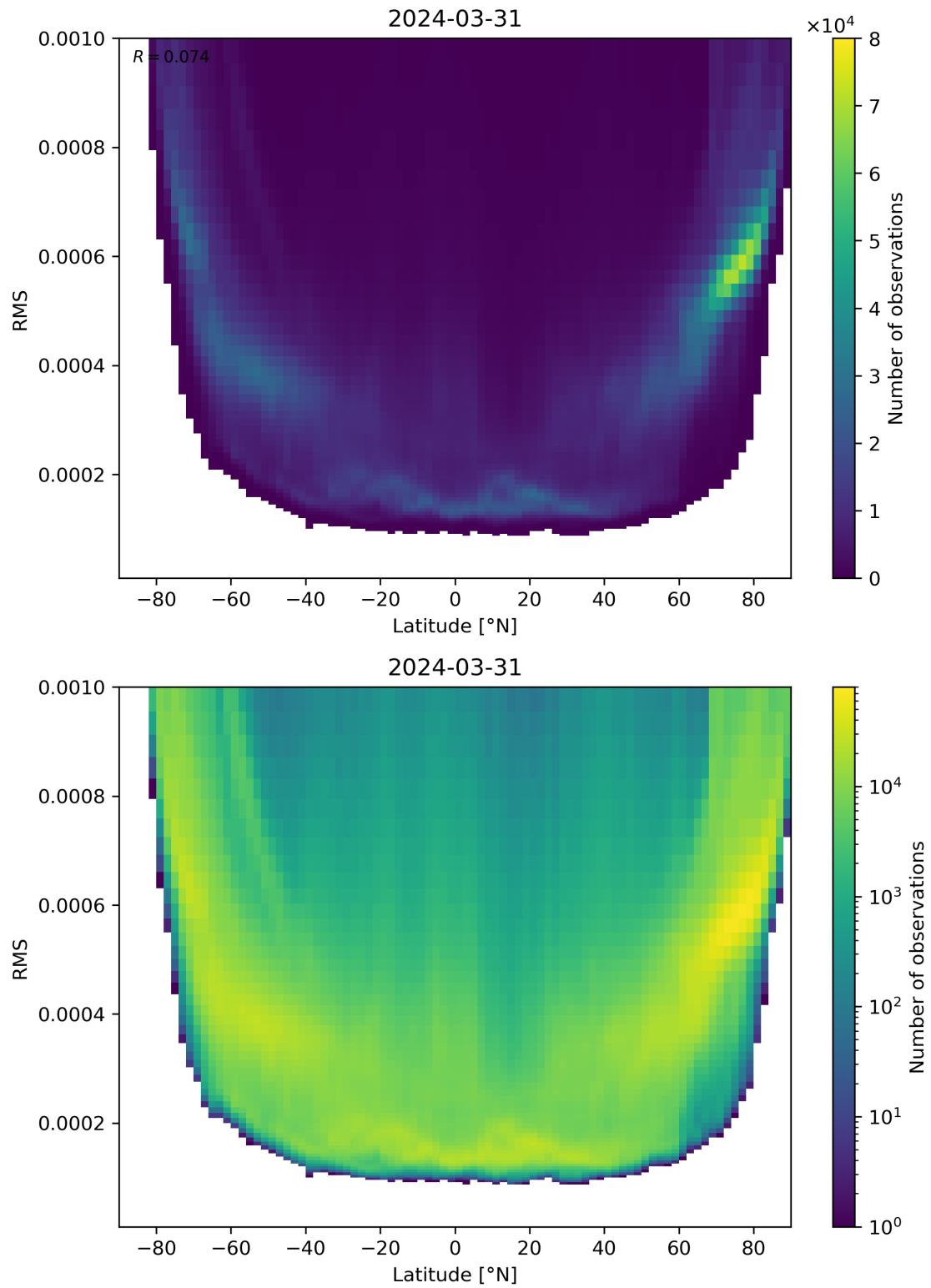
Figure 94: Scatter density plot of “Latitude” against “RMS” for 2024-03-31 to 2024-04-01.
