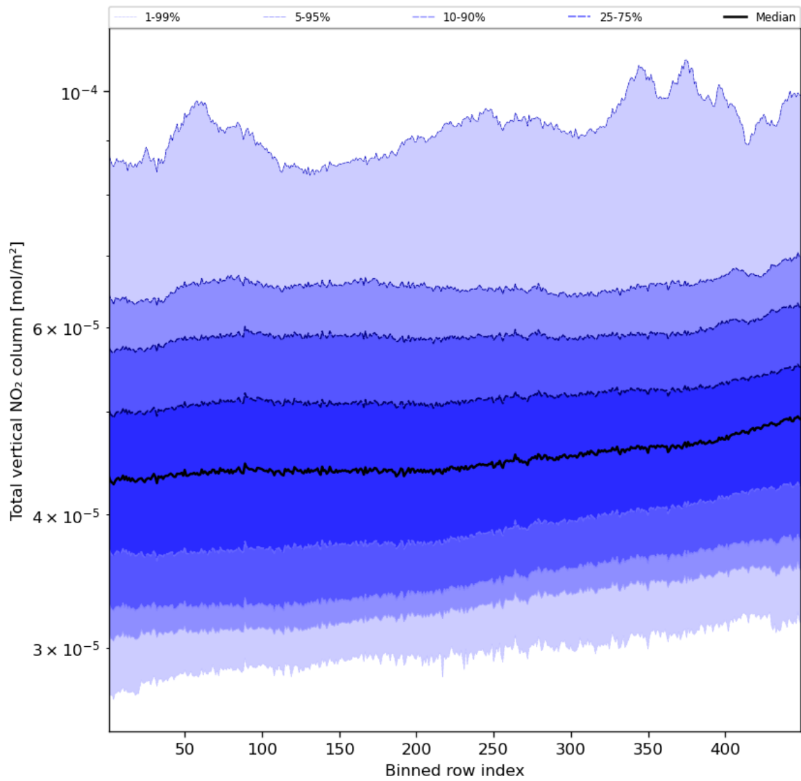
Figure 55: Along track statistics of “Total vertical NO 2 column” for 2024-03-31 to 2024-04-01
