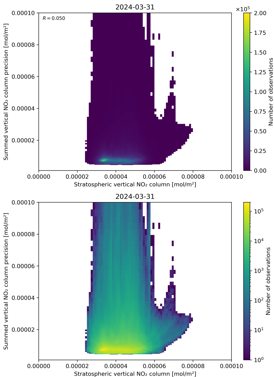
Figure 99: Scatter density plot of “Stratospheric vertical NO 2 column” against “Summed vertical NO 2 column precision” for 2024-03-31 to 2024-04-01.
