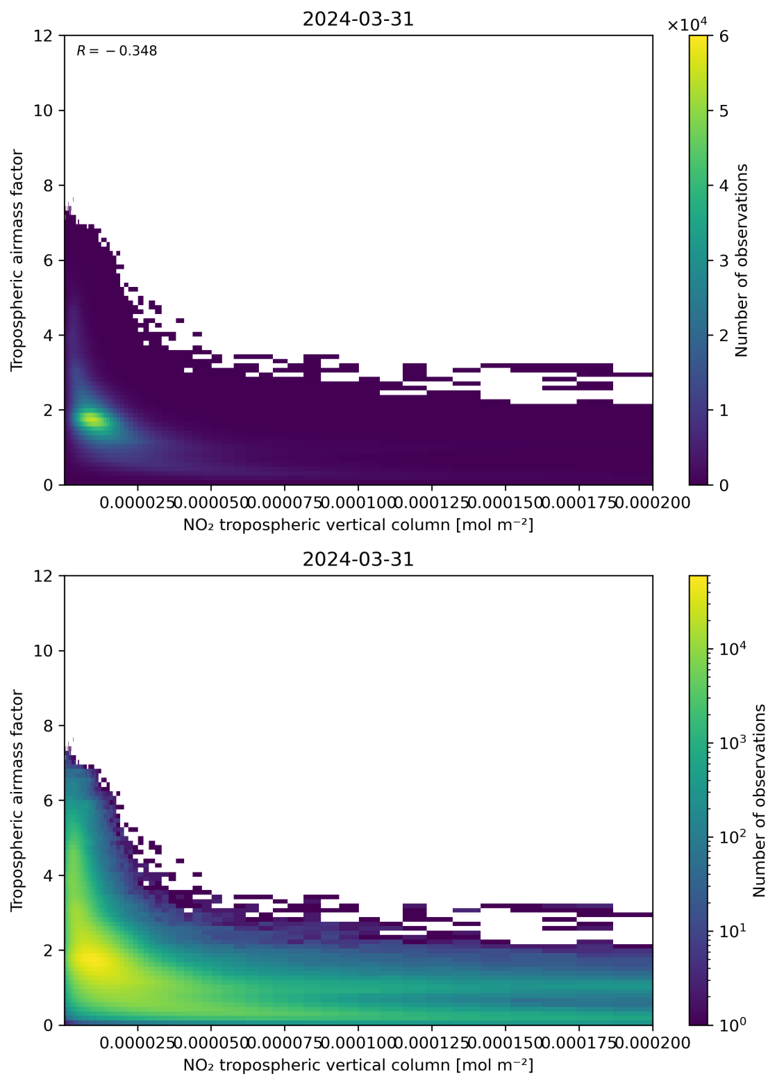
Figure 123: Scatter density plot of “NO 2 tropospheric vertical column” against “Tropospheric air mass factor” for 2024-03-31 to 2024-04-01.
