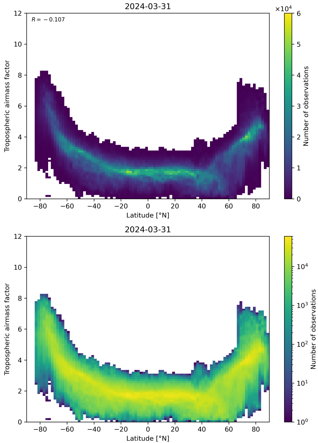
Figure 85: Scatter density plot of “Latitude” against “Tropospheric air mass factor” for 2024-03-31 to 2024-04-01.
