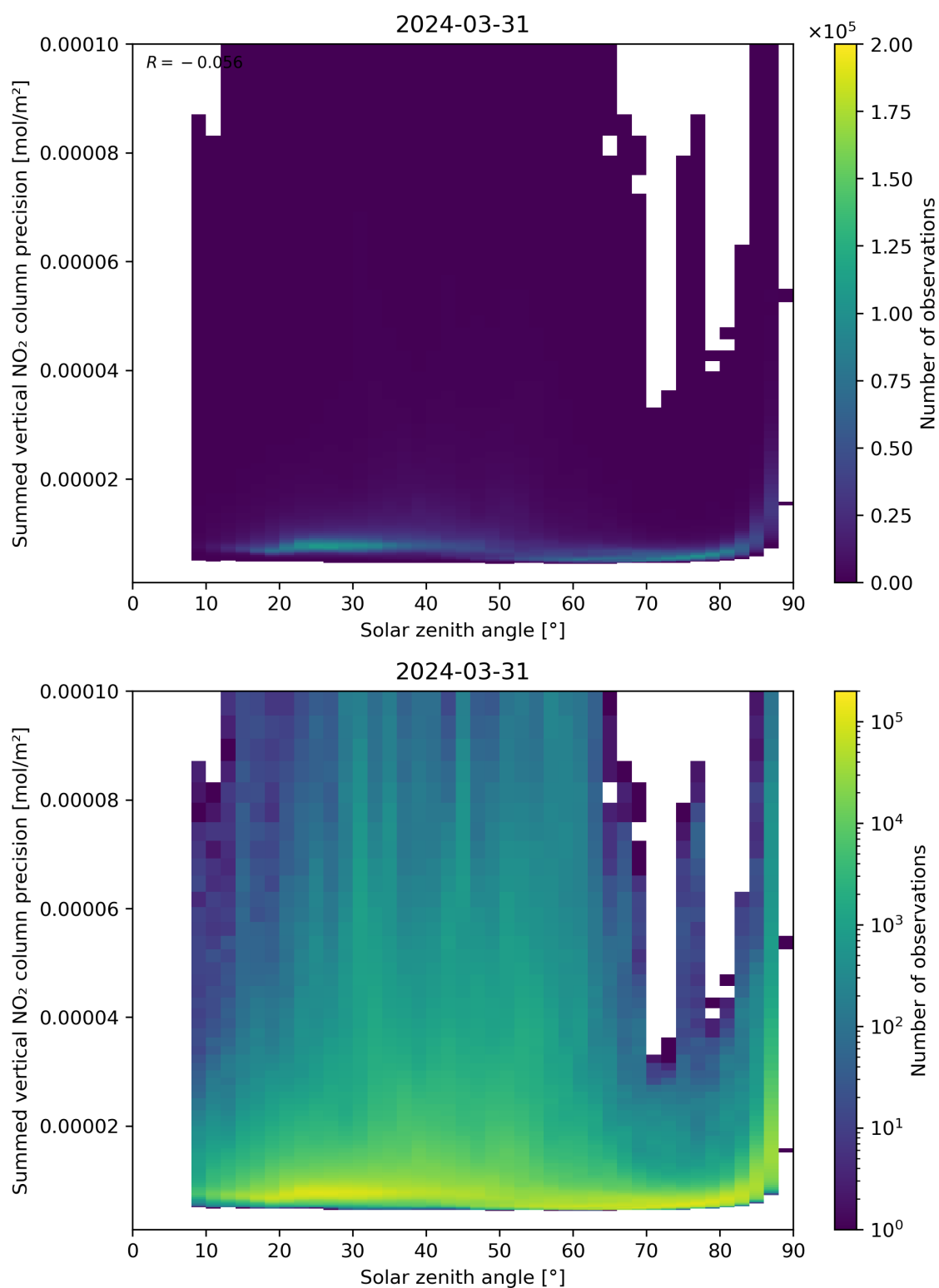
Figure 152: Scatter density plot of “Solar zenith angle” against “Summed vertical NO 2 column precision” for 2024-03-31 to 2024-04-01.
