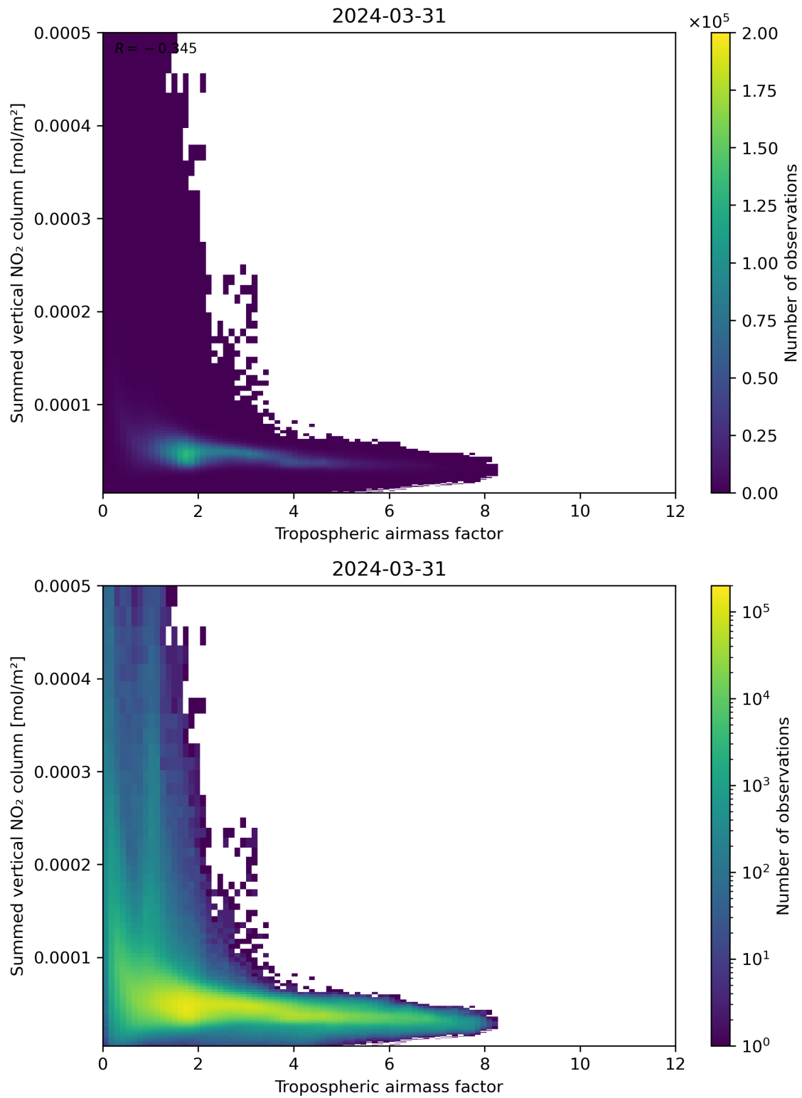
Figure 75: Scatter density plot of “Tropospheric air mass factor” against “Summed vertical NO 2 column” for 2024-03-31 to 2024-04-01.
