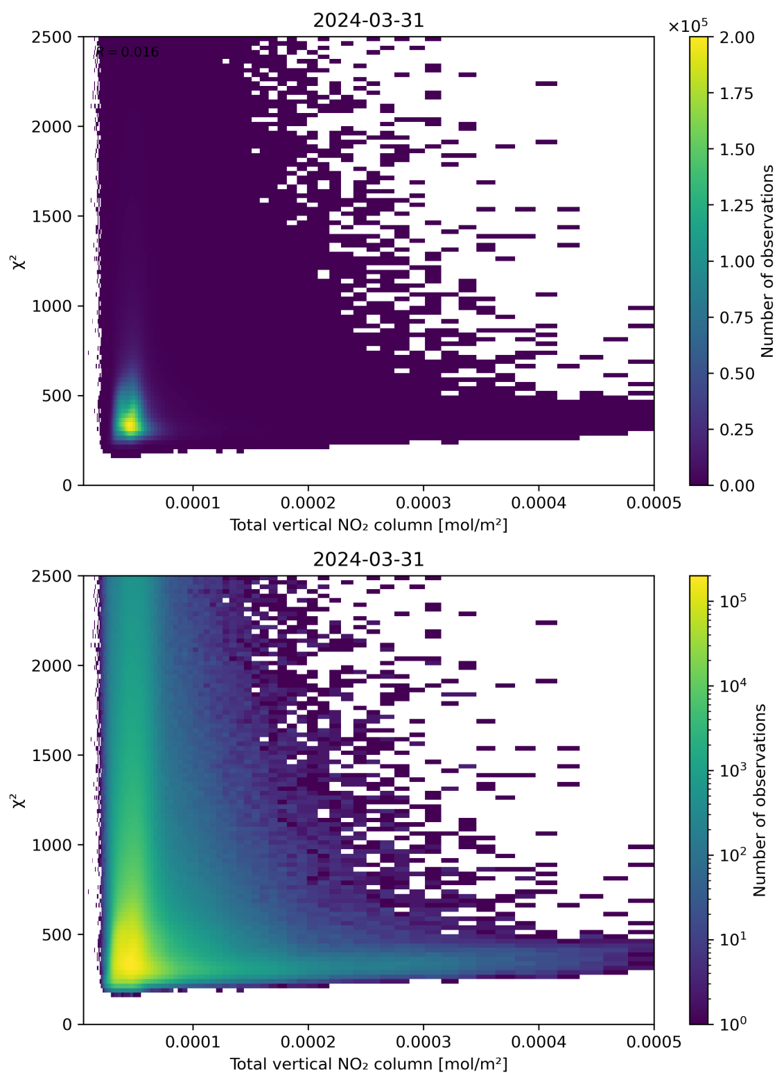
Figure 111: Scatter density plot of “Total vertical NO 2 column” against “ \chi^2 ” for 2024-03-31 to 2024-04-01.
