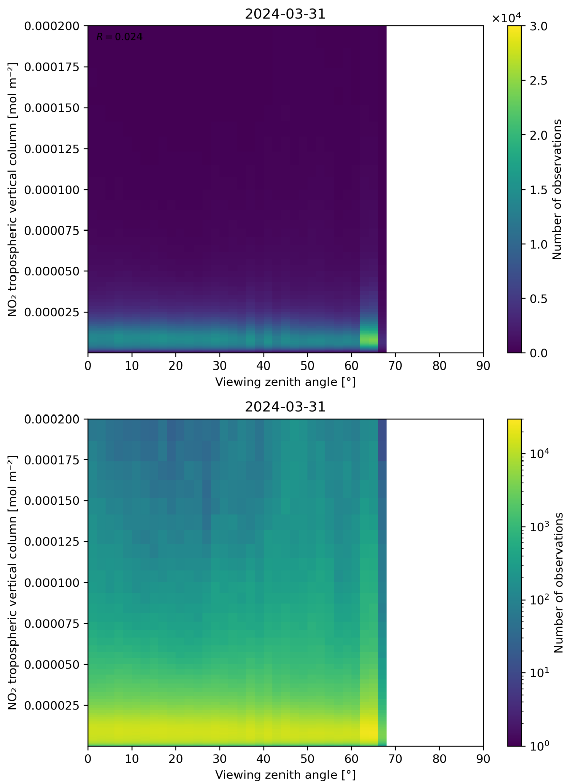
Figure 169: Scatter density plot of “Viewing zenith angle” against “NO 2 tropospheric vertical column” for 2024-03-31 to 2024-04-01.
