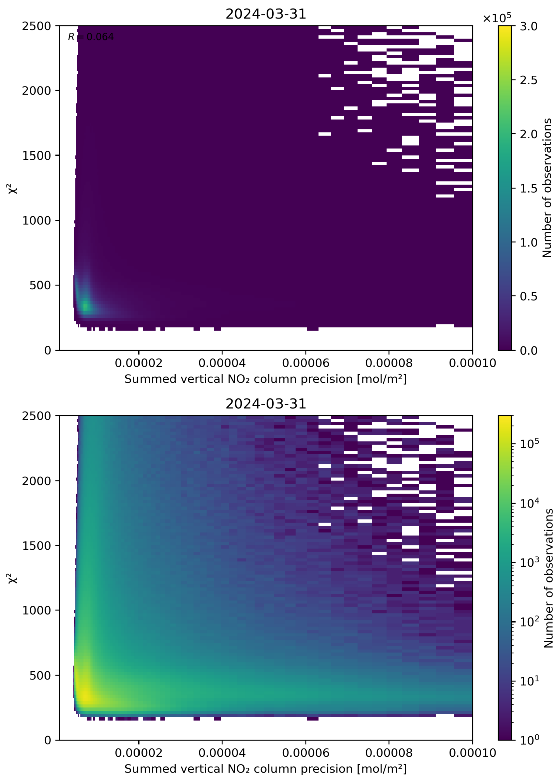
Figure 107: Scatter density plot of “Summed vertical NO 2 column precision” against “ \chi^2 ” for 2024-03-31 to 2024-04-01.
