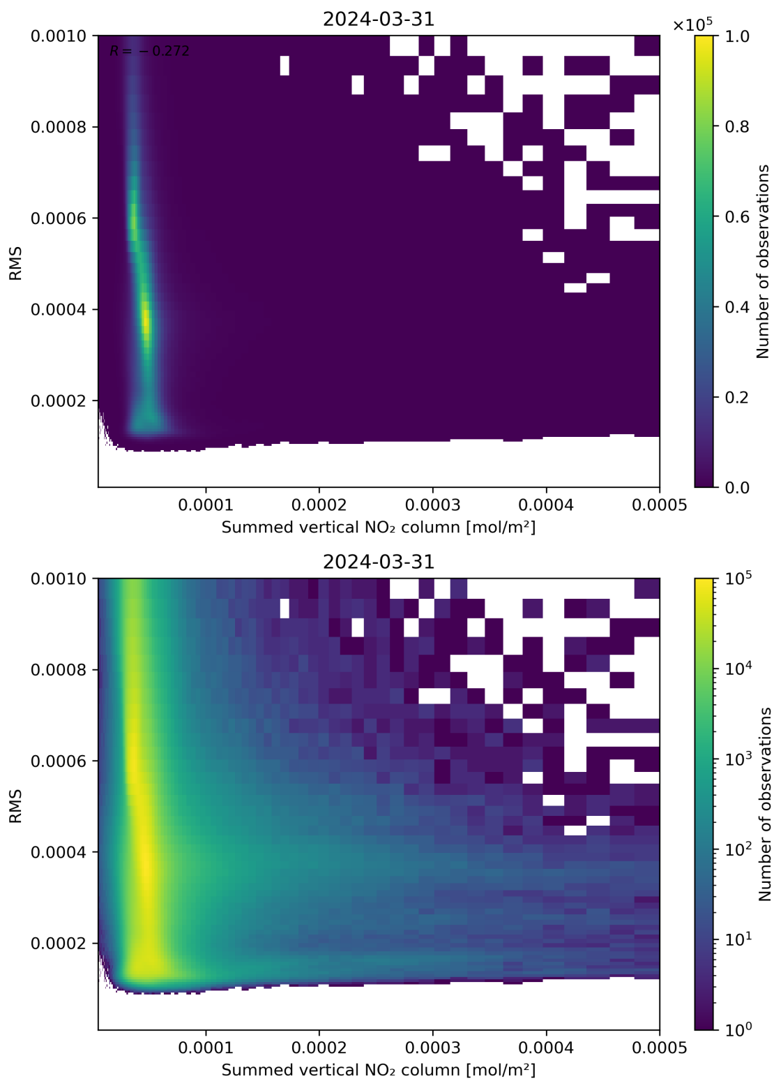
Figure 109: Scatter density plot of “Summed vertical NO 2 column” against “RMS” for 2024-03-31 to 2024-04-01.
