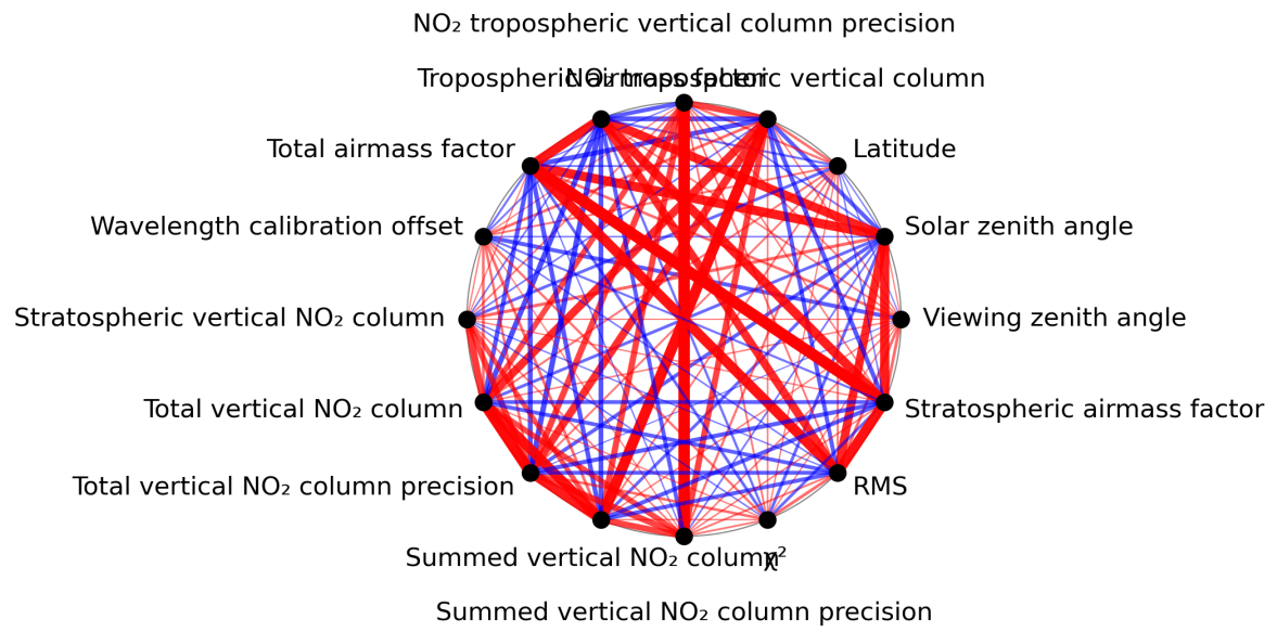
Figure 1: Map of correlation graph for 2024-03-31 to 2024-04-01.
