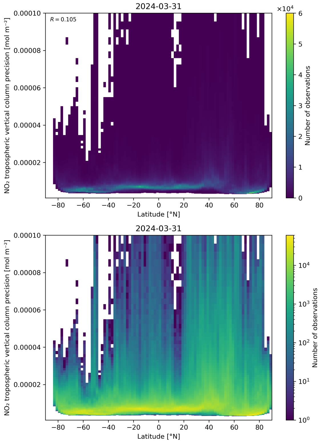
Figure 93: Scatter density plot of “Latitude” against “NO 2 tropospheric vertical column precision” for 2024-03-31 to 2024-04-01.
