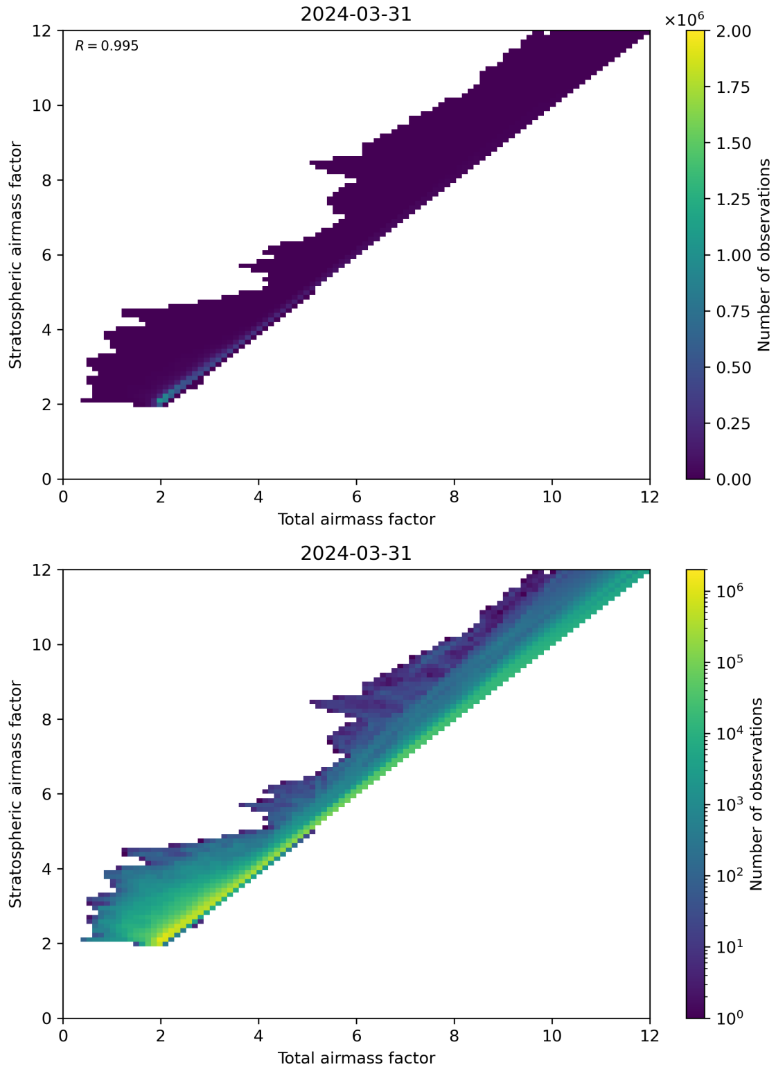
Figure 62: Scatter density plot of “Total air mass factor” against “Stratospheric air mass factor” for 2024-03-31 to 2024-04-01.
