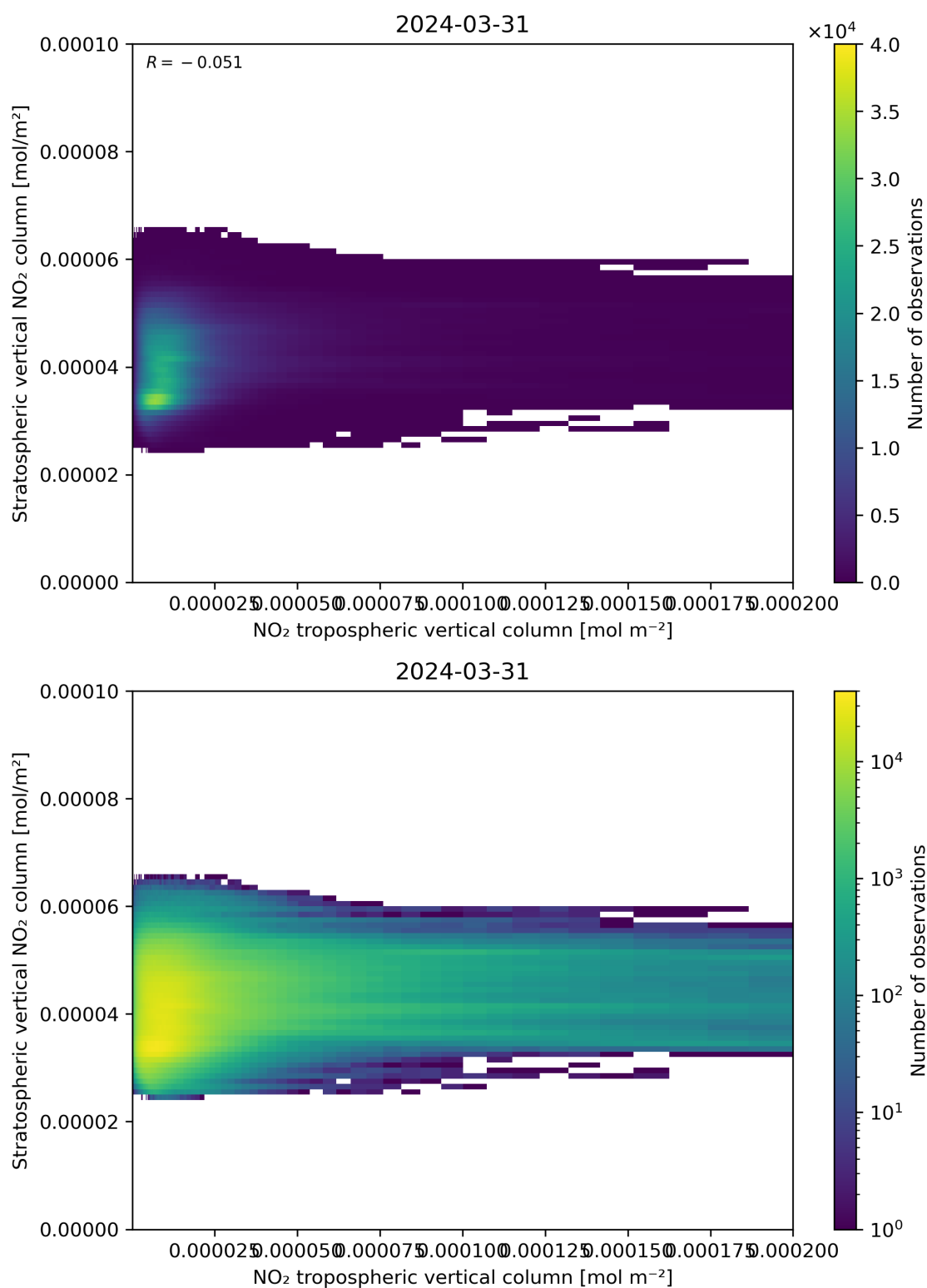
Figure 125: Scatter density plot of “NO 2 tropospheric vertical column” against “Stratospheric vertical NO 2 column” for 2024-03-31 to 2024-04-01.
