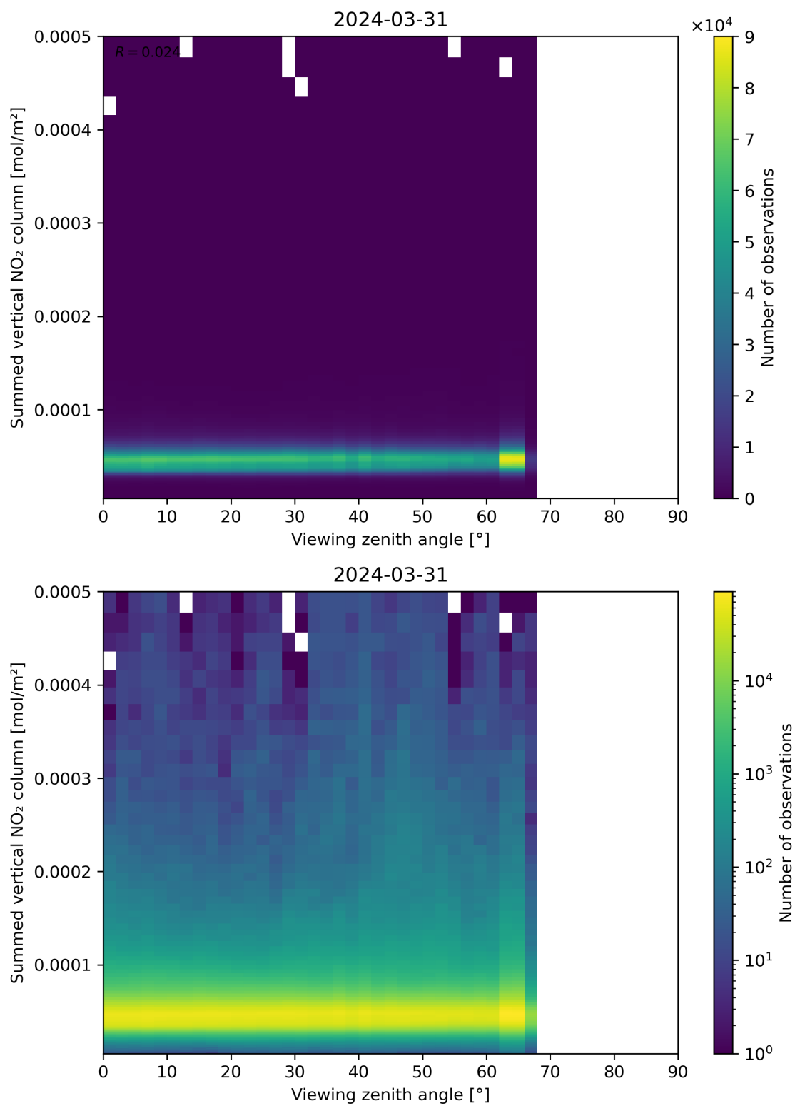
Figure 165: Scatter density plot of “Viewing zenith angle” against “Summed vertical NO 2 column” for 2024-03-31 to 2024-04-01.
