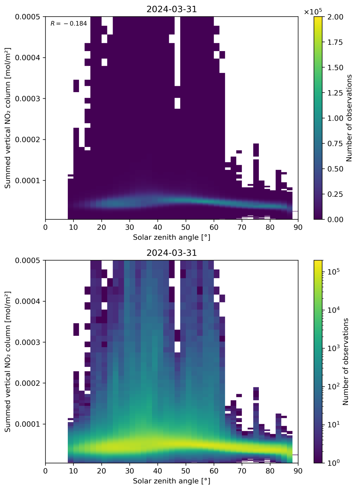
Figure 151: Scatter density plot of “Solar zenith angle” against “Summed vertical NO 2 column” for 2024-03-31 to 2024-04-01.
