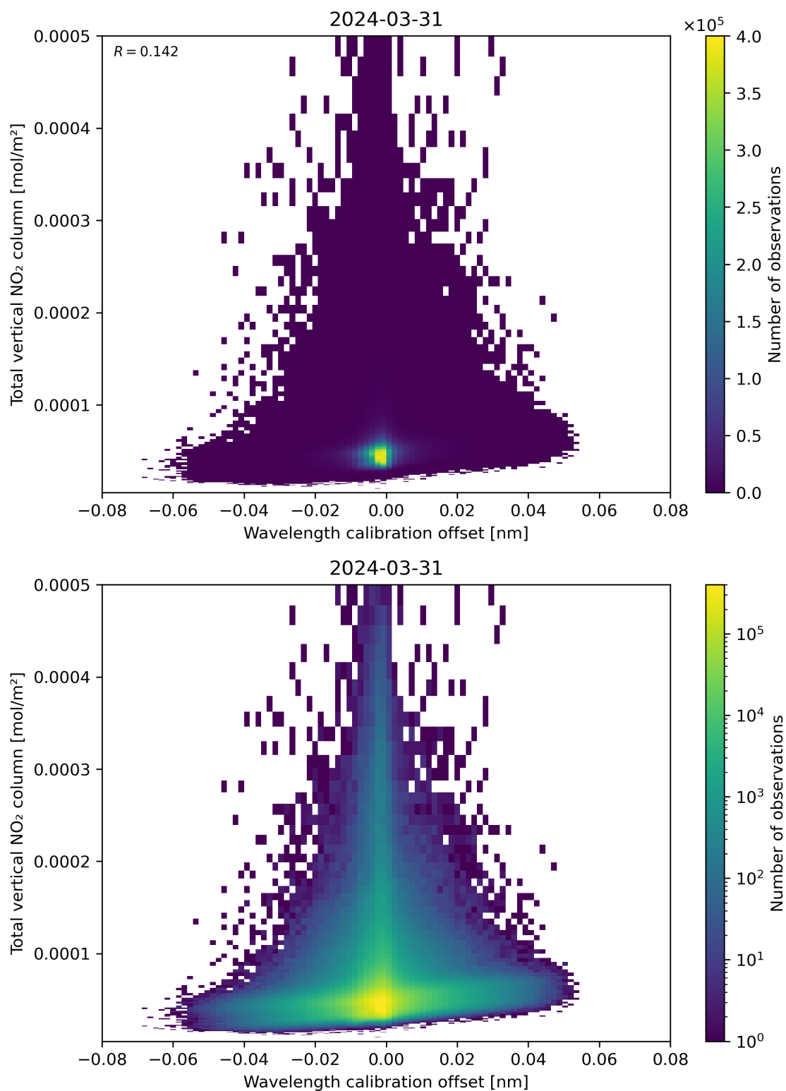
Figure 179: Scatter density plot of “Wavelength calibration offset” against “Total vertical NO 2 column” for 2024-03-31 to 2024-04-01.
