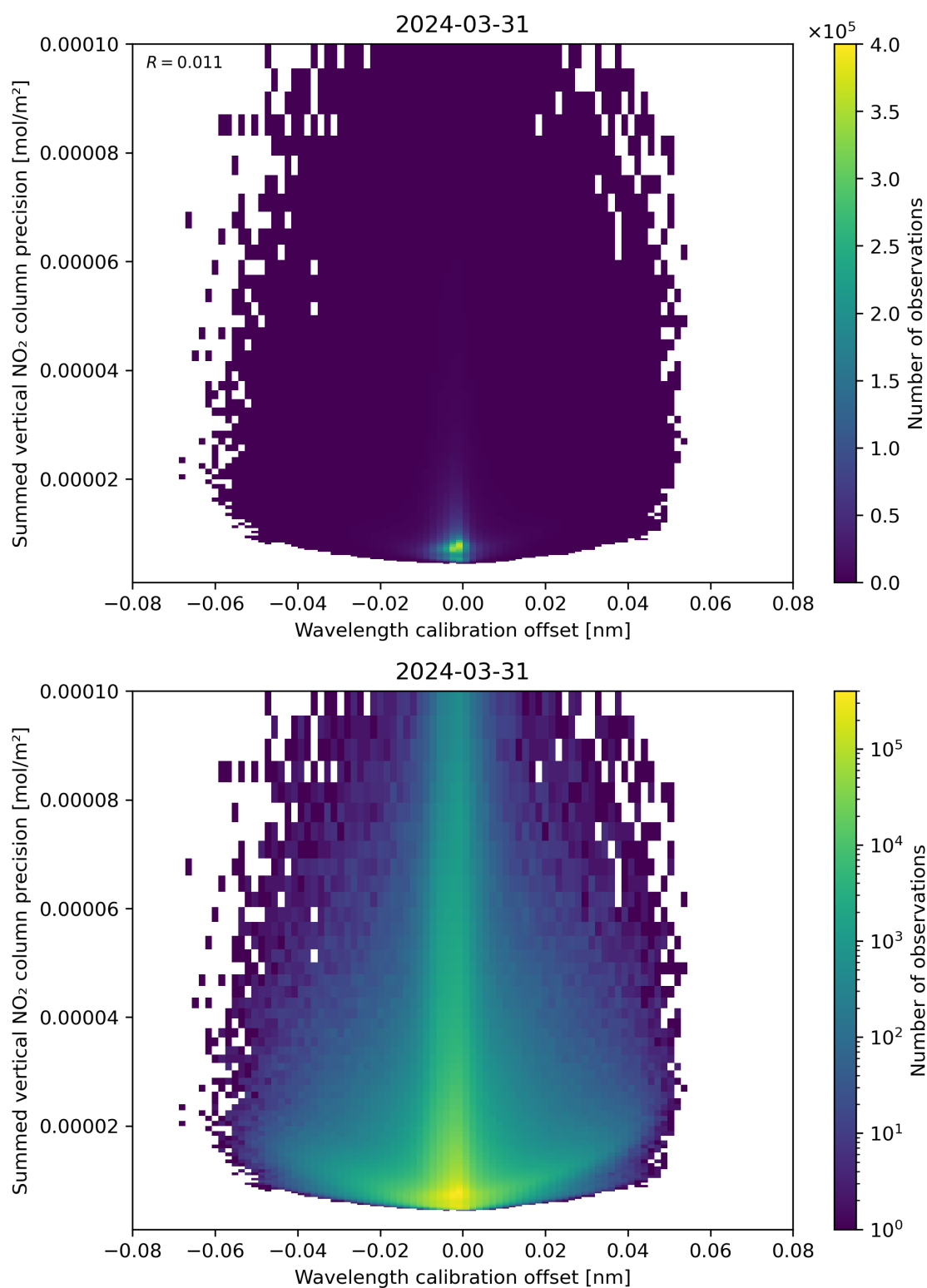
Figure 178: Scatter density plot of “Wavelength calibration offset” against “Summed vertical NO 2 column precision” for 2024-03-31 to 2024-04-01.
