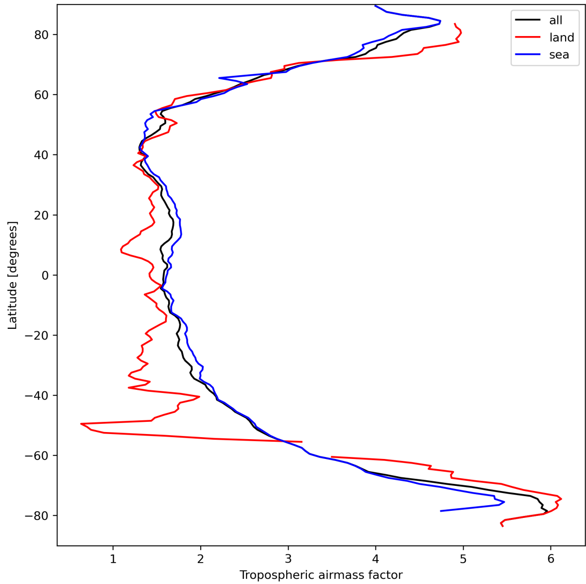
Figure 14: Zonal average of “Tropospheric air mass factor” for 2024-03-31 to 2024-04-01.
