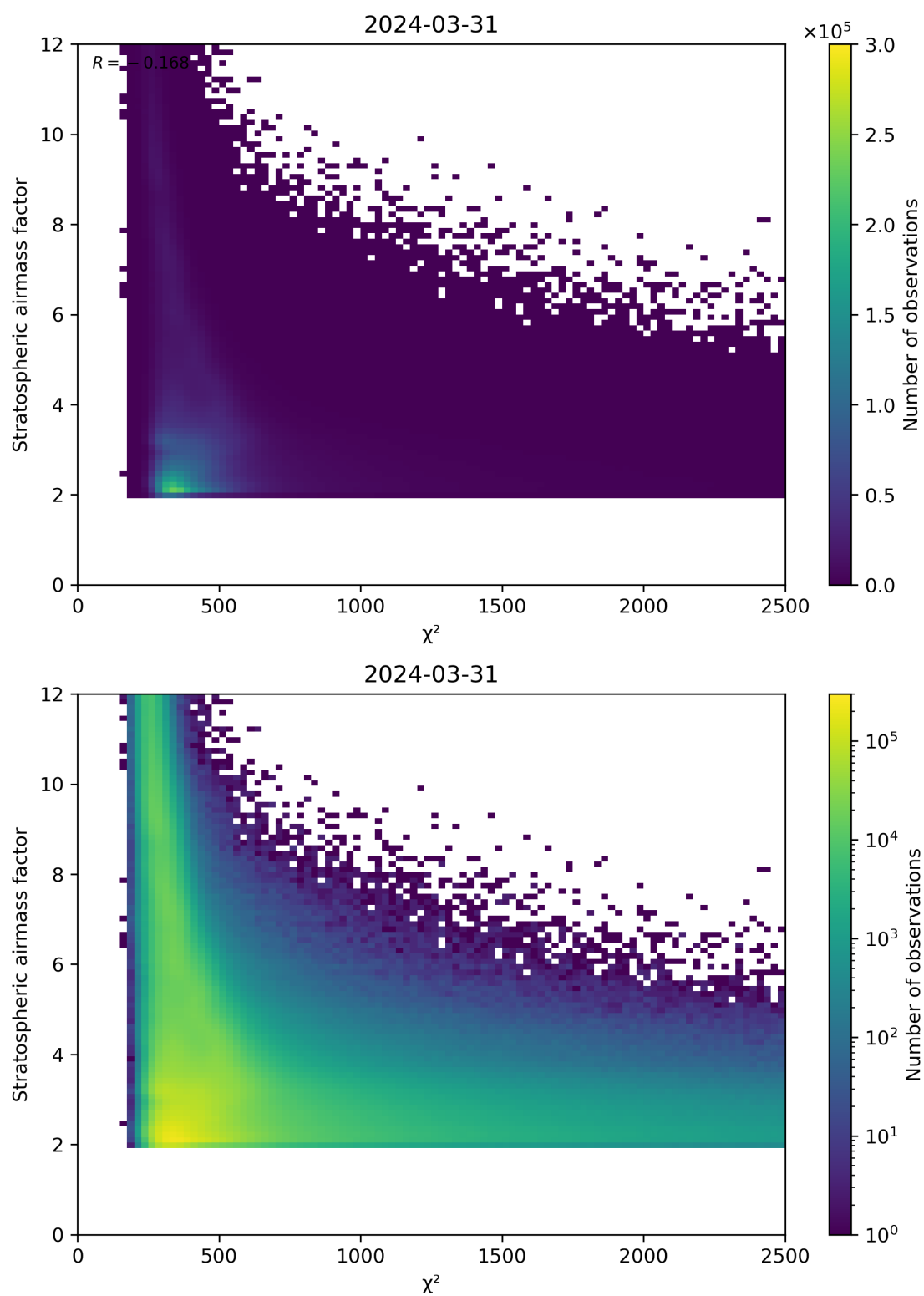
Figure 81: Scatter density plot of “ \chi^2 ” against “Stratospheric airmass factor” for 2024-03-31 to 2024-04-01.
