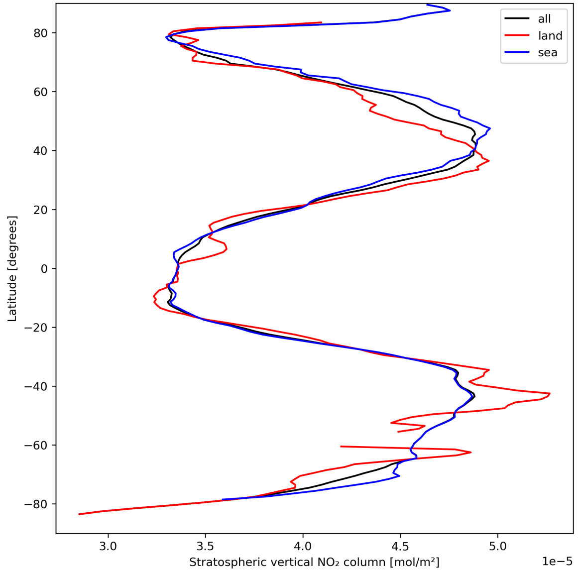
Figure 19: Zonal average of “Stratospheric vertical NO 2 column” for 2024-03-31 to 2024-04-01.
