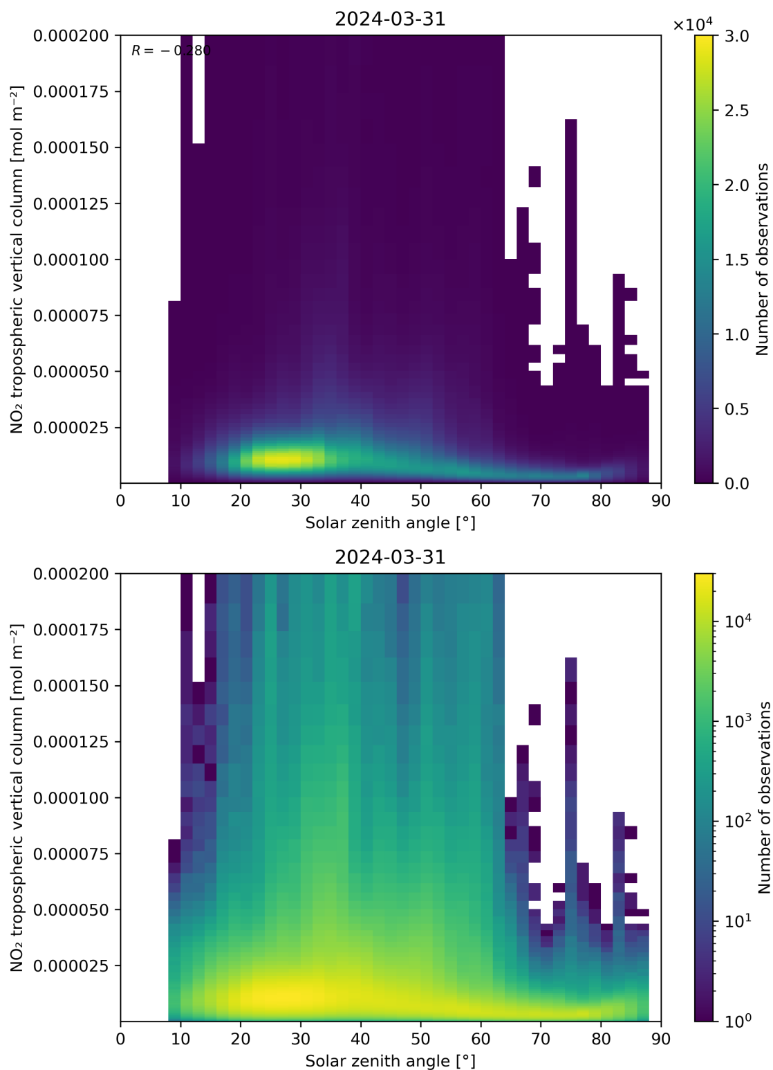
Figure 155: Scatter density plot of “Solar zenith angle” against “NO 2 tropospheric vertical column” for 2024-03-31 to 2024-04-01.
