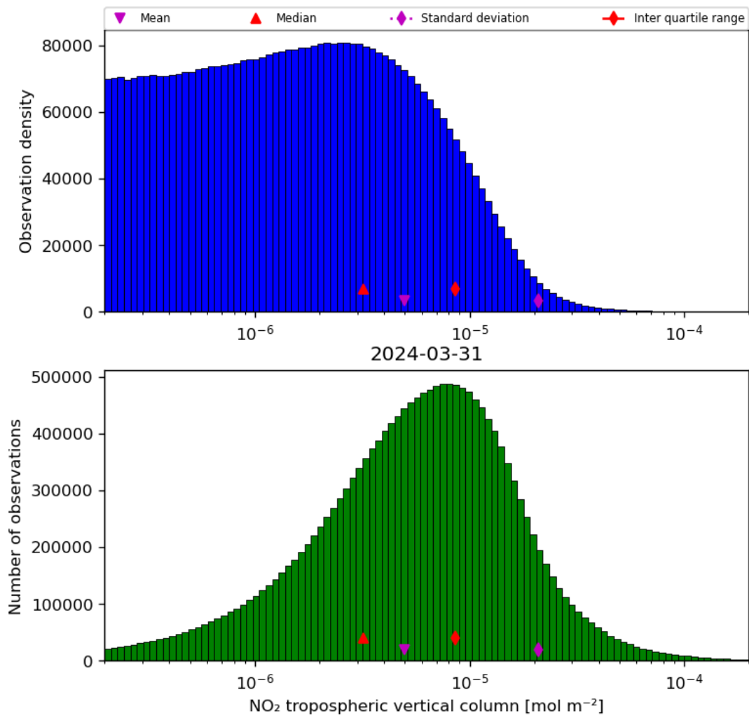
Figure 29: Histogram of “NO 2 tropospheric vertical column” for 2024-03-31 to 2024-04-01
