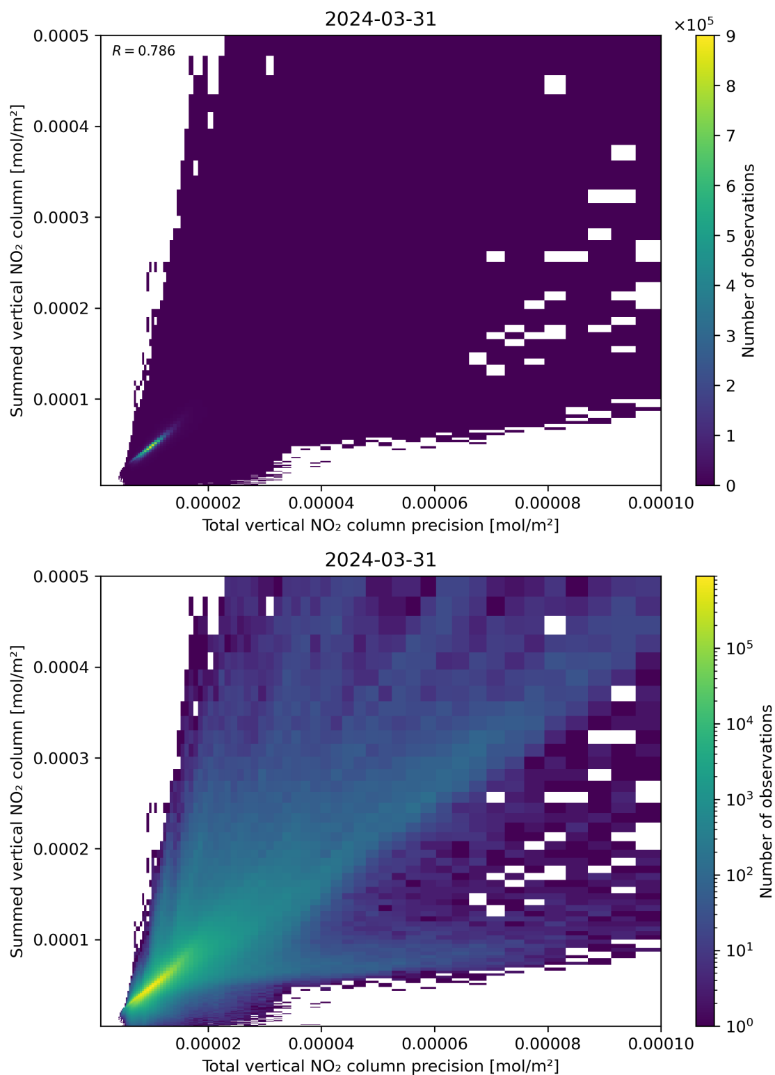
Figure 117: Scatter density plot of “Total vertical NO 2 column precision” against “Summed vertical NO 2 column” for 2024-03-31 to 2024-04-01.
