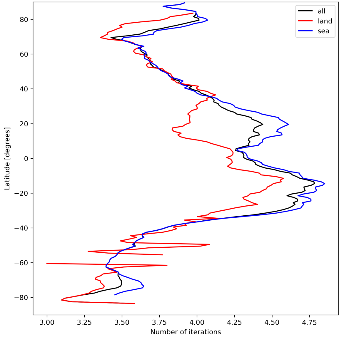
Figure 17: Zonal average of “Number of iterations” for 2024-03-31 to 2024-04-01.
