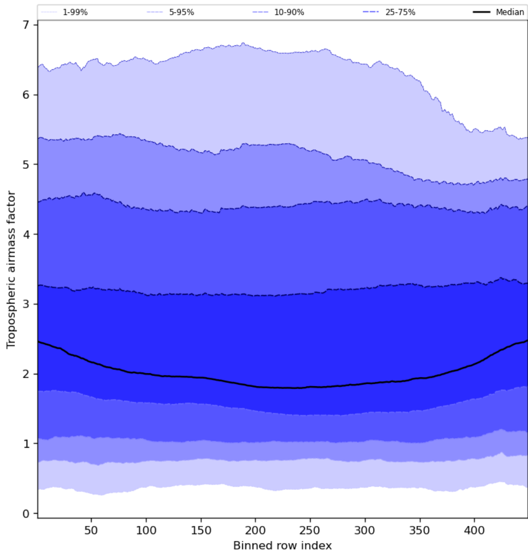
Figure 48: Along track statistics of “Tropospheric airmass factor” for 2024-03-31 to 2024-04-01
