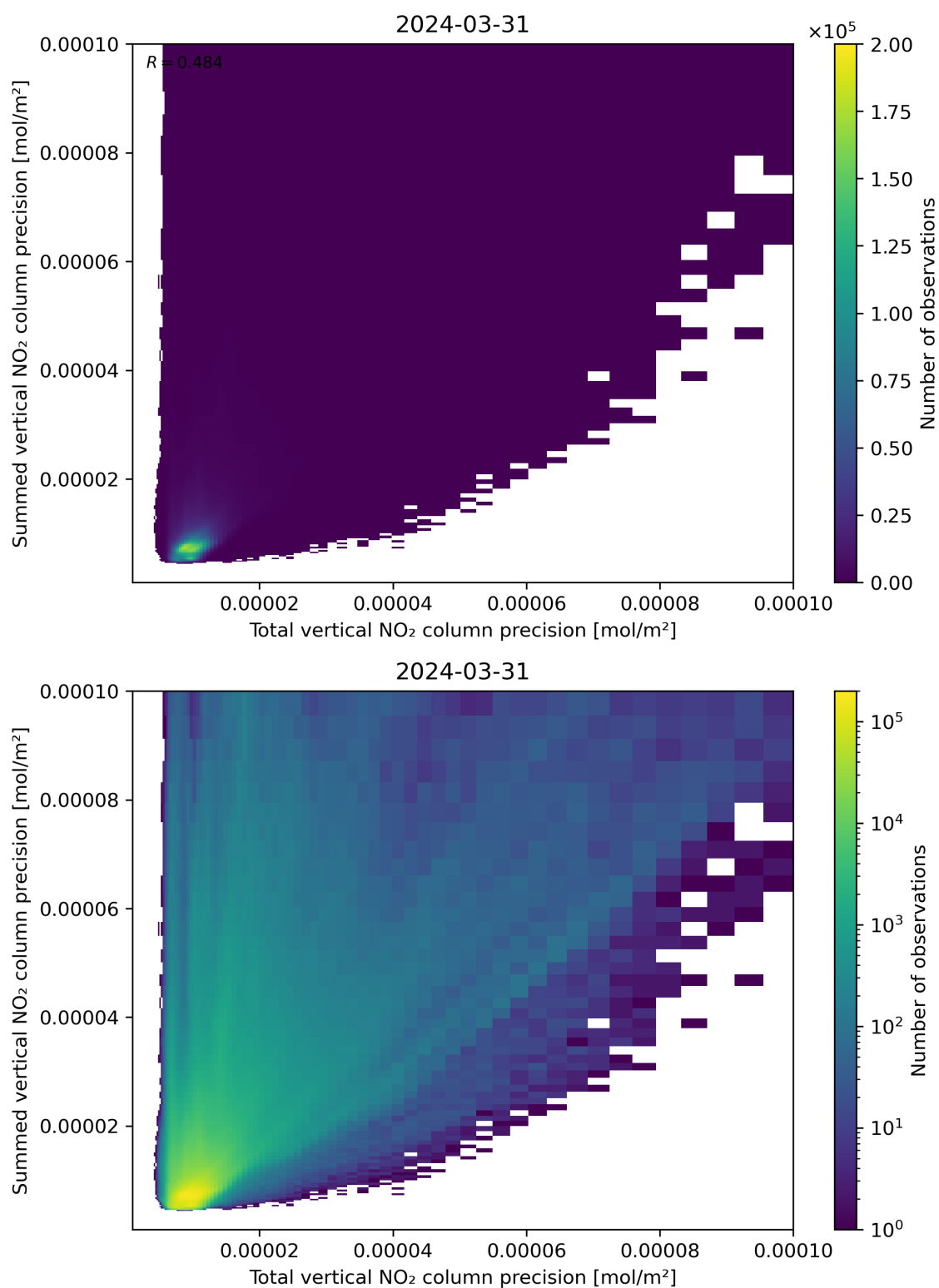
Figure 118: Scatter density plot of “Total vertical NO 2 column precision” against “Summed vertical NO 2 column precision” for 2024-03-31 to 2024-04-01.
