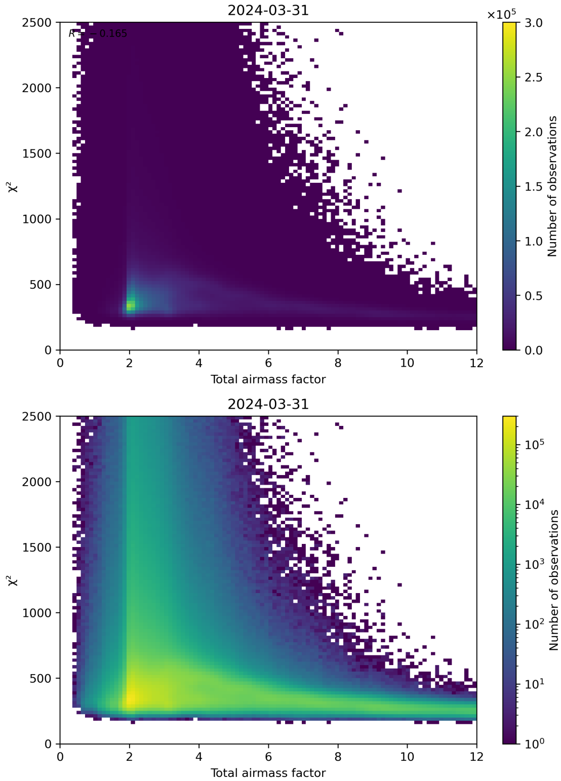
Figure 63: Scatter density plot of “Total airmass factor” against “ \chi^2 ” for 2024-03-31 to 2024-04-01.
