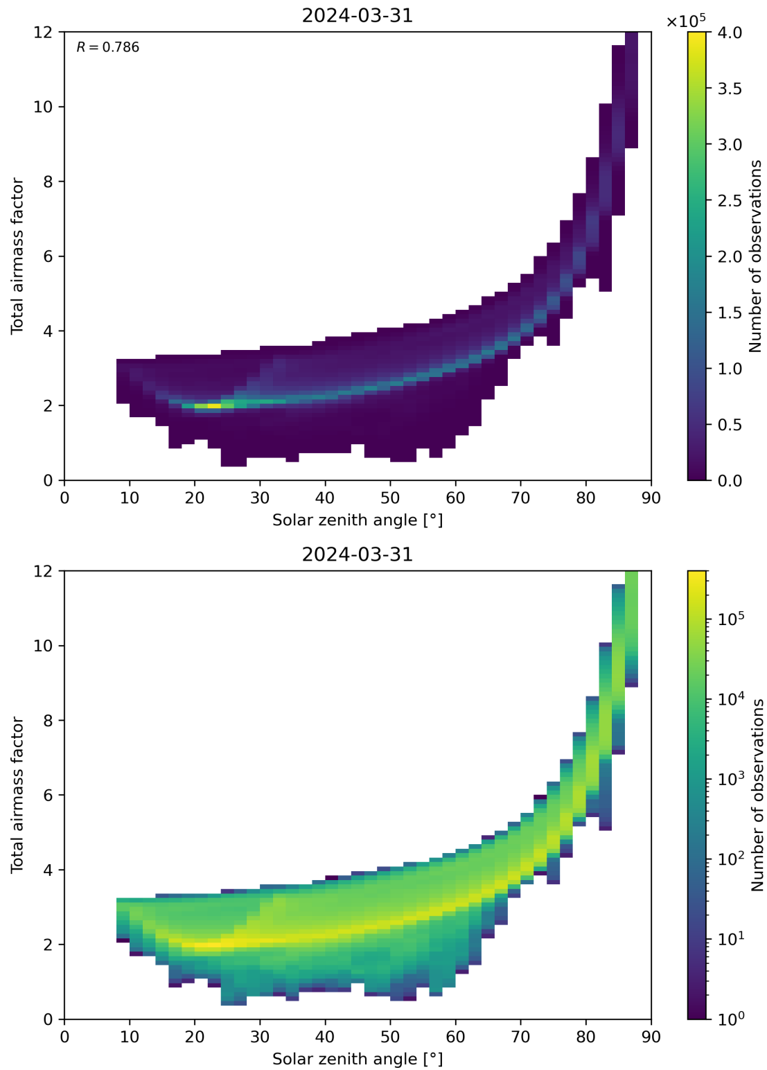
Figure 146: Scatter density plot of “Solar zenith angle” against “Total air mass factor” for 2024-03-31 to 2024-04-01.
