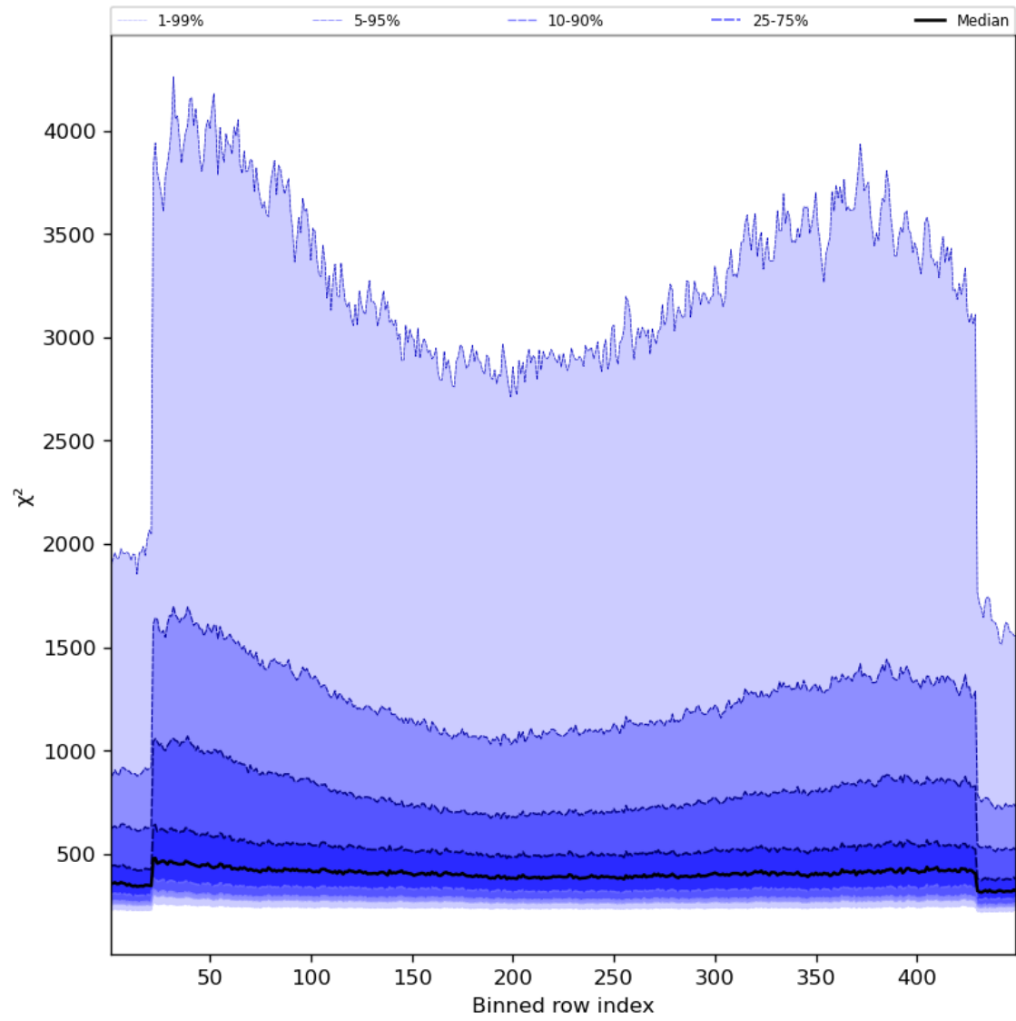
Figure 59: Along track statistics of “ \chi^2 ” for 2024-03-31 to 2024-04-01
