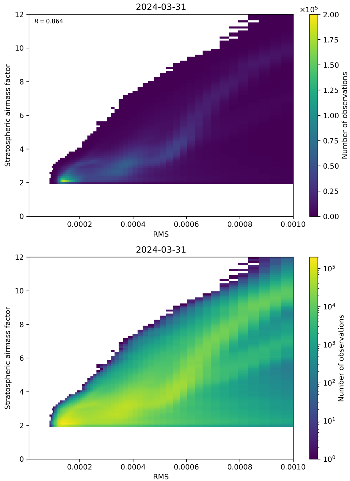
Figure 144: Scatter density plot of “RMS” against “Stratospheric airmass factor” for 2024-03-31 to 2024-04-01.
