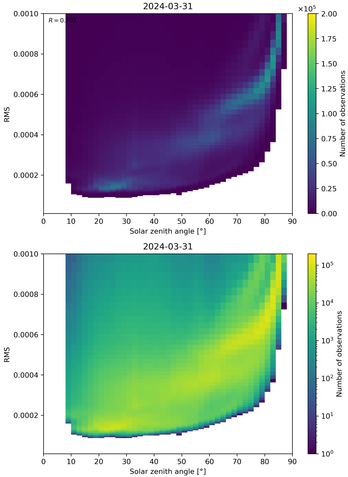
Figure 157: Scatter density plot of “Solar zenith angle” against “RMS” for 2024-03-31 to 2024-04-01.
