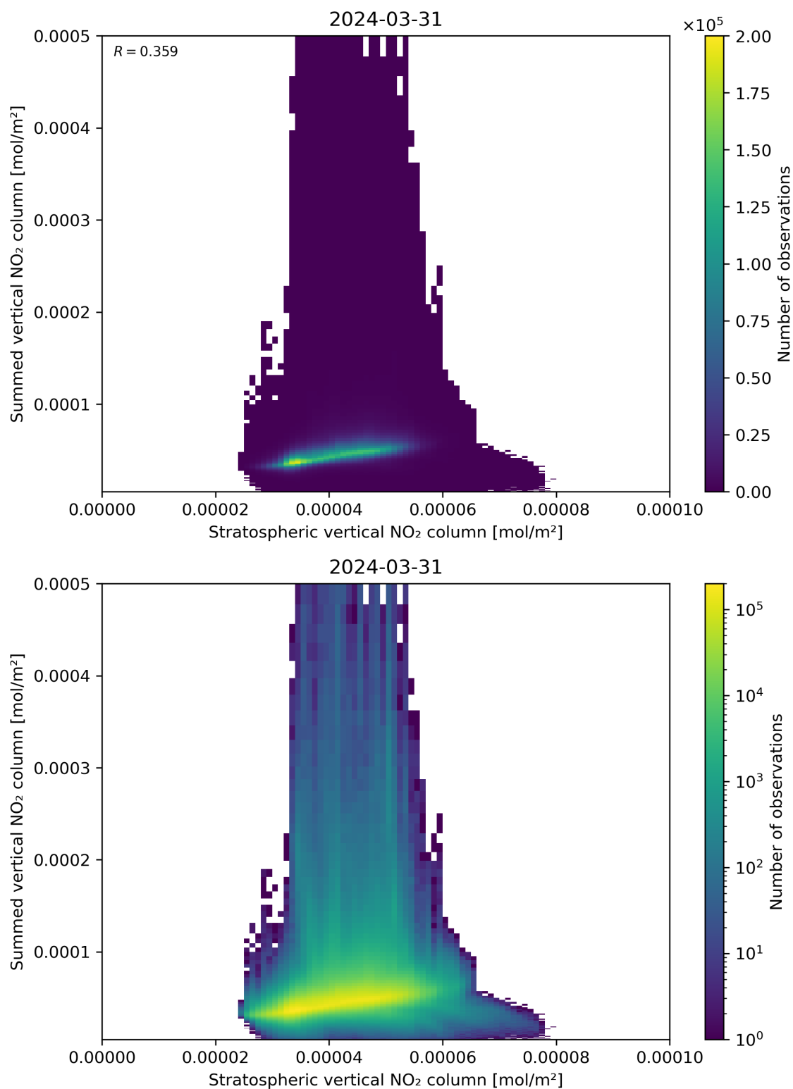
Figure 98: Scatter density plot of “Stratospheric vertical NO 2 column” against “Summed vertical NO 2 column” for 2024-03-31 to 2024-04-01.
