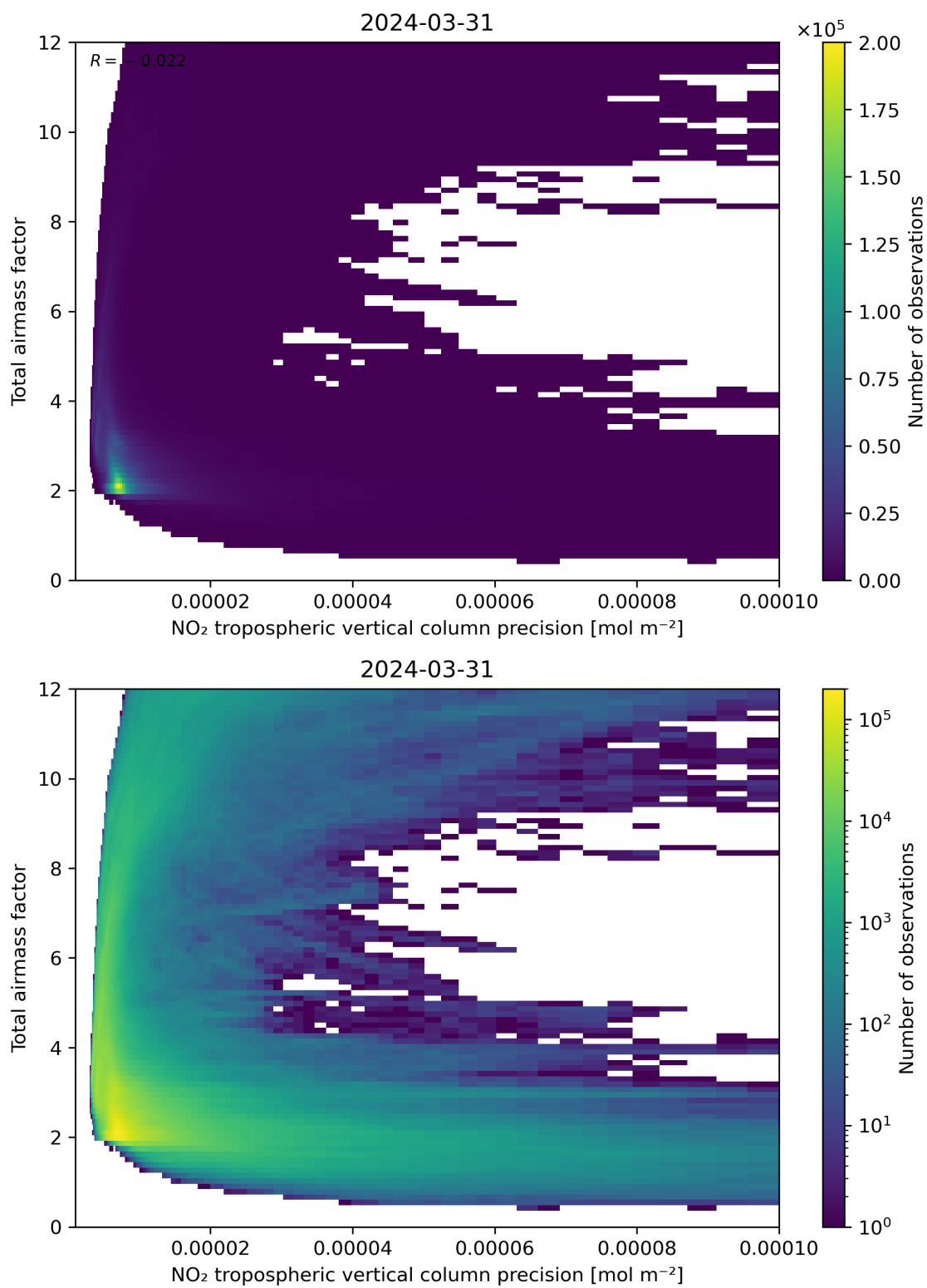
Figure 132: Scatter density plot of “NO 2 tropospheric vertical column precision” against “Total air mass factor” for 2024-03-31 to 2024-04-01.
