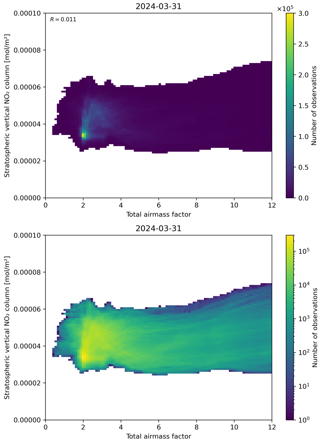
Figure 64: Scatter density plot of “Total airmass factor” against “Stratospheric vertical NO 2 column” for 2024-03-31 to 2024-04-01.
