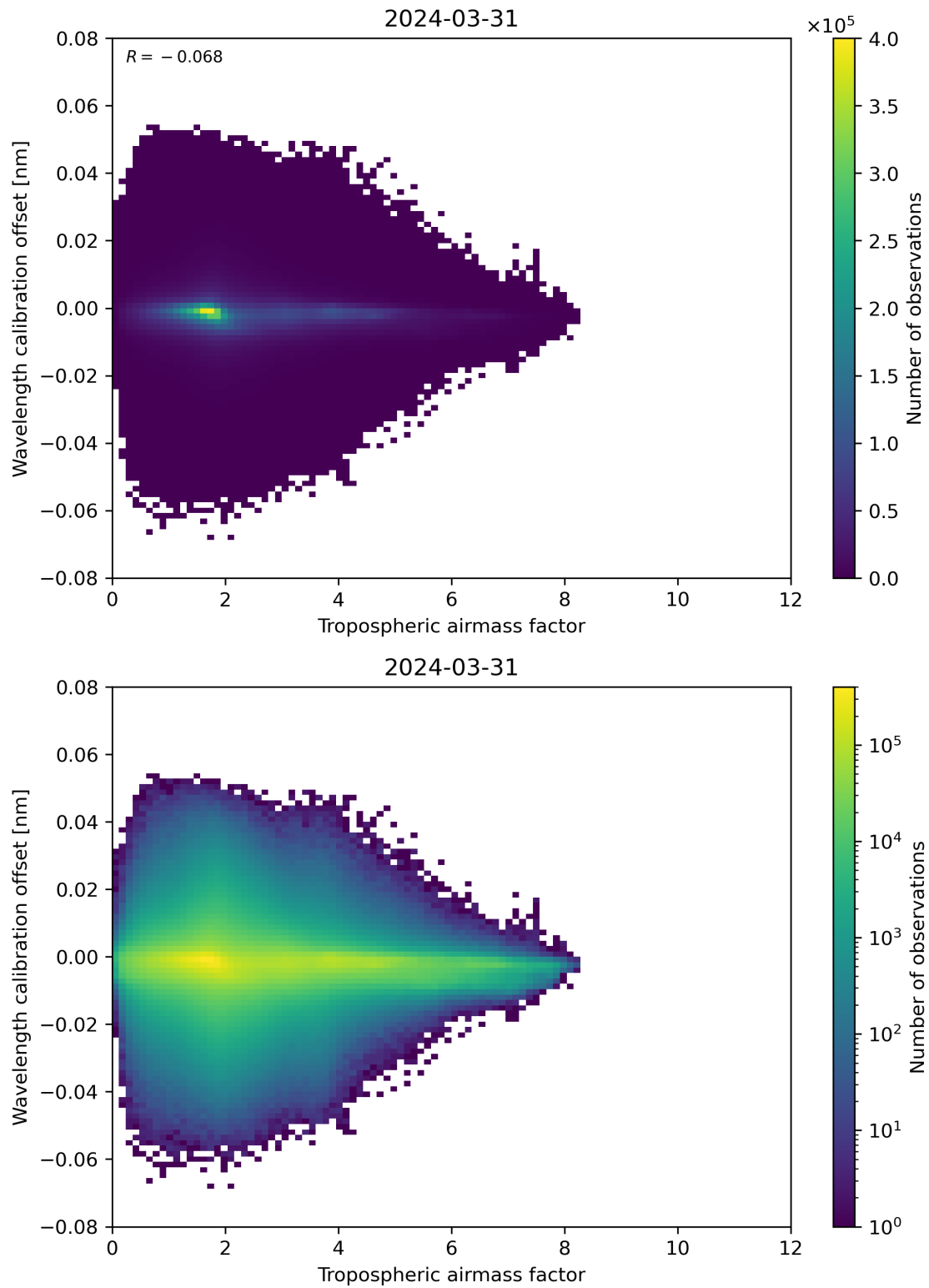
Figure 80: Scatter density plot of “Tropospheric airmass factor” against “Wavelength calibration offset” for 2024-03-31 to 2024-04-01.
