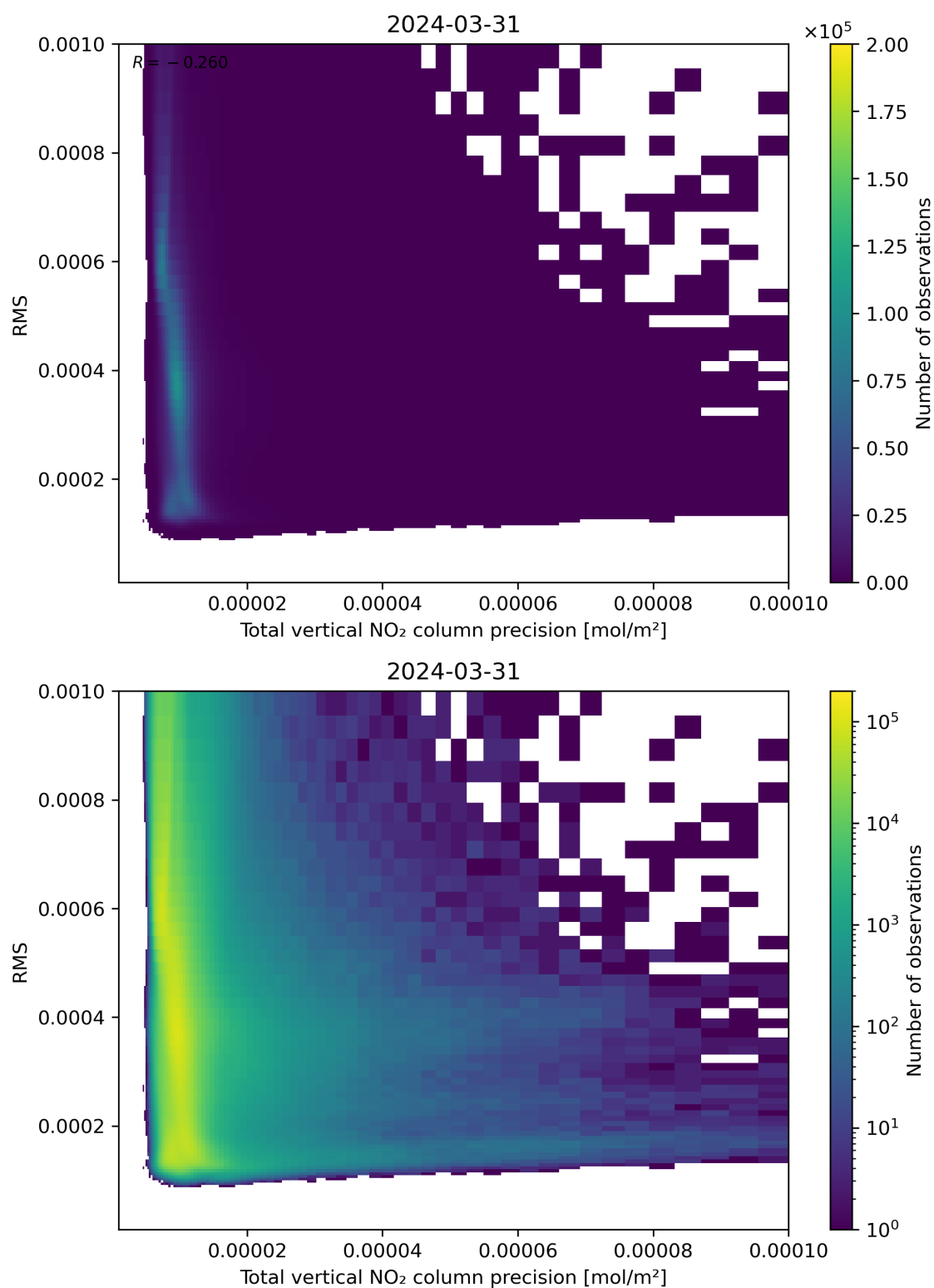
Figure 119: Scatter density plot of “Total vertical NO 2 column precision” against “RMS” for 2024-03-31 to 2024-04-01.
