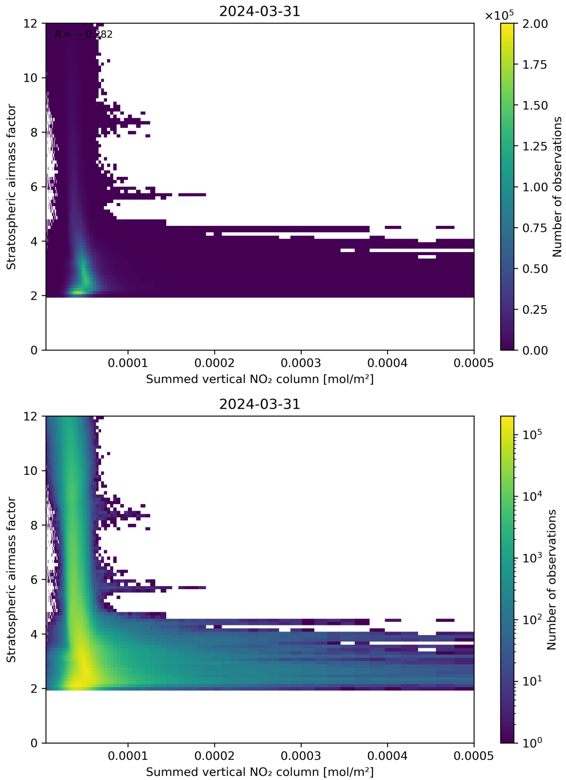
Figure 103: Scatter density plot of “Summed vertical NO 2 column” against “Stratospheric air mass factor” for 2024-03-31 to 2024-04-01.
