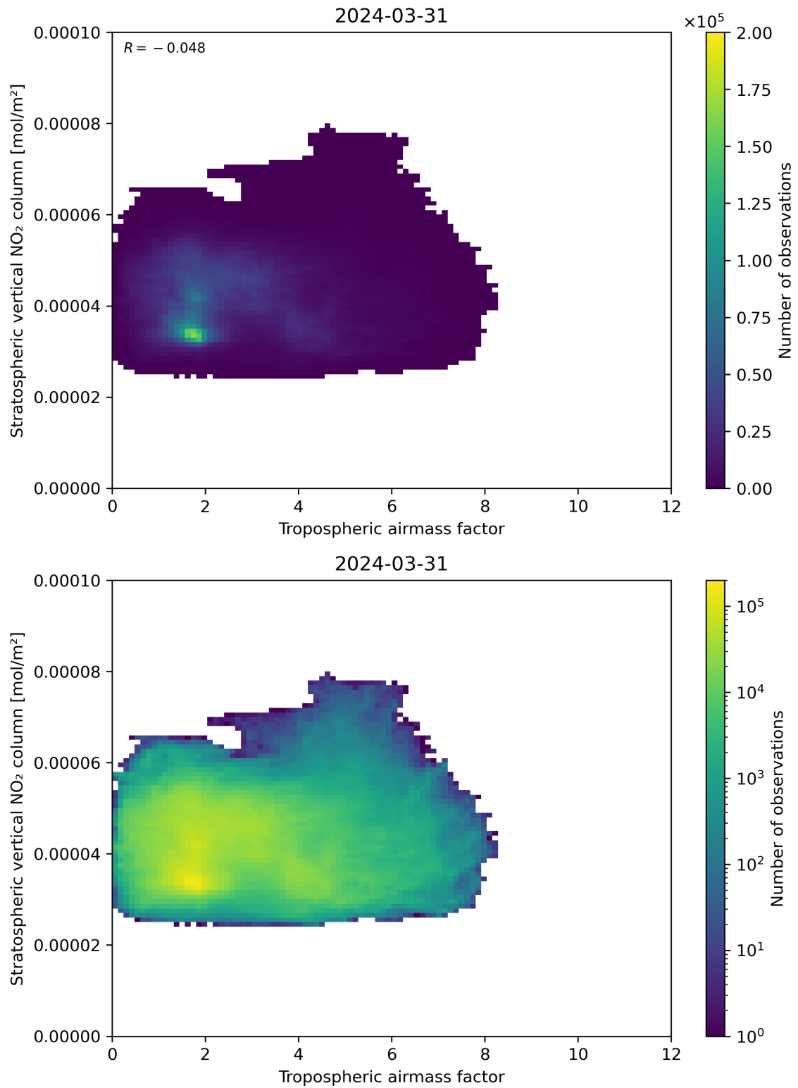
Figure 74: Scatter density plot of “Tropospheric air mass factor” against “Stratospheric vertical NO 2 column” for 2024-03-31 to 2024-04-01.
