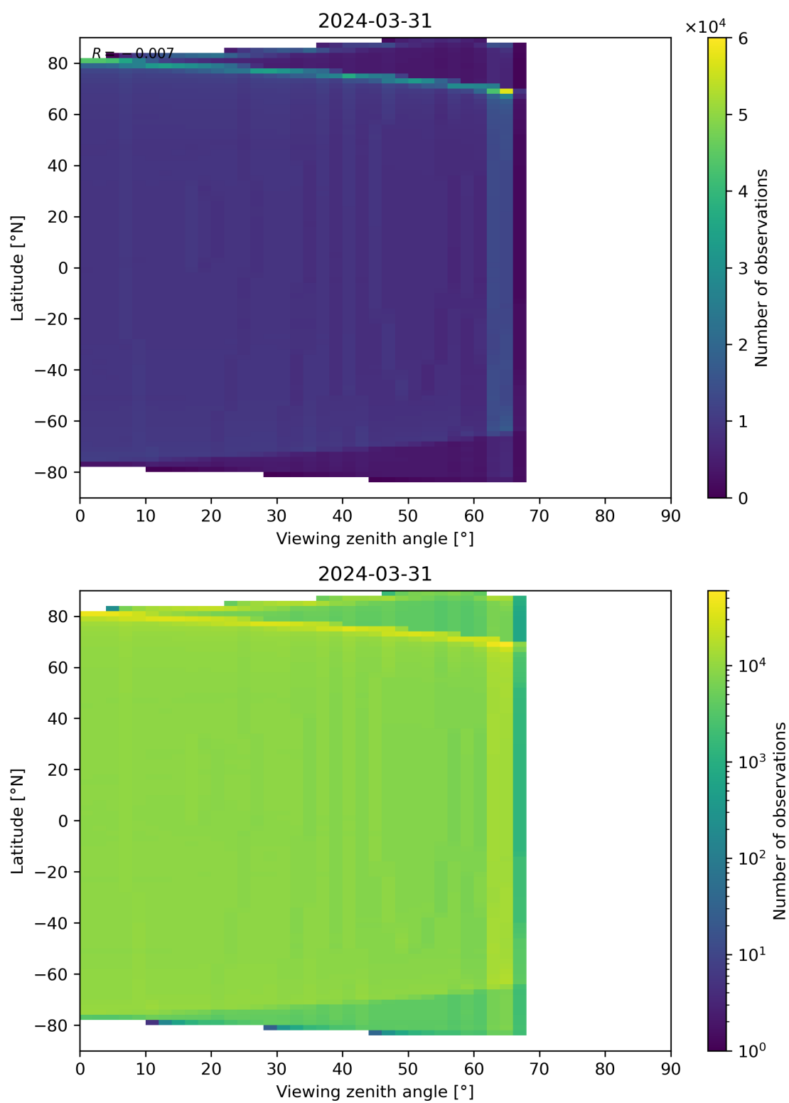
Figure 163: Scatter density plot of “Viewing zenith angle” against “Latitude” for 2024-03-31 to 2024-04-01.
