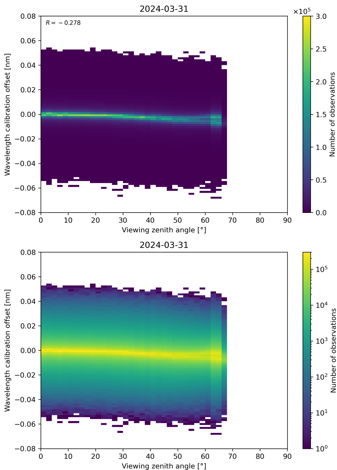
Figure 173: Scatter density plot of “Viewing zenith angle” against “Wavelength calibration offset” for 2024-03-31 to 2024-04-01.
