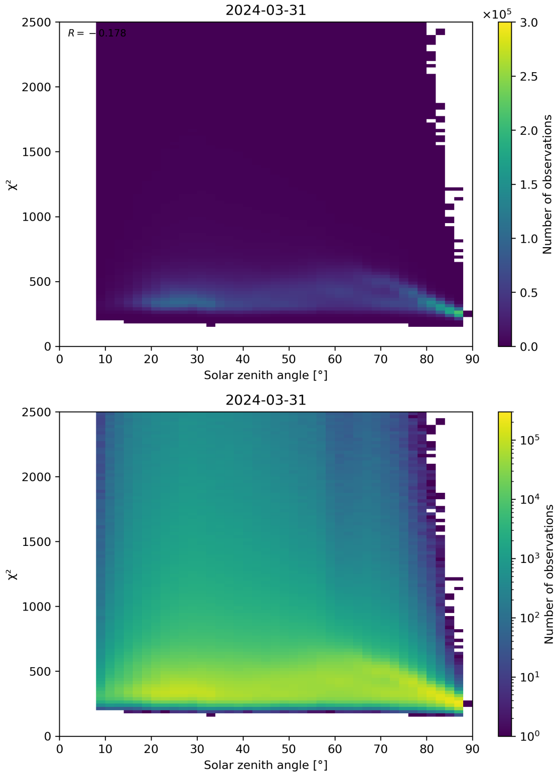
Figure 148: Scatter density plot of “Solar zenith angle” against “ \chi^2 ” for 2024-03-31 to 2024-04-01.
