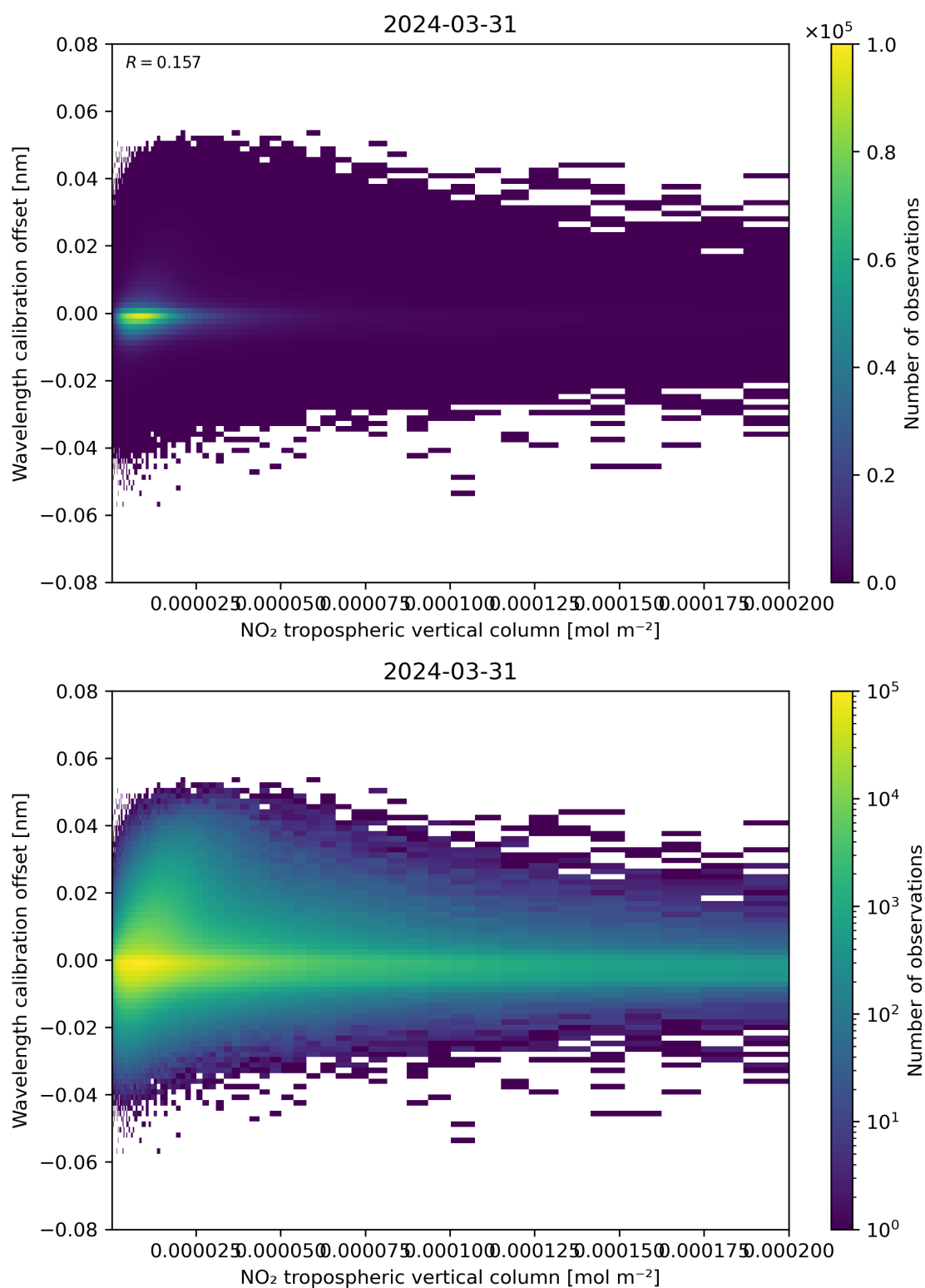
Figure 143: Scatter density plot of “NO 2 tropospheric vertical column” against “Wavelength calibration offset” for 2024-03-31 to 2024-04-01.
