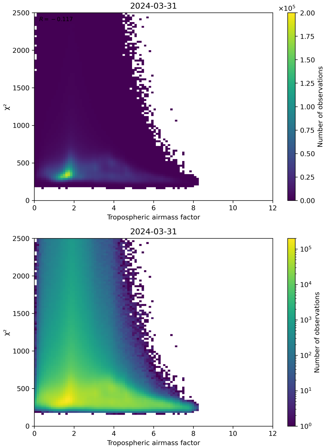
Figure 73: Scatter density plot of "Tropospheric airmass factor" against " \chi^2 " for 2024-03-31 to 2024-04-01.
