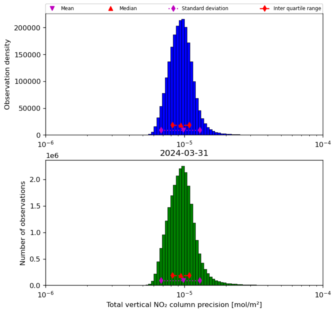
Figure 39: Histogram of "Total vertical NO 2 column precision" for 2024-03-31 to 2024-04-01
