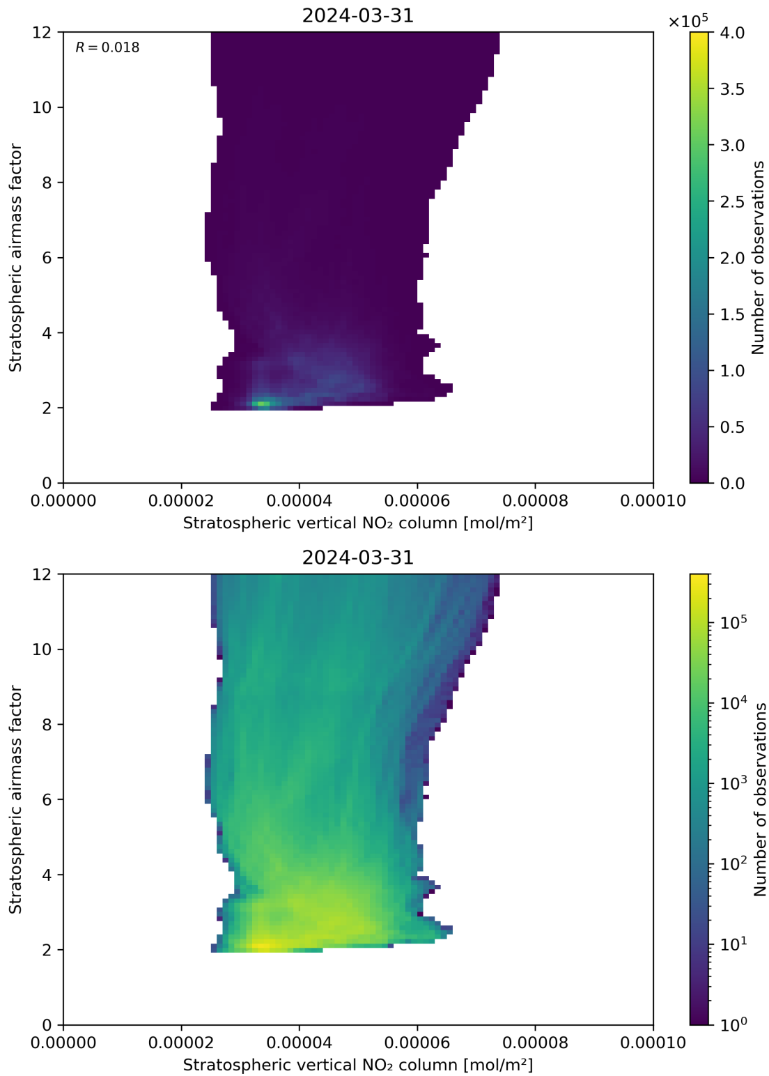
Figure 96: Scatter density plot of “Stratospheric vertical NO 2 column” against “Stratospheric airmass factor” for 2024-03-31 to 2024-04-01.
