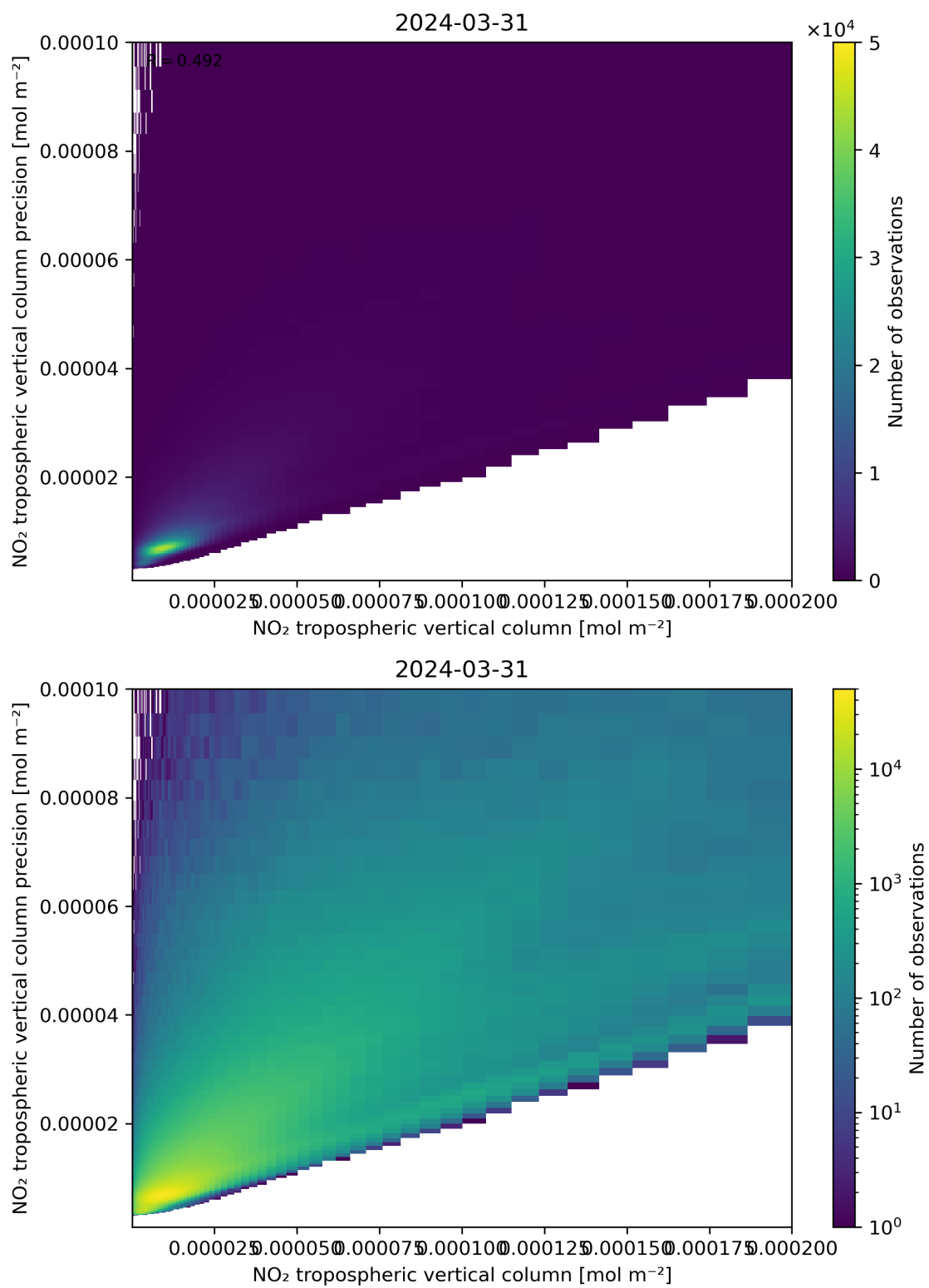
Figure 130: Scatter density plot of “NO 2 tropospheric vertical column” against “NO 2 tropospheric vertical column precision” for 2024-03-31 to 2024-04-01.
