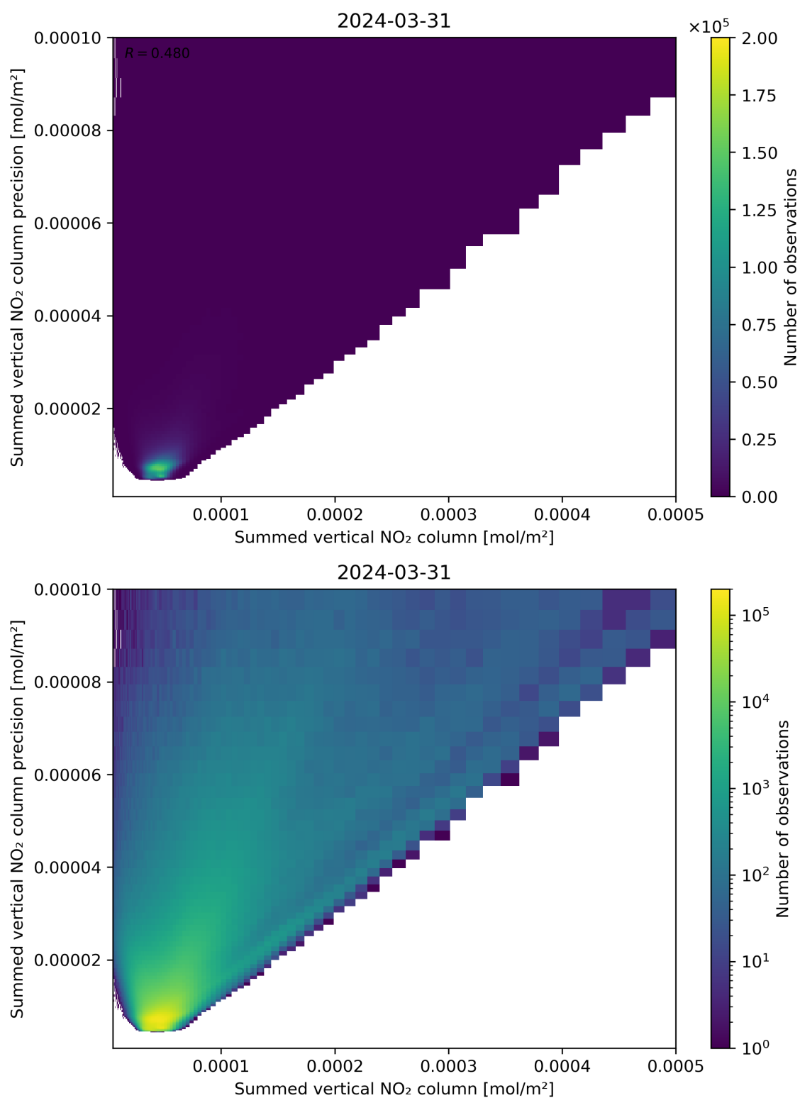
Figure 105: Scatter density plot of “Summed vertical NO 2 column” against “Summed vertical NO 2 column precision” for 2024-03-31 to 2024-04-01.
