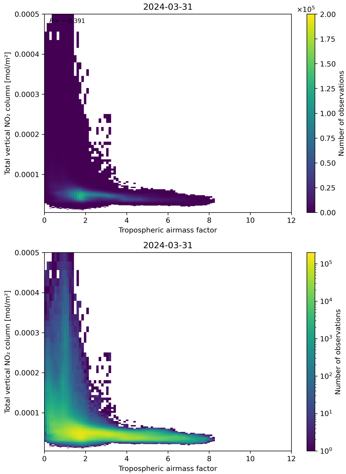
Figure 77: Scatter density plot of “Tropospheric airmass factor” against “Total vertical NO 2 column” for 2024-03-31 to 2024-04-01.
