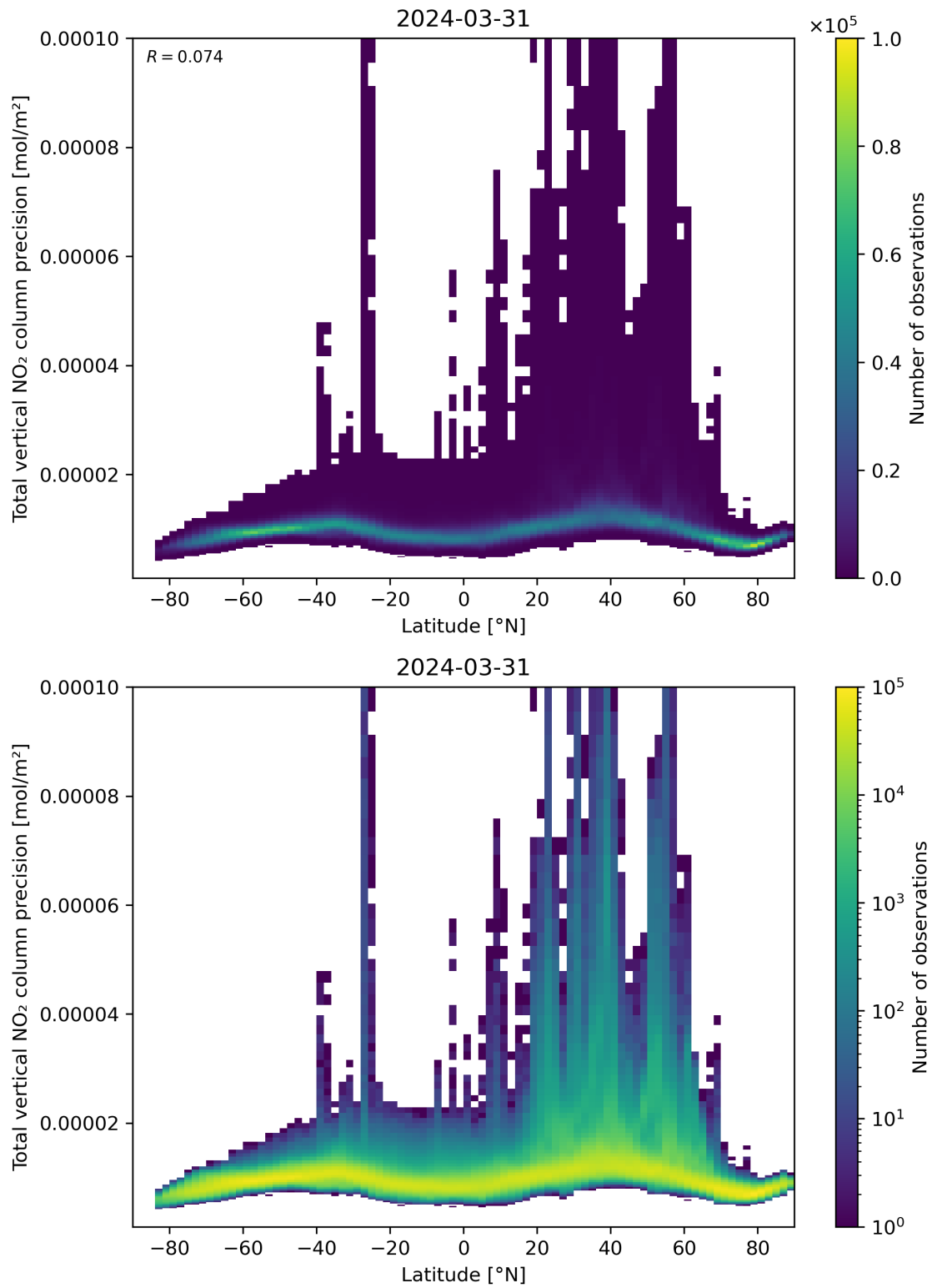
Figure 91: Scatter density plot of “Latitude” against “Total vertical NO 2 column precision” for 2024-03-31 to 2024-04-01.
