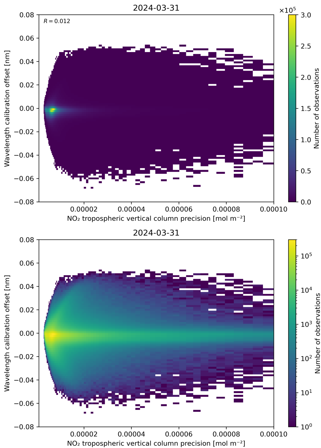
Figure 141: Scatter density plot of “NO 2 tropospheric vertical column precision” against “Wavelength calibration offset” for 2024-03-31 to 2024-04-01.
