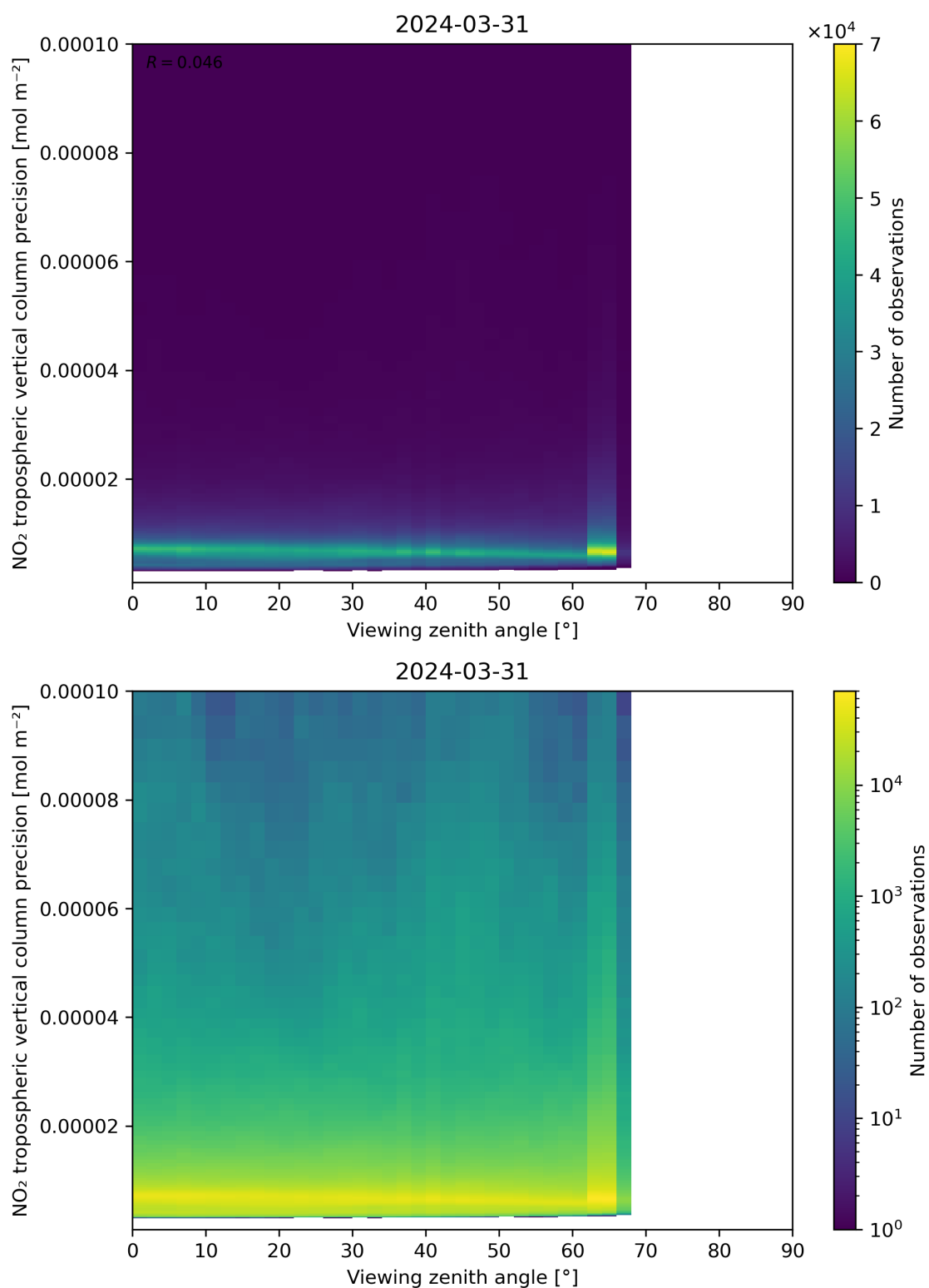
Figure 170: Scatter density plot of “Viewing zenith angle” against “NO 2 tropospheric vertical column precision” for 2024-03-31 to 2024-04-01.
