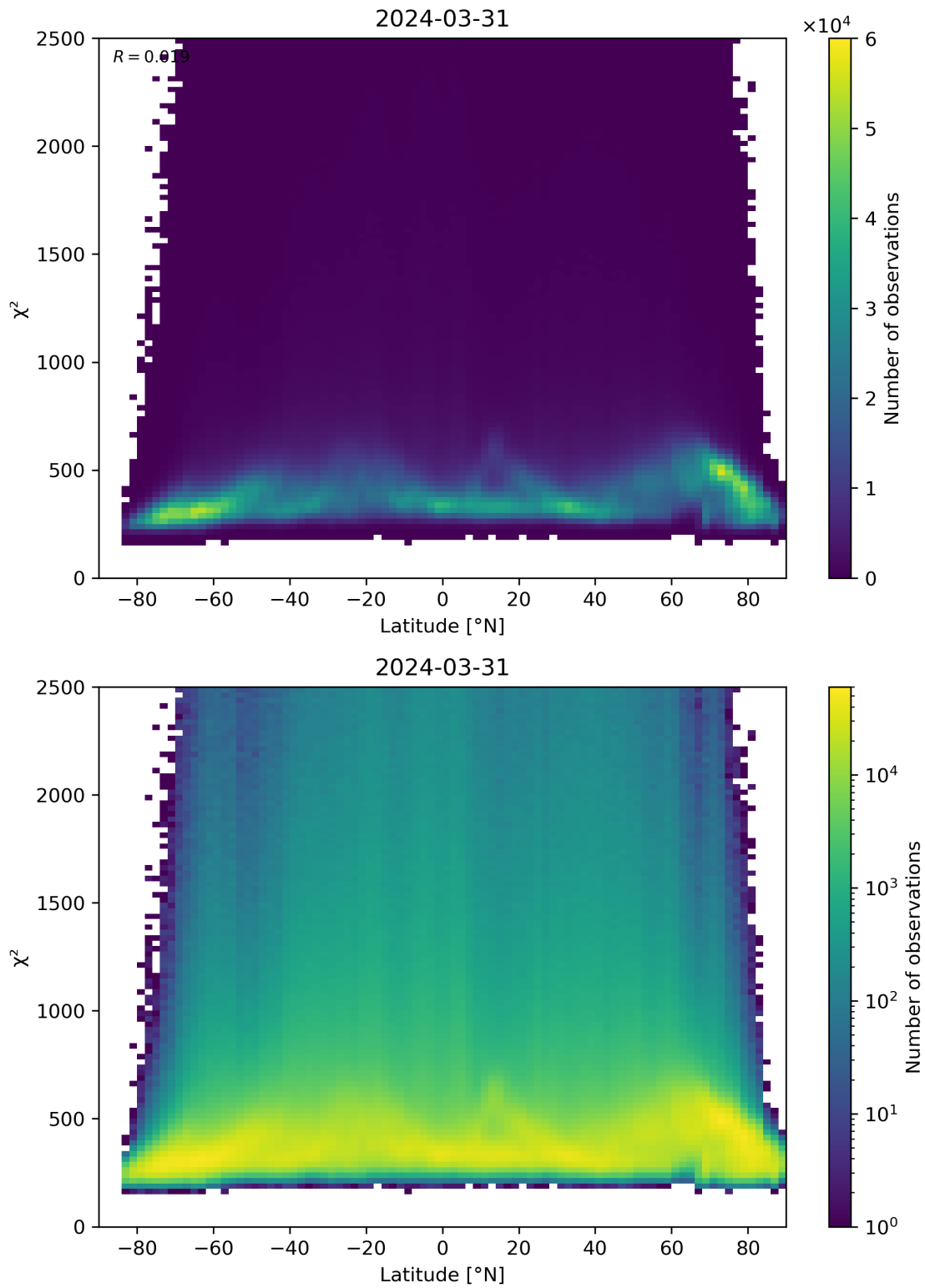
Figure 86: Scatter density plot of “Latitude” against “ \chi^2 ” for 2024-03-31 to 2024-04-01.
