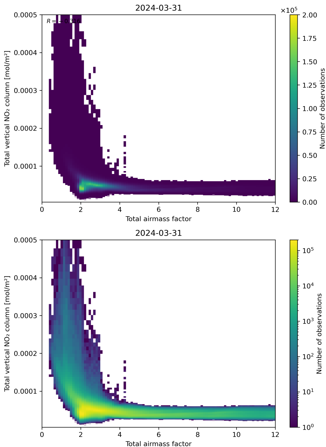
Figure 67: Scatter density plot of “Total airmass factor” against “Total vertical NO 2 column” for 2024-03-31 to 2024-04-01.
