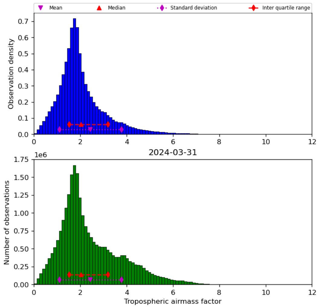
Figure 31: Histogram of “Tropospheric airmass factor” for 2024-03-31 to 2024-04-01
