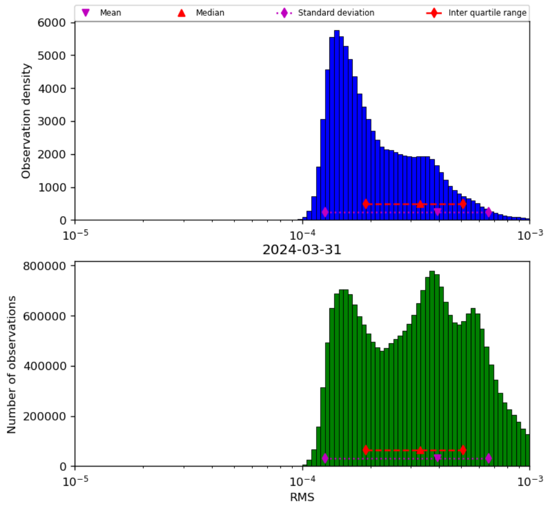
Figure 43: Histogram of “RMS” for 2024-03-31 to 2024-04-01
