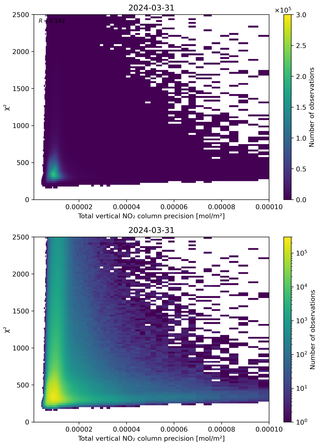
Figure 116: Scatter density plot of “Total vertical NO 2 column precision” against “ \chi^2 ” for 2024-03-31 to 2024-04-01.
