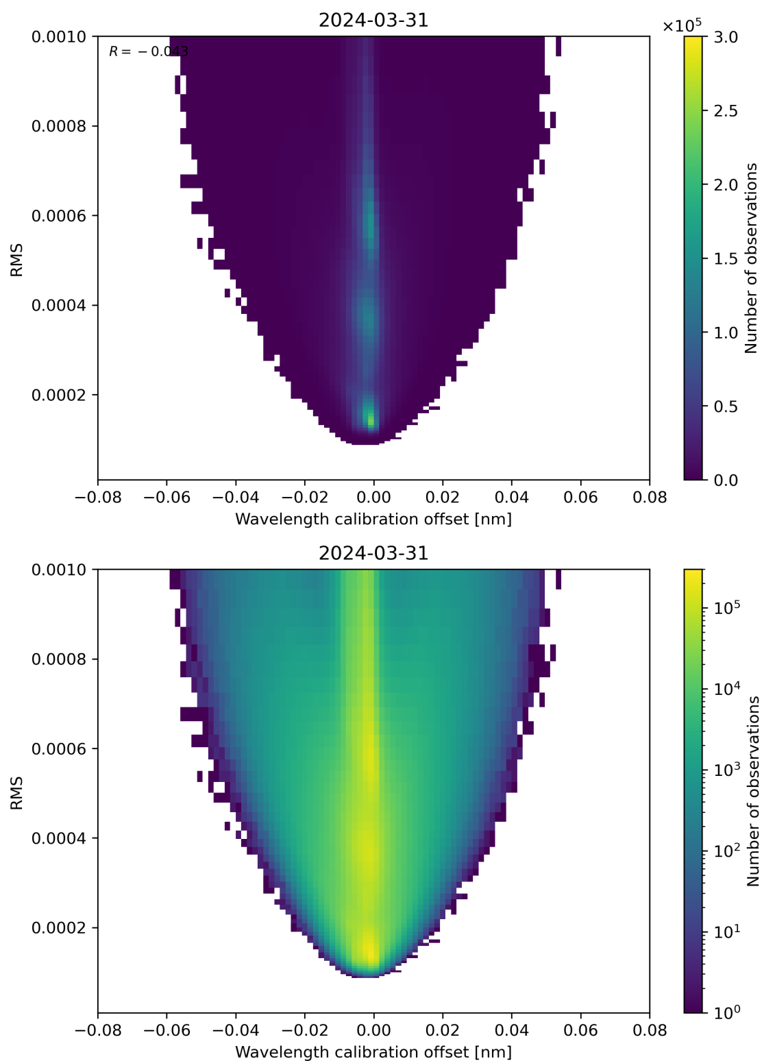
Figure 181: Scatter density plot of “Wavelength calibration offset” against “RMS” for 2024-03-31 to 2024-04-01.
