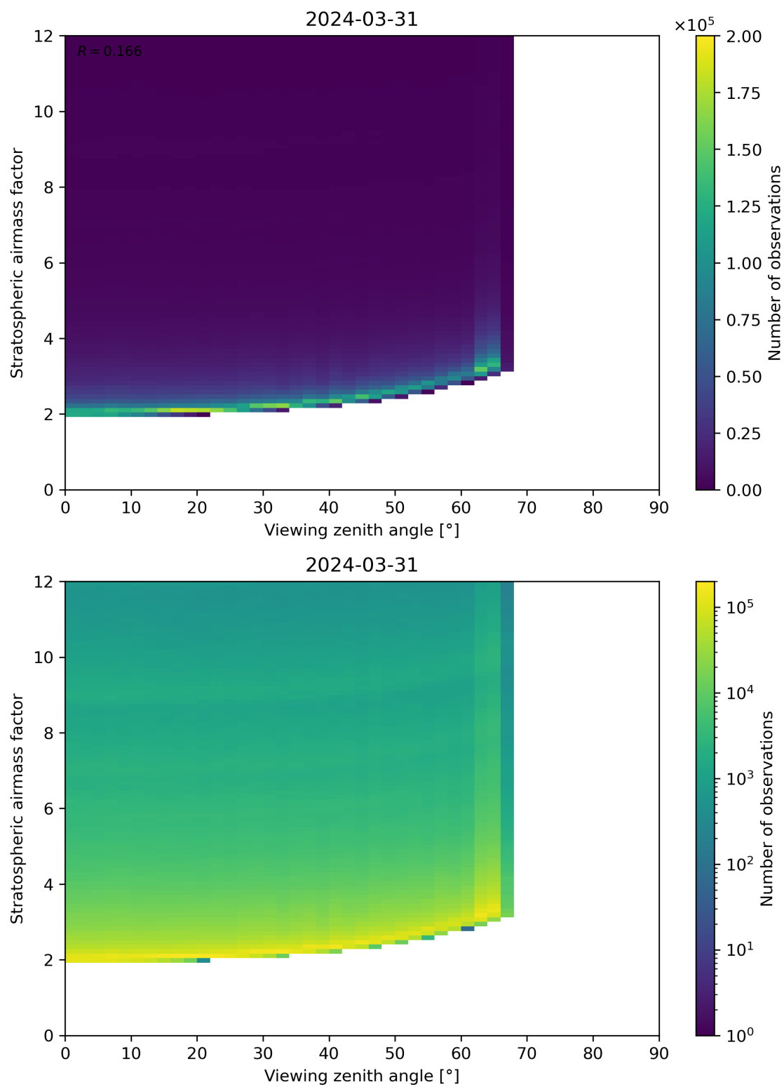
Figure 159: Scatter density plot of “Viewing zenith angle” against “Stratospheric airmass factor” for 2024-03-31 to 2024-04-01.
