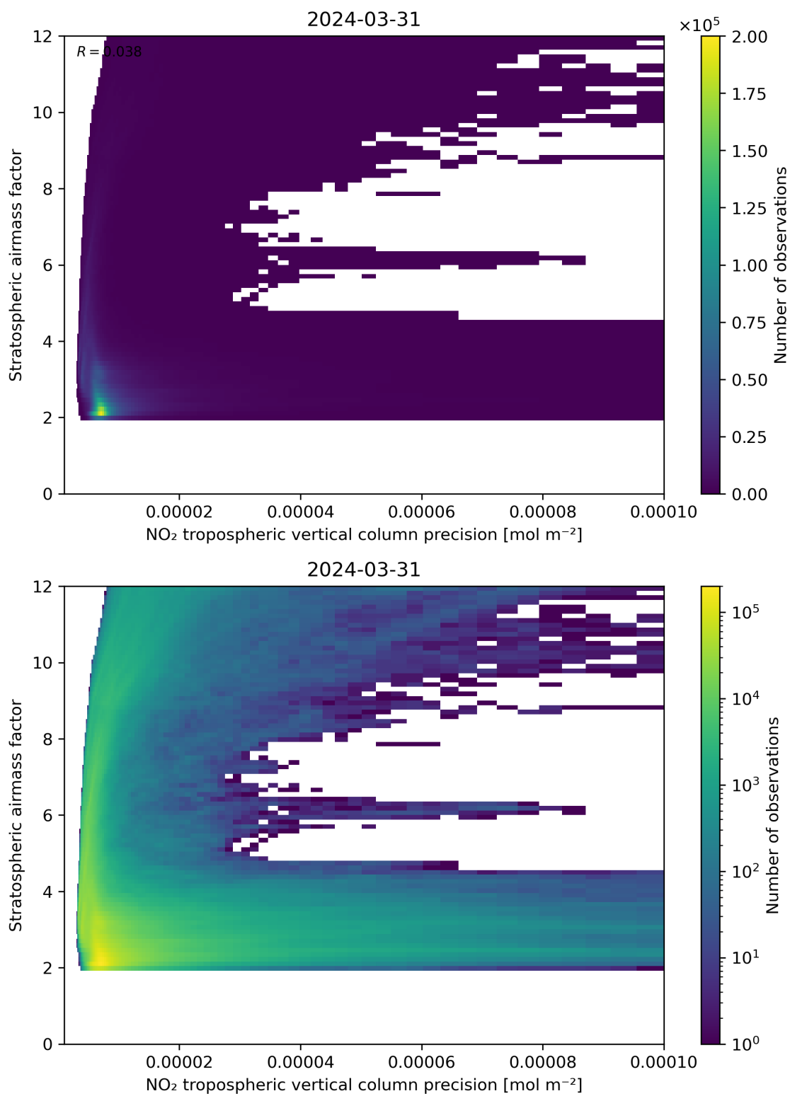
Figure 131: Scatter density plot of “NO 2 tropospheric vertical column precision” against “Stratospheric airmass factor” for 2024-03-31 to 2024-04-01.
