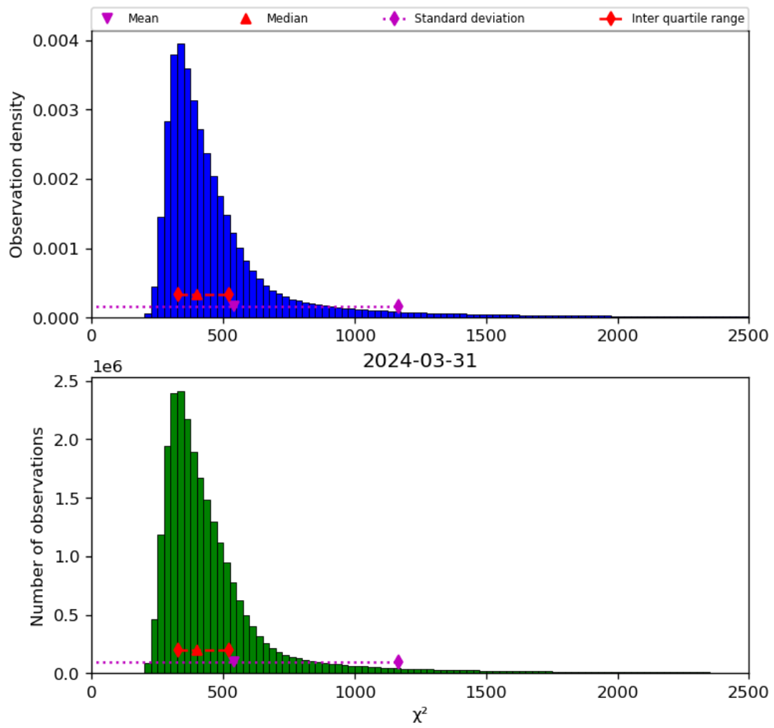
Figure 42: Histogram of “ \chi^2 ” for 2024-03-31 to 2024-04-01
