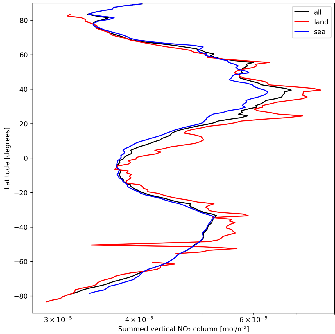
Figure 23: Zonal average of “Summed vertical NO 2 column” for 2024-03-31 to 2024-04-01.
