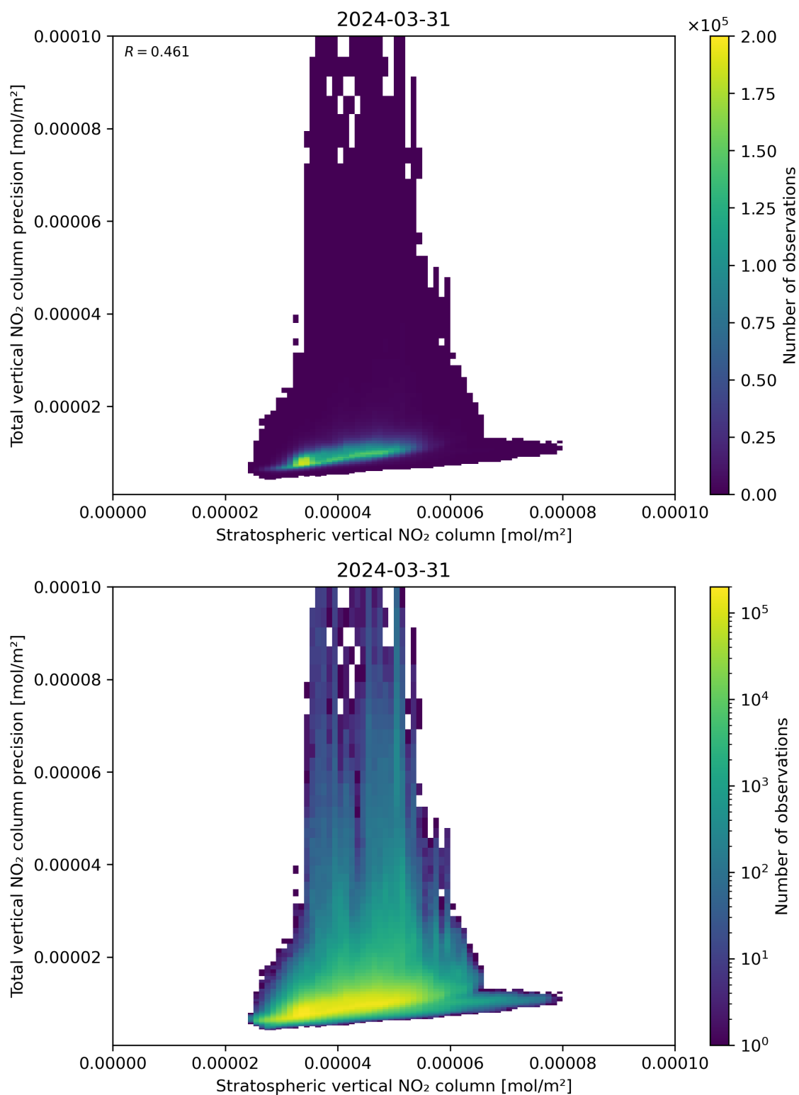
Figure 101: Scatter density plot of “Stratospheric vertical NO 2 column” against “Total vertical NO 2 column precision” for 2024-03-31 to 2024-04-01.
