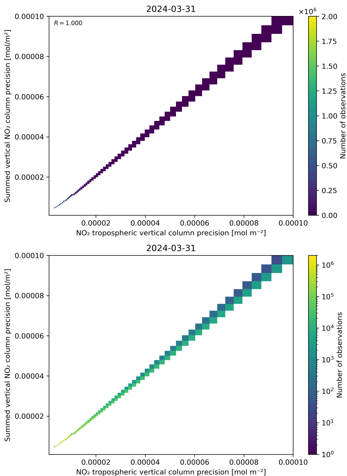
Figure 137: Scatter density plot of “NO 2 tropospheric vertical column precision” against “Summed vertical NO 2 column precision” for 2024-03-31 to 2024-04-01.
