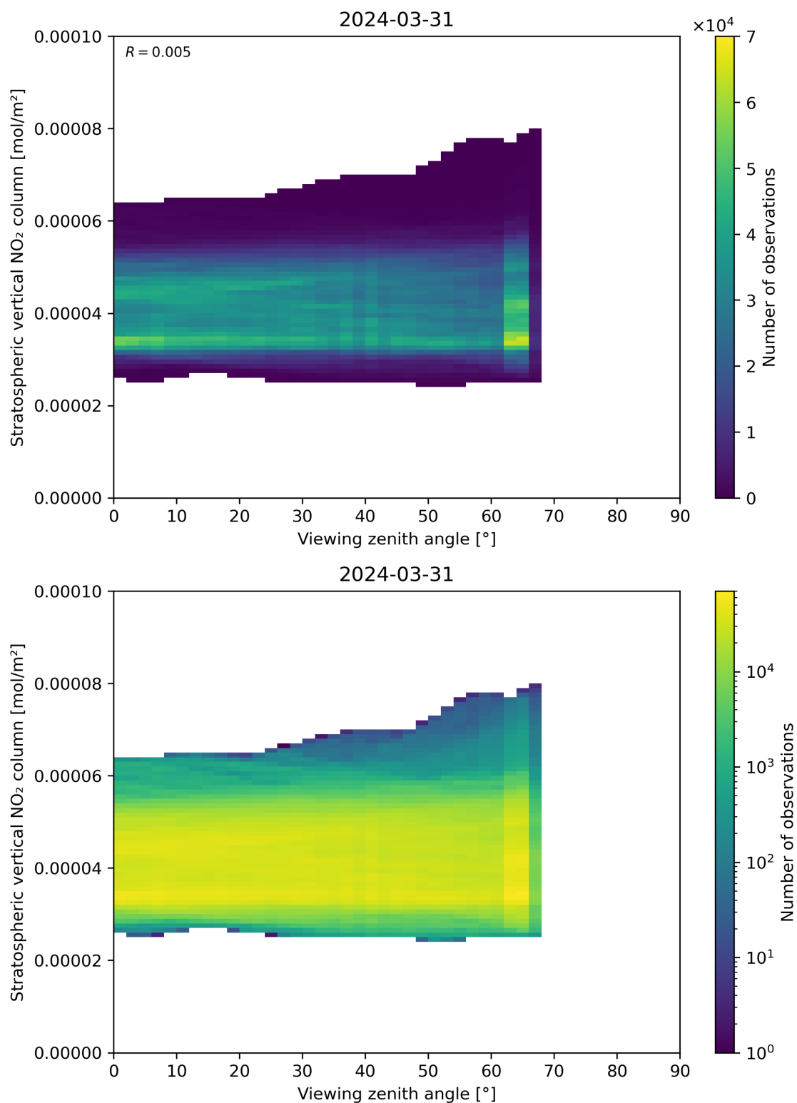
Figure 164: Scatter density plot of “Viewing zenith angle” against “Stratospheric vertical NO 2 column” for 2024-03-31 to 2024-04-01.
