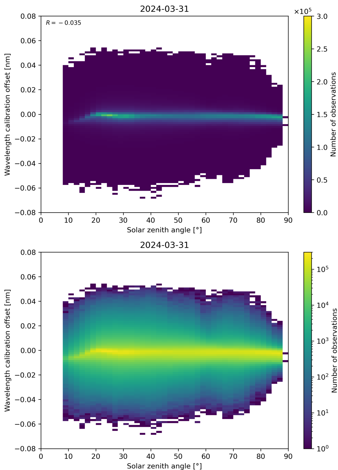
Figure 158: Scatter density plot of “Solar zenith angle” against “Wavelength calibration offset” for 2024-03-31 to 2024-04-01.
