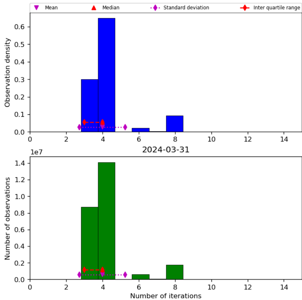
Figure 34: Histogram of “Number of iterations” for 2024-03-31 to 2024-04-01
