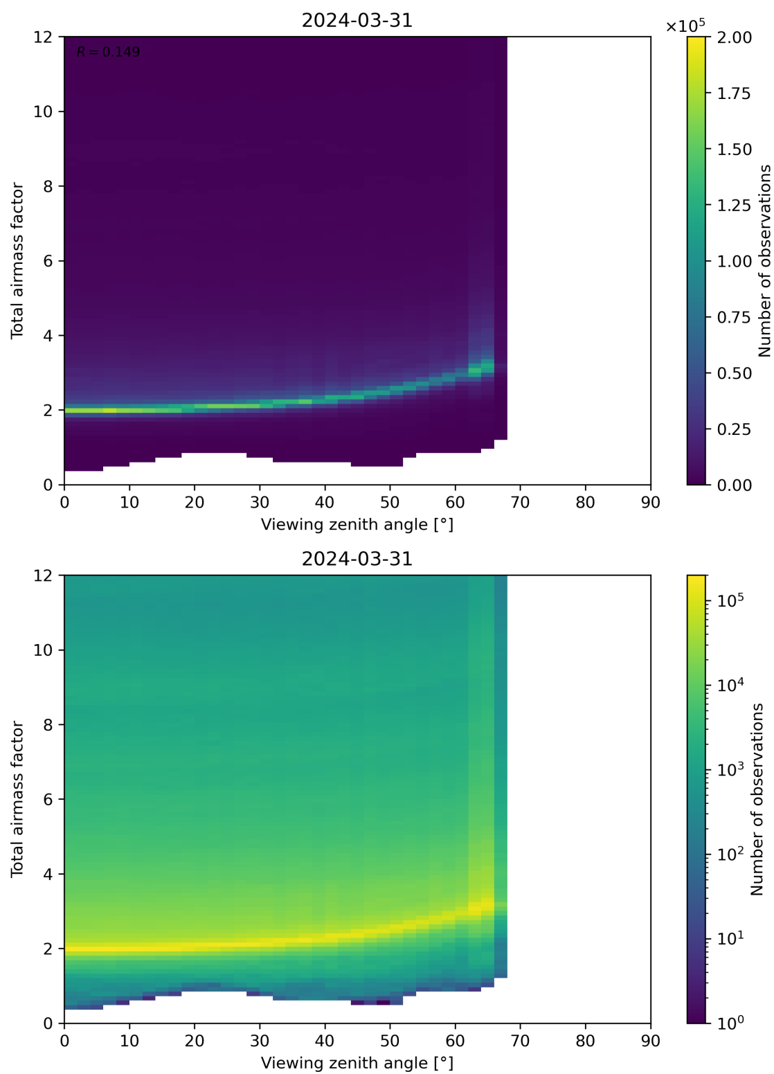
Figure 160: Scatter density plot of “Viewing zenith angle” against “Total airmass factor” for 2024-03-31 to 2024-04-01.
