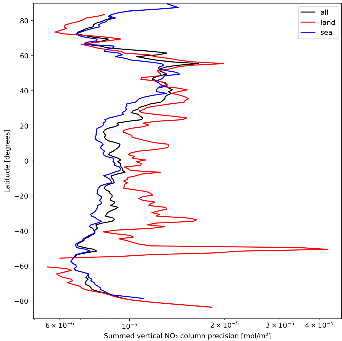
Figure 24: Zonal average of “Summed vertical NO 2 column precision” for 2024-03-31 to 2024-04-01.
