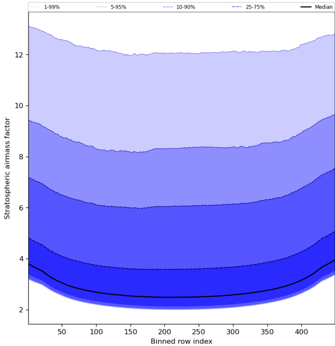
Figure 61: Along track statistics of “Stratospheric airmass factor” for 2024-03-31 to 2024-04-01
