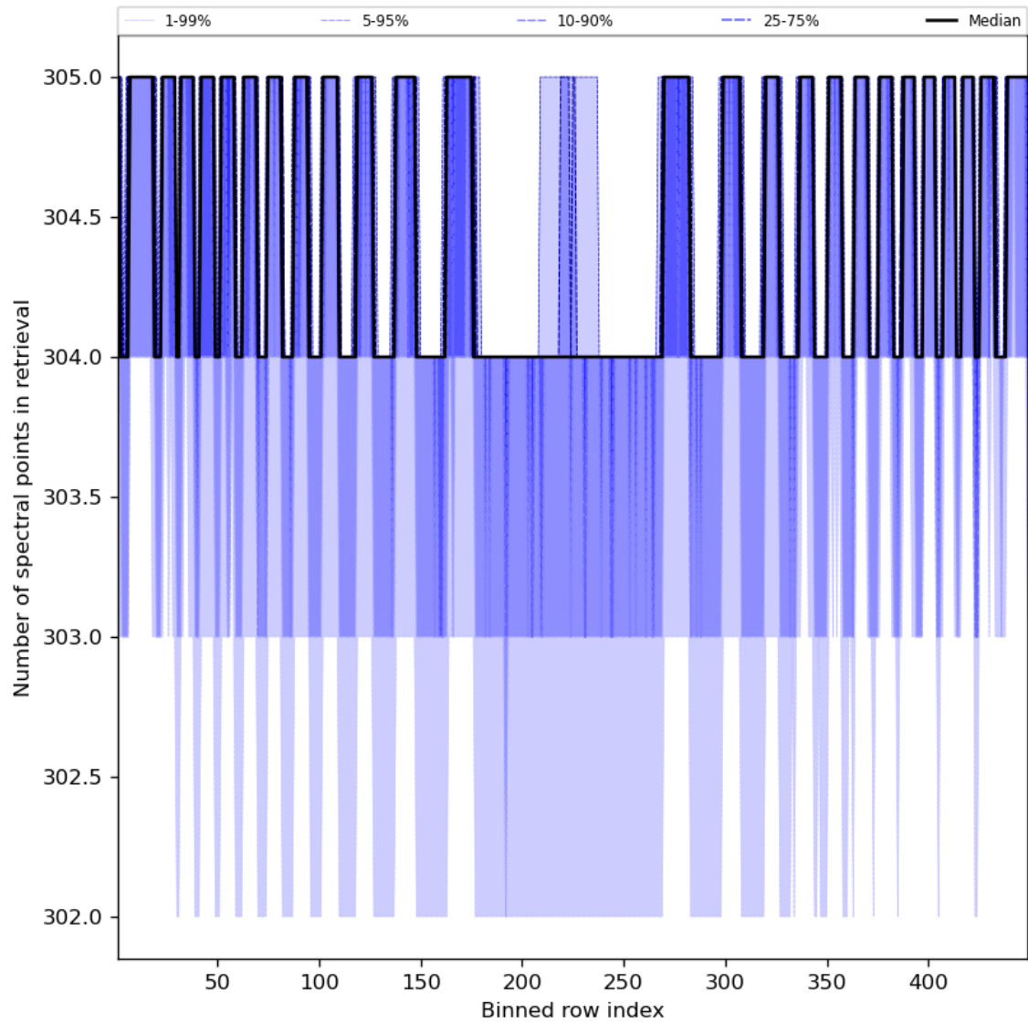
Figure 50: Along track statistics of “Number of spectral points in retrieval” for 2024-03-31 to 2024-04-01
