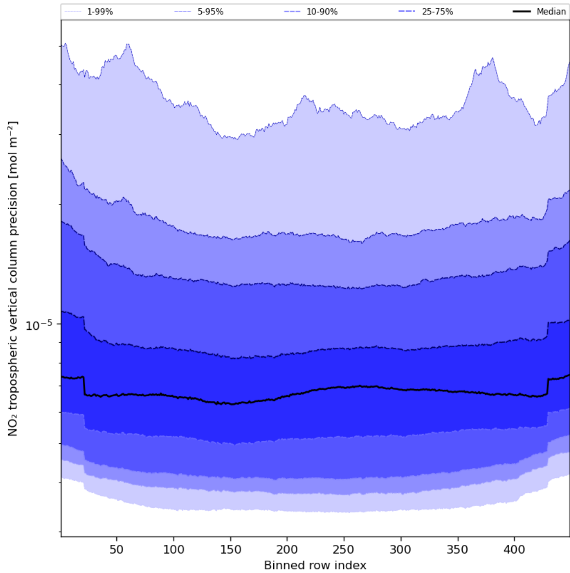
Figure 47: Along track statistics of “NO 2 tropospheric vertical column precision” for 2024-03-31 to 2024-04-01
