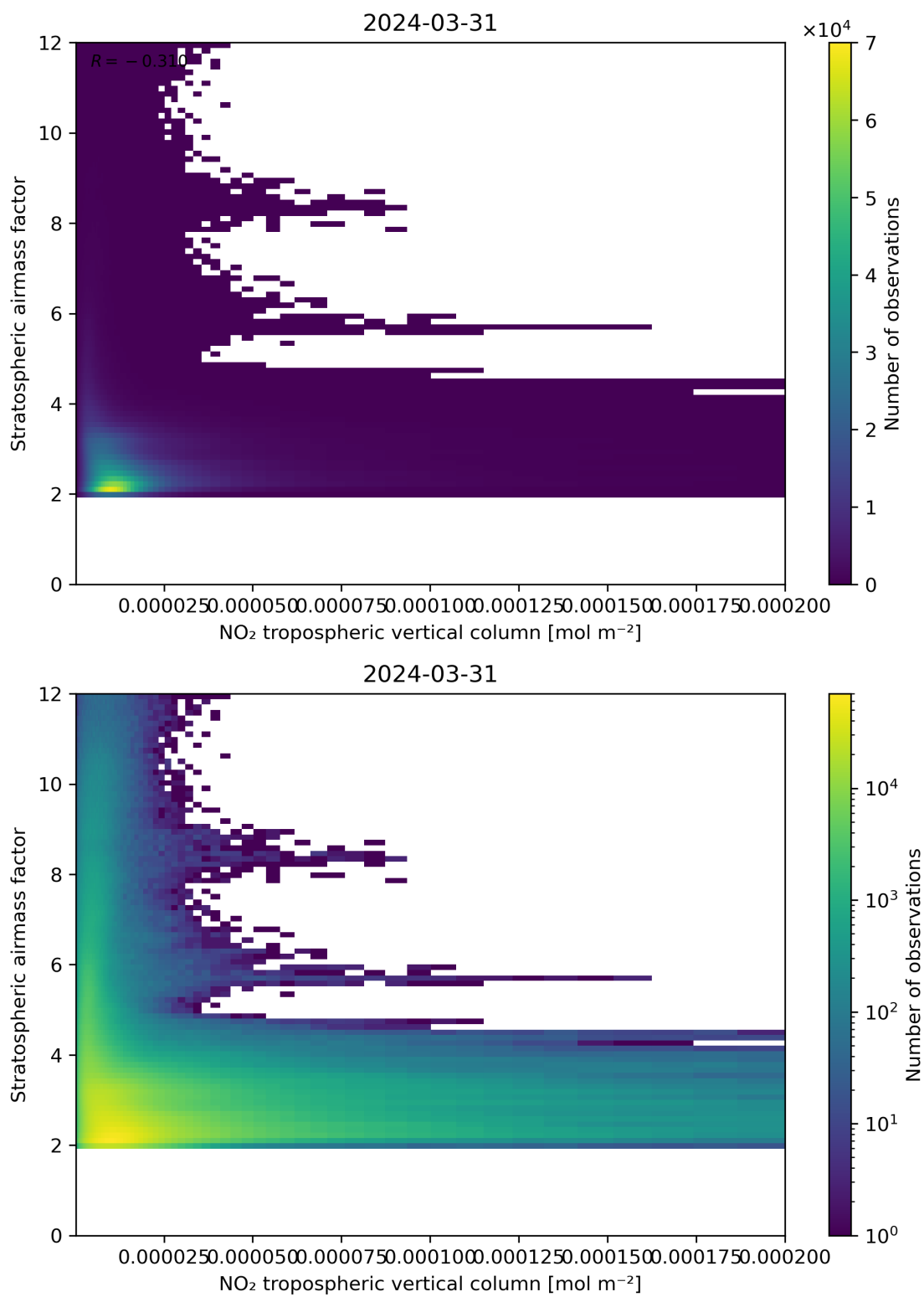
Figure 121: Scatter density plot of “NO 2 tropospheric vertical column” against “Stratospheric air mass factor” for 2024-03-31 to 2024-04-01.
