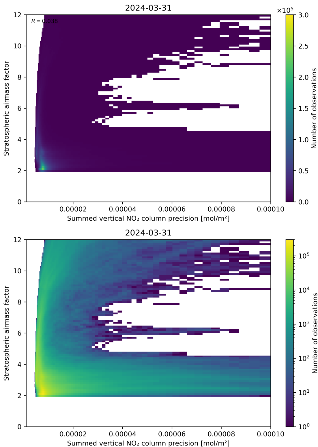
Figure 106: Scatter density plot of “Summed vertical NO 2 column precision” against “Stratospheric airmass factor” for 2024-03-31 to 2024-04-01.
