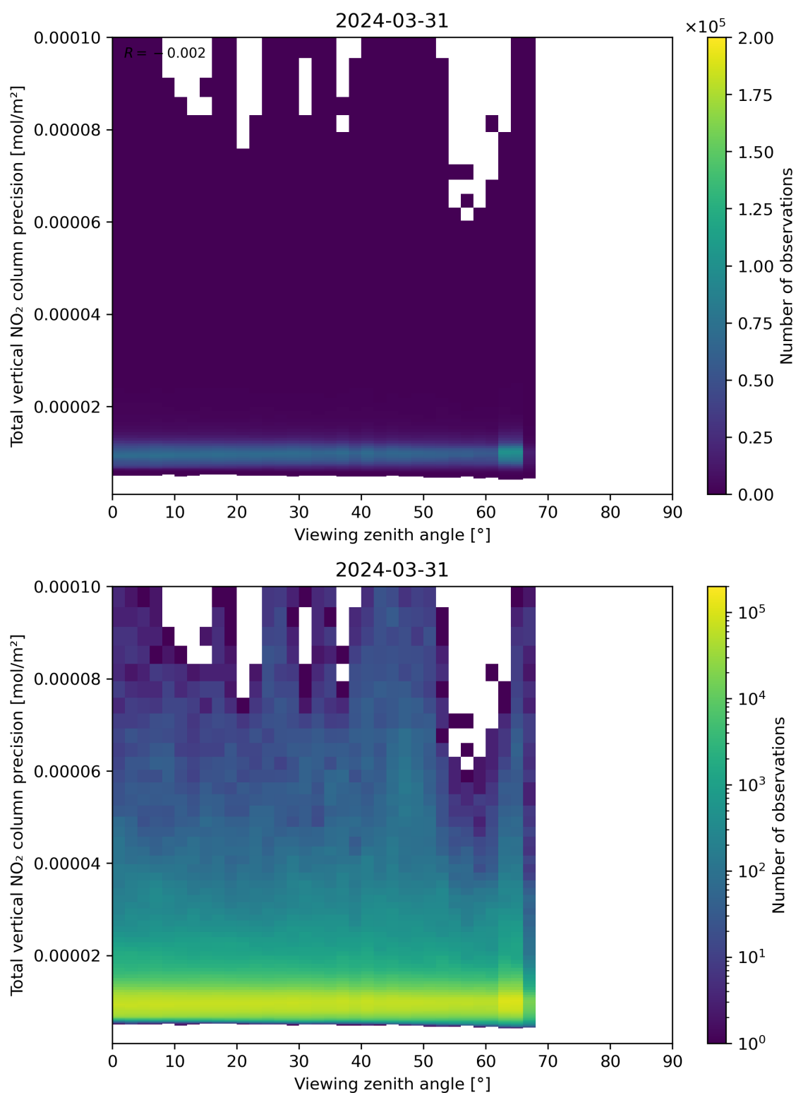
Figure 168: Scatter density plot of “Viewing zenith angle” against “Total vertical NO 2 column precision” for 2024-03-31 to 2024-04-01.
