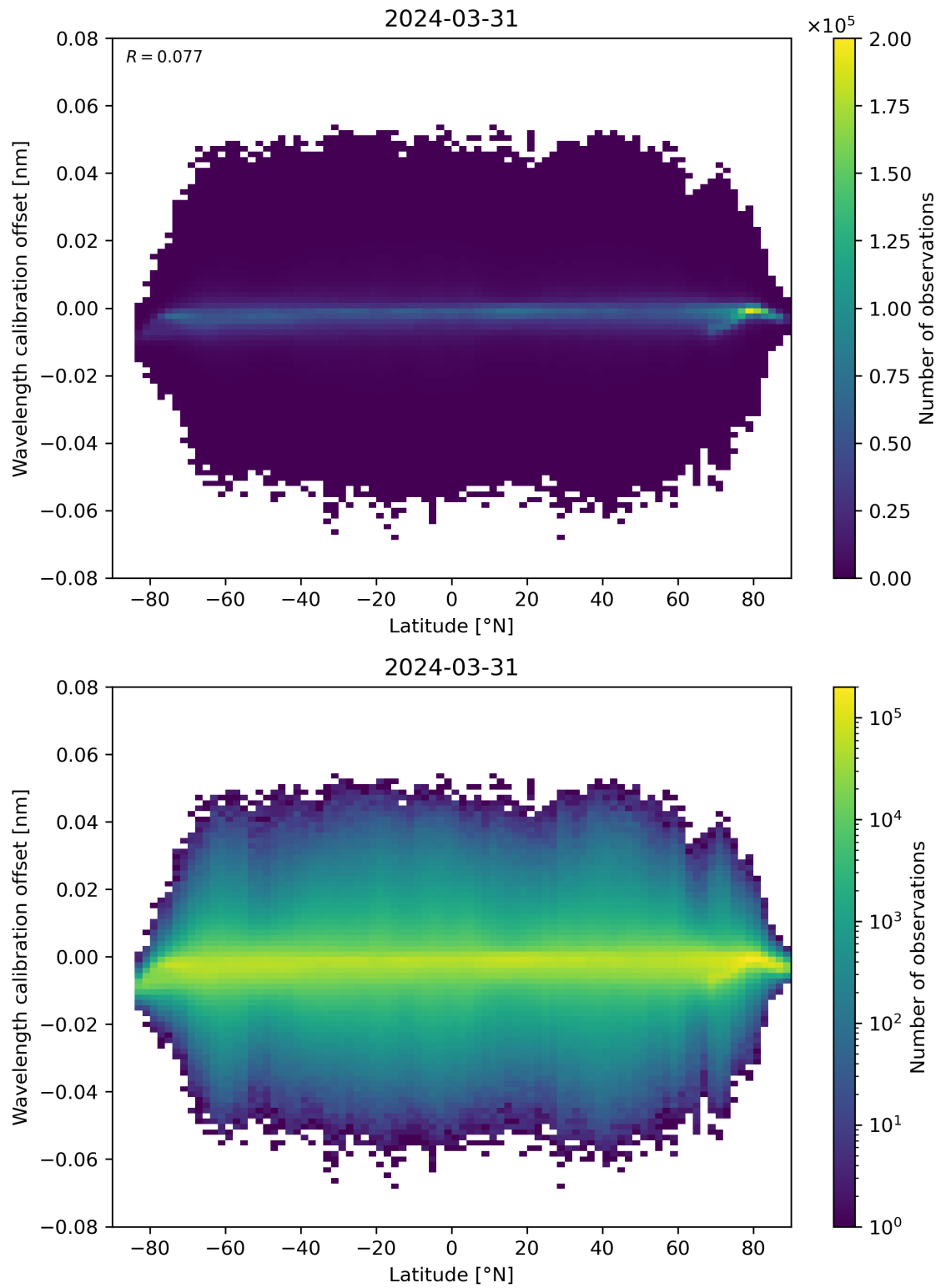
Figure 95: Scatter density plot of “Latitude” against “Wavelength calibration offset” for 2024-03-31 to 2024-04-01.
