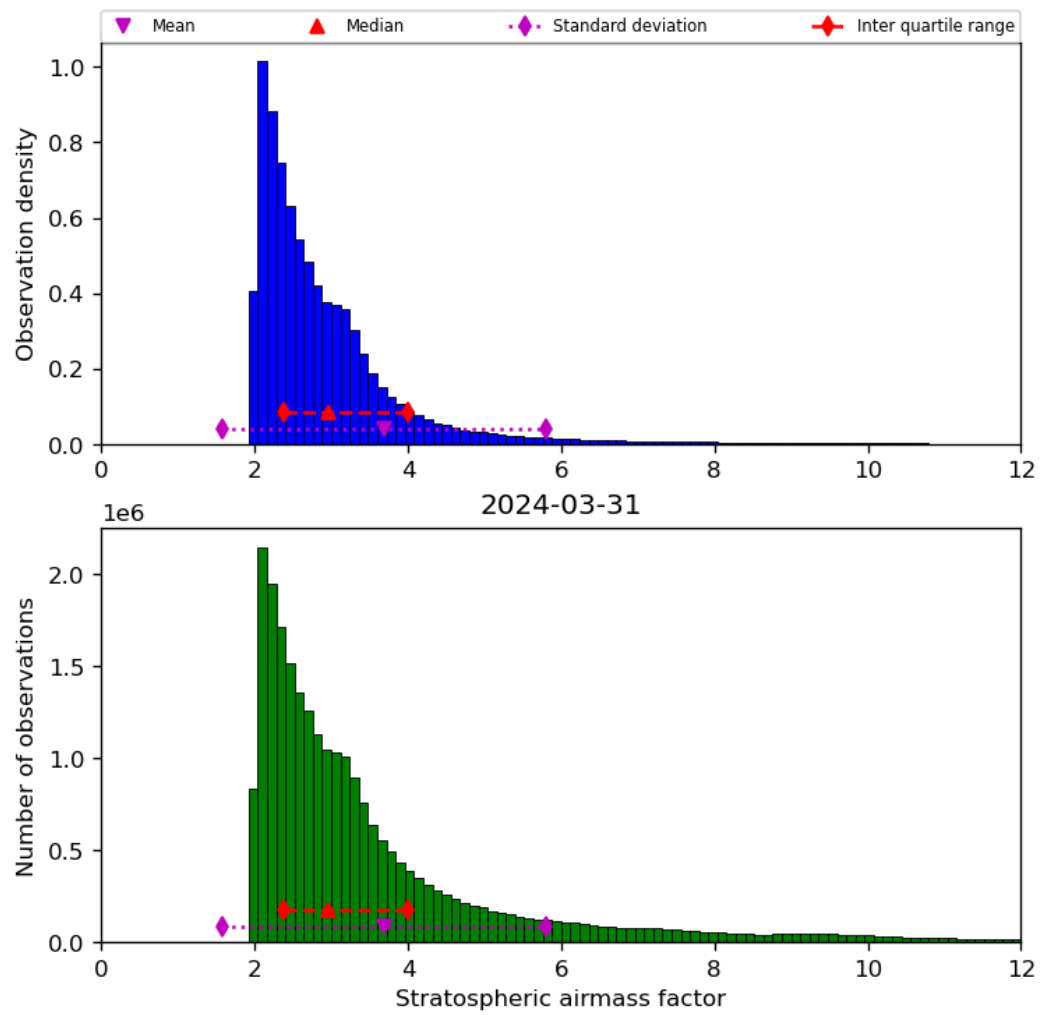
Figure 44: Histogram of “Stratospheric airmass factor” for 2024-03-31 to 2024-04-01
