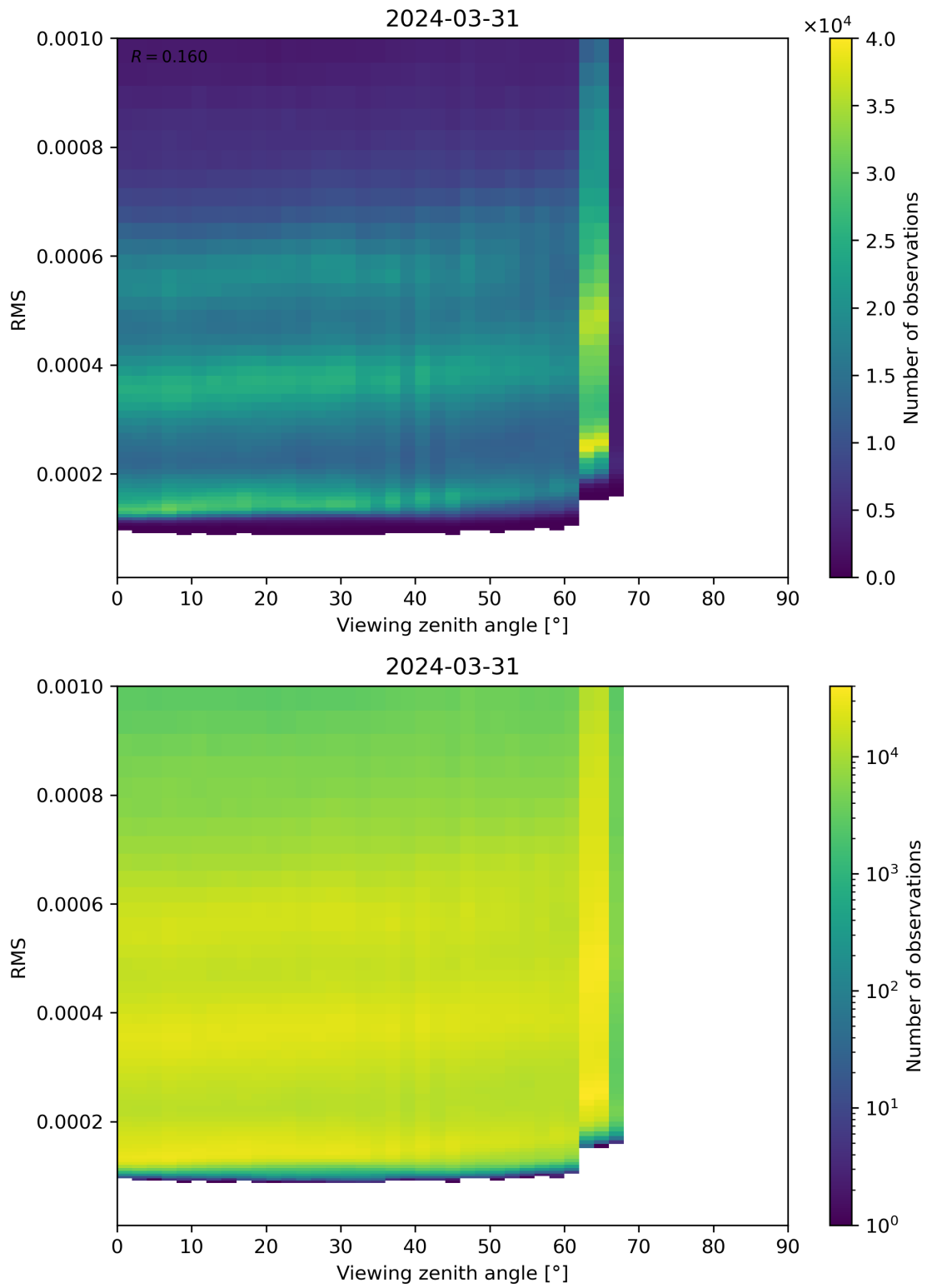
Figure 171: Scatter density plot of “Viewing zenith angle” against “RMS” for 2024-03-31 to 2024-04-01.
