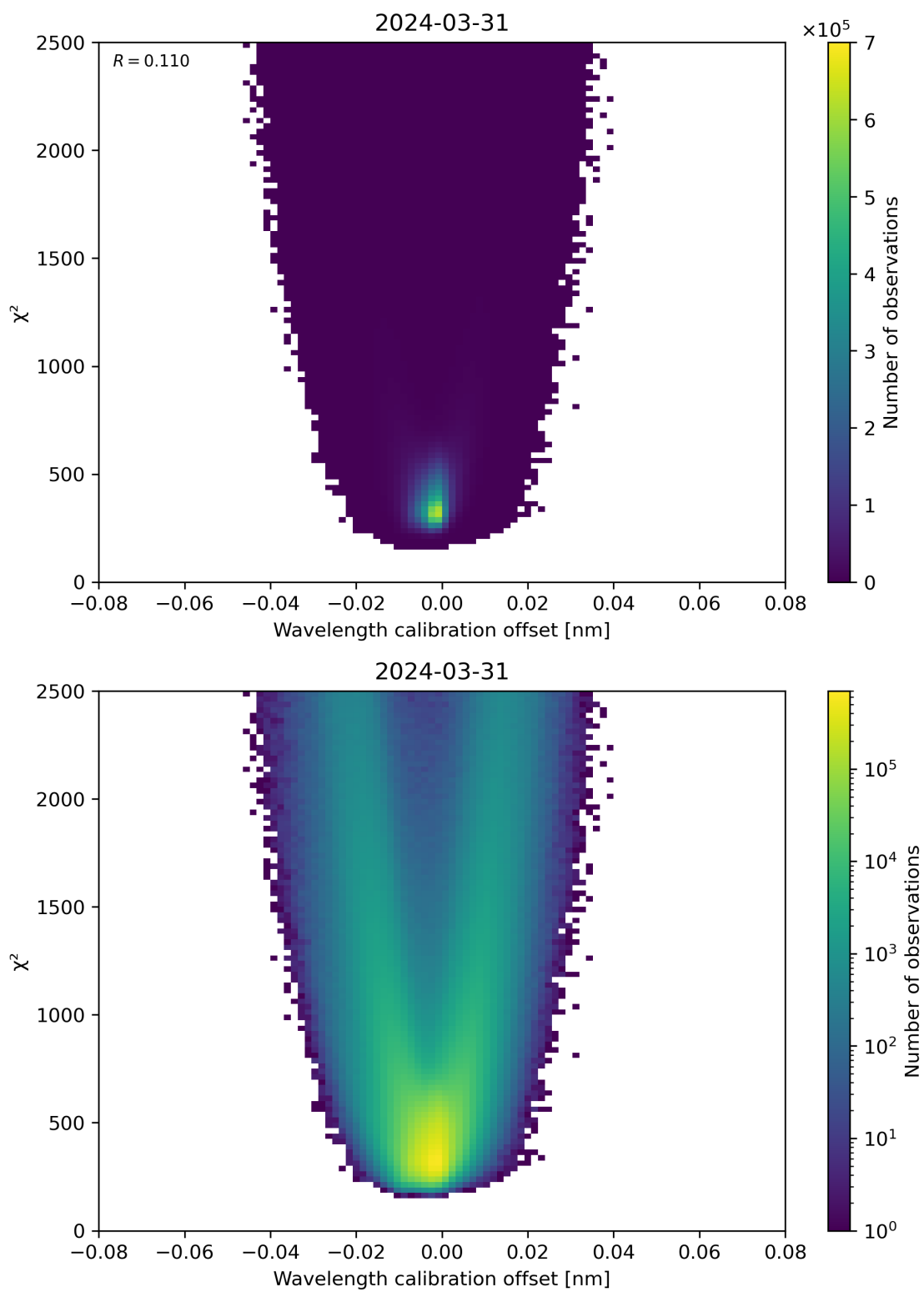
Figure 175: Scatter density plot of “Wavelength calibration offset” against “ \chi^2 ” for 2024-03-31 to 2024-04-01.
