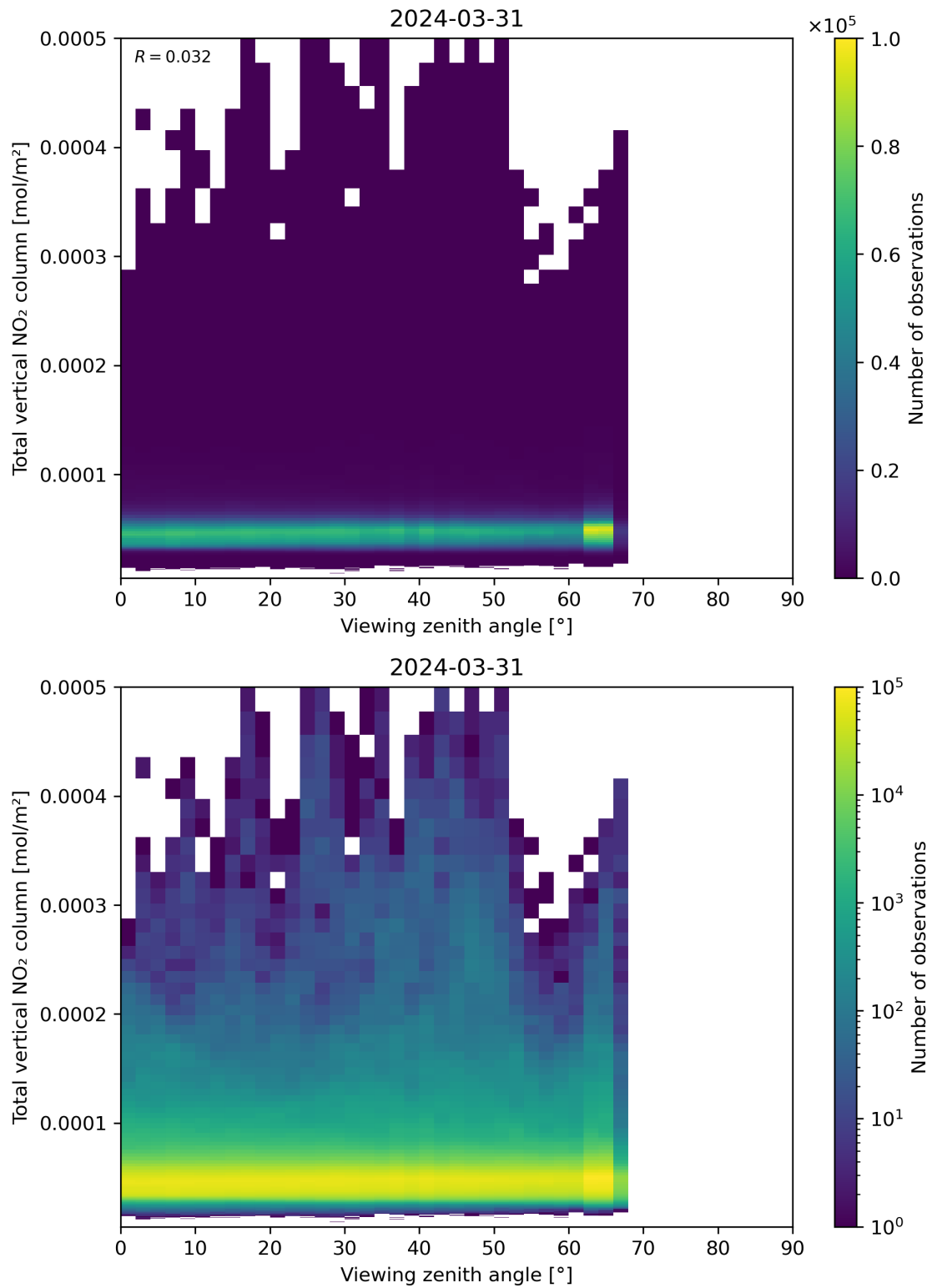
Figure 167: Scatter density plot of “Viewing zenith angle” against “Total vertical NO 2 column” for 2024-03-31 to 2024-04-01.
