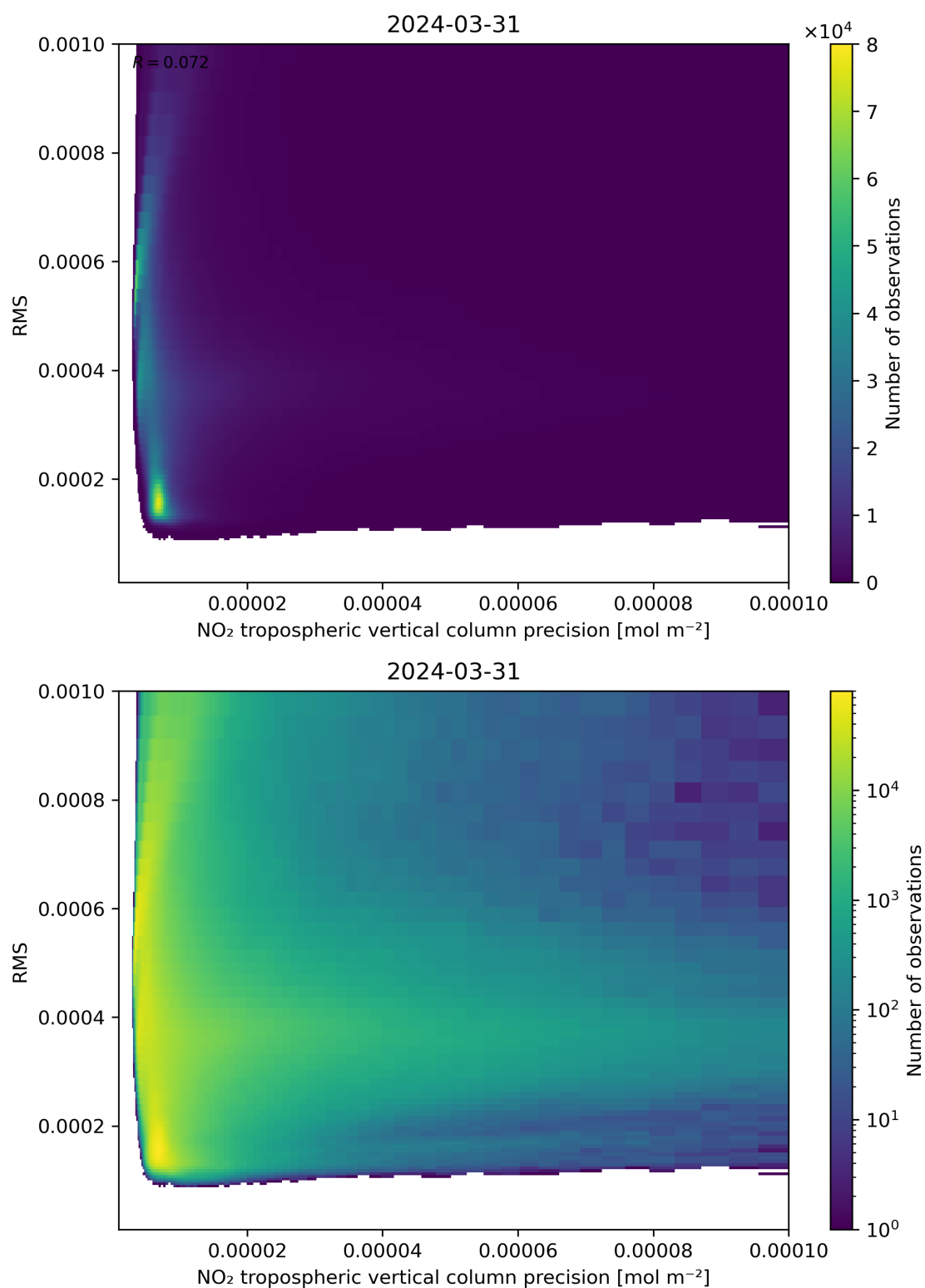
Figure 140: Scatter density plot of “NO 2 tropospheric vertical column precision” against “RMS” for 2024-03-31 to 2024-04-01.
