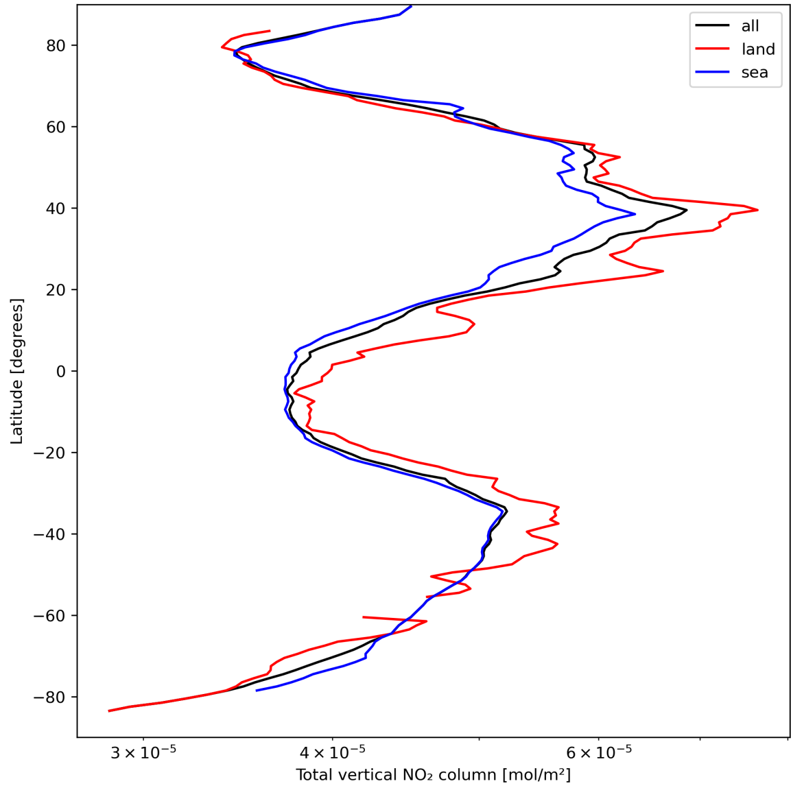
Figure 21: Zonal average of “Total vertical NO 2 column” for 2024-03-31 to 2024-04-01.
