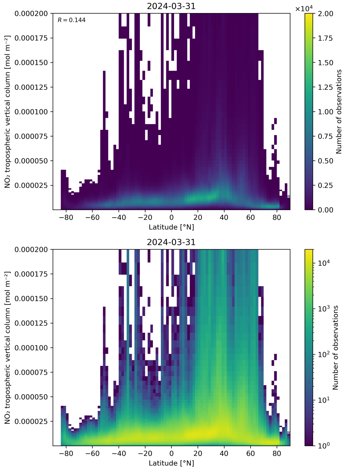
Figure 92: Scatter density plot of “Latitude” against “NO 2 tropospheric vertical column” for 2024-03-31 to 2024-04-01.
