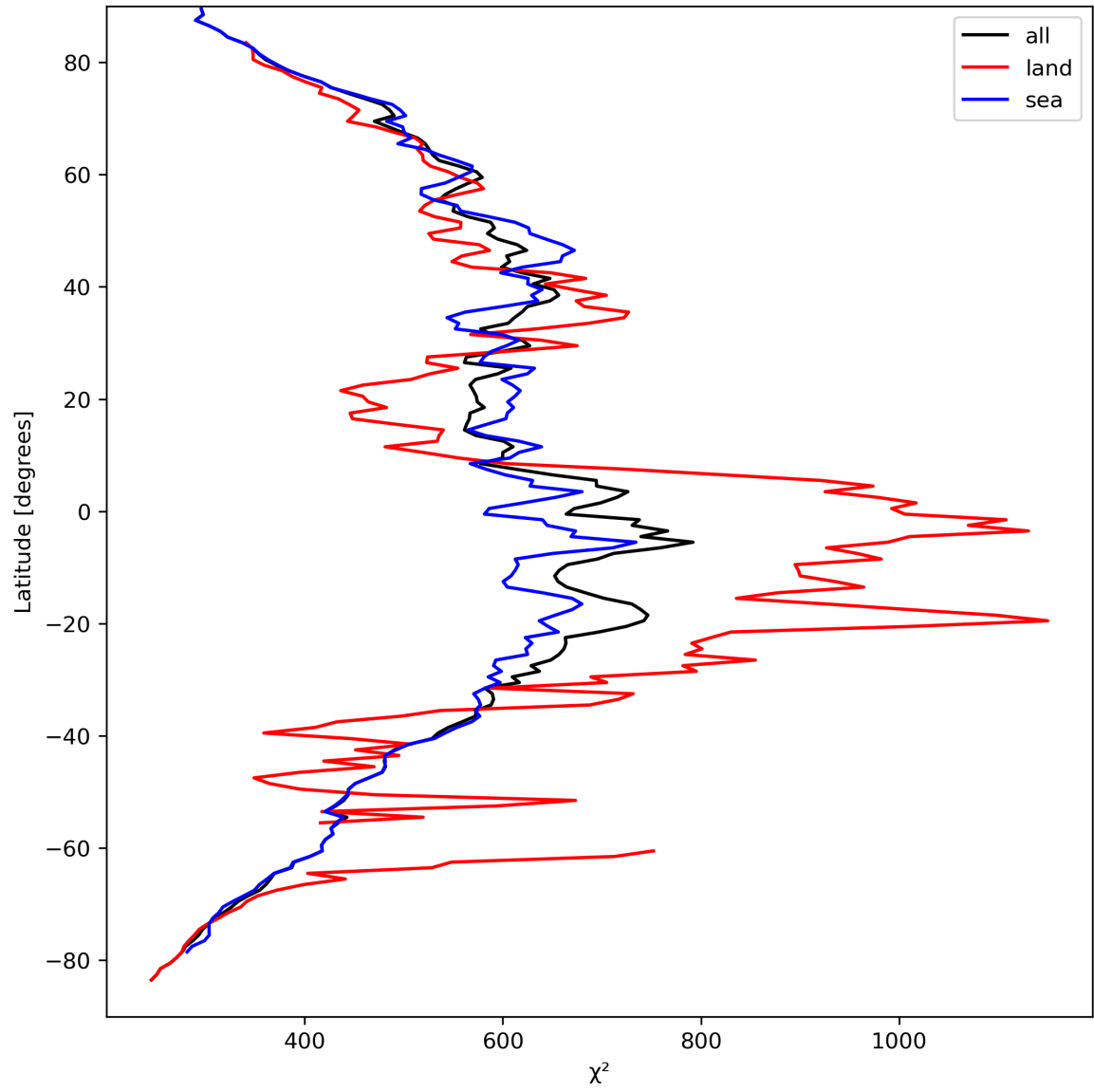
Figure 25: Zonal average of “ \chi^2 ” for 2024-03-31 to 2024-04-01.
