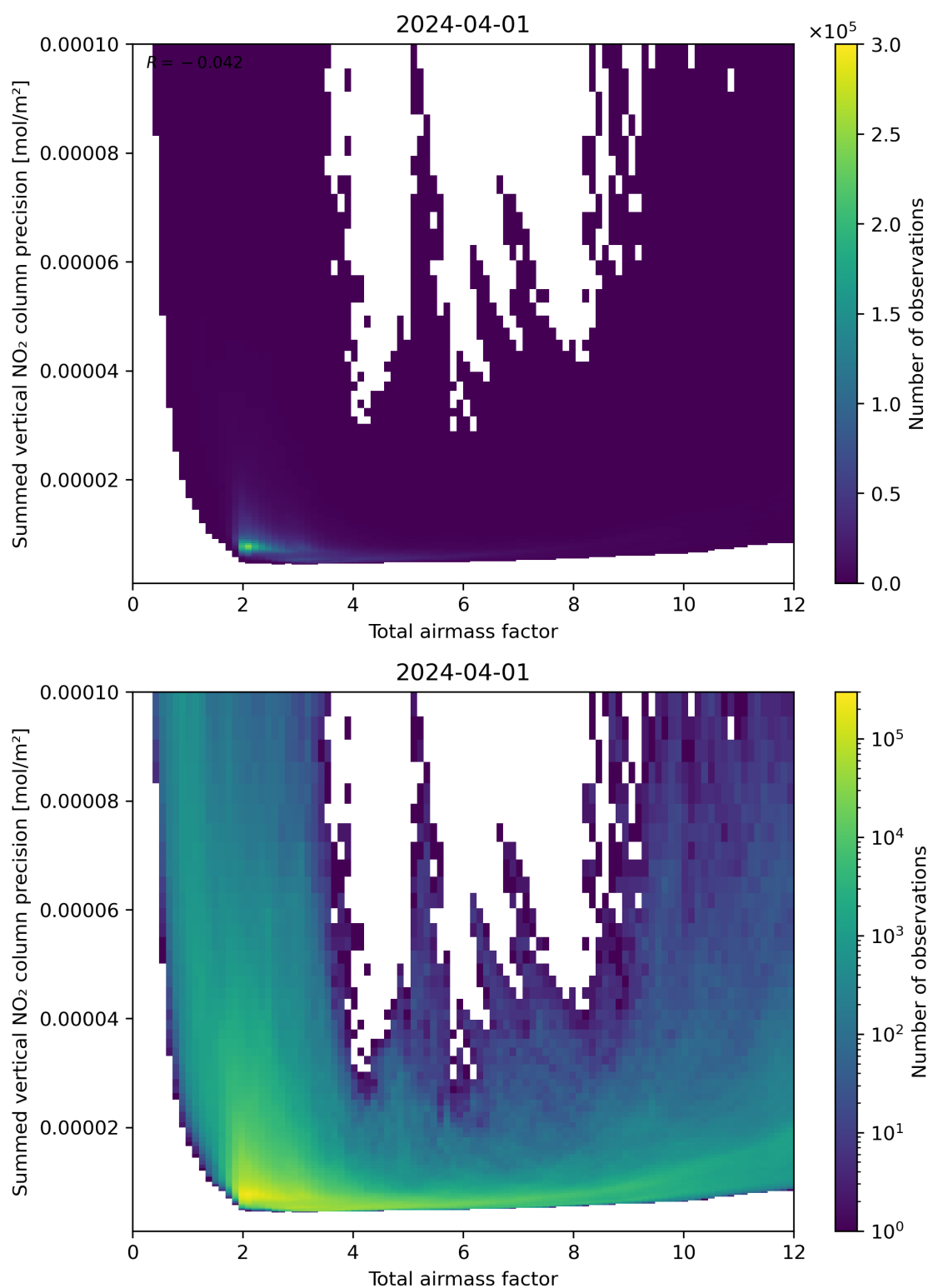
Figure 66: Scatter density plot of “Total airmass factor” against “Summed vertical NO 2 column precision” for 2024-03-31 to 2024-04-02.
