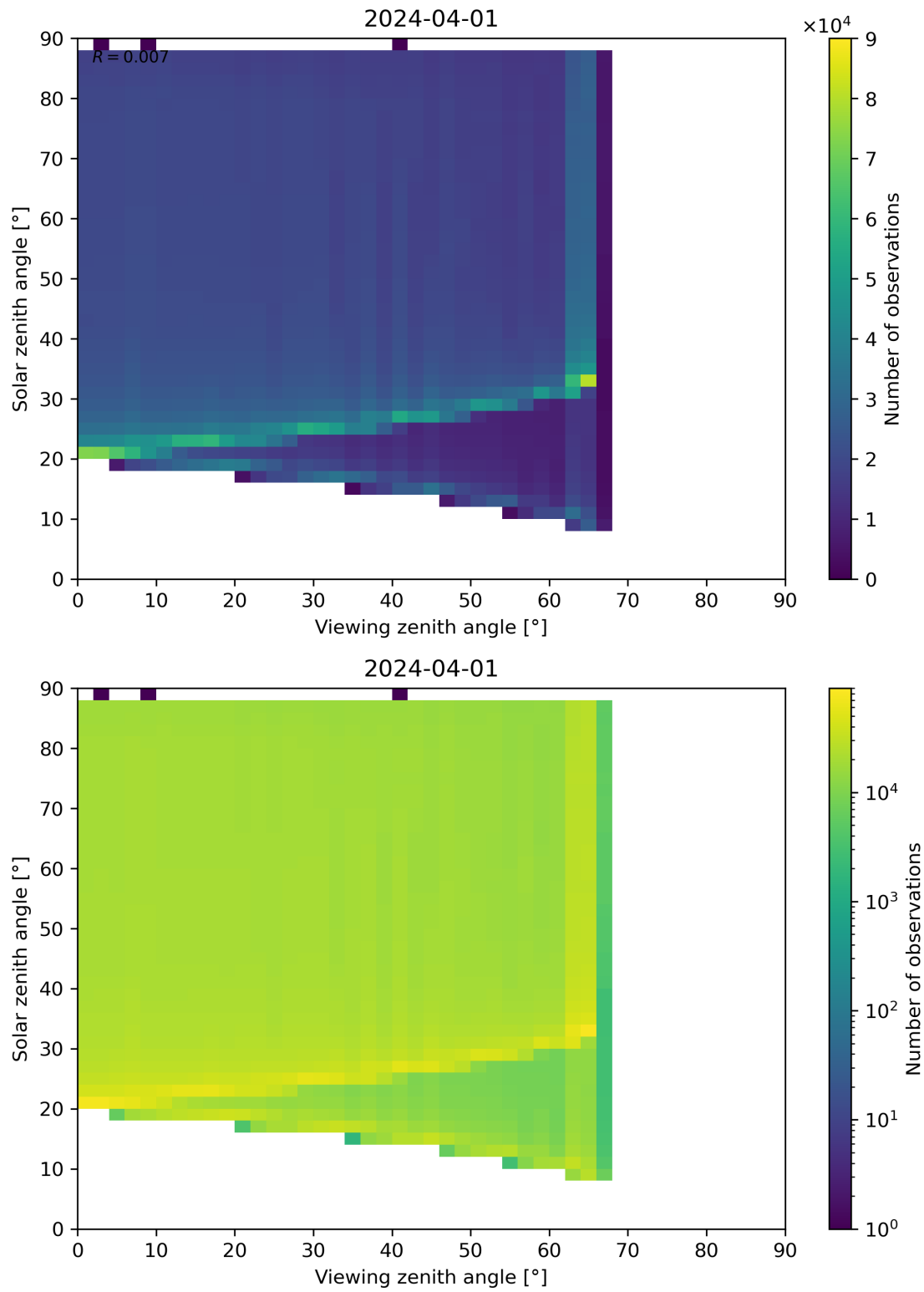
Figure 172: Scatter density plot of “Viewing zenith angle” against “Solar zenith angle” for 2024-03-31 to 2024-04-02.
