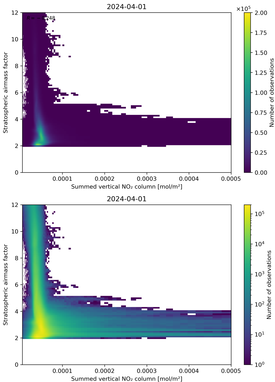
Figure 103: Scatter density plot of “Summed vertical NO 2 column” against “Stratospheric airmass factor” for 2024-03-31 to 2024-04-02.
