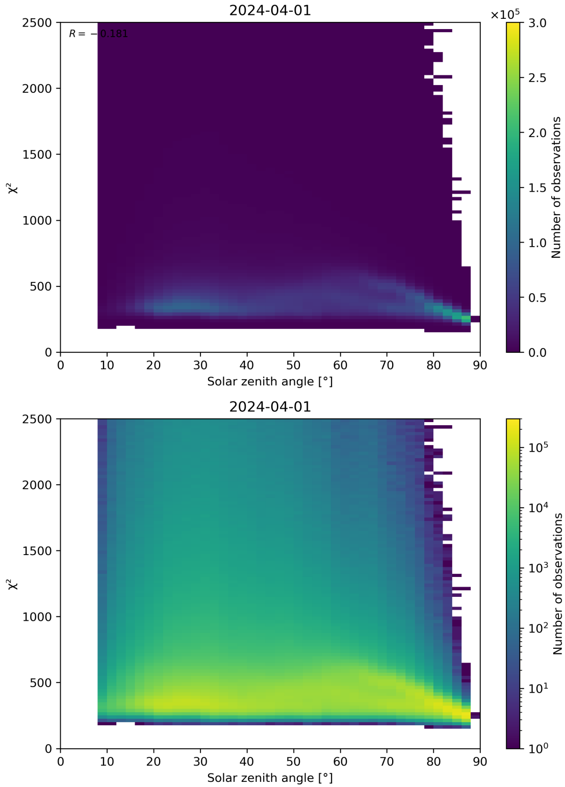
Figure 148: Scatter density plot of “Solar zenith angle” against “ \chi^2 ” for 2024-03-31 to 2024-04-02.
