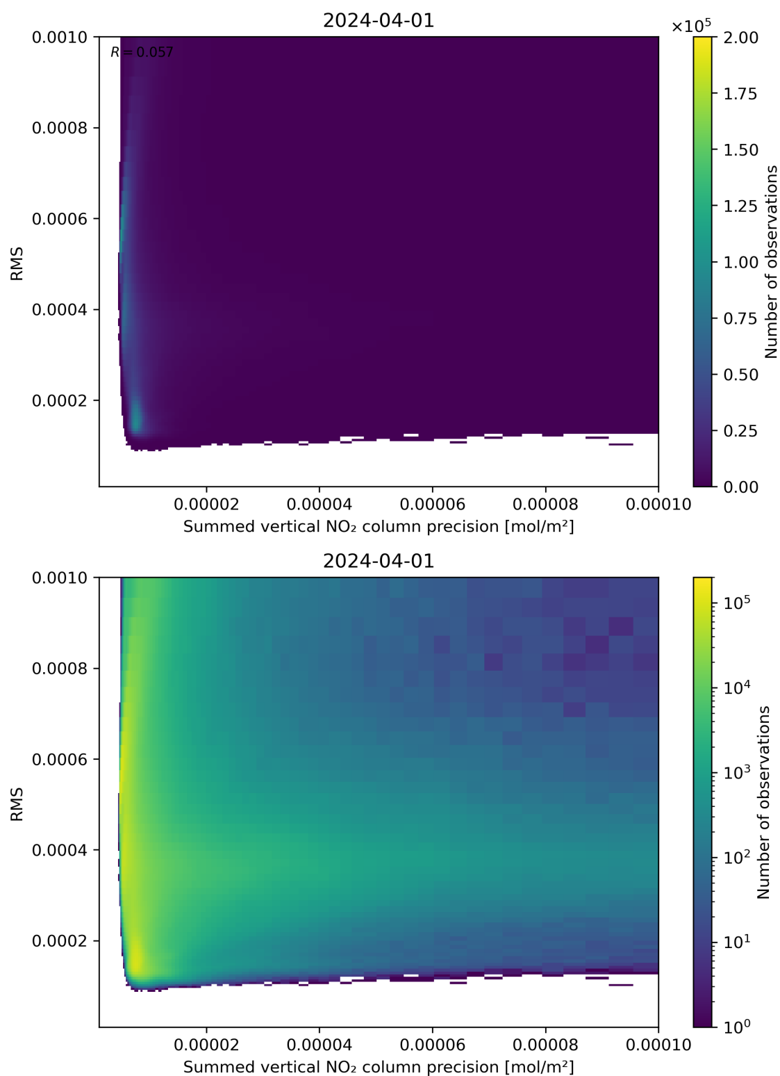
Figure 108: Scatter density plot of “Summed vertical NO 2 column precision” against “RMS” for 2024-03-31 to 2024-04-02.
