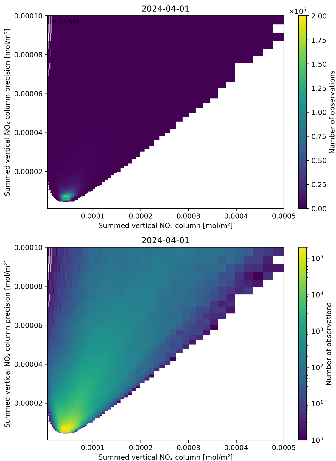
Figure 105: Scatter density plot of “Summed vertical NO 2 column” against “Summed vertical NO 2 column precision” for 2024-03-31 to 2024-04-02.
