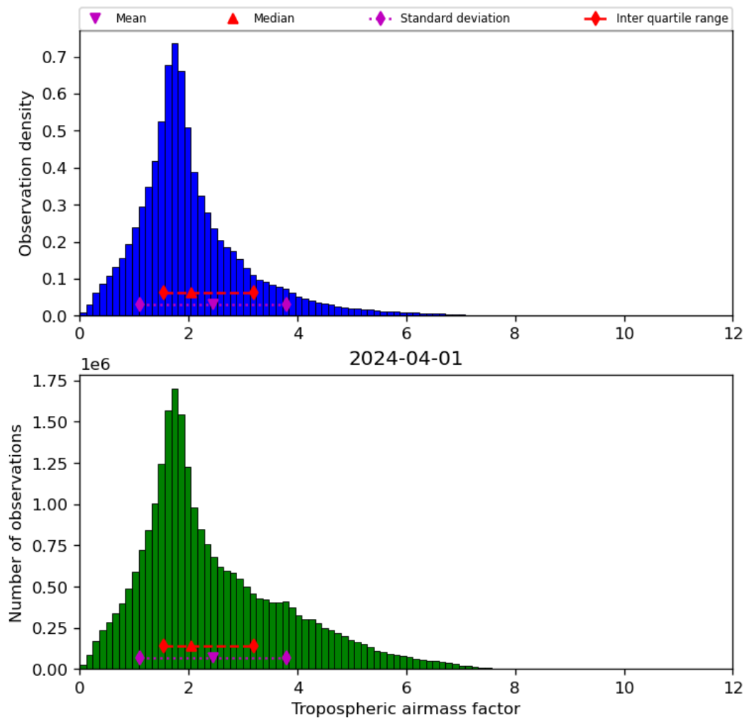
Figure 31: Histogram of “Tropospheric airmass factor” for 2024-03-31 to 2024-04-02
