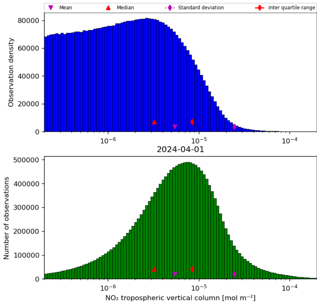
Figure 29: Histogram of “NO 2 tropospheric vertical column” for 2024-03-31 to 2024-04-02
