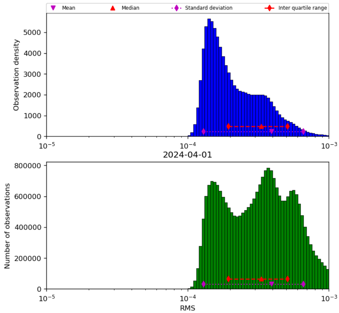
Figure 43: Histogram of “RMS” for 2024-03-31 to 2024-04-02
