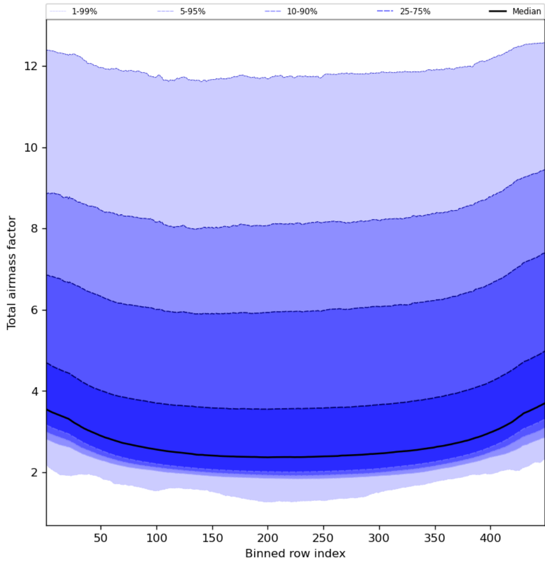
Figure 49: Along track statistics of “Total airmass factor” for 2024-03-31 to 2024-04-02
