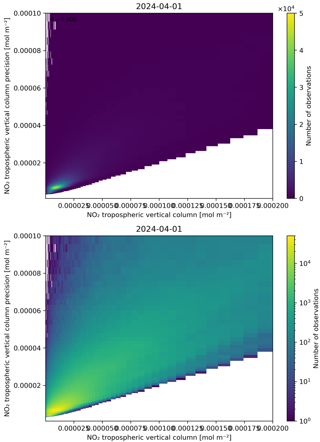
Figure 130: Scatter density plot of “NO 2 tropospheric vertical column” against “NO 2 tropospheric vertical column precision” for 2024-03-31 to 2024-04-02.
