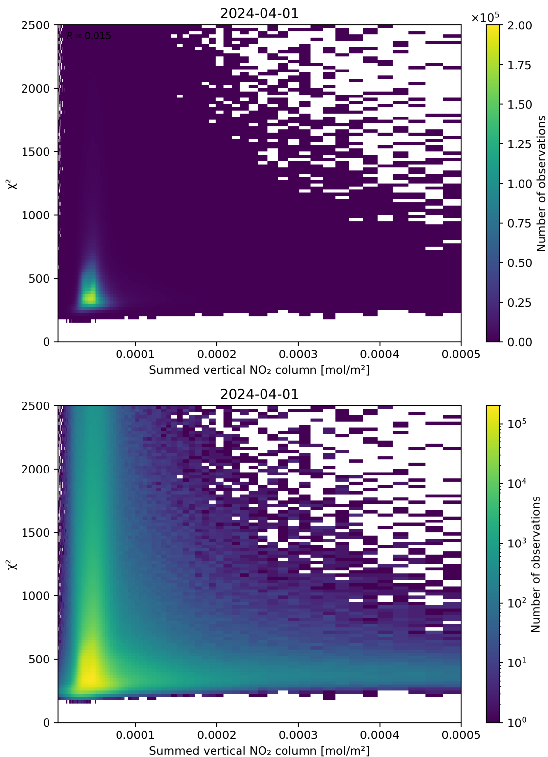
Figure 104: Scatter density plot of “Summed vertical NO 2 column” against “ \chi^2 ” for 2024-03-31 to 2024-04-02.
