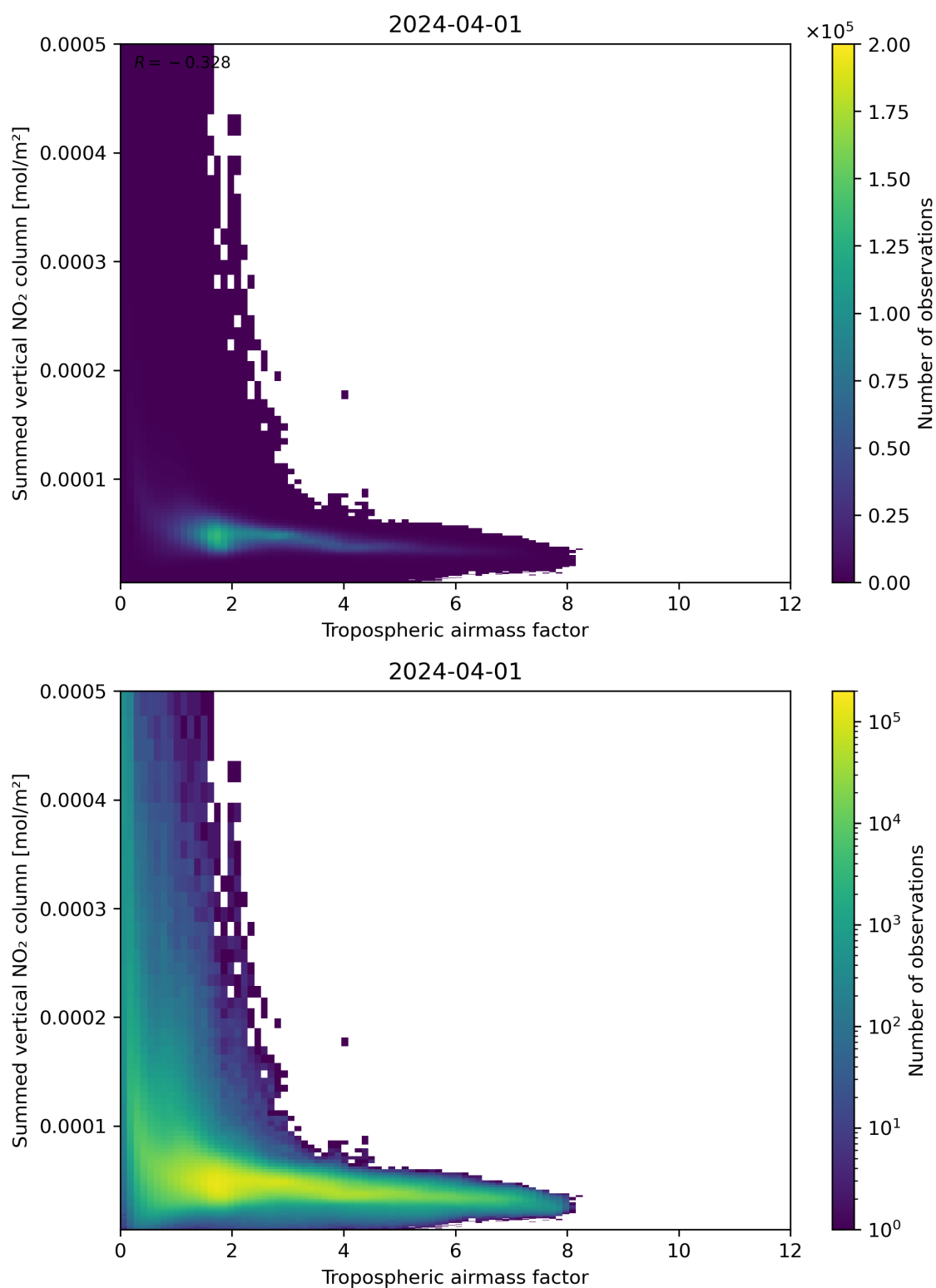
Figure 75: Scatter density plot of “Tropospheric airmass factor” against “Summed vertical NO 2 column” for 2024-03-31 to 2024-04-02.
