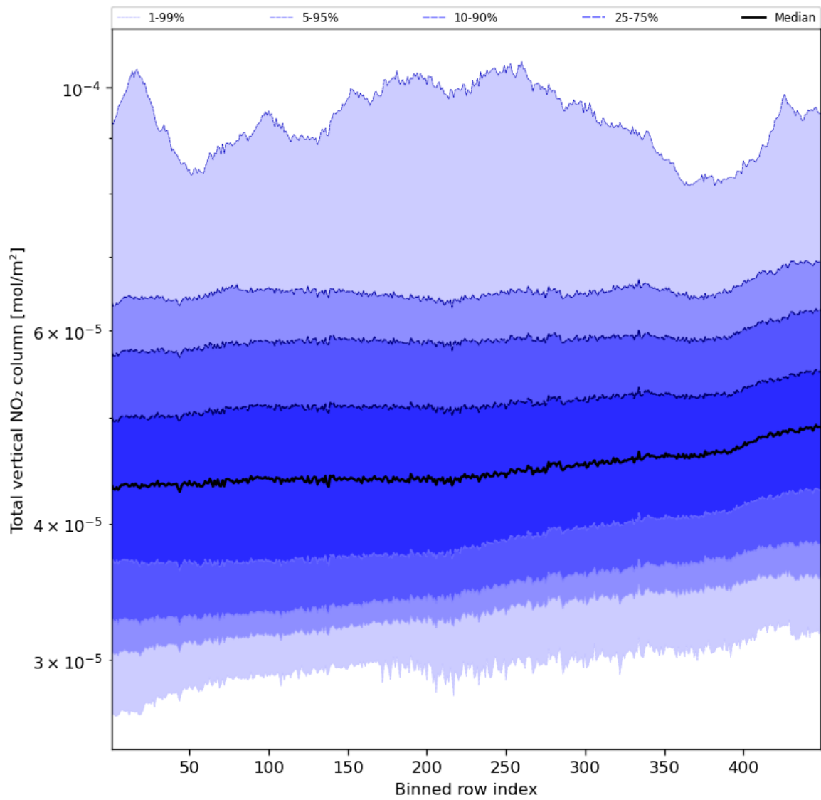
Figure 55: Along track statistics of “Total vertical NO 2 column” for 2024-03-31 to 2024-04-02
