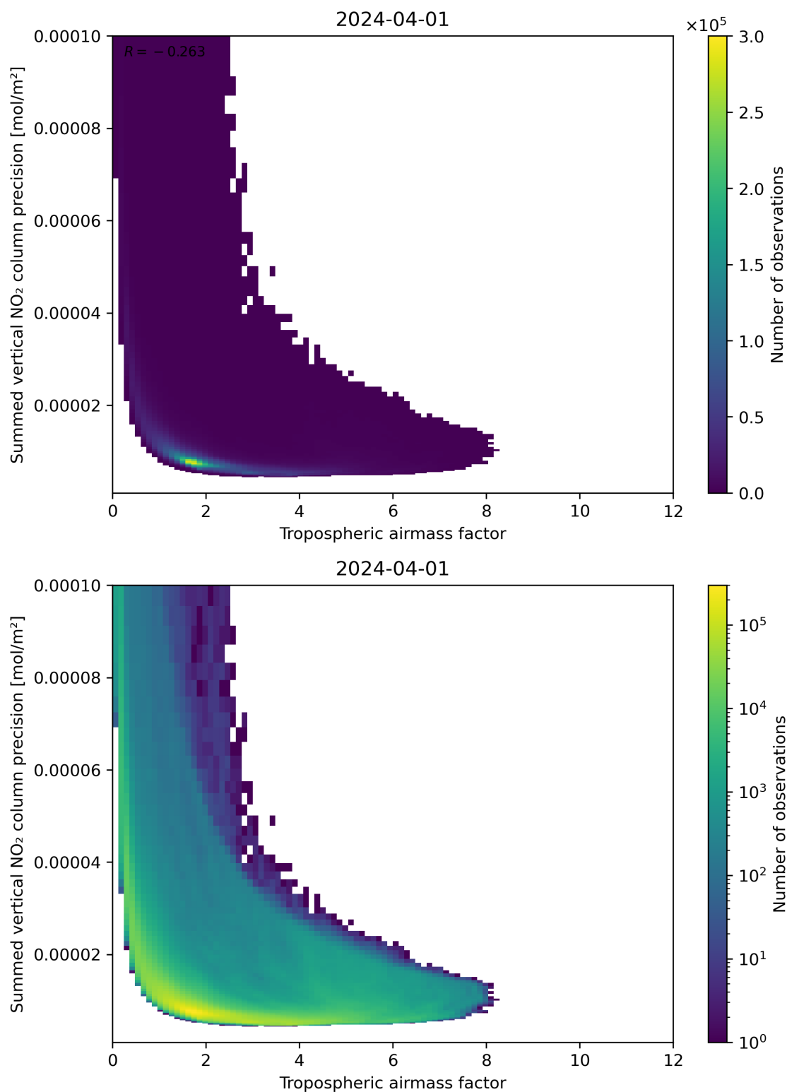
Figure 76: Scatter density plot of “Tropospheric air mass factor” against “Summed vertical NO 2 column precision” for 2024-03-31 to 2024-04-02.
