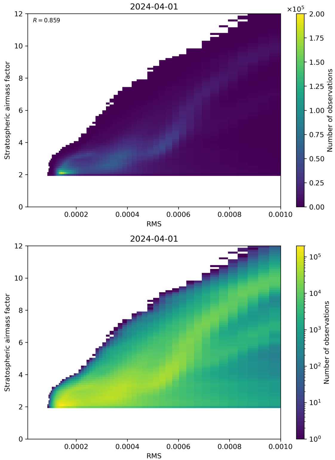
Figure 144: Scatter density plot of “RMS” against “Stratospheric airmass factor” for 2024-03-31 to 2024-04-02.
