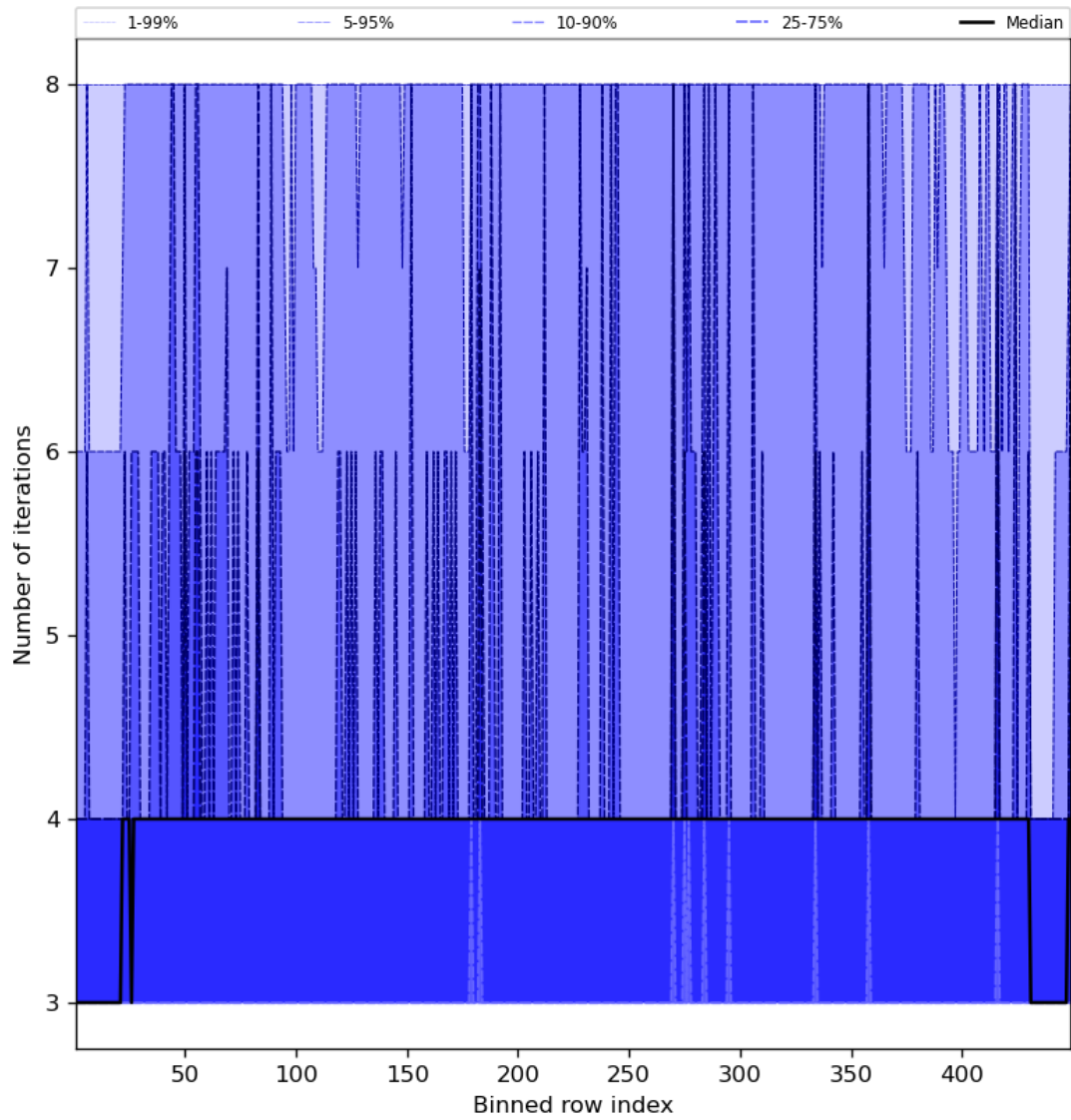
Figure 51: Along track statistics of “Number of iterations” for 2024-03-31 to 2024-04-02
