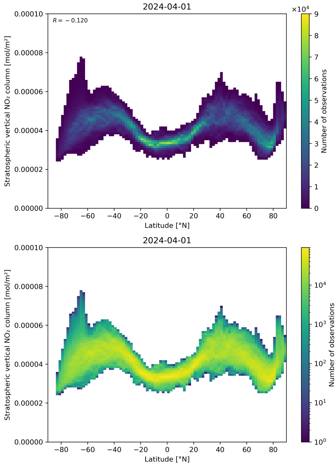
Figure 87: Scatter density plot of “Latitude” against “Stratospheric vertical \text{NO}_2 column” for 2024-03-31 to 2024-04-02.
