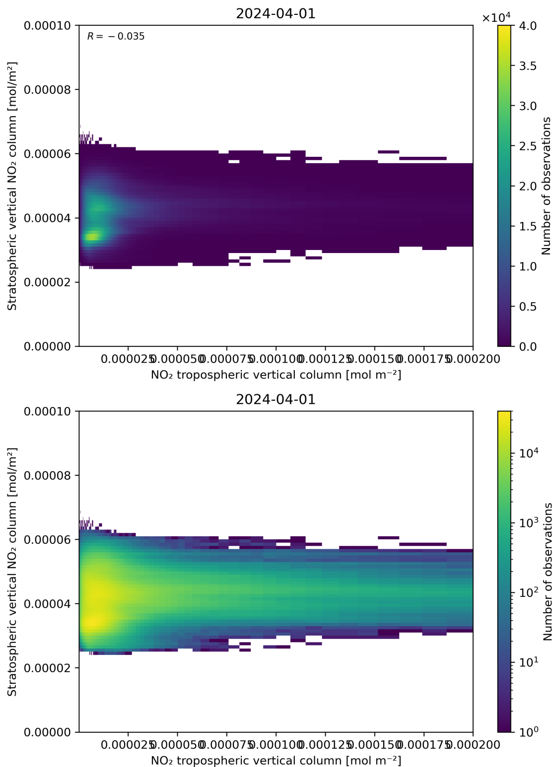
Figure 125: Scatter density plot of “NO 2 tropospheric vertical column” against “Stratospheric vertical NO 2 column” for 2024-03-31 to 2024-04-02.
