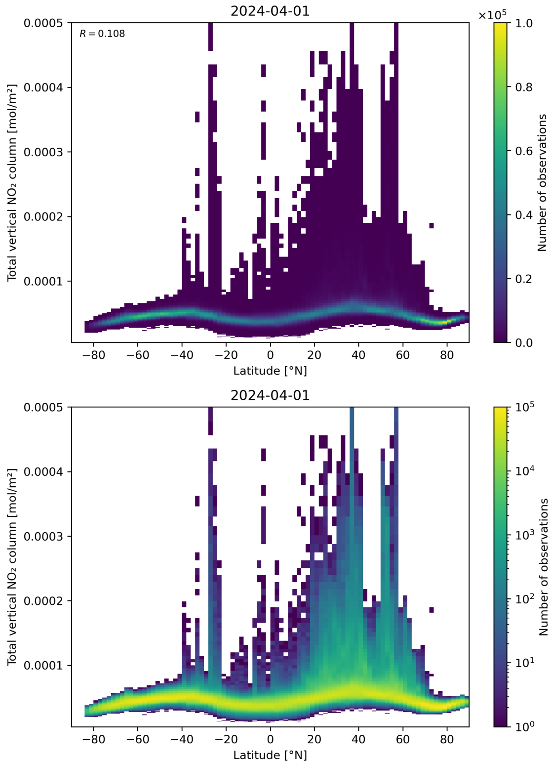
Figure 90: Scatter density plot of “Latitude” against “Total vertical NO 2 column” for 2024-03-31 to 2024-04-02.
