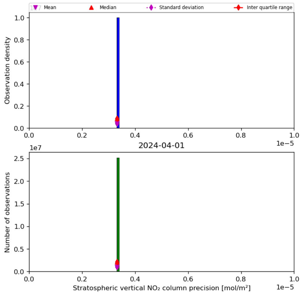
Figure 37: Histogram of “Stratospheric vertical NO 2 column precision” for 2024-03-31 to 2024-04-02
