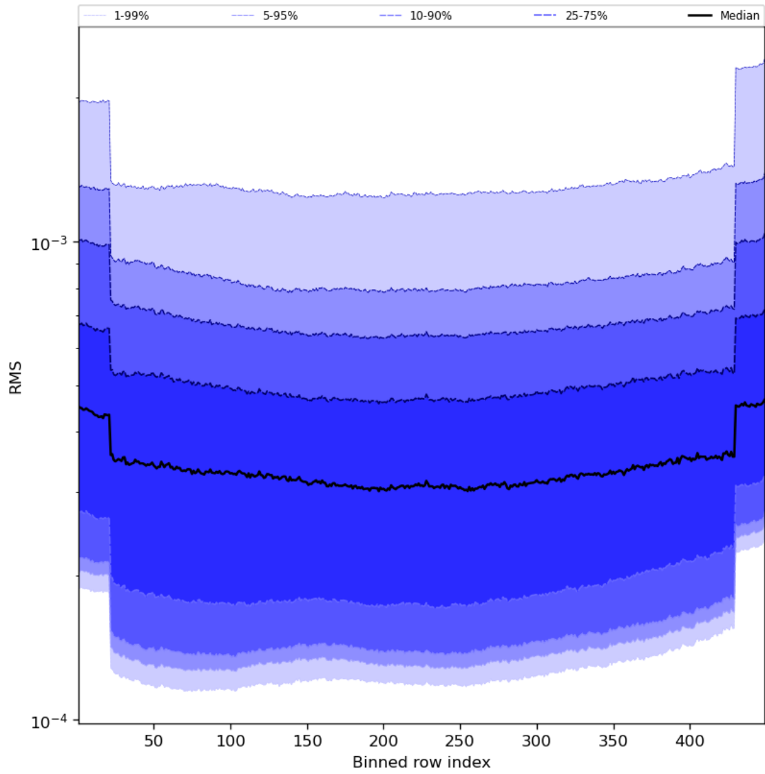
Figure 60: Along track statistics of “RMS” for 2024-03-31 to 2024-04-02
