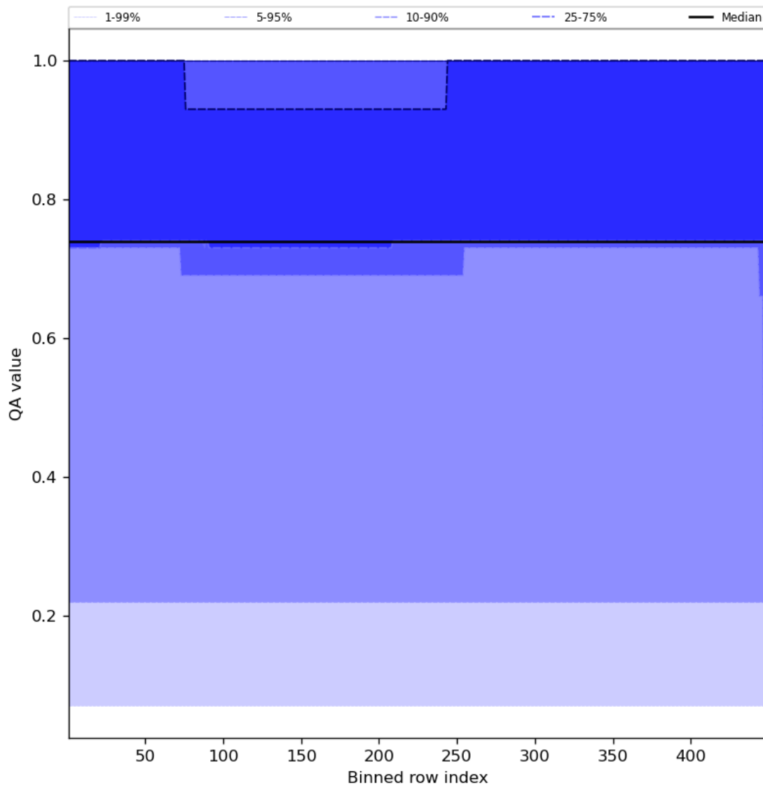
Figure 45: Along track statistics of “QA value” for 2024-03-31 to 2024-04-02
