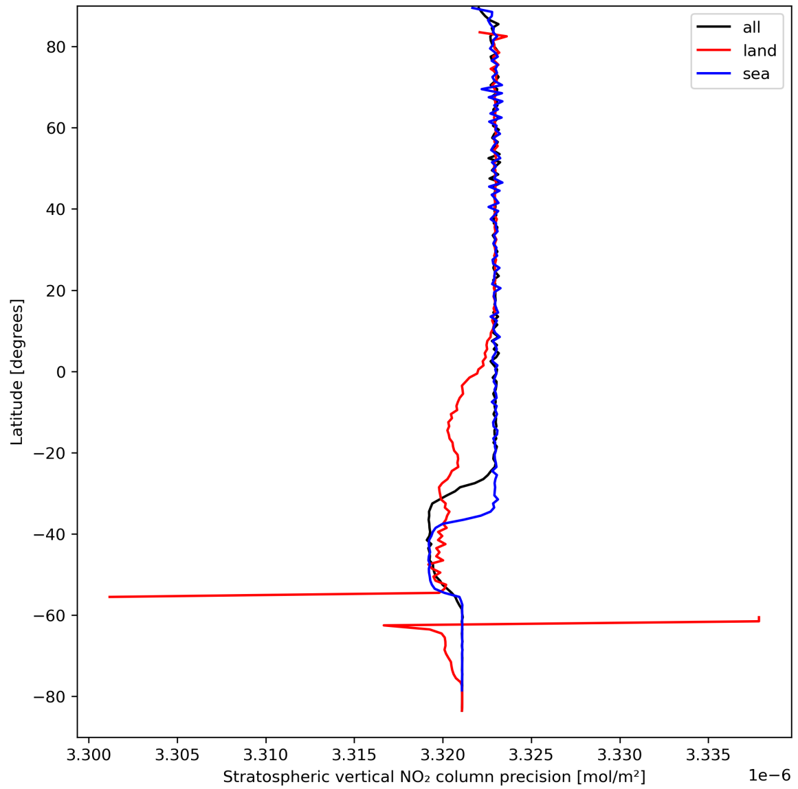
Figure 20: Zonal average of “Stratospheric vertical NO 2 column precision” for 2024-03-31 to 2024-04-02.
