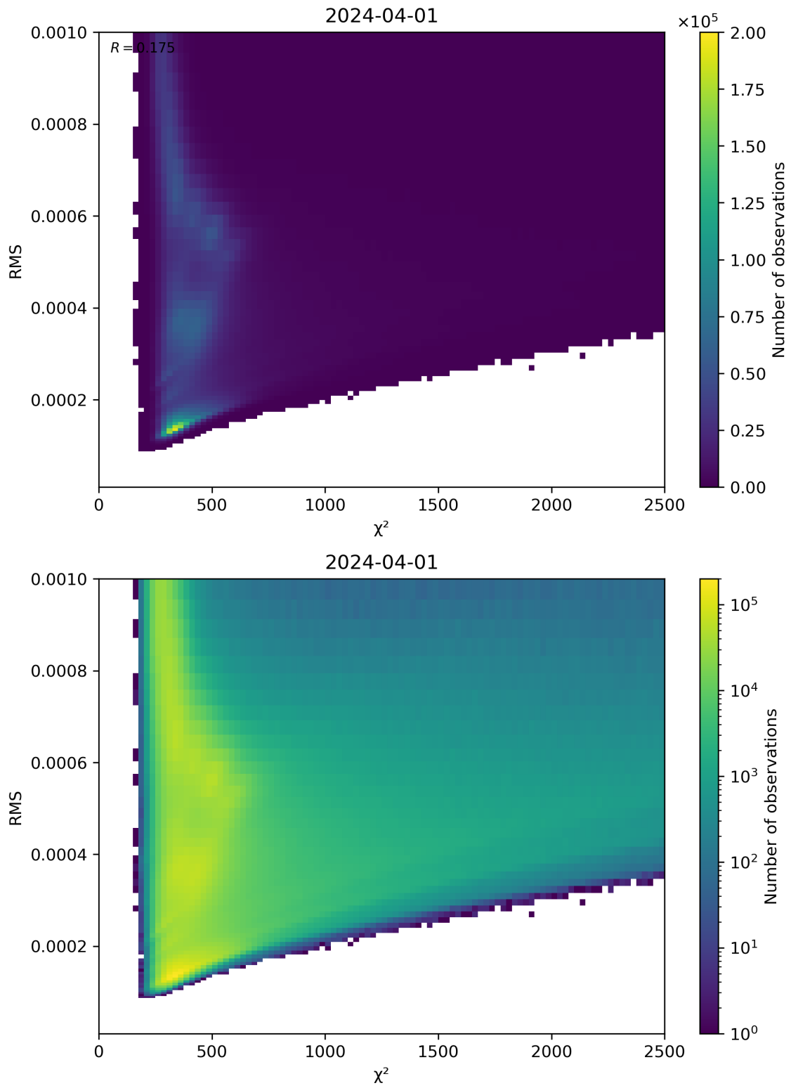
Figure 82: Scatter density plot of “ \chi^2 ” against “RMS” for 2024-03-31 to 2024-04-02.
