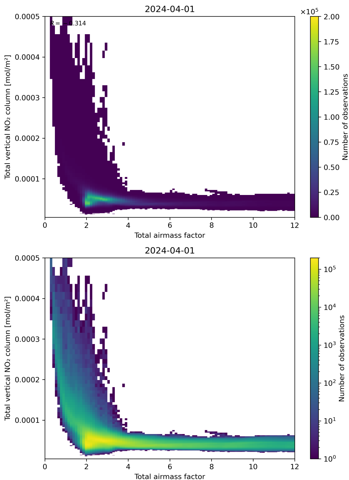
Figure 67: Scatter density plot of “Total airmass factor” against “Total vertical NO 2 column” for 2024-03-31 to 2024-04-02.
