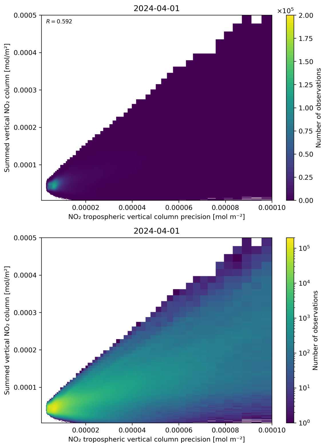
Figure 136: Scatter density plot of “NO 2 tropospheric vertical column precision” against “Summed vertical NO 2 column” for 2024-03-31 to 2024-04-02.
