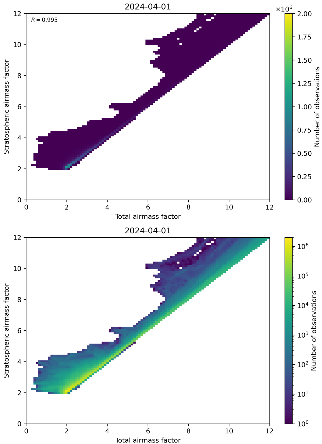
Figure 62: Scatter density plot of “Total airmass factor” against “Stratospheric airmass factor” for 2024-03-31 to 2024-04-02.
