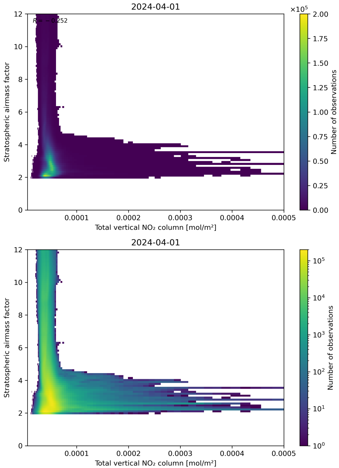
Figure 110: Scatter density plot of “Total vertical NO 2 column” against “Stratospheric airmass factor” for 2024-03-31 to 2024-04-02.
