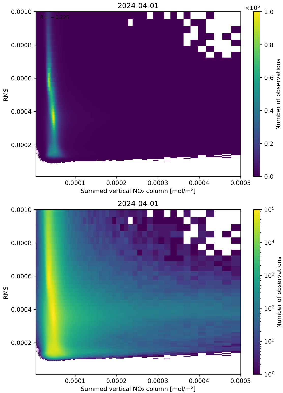
Figure 109: Scatter density plot of “Summed vertical NO 2 column” against “RMS” for 2024-03-31 to 2024-04-02.
