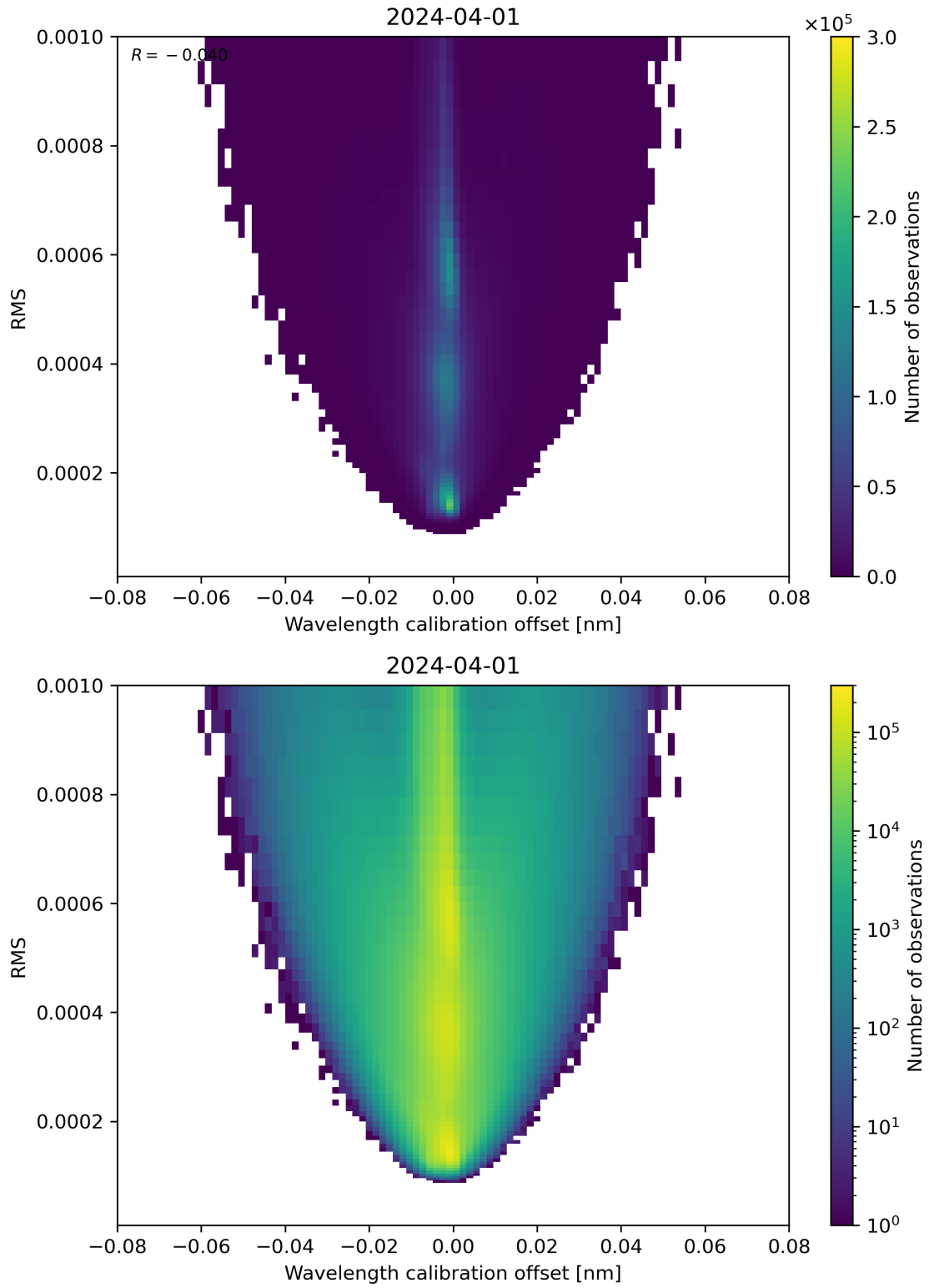
Figure 181: Scatter density plot of “Wavelength calibration offset” against “RMS” for 2024-03-31 to 2024-04-02.
