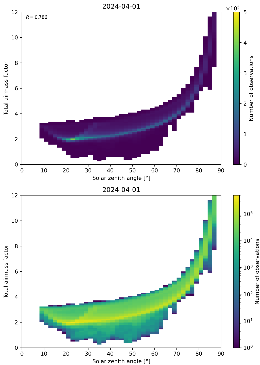
Figure 146: Scatter density plot of “Solar zenith angle” against “Total air mass factor” for 2024-03-31 to 2024-04-02.
