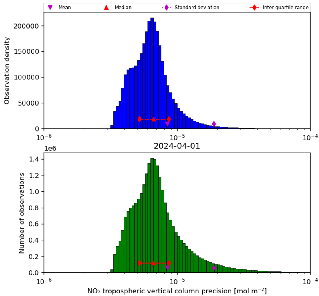
Figure 30: Histogram of “NO 2 tropospheric vertical column precision” for 2024-03-31 to 2024-04-02
