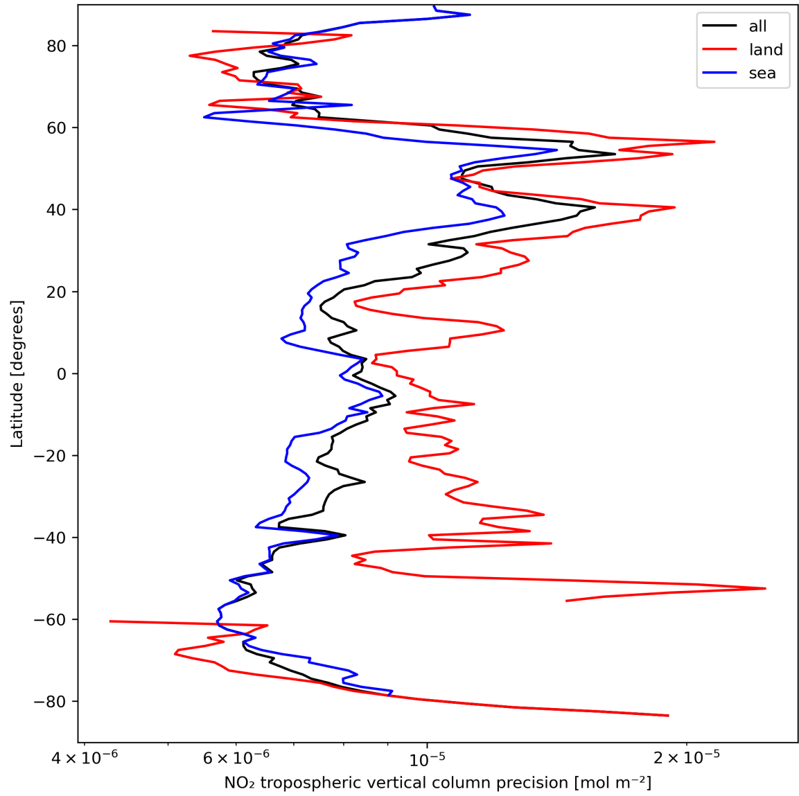
Figure 13: Zonal average of “NO 2 tropospheric vertical column precision” for 2024-03-31 to 2024-04-02.
