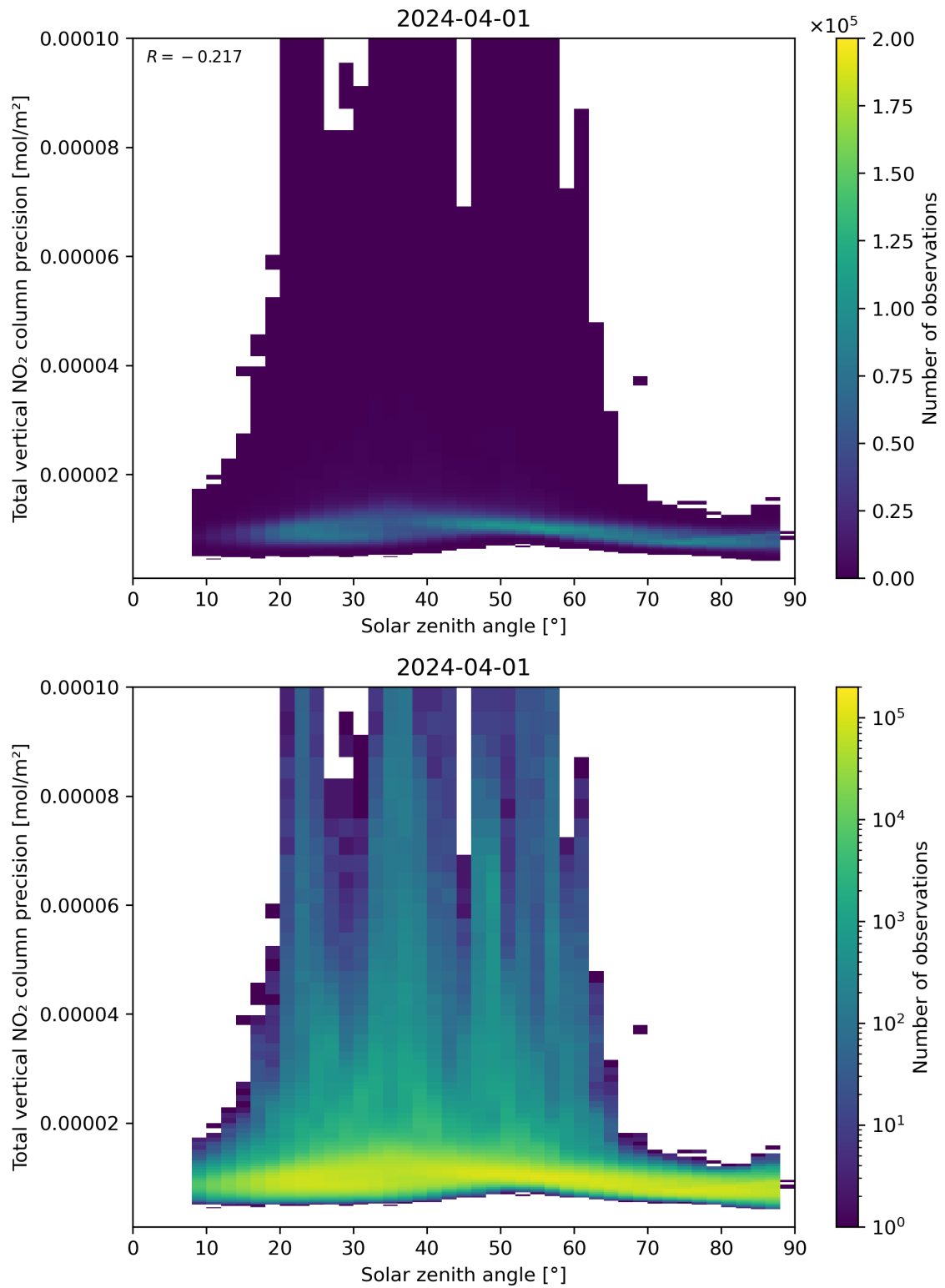
Figure 154: Scatter density plot of “Solar zenith angle” against “Total vertical NO 2 column precision” for 2024-03-31 to 2024-04-02.
