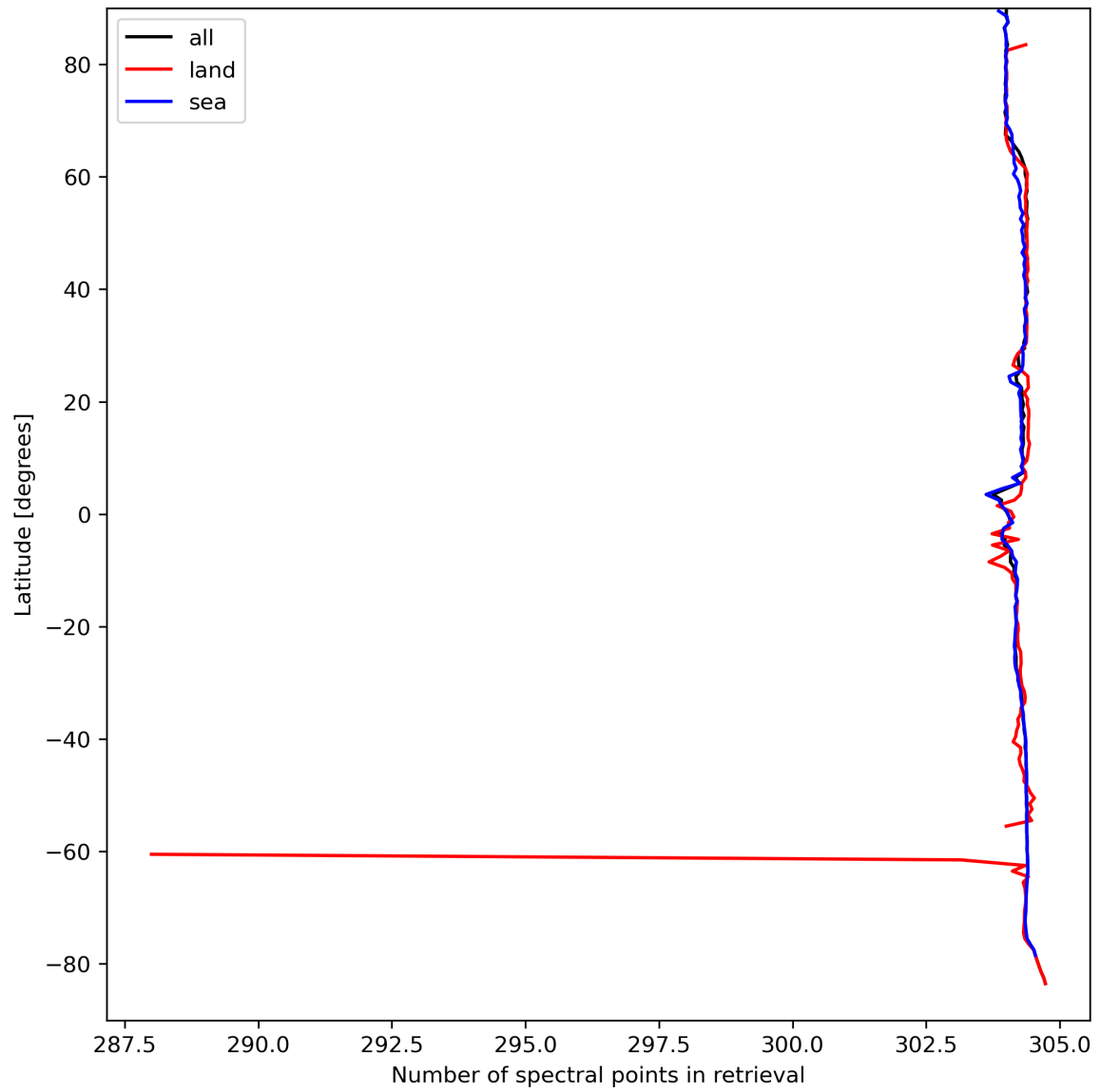
Figure 16: Zonal average of “Number of spectral points in retrieval” for 2024-03-31 to 2024-04-02.
