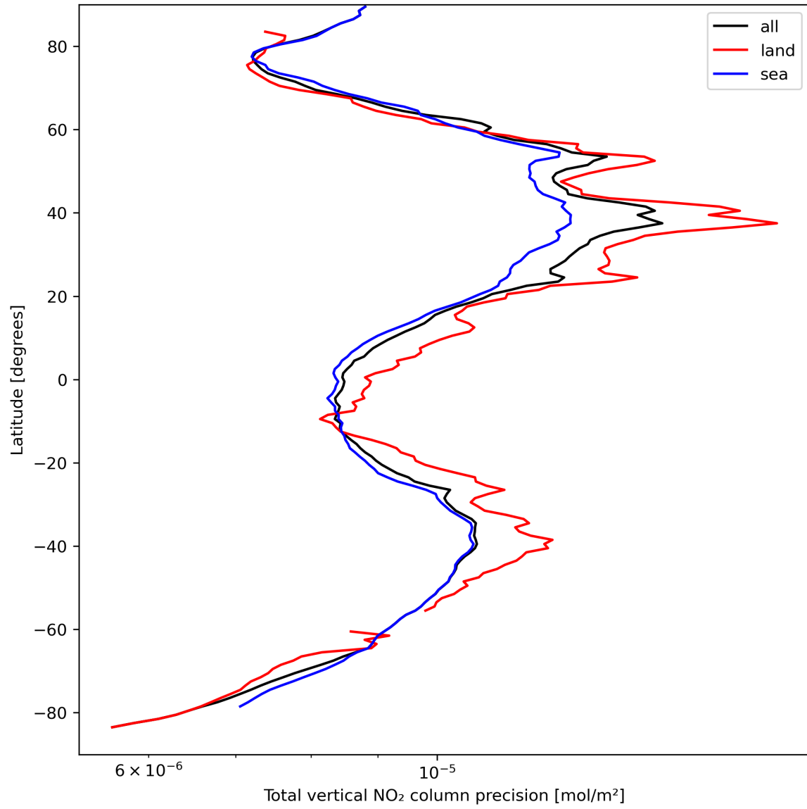
Figure 22: Zonal average of “Total vertical NO 2 column precision” for 2024-03-31 to 2024-04-02.
