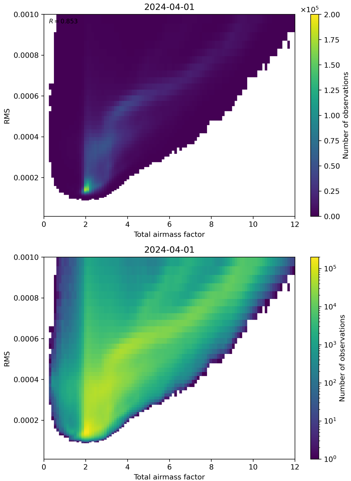
Figure 69: Scatter density plot of “Total airmass factor” against “RMS” for 2024-03-31 to 2024-04-02.
