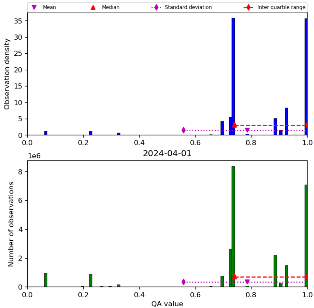
Figure 28: Histogram of “QA value” for 2024-03-31 to 2024-04-02
