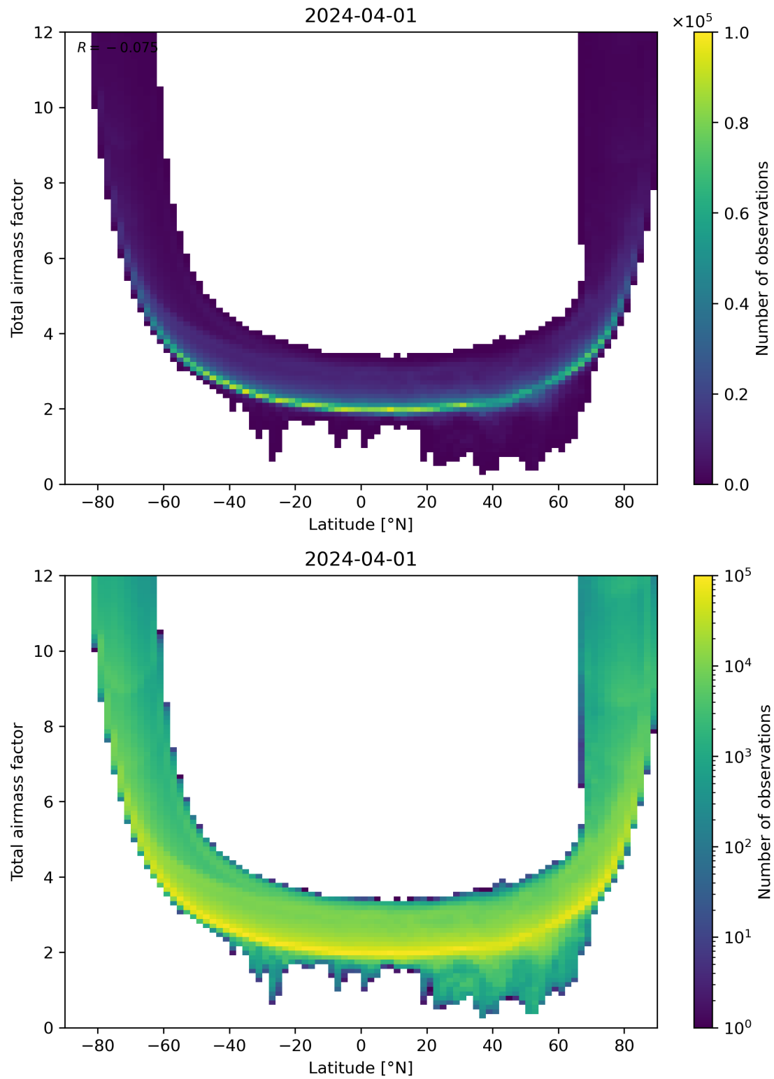
Figure 84: Scatter density plot of “Latitude” against “Total airmass factor” for 2024-03-31 to 2024-04-02.
