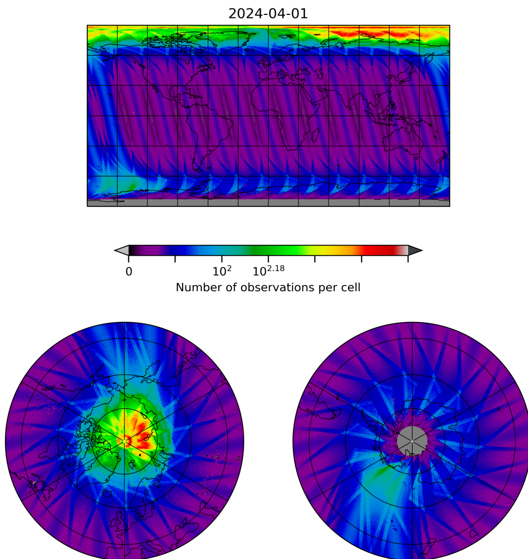
Figure 10: Map of the number of observations for 2024-03-31 to 2024-04-02
