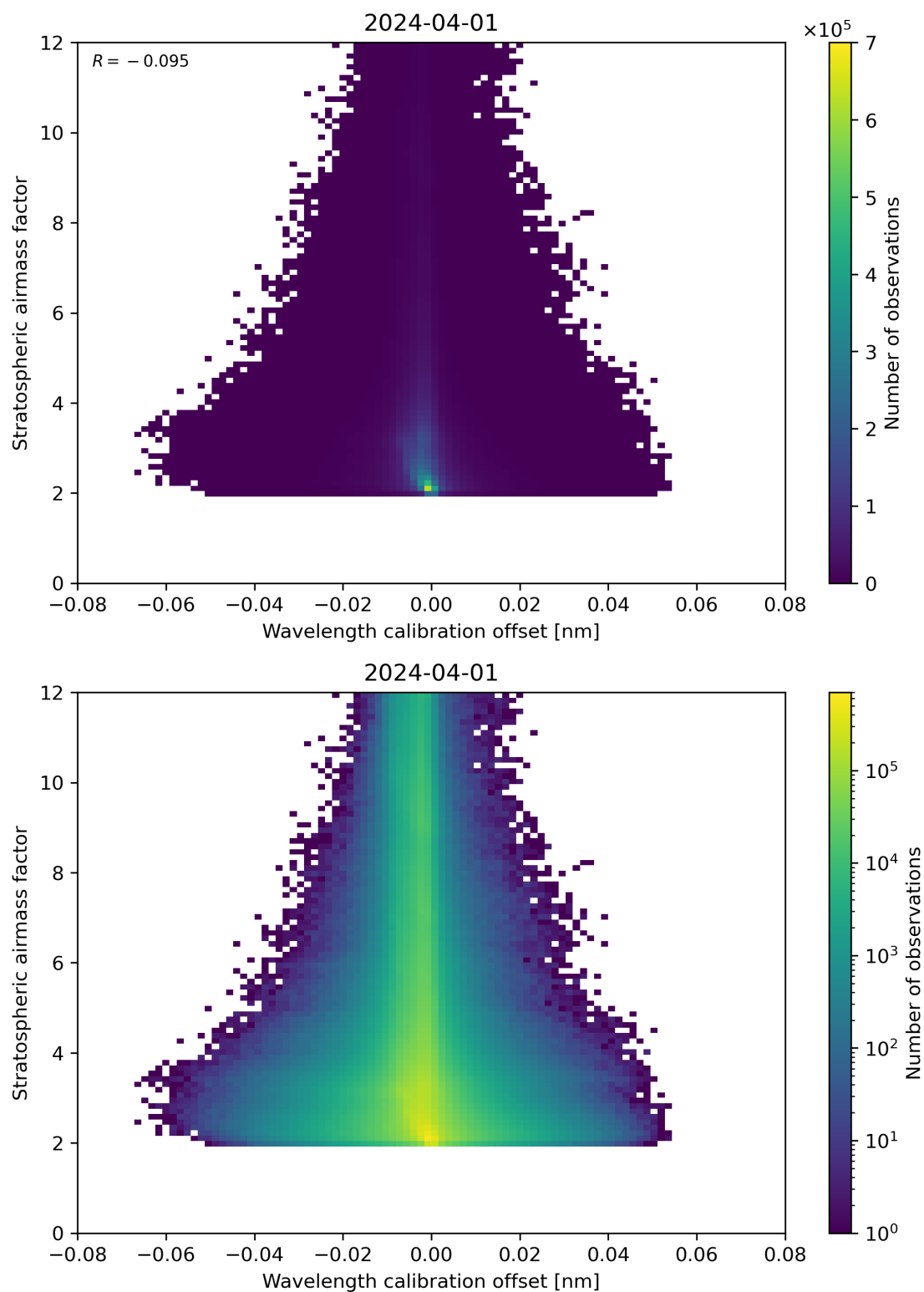
Figure 174: Scatter density plot of “Wavelength calibration offset” against “Stratospheric airmass factor” for 2024-03-31 to 2024-04-02.
