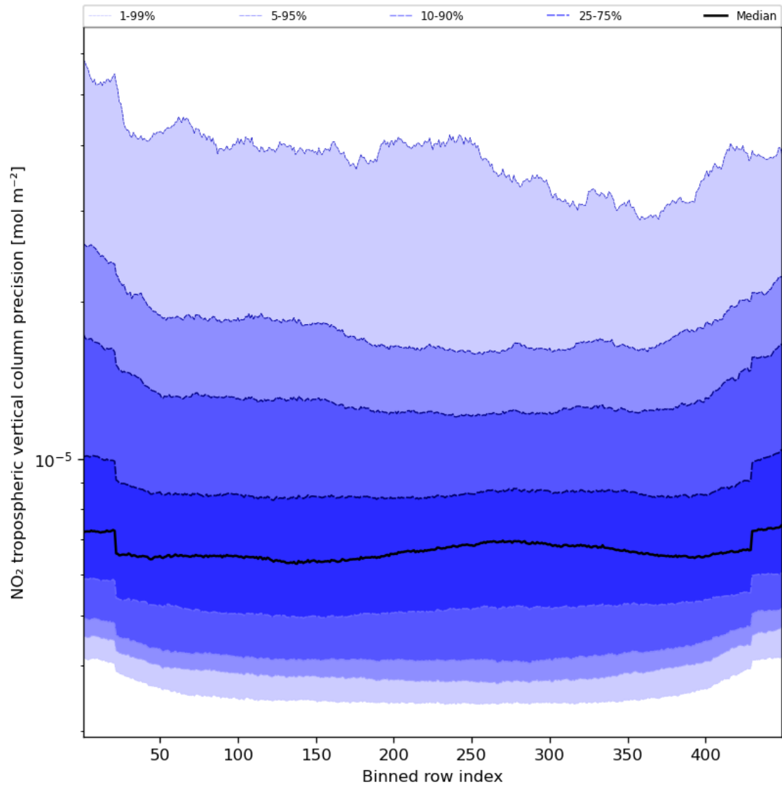
Figure 47: Along track statistics of “NO 2 tropospheric vertical column precision” for 2024-03-31 to 2024-04-02
