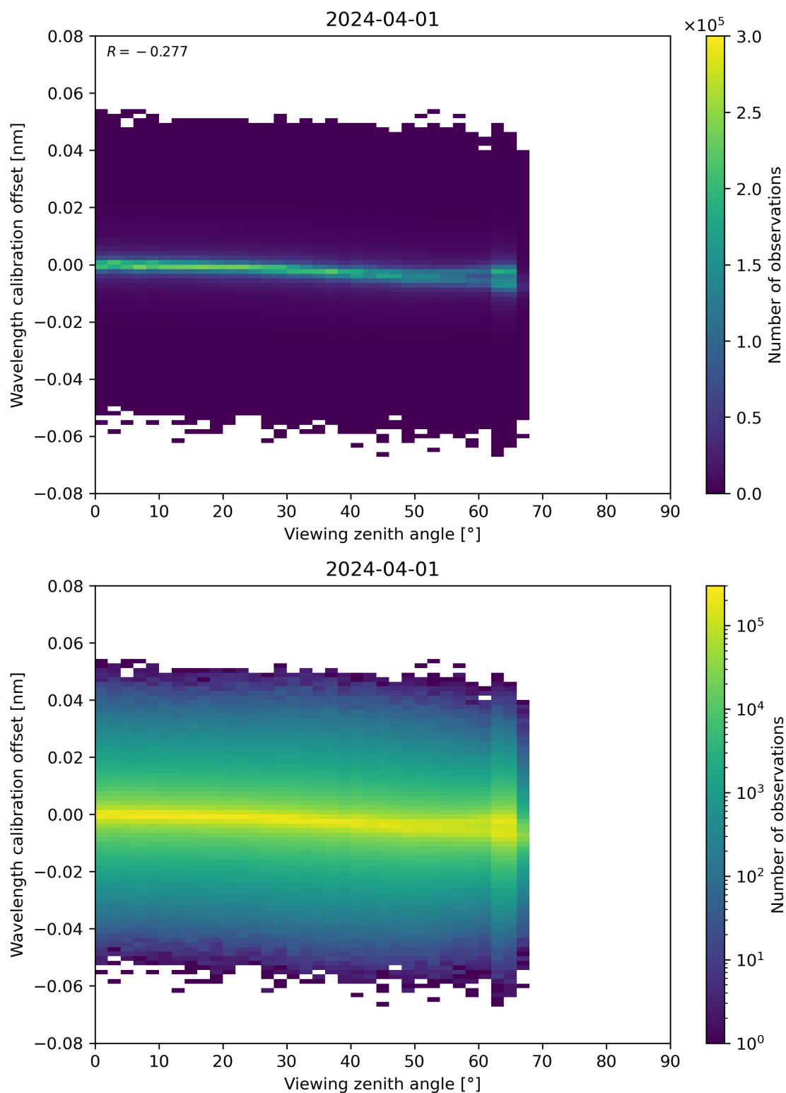
Figure 173: Scatter density plot of “Viewing zenith angle” against “Wavelength calibration offset” for 2024-03-31 to 2024-04-02.
