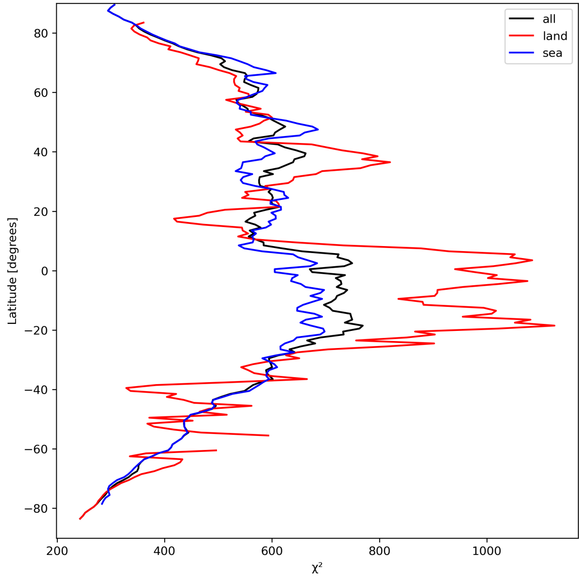
Figure 25: Zonal average of “ \chi^2 ” for 2024-03-31 to 2024-04-02.
