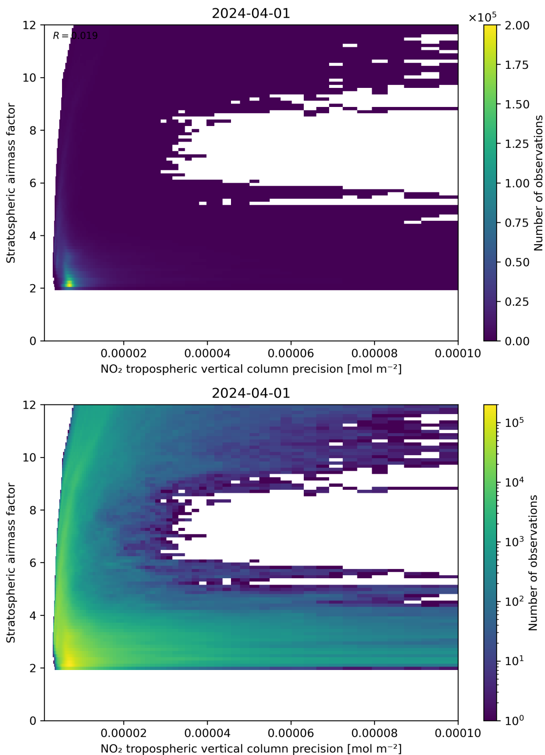
Figure 131: Scatter density plot of “NO 2 tropospheric vertical column precision” against “Stratospheric airmass factor” for 2024-03-31 to 2024-04-02.
