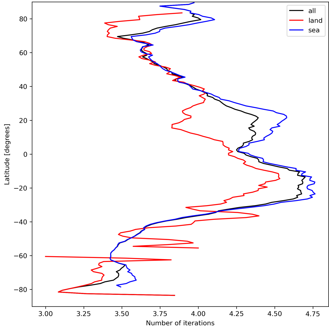
Figure 17: Zonal average of “Number of iterations” for 2024-03-31 to 2024-04-02.
