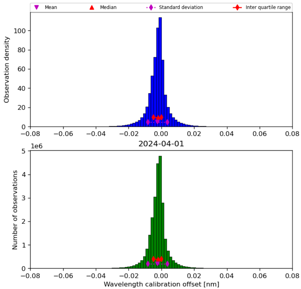
Figure 35: Histogram of “Wavelength calibration offset” for 2024-03-31 to 2024-04-02
