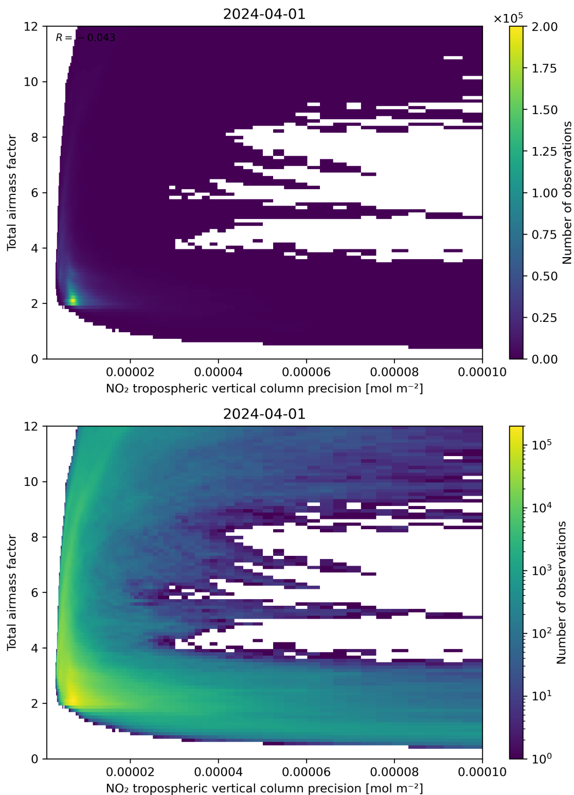
Figure 132: Scatter density plot of “NO 2 tropospheric vertical column precision” against “Total air mass factor” for 2024-03-31 to 2024-04-02.
