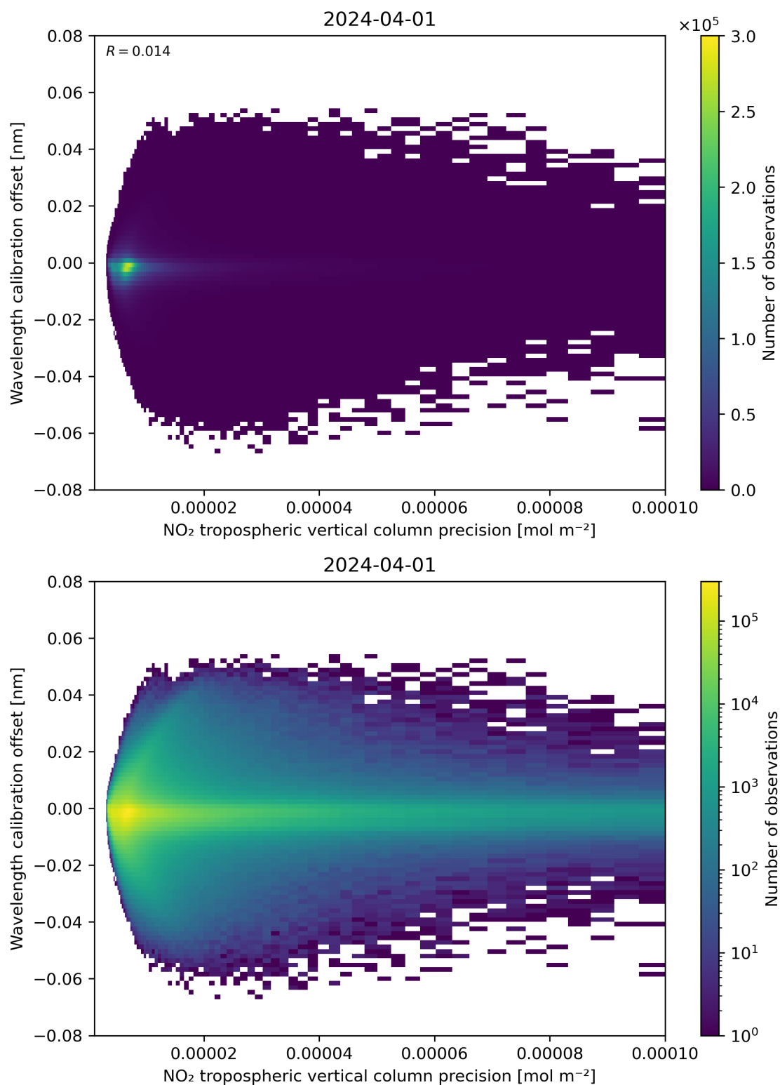
Figure 141: Scatter density plot of “NO 2 tropospheric vertical column precision” against “Wavelength calibration offset” for 2024-03-31 to 2024-04-02.
