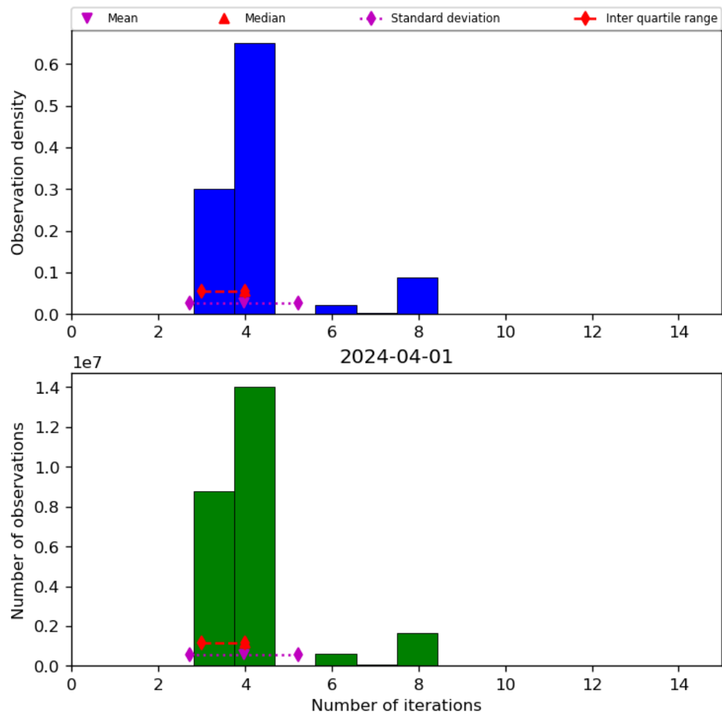
Figure 34: Histogram of “Number of iterations” for 2024-03-31 to 2024-04-02
