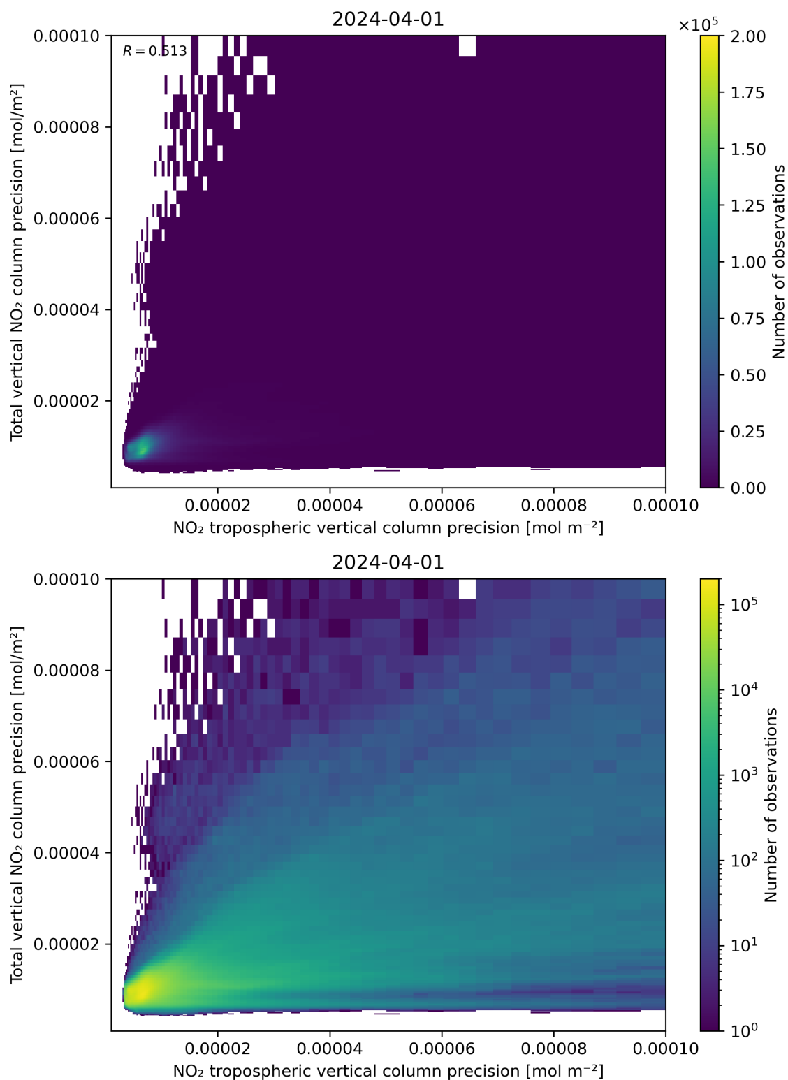
Figure 139: Scatter density plot of “NO 2 tropospheric vertical column precision” against “Total vertical NO 2 column precision” for 2024-03-31 to 2024-04-02.
