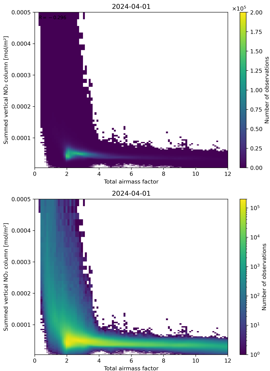
Figure 65: Scatter density plot of “Total airmass factor” against “Summed vertical NO 2 column” for 2024-03-31 to 2024-04-02.
