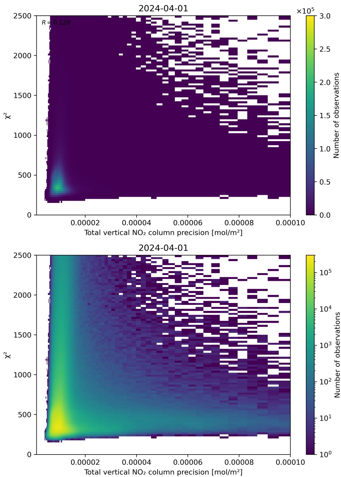
Figure 116: Scatter density plot of “Total vertical NO 2 column precision” against “ \chi^2 ” for 2024-03-31 to 2024-04-02.
