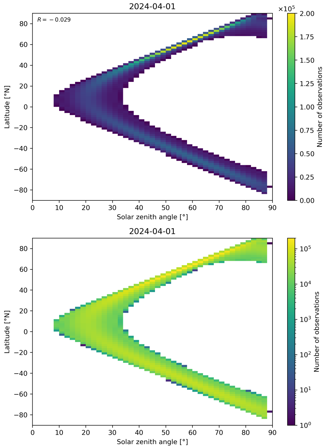
Figure 149: Scatter density plot of “Solar zenith angle” against “Latitude” for 2024-03-31 to 2024-04-02.
