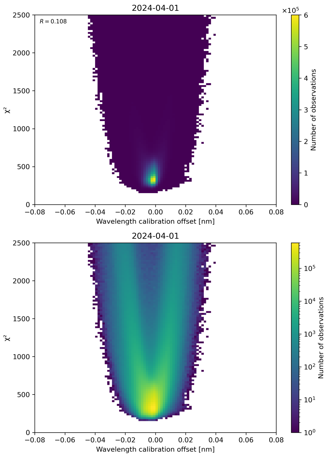
Figure 175: Scatter density plot of “Wavelength calibration offset” against “ \chi^2 ” for 2024-03-31 to 2024-04-02.
