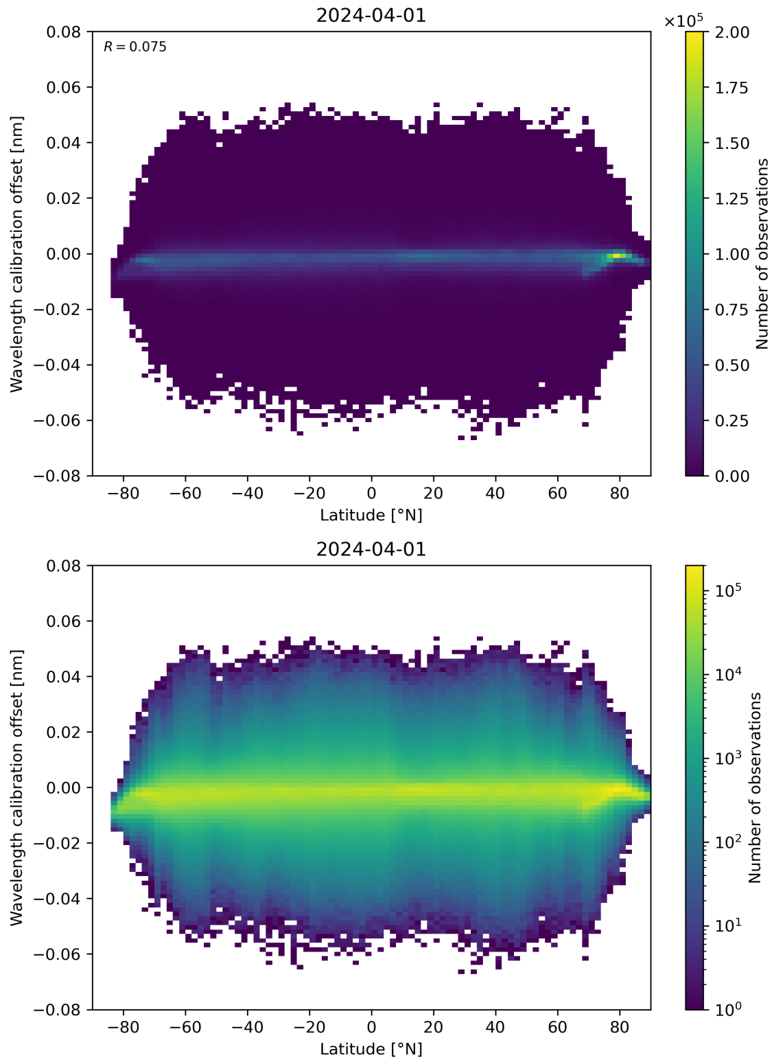
Figure 95: Scatter density plot of “Latitude” against “Wavelength calibration offset” for 2024-03-31 to 2024-04-02.
