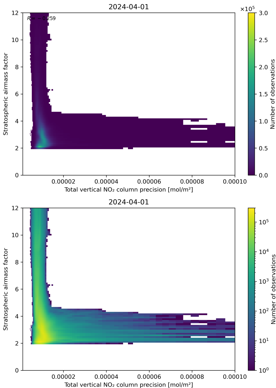
Figure 115: Scatter density plot of “Total vertical NO 2 column precision” against “Stratospheric air mass factor” for 2024-03-31 to 2024-04-02.
