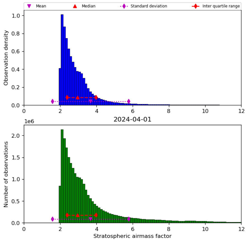
Figure 44: Histogram of “Stratospheric airmass factor” for 2024-03-31 to 2024-04-02
