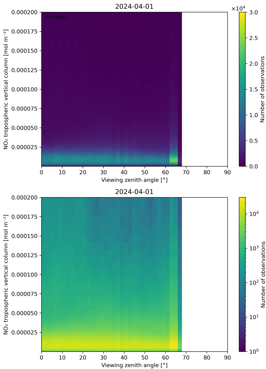
Figure 169: Scatter density plot of “Viewing zenith angle” against “NO 2 tropospheric vertical column” for 2024-03-31 to 2024-04-02.
