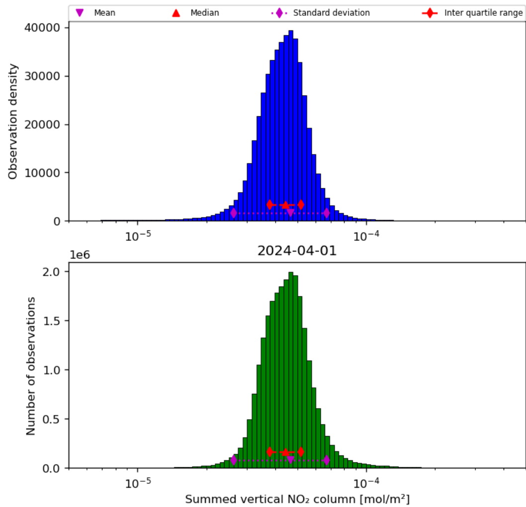
Figure 40: Histogram of “Summed vertical NO 2 column” for 2024-03-31 to 2024-04-02
