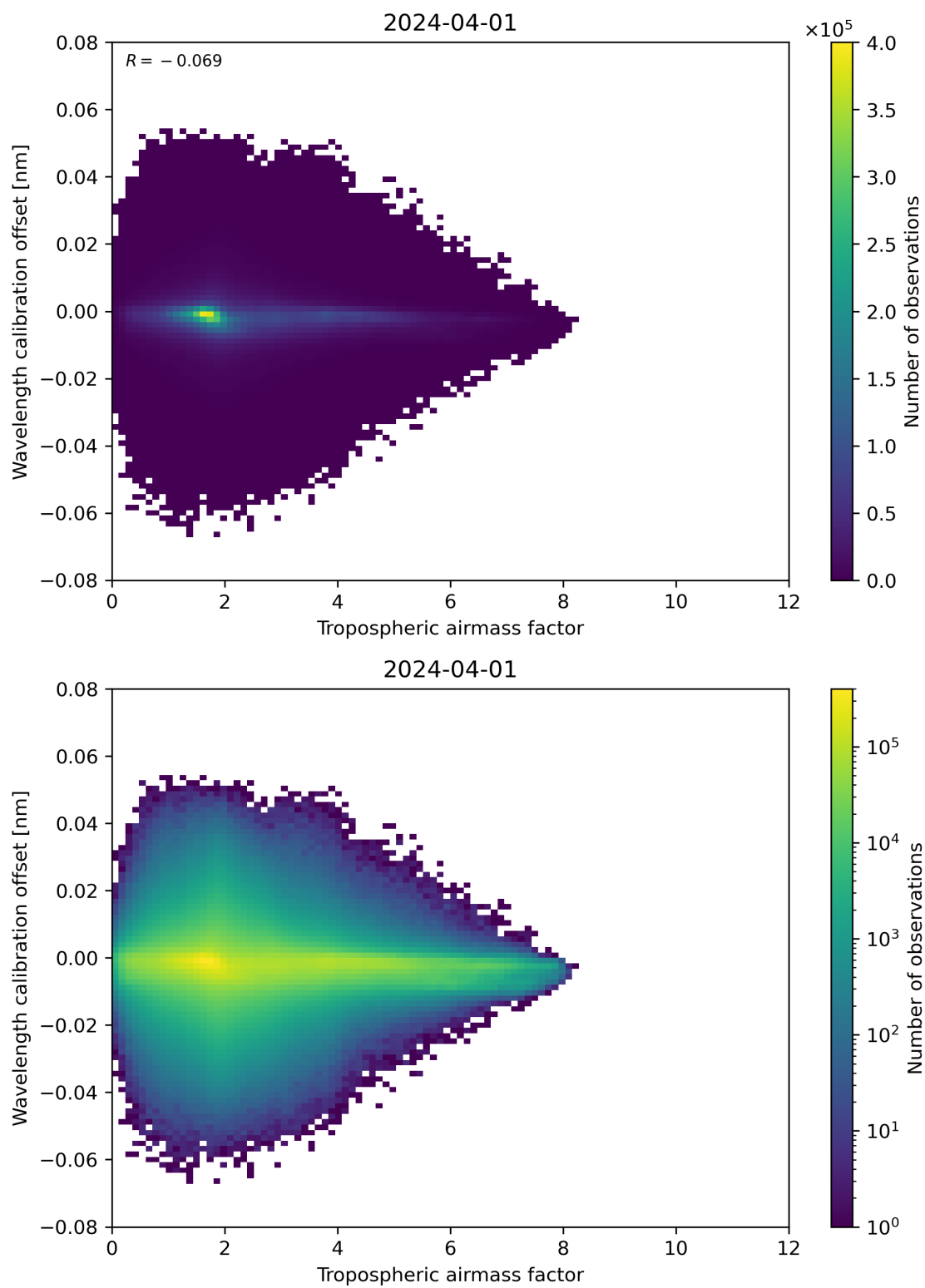
Figure 80: Scatter density plot of “Tropospheric airmass factor” against “Wavelength calibration offset” for 2024-03-31 to 2024-04-02.
