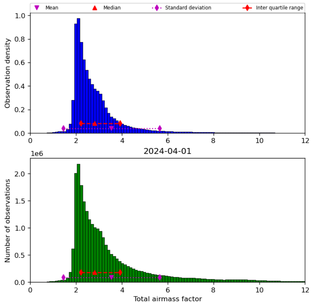
Figure 32: Histogram of “Total airmass factor” for 2024-03-31 to 2024-04-02
