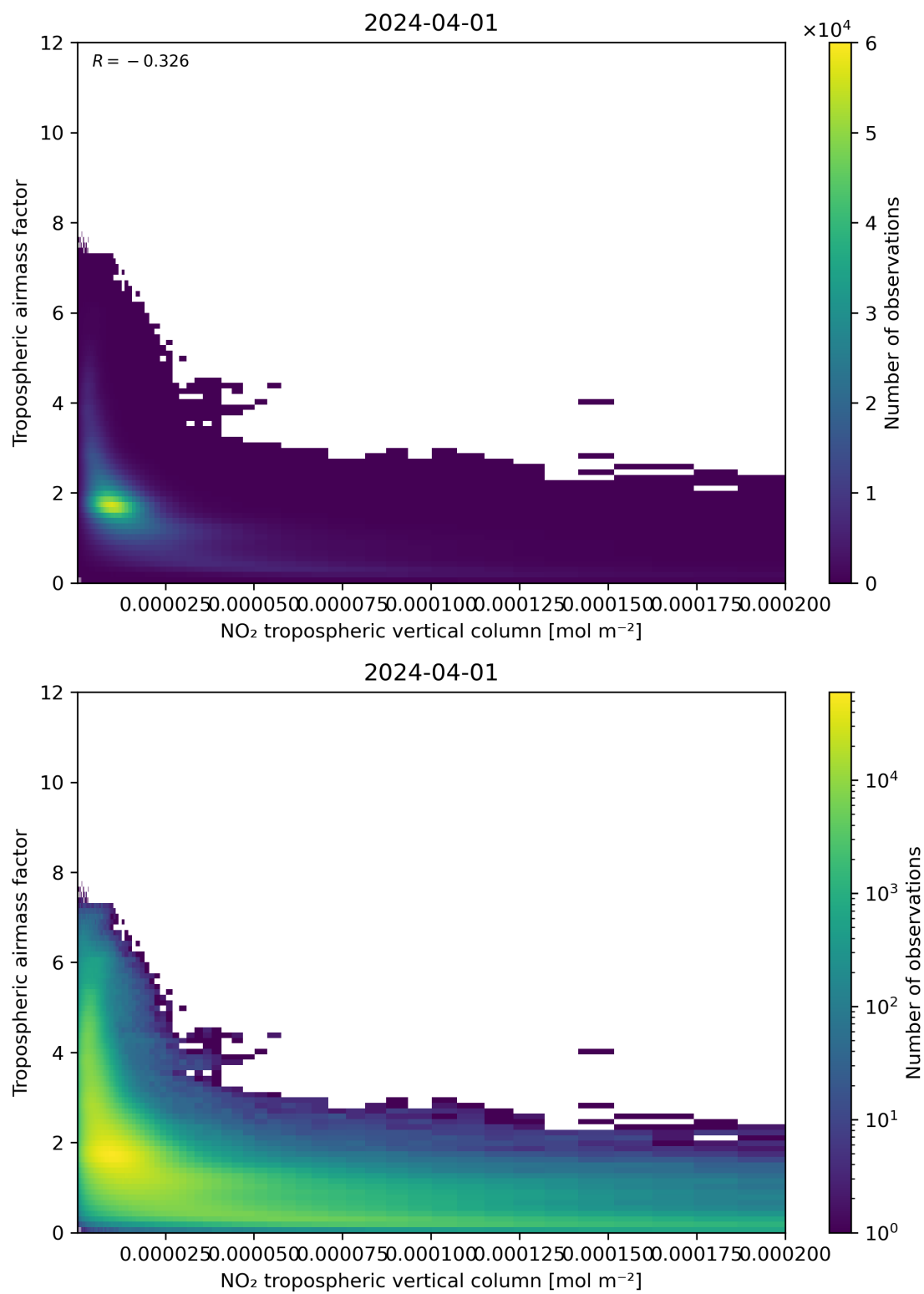
Figure 123: Scatter density plot of “NO 2 tropospheric vertical column” against “Tropospheric air mass factor” for 2024-03-31 to 2024-04-02.
