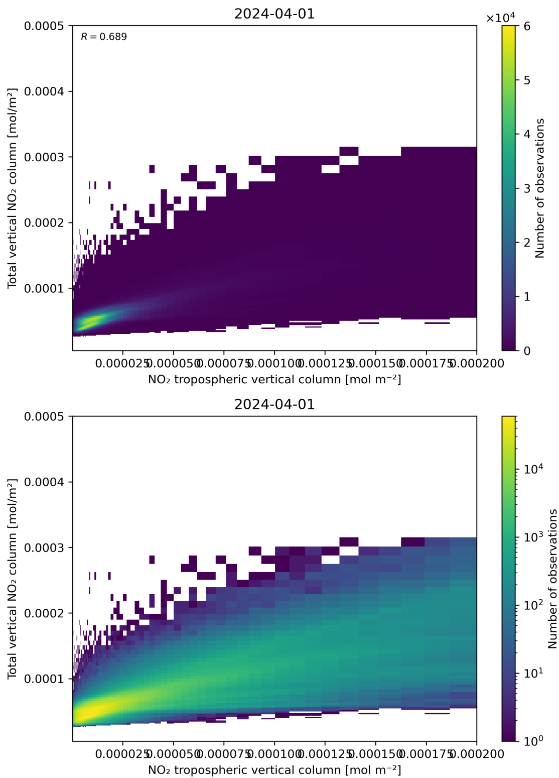
Figure 128: Scatter density plot of “NO 2 tropospheric vertical column” against “Total vertical NO 2 column” for 2024-03-31 to 2024-04-02.
