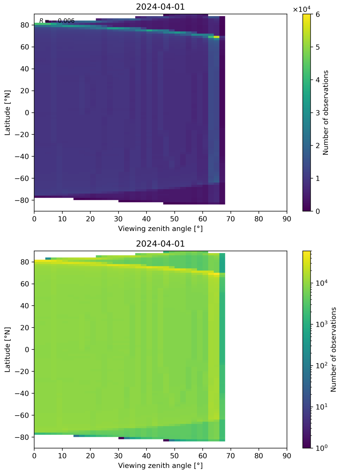
Figure 163: Scatter density plot of “Viewing zenith angle” against “Latitude” for 2024-03-31 to 2024-04-02.
