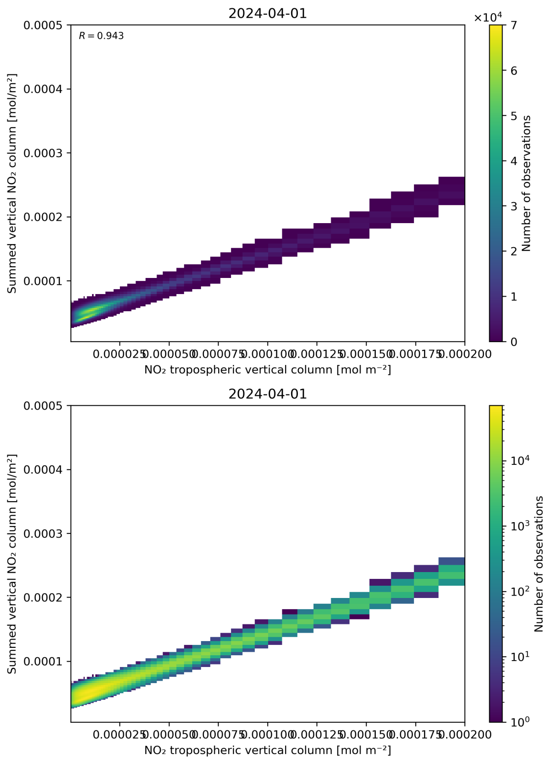
Figure 126: Scatter density plot of “NO 2 tropospheric vertical column” against “Summed vertical NO 2 column” for 2024-03-31 to 2024-04-02.
