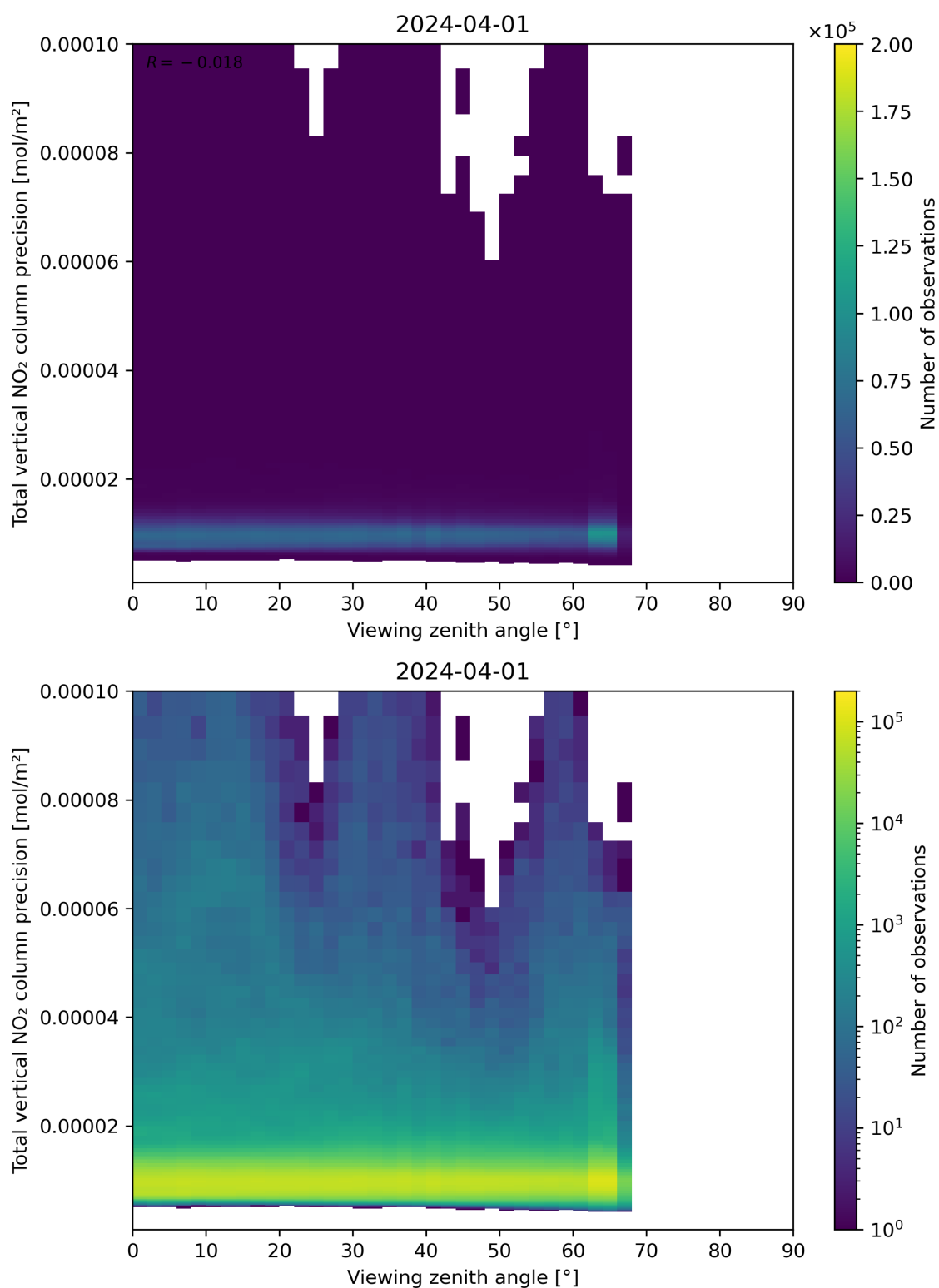
Figure 168: Scatter density plot of “Viewing zenith angle” against “Total vertical NO 2 column precision” for 2024-03-31 to 2024-04-02.
