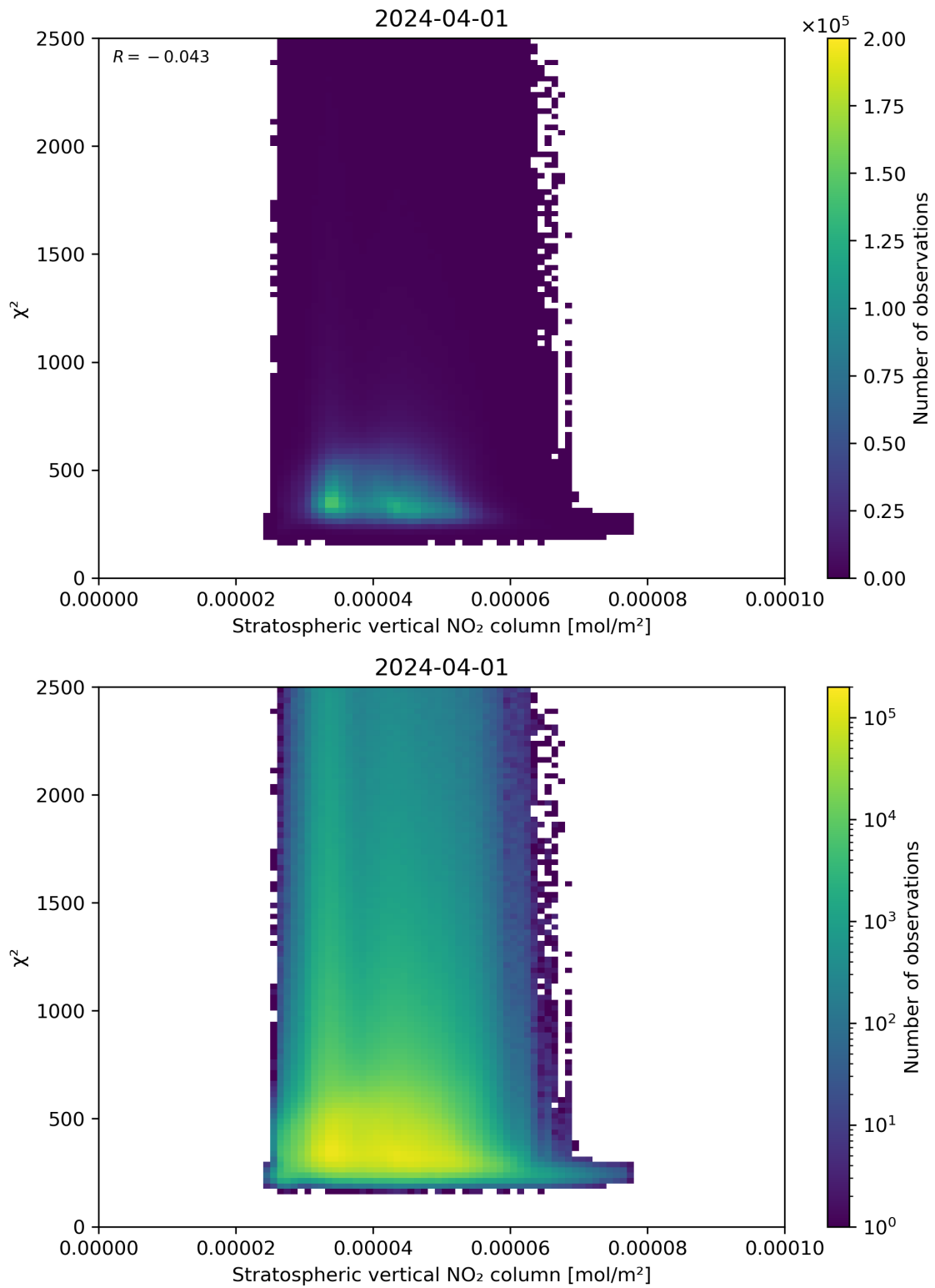
Figure 97: Scatter density plot of “Stratospheric vertical NO 2 column” against “ \chi^2 ” for 2024-03-31 to 2024-04-02.
