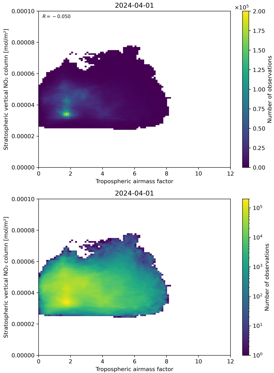
Figure 74: Scatter density plot of “Tropospheric air mass factor” against “Stratospheric vertical NO 2 column” for 2024-03-31 to 2024-04-02.
