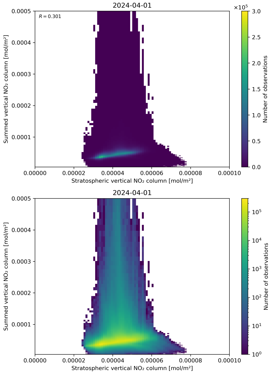
Figure 98: Scatter density plot of “Stratospheric vertical NO 2 column” against “Summed vertical NO 2 column” for 2024-03-31 to 2024-04-02.
