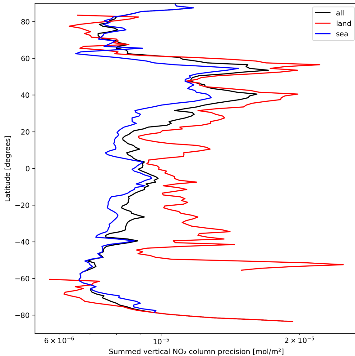
Figure 24: Zonal average of “Summed vertical NO 2 column precision” for 2024-03-31 to 2024-04-02.
