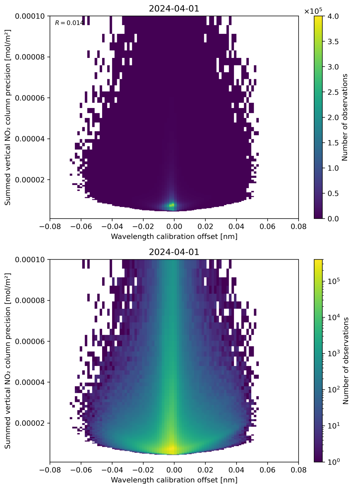
Figure 178: Scatter density plot of “Wavelength calibration offset” against “Summed vertical NO 2 column precision” for 2024-03-31 to 2024-04-02.
