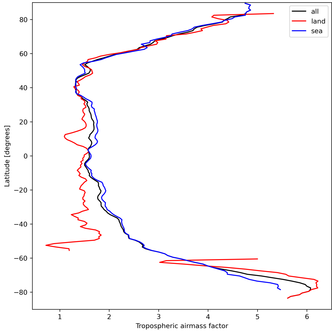
Figure 14: Zonal average of “Tropospheric airmass factor” for 2024-03-31 to 2024-04-02.
