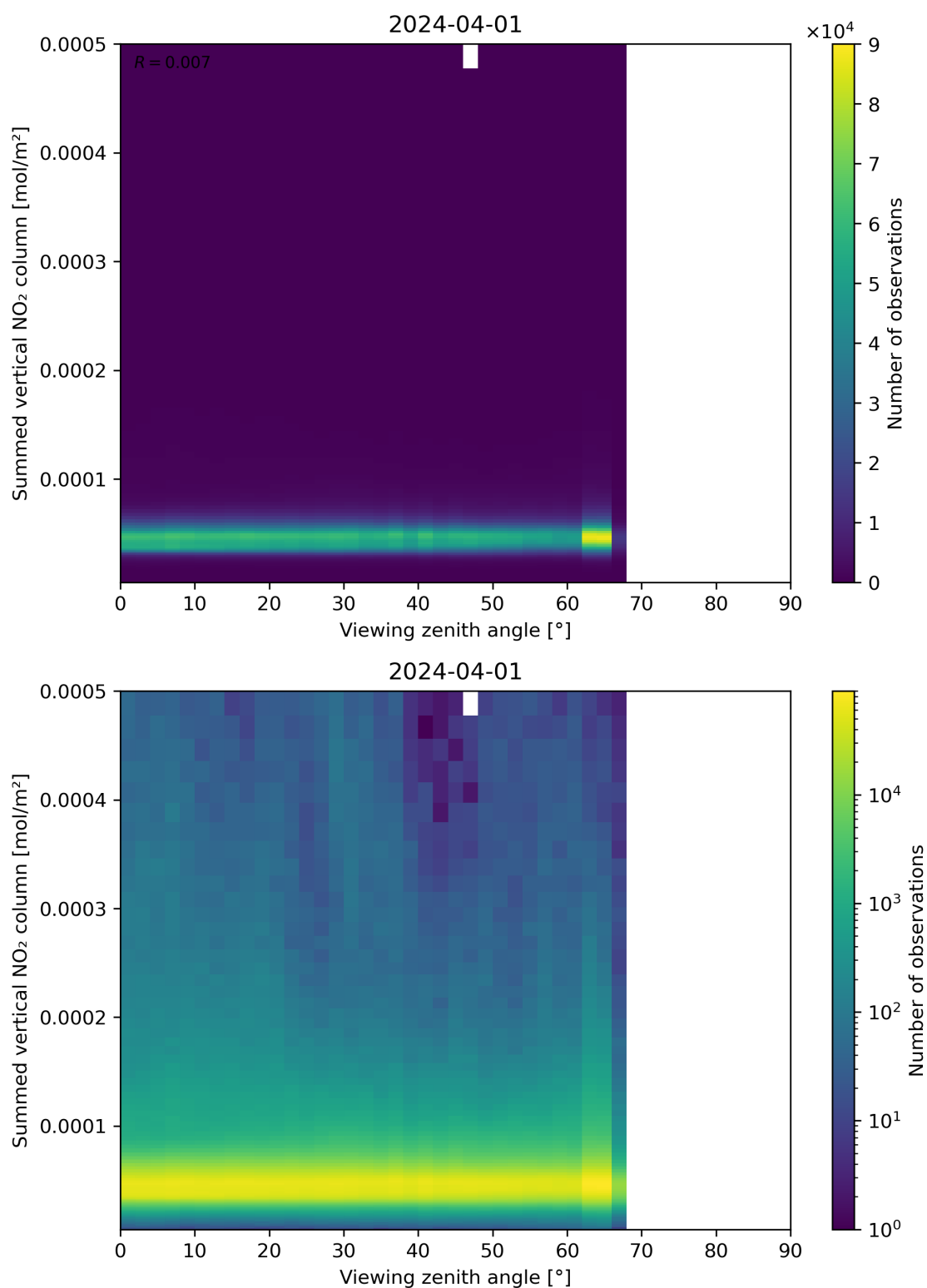
Figure 165: Scatter density plot of “Viewing zenith angle” against “Summed vertical NO 2 column” for 2024-03-31 to 2024-04-02.
