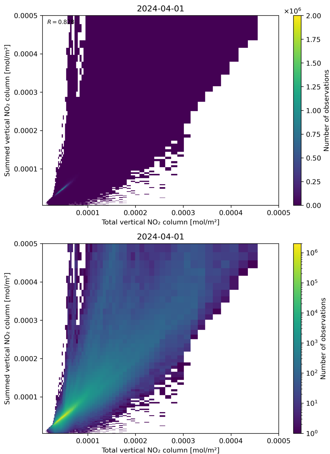
Figure 112: Scatter density plot of “Total vertical NO 2 column” against “Summed vertical NO 2 column” for 2024-03-31 to 2024-04-02.
