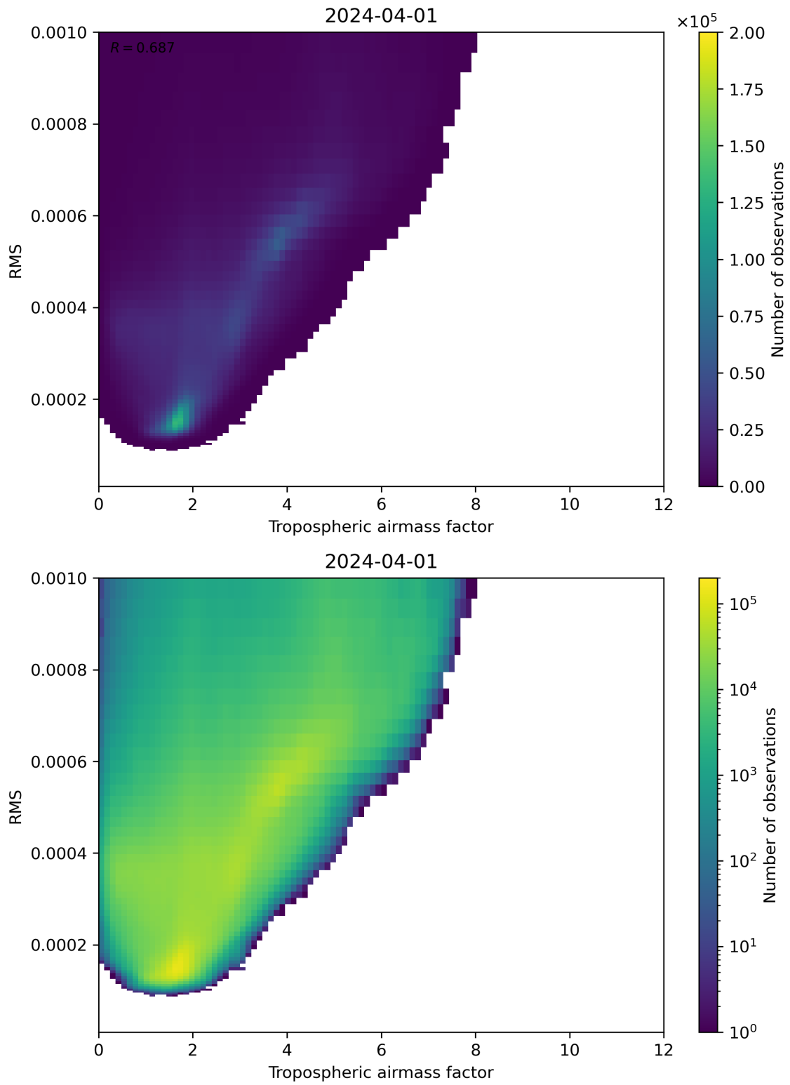
Figure 79: Scatter density plot of “Tropospheric airmass factor” against “RMS” for 2024-03-31 to 2024-04-02.
