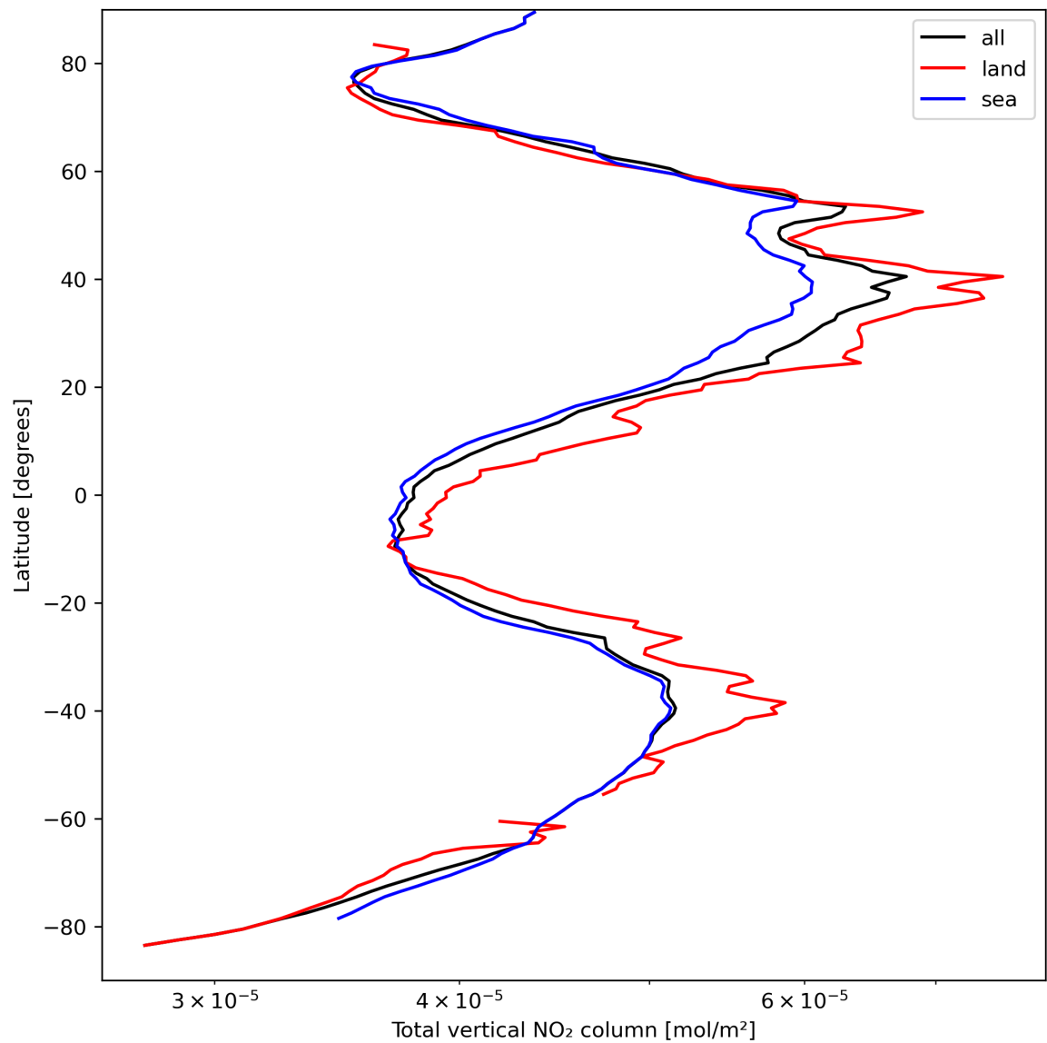
Figure 21: Zonal average of “Total vertical NO 2 column” for 2024-03-31 to 2024-04-02.
