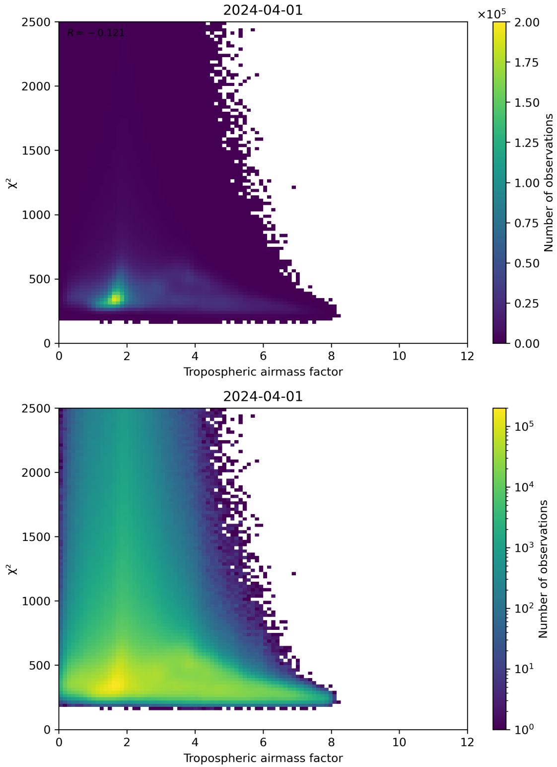
Figure 73: Scatter density plot of “Tropospheric airmass factor” against “ \chi^2 ” for 2024-03-31 to 2024-04-02.
