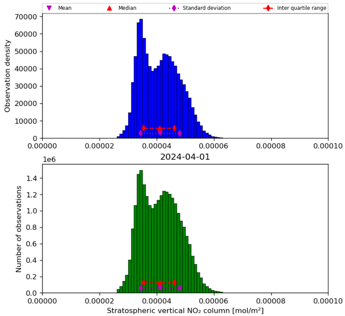
Figure 36: Histogram of “Stratospheric vertical NO 2 column” for 2024-03-31 to 2024-04-02
