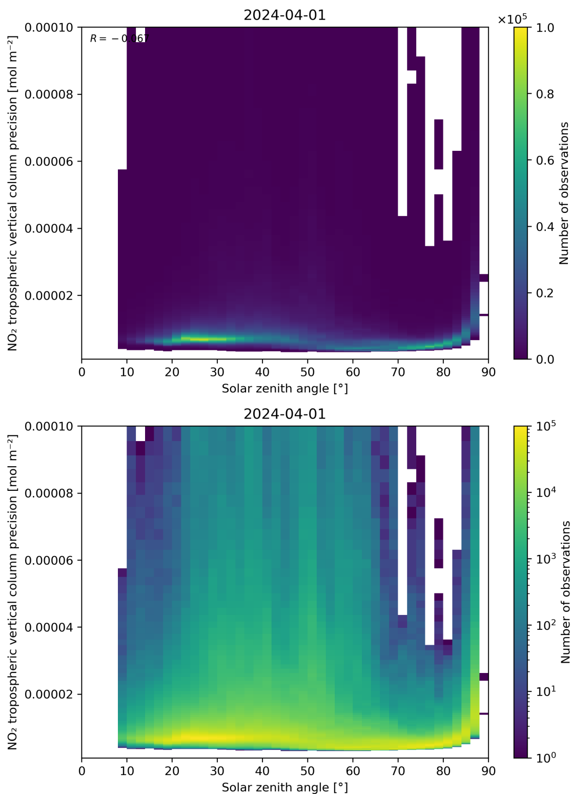
Figure 156: Scatter density plot of “Solar zenith angle” against “NO 2 tropospheric vertical column precision” for 2024-03-31 to 2024-04-02.
