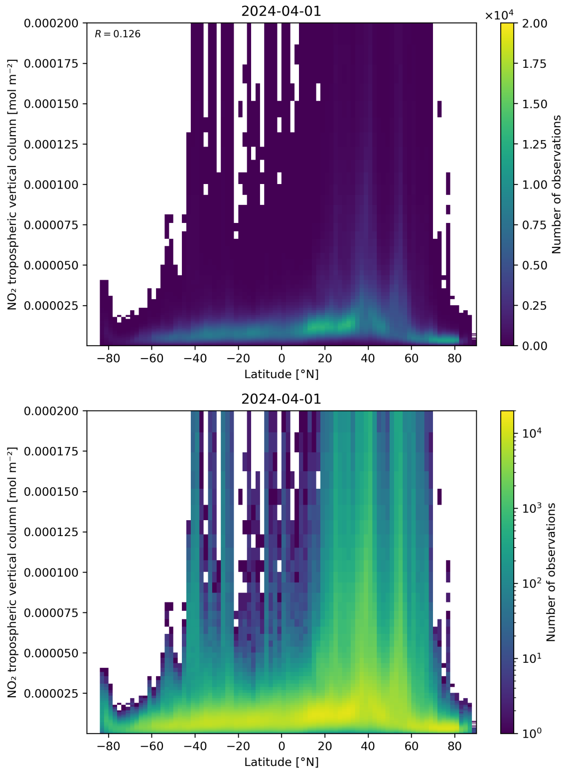
Figure 92: Scatter density plot of “Latitude” against “NO 2 tropospheric vertical column” for 2024-03-31 to 2024-04-02.
