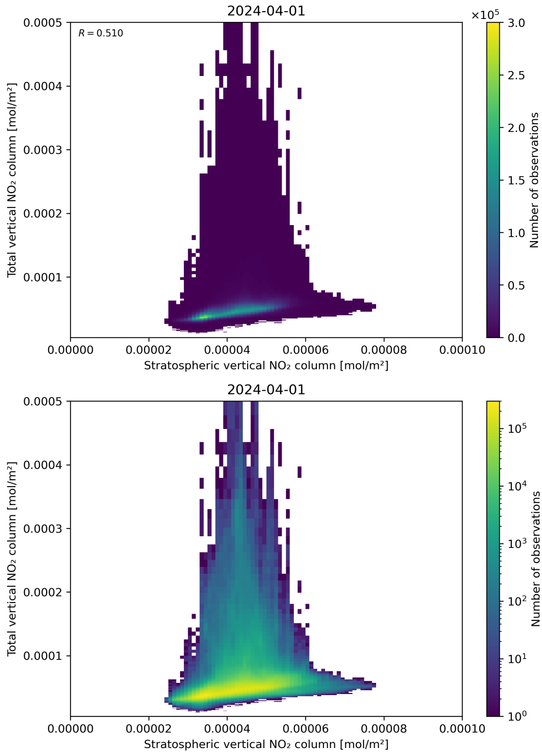
Figure 100: Scatter density plot of “Stratospheric vertical NO 2 column” against “Total vertical NO 2 column” for 2024-03-31 to 2024-04-02.
