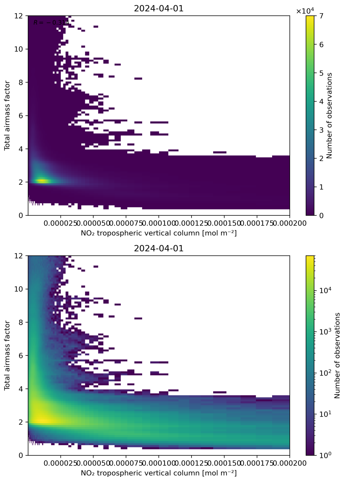
Figure 122: Scatter density plot of “NO 2 tropospheric vertical column” against “Total airmass factor” for 2024-03-31 to 2024-04-02.
