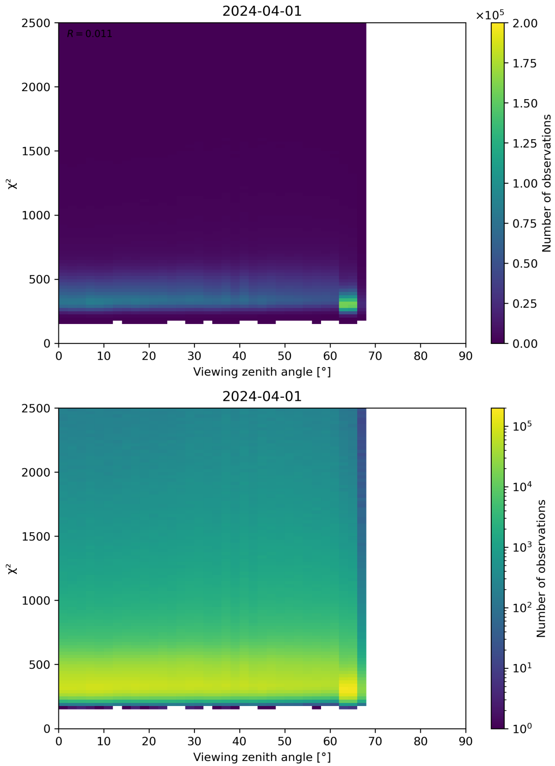
Figure 162: Scatter density plot of “Viewing zenith angle” against “ \chi^2 ” for 2024-03-31 to 2024-04-02.
