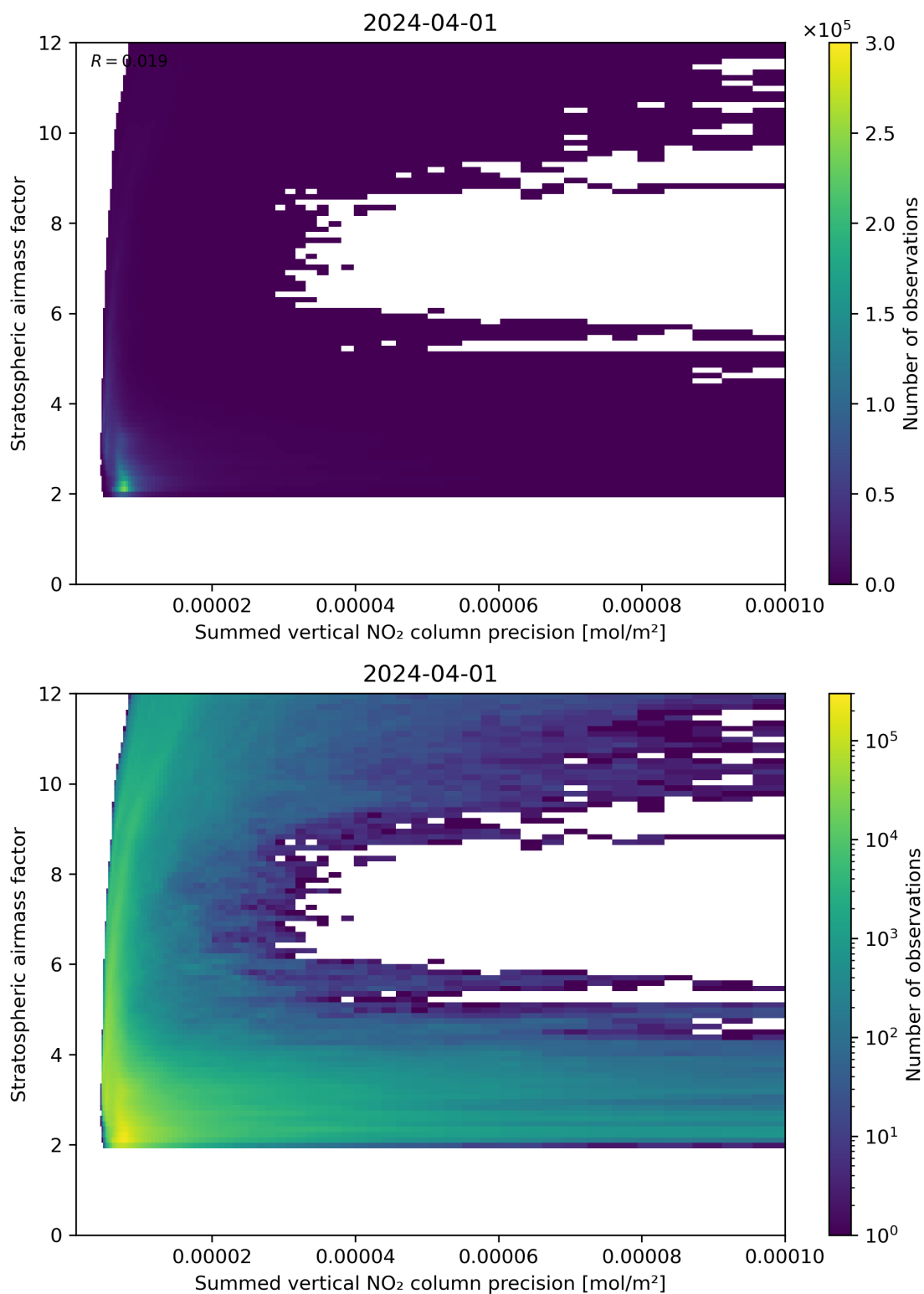
Figure 106: Scatter density plot of “Summed vertical NO 2 column precision” against “Stratospheric airmass factor” for 2024-03-31 to 2024-04-02.
