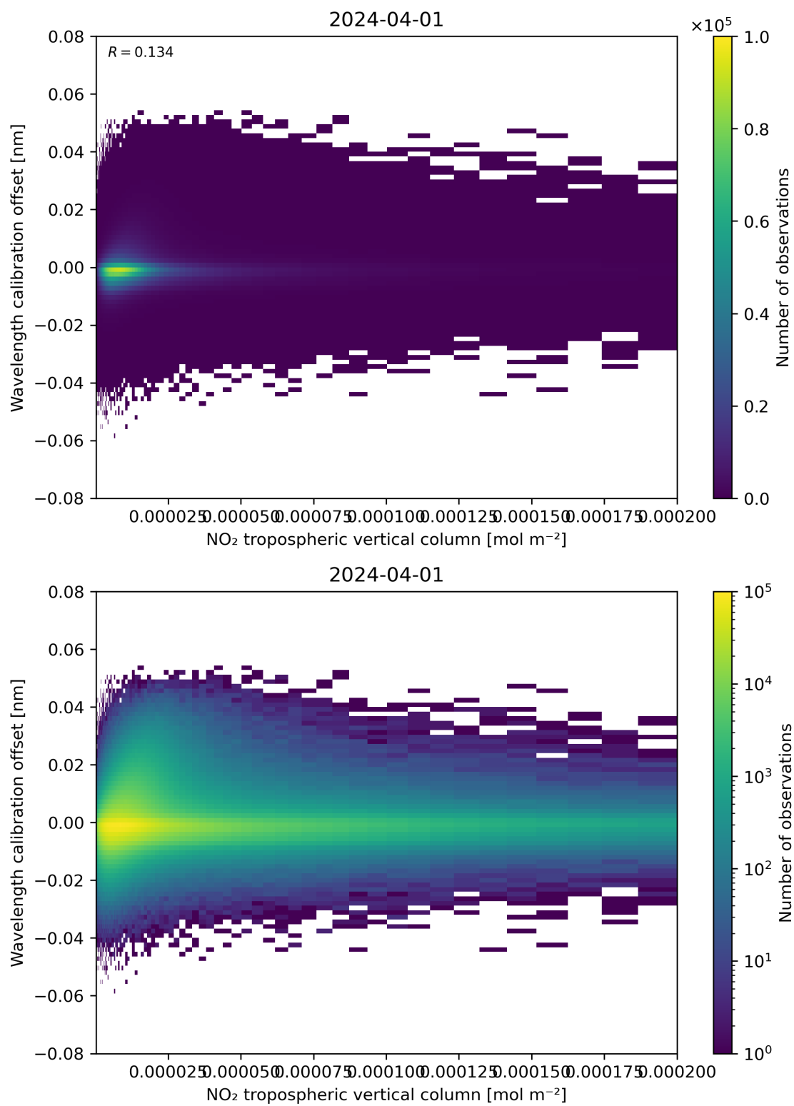
Figure 143: Scatter density plot of “NO 2 tropospheric vertical column” against “Wavelength calibration offset” for 2024-03-31 to 2024-04-02.
