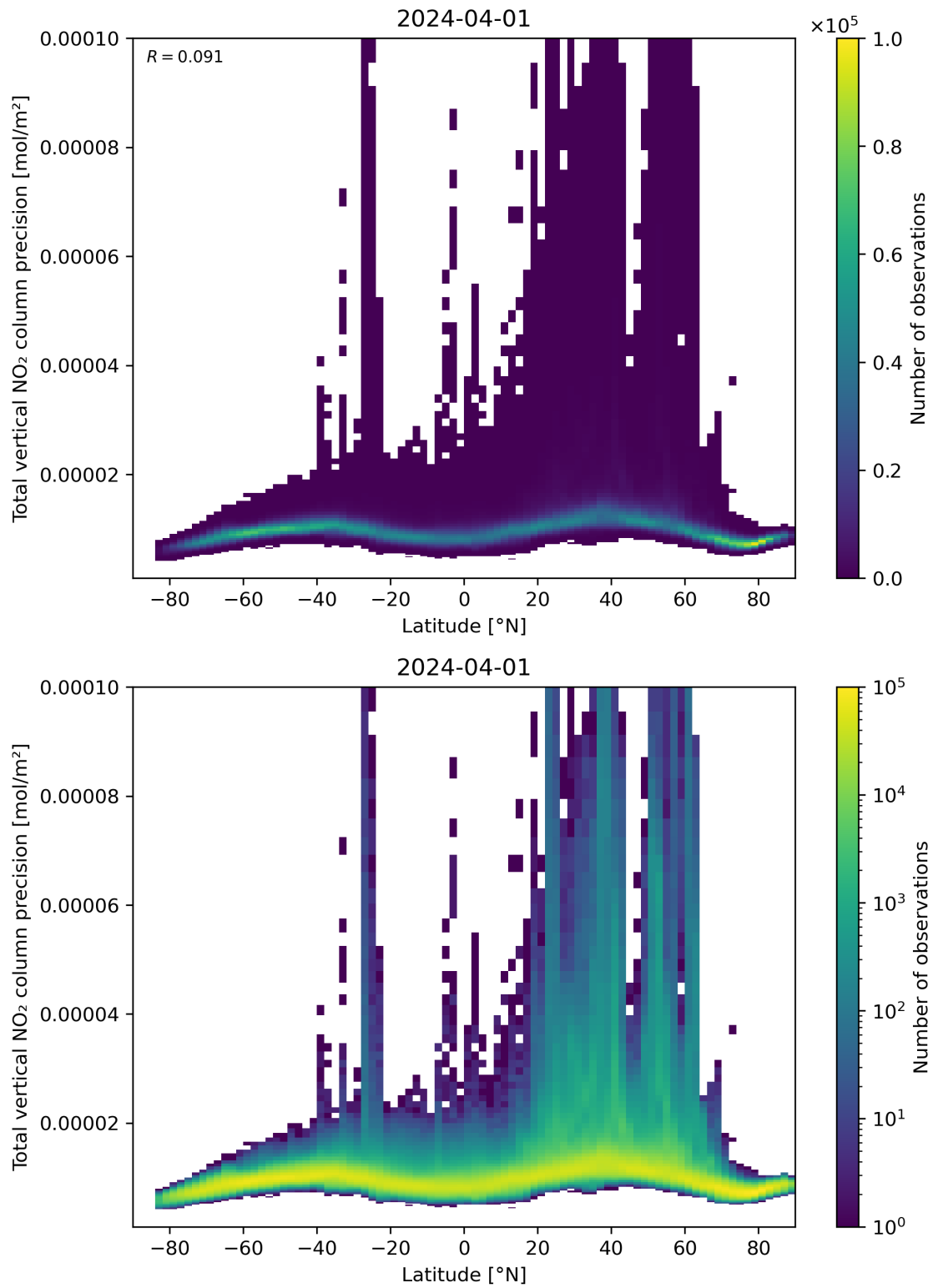
Figure 91: Scatter density plot of “Latitude” against “Total vertical NO 2 column precision” for 2024-03-31 to 2024-04-02.
