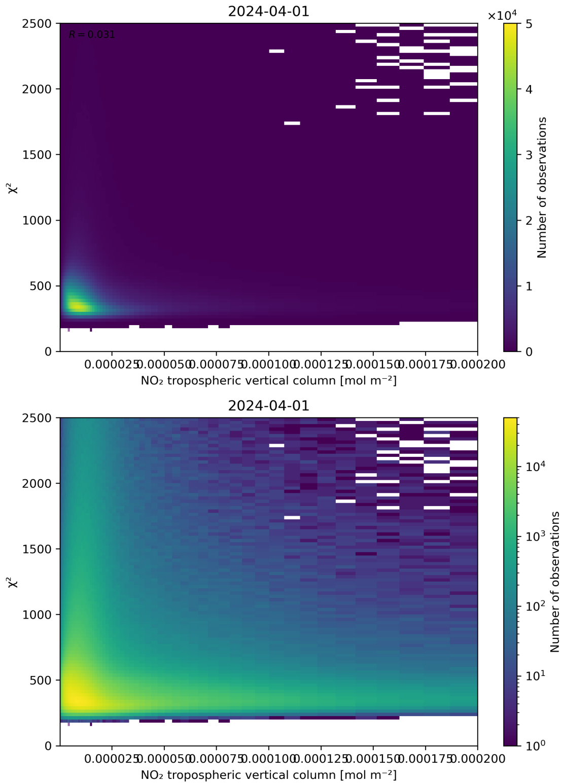
Figure 124: Scatter density plot of “NO 2 tropospheric vertical column” against “ \chi^2 ” for 2024-03-31 to 2024-04-02.
