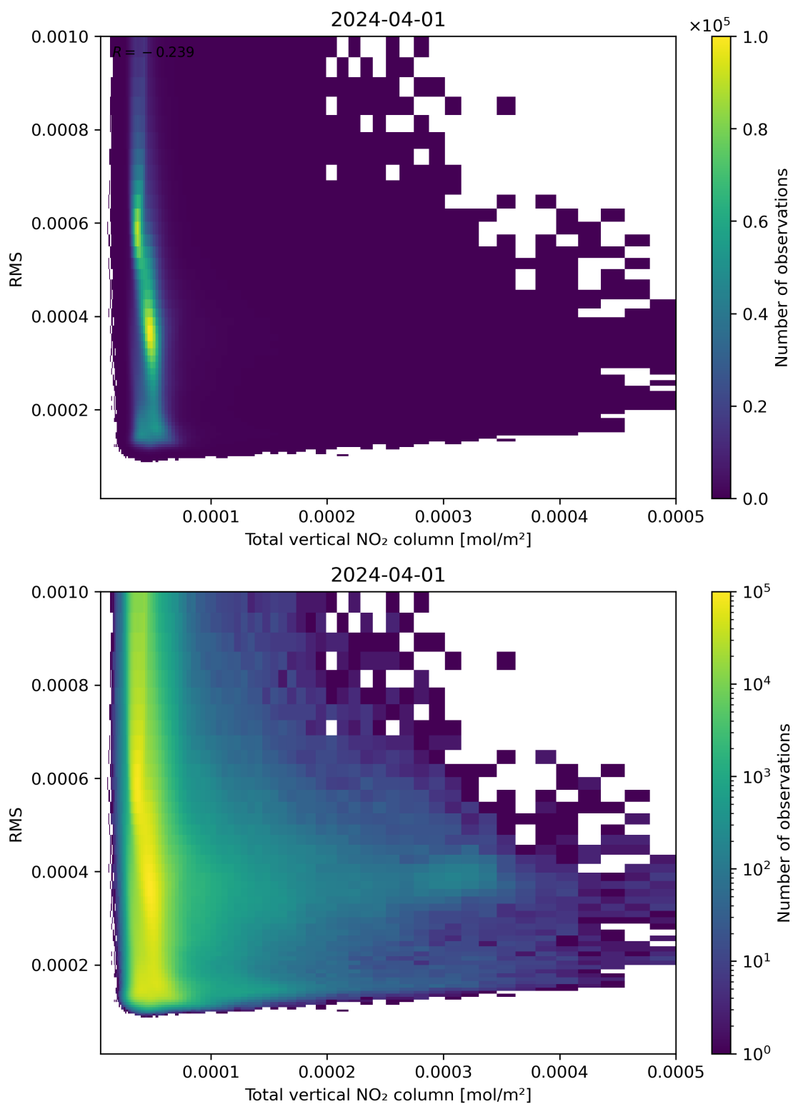
Figure 120: Scatter density plot of “Total vertical NO 2 column” against “RMS” for 2024-03-31 to 2024-04-02.
