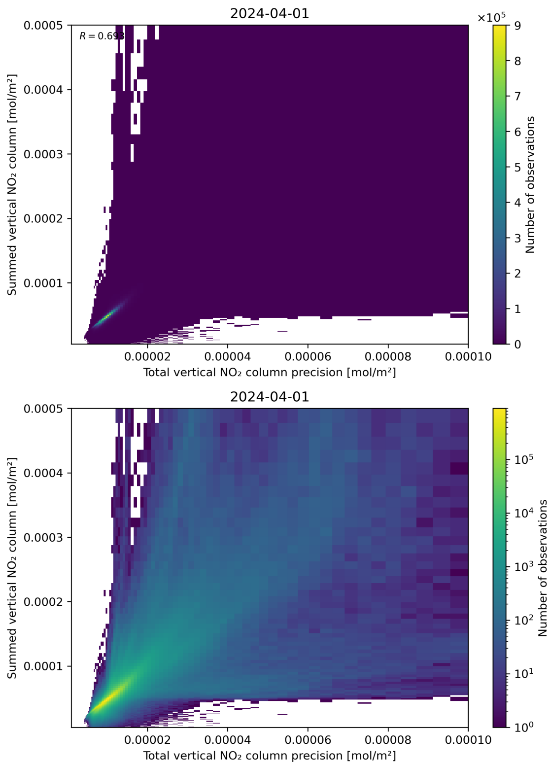
Figure 117: Scatter density plot of “Total vertical NO 2 column precision” against “Summed vertical NO 2 column” for 2024-03-31 to 2024-04-02.
