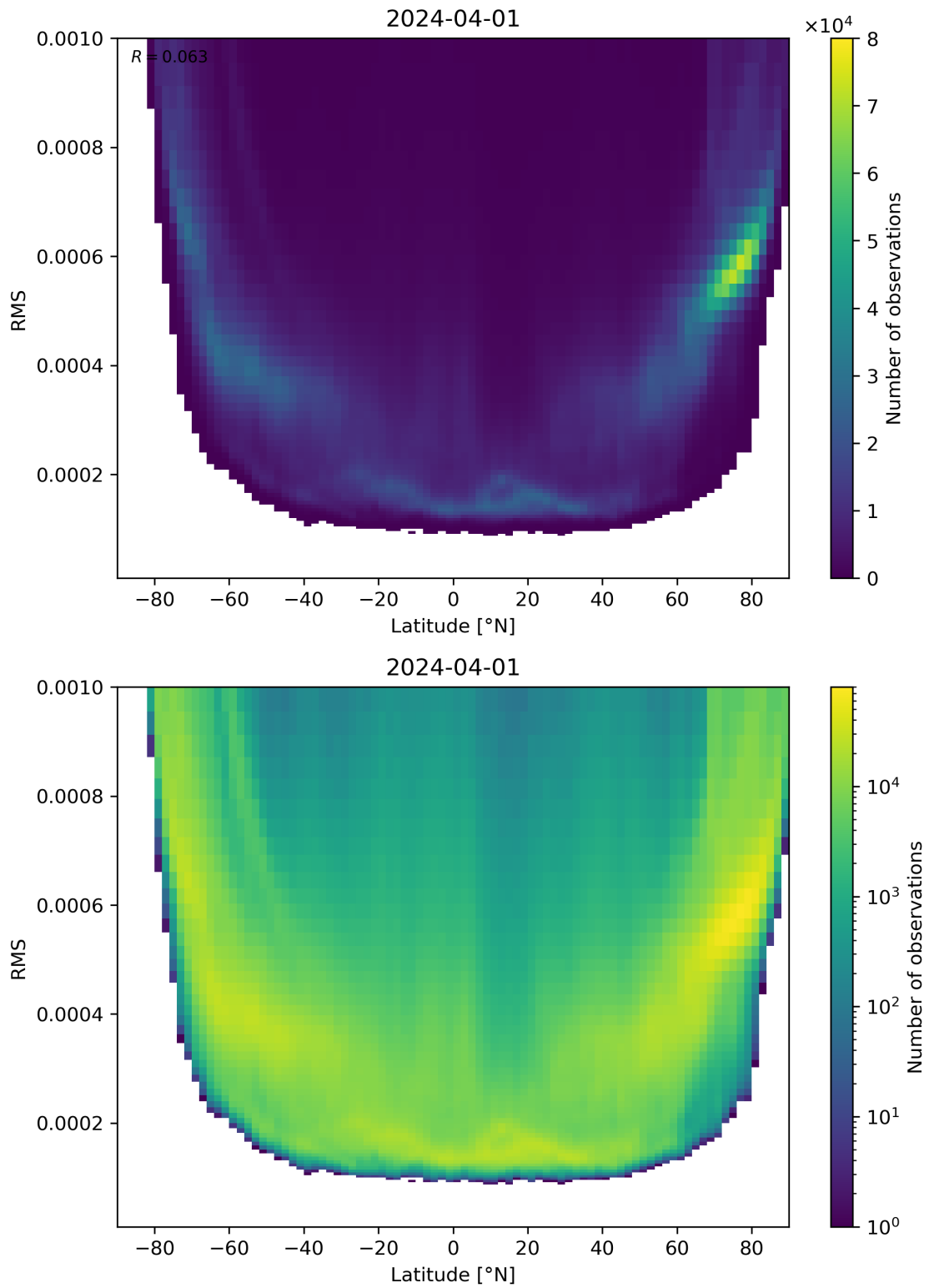
Figure 94: Scatter density plot of “Latitude” against “RMS” for 2024-03-31 to 2024-04-02.
