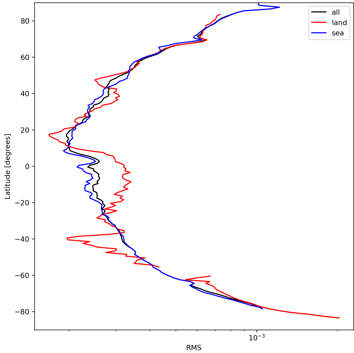
Figure 26: Zonal average of “RMS” for 2024-03-31 to 2024-04-02.
