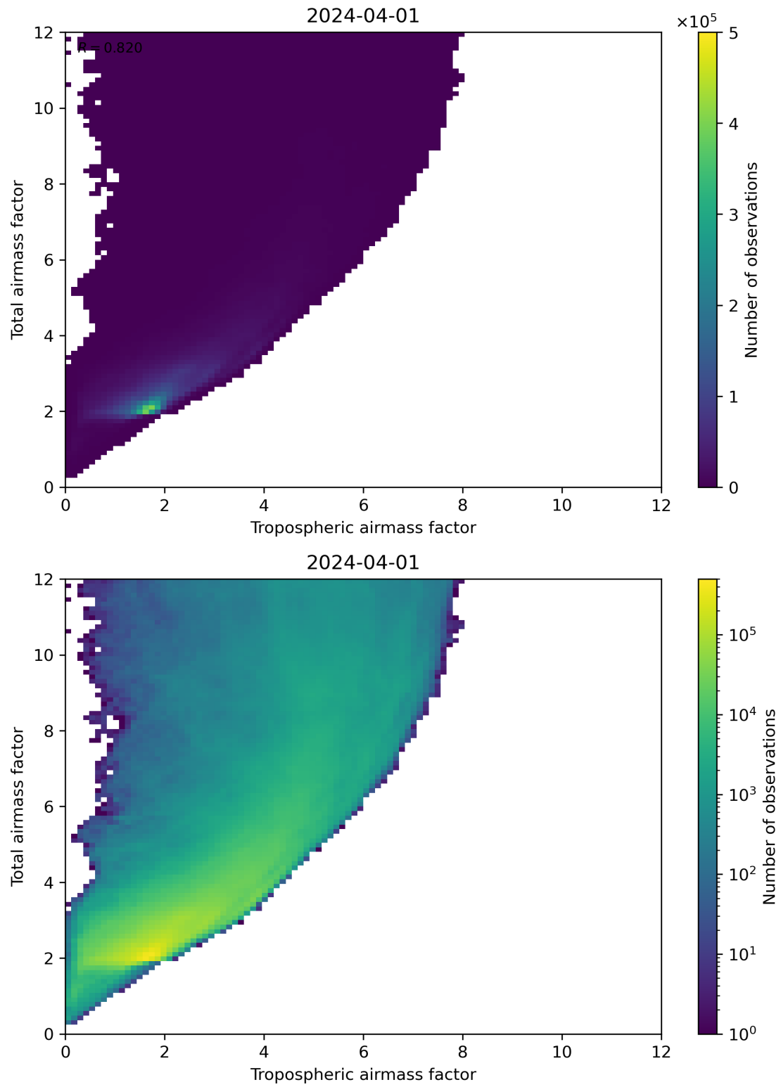
Figure 72: Scatter density plot of “Tropospheric airmass factor” against “Total airmass factor” for 2024-03-31 to 2024-04-02.
