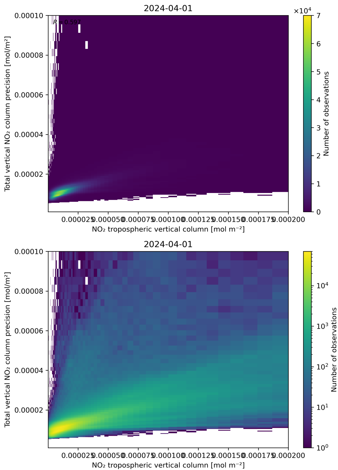
Figure 129: Scatter density plot of “NO 2 tropospheric vertical column” against “Total vertical NO 2 column precision” for 2024-03-31 to 2024-04-02.
