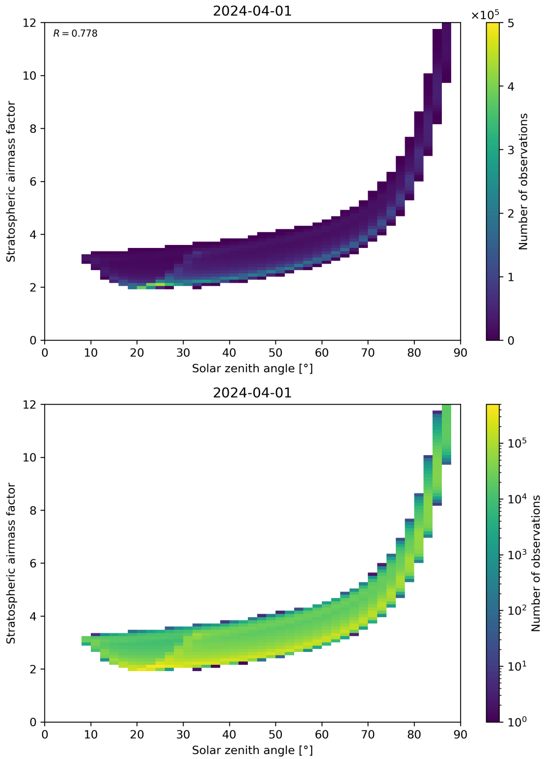
Figure 145: Scatter density plot of “Solar zenith angle” against “Stratospheric airmass factor” for 2024-03-31 to 2024-04-02.
