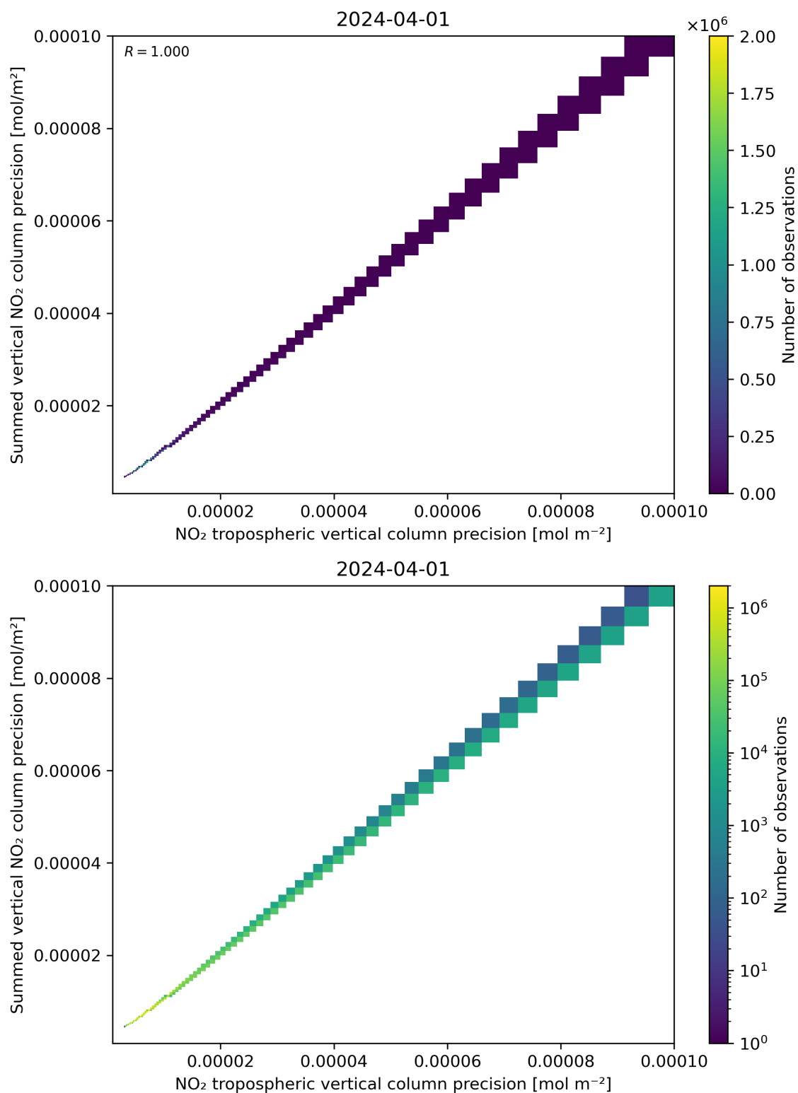
Figure 137: Scatter density plot of “NO 2 tropospheric vertical column precision” against “Summed vertical NO 2 column precision” for 2024-03-31 to 2024-04-02.
