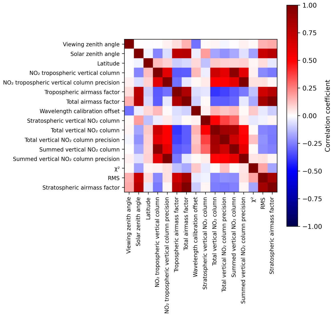
Figure 2: Map of correlation matrix for 2024-03-31 to 2024-04-02.
