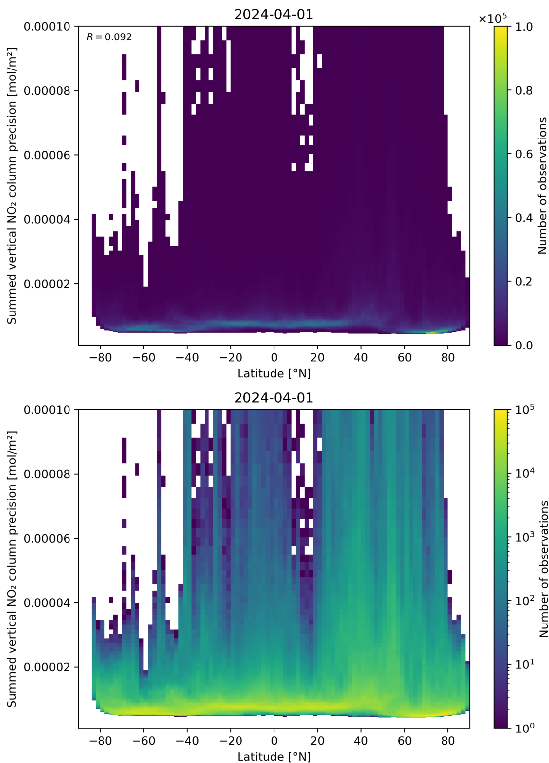
Figure 89: Scatter density plot of “Latitude” against “Summed vertical NO 2 column precision” for 2024-03-31 to 2024-04-02.
