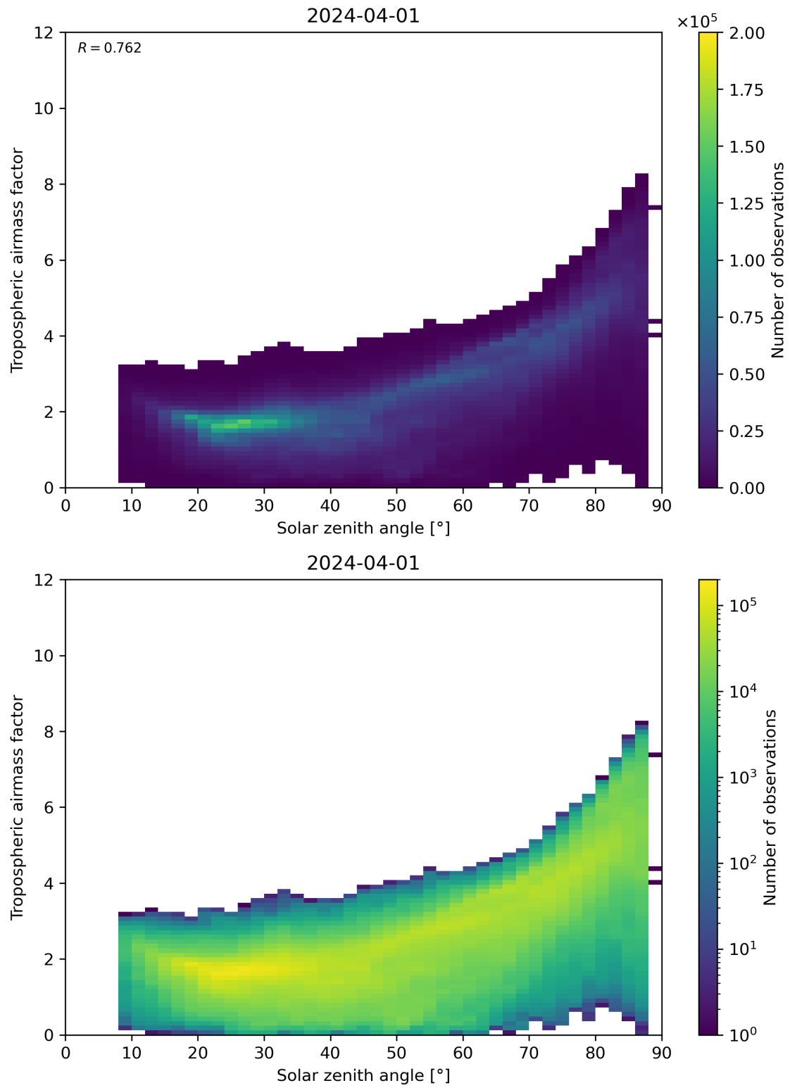
Figure 147: Scatter density plot of “Solar zenith angle” against “Tropospheric airmass factor” for 2024-03-31 to 2024-04-02.
