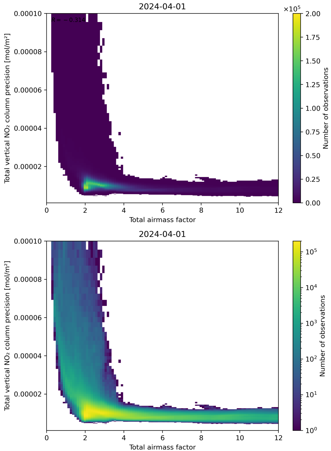
Figure 68: Scatter density plot of “Total airmass factor” against “Total vertical NO 2 column precision” for 2024-03-31 to 2024-04-02.
