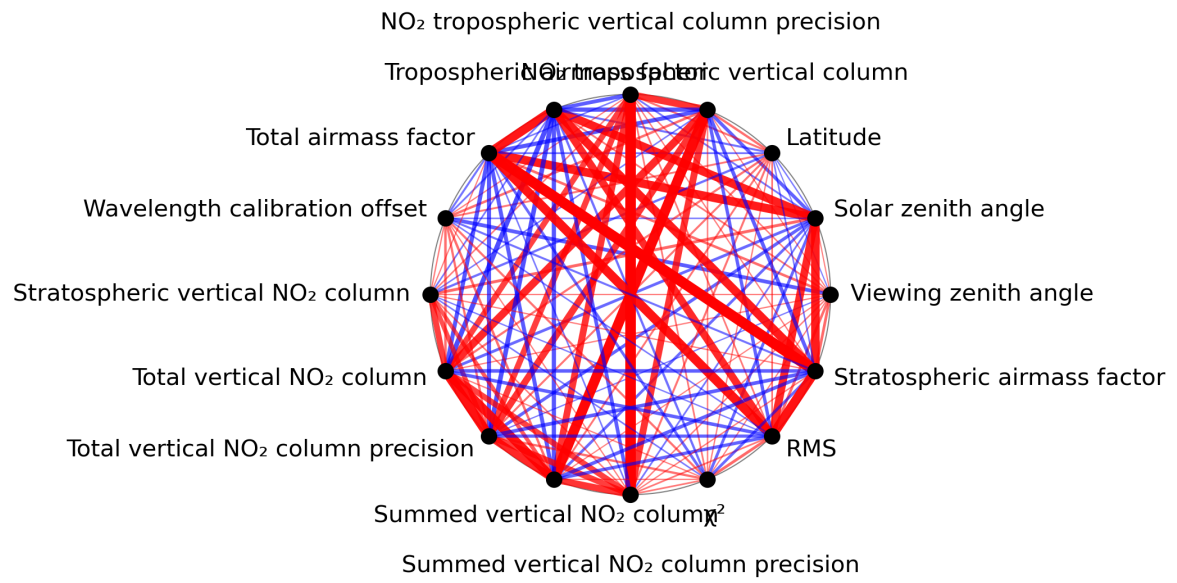
Figure 1: Map of correlation graph for 2024-03-31 to 2024-04-02.
