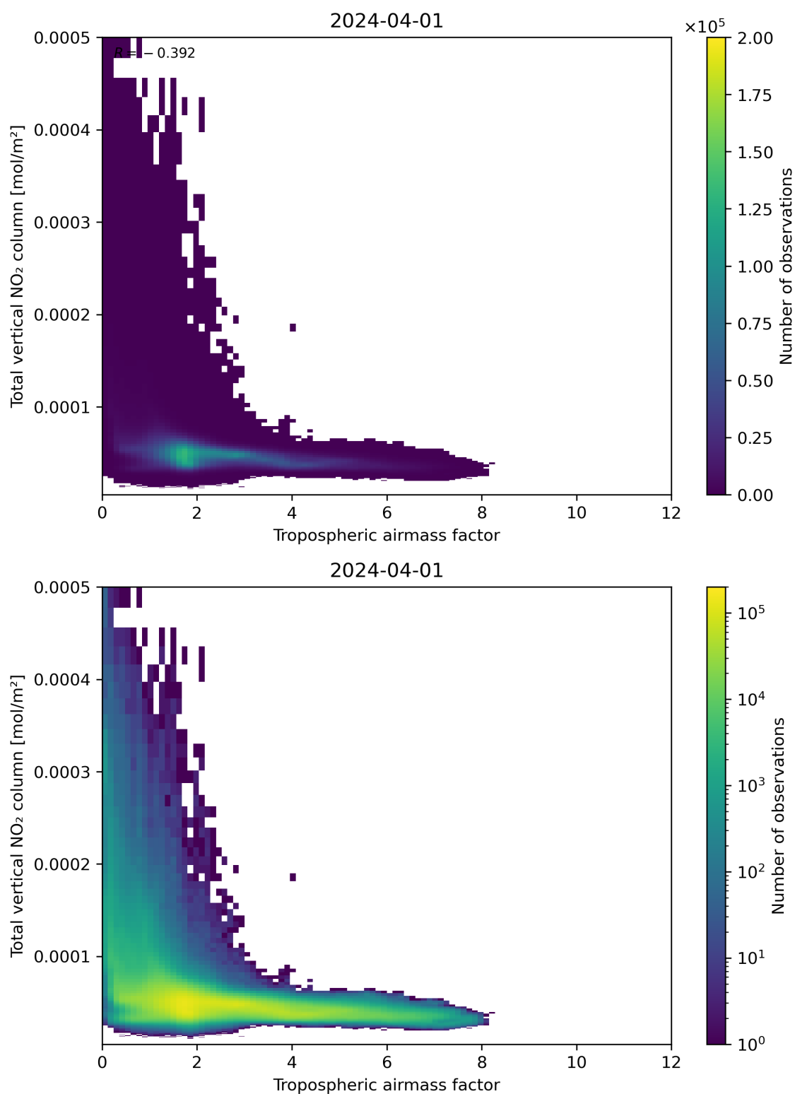
Figure 77: Scatter density plot of “Tropospheric airmass factor” against “Total vertical NO 2 column” for 2024-03-31 to 2024-04-02.
