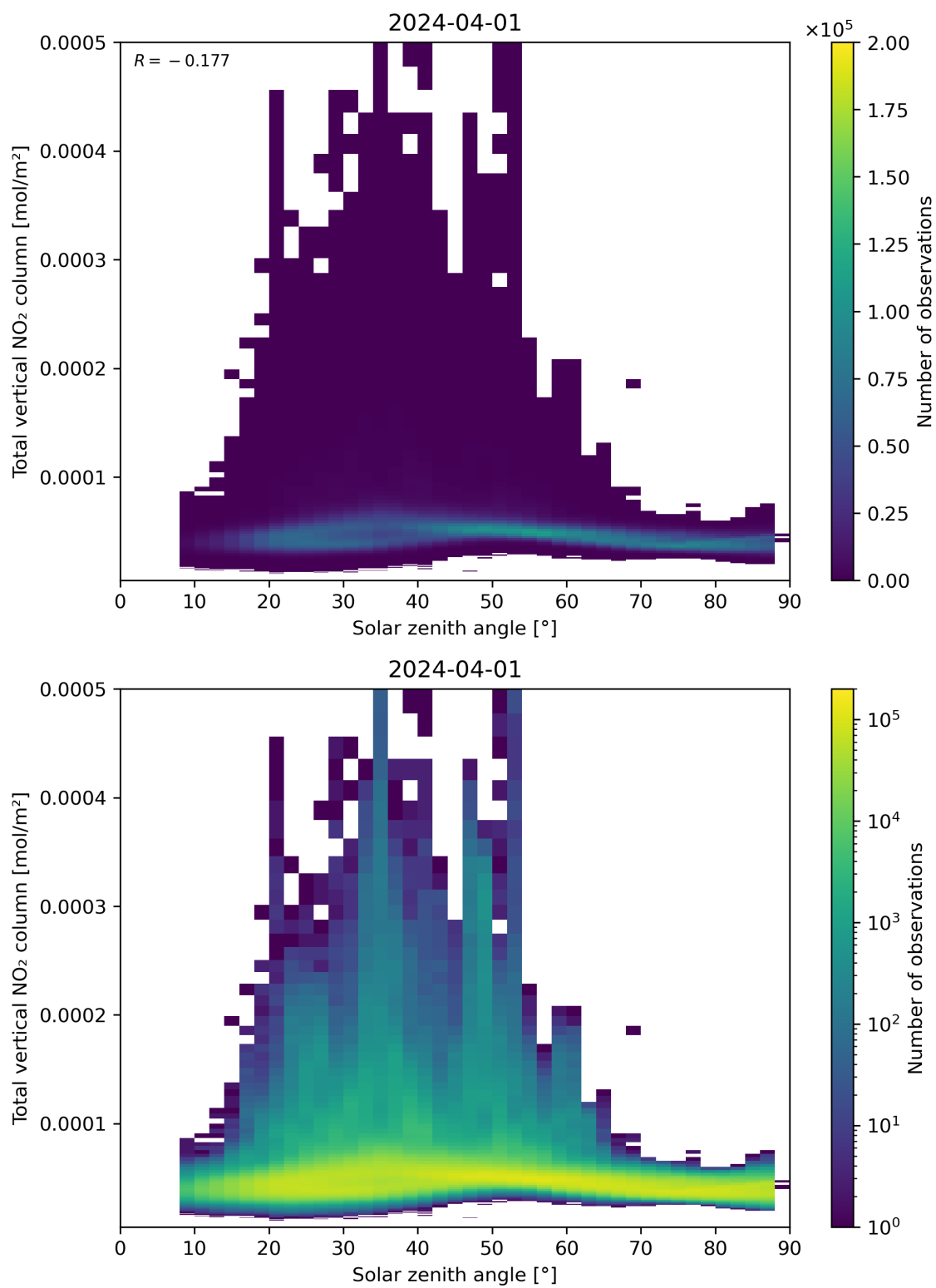
Figure 153: Scatter density plot of “Solar zenith angle” against “Total vertical NO 2 column” for 2024-03-31 to 2024-04-02.
