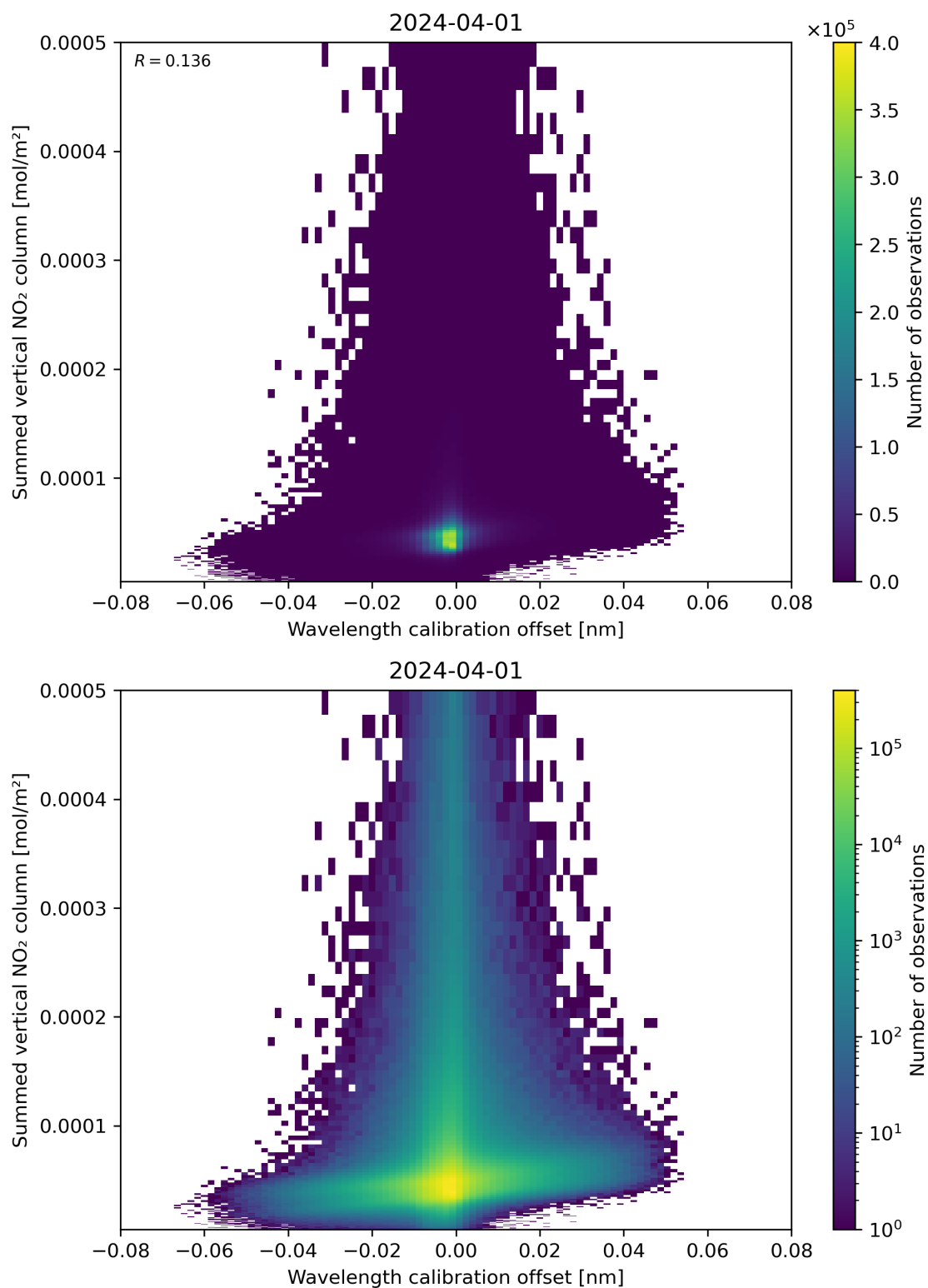
Figure 177: Scatter density plot of “Wavelength calibration offset” against “Summed vertical NO 2 column” for 2024-03-31 to 2024-04-02.
