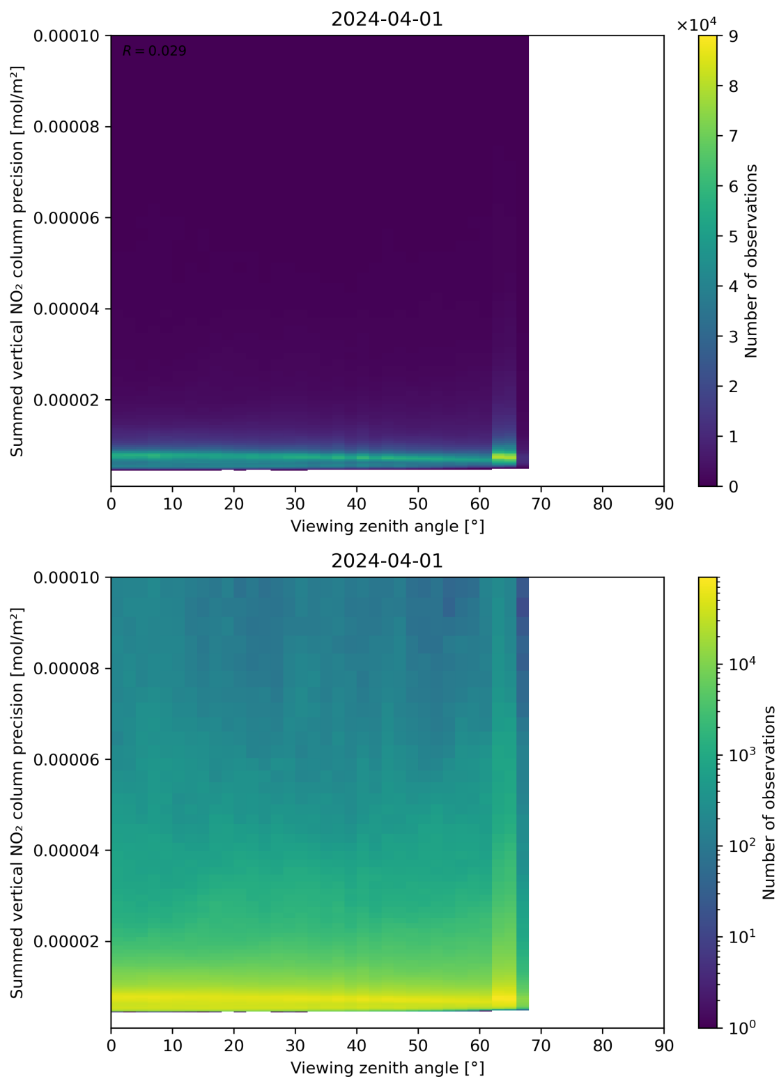
Figure 166: Scatter density plot of “Viewing zenith angle” against “Summed vertical NO 2 column precision” for 2024-03-31 to 2024-04-02.
