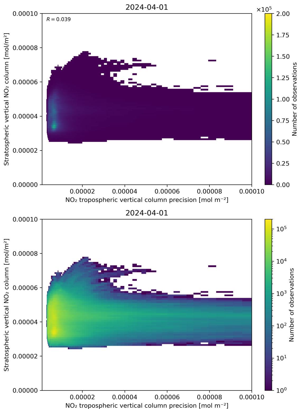
Figure 135: Scatter density plot of “NO 2 tropospheric vertical column precision” against “Stratospheric vertical NO 2 column” for 2024-03-31 to 2024-04-02.
