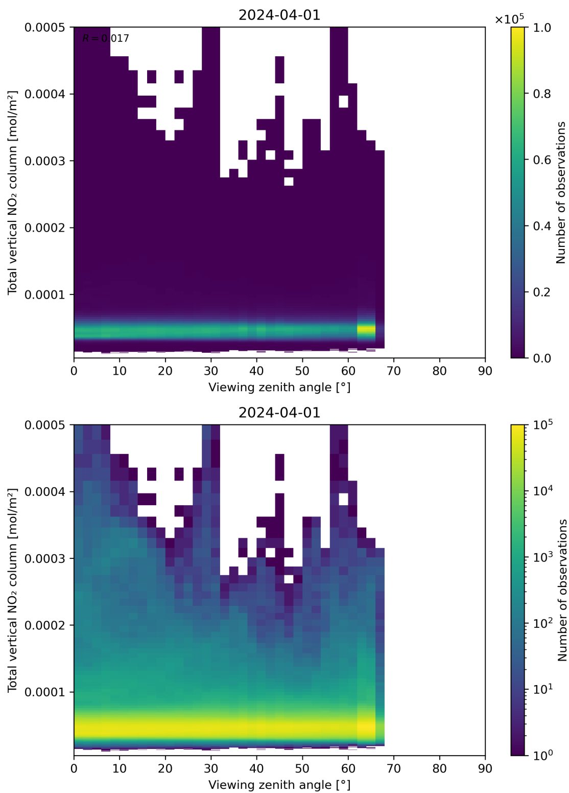
Figure 167: Scatter density plot of “Viewing zenith angle” against “Total vertical NO 2 column” for 2024-03-31 to 2024-04-02.
