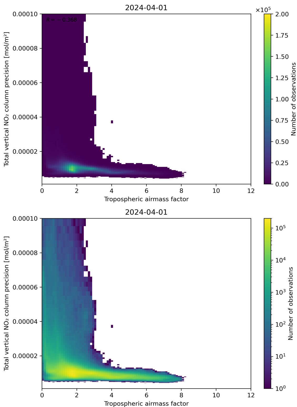
Figure 78: Scatter density plot of “Tropospheric air mass factor” against “Total vertical NO 2 column precision” for 2024-03-31 to 2024-04-02.
