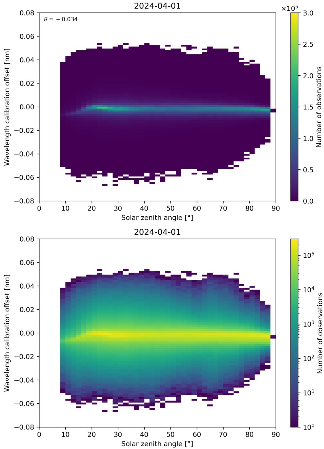
Figure 158: Scatter density plot of “Solar zenith angle” against “Wavelength calibration offset” for 2024-03-31 to 2024-04-02.
