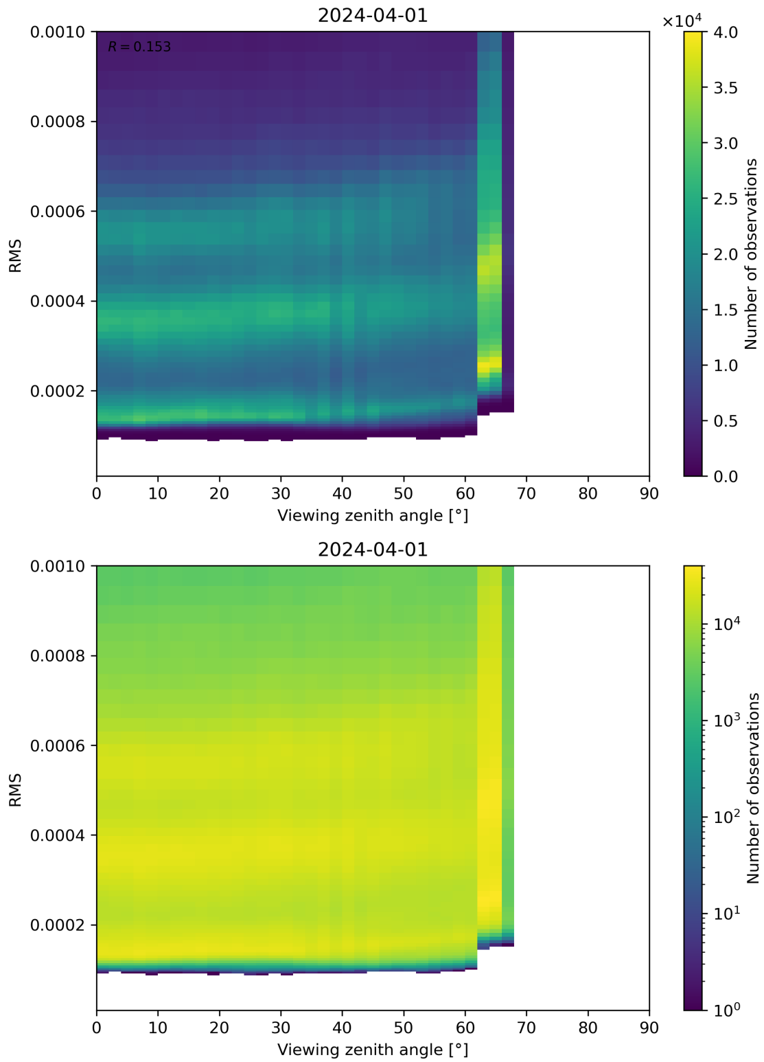
Figure 171: Scatter density plot of “Viewing zenith angle” against “RMS” for 2024-03-31 to 2024-04-02.
