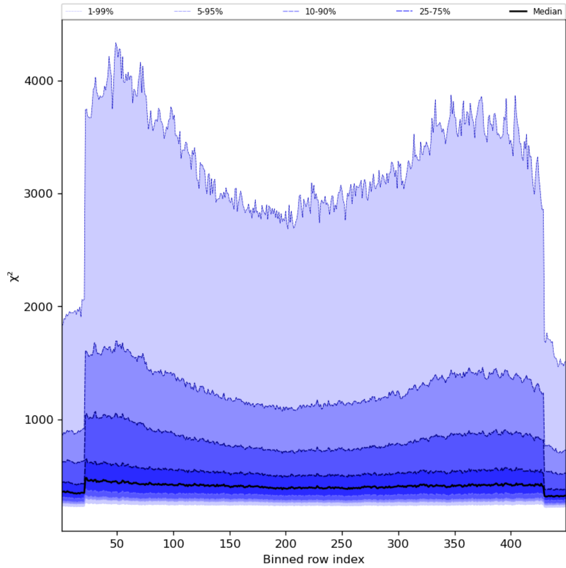
Figure 59: Along track statistics of “ \chi^2 ” for 2024-03-31 to 2024-04-02
