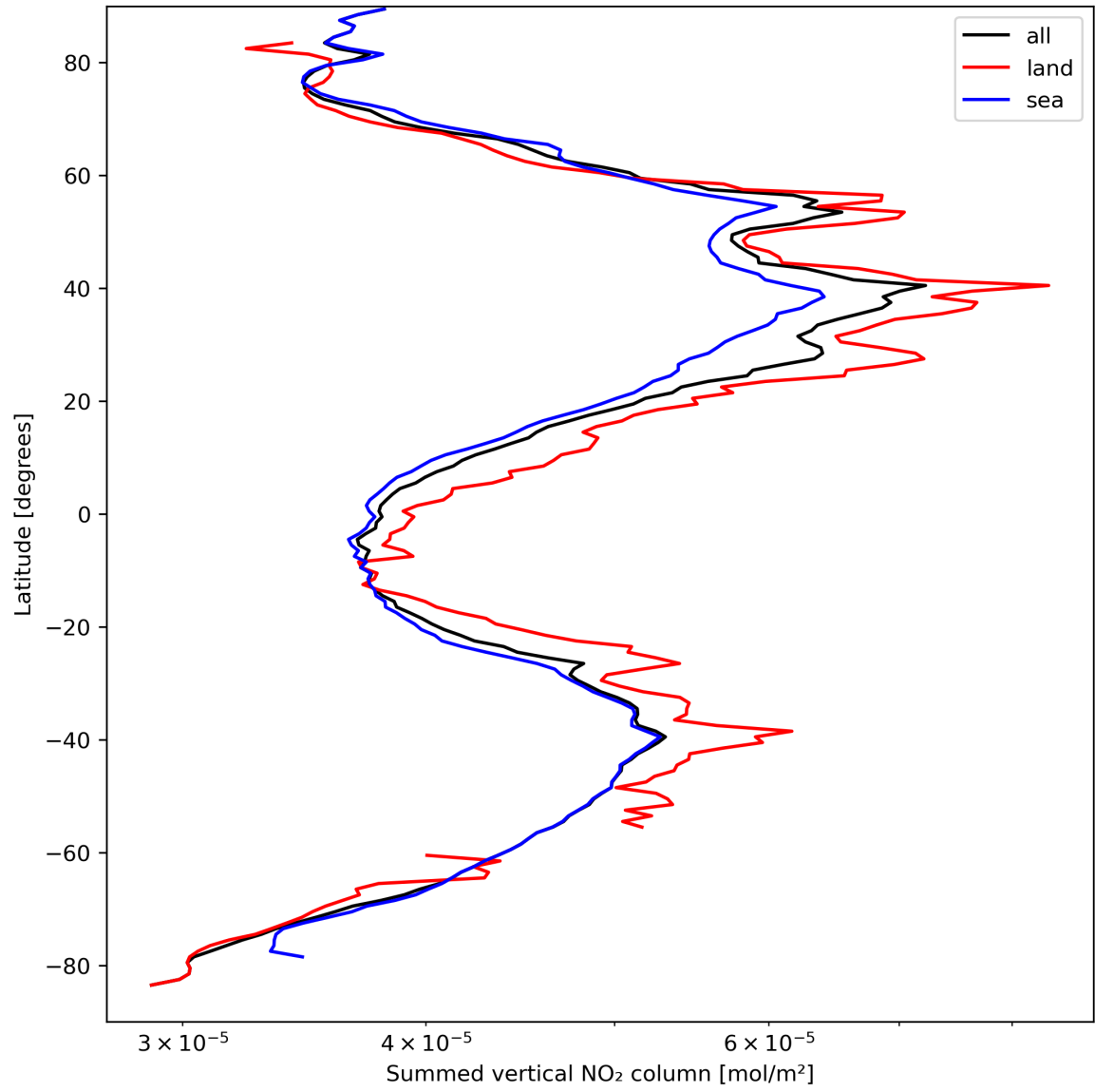
Figure 23: Zonal average of “Summed vertical NO 2 column” for 2024-03-31 to 2024-04-02.
