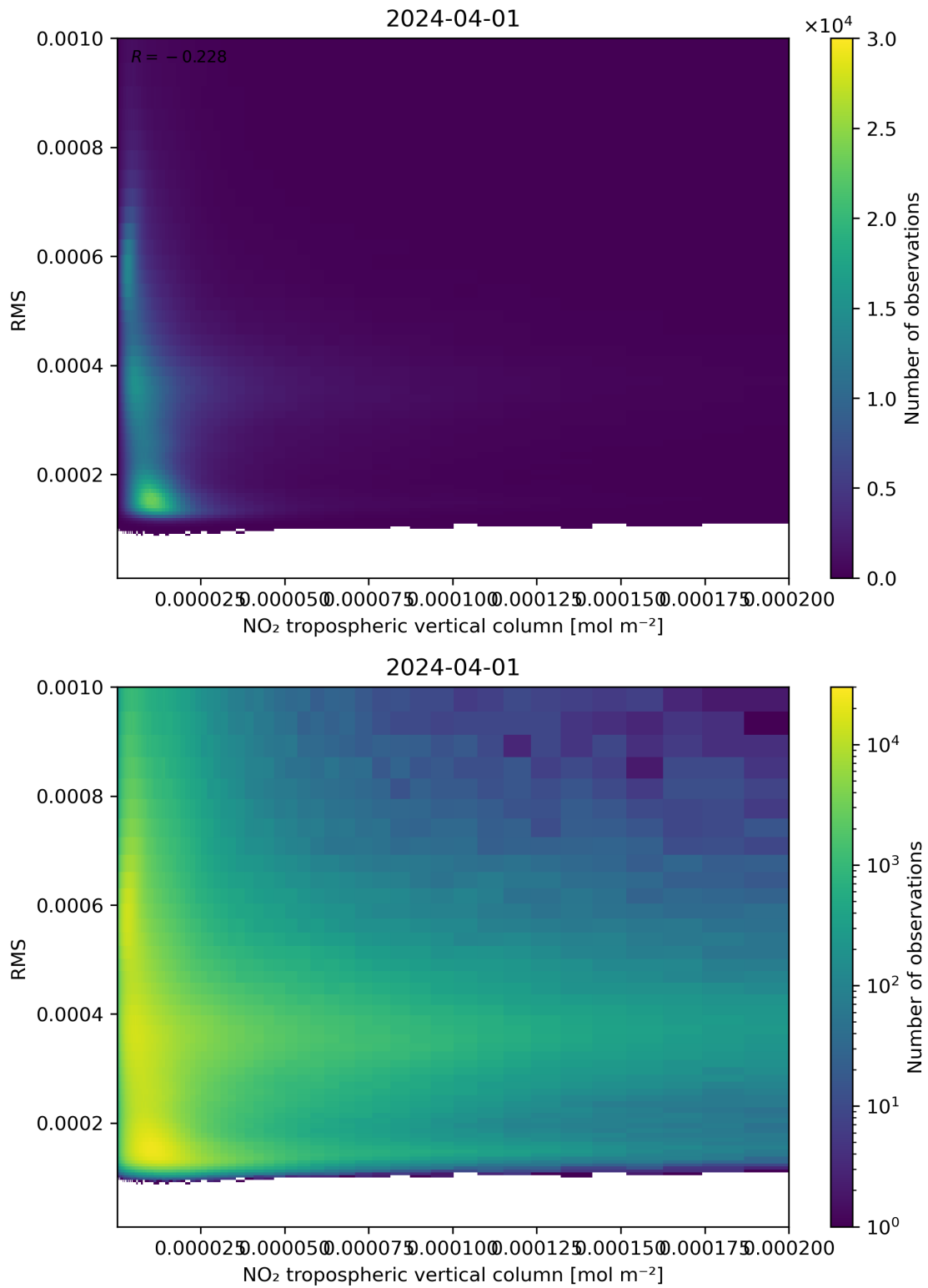
Figure 142: Scatter density plot of “NO 2 tropospheric vertical column” against “RMS” for 2024-03-31 to 2024-04-02.
