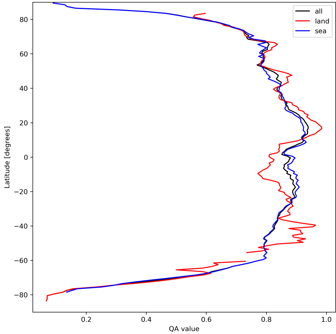
Figure 11: Zonal average of “QA value” for 2024-03-31 to 2024-04-02.
