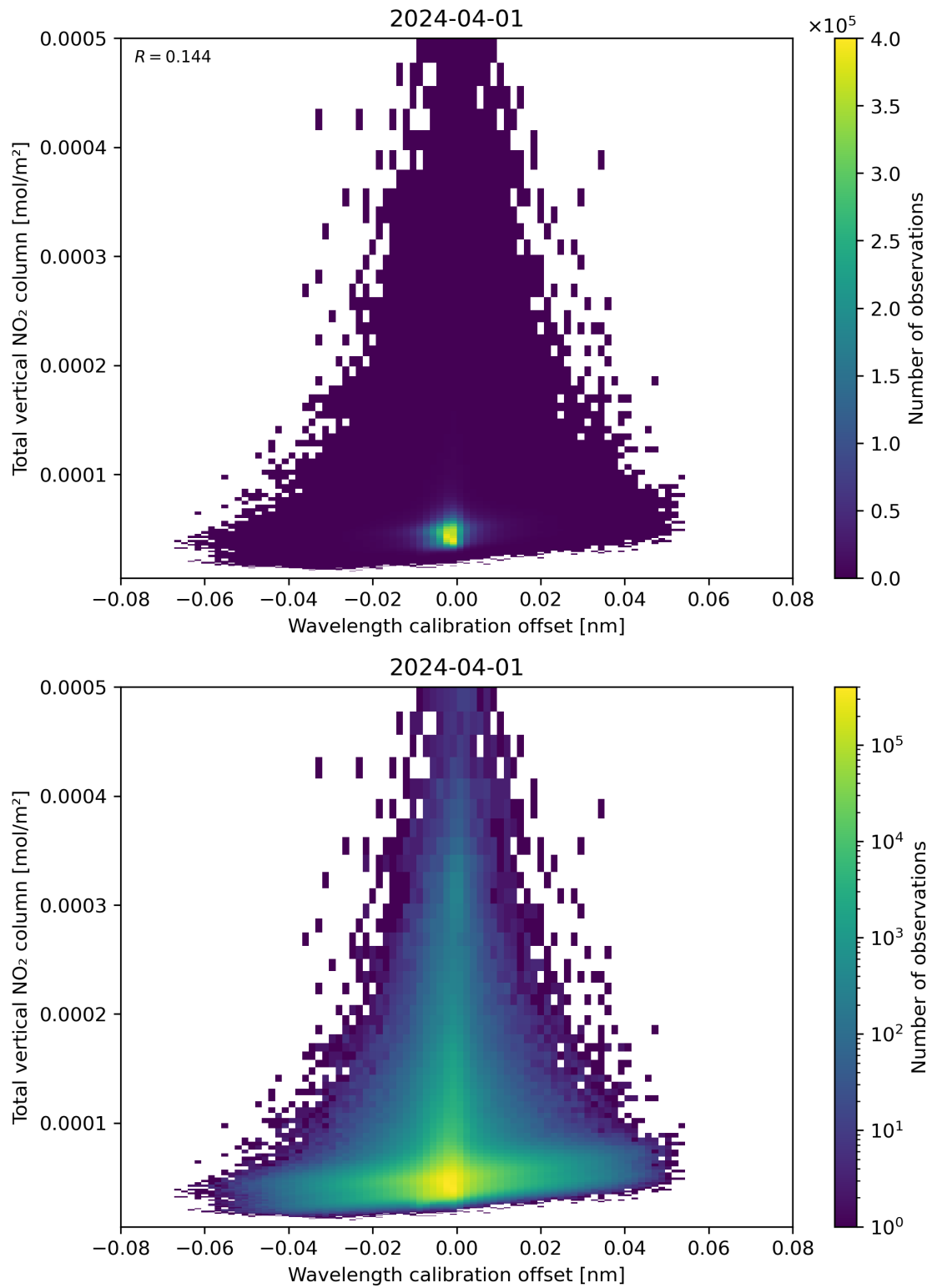
Figure 179: Scatter density plot of “Wavelength calibration offset” against “Total vertical NO 2 column” for 2024-03-31 to 2024-04-02.
