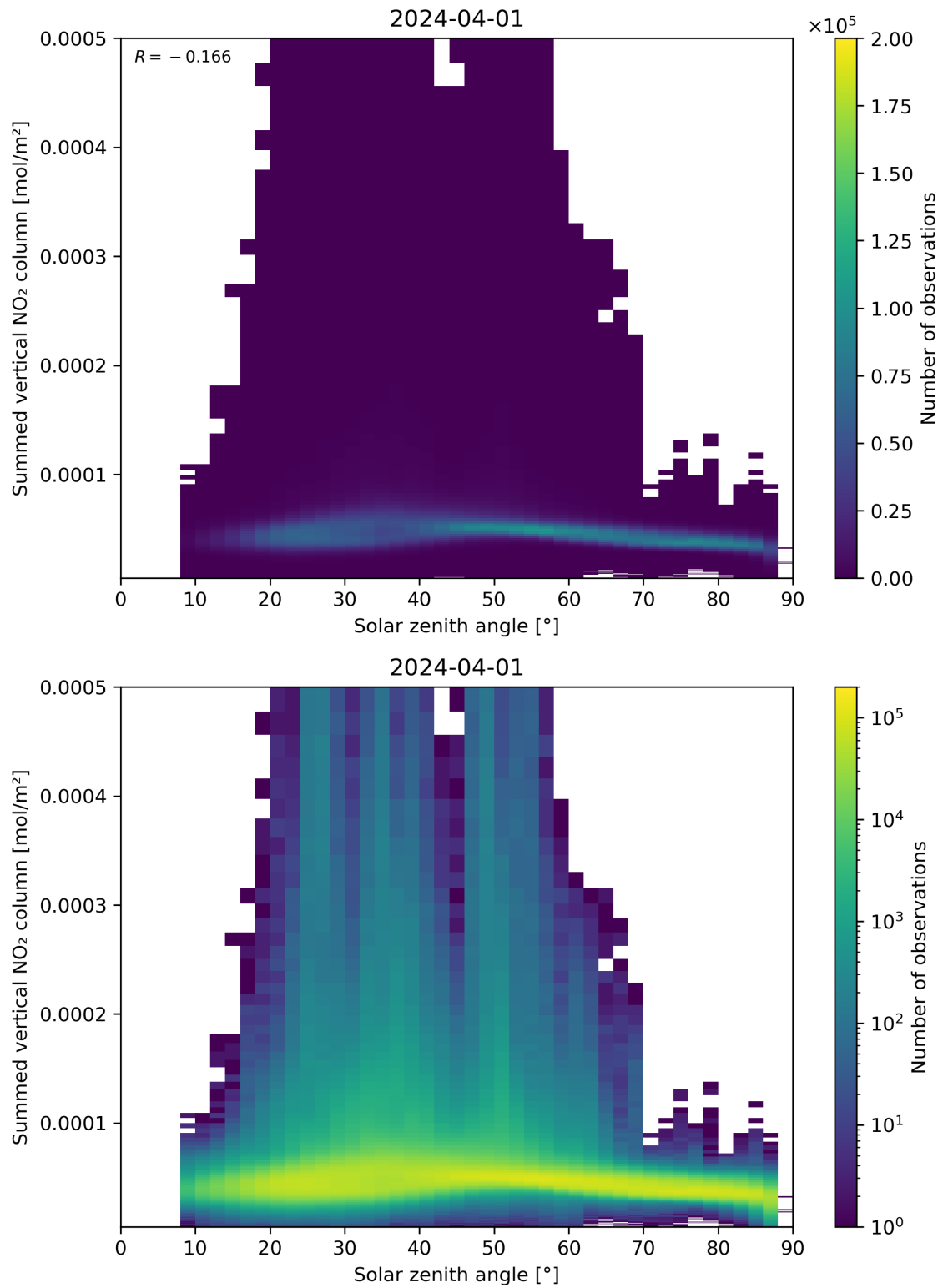
Figure 151: Scatter density plot of “Solar zenith angle” against “Summed vertical NO 2 column” for 2024-03-31 to 2024-04-02.
