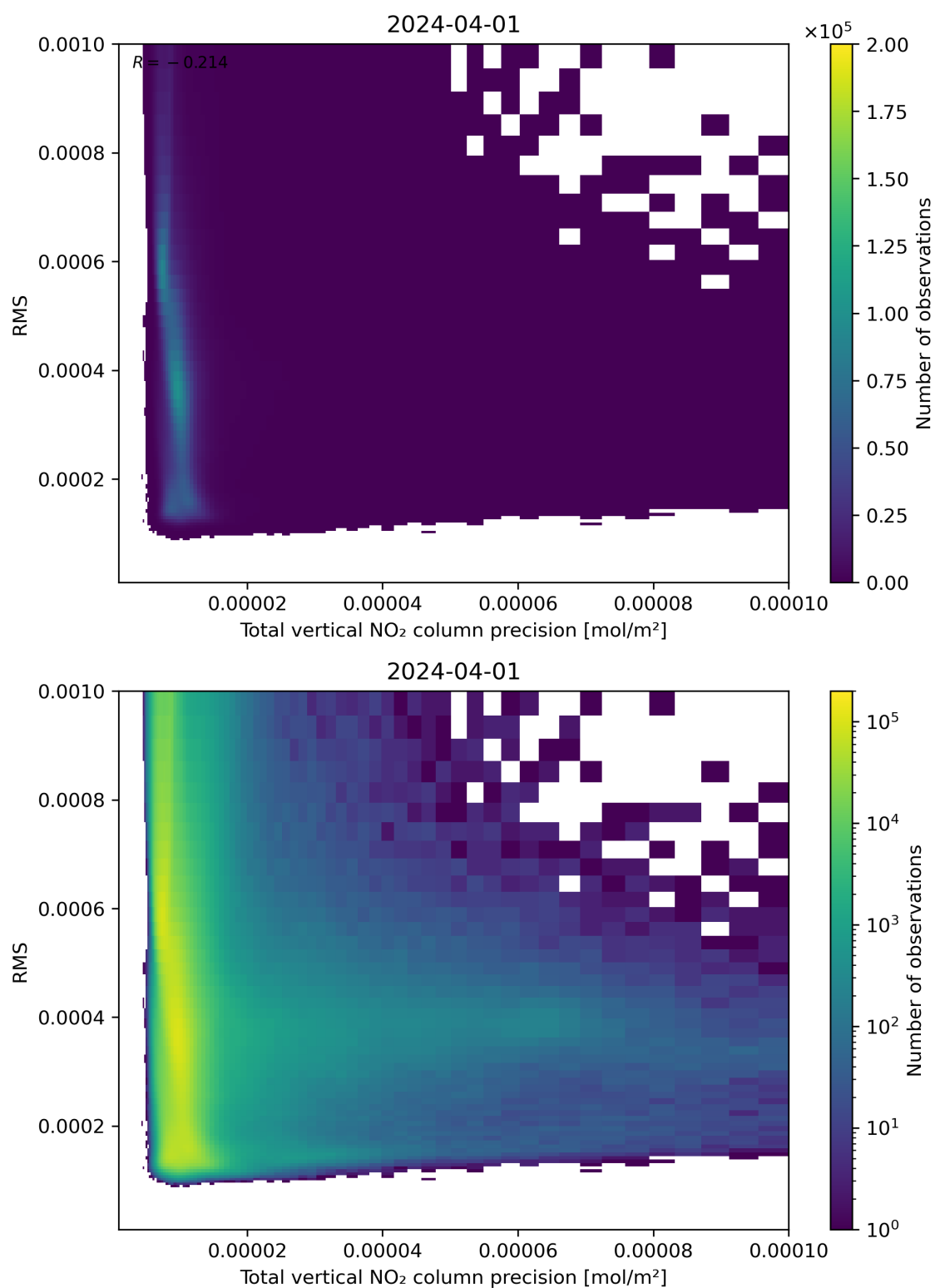
Figure 119: Scatter density plot of “Total vertical NO 2 column precision” against “RMS” for 2024-03-31 to 2024-04-02.
