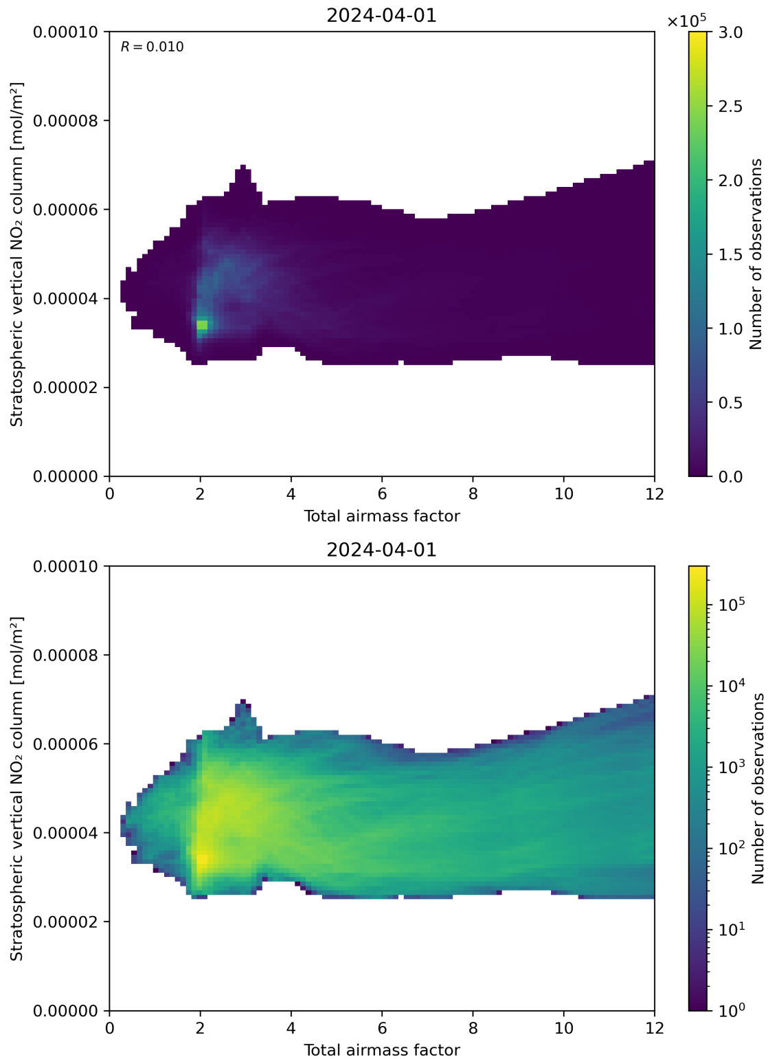
Figure 64: Scatter density plot of “Total airmass factor” against “Stratospheric vertical NO 2 column” for 2024-03-31 to 2024-04-02.
