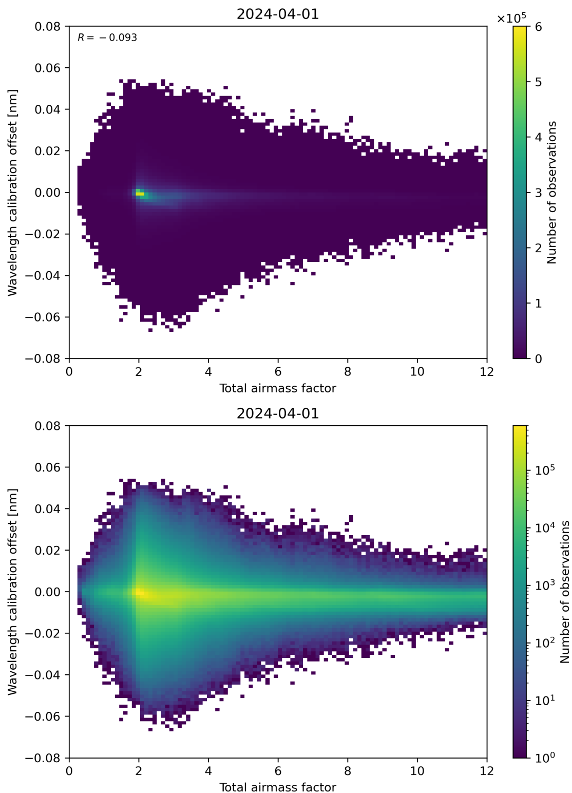
Figure 70: Scatter density plot of “Total airmass factor” against “Wavelength calibration offset” for 2024-03-31 to 2024-04-02.
