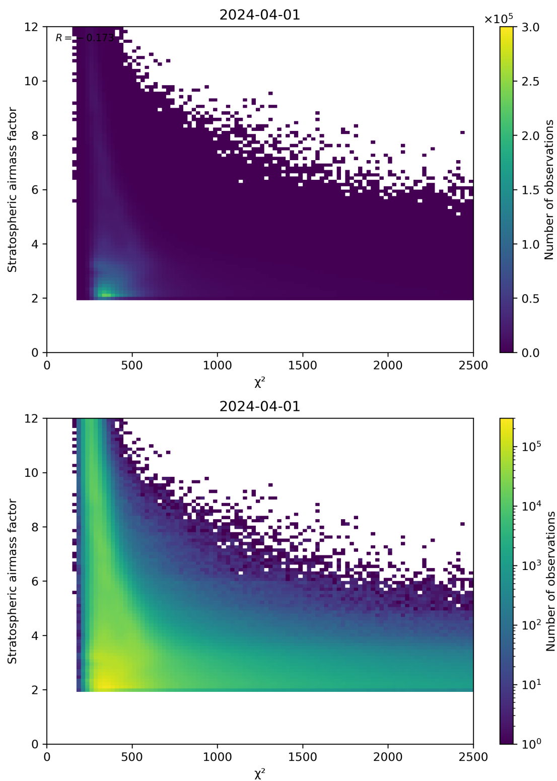
Figure 81: Scatter density plot of “ \chi^2 ” against “Stratospheric airmass factor” for 2024-03-31 to 2024-04-02.
