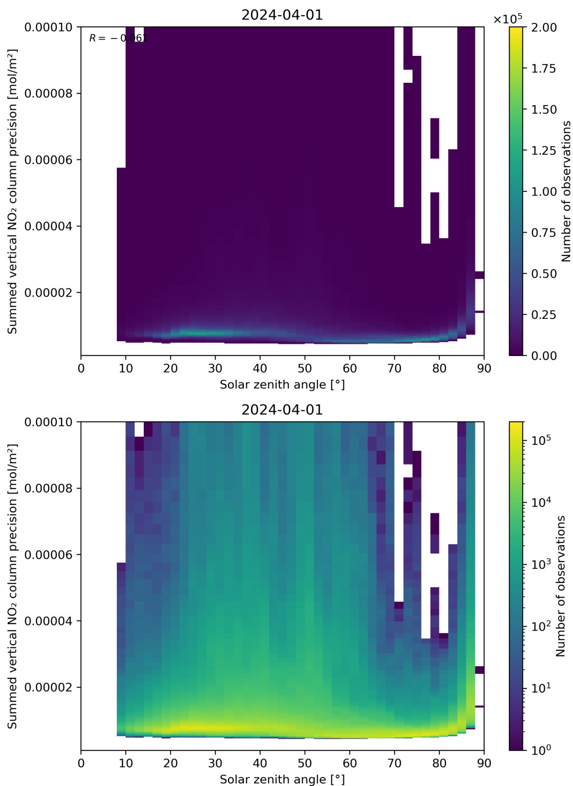
Figure 152: Scatter density plot of “Solar zenith angle” against “Summed vertical NO 2 column precision” for 2024-03-31 to 2024-04-02.
