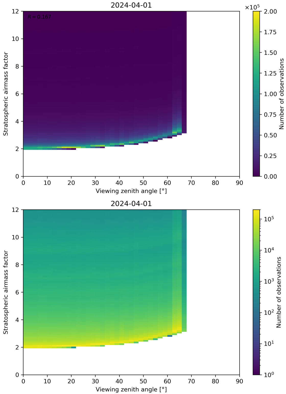
Figure 159: Scatter density plot of “Viewing zenith angle” against “Stratospheric airmass factor” for 2024-03-31 to 2024-04-02.
