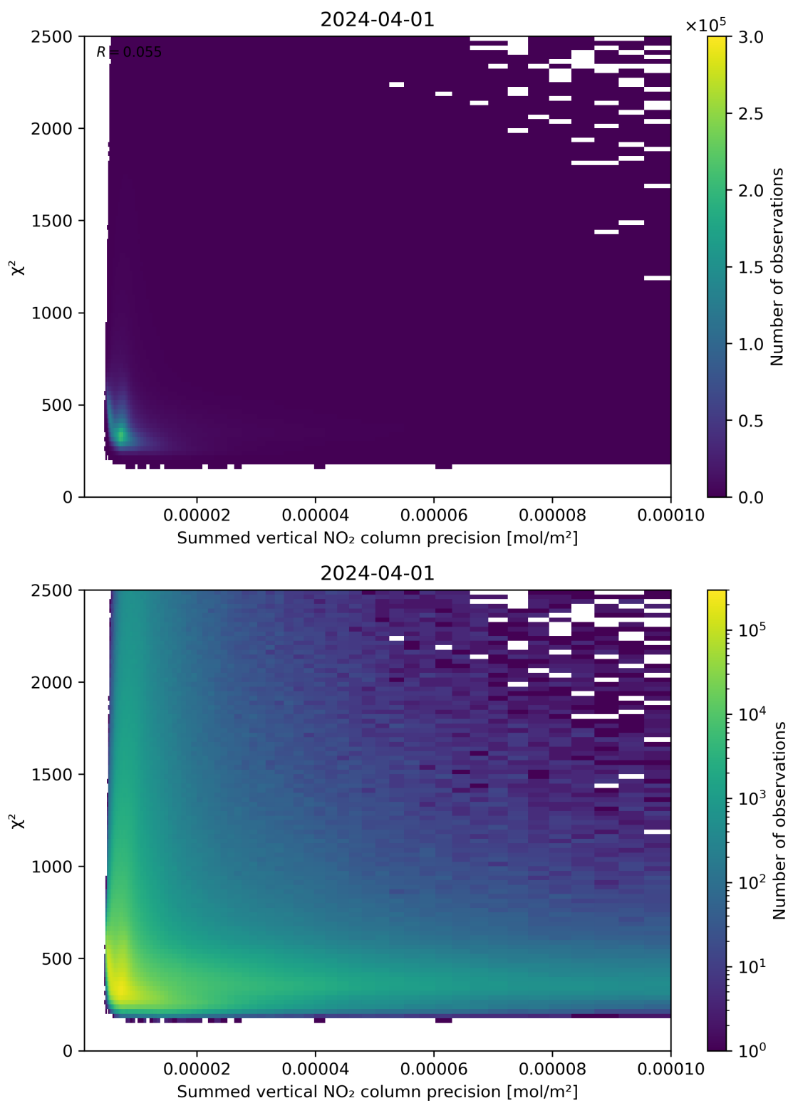
Figure 107: Scatter density plot of “Summed vertical NO 2 column precision” against “ \chi^2 ” for 2024-03-31 to 2024-04-02.
