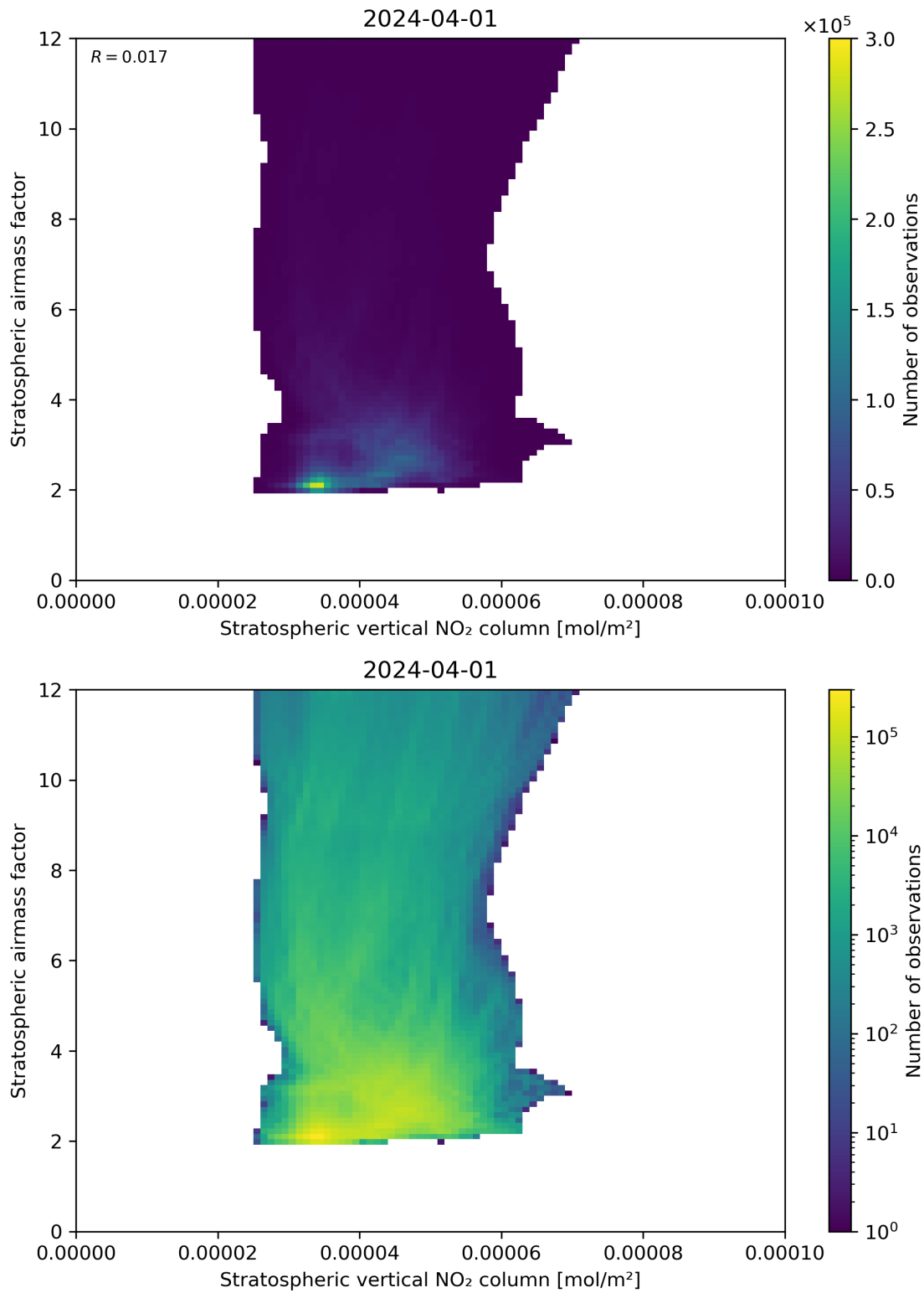
Figure 96: Scatter density plot of “Stratospheric vertical NO 2 column” against “Stratospheric airmass factor” for 2024-03-31 to 2024-04-02.
