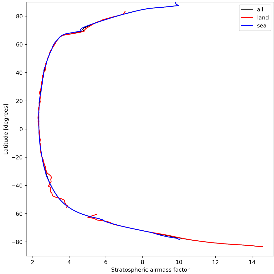
Figure 27: Zonal average of “Stratospheric airmass factor” for 2024-03-31 to 2024-04-02.
