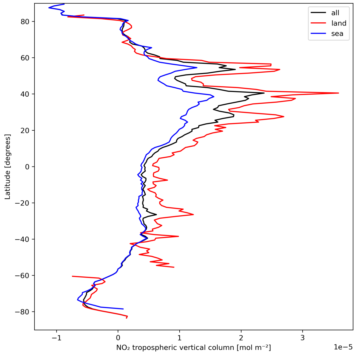
Figure 12: Zonal average of “NO 2 tropospheric vertical column” for 2024-03-31 to 2024-04-02.
