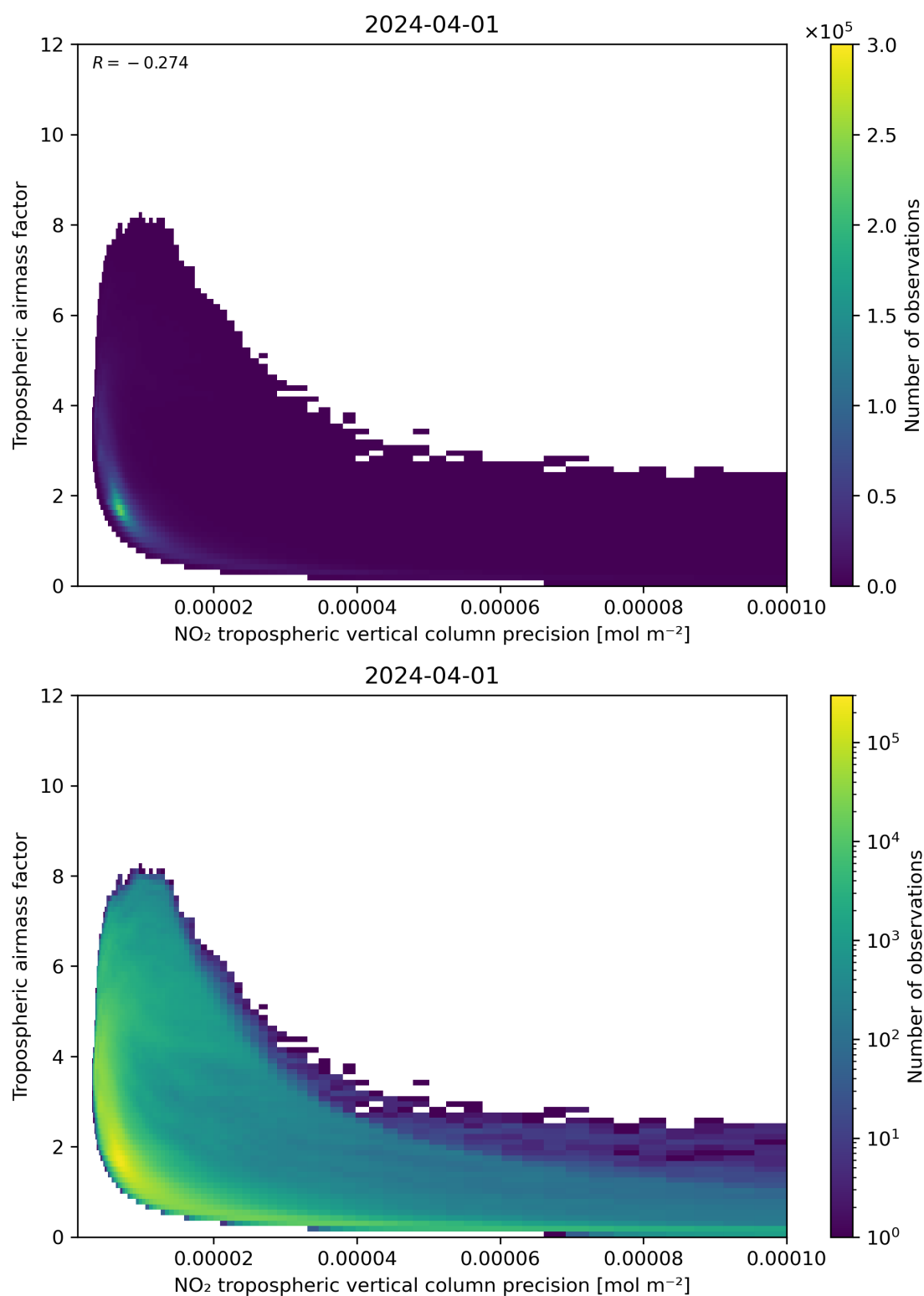
Figure 133: Scatter density plot of “NO 2 tropospheric vertical column precision” against “Tropospheric airmass factor” for 2024-03-31 to 2024-04-02.
