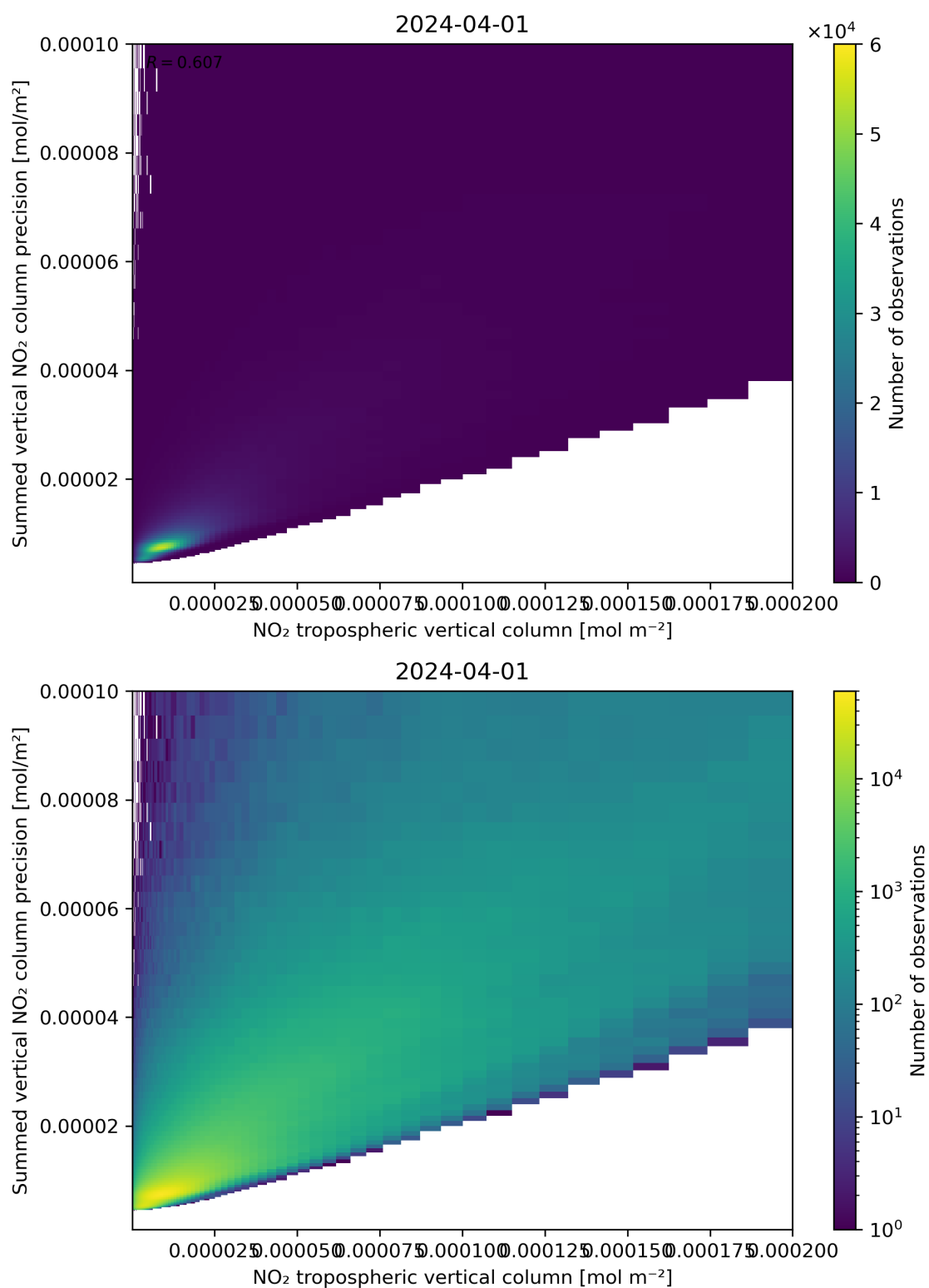
Figure 127: Scatter density plot of “NO 2 tropospheric vertical column” against “Summed vertical NO 2 column precision” for 2024-03-31 to 2024-04-02.
