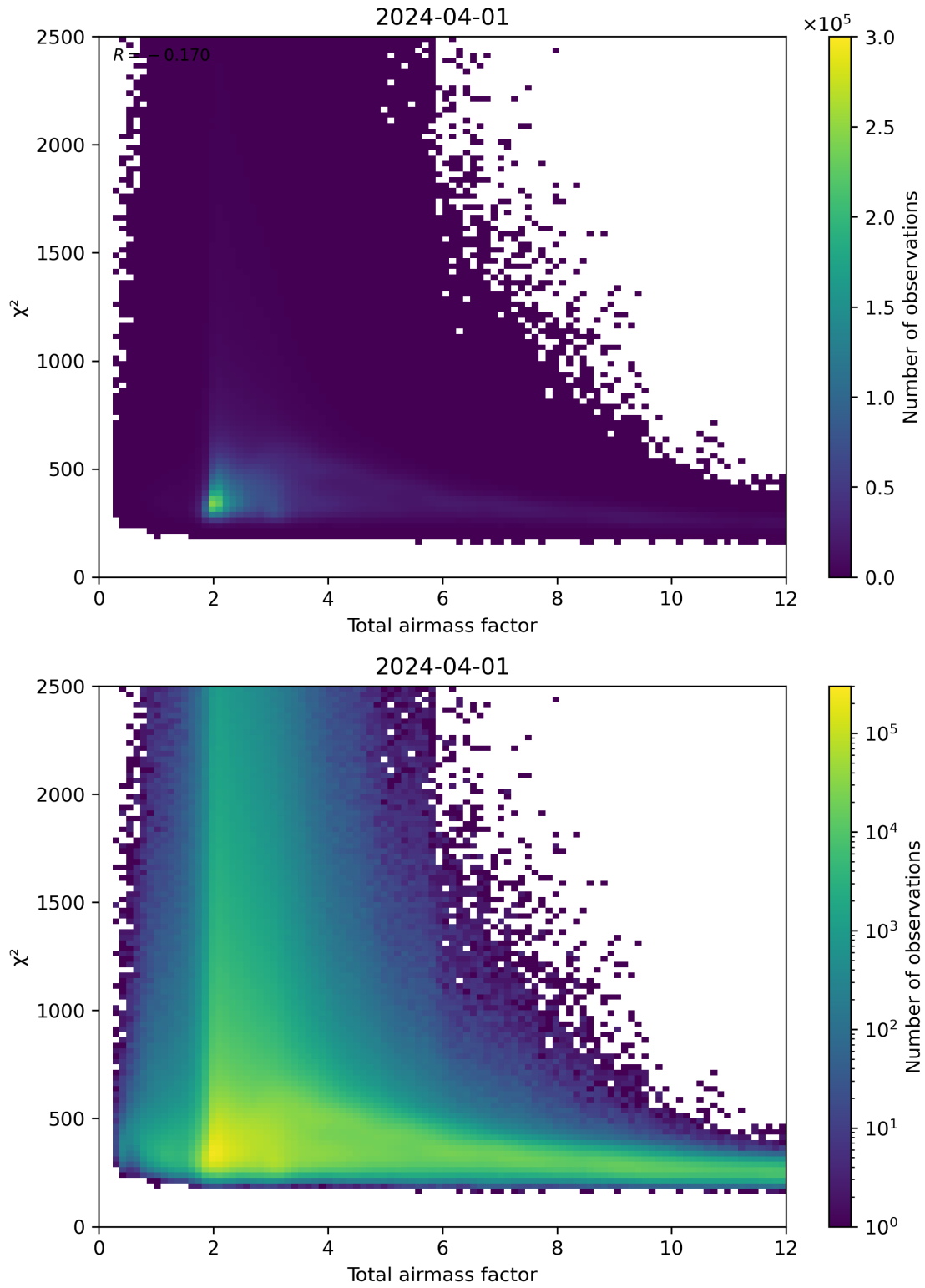
Figure 63: Scatter density plot of “Total airmass factor” against “ \chi^2 ” for 2024-03-31 to 2024-04-02.
