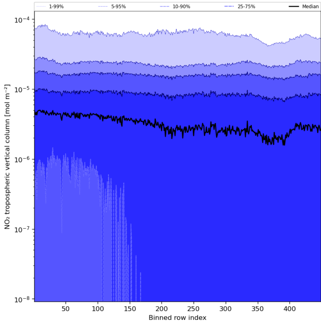
Figure 46: Along track statistics of "NO 2 tropospheric vertical column" for 2024-03-31 to 2024-04-02
