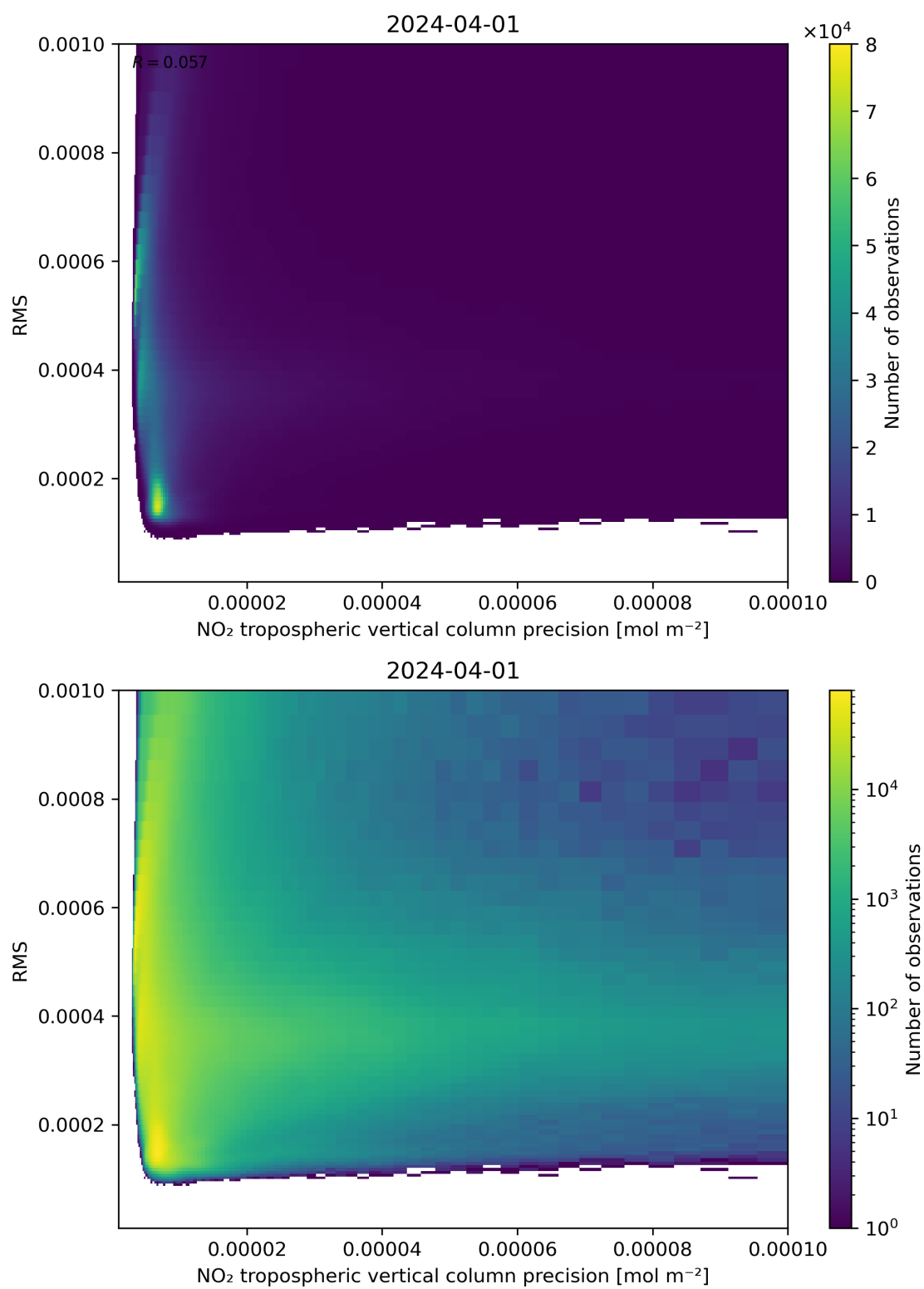
Figure 140: Scatter density plot of “NO 2 tropospheric vertical column precision” against “RMS” for 2024-03-31 to 2024-04-02.
