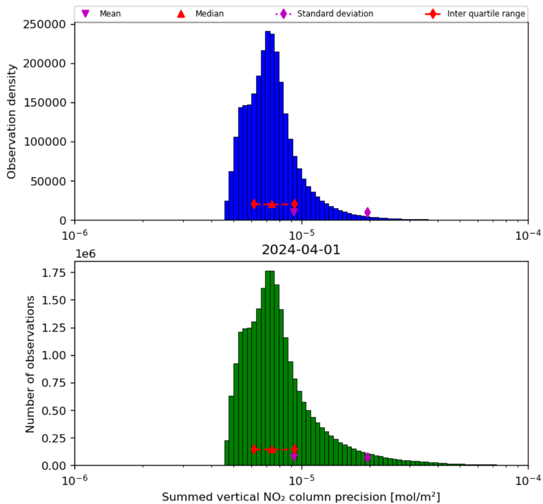
Figure 41: Histogram of "Summed vertical NO 2 column precision" for 2024-03-31 to 2024-04-02
