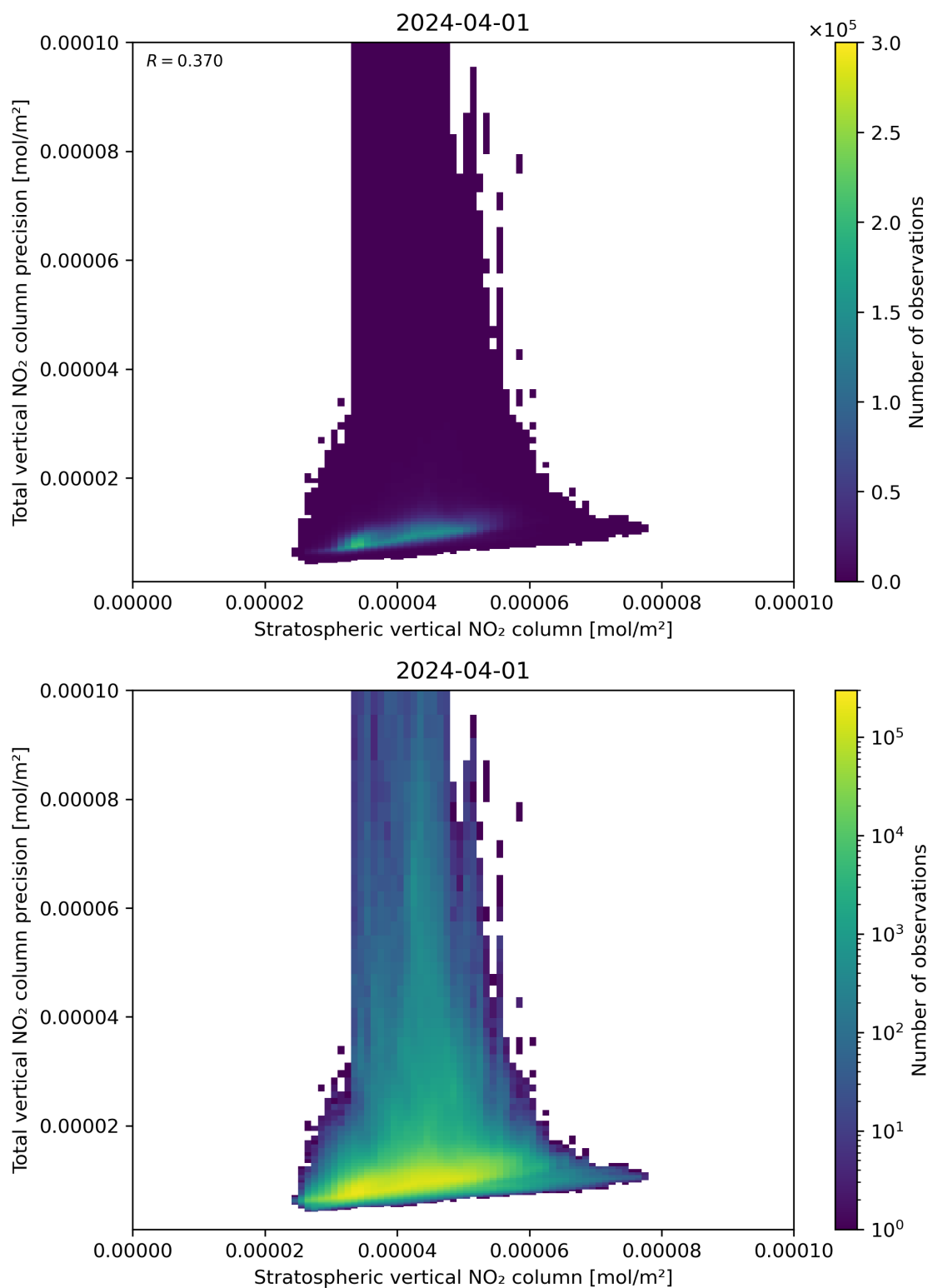
Figure 101: Scatter density plot of “Stratospheric vertical NO 2 column” against “Total vertical NO 2 column precision” for 2024-03-31 to 2024-04-02.
