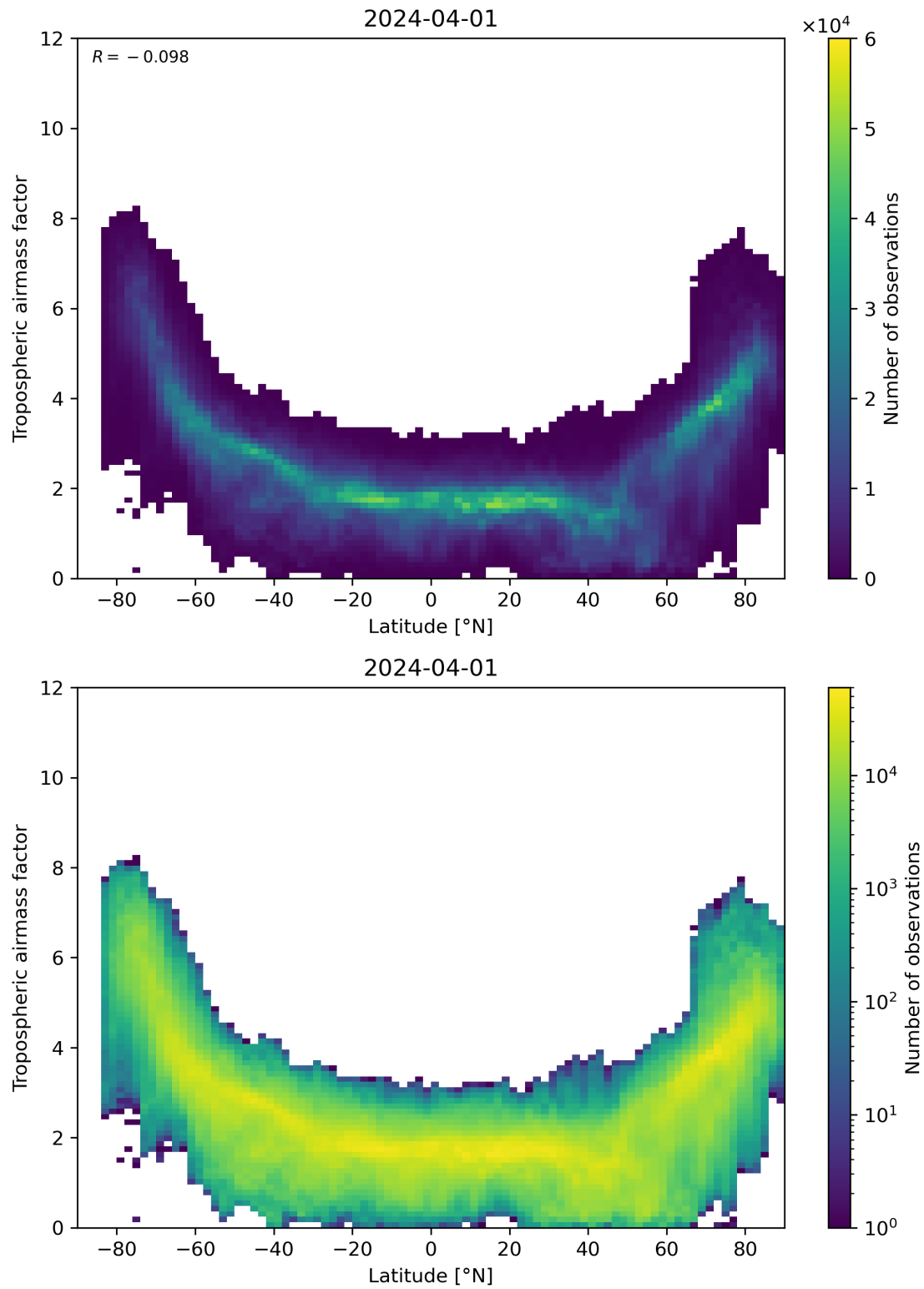
Figure 85: Scatter density plot of “Latitude” against “Tropospheric air mass factor” for 2024-03-31 to 2024-04-02.
