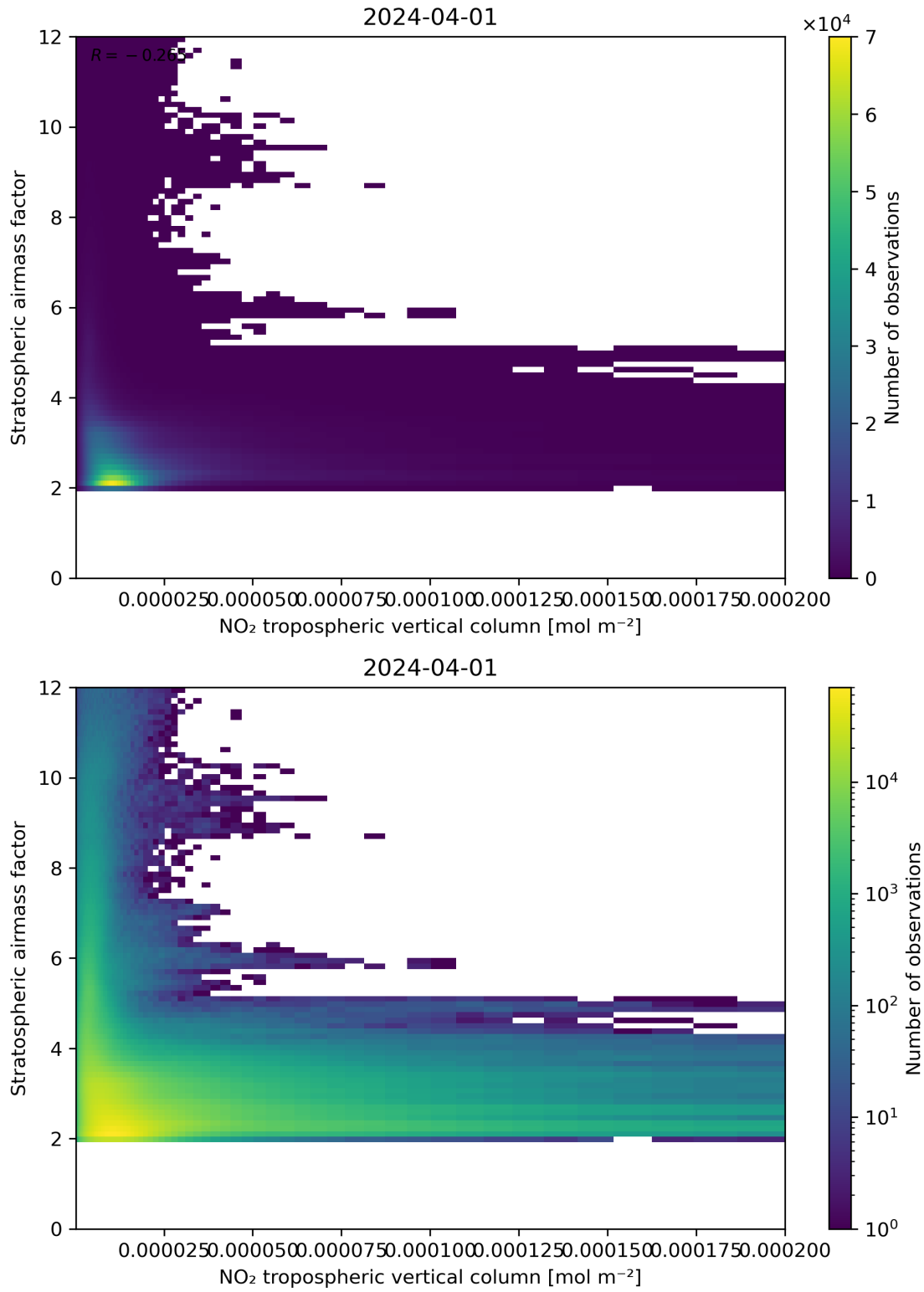
Figure 121: Scatter density plot of “NO 2 tropospheric vertical column” against “Stratospheric air mass factor” for 2024-03-31 to 2024-04-02.
