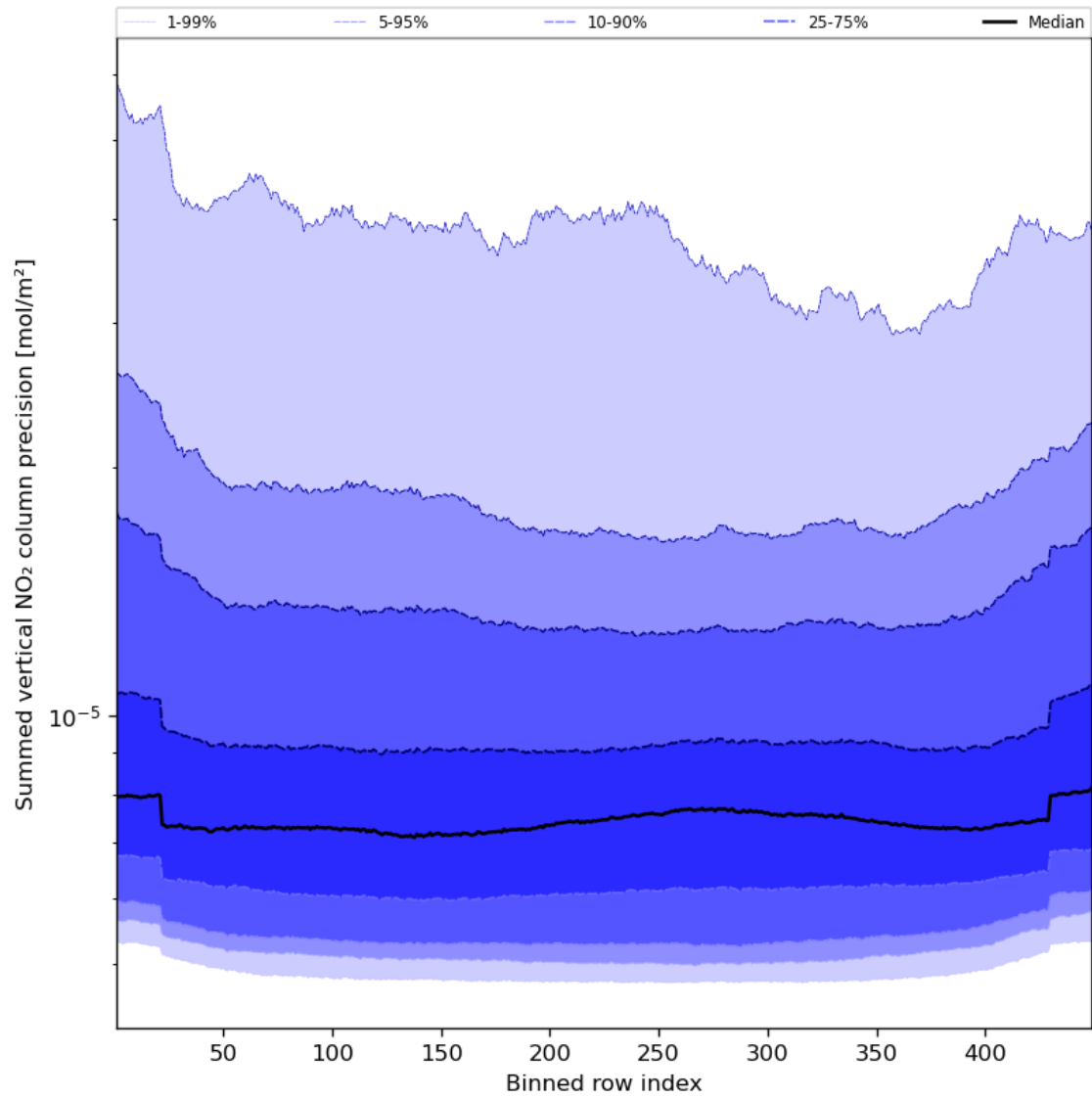
Figure 58: Along track statistics of “Summed vertical NO 2 column precision” for 2024-03-31 to 2024-04-02
