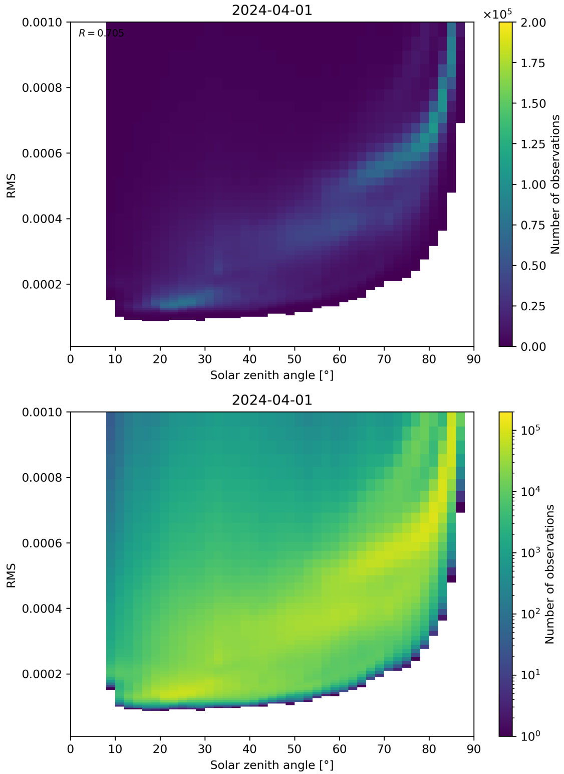
Figure 157: Scatter density plot of “Solar zenith angle” against “RMS” for 2024-03-31 to 2024-04-02.
