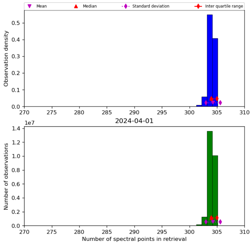
Figure 33: Histogram of “Number of spectral points in retrieval” for 2024-03-31 to 2024-04-02
