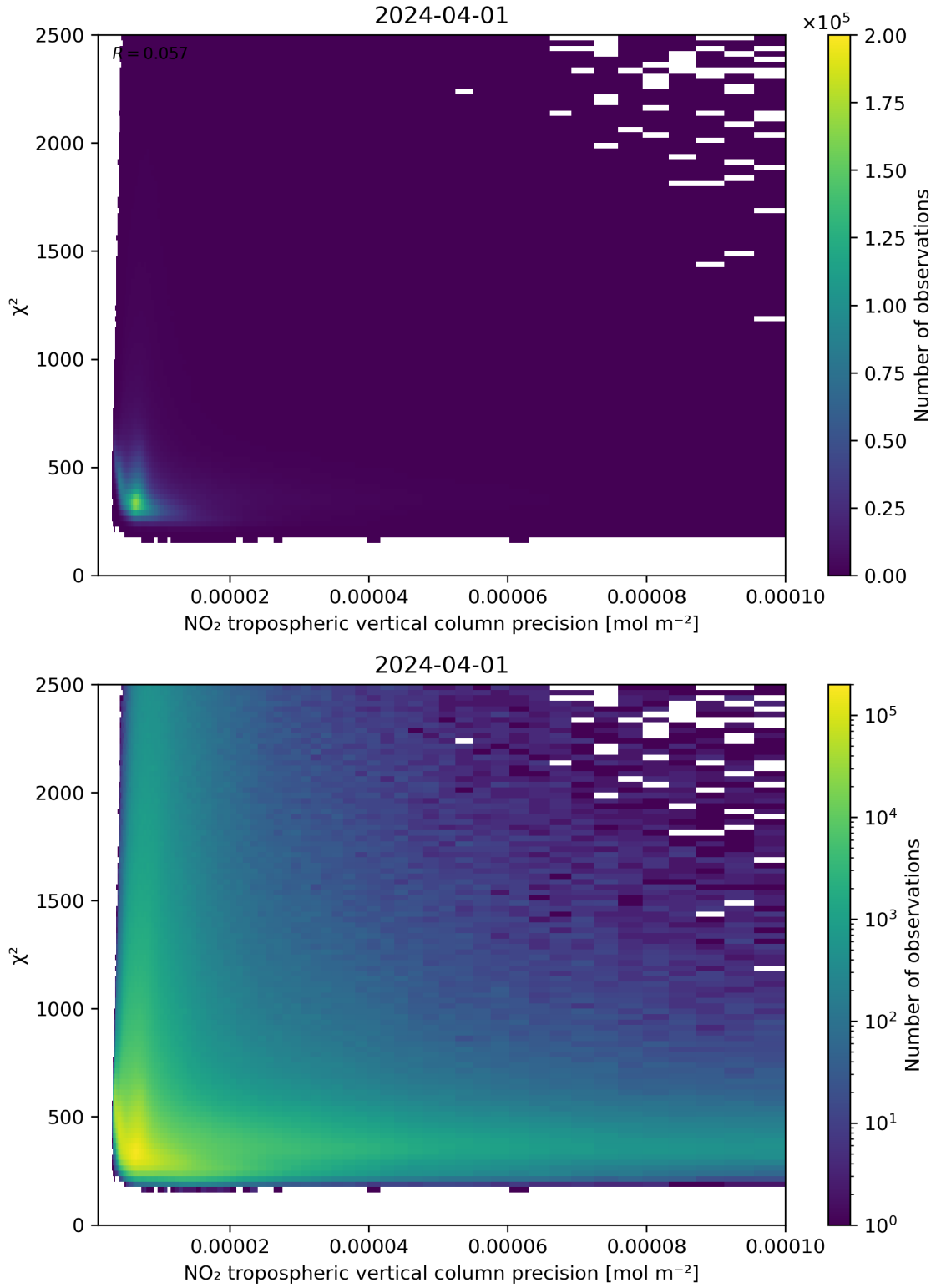
Figure 134: Scatter density plot of “NO 2 tropospheric vertical column precision” against “ \chi^2 ” for 2024-03-31 to 2024-04-02.
