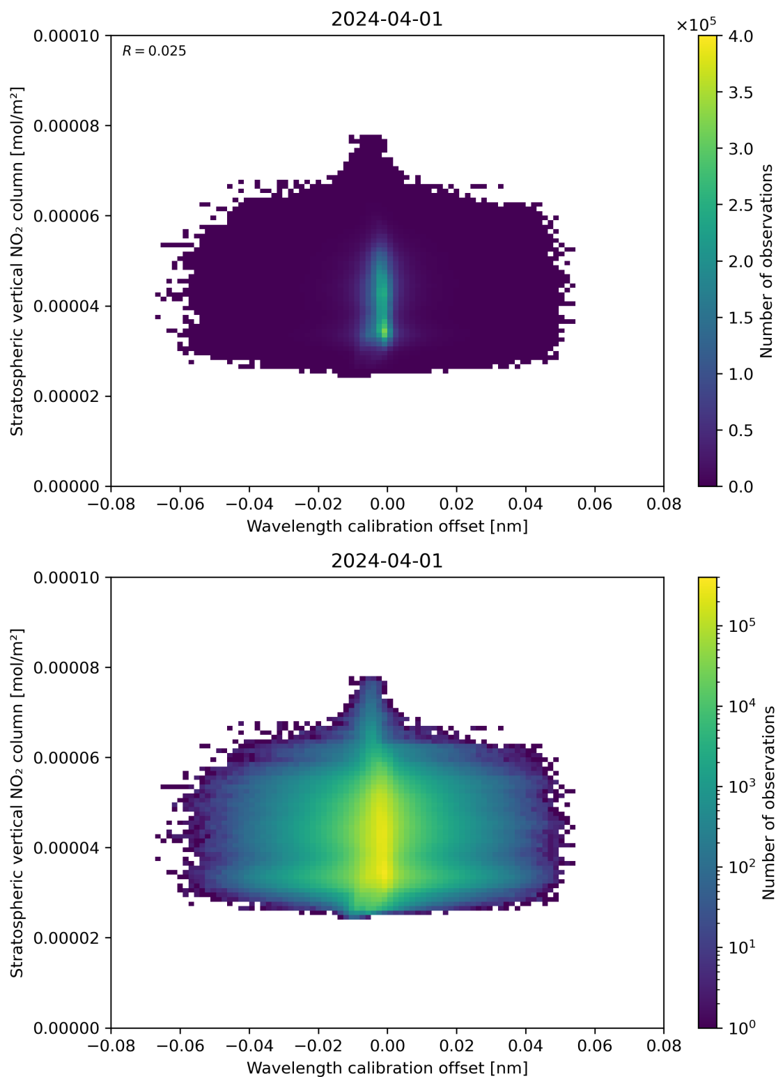
Figure 176: Scatter density plot of “Wavelength calibration offset” against “Stratospheric vertical NO 2 column” for 2024-03-31 to 2024-04-02.
