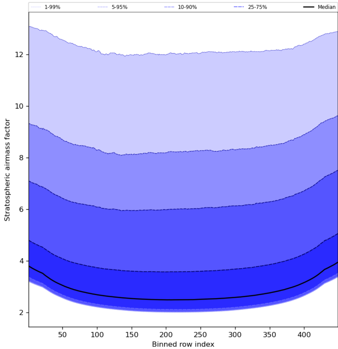
Figure 61: Along track statistics of “Stratospheric airmass factor” for 2024-03-31 to 2024-04-02
