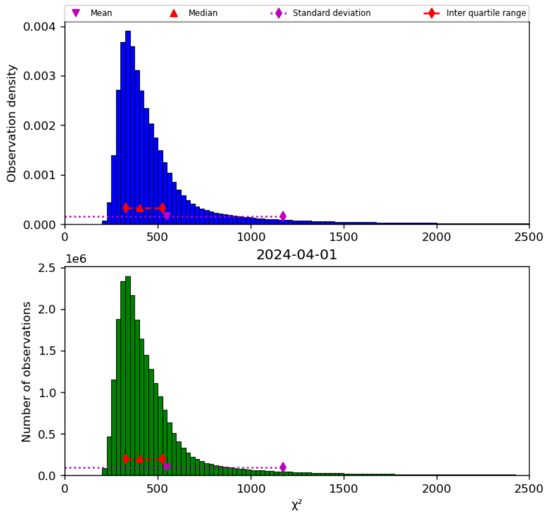
Figure 42: Histogram of “ \chi^2 ” for 2024-03-31 to 2024-04-02
