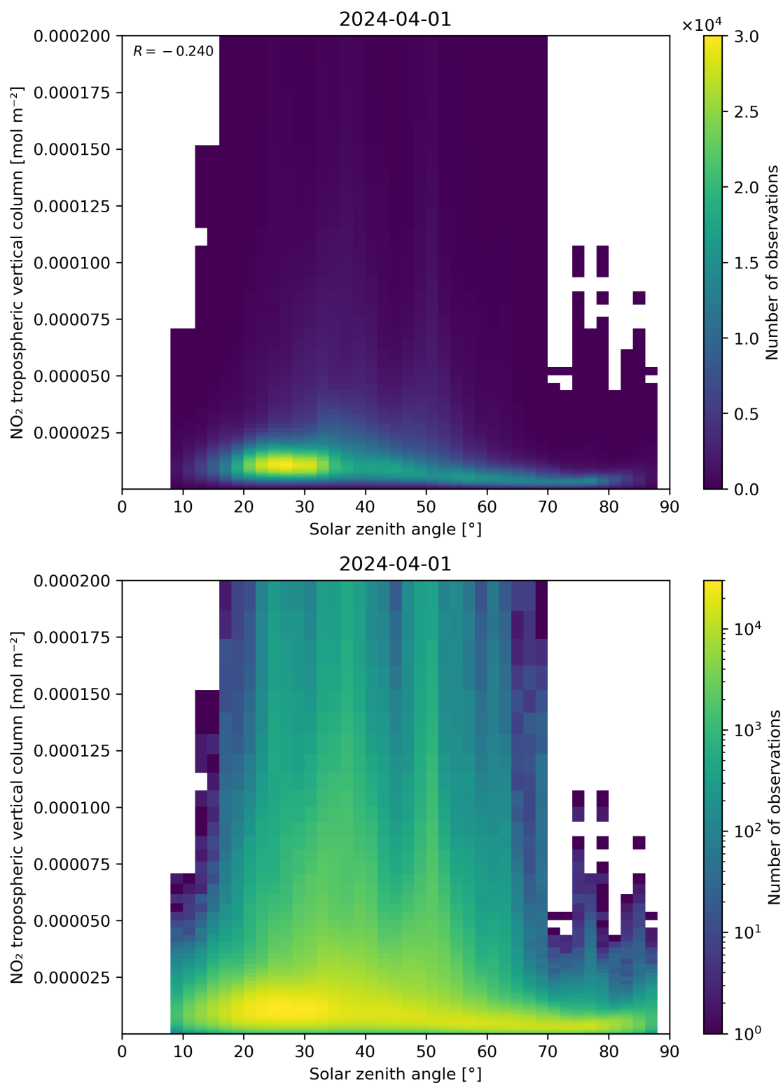
Figure 155: Scatter density plot of “Solar zenith angle” against “NO 2 tropospheric vertical column” for 2024-03-31 to 2024-04-02.
