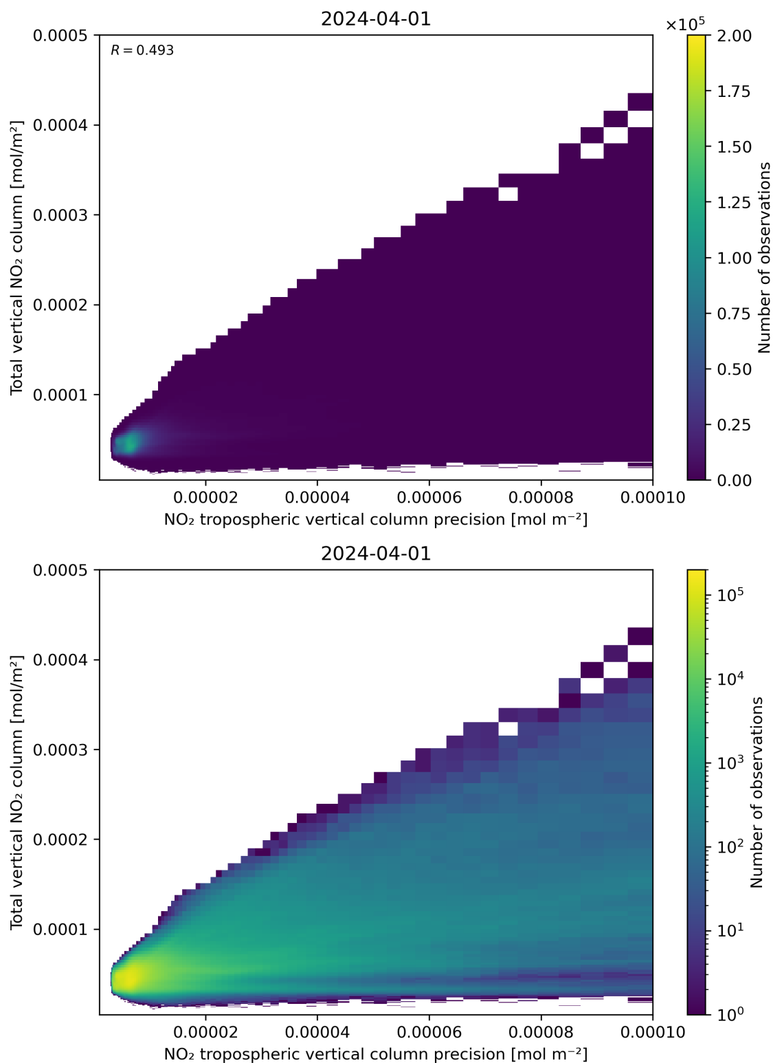
Figure 138: Scatter density plot of “NO 2 tropospheric vertical column precision” against “Total vertical NO 2 column” for 2024-03-31 to 2024-04-02.
