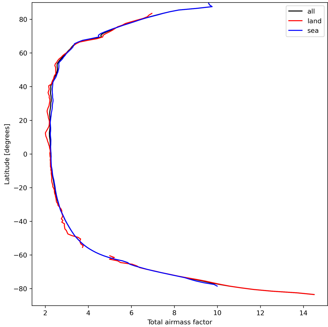
Figure 15: Zonal average of “Total airmass factor” for 2024-03-31 to 2024-04-02.
