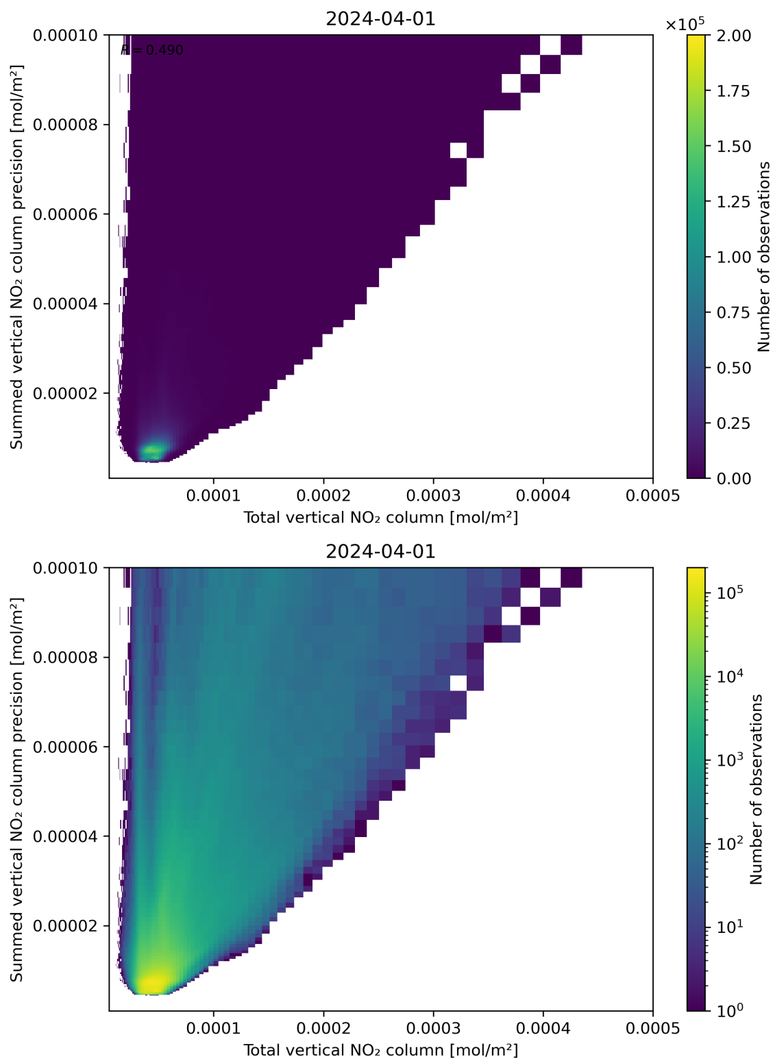
Figure 113: Scatter density plot of “Total vertical NO 2 column” against “Summed vertical NO 2 column precision” for 2024-03-31 to 2024-04-02.
