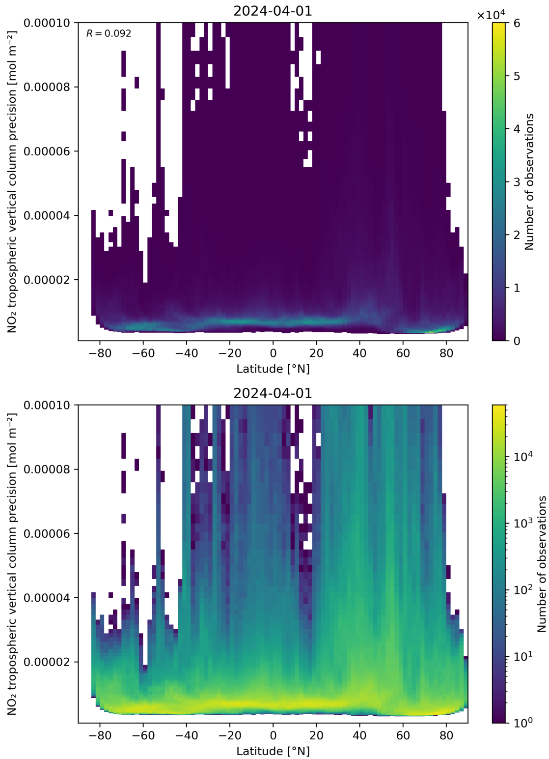
Figure 93: Scatter density plot of “Latitude” against “NO 2 tropospheric vertical column precision” for 2024-03-31 to 2024-04-02.
