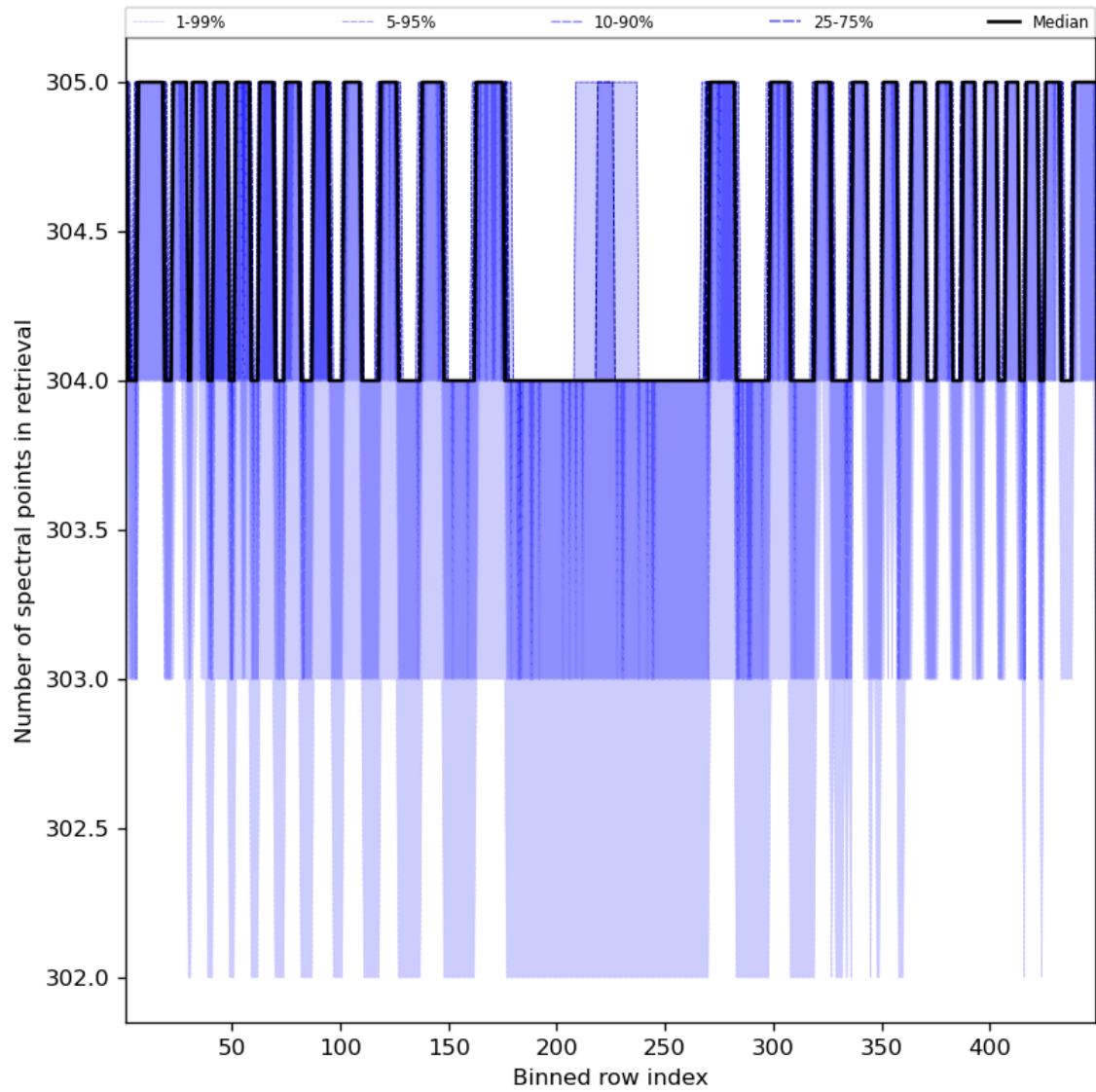
Figure 50: Along track statistics of “Number of spectral points in retrieval” for 2024-03-31 to 2024-04-02
