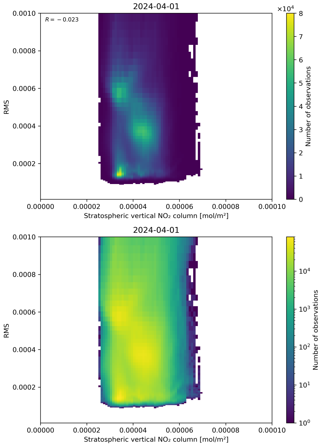
Figure 102: Scatter density plot of “Stratospheric vertical NO 2 column” against “RMS” for 2024-03-31 to 2024-04-02.
