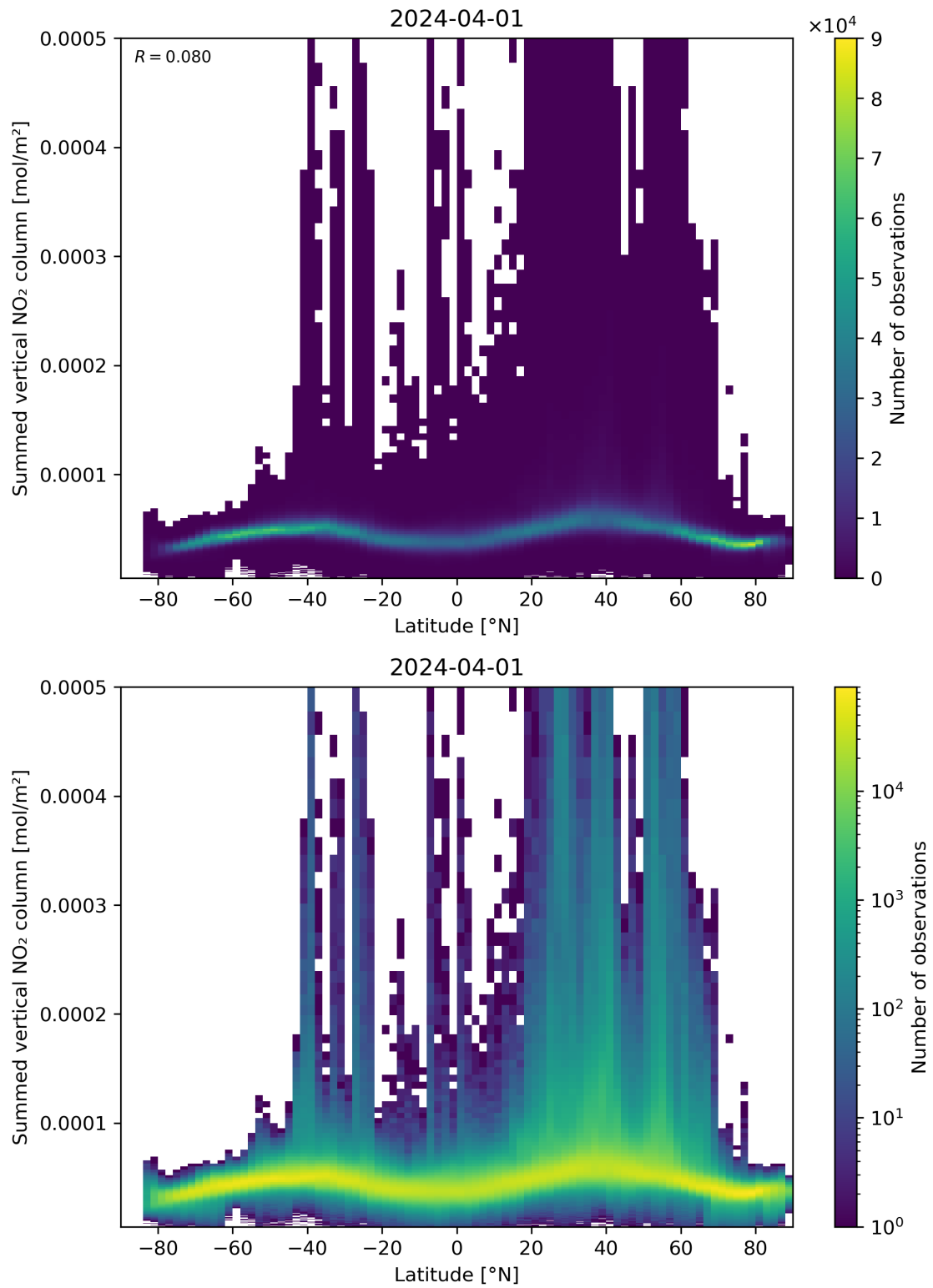
Figure 88: Scatter density plot of “Latitude” against “Summed vertical NO 2 column” for 2024-03-31 to 2024-04-02.
