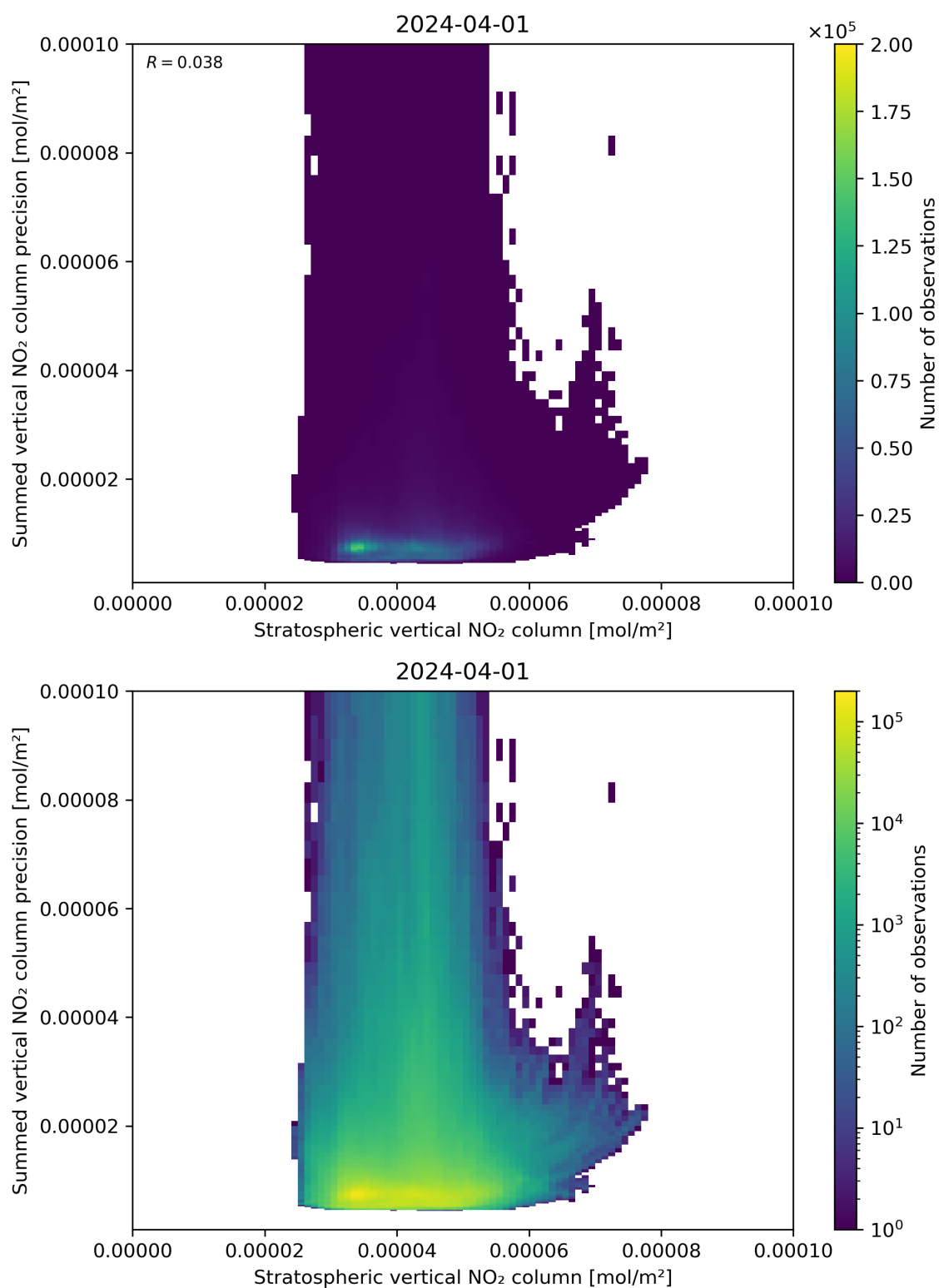
Figure 99: Scatter density plot of “Stratospheric vertical NO 2 column” against “Summed vertical NO 2 column precision” for 2024-03-31 to 2024-04-02.
