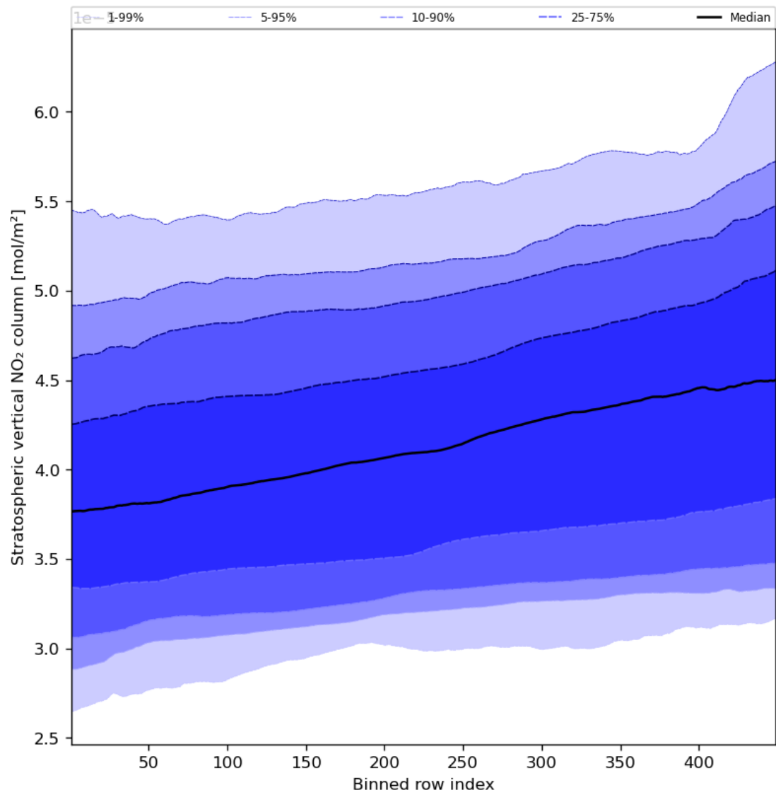
Figure 53: Along track statistics of “Stratospheric vertical NO 2 column” for 2024-03-31 to 2024-04-02
