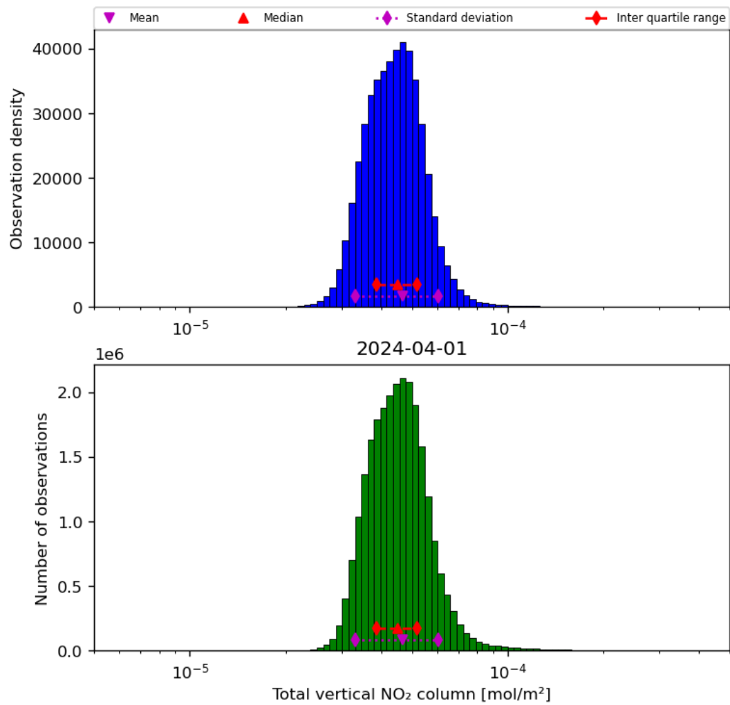
Figure 38: Histogram of “Total vertical NO 2 column” for 2024-03-31 to 2024-04-02
