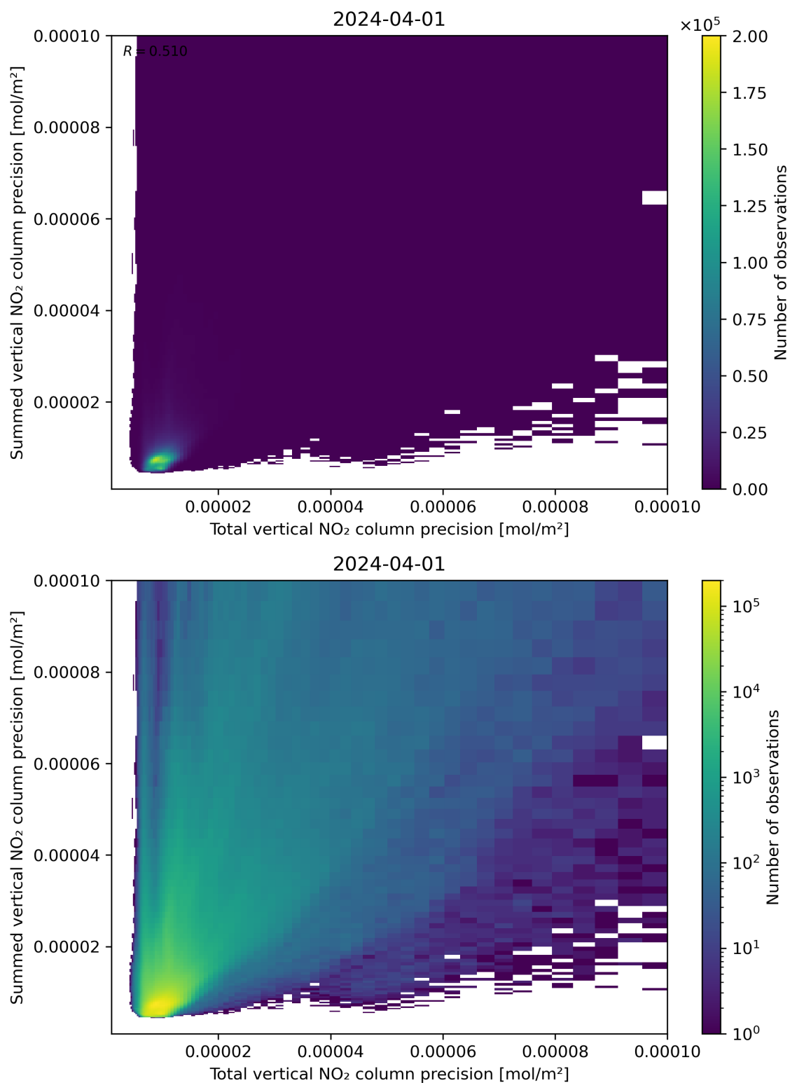
Figure 118: Scatter density plot of “Total vertical NO 2 column precision” against “Summed vertical NO 2 column precision” for 2024-03-31 to 2024-04-02.
