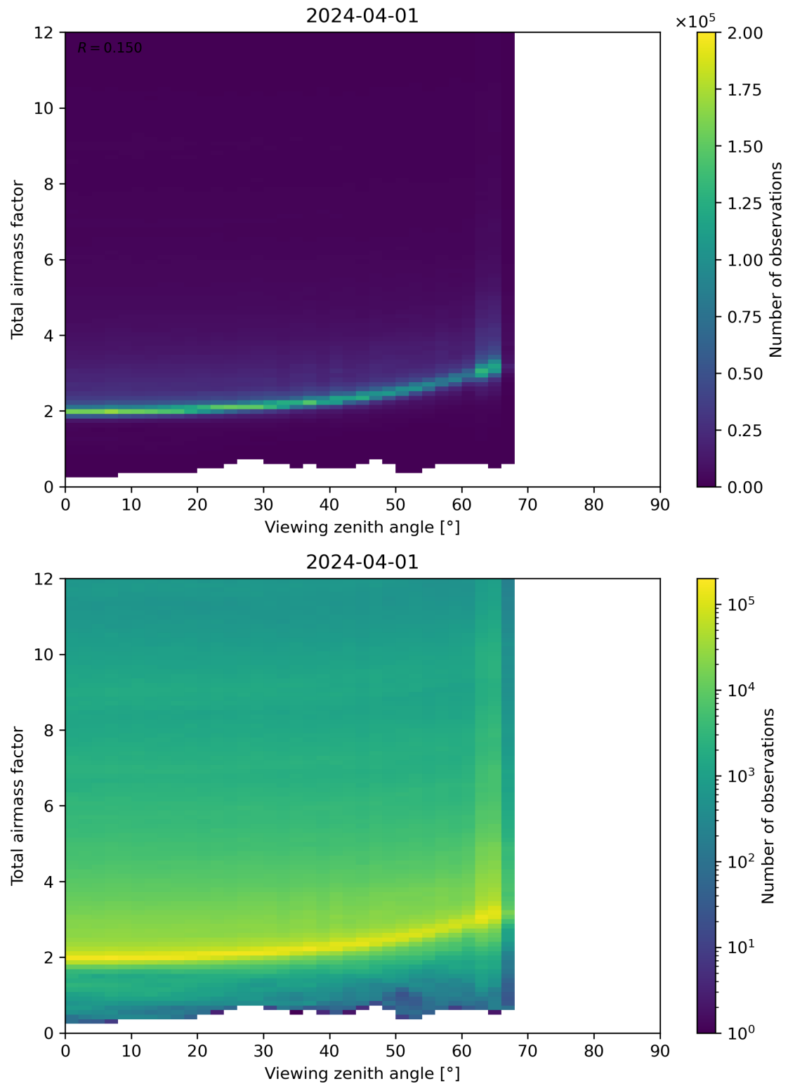
Figure 160: Scatter density plot of “Viewing zenith angle” against “Total airmass factor” for 2024-03-31 to 2024-04-02.
