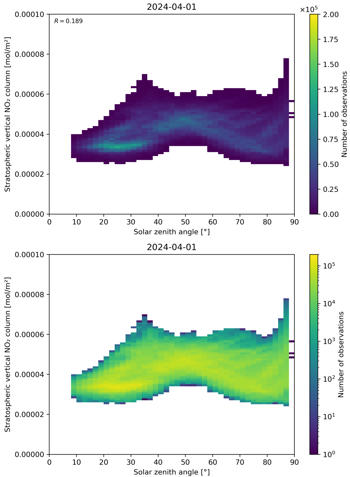
Figure 150: Scatter density plot of “Solar zenith angle” against “Stratospheric vertical NO 2 column” for 2024-03-31 to 2024-04-02.
