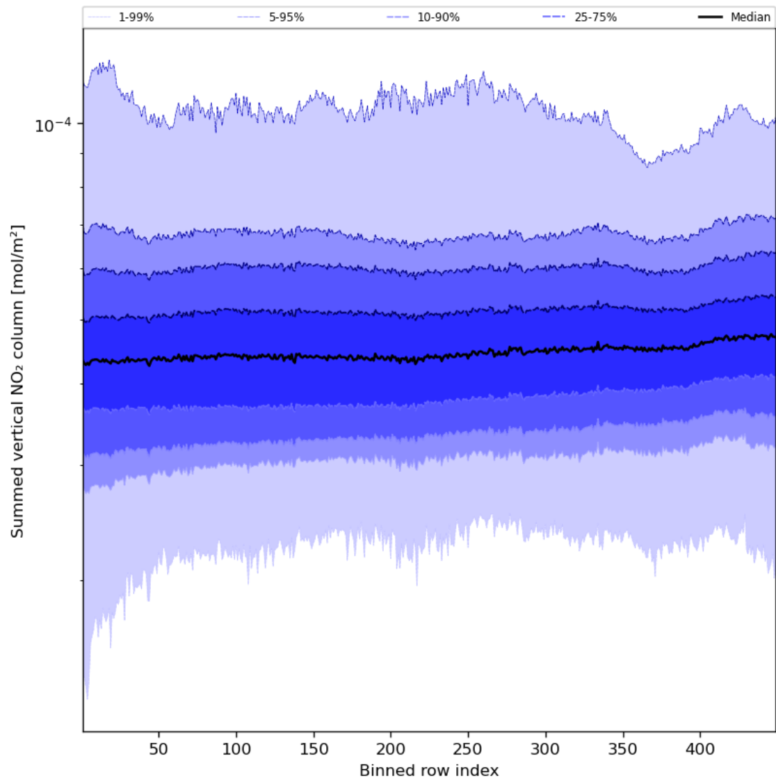
Figure 57: Along track statistics of “Summed vertical NO 2 column” for 2024-03-31 to 2024-04-02
