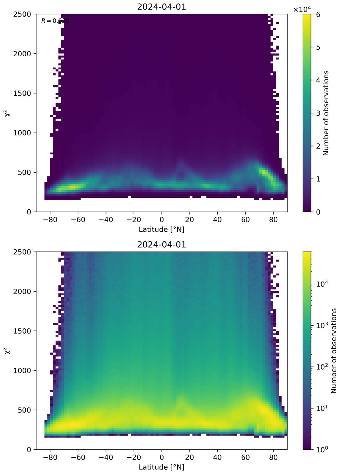
Figure 86: Scatter density plot of “Latitude” against “ \chi^2 ” for 2024-03-31 to 2024-04-02.
