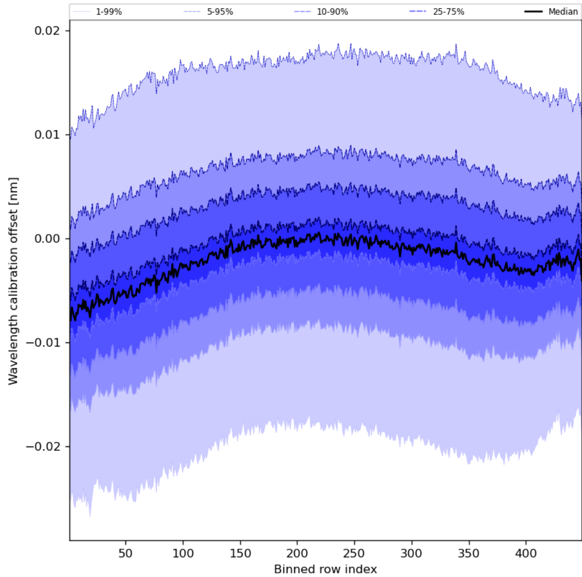
Figure 52: Along track statistics of “Wavelength calibration offset” for 2024-03-31 to 2024-04-02
