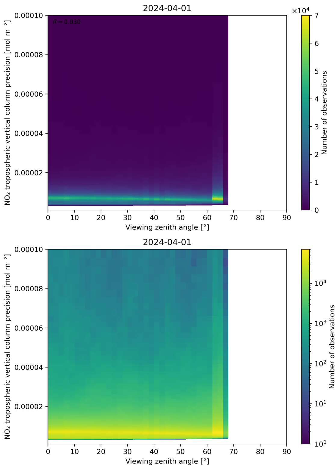
Figure 170: Scatter density plot of “Viewing zenith angle” against “NO 2 tropospheric vertical column precision” for 2024-03-31 to 2024-04-02.
