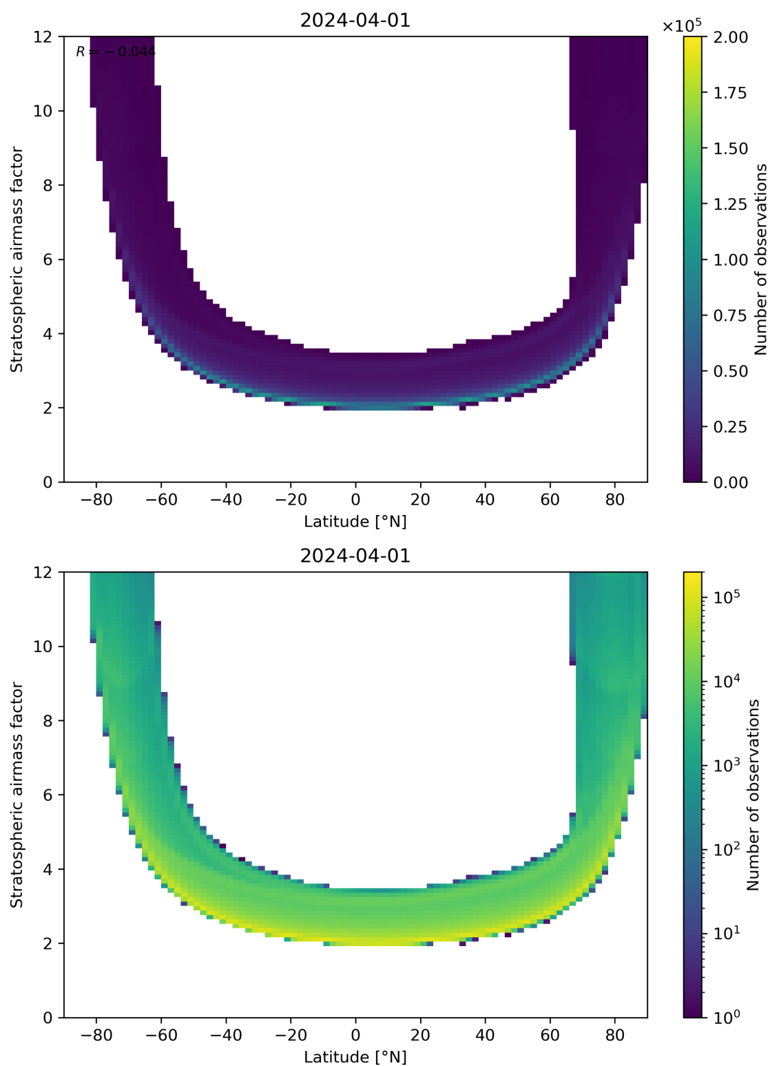
Figure 83: Scatter density plot of “Latitude” against “Stratospheric airmass factor” for 2024-03-31 to 2024-04-02.
