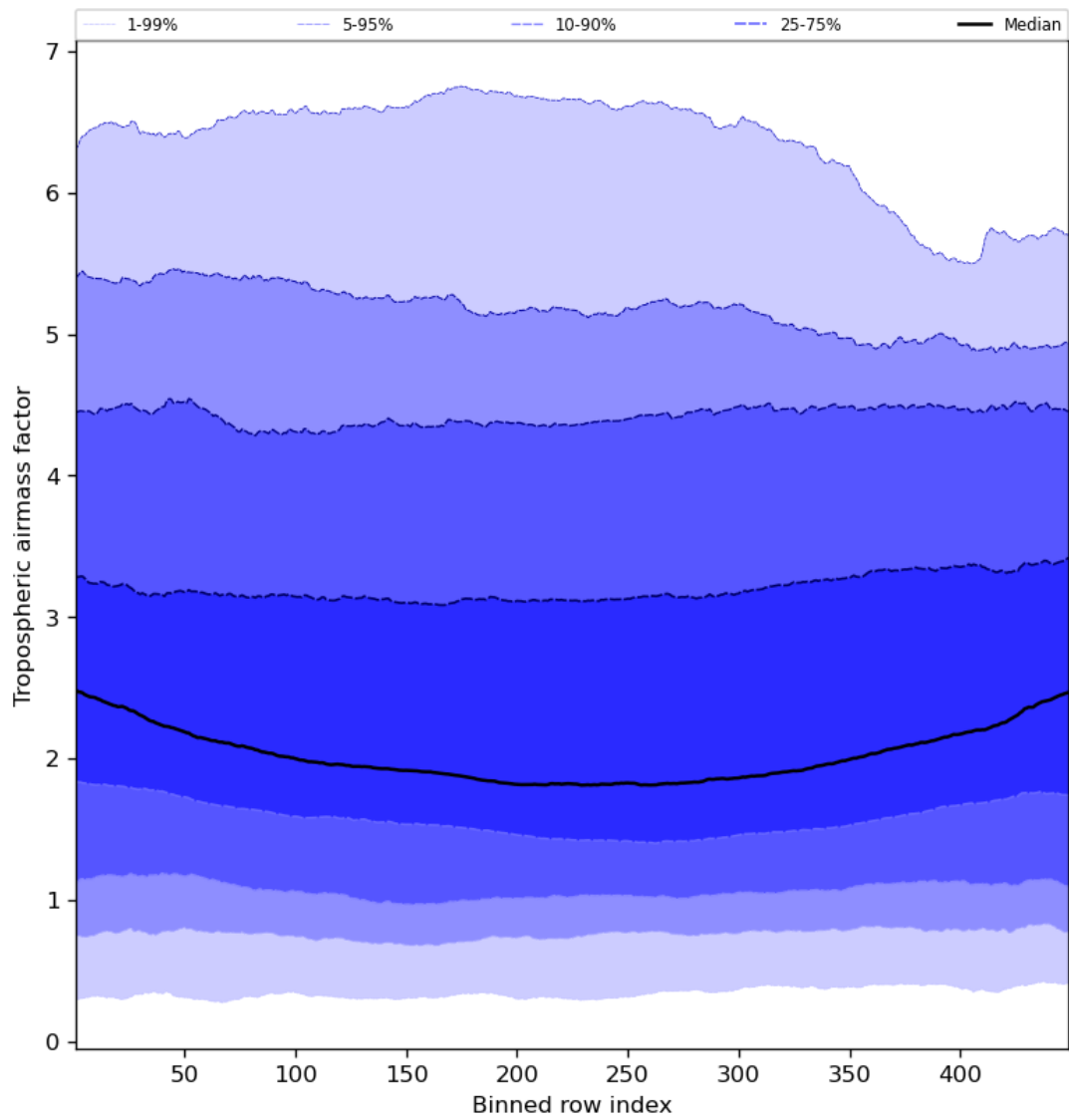
Figure 48: Along track statistics of “Tropospheric air mass factor” for 2024-03-31 to 2024-04-02
