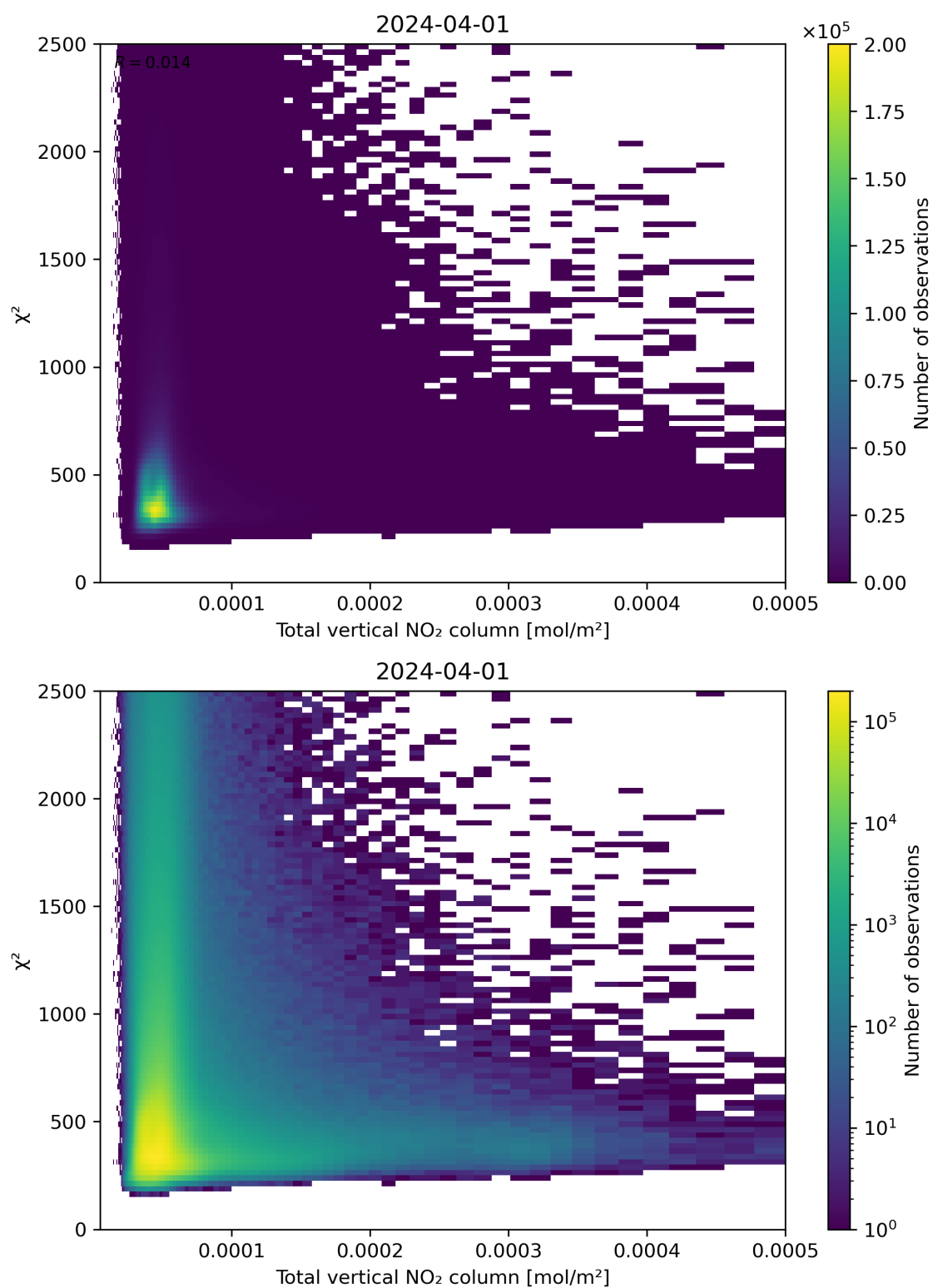
Figure 111: Scatter density plot of “Total vertical NO 2 column” against “ \chi^2 ” for 2024-03-31 to 2024-04-02.
