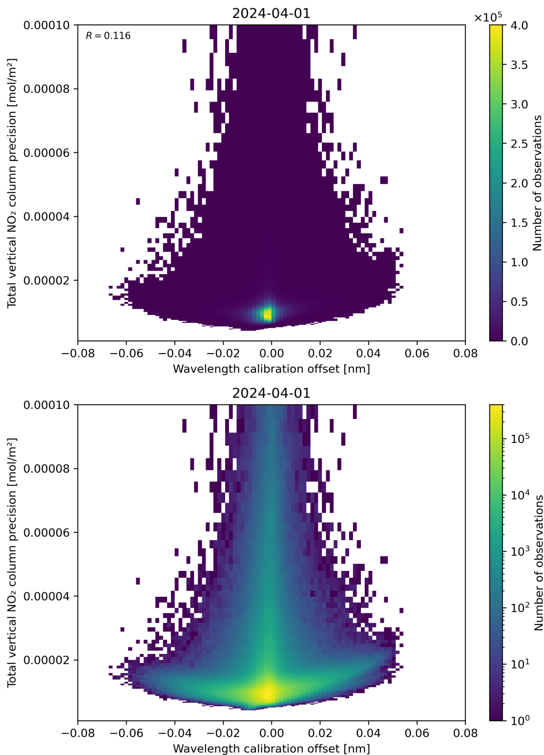
Figure 180: Scatter density plot of “Wavelength calibration offset” against “Total vertical NO 2 column precision” for 2024-03-31 to 2024-04-02.
