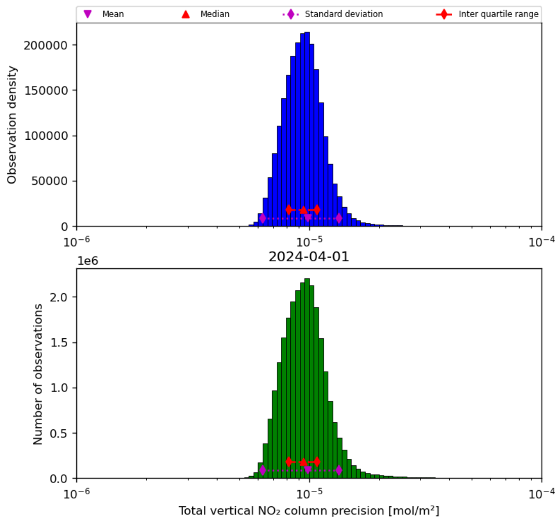
Figure 39: Histogram of “Total vertical NO 2 column precision” for 2024-03-31 to 2024-04-02
