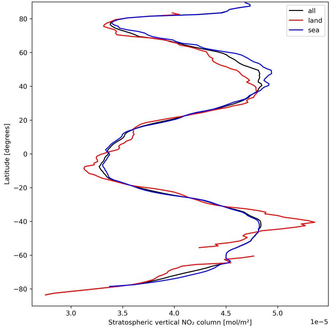
Figure 19: Zonal average of “Stratospheric vertical NO 2 column” for 2024-03-31 to 2024-04-02.
