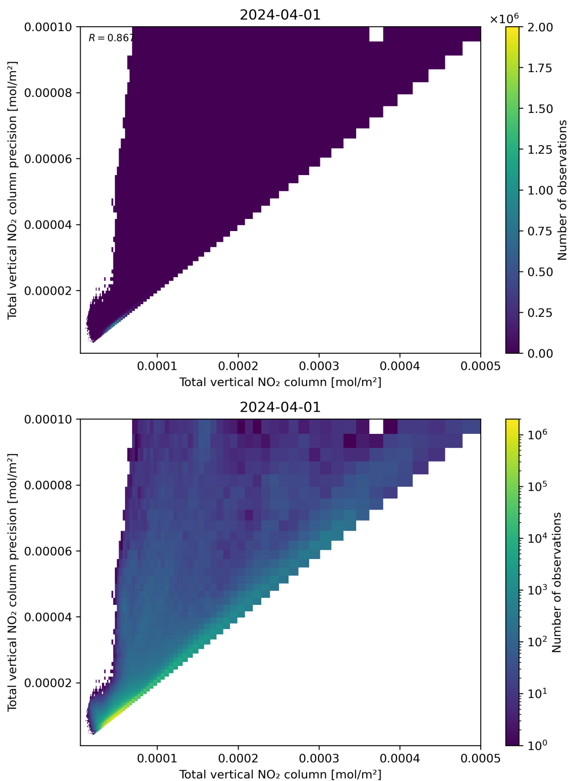
Figure 114: Scatter density plot of “Total vertical NO 2 column” against “Total vertical NO 2 column precision” for 2024-03-31 to 2024-04-02.
