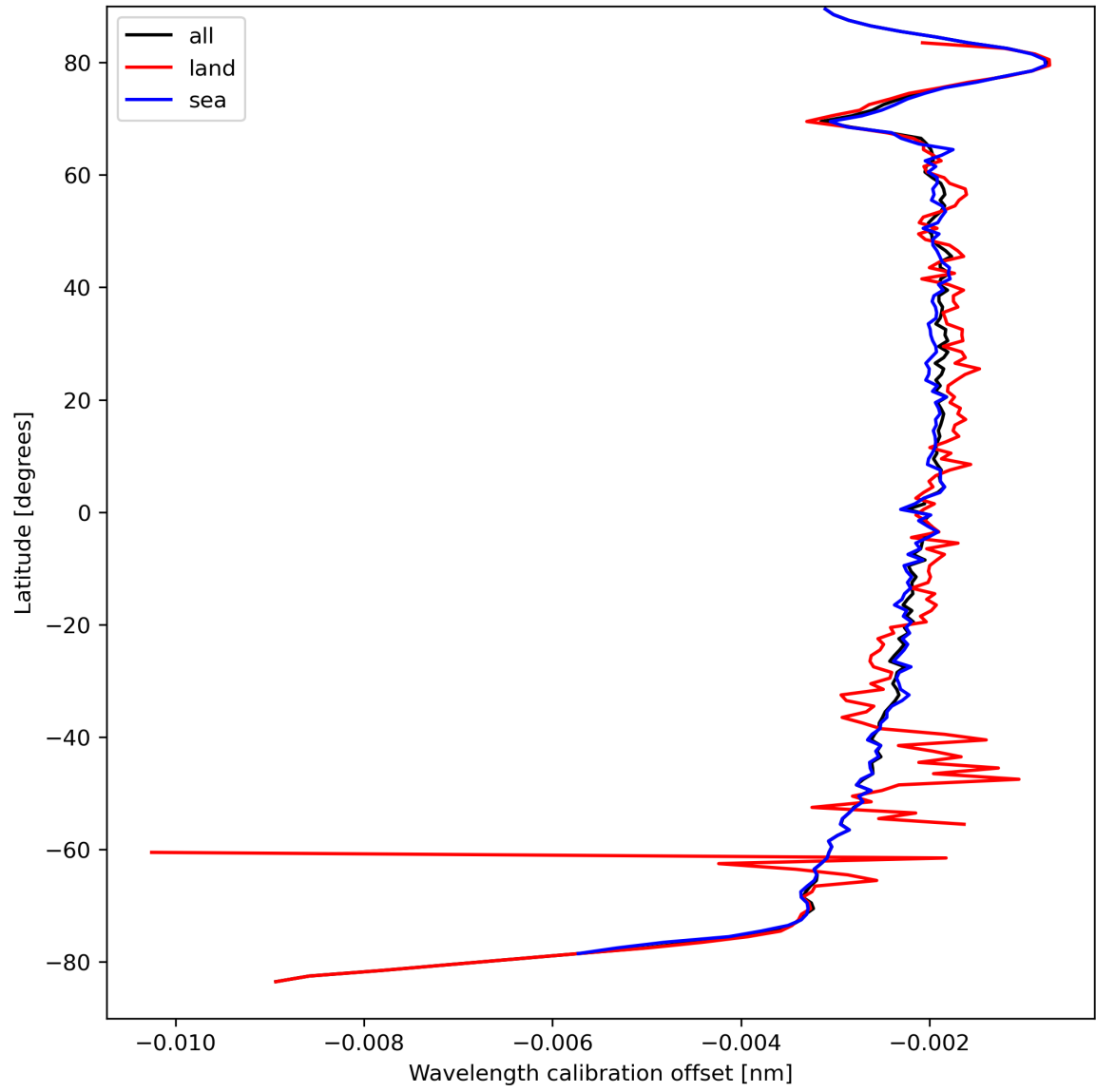
Figure 18: Zonal average of “Wavelength calibration offset” for 2024-03-31 to 2024-04-02.
