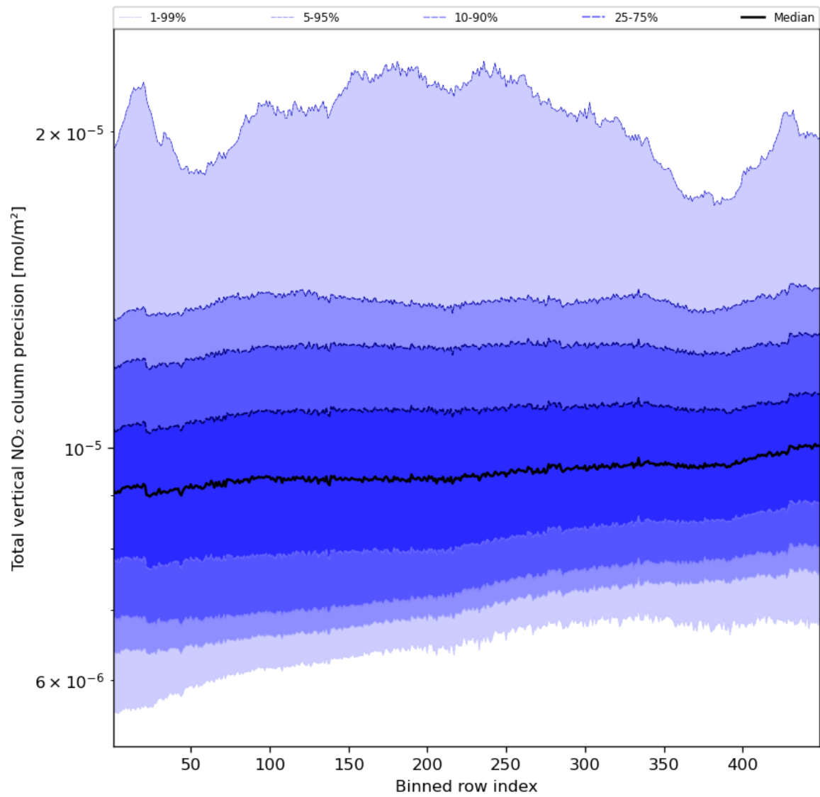
Figure 56: Along track statistics of “Total vertical NO 2 column precision” for 2024-03-31 to 2024-04-02
