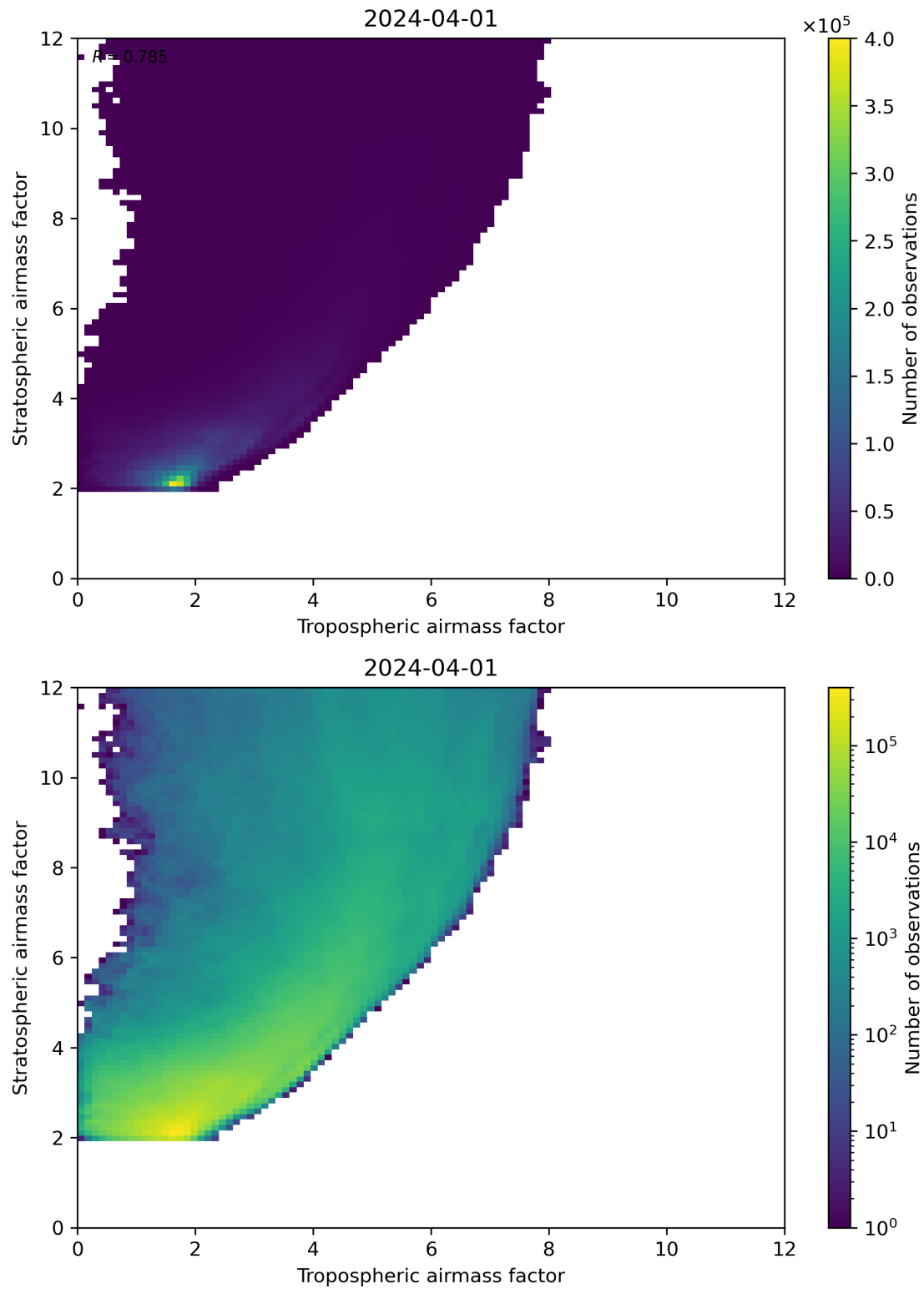
Figure 71: Scatter density plot of “Tropospheric airmass factor” against “Stratospheric airmass factor” for 2024-03-31 to 2024-04-02.
