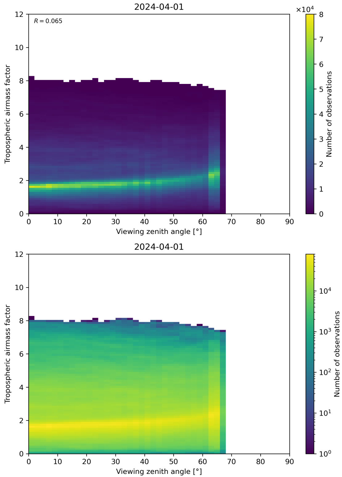
Figure 161: Scatter density plot of “Viewing zenith angle” against “Tropospheric airmass factor” for 2024-03-31 to 2024-04-02.
