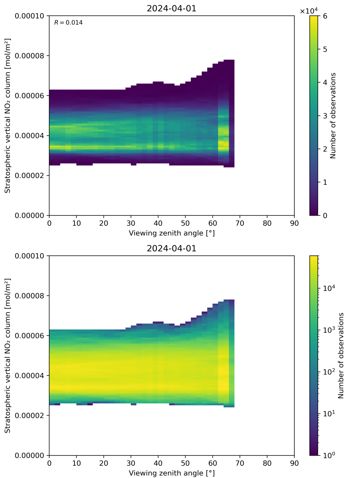
Figure 164: Scatter density plot of “Viewing zenith angle” against “Stratospheric vertical NO 2 column” for 2024-03-31 to 2024-04-02.
