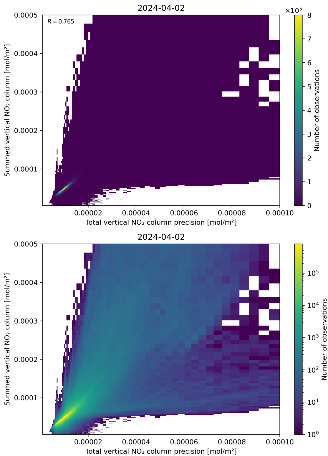
Figure 117: Scatter density plot of “Total vertical NO 2 column precision” against “Summed vertical NO 2 column” for 2024-04-01 to 2024-04-03.
