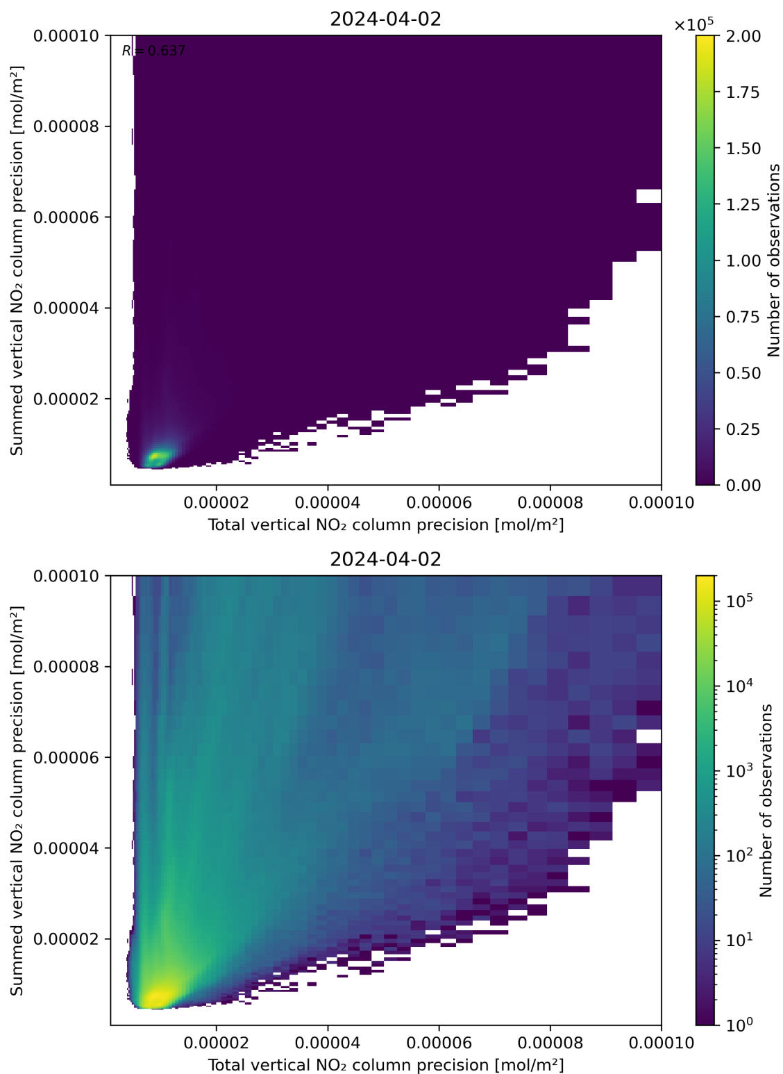
Figure 118: Scatter density plot of “Total vertical NO 2 column precision” against “Summed vertical NO 2 column precision” for 2024-04-01 to 2024-04-03.
