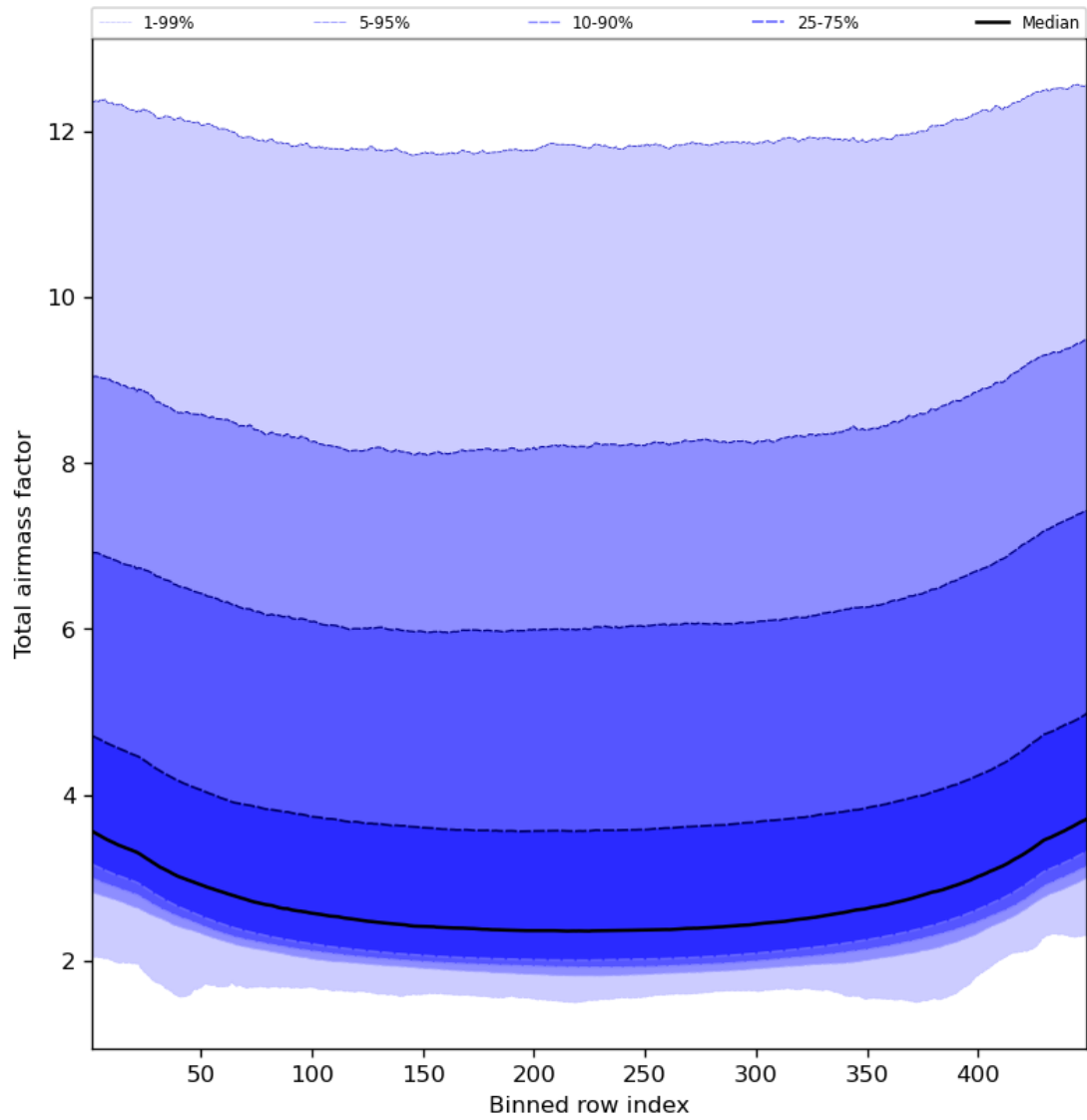
Figure 49: Along track statistics of “Total airmass factor” for 2024-04-01 to 2024-04-03
