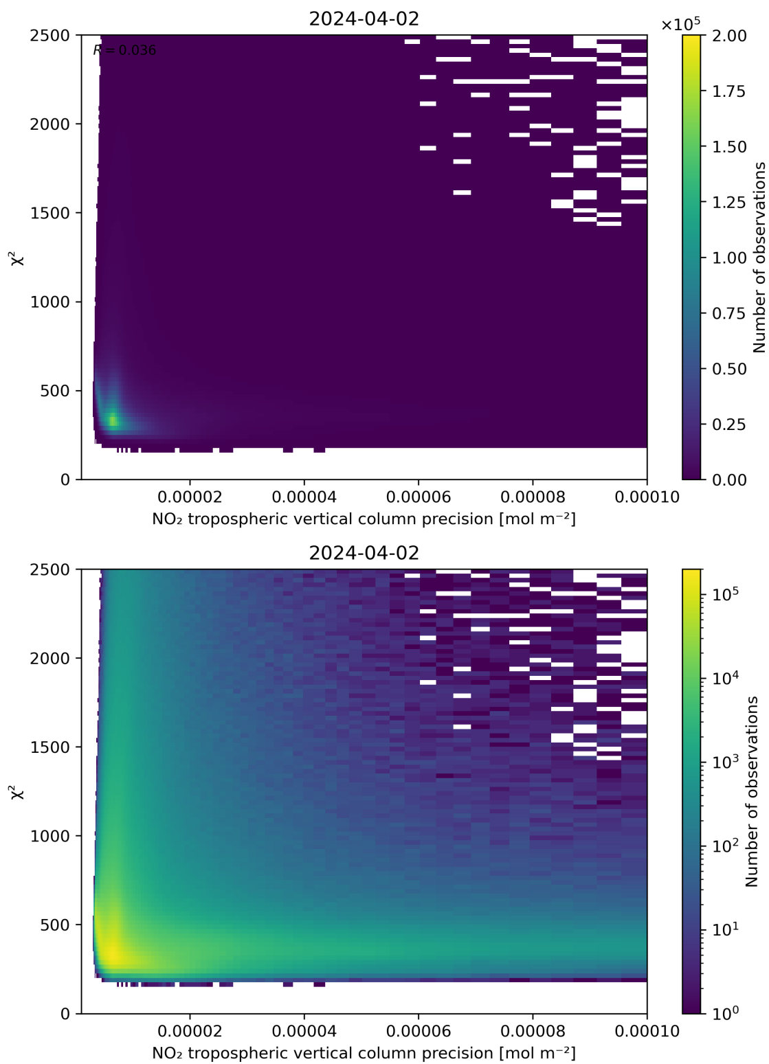
Figure 134: Scatter density plot of “NO 2 tropospheric vertical column precision” against “ \chi^2 ” for 2024-04-01 to 2024-04-03.
