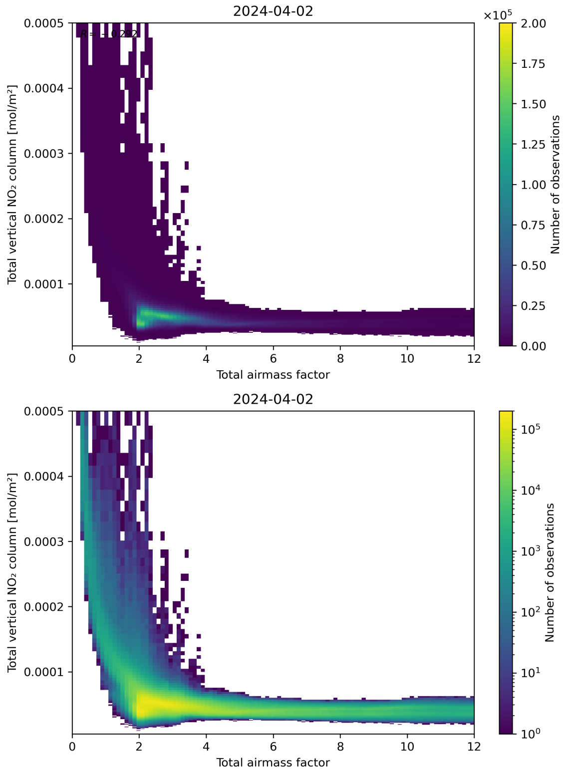
Figure 67: Scatter density plot of “Total airmass factor” against “Total vertical NO 2 column” for 2024-04-01 to 2024-04-03.
