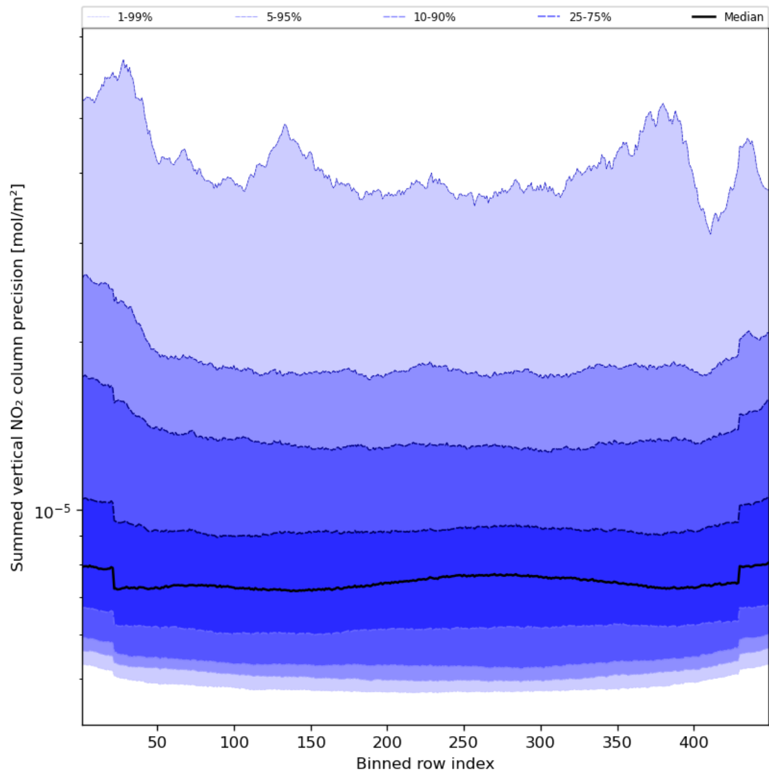
Figure 58: Along track statistics of “Summed vertical NO 2 column precision” for 2024-04-01 to 2024-04-03
