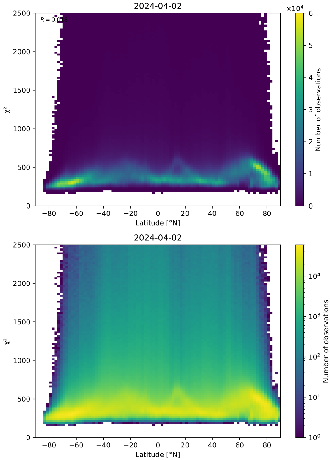
Figure 86: Scatter density plot of “Latitude” against “ \chi^2 ” for 2024-04-01 to 2024-04-03.
