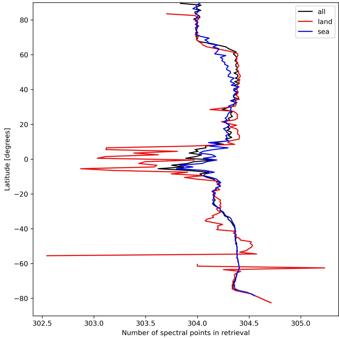
Figure 16: Zonal average of “Number of spectral points in retrieval” for 2024-04-01 to 2024-04-03.
