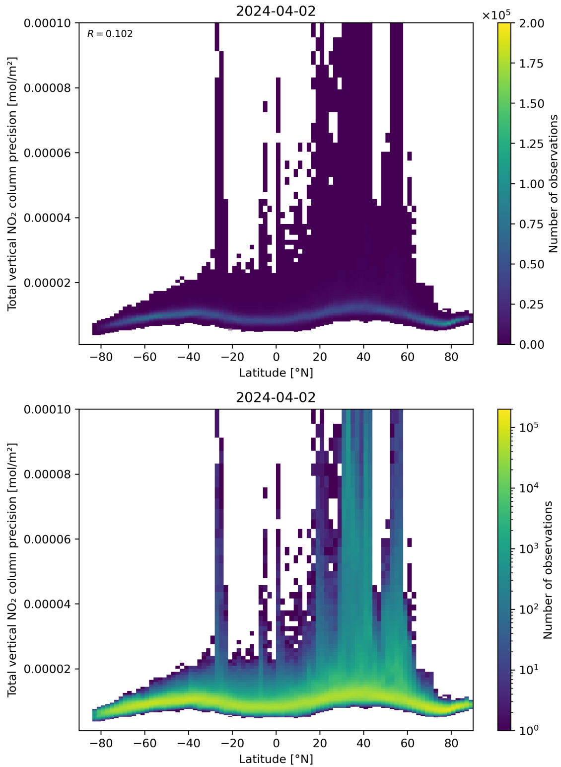
Figure 91: Scatter density plot of “Latitude” against “Total vertical NO 2 column precision” for 2024-04-01 to 2024-04-03.
