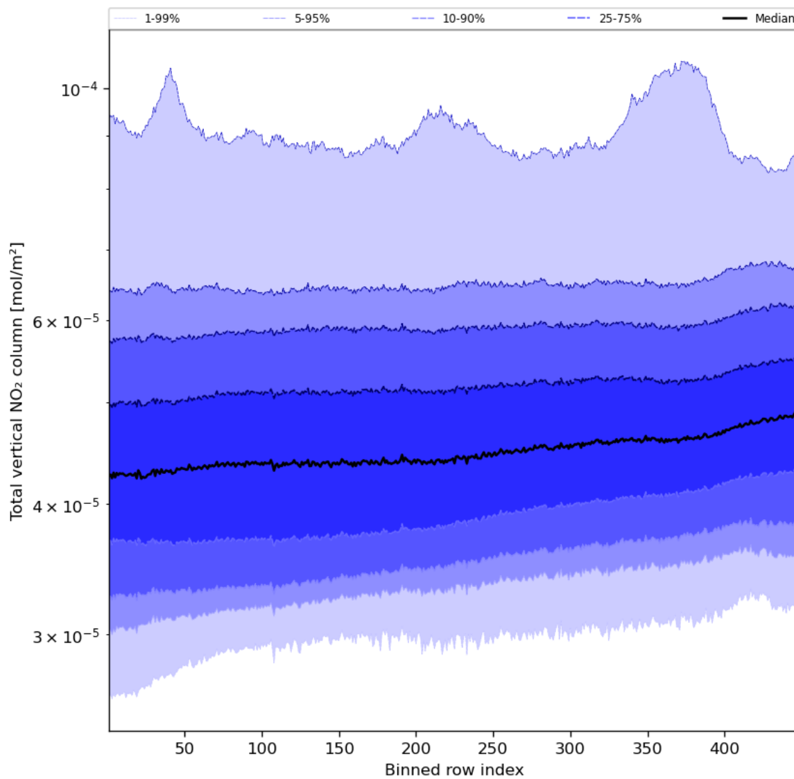
Figure 55: Along track statistics of “Total vertical NO 2 column” for 2024-04-01 to 2024-04-03
