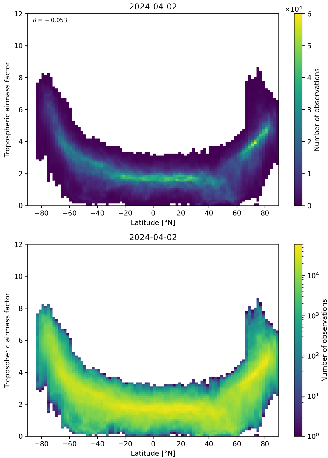
Figure 85: Scatter density plot of “Latitude” against “Tropospheric air mass factor” for 2024-04-01 to 2024-04-03.
