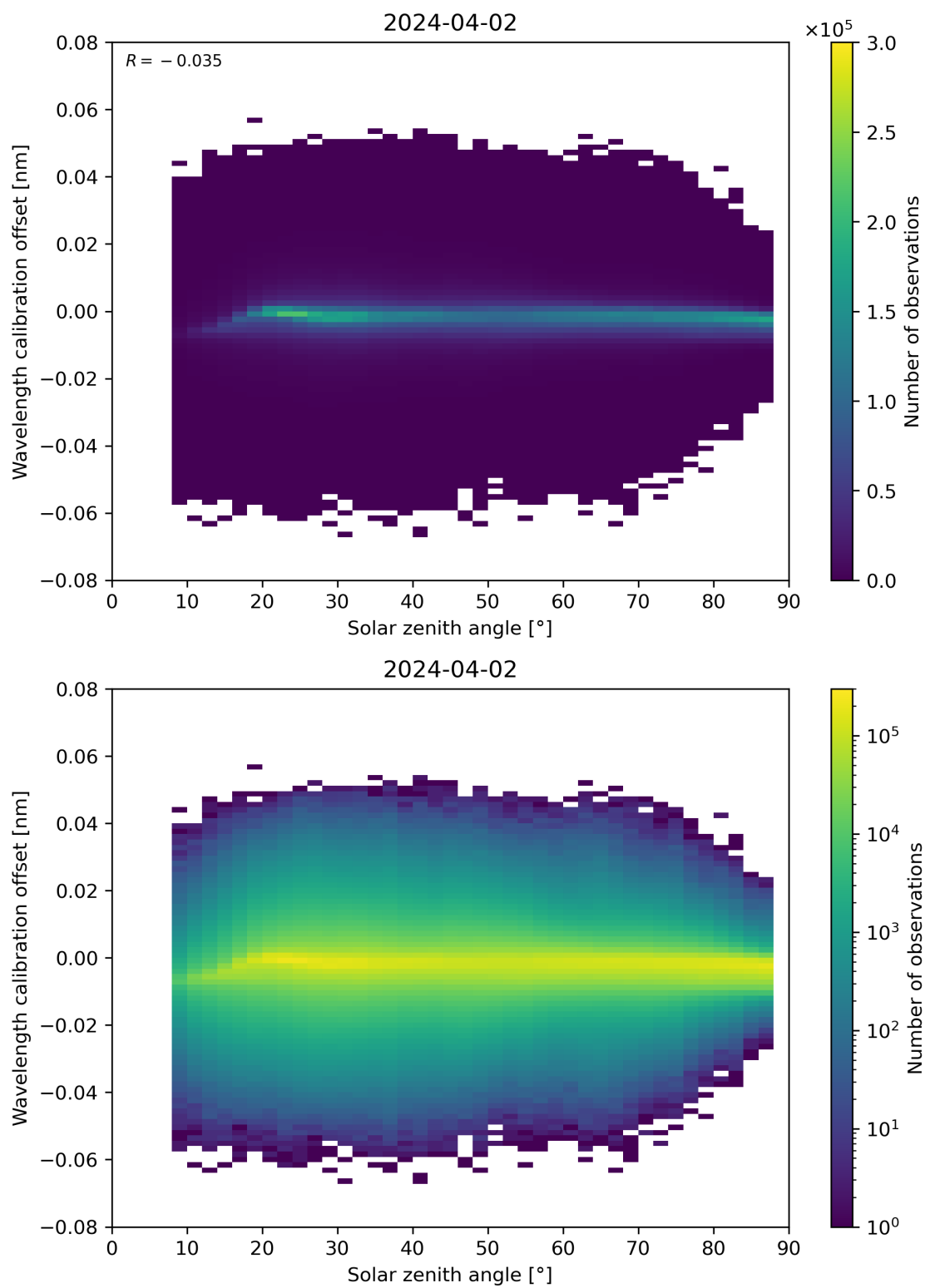
Figure 158: Scatter density plot of “Solar zenith angle” against “Wavelength calibration offset” for 2024-04-01 to 2024-04-03.
