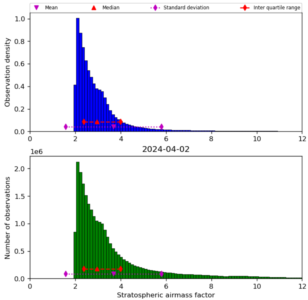
Figure 44: Histogram of “Stratospheric airmass factor” for 2024-04-01 to 2024-04-03
