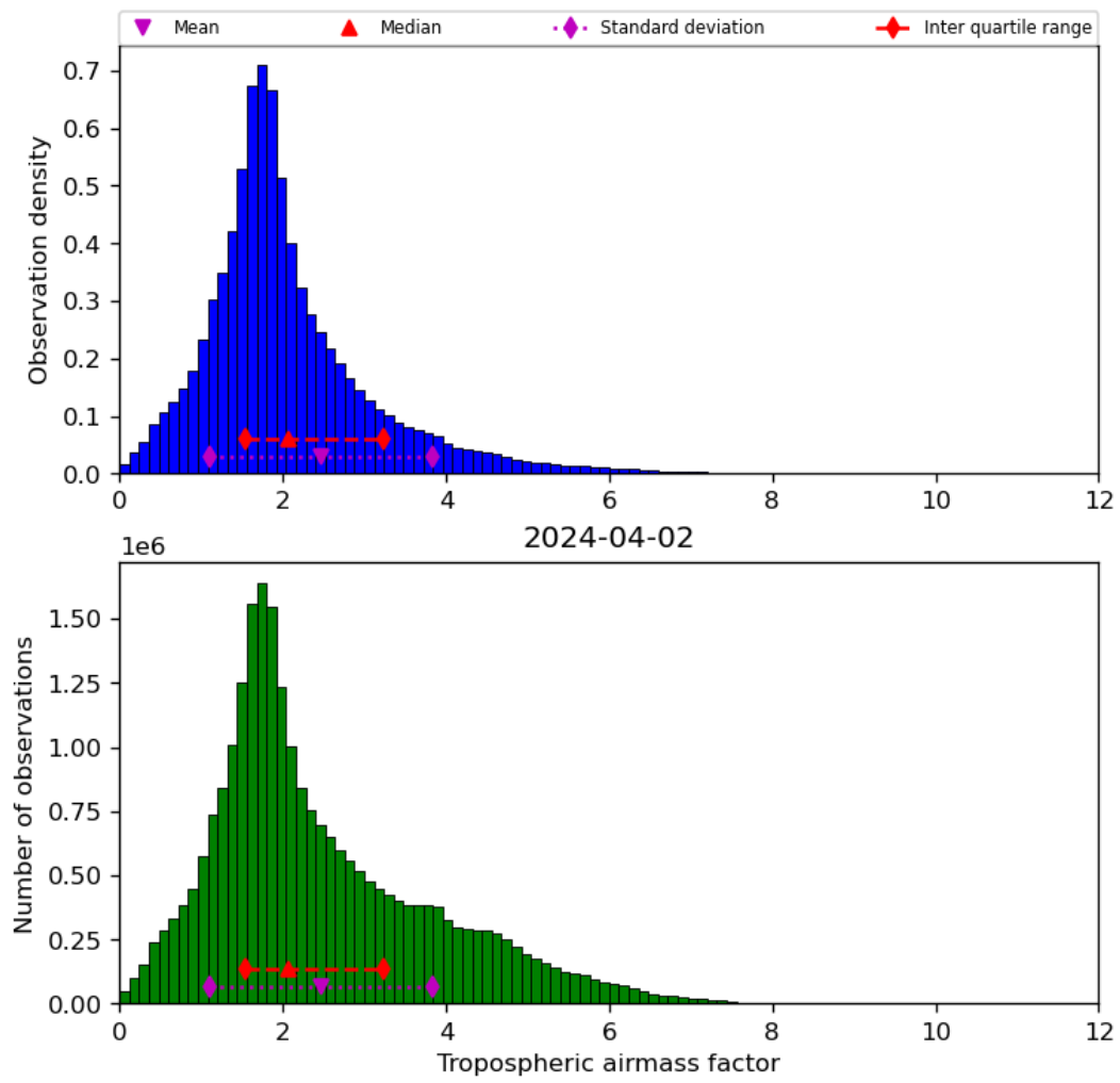
Figure 31: Histogram of “Tropospheric airmass factor” for 2024-04-01 to 2024-04-03
