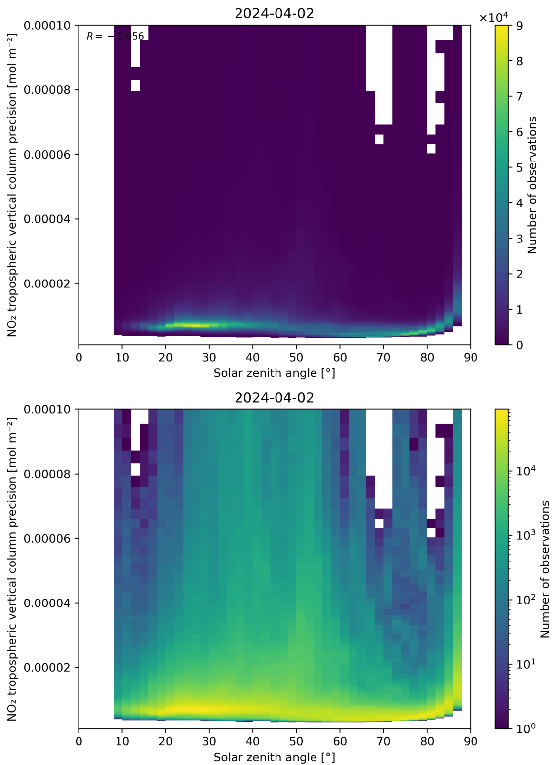
Figure 156: Scatter density plot of “Solar zenith angle” against “NO 2 tropospheric vertical column precision” for 2024-04-01 to 2024-04-03.
