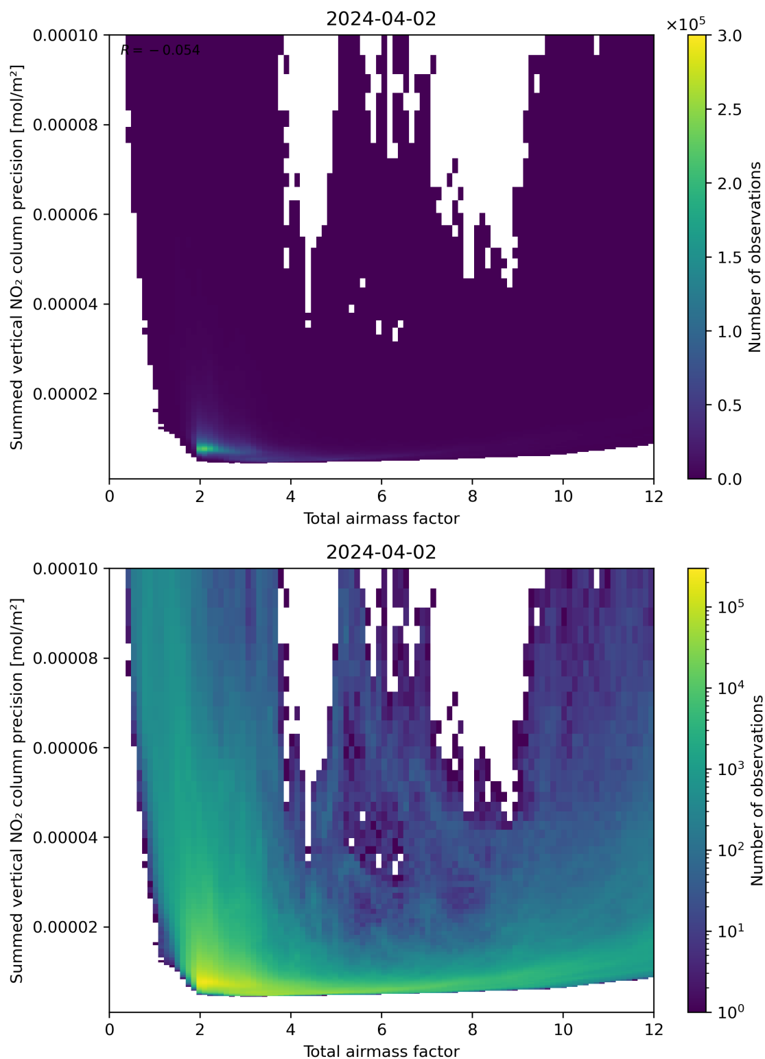
Figure 66: Scatter density plot of “Total airmass factor” against “Summed vertical NO 2 column precision” for 2024-04-01 to 2024-04-03.
