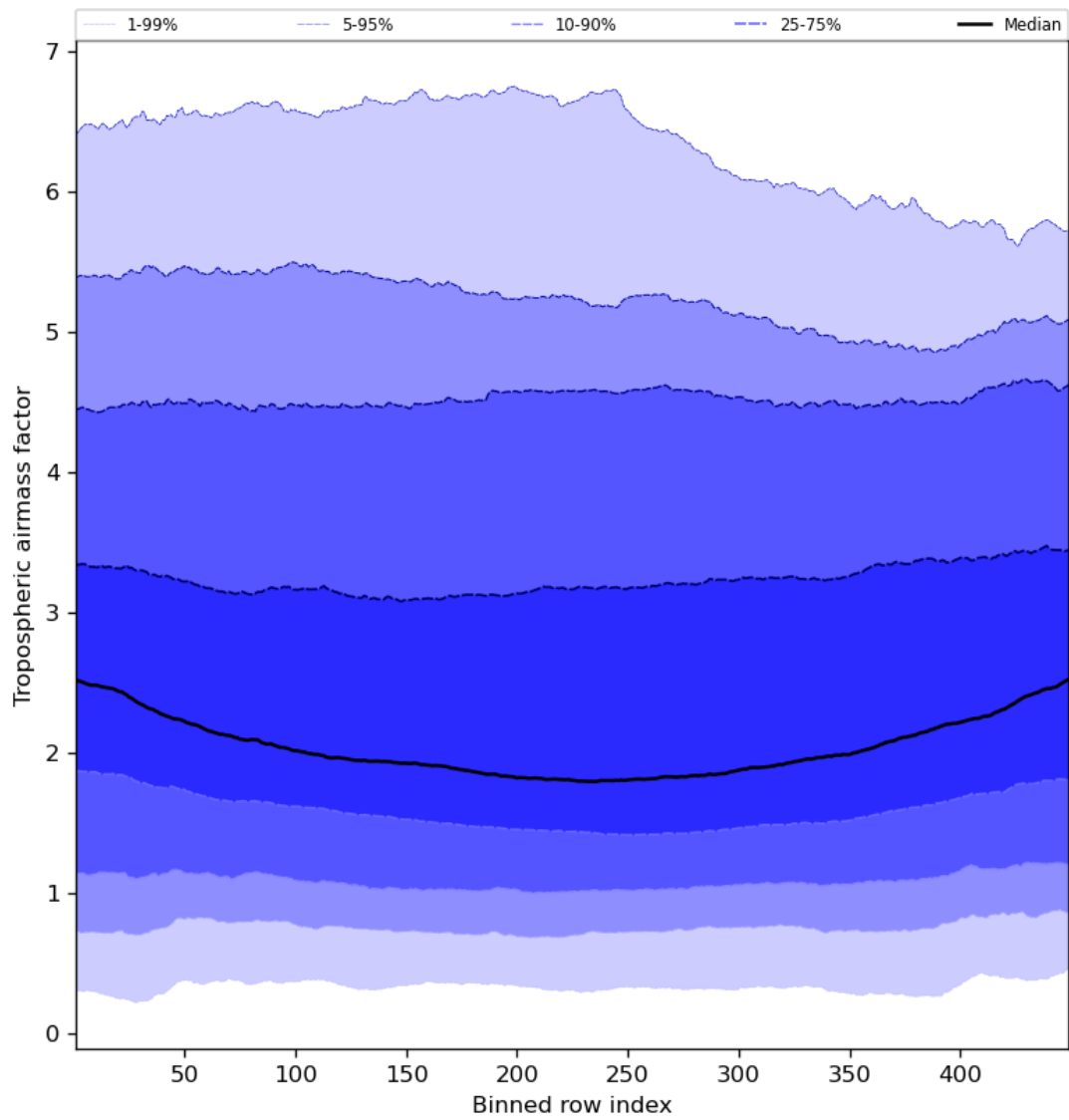
Figure 48: Along track statistics of “Tropospheric airmass factor” for 2024-04-01 to 2024-04-03
