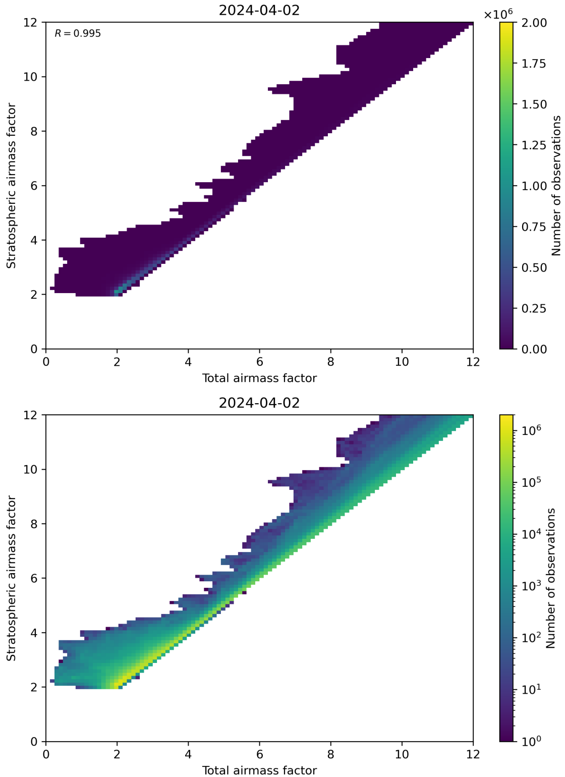
Figure 62: Scatter density plot of “Total airmass factor” against “Stratospheric airmass factor” for 2024-04-01 to 2024-04-03.
