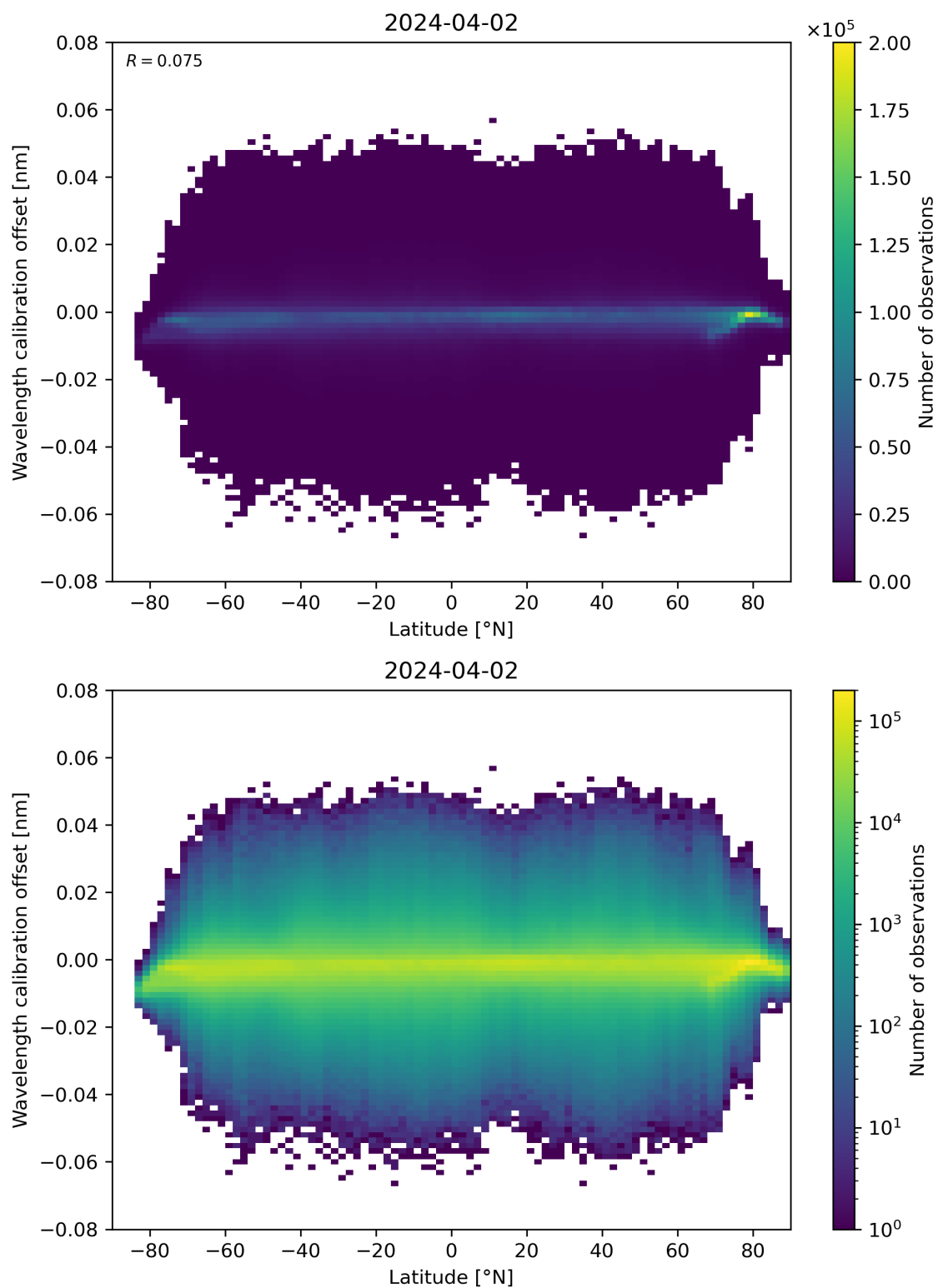
Figure 95: Scatter density plot of “Latitude” against “Wavelength calibration offset” for 2024-04-01 to 2024-04-03.
