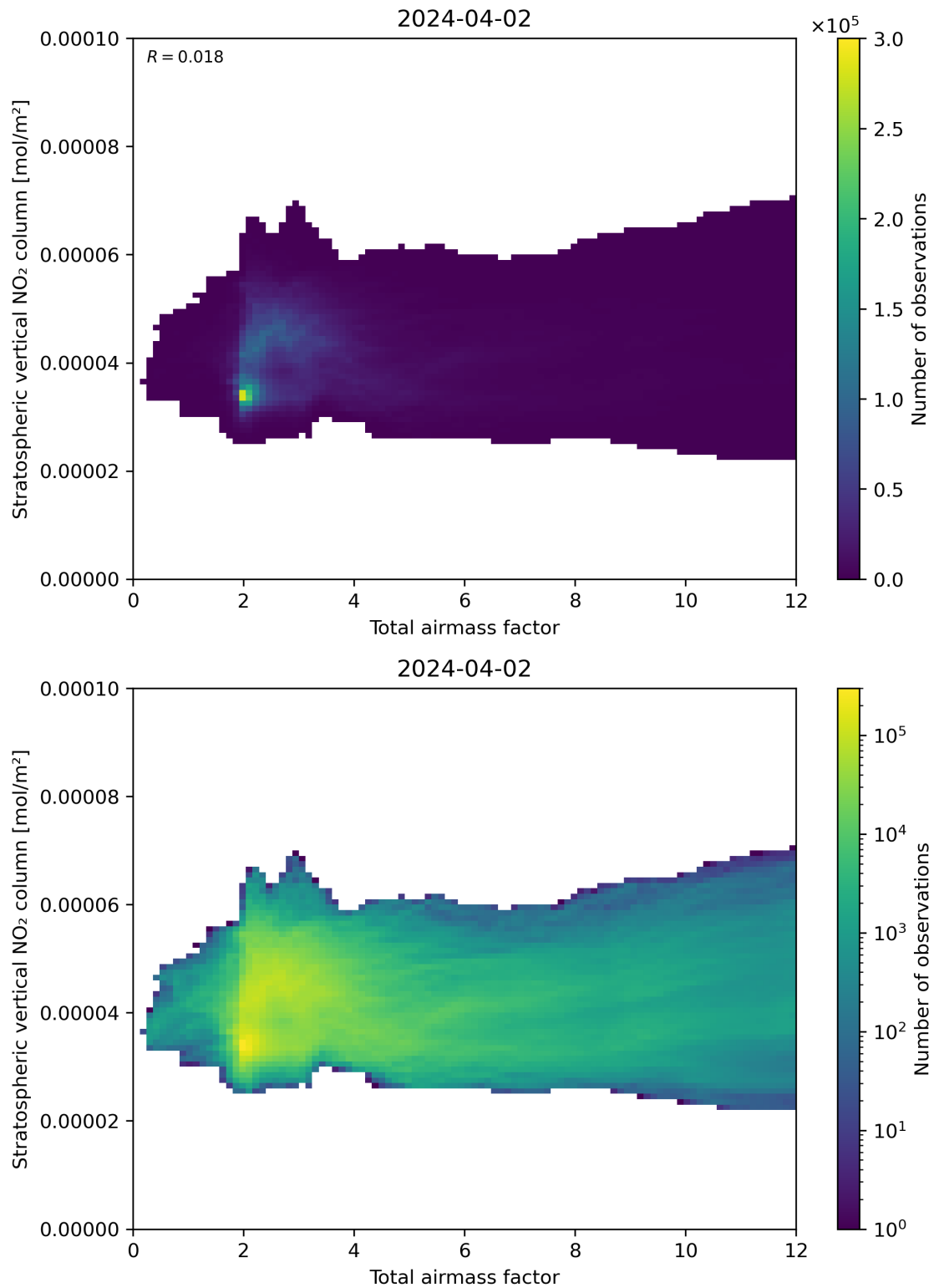
Figure 64: Scatter density plot of “Total airmass factor” against “Stratospheric vertical \text{NO}_2 column” for 2024-04-01 to 2024-04-03.
