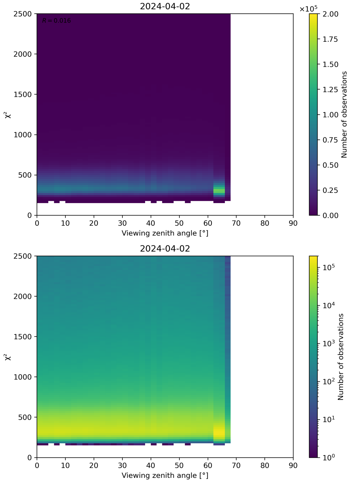
Figure 162: Scatter density plot of “Viewing zenith angle” against “ \chi^2 ” for 2024-04-01 to 2024-04-03.
