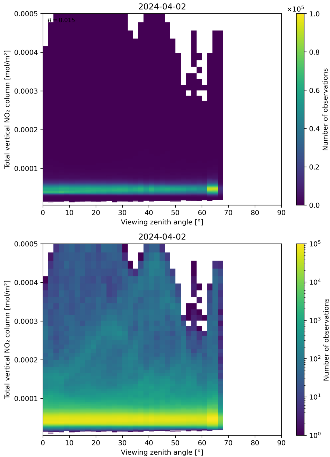
Figure 167: Scatter density plot of “Viewing zenith angle” against “Total vertical NO 2 column” for 2024-04-01 to 2024-04-03.
