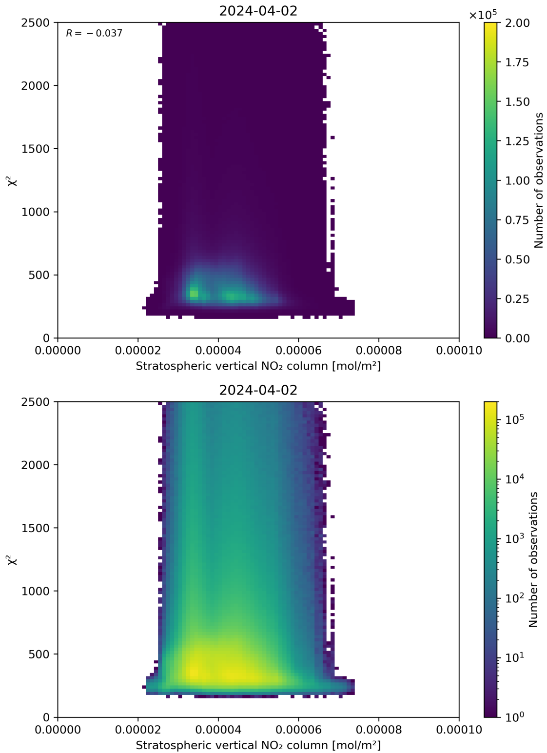
Figure 97: Scatter density plot of “Stratospheric vertical NO 2 column” against “ \chi^2 ” for 2024-04-01 to 2024-04-03.
