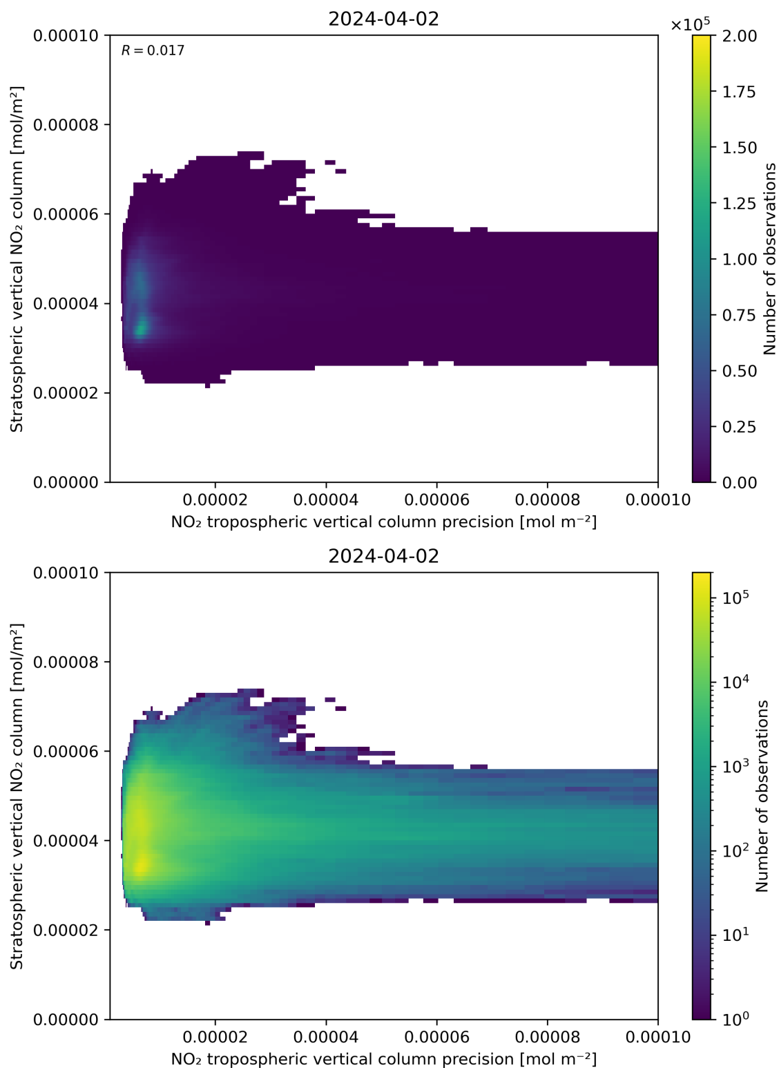
Figure 135: Scatter density plot of “NO 2 tropospheric vertical column precision” against “Stratospheric vertical NO 2 column” for 2024-04-01 to 2024-04-03.
