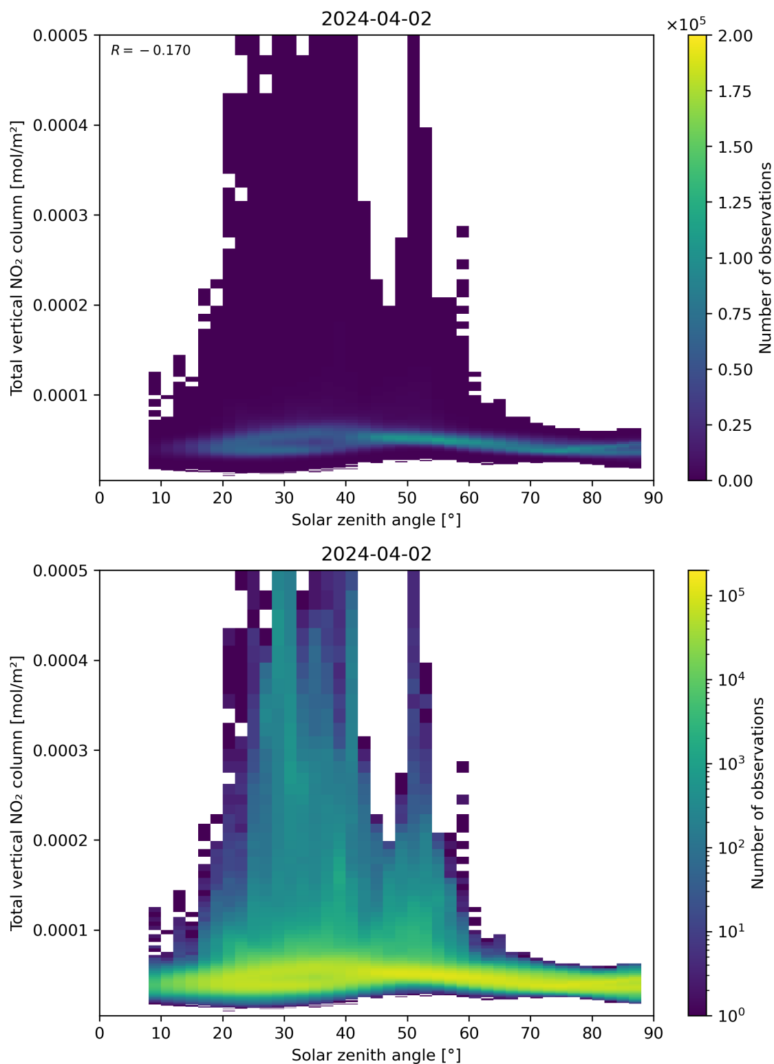
Figure 153: Scatter density plot of “Solar zenith angle” against “Total vertical NO 2 column” for 2024-04-01 to 2024-04-03.
