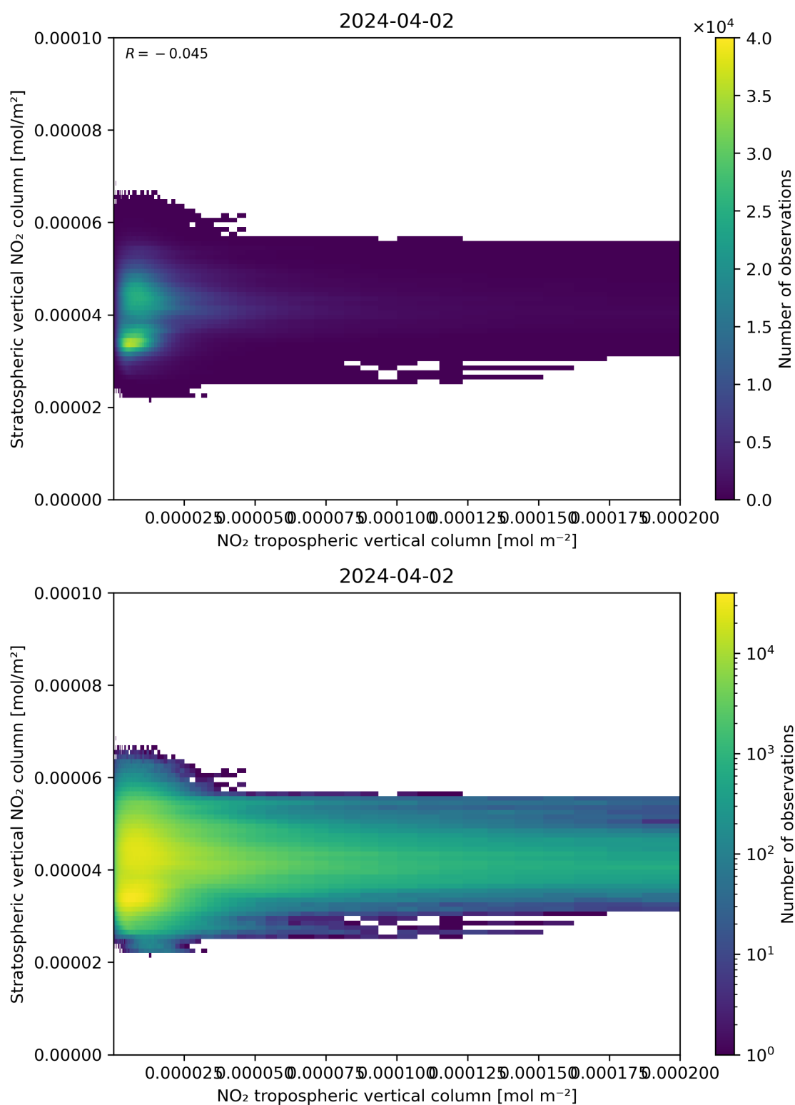
Figure 125: Scatter density plot of “NO 2 tropospheric vertical column” against “Stratospheric vertical NO 2 column” for 2024-04-01 to 2024-04-03.
