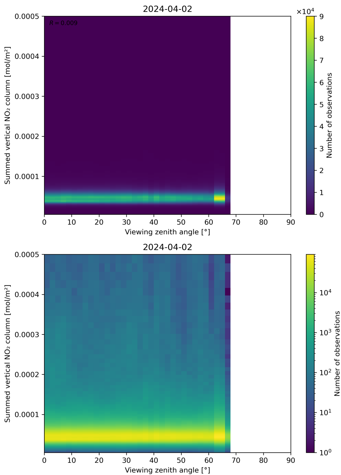
Figure 165: Scatter density plot of “Viewing zenith angle” against “Summed vertical NO 2 column” for 2024-04-01 to 2024-04-03.
