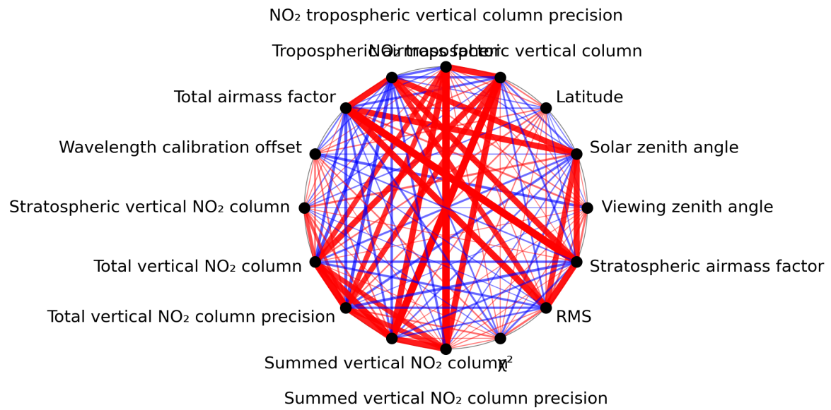
Figure 1: Map of correlation graph for 2024-04-01 to 2024-04-03.
