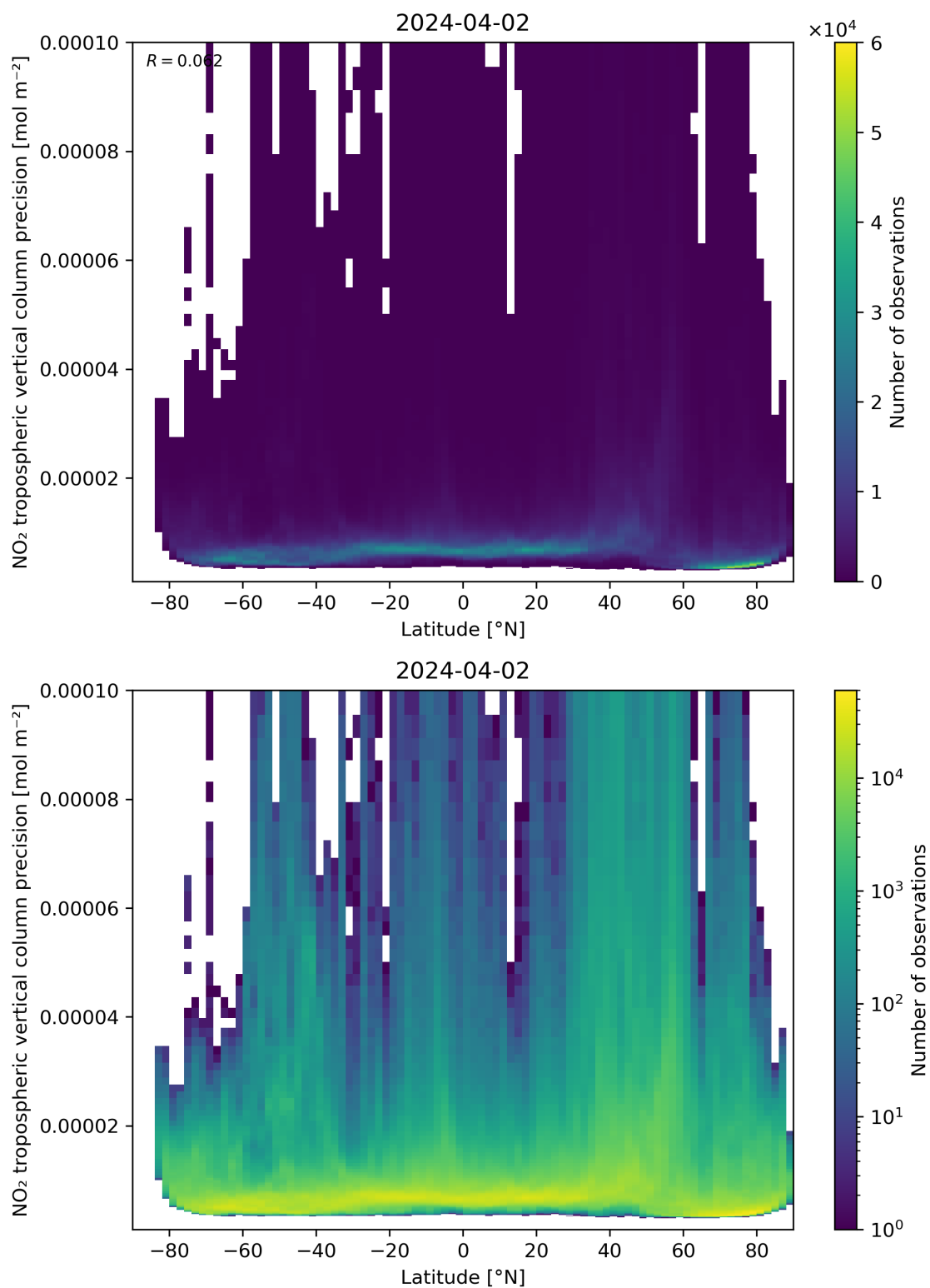
Figure 93: Scatter density plot of “Latitude” against “NO 2 tropospheric vertical column precision” for 2024-04-01 to 2024-04-03.
