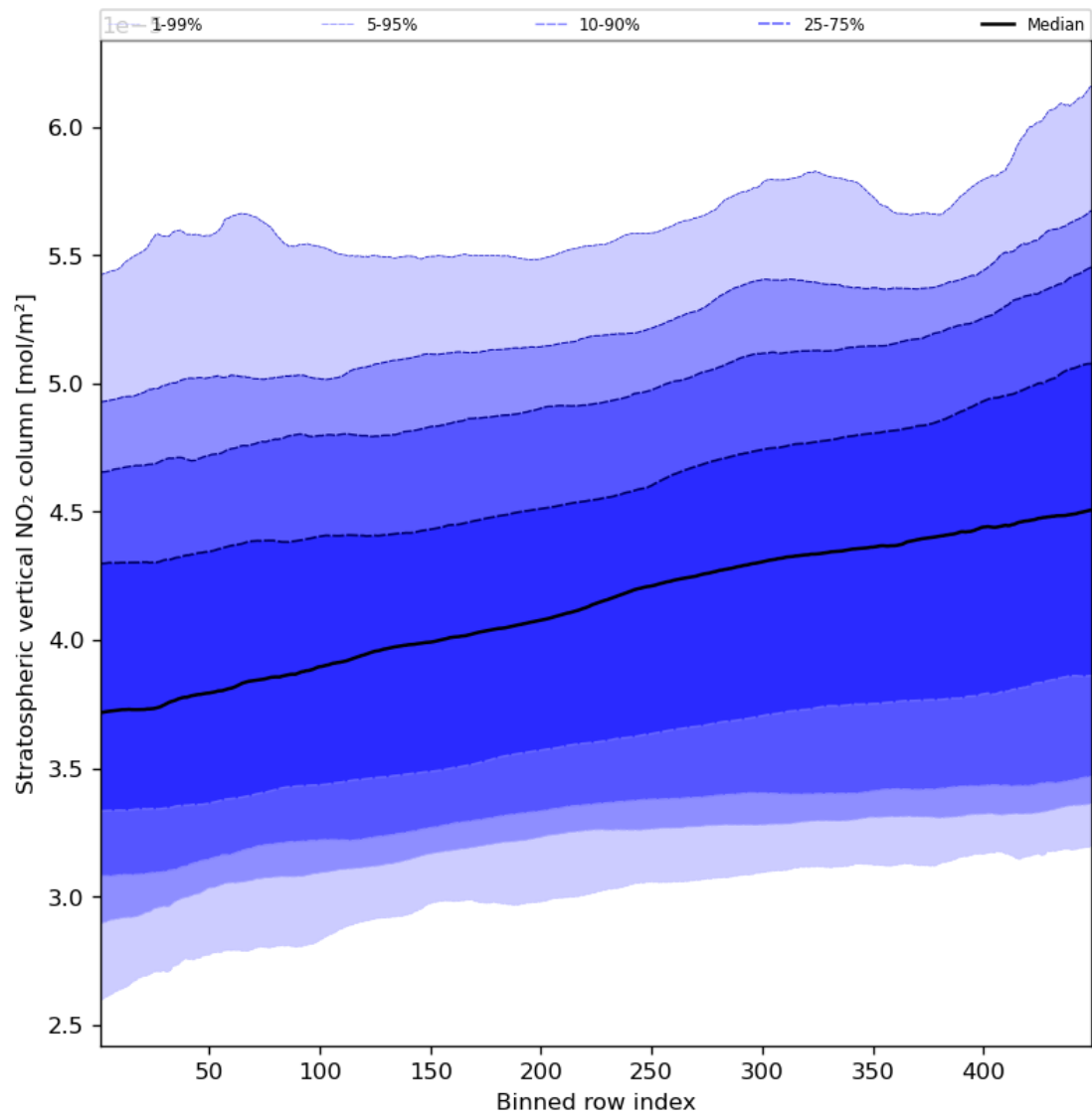
Figure 53: Along track statistics of “Stratospheric vertical NO 2 column” for 2024-04-01 to 2024-04-03
