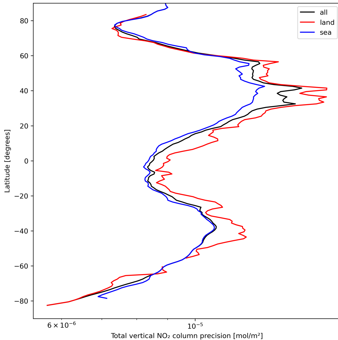
Figure 22: Zonal average of “Total vertical NO 2 column precision” for 2024-04-01 to 2024-04-03.
