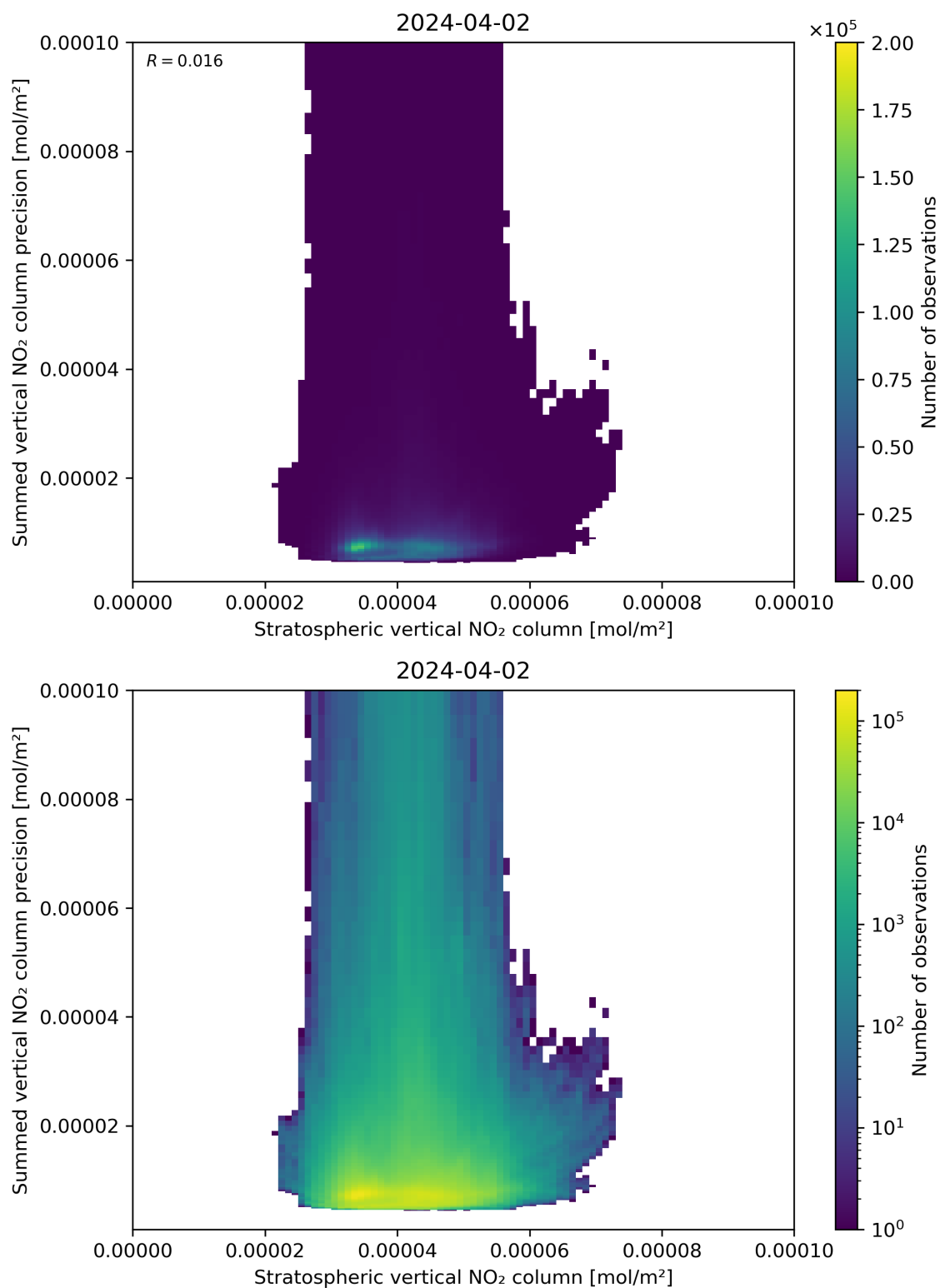
Figure 99: Scatter density plot of “Stratospheric vertical NO 2 column” against “Summed vertical NO 2 column precision” for 2024-04-01 to 2024-04-03.
