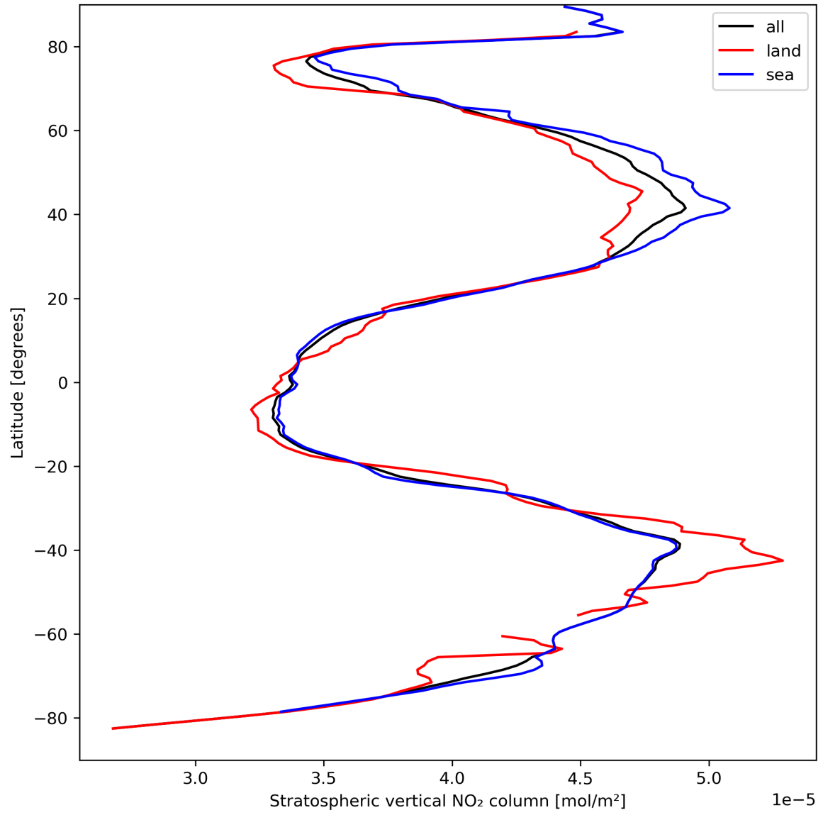
Figure 19: Zonal average of “Stratospheric vertical NO 2 column” for 2024-04-01 to 2024-04-03.
