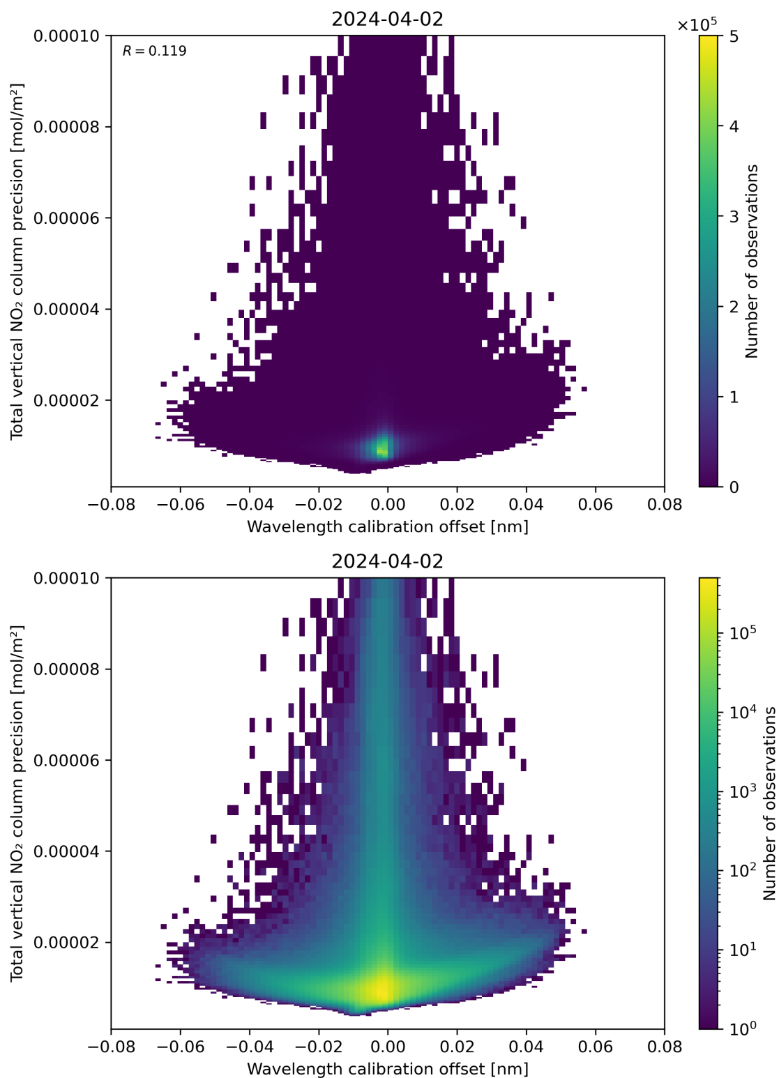
Figure 180: Scatter density plot of “Wavelength calibration offset” against “Total vertical NO 2 column precision” for 2024-04-01 to 2024-04-03.
