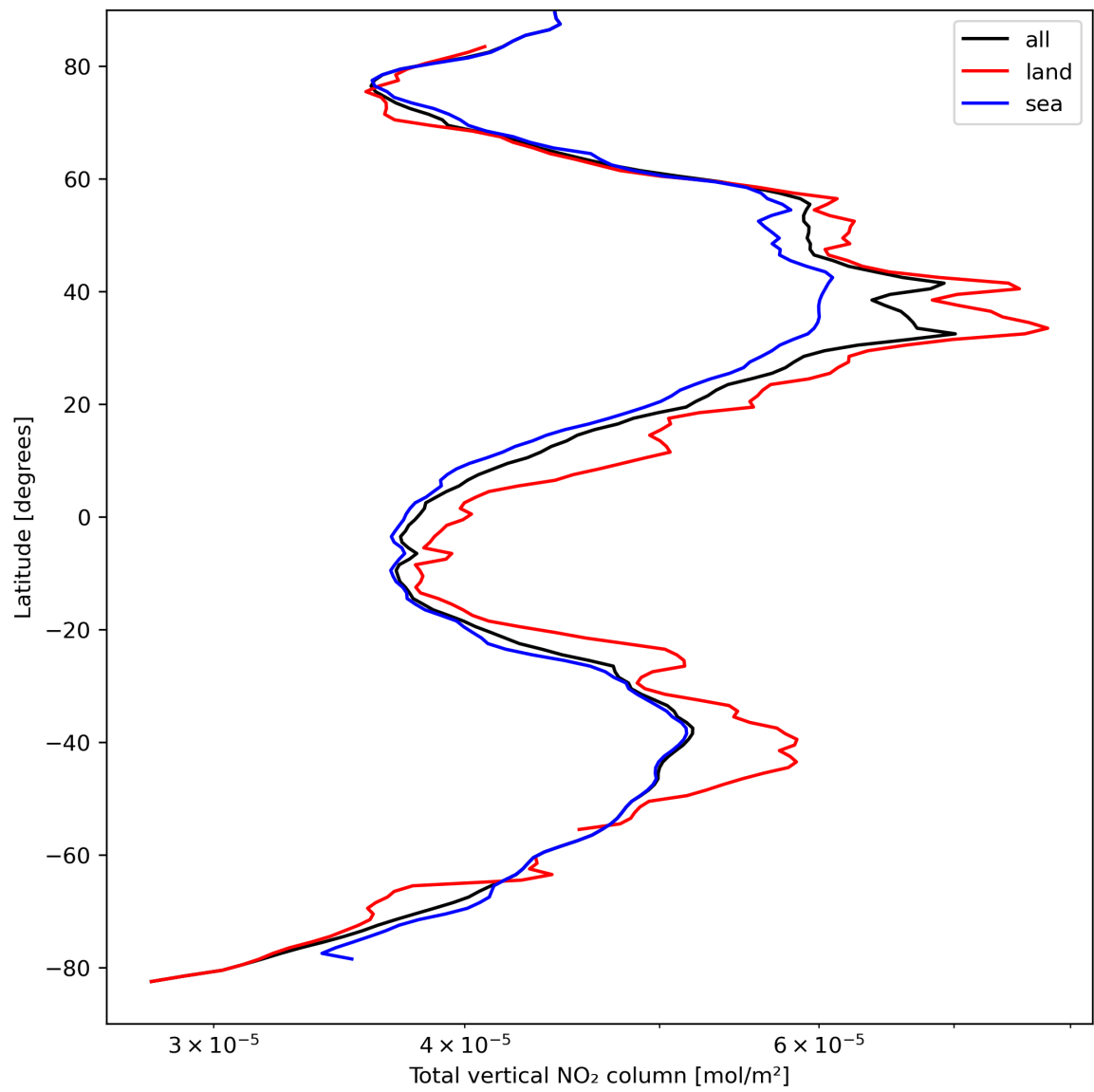
Figure 21: Zonal average of “Total vertical NO 2 column” for 2024-04-01 to 2024-04-03.
