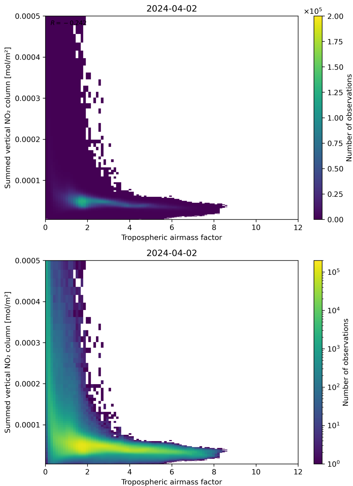
Figure 75: Scatter density plot of “Tropospheric airmass factor” against “Summed vertical NO 2 column” for 2024-04-01 to 2024-04-03.
