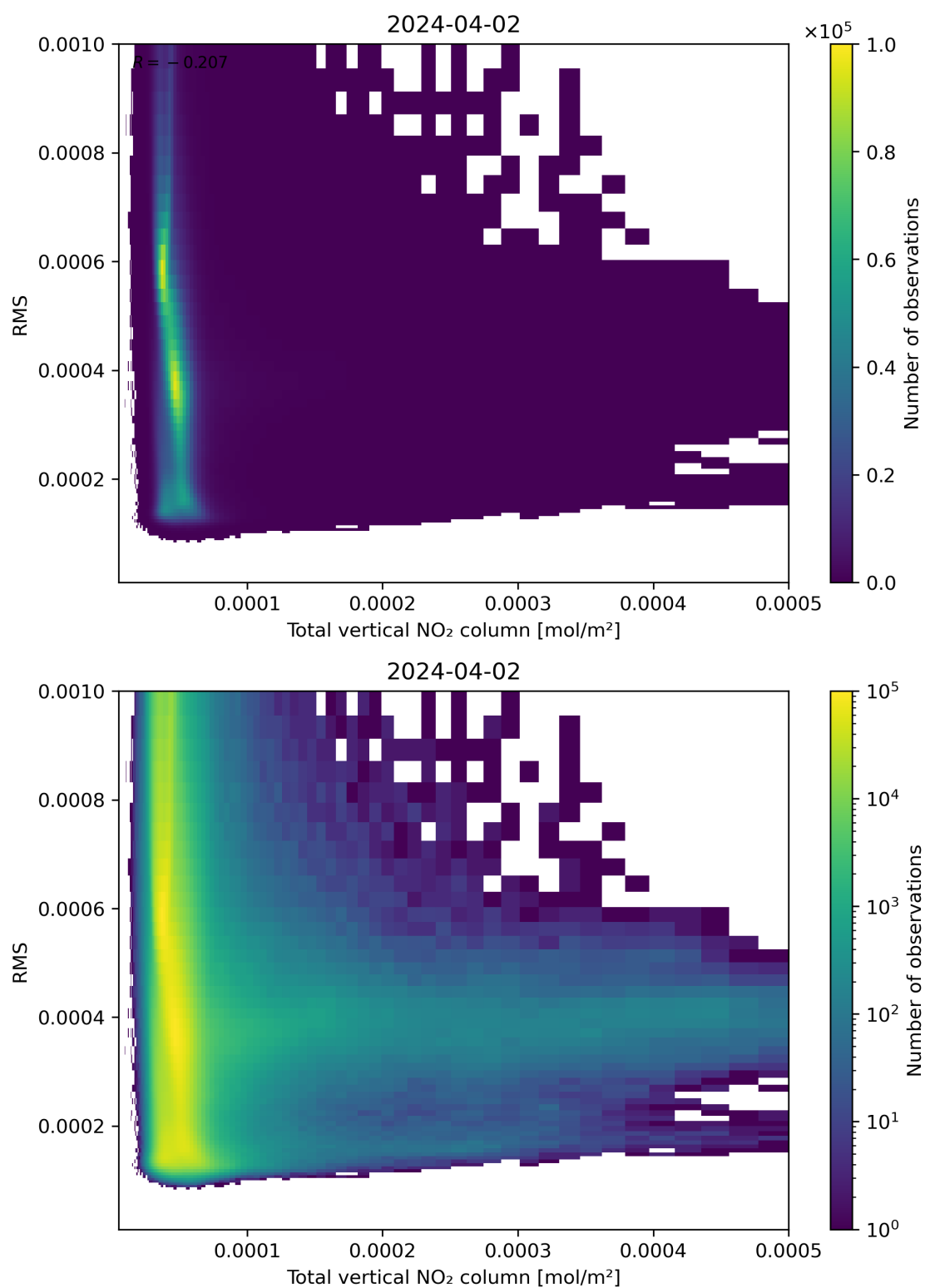
Figure 120: Scatter density plot of “Total vertical NO 2 column” against “RMS” for 2024-04-01 to 2024-04-03.
