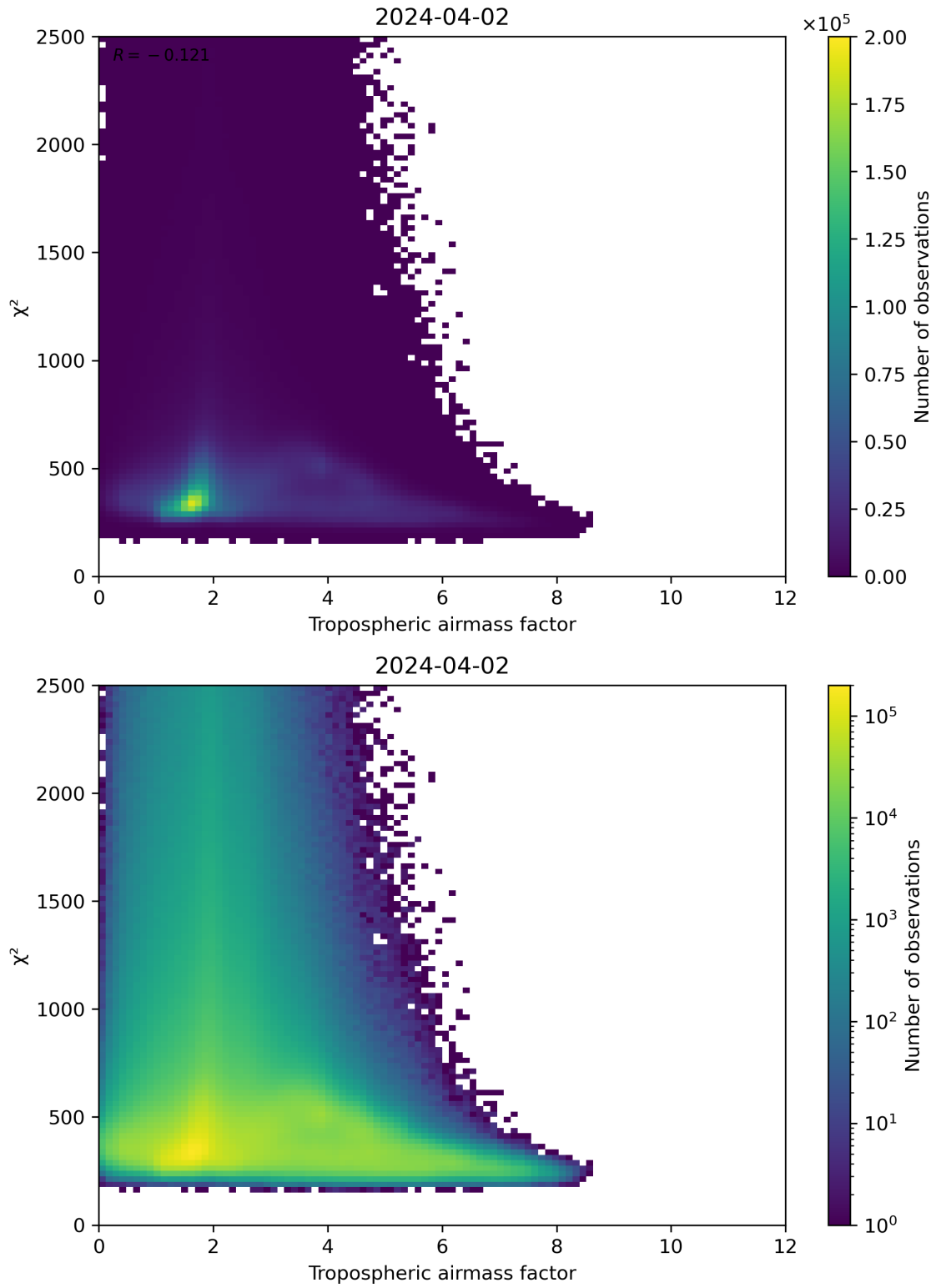
Figure 73: Scatter density plot of “Tropospheric airmass factor” against “ \chi^2 ” for 2024-04-01 to 2024-04-03.
