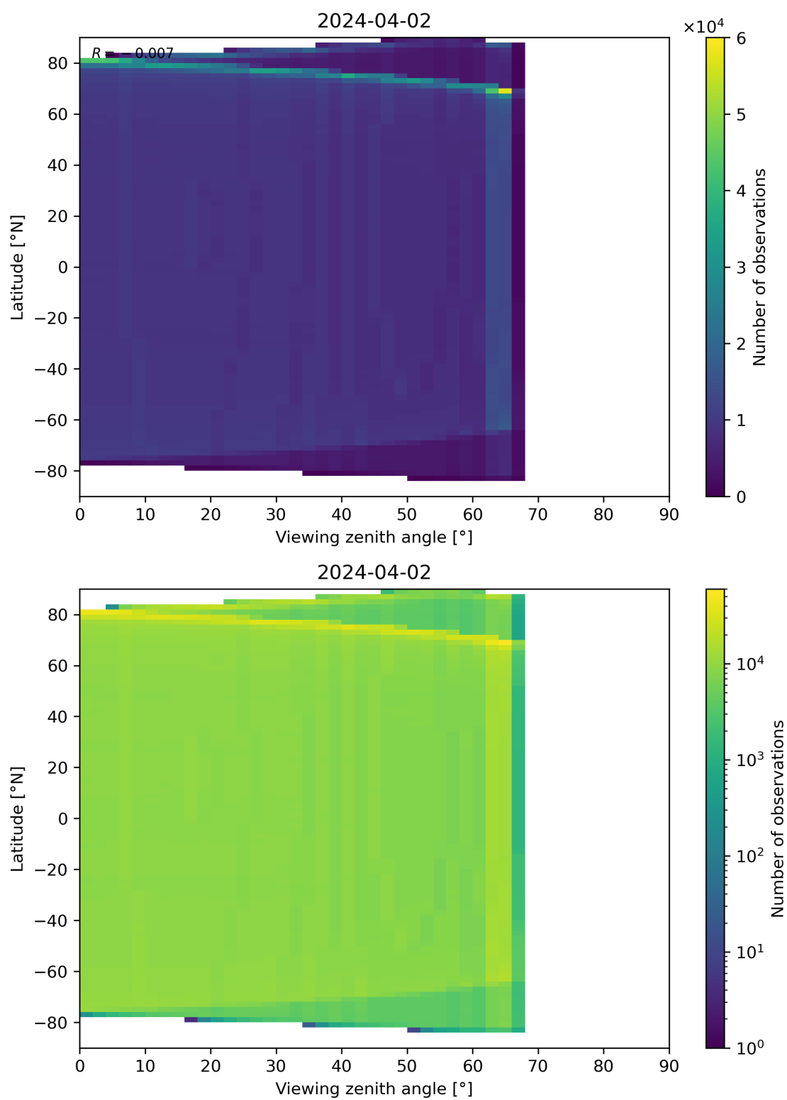
Figure 163: Scatter density plot of “Viewing zenith angle” against “Latitude” for 2024-04-01 to 2024-04-03.
