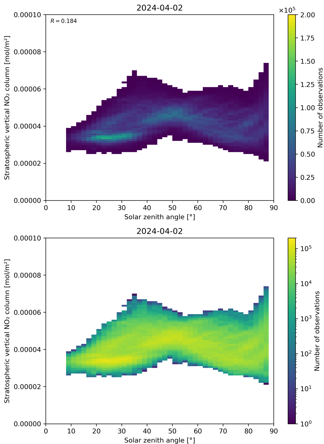
Figure 150: Scatter density plot of “Solar zenith angle” against “Stratospheric vertical NO 2 column” for 2024-04-01 to 2024-04-03.
