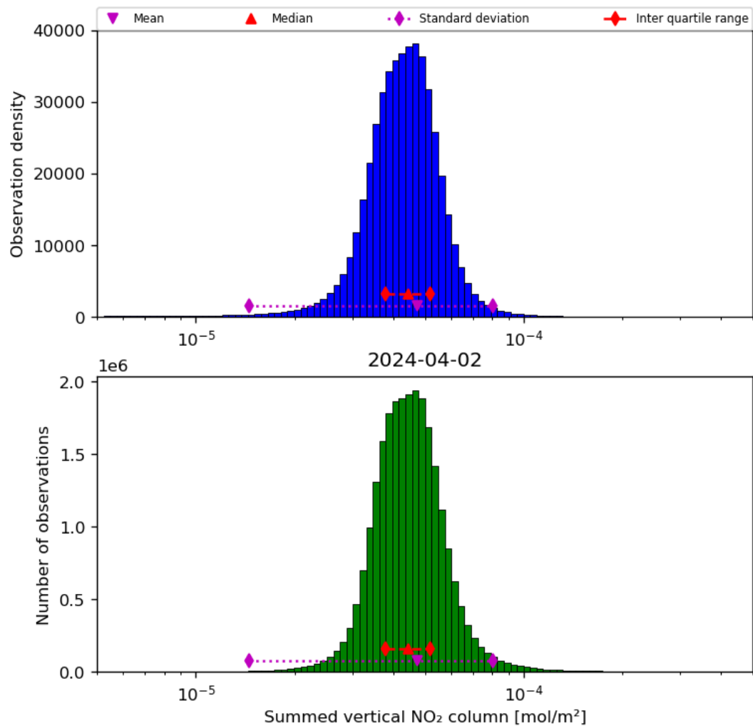
Figure 40: Histogram of “Summed vertical NO 2 column” for 2024-04-01 to 2024-04-03
