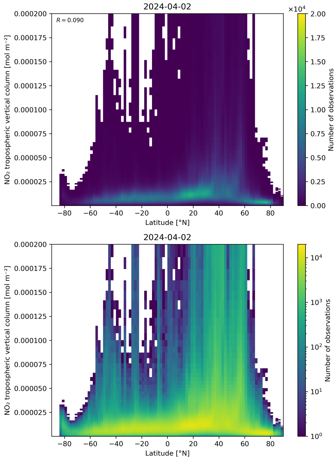
Figure 92: Scatter density plot of “Latitude” against “NO 2 tropospheric vertical column” for 2024-04-01 to 2024-04-03.
