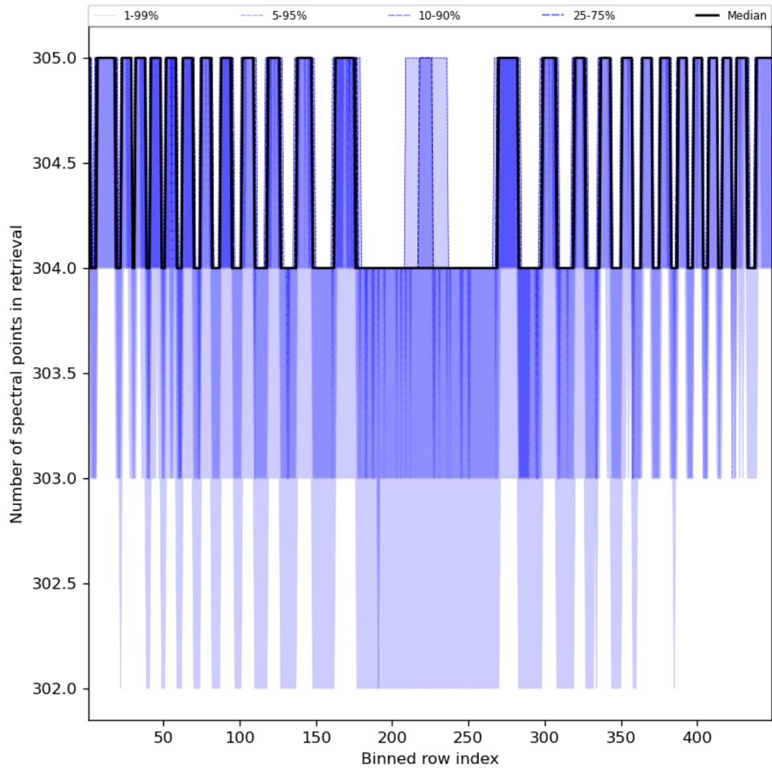
Figure 50: Along track statistics of “Number of spectral points in retrieval” for 2024-04-01 to 2024-04-03
