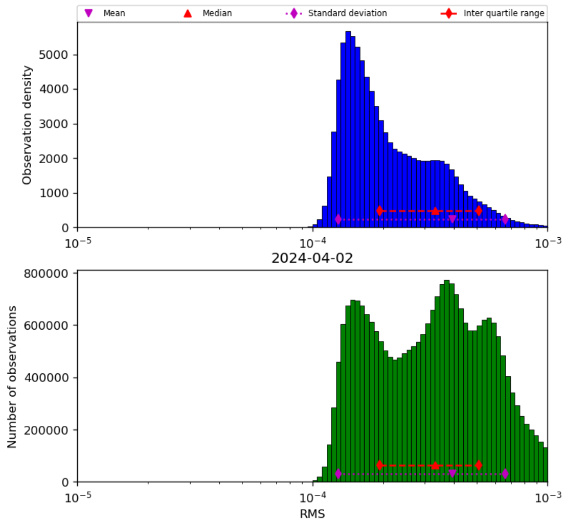
Figure 43: Histogram of “RMS” for 2024-04-01 to 2024-04-03
