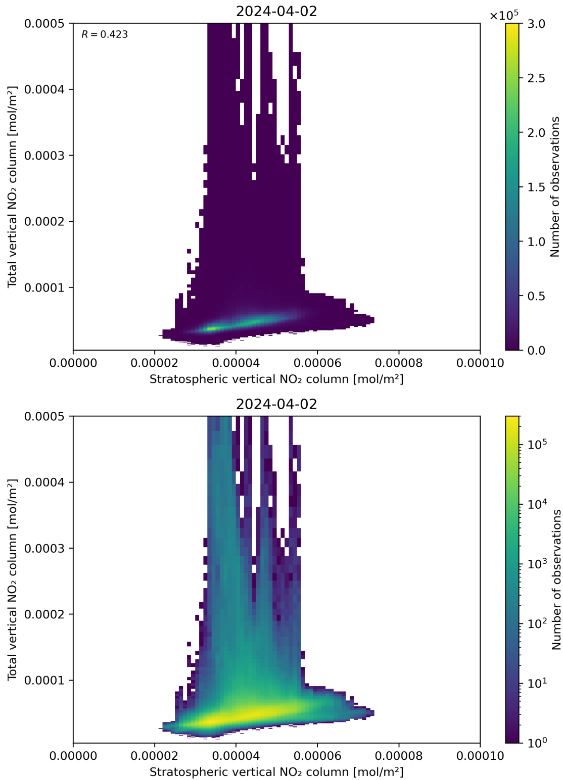
Figure 100: Scatter density plot of “Stratospheric vertical NO 2 column” against “Total vertical NO 2 column” for 2024-04-01 to 2024-04-03.
