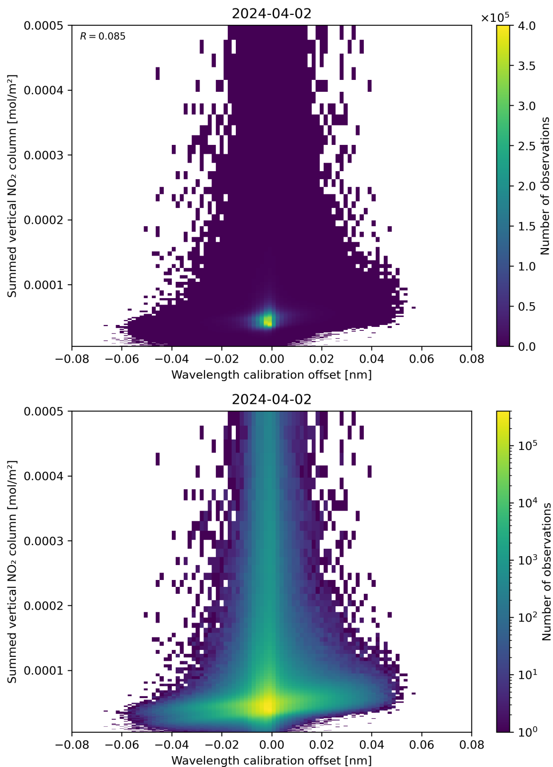
Figure 177: Scatter density plot of “Wavelength calibration offset” against “Summed vertical NO 2 column” for 2024-04-01 to 2024-04-03.
