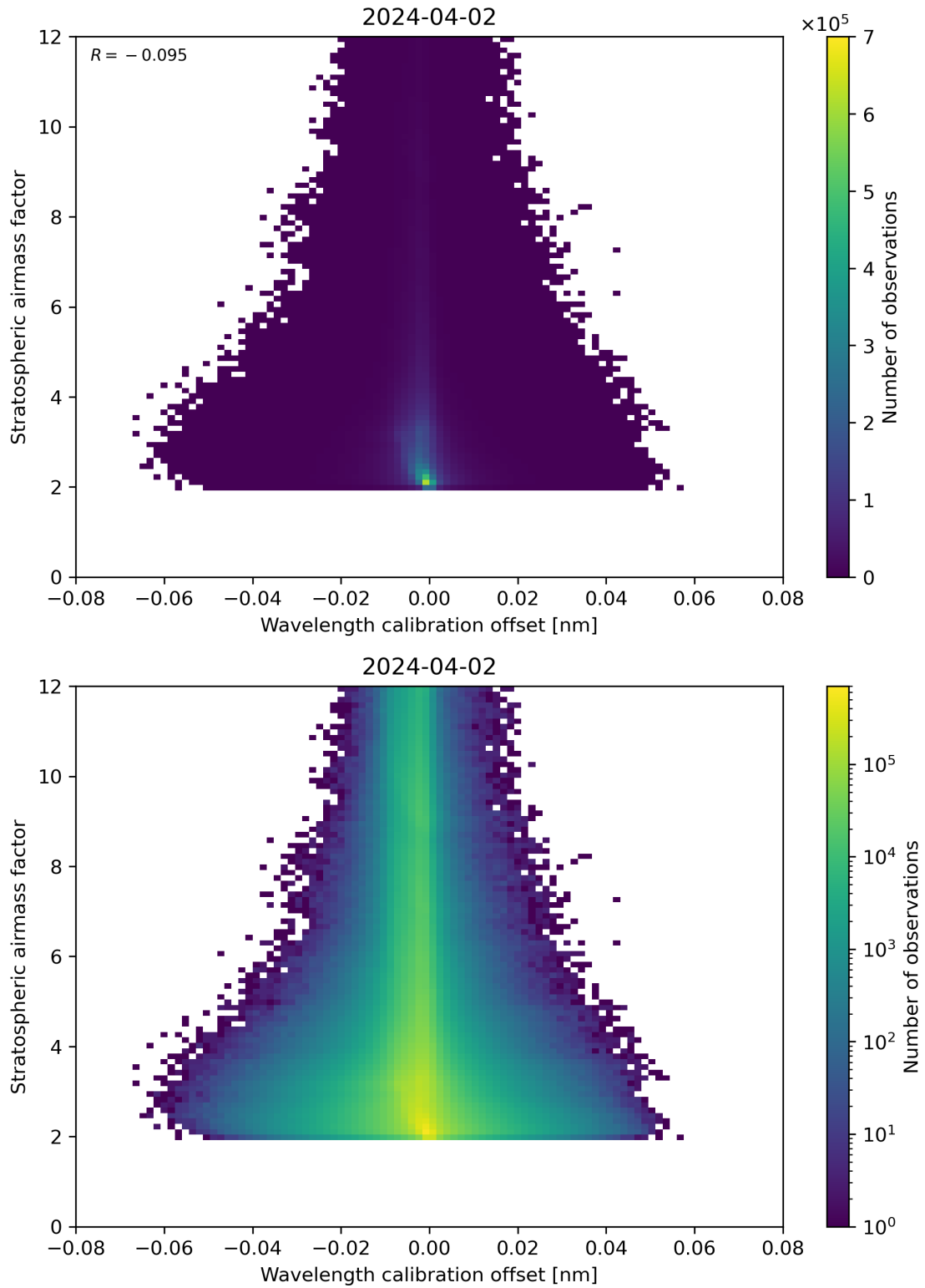
Figure 174: Scatter density plot of “Wavelength calibration offset” against “Stratospheric air mass factor” for 2024-04-01 to 2024-04-03.
