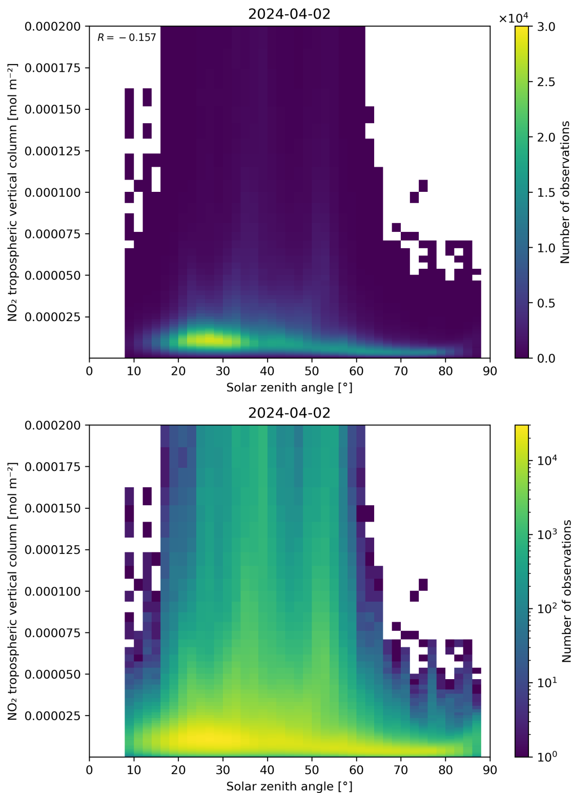
Figure 155: Scatter density plot of “Solar zenith angle” against “NO 2 tropospheric vertical column” for 2024-04-01 to 2024-04-03.
