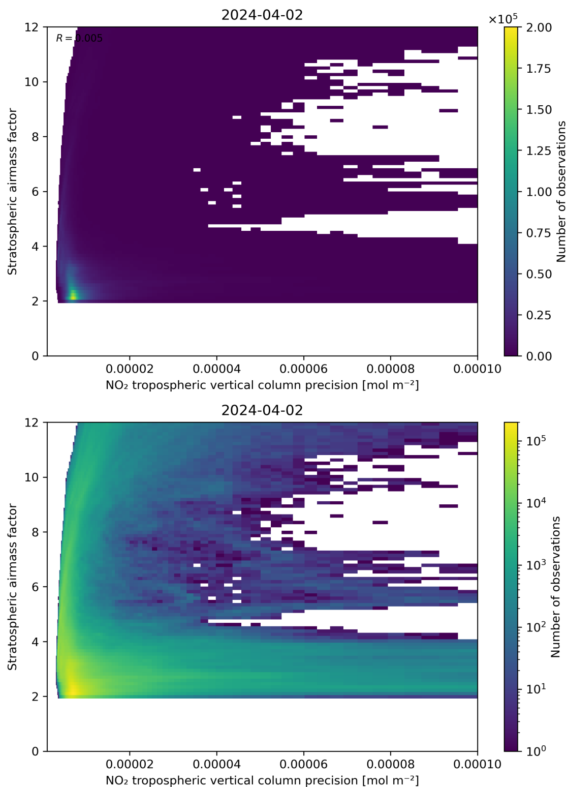
Figure 131: Scatter density plot of “NO 2 tropospheric vertical column precision” against “Stratospheric airmass factor” for 2024-04-01 to 2024-04-03.
