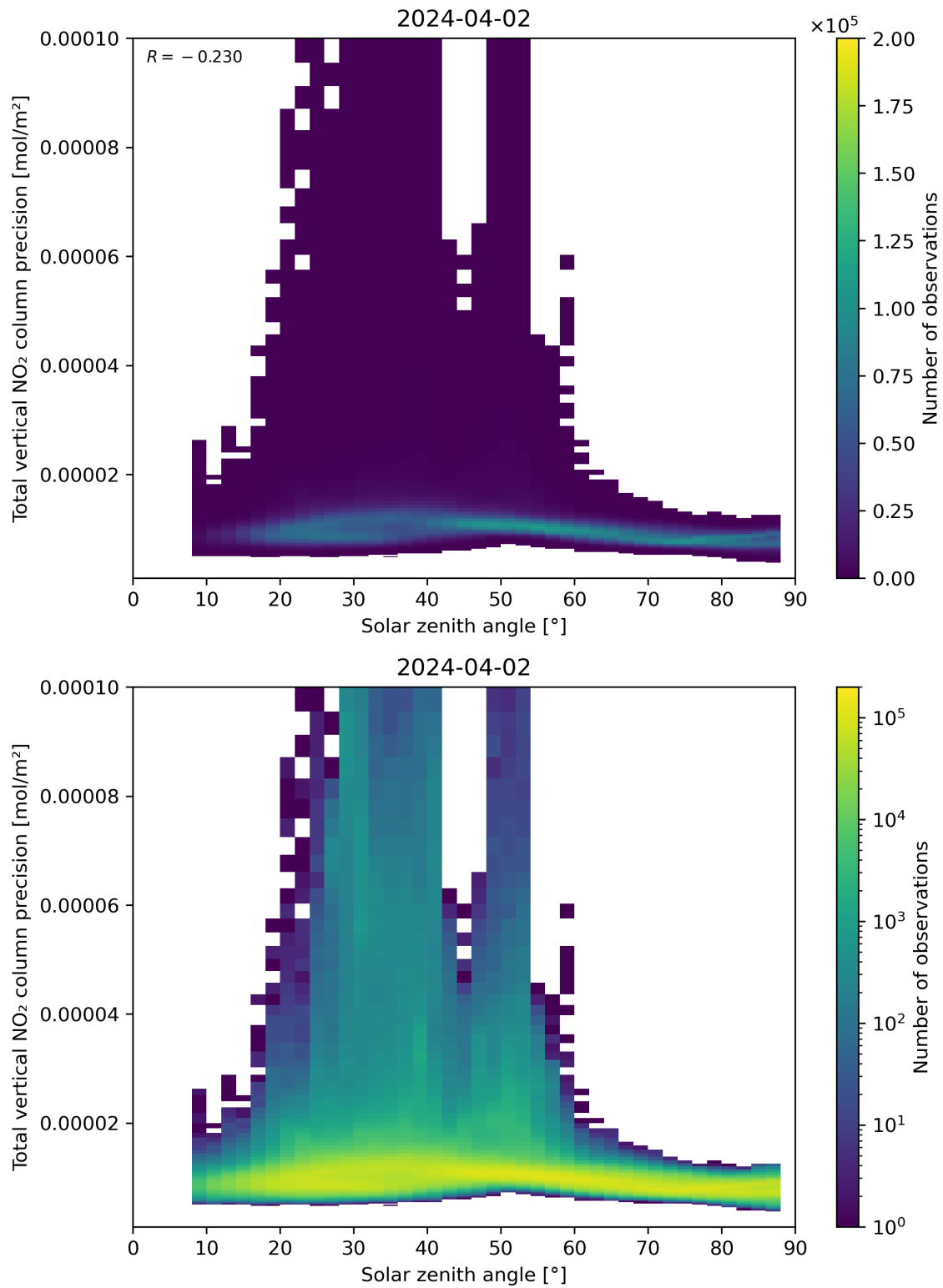
Figure 154: Scatter density plot of “Solar zenith angle” against “Total vertical NO 2 column precision” for 2024-04-01 to 2024-04-03.
