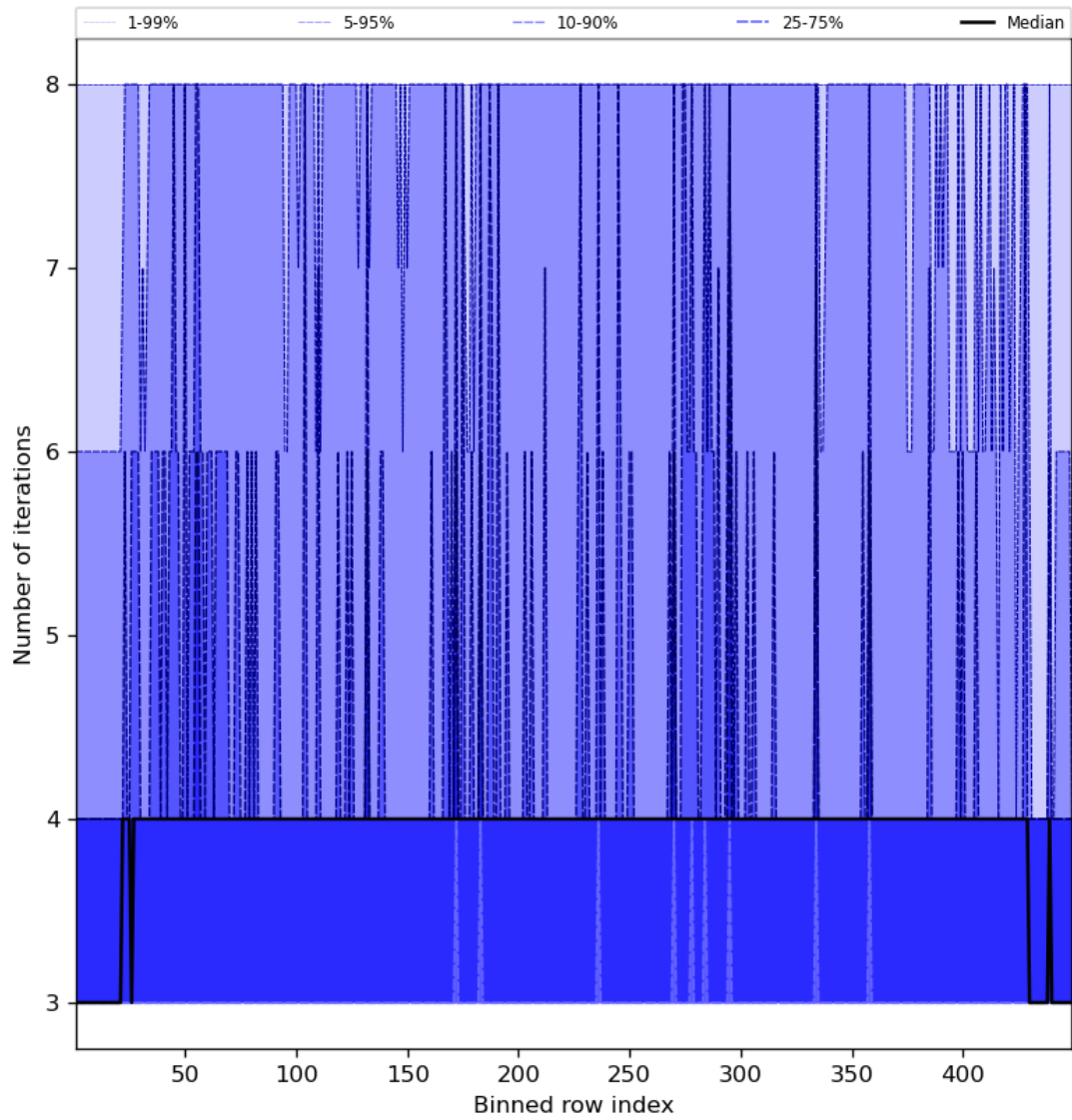
Figure 51: Along track statistics of “Number of iterations” for 2024-04-01 to 2024-04-03
