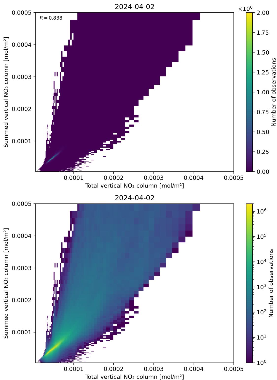
Figure 112: Scatter density plot of “Total vertical NO 2 column” against “Summed vertical NO 2 column” for 2024-04-01 to 2024-04-03.
