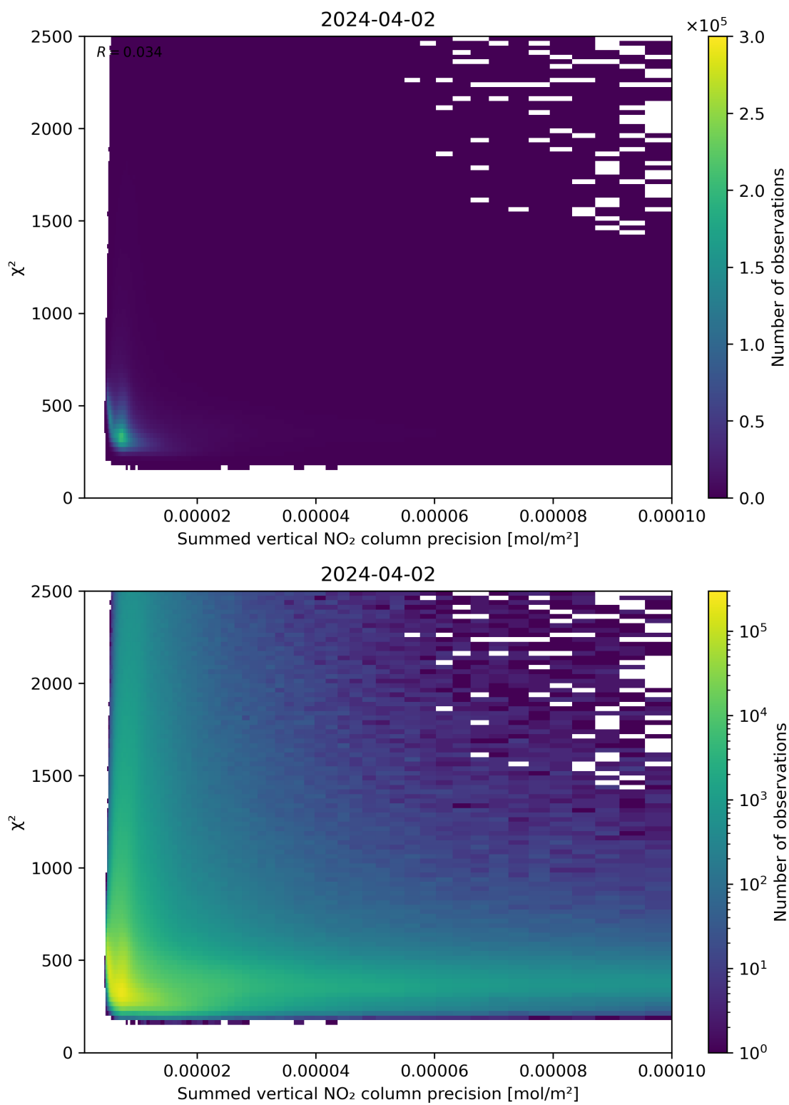
Figure 107: Scatter density plot of “Summed vertical NO 2 column precision” against “ \chi^2 ” for 2024-04-01 to 2024-04-03.
