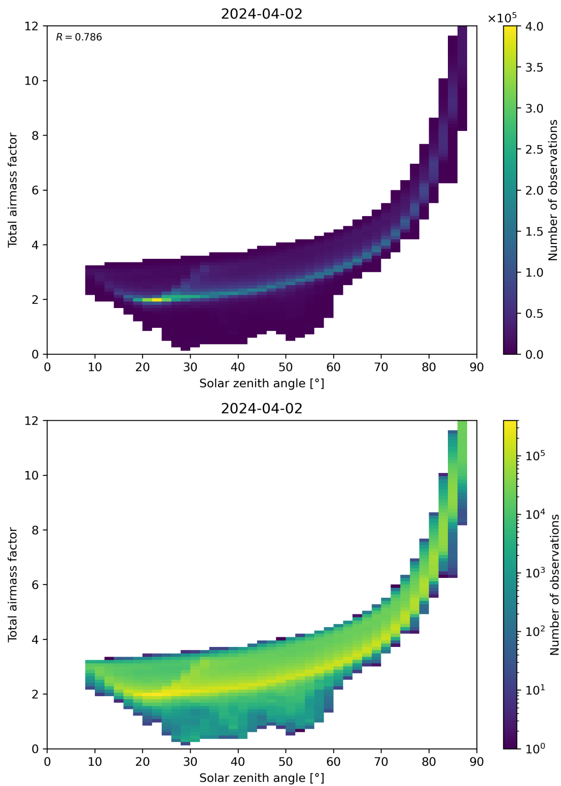
Figure 146: Scatter density plot of “Solar zenith angle” against “Total air mass factor” for 2024-04-01 to 2024-04-03.
