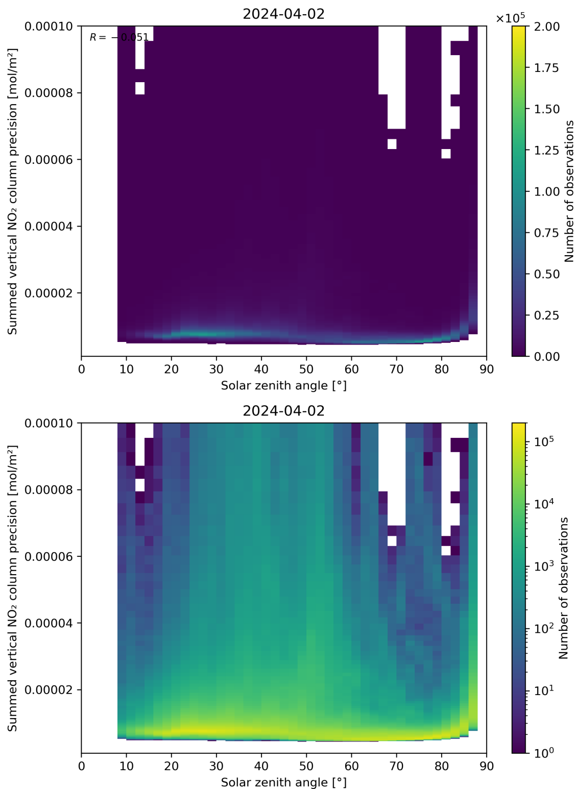
Figure 152: Scatter density plot of “Solar zenith angle” against “Summed vertical NO 2 column precision” for 2024-04-01 to 2024-04-03.
