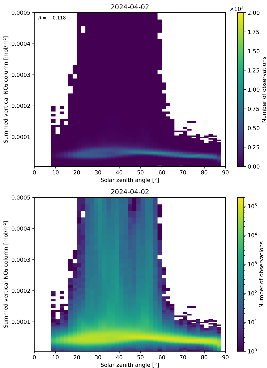
Figure 151: Scatter density plot of “Solar zenith angle” against “Summed vertical NO 2 column” for 2024-04-01 to 2024-04-03.
