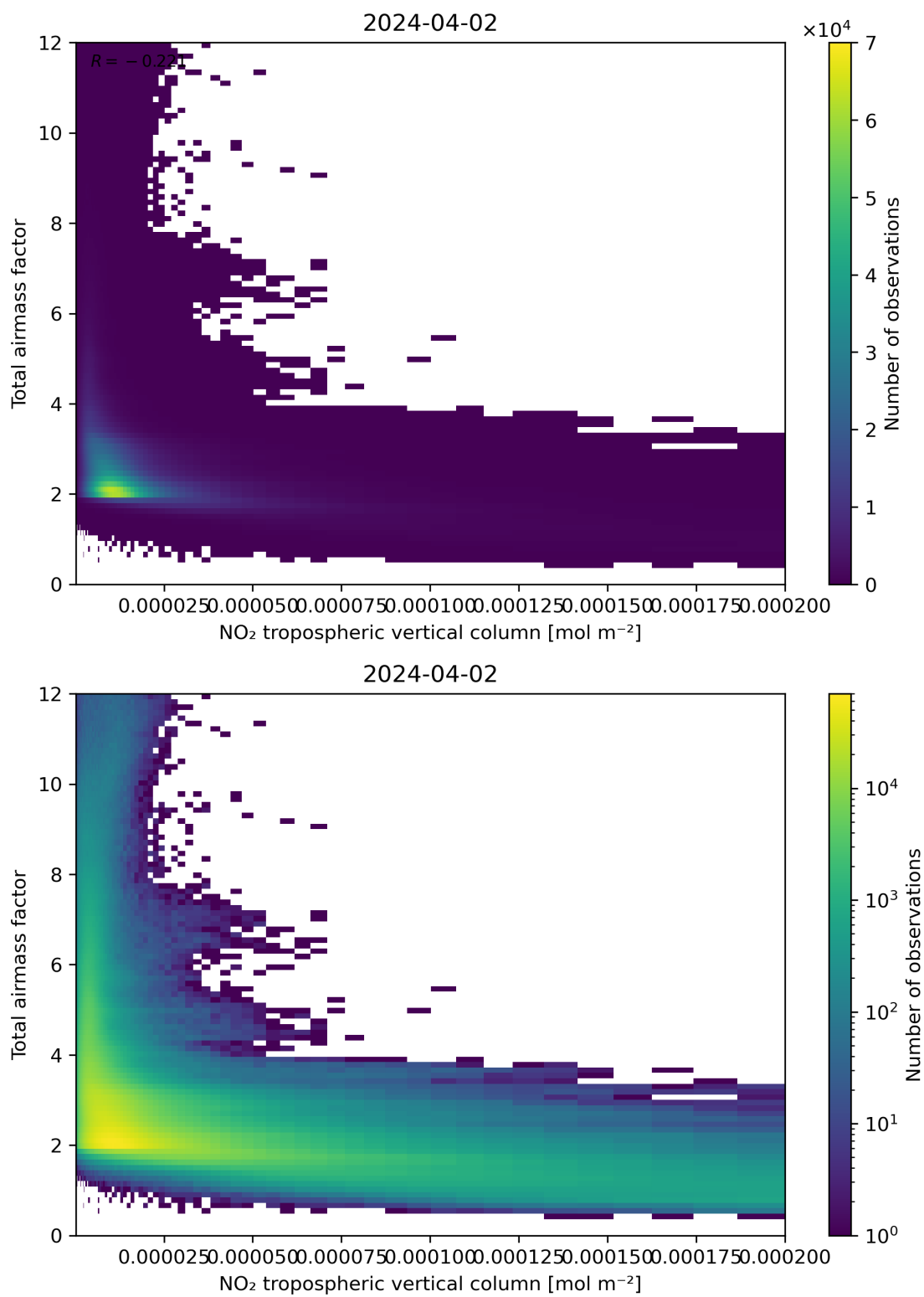
Figure 122: Scatter density plot of “NO 2 tropospheric vertical column” against “Total air mass factor” for 2024-04-01 to 2024-04-03.
