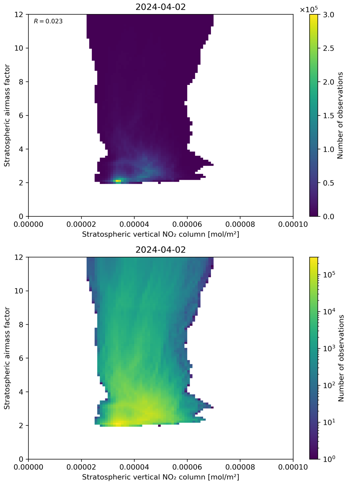
Figure 96: Scatter density plot of “Stratospheric vertical NO 2 column” against “Stratospheric airmass factor” for 2024-04-01 to 2024-04-03.
