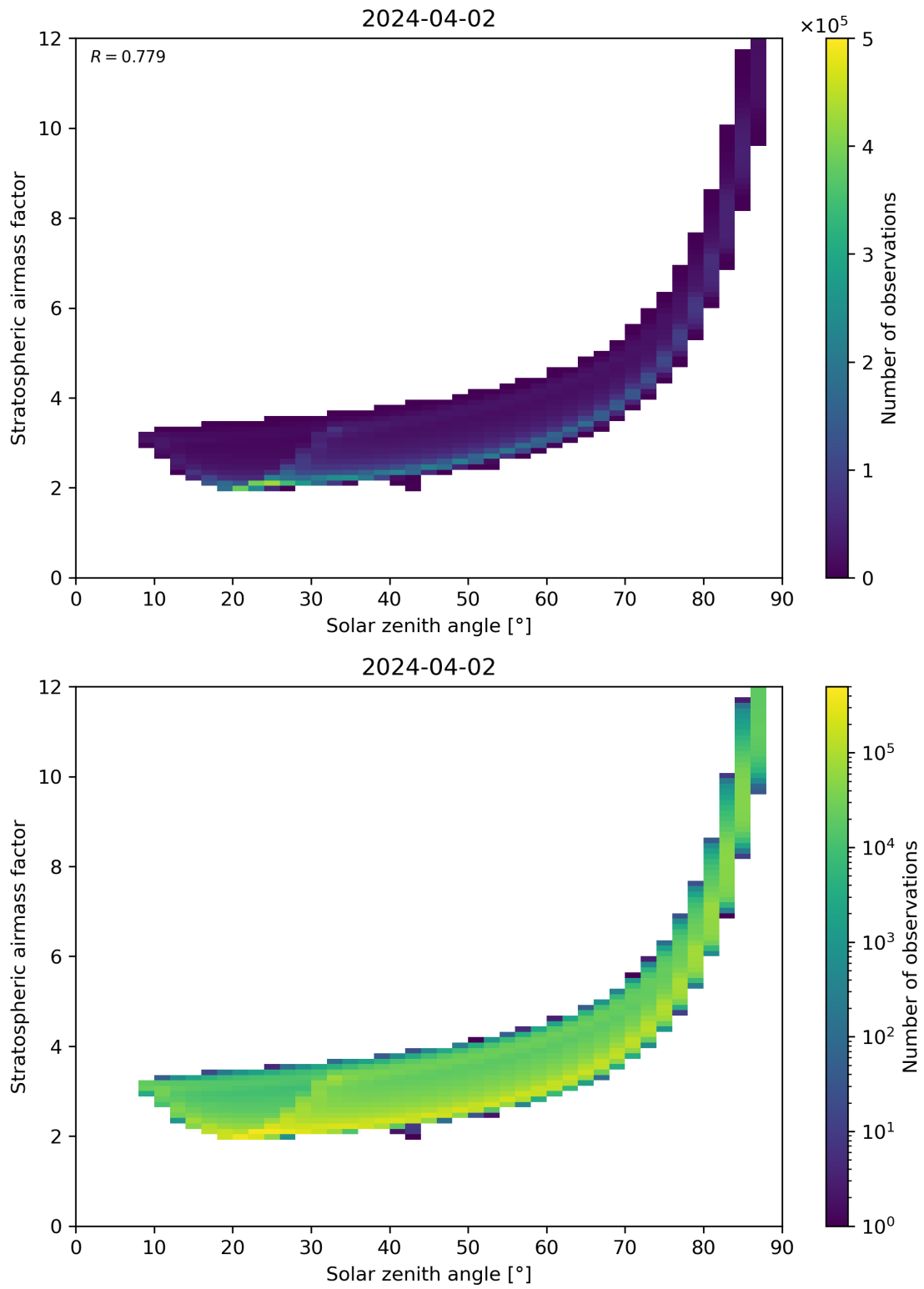
Figure 145: Scatter density plot of “Solar zenith angle” against “Stratospheric airmass factor” for 2024-04-01 to 2024-04-03.
