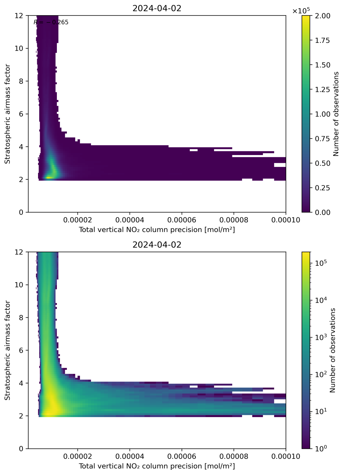
Figure 115: Scatter density plot of “Total vertical NO 2 column precision” against “Stratospheric air mass factor” for 2024-04-01 to 2024-04-03.
