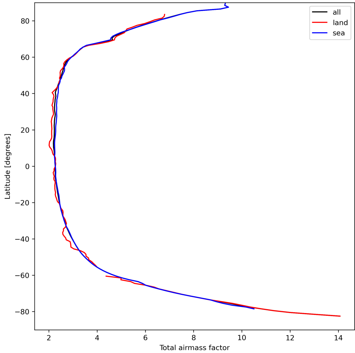
Figure 15: Zonal average of “Total airmass factor” for 2024-04-01 to 2024-04-03.
