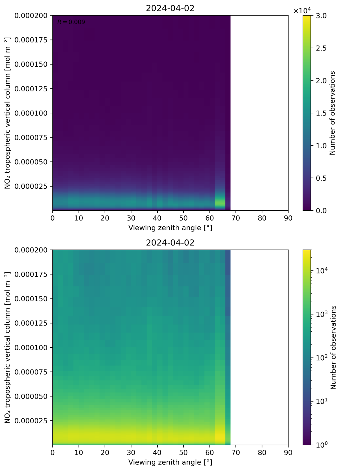
Figure 169: Scatter density plot of “Viewing zenith angle” against “NO 2 tropospheric vertical column” for 2024-04-01 to 2024-04-03.
