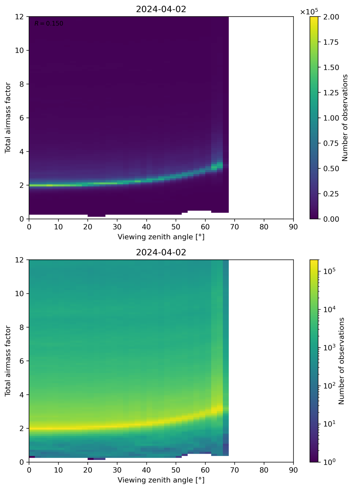
Figure 160: Scatter density plot of “Viewing zenith angle” against “Total airmass factor” for 2024-04-01 to 2024-04-03.
