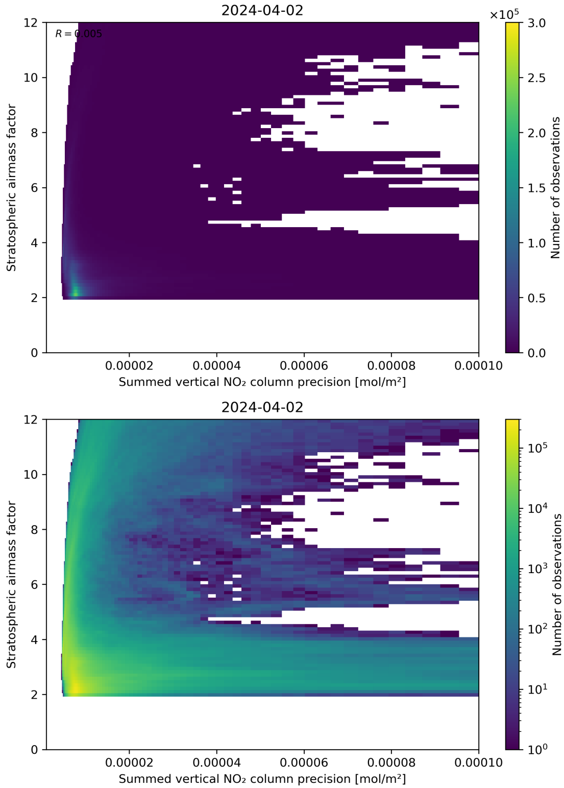
Figure 106: Scatter density plot of “Summed vertical NO 2 column precision” against “Stratospheric airmass factor” for 2024-04-01 to 2024-04-03.
