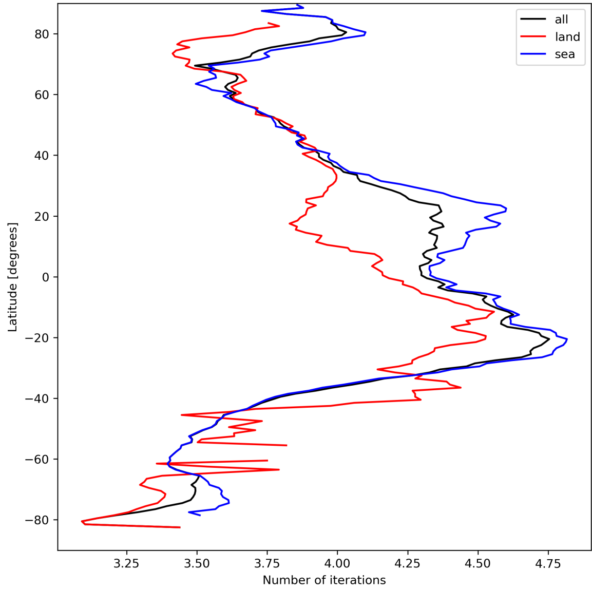
Figure 17: Zonal average of “Number of iterations” for 2024-04-01 to 2024-04-03.
