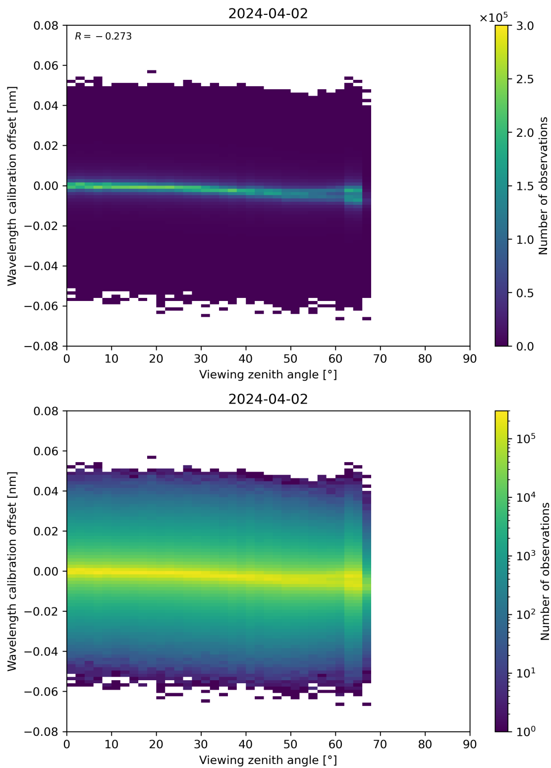
Figure 173: Scatter density plot of “Viewing zenith angle” against “Wavelength calibration offset” for 2024-04-01 to 2024-04-03.
