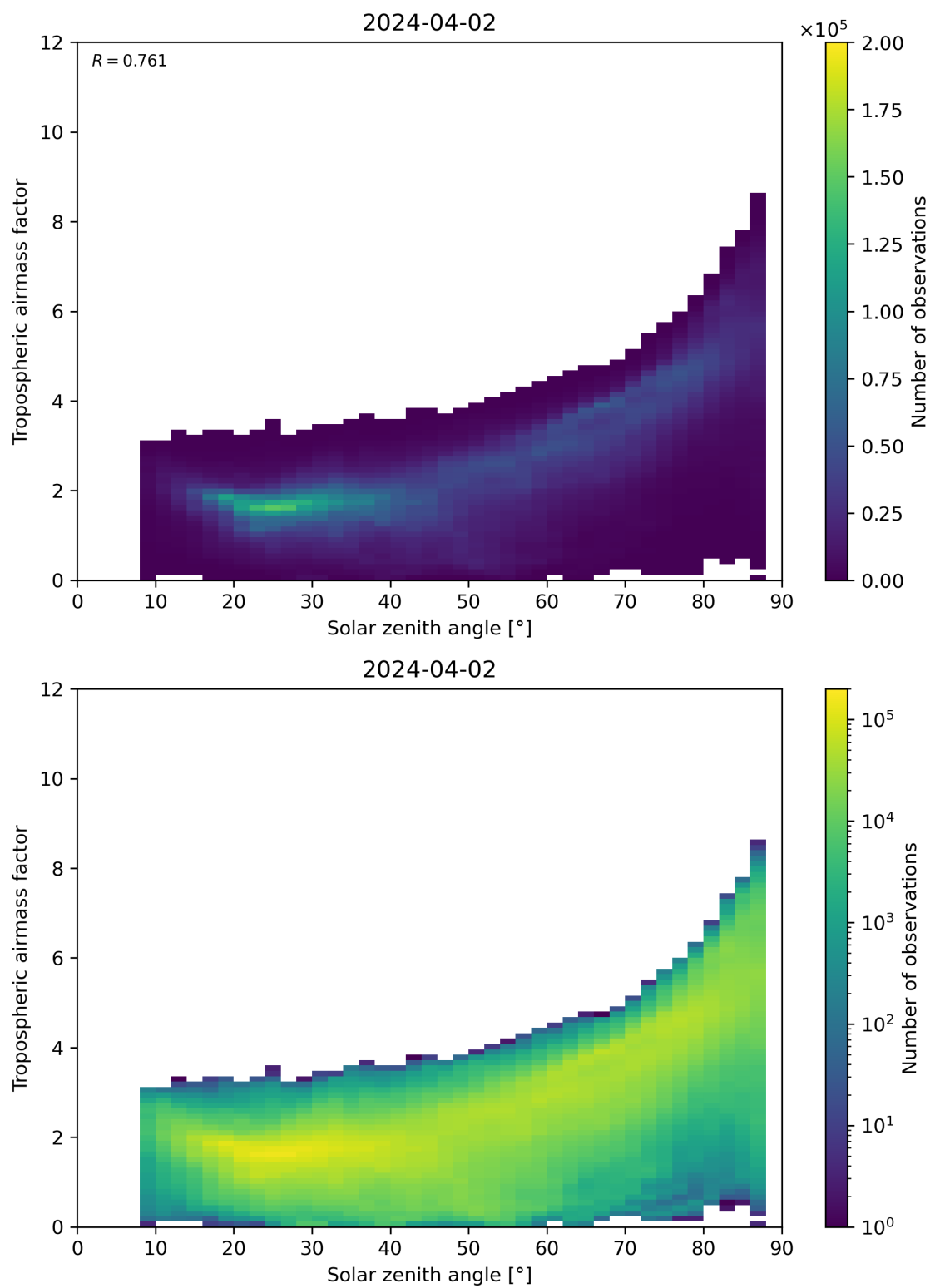
Figure 147: Scatter density plot of “Solar zenith angle” against “Tropospheric airmass factor” for 2024-04-01 to 2024-04-03.
