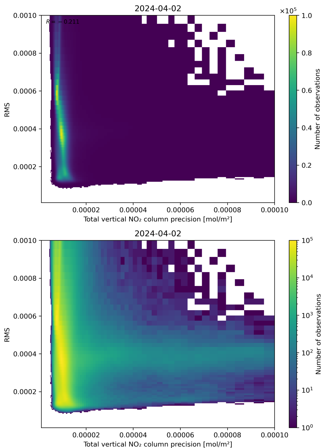
Figure 119: Scatter density plot of “Total vertical NO 2 column precision” against “RMS” for 2024-04-01 to 2024-04-03.
