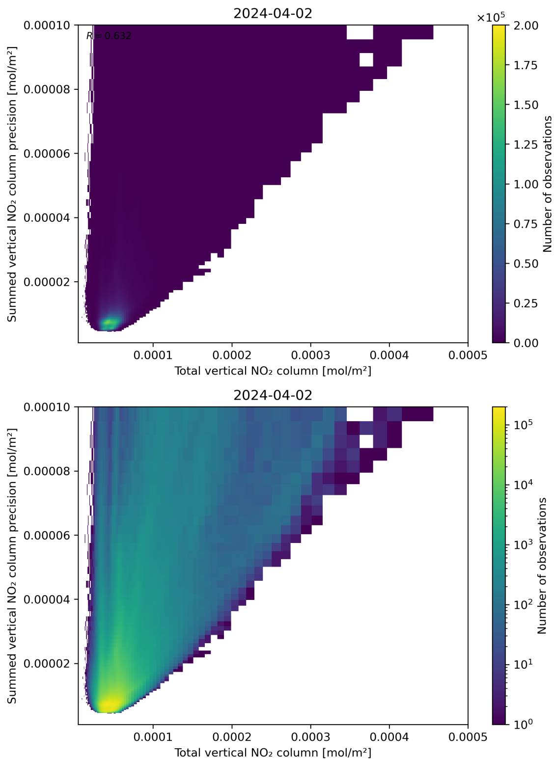
Figure 113: Scatter density plot of “Total vertical NO 2 column” against “Summed vertical NO 2 column precision” for 2024-04-01 to 2024-04-03.
