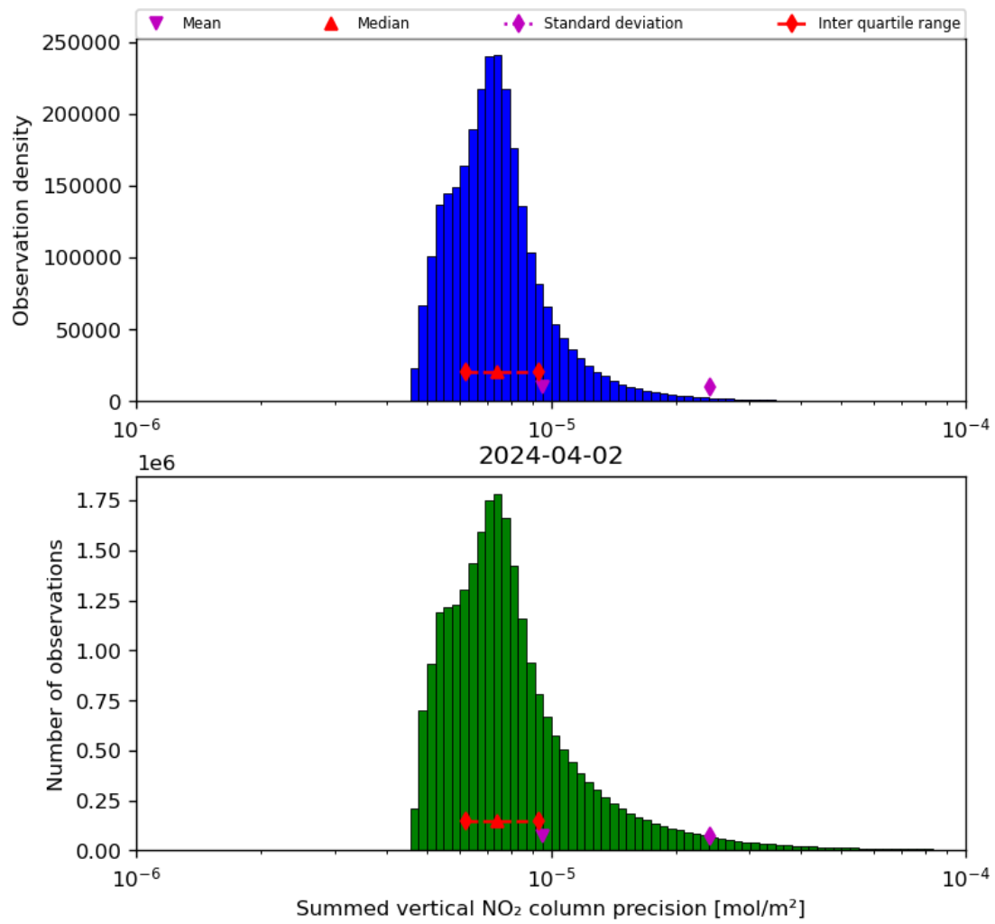
Figure 41: Histogram of "Summed vertical NO 2 column precision" for 2024-04-01 to 2024-04-03
