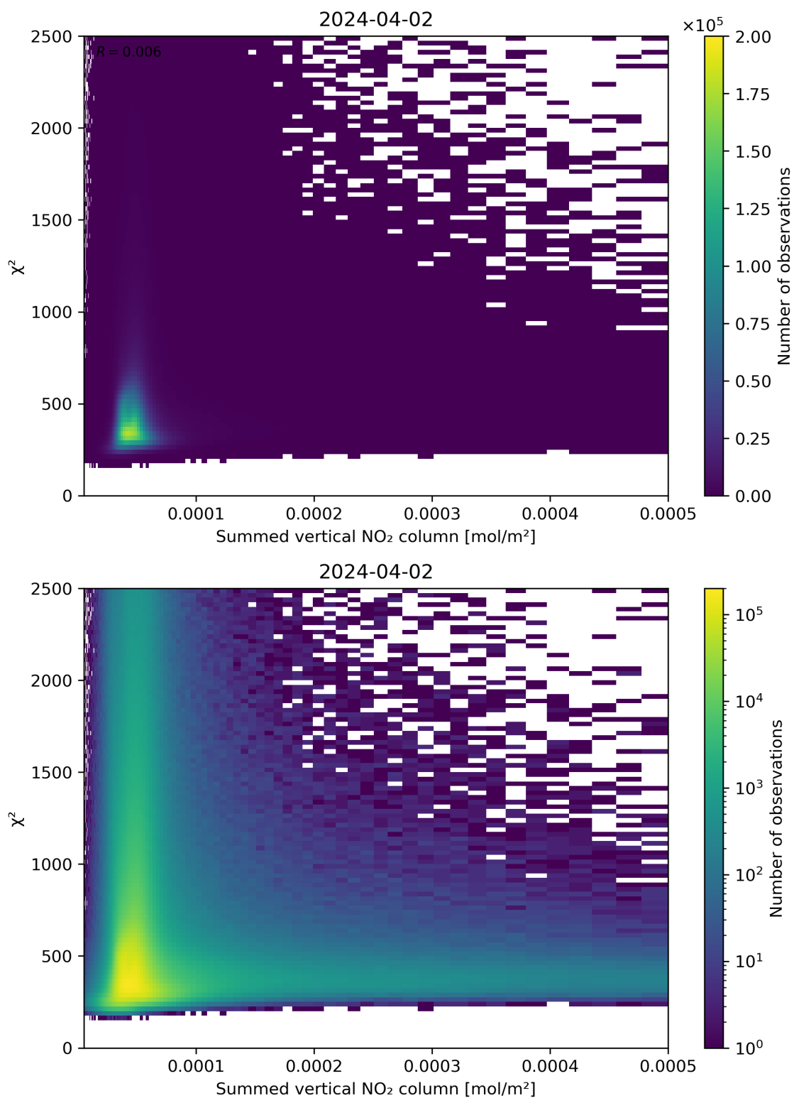
Figure 104: Scatter density plot of “Summed vertical NO 2 column” against “ \chi^2 ” for 2024-04-01 to 2024-04-03.
