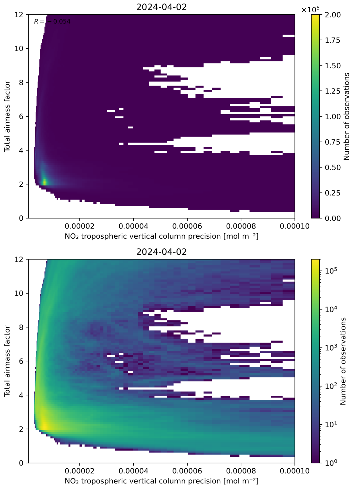
Figure 132: Scatter density plot of “NO 2 tropospheric vertical column precision” against “Total air mass factor” for 2024-04-01 to 2024-04-03.
