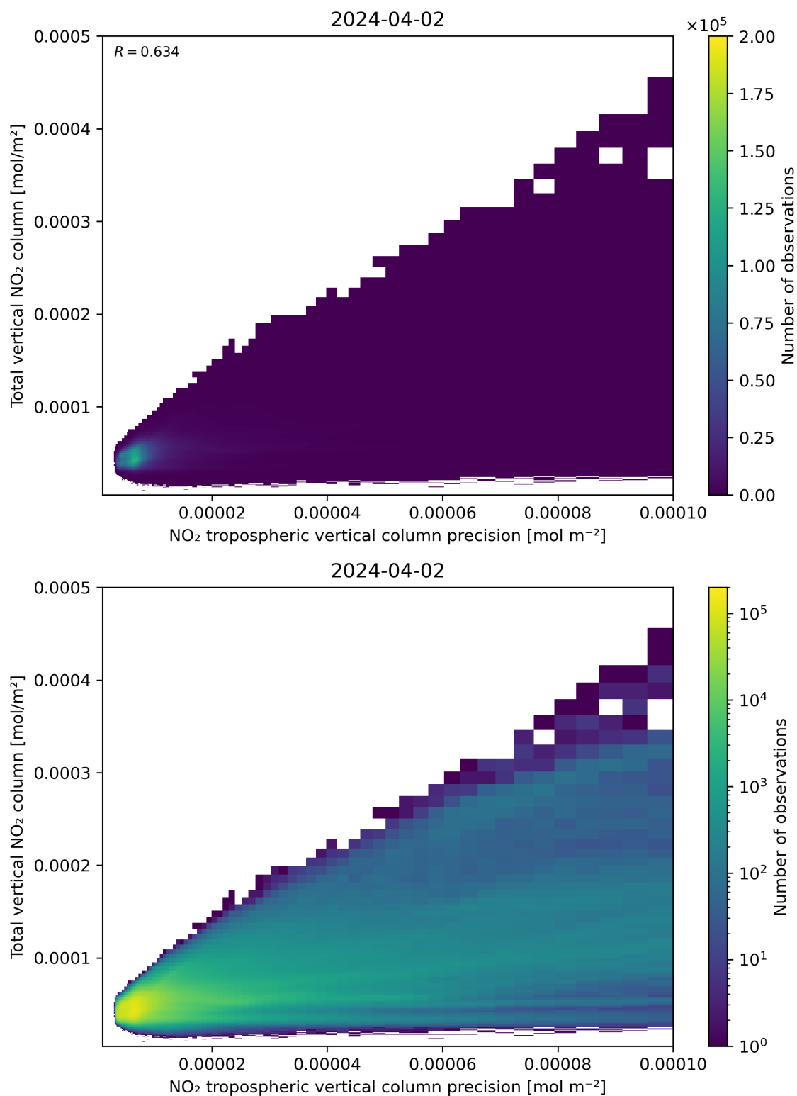
Figure 138: Scatter density plot of “NO 2 tropospheric vertical column precision” against “Total vertical NO 2 column” for 2024-04-01 to 2024-04-03.
