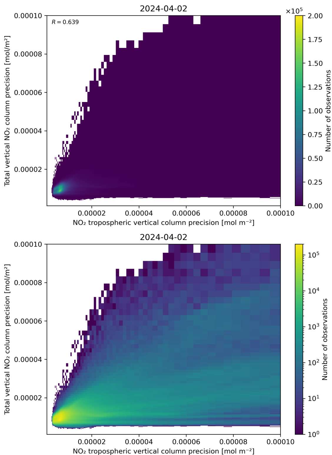
Figure 139: Scatter density plot of “NO 2 tropospheric vertical column precision” against “Total vertical NO 2 column precision” for 2024-04-01 to 2024-04-03.
