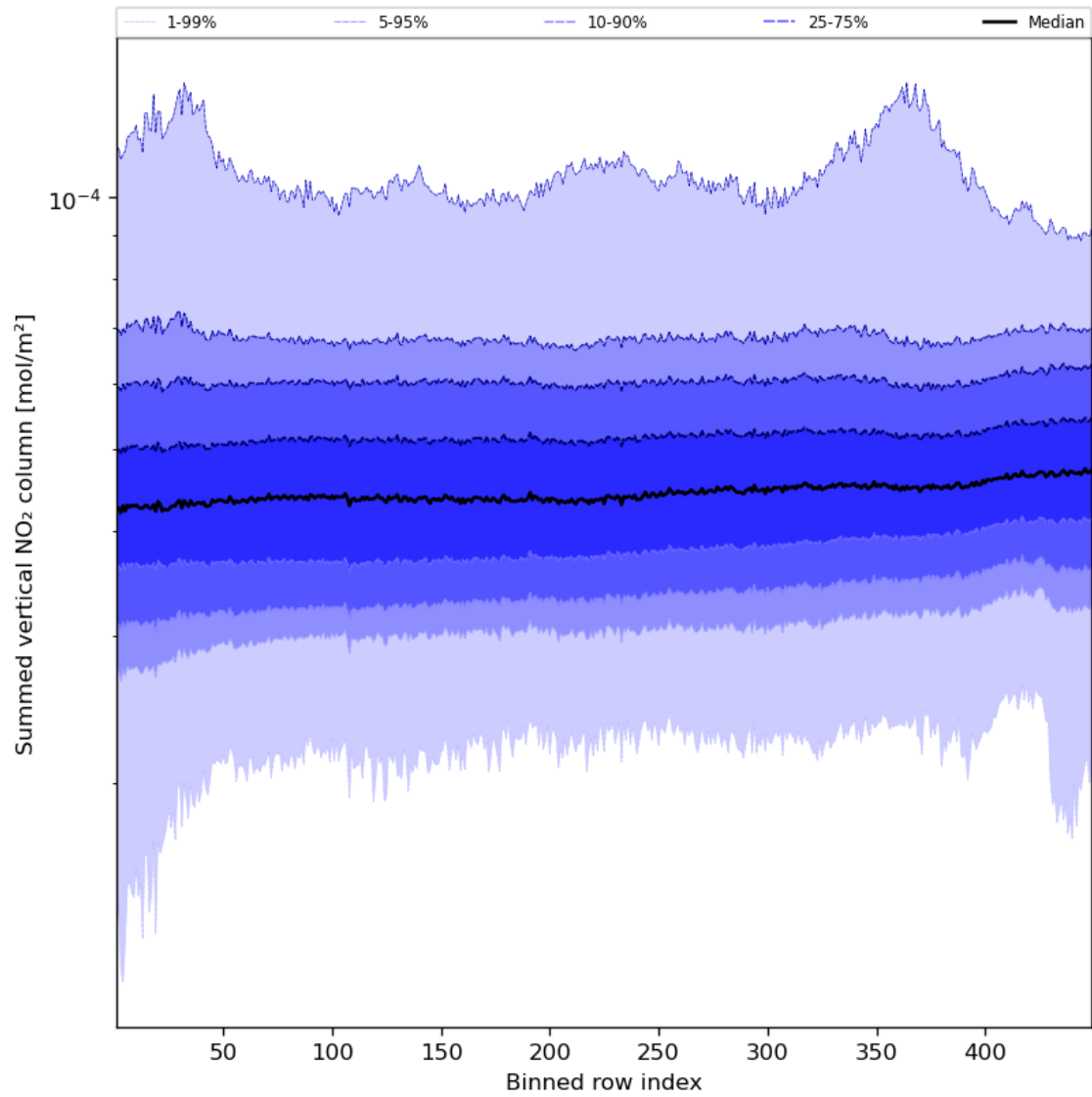
Figure 57: Along track statistics of “Summed vertical NO 2 column” for 2024-04-01 to 2024-04-03
