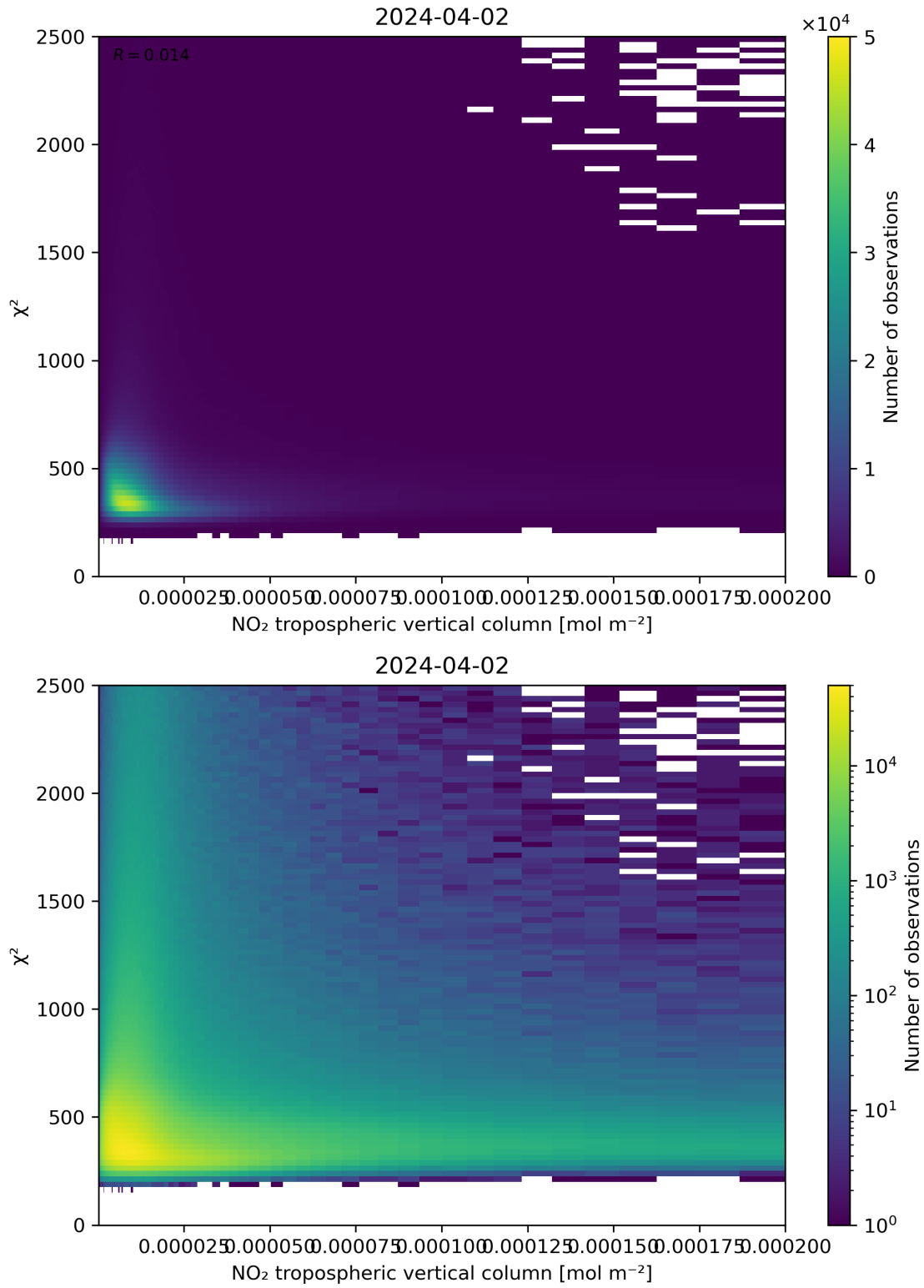
Figure 124: Scatter density plot of “NO 2 tropospheric vertical column” against “ \chi^2 ” for 2024-04-01 to 2024-04-03.
