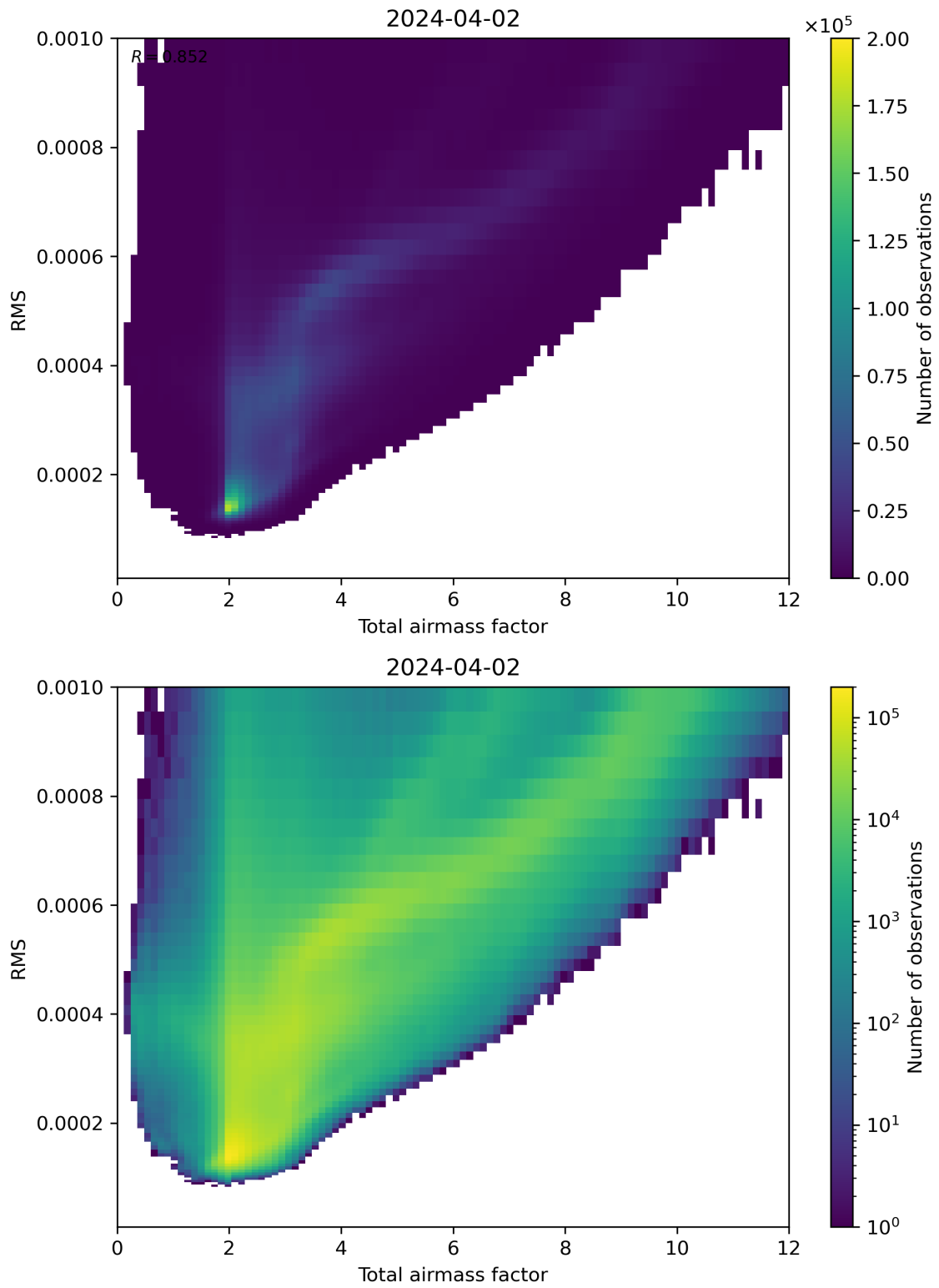
Figure 69: Scatter density plot of “Total airmass factor” against “RMS” for 2024-04-01 to 2024-04-03.
