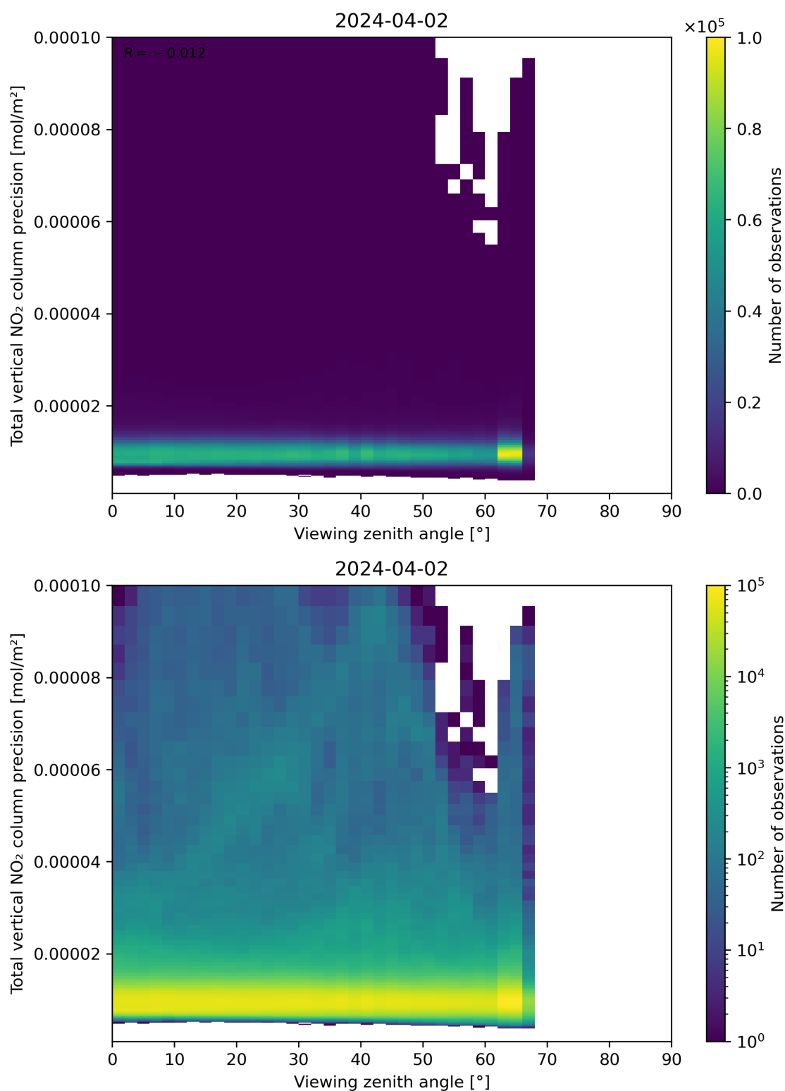
Figure 168: Scatter density plot of “Viewing zenith angle” against “Total vertical NO 2 column precision” for 2024-04-01 to 2024-04-03.
