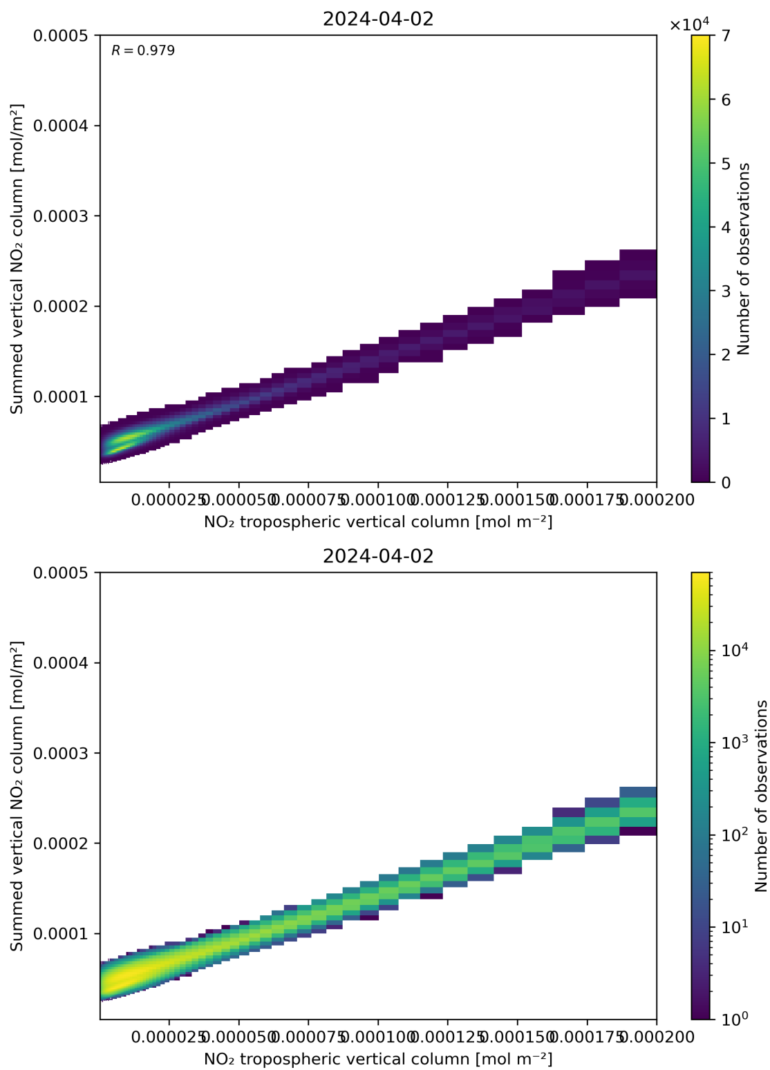
Figure 126: Scatter density plot of “NO 2 tropospheric vertical column” against “Summed vertical NO 2 column” for 2024-04-01 to 2024-04-03.
