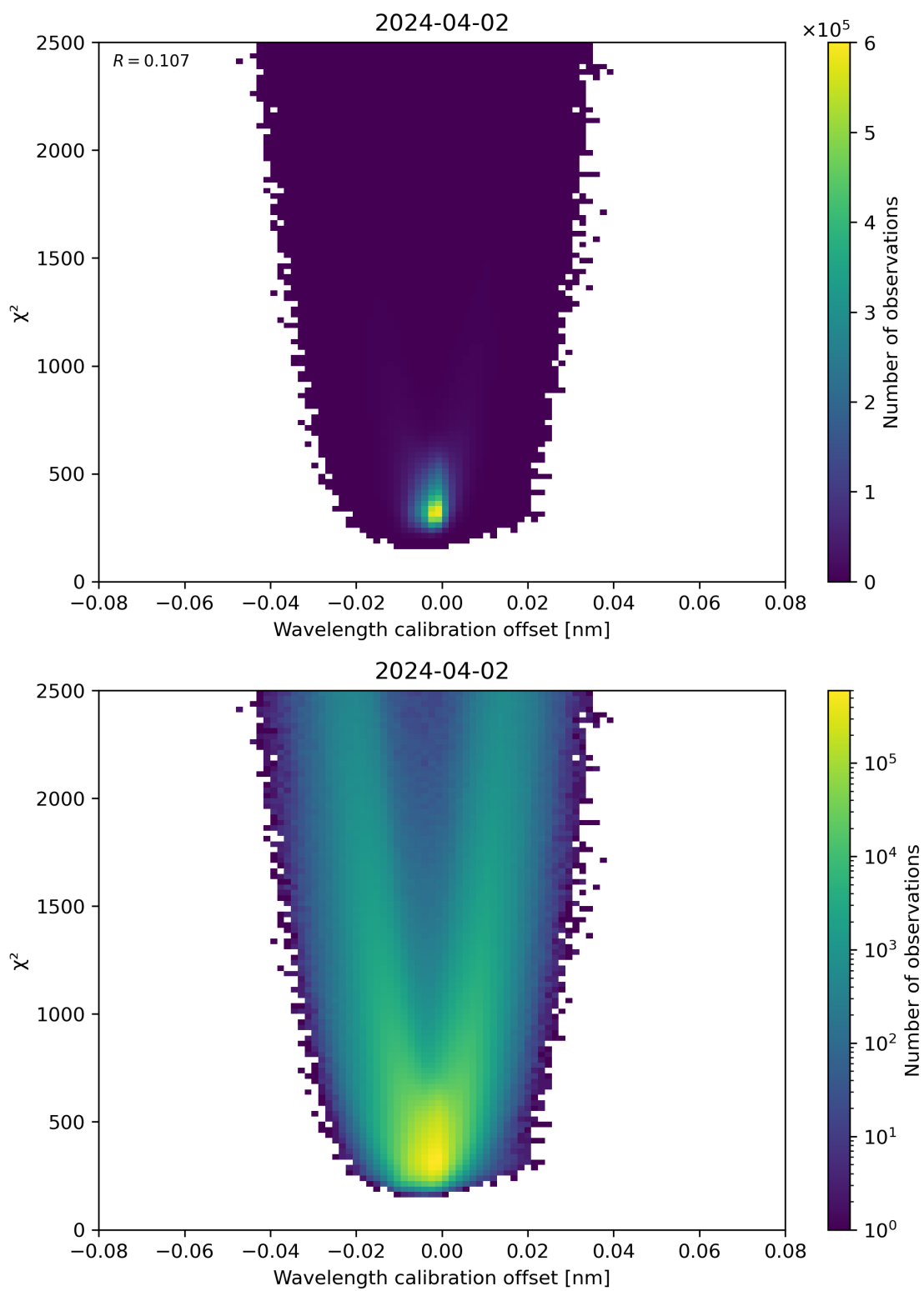
Figure 175: Scatter density plot of “Wavelength calibration offset” against “ \chi^2 ” for 2024-04-01 to 2024-04-03.
