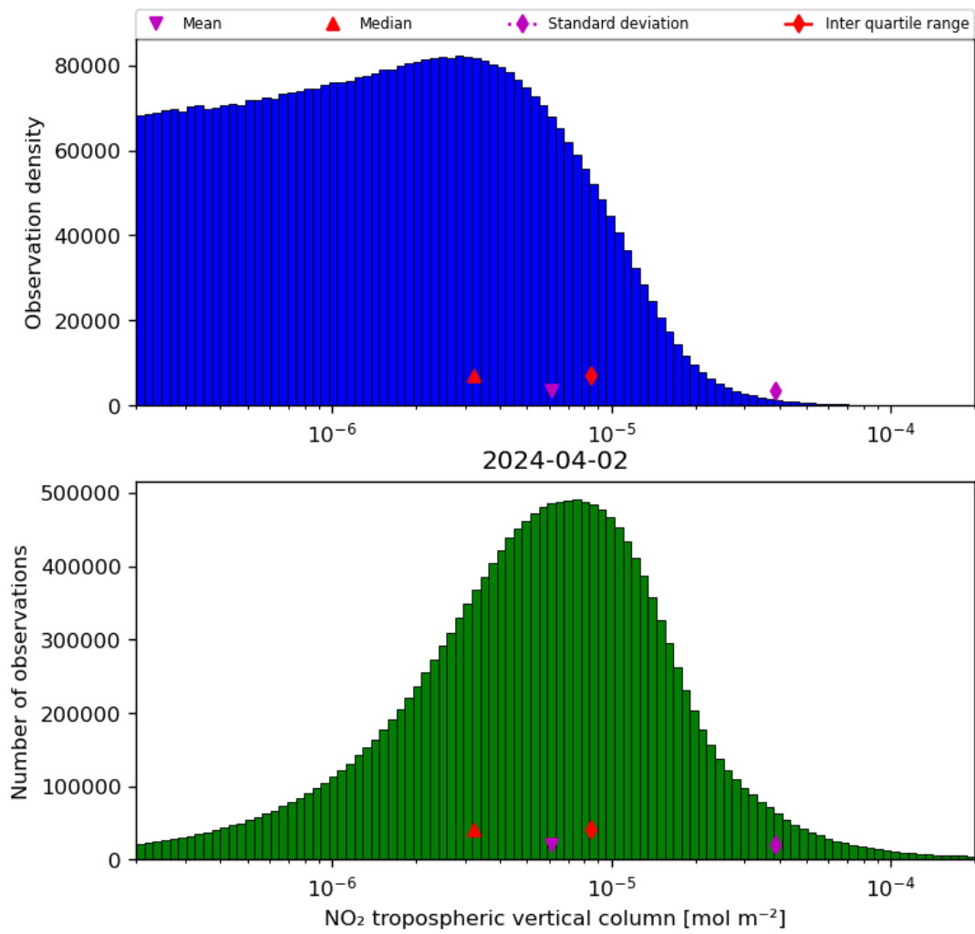
Figure 29: Histogram of “NO 2 tropospheric vertical column” for 2024-04-01 to 2024-04-03
