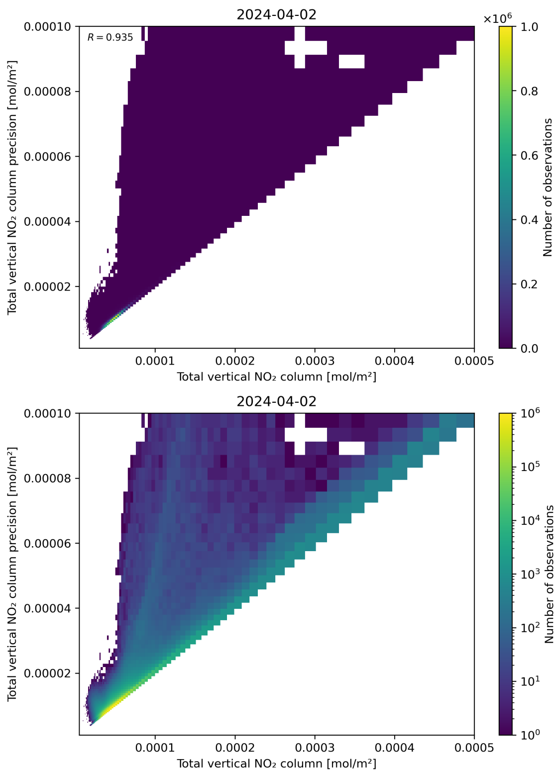
Figure 114: Scatter density plot of “Total vertical NO 2 column” against “Total vertical NO 2 column precision” for 2024-04-01 to 2024-04-03.
