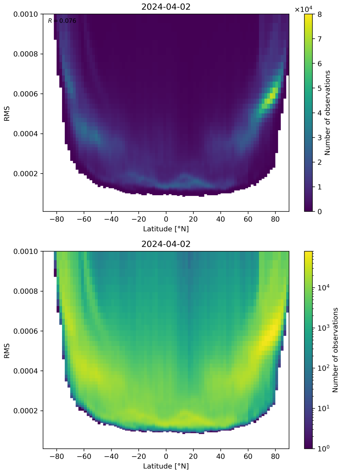
Figure 94: Scatter density plot of “Latitude” against “RMS” for 2024-04-01 to 2024-04-03.
