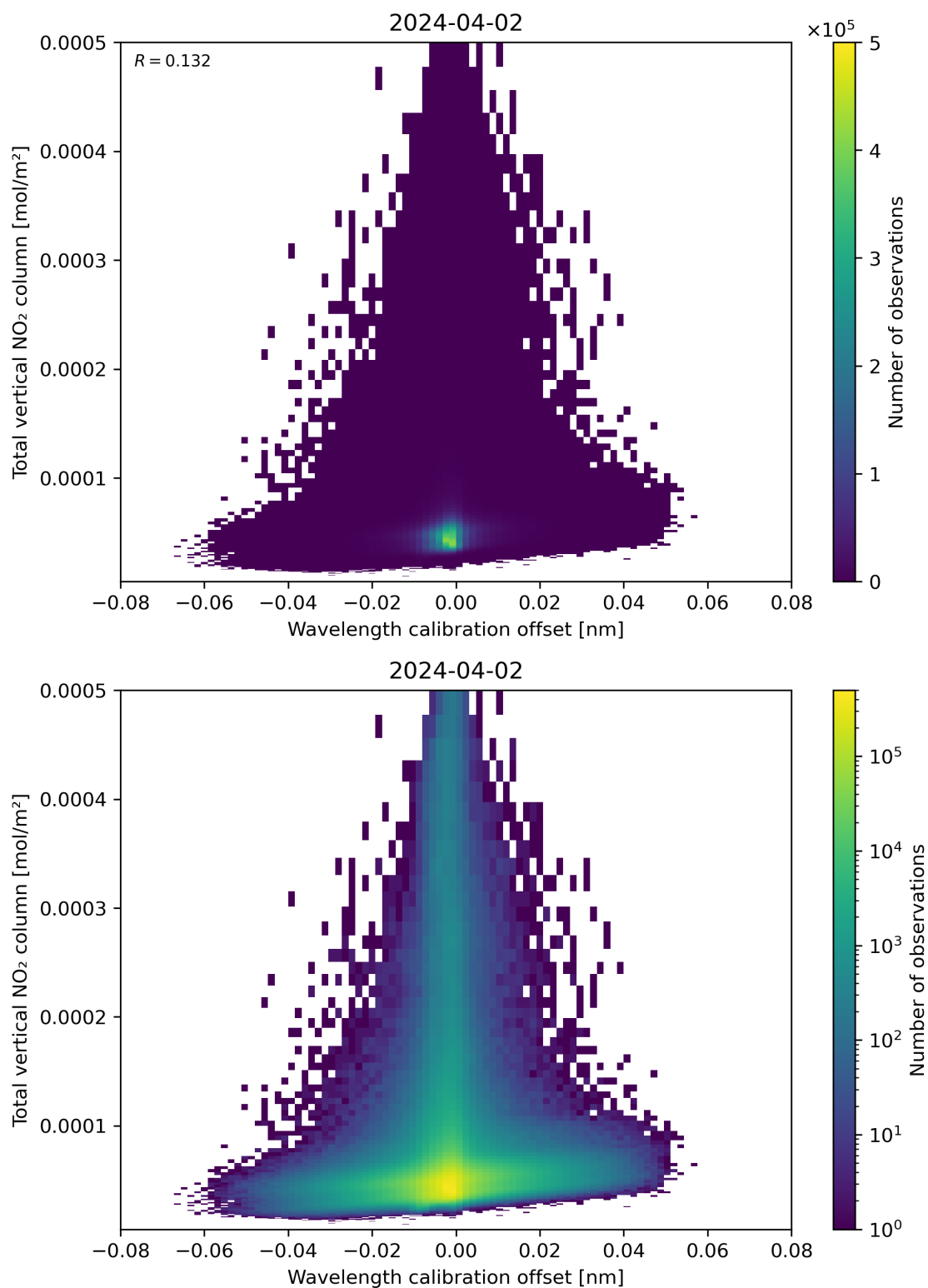
Figure 179: Scatter density plot of “Wavelength calibration offset” against “Total vertical NO 2 column” for 2024-04-01 to 2024-04-03.
