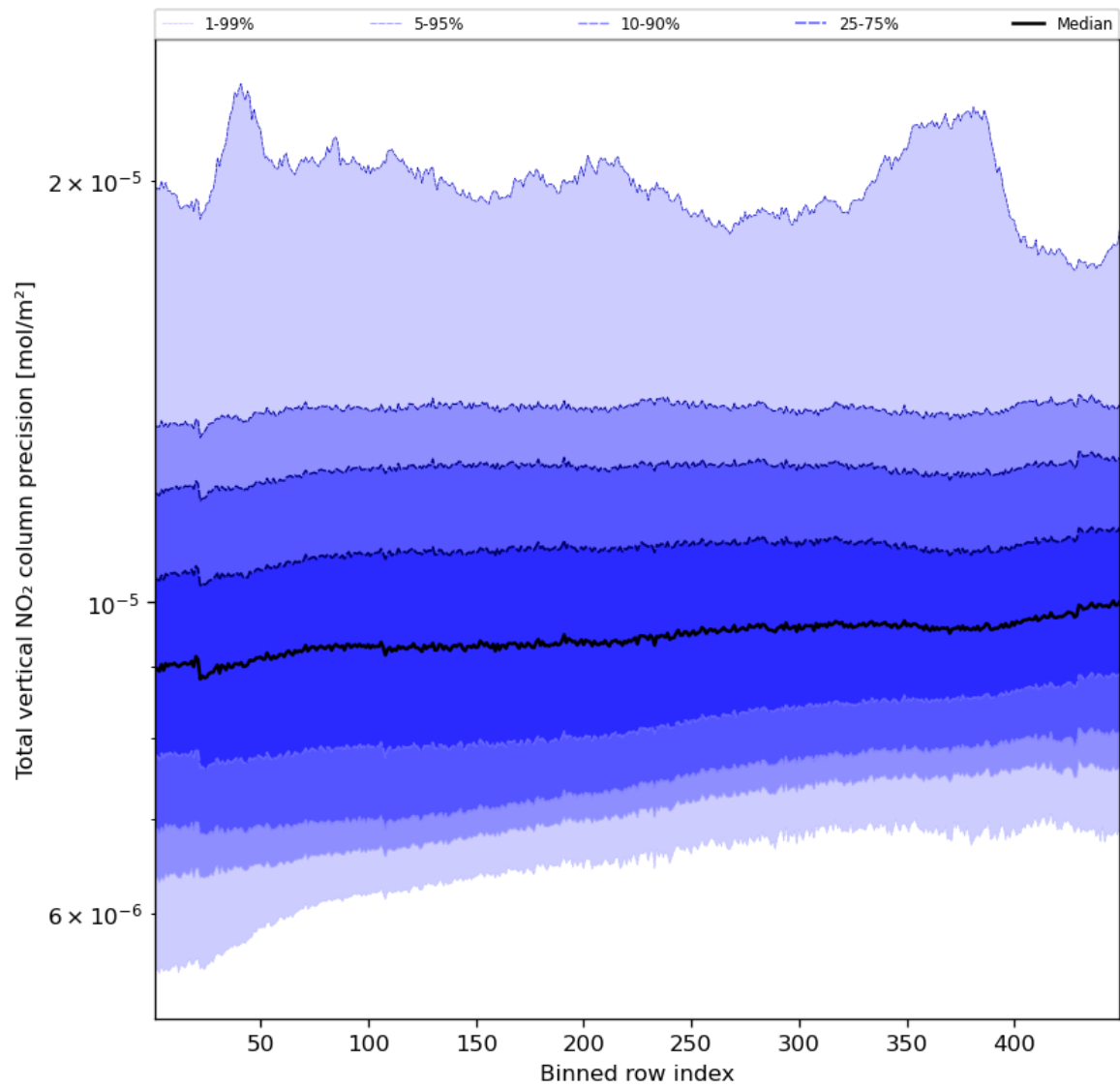
Figure 56: Along track statistics of “Total vertical NO 2 column precision” for 2024-04-01 to 2024-04-03
