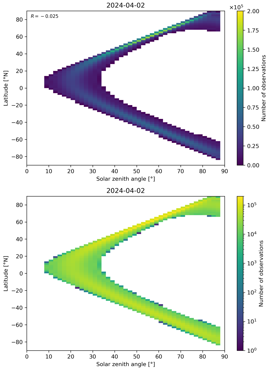
Figure 149: Scatter density plot of “Solar zenith angle” against “Latitude” for 2024-04-01 to 2024-04-03.
