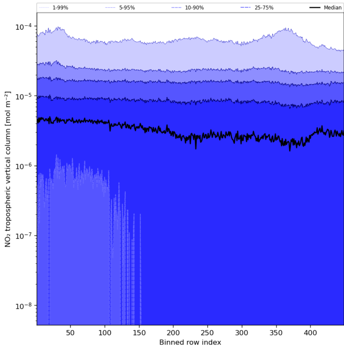
Figure 46: Along track statistics of “NO 2 tropospheric vertical column” for 2024-04-01 to 2024-04-03
