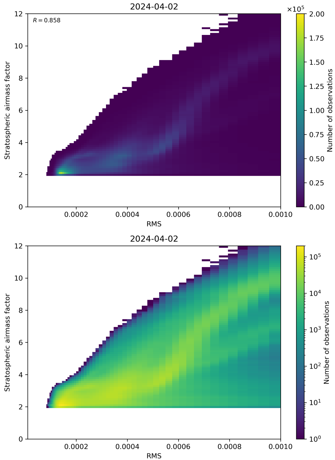
Figure 144: Scatter density plot of “RMS” against “Stratospheric airmass factor” for 2024-04-01 to 2024-04-03.
