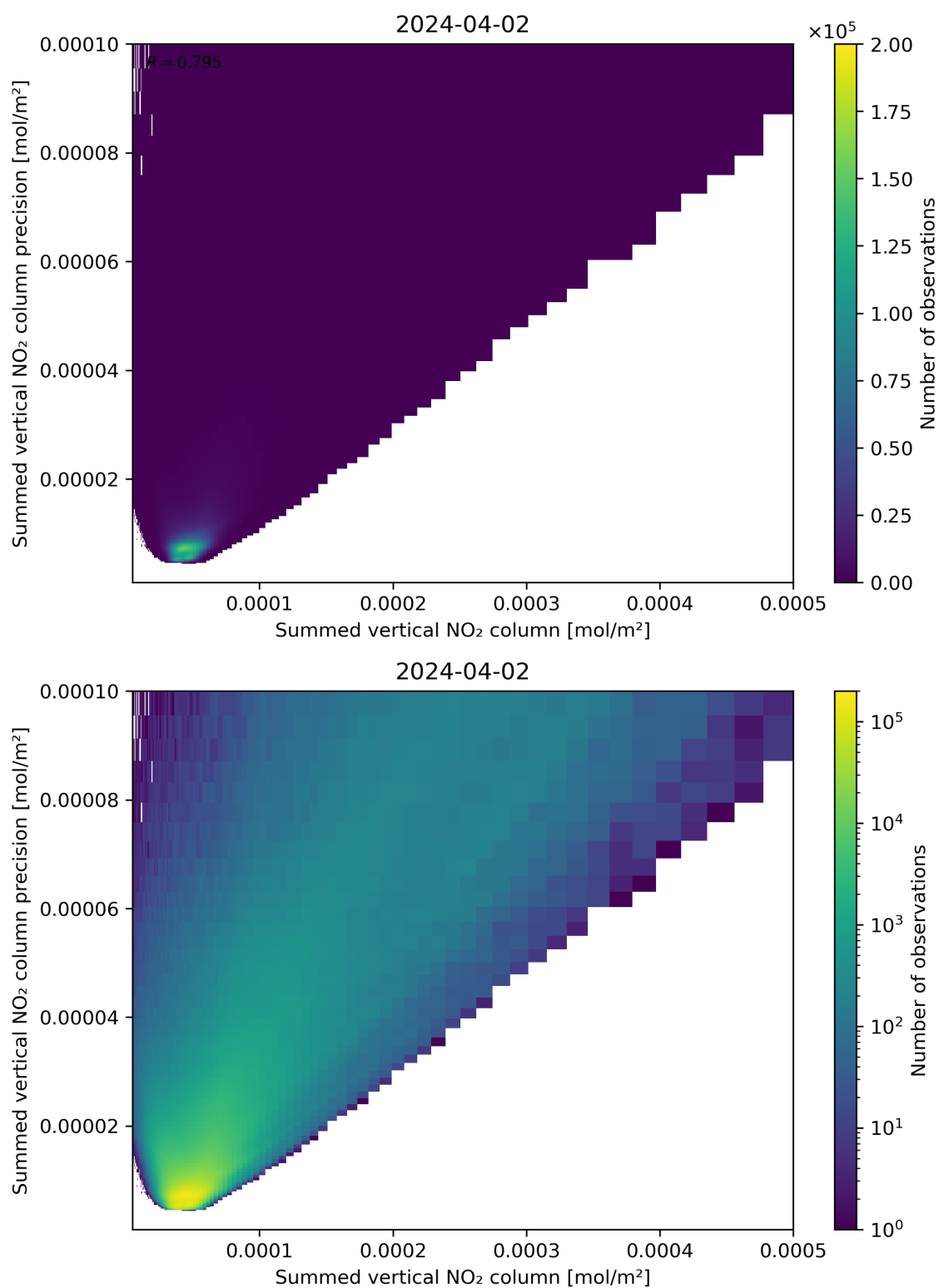
Figure 105: Scatter density plot of “Summed vertical NO 2 column” against “Summed vertical NO 2 column precision” for 2024-04-01 to 2024-04-03.
