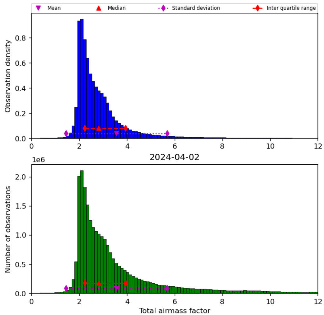
Figure 32: Histogram of “Total airmass factor” for 2024-04-01 to 2024-04-03
