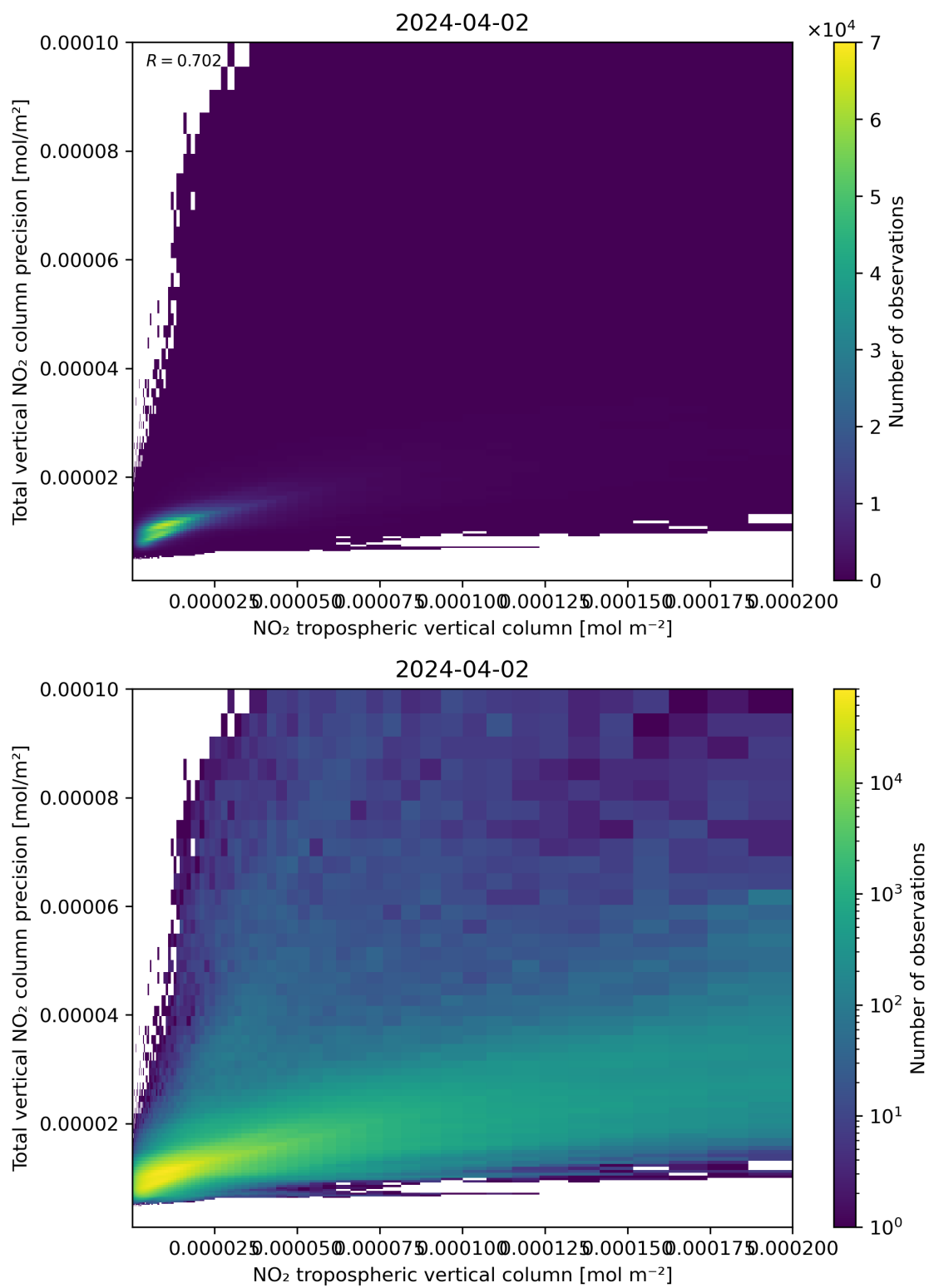
Figure 129: Scatter density plot of “NO 2 tropospheric vertical column” against “Total vertical NO 2 column precision” for 2024-04-01 to 2024-04-03.
