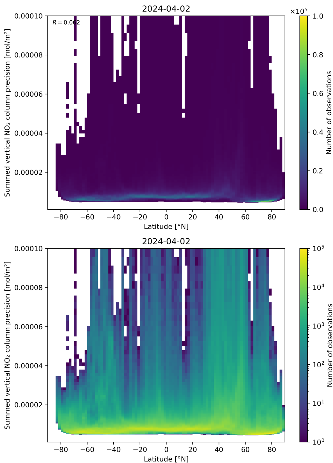
Figure 89: Scatter density plot of “Latitude” against “Summed vertical NO 2 column precision” for 2024-04-01 to 2024-04-03.
