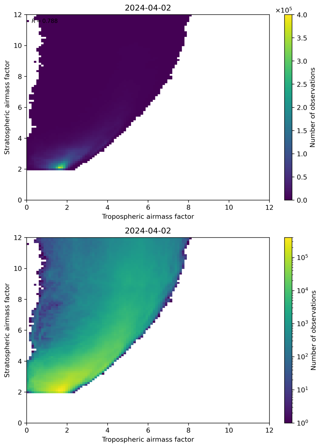
Figure 71: Scatter density plot of “Tropospheric airmass factor” against “Stratospheric airmass factor” for 2024-04-01 to 2024-04-03.
