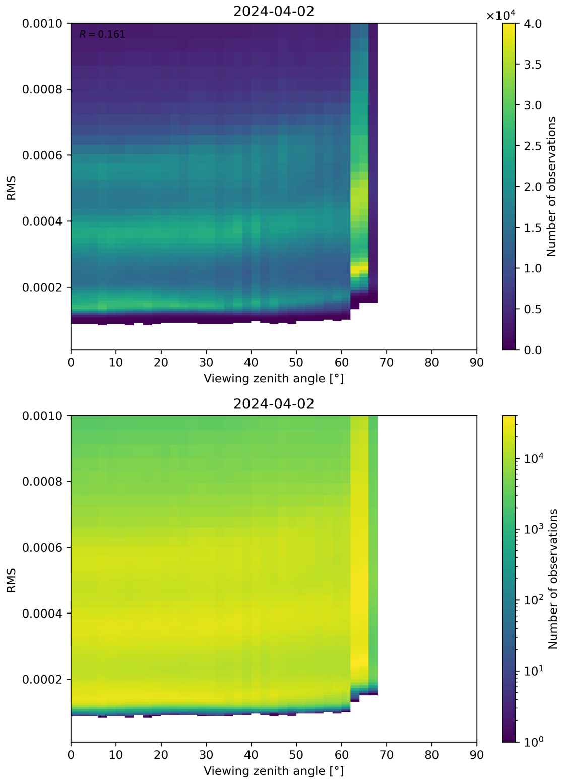
Figure 171: Scatter density plot of “Viewing zenith angle” against “RMS” for 2024-04-01 to 2024-04-03.
