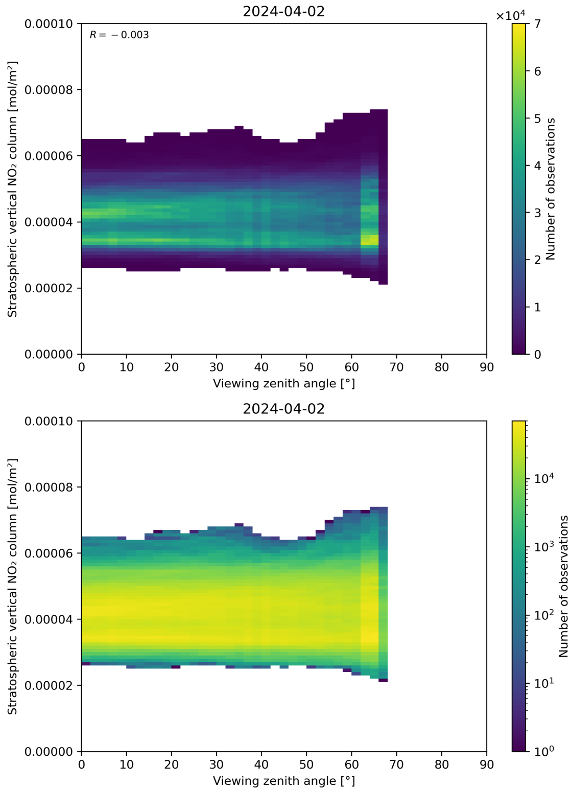
Figure 164: Scatter density plot of “Viewing zenith angle” against “Stratospheric vertical NO 2 column” for 2024-04-01 to 2024-04-03.
