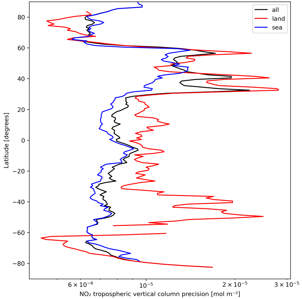
Figure 13: Zonal average of “NO 2 tropospheric vertical column precision” for 2024-04-01 to 2024-04-03.
