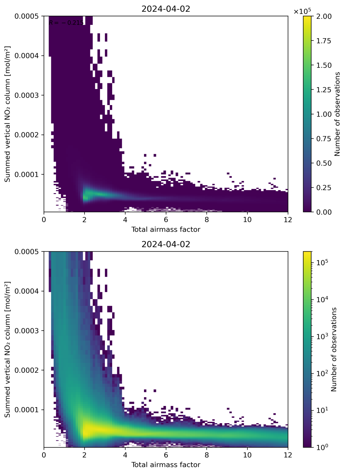
Figure 65: Scatter density plot of “Total airmass factor” against “Summed vertical NO 2 column” for 2024-04-01 to 2024-04-03.
