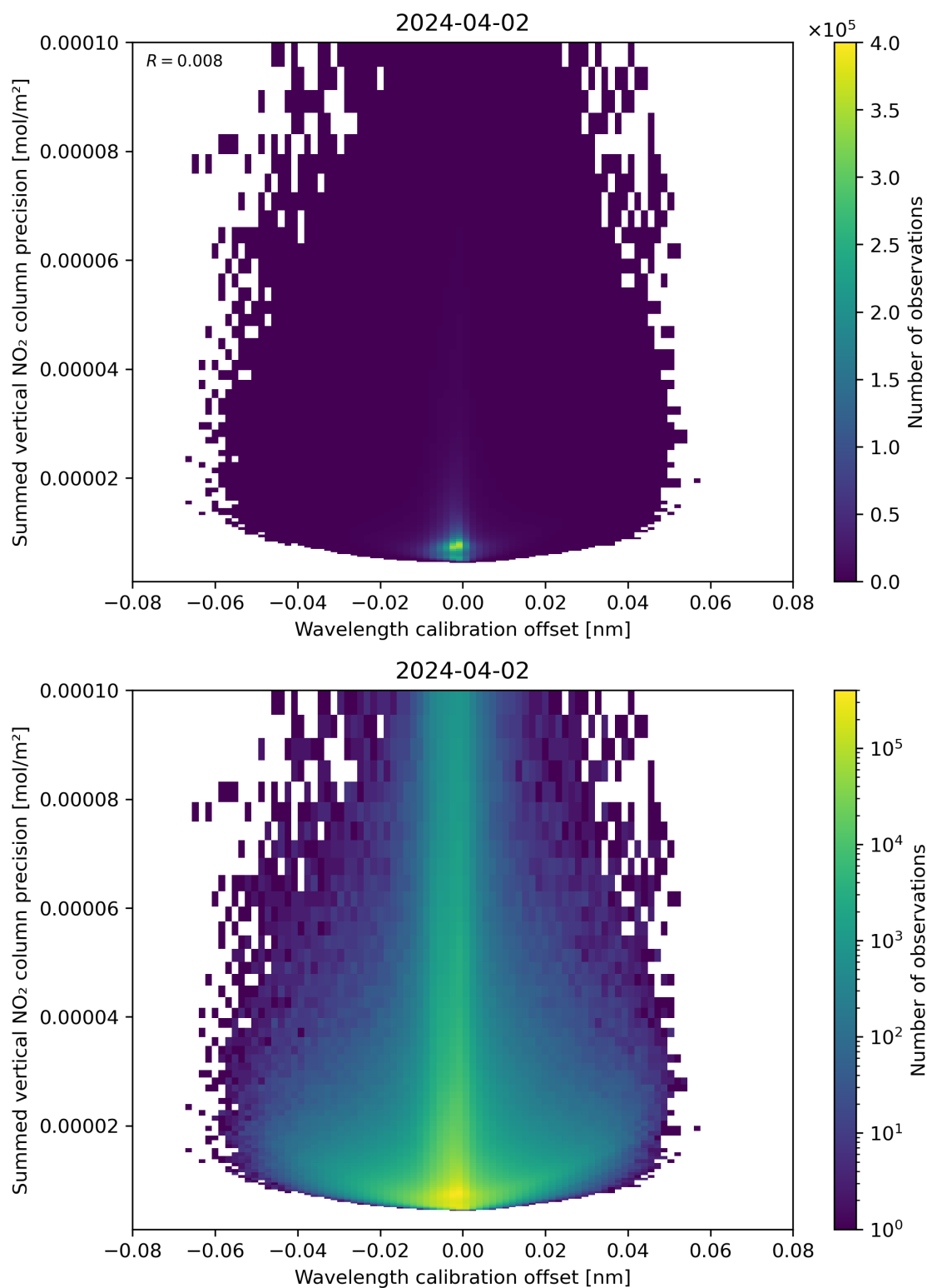
Figure 178: Scatter density plot of “Wavelength calibration offset” against “Summed vertical NO 2 column precision” for 2024-04-01 to 2024-04-03.
