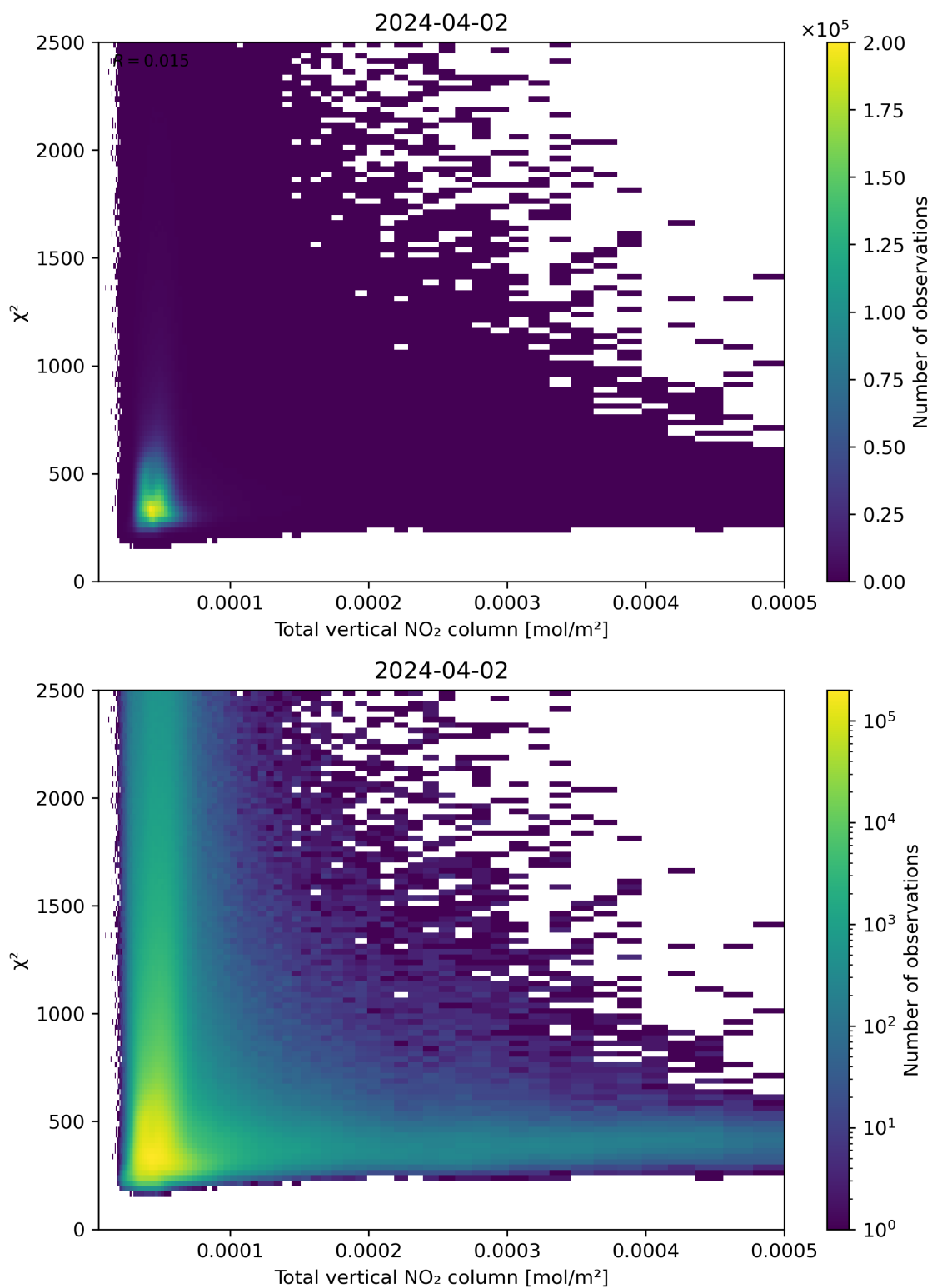
Figure 111: Scatter density plot of “Total vertical NO 2 column” against “ \chi^2 ” for 2024-04-01 to 2024-04-03.
