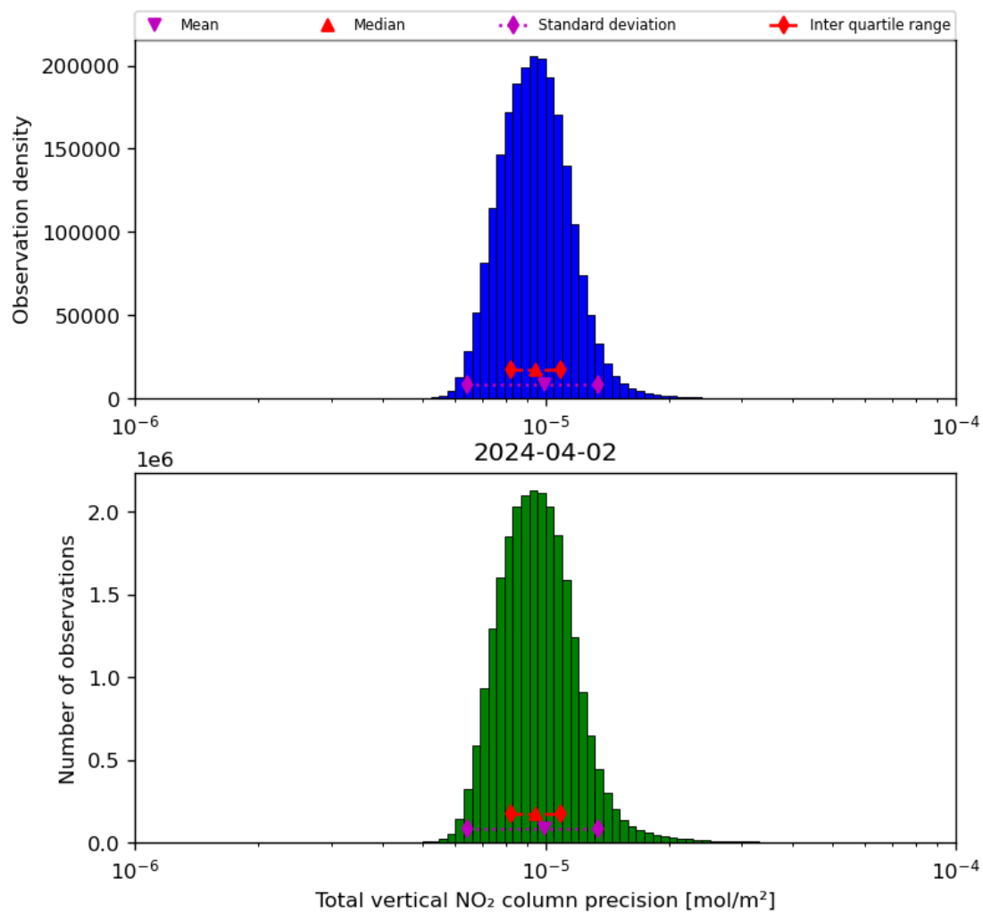
Figure 39: Histogram of “Total vertical NO 2 column precision” for 2024-04-01 to 2024-04-03
