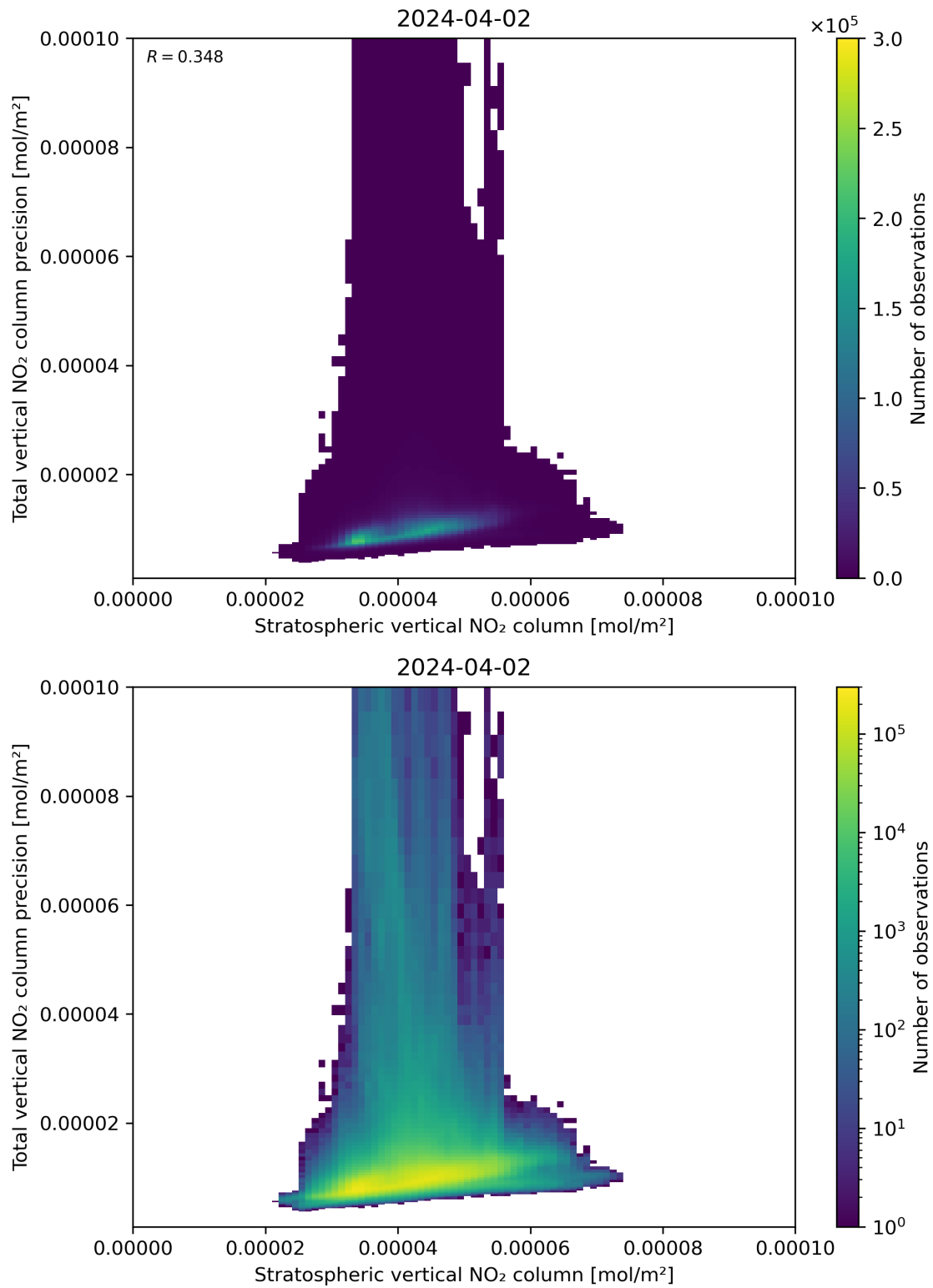
Figure 101: Scatter density plot of “Stratospheric vertical NO 2 column” against “Total vertical NO 2 column precision” for 2024-04-01 to 2024-04-03.
