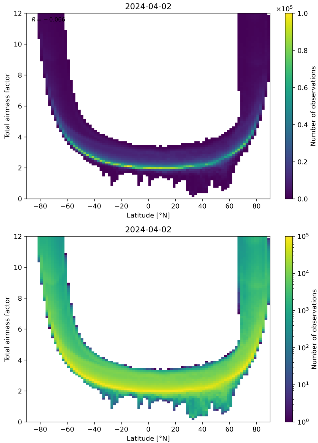
Figure 84: Scatter density plot of “Latitude” against “Total airmass factor” for 2024-04-01 to 2024-04-03.
