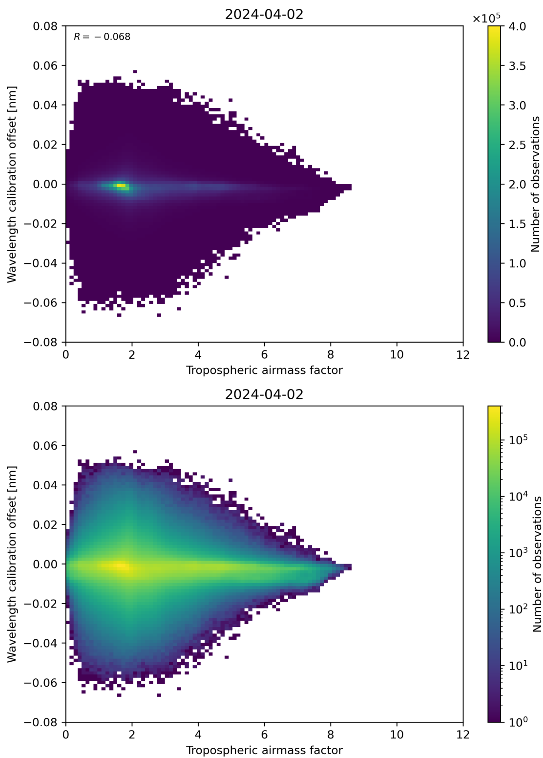
Figure 80: Scatter density plot of “Tropospheric airmass factor” against “Wavelength calibration offset” for 2024-04-01 to 2024-04-03.
