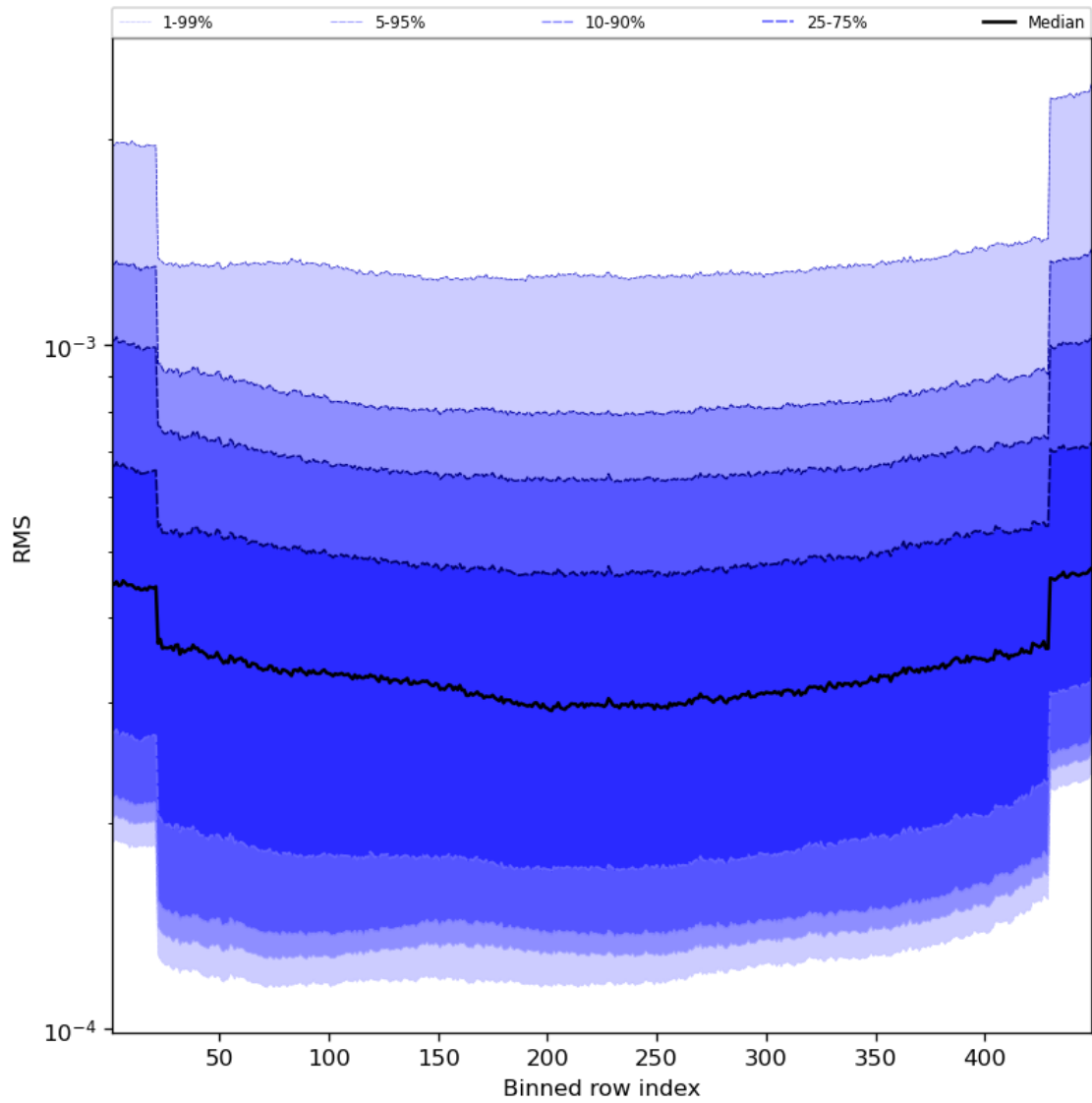
Figure 60: Along track statistics of “RMS” for 2024-04-01 to 2024-04-03
