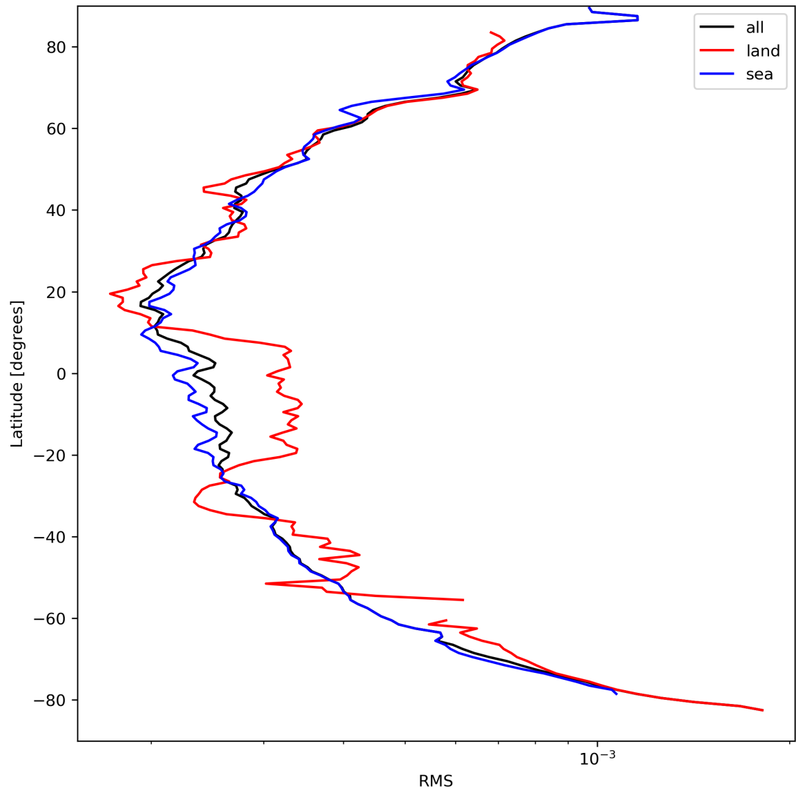
Figure 26: Zonal average of “RMS” for 2024-04-01 to 2024-04-03.
