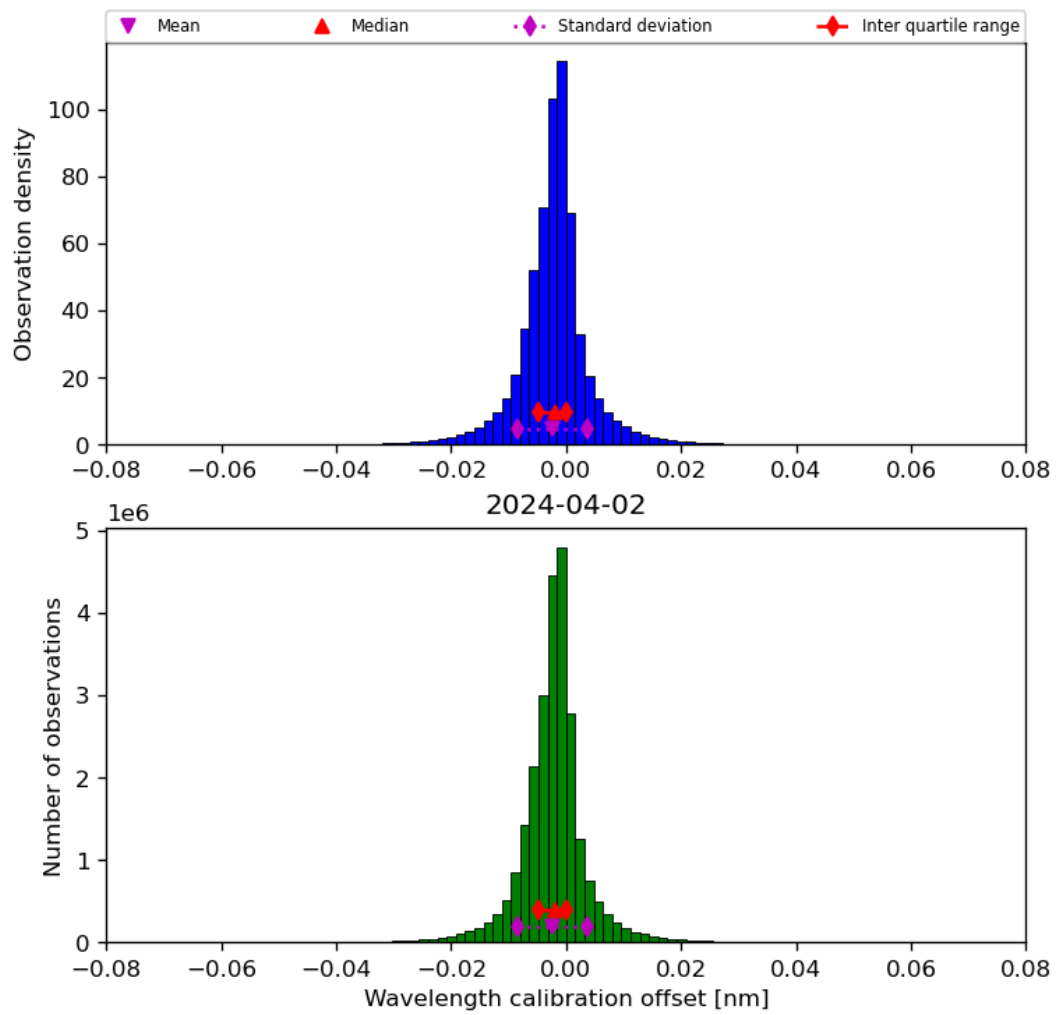
Figure 35: Histogram of “Wavelength calibration offset” for 2024-04-01 to 2024-04-03
