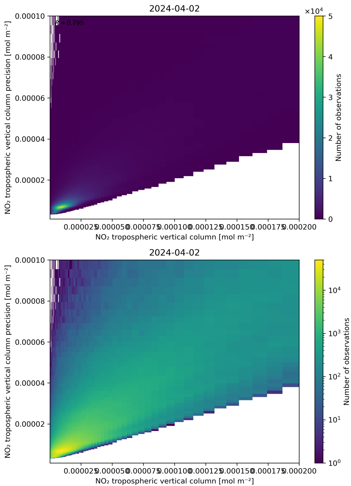
Figure 130: Scatter density plot of “NO 2 tropospheric vertical column” against “NO 2 tropospheric vertical column precision” for 2024-04-01 to 2024-04-03.
