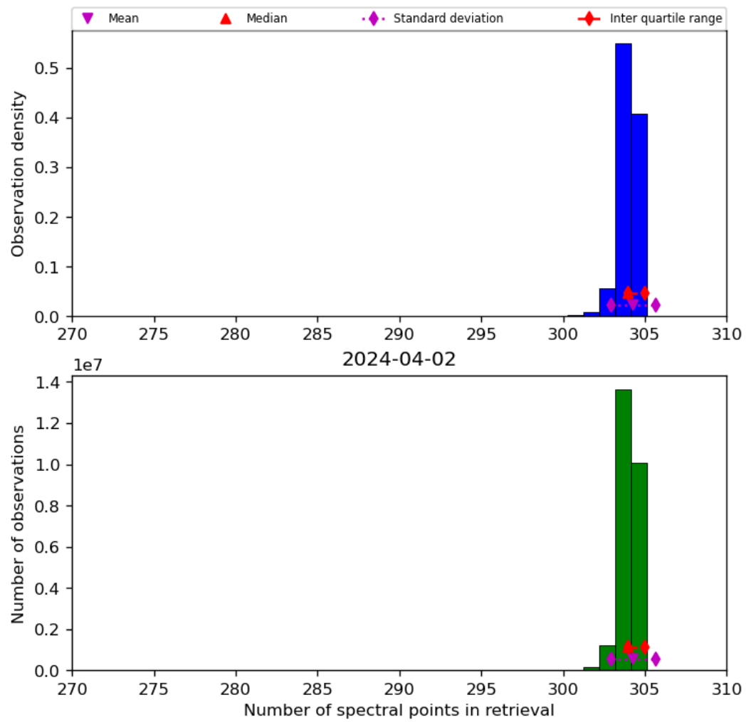
Figure 33: Histogram of “Number of spectral points in retrieval” for 2024-04-01 to 2024-04-03
