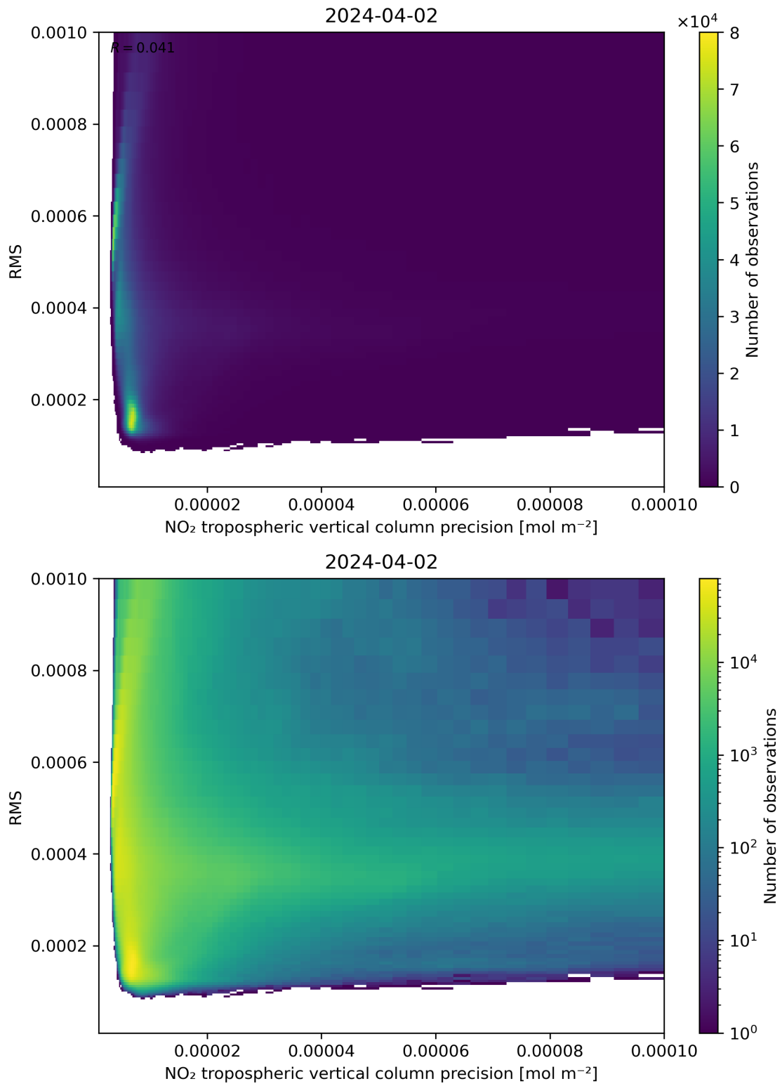
Figure 140: Scatter density plot of “NO 2 tropospheric vertical column precision” against “RMS” for 2024-04-01 to 2024-04-03.
