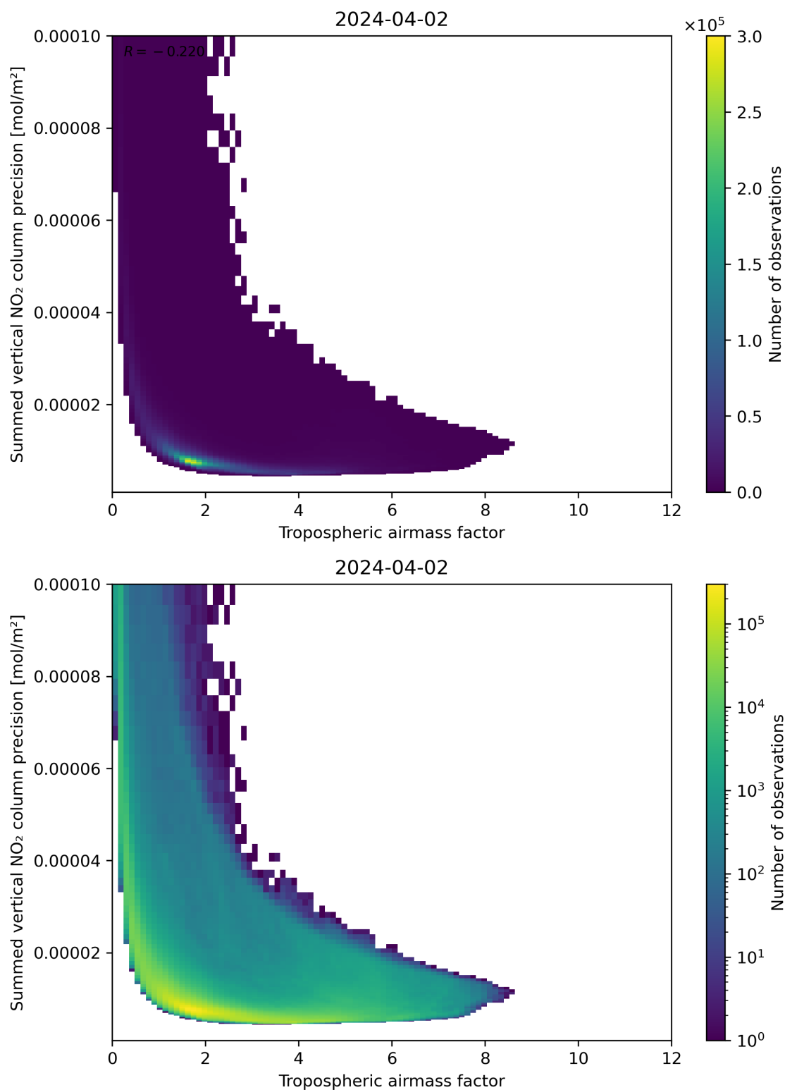
Figure 76: Scatter density plot of “Tropospheric air mass factor” against “Summed vertical NO 2 column precision” for 2024-04-01 to 2024-04-03.
