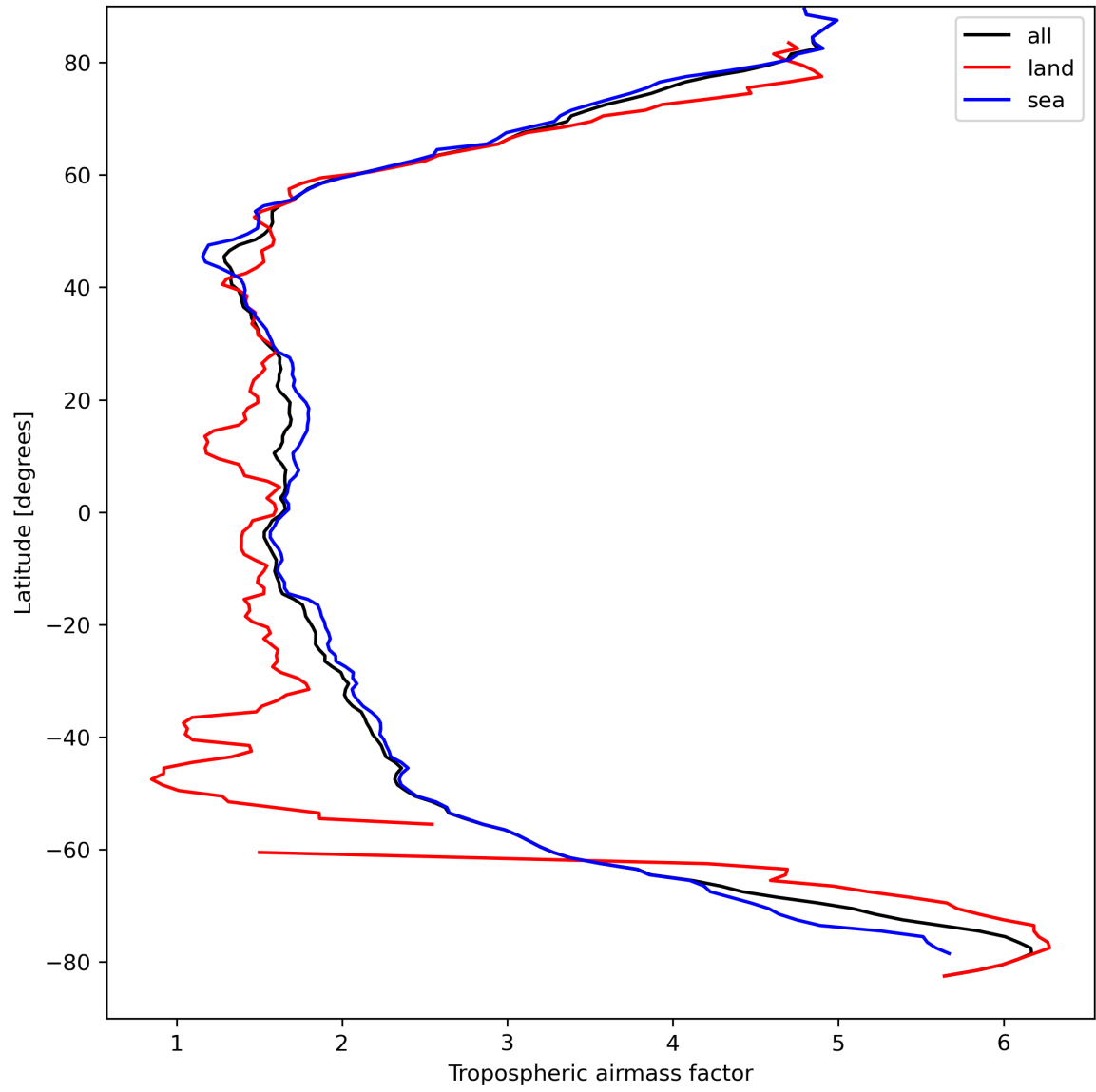
Figure 14: Zonal average of “Tropospheric air mass factor” for 2024-04-01 to 2024-04-03.
