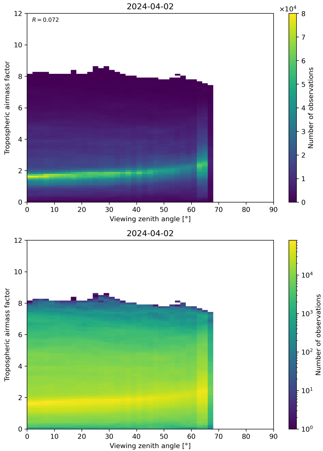
Figure 161: Scatter density plot of “Viewing zenith angle” against “Tropospheric airmass factor” for 2024-04-01 to 2024-04-03.
