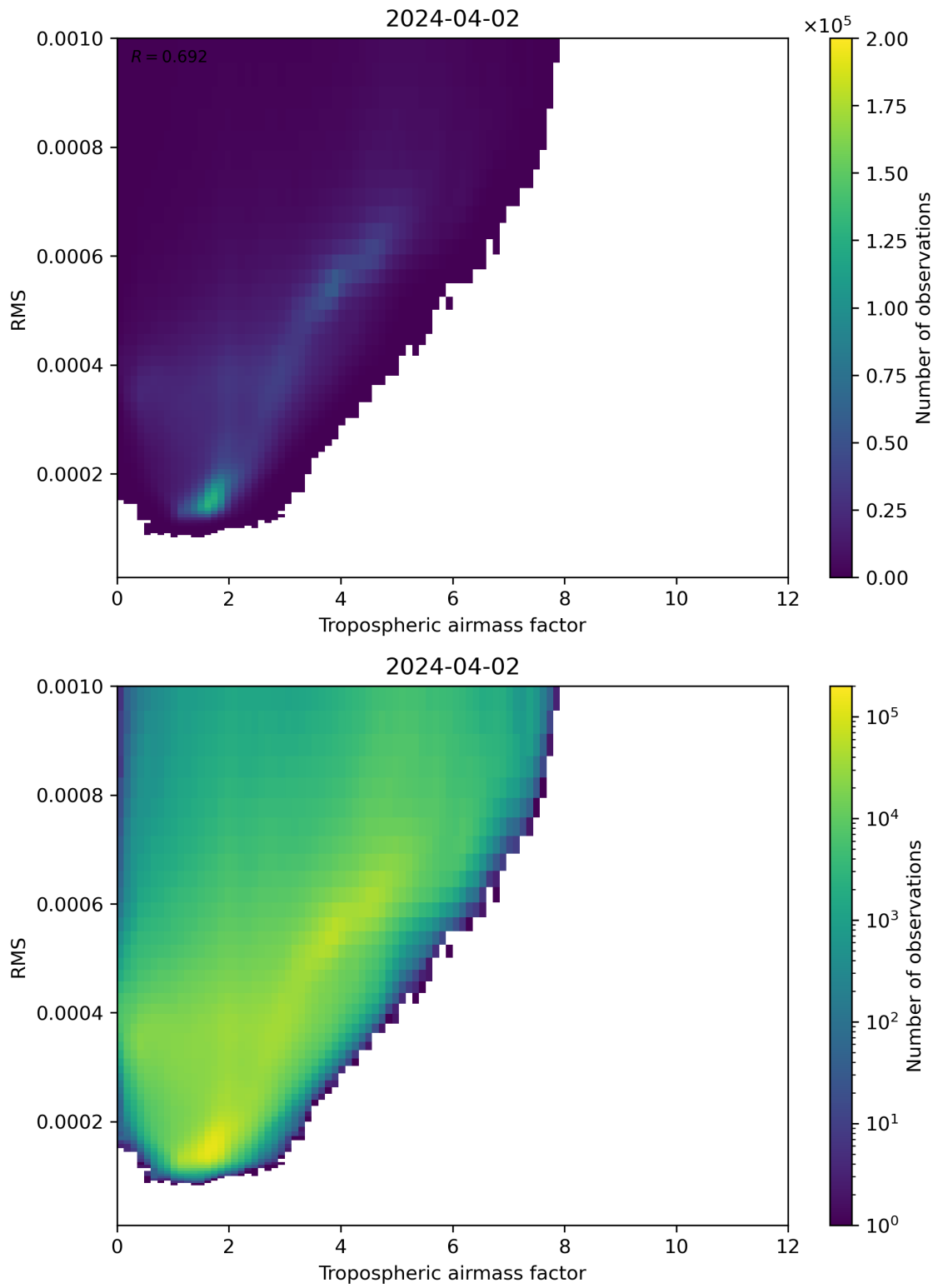
Figure 79: Scatter density plot of “Tropospheric airmass factor” against “RMS” for 2024-04-01 to 2024-04-03.
