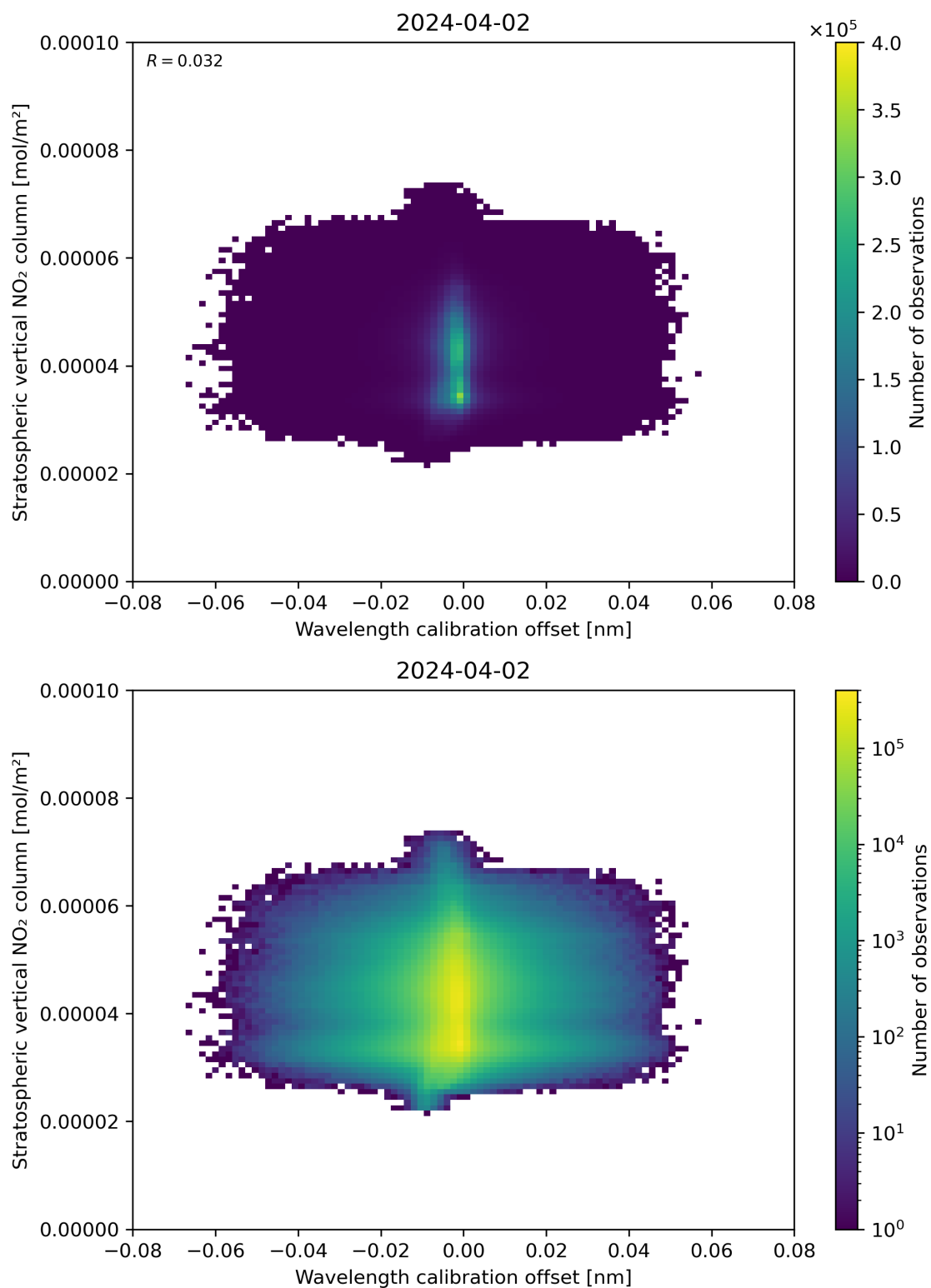
Figure 176: Scatter density plot of “Wavelength calibration offset” against “Stratospheric vertical NO 2 column” for 2024-04-01 to 2024-04-03.
