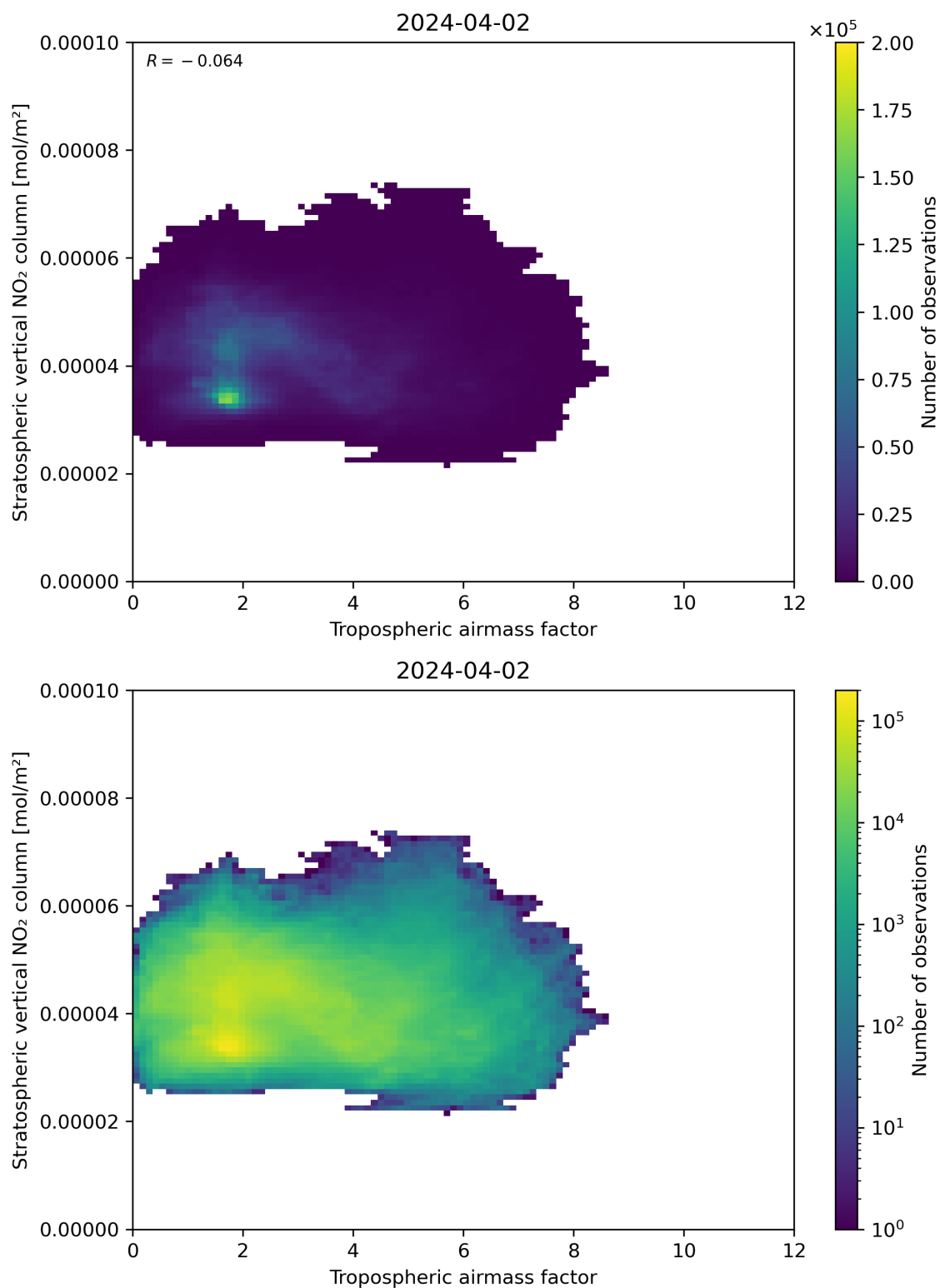
Figure 74: Scatter density plot of “Tropospheric air mass factor” against “Stratospheric vertical NO 2 column” for 2024-04-01 to 2024-04-03.
