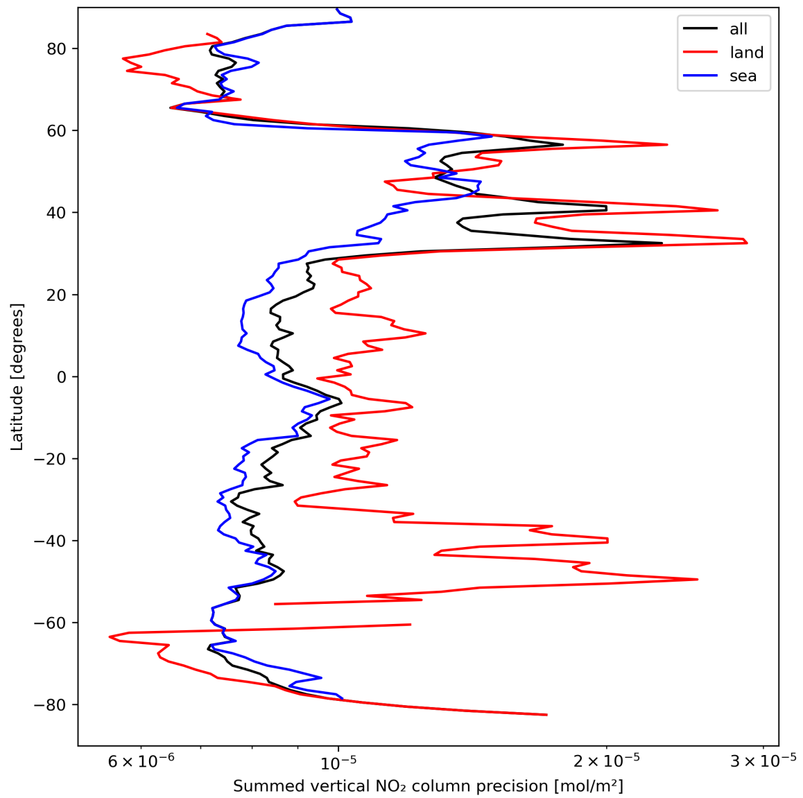
Figure 24: Zonal average of “Summed vertical NO 2 column precision” for 2024-04-01 to 2024-04-03.
