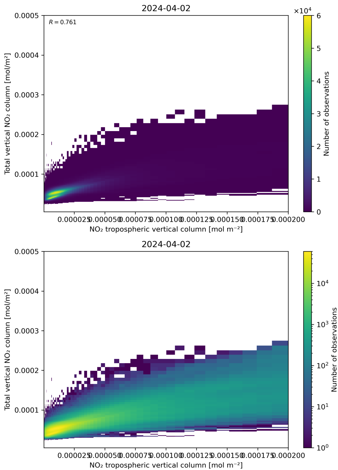
Figure 128: Scatter density plot of “NO 2 tropospheric vertical column” against “Total vertical NO 2 column” for 2024-04-01 to 2024-04-03.
