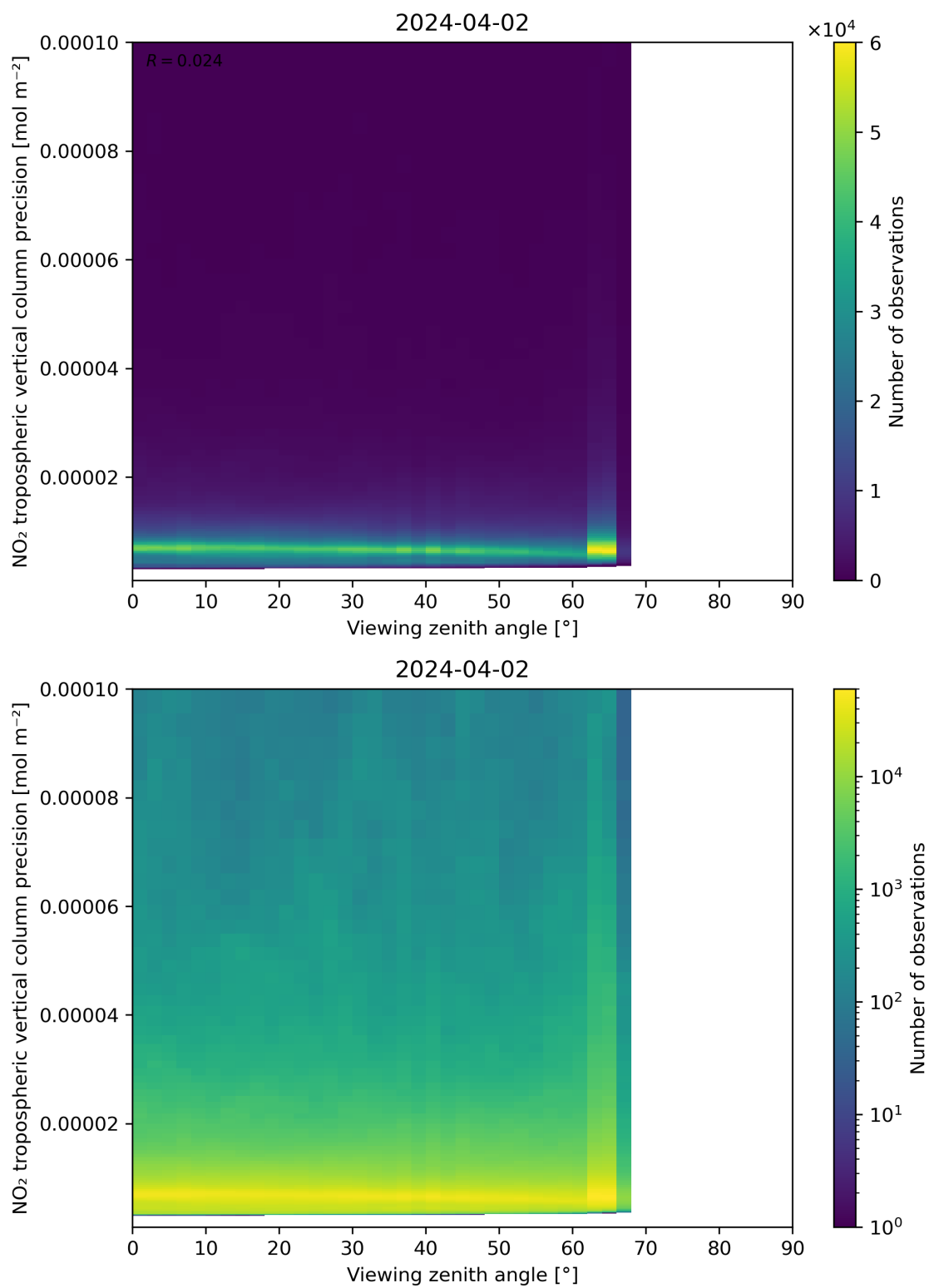
Figure 170: Scatter density plot of “Viewing zenith angle” against “NO 2 tropospheric vertical column precision” for 2024-04-01 to 2024-04-03.
