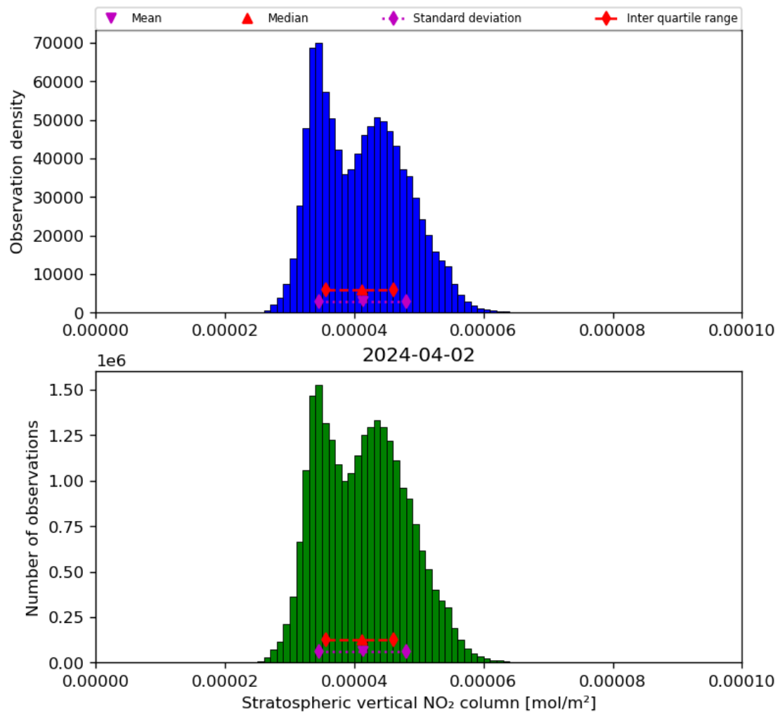
Figure 36: Histogram of “Stratospheric vertical NO 2 column” for 2024-04-01 to 2024-04-03
