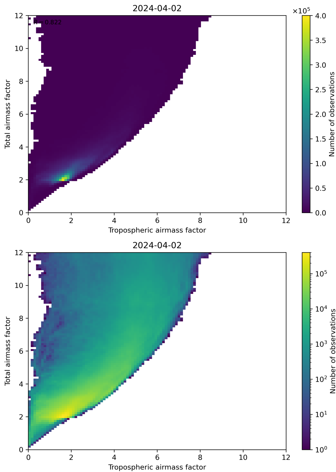
Figure 72: Scatter density plot of “Tropospheric airmass factor” against “Total airmass factor” for 2024-04-01 to 2024-04-03.
