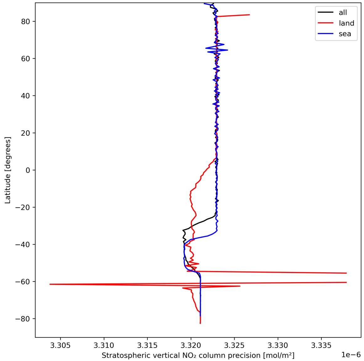
Figure 20: Zonal average of “Stratospheric vertical NO 2 column precision” for 2024-04-01 to 2024-04-03.
