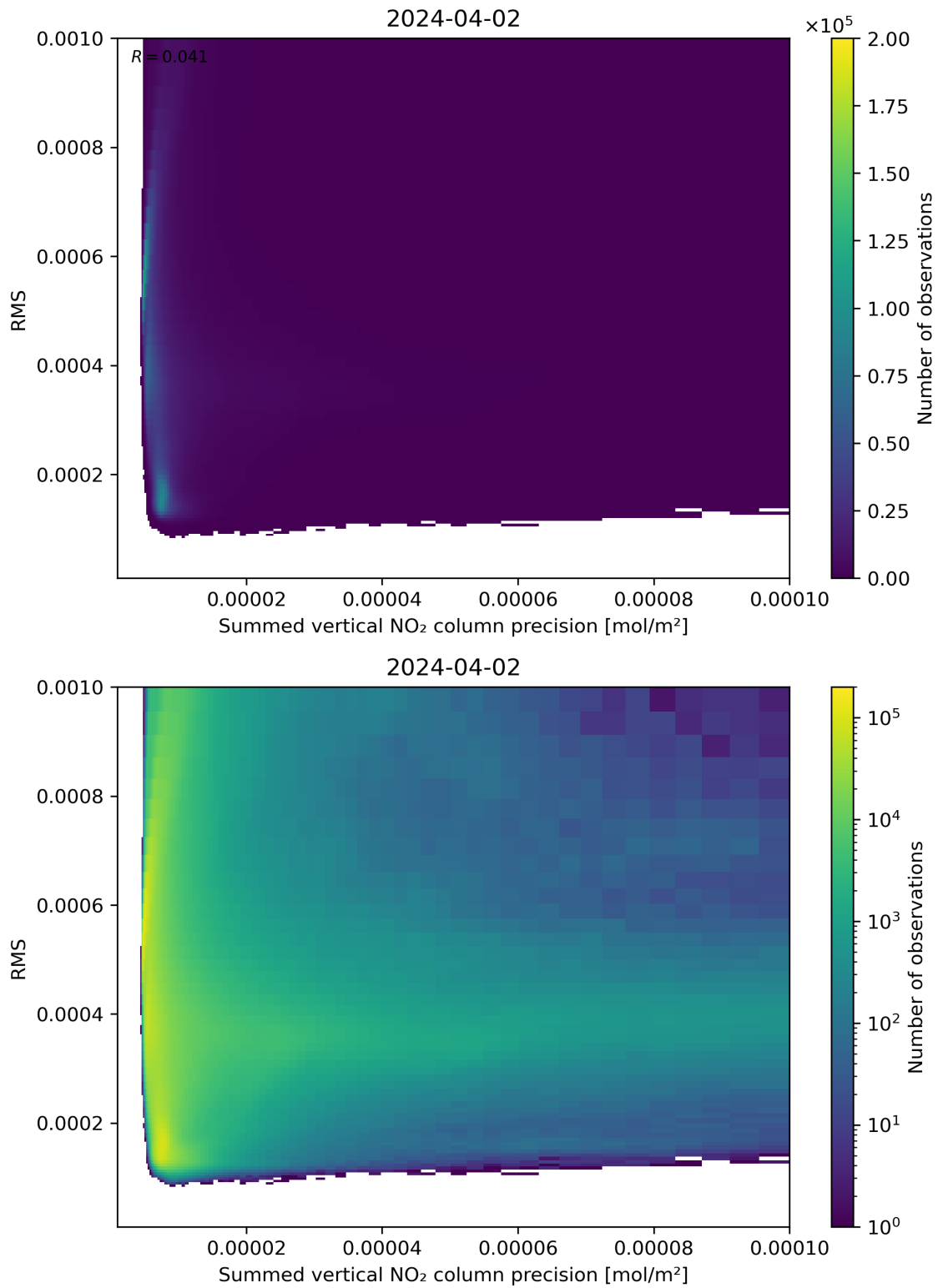
Figure 108: Scatter density plot of “Summed vertical NO 2 column precision” against “RMS” for 2024-04-01 to 2024-04-03.
