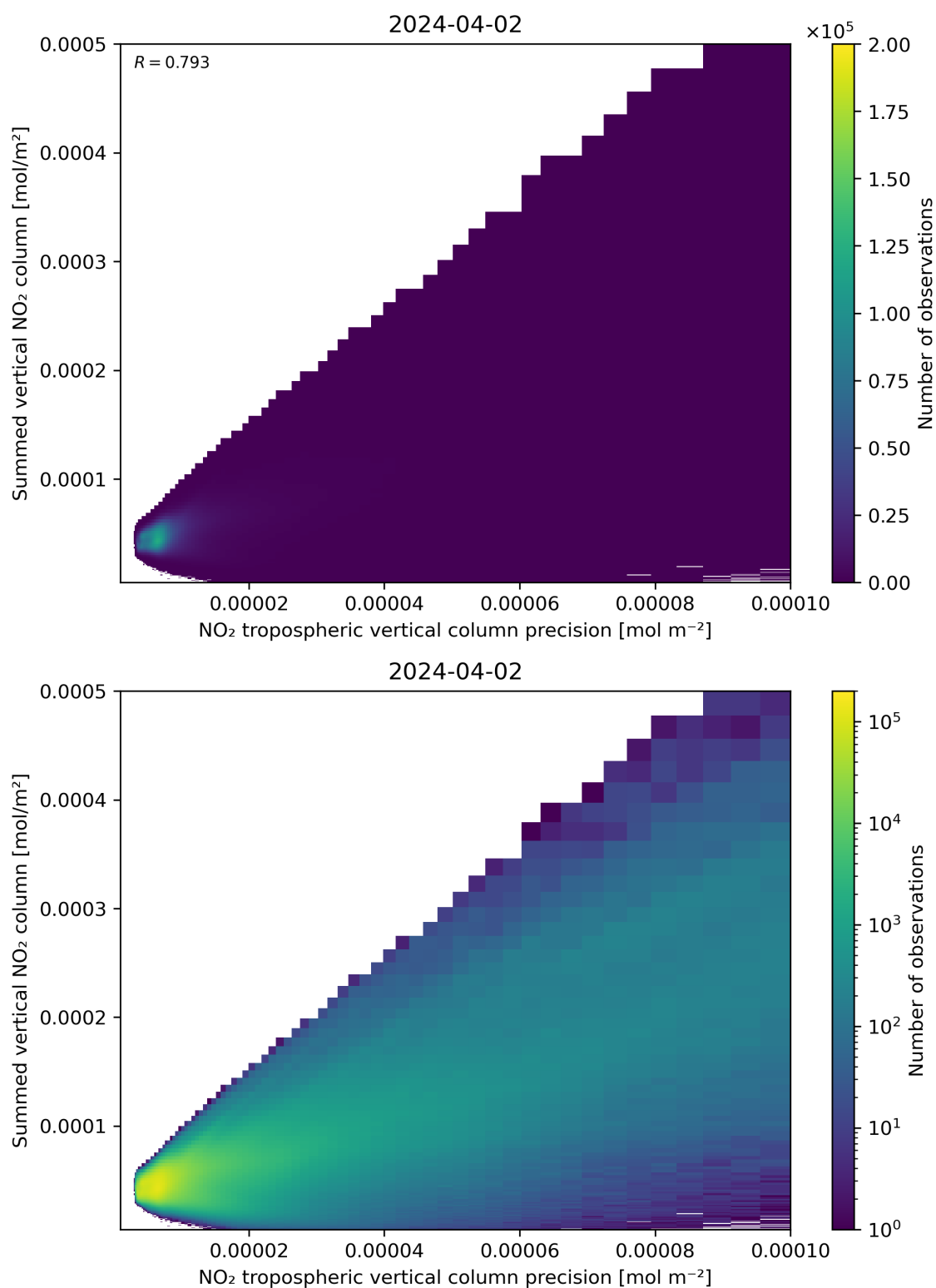
Figure 136: Scatter density plot of “NO 2 tropospheric vertical column precision” against “Summed vertical NO 2 column” for 2024-04-01 to 2024-04-03.
