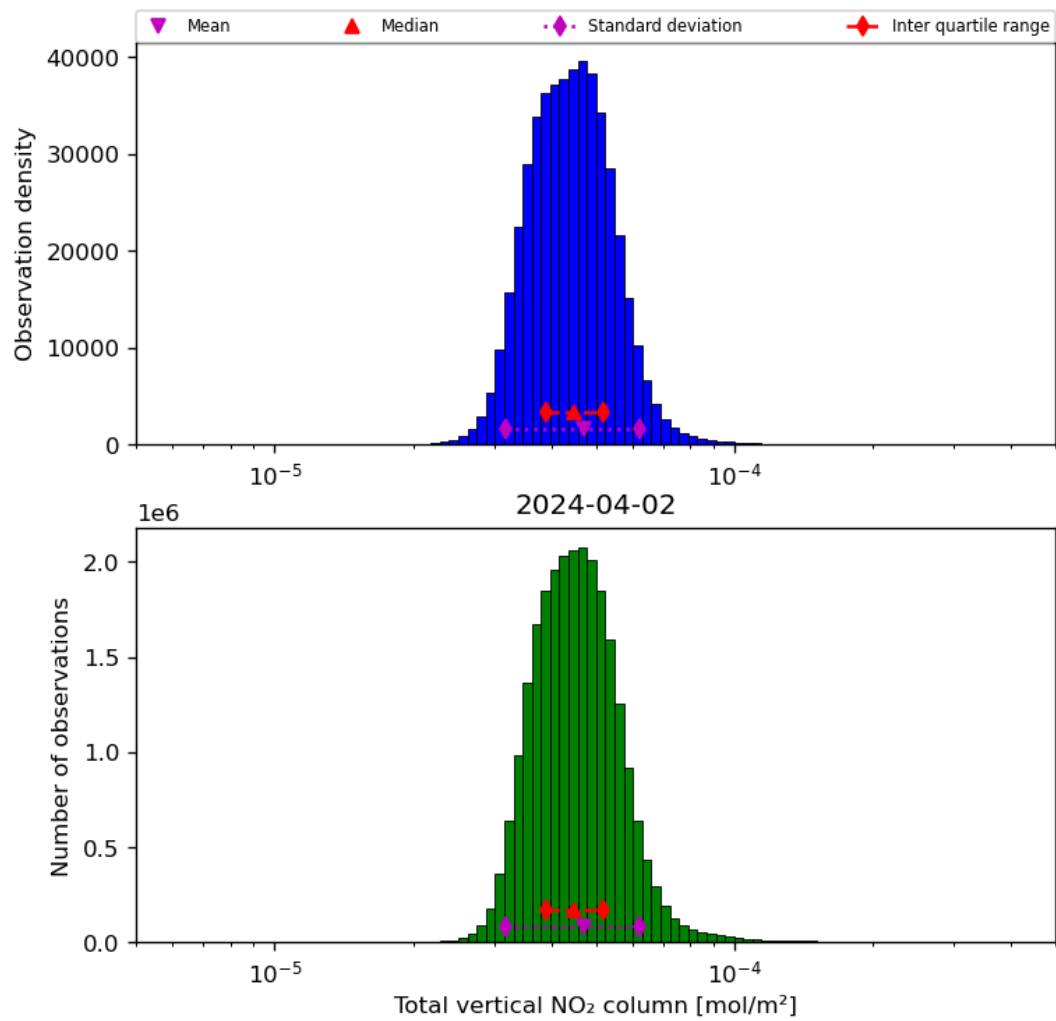
Figure 38: Histogram of "Total vertical NO 2 column" for 2024-04-01 to 2024-04-03
