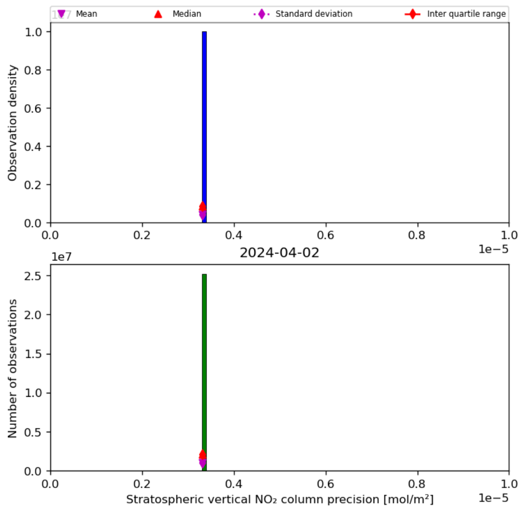
Figure 37: Histogram of “Stratospheric vertical NO 2 column precision” for 2024-04-01 to 2024-04-03
