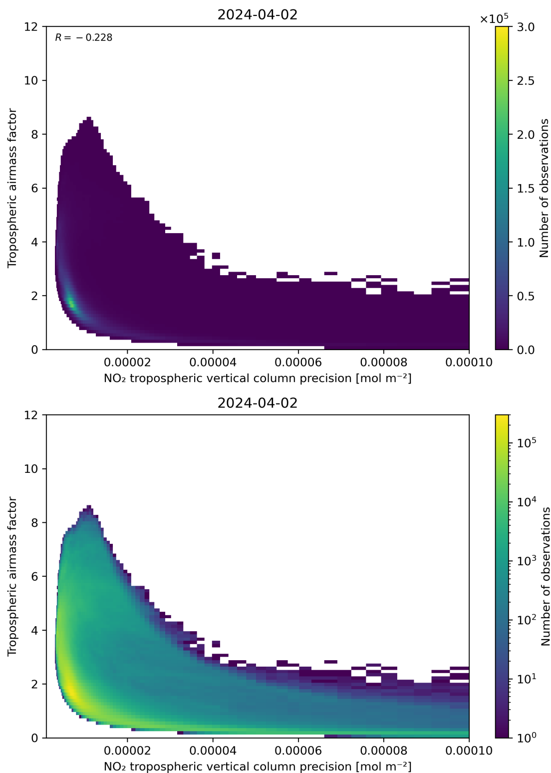
Figure 133: Scatter density plot of “NO 2 tropospheric vertical column precision” against “Tropospheric airmass factor” for 2024-04-01 to 2024-04-03.
