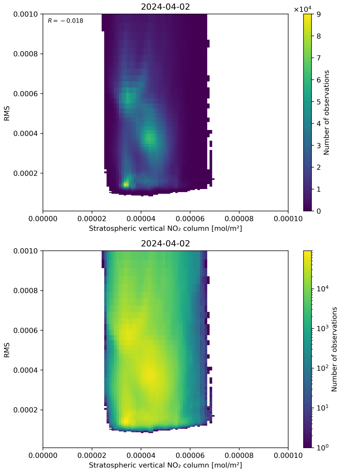
Figure 102: Scatter density plot of “Stratospheric vertical NO 2 column” against “RMS” for 2024-04-01 to 2024-04-03.
