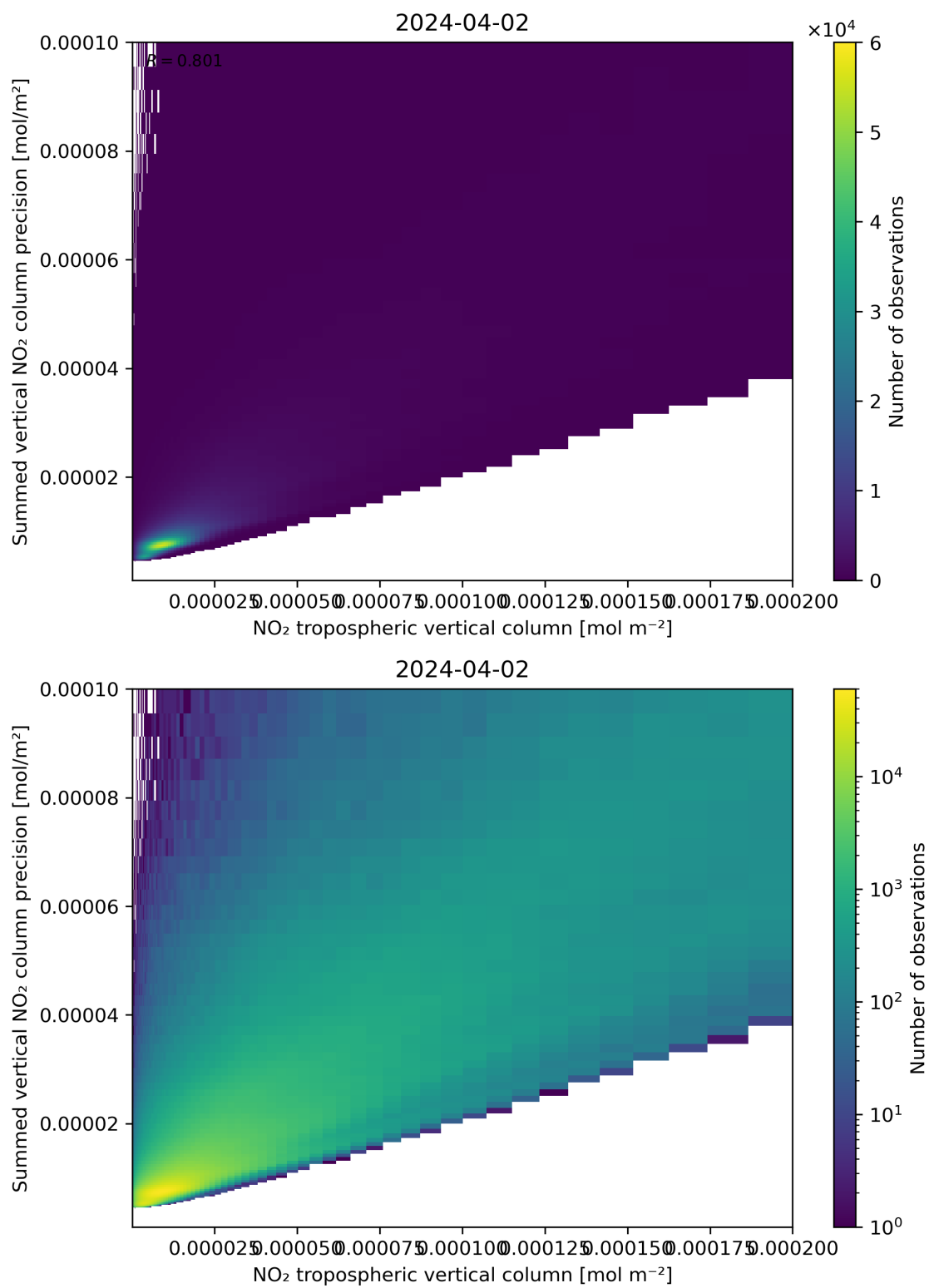
Figure 127: Scatter density plot of “NO 2 tropospheric vertical column” against “Summed vertical NO 2 column precision” for 2024-04-01 to 2024-04-03.
