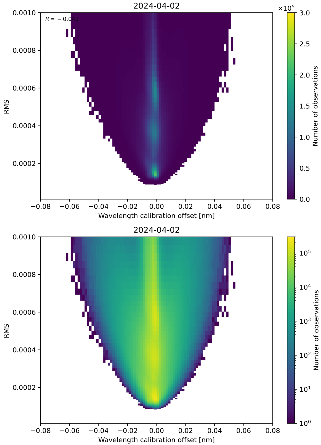
Figure 181: Scatter density plot of “Wavelength calibration offset” against “RMS” for 2024-04-01 to 2024-04-03.
