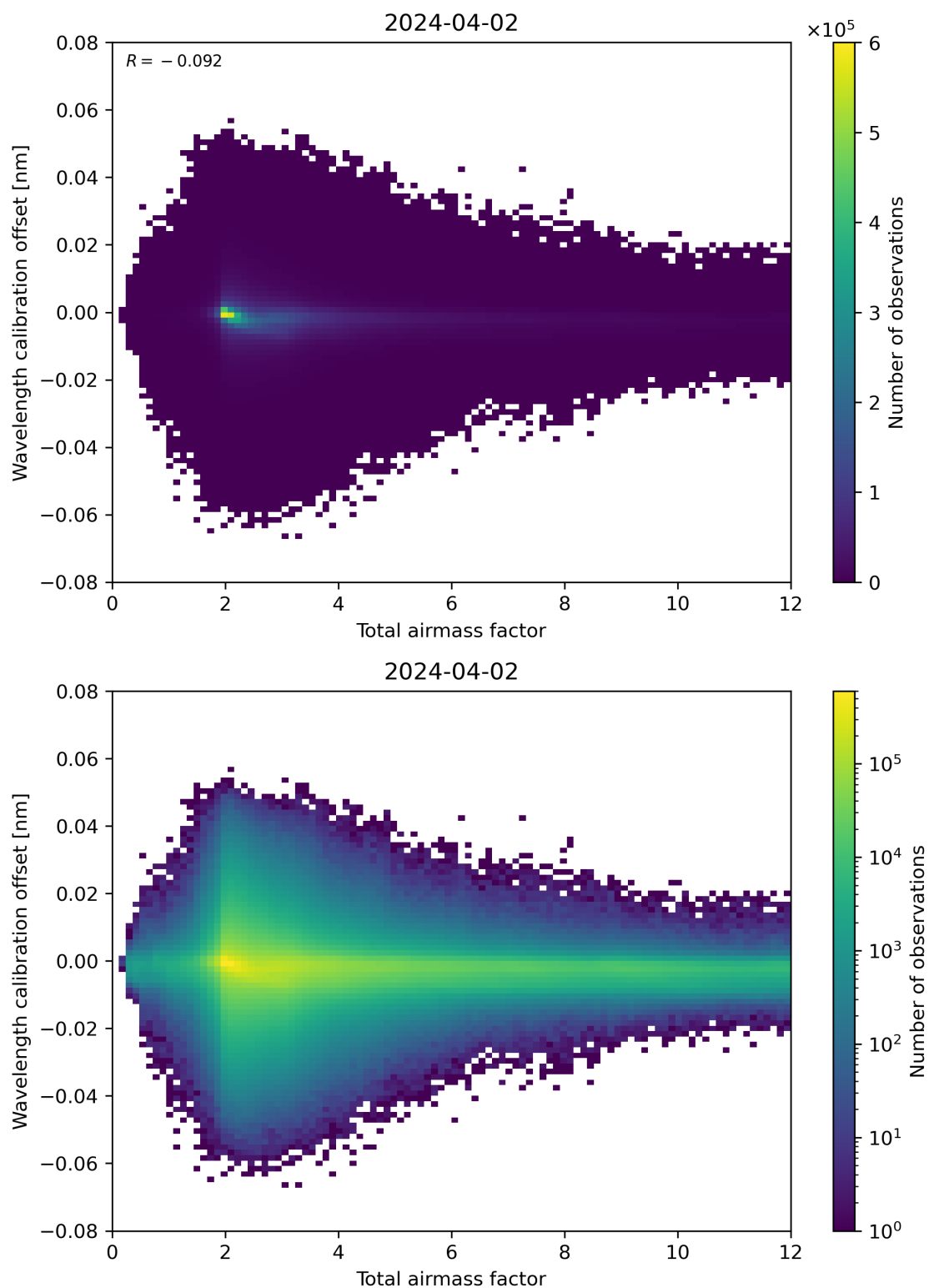
Figure 70: Scatter density plot of “Total airmass factor” against “Wavelength calibration offset” for 2024-04-01 to 2024-04-03.
