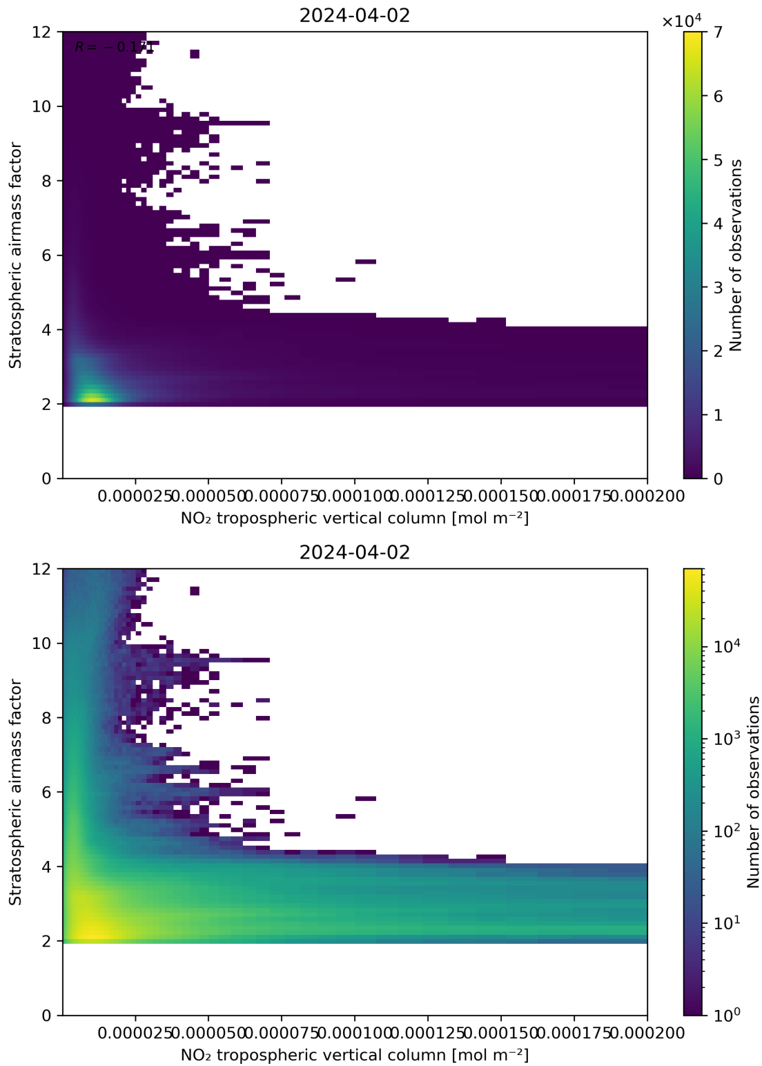
Figure 121: Scatter density plot of “NO 2 tropospheric vertical column” against “Stratospheric air mass factor” for 2024-04-01 to 2024-04-03.
