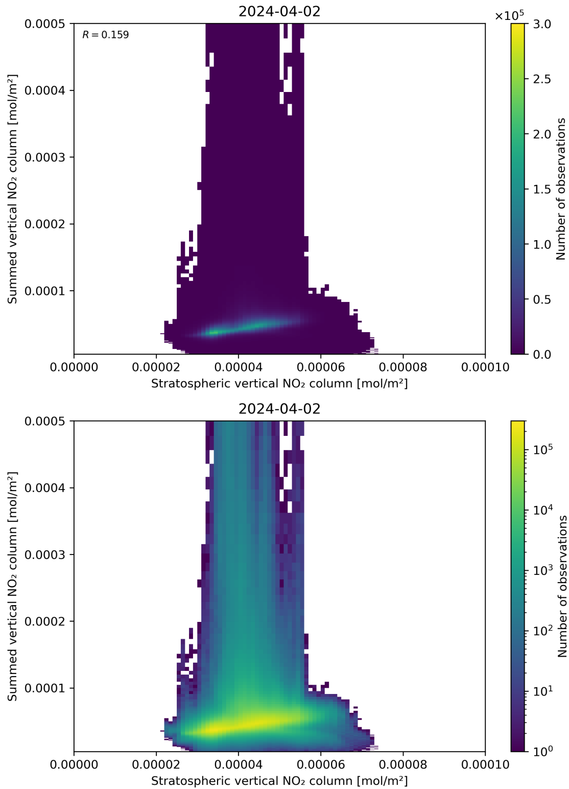
Figure 98: Scatter density plot of “Stratospheric vertical NO 2 column” against “Summed vertical NO 2 column” for 2024-04-01 to 2024-04-03.
