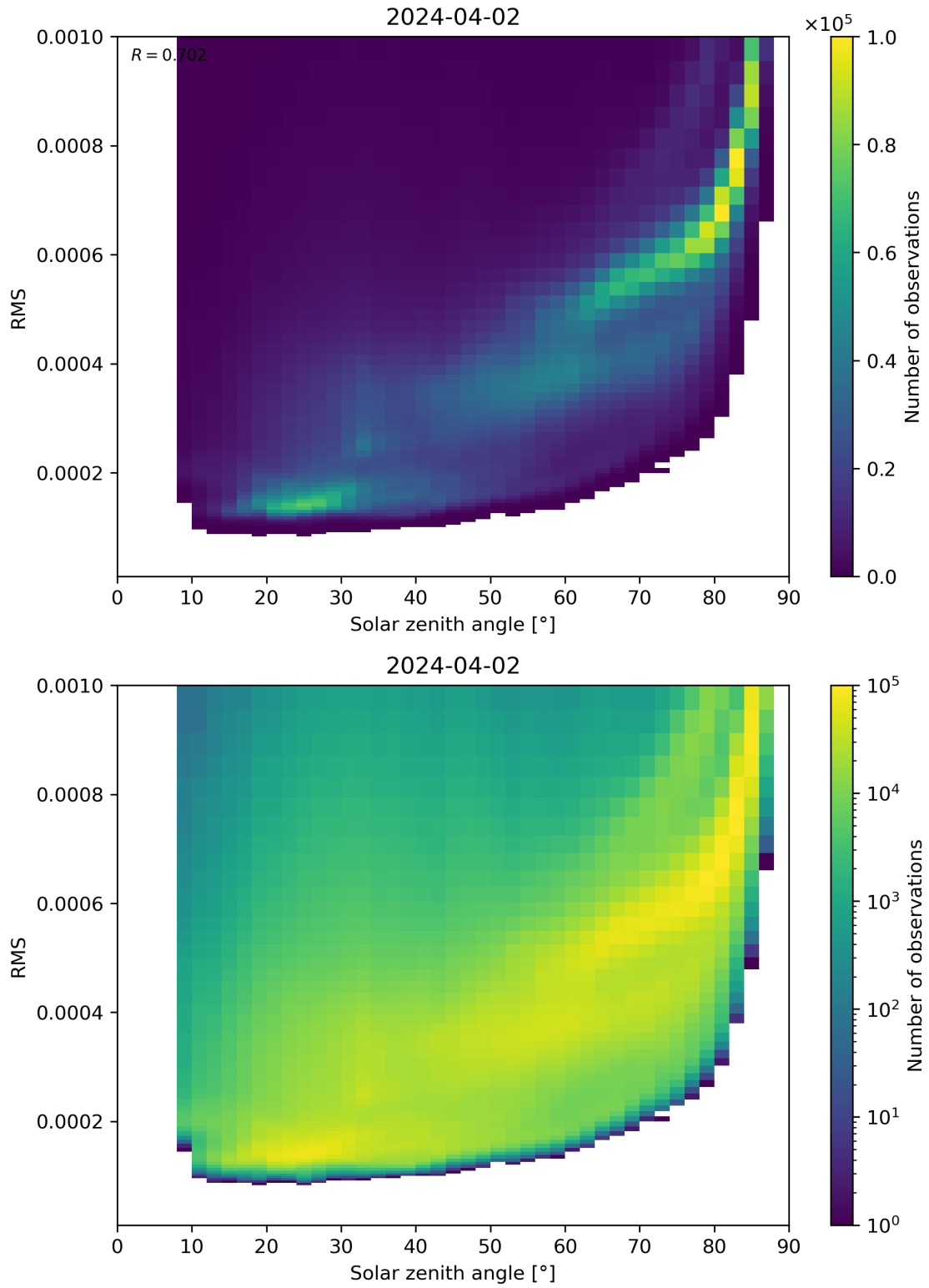
Figure 157: Scatter density plot of “Solar zenith angle” against “RMS” for 2024-04-01 to 2024-04-03.
