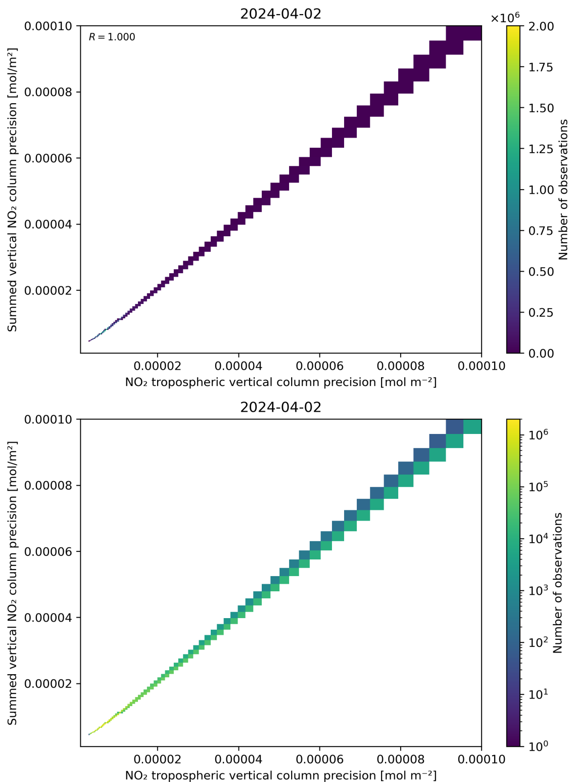
Figure 137: Scatter density plot of “NO 2 tropospheric vertical column precision” against “Summed vertical NO 2 column precision” for 2024-04-01 to 2024-04-03.
