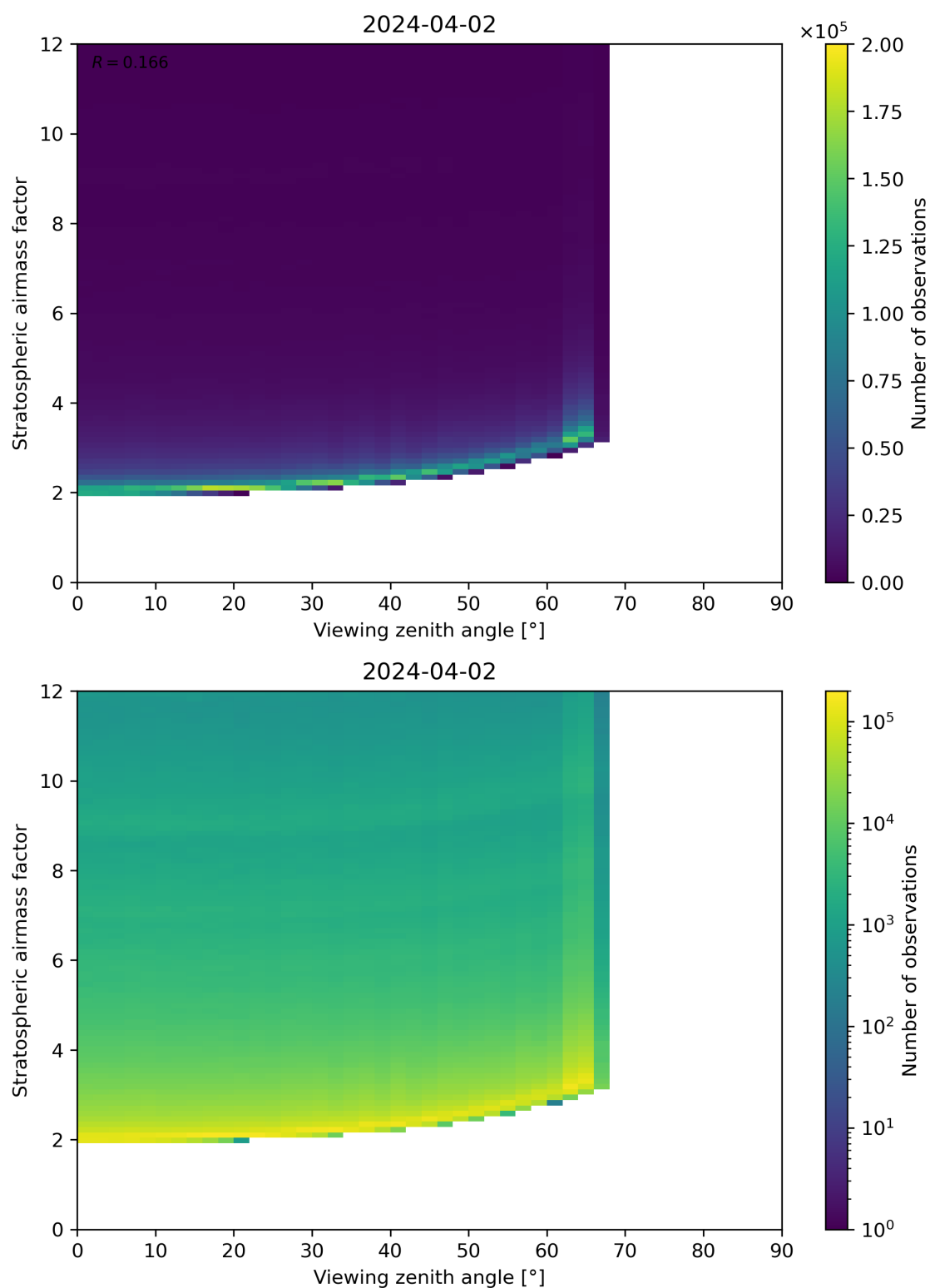
Figure 159: Scatter density plot of “Viewing zenith angle” against “Stratospheric airmass factor” for 2024-04-01 to 2024-04-03.
