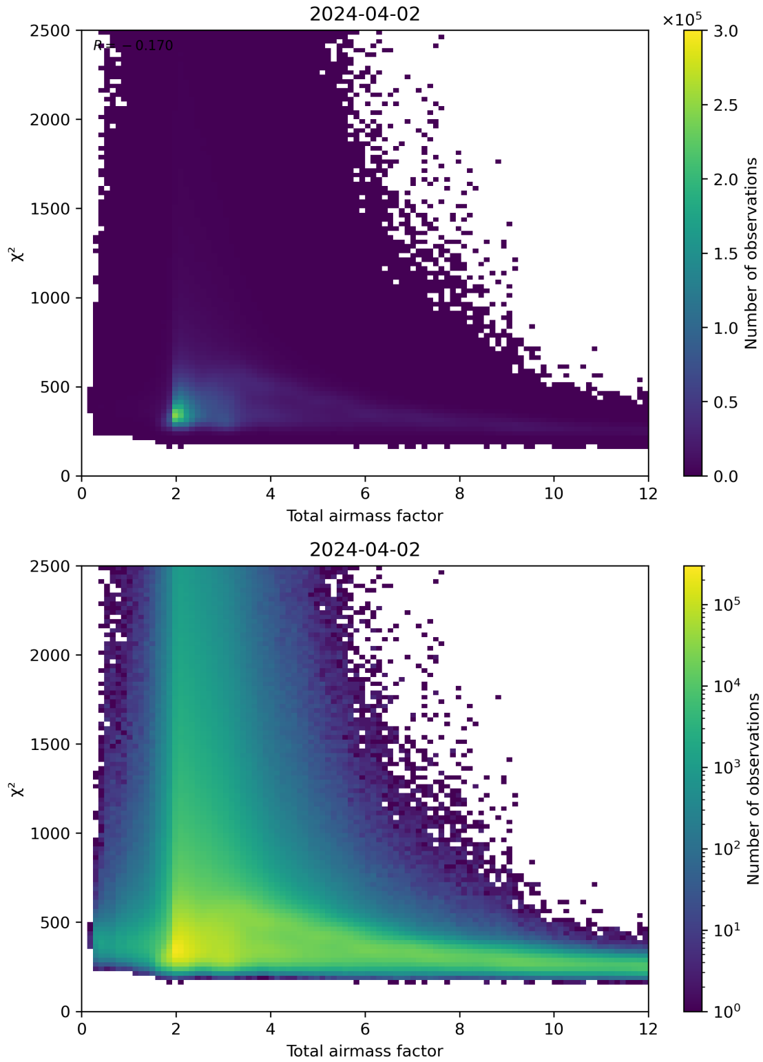
Figure 63: Scatter density plot of “Total airmass factor” against “ \chi^2 ” for 2024-04-01 to 2024-04-03.
