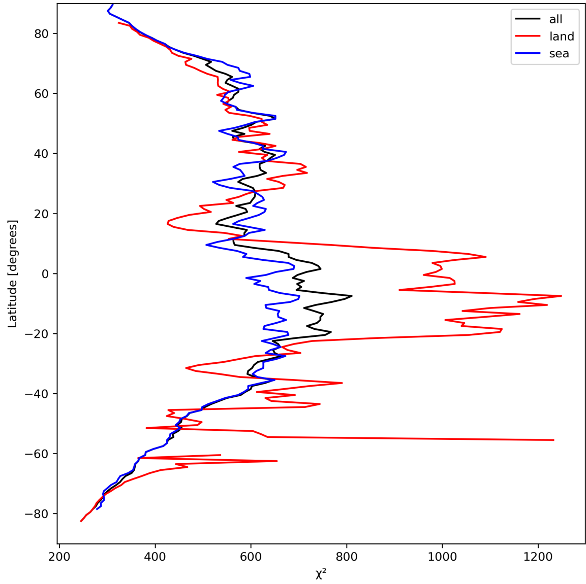
Figure 25: Zonal average of “ \chi^2 ” for 2024-04-01 to 2024-04-03.
