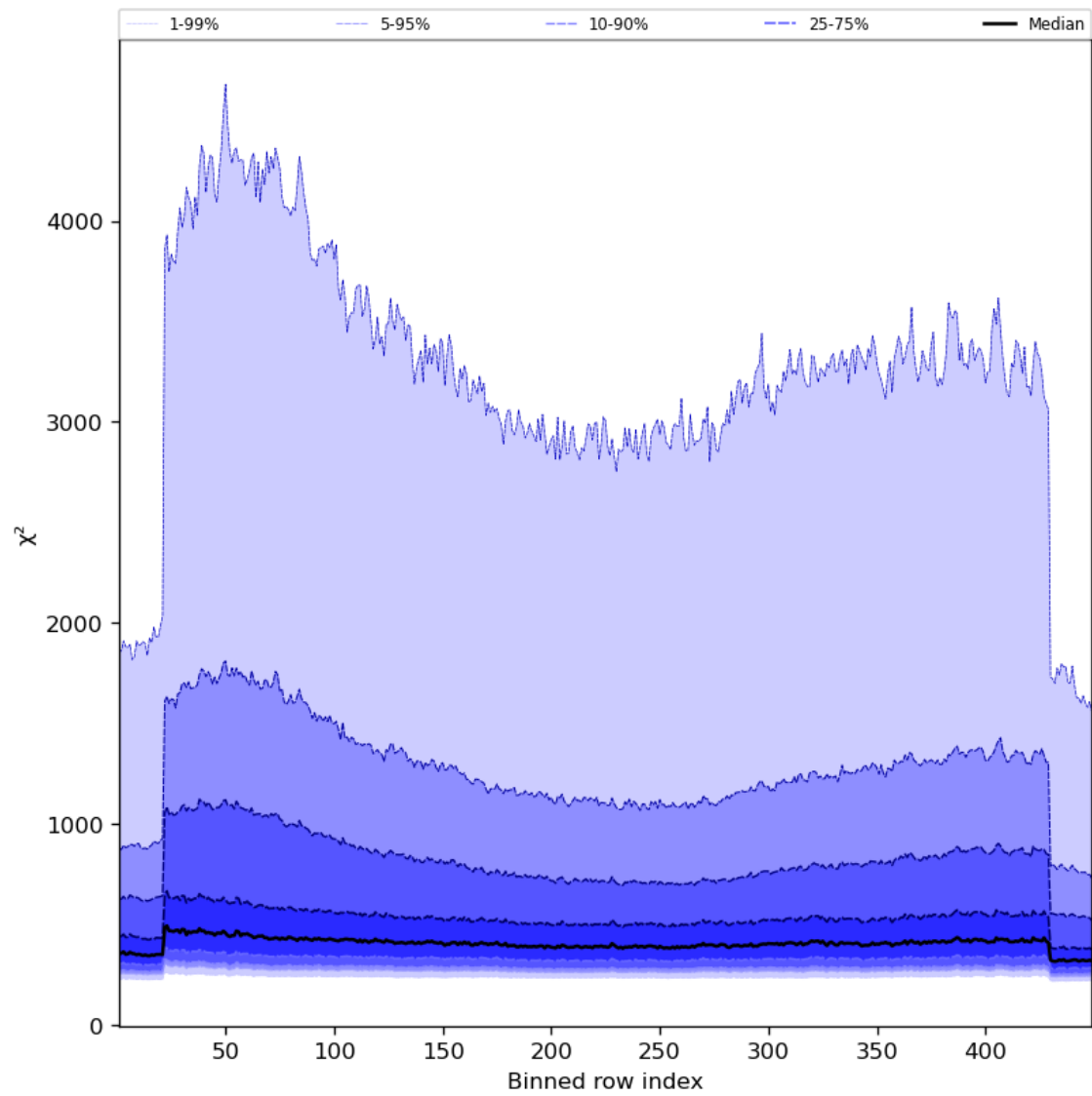
Figure 59: Along track statistics of “ \chi^2 ” for 2024-04-01 to 2024-04-03
