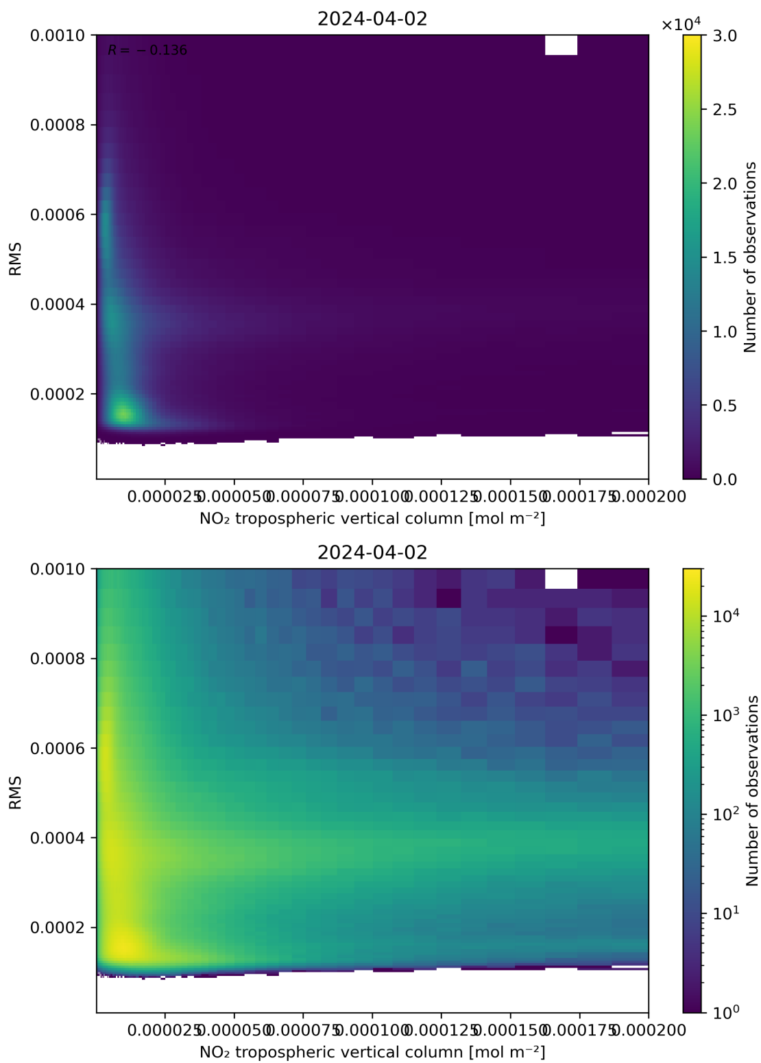
Figure 142: Scatter density plot of “NO 2 tropospheric vertical column” against “RMS” for 2024-04-01 to 2024-04-03.
