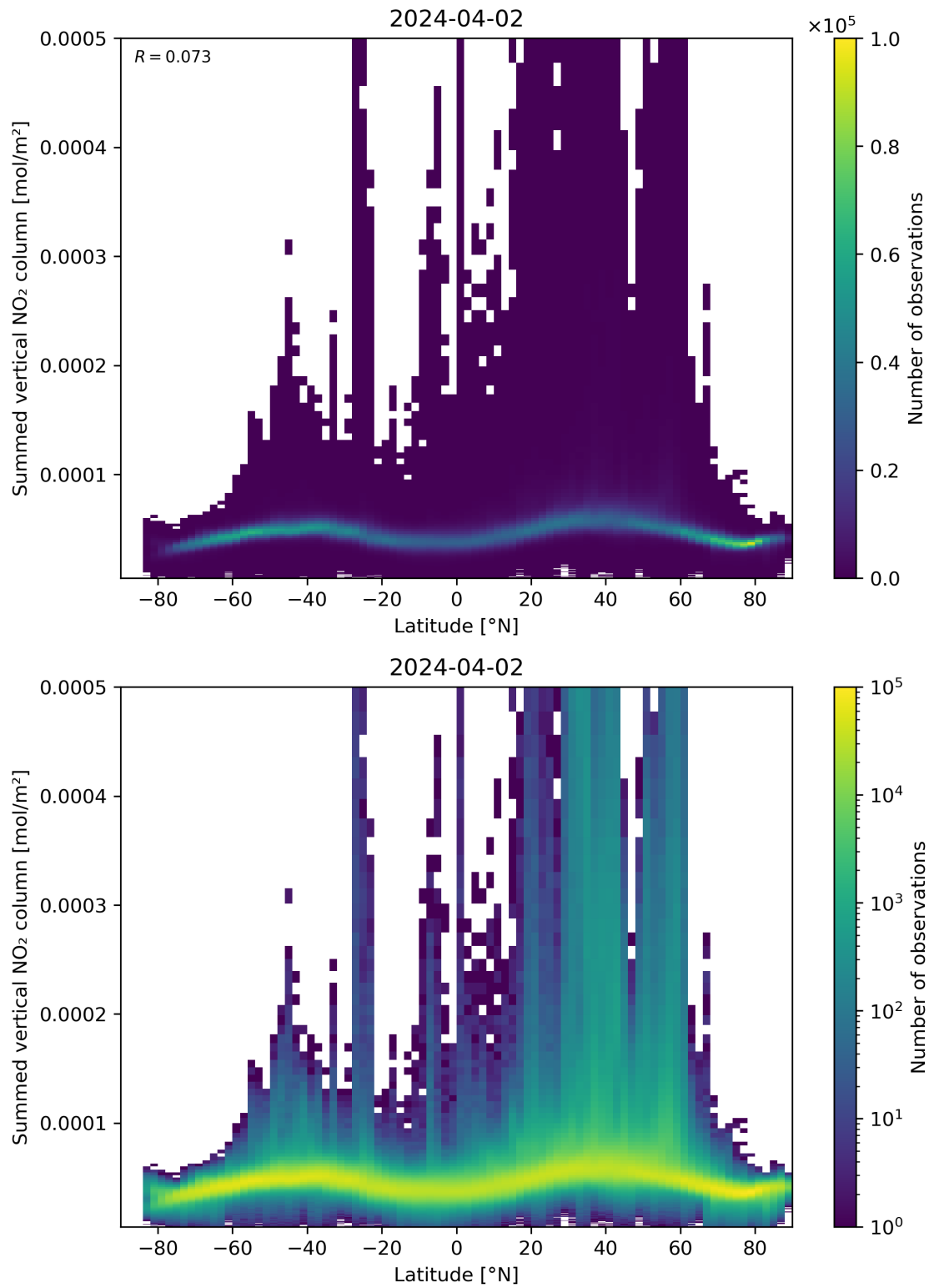
Figure 88: Scatter density plot of “Latitude” against “Summed vertical NO 2 column” for 2024-04-01 to 2024-04-03.
