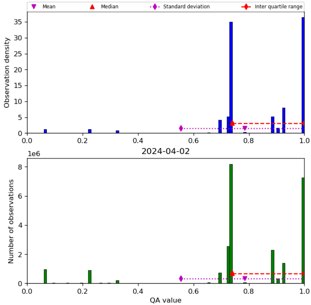
Figure 28: Histogram of “QA value” for 2024-04-01 to 2024-04-03
