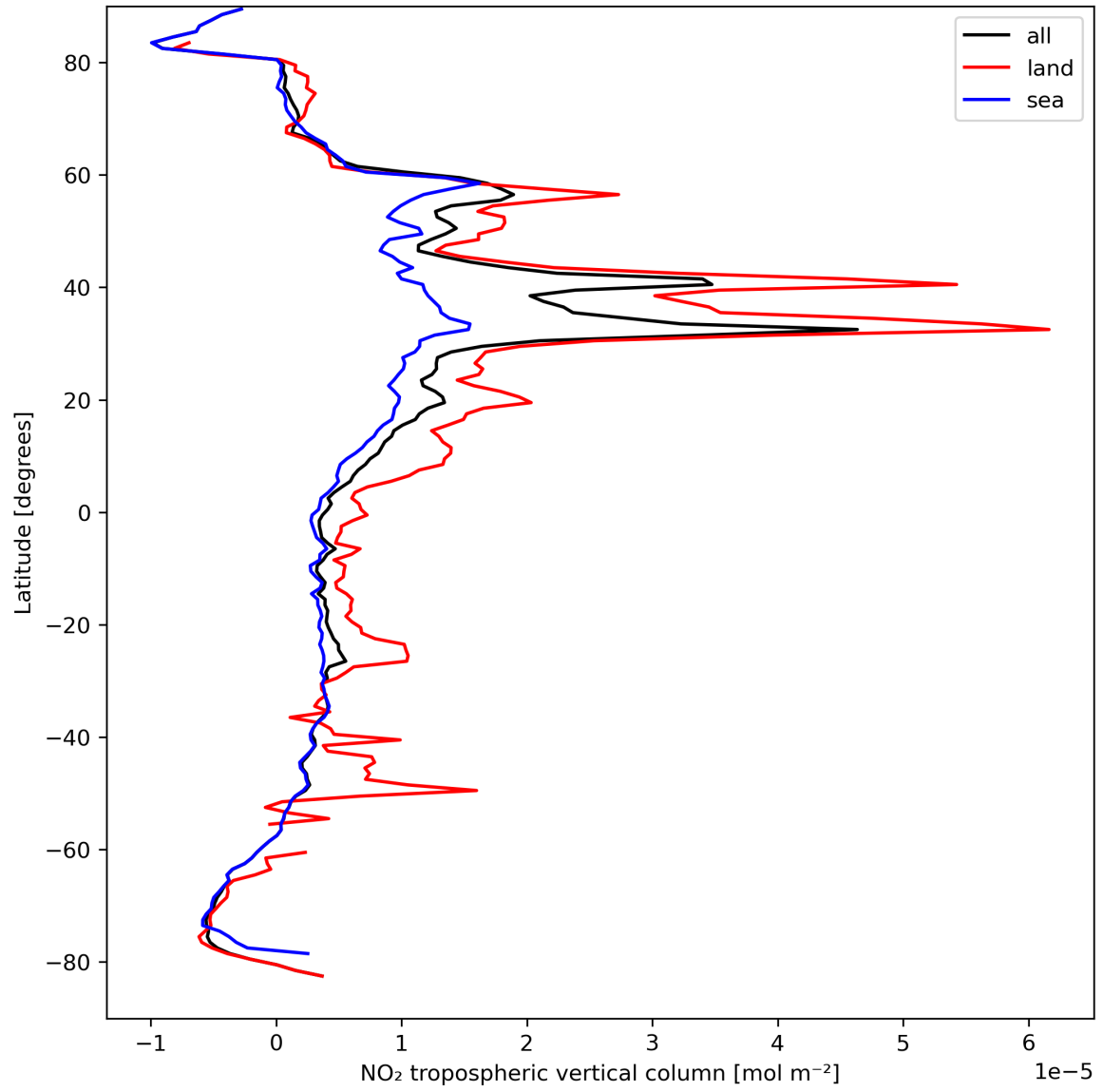
Figure 12: Zonal average of “NO 2 tropospheric vertical column” for 2024-04-01 to 2024-04-03.
