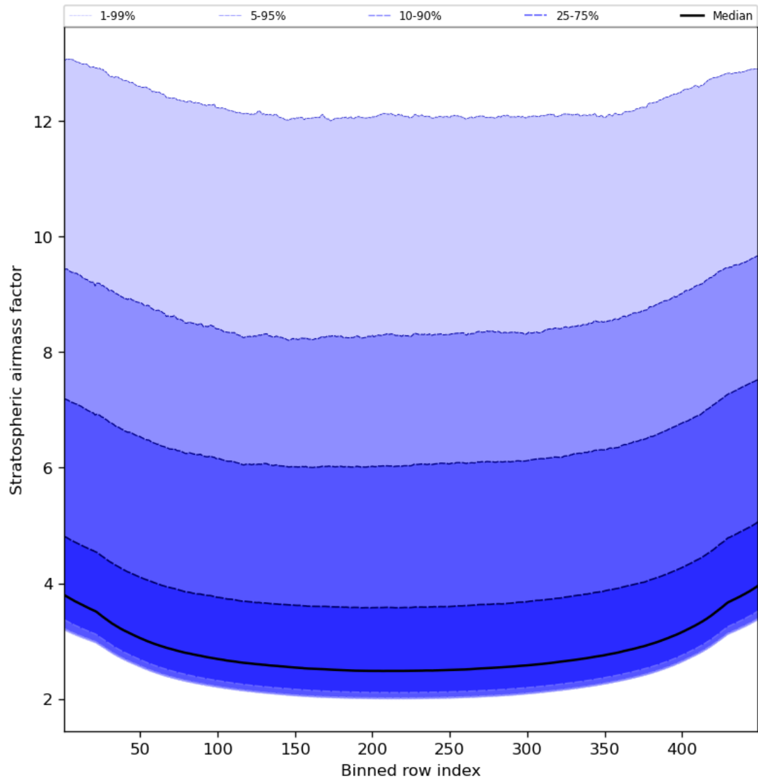
Figure 61: Along track statistics of “Stratospheric air mass factor” for 2024-04-01 to 2024-04-03
