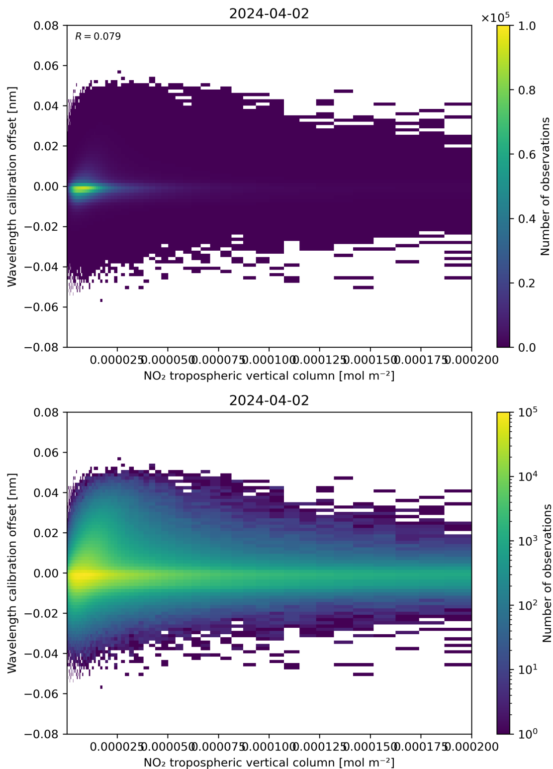
Figure 143: Scatter density plot of “NO 2 tropospheric vertical column” against “Wavelength calibration offset” for 2024-04-01 to 2024-04-03.
