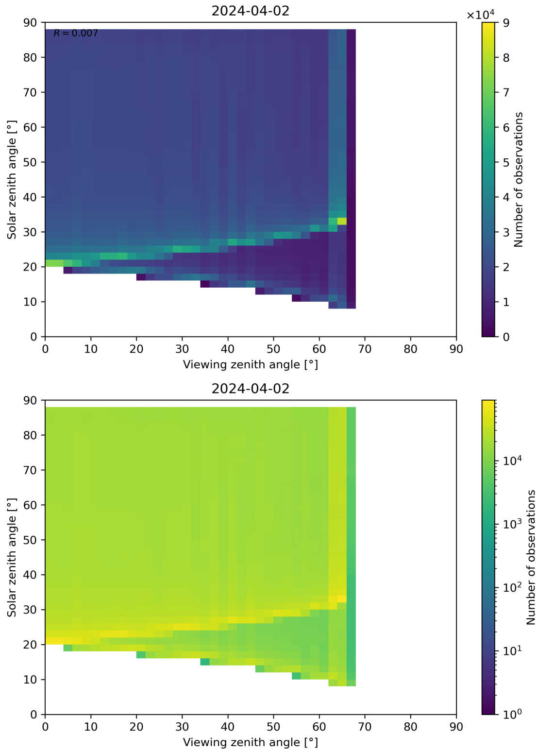
Figure 172: Scatter density plot of “Viewing zenith angle” against “Solar zenith angle” for 2024-04-01 to 2024-04-03.
