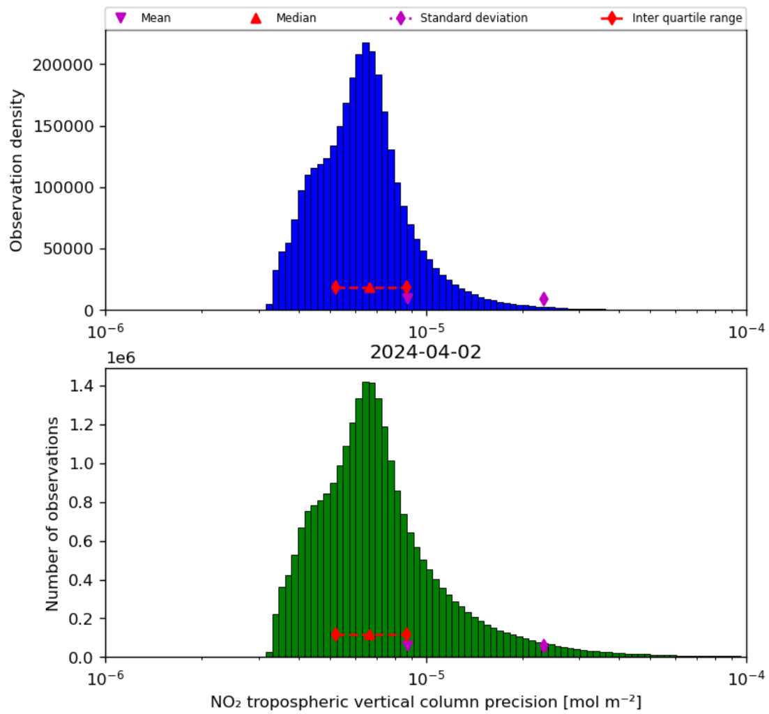
Figure 30: Histogram of “NO 2 tropospheric vertical column precision” for 2024-04-01 to 2024-04-03
