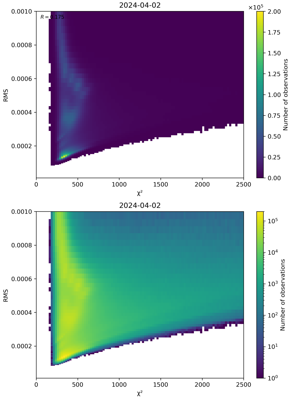
Figure 82: Scatter density plot of “ \chi^2 ” against “RMS” for 2024-04-01 to 2024-04-03.
