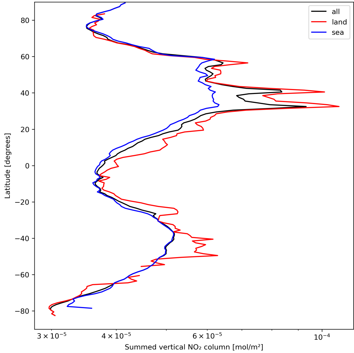
Figure 23: Zonal average of “Summed vertical NO 2 column” for 2024-04-01 to 2024-04-03.
