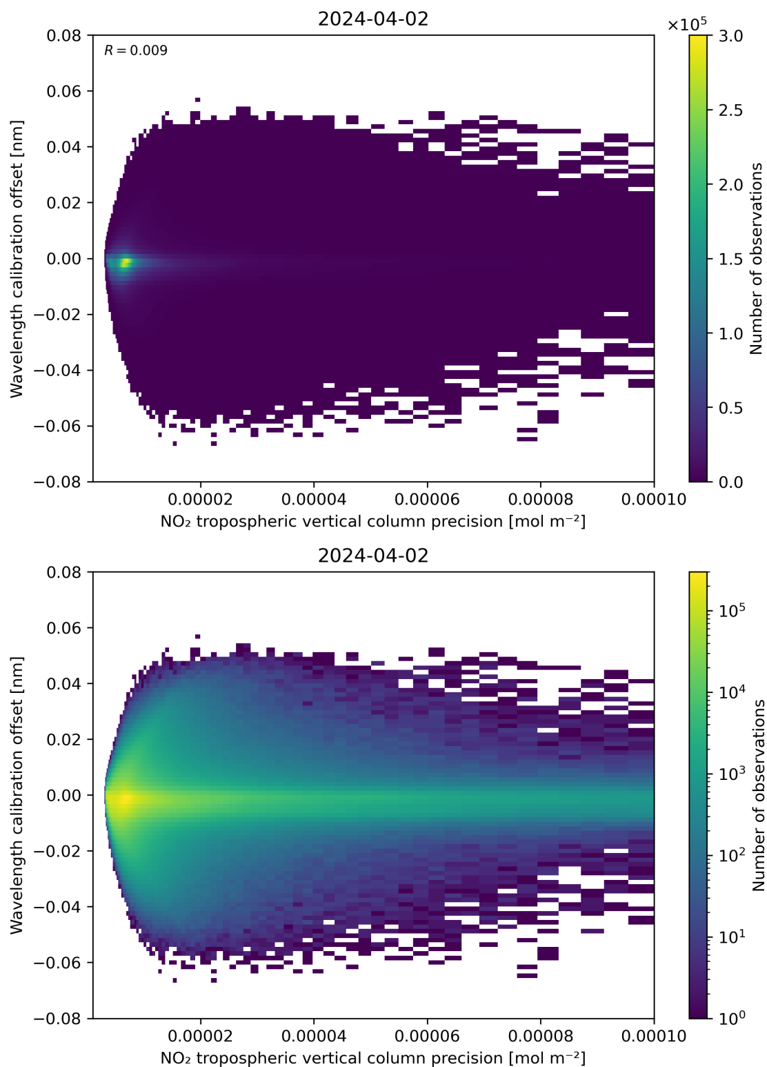
Figure 141: Scatter density plot of “NO 2 tropospheric vertical column precision” against “Wavelength calibration offset” for 2024-04-01 to 2024-04-03.
