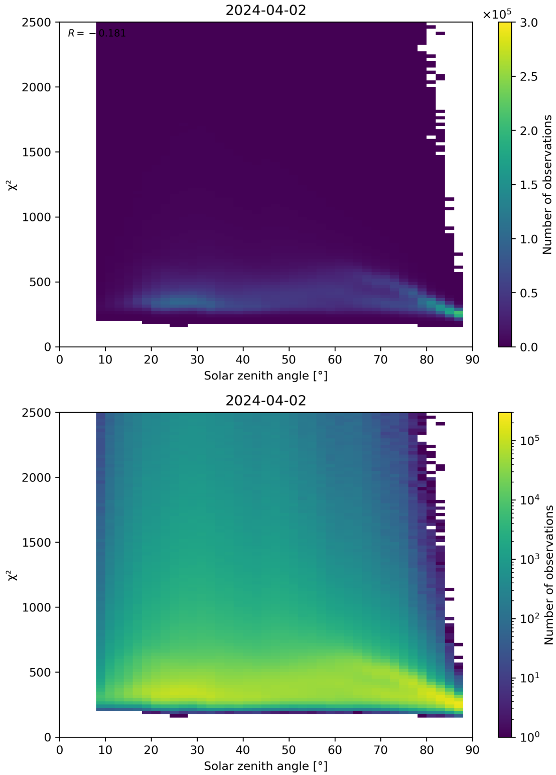
Figure 148: Scatter density plot of “Solar zenith angle” against “ \chi^2 ” for 2024-04-01 to 2024-04-03.
