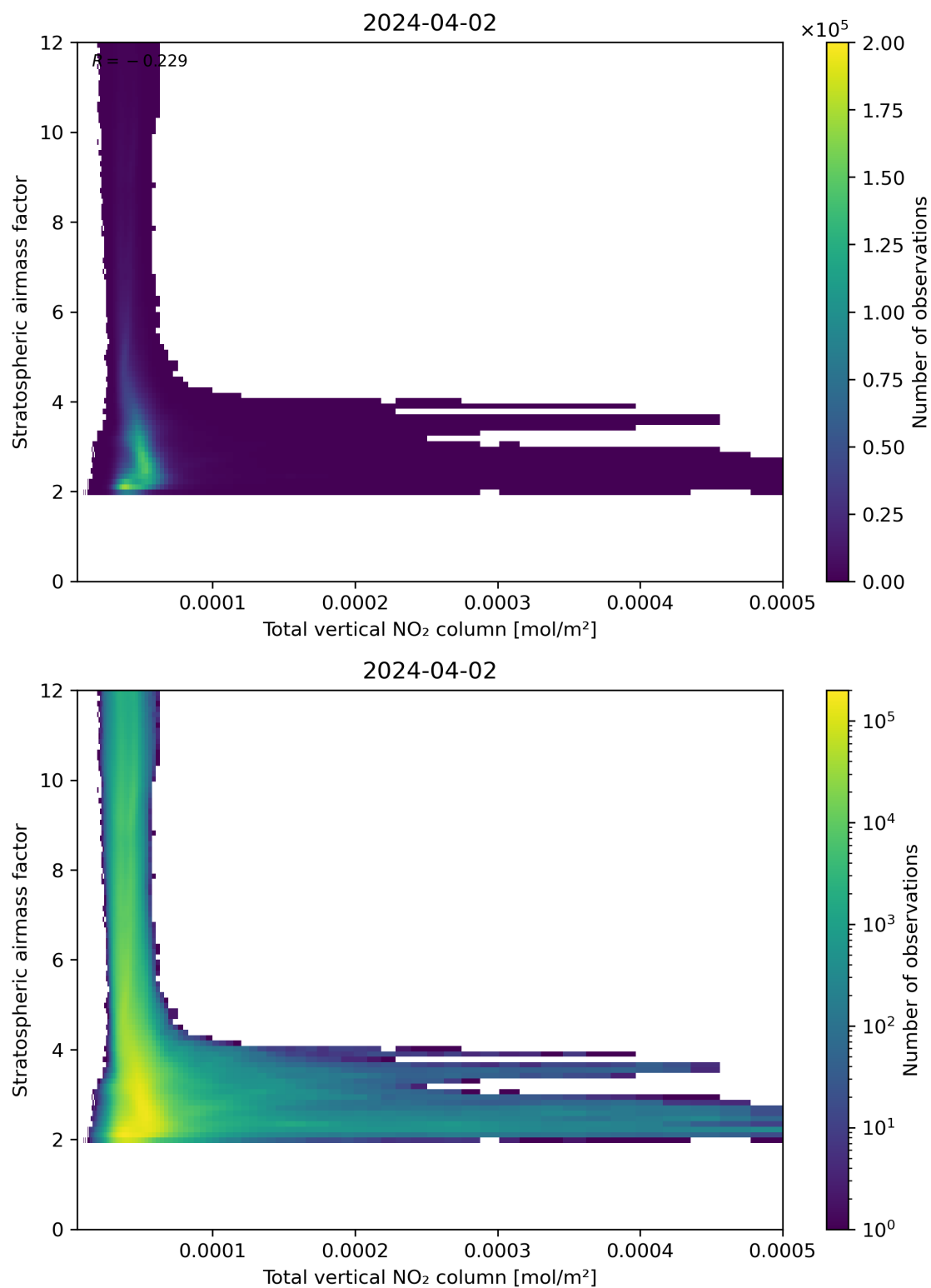
Figure 110: Scatter density plot of “Total vertical NO 2 column” against “Stratospheric airmass factor” for 2024-04-01 to 2024-04-03.
