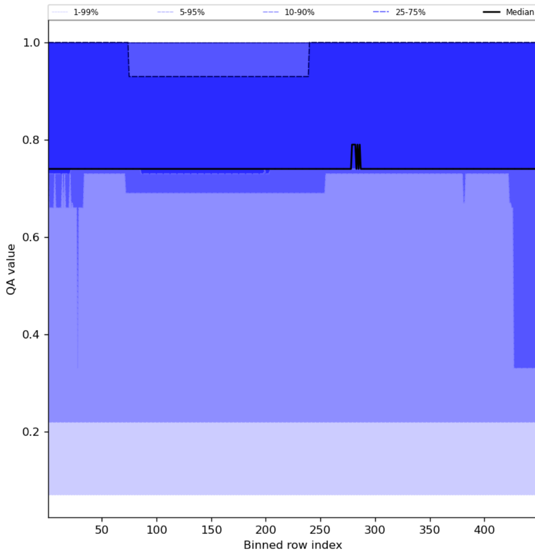
Figure 45: Along track statistics of “QA value” for 2024-04-01 to 2024-04-03
