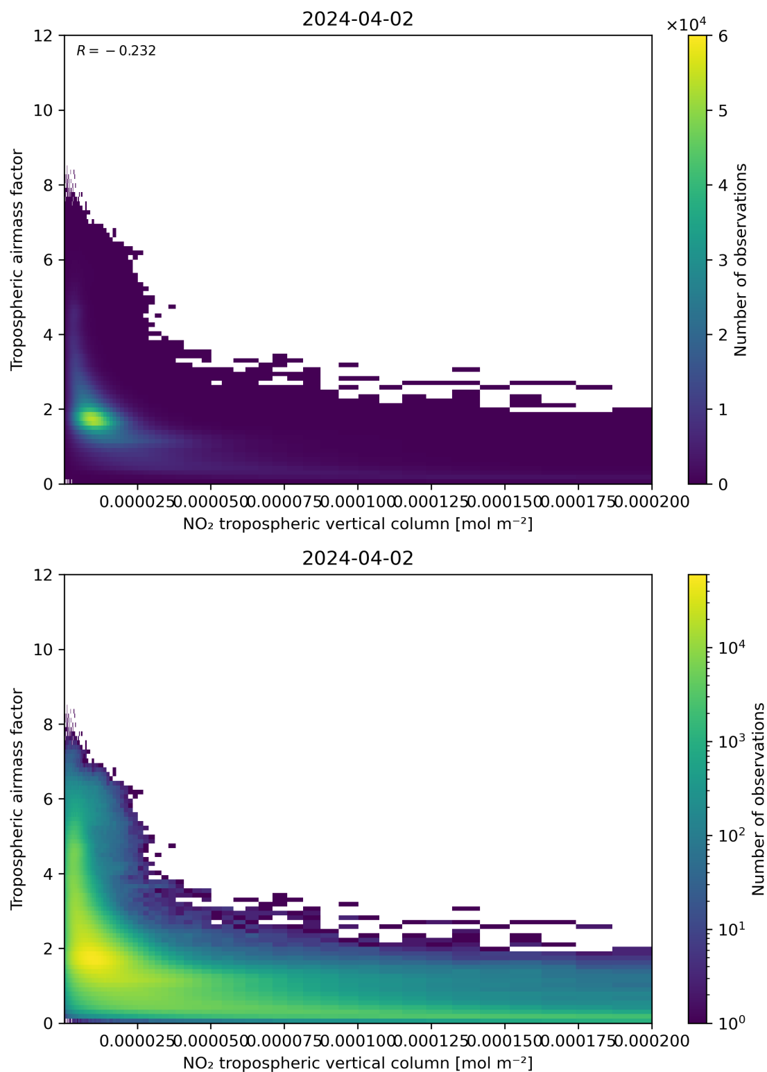
Figure 123: Scatter density plot of “NO 2 tropospheric vertical column” against “Tropospheric air mass factor” for 2024-04-01 to 2024-04-03.
