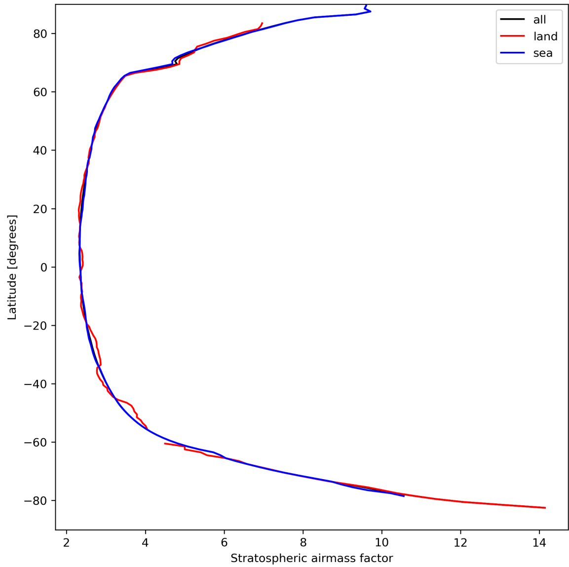
Figure 27: Zonal average of “Stratospheric air mass factor” for 2024-04-01 to 2024-04-03.
