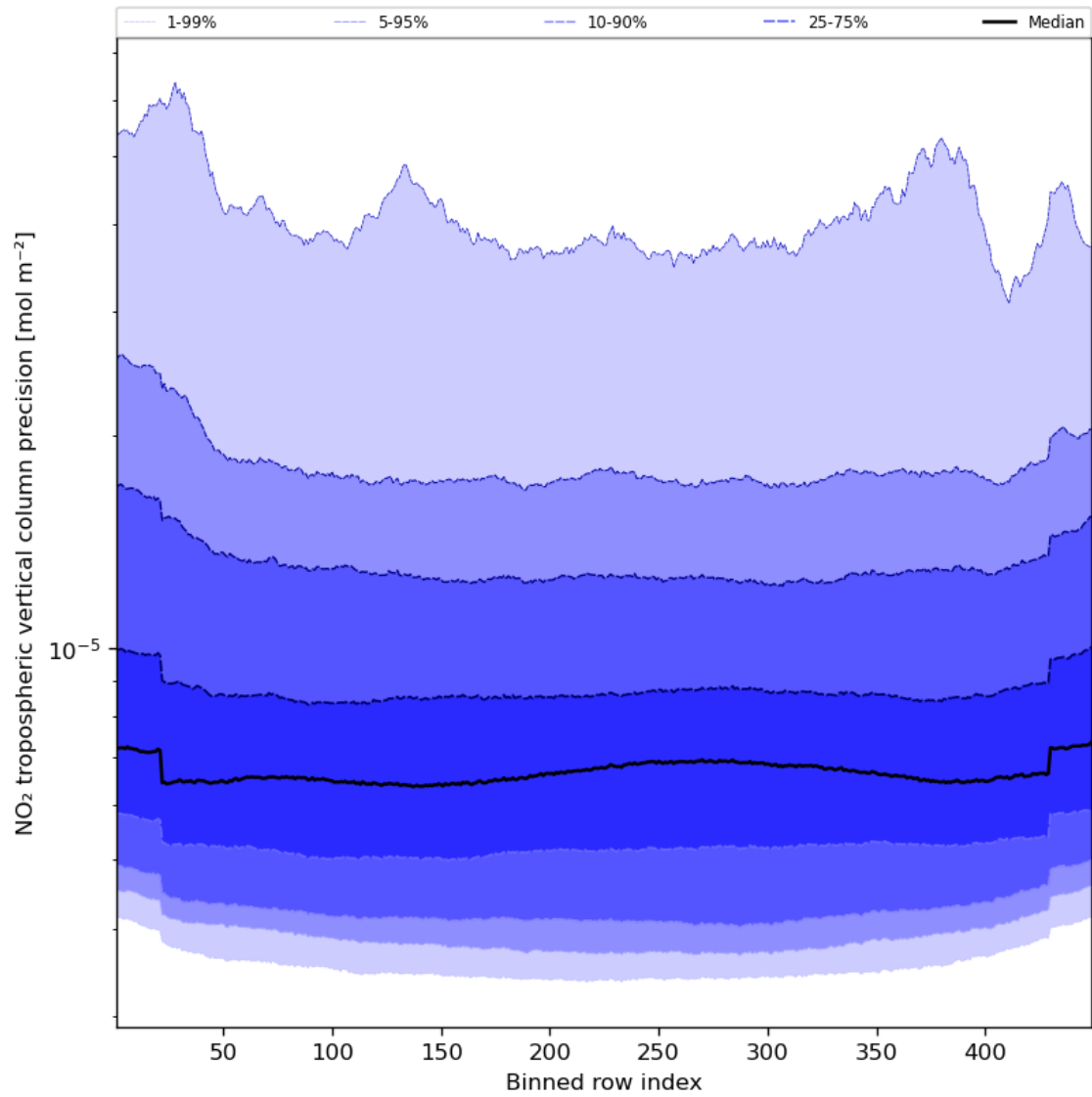
Figure 47: Along track statistics of “NO 2 tropospheric vertical column precision” for 2024-04-01 to 2024-04-03
