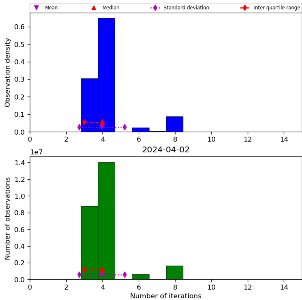
Figure 34: Histogram of “Number of iterations” for 2024-04-01 to 2024-04-03
