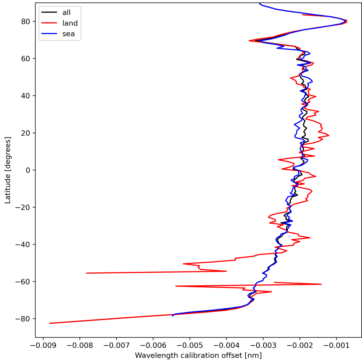
Figure 18: Zonal average of “Wavelength calibration offset” for 2024-04-01 to 2024-04-03.
