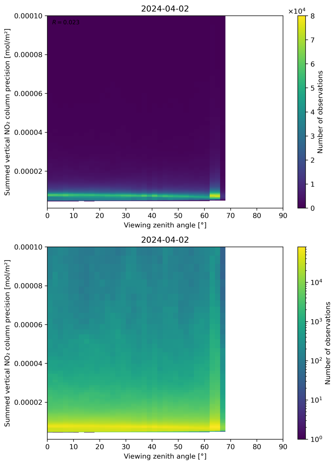
Figure 166: Scatter density plot of “Viewing zenith angle” against “Summed vertical NO 2 column precision” for 2024-04-01 to 2024-04-03.
