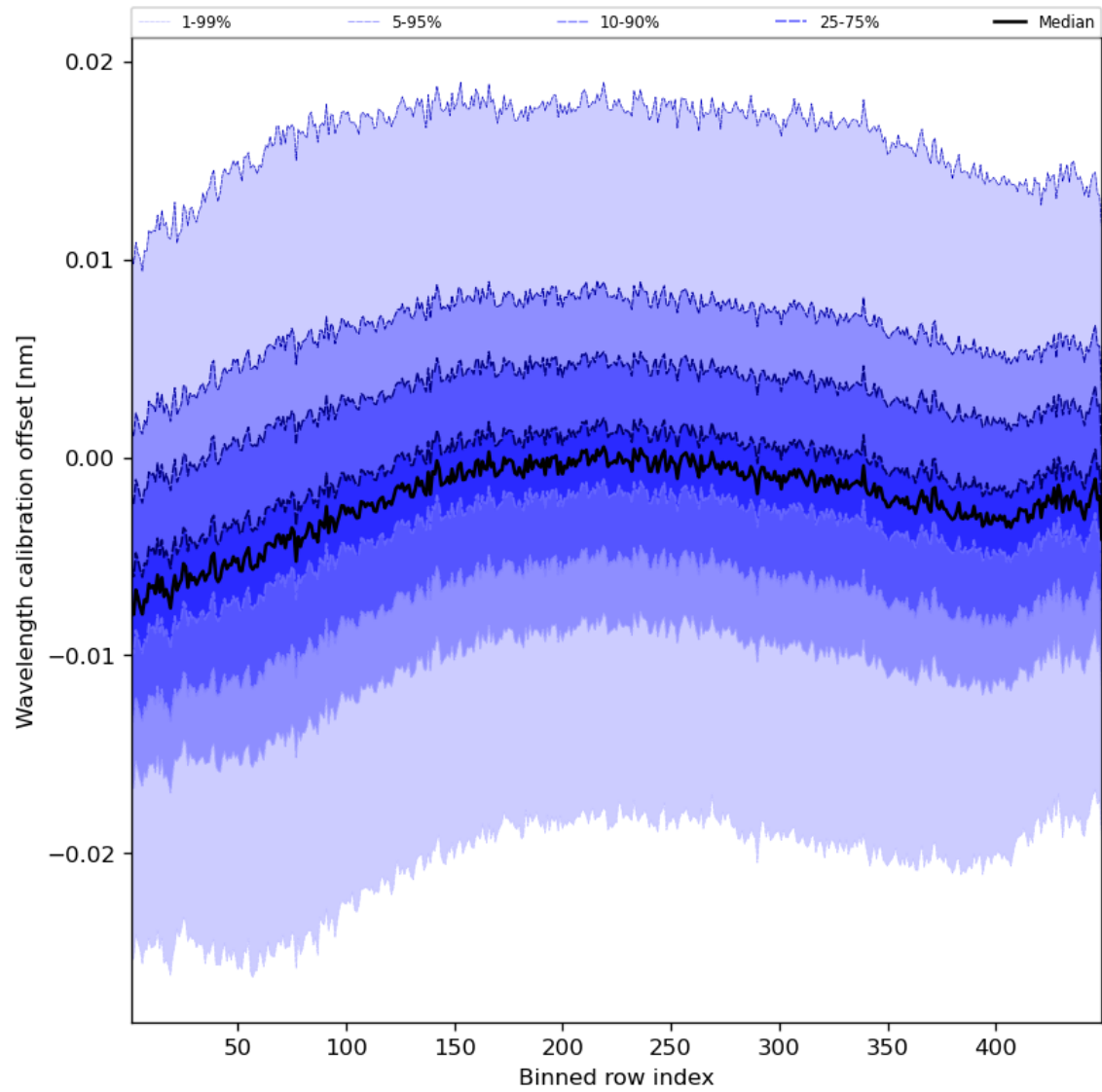
Figure 52: Along track statistics of “Wavelength calibration offset” for 2024-04-01 to 2024-04-03
