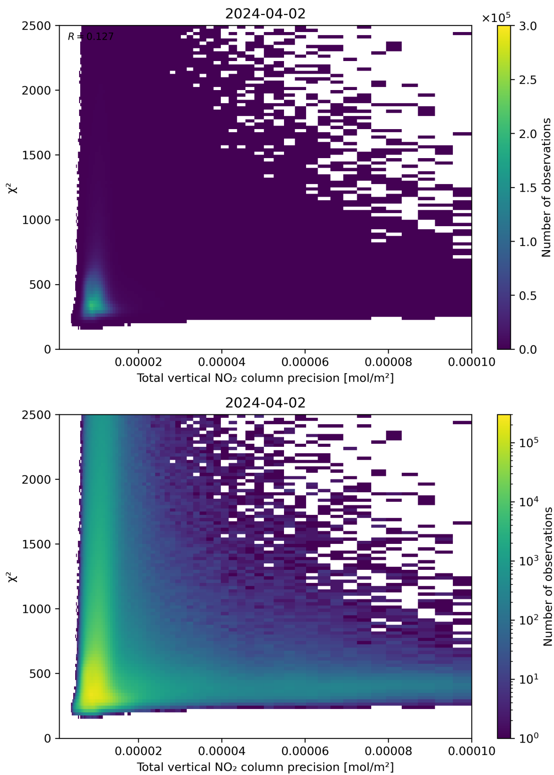
Figure 116: Scatter density plot of “Total vertical NO 2 column precision” against “ \chi^2 ” for 2024-04-01 to 2024-04-03.
