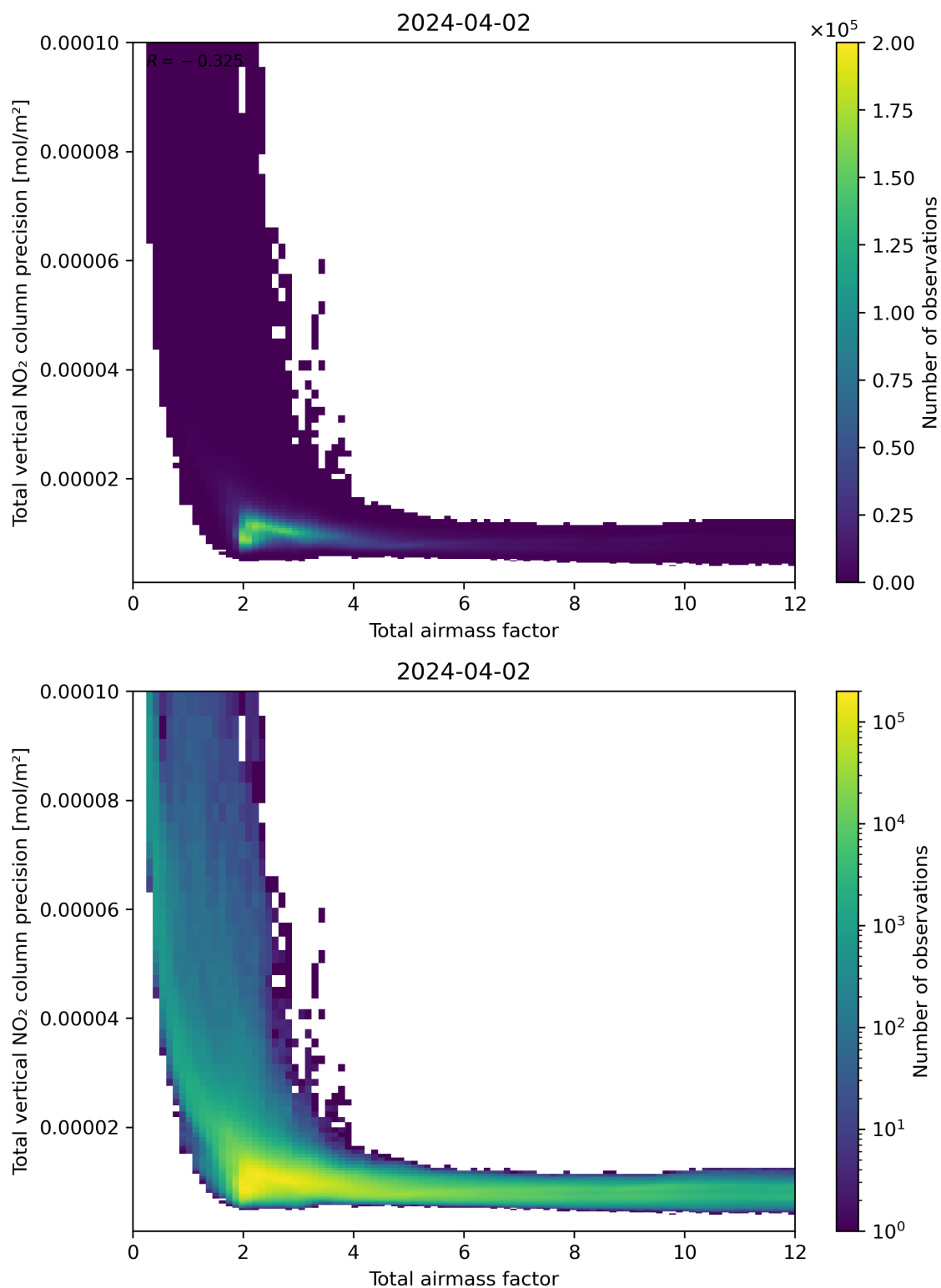
Figure 68: Scatter density plot of “Total airmass factor” against “Total vertical NO 2 column precision” for 2024-04-01 to 2024-04-03.
