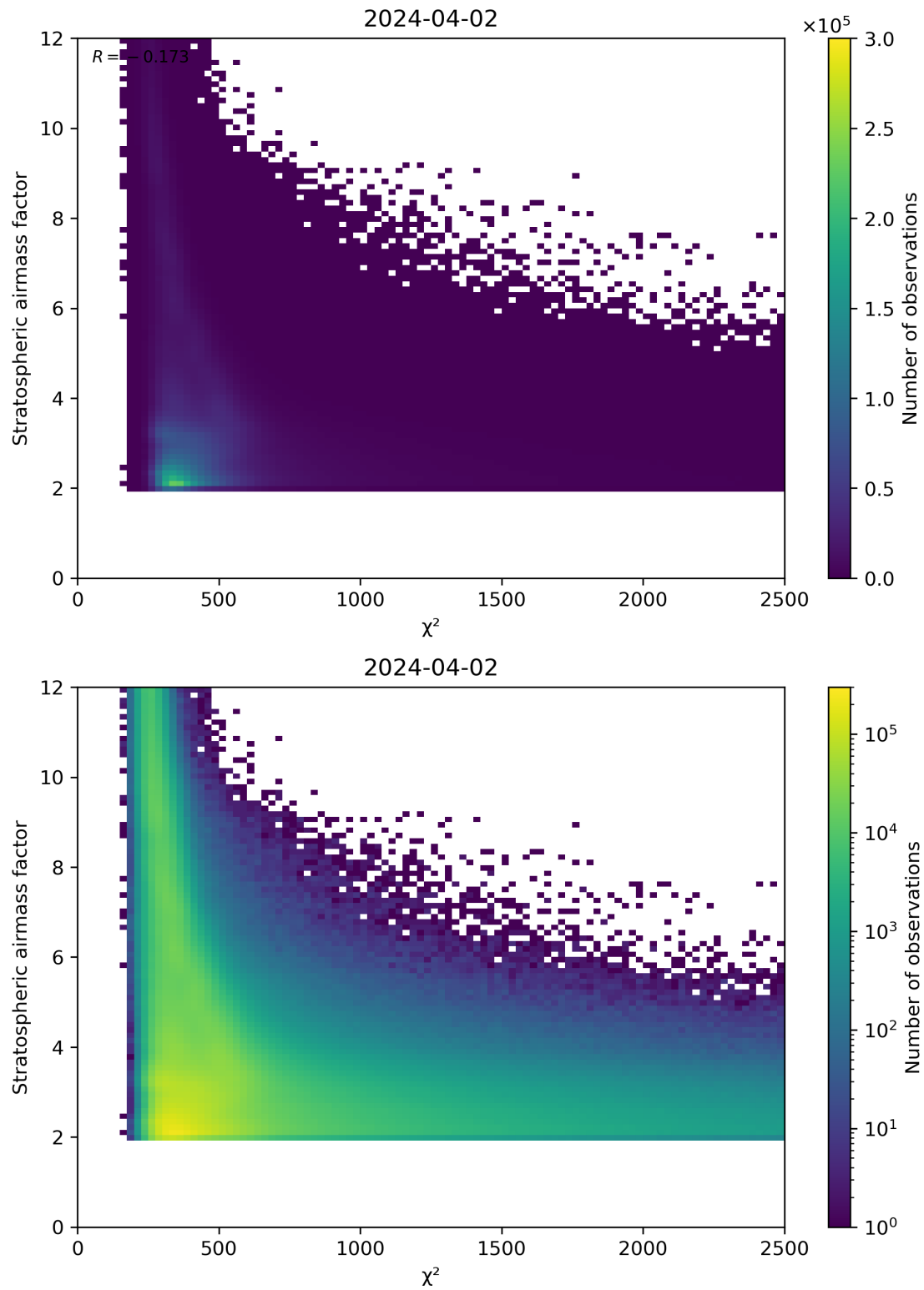
Figure 81: Scatter density plot of “ \chi^2 ” against “Stratospheric airmass factor” for 2024-04-01 to 2024-04-03.
