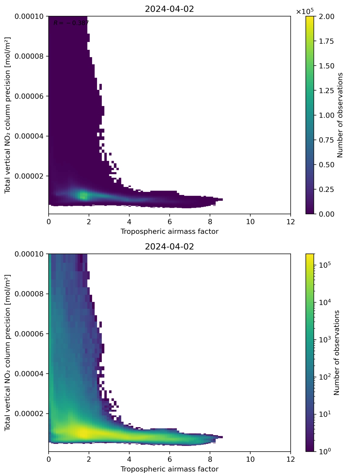
Figure 78: Scatter density plot of “Tropospheric air mass factor” against “Total vertical NO 2 column precision” for 2024-04-01 to 2024-04-03.
