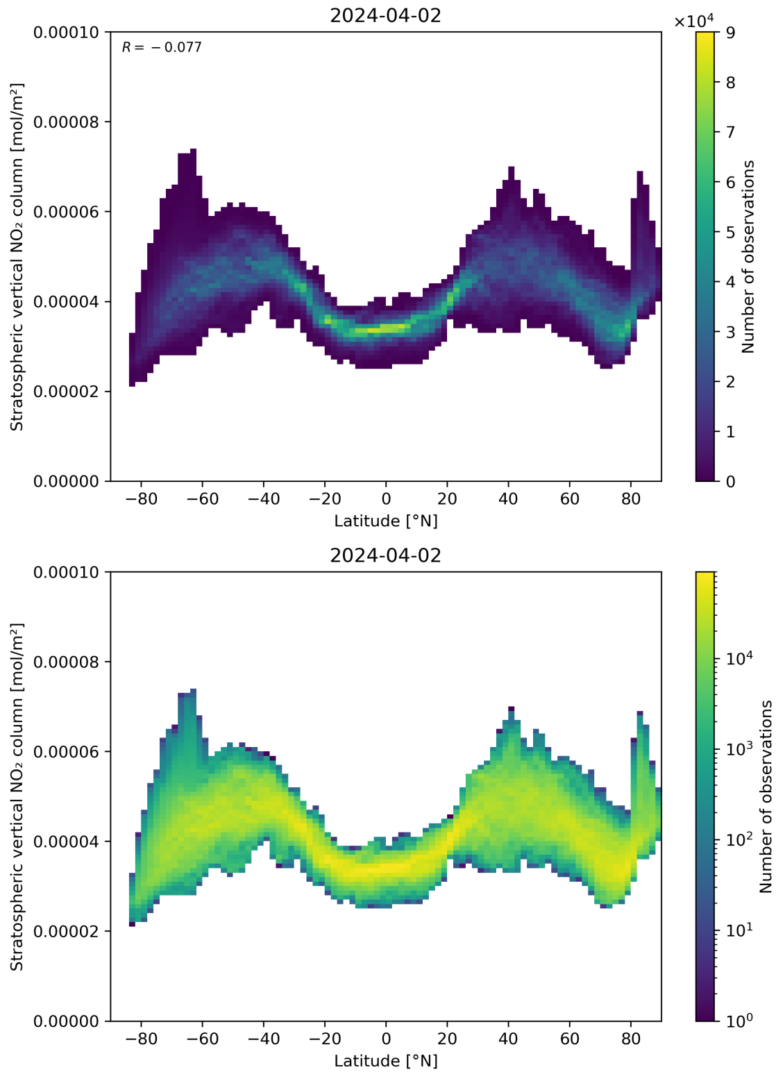
Figure 87: Scatter density plot of “Latitude” against “Stratospheric vertical NO 2 column” for 2024-04-01 to 2024-04-03.
