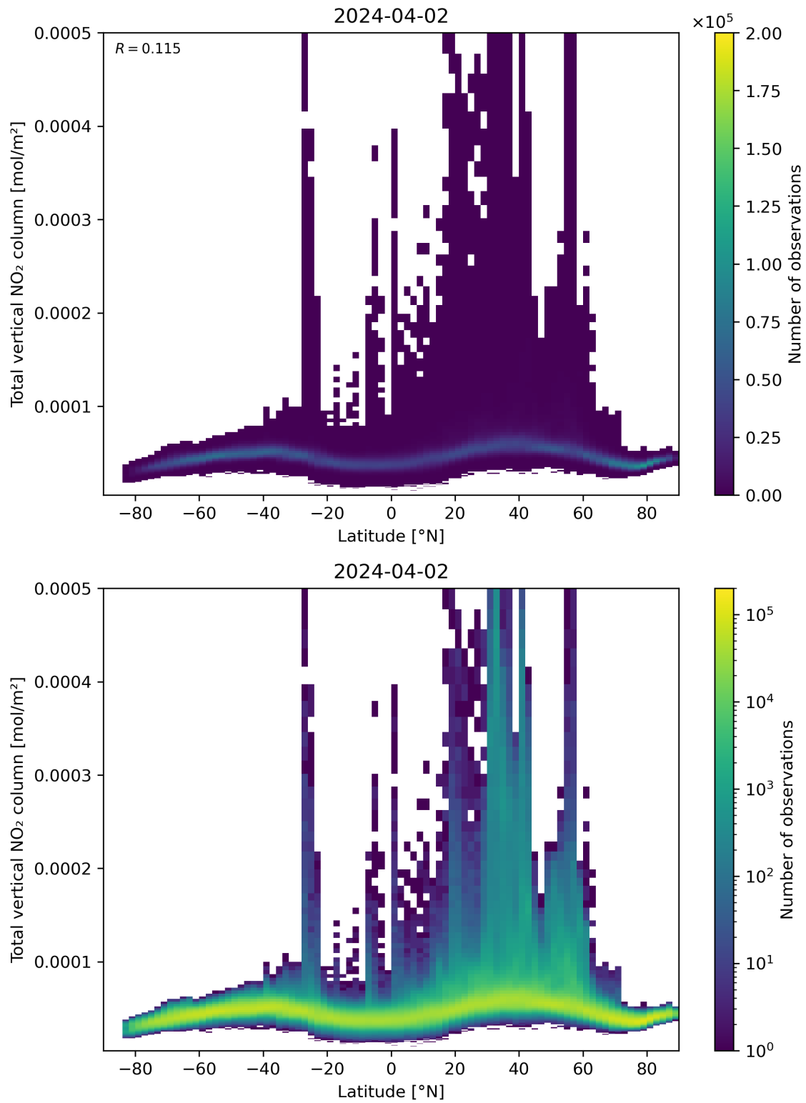
Figure 90: Scatter density plot of “Latitude” against “Total vertical NO 2 column” for 2024-04-01 to 2024-04-03.
