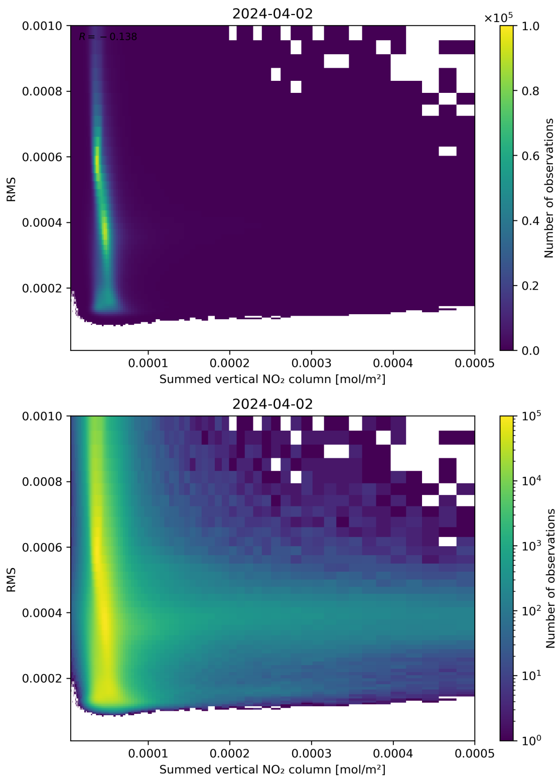
Figure 109: Scatter density plot of “Summed vertical NO 2 column” against “RMS” for 2024-04-01 to 2024-04-03.
