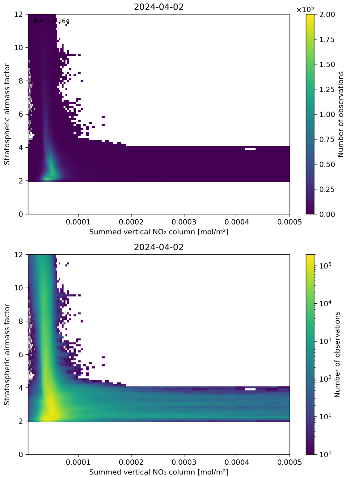
Figure 103: Scatter density plot of “Summed vertical NO 2 column” against “Stratospheric air mass factor” for 2024-04-01 to 2024-04-03.
