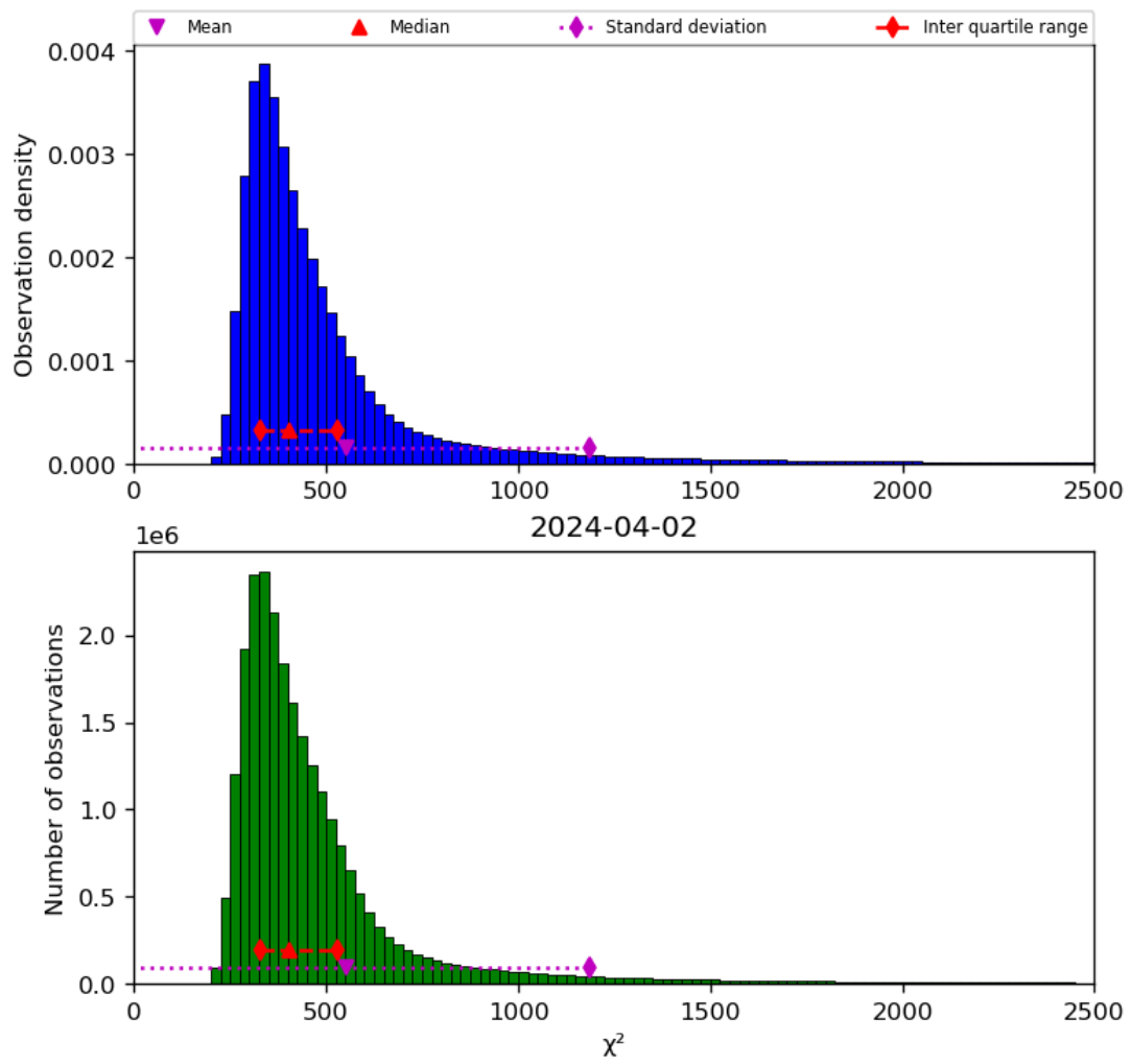
Figure 42: Histogram of “ \chi^2 ” for 2024-04-01 to 2024-04-03
