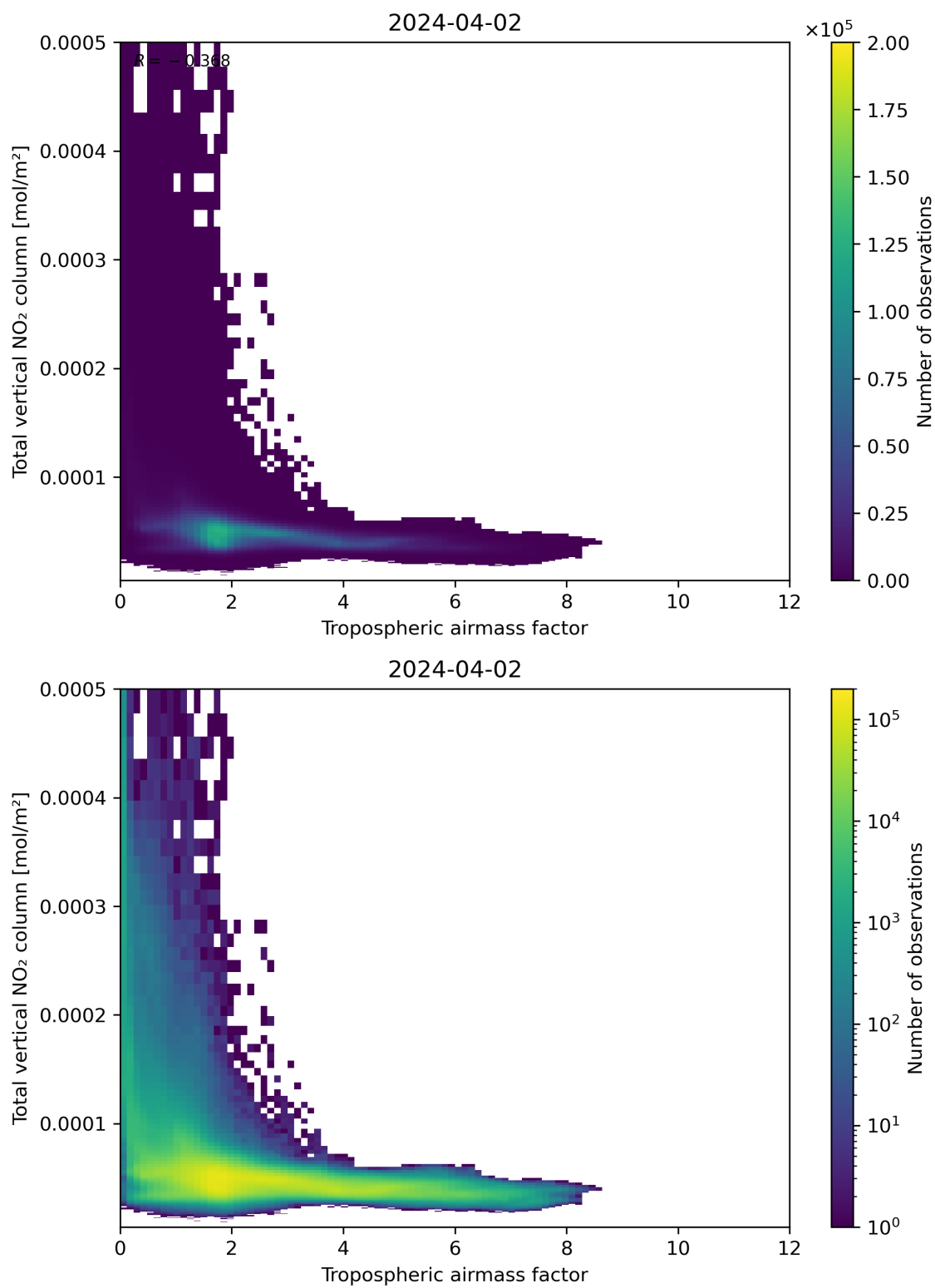
Figure 77: Scatter density plot of “Tropospheric airmass factor” against “Total vertical NO 2 column” for 2024-04-01 to 2024-04-03.
