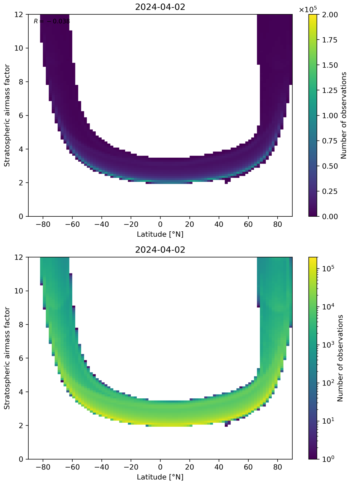
Figure 83: Scatter density plot of “Latitude” against “Stratospheric air mass factor” for 2024-04-01 to 2024-04-03.
