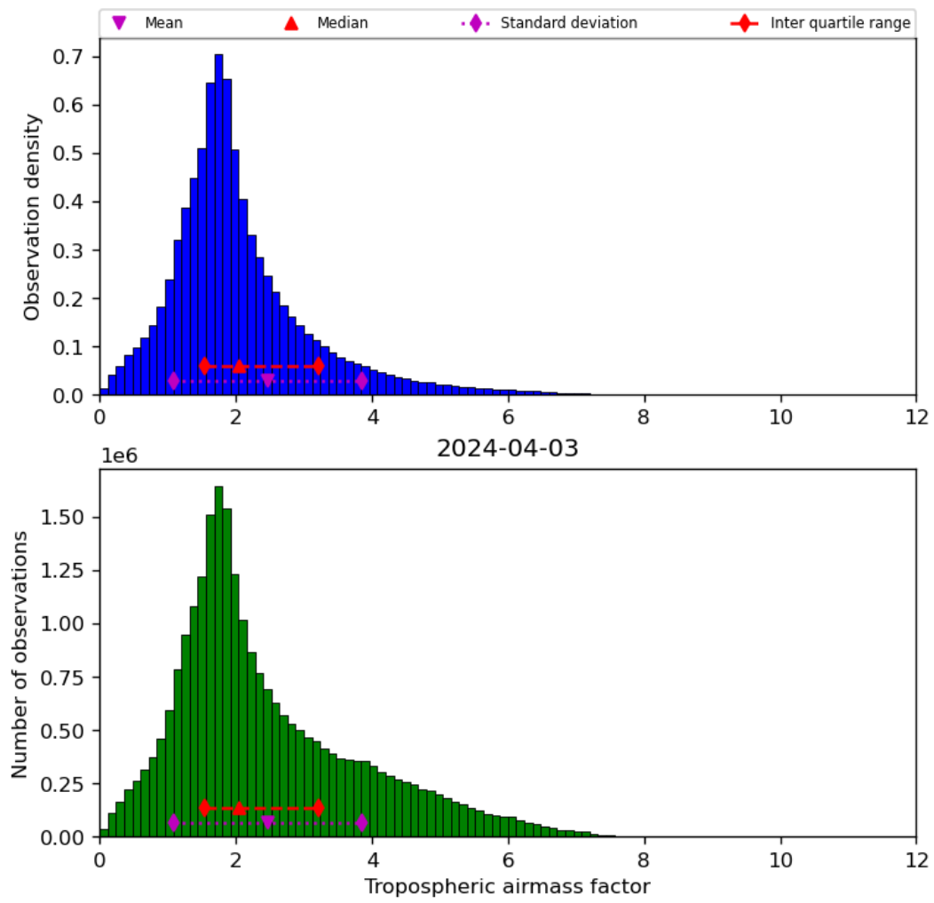
Figure 31: Histogram of “Tropospheric airmass factor” for 2024-04-02 to 2024-04-04
