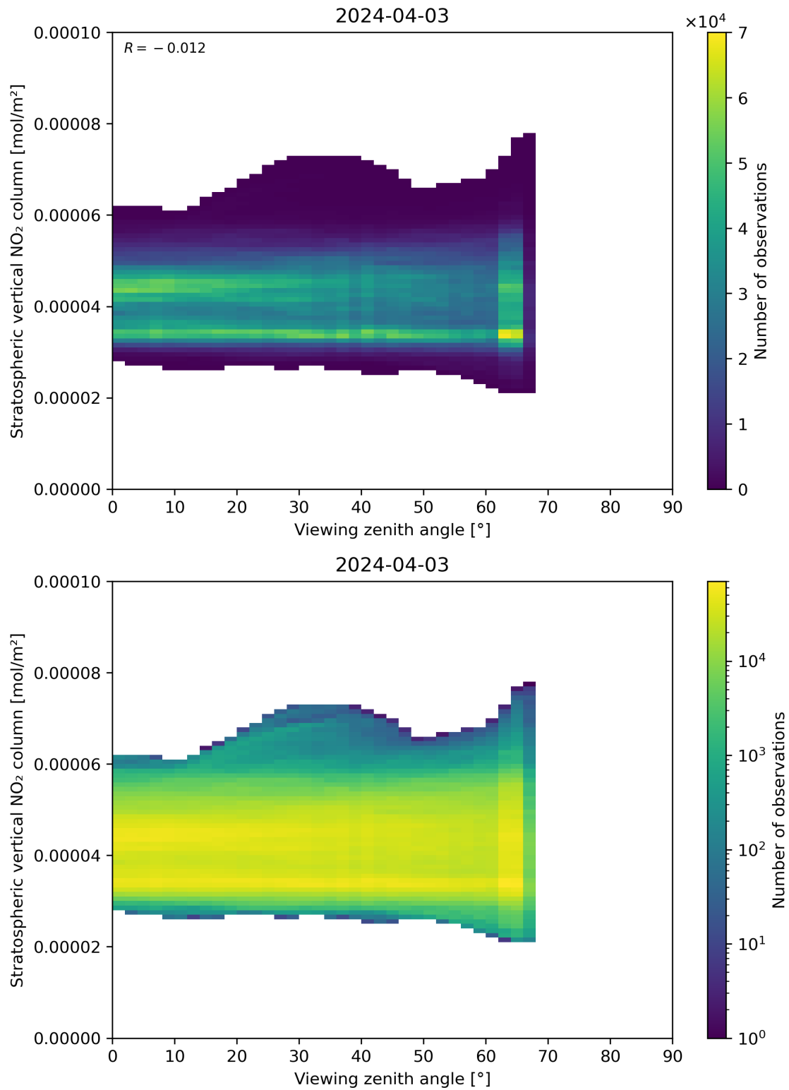
Figure 164: Scatter density plot of “Viewing zenith angle” against “Stratospheric vertical NO 2 column” for 2024-04-02 to 2024-04-04.
