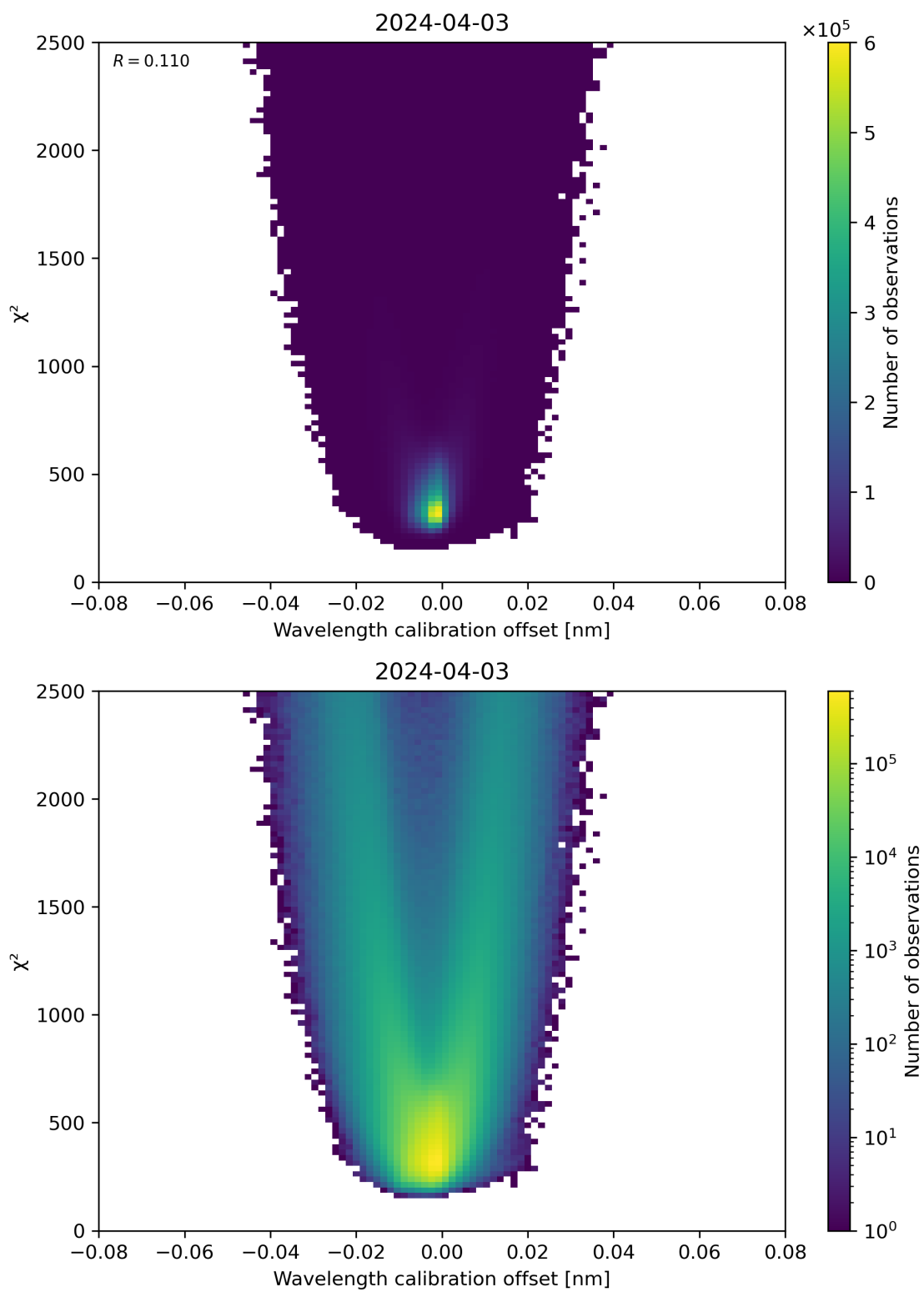
Figure 175: Scatter density plot of “Wavelength calibration offset” against “ \chi^2 ” for 2024-04-02 to 2024-04-04.
