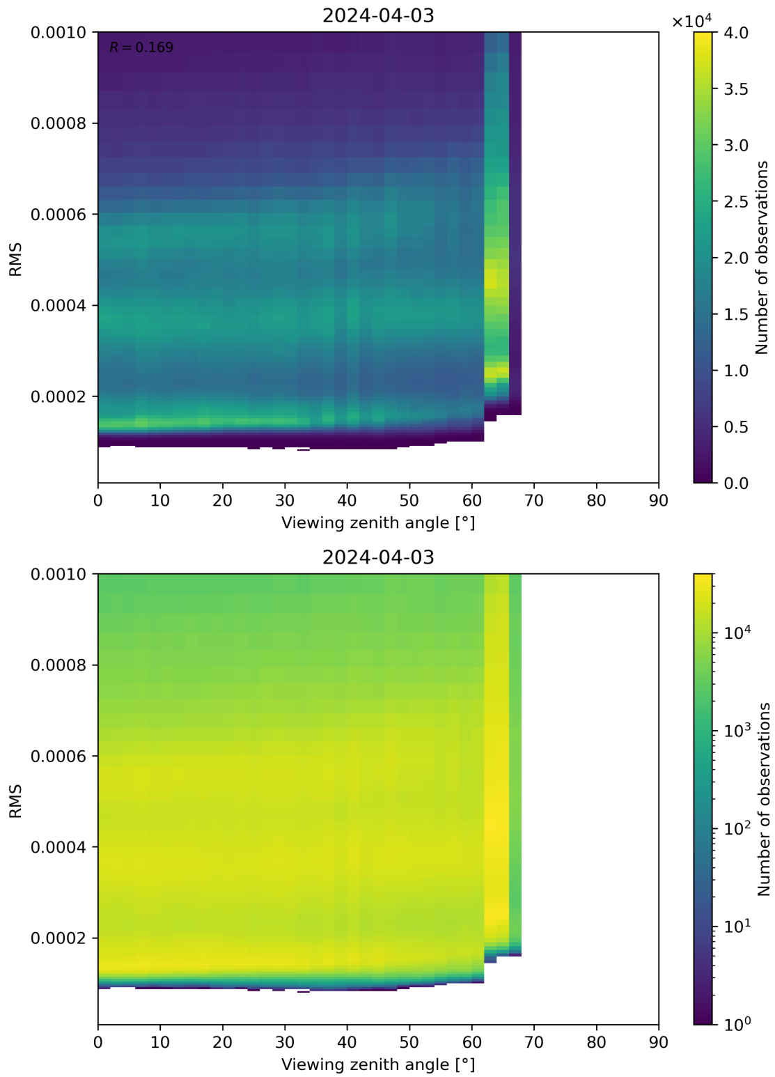
Figure 171: Scatter density plot of “Viewing zenith angle” against “RMS” for 2024-04-02 to 2024-04-04.
