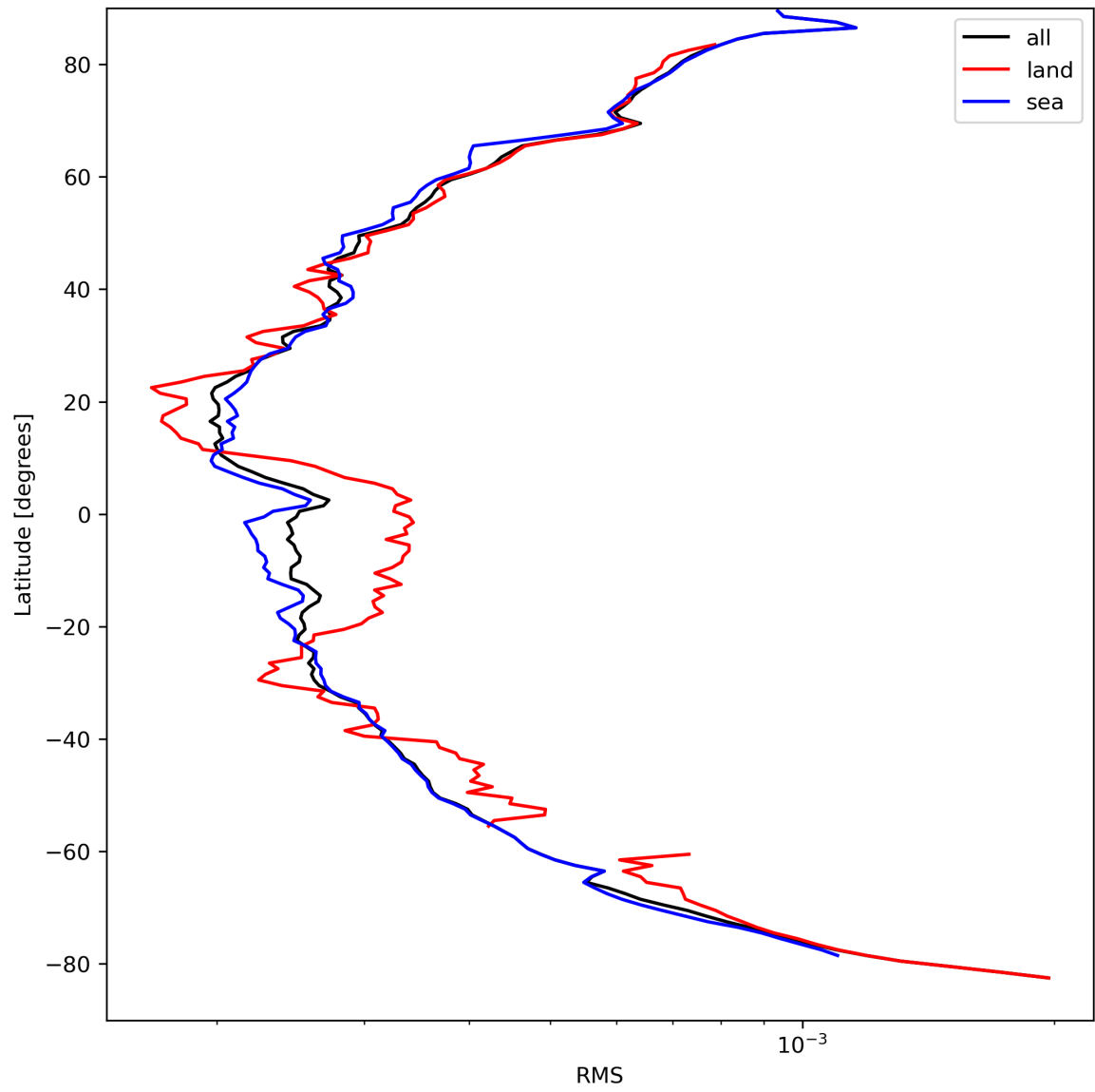
Figure 26: Zonal average of “RMS” for 2024-04-02 to 2024-04-04.
