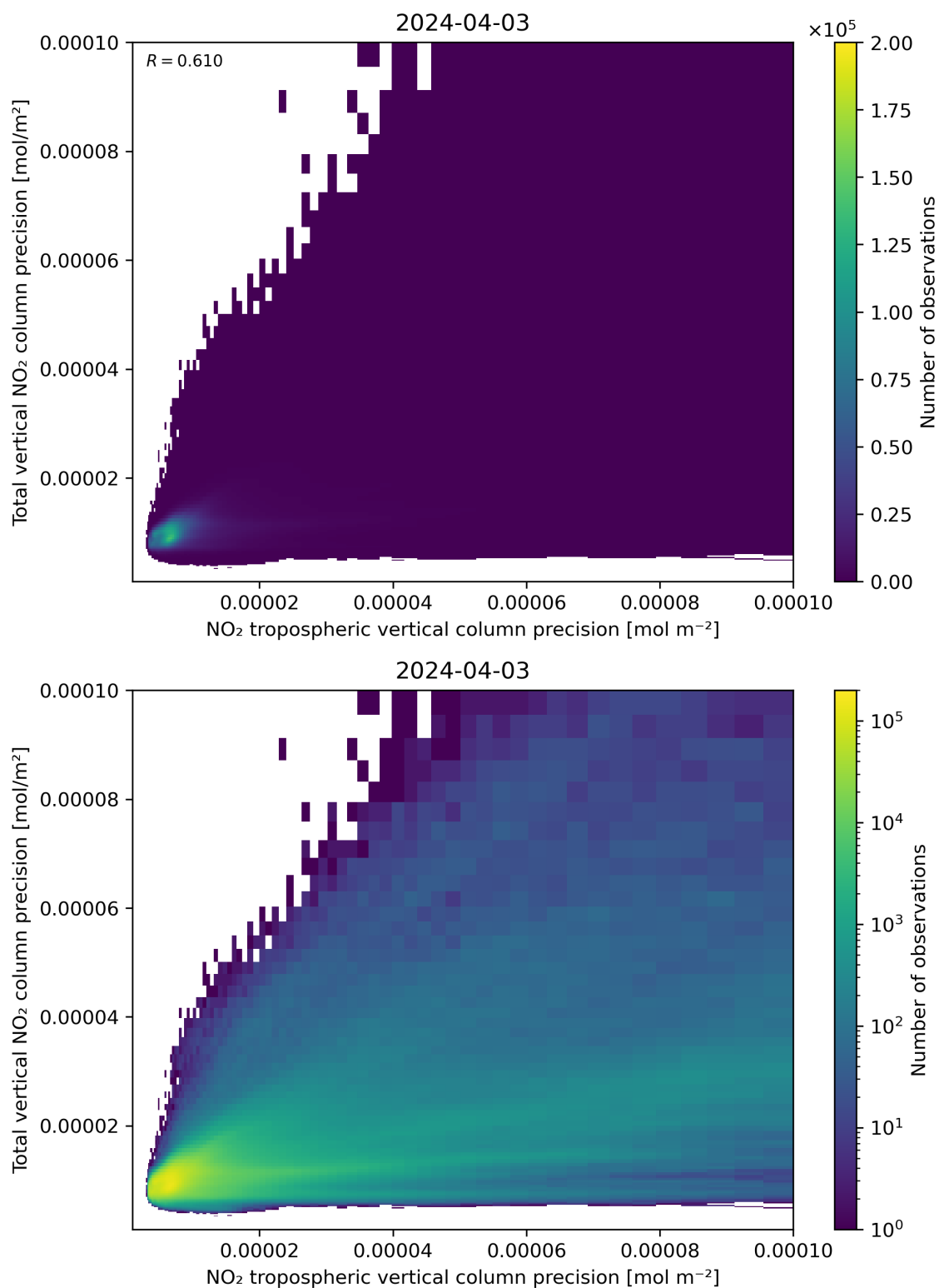
Figure 139: Scatter density plot of “NO 2 tropospheric vertical column precision” against “Total vertical NO 2 column precision” for 2024-04-02 to 2024-04-04.
