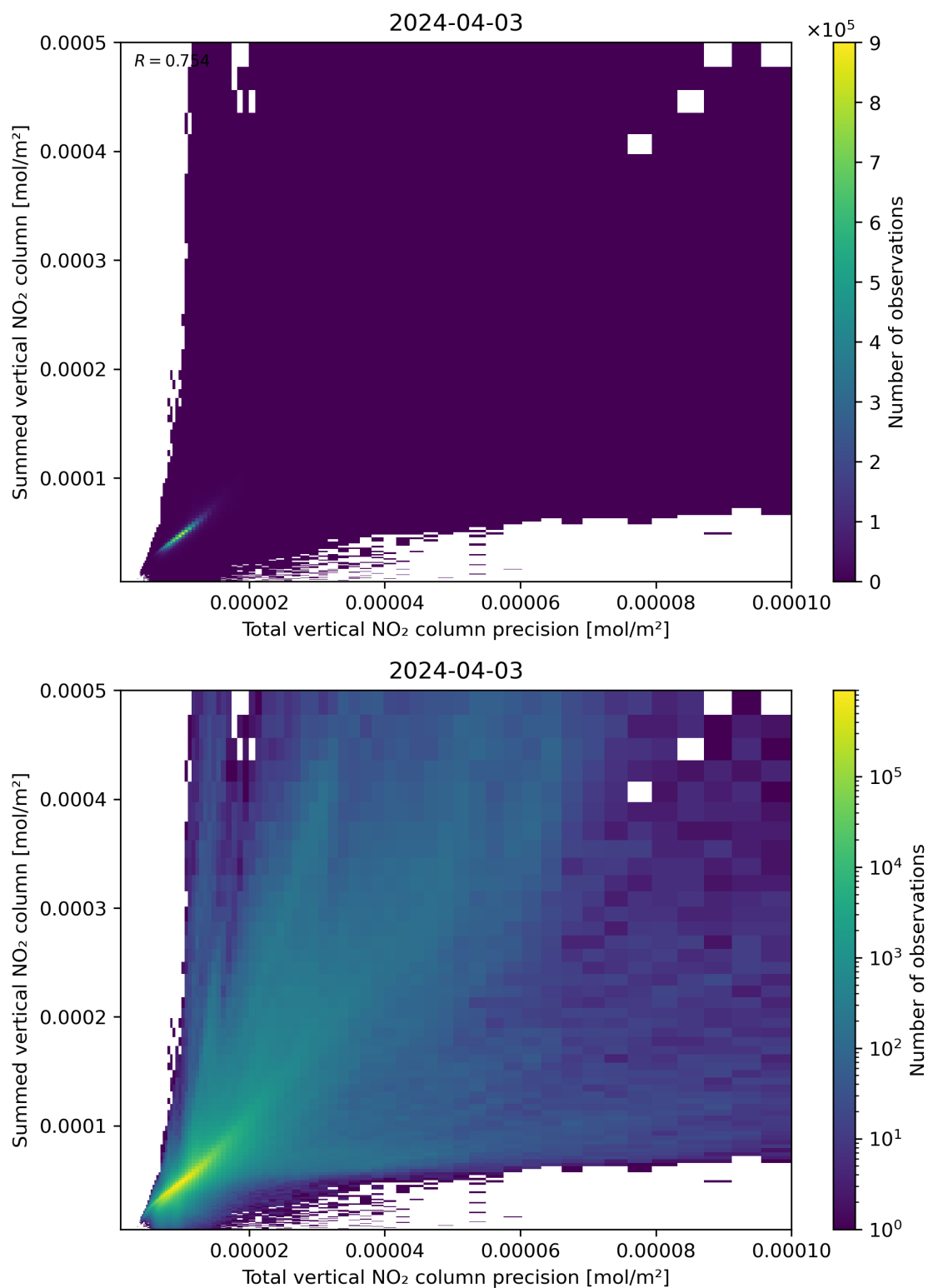
Figure 117: Scatter density plot of “Total vertical NO 2 column precision” against “Summed vertical NO 2 column” for 2024-04-02 to 2024-04-04.
