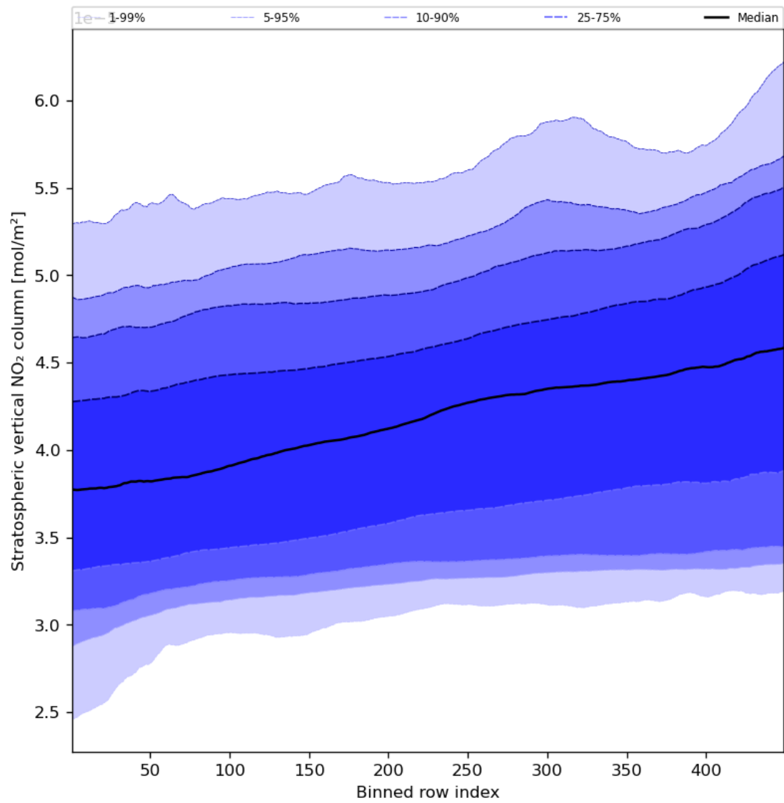
Figure 53: Along track statistics of “Stratospheric vertical NO 2 column” for 2024-04-02 to 2024-04-04
