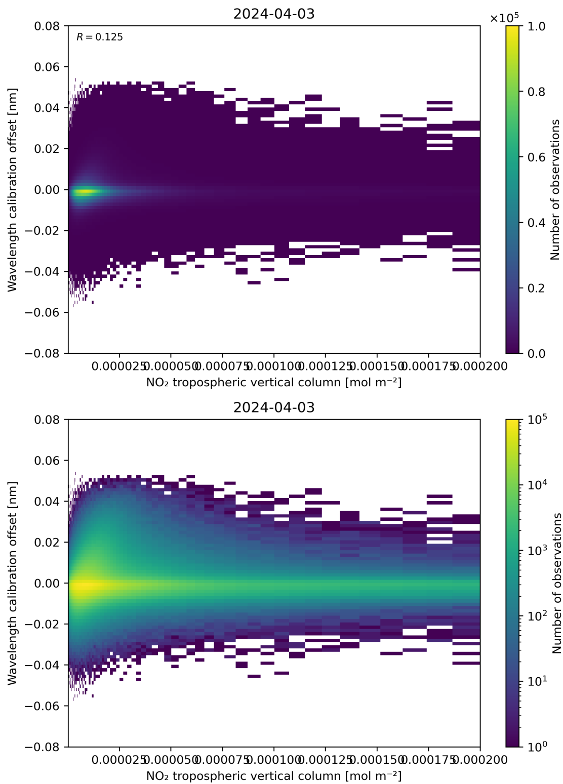
Figure 143: Scatter density plot of “NO 2 tropospheric vertical column” against “Wavelength calibration offset” for 2024-04-02 to 2024-04-04.
