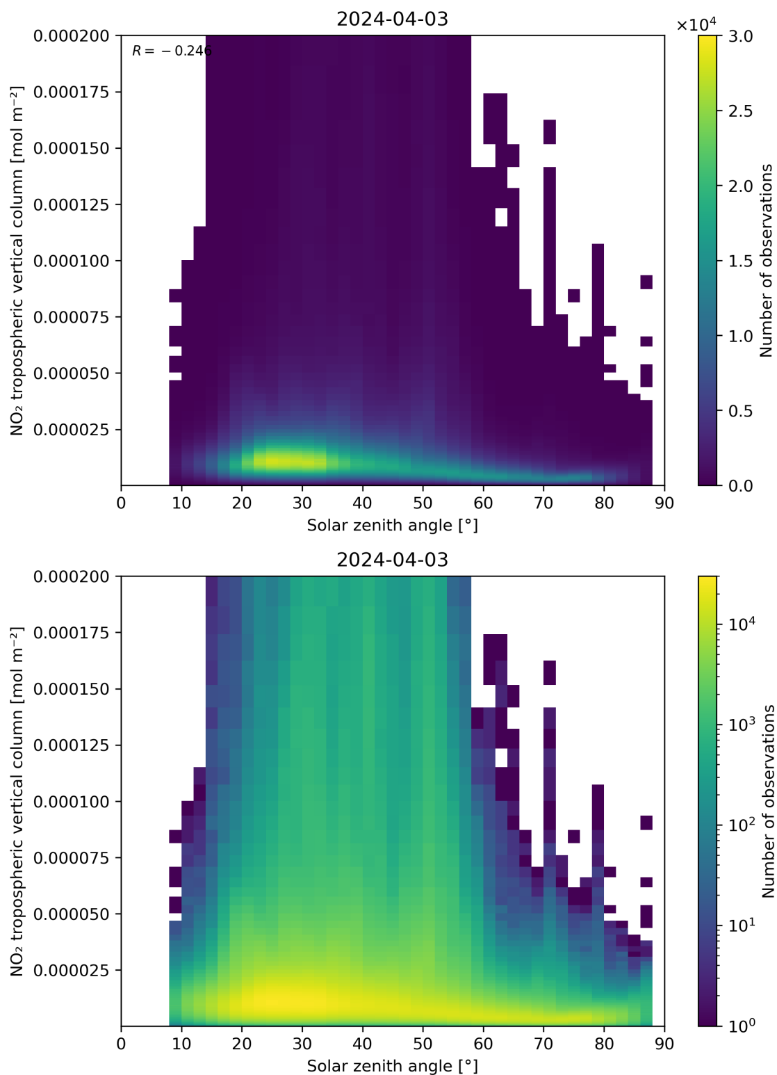
Figure 155: Scatter density plot of “Solar zenith angle” against “NO 2 tropospheric vertical column” for 2024-04-02 to 2024-04-04.
