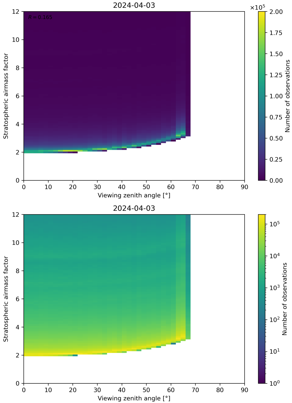
Figure 159: Scatter density plot of “Viewing zenith angle” against “Stratospheric airmass factor” for 2024-04-02 to 2024-04-04.
