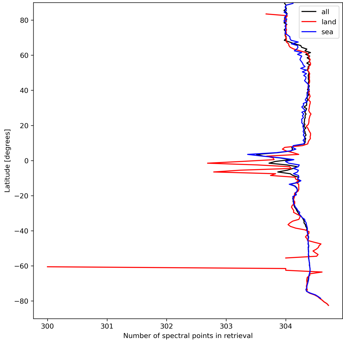
Figure 16: Zonal average of “Number of spectral points in retrieval” for 2024-04-02 to 2024-04-04.
