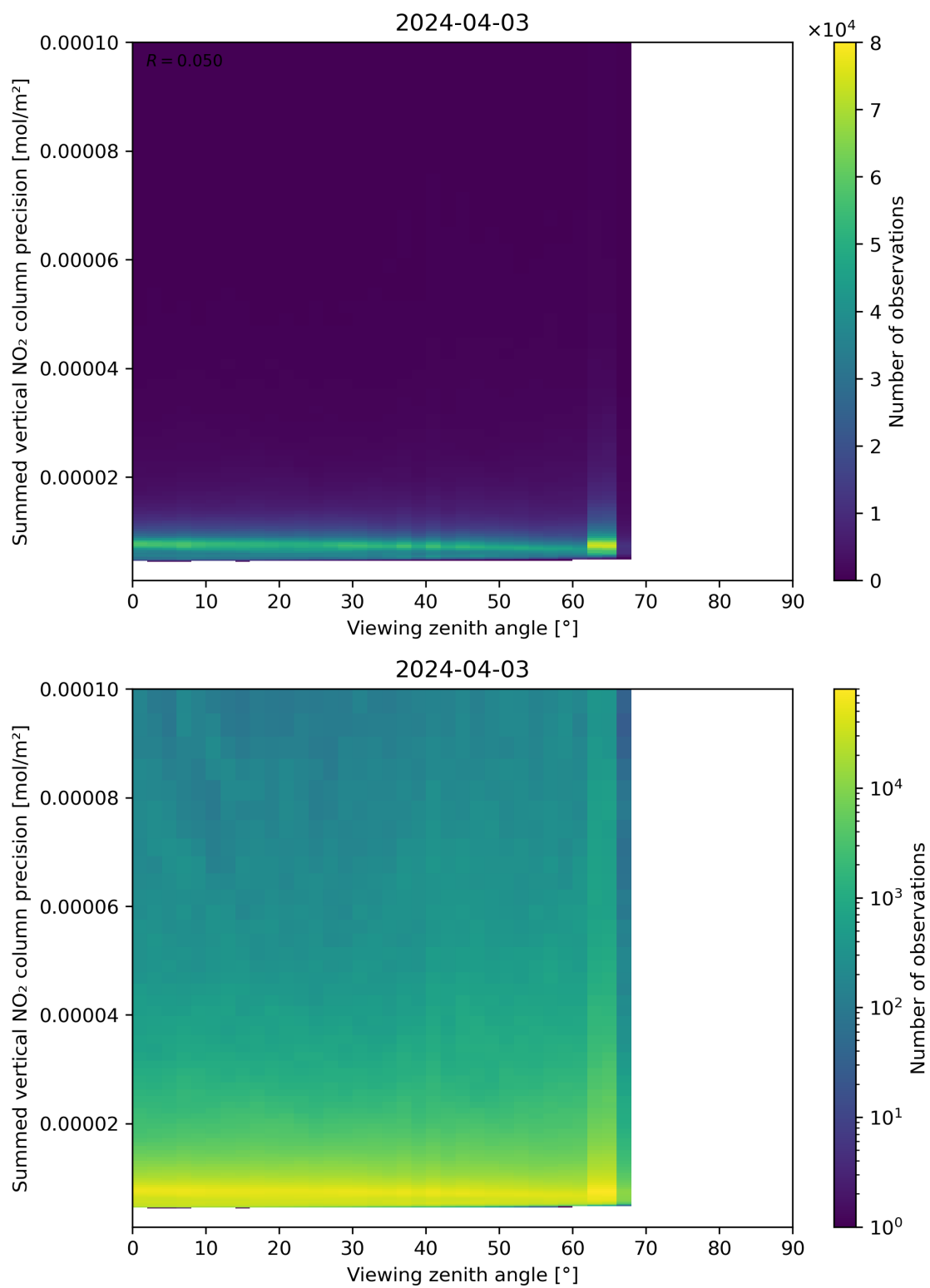
Figure 166: Scatter density plot of “Viewing zenith angle” against “Summed vertical NO 2 column precision” for 2024-04-02 to 2024-04-04.
