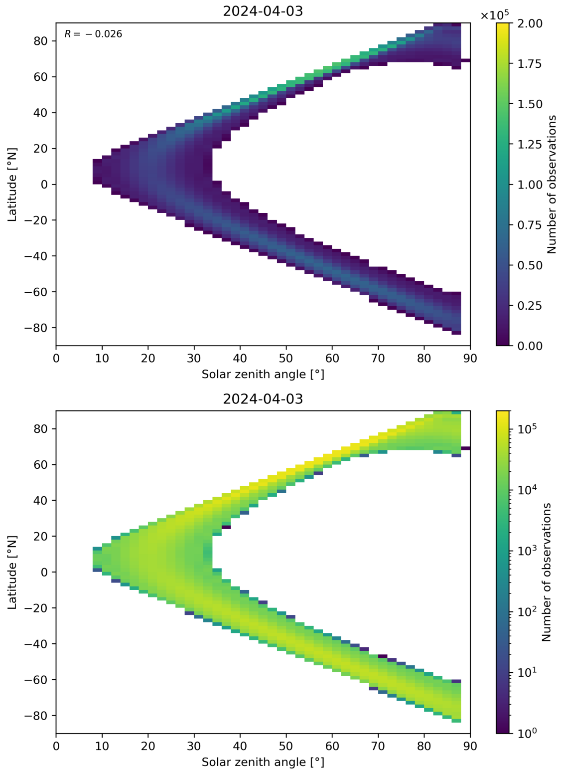
Figure 149: Scatter density plot of “Solar zenith angle” against “Latitude” for 2024-04-02 to 2024-04-04.
