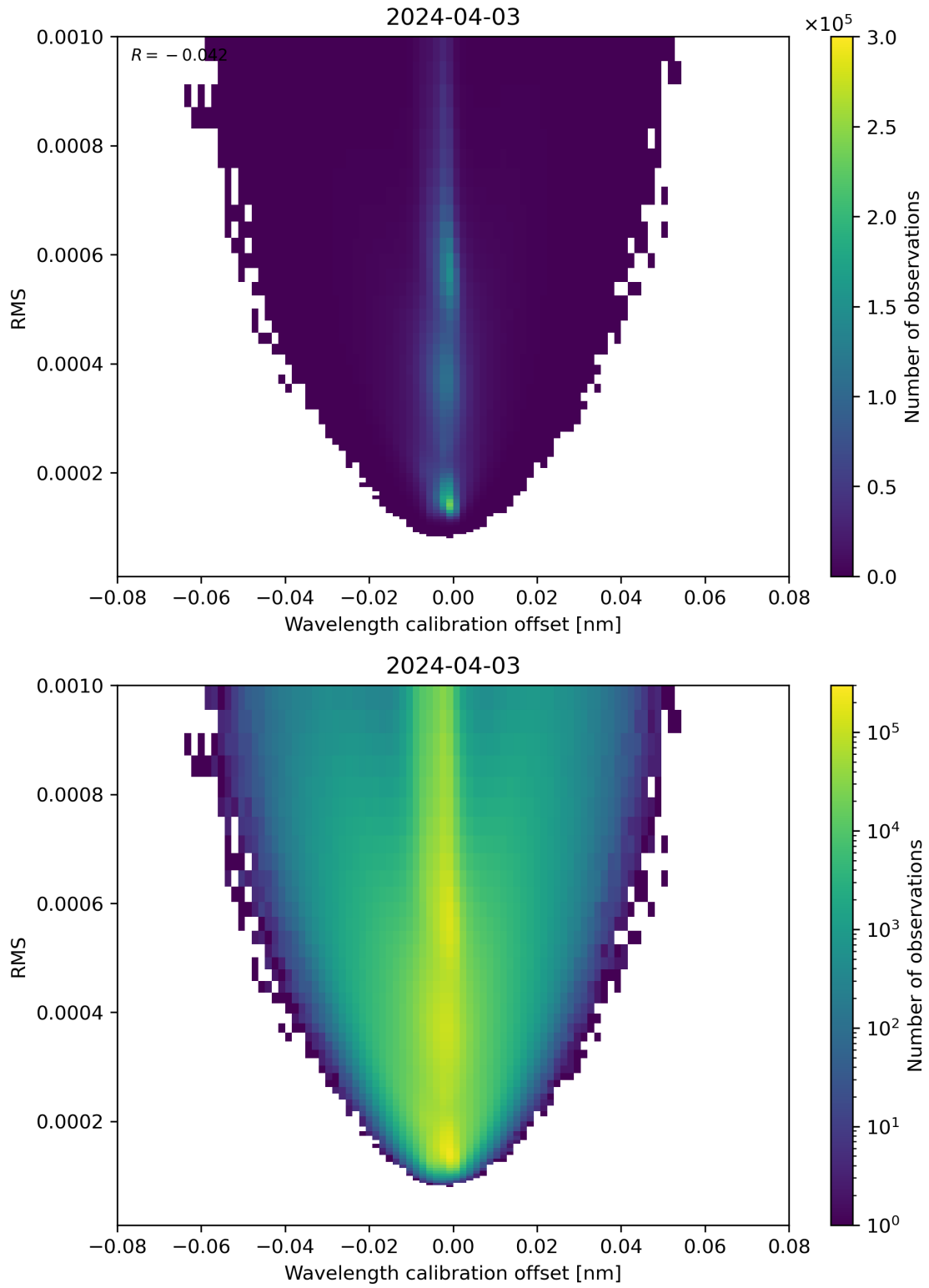
Figure 181: Scatter density plot of “Wavelength calibration offset” against “RMS” for 2024-04-02 to 2024-04-04.
