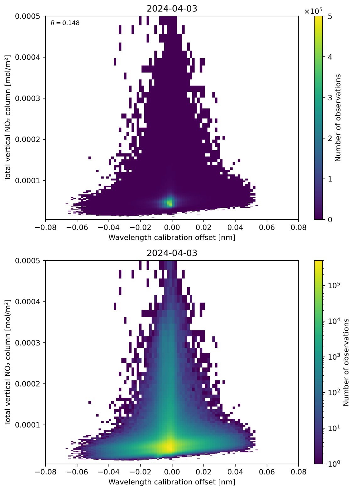
Figure 179: Scatter density plot of “Wavelength calibration offset” against “Total vertical NO 2 column” for 2024-04-02 to 2024-04-04.
