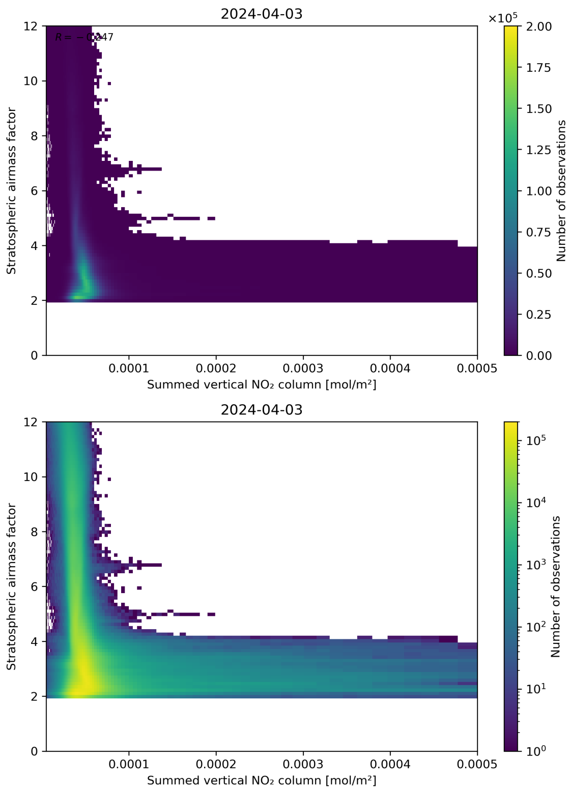
Figure 103: Scatter density plot of “Summed vertical NO 2 column” against “Stratospheric airmass factor” for 2024-04-02 to 2024-04-04.
