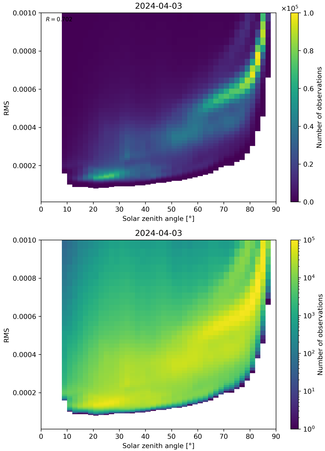
Figure 157: Scatter density plot of “Solar zenith angle” against “RMS” for 2024-04-02 to 2024-04-04.
