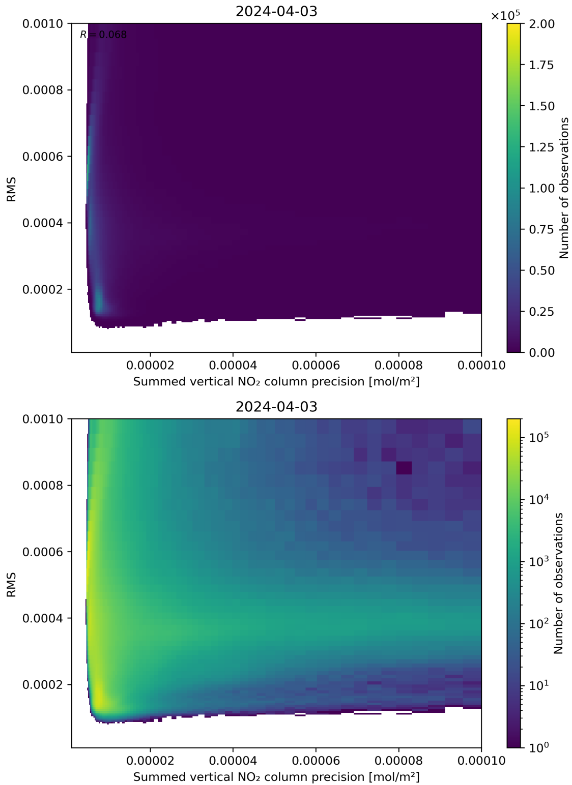
Figure 108: Scatter density plot of “Summed vertical NO 2 column precision” against “RMS” for 2024-04-02 to 2024-04-04.
