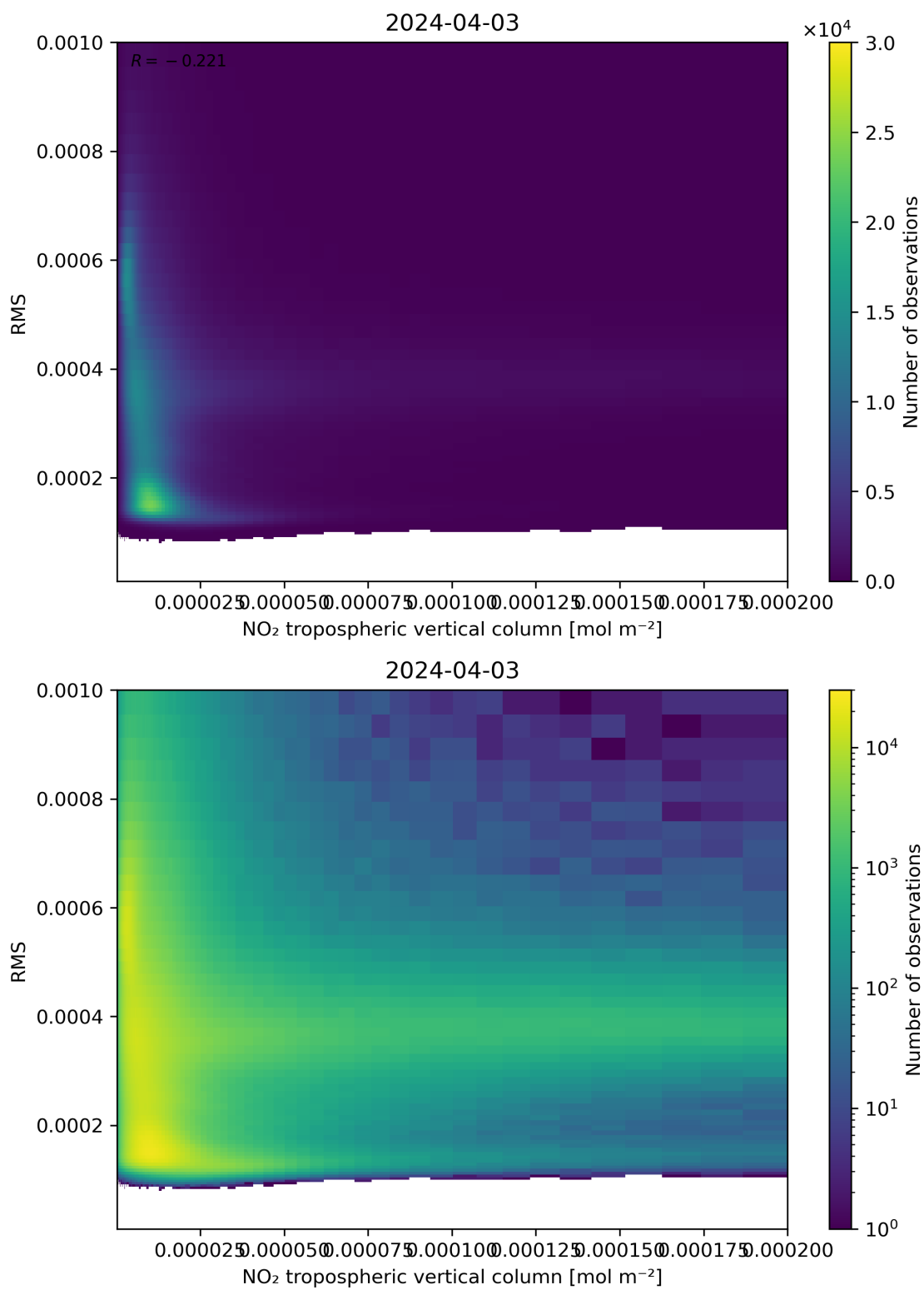
Figure 142: Scatter density plot of “NO 2 tropospheric vertical column” against “RMS” for 2024-04-02 to 2024-04-04.
