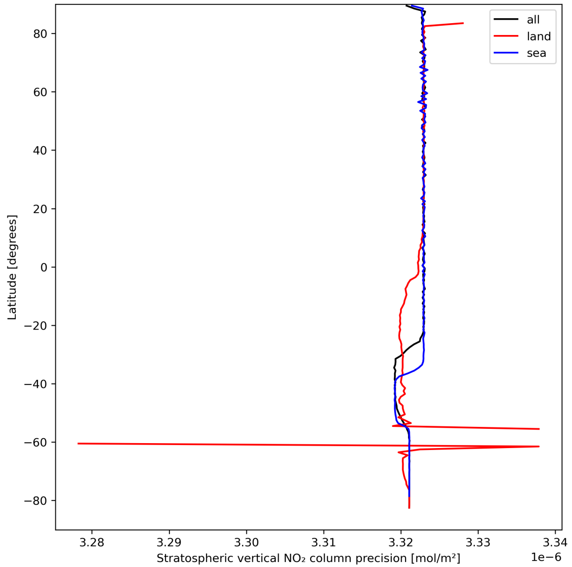
Figure 20: Zonal average of “Stratospheric vertical NO 2 column precision” for 2024-04-02 to 2024-04-04.
