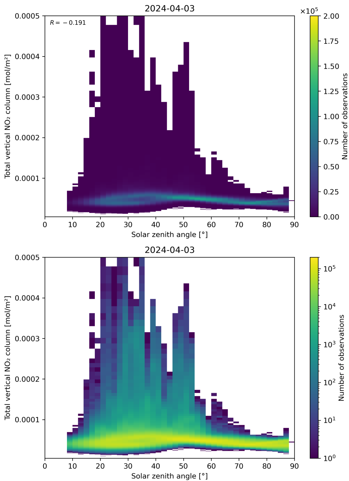
Figure 153: Scatter density plot of “Solar zenith angle” against “Total vertical NO 2 column” for 2024-04-02 to 2024-04-04.
