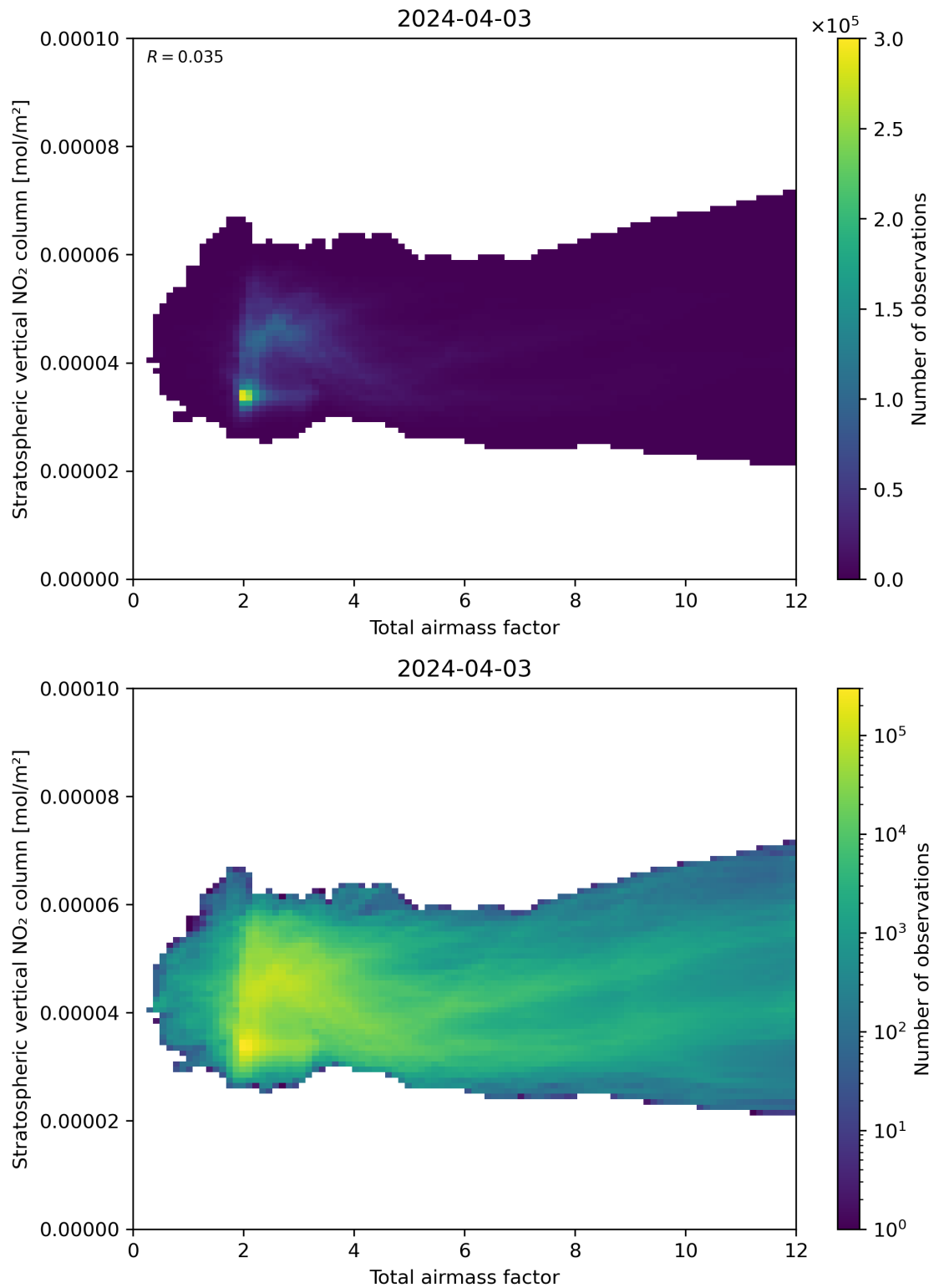
Figure 64: Scatter density plot of “Total airmass factor” against “Stratospheric vertical \text{NO}_2 column” for 2024-04-02 to 2024-04-04.
