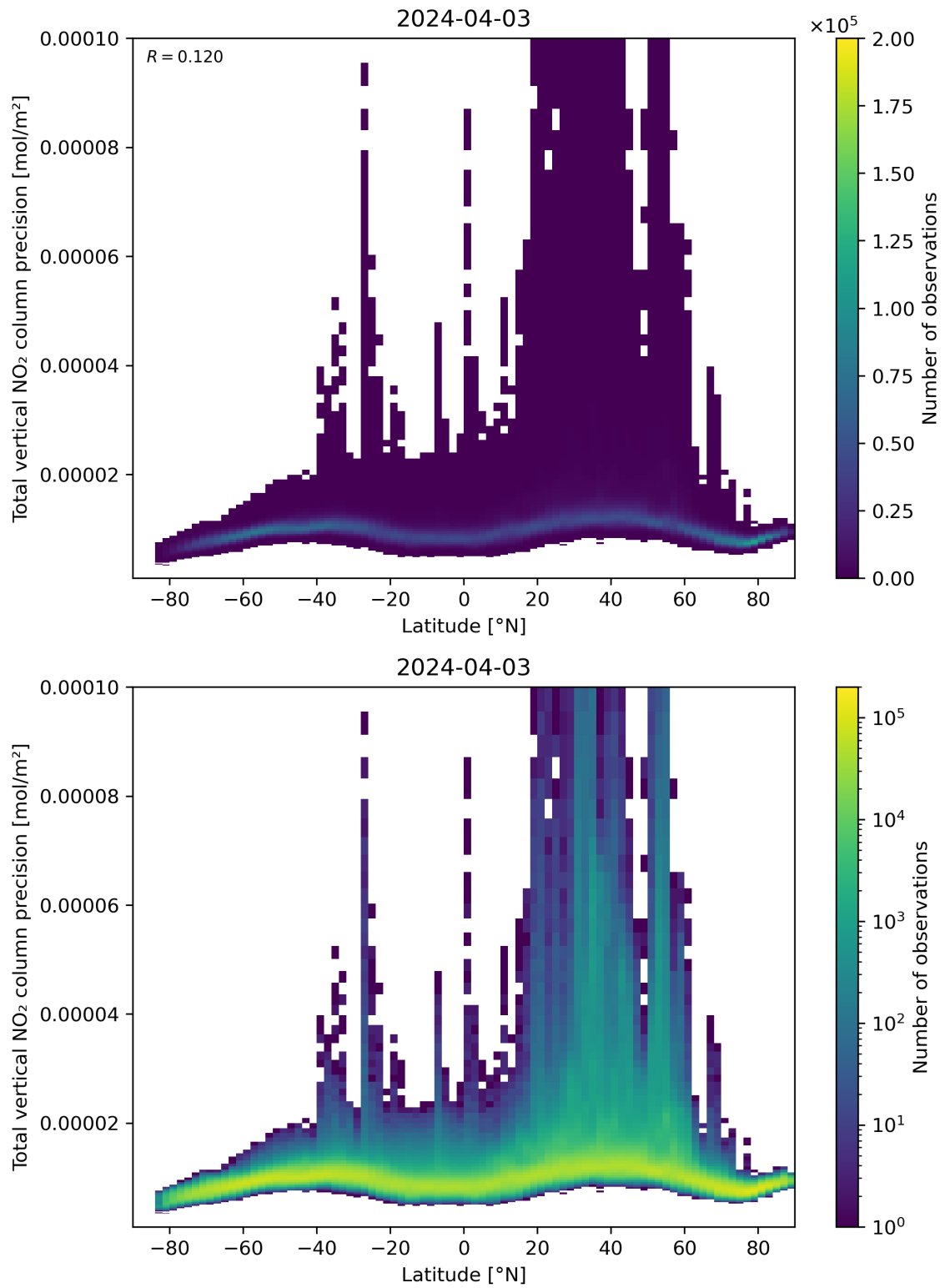
Figure 91: Scatter density plot of “Latitude” against “Total vertical NO 2 column precision” for 2024-04-02 to 2024-04-04.
