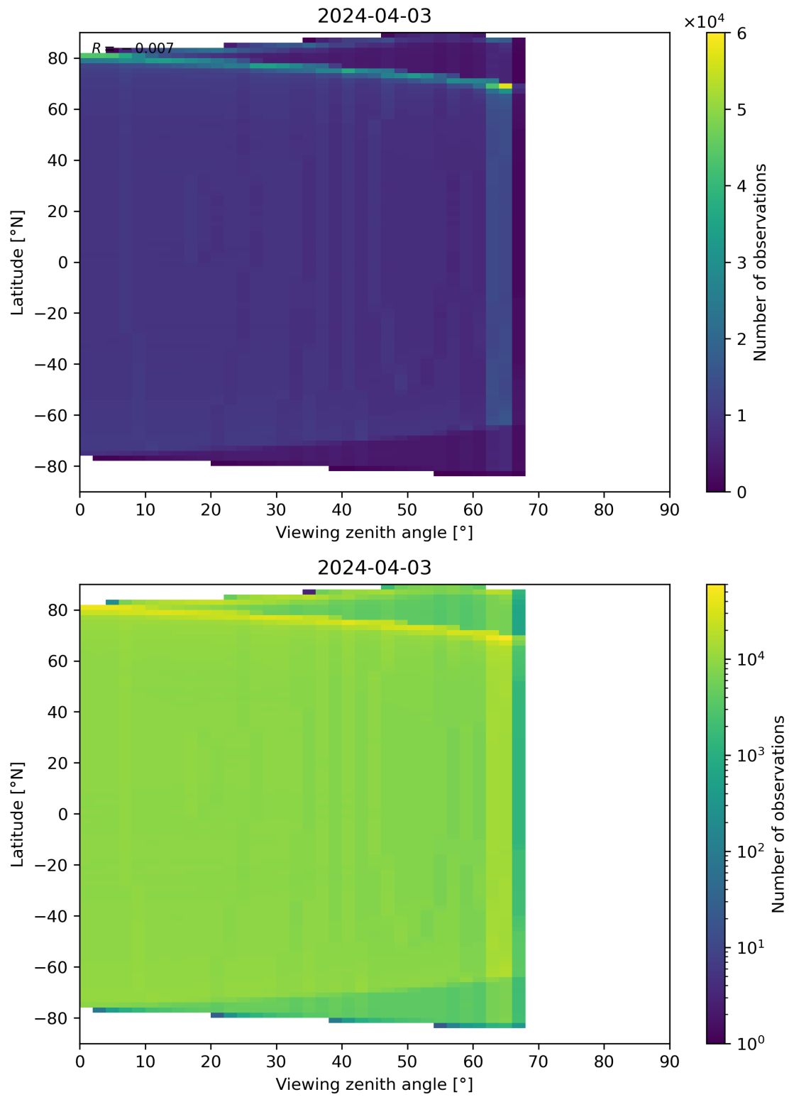
Figure 163: Scatter density plot of “Viewing zenith angle” against “Latitude” for 2024-04-02 to 2024-04-04.
