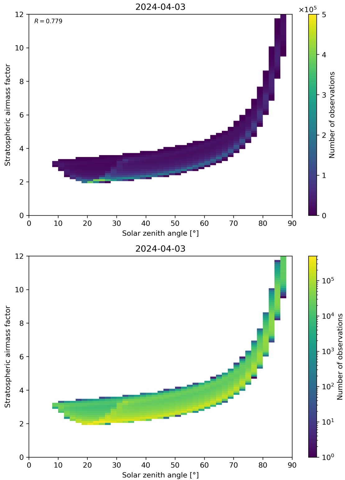
Figure 145: Scatter density plot of “Solar zenith angle” against “Stratospheric airmass factor” for 2024-04-02 to 2024-04-04.
