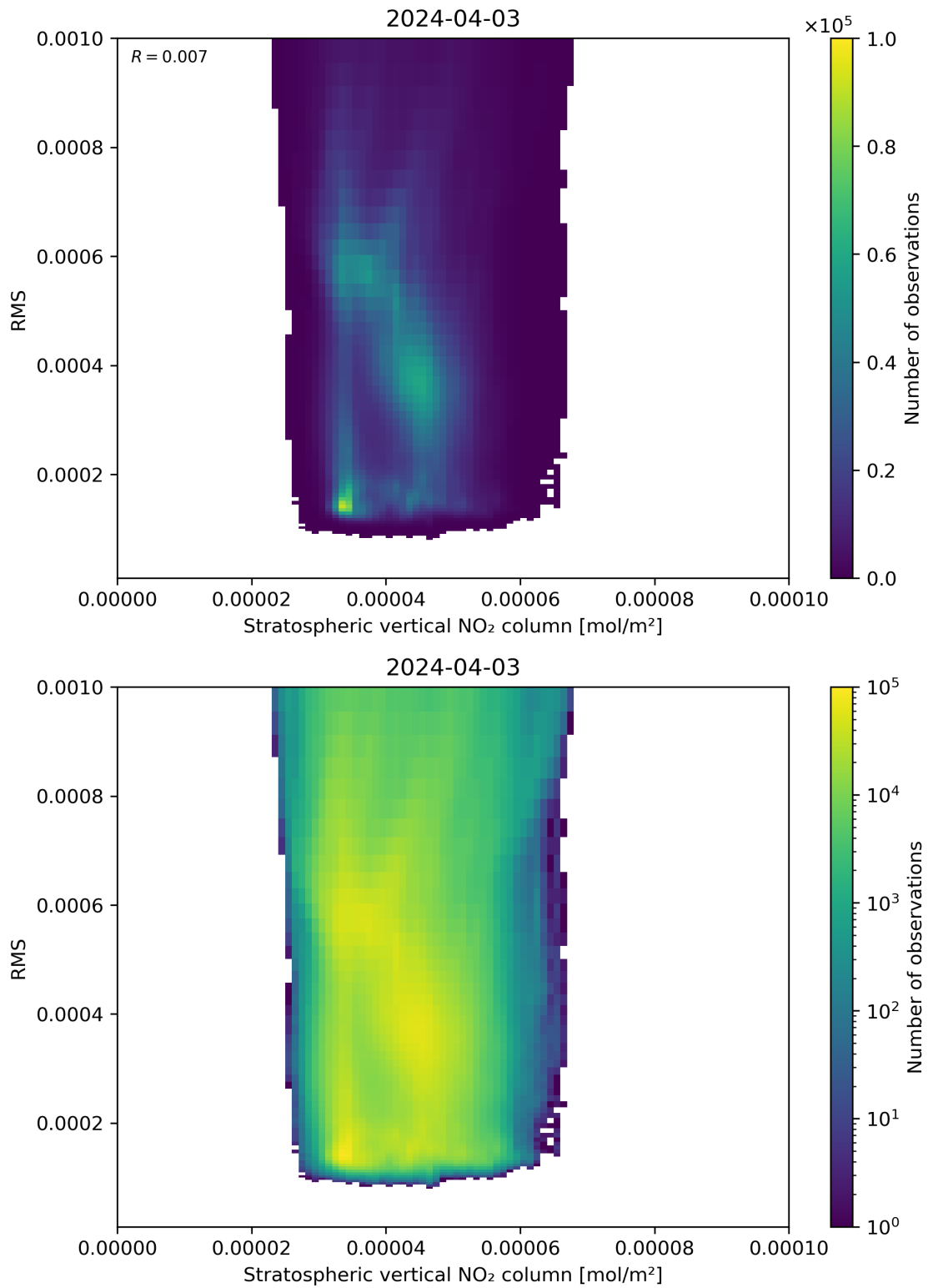
Figure 102: Scatter density plot of “Stratospheric vertical NO 2 column” against “RMS” for 2024-04-02 to 2024-04-04.
