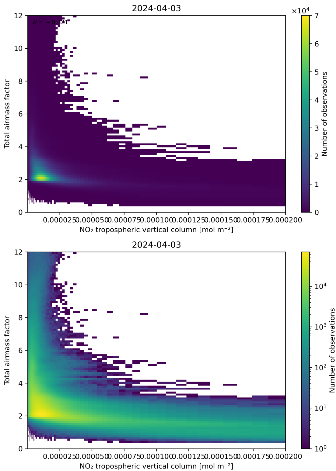
Figure 122: Scatter density plot of “NO 2 tropospheric vertical column” against “Total air mass factor” for 2024-04-02 to 2024-04-04.
