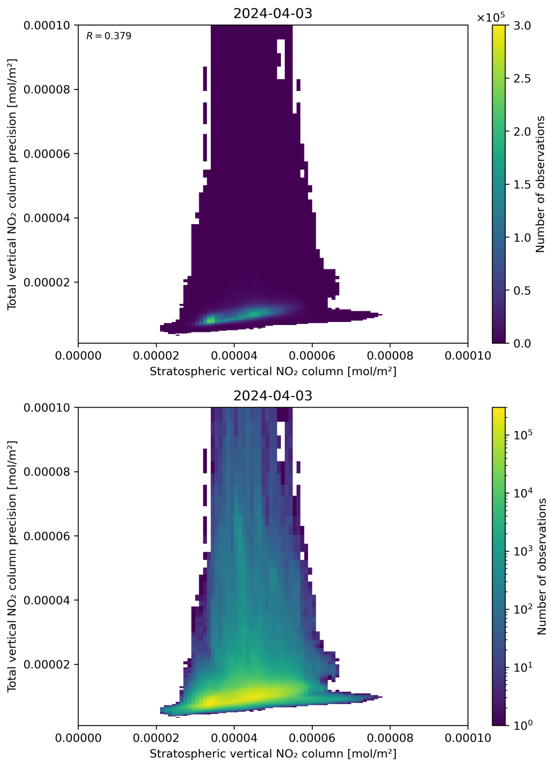
Figure 101: Scatter density plot of “Stratospheric vertical NO 2 column” against “Total vertical NO 2 column precision” for 2024-04-02 to 2024-04-04.
