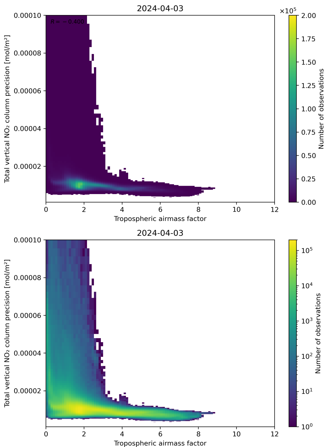
Figure 78: Scatter density plot of “Tropospheric air mass factor” against “Total vertical NO 2 column precision” for 2024-04-02 to 2024-04-04.
