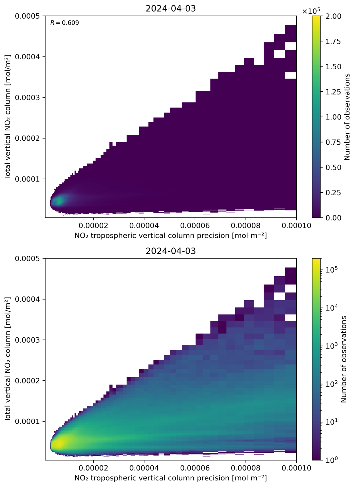
Figure 138: Scatter density plot of “NO 2 tropospheric vertical column precision” against “Total vertical NO 2 column” for 2024-04-02 to 2024-04-04.
