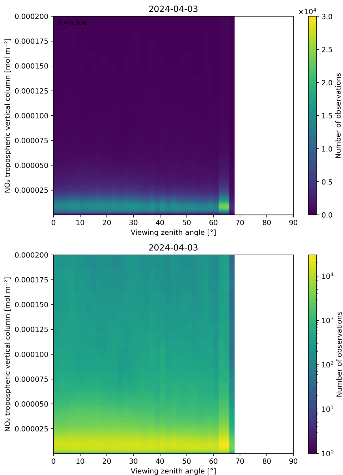
Figure 169: Scatter density plot of “Viewing zenith angle” against “NO 2 tropospheric vertical column” for 2024-04-02 to 2024-04-04.
