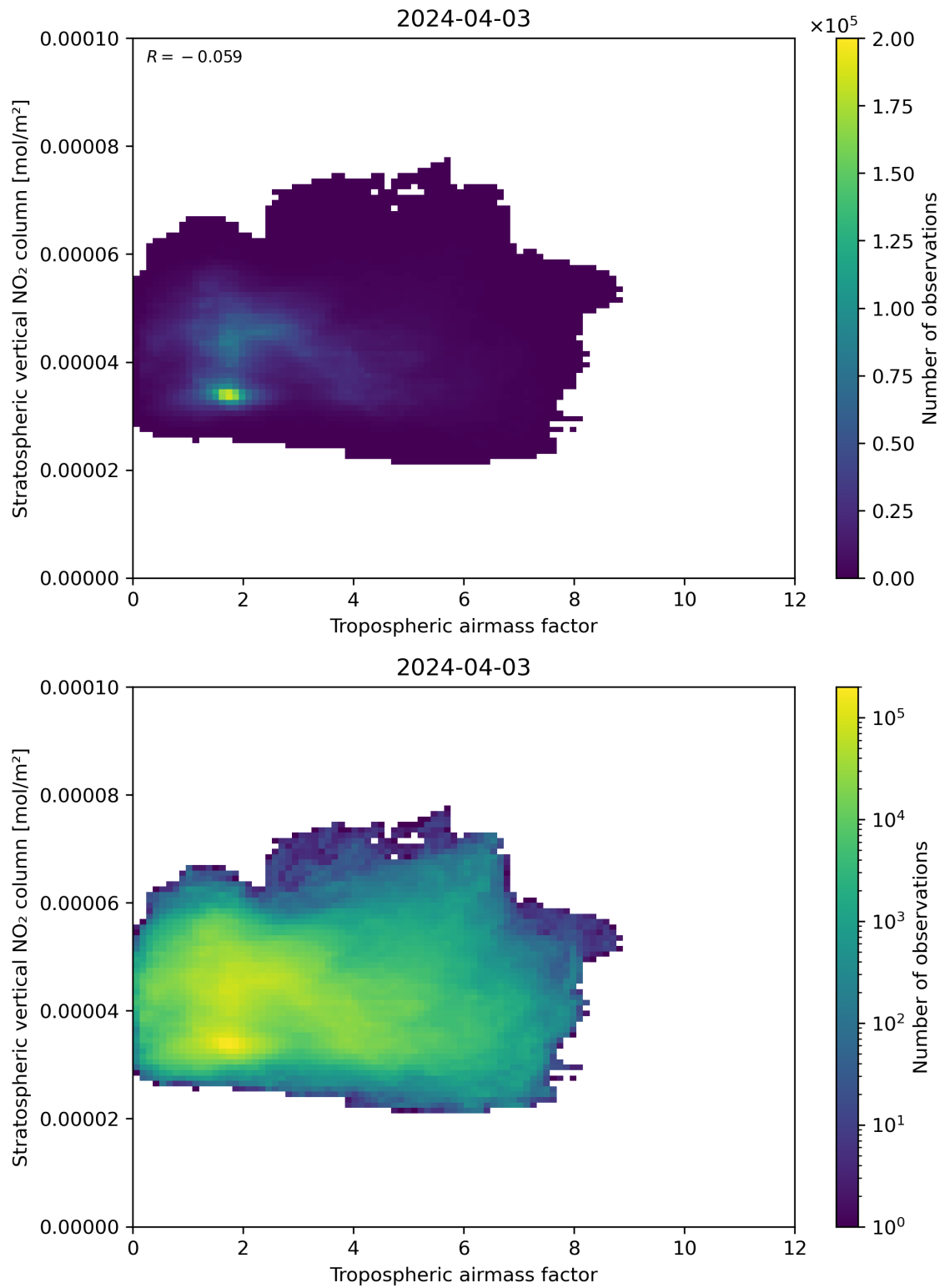
Figure 74: Scatter density plot of “Tropospheric air mass factor” against “Stratospheric vertical NO 2 column” for 2024-04-02 to 2024-04-04.
