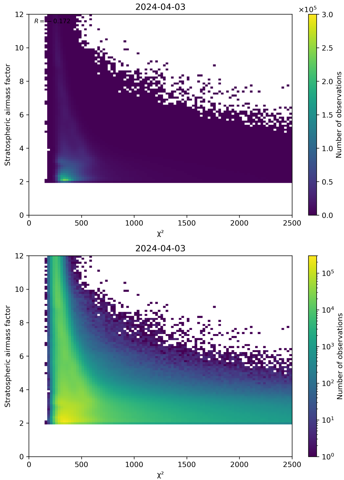
Figure 81: Scatter density plot of “ \chi^2 ” against “Stratospheric airmass factor” for 2024-04-02 to 2024-04-04.
