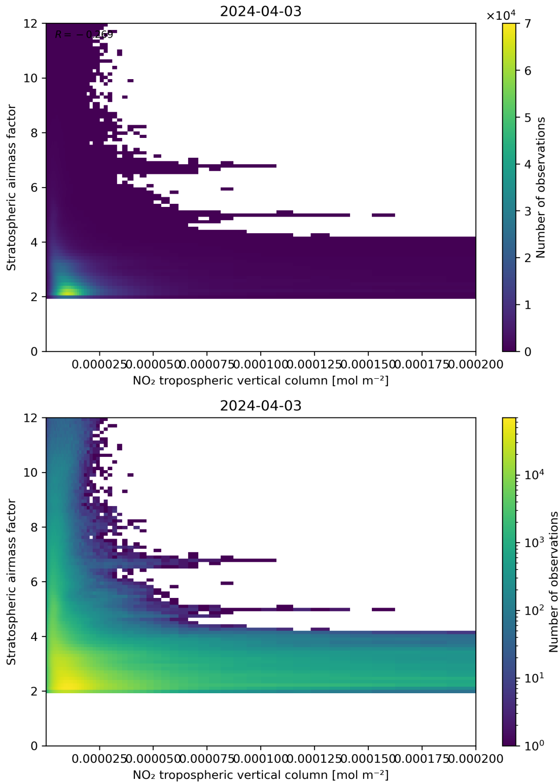
Figure 121: Scatter density plot of “NO 2 tropospheric vertical column” against “Stratospheric airmass factor” for 2024-04-02 to 2024-04-04.
