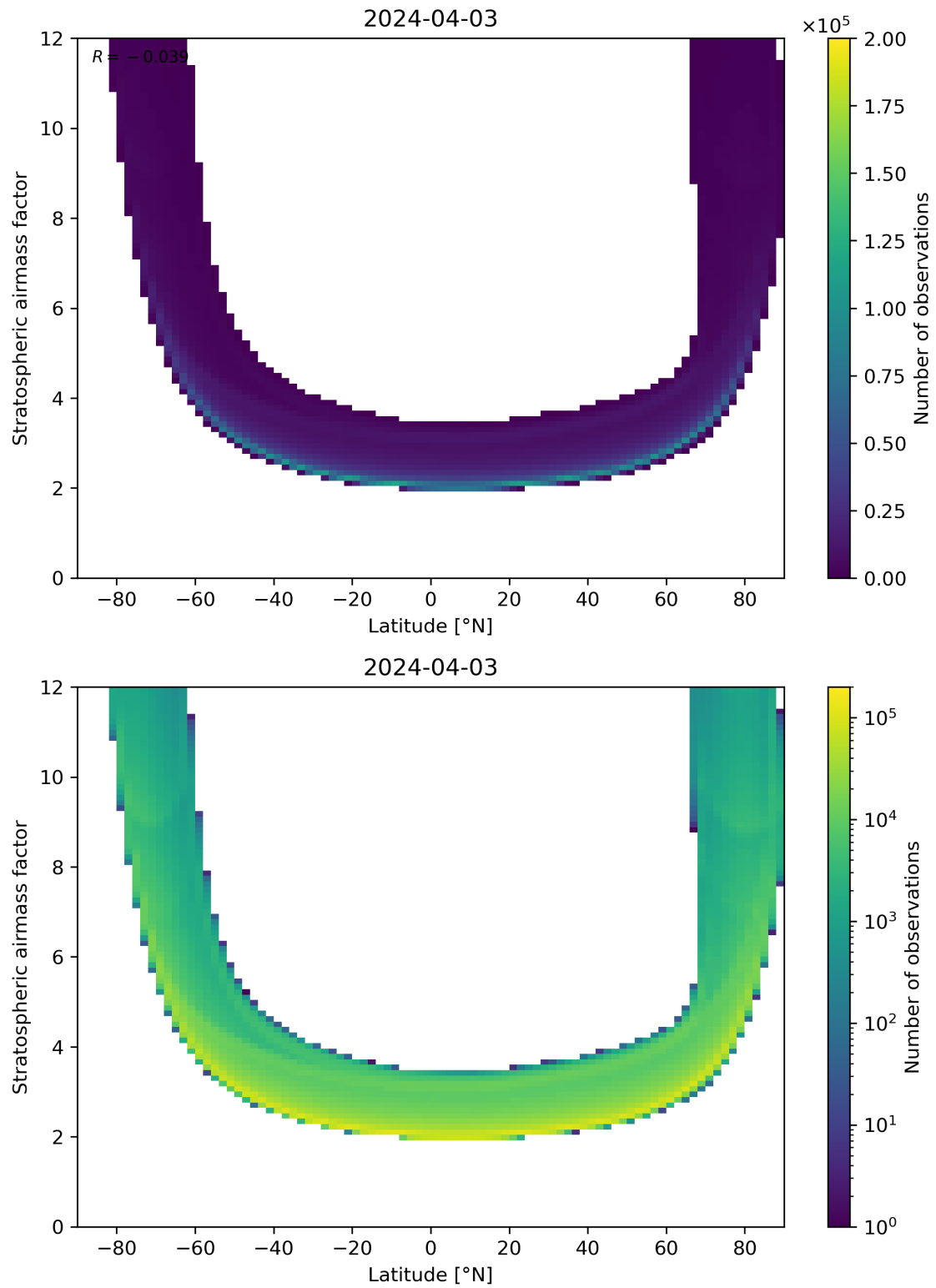
Figure 83: Scatter density plot of “Latitude” against “Stratospheric airmass factor” for 2024-04-02 to 2024-04-04.
