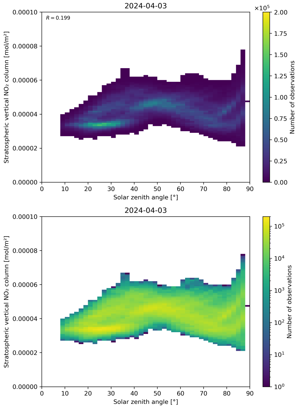
Figure 150: Scatter density plot of “Solar zenith angle” against “Stratospheric vertical NO 2 column” for 2024-04-02 to 2024-04-04.
