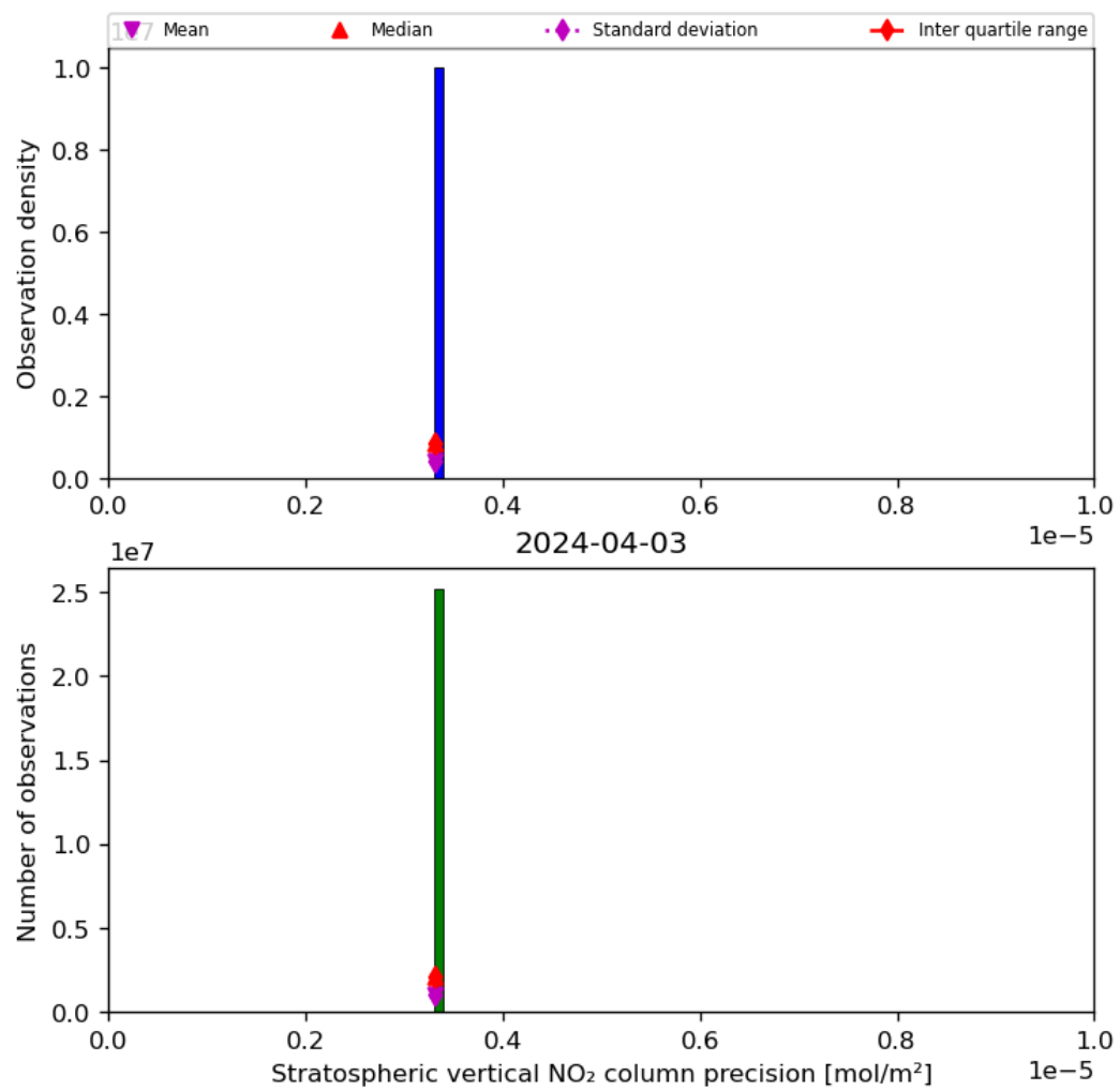
Figure 37: Histogram of “Stratospheric vertical NO 2 column precision” for 2024-04-02 to 2024-04-04
