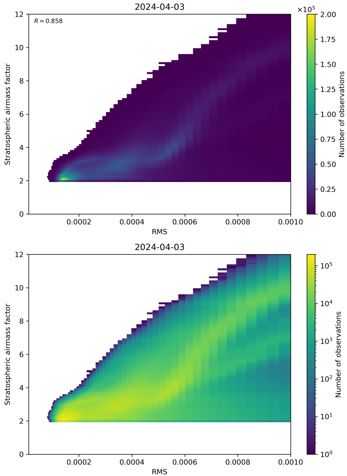
Figure 144: Scatter density plot of “RMS” against “Stratospheric airmass factor” for 2024-04-02 to 2024-04-04.
