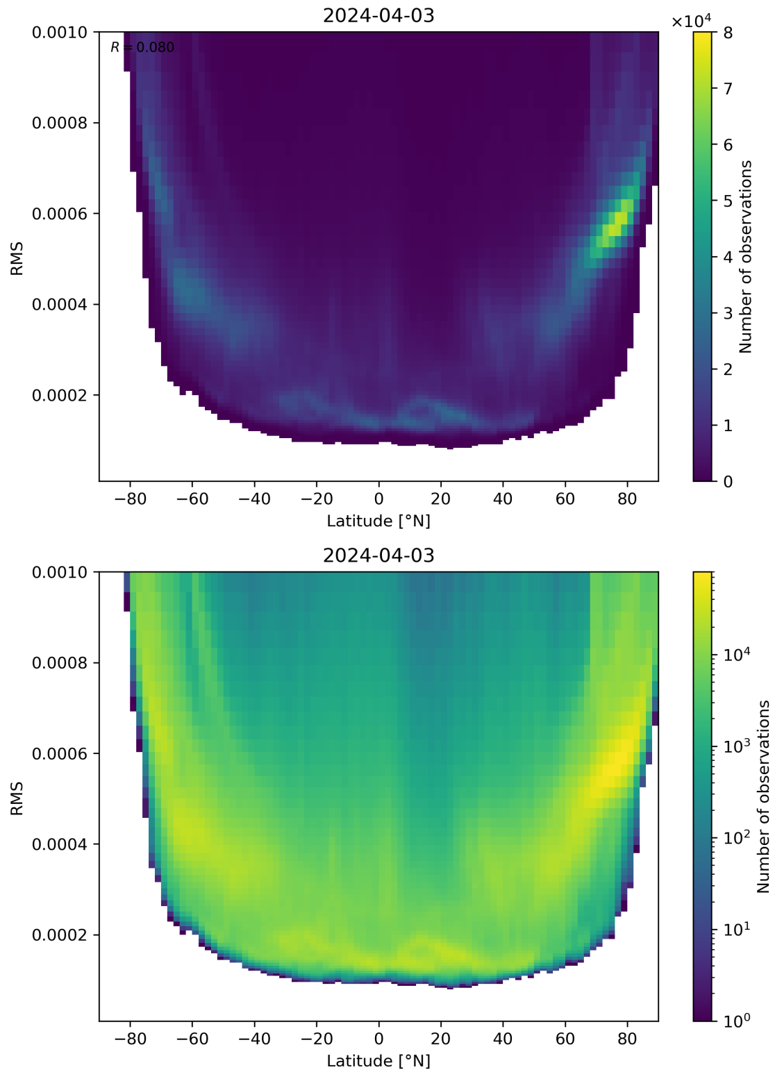
Figure 94: Scatter density plot of “Latitude” against “RMS” for 2024-04-02 to 2024-04-04.
