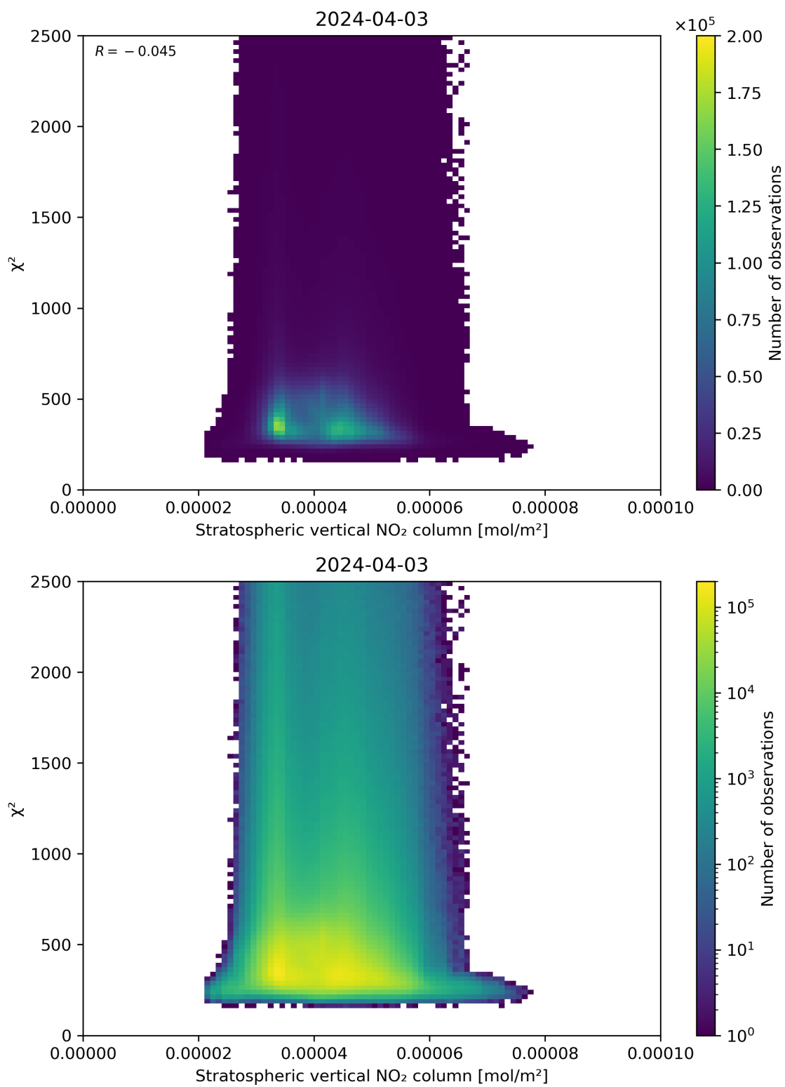
Figure 97: Scatter density plot of “Stratospheric vertical NO 2 column” against “ \chi^2 ” for 2024-04-02 to 2024-04-04.
