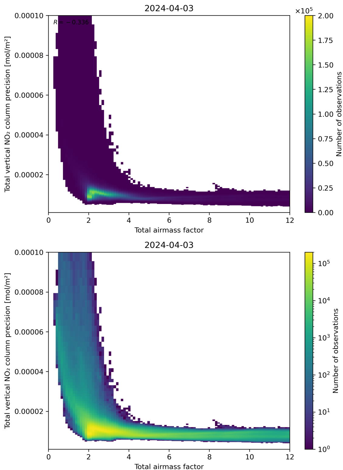
Figure 68: Scatter density plot of “Total airmass factor” against “Total vertical NO 2 column precision” for 2024-04-02 to 2024-04-04.
