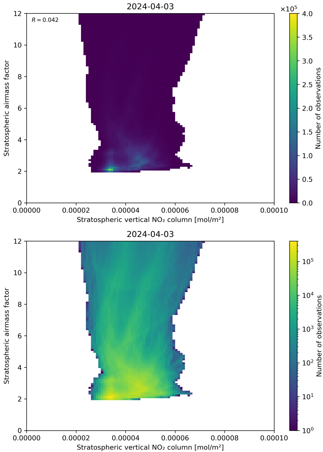
Figure 96: Scatter density plot of “Stratospheric vertical NO 2 column” against “Stratospheric airmass factor” for 2024-04-02 to 2024-04-04.
