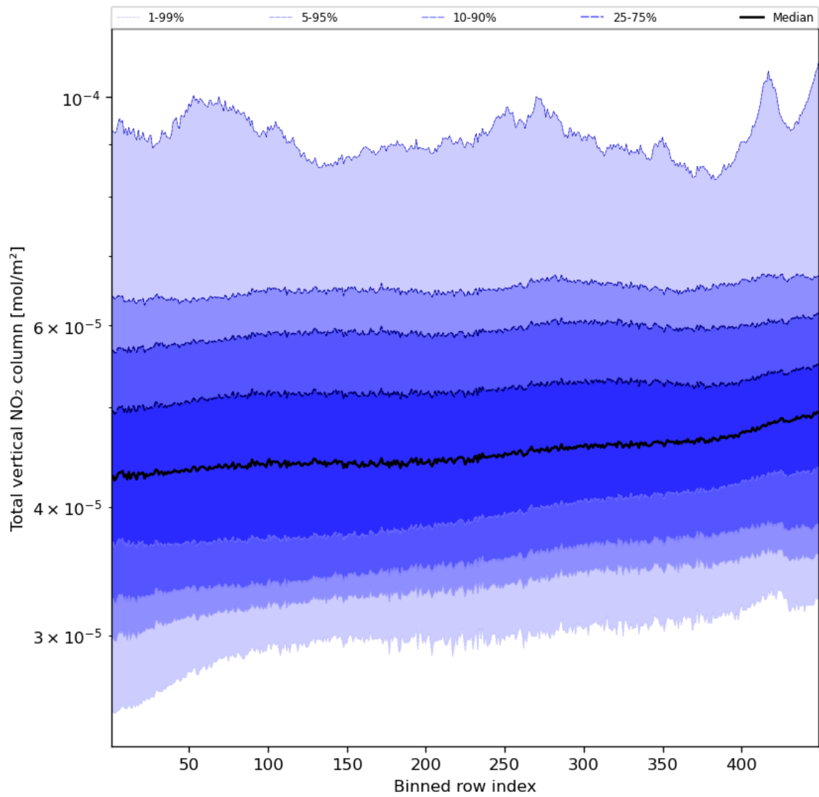
Figure 55: Along track statistics of “Total vertical NO 2 column” for 2024-04-02 to 2024-04-04
