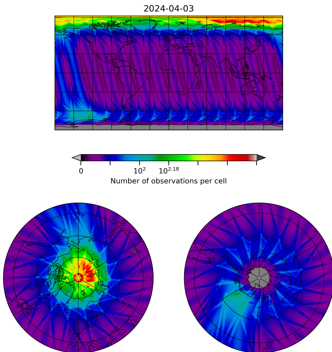
Figure 10: Map of the number of observations for 2024-04-02 to 2024-04-04
