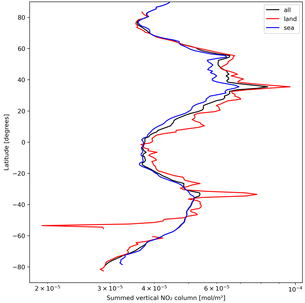
Figure 23: Zonal average of “Summed vertical NO 2 column” for 2024-04-02 to 2024-04-04.
