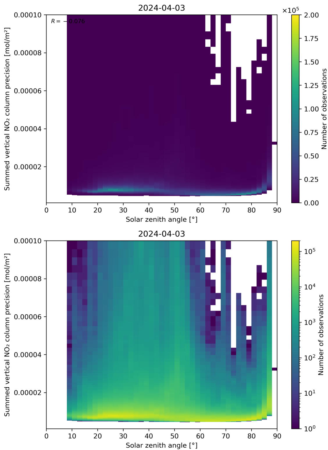
Figure 152: Scatter density plot of “Solar zenith angle” against “Summed vertical NO 2 column precision” for 2024-04-02 to 2024-04-04.
