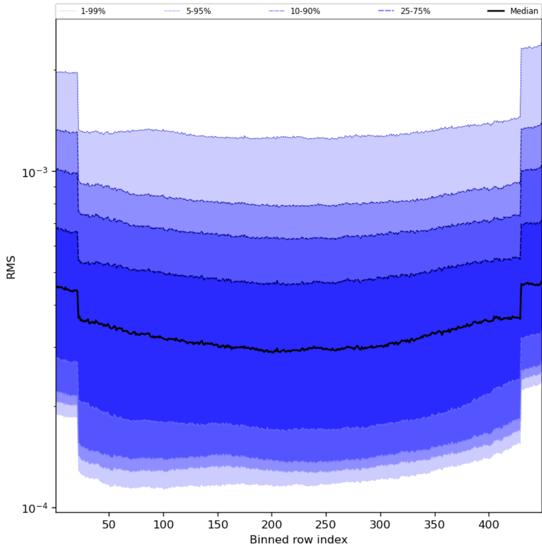
Figure 60: Along track statistics of “RMS” for 2024-04-02 to 2024-04-04
