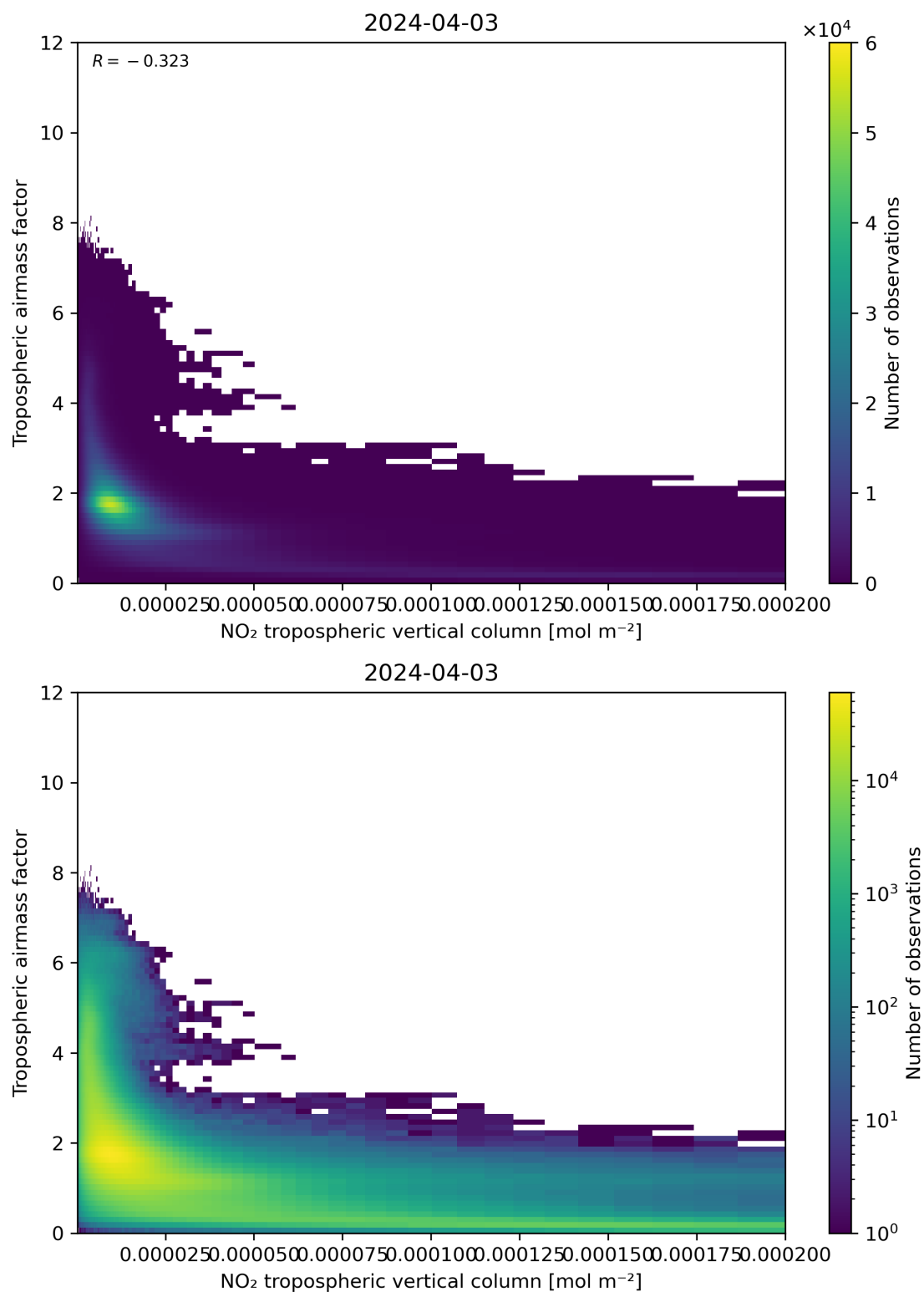
Figure 123: Scatter density plot of “NO 2 tropospheric vertical column” against “Tropospheric airmass factor” for 2024-04-02 to 2024-04-04.
