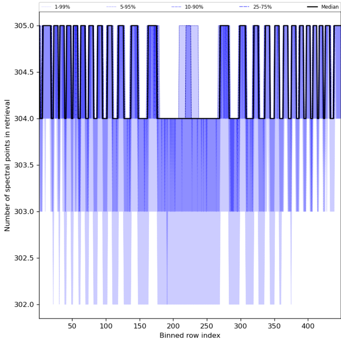
Figure 50: Along track statistics of “Number of spectral points in retrieval” for 2024-04-02 to 2024-04-04
