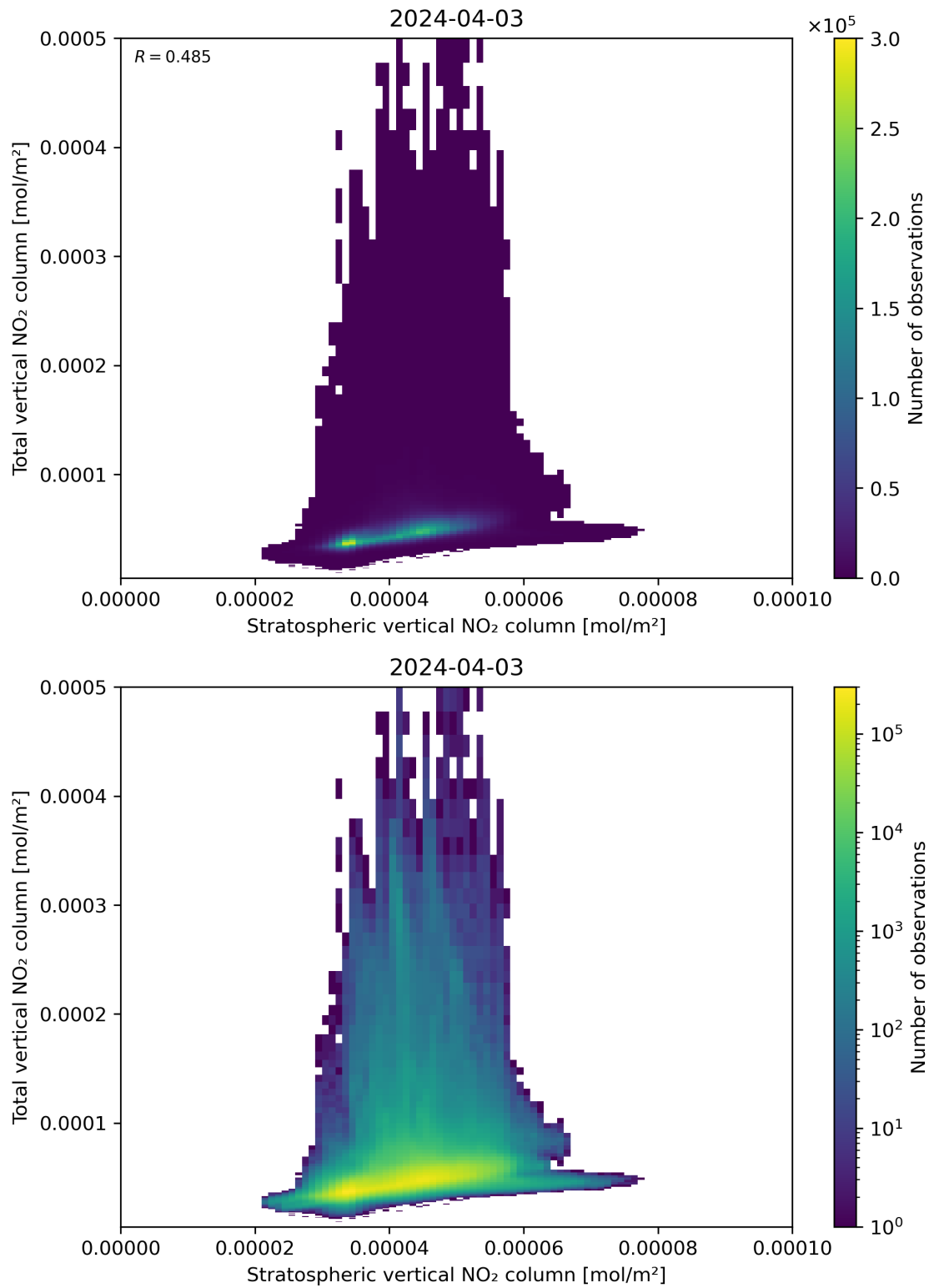
Figure 100: Scatter density plot of “Stratospheric vertical NO 2 column” against “Total vertical NO 2 column” for 2024-04-02 to 2024-04-04.
