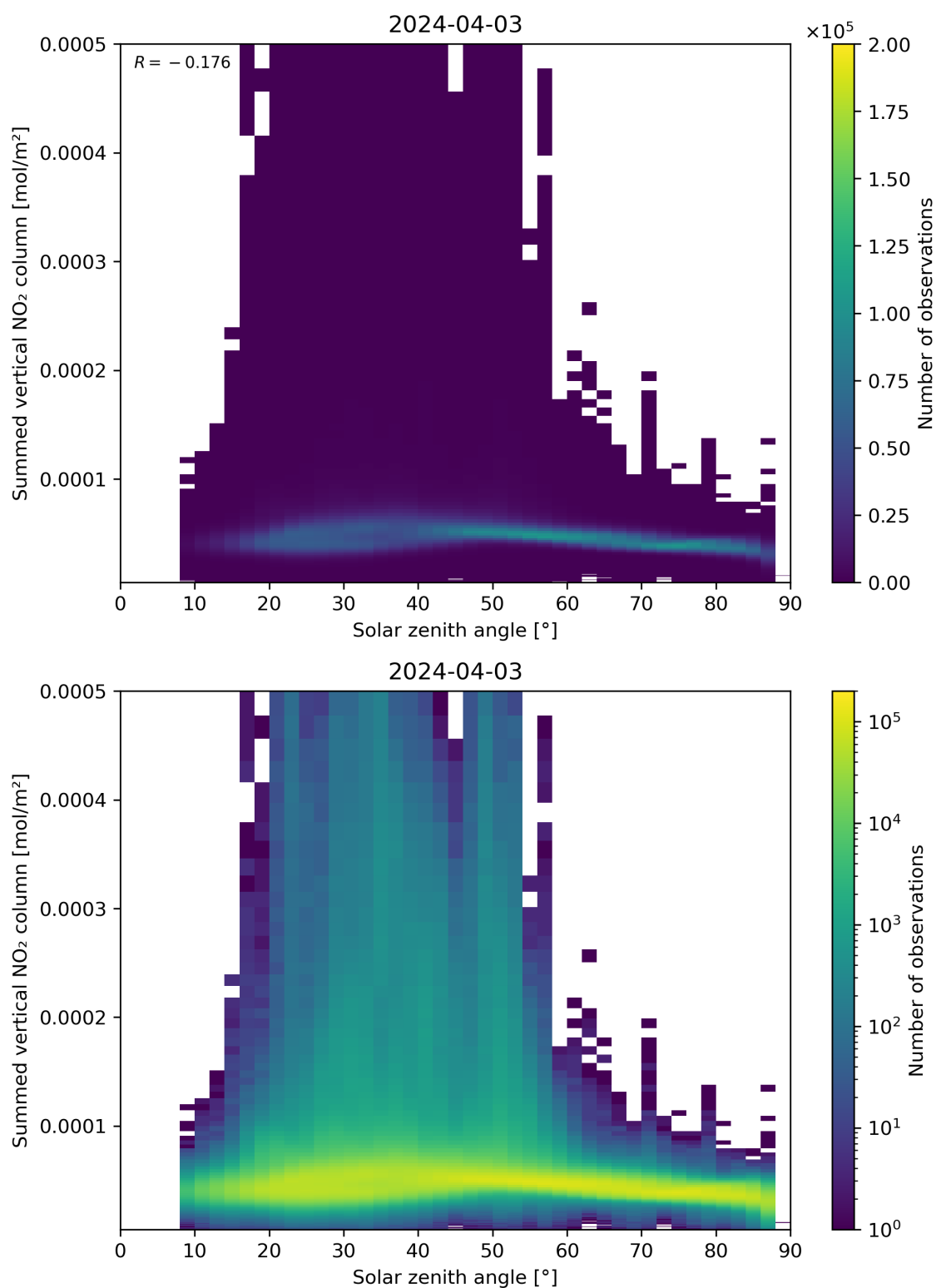
Figure 151: Scatter density plot of “Solar zenith angle” against “Summed vertical NO 2 column” for 2024-04-02 to 2024-04-04.
