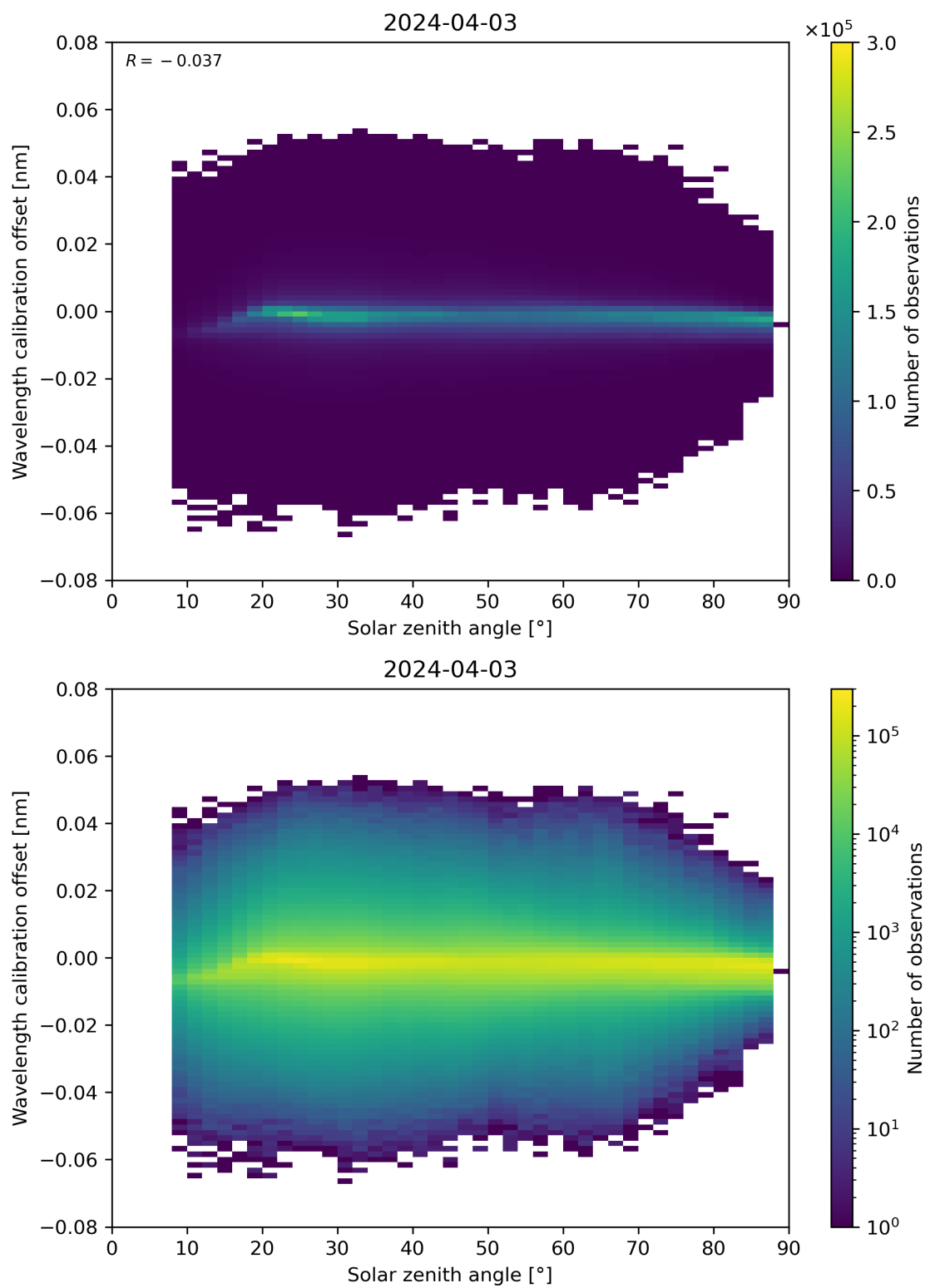
Figure 158: Scatter density plot of “Solar zenith angle” against “Wavelength calibration offset” for 2024-04-02 to 2024-04-04.
