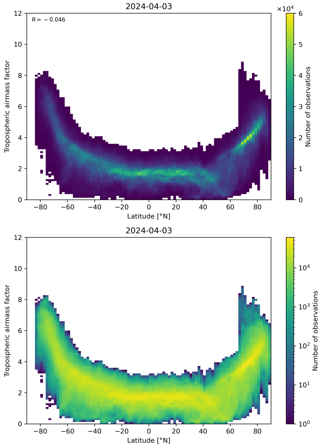
Figure 85: Scatter density plot of “Latitude” against “Tropospheric air mass factor” for 2024-04-02 to 2024-04-04.
