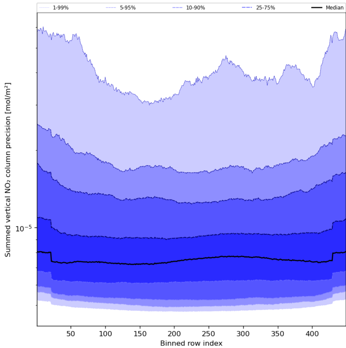
Figure 58: Along track statistics of “Summed vertical NO 2 column precision” for 2024-04-02 to 2024-04-04
