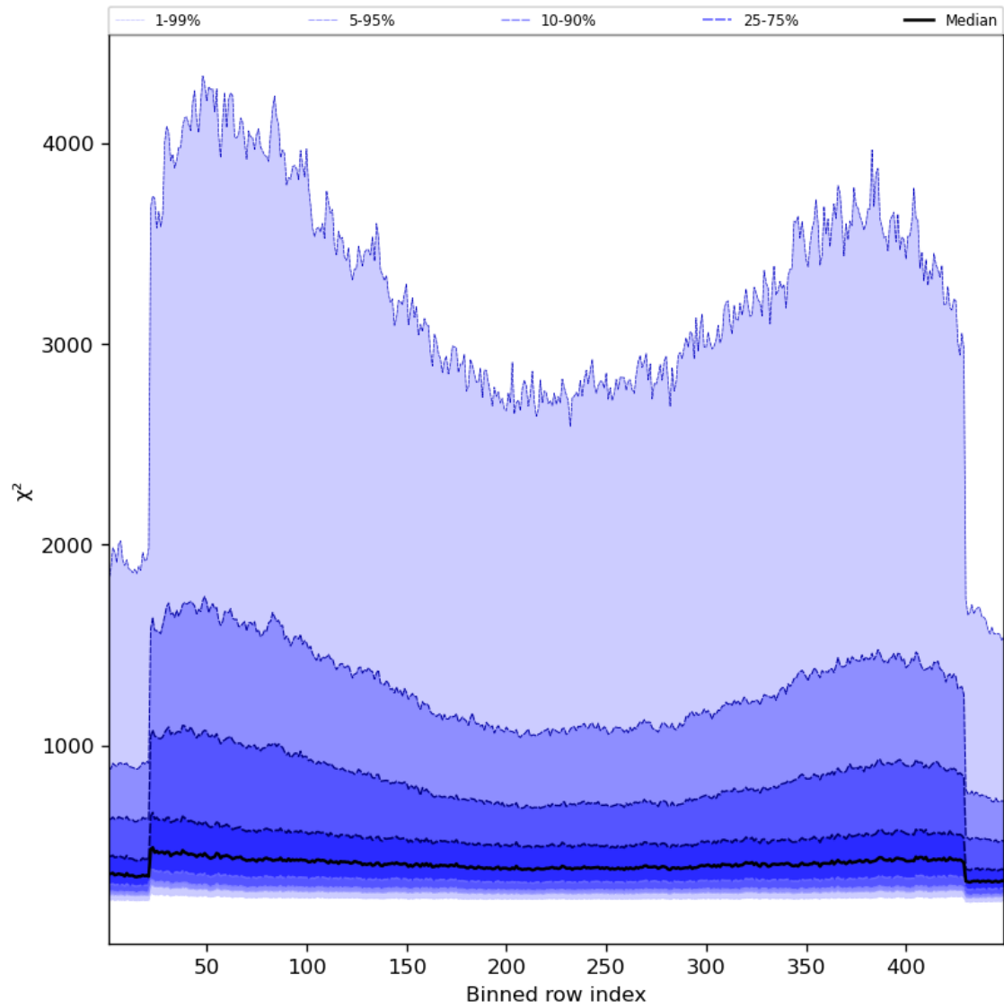
Figure 59: Along track statistics of “ \chi^2 ” for 2024-04-02 to 2024-04-04
