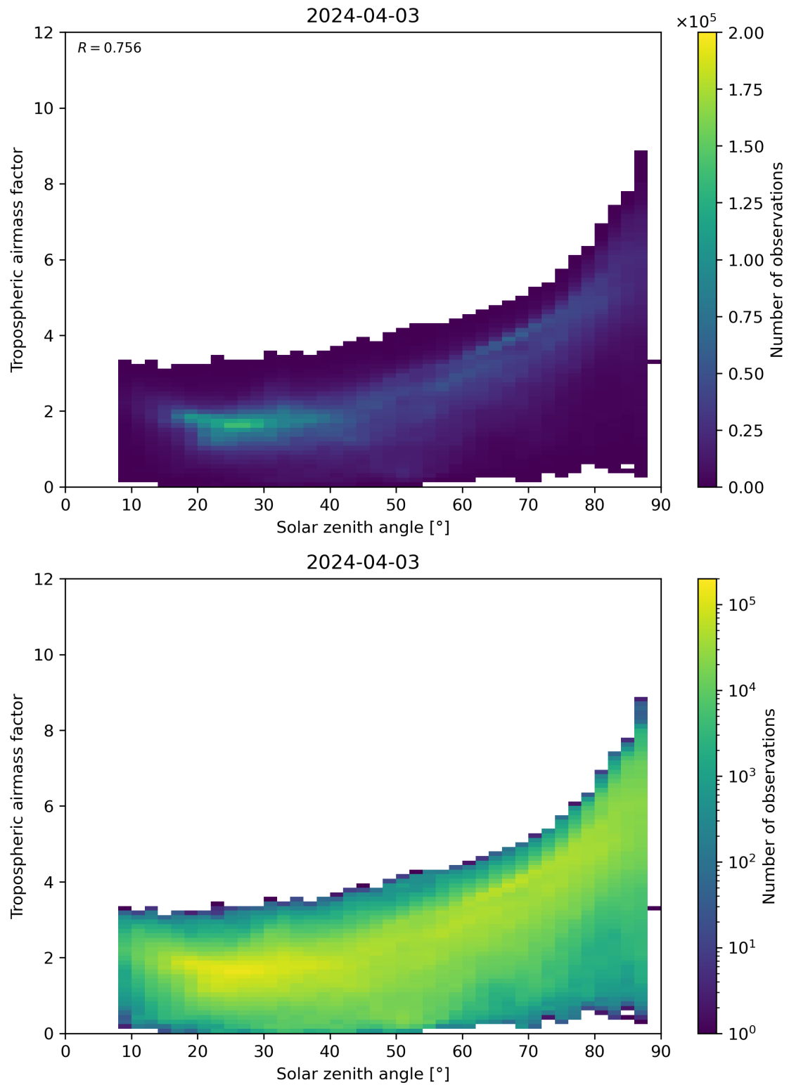
Figure 147: Scatter density plot of “Solar zenith angle” against “Tropospheric airmass factor” for 2024-04-02 to 2024-04-04.
