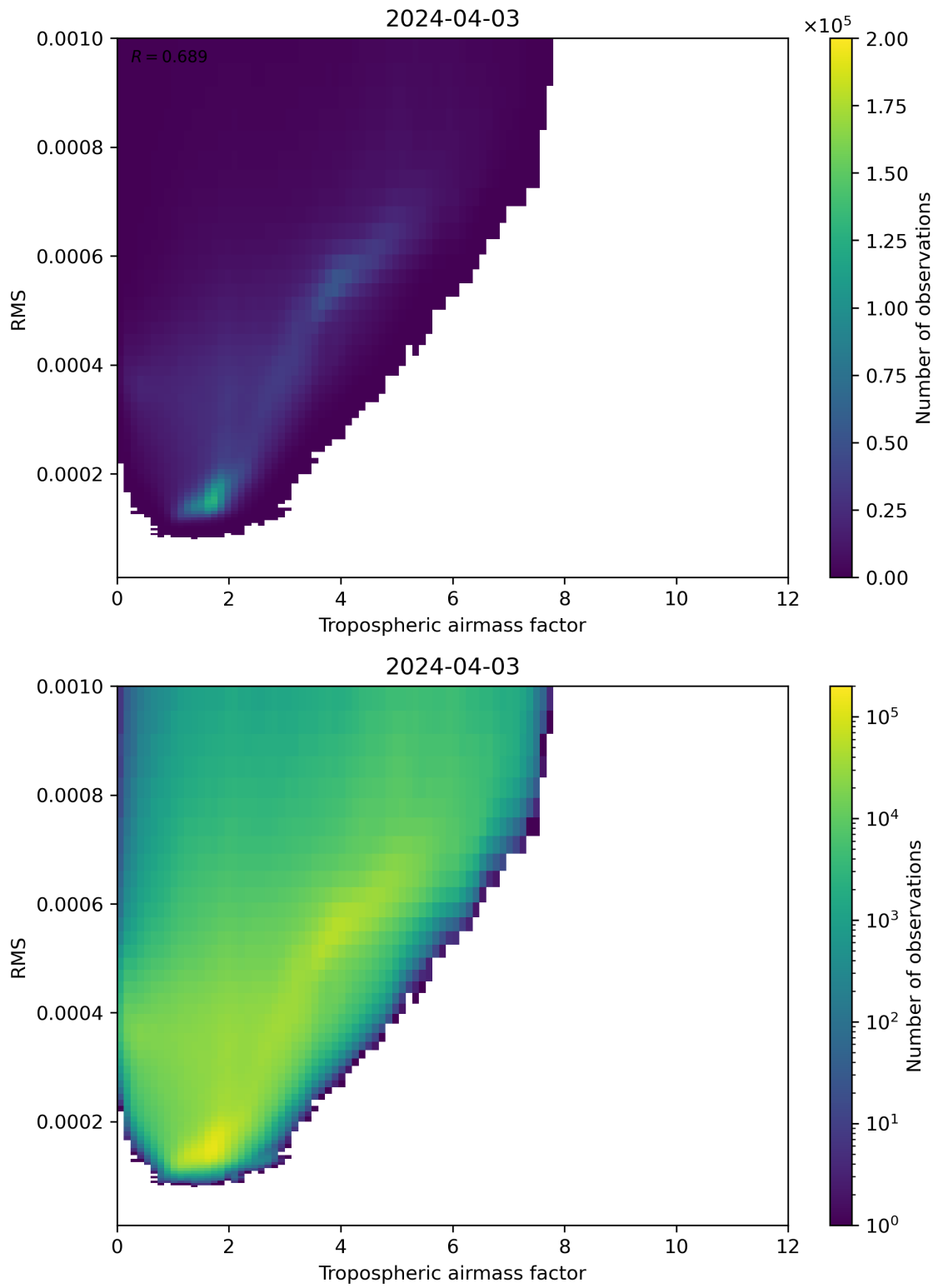
Figure 79: Scatter density plot of “Tropospheric airmass factor” against “RMS” for 2024-04-02 to 2024-04-04.
