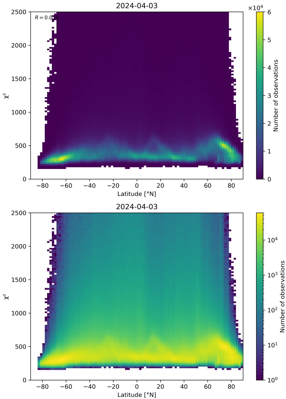
Figure 86: Scatter density plot of “Latitude” against “ \chi^2 ” for 2024-04-02 to 2024-04-04.
