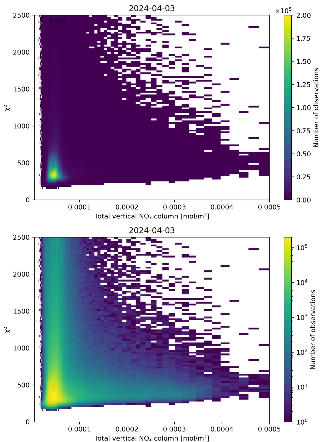
Figure 111: Scatter density plot of “Total vertical NO 2 column” against “ \chi^2 ” for 2024-04-02 to 2024-04-04.
