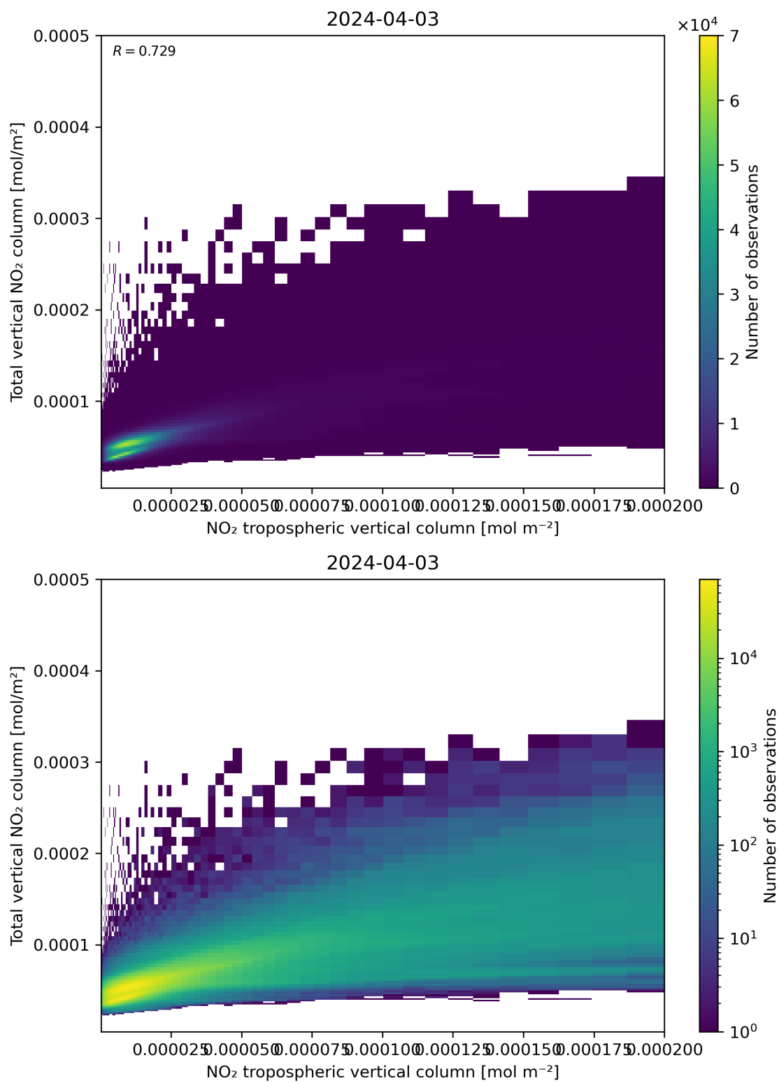
Figure 128: Scatter density plot of “NO 2 tropospheric vertical column” against “Total vertical NO 2 column” for 2024-04-02 to 2024-04-04.
