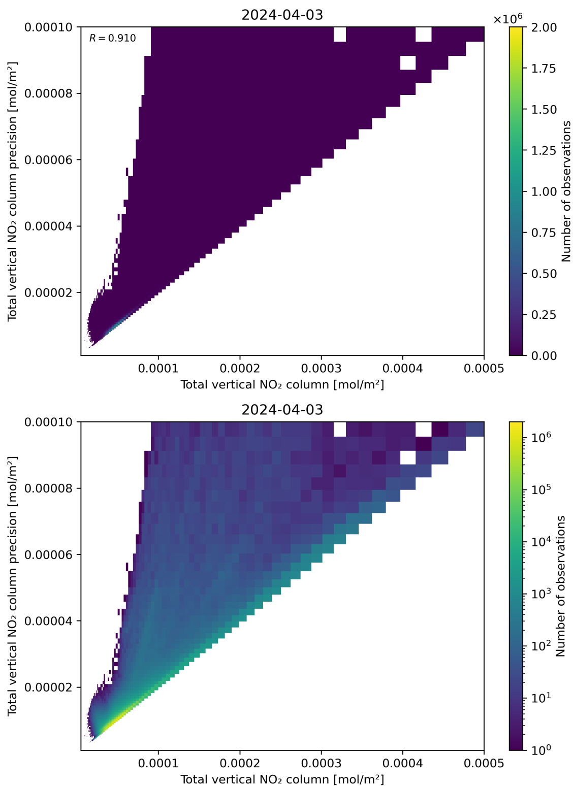
Figure 114: Scatter density plot of “Total vertical NO 2 column” against “Total vertical NO 2 column precision” for 2024-04-02 to 2024-04-04.
