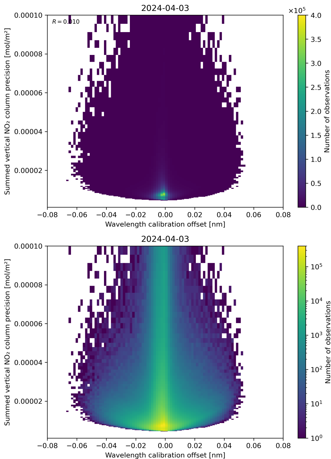
Figure 178: Scatter density plot of “Wavelength calibration offset” against “Summed vertical NO 2 column precision” for 2024-04-02 to 2024-04-04.
