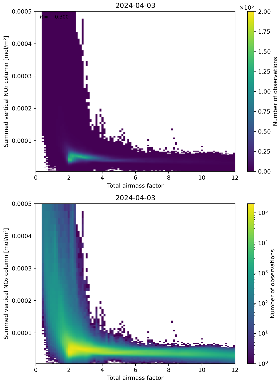
Figure 65: Scatter density plot of “Total airmass factor” against “Summed vertical NO 2 column” for 2024-04-02 to 2024-04-04.
