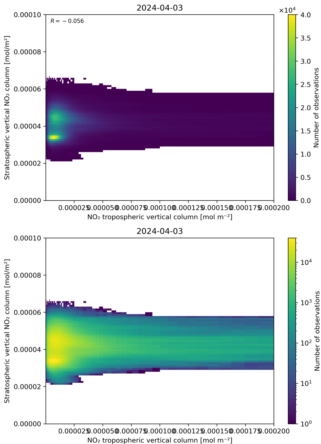
Figure 125: Scatter density plot of “NO 2 tropospheric vertical column” against “Stratospheric vertical NO 2 column” for 2024-04-02 to 2024-04-04.
