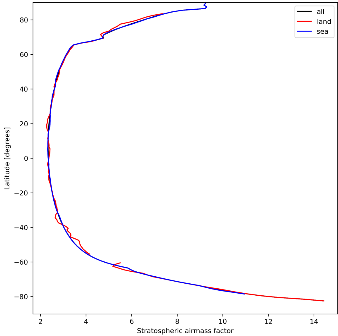
Figure 27: Zonal average of “Stratospheric airmass factor” for 2024-04-02 to 2024-04-04.
