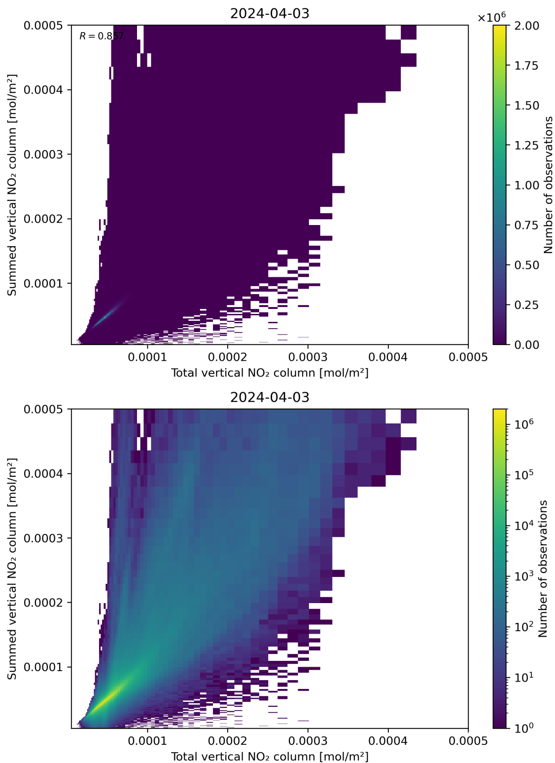
Figure 112: Scatter density plot of “Total vertical NO 2 column” against “Summed vertical NO 2 column” for 2024-04-02 to 2024-04-04.
