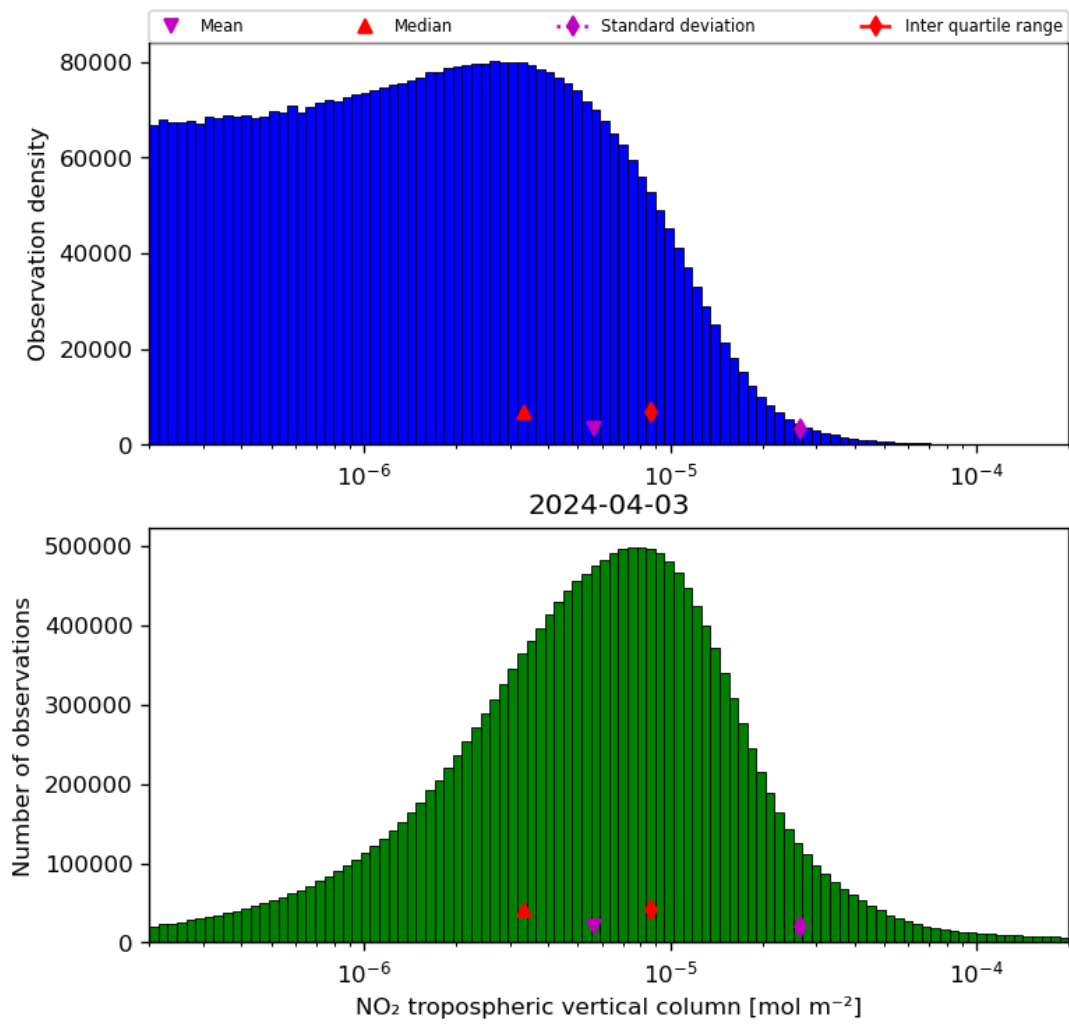
Figure 29: Histogram of “NO 2 tropospheric vertical column” for 2024-04-02 to 2024-04-04
