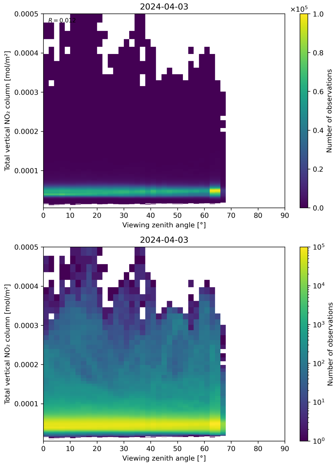
Figure 167: Scatter density plot of “Viewing zenith angle” against “Total vertical NO 2 column” for 2024-04-02 to 2024-04-04.
