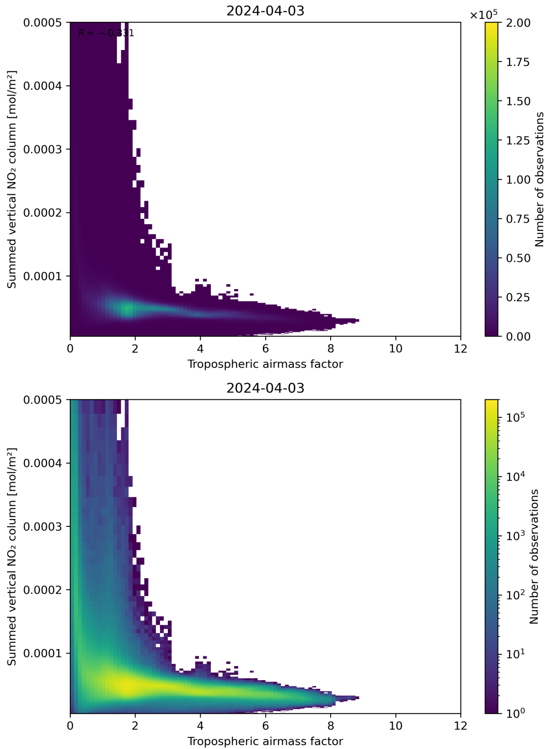
Figure 75: Scatter density plot of “Tropospheric airmass factor” against “Summed vertical NO 2 column” for 2024-04-02 to 2024-04-04.
