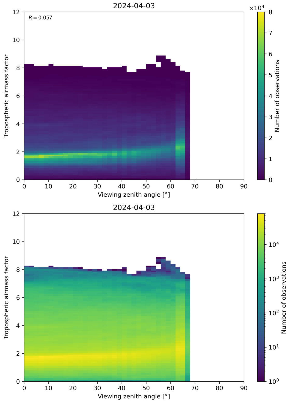
Figure 161: Scatter density plot of “Viewing zenith angle” against “Tropospheric airmass factor” for 2024-04-02 to 2024-04-04.
