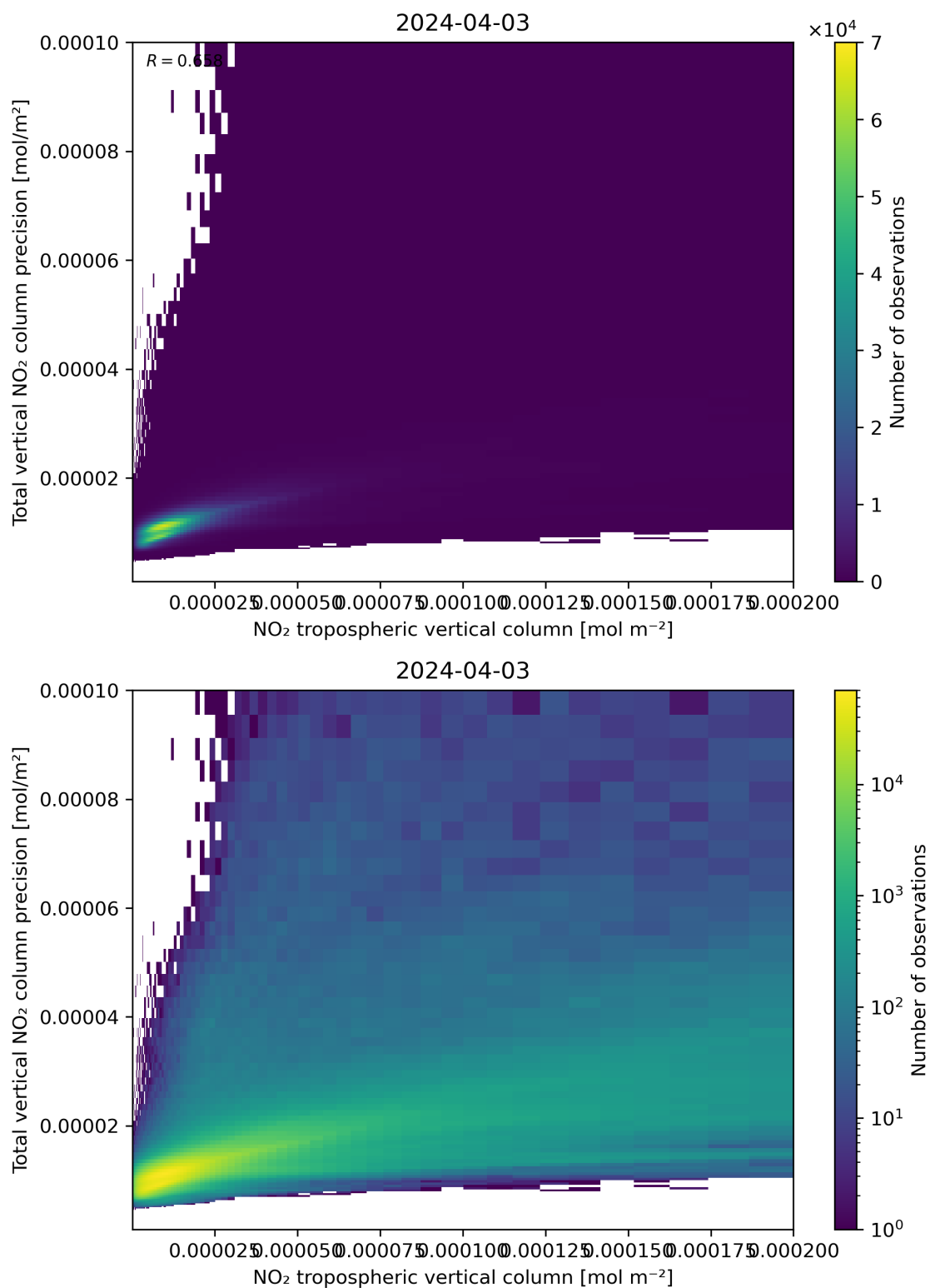
Figure 129: Scatter density plot of “NO 2 tropospheric vertical column” against “Total vertical NO 2 column precision” for 2024-04-02 to 2024-04-04.
