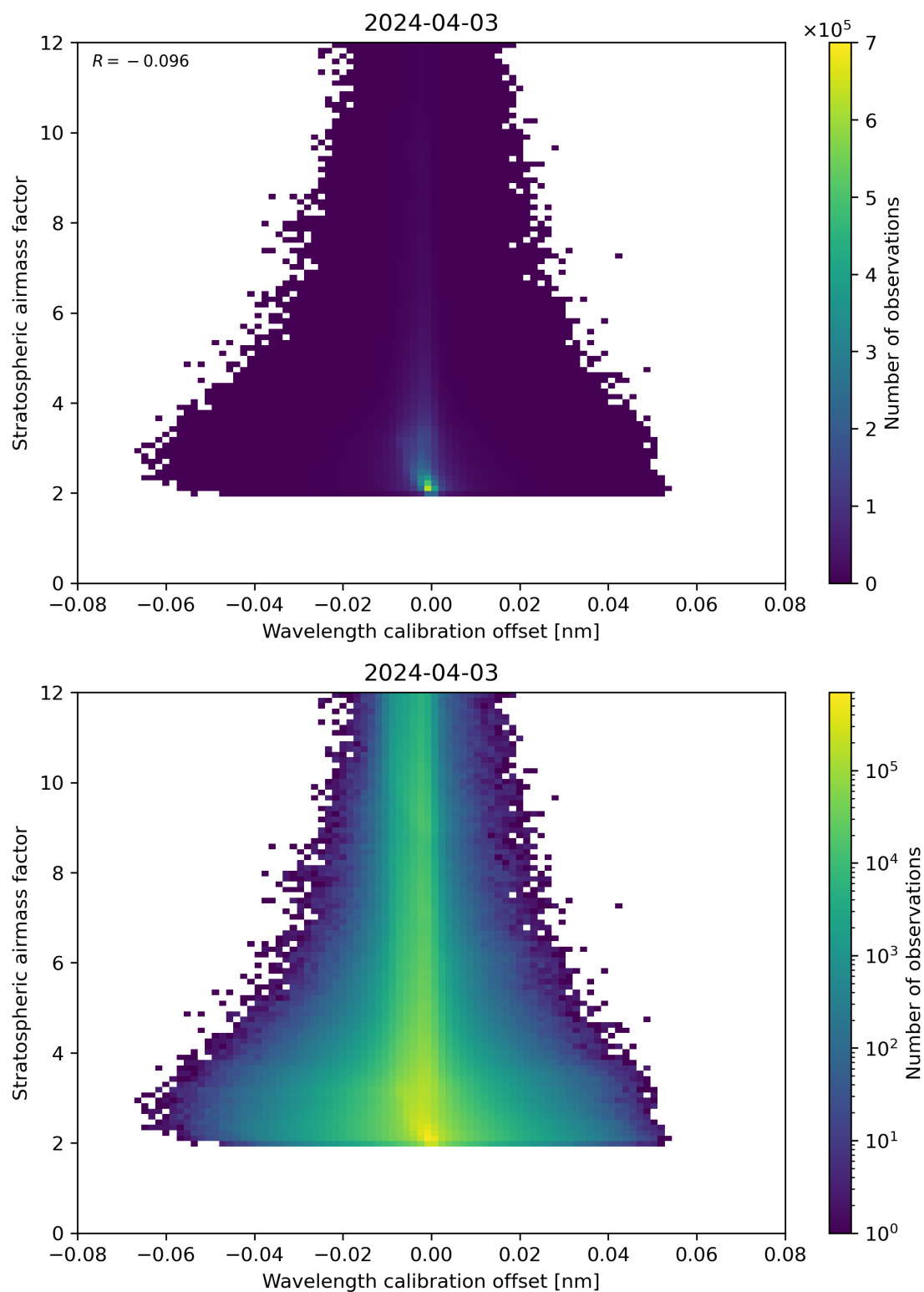
Figure 174: Scatter density plot of “Wavelength calibration offset” against “Stratospheric airmass factor” for 2024-04-02 to 2024-04-04.
