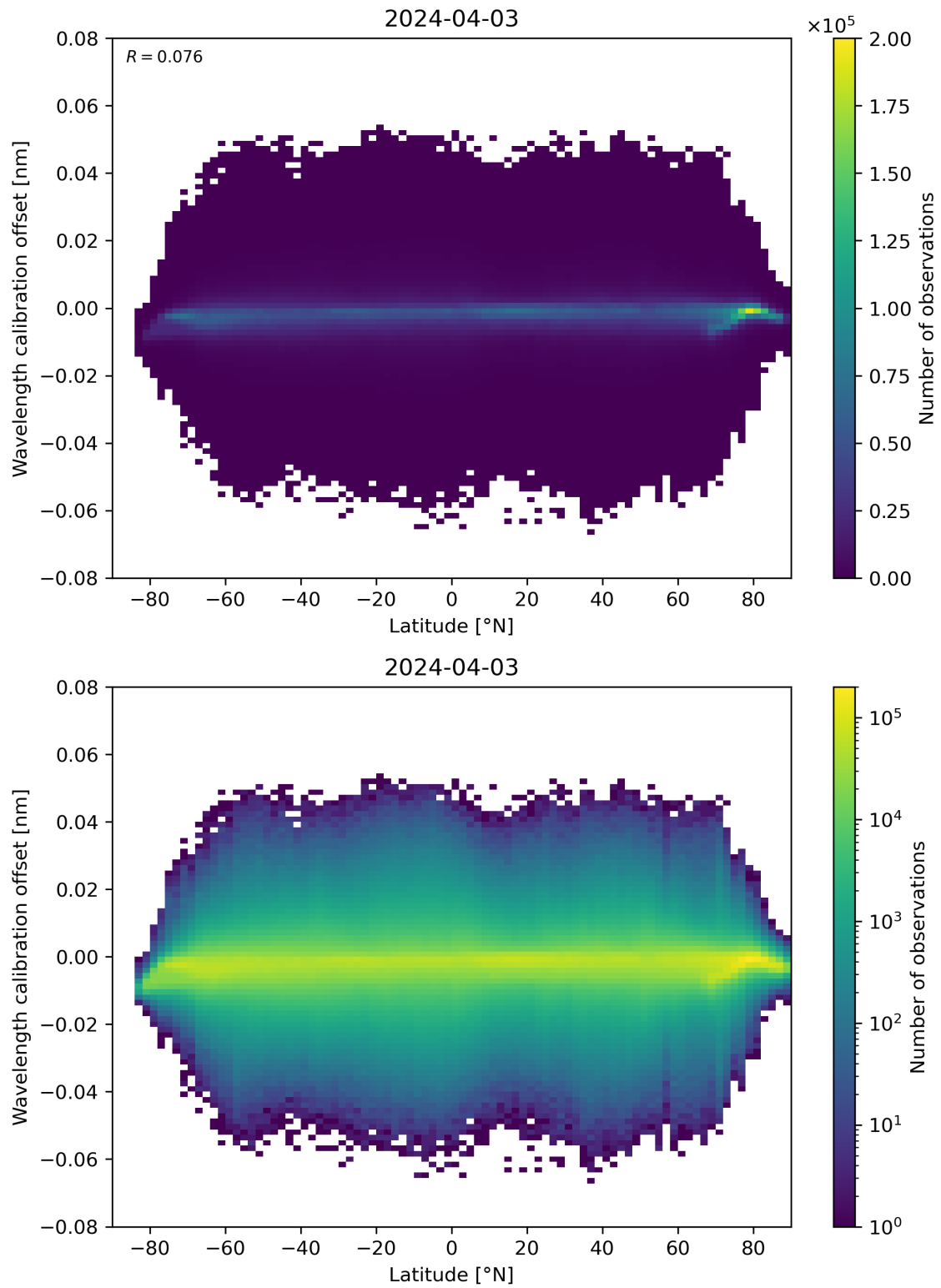
Figure 95: Scatter density plot of “Latitude” against “Wavelength calibration offset” for 2024-04-02 to 2024-04-04.
