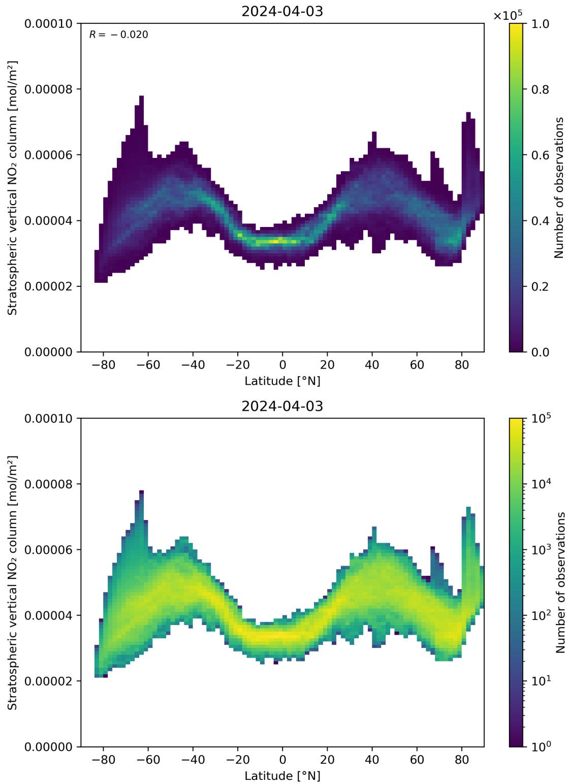
Figure 87: Scatter density plot of “Latitude” against “Stratospheric vertical NO 2 column” for 2024-04-02 to 2024-04-04.
