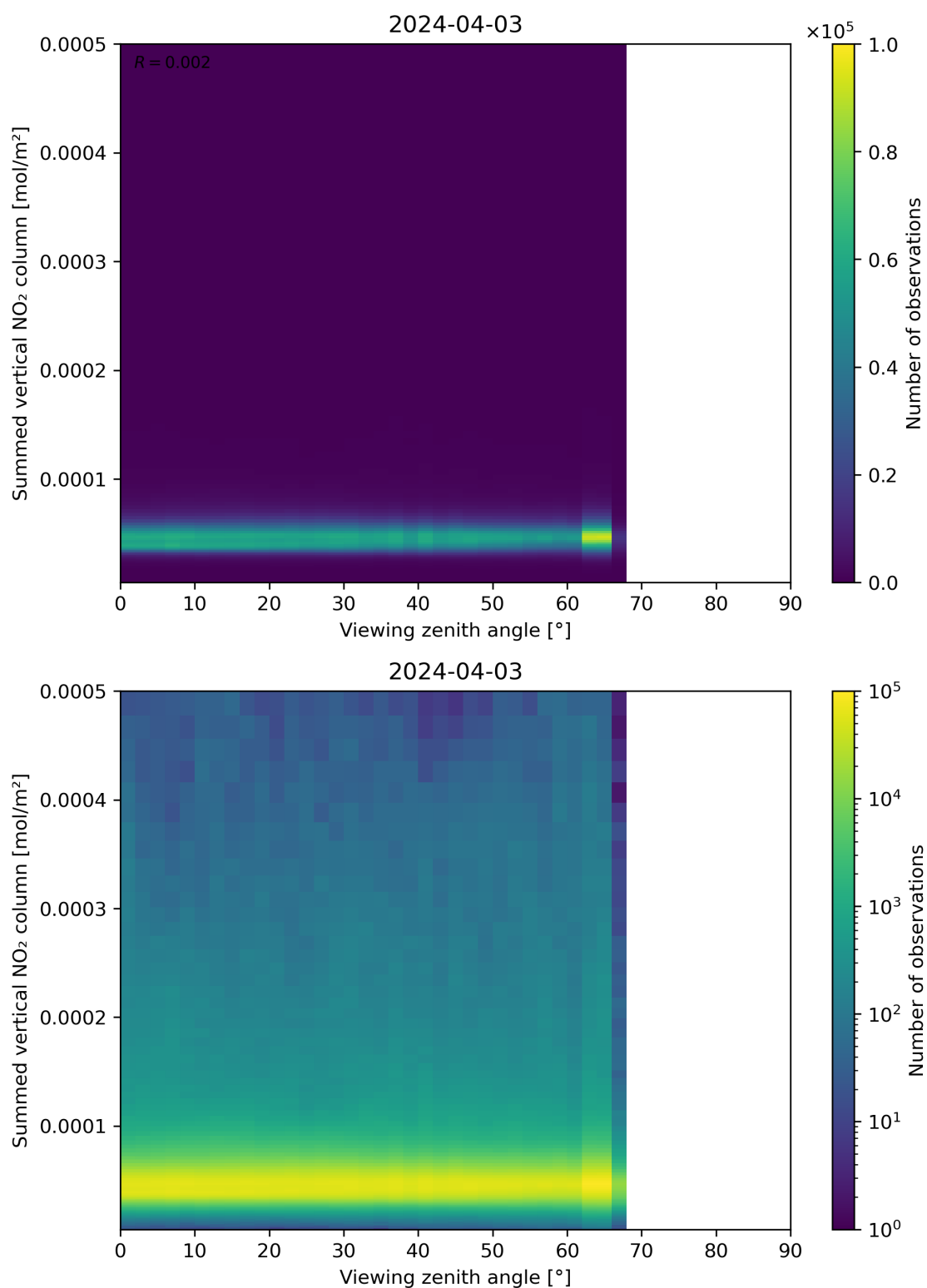
Figure 165: Scatter density plot of “Viewing zenith angle” against “Summed vertical NO 2 column” for 2024-04-02 to 2024-04-04.
