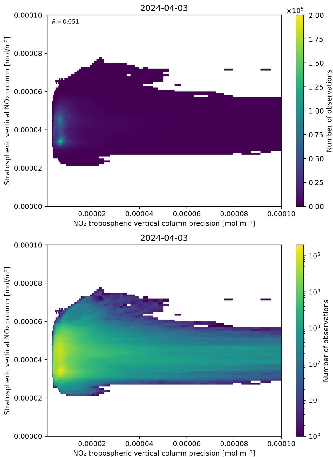
Figure 135: Scatter density plot of “NO 2 tropospheric vertical column precision” against “Stratospheric vertical NO 2 column” for 2024-04-02 to 2024-04-04.
