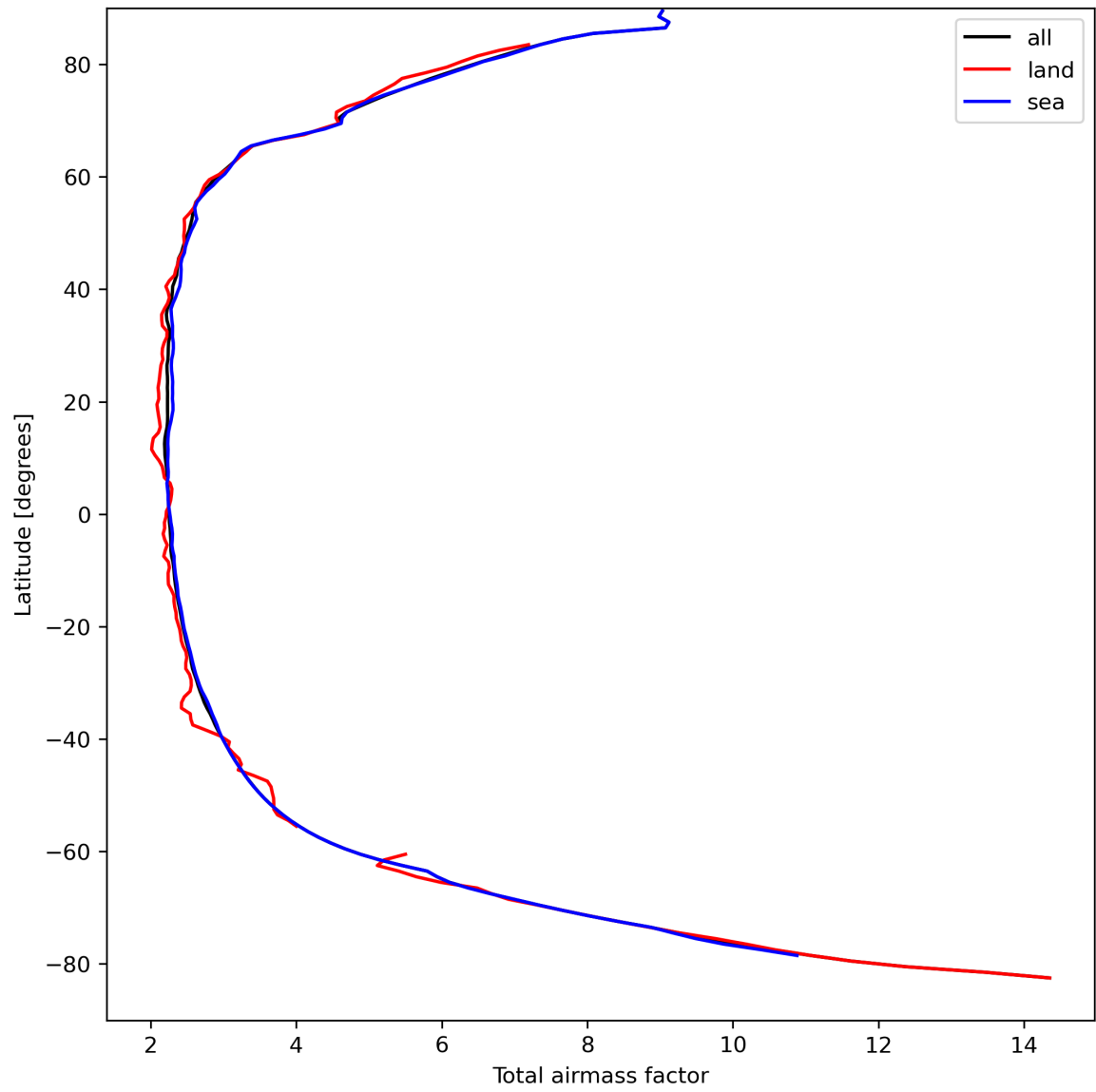
Figure 15: Zonal average of “Total airmass factor” for 2024-04-02 to 2024-04-04.
