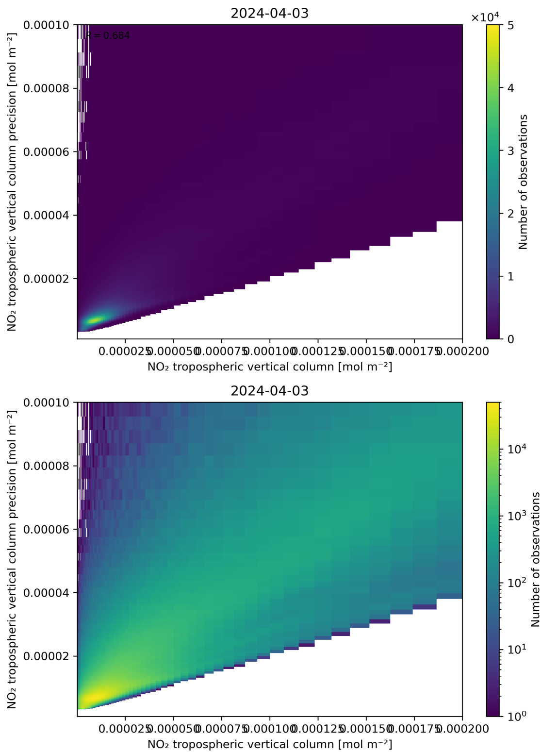
Figure 130: Scatter density plot of “NO 2 tropospheric vertical column” against “NO 2 tropospheric vertical column precision” for 2024-04-02 to 2024-04-04.
