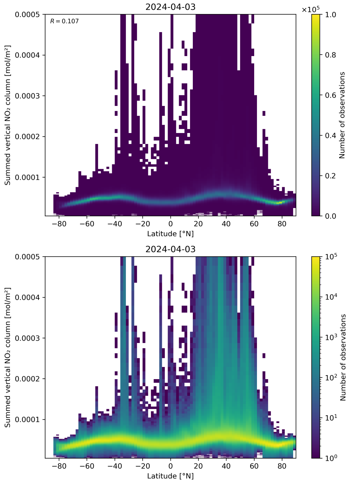
Figure 88: Scatter density plot of “Latitude” against “Summed vertical NO 2 column” for 2024-04-02 to 2024-04-04.
