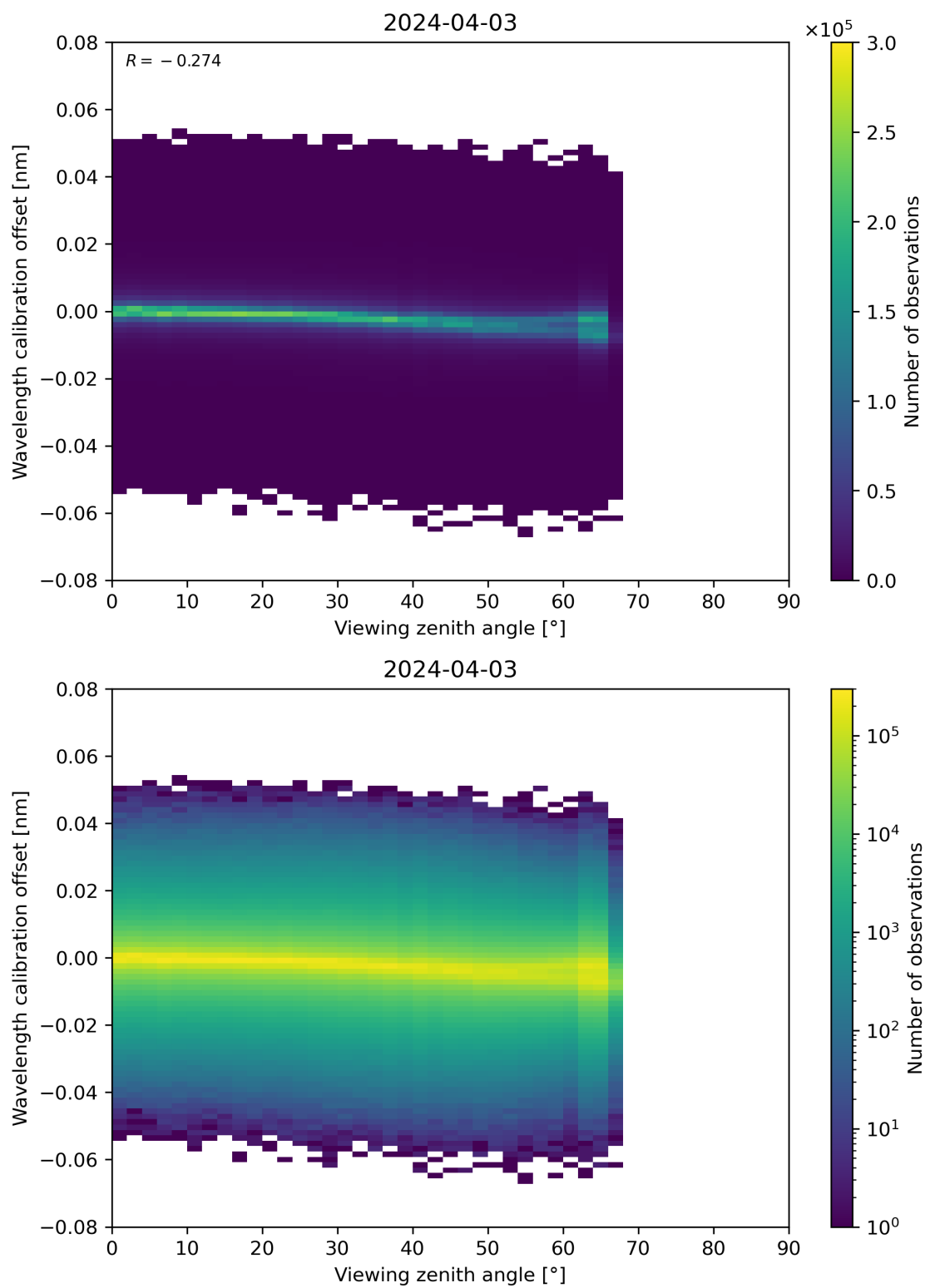
Figure 173: Scatter density plot of “Viewing zenith angle” against “Wavelength calibration offset” for 2024-04-02 to 2024-04-04.
