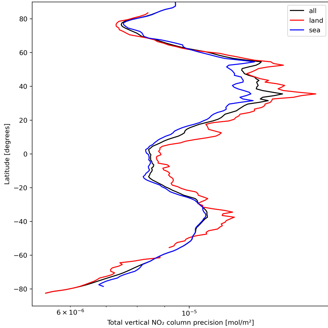
Figure 22: Zonal average of “Total vertical NO 2 column precision” for 2024-04-02 to 2024-04-04.
