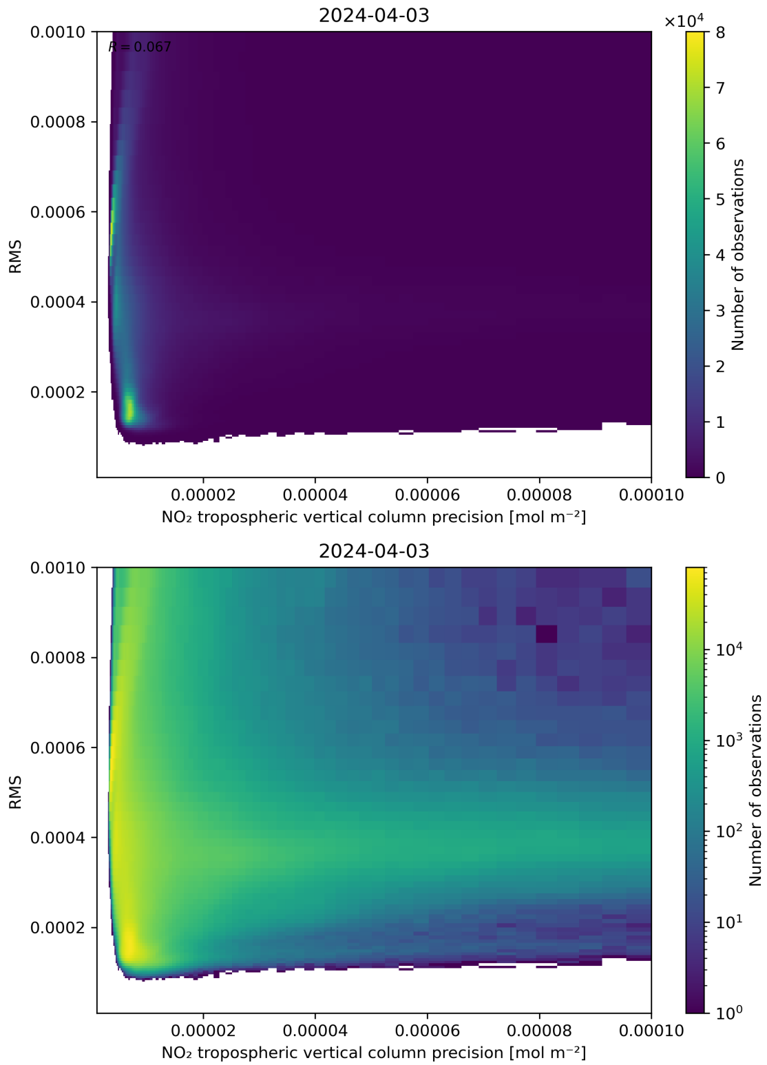
Figure 140: Scatter density plot of “NO 2 tropospheric vertical column precision” against “RMS” for 2024-04-02 to 2024-04-04.
