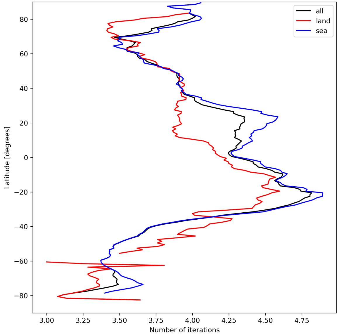
Figure 17: Zonal average of “Number of iterations” for 2024-04-02 to 2024-04-04.
