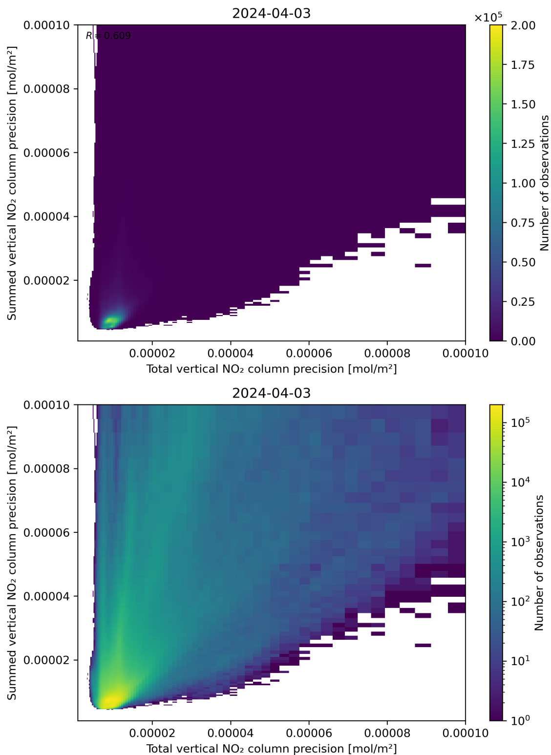
Figure 118: Scatter density plot of “Total vertical NO 2 column precision” against “Summed vertical NO 2 column precision” for 2024-04-02 to 2024-04-04.
