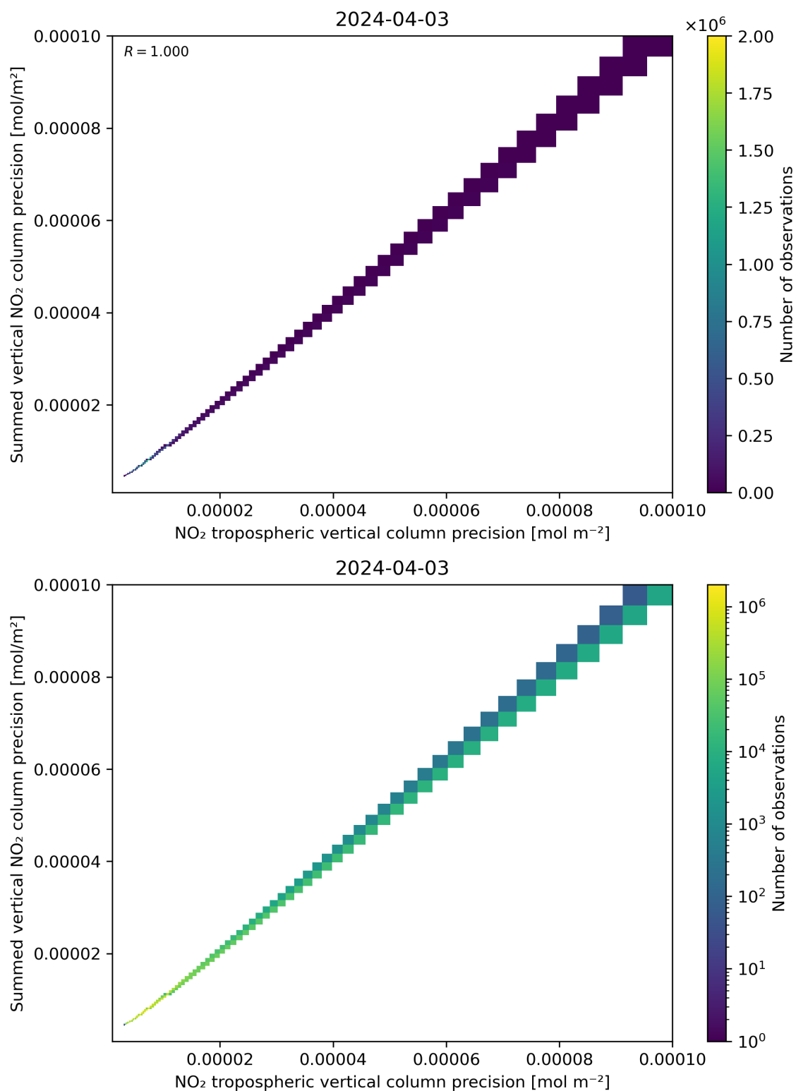
Figure 137: Scatter density plot of “NO 2 tropospheric vertical column precision” against “Summed vertical NO 2 column precision” for 2024-04-02 to 2024-04-04.
