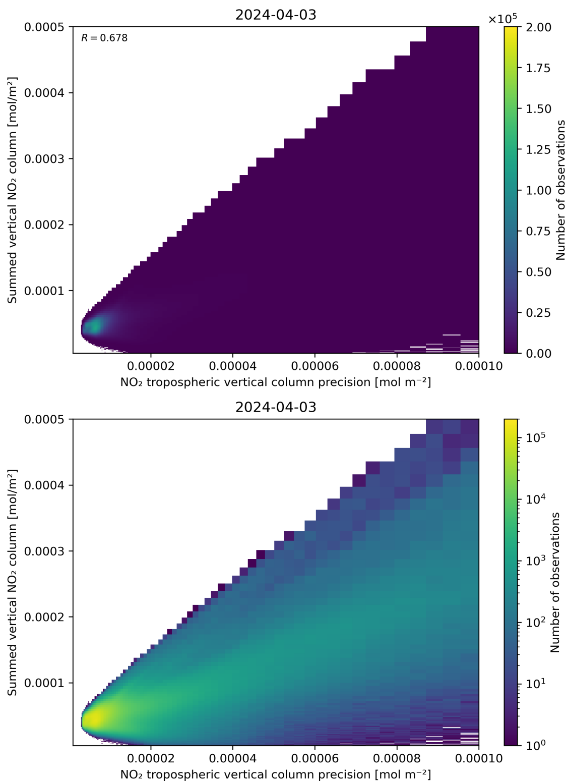
Figure 136: Scatter density plot of “NO 2 tropospheric vertical column precision” against “Summed vertical NO 2 column” for 2024-04-02 to 2024-04-04.
