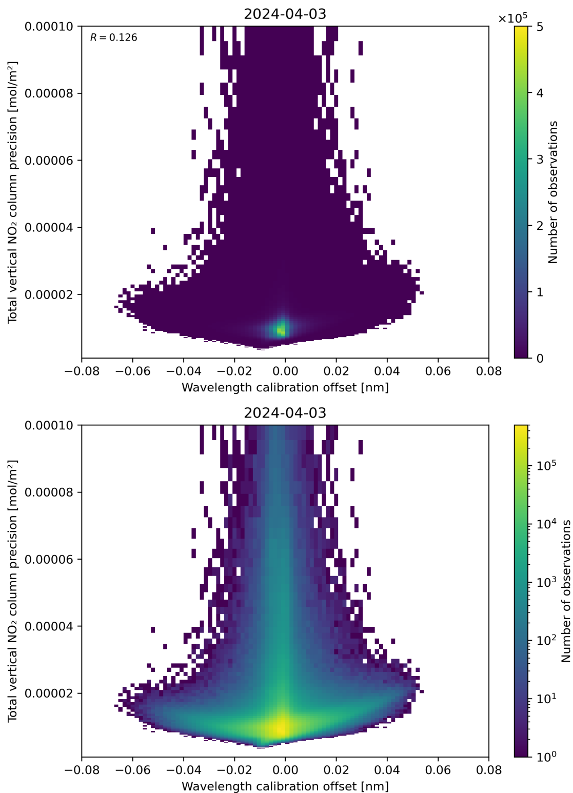
Figure 180: Scatter density plot of “Wavelength calibration offset” against “Total vertical NO 2 column precision” for 2024-04-02 to 2024-04-04.
