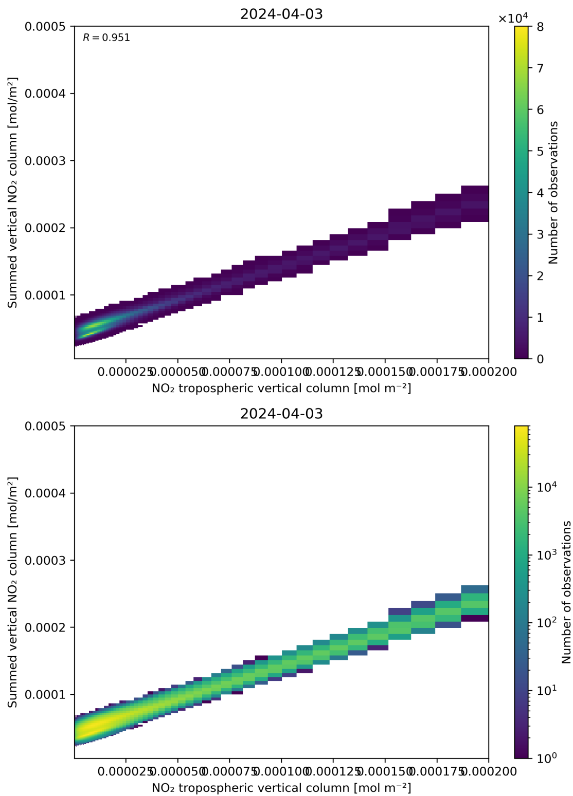
Figure 126: Scatter density plot of “NO 2 tropospheric vertical column” against “Summed vertical NO 2 column” for 2024-04-02 to 2024-04-04.
