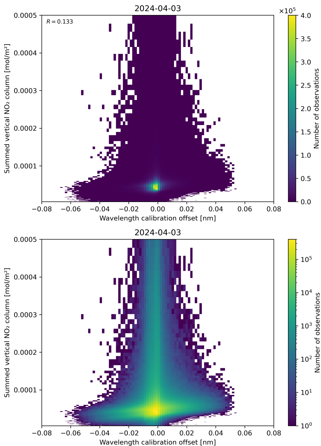
Figure 177: Scatter density plot of “Wavelength calibration offset” against “Summed vertical NO 2 column” for 2024-04-02 to 2024-04-04.
