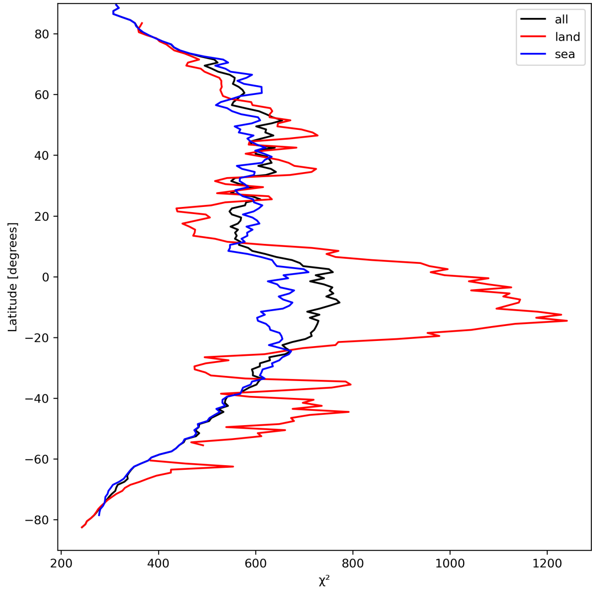
Figure 25: Zonal average of “ \chi^2 ” for 2024-04-02 to 2024-04-04.
