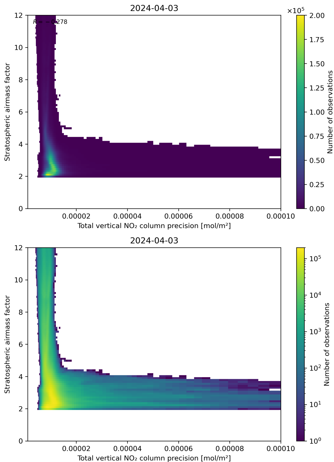
Figure 115: Scatter density plot of “Total vertical NO 2 column precision” against “Stratospheric air mass factor” for 2024-04-02 to 2024-04-04.
