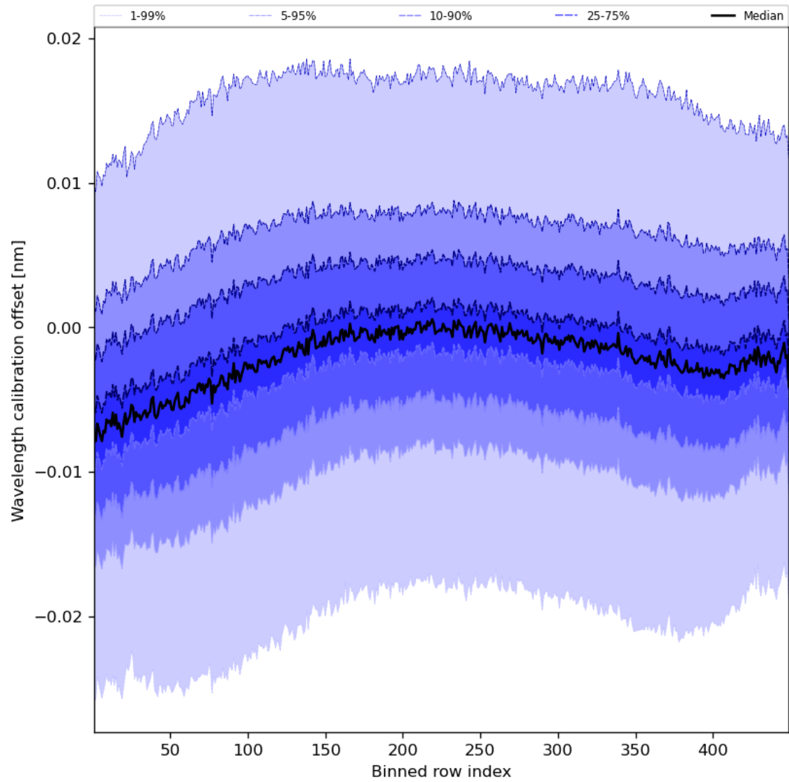
Figure 52: Along track statistics of “Wavelength calibration offset” for 2024-04-02 to 2024-04-04
