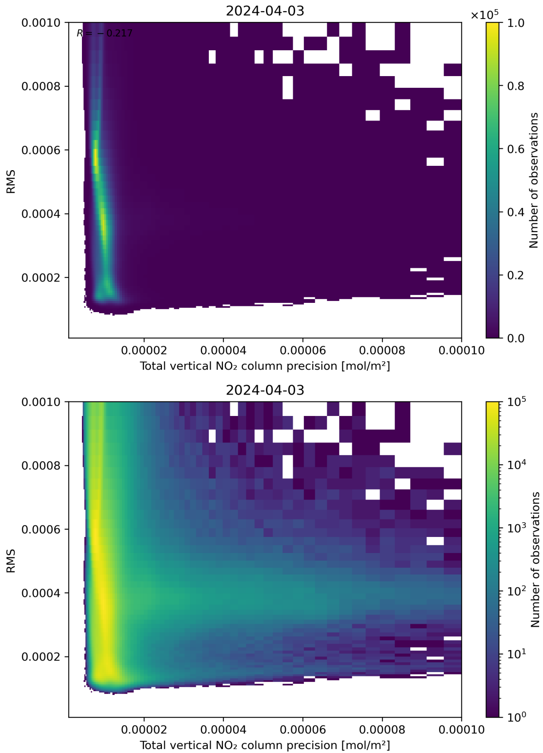
Figure 119: Scatter density plot of “Total vertical NO 2 column precision” against “RMS” for 2024-04-02 to 2024-04-04.
