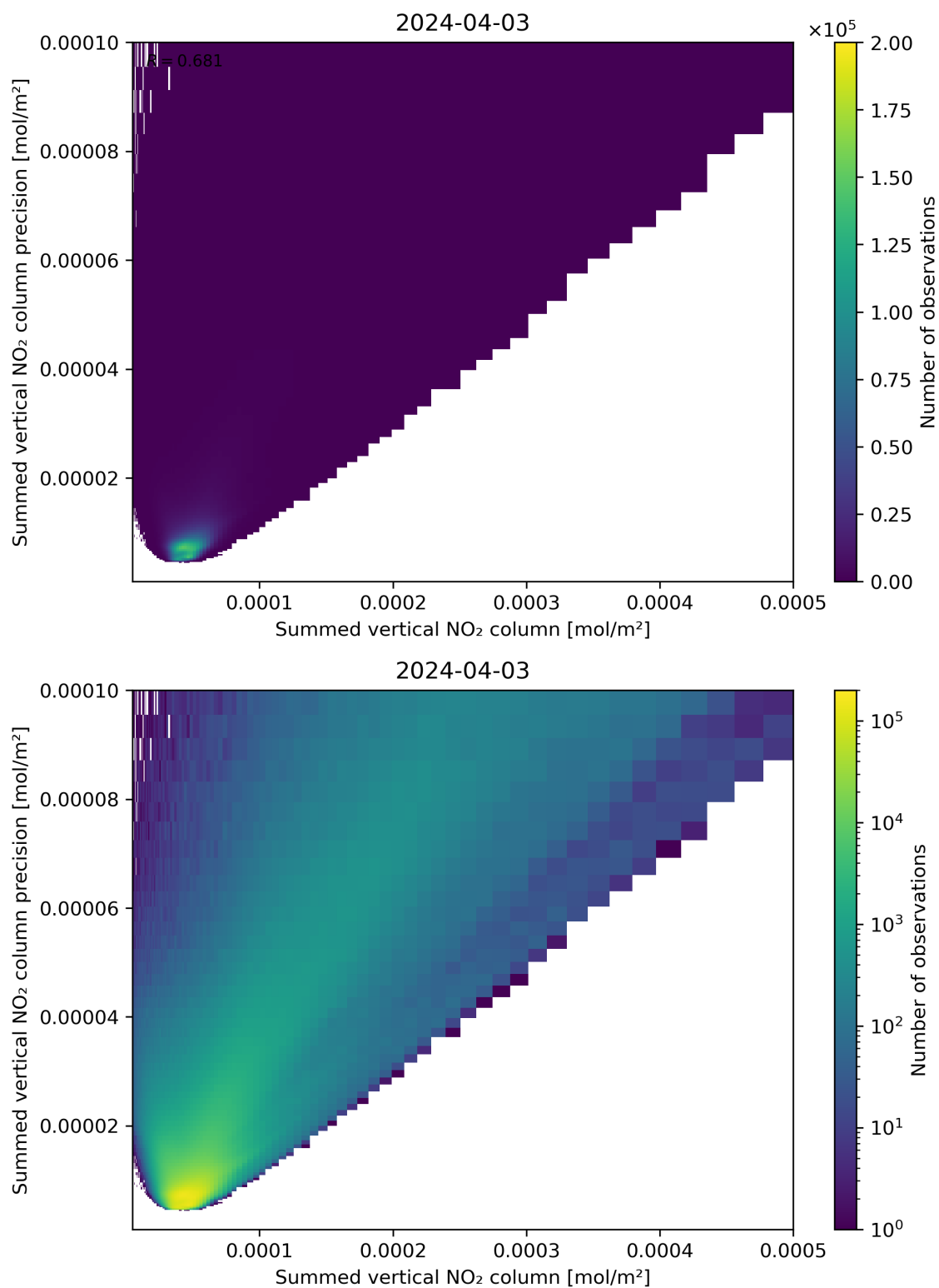
Figure 105: Scatter density plot of “Summed vertical NO 2 column” against “Summed vertical NO 2 column precision” for 2024-04-02 to 2024-04-04.
