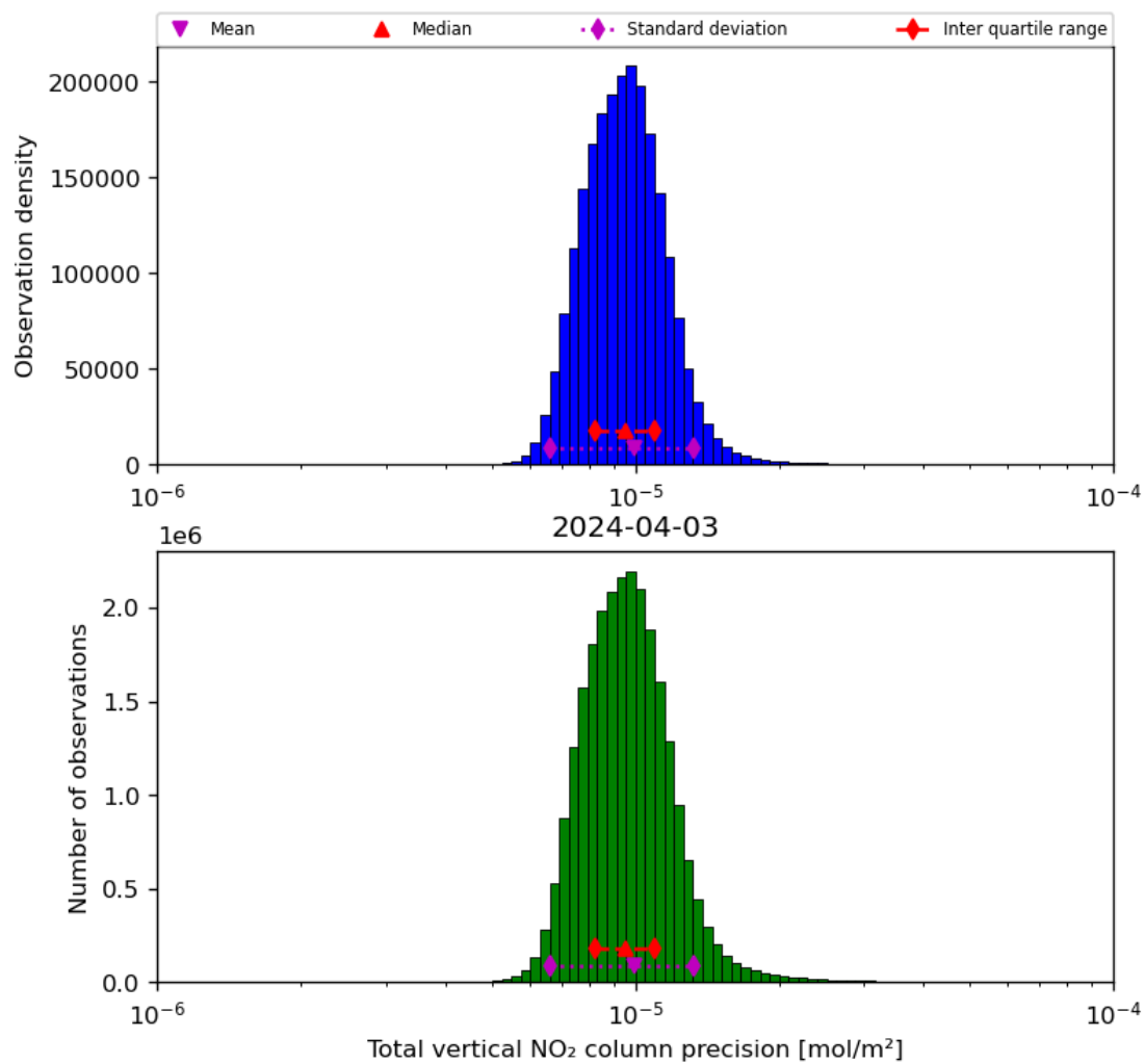
Figure 39: Histogram of “Total vertical NO 2 column precision” for 2024-04-02 to 2024-04-04
