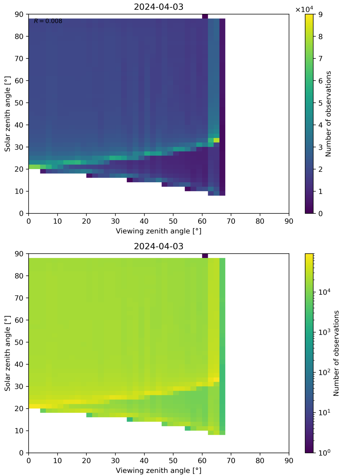
Figure 172: Scatter density plot of “Viewing zenith angle” against “Solar zenith angle” for 2024-04-02 to 2024-04-04.
