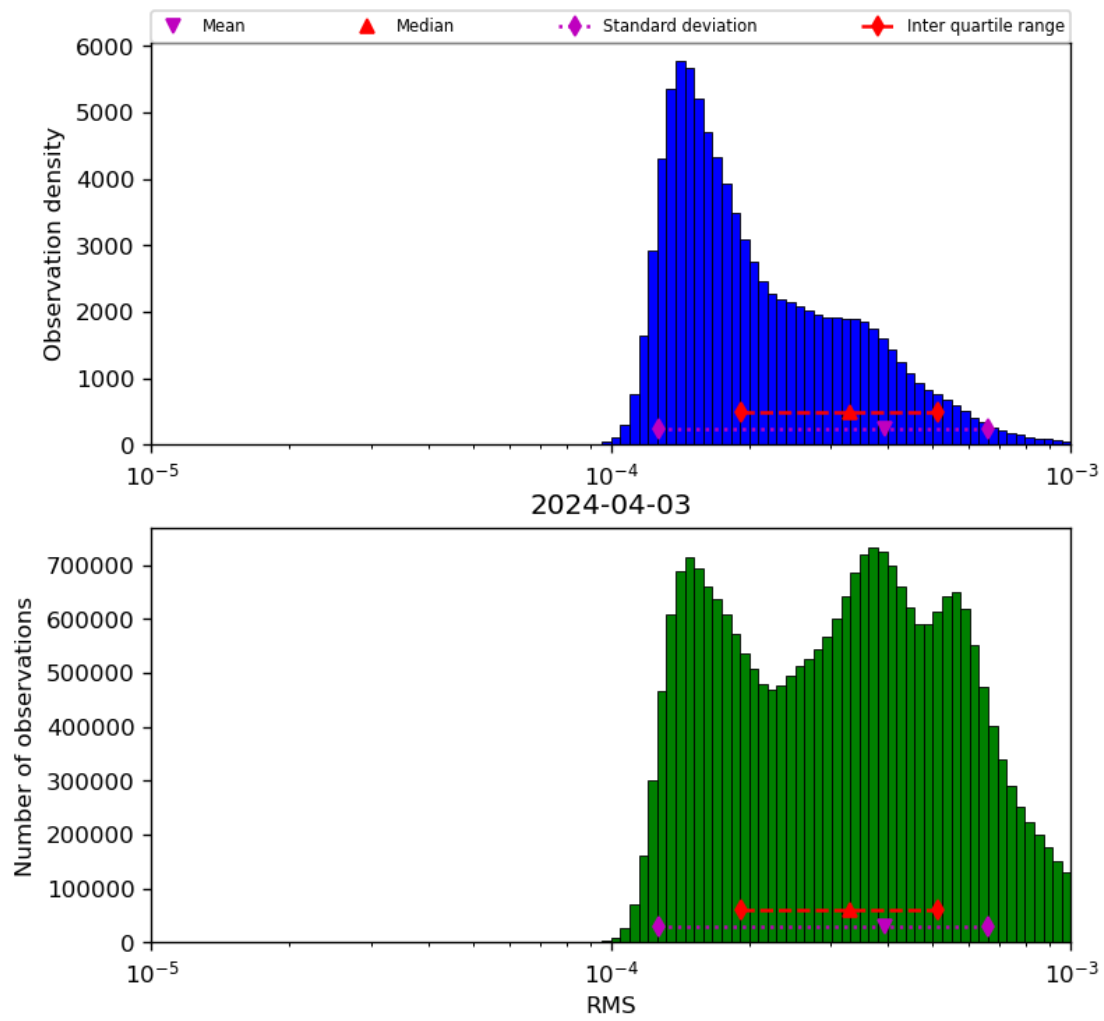
Figure 43: Histogram of “RMS” for 2024-04-02 to 2024-04-04
