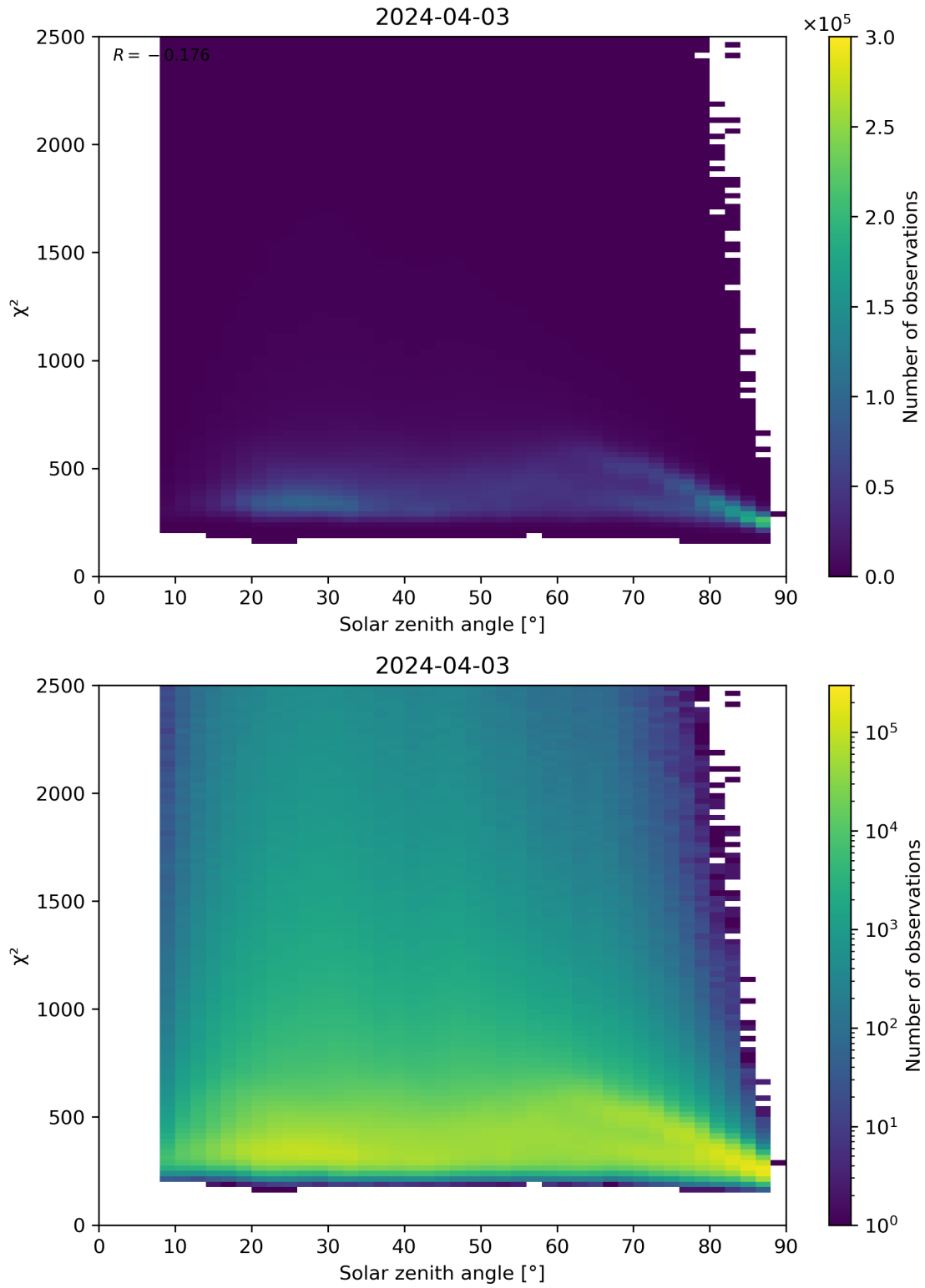
Figure 148: Scatter density plot of “Solar zenith angle” against “ \chi^2 ” for 2024-04-02 to 2024-04-04.
