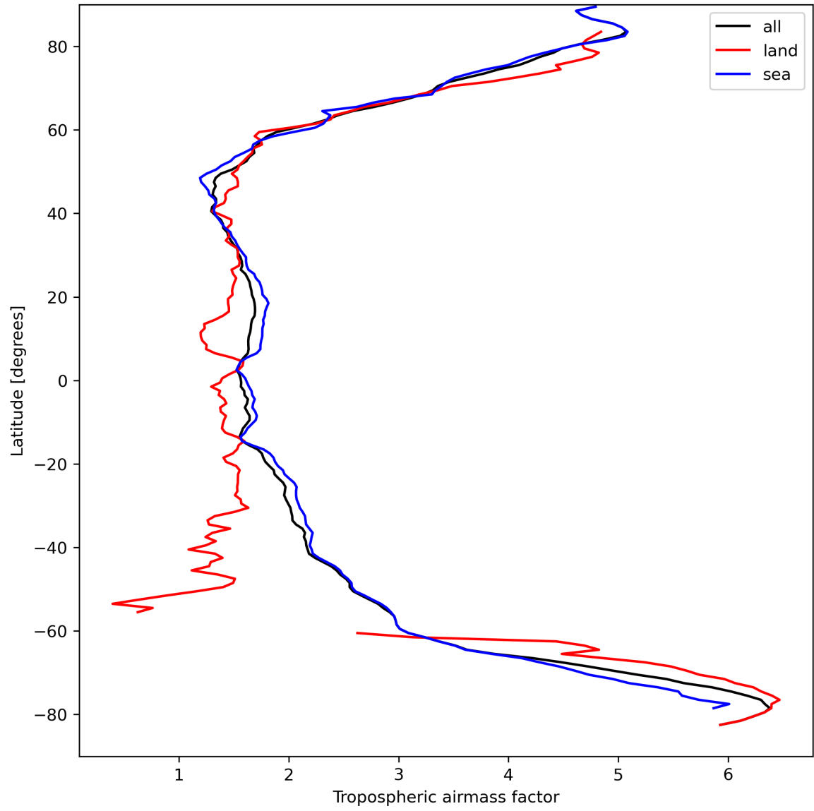
Figure 14: Zonal average of “Tropospheric airmass factor” for 2024-04-02 to 2024-04-04.
