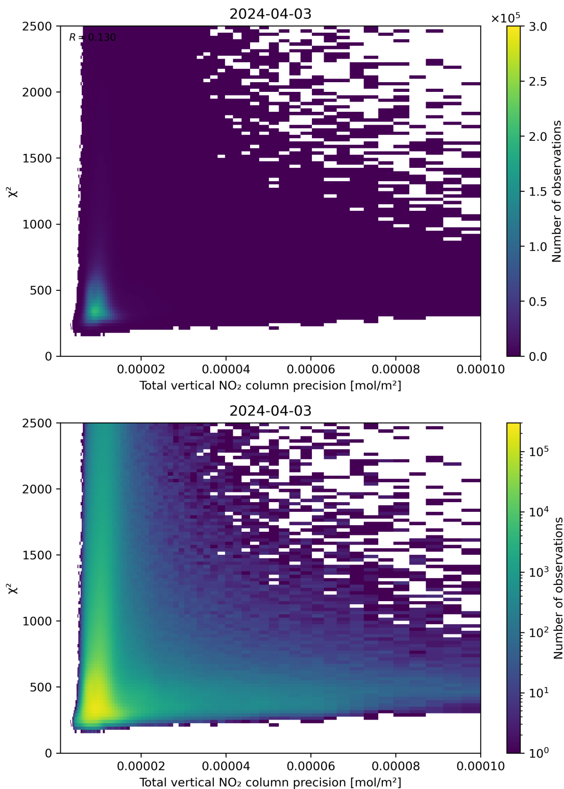
Figure 116: Scatter density plot of “Total vertical NO 2 column precision” against “ \chi^2 ” for 2024-04-02 to 2024-04-04.
