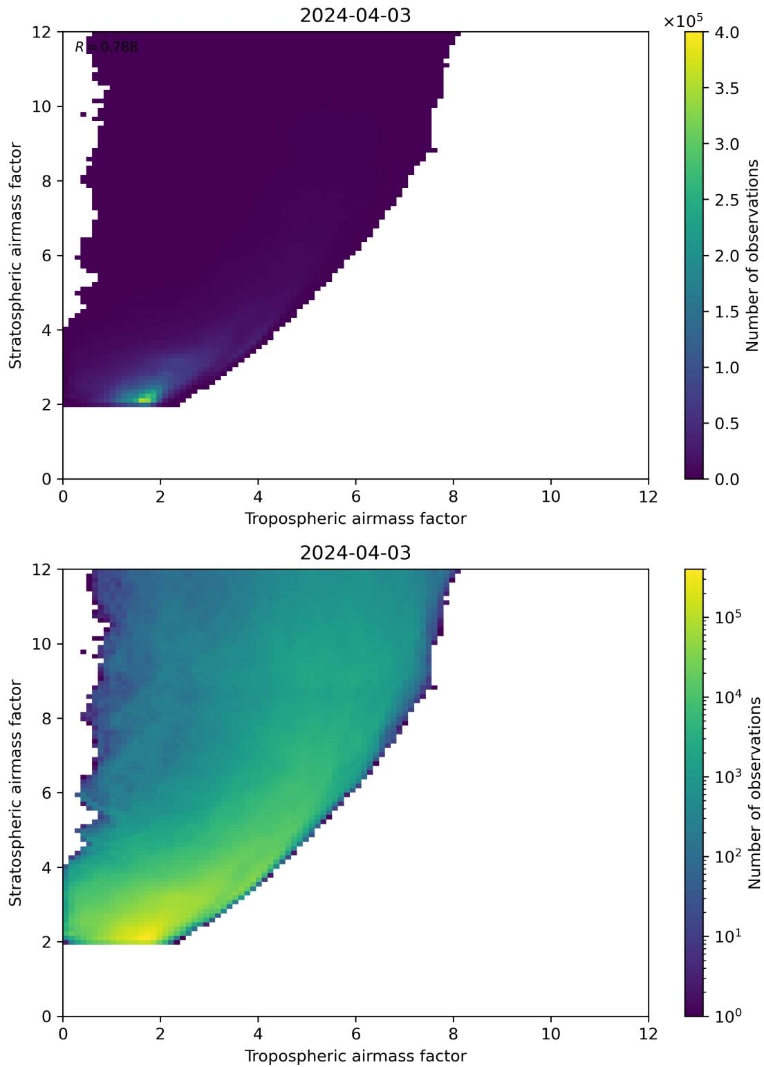
Figure 71: Scatter density plot of “Tropospheric airmass factor” against “Stratospheric airmass factor” for 2024-04-02 to 2024-04-04.
