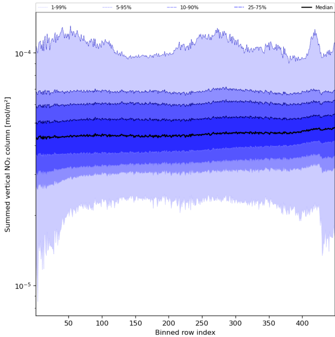
Figure 57: Along track statistics of “Summed vertical NO 2 column” for 2024-04-02 to 2024-04-04
