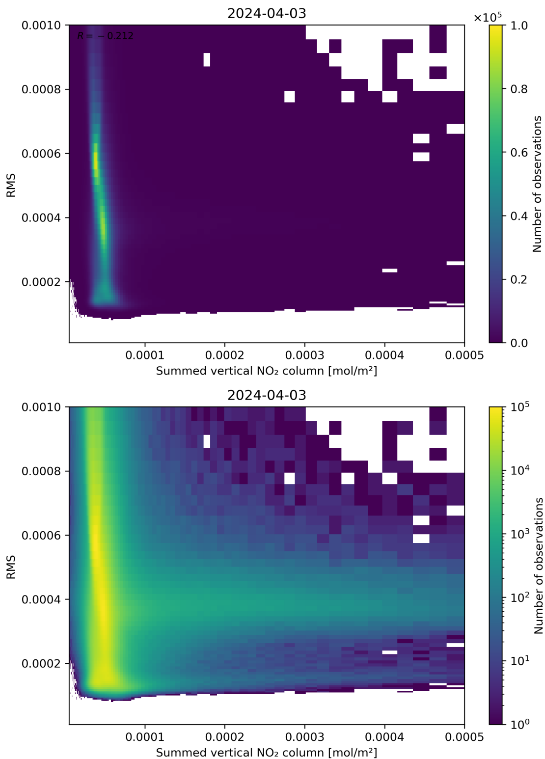
Figure 109: Scatter density plot of “Summed vertical NO 2 column” against “RMS” for 2024-04-02 to 2024-04-04.
