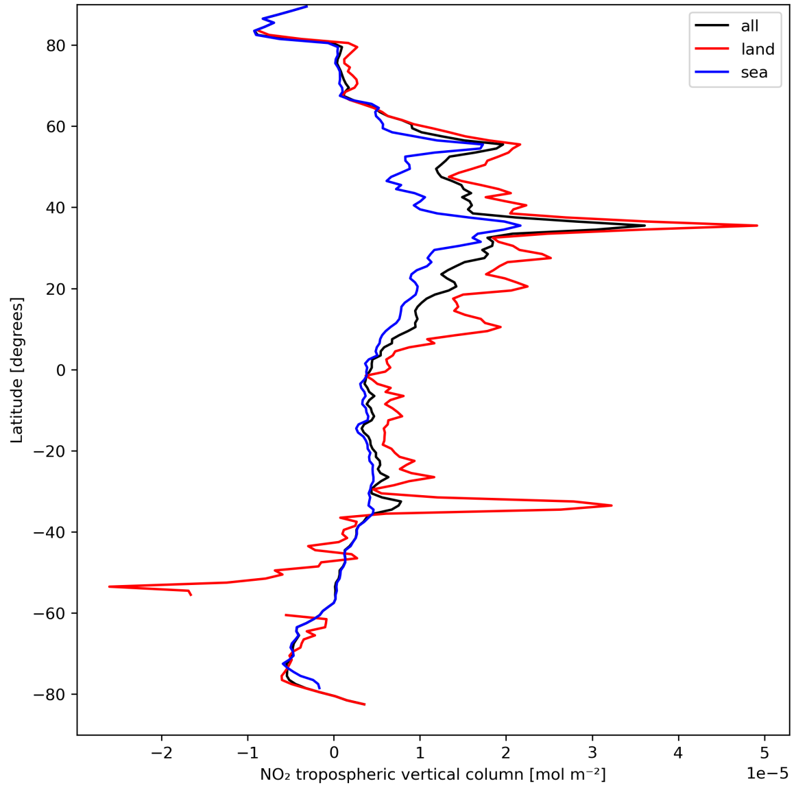
Figure 12: Zonal average of “NO 2 tropospheric vertical column” for 2024-04-02 to 2024-04-04.
