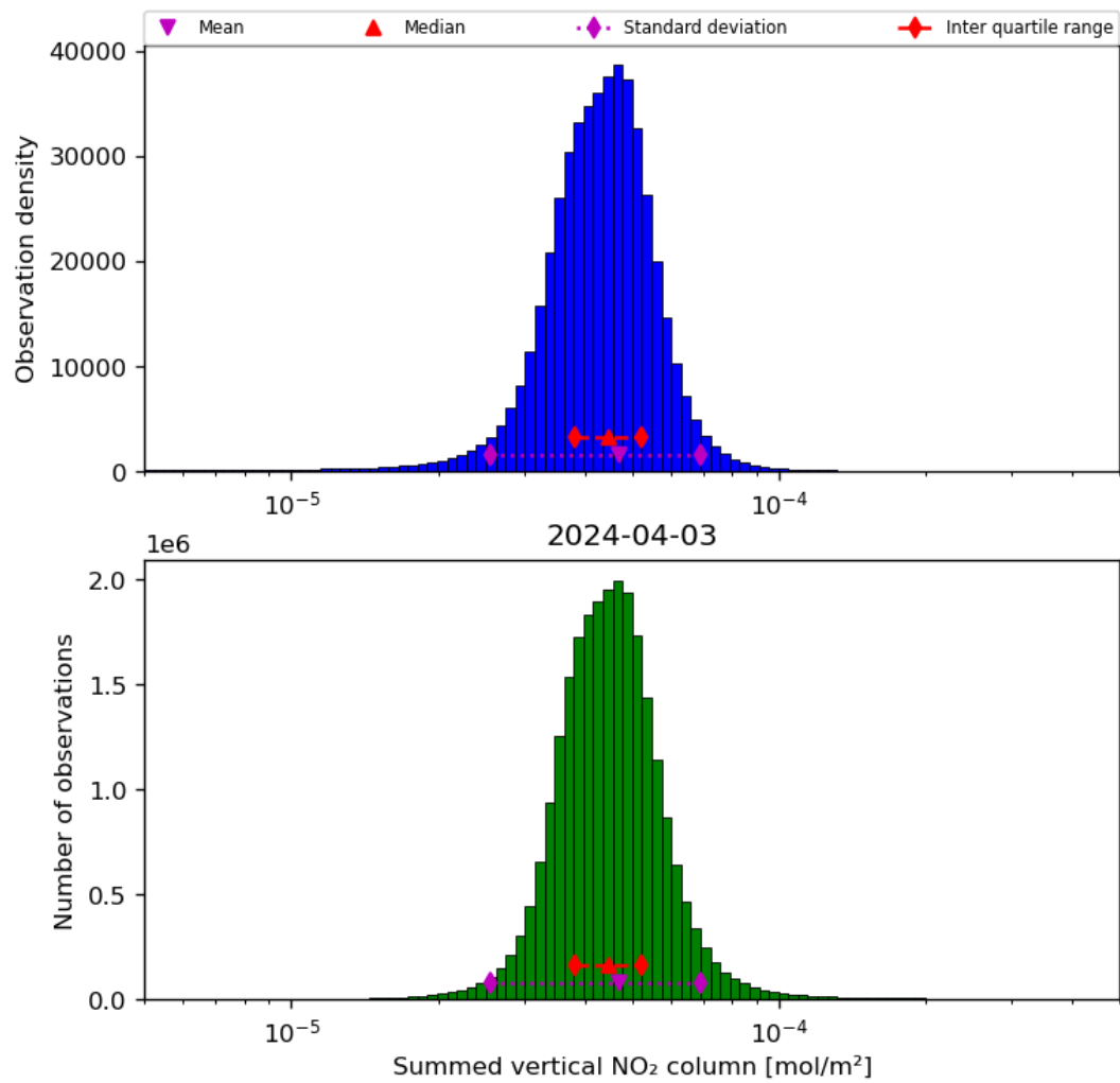
Figure 40: Histogram of “Summed vertical NO 2 column” for 2024-04-02 to 2024-04-04
