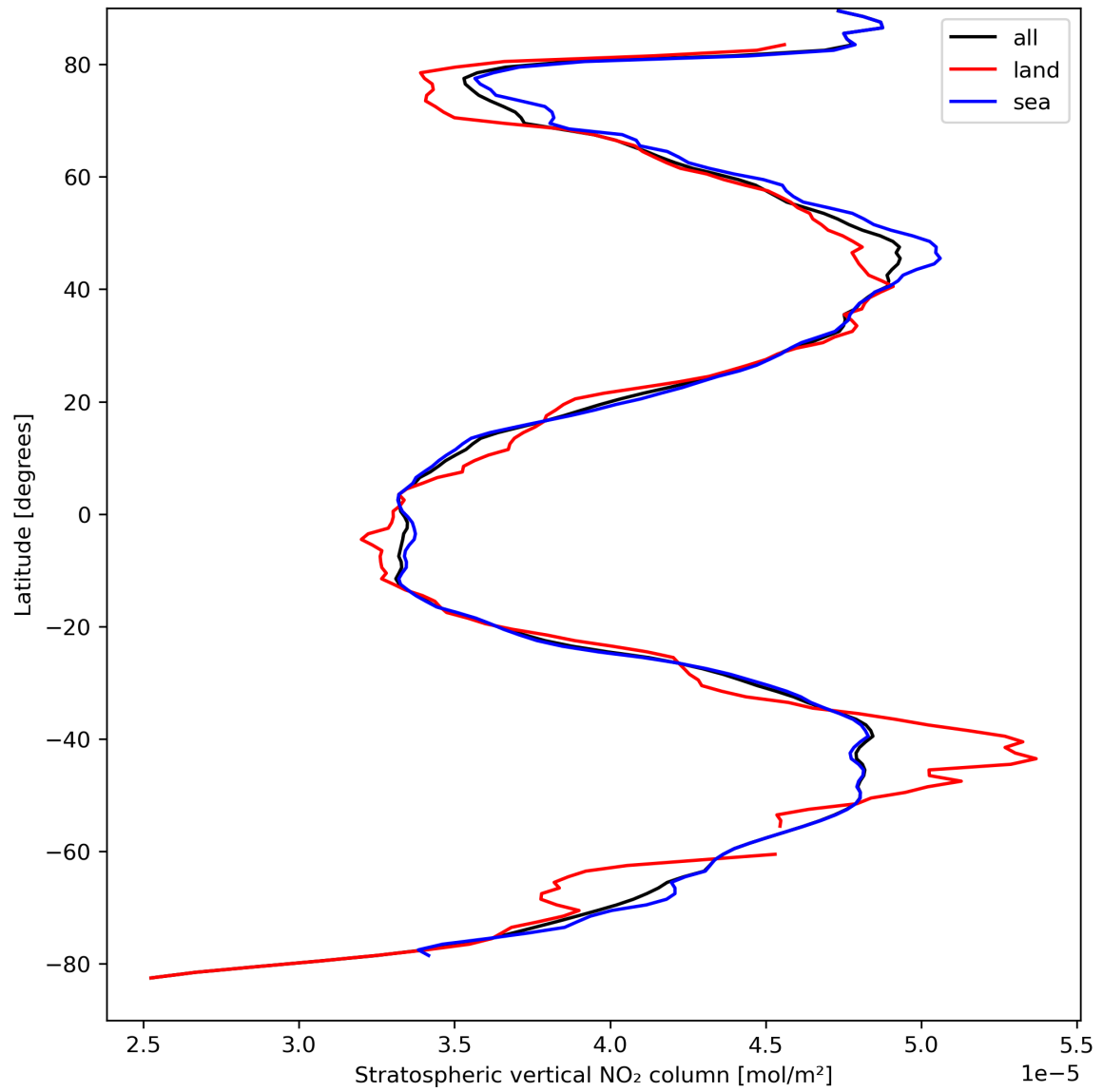
Figure 19: Zonal average of “Stratospheric vertical NO 2 column” for 2024-04-02 to 2024-04-04.
