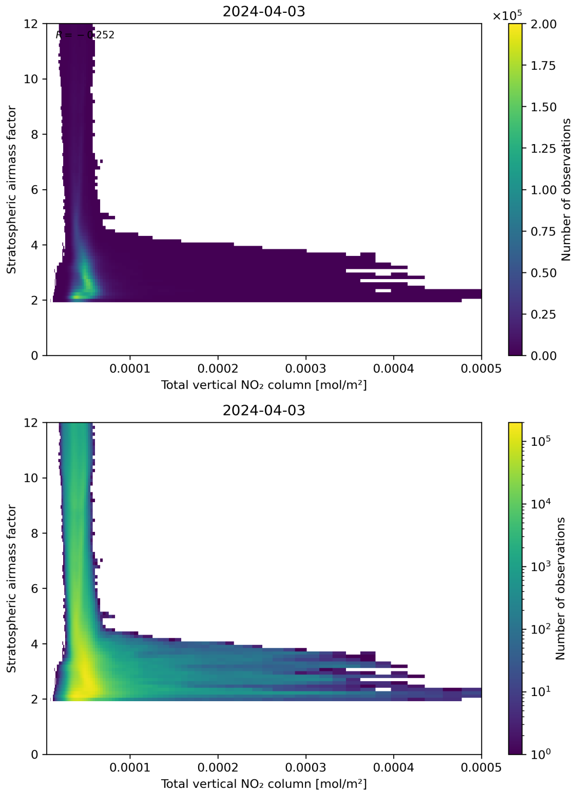
Figure 110: Scatter density plot of “Total vertical NO 2 column” against “Stratospheric airmass factor” for 2024-04-02 to 2024-04-04.
