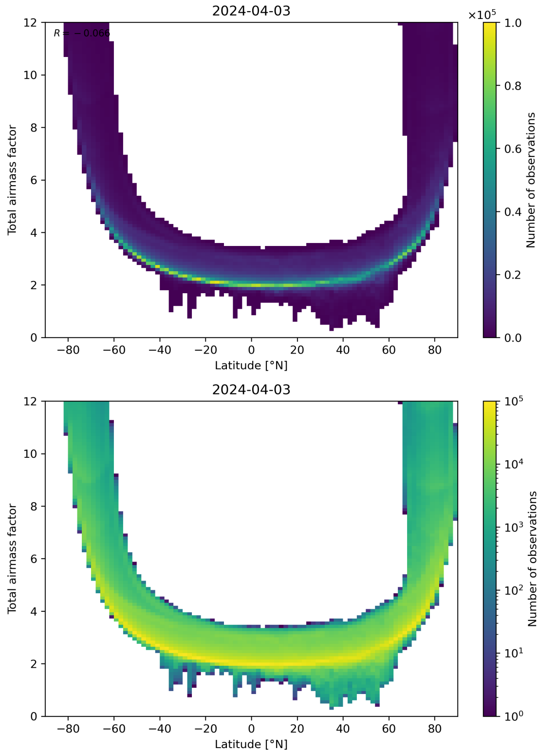
Figure 84: Scatter density plot of “Latitude” against “Total airmass factor” for 2024-04-02 to 2024-04-04.
