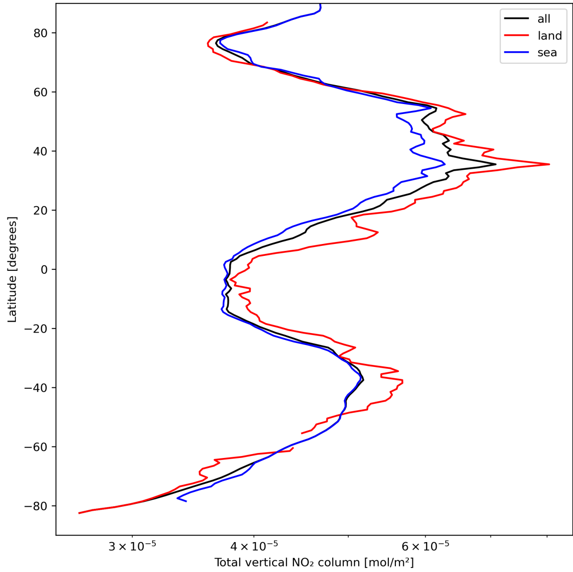
Figure 21: Zonal average of “Total vertical NO 2 column” for 2024-04-02 to 2024-04-04.
