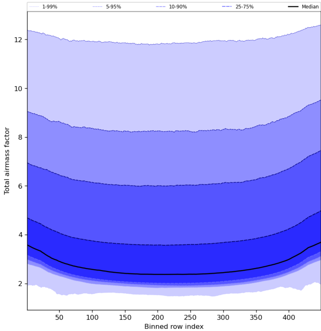
Figure 49: Along track statistics of “Total airmass factor” for 2024-04-02 to 2024-04-04
