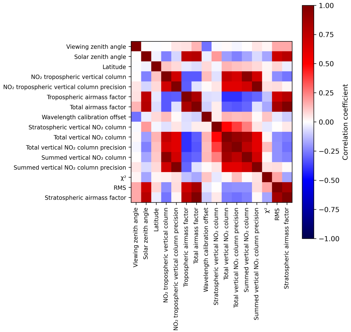
Figure 2: Map of correlation matrix for 2024-04-02 to 2024-04-04.
