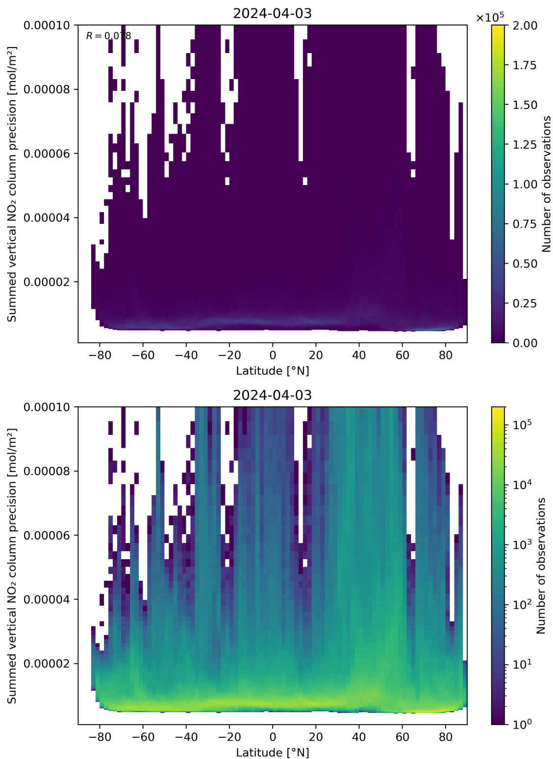
Figure 89: Scatter density plot of “Latitude” against “Summed vertical NO 2 column precision” for 2024-04-02 to 2024-04-04.
