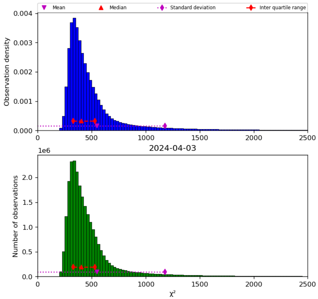
Figure 42: Histogram of “ \chi^2 ” for 2024-04-02 to 2024-04-04
