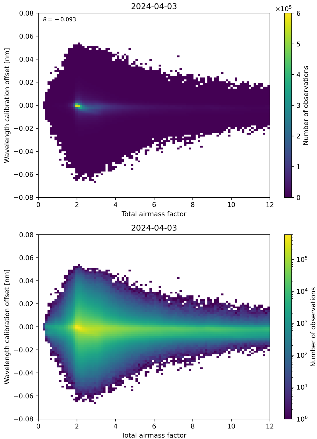
Figure 70: Scatter density plot of “Total airmass factor” against “Wavelength calibration offset” for 2024-04-02 to 2024-04-04.
