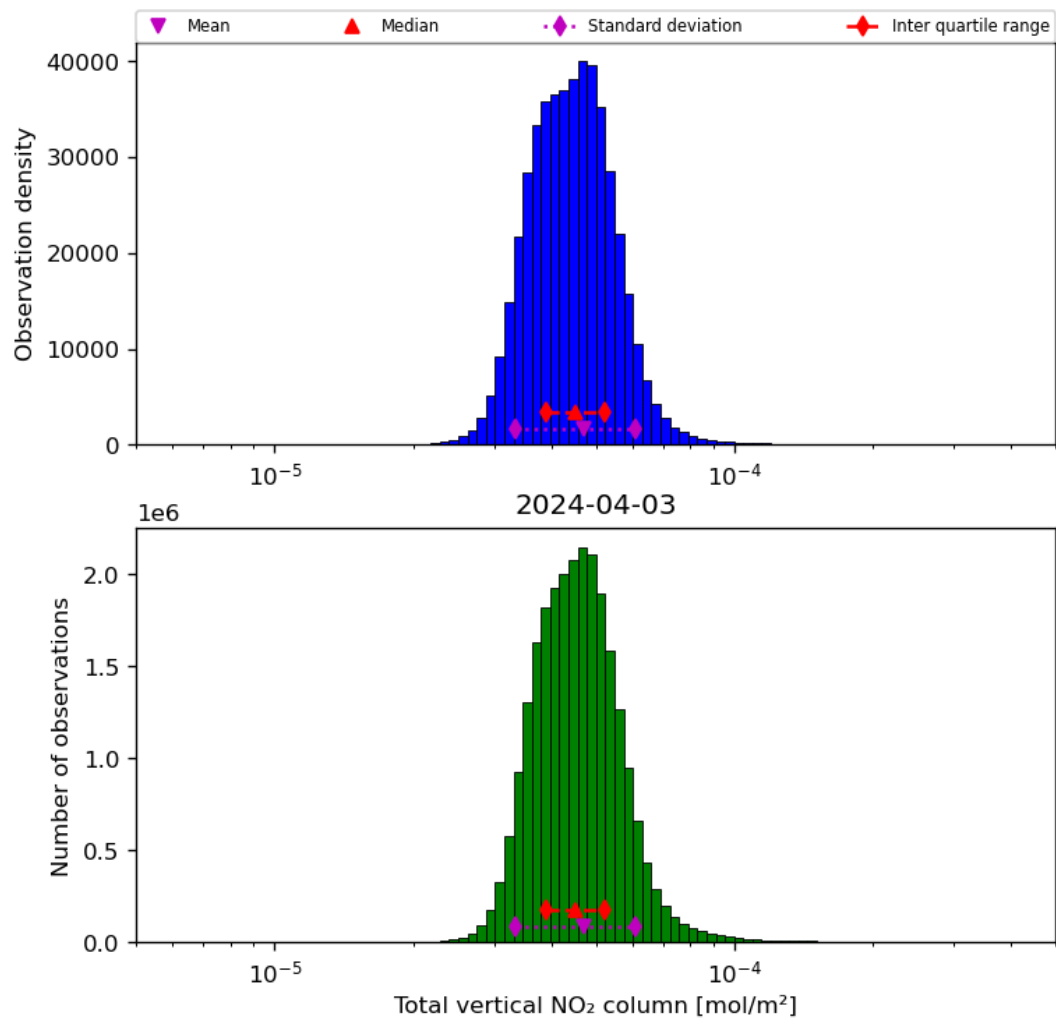
Figure 38: Histogram of “Total vertical NO 2 column” for 2024-04-02 to 2024-04-04
