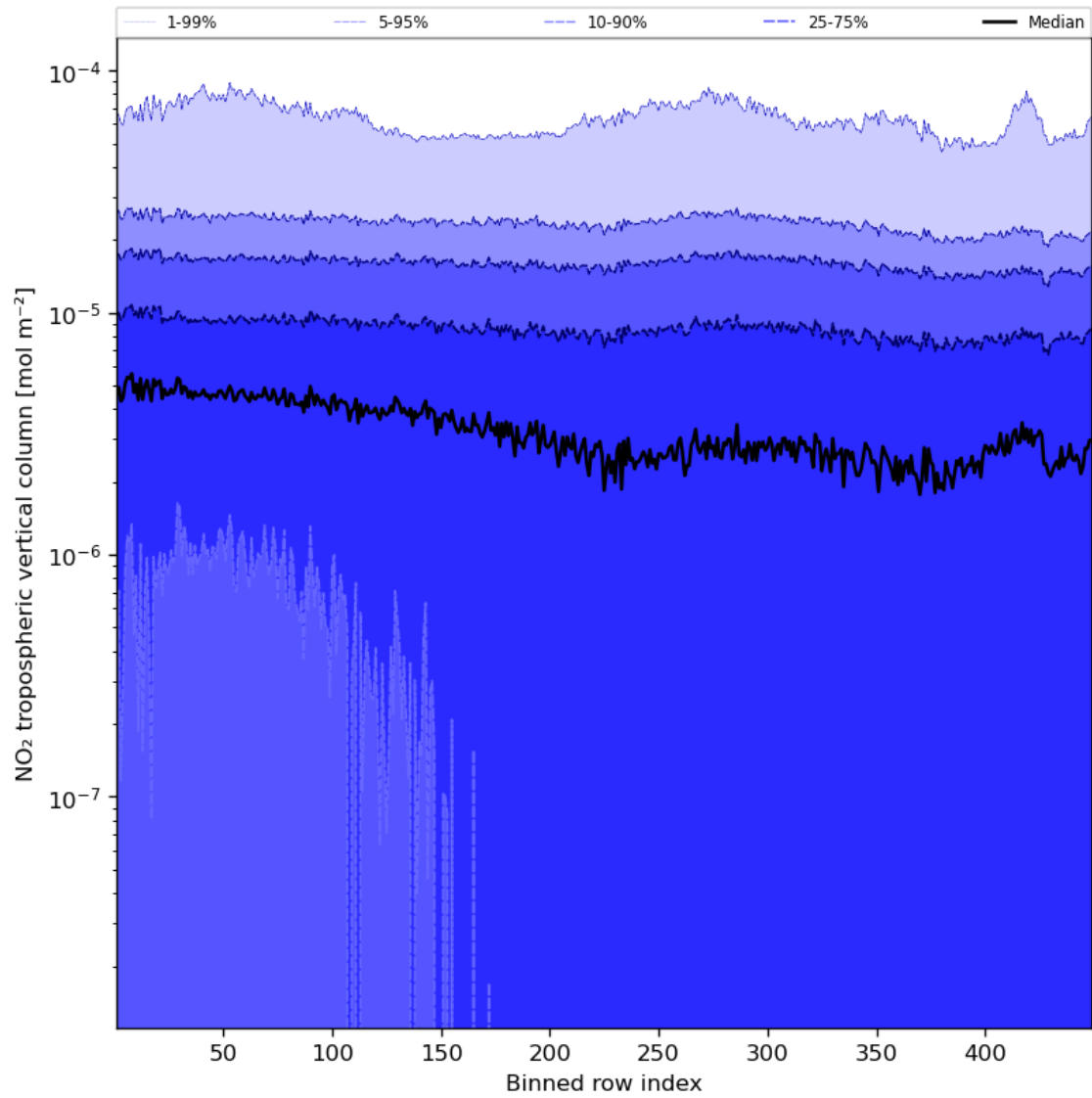
Figure 46: Along track statistics of “NO 2 tropospheric vertical column” for 2024-04-02 to 2024-04-04
