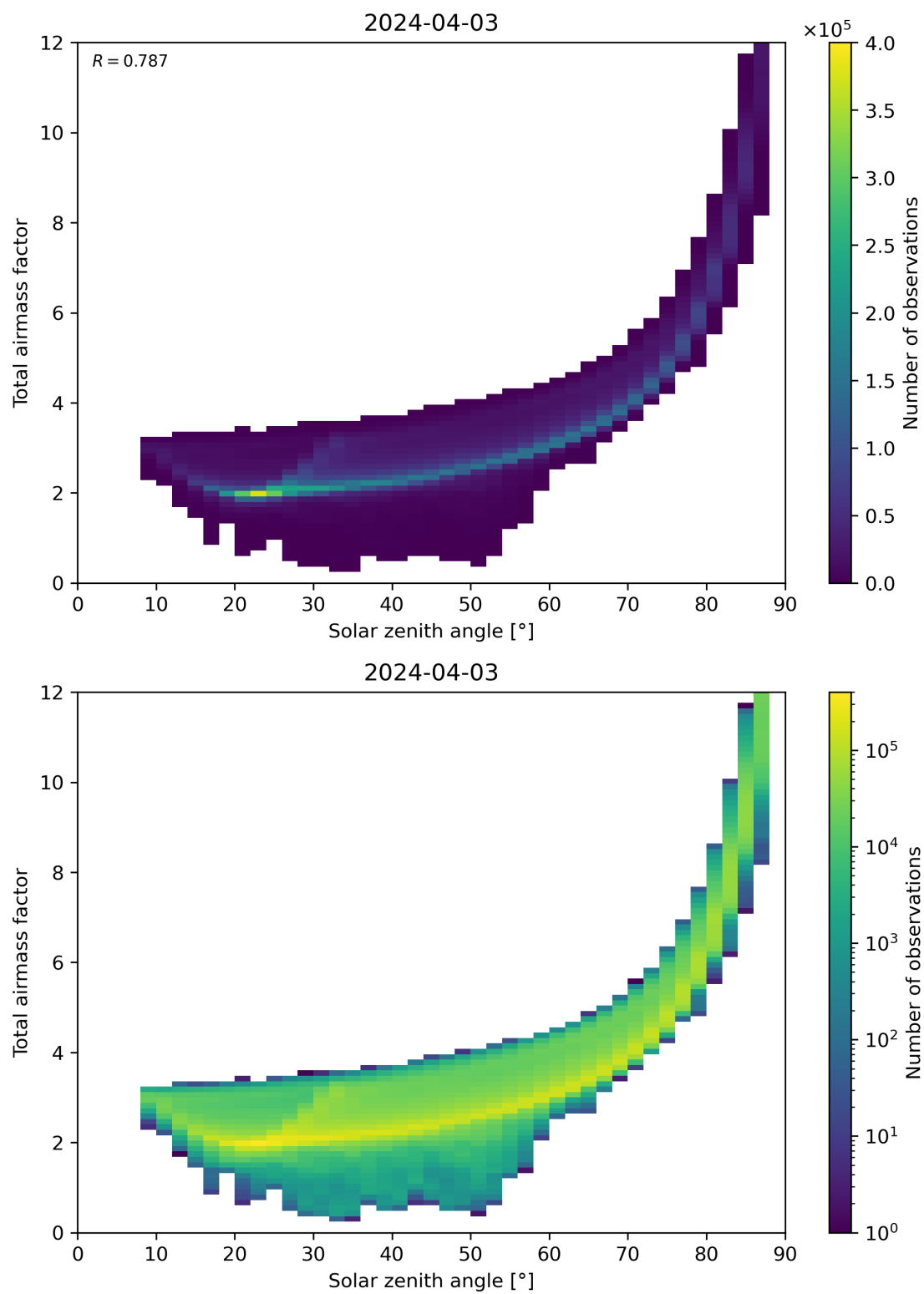
Figure 146: Scatter density plot of “Solar zenith angle” against “Total airmass factor” for 2024-04-02 to 2024-04-04.
