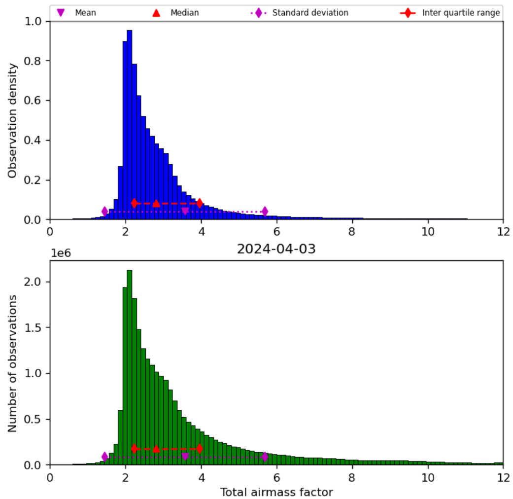
Figure 32: Histogram of “Total airmass factor” for 2024-04-02 to 2024-04-04
