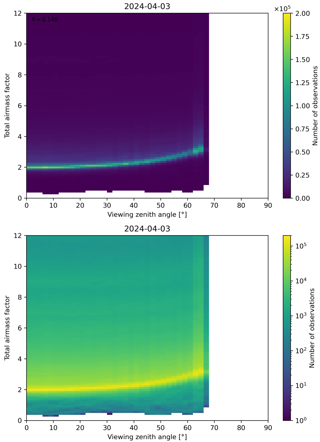
Figure 160: Scatter density plot of “Viewing zenith angle” against “Total airmass factor” for 2024-04-02 to 2024-04-04.
