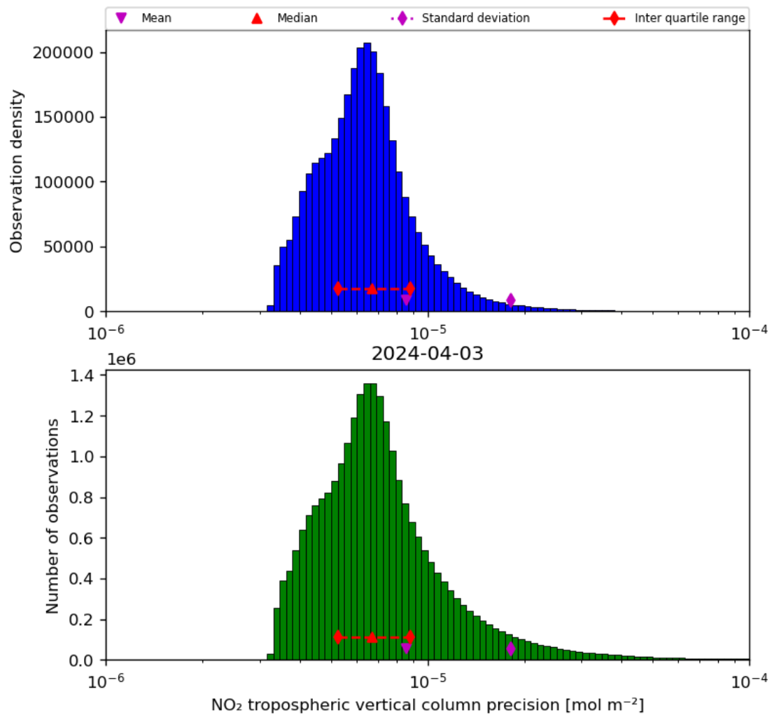
Figure 30: Histogram of “NO 2 tropospheric vertical column precision” for 2024-04-02 to 2024-04-04
