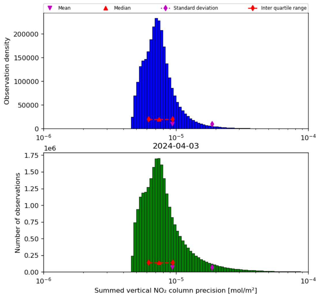
Figure 41: Histogram of "Summed vertical NO 2 column precision" for 2024-04-02 to 2024-04-04
