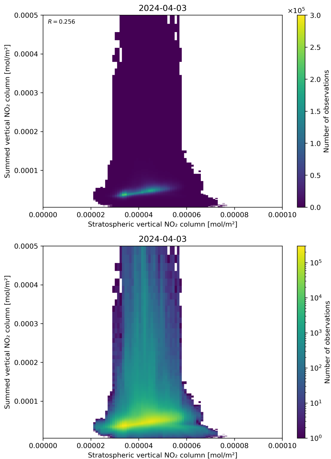
Figure 98: Scatter density plot of “Stratospheric vertical NO 2 column” against “Summed vertical NO 2 column” for 2024-04-02 to 2024-04-04.
