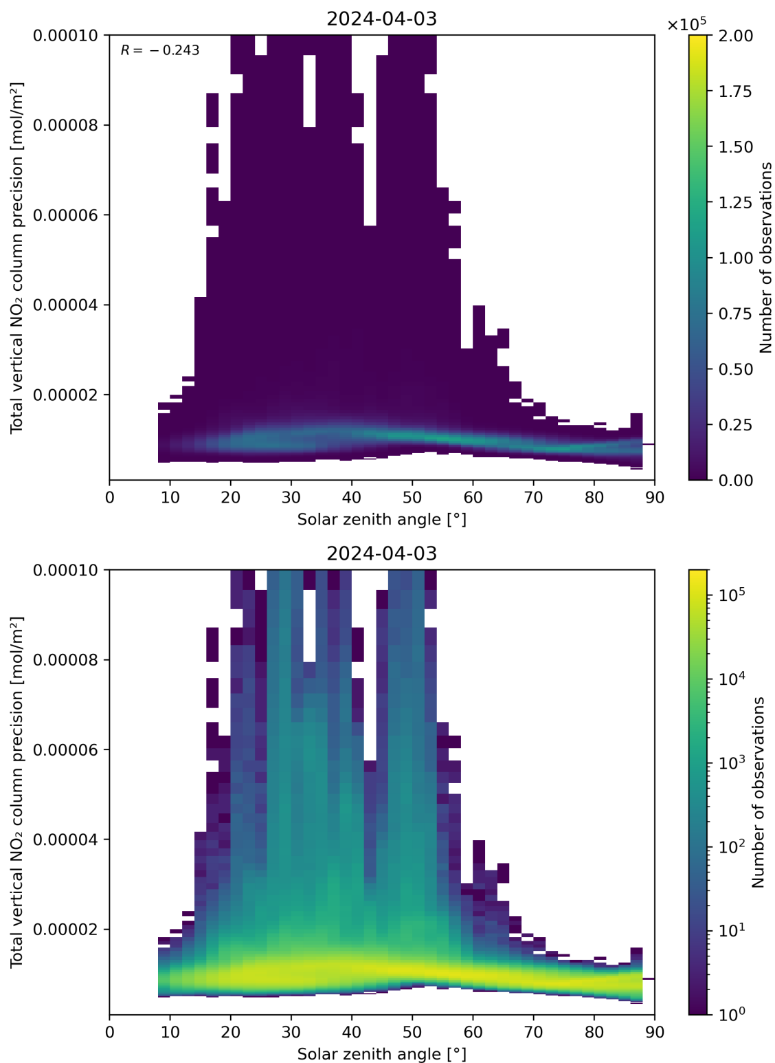
Figure 154: Scatter density plot of “Solar zenith angle” against “Total vertical NO 2 column precision” for 2024-04-02 to 2024-04-04.
