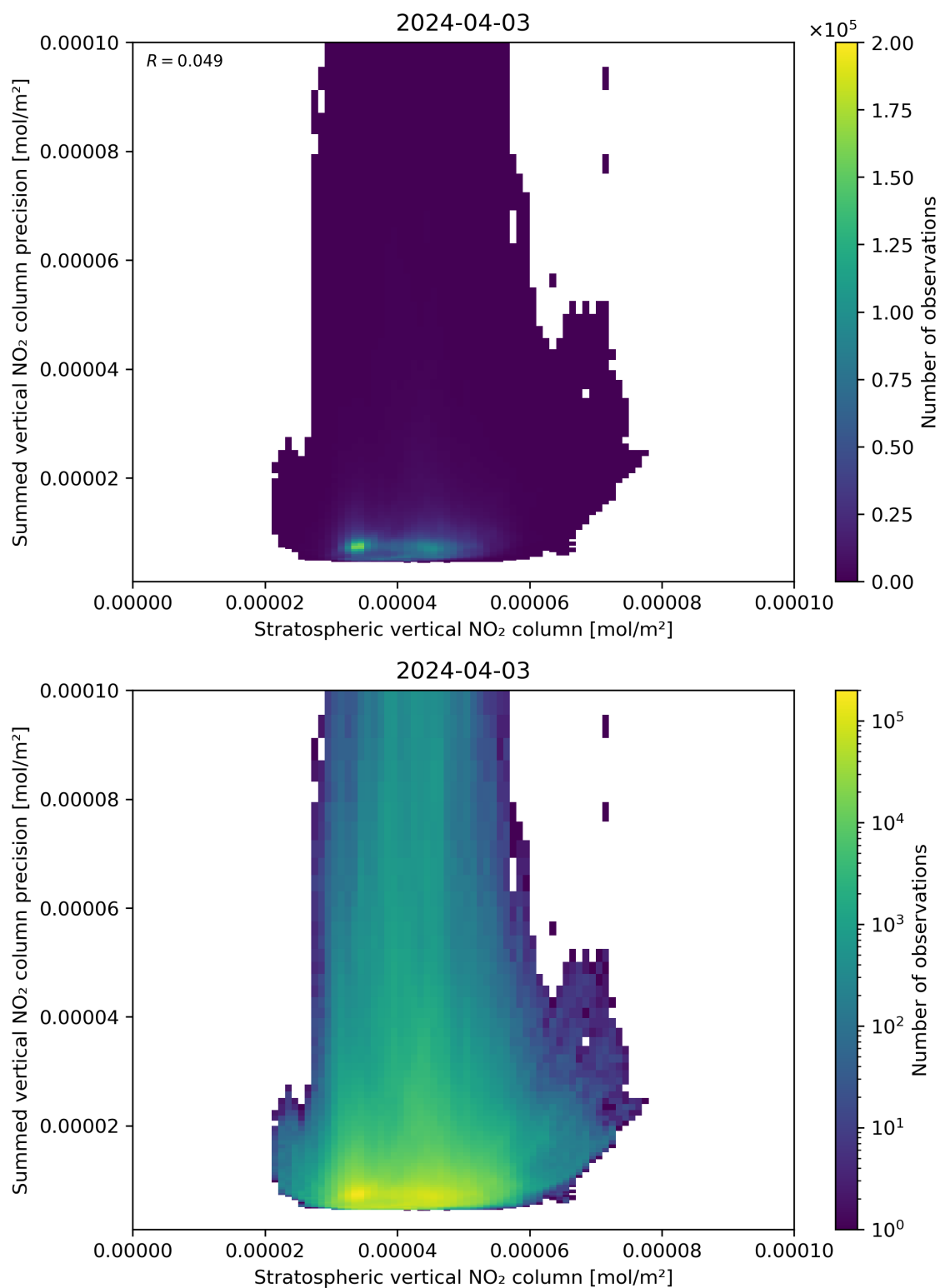
Figure 99: Scatter density plot of “Stratospheric vertical NO 2 column” against “Summed vertical NO 2 column precision” for 2024-04-02 to 2024-04-04.
