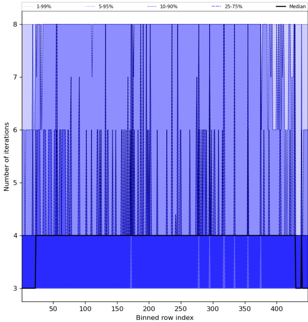
Figure 51: Along track statistics of “Number of iterations” for 2024-04-02 to 2024-04-04
