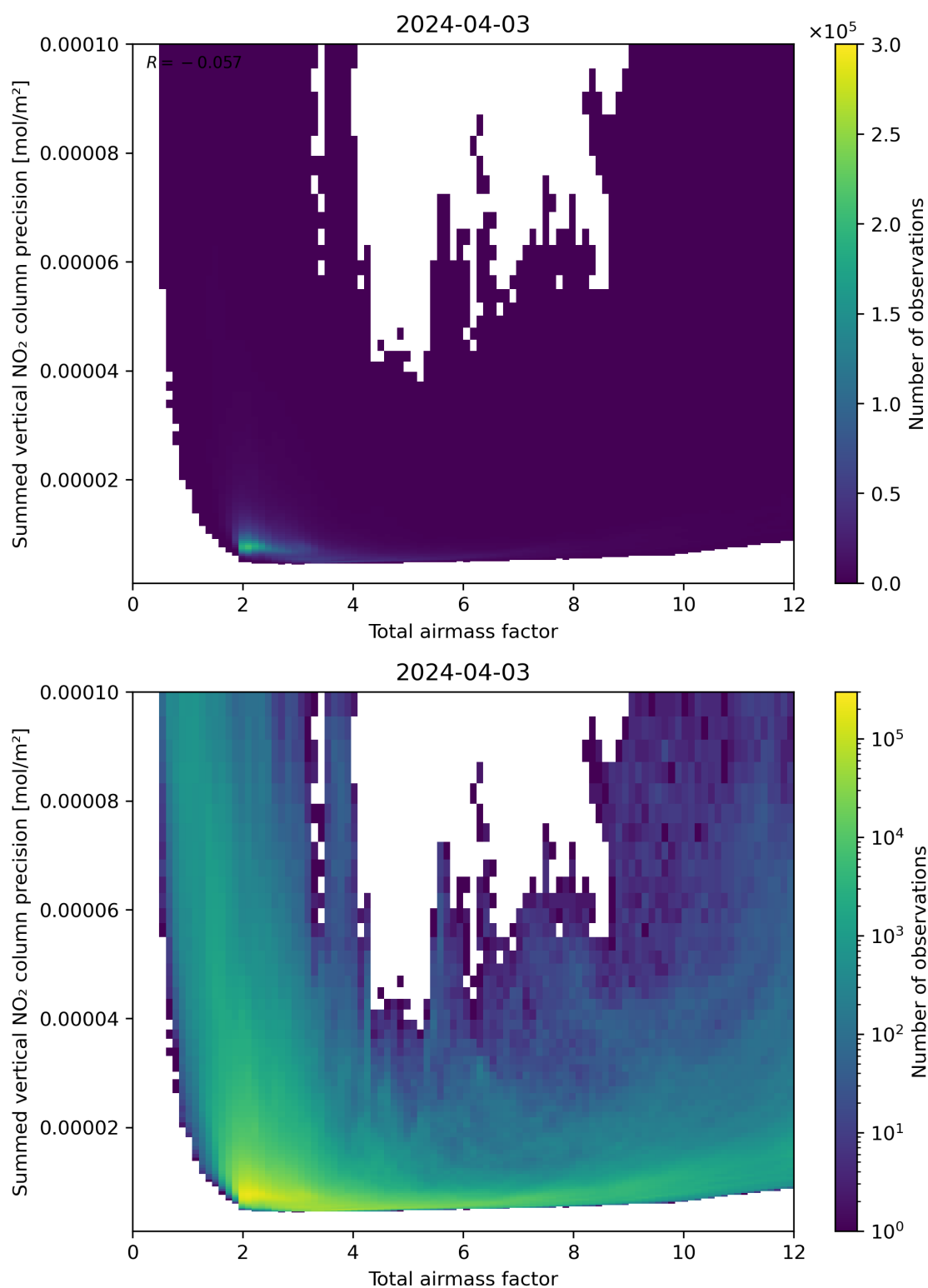
Figure 66: Scatter density plot of “Total airmass factor” against “Summed vertical NO 2 column precision” for 2024-04-02 to 2024-04-04.
