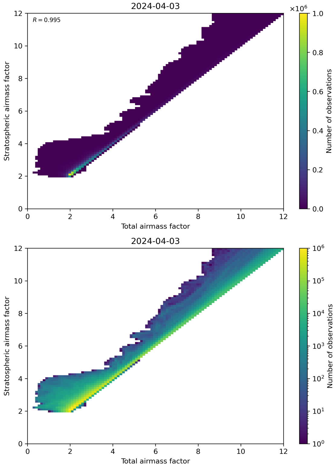
Figure 62: Scatter density plot of “Total airmass factor” against “Stratospheric airmass factor” for 2024-04-02 to 2024-04-04.
