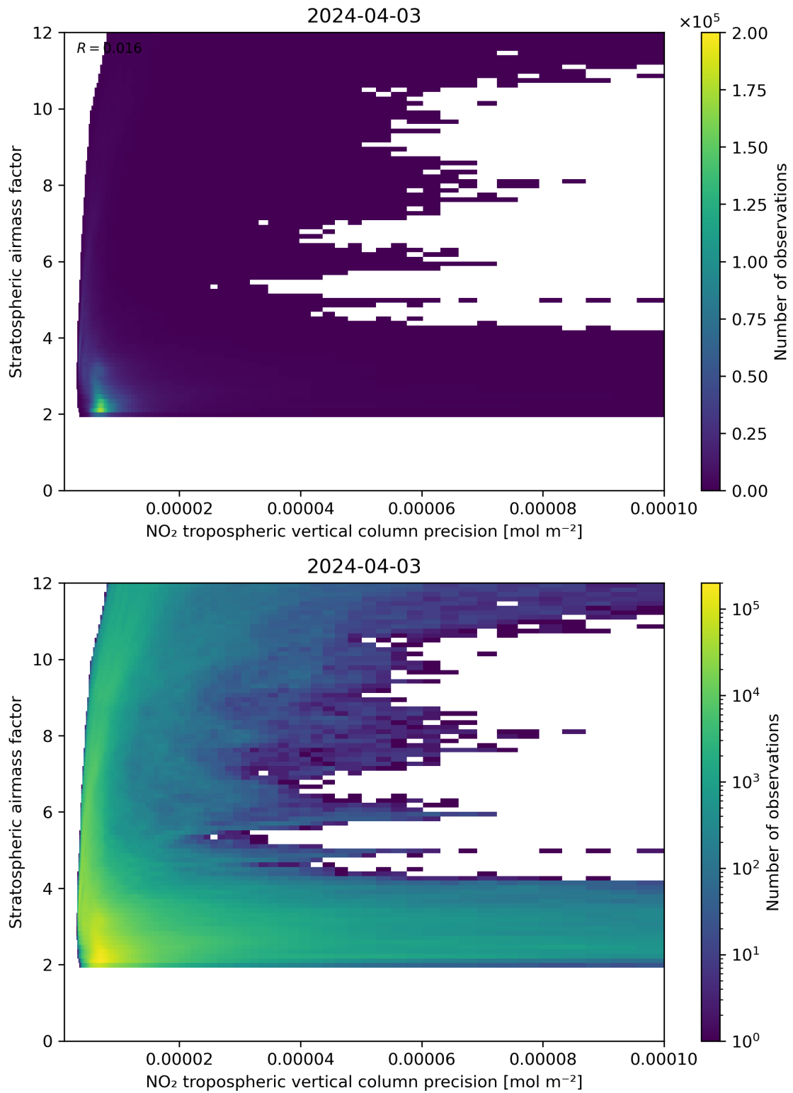
Figure 131: Scatter density plot of “NO 2 tropospheric vertical column precision” against “Stratospheric airmass factor” for 2024-04-02 to 2024-04-04.
