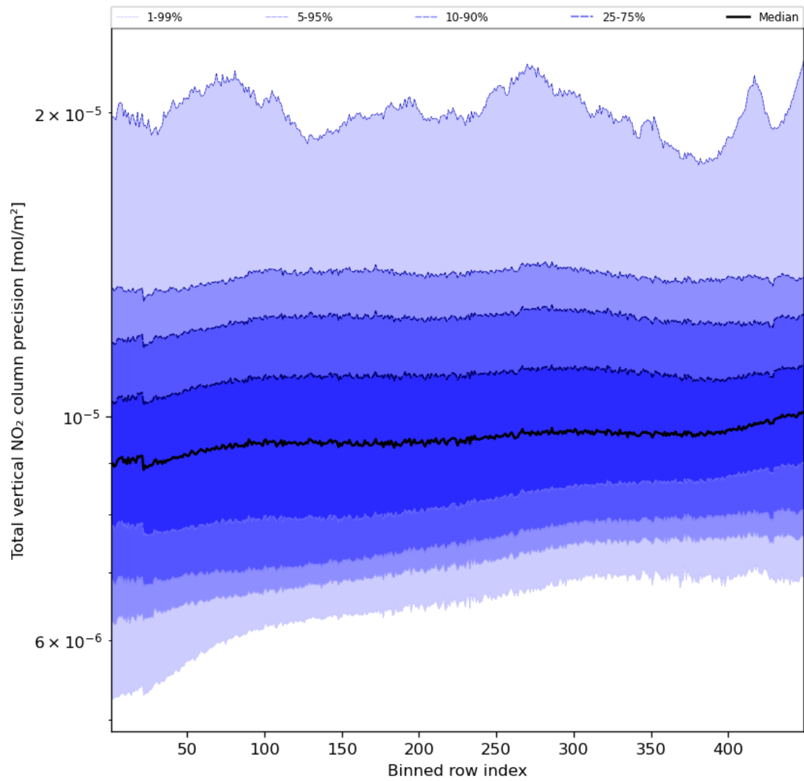
Figure 56: Along track statistics of “Total vertical NO 2 column precision” for 2024-04-02 to 2024-04-04
