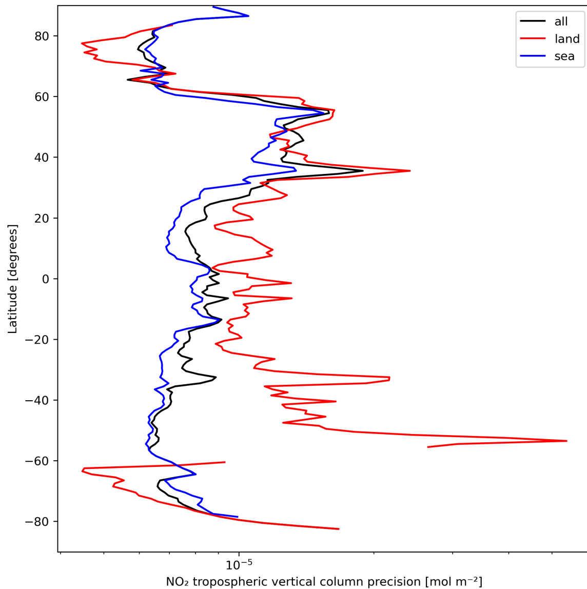
Figure 13: Zonal average of “NO 2 tropospheric vertical column precision” for 2024-04-02 to 2024-04-04.
