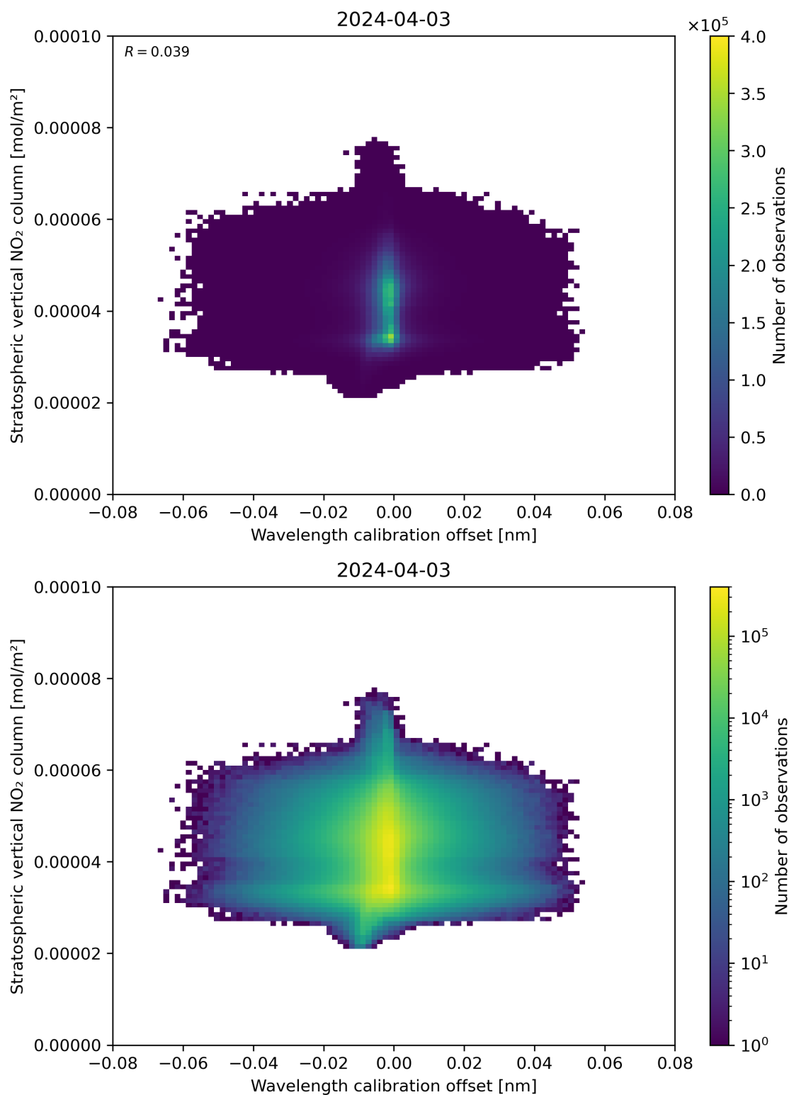
Figure 176: Scatter density plot of “Wavelength calibration offset” against “Stratospheric vertical NO 2 column” for 2024-04-02 to 2024-04-04.
