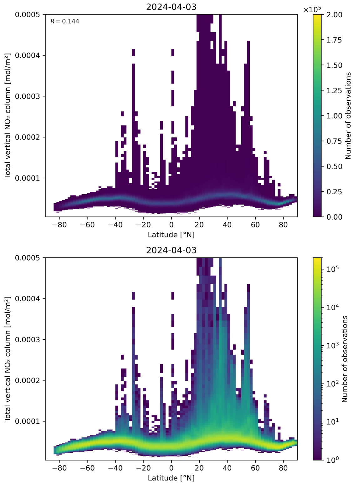
Figure 90: Scatter density plot of “Latitude” against “Total vertical NO 2 column” for 2024-04-02 to 2024-04-04.
