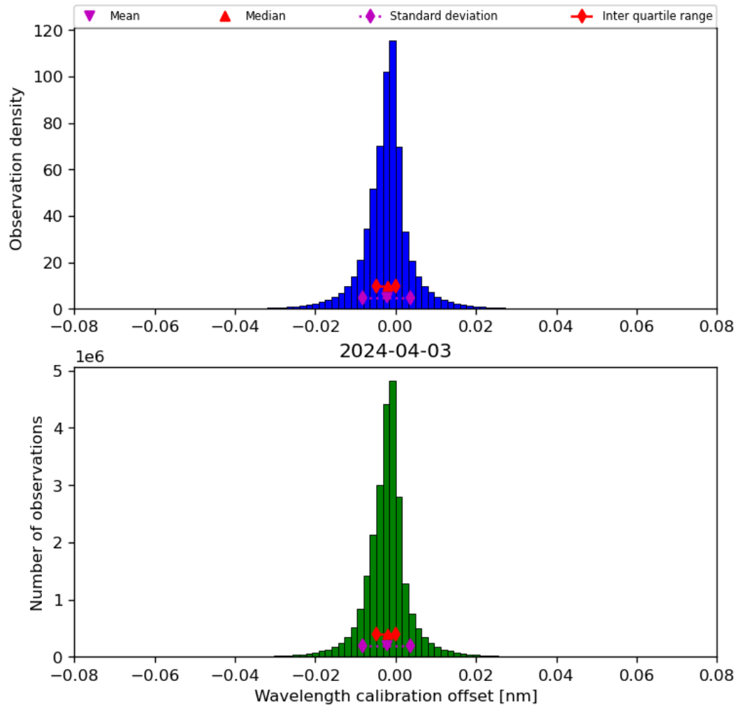
Figure 35: Histogram of “Wavelength calibration offset” for 2024-04-02 to 2024-04-04
