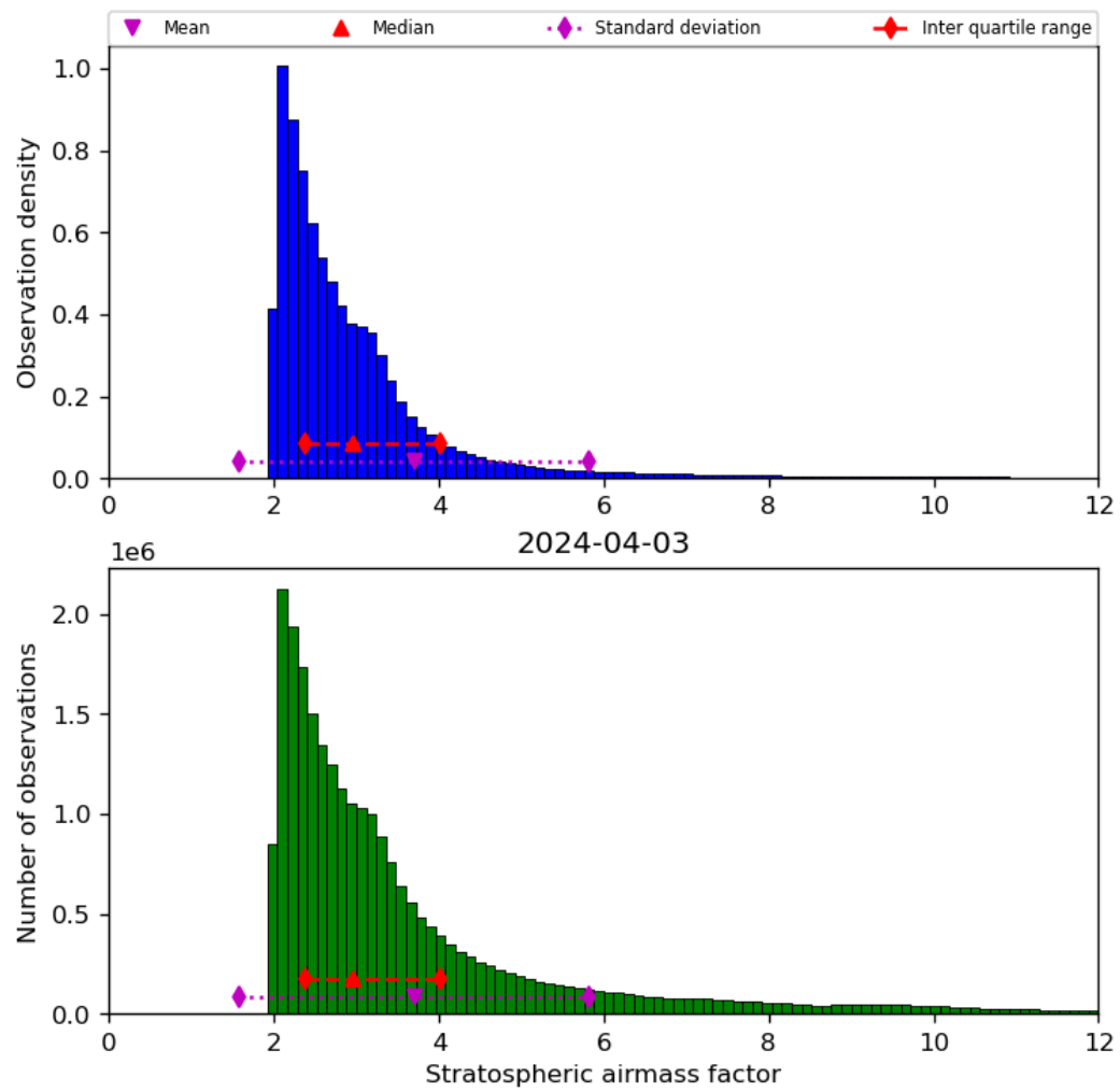
Figure 44: Histogram of “Stratospheric airmass factor” for 2024-04-02 to 2024-04-04
