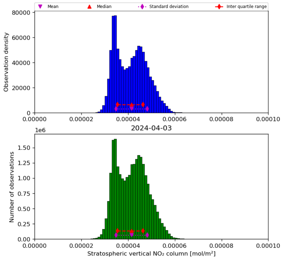
Figure 36: Histogram of “Stratospheric vertical NO 2 column” for 2024-04-02 to 2024-04-04
