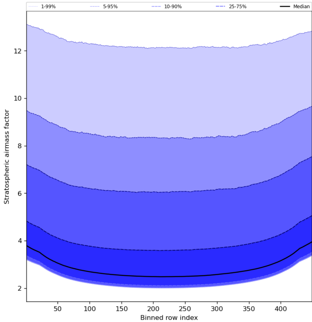
Figure 61: Along track statistics of “Stratospheric airmass factor” for 2024-04-02 to 2024-04-04
