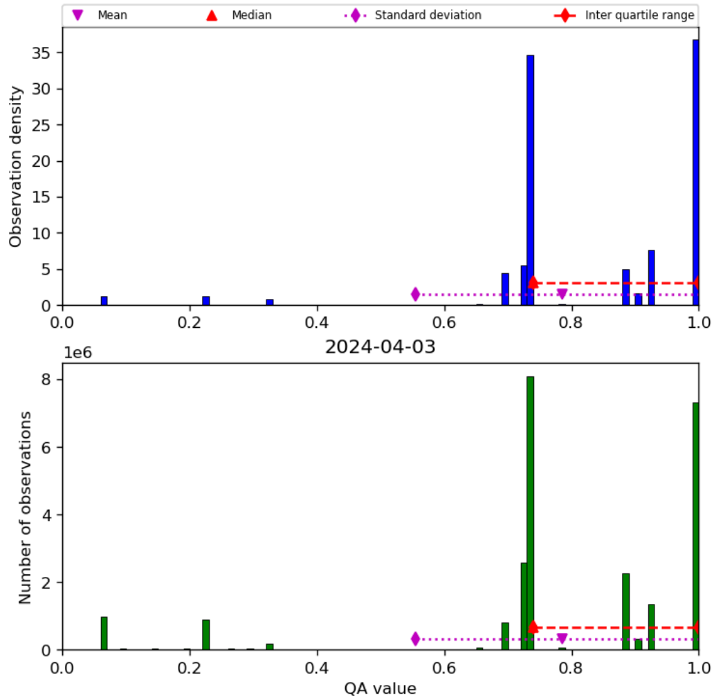
Figure 28: Histogram of “QA value” for 2024-04-02 to 2024-04-04
