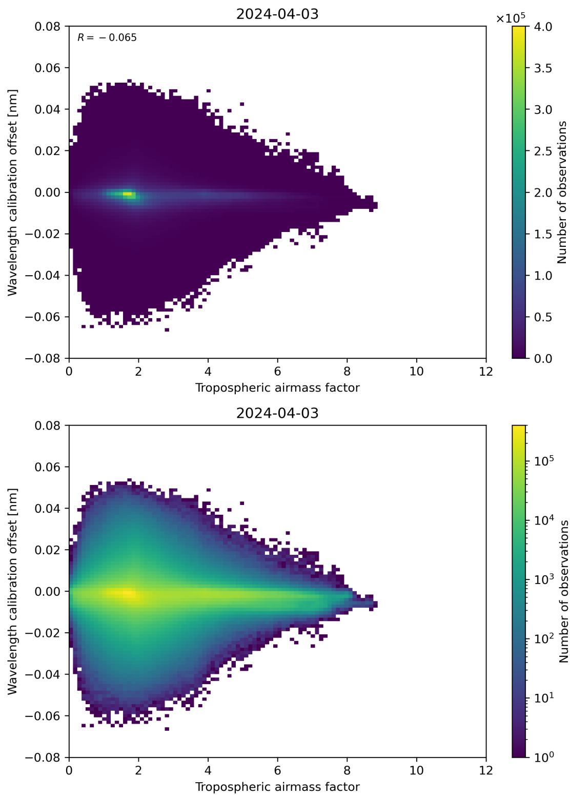
Figure 80: Scatter density plot of “Tropospheric airmass factor” against “Wavelength calibration offset” for 2024-04-02 to 2024-04-04.
