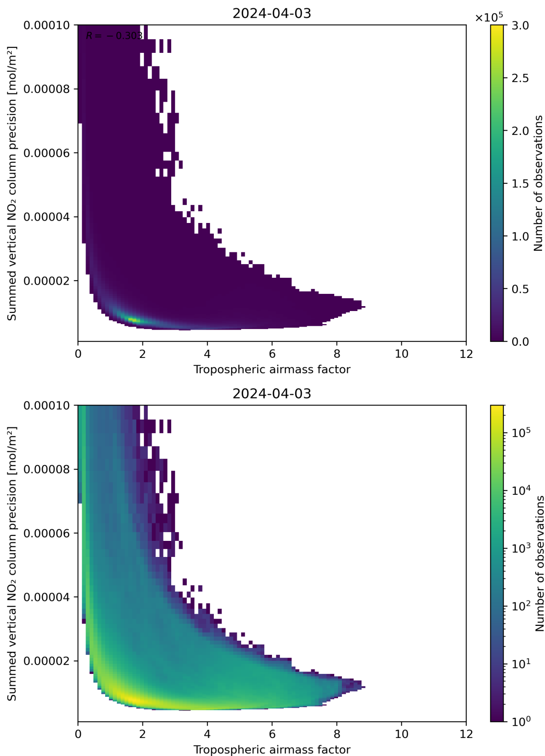
Figure 76: Scatter density plot of “Tropospheric air mass factor” against “Summed vertical NO 2 column precision” for 2024-04-02 to 2024-04-04.
