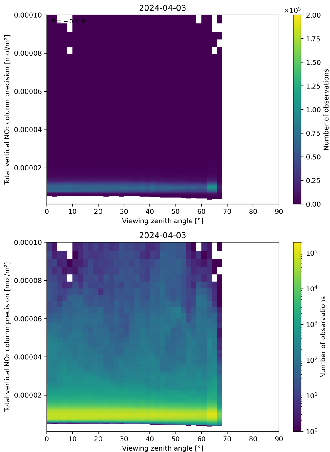
Figure 168: Scatter density plot of “Viewing zenith angle” against “Total vertical NO 2 column precision” for 2024-04-02 to 2024-04-04.
