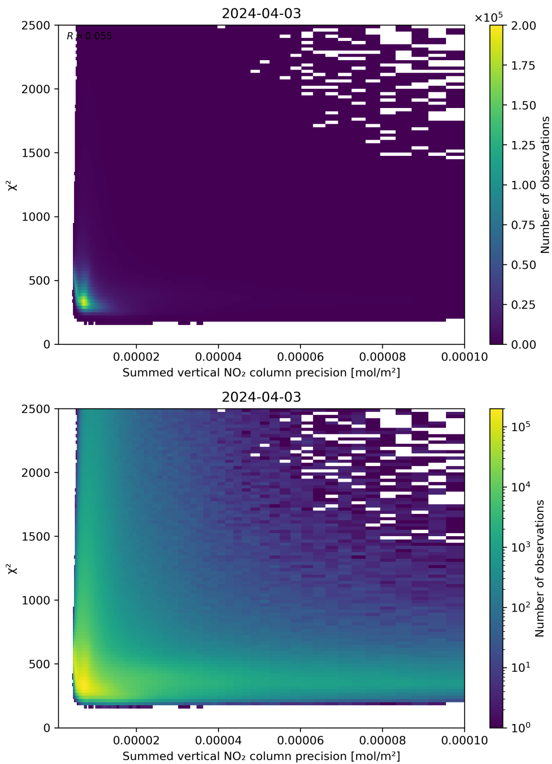
Figure 107: Scatter density plot of “Summed vertical NO 2 column precision” against “ \chi^2 ” for 2024-04-02 to 2024-04-04.
