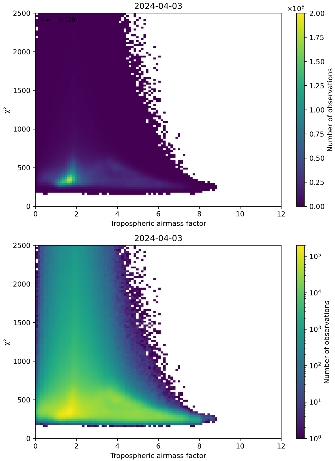
Figure 73: Scatter density plot of “Tropospheric airmass factor” against “ \chi^2 ” for 2024-04-02 to 2024-04-04.
