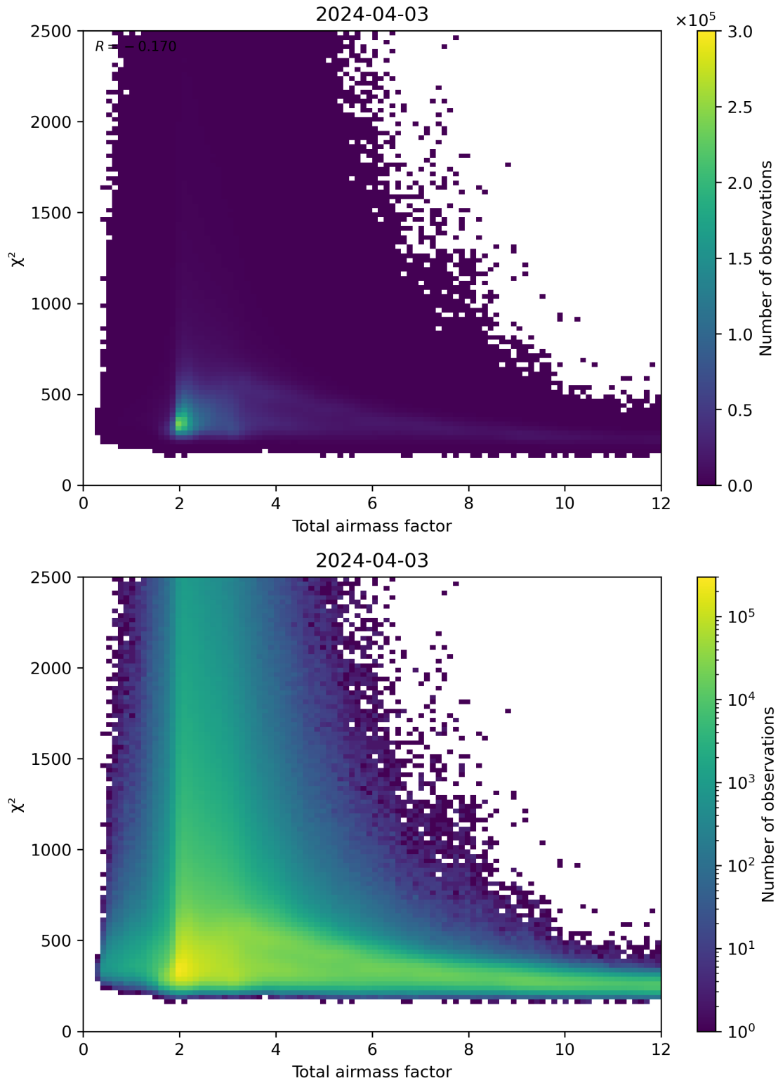
Figure 63: Scatter density plot of “Total airmass factor” against “ \chi^2 ” for 2024-04-02 to 2024-04-04.
