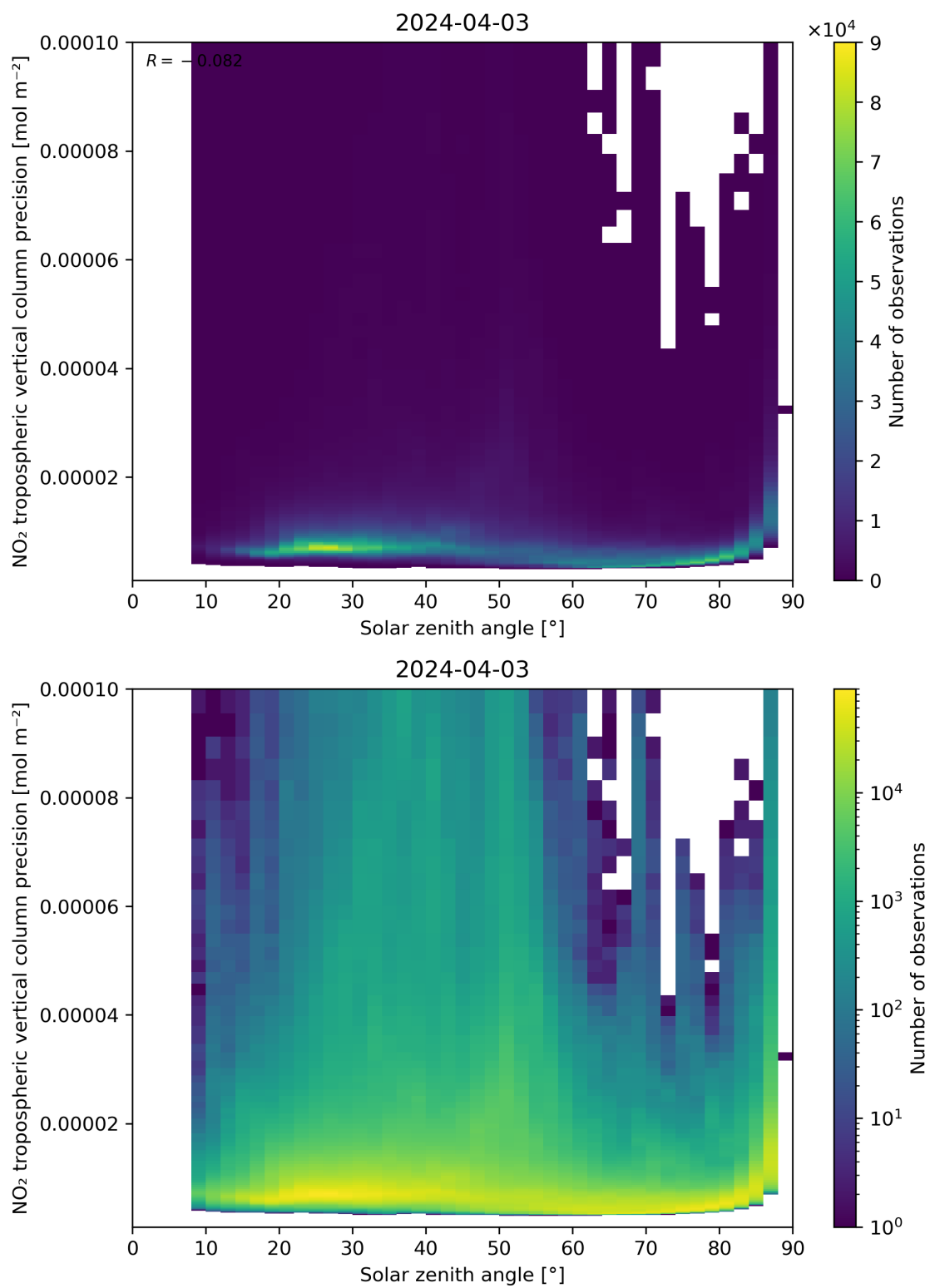
Figure 156: Scatter density plot of “Solar zenith angle” against “NO 2 tropospheric vertical column precision” for 2024-04-02 to 2024-04-04.
