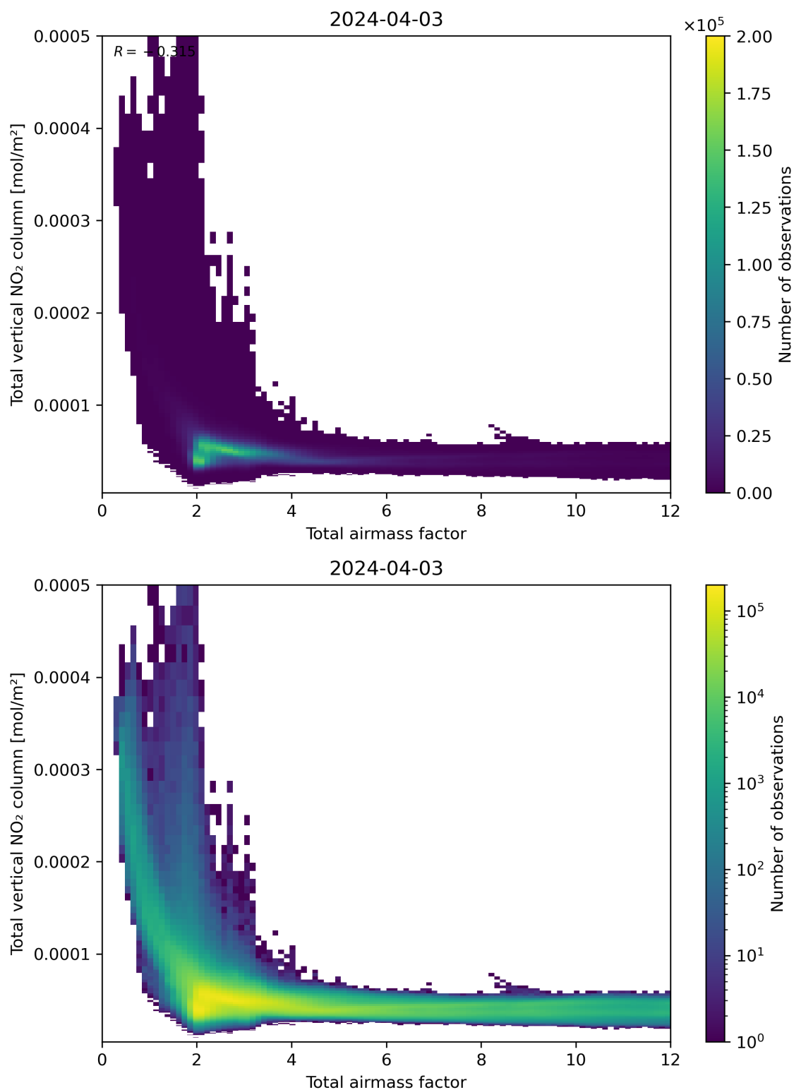
Figure 67: Scatter density plot of “Total airmass factor” against “Total vertical NO 2 column” for 2024-04-02 to 2024-04-04.
