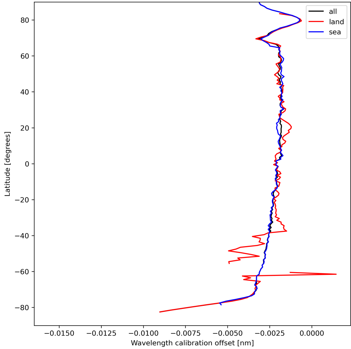
Figure 18: Zonal average of “Wavelength calibration offset” for 2024-04-02 to 2024-04-04.
