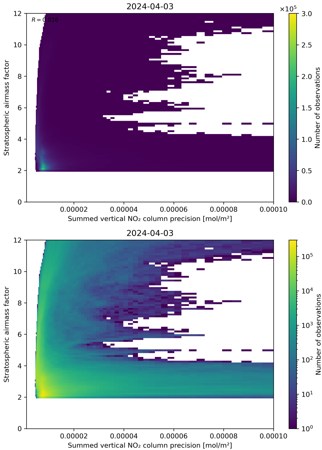
Figure 106: Scatter density plot of “Summed vertical NO 2 column precision” against “Stratospheric airmass factor” for 2024-04-02 to 2024-04-04.
