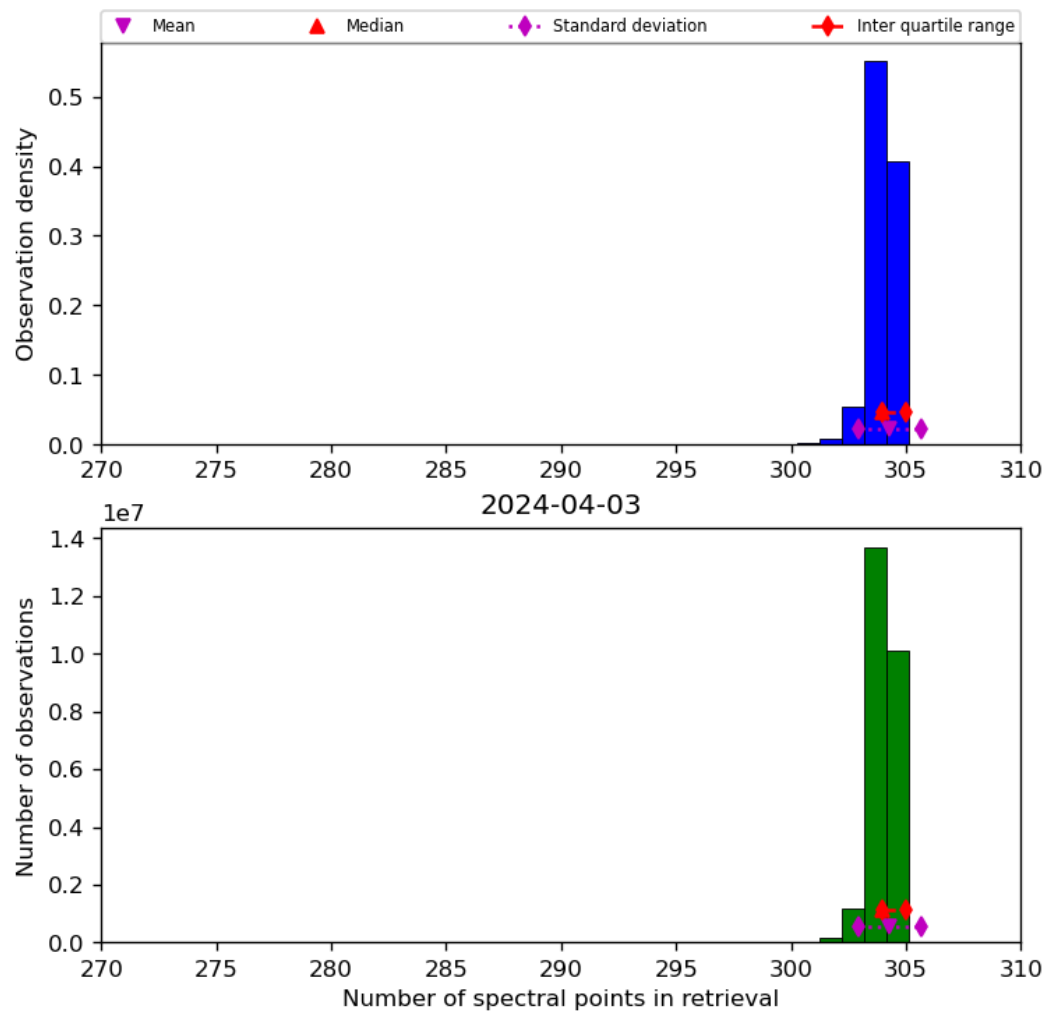
Figure 33: Histogram of “Number of spectral points in retrieval” for 2024-04-02 to 2024-04-04
