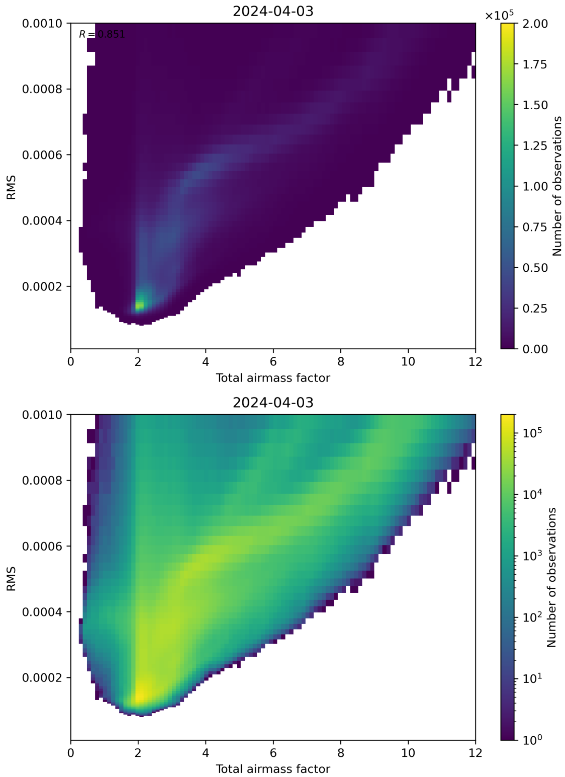
Figure 69: Scatter density plot of “Total airmass factor” against “RMS” for 2024-04-02 to 2024-04-04.
