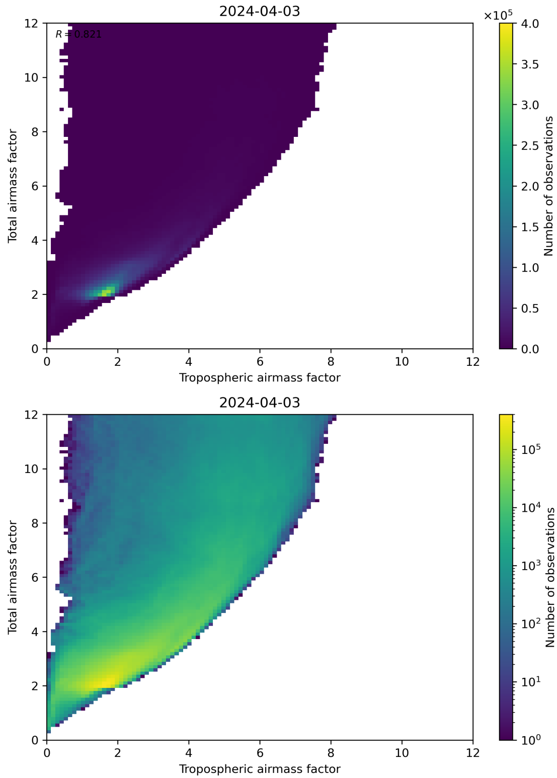
Figure 72: Scatter density plot of “Tropospheric airmass factor” against “Total airmass factor” for 2024-04-02 to 2024-04-04.
