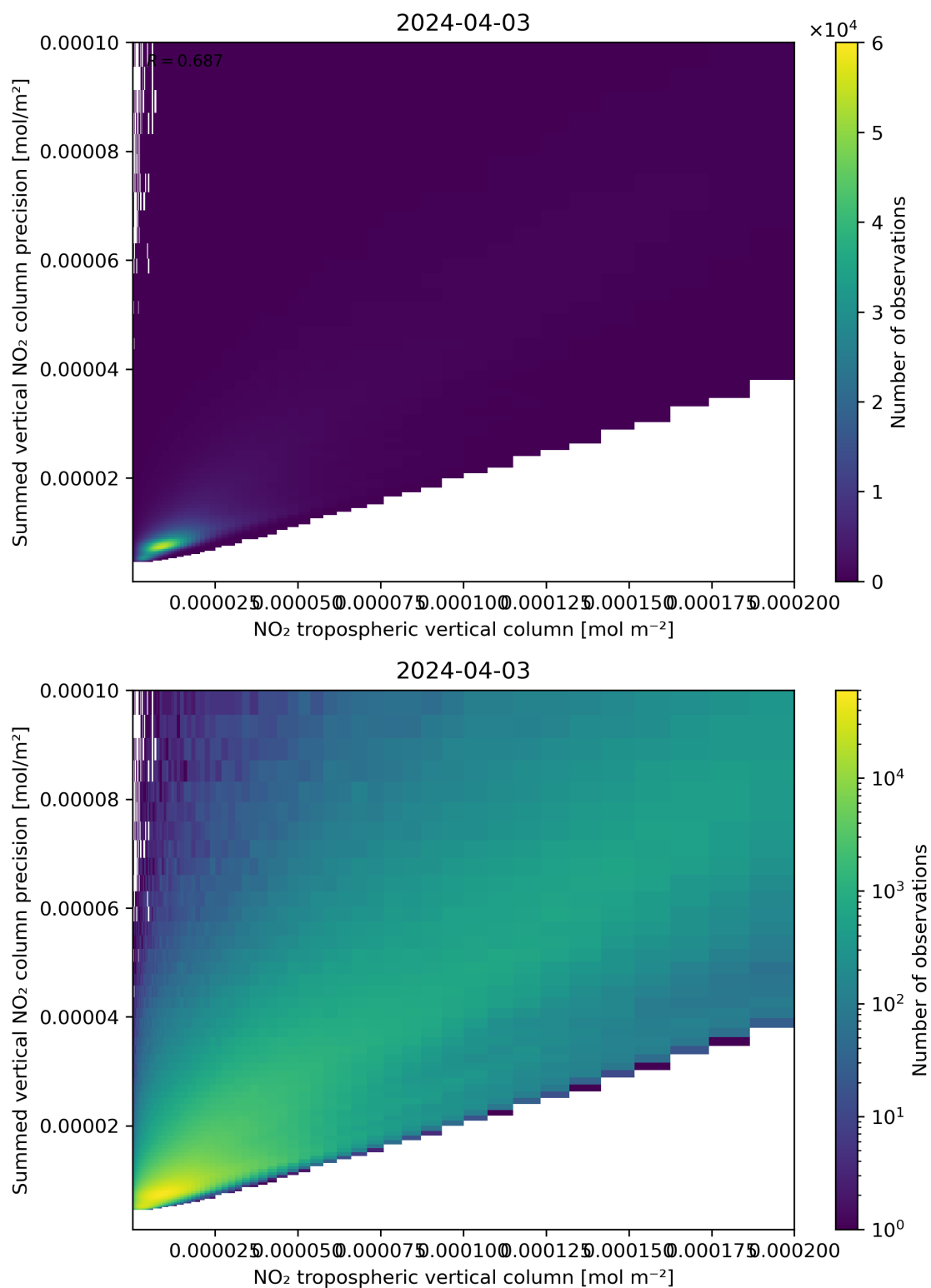
Figure 127: Scatter density plot of “NO 2 tropospheric vertical column” against “Summed vertical NO 2 column precision” for 2024-04-02 to 2024-04-04.
