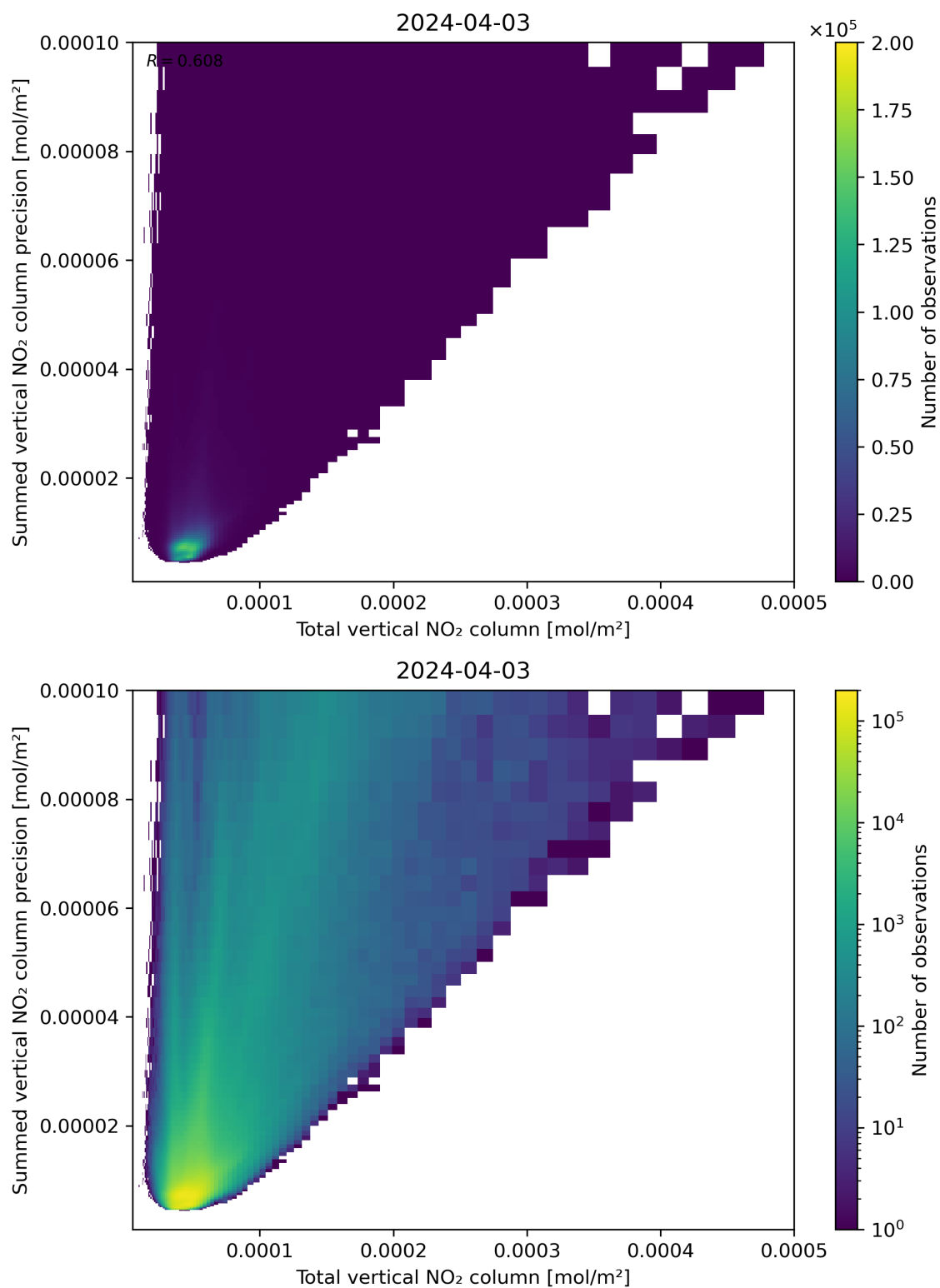
Figure 113: Scatter density plot of “Total vertical NO 2 column” against “Summed vertical NO 2 column precision” for 2024-04-02 to 2024-04-04.
