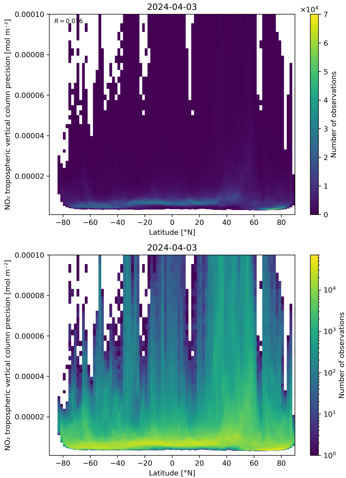
Figure 93: Scatter density plot of “Latitude” against “NO 2 tropospheric vertical column precision” for 2024-04-02 to 2024-04-04.
