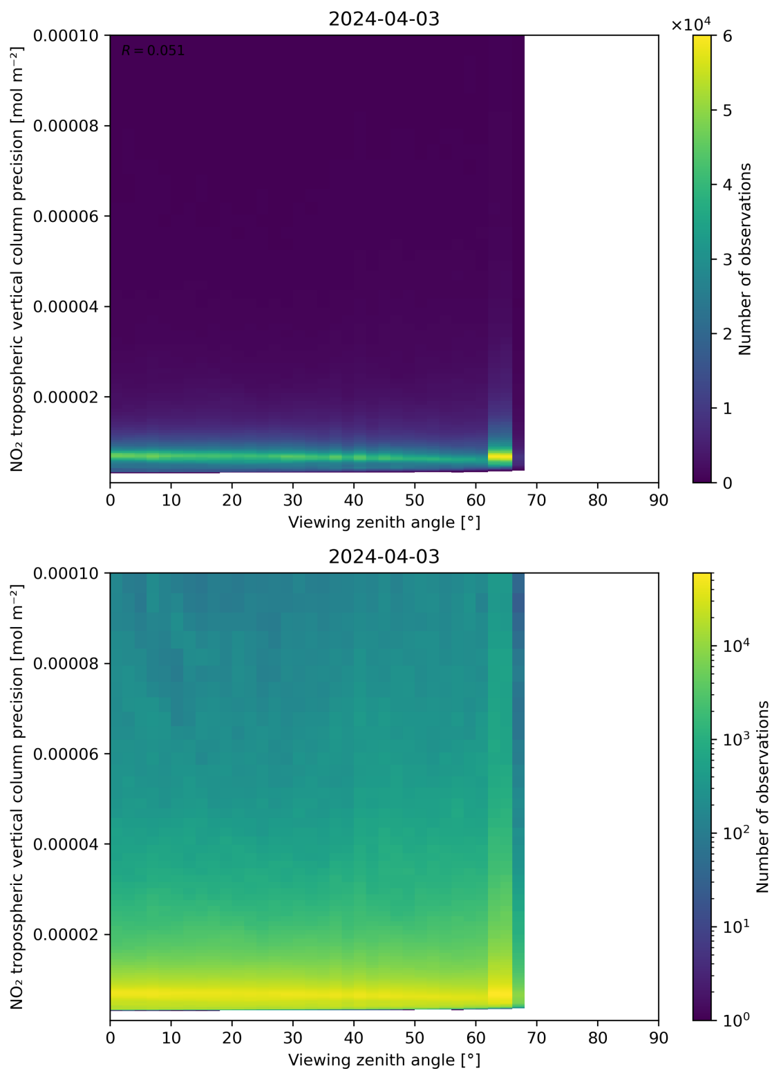
Figure 170: Scatter density plot of “Viewing zenith angle” against “NO 2 tropospheric vertical column precision” for 2024-04-02 to 2024-04-04.
