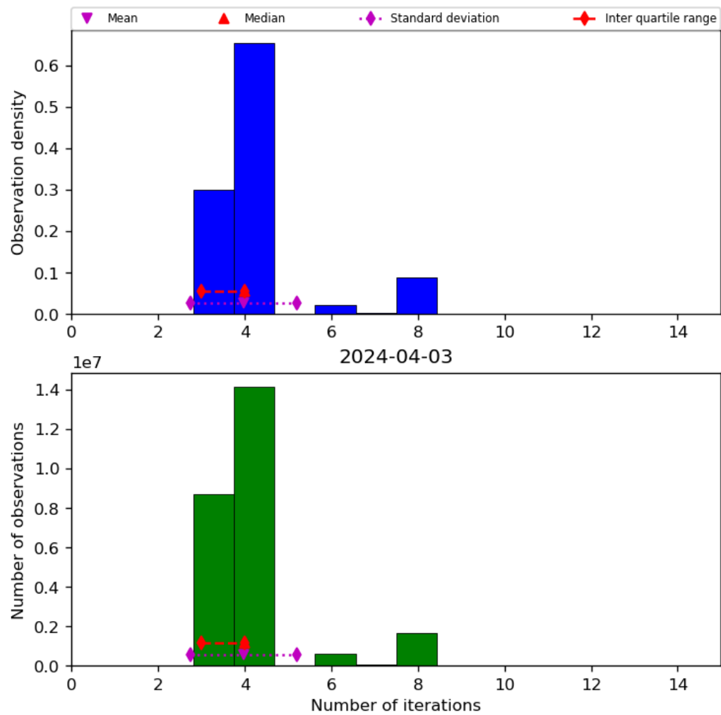
Figure 34: Histogram of “Number of iterations” for 2024-04-02 to 2024-04-04
