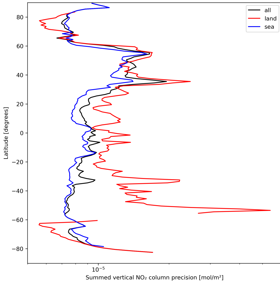
Figure 24: Zonal average of “Summed vertical NO 2 column precision” for 2024-04-02 to 2024-04-04.
