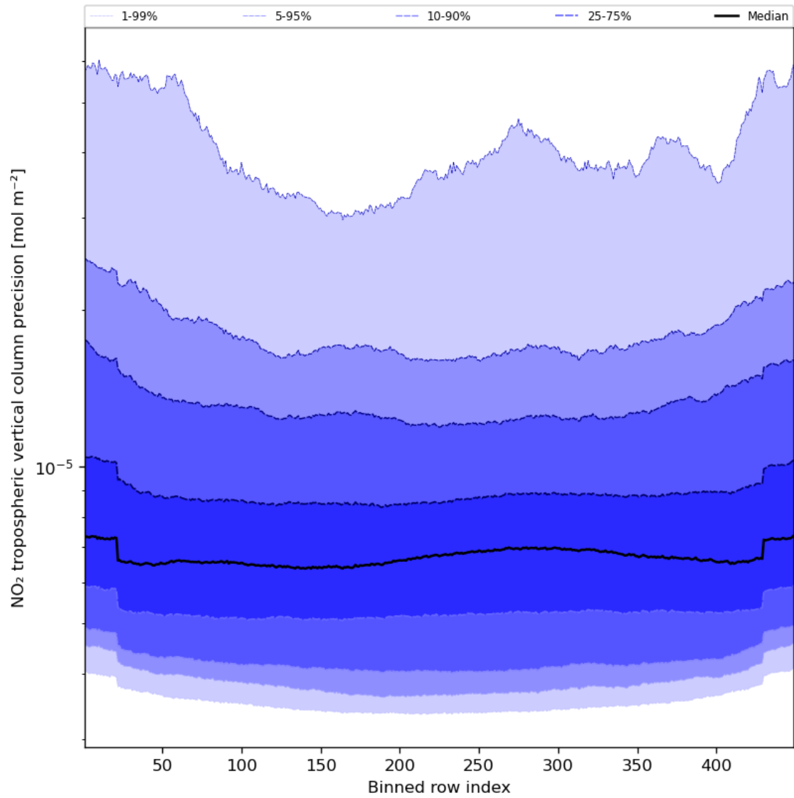
Figure 47: Along track statistics of “NO 2 tropospheric vertical column precision” for 2024-04-02 to 2024-04-04
