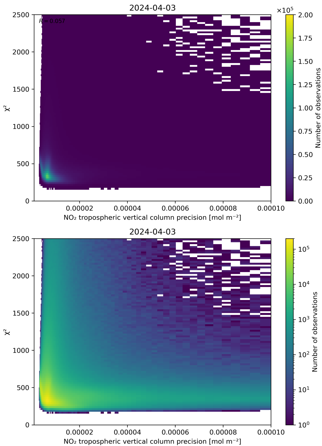
Figure 134: Scatter density plot of “NO 2 tropospheric vertical column precision” against “ \chi^2 ” for 2024-04-02 to 2024-04-04.
