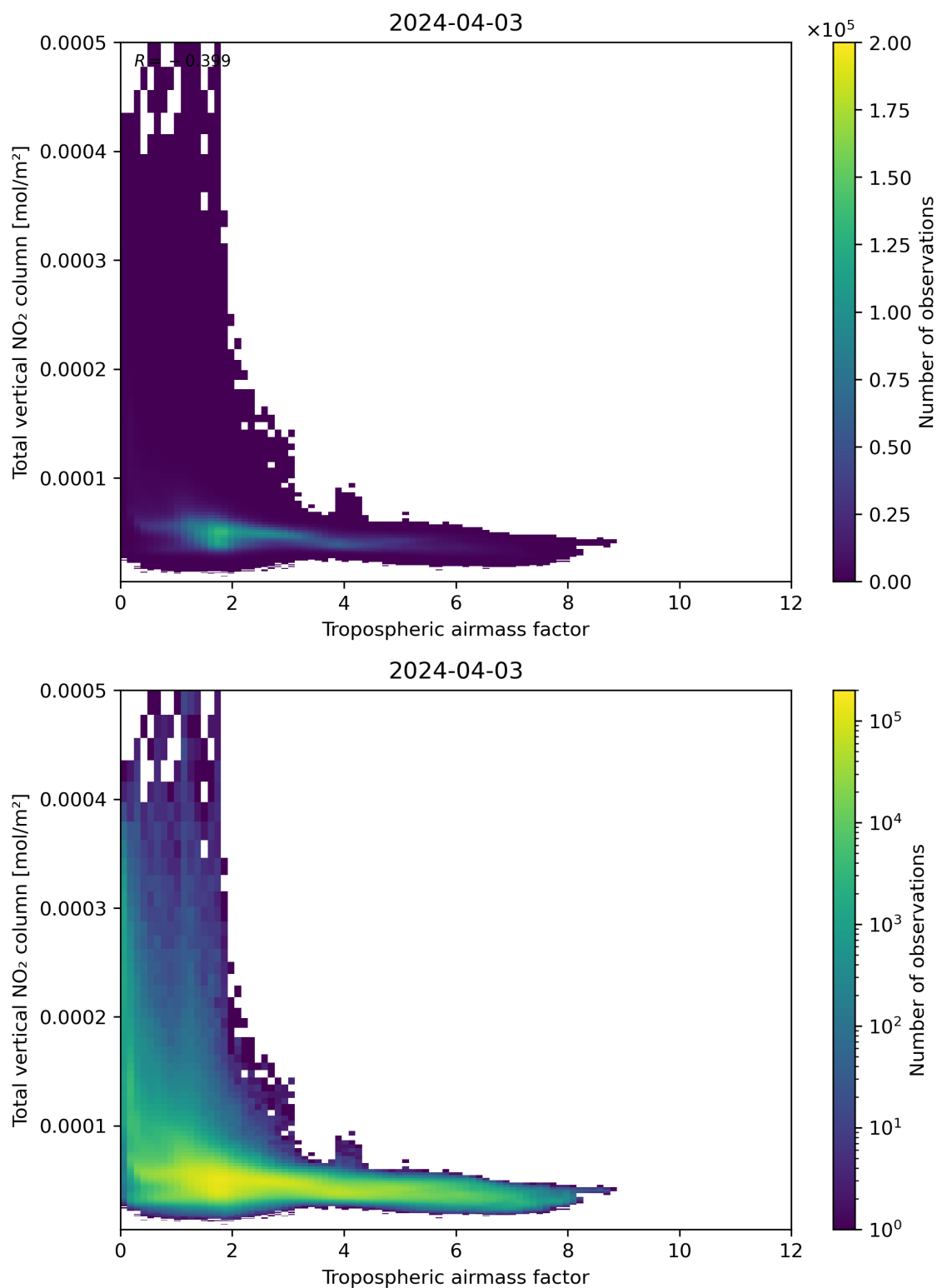
Figure 77: Scatter density plot of “Tropospheric airmass factor” against “Total vertical NO 2 column” for 2024-04-02 to 2024-04-04.
