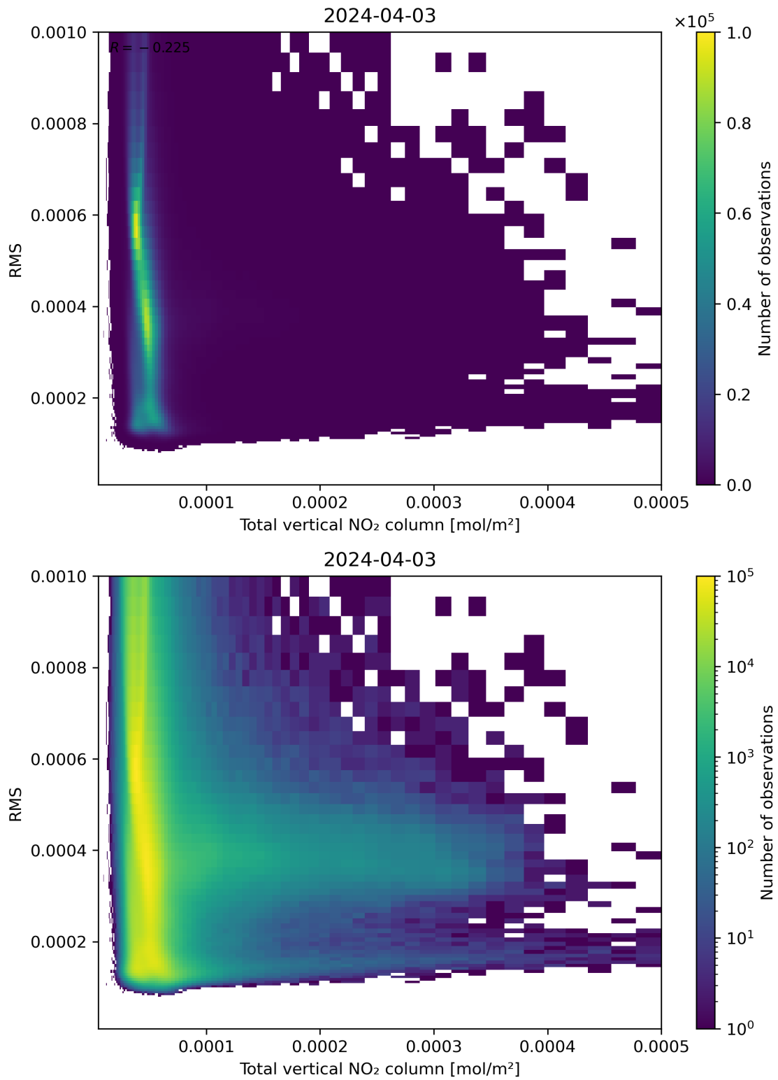
Figure 120: Scatter density plot of “Total vertical NO 2 column” against “RMS” for 2024-04-02 to 2024-04-04.
