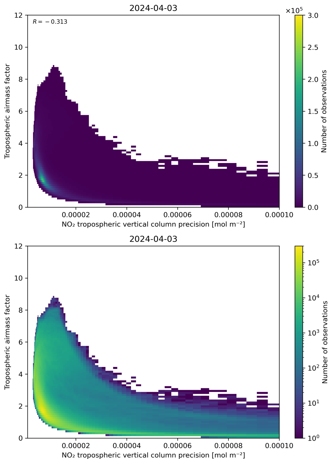
Figure 133: Scatter density plot of “NO 2 tropospheric vertical column precision” against “Tropospheric airmass factor” for 2024-04-02 to 2024-04-04.
