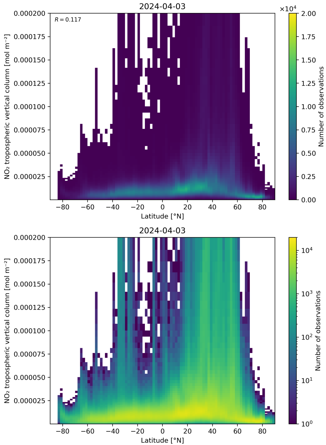
Figure 92: Scatter density plot of “Latitude” against “NO 2 tropospheric vertical column” for 2024-04-02 to 2024-04-04.
