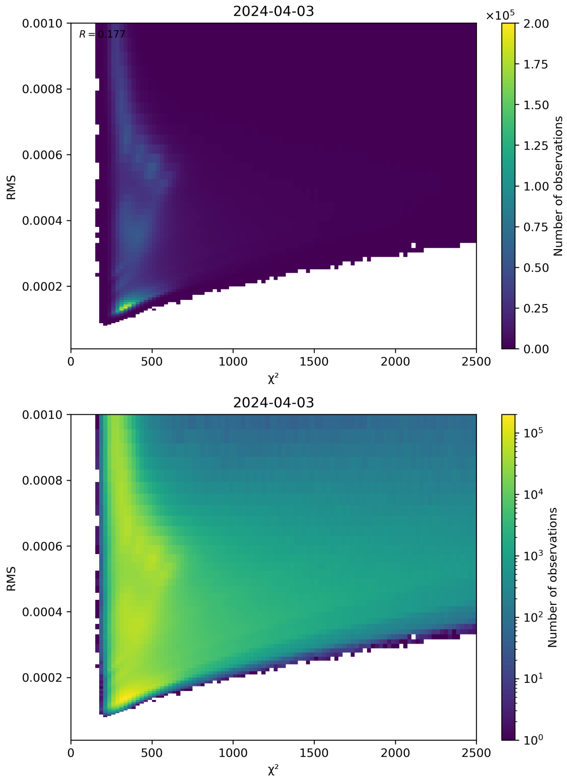
Figure 82: Scatter density plot of “ \chi^2 ” against “RMS” for 2024-04-02 to 2024-04-04.
