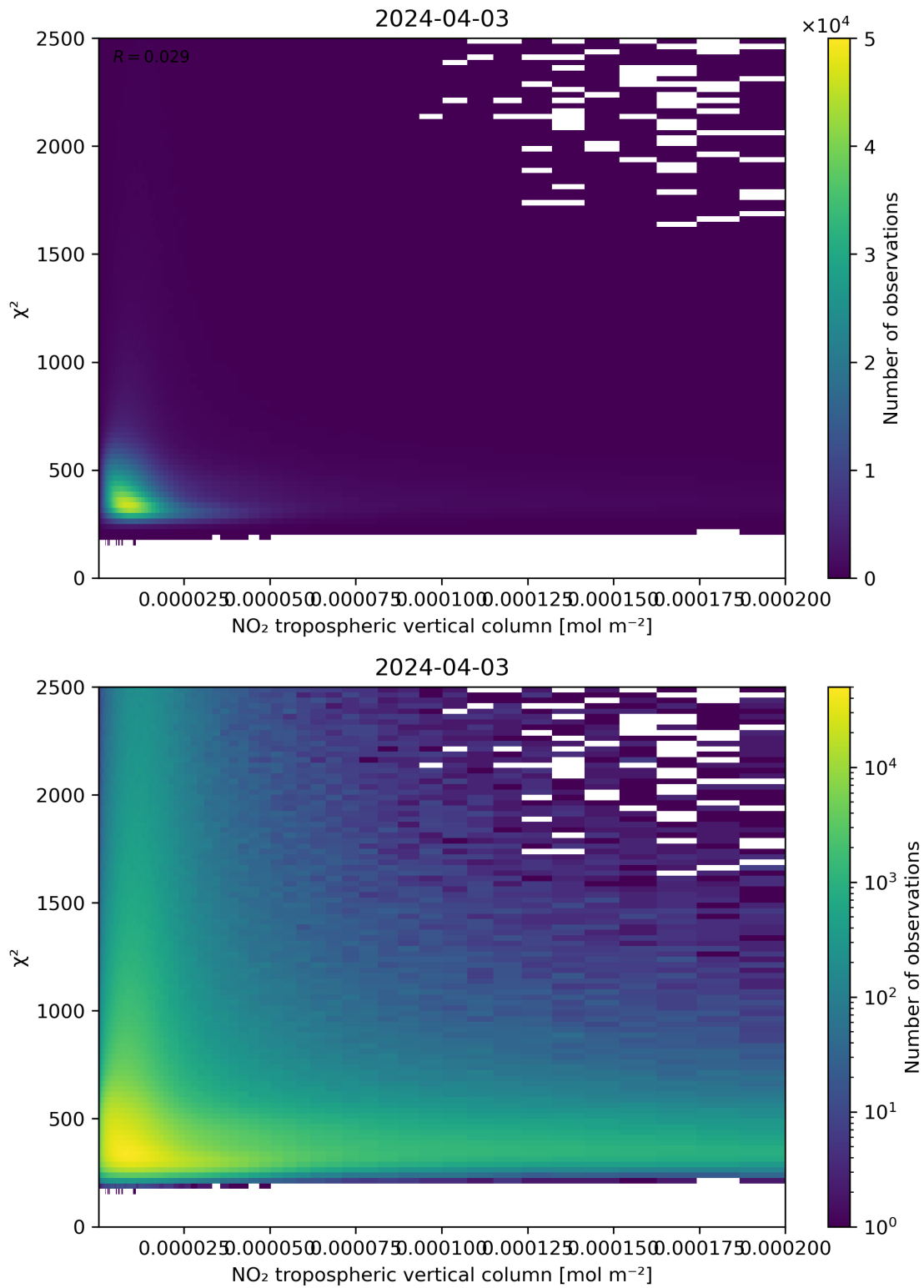
Figure 124: Scatter density plot of “NO 2 tropospheric vertical column” against “ \chi^2 ” for 2024-04-02 to 2024-04-04.
