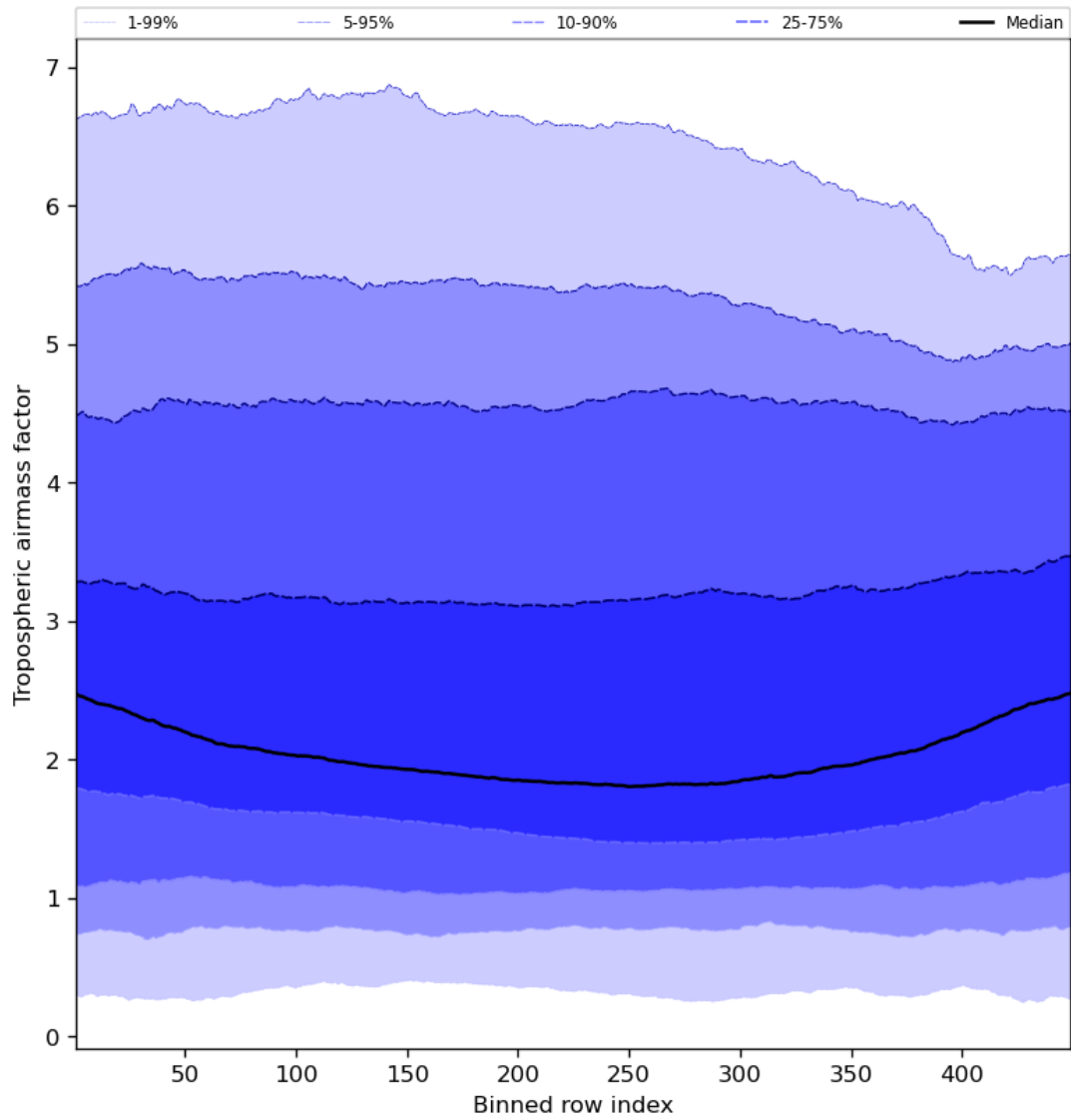
Figure 48: Along track statistics of “Tropospheric airmass factor” for 2024-04-02 to 2024-04-04
