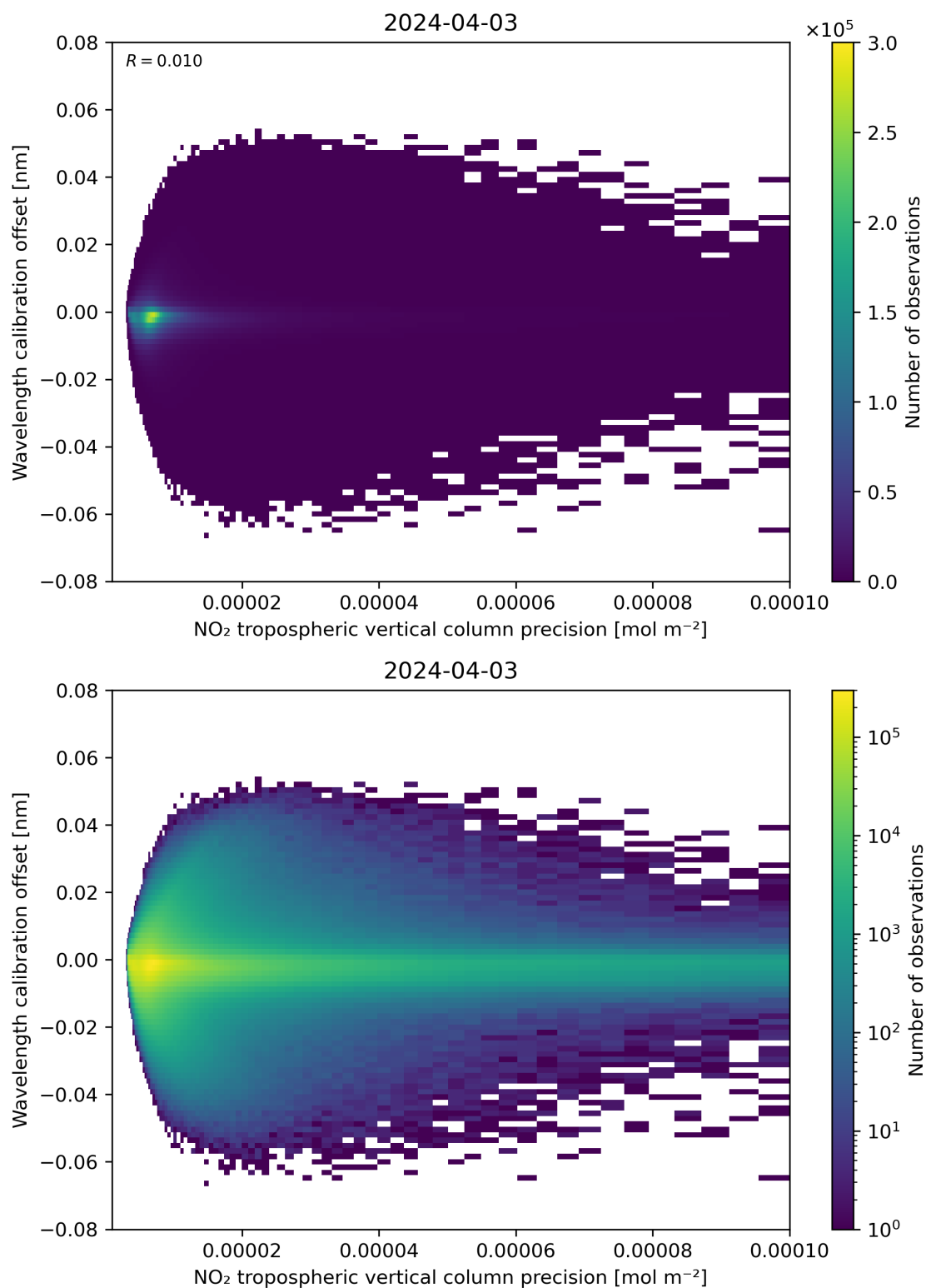
Figure 141: Scatter density plot of “NO 2 tropospheric vertical column precision” against “Wavelength calibration offset” for 2024-04-02 to 2024-04-04.
