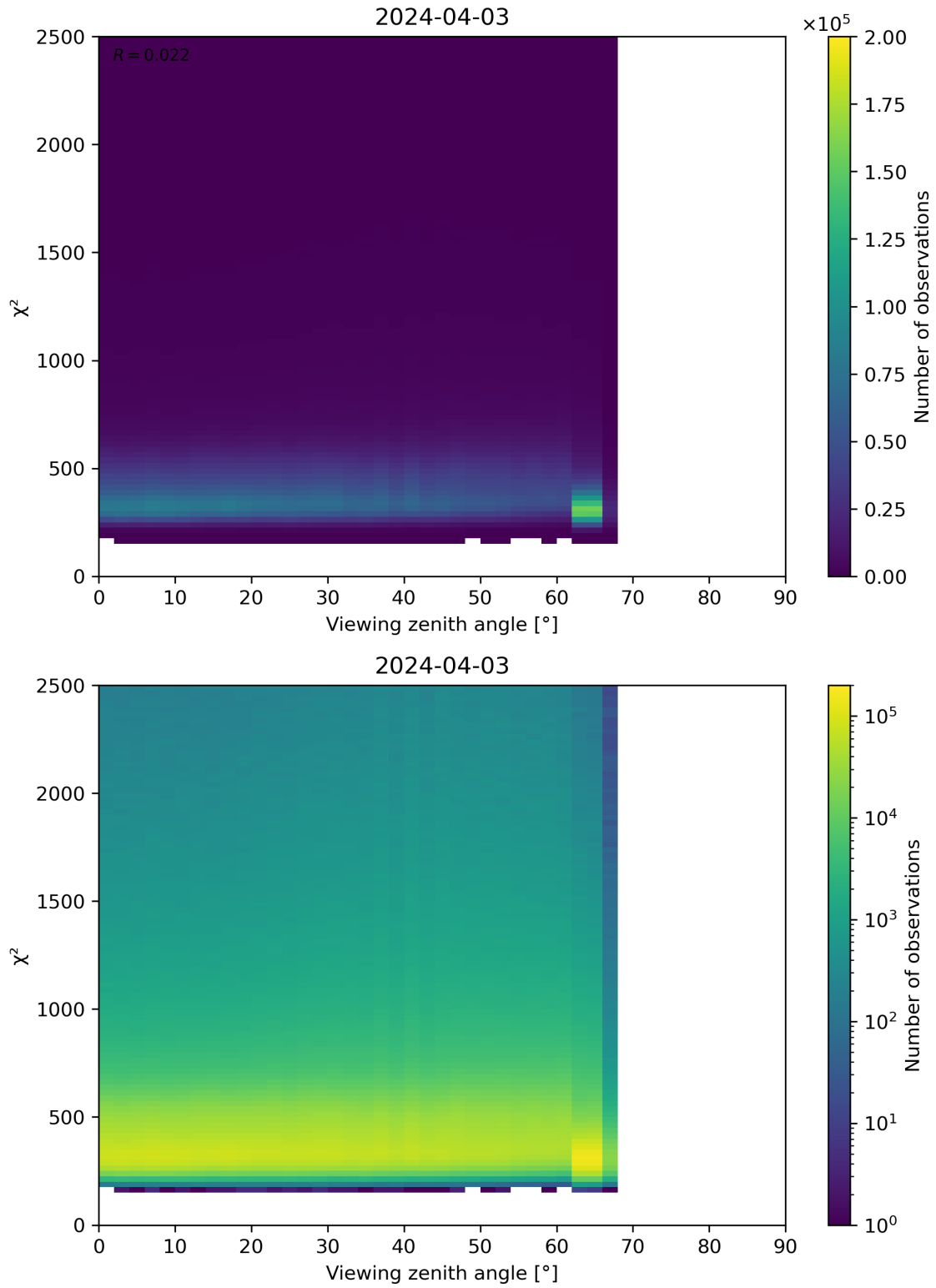
Figure 162: Scatter density plot of “Viewing zenith angle” against “ \chi^2 ” for 2024-04-02 to 2024-04-04.
