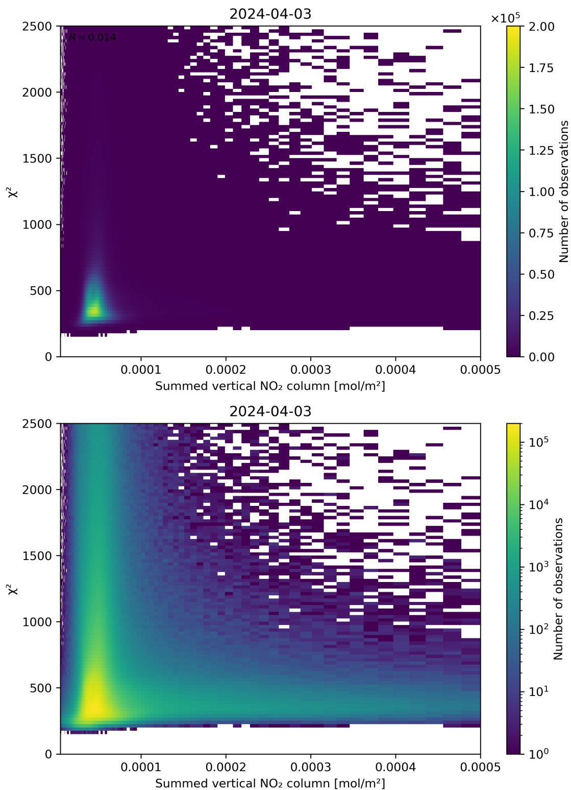
Figure 104: Scatter density plot of “Summed vertical NO 2 column” against “ \chi^2 ” for 2024-04-02 to 2024-04-04.
