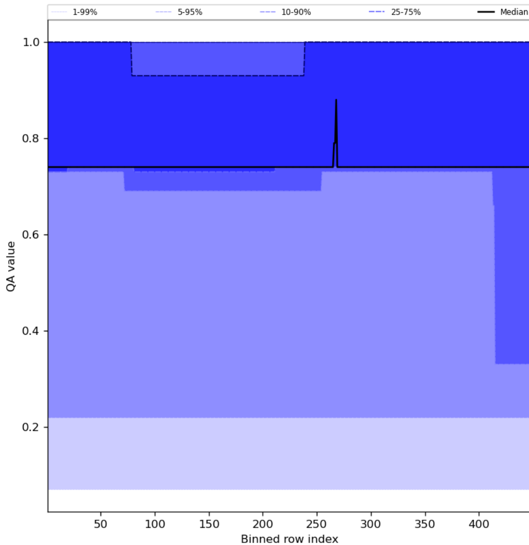
Figure 45: Along track statistics of “QA value” for 2024-04-02 to 2024-04-04
