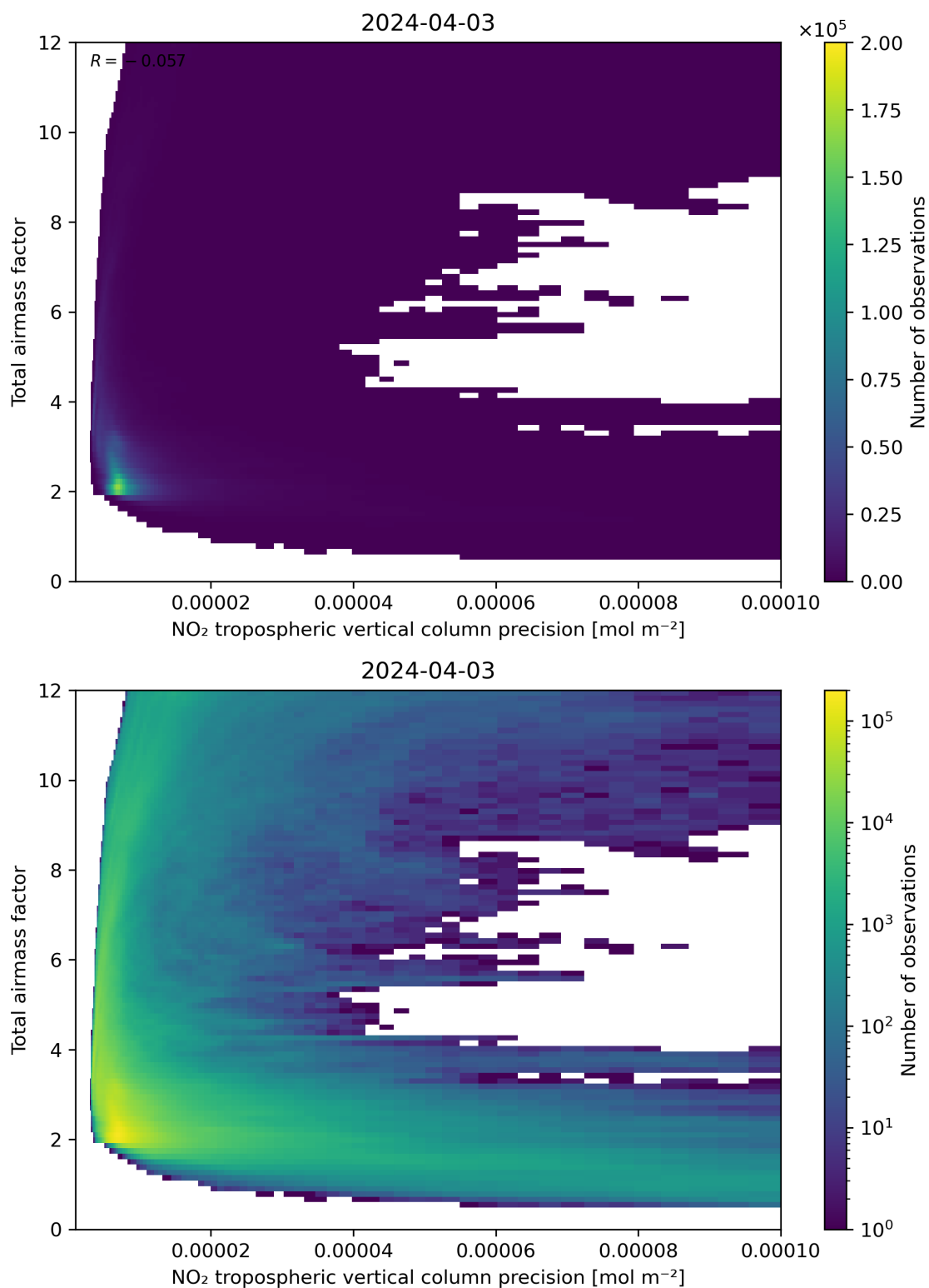
Figure 132: Scatter density plot of “NO 2 tropospheric vertical column precision” against “Total air mass factor” for 2024-04-02 to 2024-04-04.
