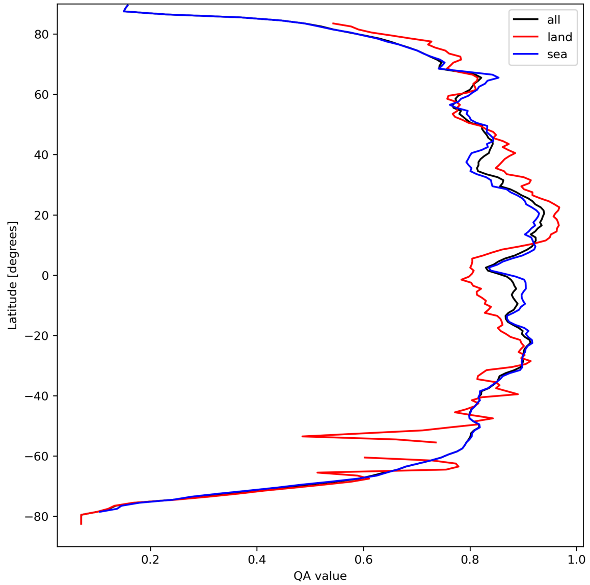
Figure 11: Zonal average of “QA value” for 2024-04-02 to 2024-04-04.
