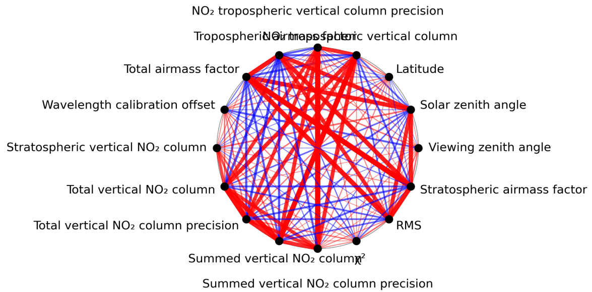
Figure 1: Map of correlation graph for 2024-04-02 to 2024-04-04.
