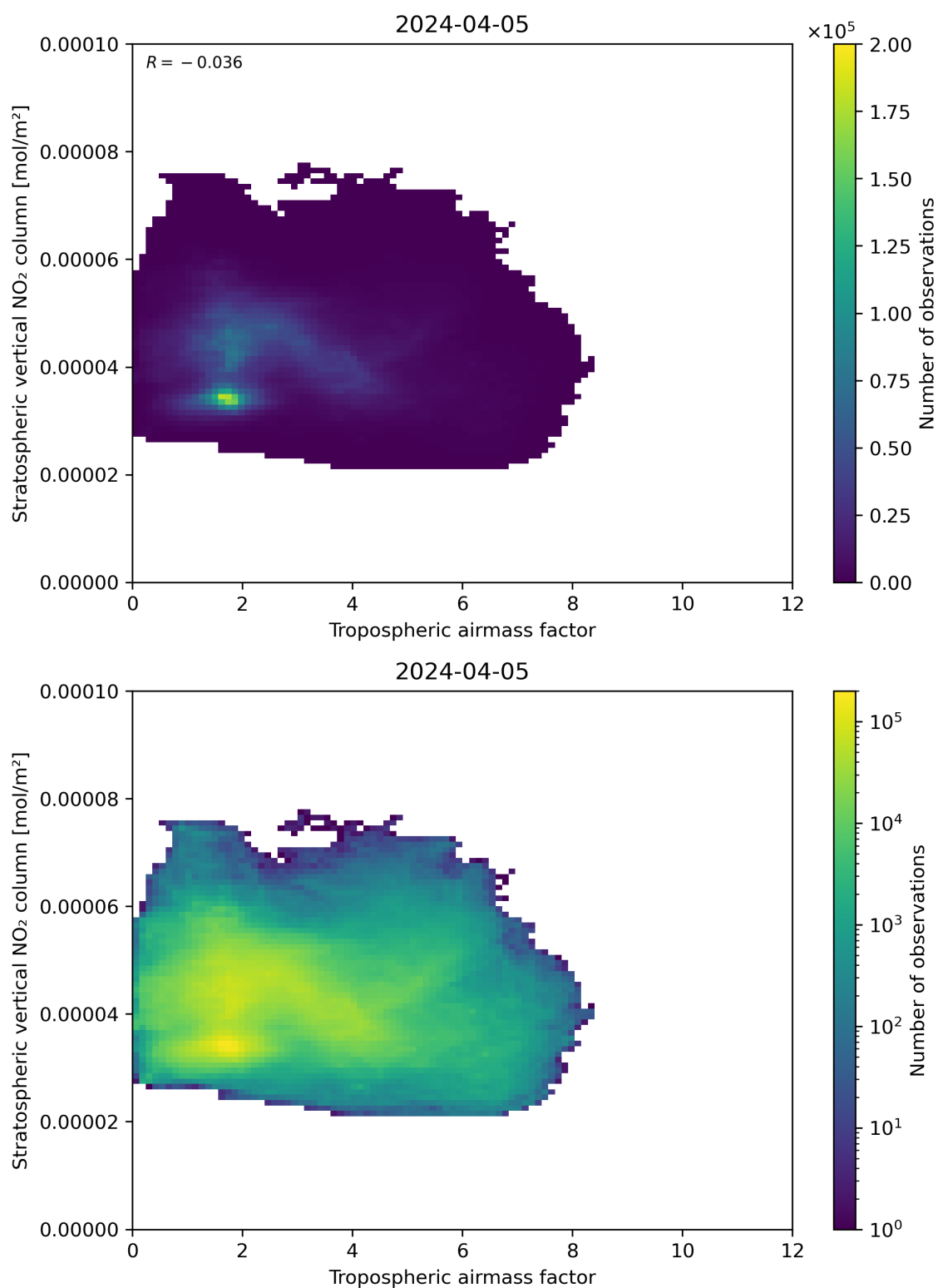
Figure 74: Scatter density plot of “Tropospheric air mass factor” against “Stratospheric vertical NO 2 column” for 2024-04-05 to 2024-04-06.
