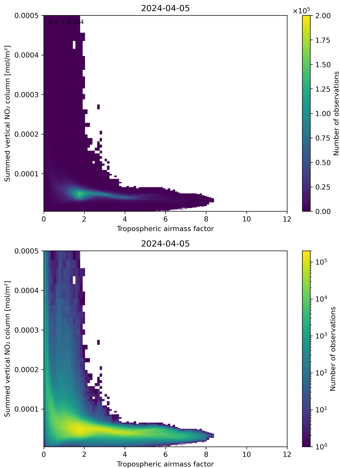
Figure 75: Scatter density plot of “Tropospheric air mass factor” against “Summed vertical NO 2 column” for 2024-04-05 to 2024-04-06.
