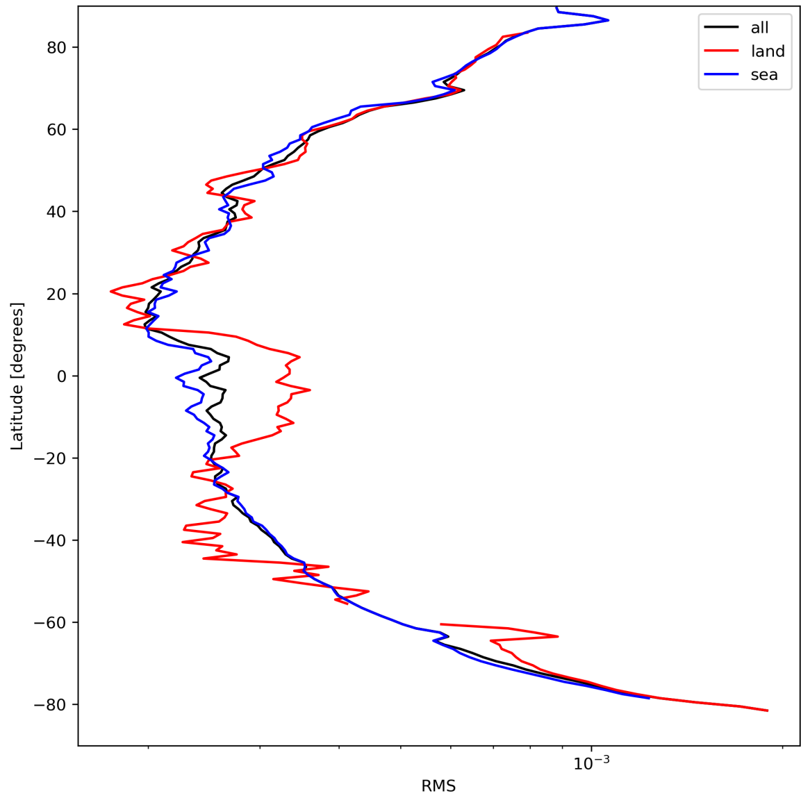
Figure 26: Zonal average of “RMS” for 2024-04-05 to 2024-04-06.
