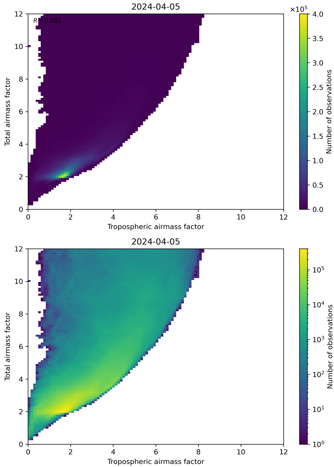
Figure 72: Scatter density plot of “Tropospheric airmass factor” against “Total airmass factor” for 2024-04-05 to 2024-04-06.
