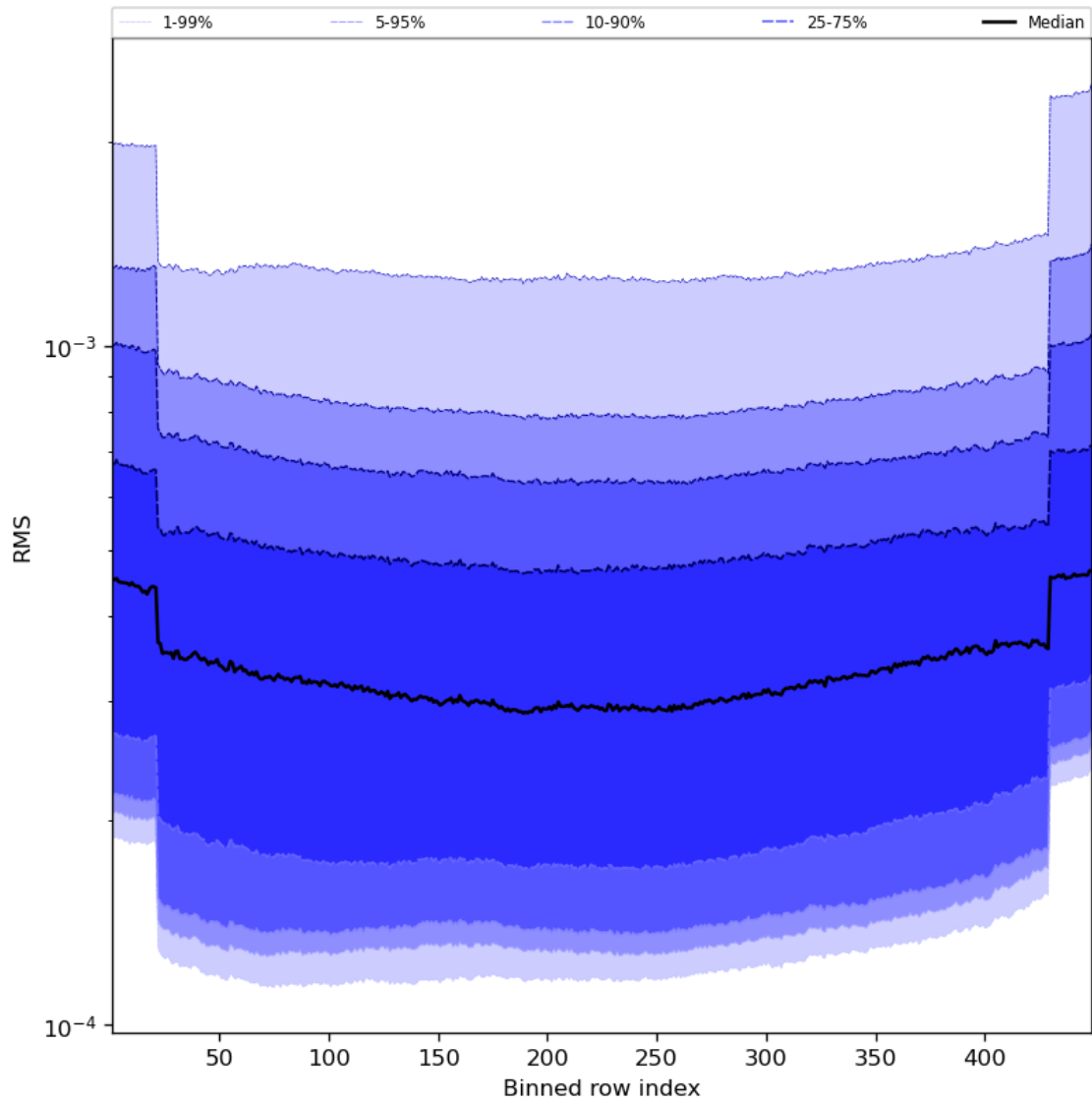
Figure 60: Along track statistics of “RMS” for 2024-04-05 to 2024-04-06
