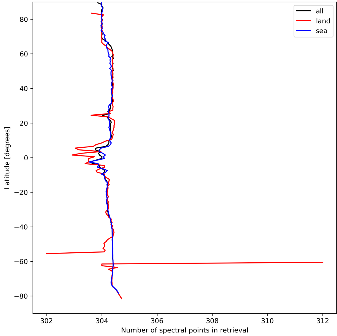
Figure 16: Zonal average of “Number of spectral points in retrieval” for 2024-04-05 to 2024-04-06.
