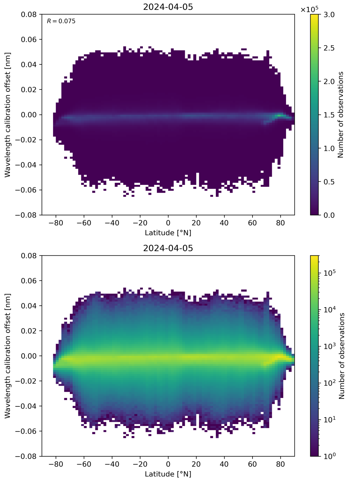
Figure 95: Scatter density plot of “Latitude” against “Wavelength calibration offset” for 2024-04-05 to 2024-04-06.
