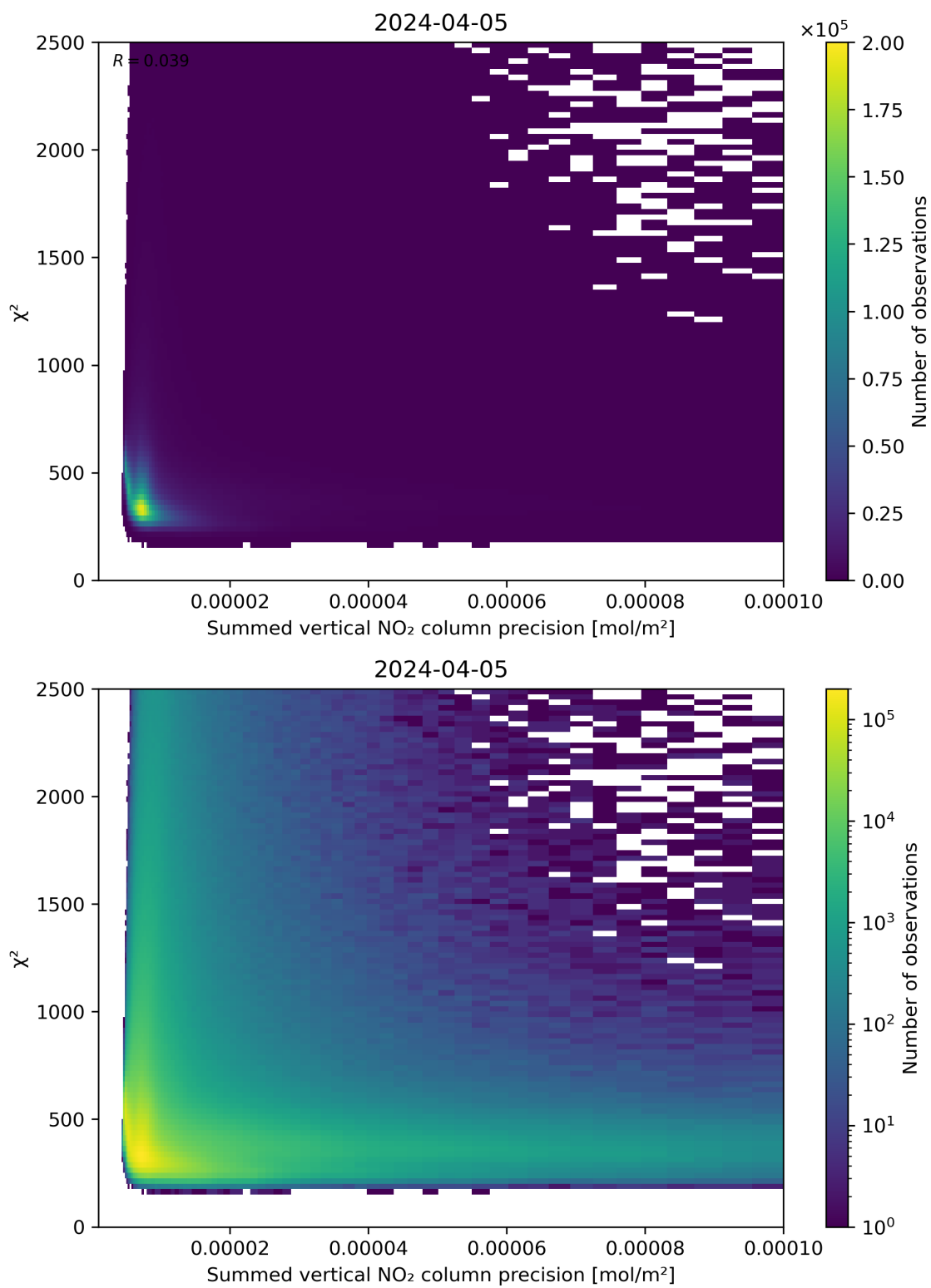
Figure 107: Scatter density plot of “Summed vertical NO 2 column precision” against “ \chi^2 ” for 2024-04-05 to 2024-04-06.
