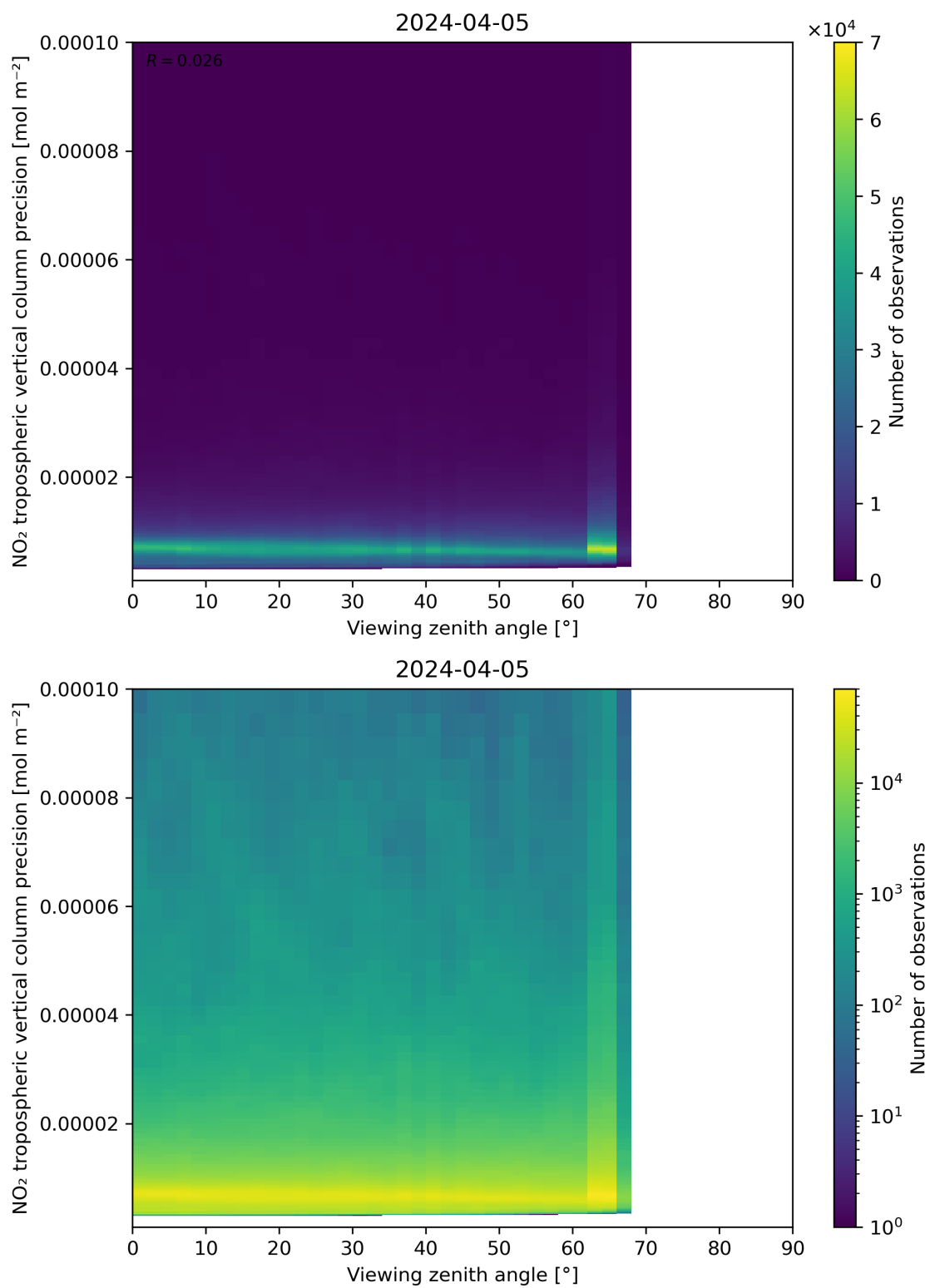
Figure 170: Scatter density plot of “Viewing zenith angle” against “NO 2 tropospheric vertical column precision” for 2024-04-05 to 2024-04-06.
