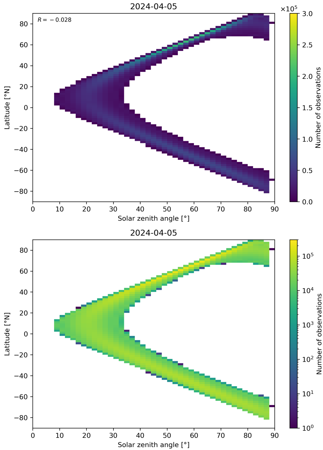
Figure 149: Scatter density plot of “Solar zenith angle” against “Latitude” for 2024-04-05 to 2024-04-06.
