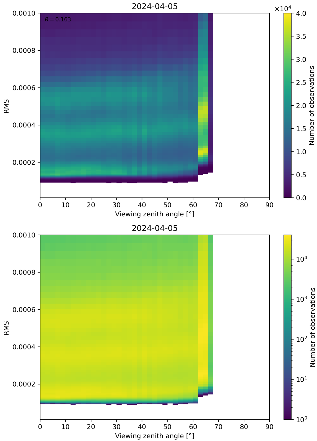
Figure 171: Scatter density plot of “Viewing zenith angle” against “RMS” for 2024-04-05 to 2024-04-06.
