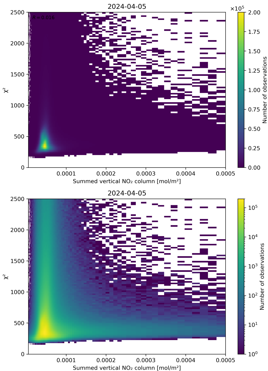
Figure 104: Scatter density plot of “Summed vertical NO 2 column” against “ \chi^2 ” for 2024-04-05 to 2024-04-06.
