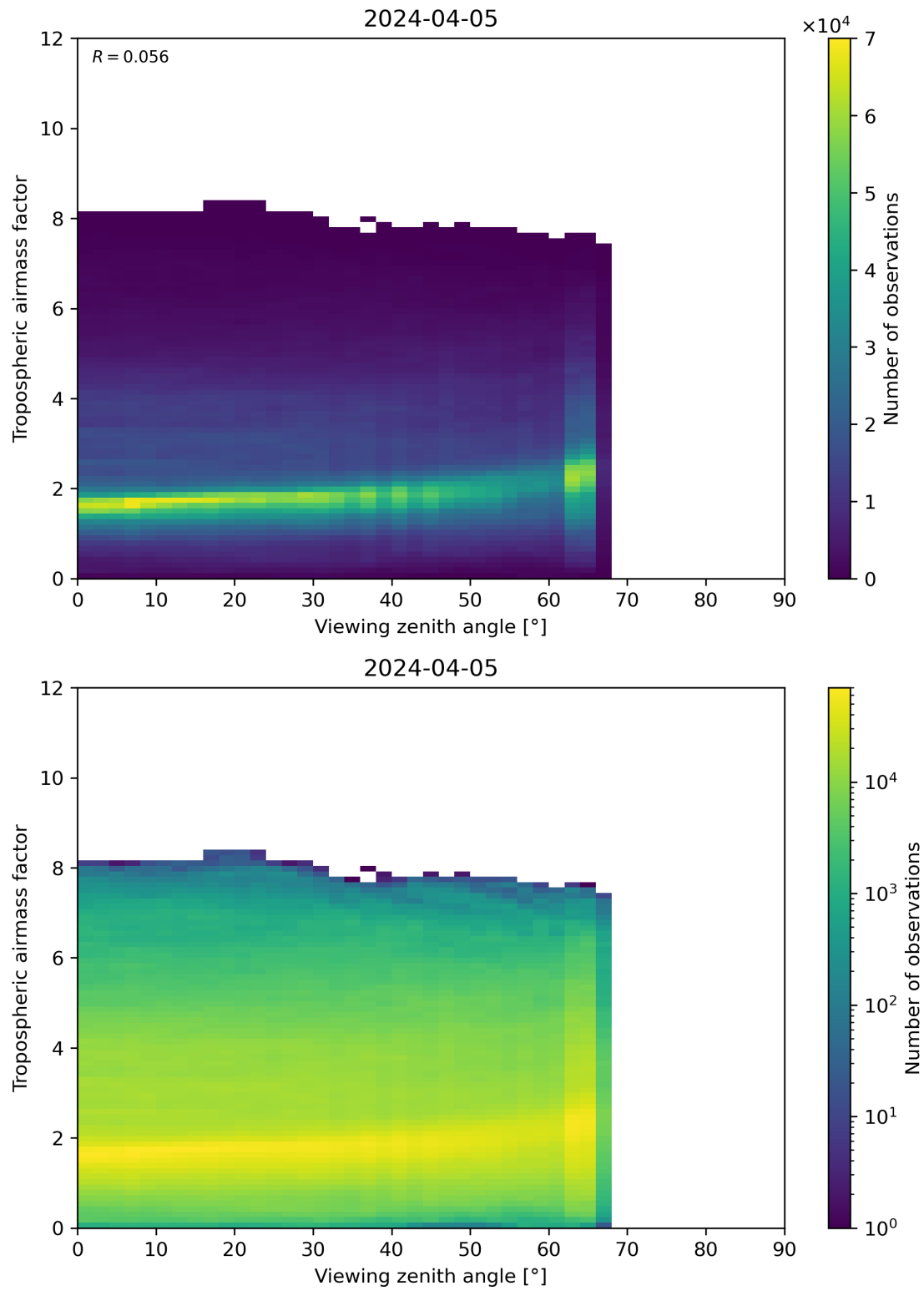
Figure 161: Scatter density plot of “Viewing zenith angle” against “Tropospheric airmass factor” for 2024-04-05 to 2024-04-06.
