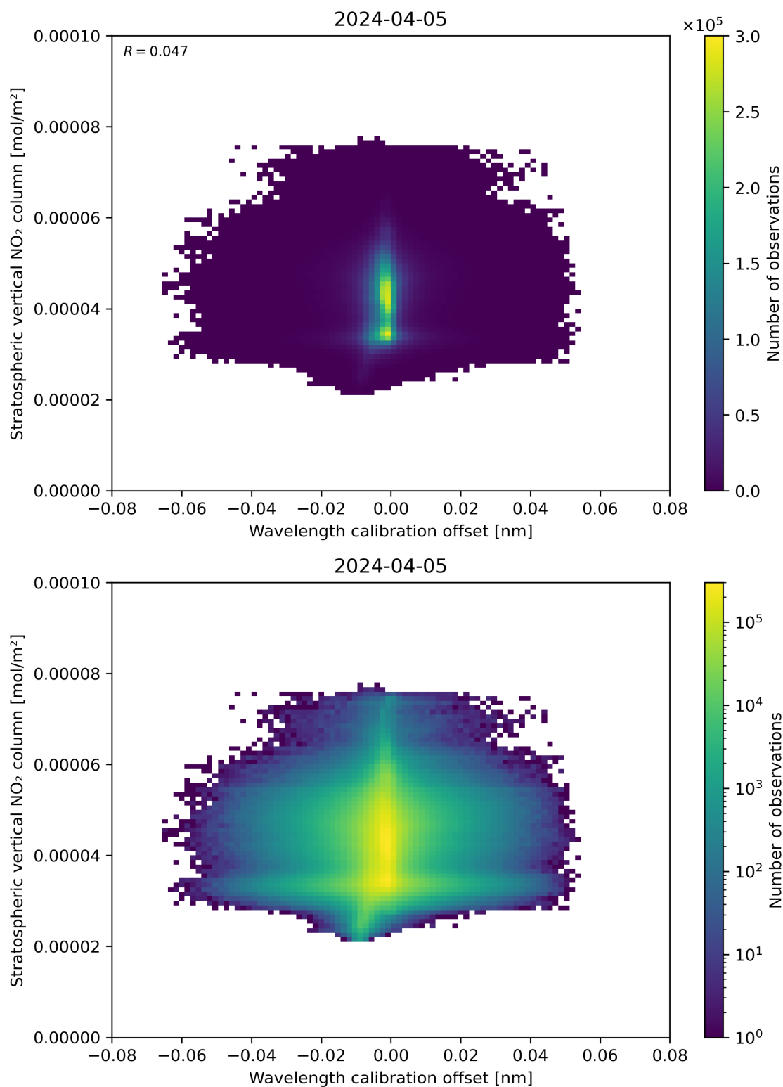
Figure 176: Scatter density plot of “Wavelength calibration offset” against “Stratospheric vertical NO 2 column” for 2024-04-05 to 2024-04-06.
