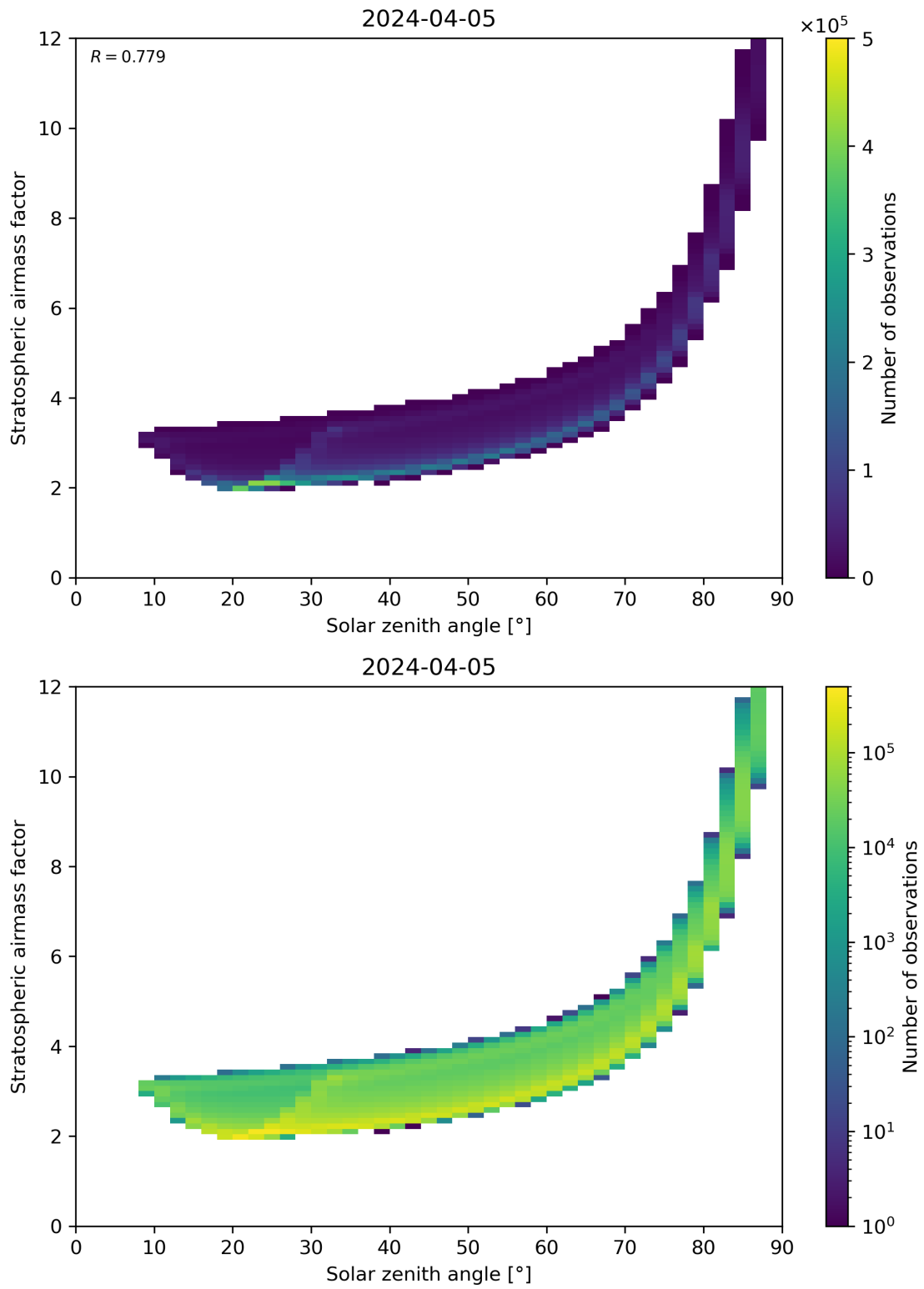
Figure 145: Scatter density plot of “Solar zenith angle” against “Stratospheric airmass factor” for 2024-04-05 to 2024-04-06.
