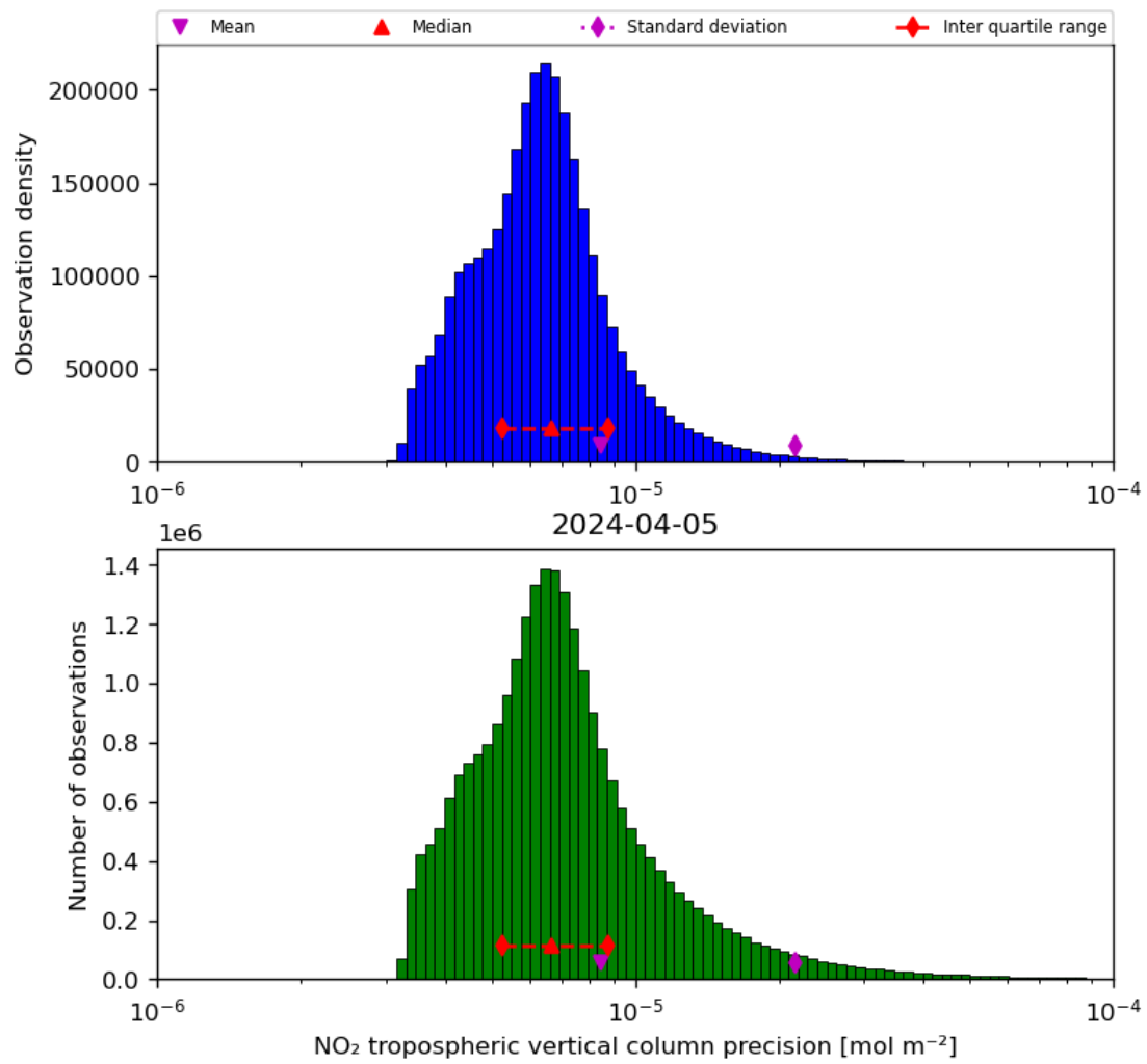
Figure 30: Histogram of “NO 2 tropospheric vertical column precision” for 2024-04-05 to 2024-04-06
