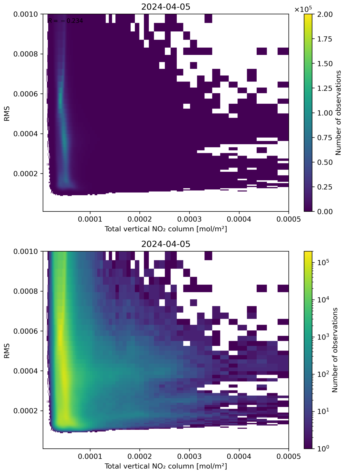
Figure 120: Scatter density plot of “Total vertical NO 2 column” against “RMS” for 2024-04-05 to 2024-04-06.
