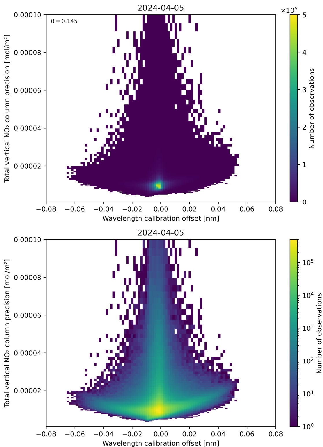
Figure 180: Scatter density plot of “Wavelength calibration offset” against “Total vertical NO 2 column precision” for 2024-04-05 to 2024-04-06.
