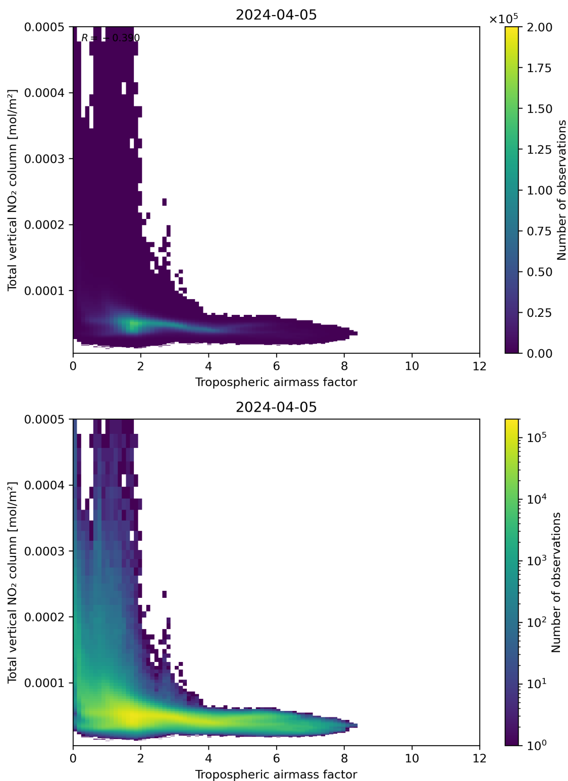
Figure 77: Scatter density plot of “Tropospheric airmass factor” against “Total vertical NO 2 column” for 2024-04-05 to 2024-04-06.
