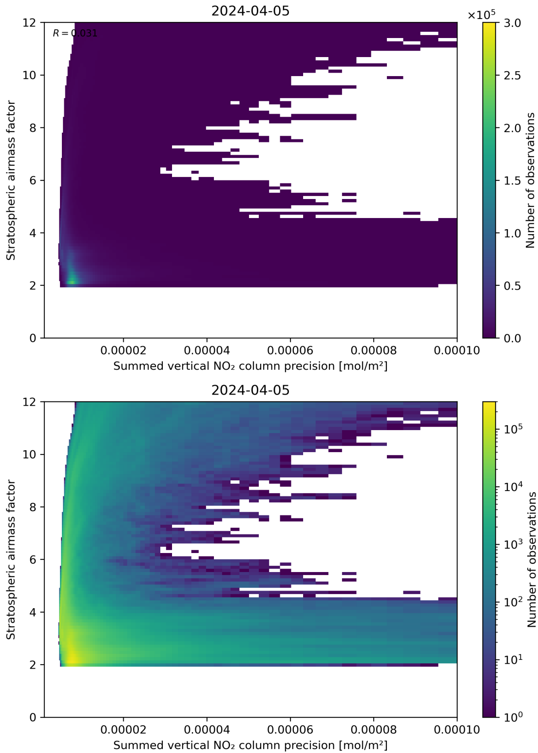
Figure 106: Scatter density plot of “Summed vertical NO 2 column precision” against “Stratospheric airmass factor” for 2024-04-05 to 2024-04-06.
