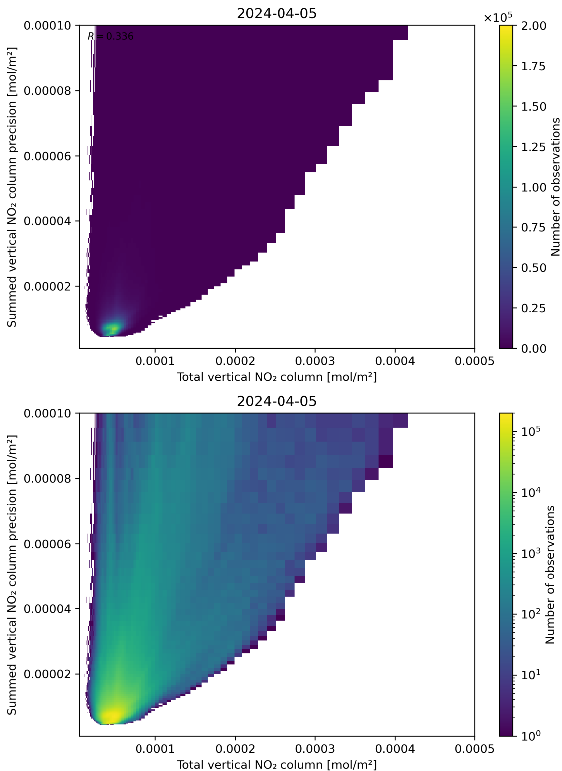
Figure 113: Scatter density plot of “Total vertical NO 2 column” against “Summed vertical NO 2 column precision” for 2024-04-05 to 2024-04-06.
