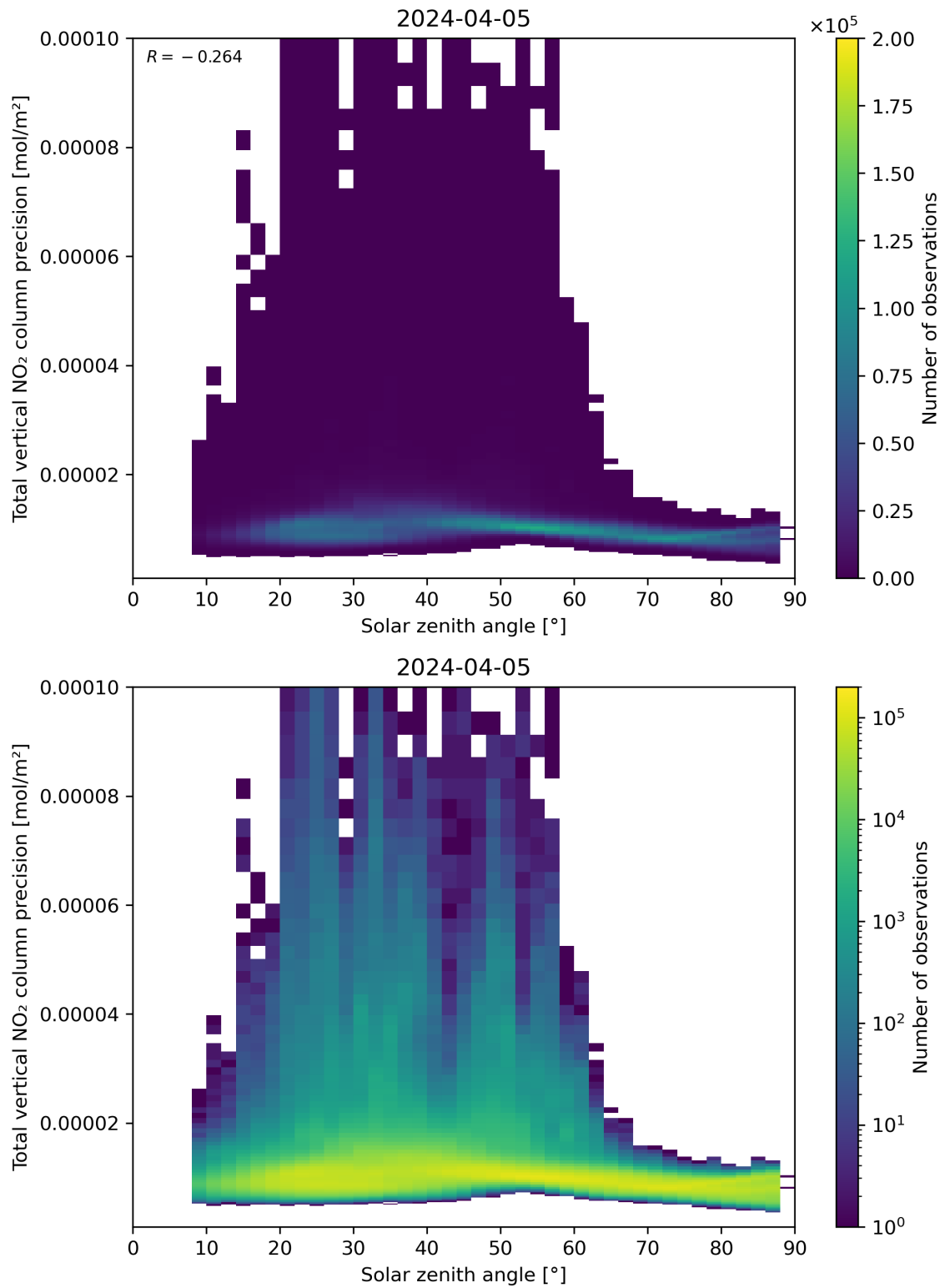
Figure 154: Scatter density plot of “Solar zenith angle” against “Total vertical NO 2 column precision” for 2024-04-05 to 2024-04-06.
