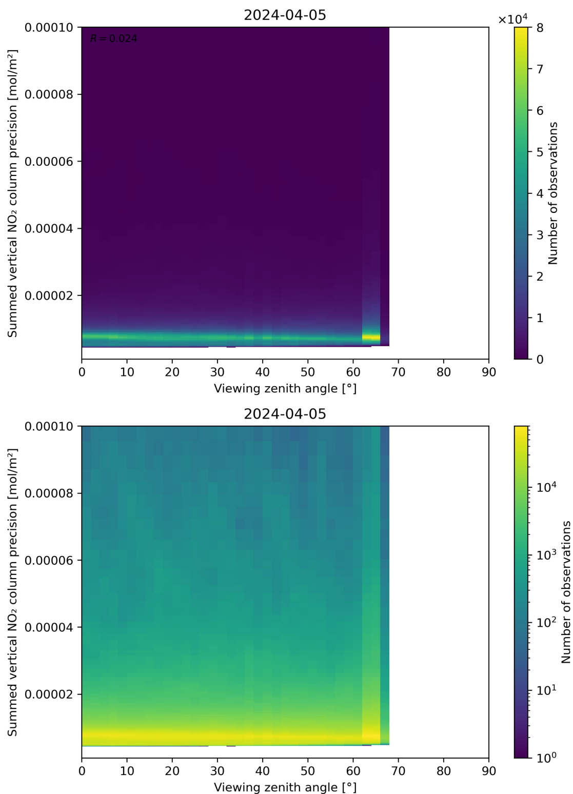
Figure 166: Scatter density plot of “Viewing zenith angle” against “Summed vertical NO 2 column precision” for 2024-04-05 to 2024-04-06.
