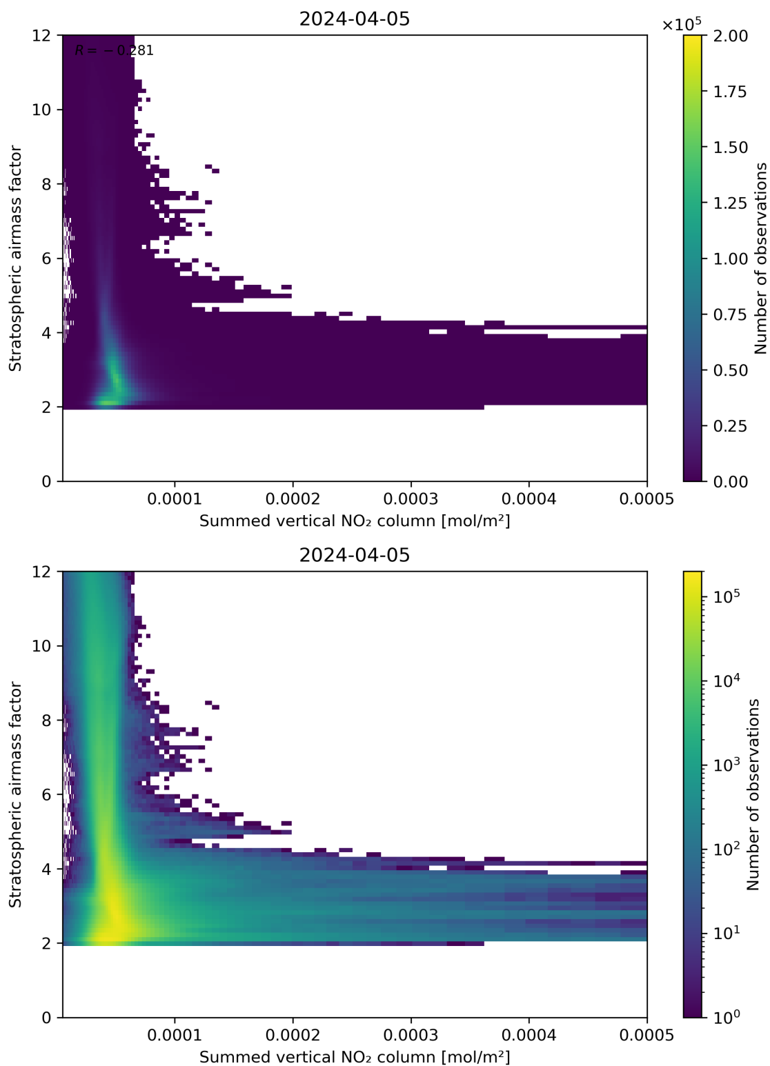
Figure 103: Scatter density plot of “Summed vertical NO 2 column” against “Stratospheric airmass factor” for 2024-04-05 to 2024-04-06.
