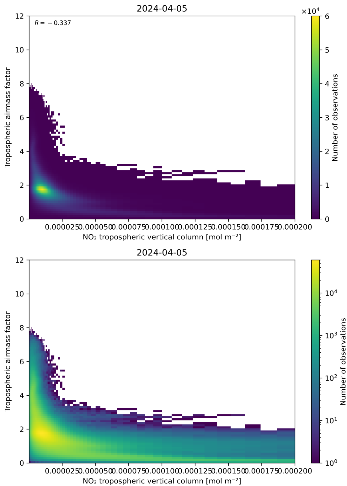
Figure 123: Scatter density plot of “NO 2 tropospheric vertical column” against “Tropospheric air mass factor” for 2024-04-05 to 2024-04-06.
