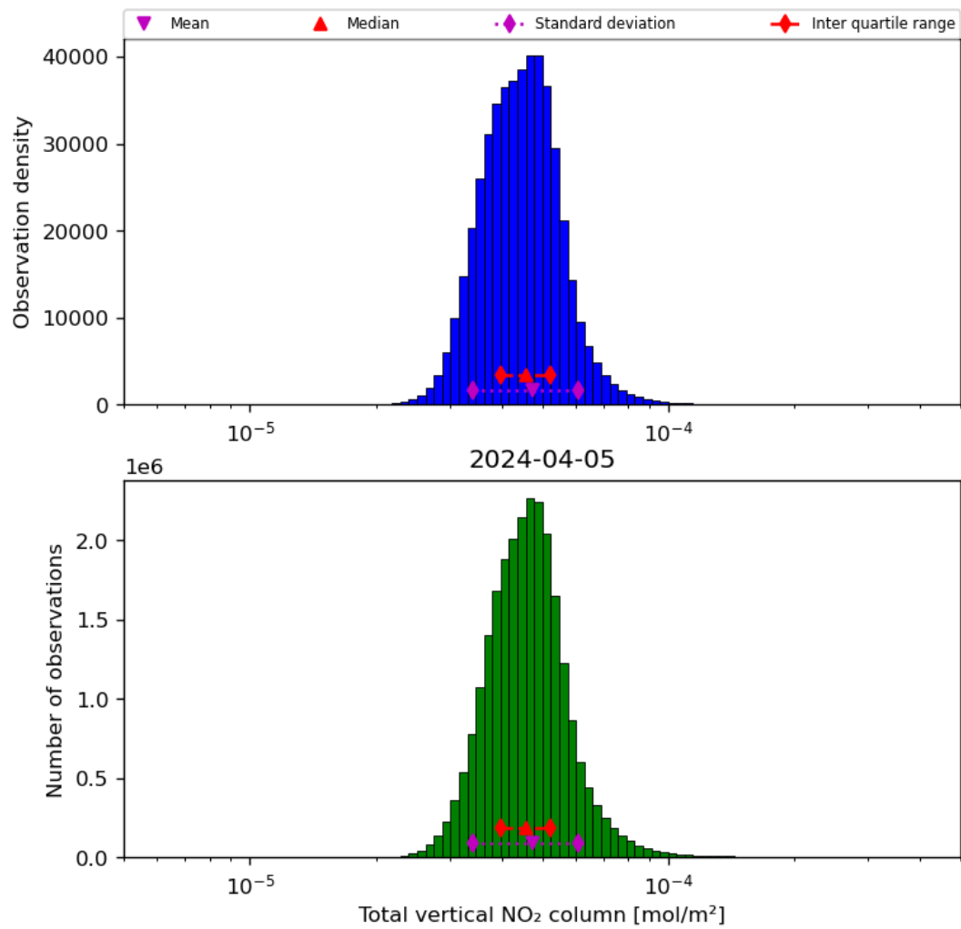
Figure 38: Histogram of "Total vertical NO 2 column" for 2024-04-05 to 2024-04-06
