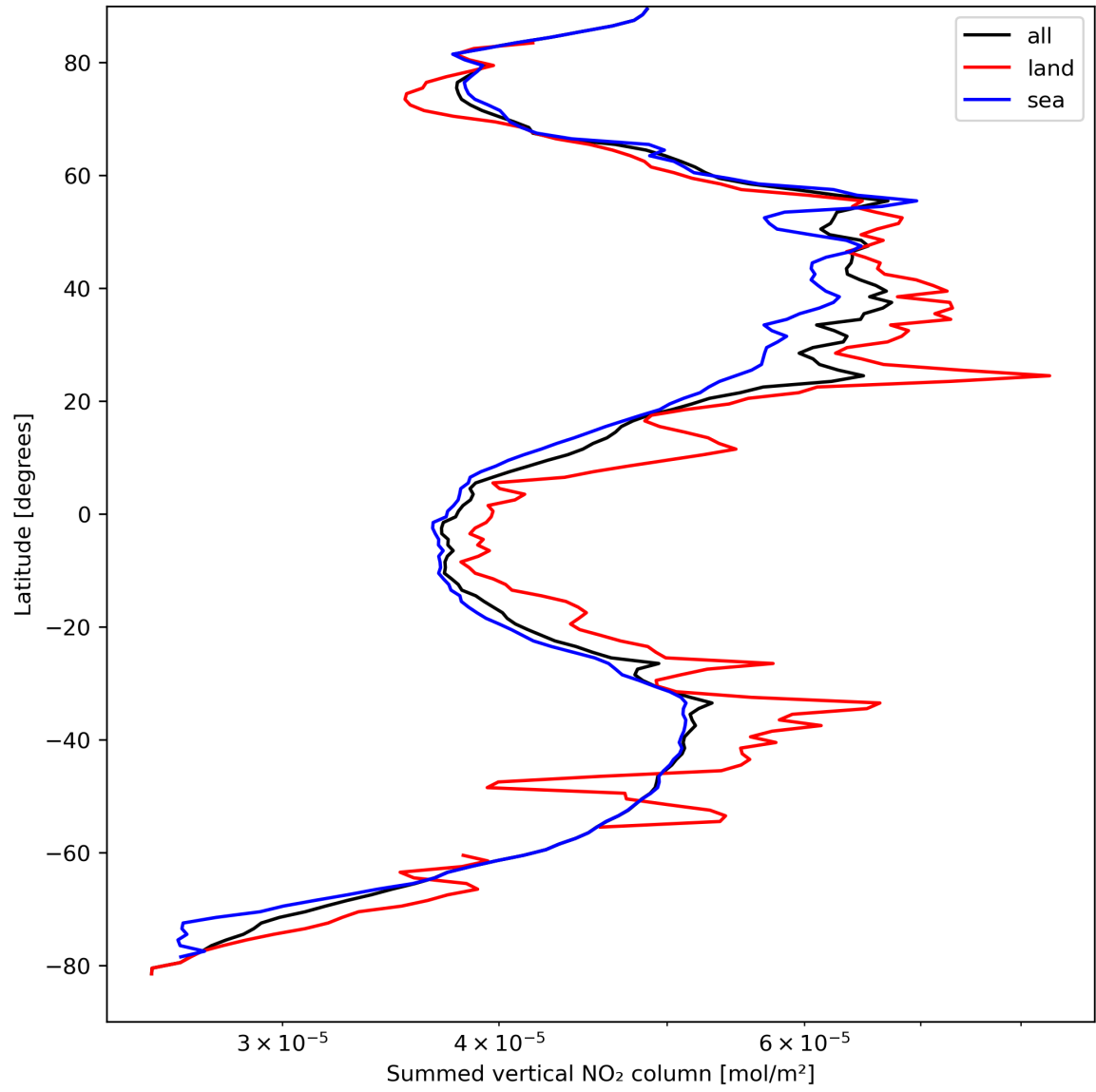
Figure 23: Zonal average of “Summed vertical NO 2 column” for 2024-04-05 to 2024-04-06.
