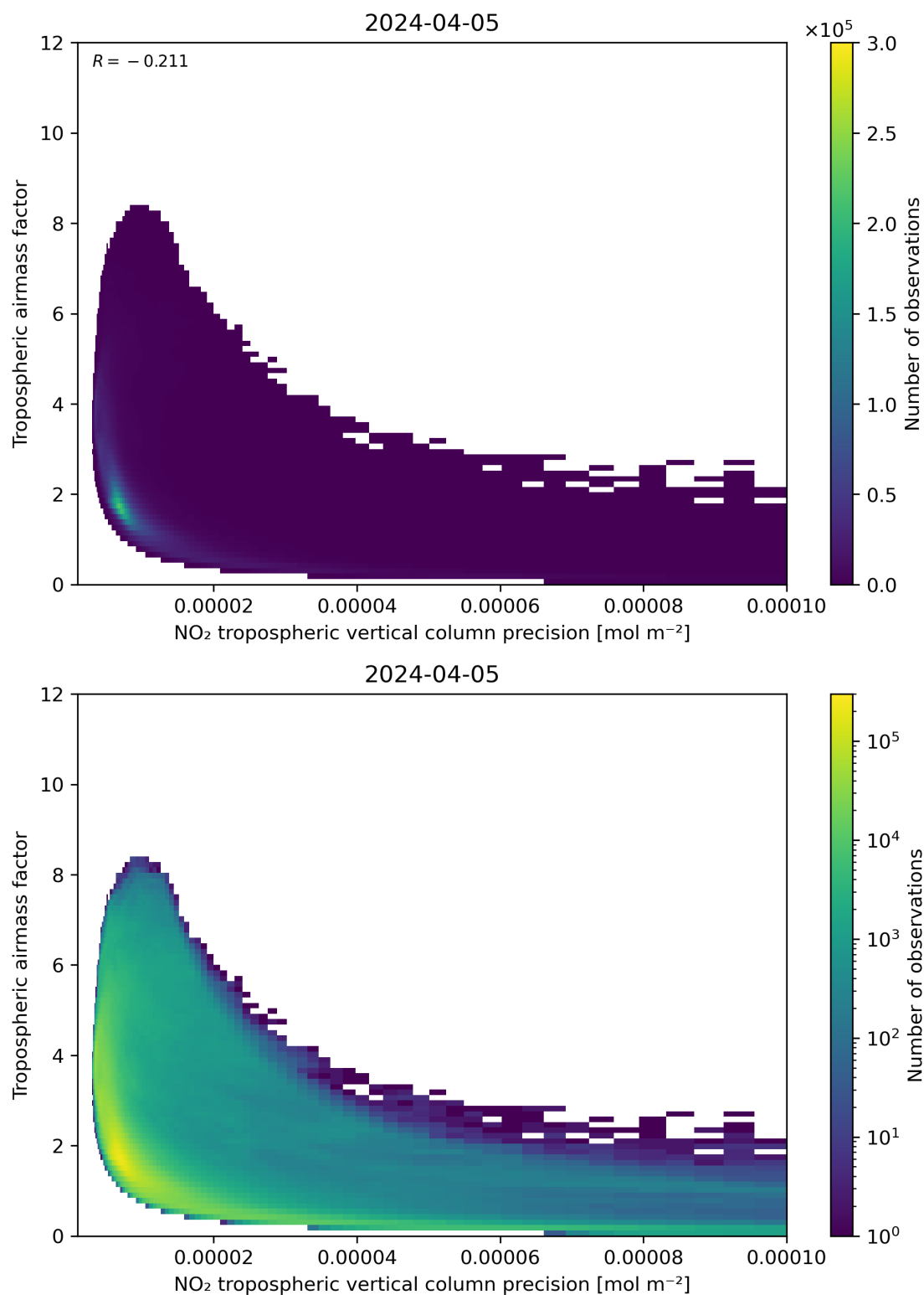
Figure 133: Scatter density plot of “NO 2 tropospheric vertical column precision” against “Tropospheric air mass factor” for 2024-04-05 to 2024-04-06.
