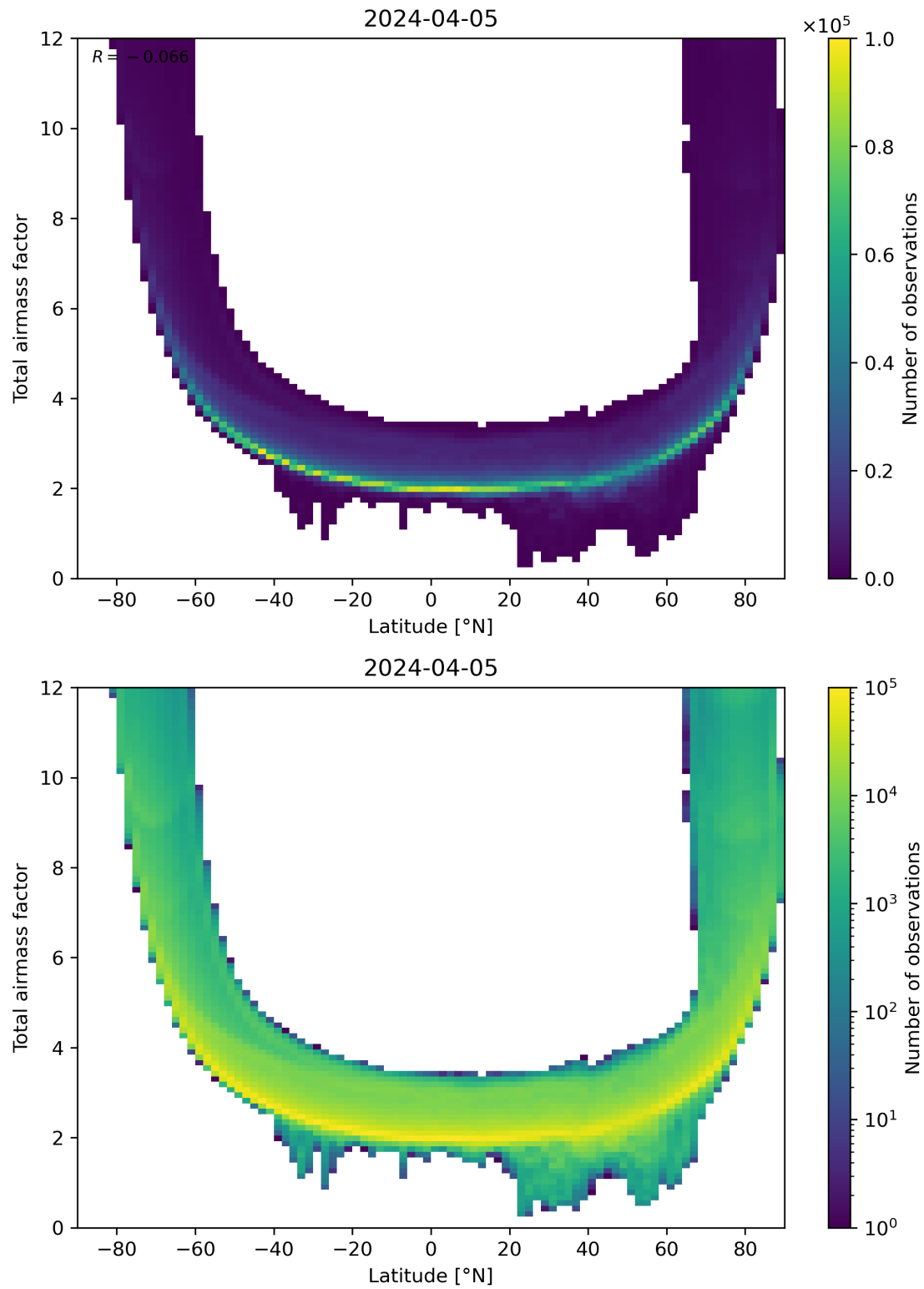
Figure 84: Scatter density plot of “Latitude” against “Total airmass factor” for 2024-04-05 to 2024-04-06.
