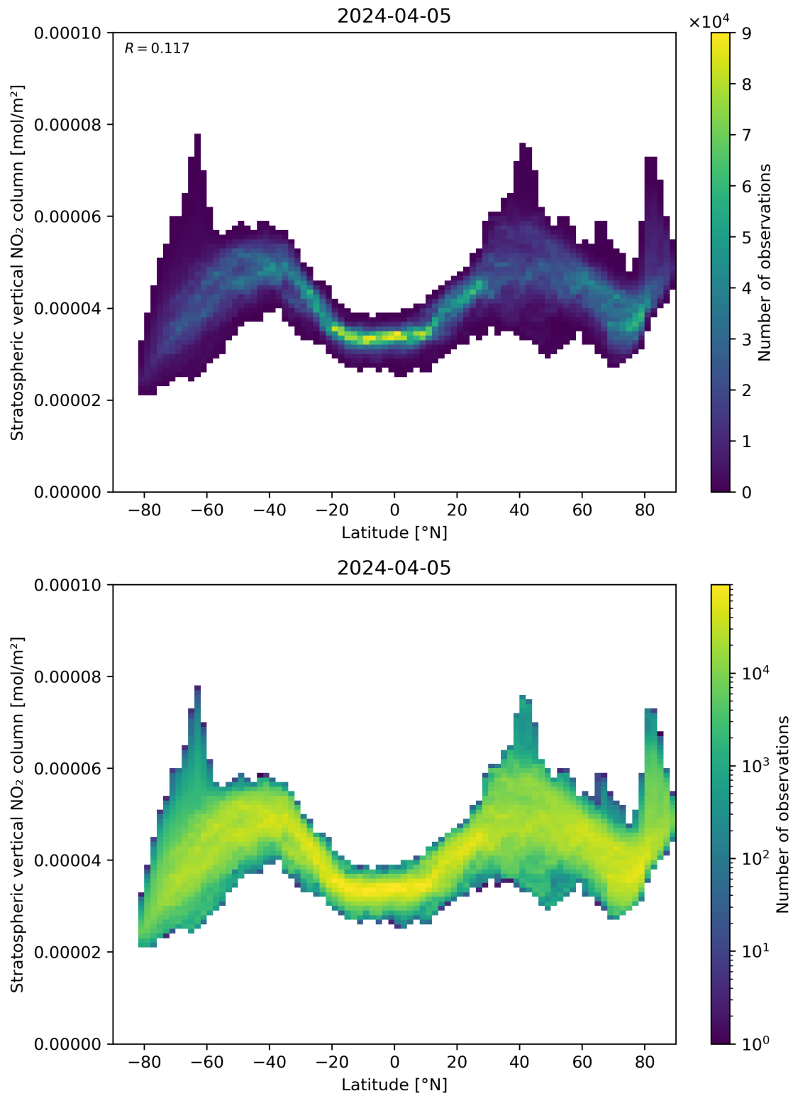
Figure 87: Scatter density plot of “Latitude” against “Stratospheric vertical NO 2 column” for 2024-04-05 to 2024-04-06.
