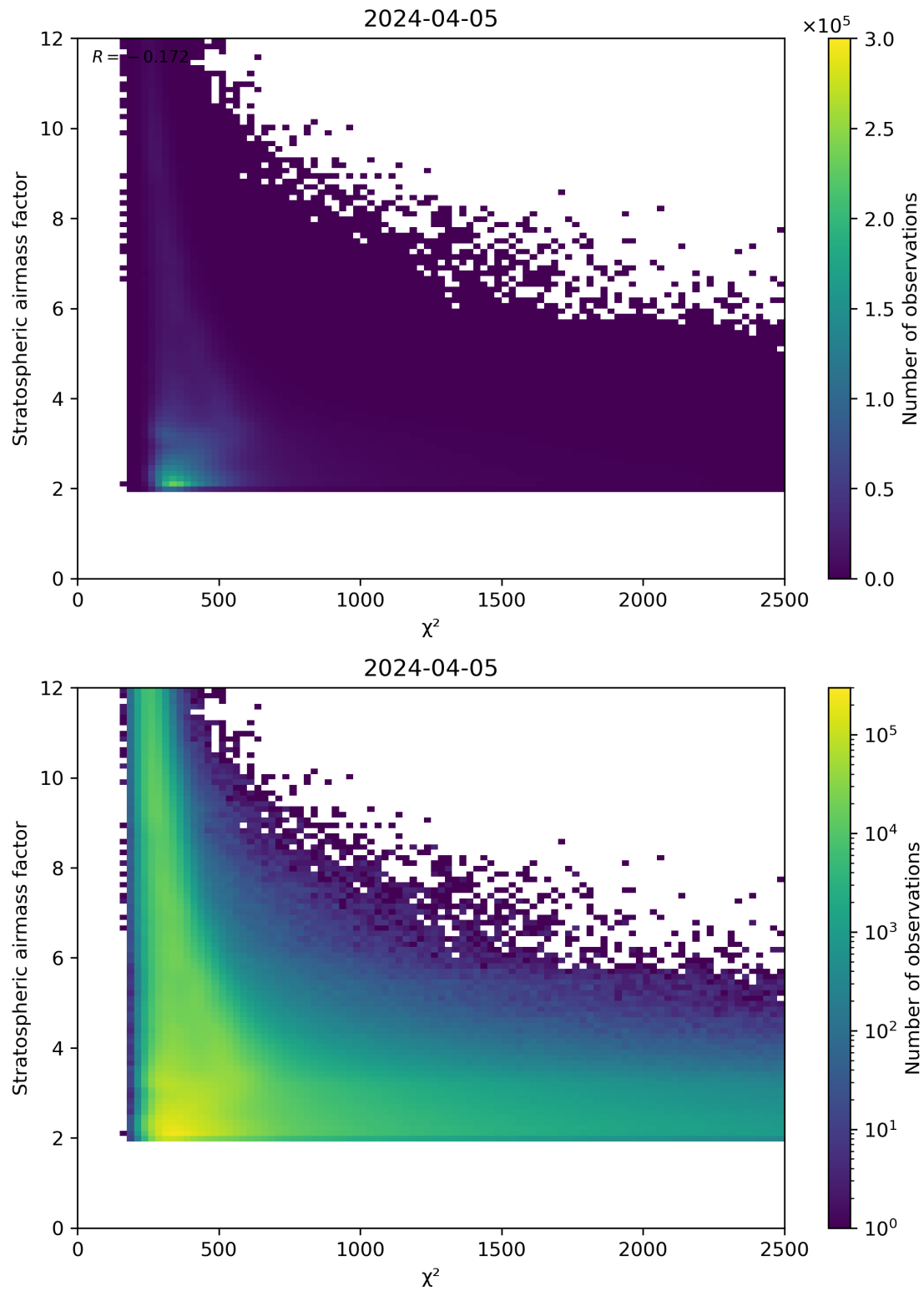
Figure 81: Scatter density plot of “ \chi^2 ” against “Stratospheric airmass factor” for 2024-04-05 to 2024-04-06.
