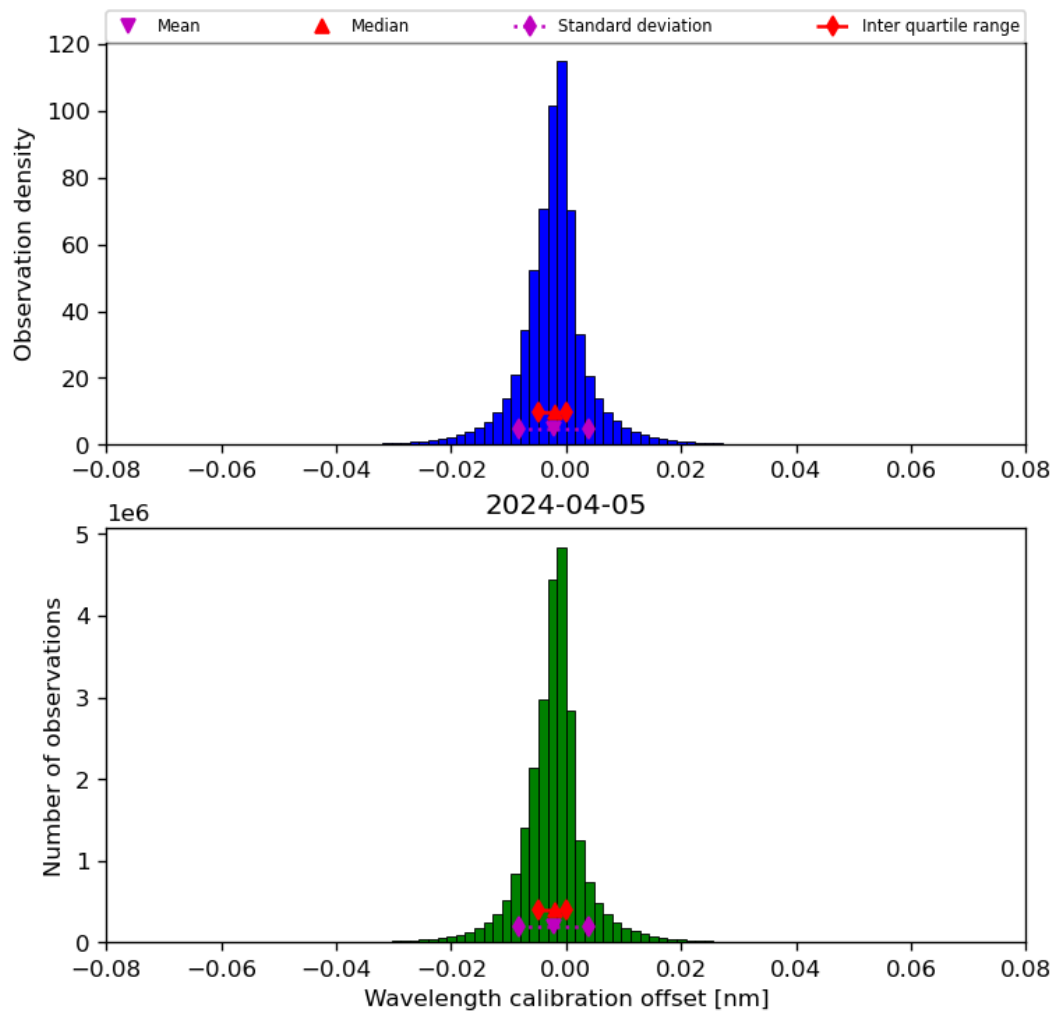
Figure 35: Histogram of “Wavelength calibration offset” for 2024-04-05 to 2024-04-06
