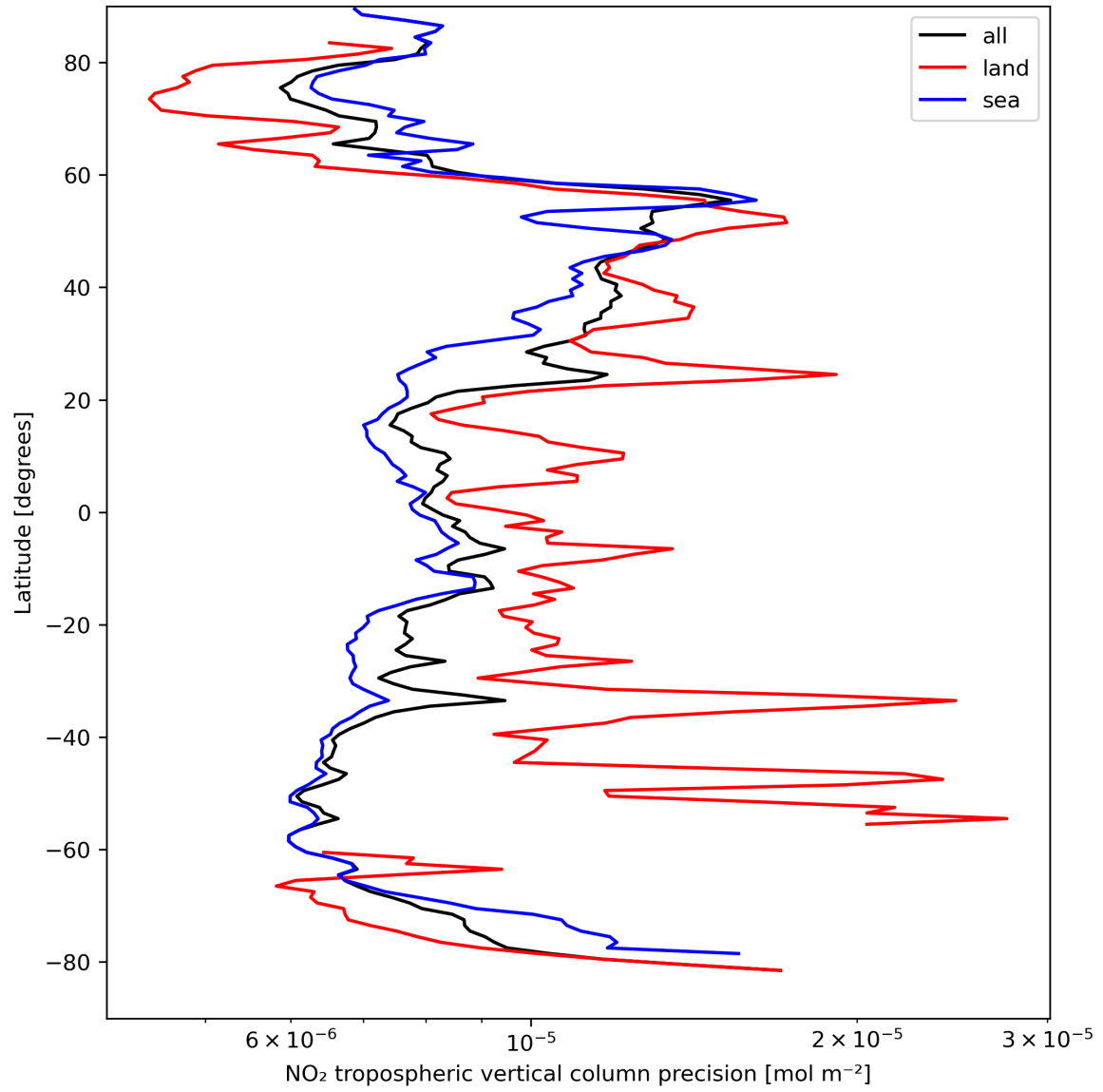
Figure 13: Zonal average of “NO 2 tropospheric vertical column precision” for 2024-04-05 to 2024-04-06.
