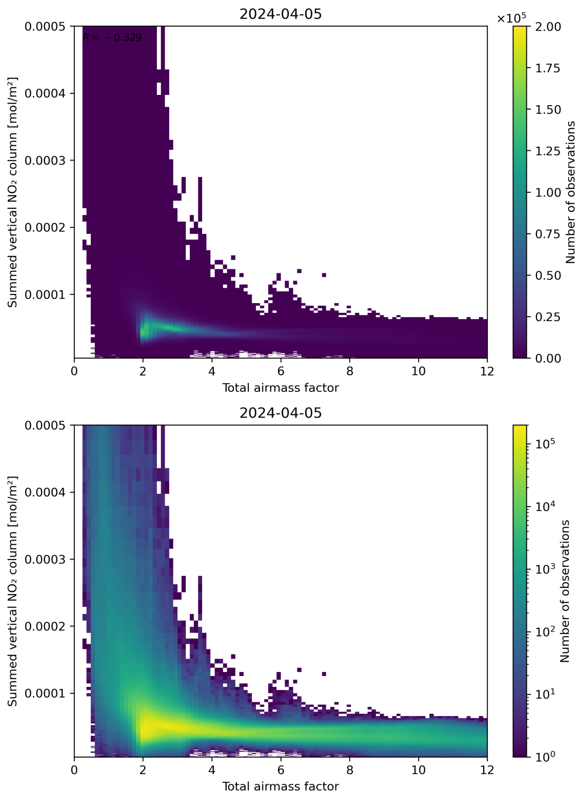
Figure 65: Scatter density plot of “Total airmass factor” against “Summed vertical NO 2 column” for 2024-04-05 to 2024-04-06.
