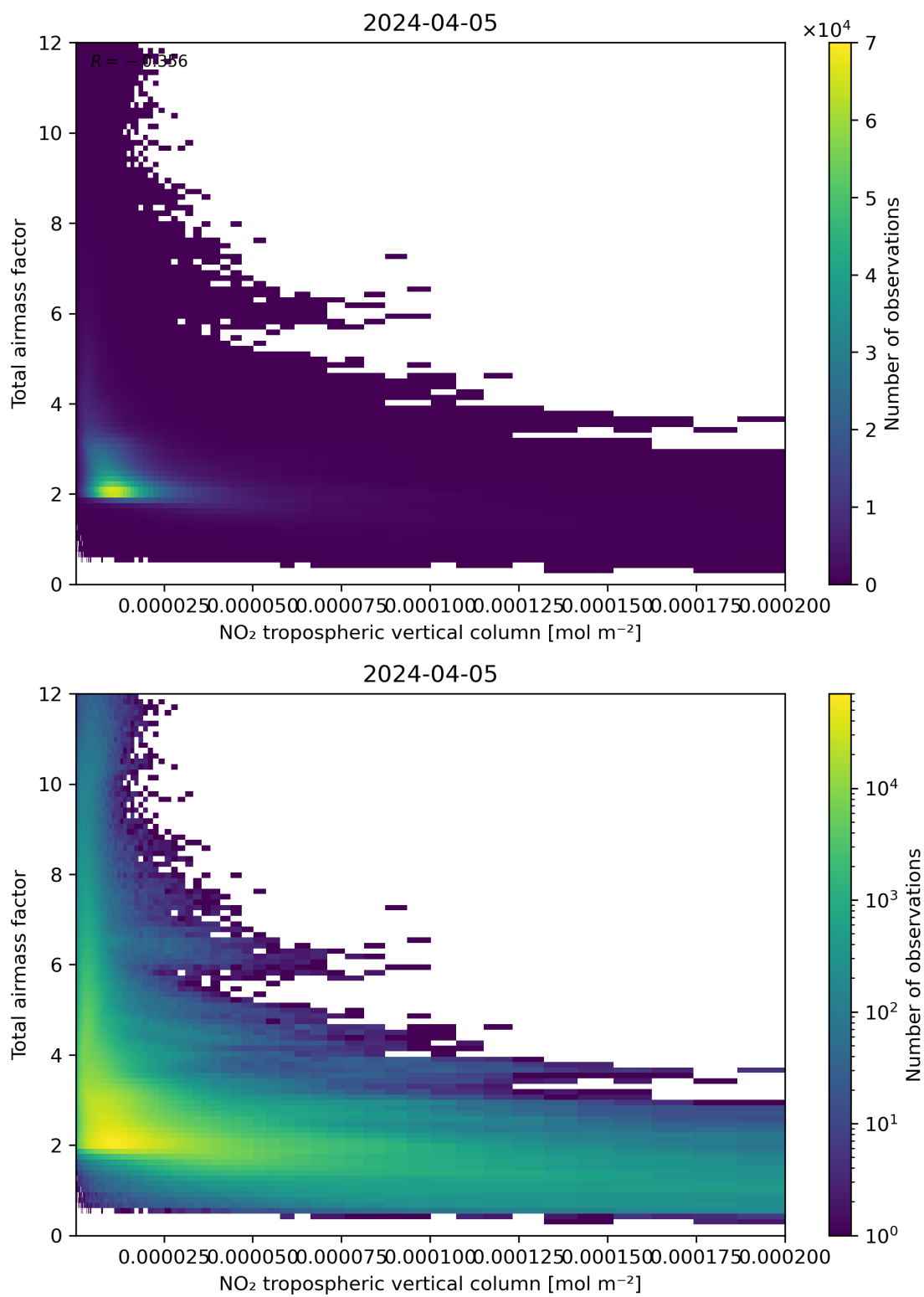
Figure 122: Scatter density plot of “NO 2 tropospheric vertical column” against “Total air mass factor” for 2024-04-05 to 2024-04-06.
