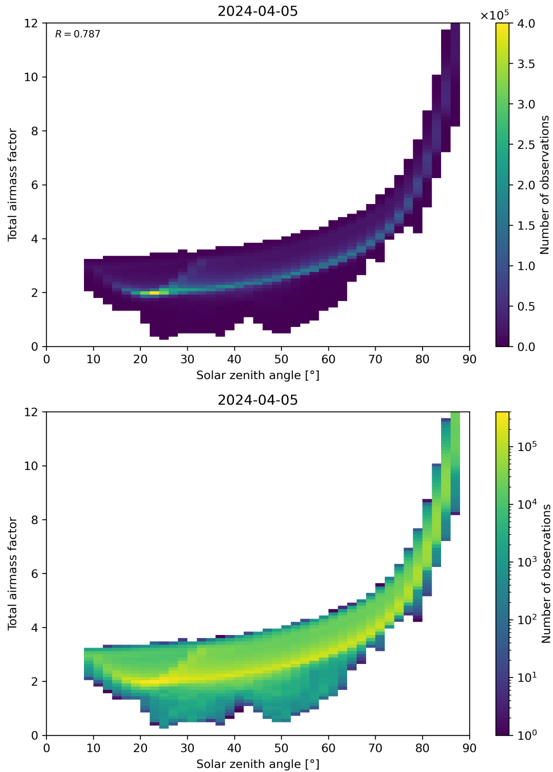
Figure 146: Scatter density plot of “Solar zenith angle” against “Total air mass factor” for 2024-04-05 to 2024-04-06.
