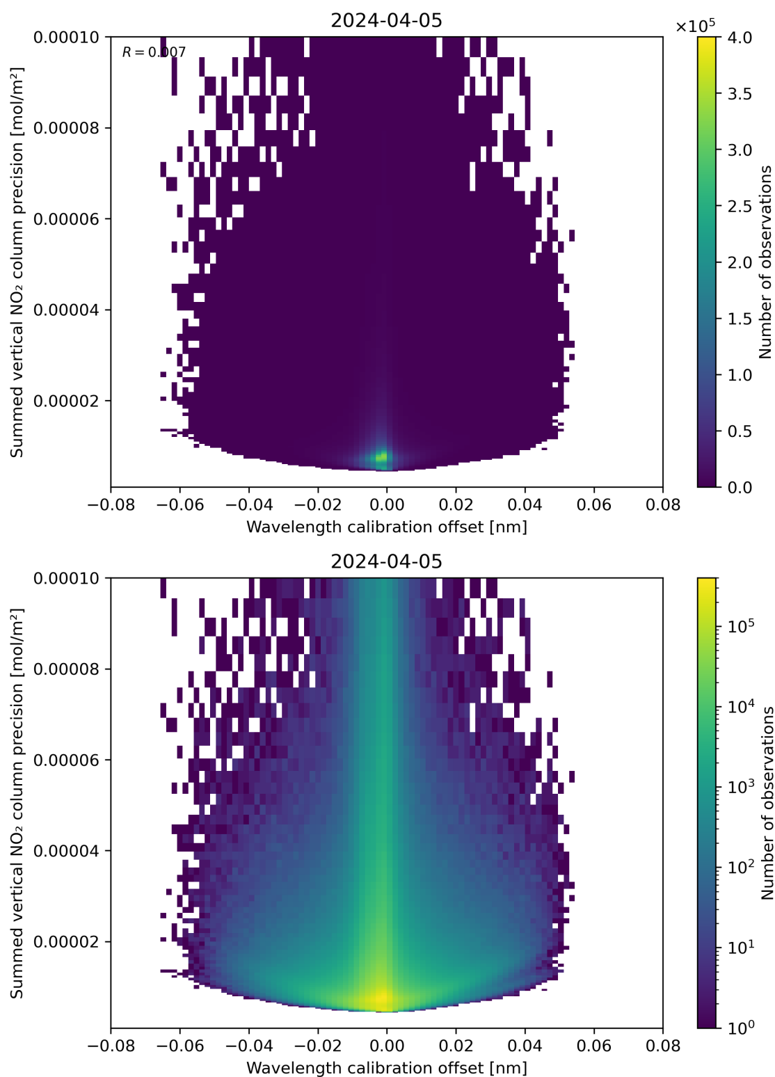
Figure 178: Scatter density plot of “Wavelength calibration offset” against “Summed vertical NO 2 column precision” for 2024-04-05 to 2024-04-06.
