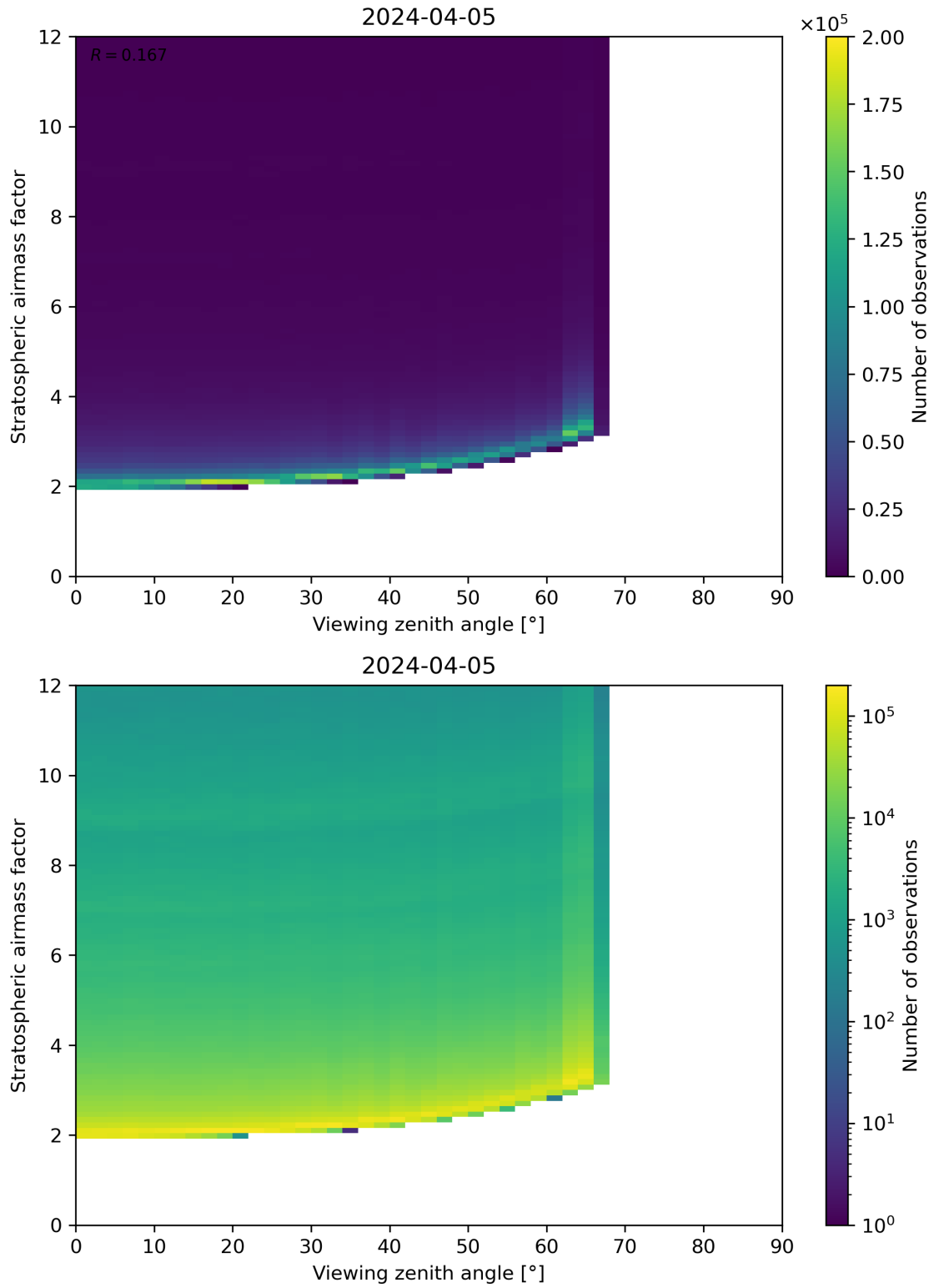
Figure 159: Scatter density plot of “Viewing zenith angle” against “Stratospheric airmass factor” for 2024-04-05 to 2024-04-06.
