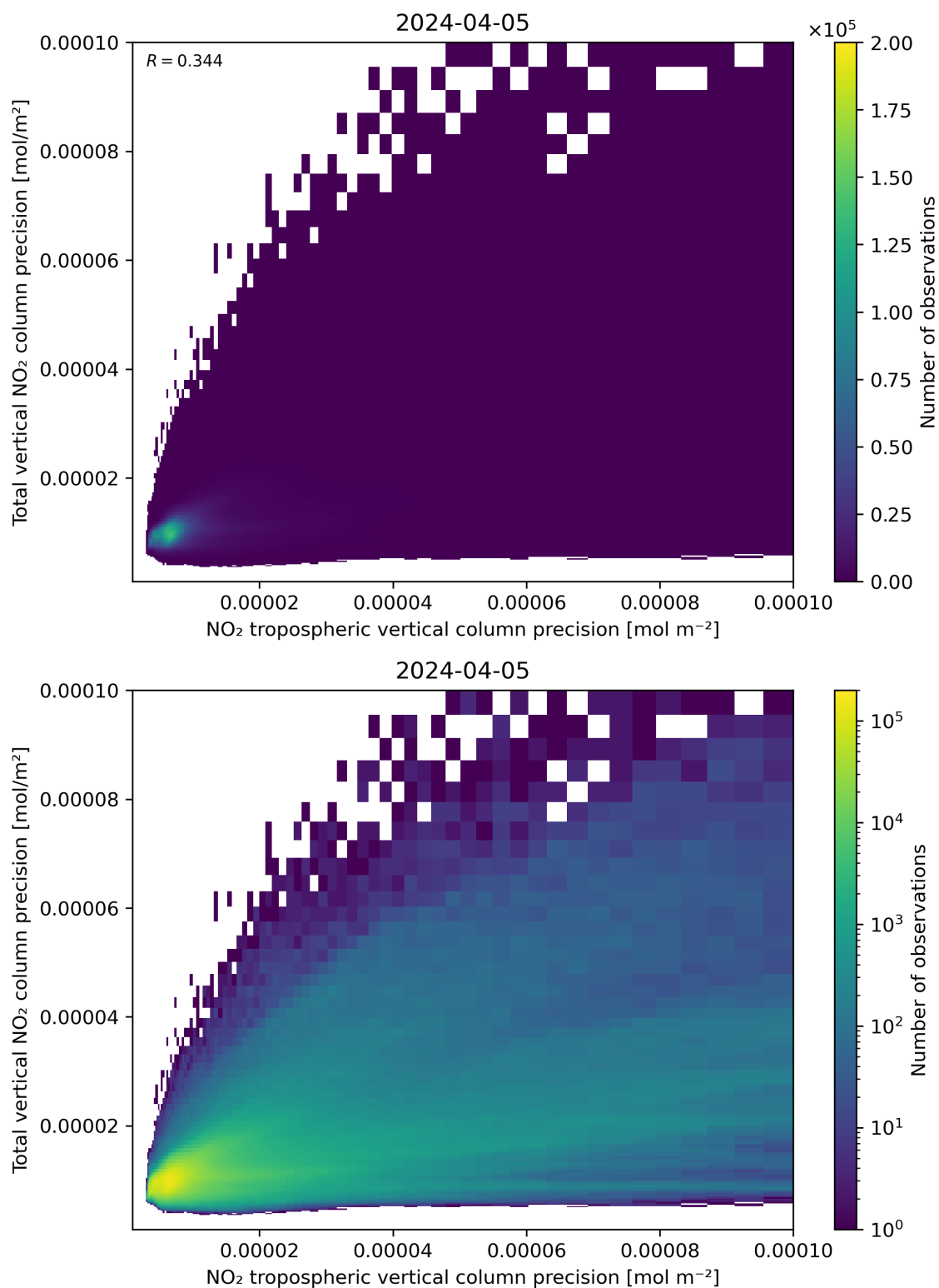
Figure 139: Scatter density plot of “NO 2 tropospheric vertical column precision” against “Total vertical NO 2 column precision” for 2024-04-05 to 2024-04-06.
