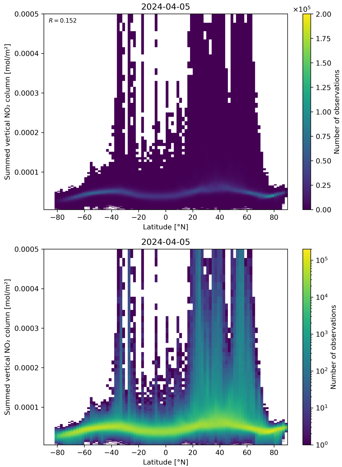
Figure 88: Scatter density plot of “Latitude” against “Summed vertical NO 2 column” for 2024-04-05 to 2024-04-06.
