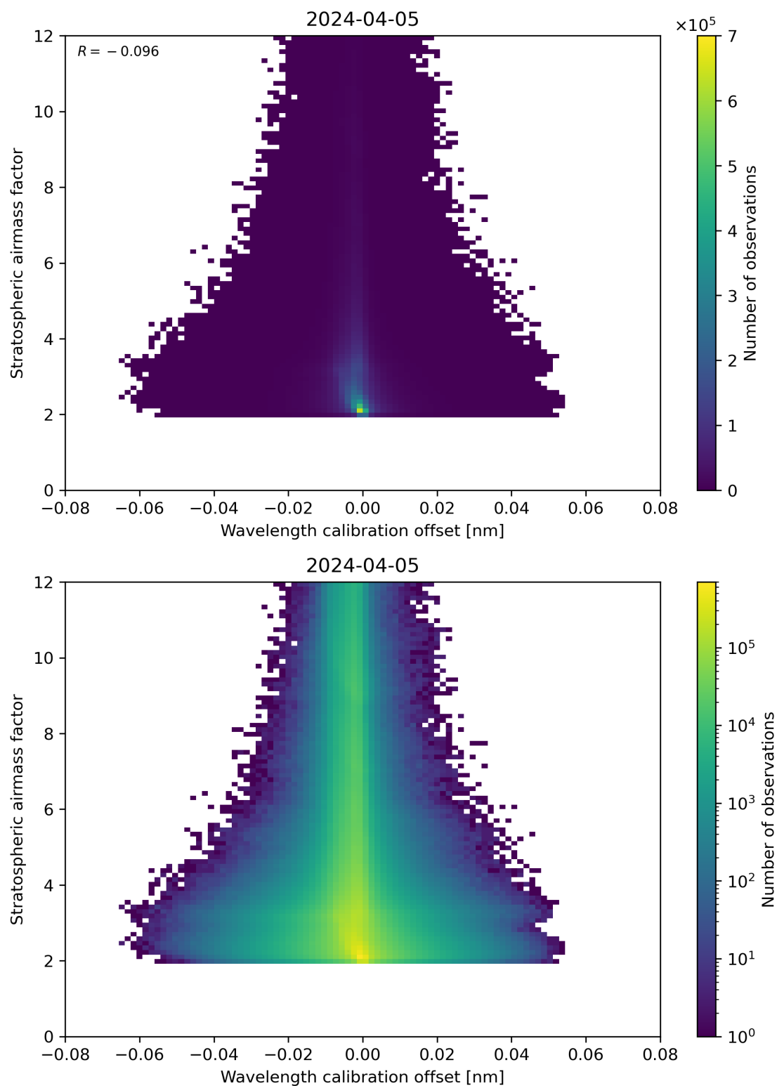
Figure 174: Scatter density plot of “Wavelength calibration offset” against “Stratospheric air mass factor” for 2024-04-05 to 2024-04-06.
