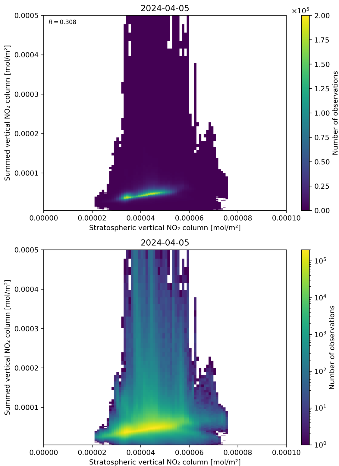
Figure 98: Scatter density plot of “Stratospheric vertical NO 2 column” against “Summed vertical NO 2 column” for 2024-04-05 to 2024-04-06.
