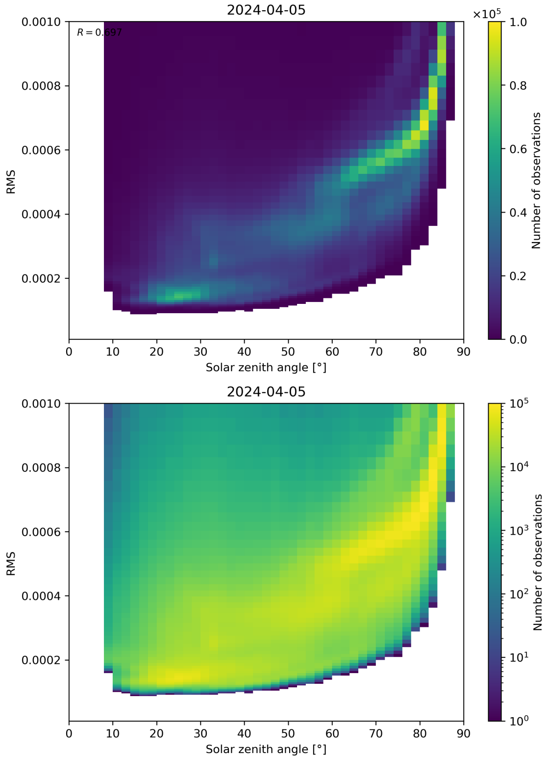
Figure 157: Scatter density plot of “Solar zenith angle” against “RMS” for 2024-04-05 to 2024-04-06.
