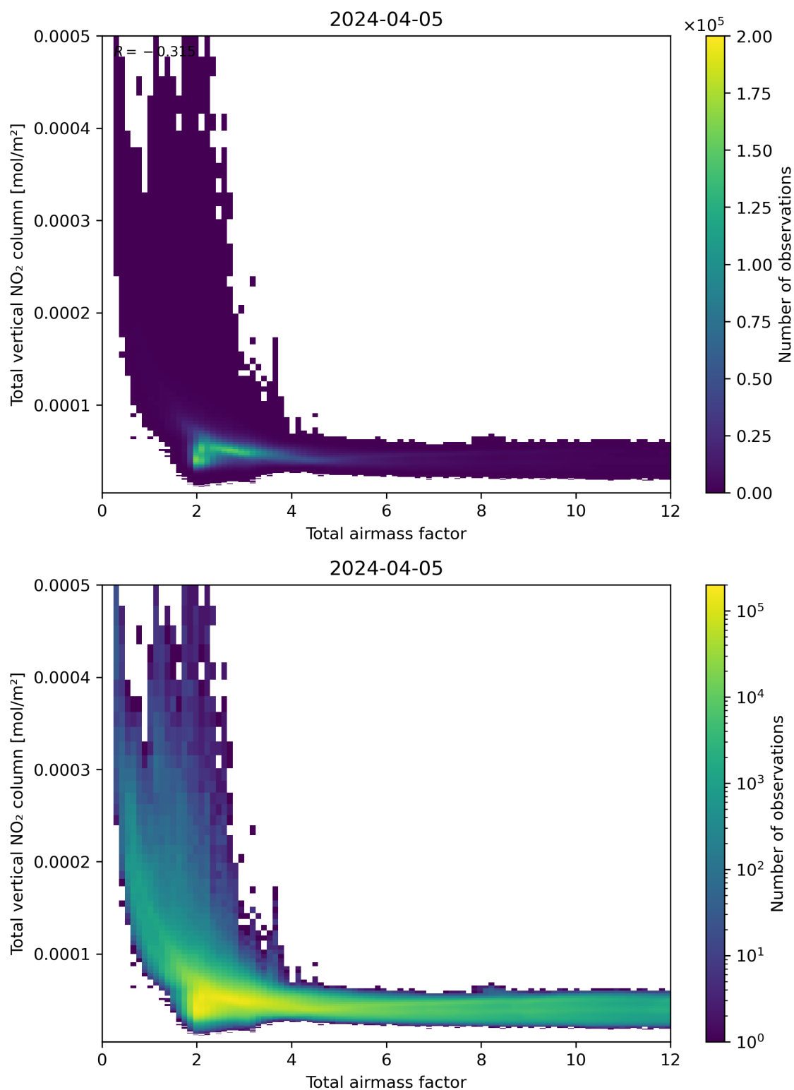
Figure 67: Scatter density plot of “Total airmass factor” against “Total vertical NO 2 column” for 2024-04-05 to 2024-04-06.
