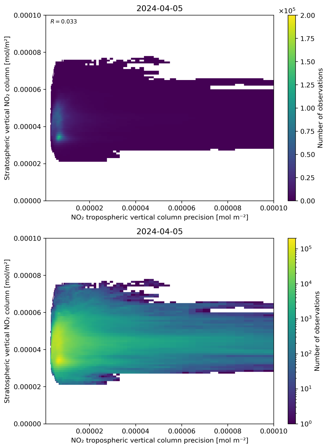
Figure 135: Scatter density plot of “NO 2 tropospheric vertical column precision” against “Stratospheric vertical NO 2 column” for 2024-04-05 to 2024-04-06.
