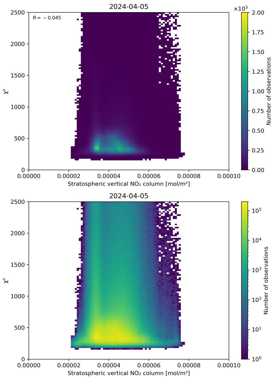
Figure 97: Scatter density plot of “Stratospheric vertical NO 2 column” against “ \chi^2 ” for 2024-04-05 to 2024-04-06.
