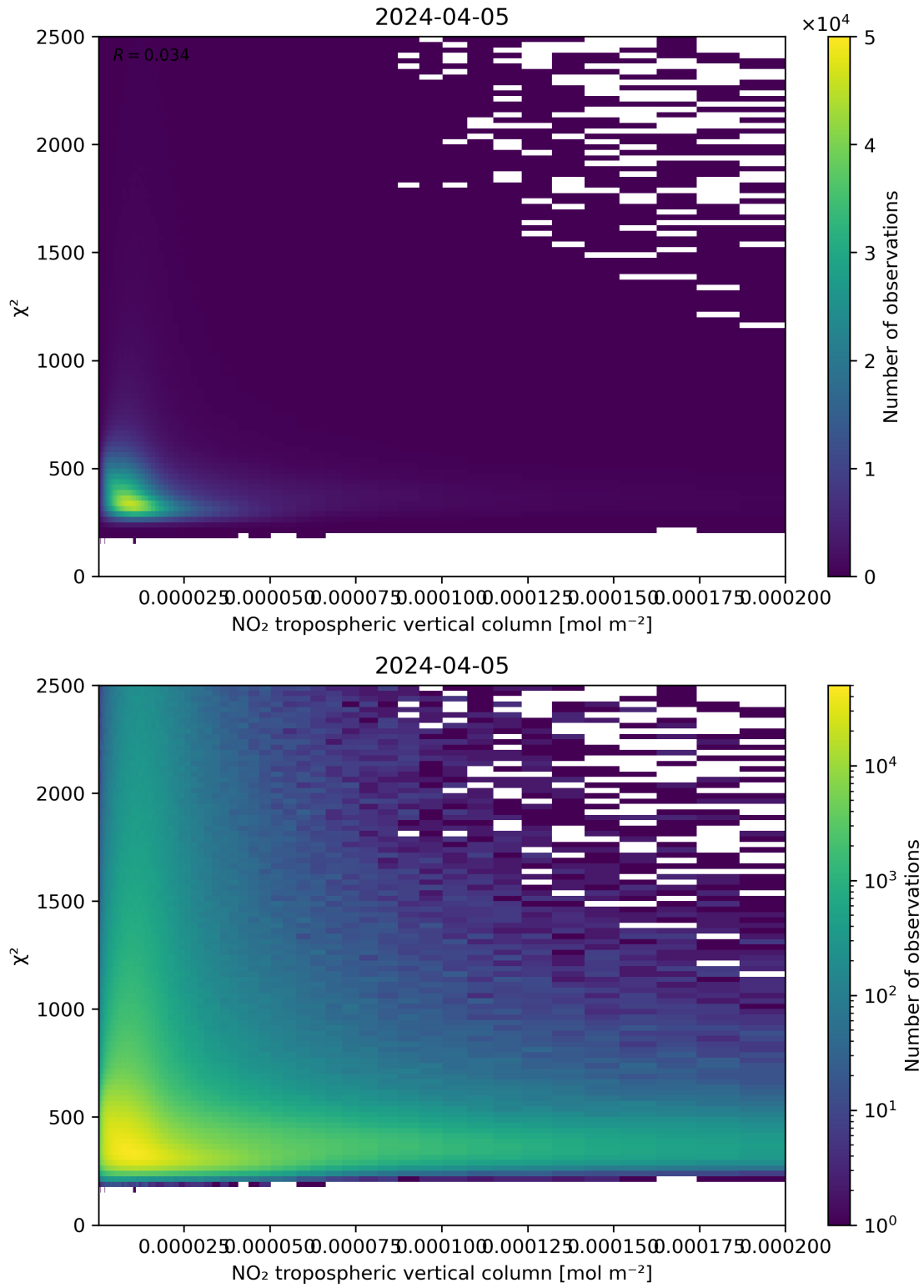
Figure 124: Scatter density plot of “NO 2 tropospheric vertical column” against “ \chi^2 ” for 2024-04-05 to 2024-04-06.
