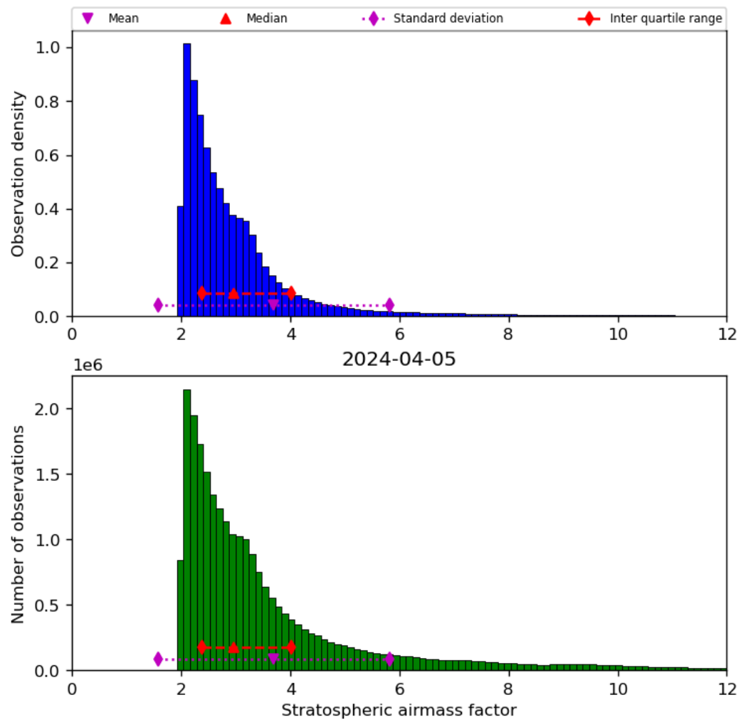
Figure 44: Histogram of “Stratospheric airmass factor” for 2024-04-05 to 2024-04-06
