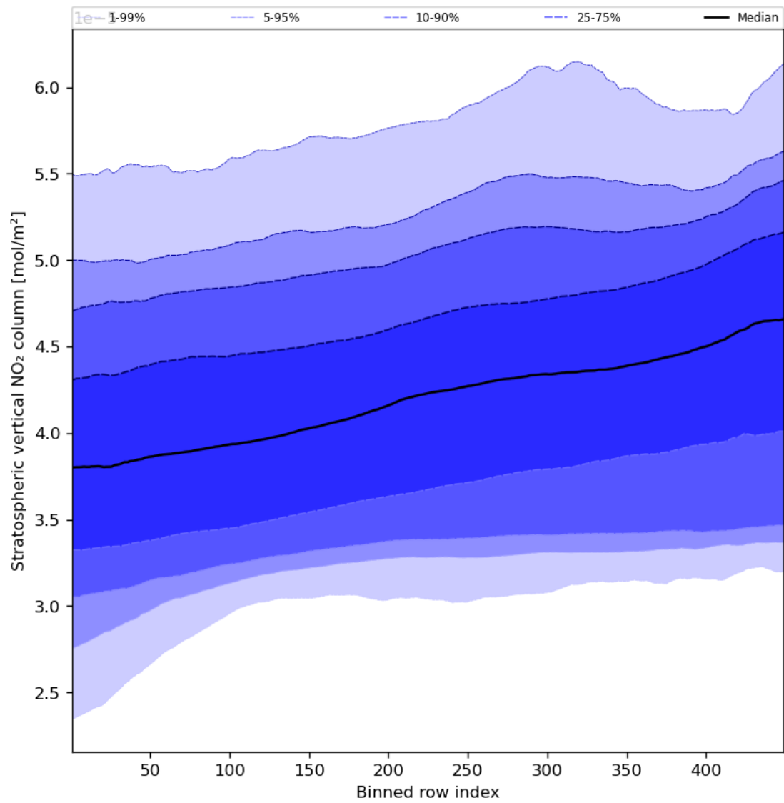
Figure 53: Along track statistics of “Stratospheric vertical NO 2 column” for 2024-04-05 to 2024-04-06
