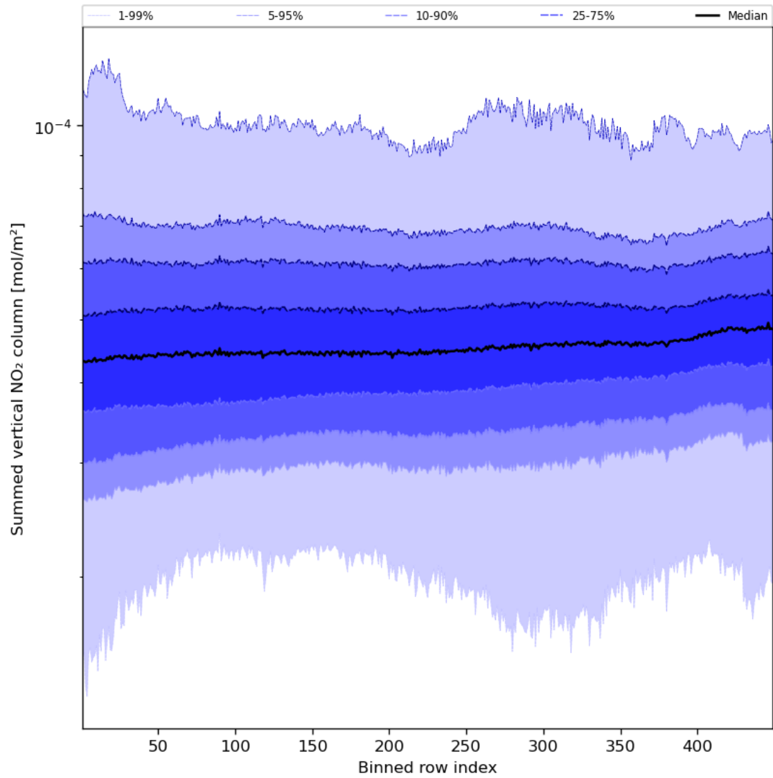
Figure 57: Along track statistics of “Summed vertical NO 2 column” for 2024-04-05 to 2024-04-06
