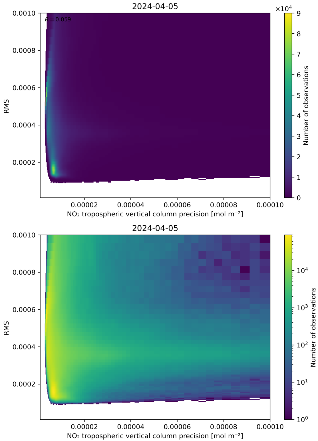
Figure 140: Scatter density plot of “NO 2 tropospheric vertical column precision” against “RMS” for 2024-04-05 to 2024-04-06.
