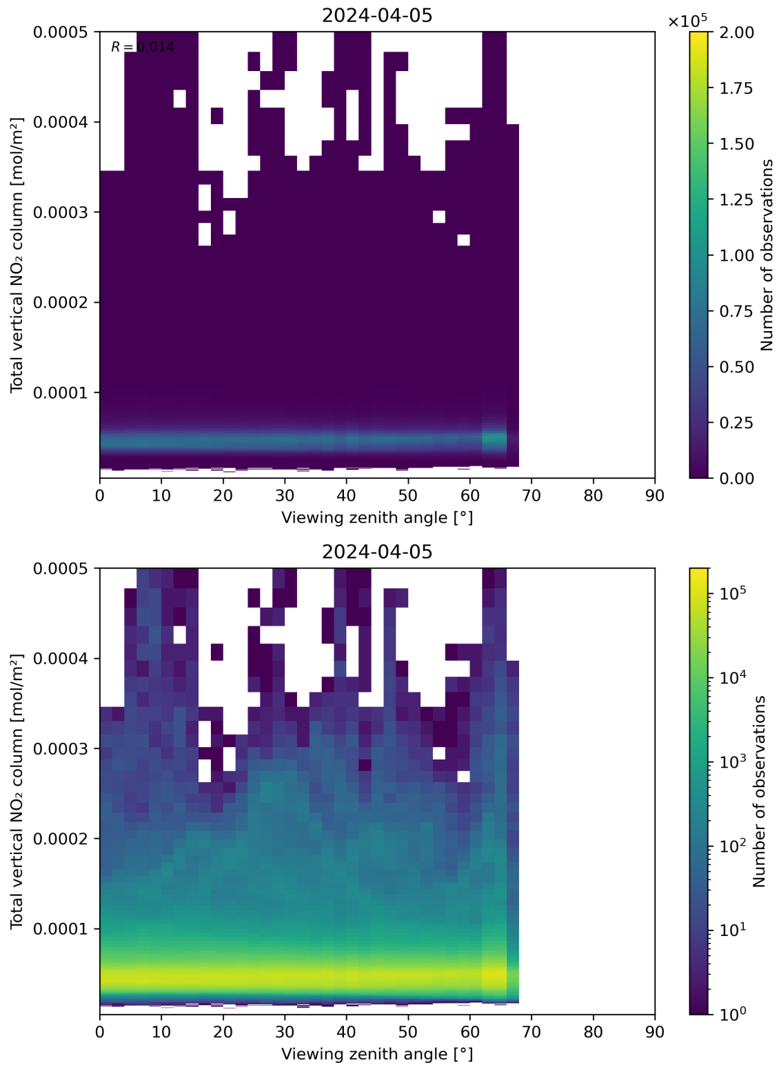
Figure 167: Scatter density plot of “Viewing zenith angle” against “Total vertical NO 2 column” for 2024-04-05 to 2024-04-06.
