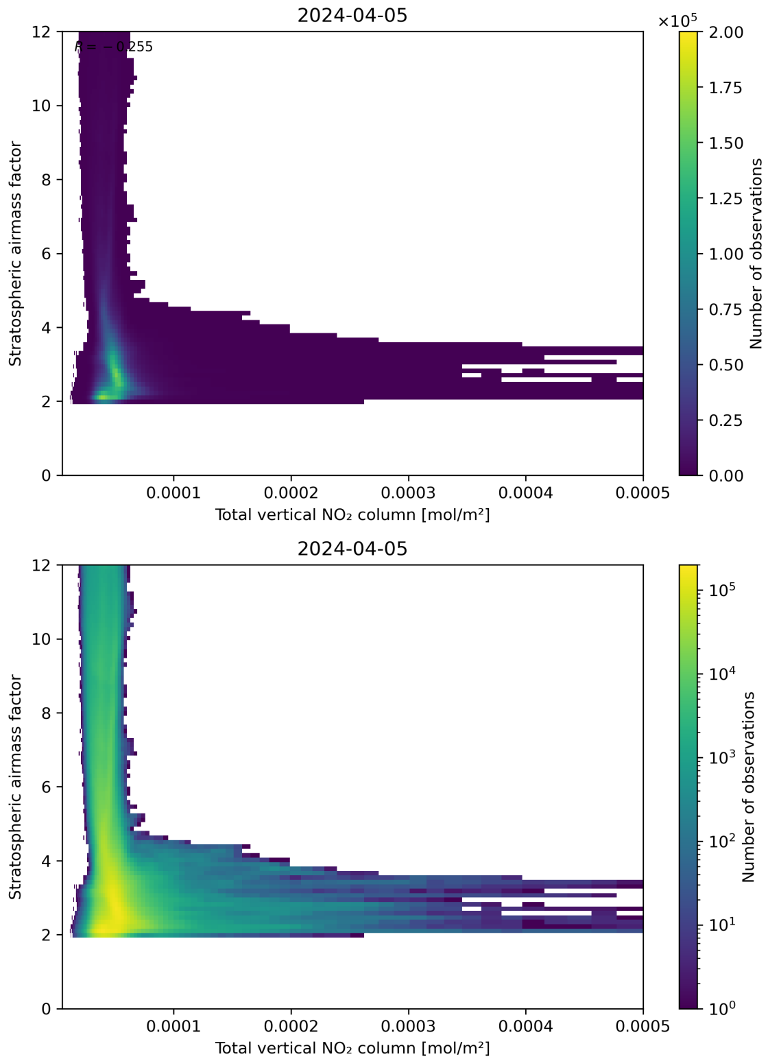
Figure 110: Scatter density plot of “Total vertical NO 2 column” against “Stratospheric airmass factor” for 2024-04-05 to 2024-04-06.
