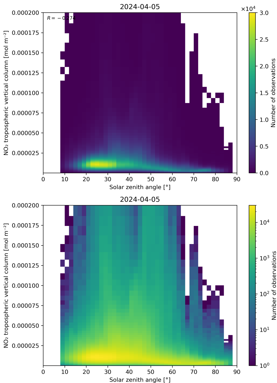
Figure 155: Scatter density plot of “Solar zenith angle” against “NO 2 tropospheric vertical column” for 2024-04-05 to 2024-04-06.
