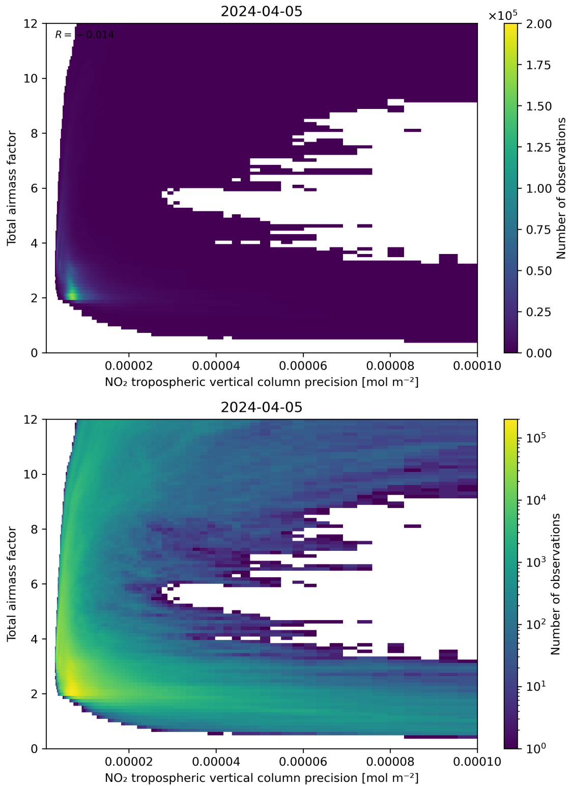
Figure 132: Scatter density plot of “NO 2 tropospheric vertical column precision” against “Total air mass factor” for 2024-04-05 to 2024-04-06.
