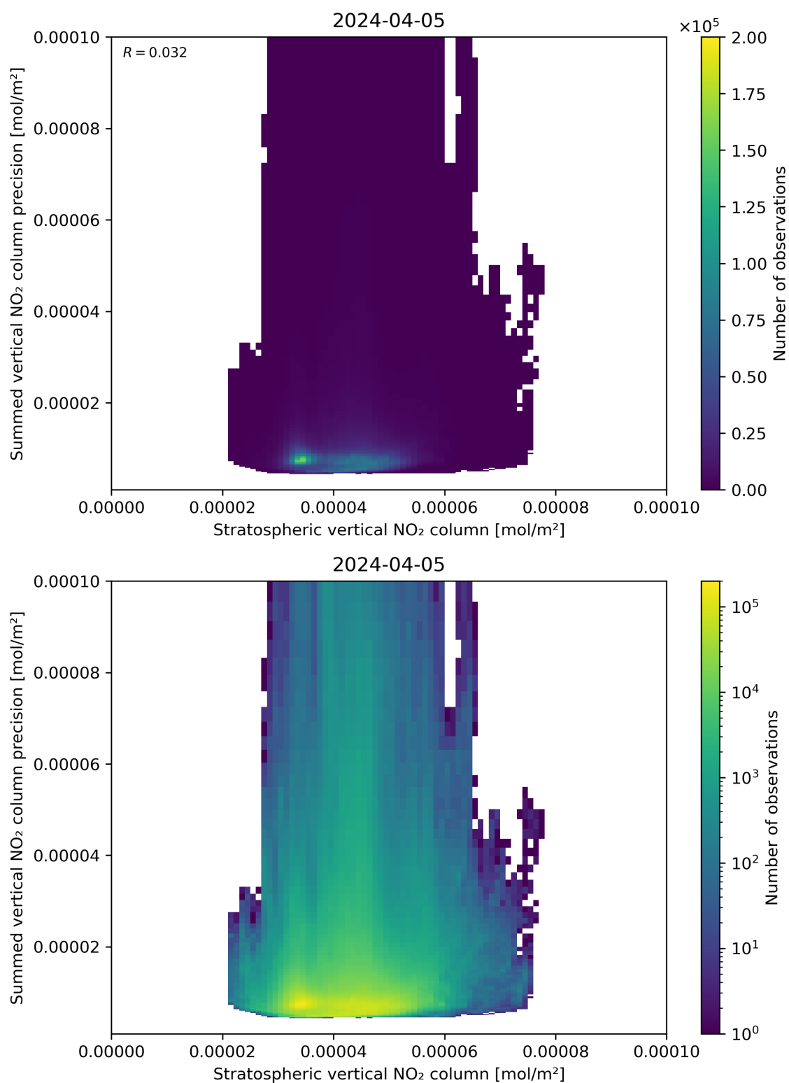
Figure 99: Scatter density plot of “Stratospheric vertical NO 2 column” against “Summed vertical NO 2 column precision” for 2024-04-05 to 2024-04-06.
