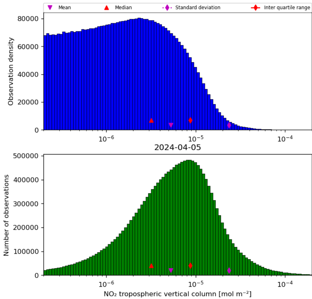
Figure 29: Histogram of “ \text{NO}_2 tropospheric vertical column” for 2024-04-05 to 2024-04-06
