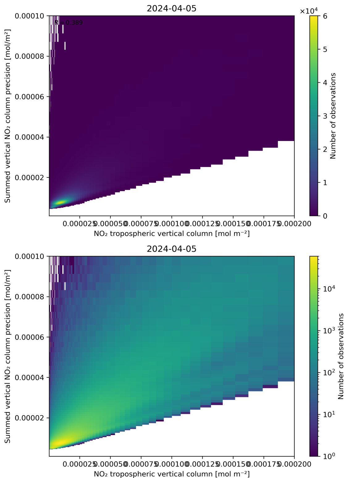
Figure 127: Scatter density plot of “NO 2 tropospheric vertical column” against “Summed vertical NO 2 column precision” for 2024-04-05 to 2024-04-06.
