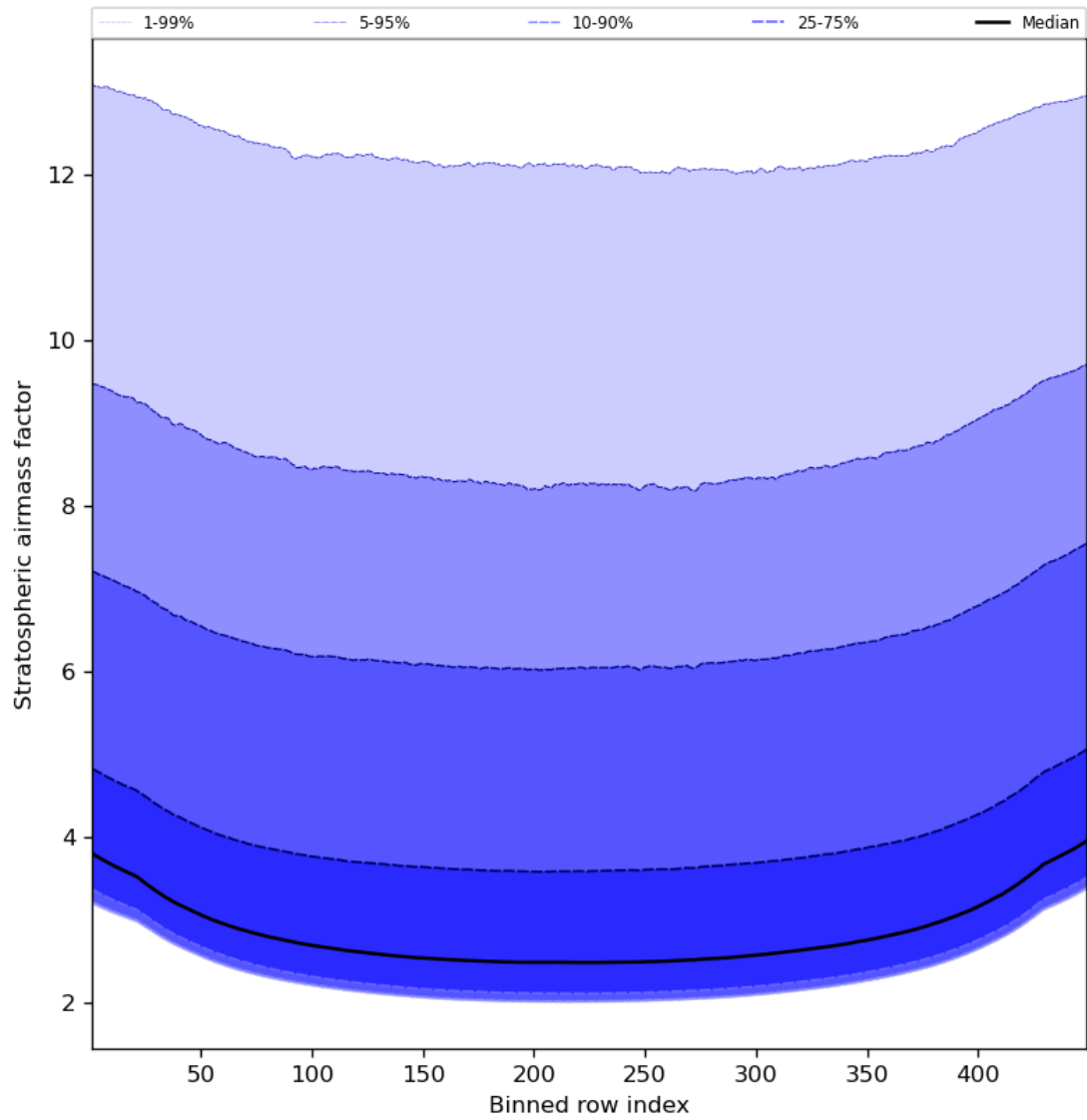
Figure 61: Along track statistics of “Stratospheric airmass factor” for 2024-04-05 to 2024-04-06
