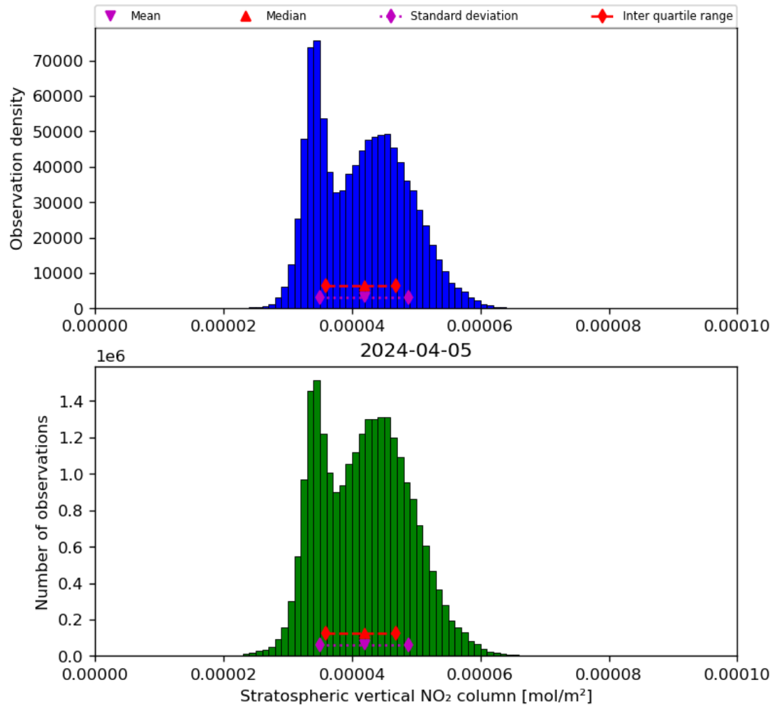
Figure 36: Histogram of “Stratospheric vertical NO 2 column” for 2024-04-05 to 2024-04-06
