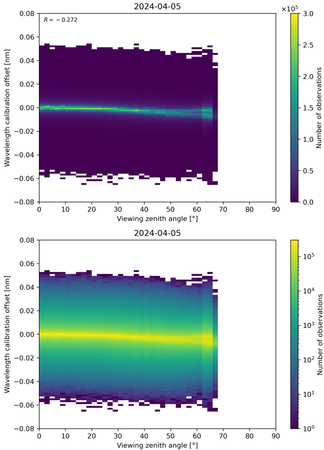
Figure 173: Scatter density plot of “Viewing zenith angle” against “Wavelength calibration offset” for 2024-04-05 to 2024-04-06.
