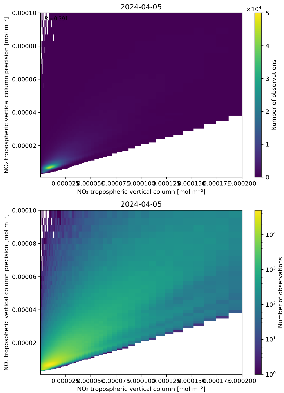
Figure 130: Scatter density plot of “NO 2 tropospheric vertical column” against “NO 2 tropospheric vertical column precision” for 2024-04-05 to 2024-04-06.
