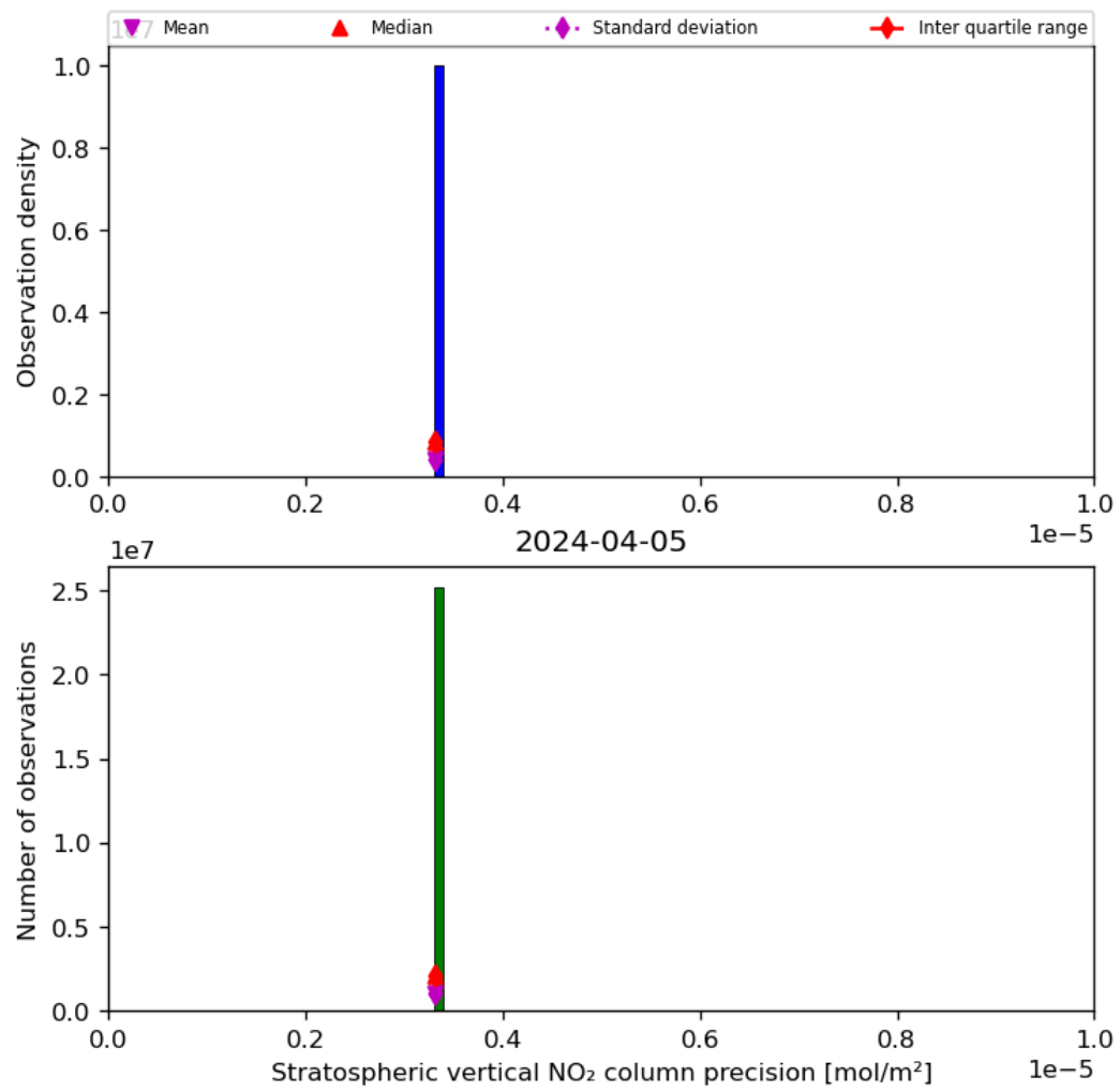
Figure 37: Histogram of “Stratospheric vertical NO 2 column precision” for 2024-04-05 to 2024-04-06
