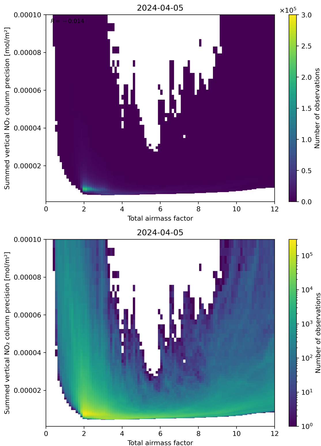
Figure 66: Scatter density plot of “Total airmass factor” against “Summed vertical NO 2 column precision” for 2024-04-05 to 2024-04-06.
