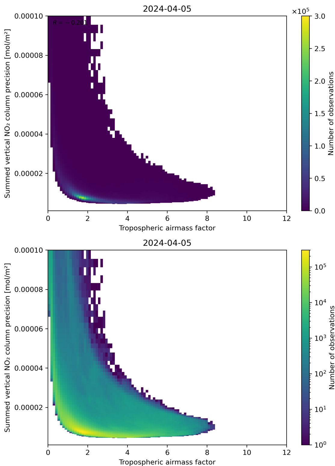
Figure 76: Scatter density plot of “Tropospheric air mass factor” against “Summed vertical NO 2 column precision” for 2024-04-05 to 2024-04-06.
