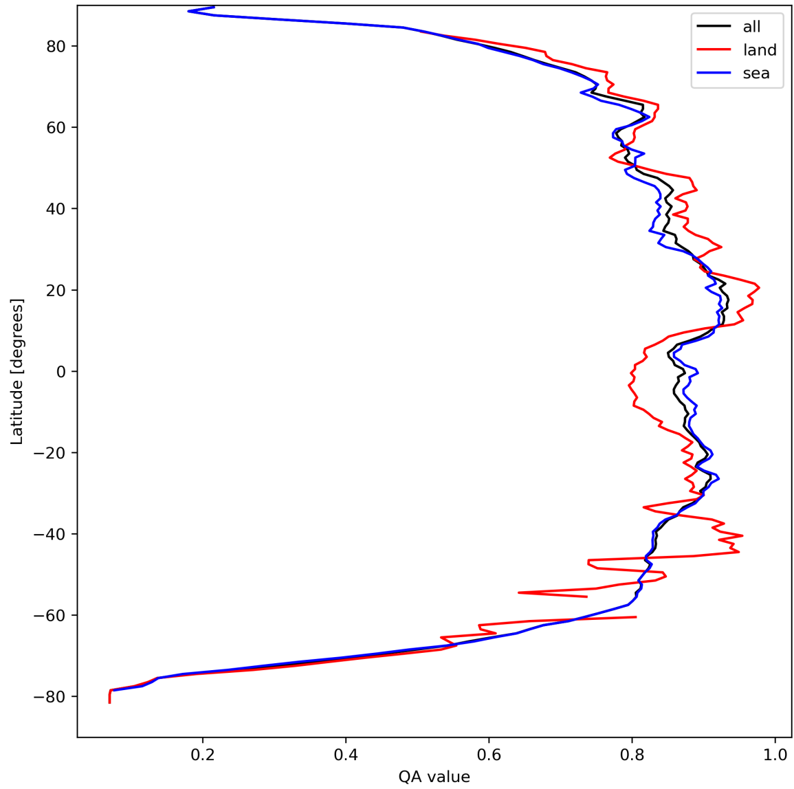
Figure 11: Zonal average of “QA value” for 2024-04-05 to 2024-04-06.
