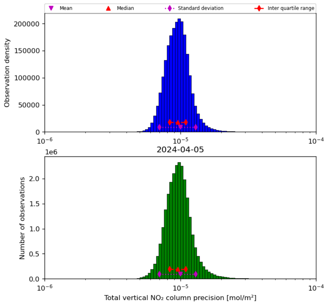
Figure 39: Histogram of “Total vertical NO 2 column precision” for 2024-04-05 to 2024-04-06
