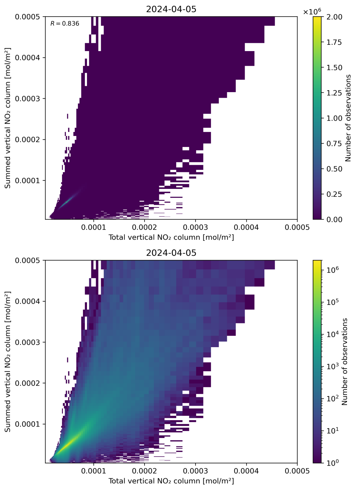
Figure 112: Scatter density plot of “Total vertical NO 2 column” against “Summed vertical NO 2 column” for 2024-04-05 to 2024-04-06.
