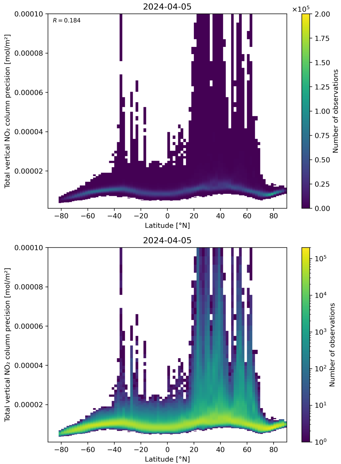
Figure 91: Scatter density plot of “Latitude” against “Total vertical NO 2 column precision” for 2024-04-05 to 2024-04-06.
