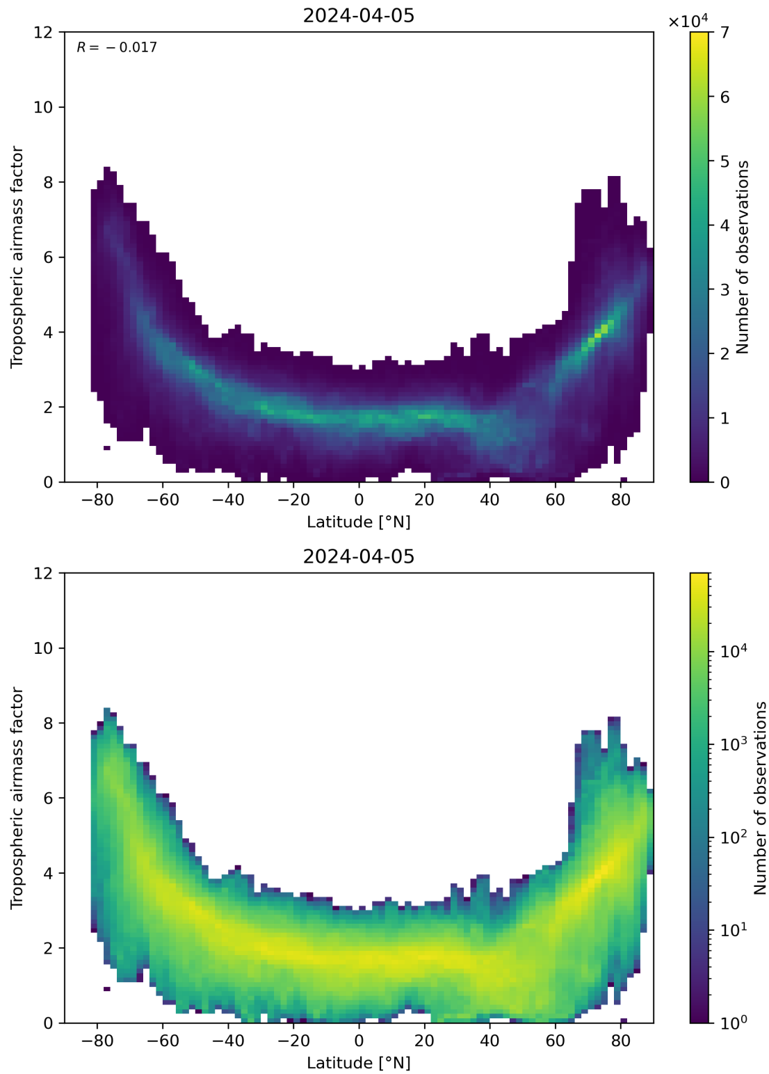
Figure 85: Scatter density plot of “Latitude” against “Tropospheric airmass factor” for 2024-04-05 to 2024-04-06.
