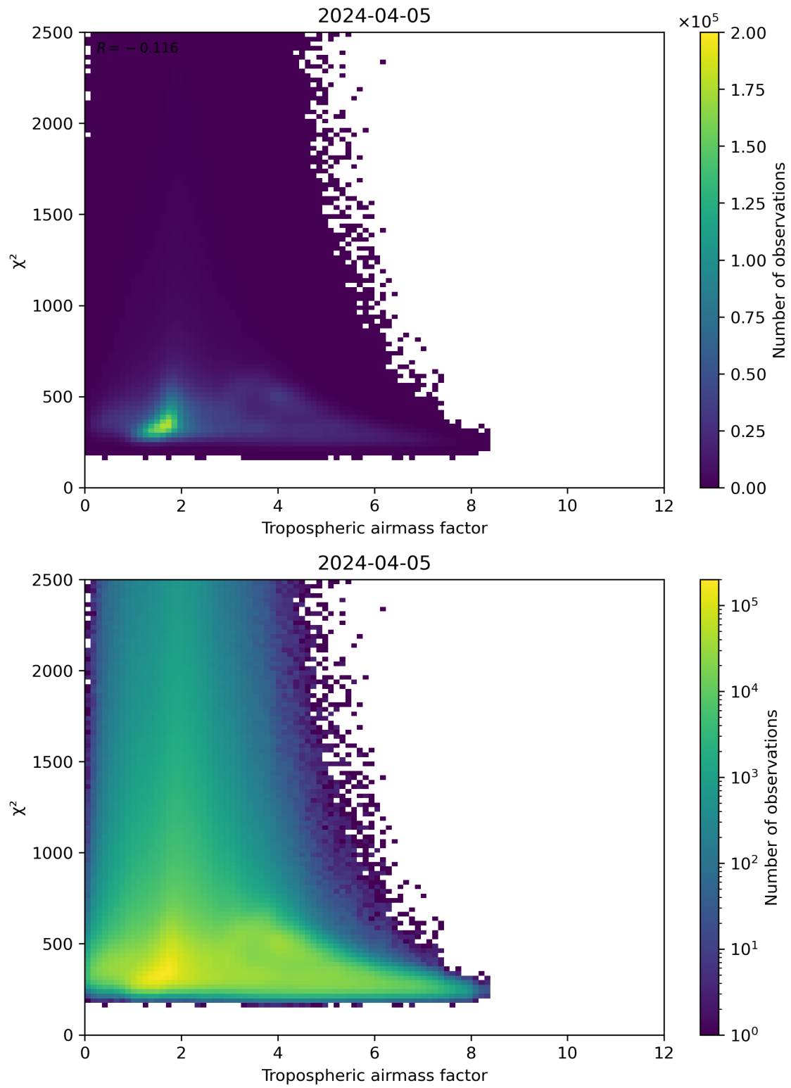
Figure 73: Scatter density plot of “Tropospheric airmass factor” against “ \chi^2 ” for 2024-04-05 to 2024-04-06.
