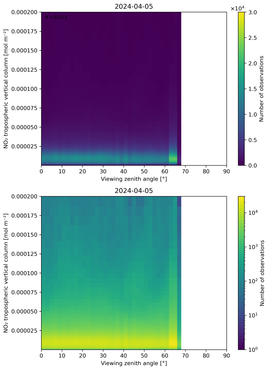
Figure 169: Scatter density plot of “Viewing zenith angle” against “NO 2 tropospheric vertical column” for 2024-04-05 to 2024-04-06.
