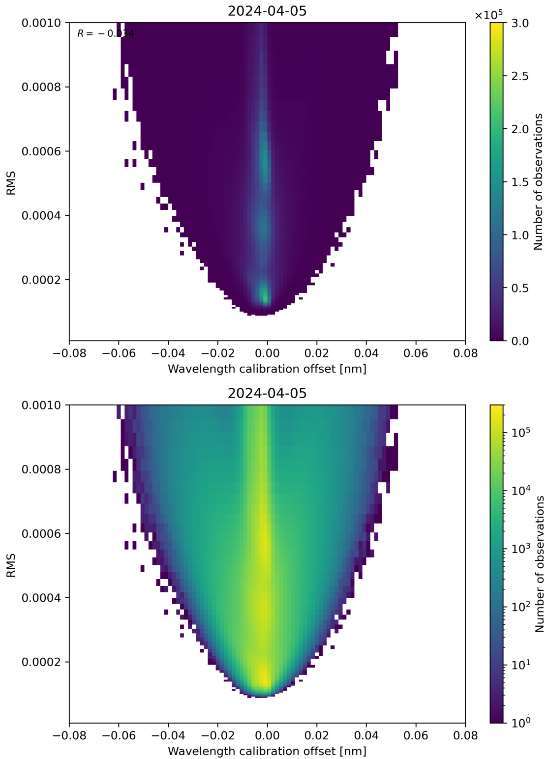
Figure 181: Scatter density plot of “Wavelength calibration offset” against “RMS” for 2024-04-05 to 2024-04-06.
