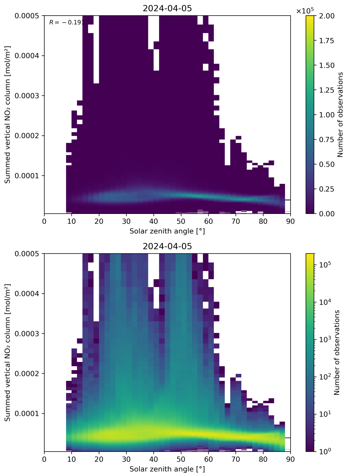
Figure 151: Scatter density plot of “Solar zenith angle” against “Summed vertical NO 2 column” for 2024-04-05 to 2024-04-06.
