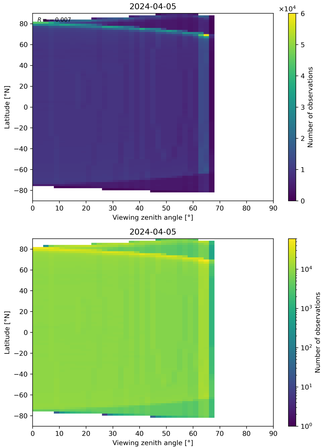
Figure 163: Scatter density plot of “Viewing zenith angle” against “Latitude” for 2024-04-05 to 2024-04-06.
