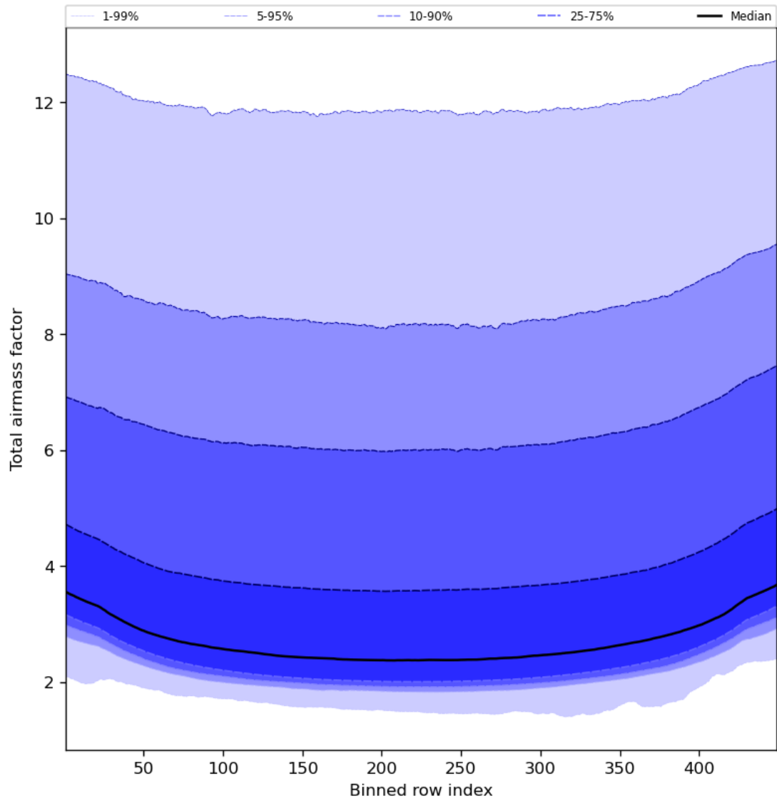
Figure 49: Along track statistics of “Total airmass factor” for 2024-04-05 to 2024-04-06
