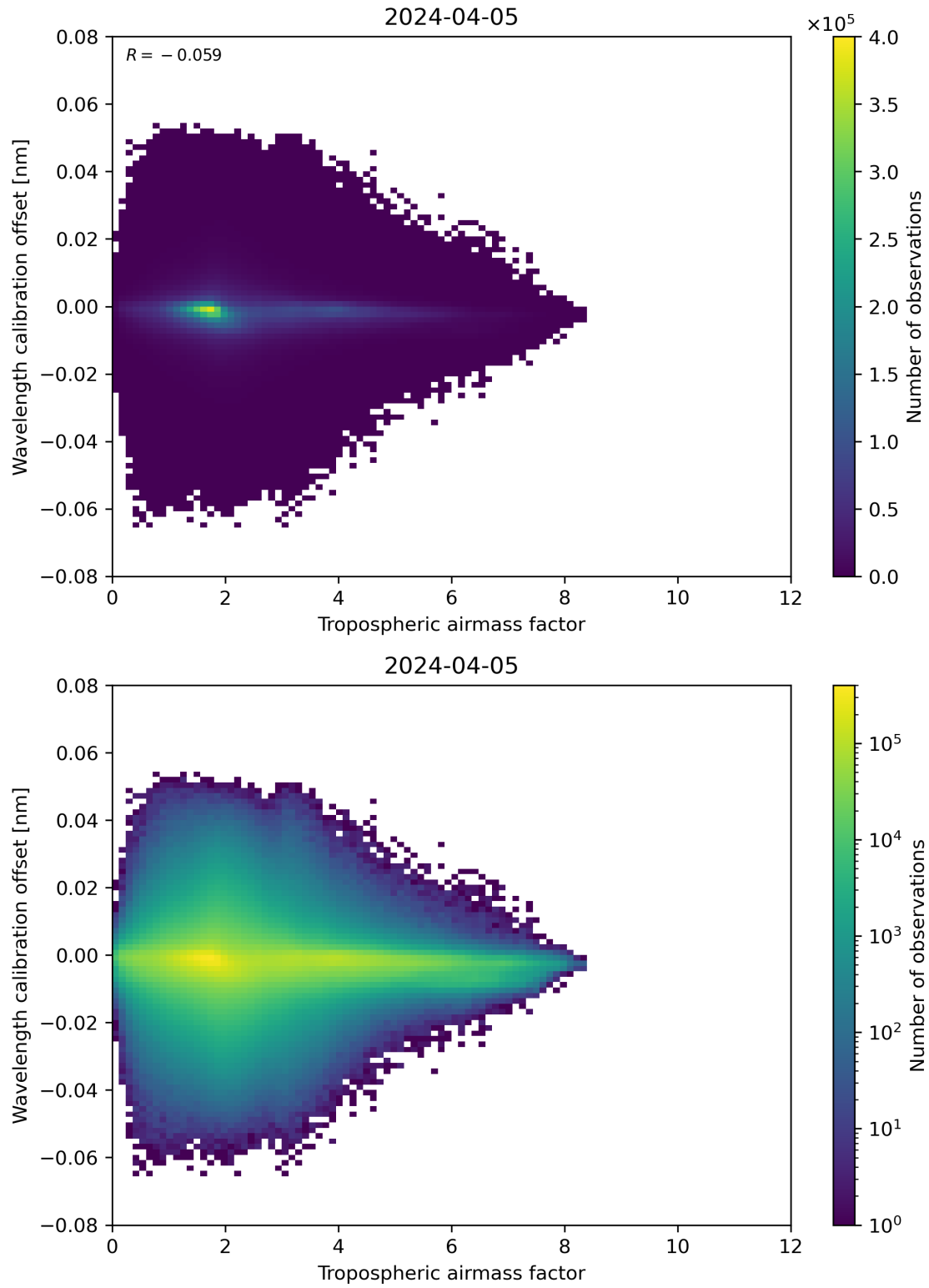
Figure 80: Scatter density plot of “Tropospheric airmass factor” against “Wavelength calibration offset” for 2024-04-05 to 2024-04-06.
