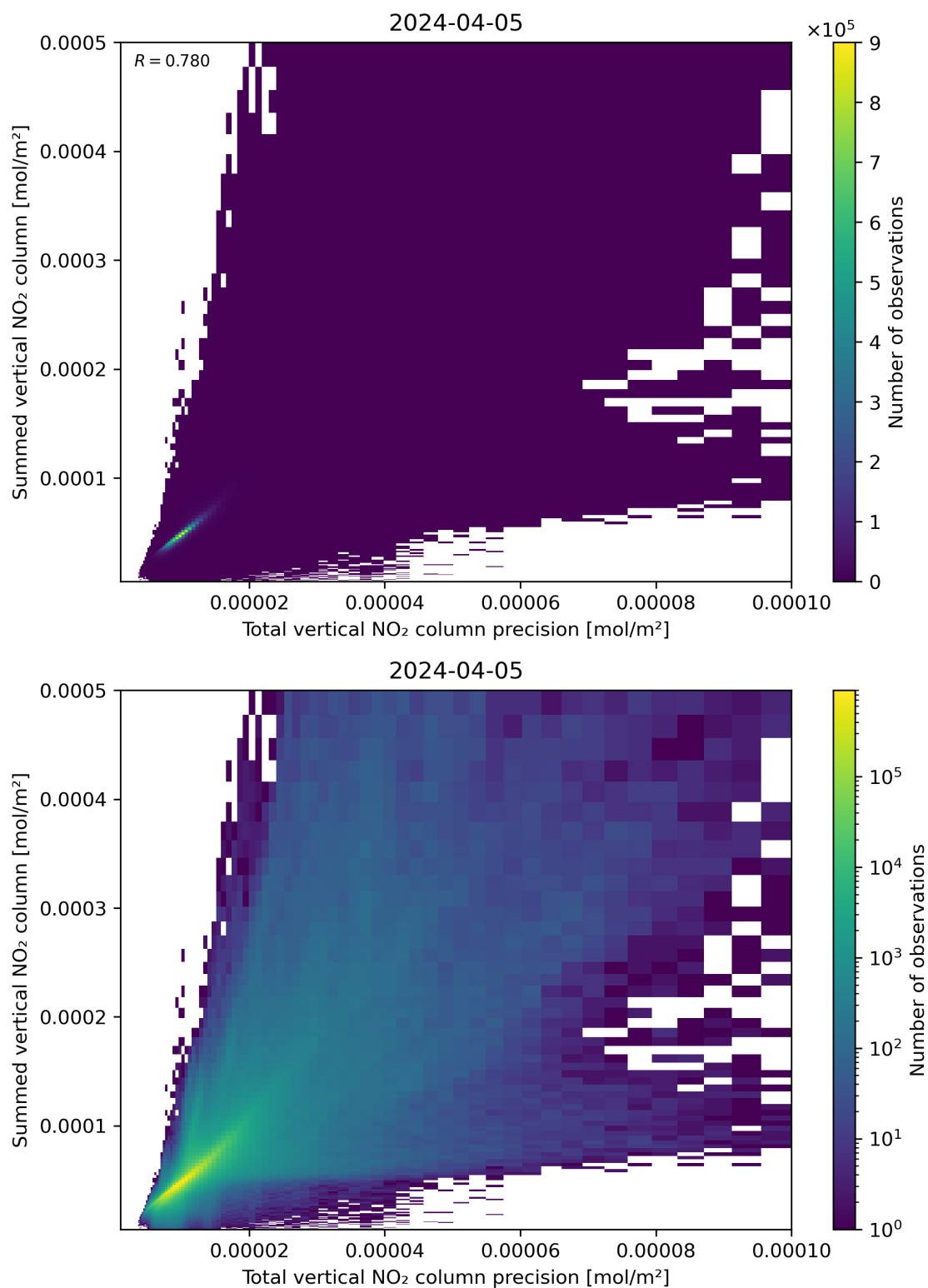
Figure 117: Scatter density plot of “Total vertical NO 2 column precision” against “Summed vertical NO 2 column” for 2024-04-05 to 2024-04-06.
