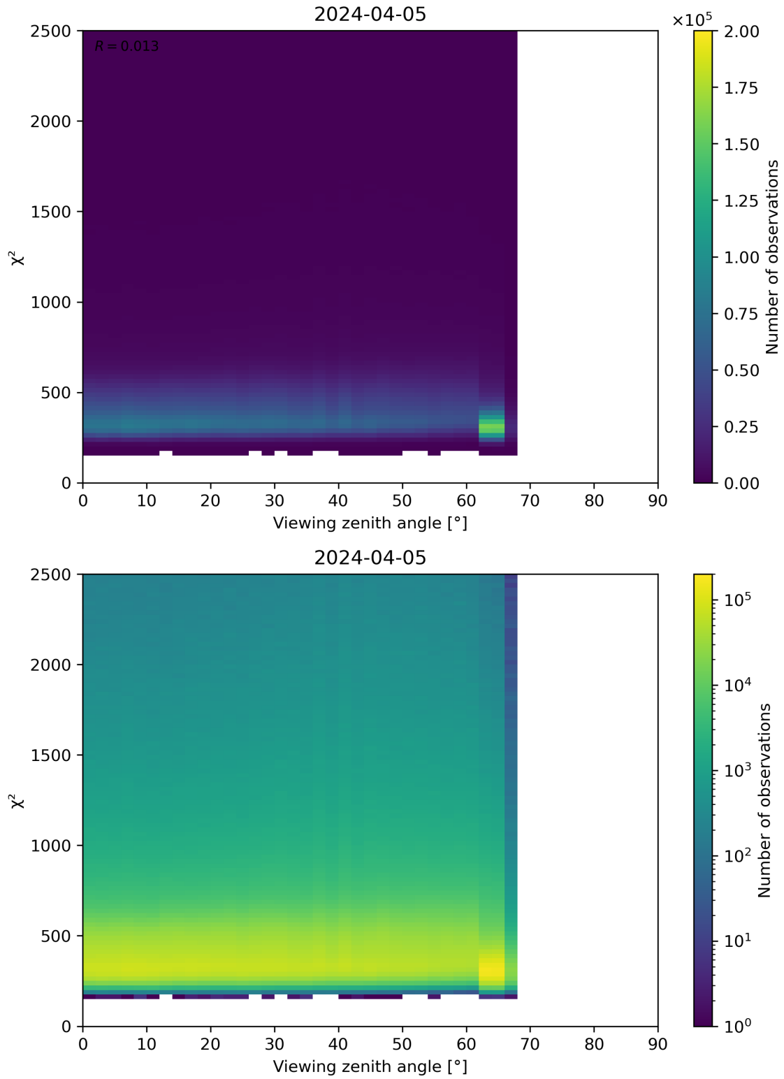
Figure 162: Scatter density plot of “Viewing zenith angle” against “ \chi^2 ” for 2024-04-05 to 2024-04-06.
