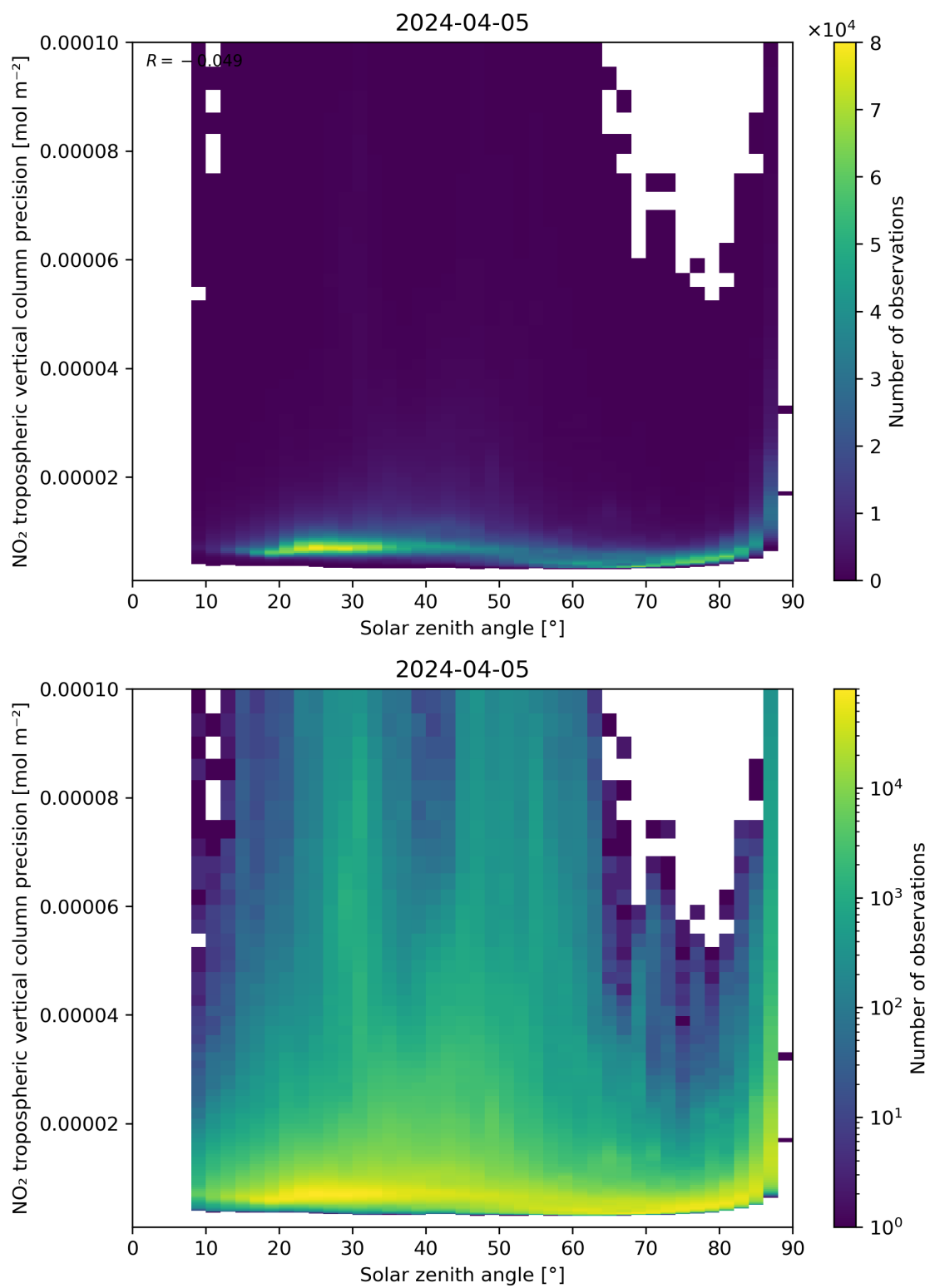
Figure 156: Scatter density plot of “Solar zenith angle” against “NO 2 tropospheric vertical column precision” for 2024-04-05 to 2024-04-06.
