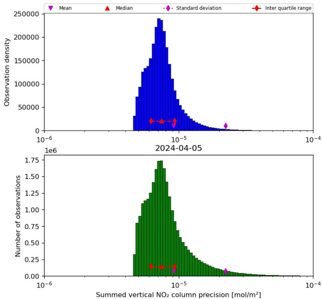
Figure 41: Histogram of “Summed vertical NO 2 column precision” for 2024-04-05 to 2024-04-06
