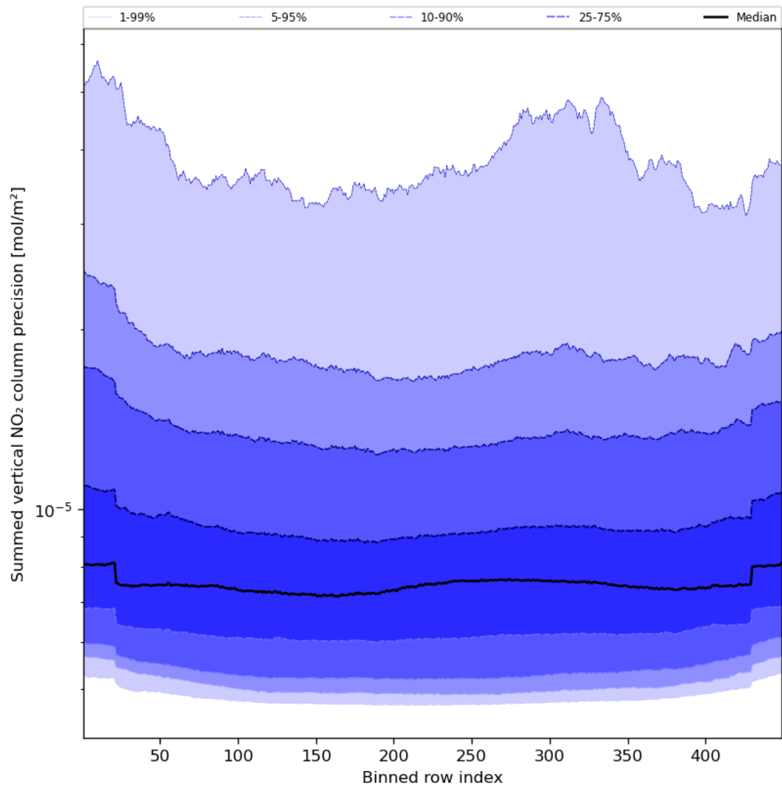
Figure 58: Along track statistics of “Summed vertical NO 2 column precision” for 2024-04-05 to 2024-04-06
