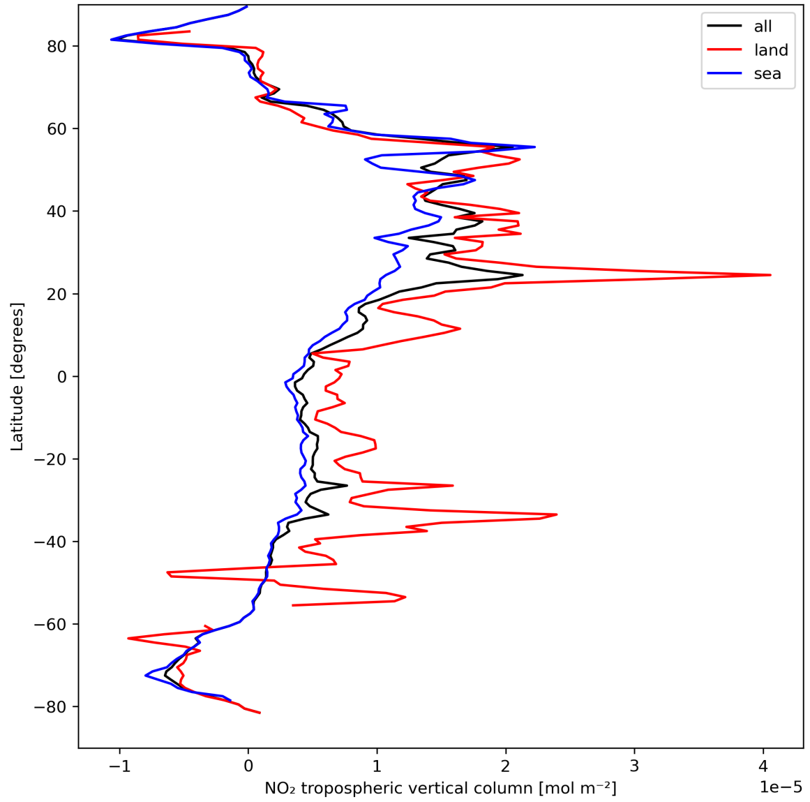
Figure 12: Zonal average of “NO 2 tropospheric vertical column” for 2024-04-05 to 2024-04-06.
