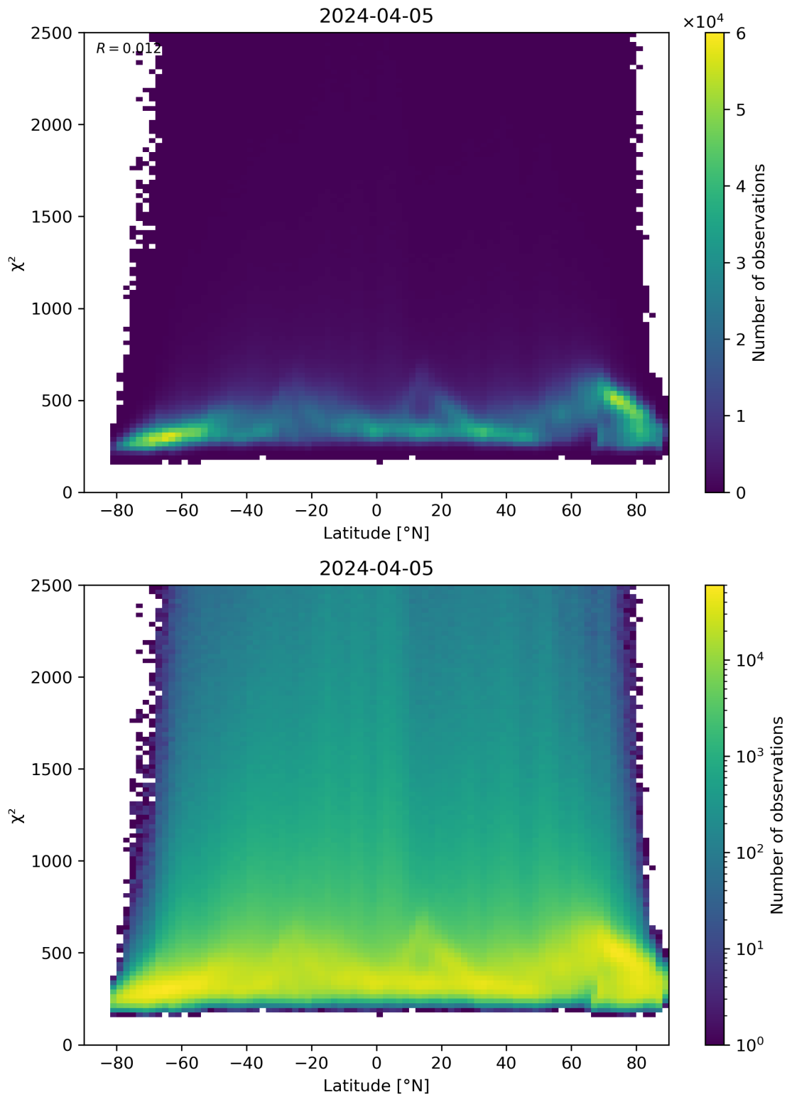
Figure 86: Scatter density plot of “Latitude” against “ \chi^2 ” for 2024-04-05 to 2024-04-06.
