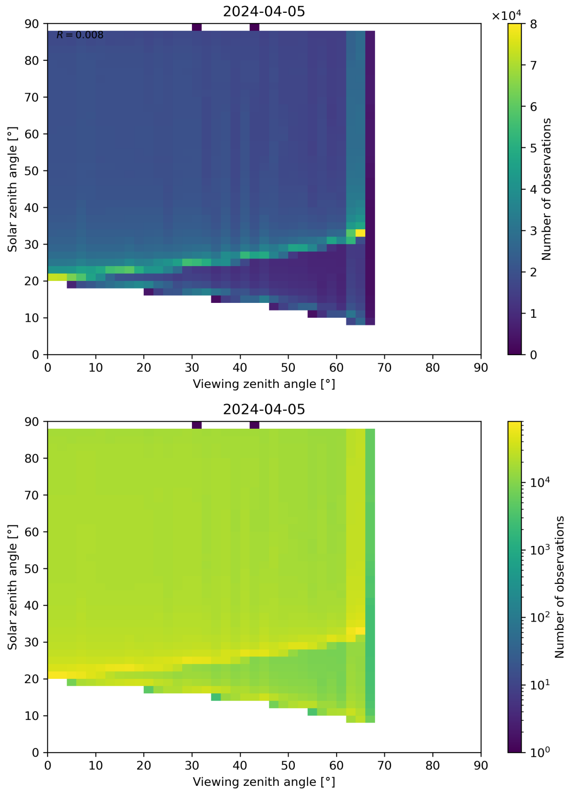
Figure 172: Scatter density plot of “Viewing zenith angle” against “Solar zenith angle” for 2024-04-05 to 2024-04-06.
