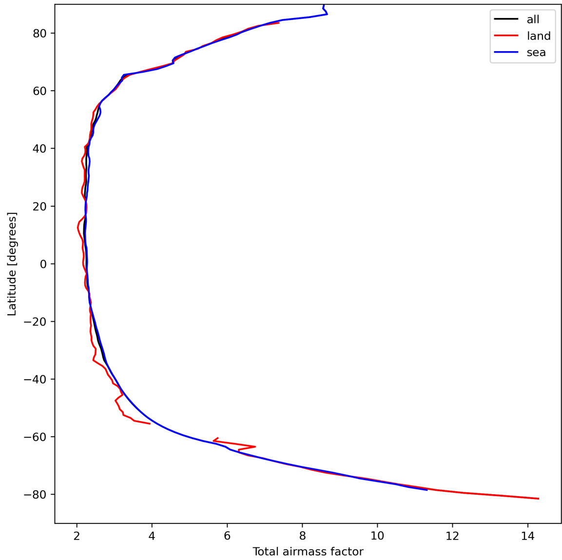
Figure 15: Zonal average of “Total airmass factor” for 2024-04-05 to 2024-04-06.
