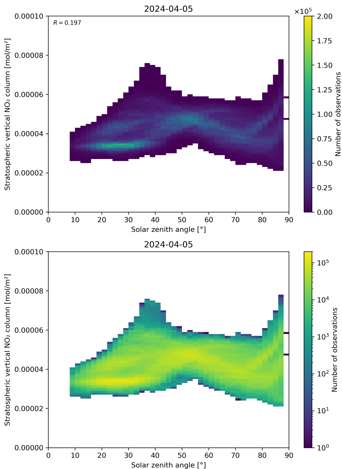
Figure 150: Scatter density plot of “Solar zenith angle” against “Stratospheric vertical NO 2 column” for 2024-04-05 to 2024-04-06.
