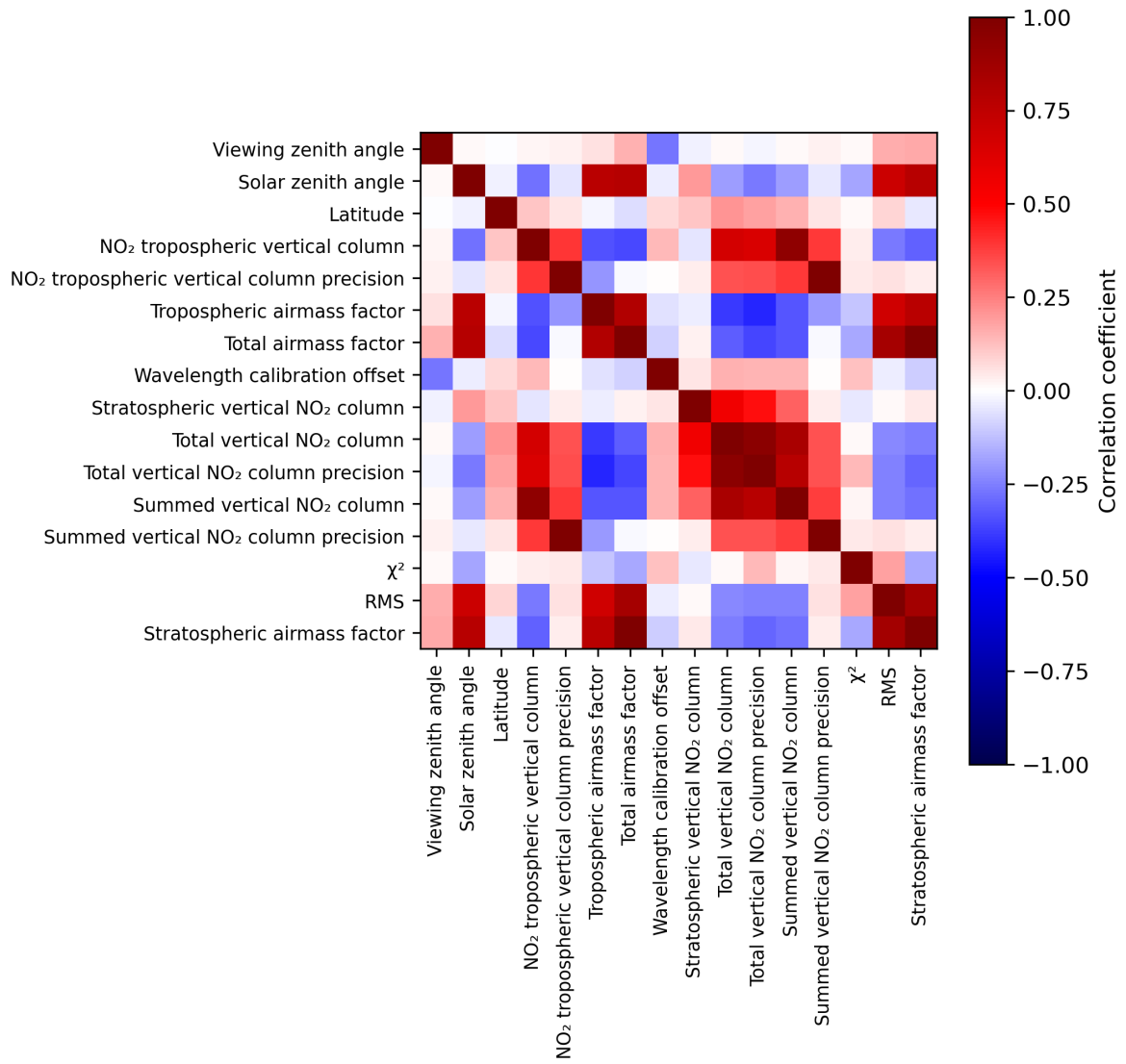
Figure 2: Map of correlation matrix for 2024-04-05 to 2024-04-06.
