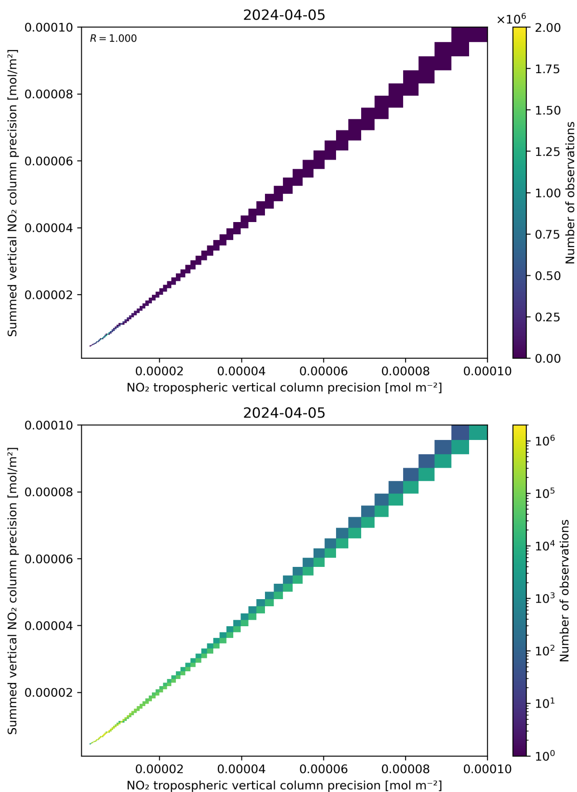
Figure 137: Scatter density plot of “NO 2 tropospheric vertical column precision” against “Summed vertical NO 2 column precision” for 2024-04-05 to 2024-04-06.
