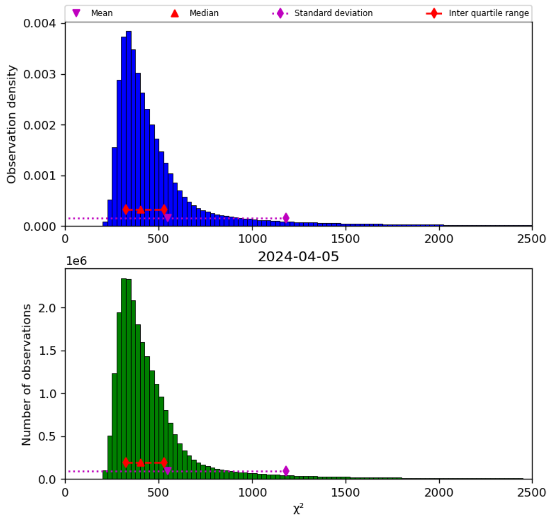
Figure 42: Histogram of “ \chi^2 ” for 2024-04-05 to 2024-04-06
