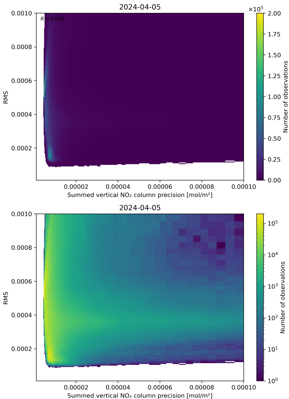
Figure 108: Scatter density plot of “Summed vertical NO 2 column precision” against “RMS” for 2024-04-05 to 2024-04-06.
