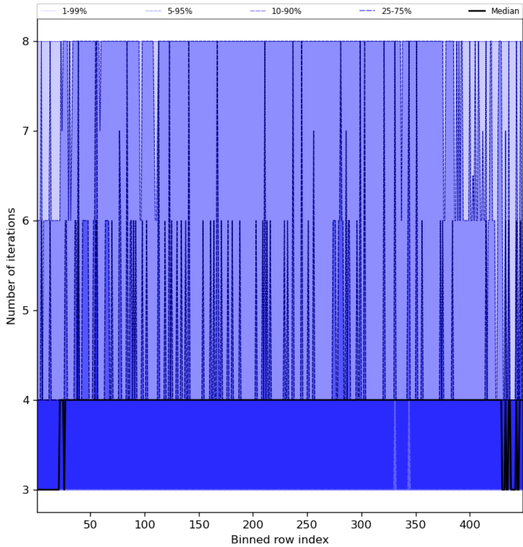
Figure 51: Along track statistics of “Number of iterations” for 2024-04-05 to 2024-04-06
