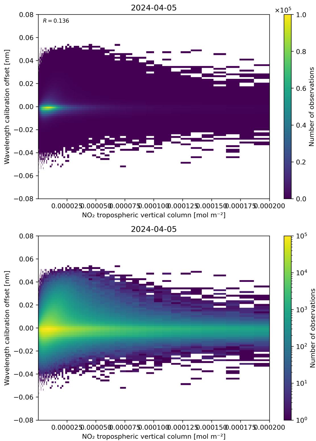
Figure 143: Scatter density plot of “NO 2 tropospheric vertical column” against “Wavelength calibration offset” for 2024-04-05 to 2024-04-06.
