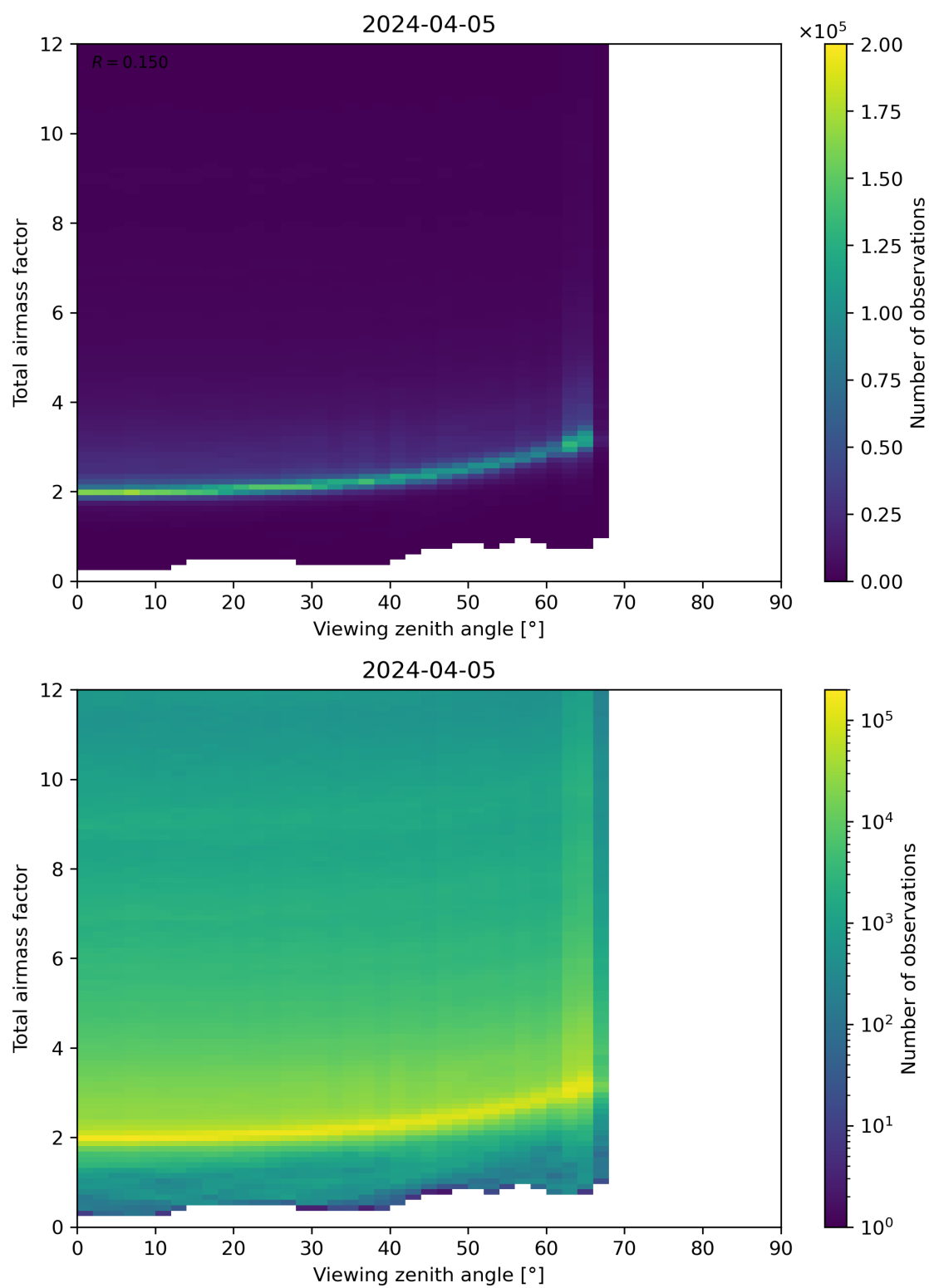
Figure 160: Scatter density plot of “Viewing zenith angle” against “Total airmass factor” for 2024-04-05 to 2024-04-06.
