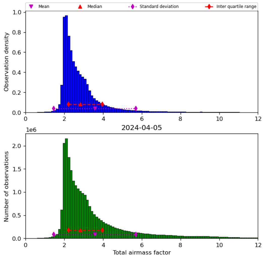
Figure 32: Histogram of “Total airmass factor” for 2024-04-05 to 2024-04-06
