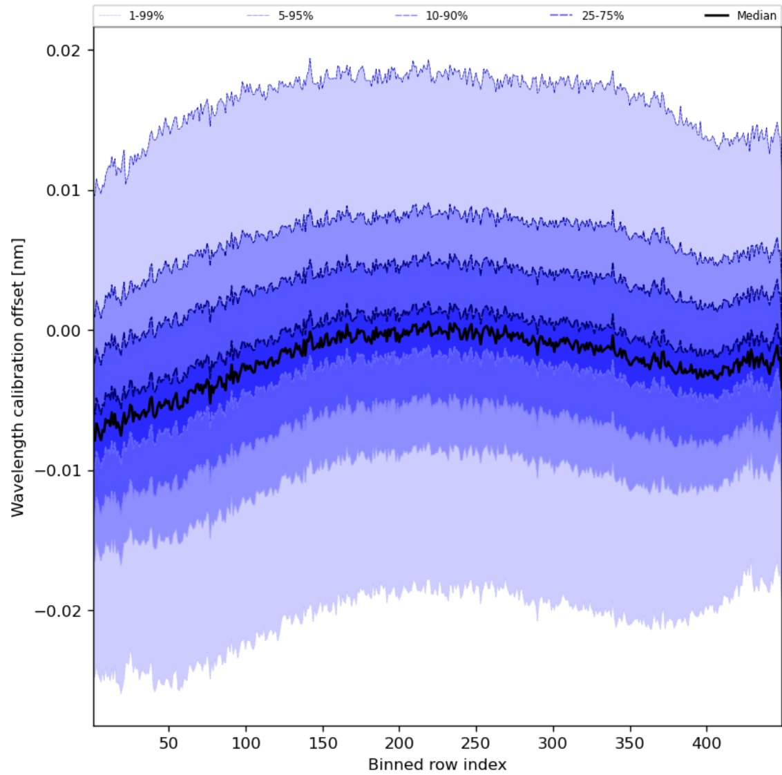
Figure 52: Along track statistics of “Wavelength calibration offset” for 2024-04-05 to 2024-04-06
