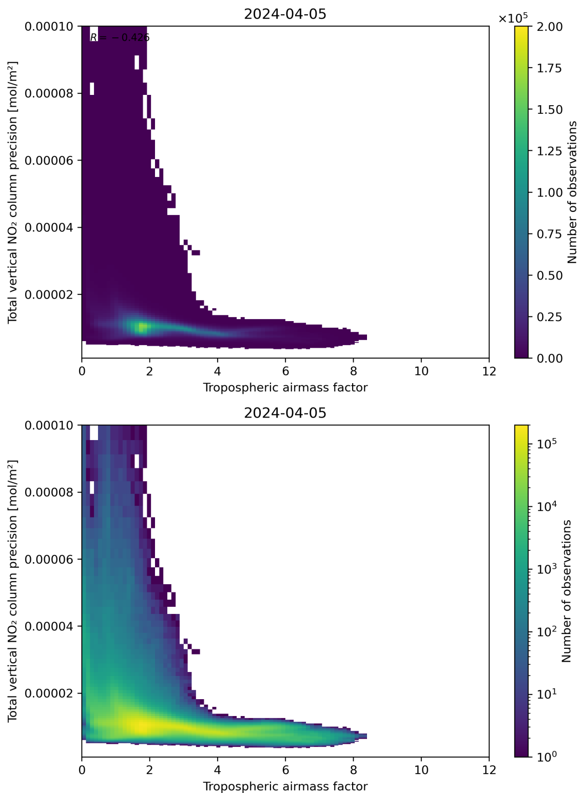
Figure 78: Scatter density plot of “Tropospheric air mass factor” against “Total vertical NO 2 column precision” for 2024-04-05 to 2024-04-06.
