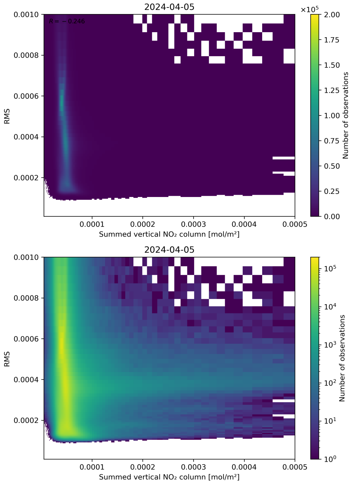
Figure 109: Scatter density plot of “Summed vertical NO 2 column” against “RMS” for 2024-04-05 to 2024-04-06.
