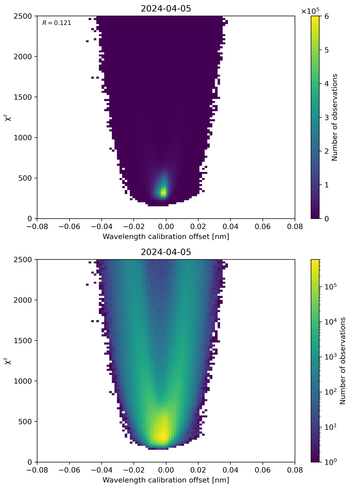
Figure 175: Scatter density plot of “Wavelength calibration offset” against “ \chi^2 ” for 2024-04-05 to 2024-04-06.
