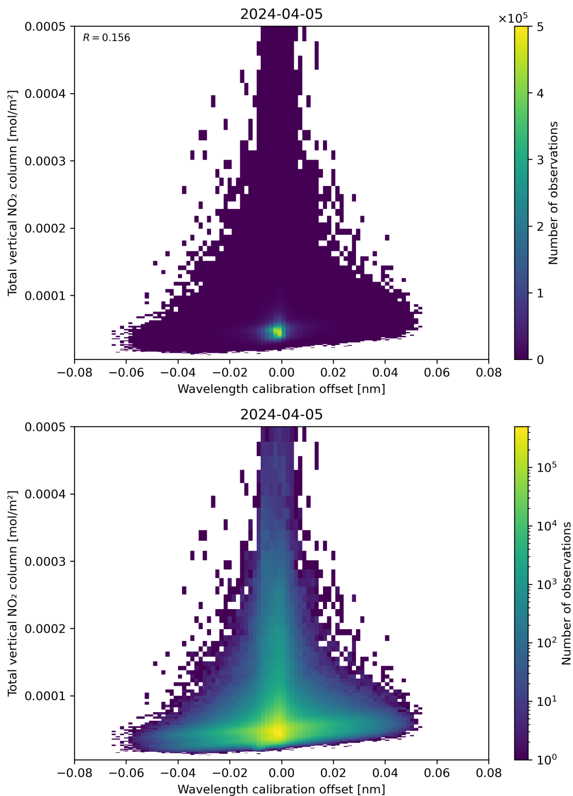
Figure 179: Scatter density plot of “Wavelength calibration offset” against “Total vertical NO 2 column” for 2024-04-05 to 2024-04-06.
