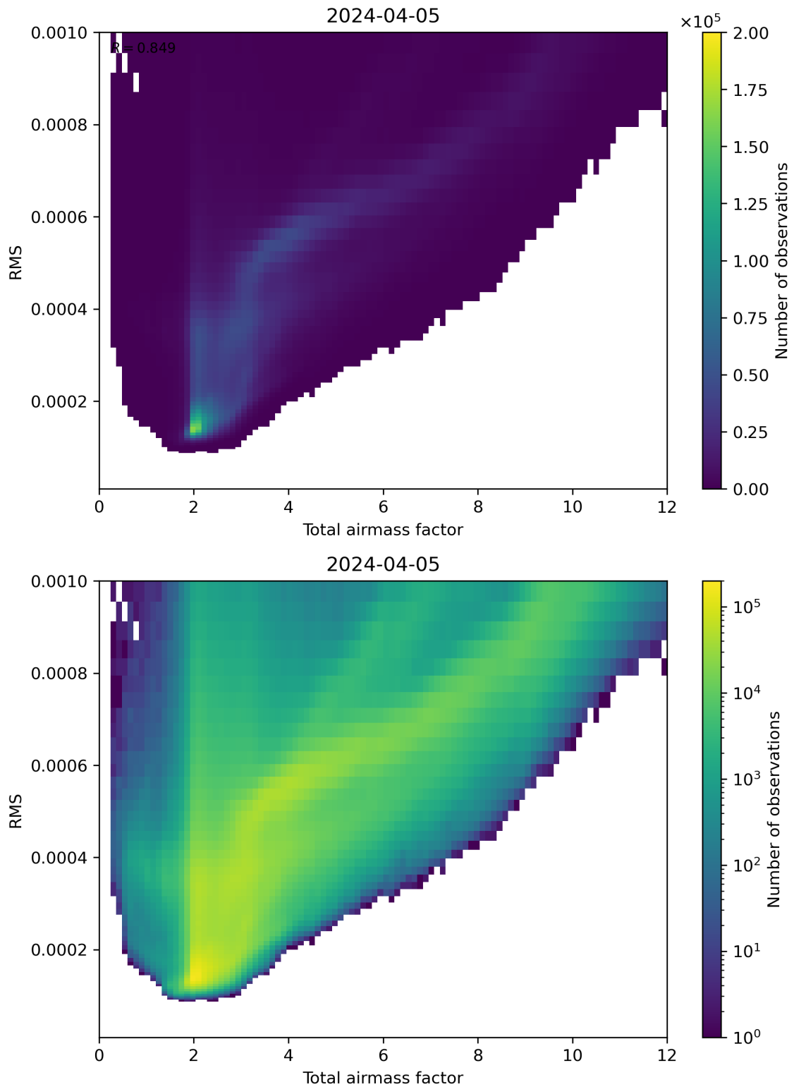
Figure 69: Scatter density plot of “Total airmass factor” against “RMS” for 2024-04-05 to 2024-04-06.
