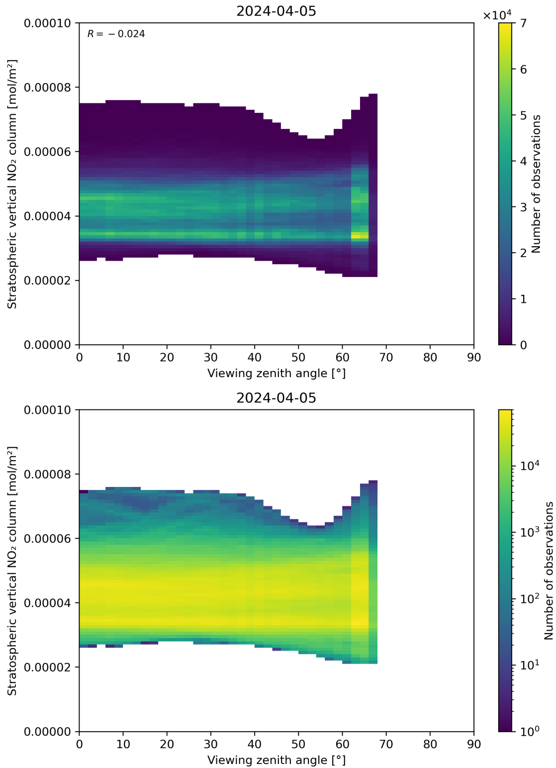
Figure 164: Scatter density plot of “Viewing zenith angle” against “Stratospheric vertical NO 2 column” for 2024-04-05 to 2024-04-06.
