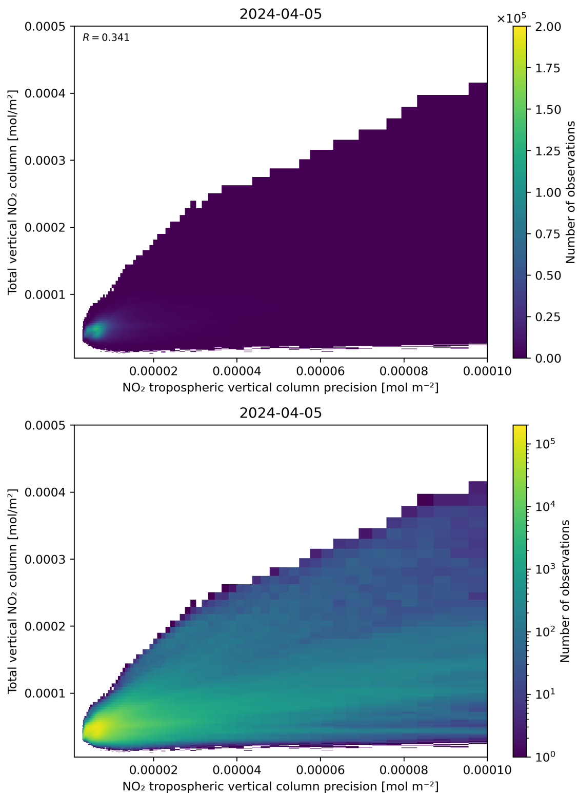
Figure 138: Scatter density plot of “NO 2 tropospheric vertical column precision” against “Total vertical NO 2 column” for 2024-04-05 to 2024-04-06.
