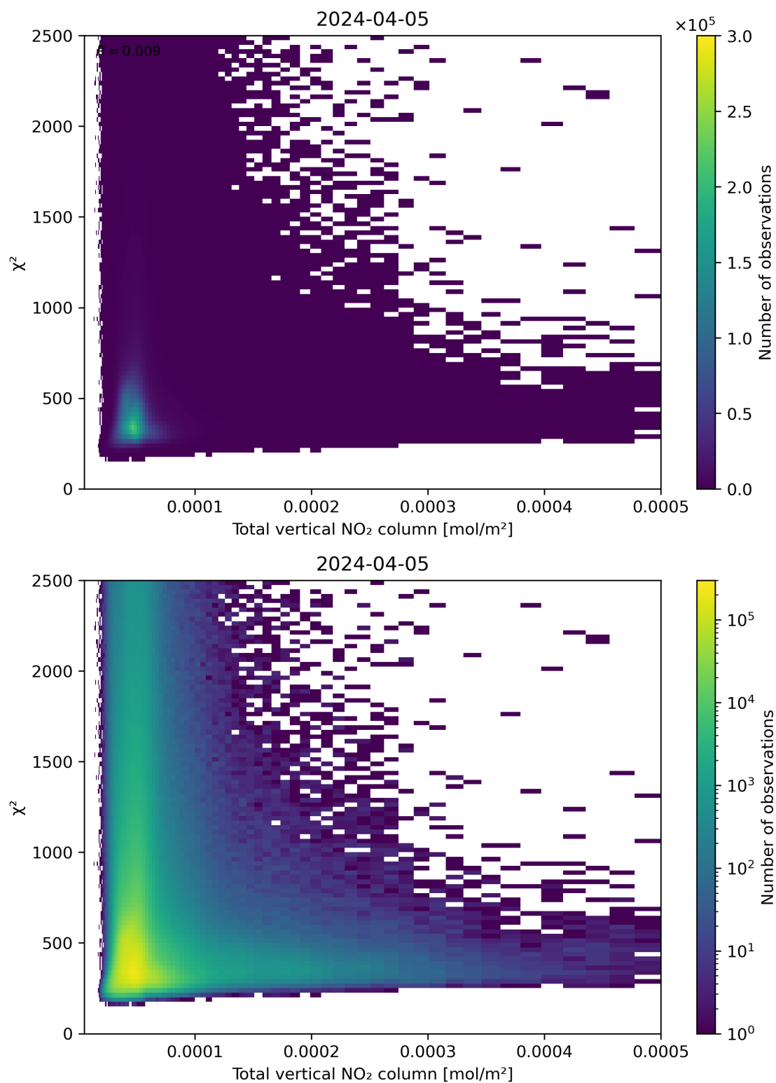
Figure 111: Scatter density plot of “Total vertical NO 2 column” against “ \chi^2 ” for 2024-04-05 to 2024-04-06.
