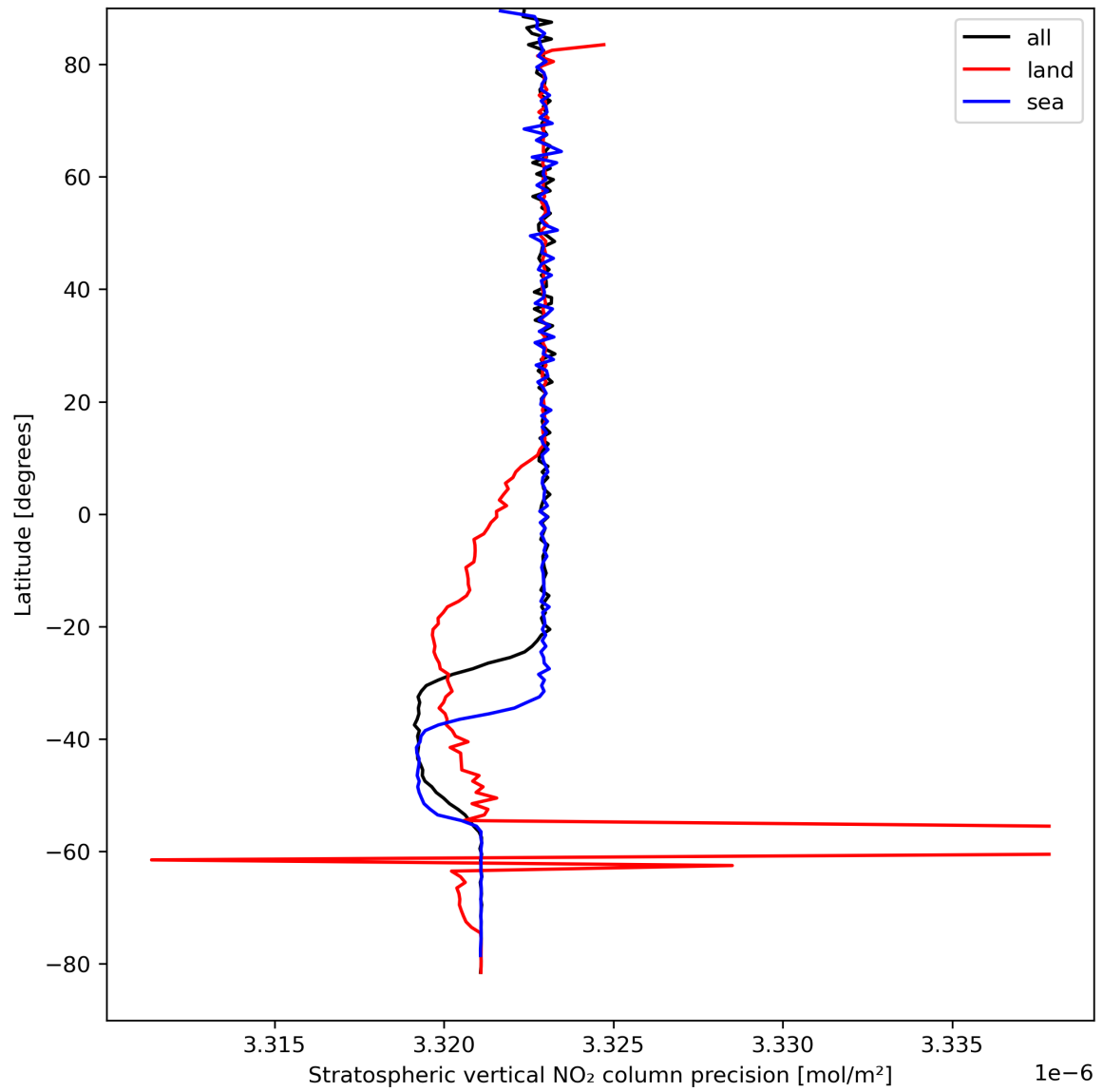
Figure 20: Zonal average of “Stratospheric vertical NO 2 column precision” for 2024-04-05 to 2024-04-06.
