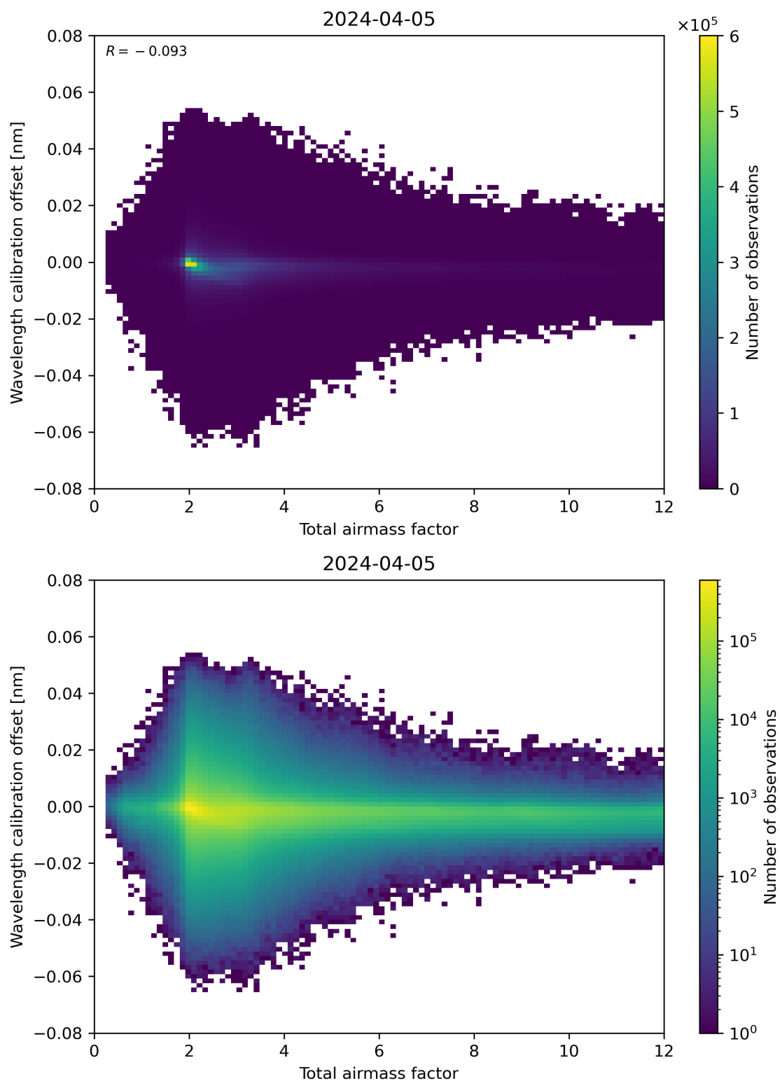
Figure 70: Scatter density plot of “Total airmass factor” against “Wavelength calibration offset” for 2024-04-05 to 2024-04-06.
