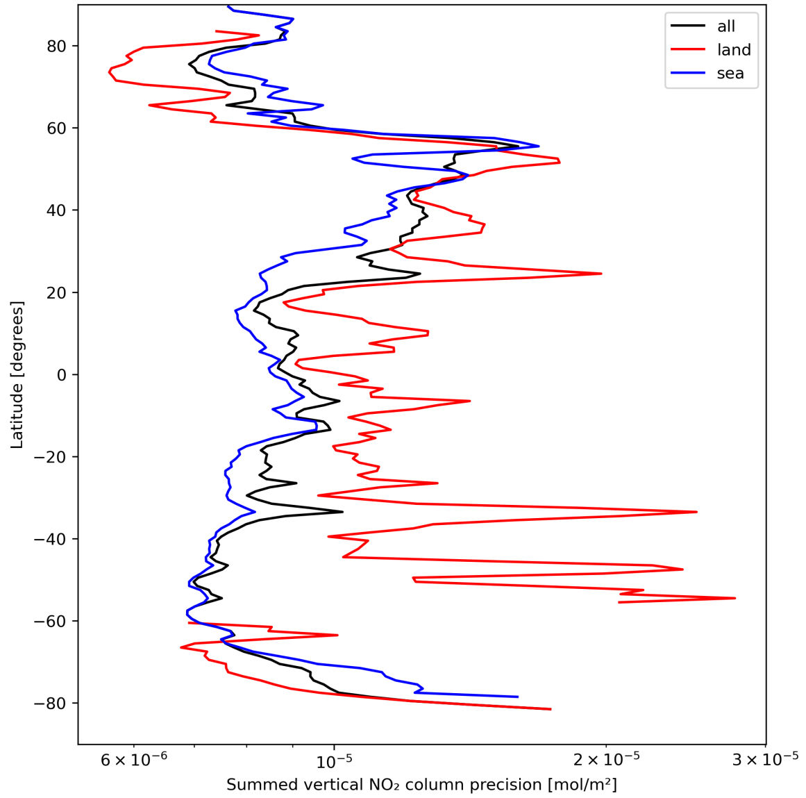
Figure 24: Zonal average of "Summed vertical NO 2 column precision" for 2024-04-05 to 2024-04-06.
