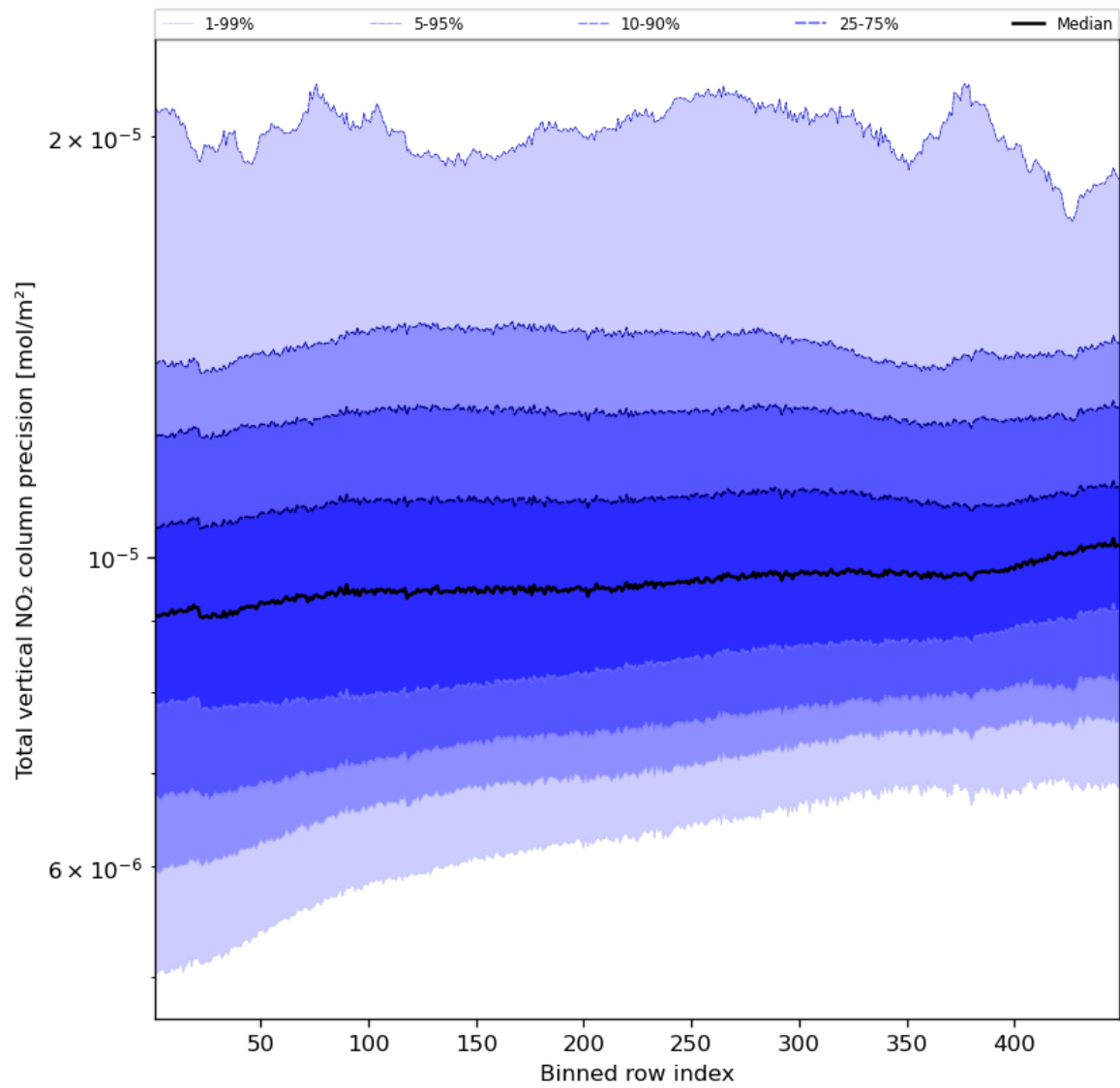
Figure 56: Along track statistics of “Total vertical NO 2 column precision” for 2024-04-05 to 2024-04-06
