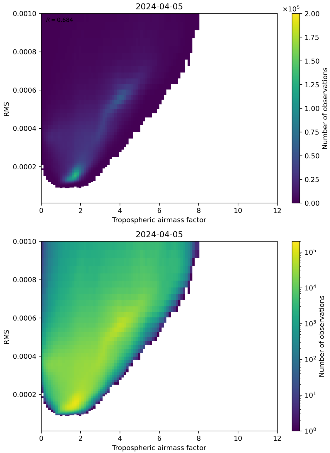
Figure 79: Scatter density plot of “Tropospheric airmass factor” against “RMS” for 2024-04-05 to 2024-04-06.
