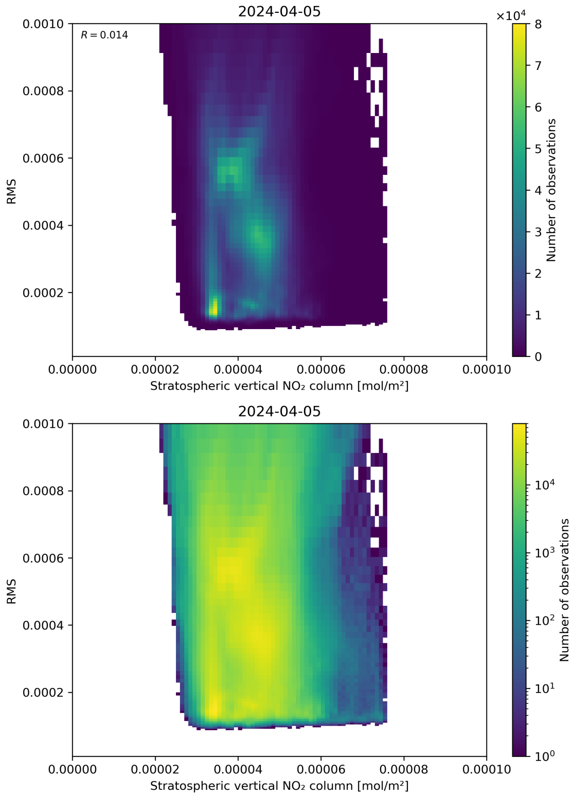
Figure 102: Scatter density plot of “Stratospheric vertical NO 2 column” against “RMS” for 2024-04-05 to 2024-04-06.
