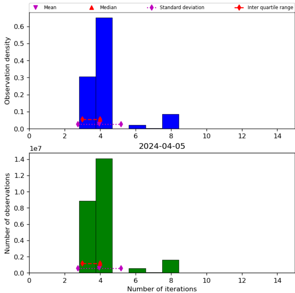
Figure 34: Histogram of “Number of iterations” for 2024-04-05 to 2024-04-06
