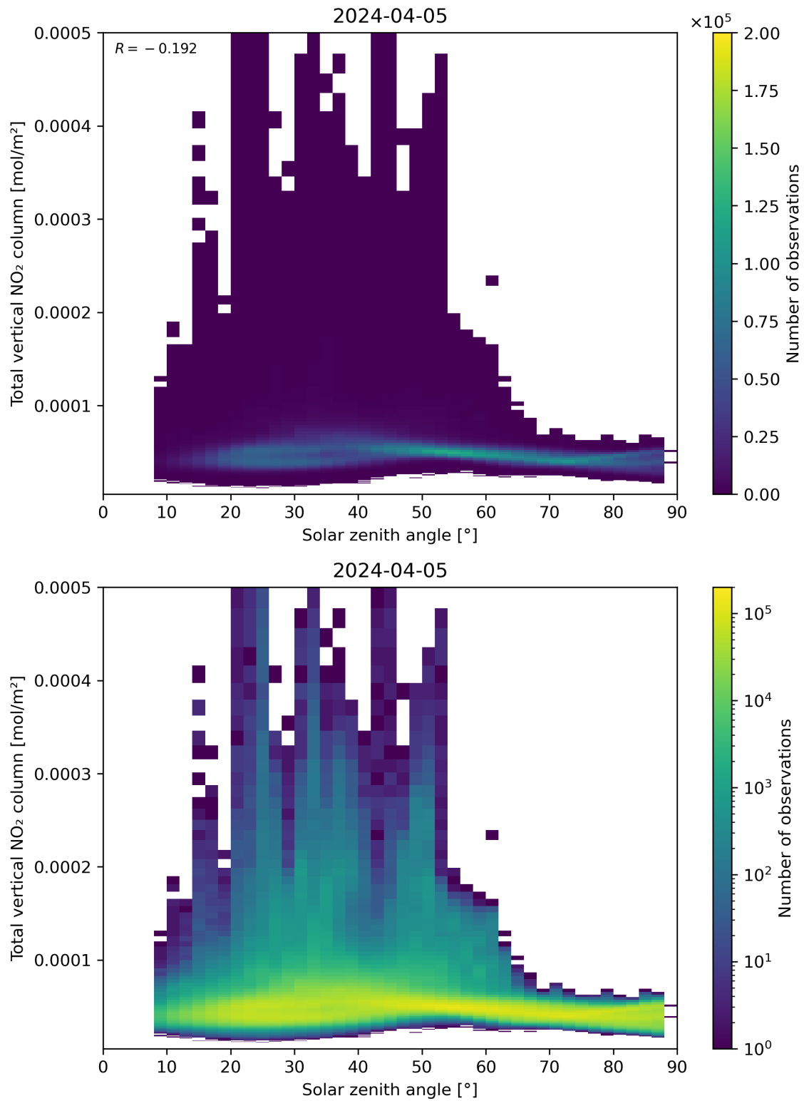
Figure 153: Scatter density plot of “Solar zenith angle” against “Total vertical NO 2 column” for 2024-04-05 to 2024-04-06.
