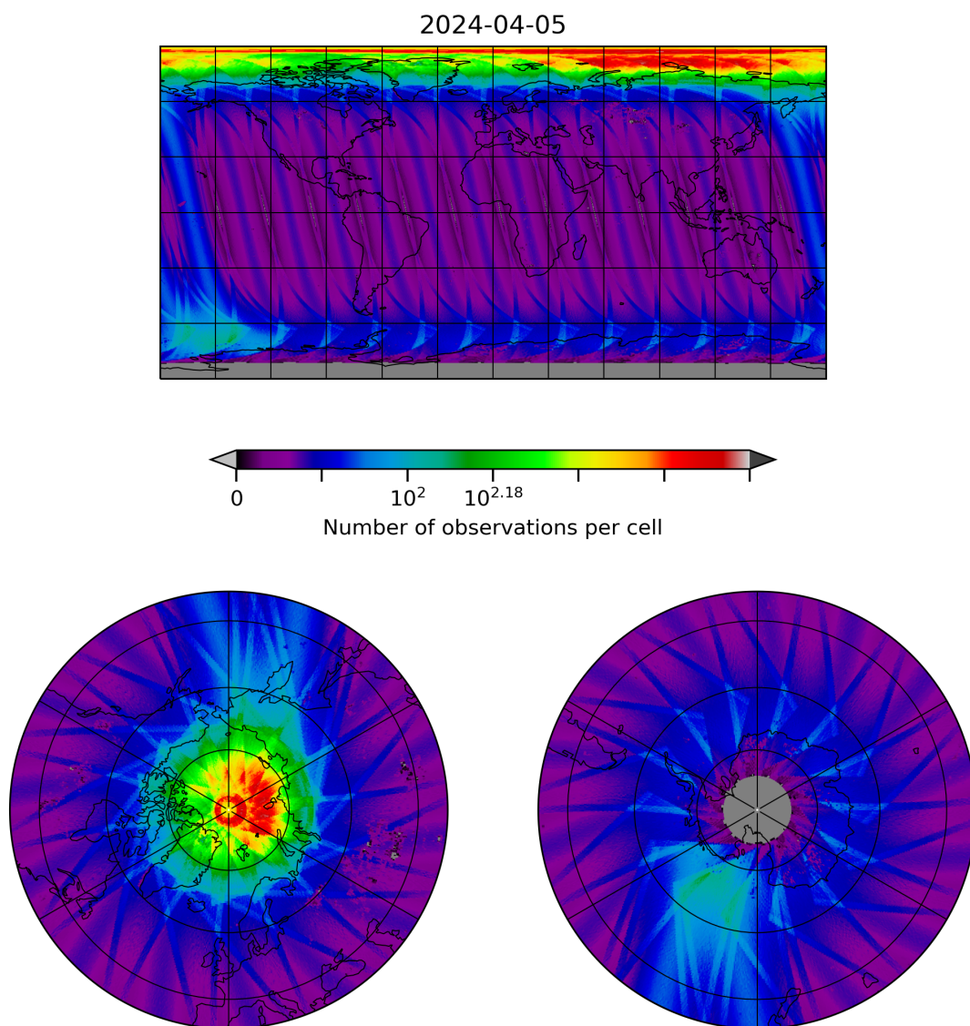
Figure 10: Map of the number of observations for 2024-04-05 to 2024-04-06
