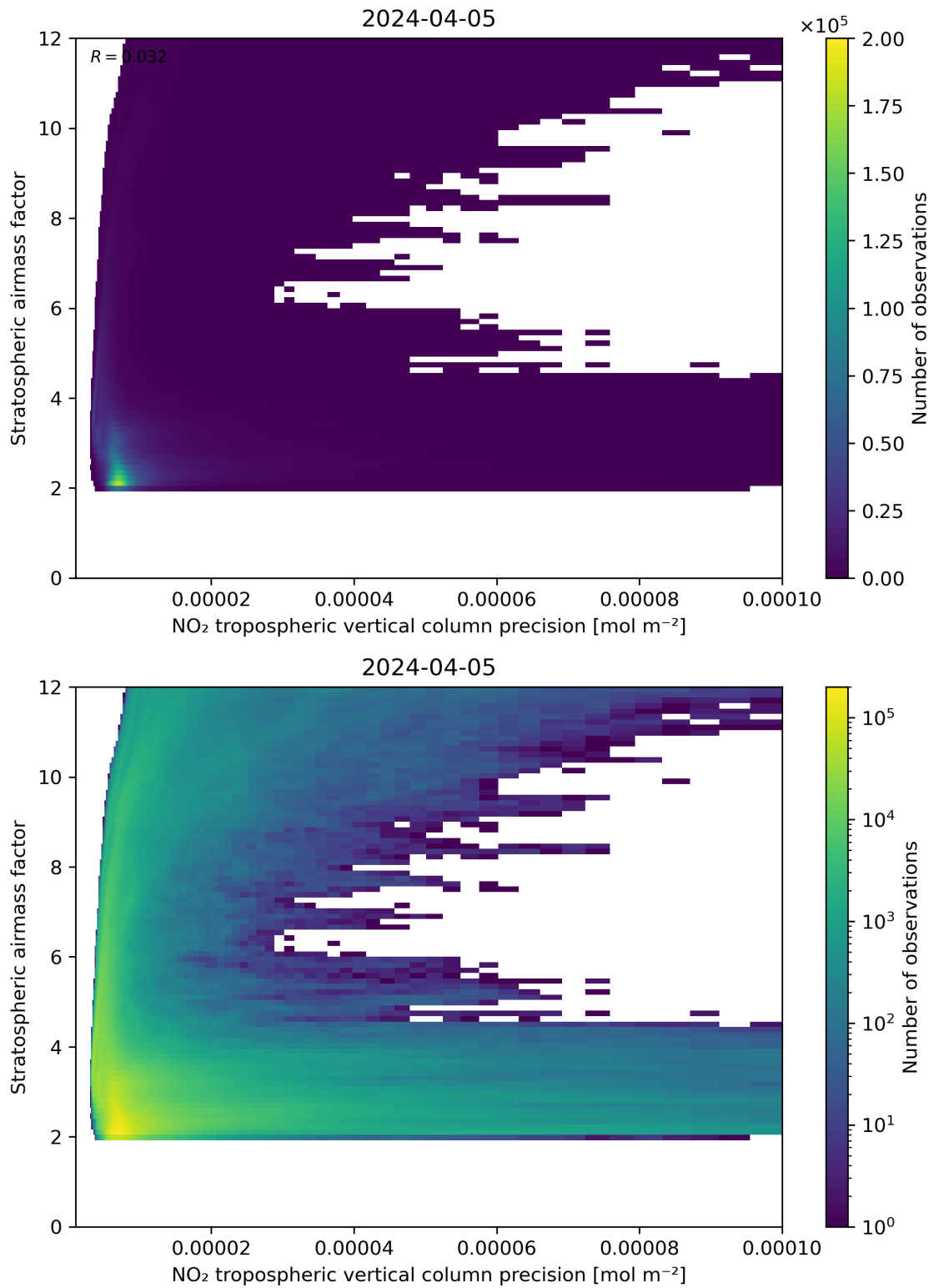
Figure 131: Scatter density plot of “NO 2 tropospheric vertical column precision” against “Stratospheric airmass factor” for 2024-04-05 to 2024-04-06.
