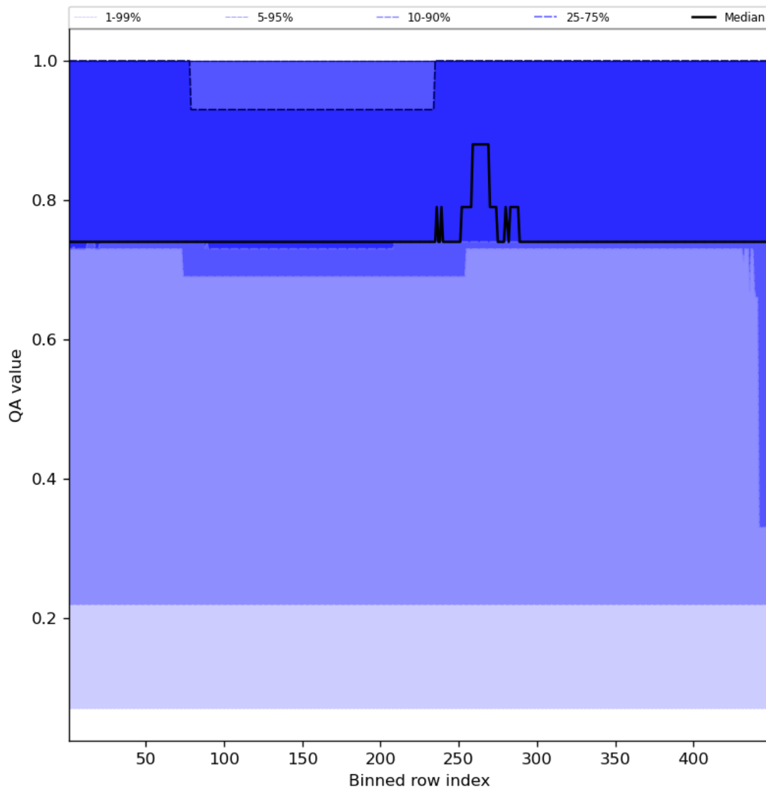
Figure 45: Along track statistics of “QA value” for 2024-04-05 to 2024-04-06
