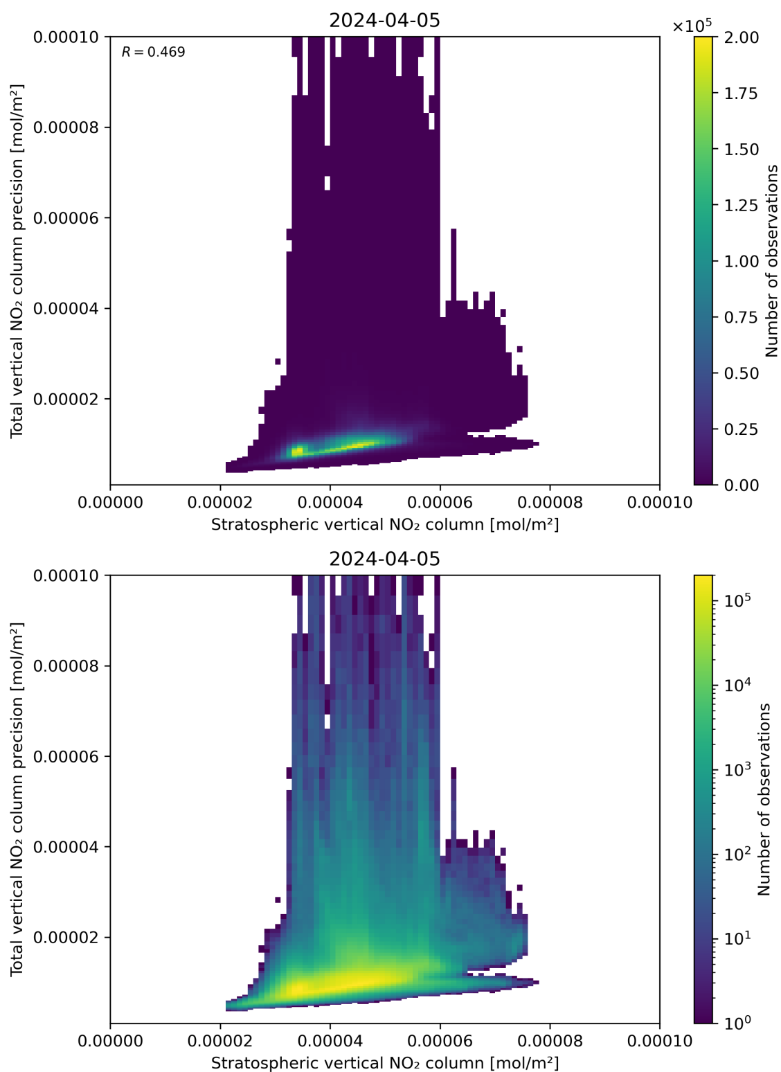
Figure 101: Scatter density plot of “Stratospheric vertical NO 2 column” against “Total vertical NO 2 column precision” for 2024-04-05 to 2024-04-06.
