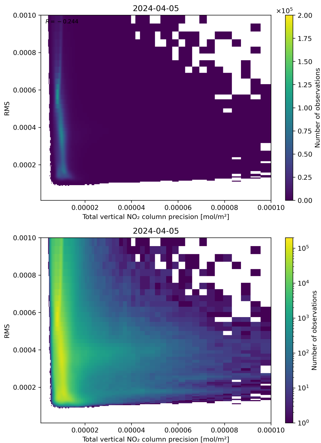
Figure 119: Scatter density plot of “Total vertical NO 2 column precision” against “RMS” for 2024-04-05 to 2024-04-06.
