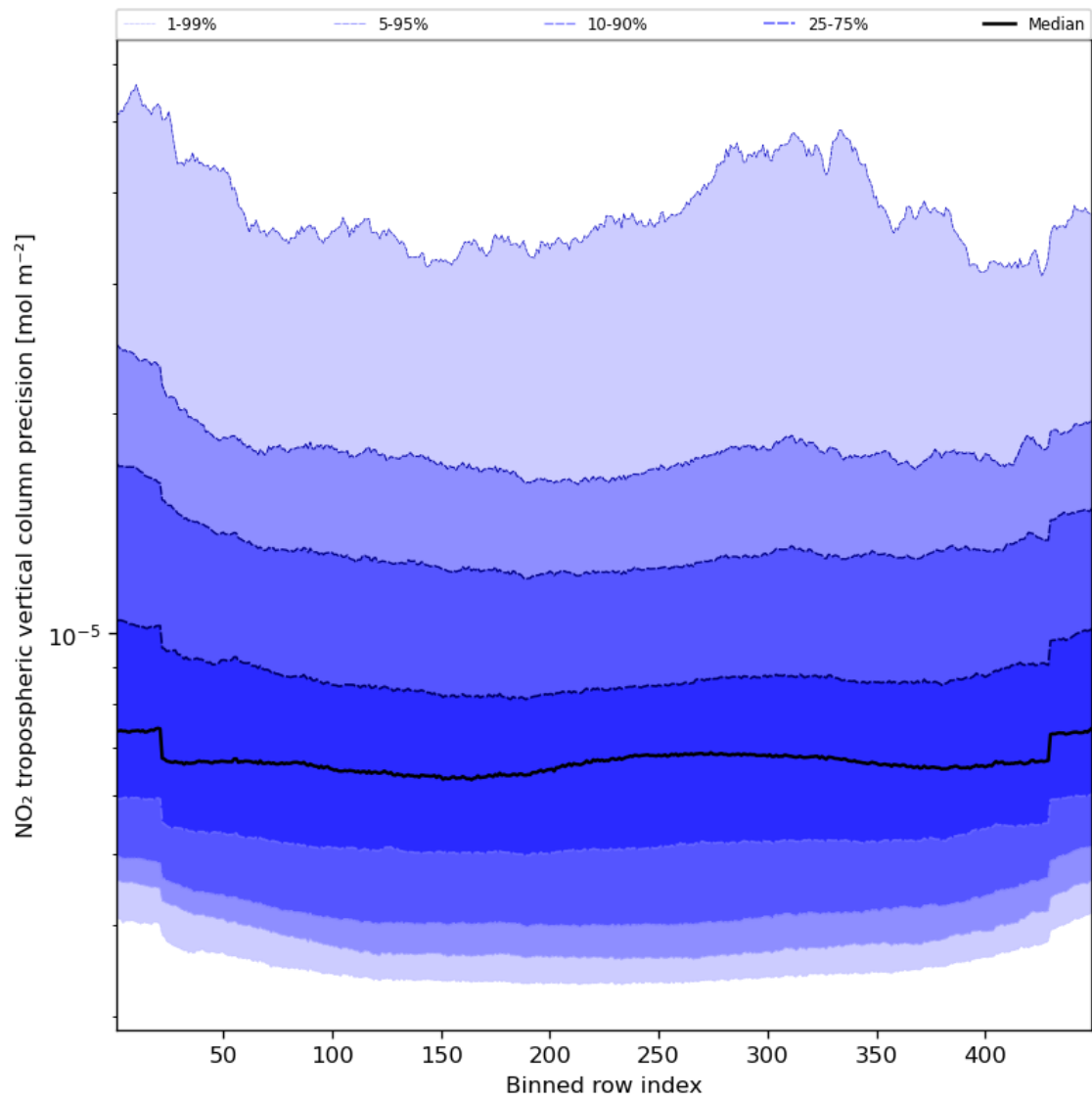
Figure 47: Along track statistics of “NO 2 tropospheric vertical column precision” for 2024-04-05 to 2024-04-06
