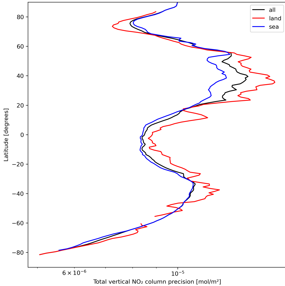
Figure 22: Zonal average of “Total vertical NO 2 column precision” for 2024-04-05 to 2024-04-06.
