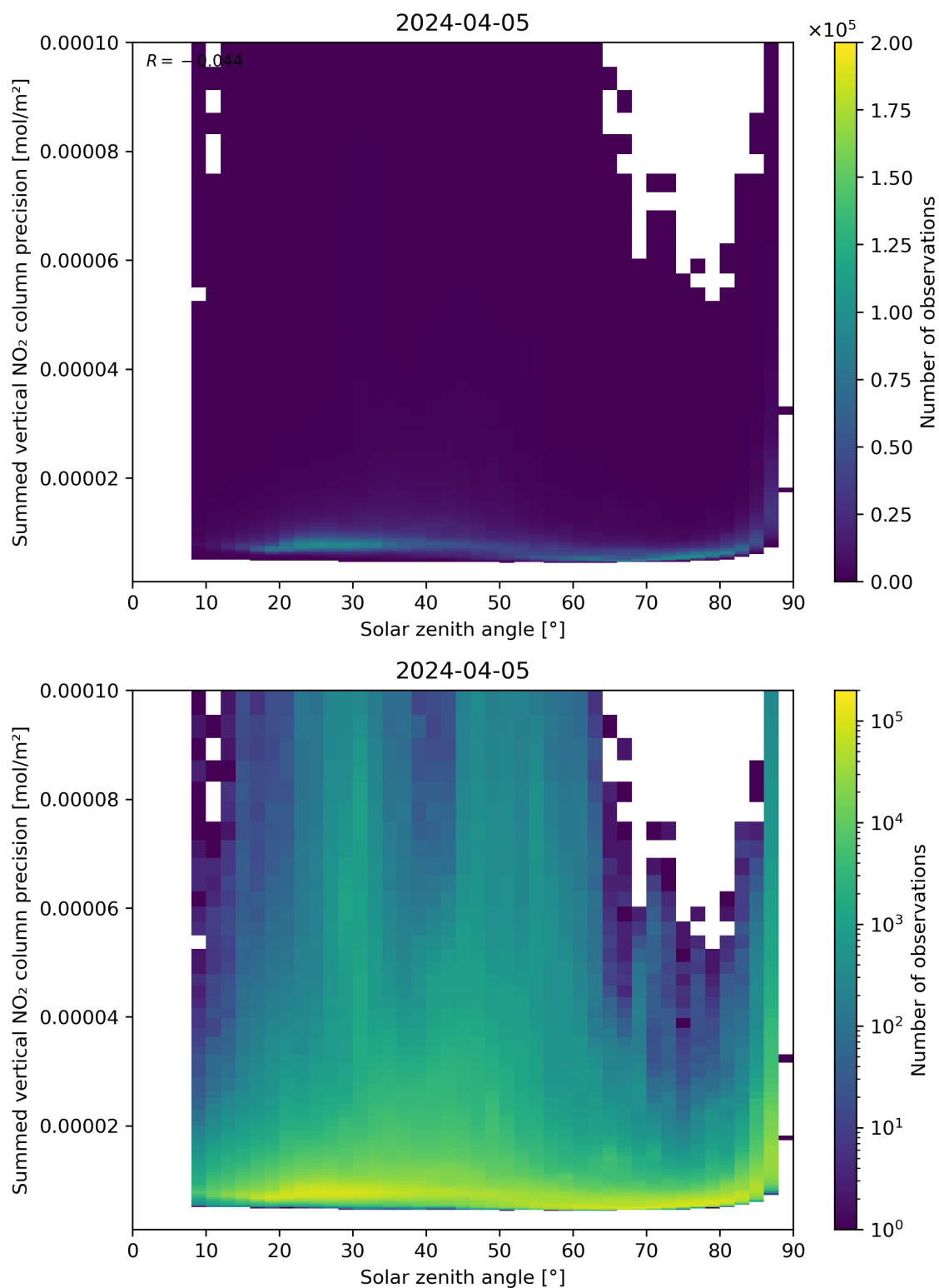
Figure 152: Scatter density plot of “Solar zenith angle” against “Summed vertical NO 2 column precision” for 2024-04-05 to 2024-04-06.
