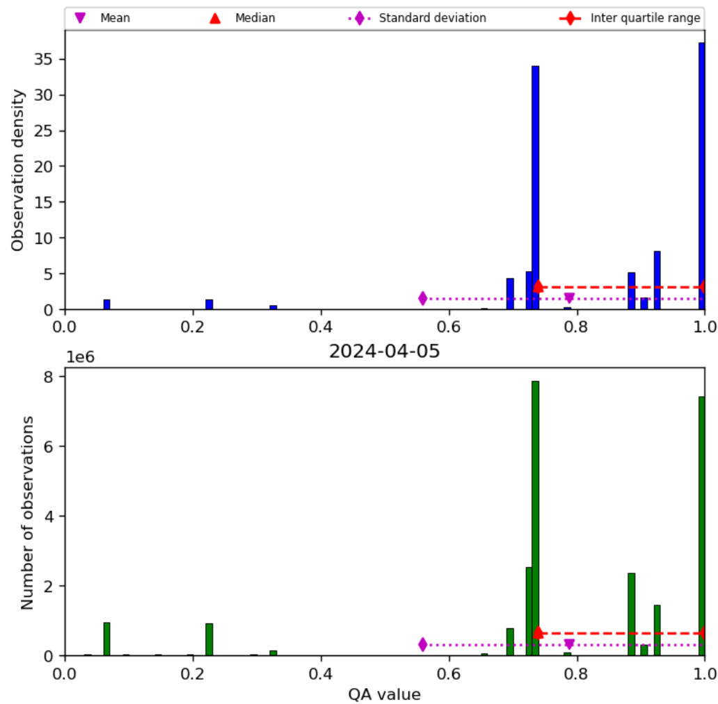
Figure 28: Histogram of “QA value” for 2024-04-05 to 2024-04-06
