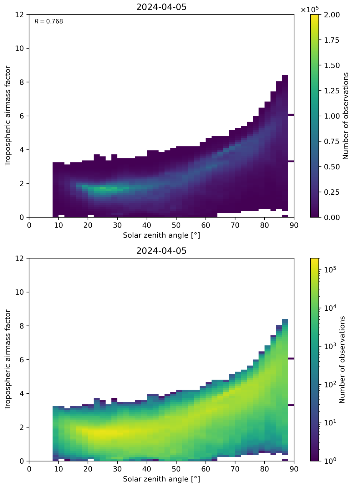
Figure 147: Scatter density plot of “Solar zenith angle” against “Tropospheric airmass factor” for 2024-04-05 to 2024-04-06.
