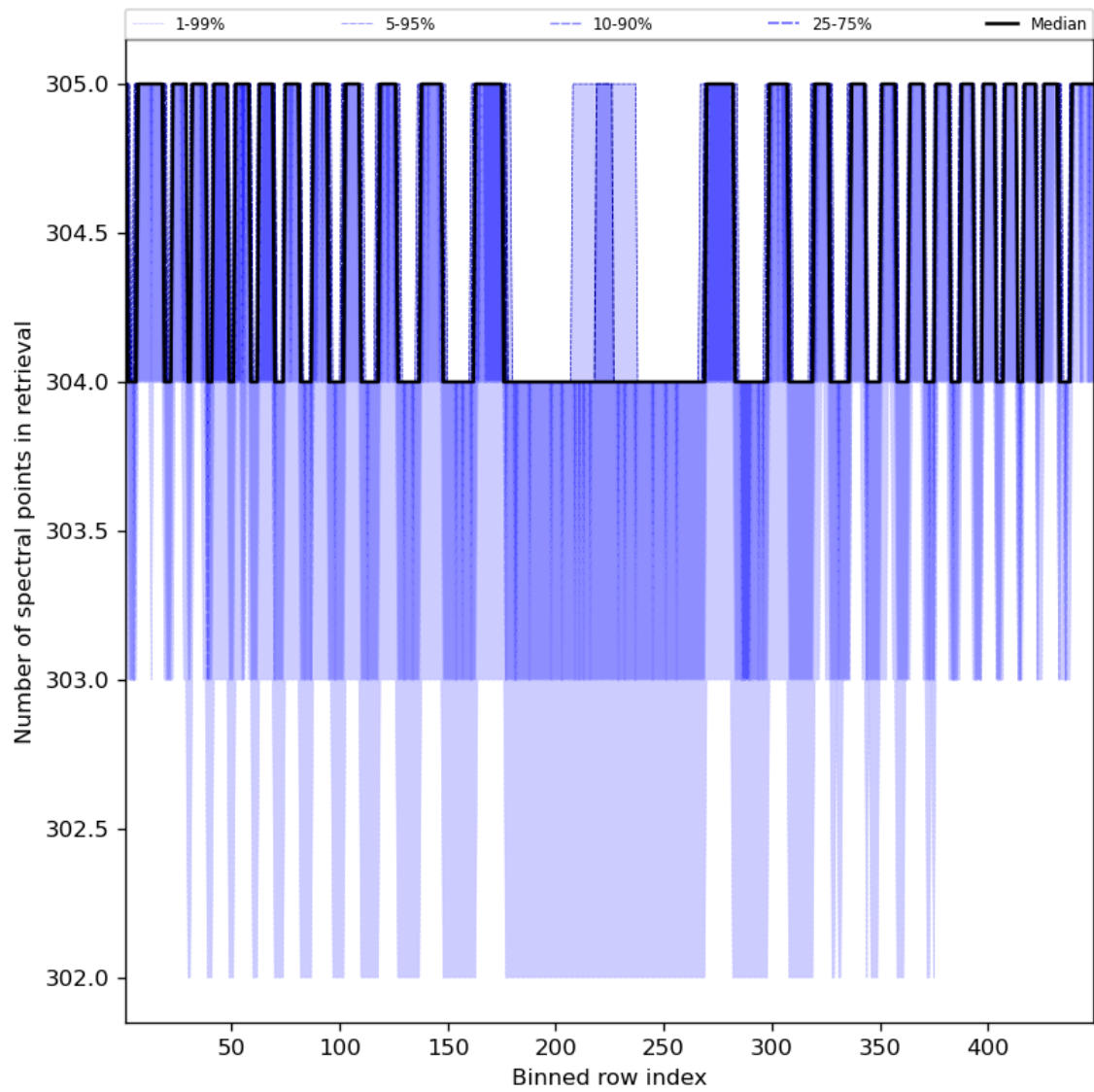
Figure 50: Along track statistics of “Number of spectral points in retrieval” for 2024-04-05 to 2024-04-06
