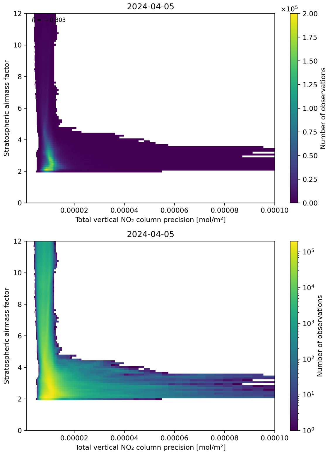
Figure 115: Scatter density plot of “Total vertical NO 2 column precision” against “Stratospheric air mass factor” for 2024-04-05 to 2024-04-06.
