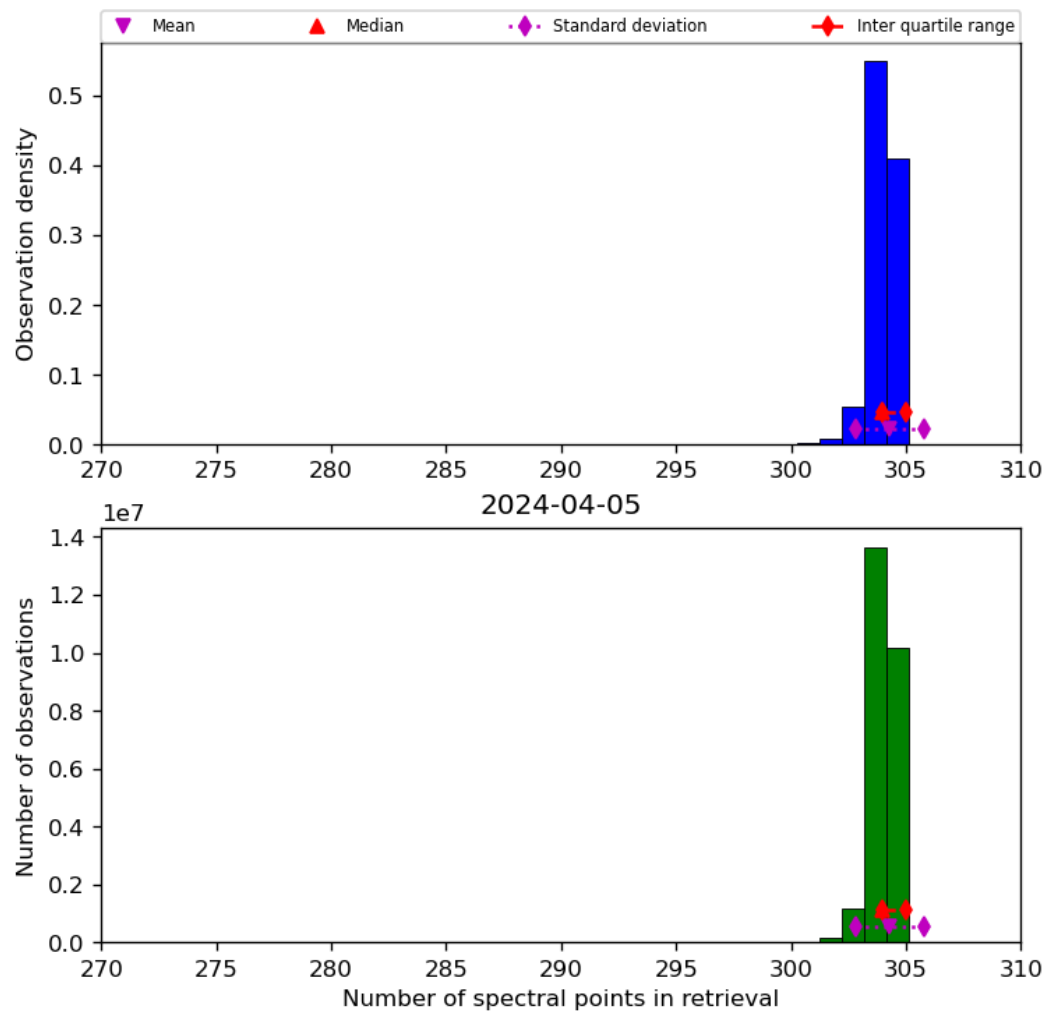
Figure 33: Histogram of “Number of spectral points in retrieval” for 2024-04-05 to 2024-04-06
