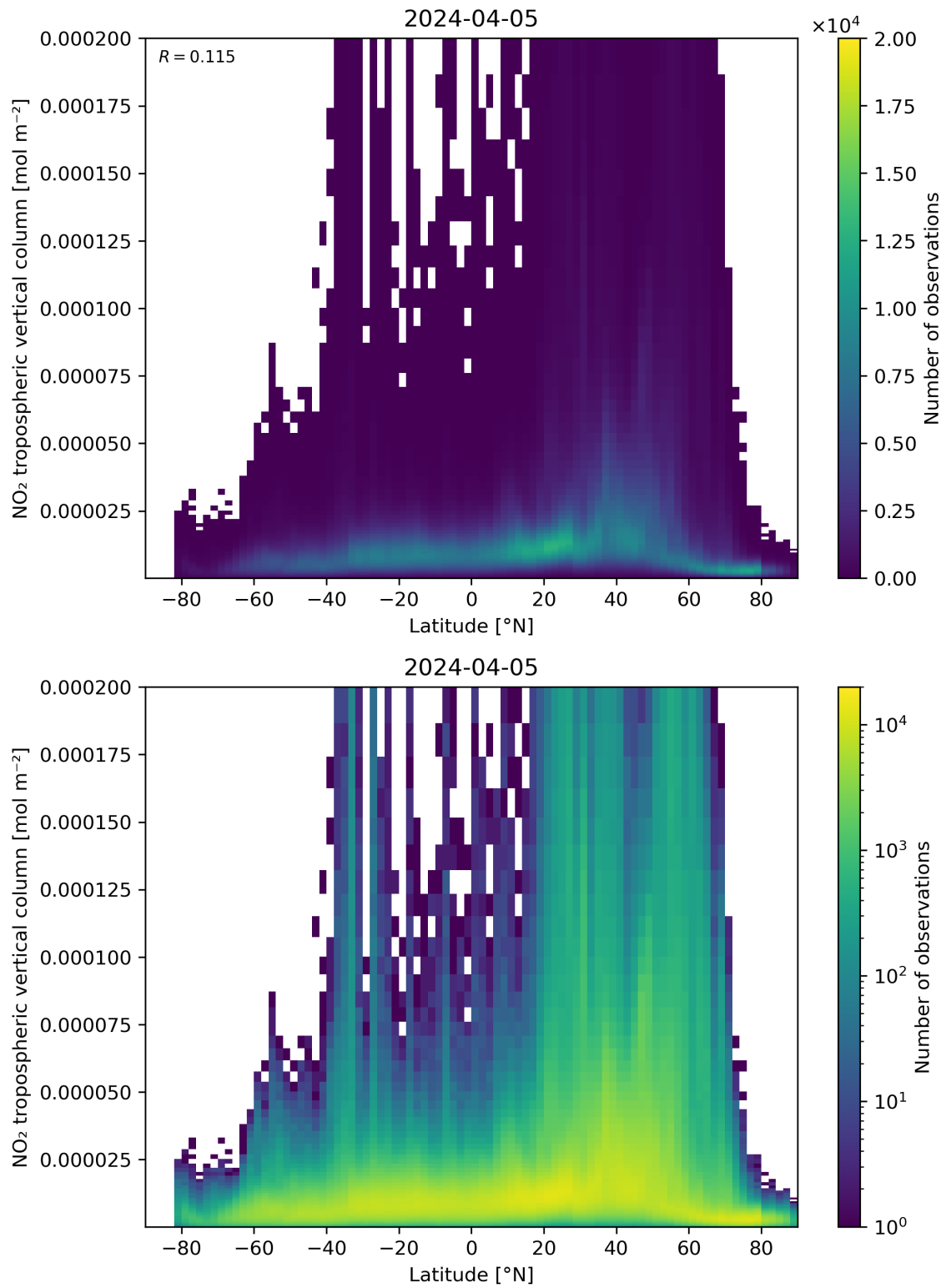
Figure 92: Scatter density plot of “Latitude” against “NO 2 tropospheric vertical column” for 2024-04-05 to 2024-04-06.
