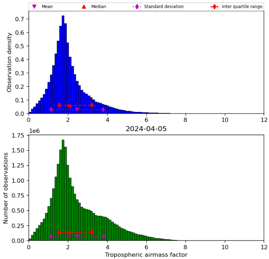
Figure 31: Histogram of “Tropospheric airmass factor” for 2024-04-05 to 2024-04-06
