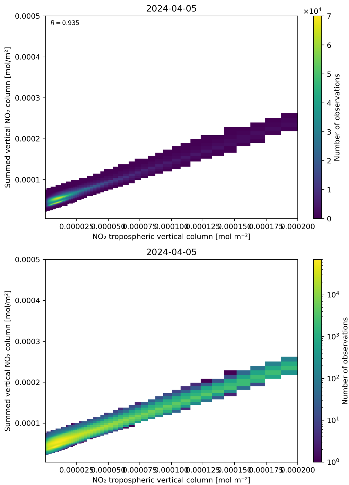
Figure 126: Scatter density plot of “NO 2 tropospheric vertical column” against “Summed vertical NO 2 column” for 2024-04-05 to 2024-04-06.
