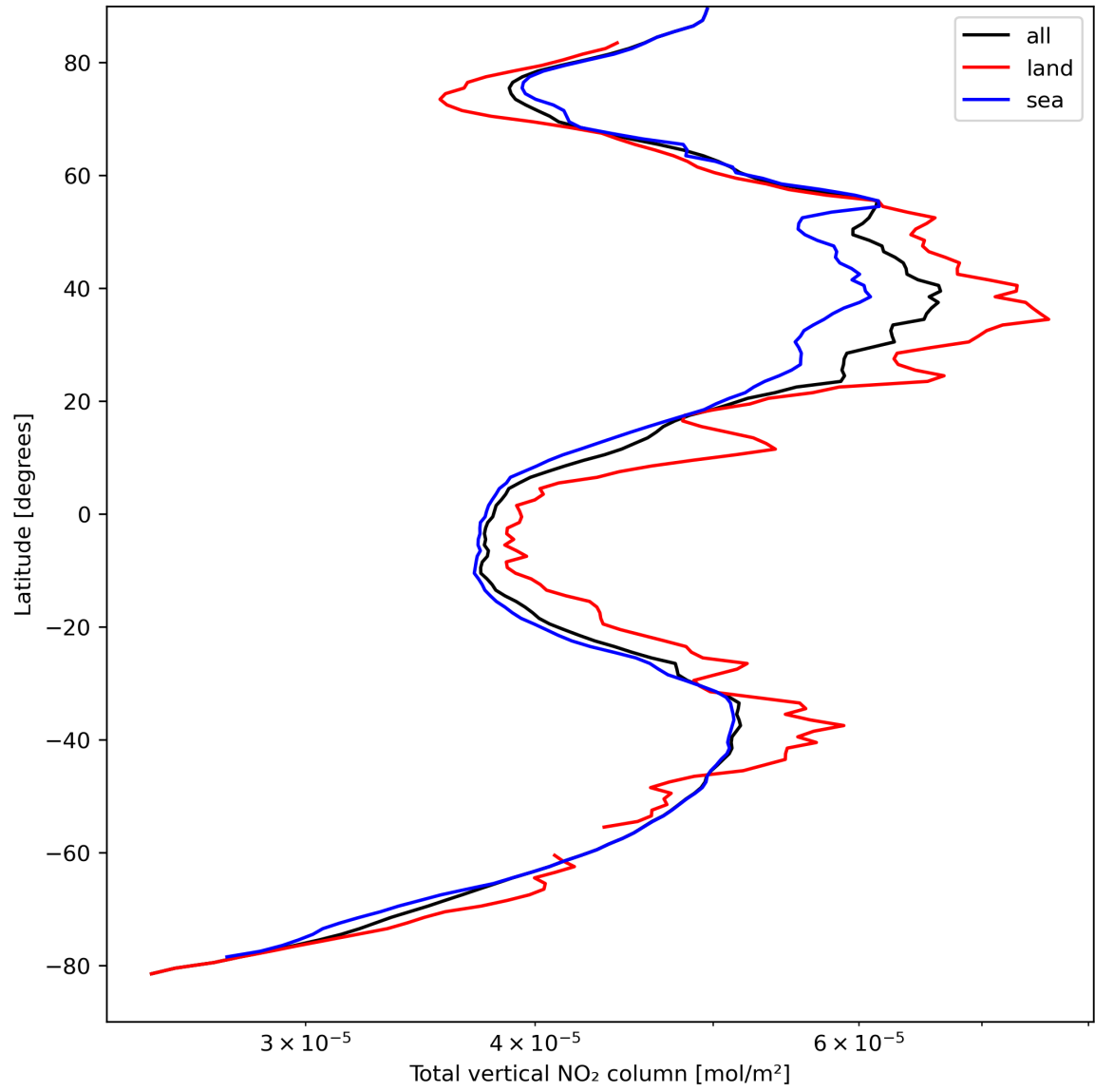
Figure 21: Zonal average of “Total vertical NO 2 column” for 2024-04-05 to 2024-04-06.
