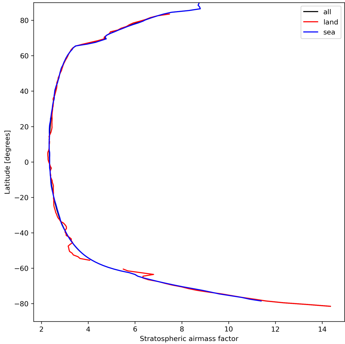
Figure 27: Zonal average of “Stratospheric air mass factor” for 2024-04-05 to 2024-04-06.
