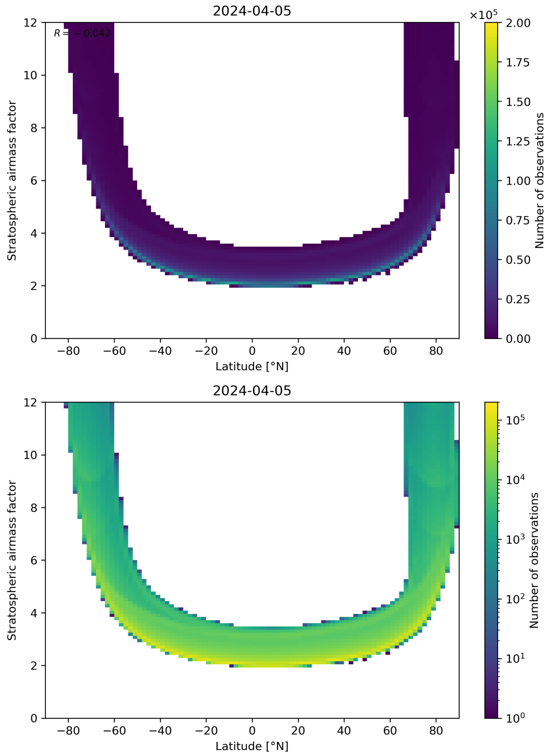
Figure 83: Scatter density plot of “Latitude” against “Stratospheric airmass factor” for 2024-04-05 to 2024-04-06.
