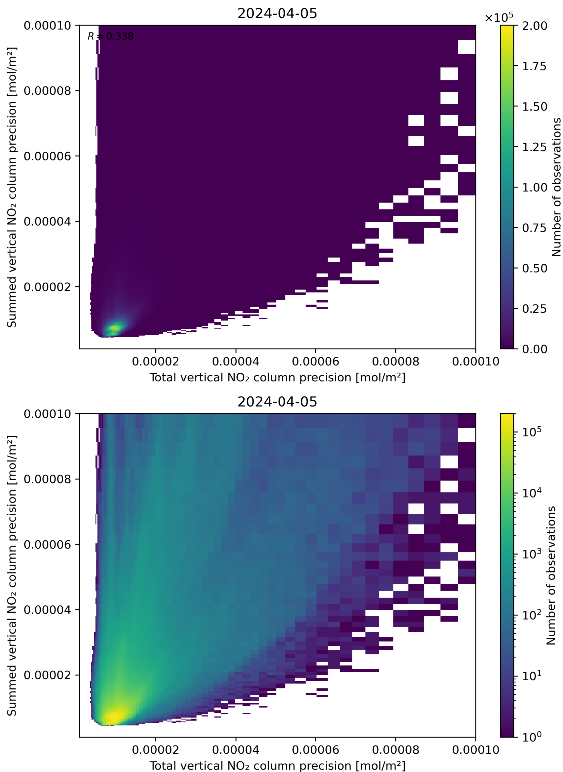
Figure 118: Scatter density plot of “Total vertical NO 2 column precision” against “Summed vertical NO 2 column precision” for 2024-04-05 to 2024-04-06.
