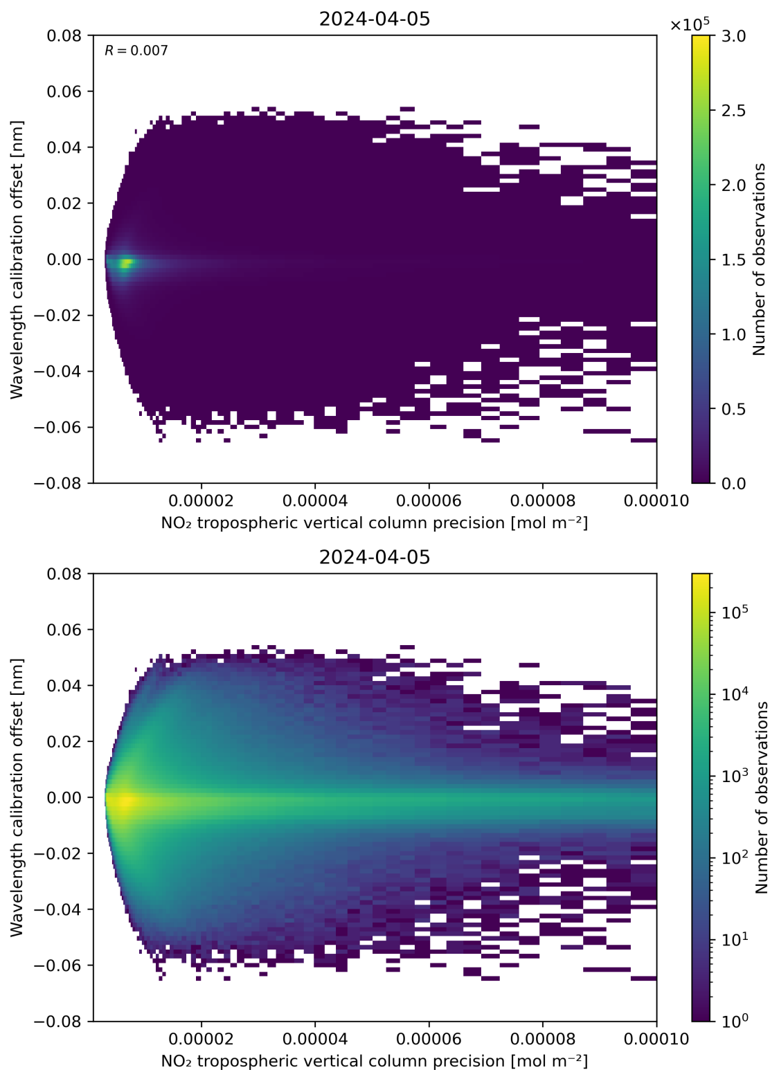
Figure 141: Scatter density plot of “NO 2 tropospheric vertical column precision” against “Wavelength calibration offset” for 2024-04-05 to 2024-04-06.
