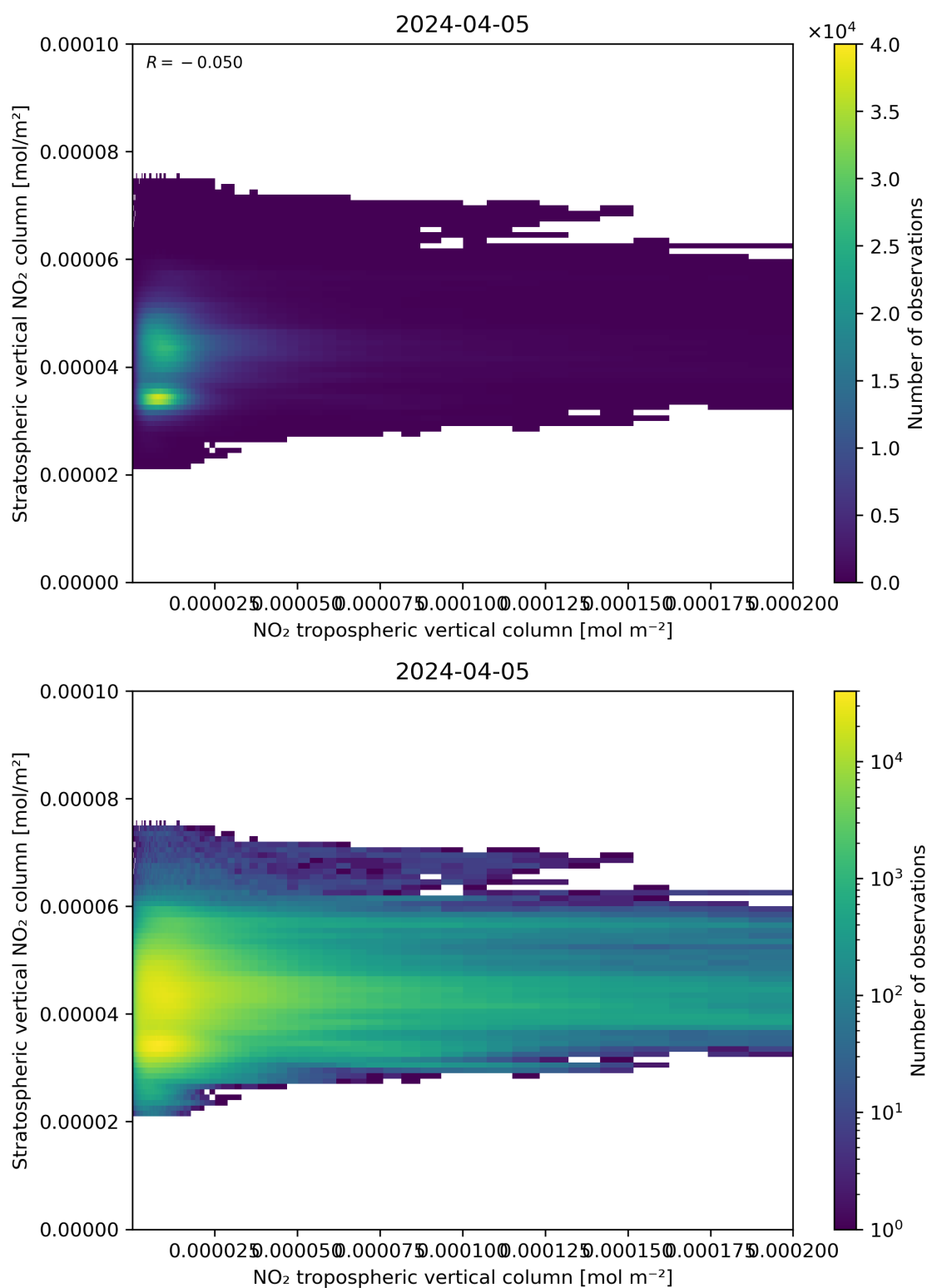
Figure 125: Scatter density plot of “NO 2 tropospheric vertical column” against “Stratospheric vertical NO 2 column” for 2024-04-05 to 2024-04-06.
