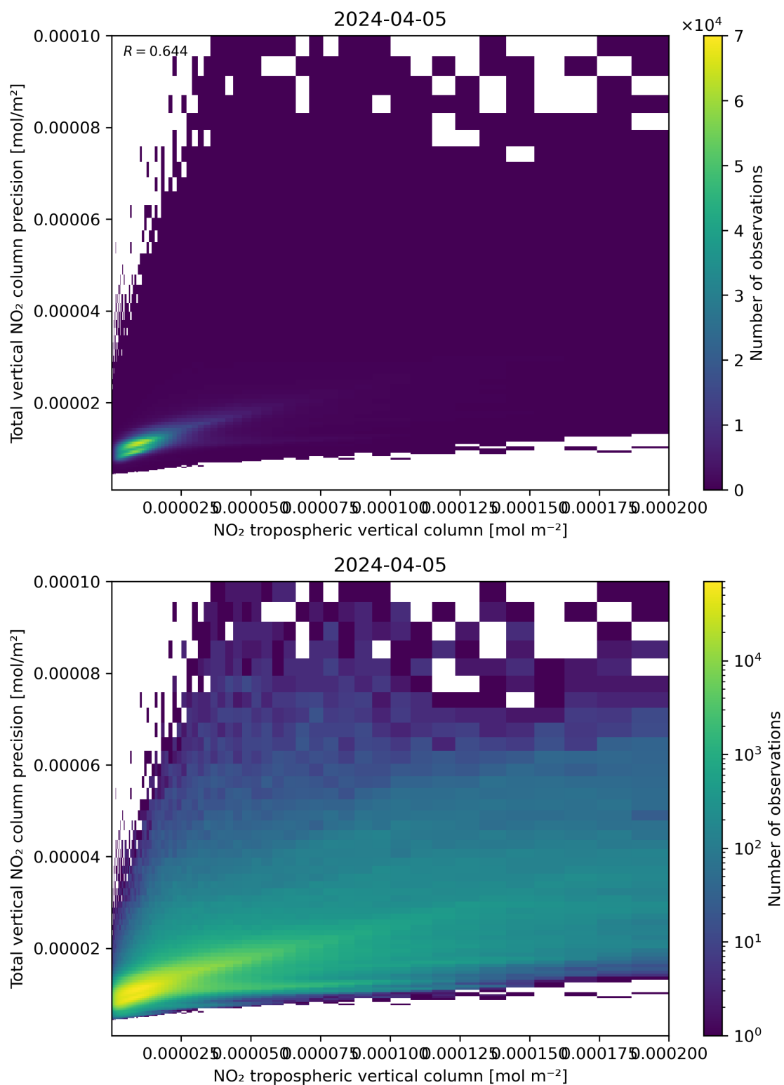
Figure 129: Scatter density plot of “NO 2 tropospheric vertical column” against “Total vertical NO 2 column precision” for 2024-04-05 to 2024-04-06.
