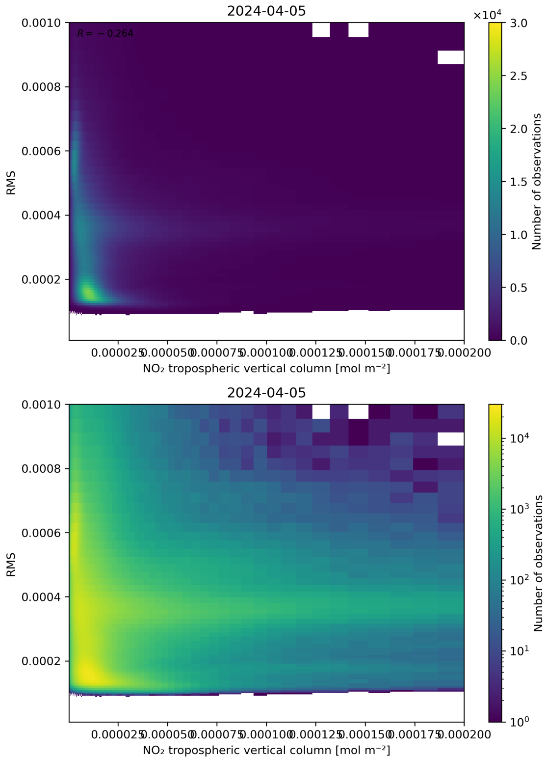
Figure 142: Scatter density plot of “NO 2 tropospheric vertical column” against “RMS” for 2024-04-05 to 2024-04-06.
