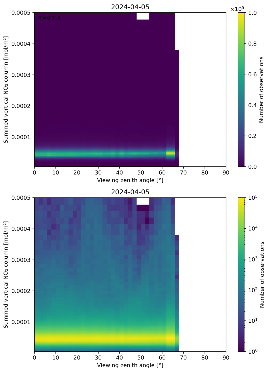
Figure 165: Scatter density plot of “Viewing zenith angle” against “Summed vertical NO 2 column” for 2024-04-05 to 2024-04-06.
