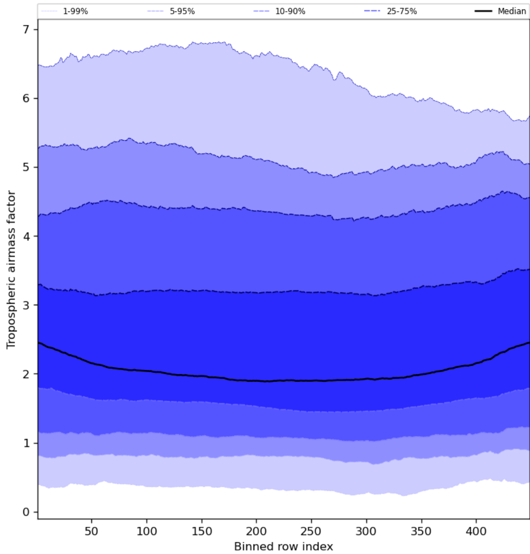
Figure 48: Along track statistics of “Tropospheric airmass factor” for 2024-04-05 to 2024-04-06
