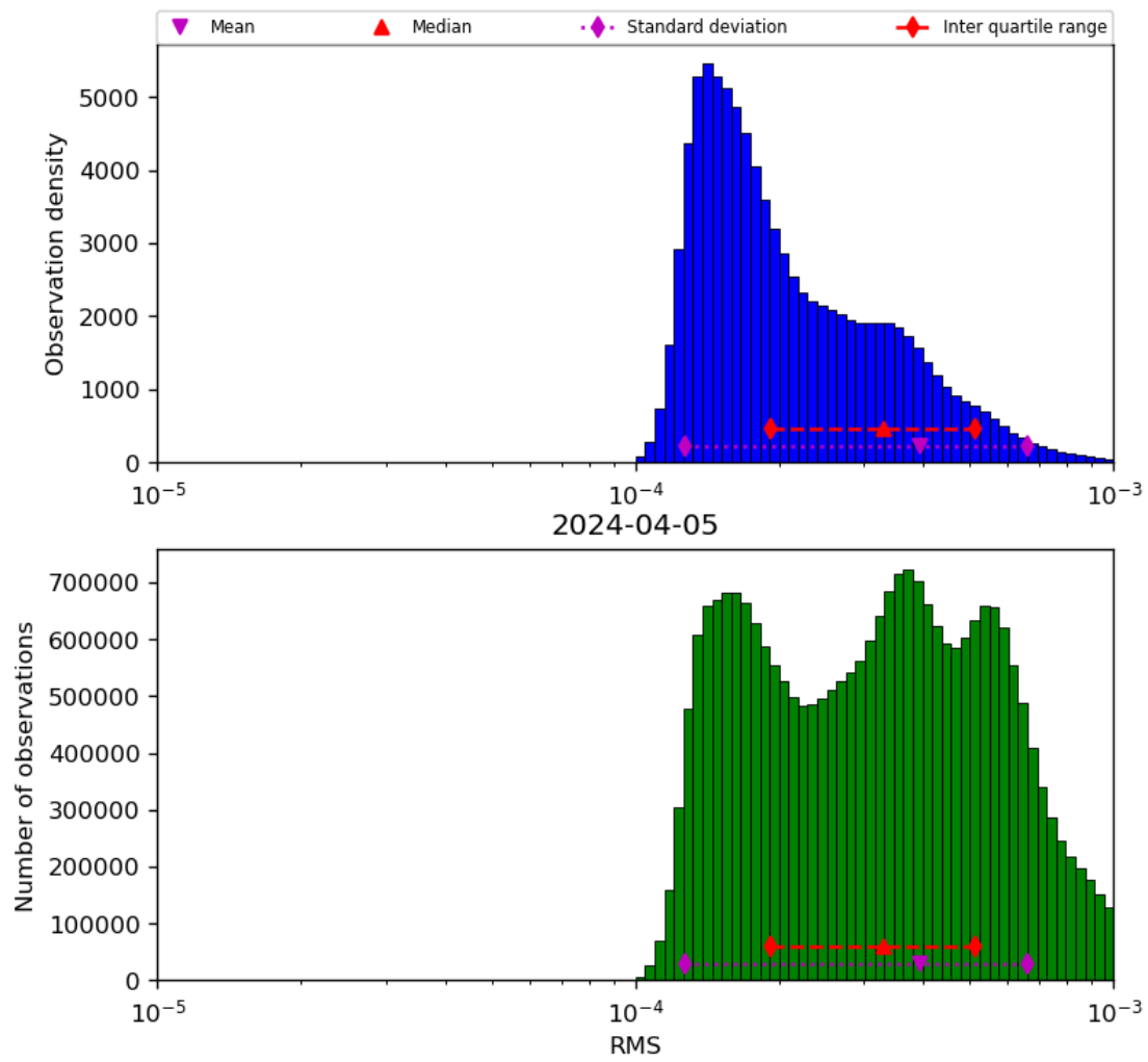
Figure 43: Histogram of “RMS” for 2024-04-05 to 2024-04-06
