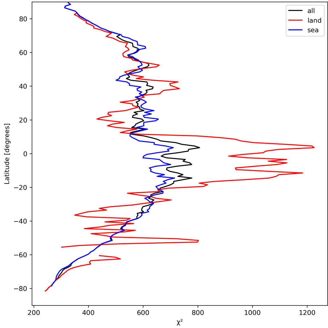
Figure 25: Zonal average of “ \chi^2 ” for 2024-04-05 to 2024-04-06.
