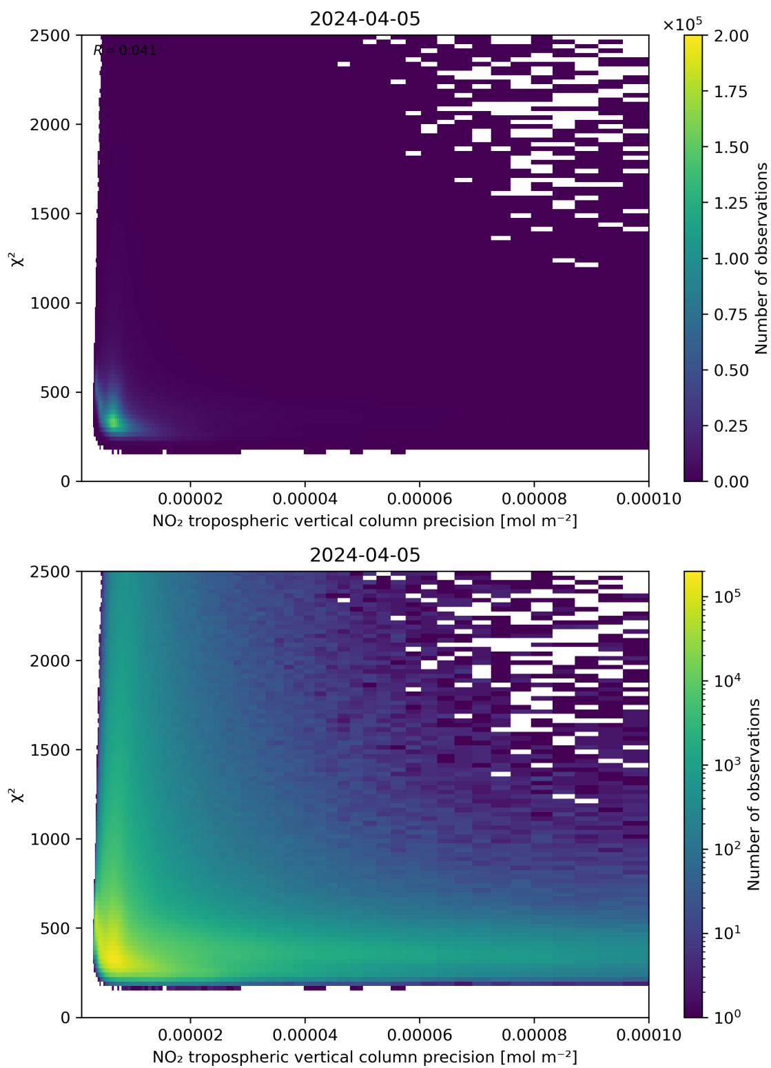
Figure 134: Scatter density plot of “NO 2 tropospheric vertical column precision” against “ \chi^2 ” for 2024-04-05 to 2024-04-06.
