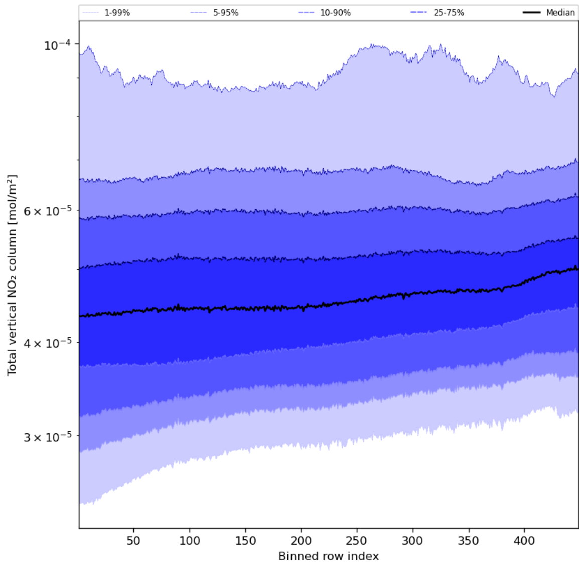
Figure 55: Along track statistics of “Total vertical NO 2 column” for 2024-04-05 to 2024-04-06
