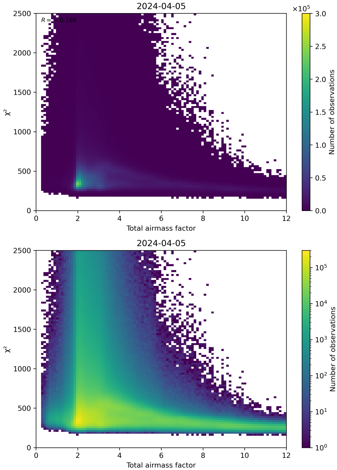
Figure 63: Scatter density plot of “Total airmass factor” against “ \chi^2 ” for 2024-04-05 to 2024-04-06.
