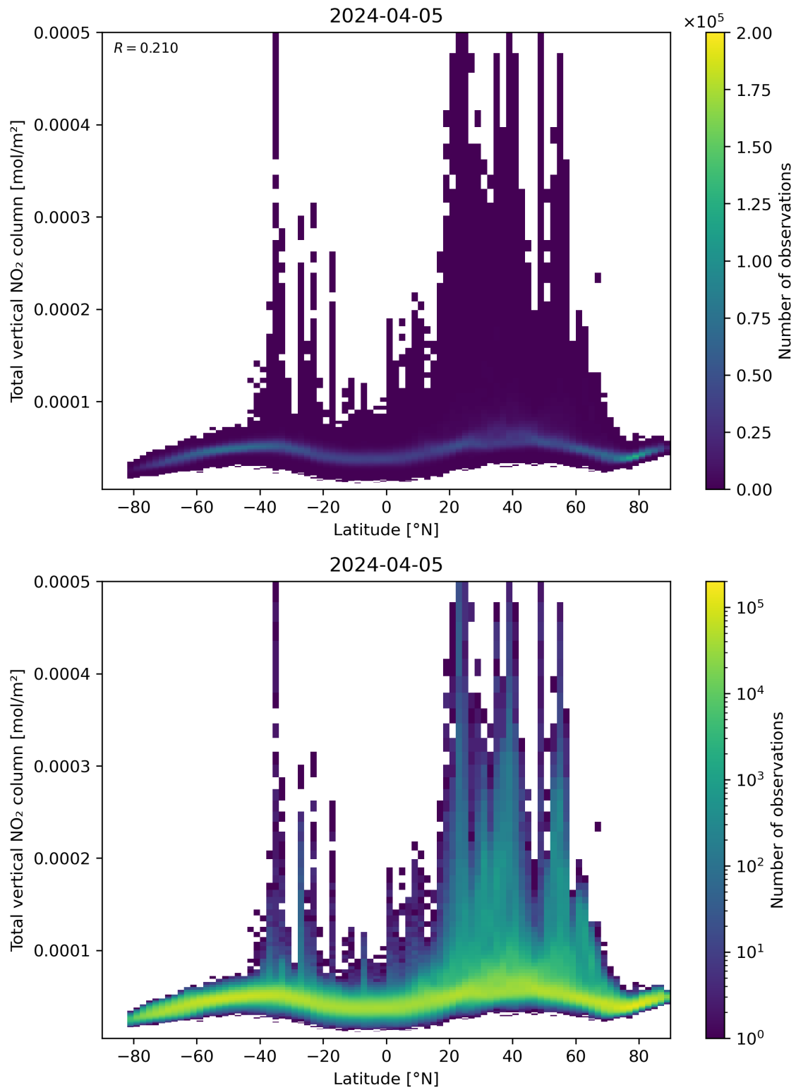
Figure 90: Scatter density plot of “Latitude” against “Total vertical NO 2 column” for 2024-04-05 to 2024-04-06.
