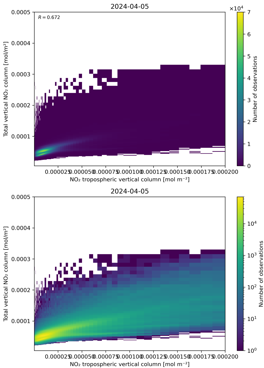
Figure 128: Scatter density plot of “NO 2 tropospheric vertical column” against “Total vertical NO 2 column” for 2024-04-05 to 2024-04-06.
