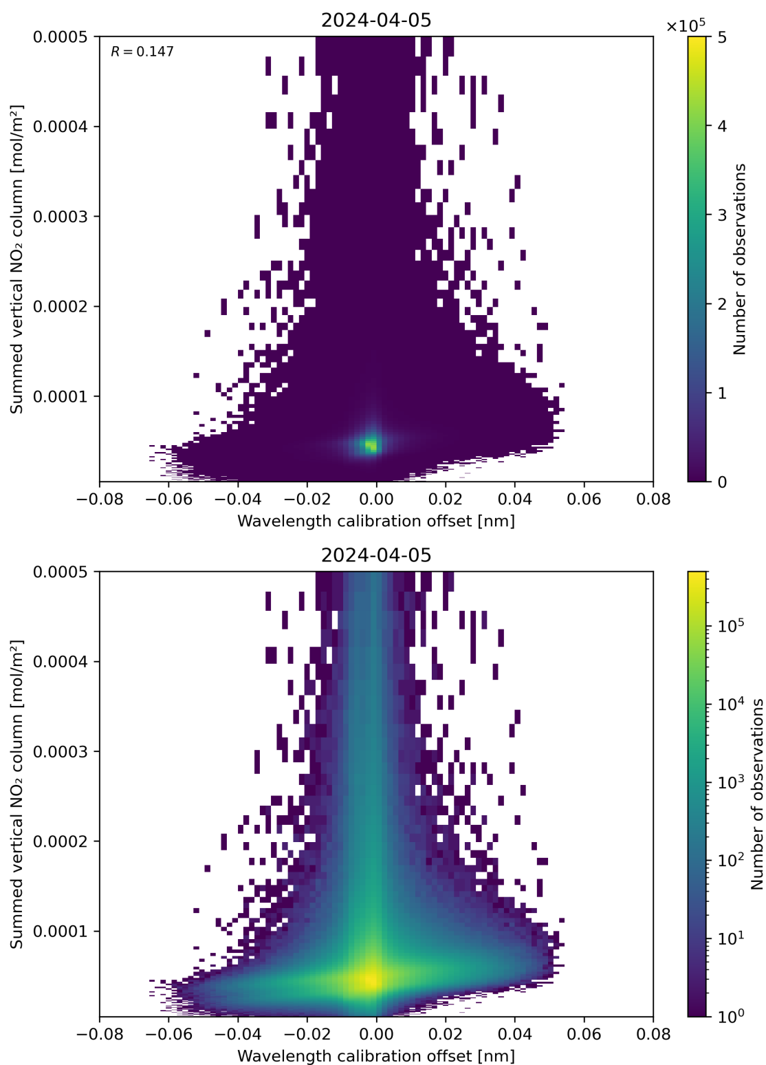
Figure 177: Scatter density plot of “Wavelength calibration offset” against “Summed vertical NO 2 column” for 2024-04-05 to 2024-04-06.
