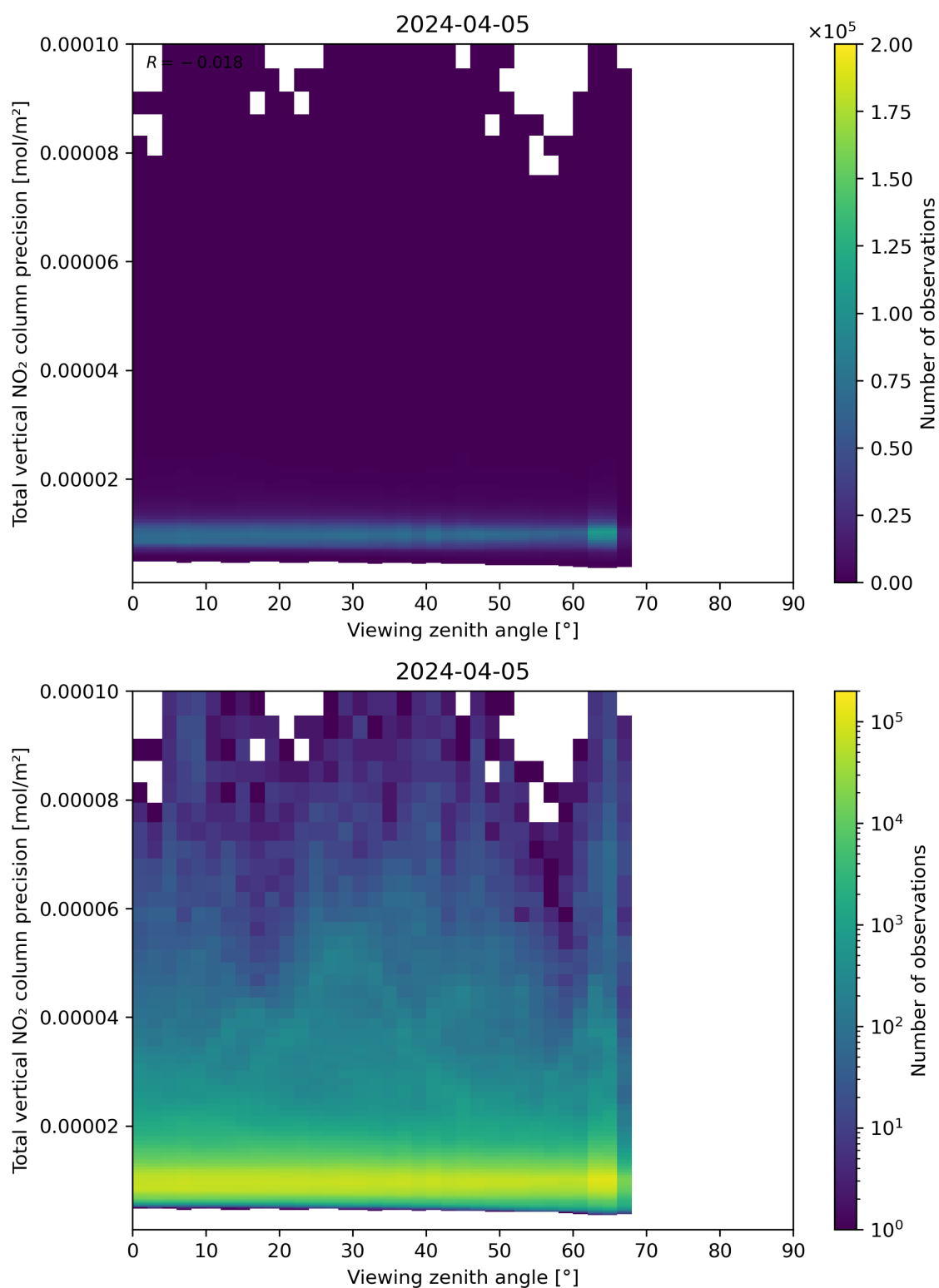
Figure 168: Scatter density plot of “Viewing zenith angle” against “Total vertical NO 2 column precision” for 2024-04-05 to 2024-04-06.
