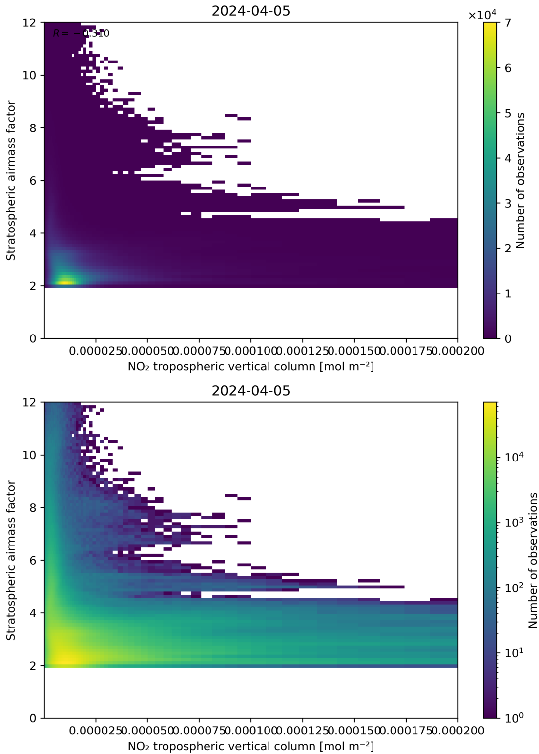
Figure 121: Scatter density plot of “NO 2 tropospheric vertical column” against “Stratospheric air mass factor” for 2024-04-05 to 2024-04-06.
