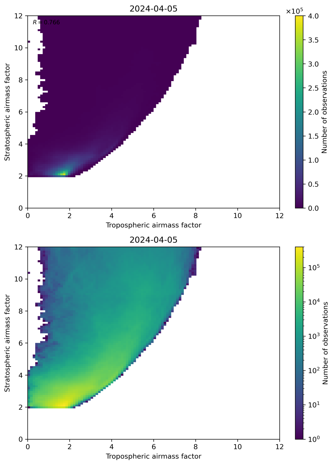
Figure 71: Scatter density plot of “Tropospheric airmass factor” against “Stratospheric airmass factor” for 2024-04-05 to 2024-04-06.
