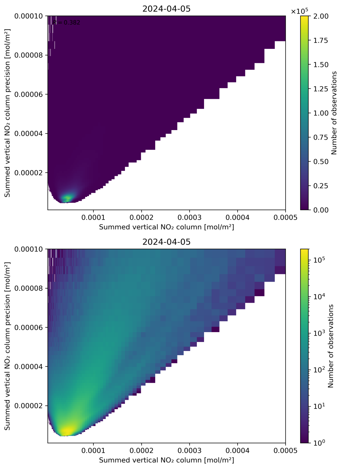
Figure 105: Scatter density plot of “Summed vertical NO 2 column” against “Summed vertical NO 2 column precision” for 2024-04-05 to 2024-04-06.
