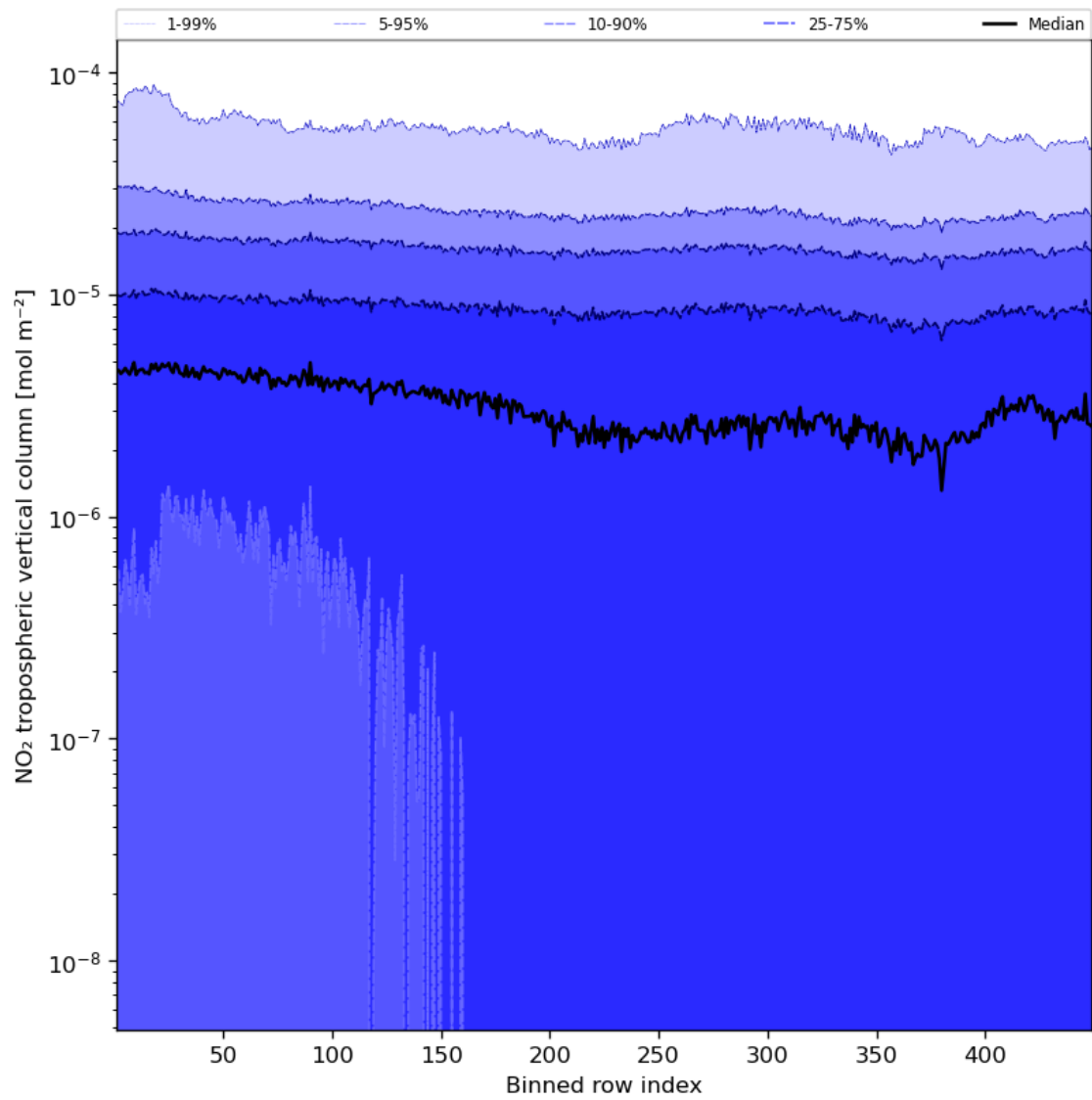
Figure 46: Along track statistics of “NO 2 tropospheric vertical column” for 2024-04-05 to 2024-04-06
