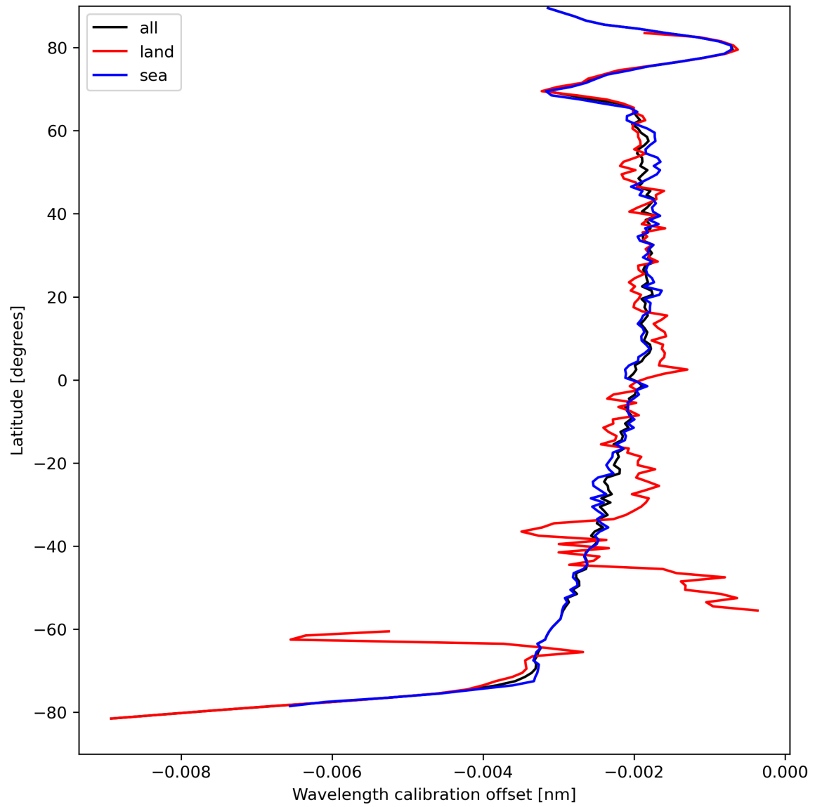
Figure 18: Zonal average of “Wavelength calibration offset” for 2024-04-05 to 2024-04-06.
