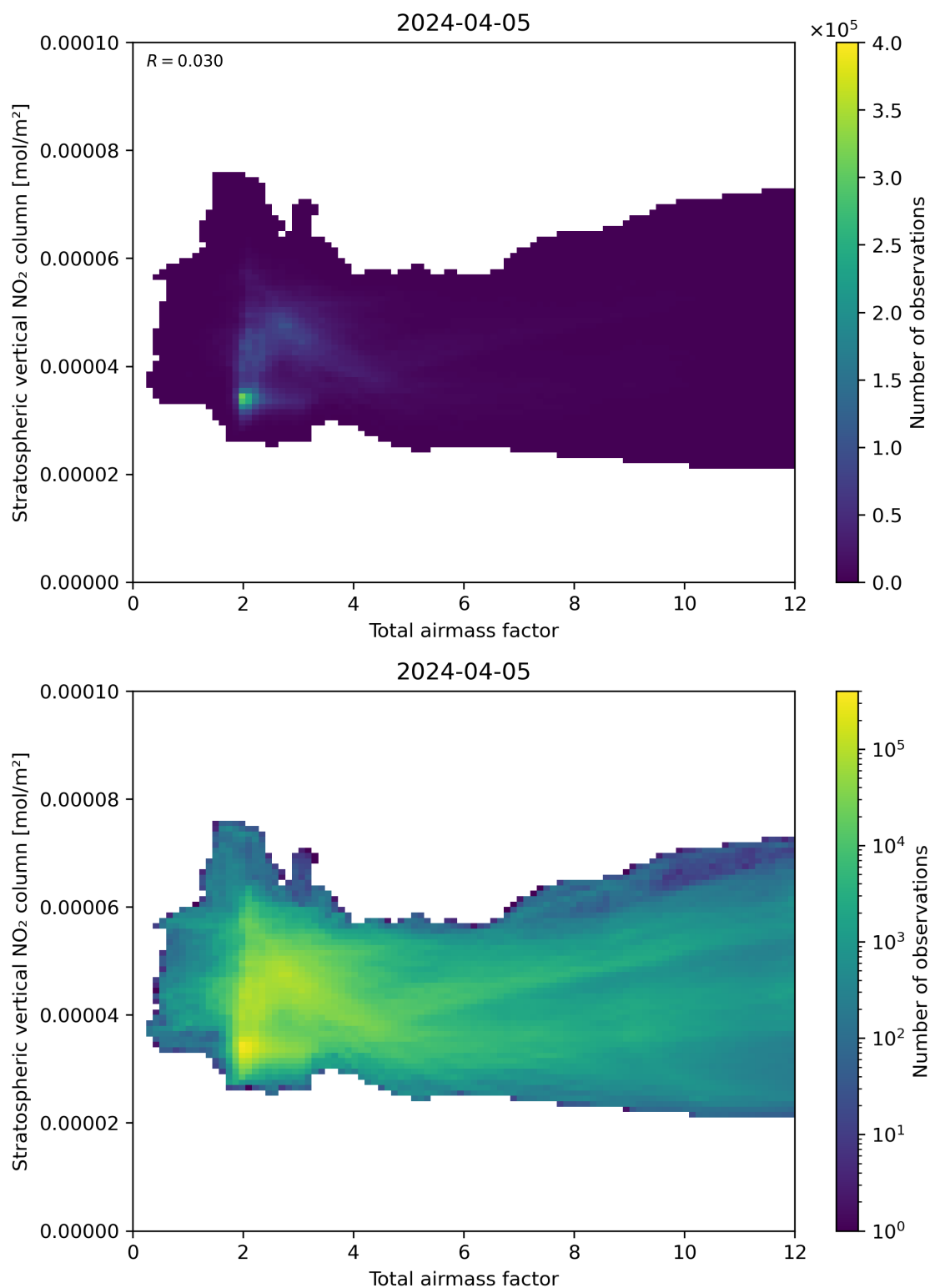
Figure 64: Scatter density plot of “Total airmass factor” against “Stratospheric vertical \text{NO}_2 column” for 2024-04-05 to 2024-04-06.
