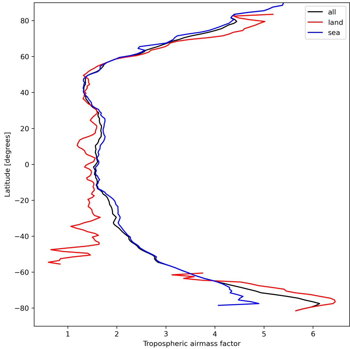
Figure 14: Zonal average of “Tropospheric airmass factor” for 2024-04-05 to 2024-04-06.
