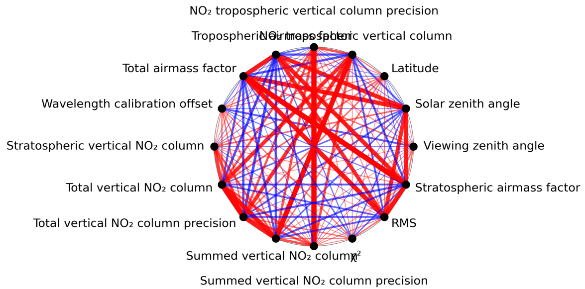
Figure 1: Map of correlation graph for 2024-04-05 to 2024-04-06.
