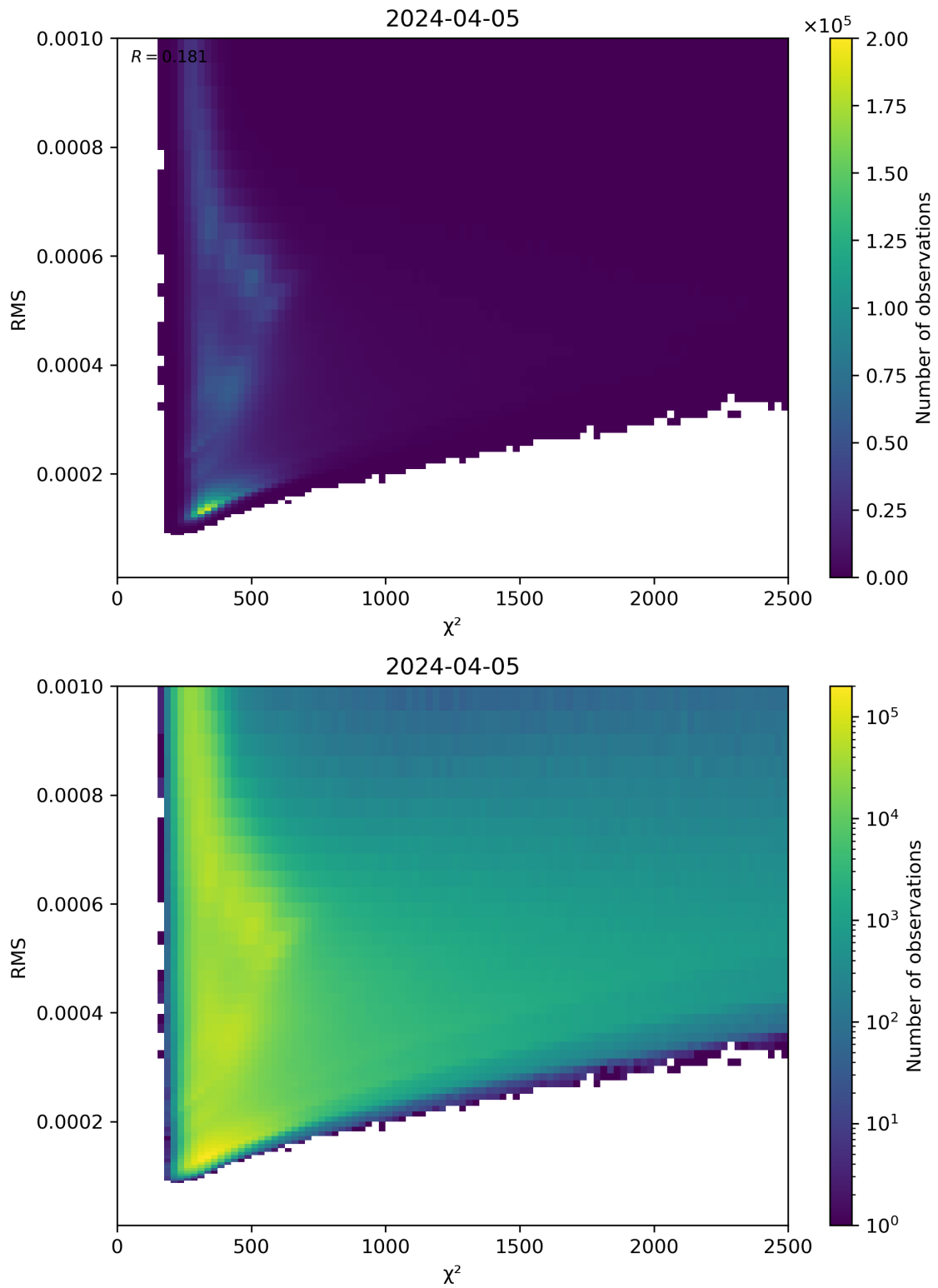
Figure 82: Scatter density plot of “ \chi^2 ” against “RMS” for 2024-04-05 to 2024-04-06.
