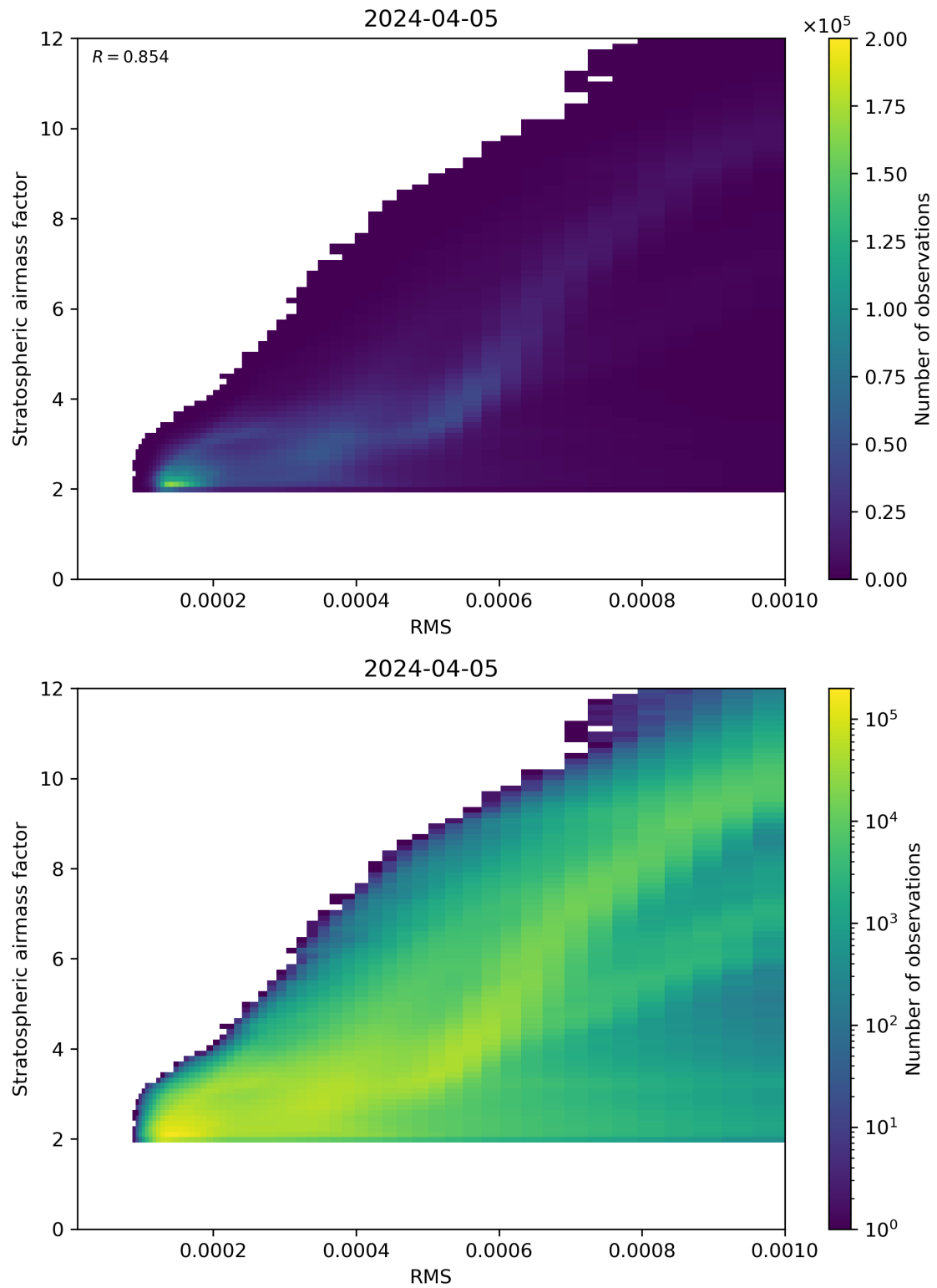
Figure 144: Scatter density plot of “RMS” against “Stratospheric airmass factor” for 2024-04-05 to 2024-04-06.
