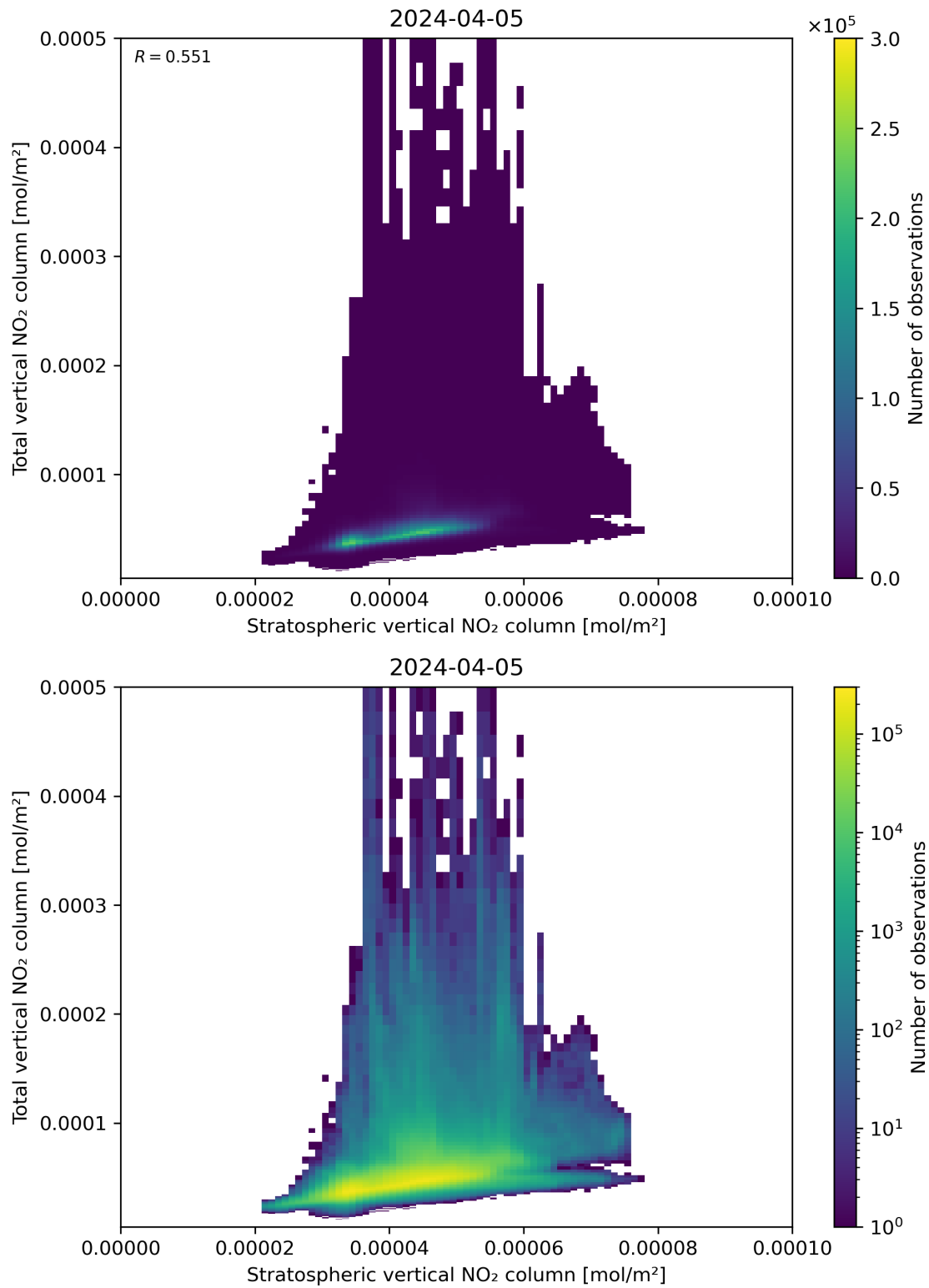
Figure 100: Scatter density plot of “Stratospheric vertical NO 2 column” against “Total vertical NO 2 column” for 2024-04-05 to 2024-04-06.
