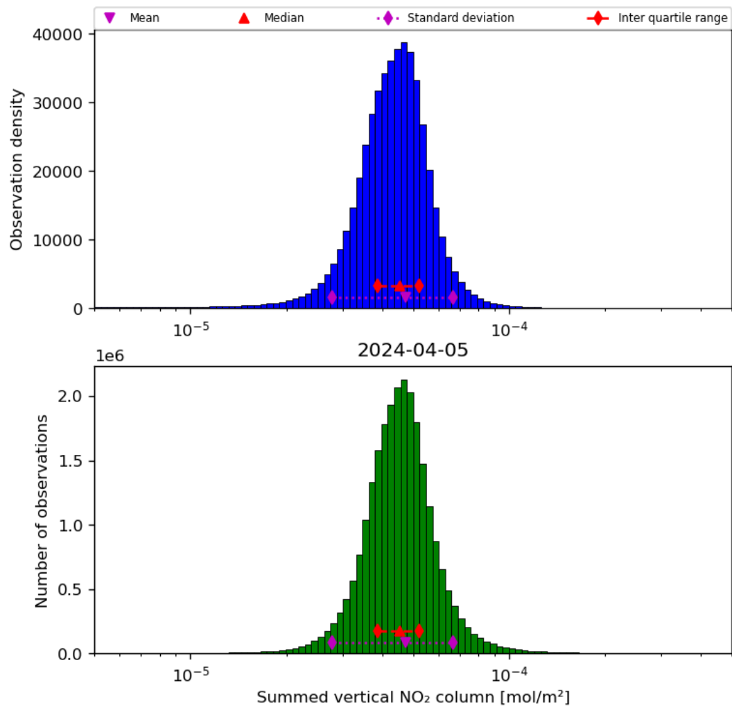
Figure 40: Histogram of “Summed vertical NO 2 column” for 2024-04-05 to 2024-04-06
