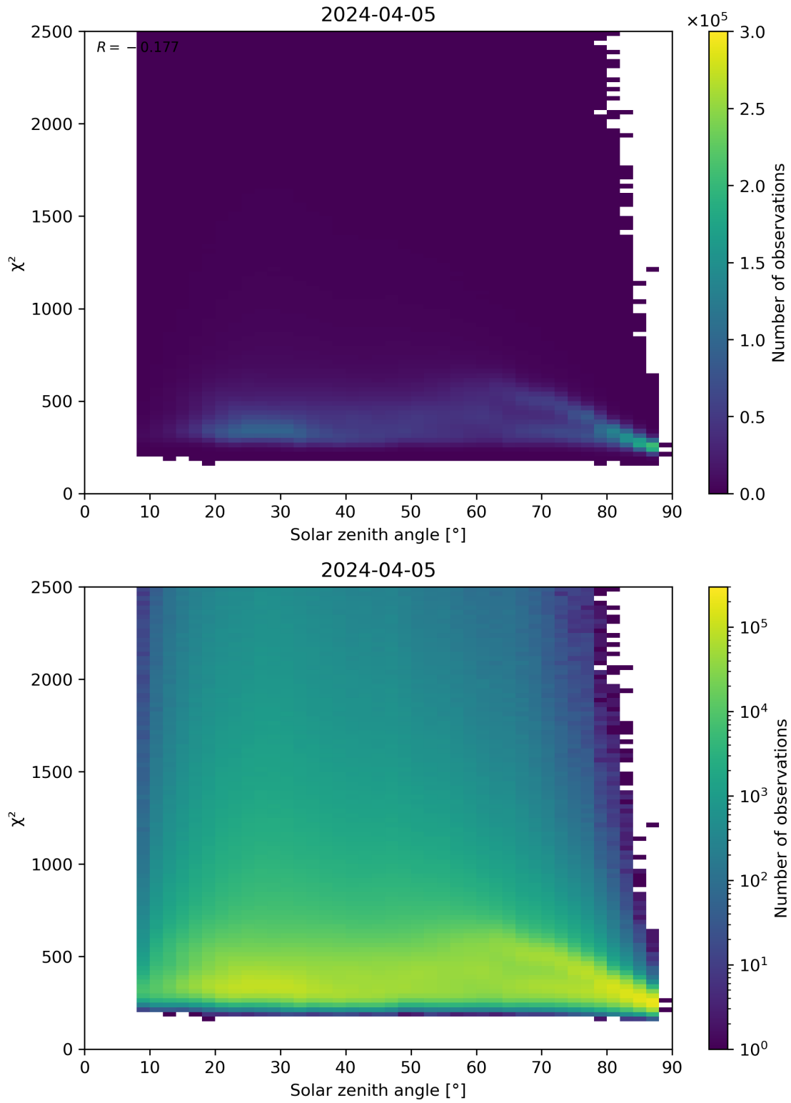
Figure 148: Scatter density plot of “Solar zenith angle” against “ \chi^2 ” for 2024-04-05 to 2024-04-06.
