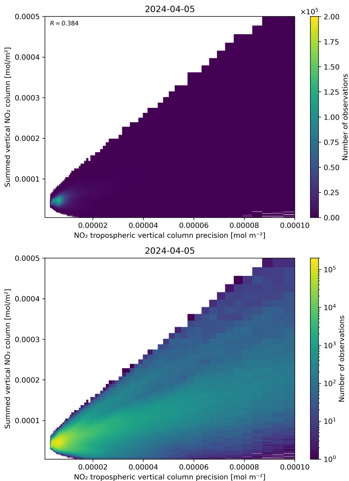
Figure 136: Scatter density plot of “NO 2 tropospheric vertical column precision” against “Summed vertical NO 2 column” for 2024-04-05 to 2024-04-06.
