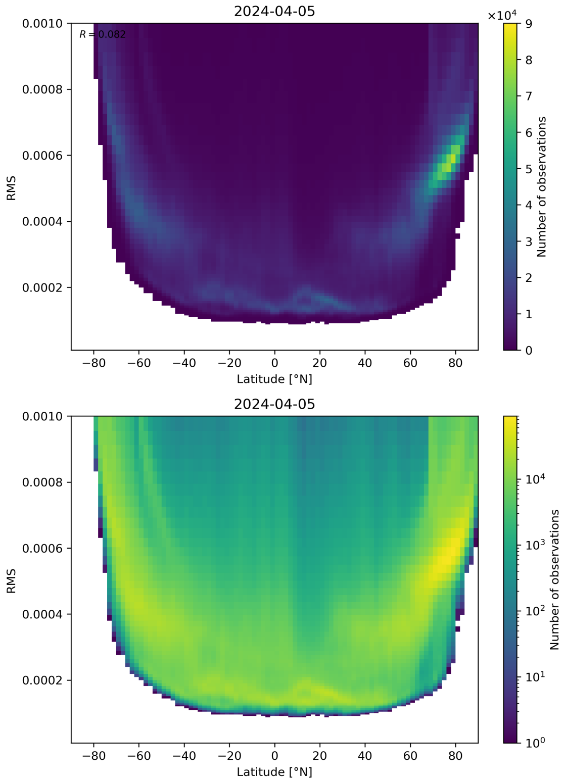
Figure 94: Scatter density plot of “Latitude” against “RMS” for 2024-04-05 to 2024-04-06.
