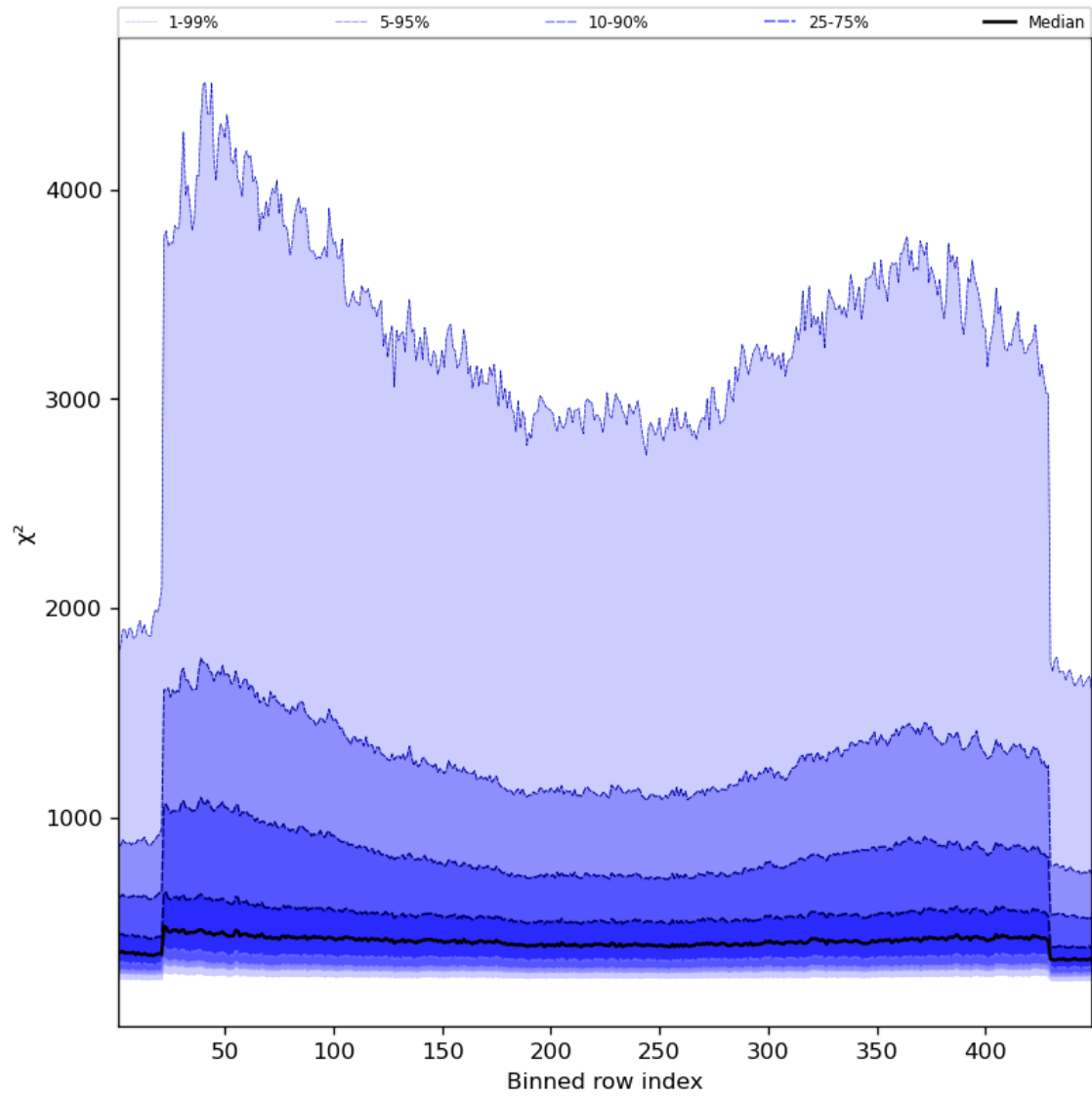
Figure 59: Along track statistics of “ \chi^2 ” for 2024-04-05 to 2024-04-06
