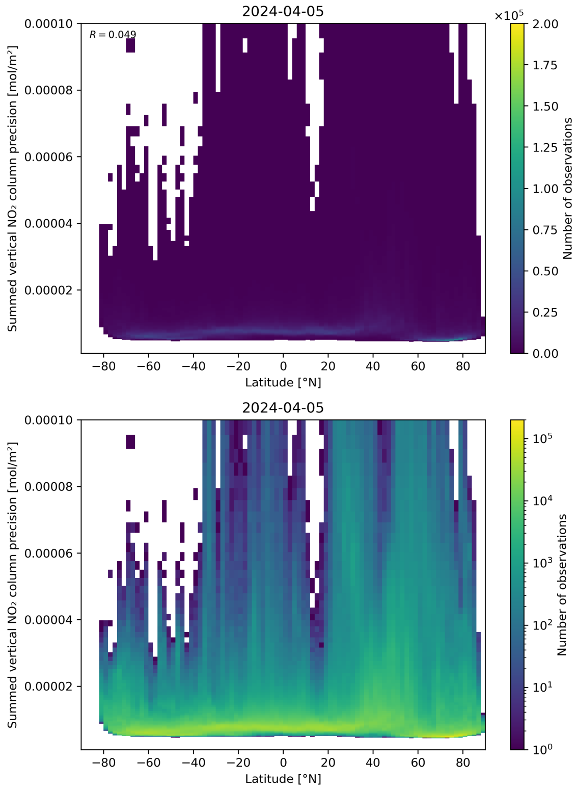
Figure 89: Scatter density plot of “Latitude” against “Summed vertical NO 2 column precision” for 2024-04-05 to 2024-04-06.
