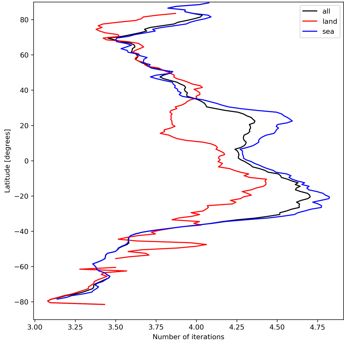
Figure 17: Zonal average of “Number of iterations” for 2024-04-05 to 2024-04-06.
