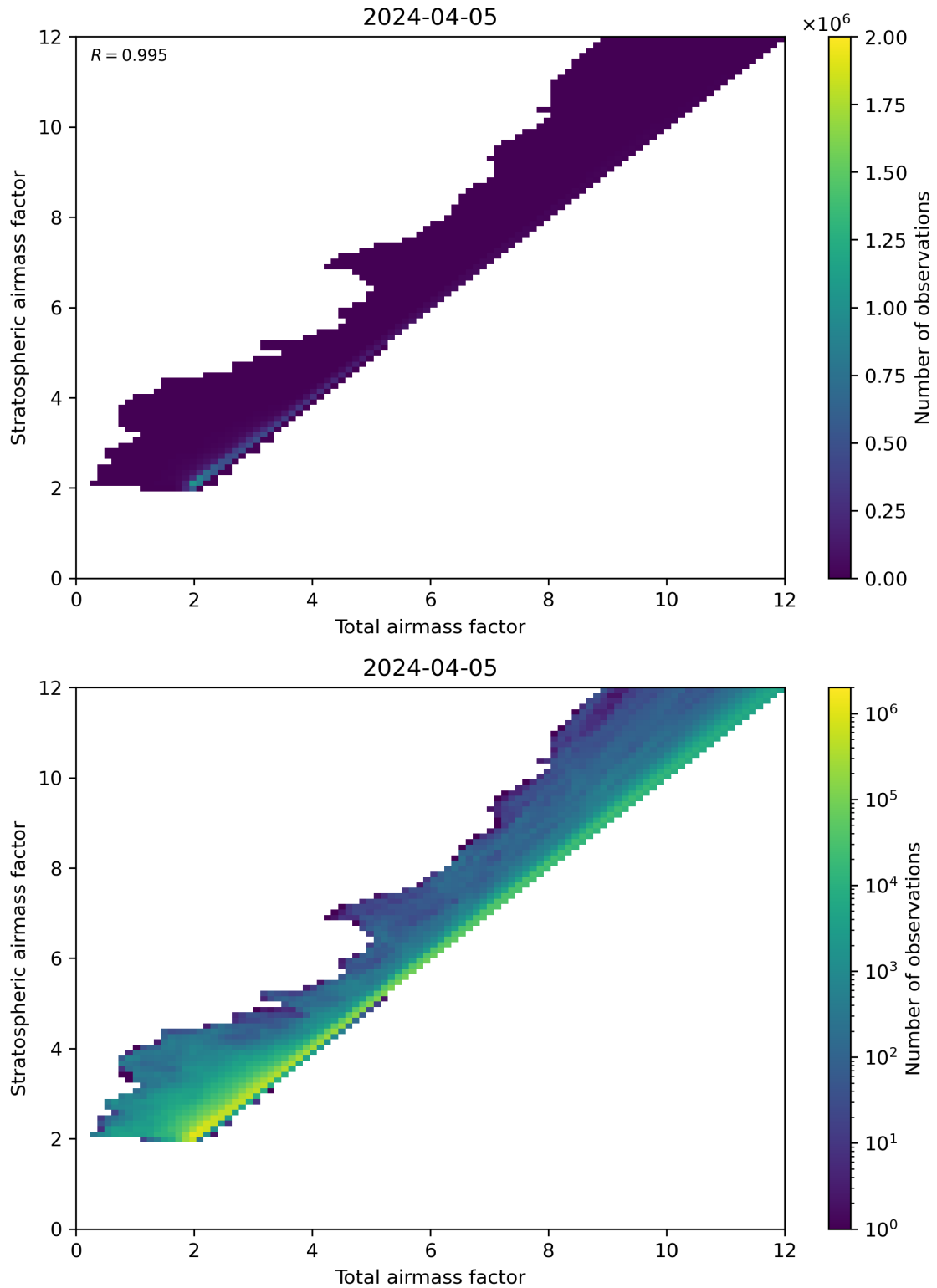
Figure 62: Scatter density plot of “Total airmass factor” against “Stratospheric airmass factor” for 2024-04-05 to 2024-04-06.
