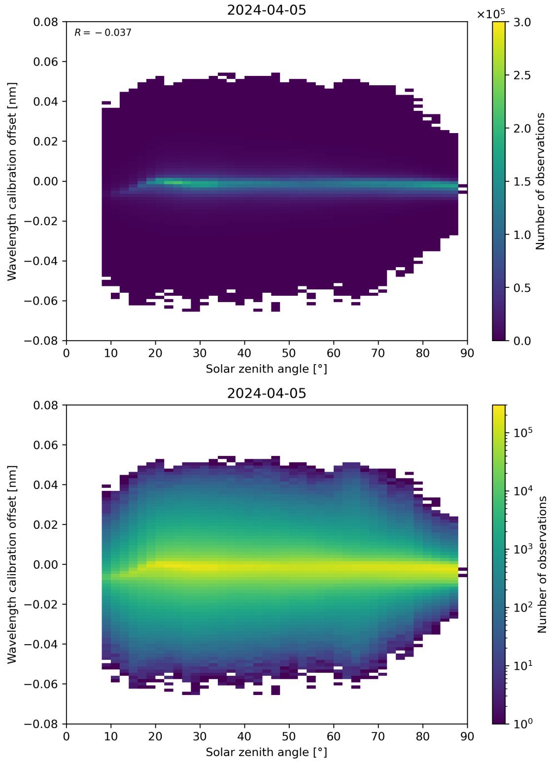
Figure 158: Scatter density plot of “Solar zenith angle” against “Wavelength calibration offset” for 2024-04-05 to 2024-04-06.
