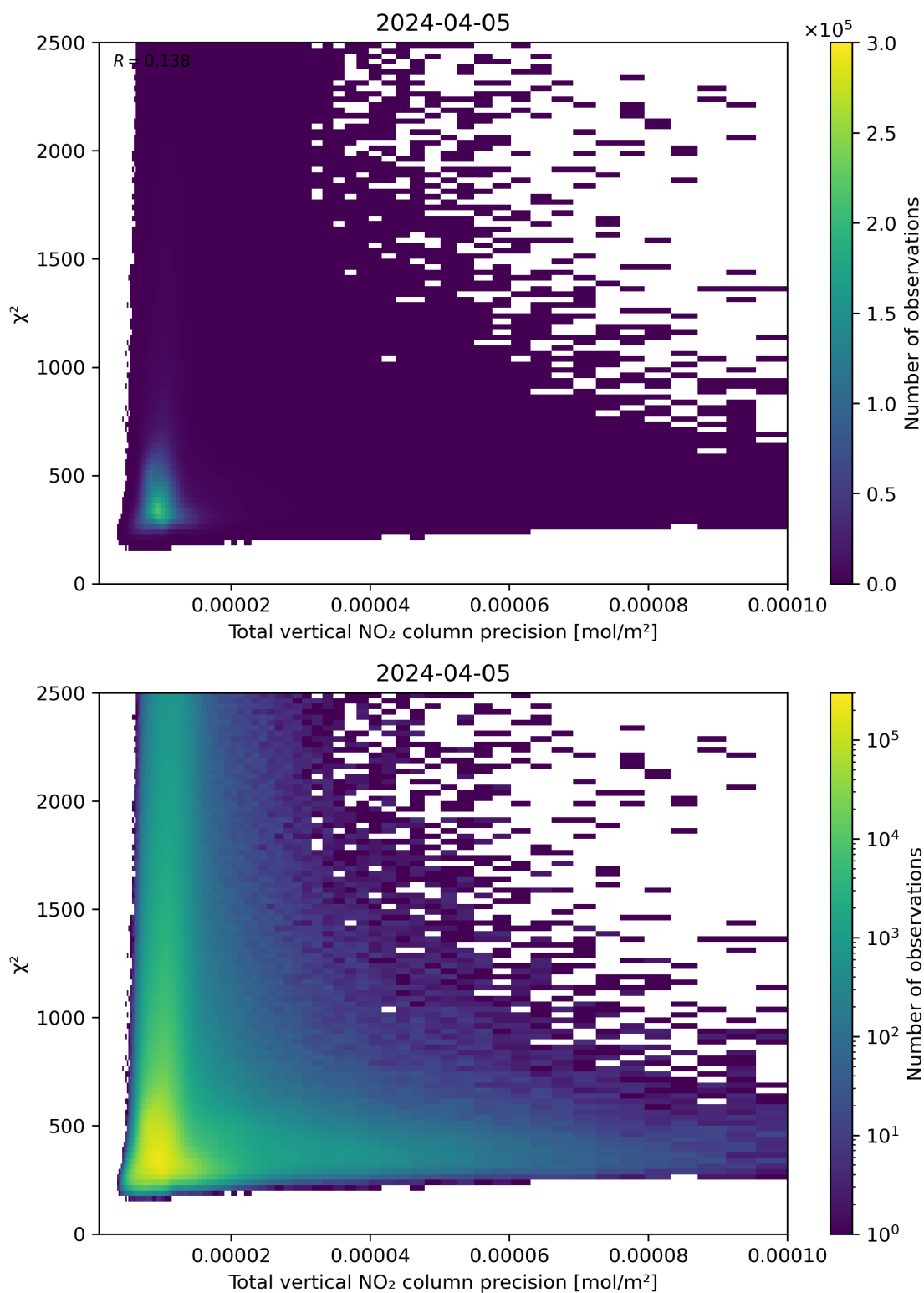
Figure 116: Scatter density plot of “Total vertical NO 2 column precision” against “ \chi^2 ” for 2024-04-05 to 2024-04-06.
