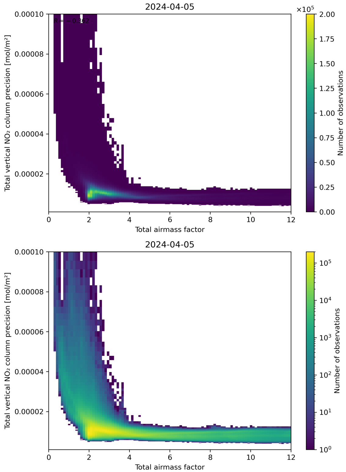
Figure 68: Scatter density plot of “Total airmass factor” against “Total vertical NO 2 column precision” for 2024-04-05 to 2024-04-06.
