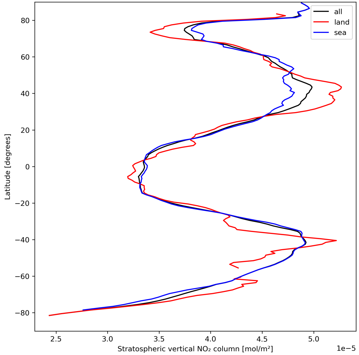
Figure 19: Zonal average of “Stratospheric vertical NO 2 column” for 2024-04-05 to 2024-04-06.
