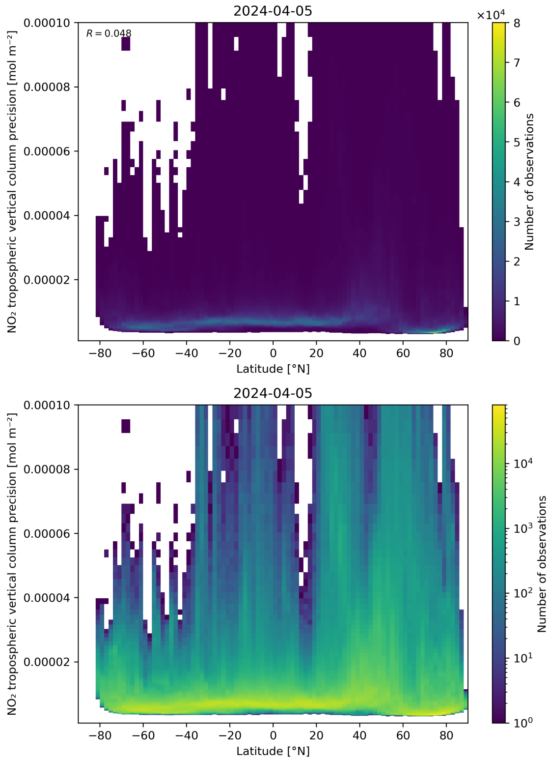
Figure 93: Scatter density plot of “Latitude” against “NO 2 tropospheric vertical column precision” for 2024-04-05 to 2024-04-06.
