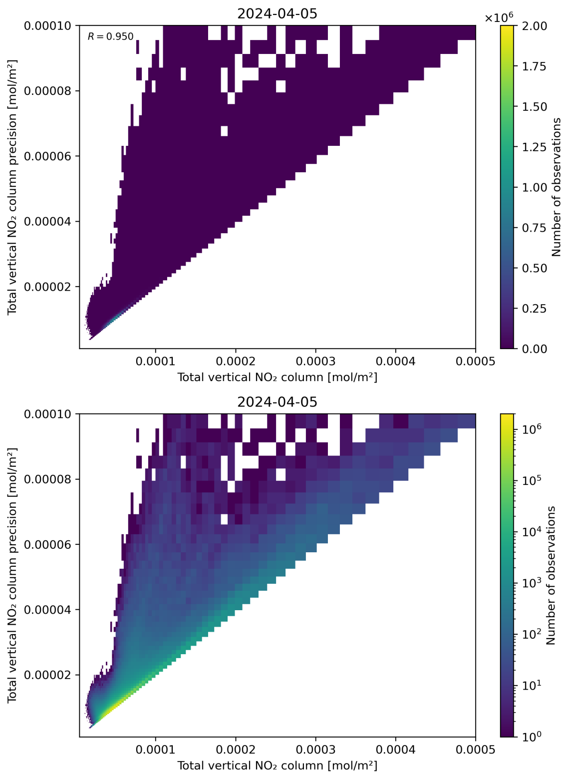
Figure 114: Scatter density plot of “Total vertical NO 2 column” against “Total vertical NO 2 column precision” for 2024-04-05 to 2024-04-06.
