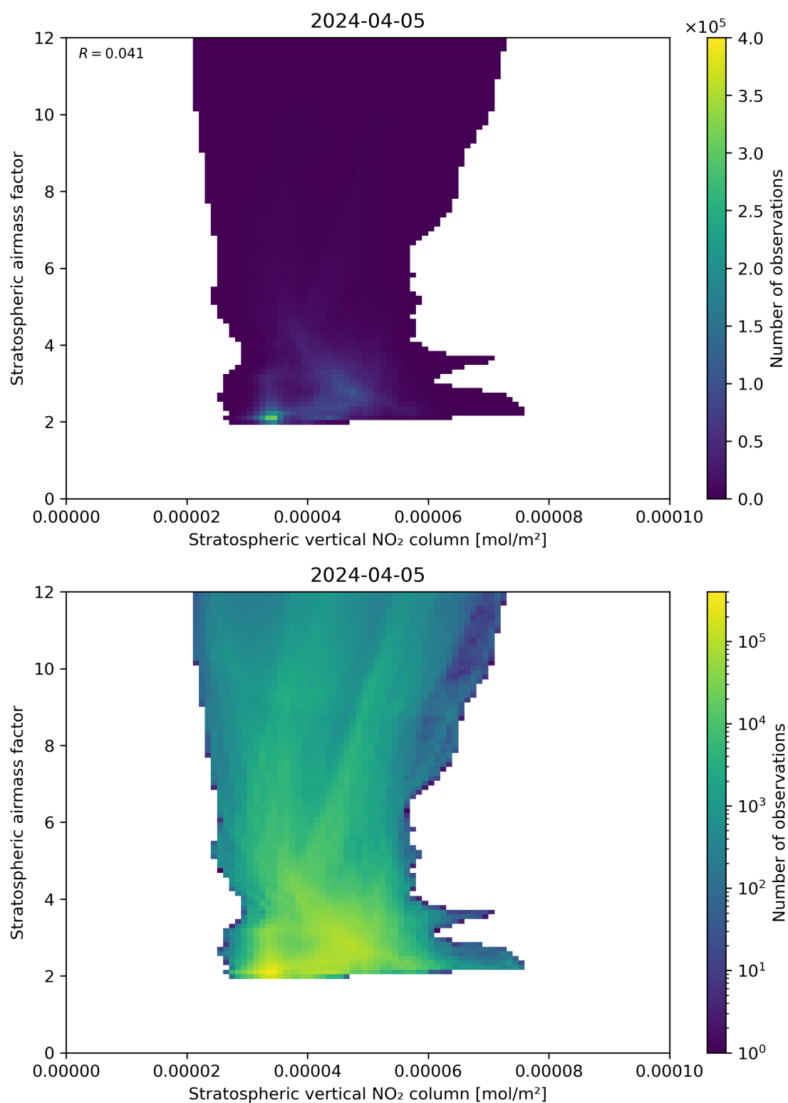
Figure 96: Scatter density plot of “Stratospheric vertical NO 2 column” against “Stratospheric airmass factor” for 2024-04-05 to 2024-04-06.
