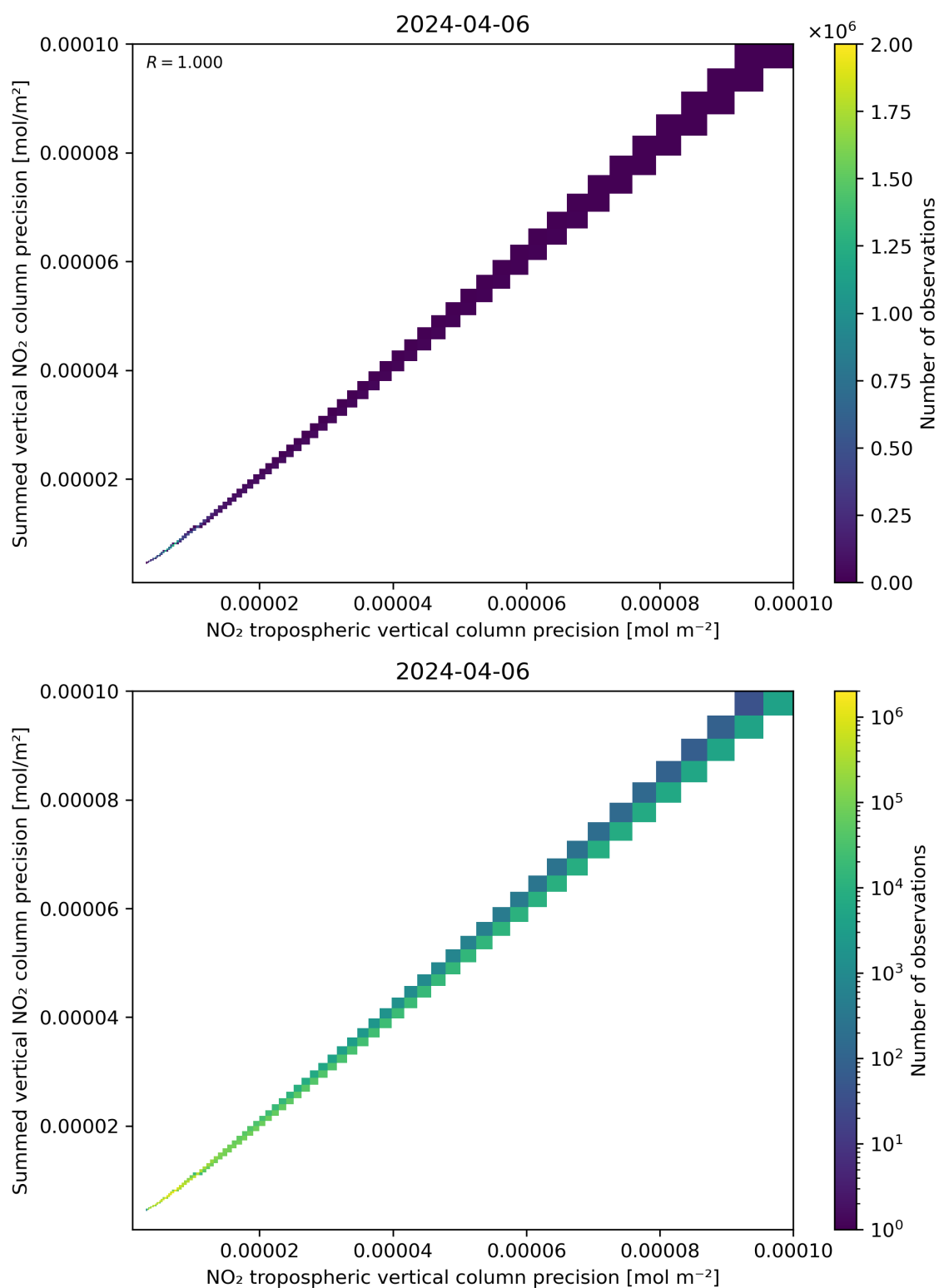
Figure 137: Scatter density plot of “NO 2 tropospheric vertical column precision” against “Summed vertical NO 2 column precision” for 2024-04-05 to 2024-04-07.
