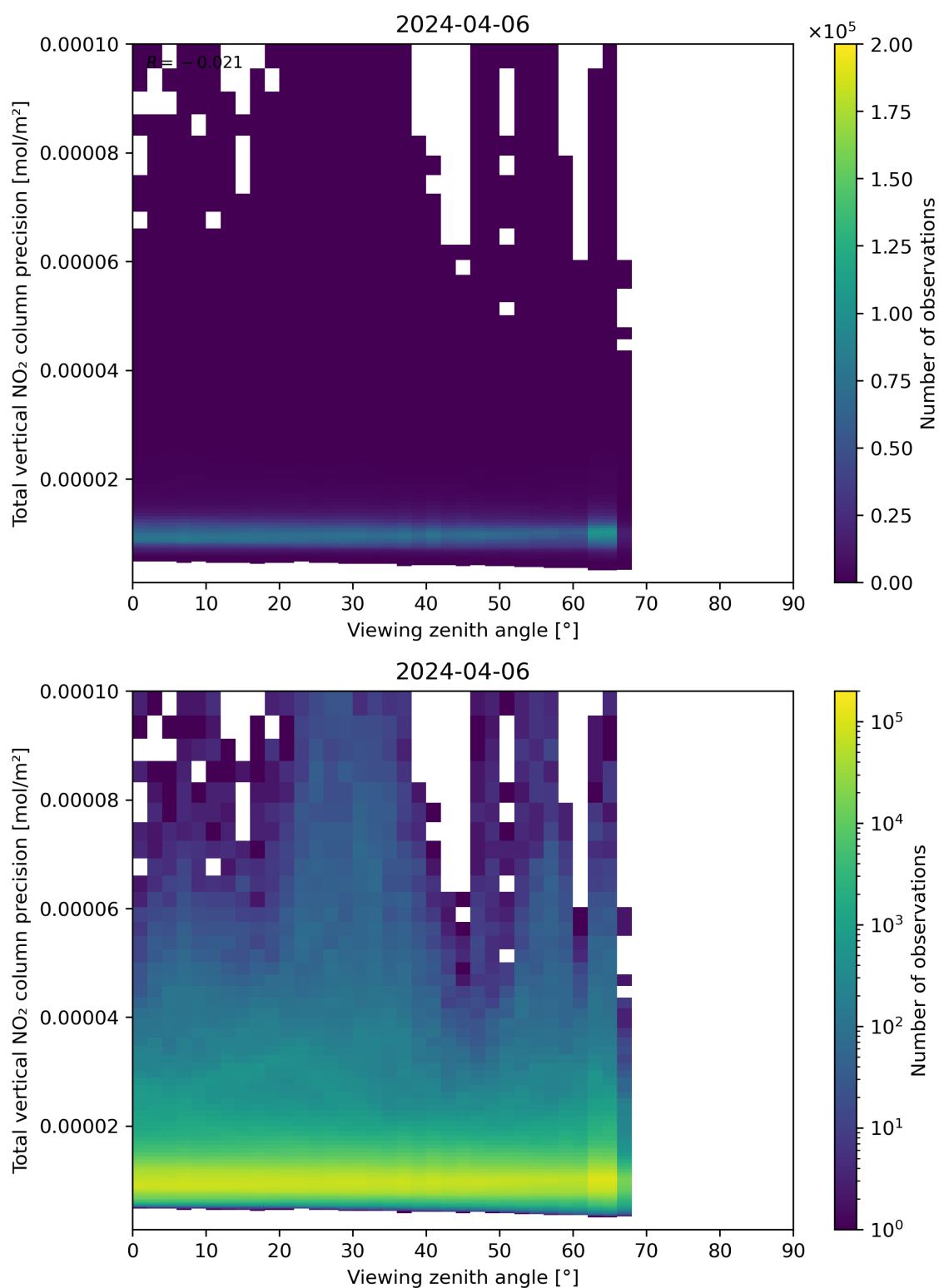
Figure 168: Scatter density plot of “Viewing zenith angle” against “Total vertical NO 2 column precision” for 2024-04-05 to 2024-04-07.
