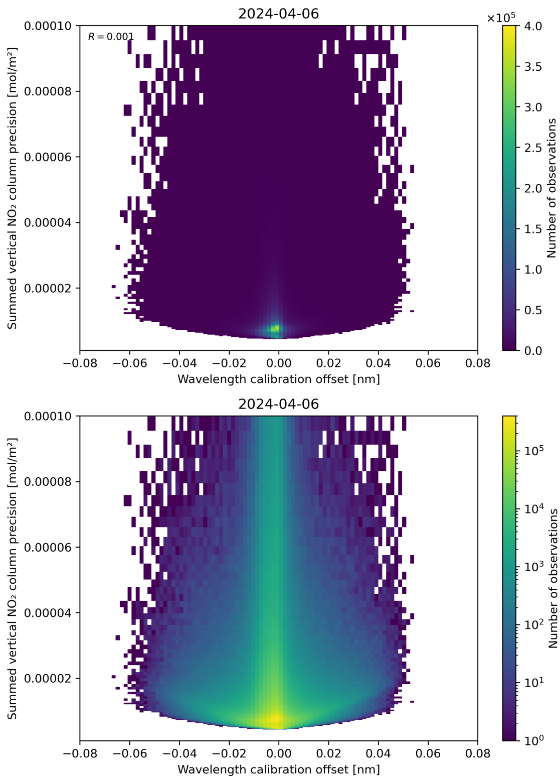
Figure 178: Scatter density plot of “Wavelength calibration offset” against “Summed vertical NO 2 column precision” for 2024-04-05 to 2024-04-07.
