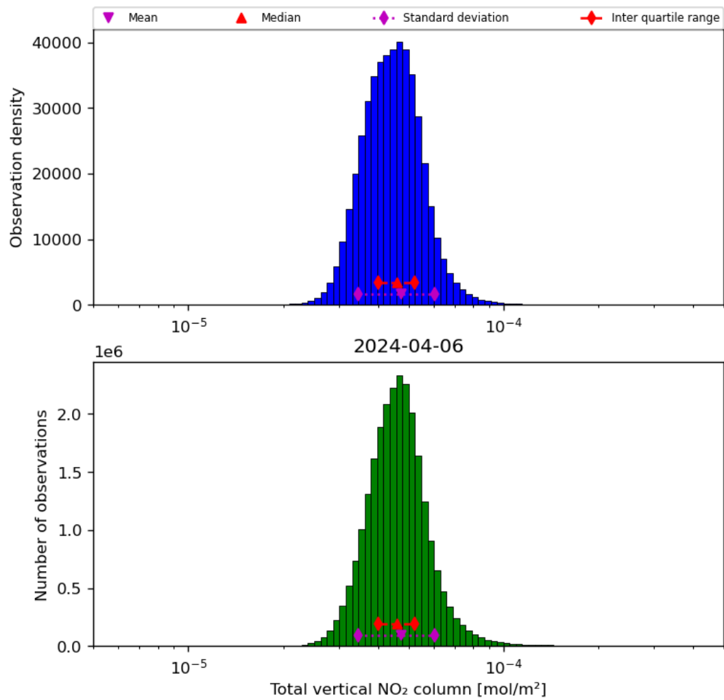
Figure 38: Histogram of “Total vertical NO 2 column” for 2024-04-05 to 2024-04-07
