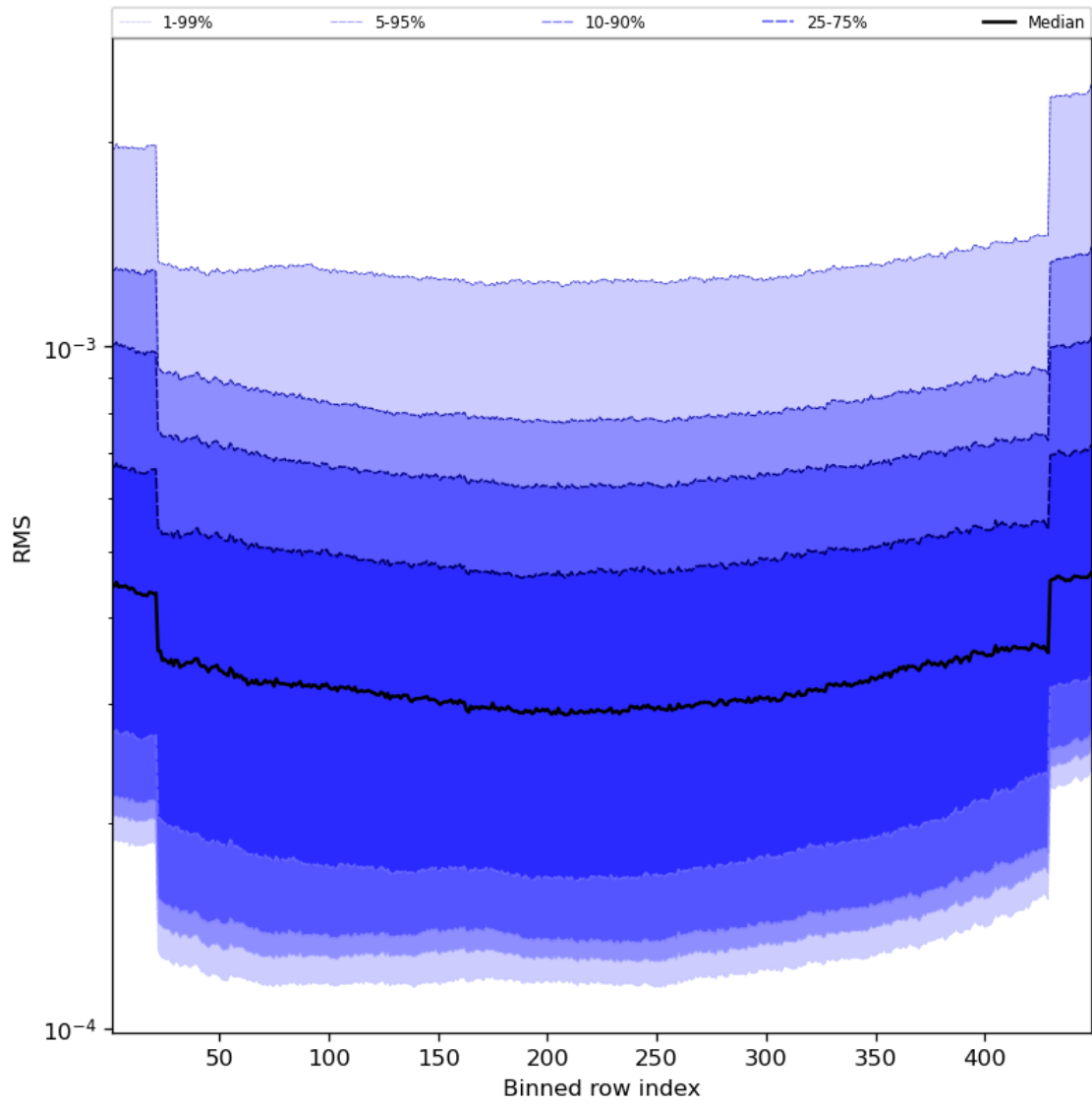
Figure 60: Along track statistics of “RMS” for 2024-04-05 to 2024-04-07
