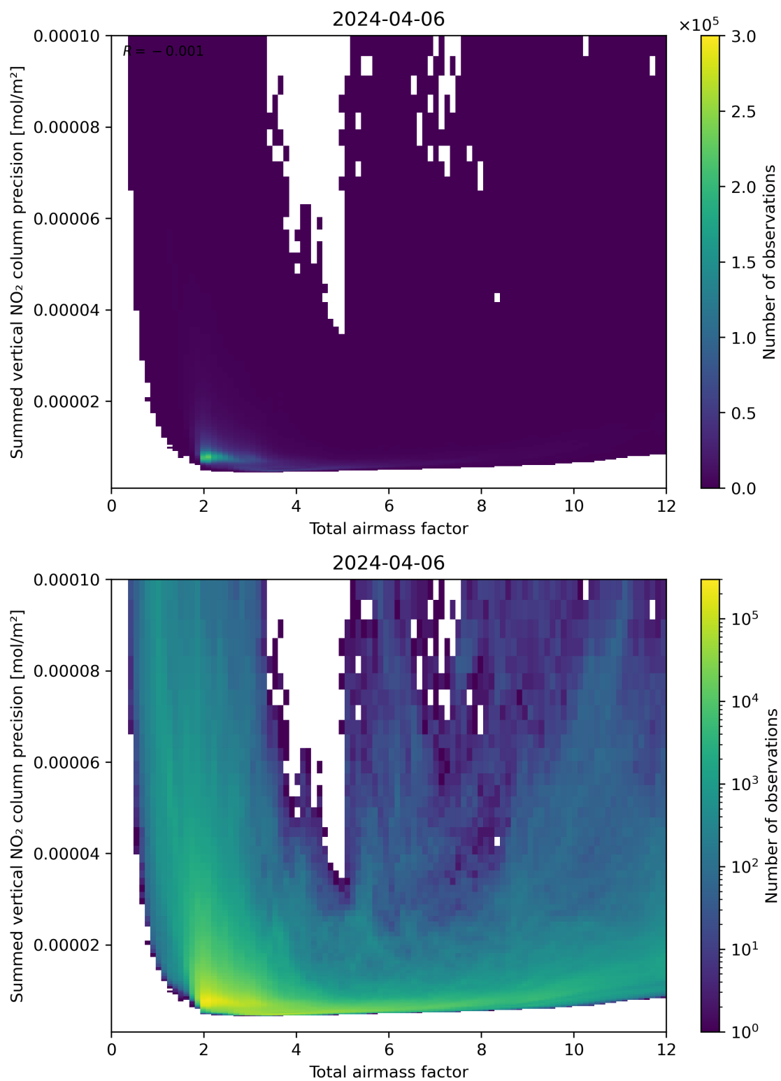
Figure 66: Scatter density plot of “Total airmass factor” against “Summed vertical NO 2 column precision” for 2024-04-05 to 2024-04-07.
