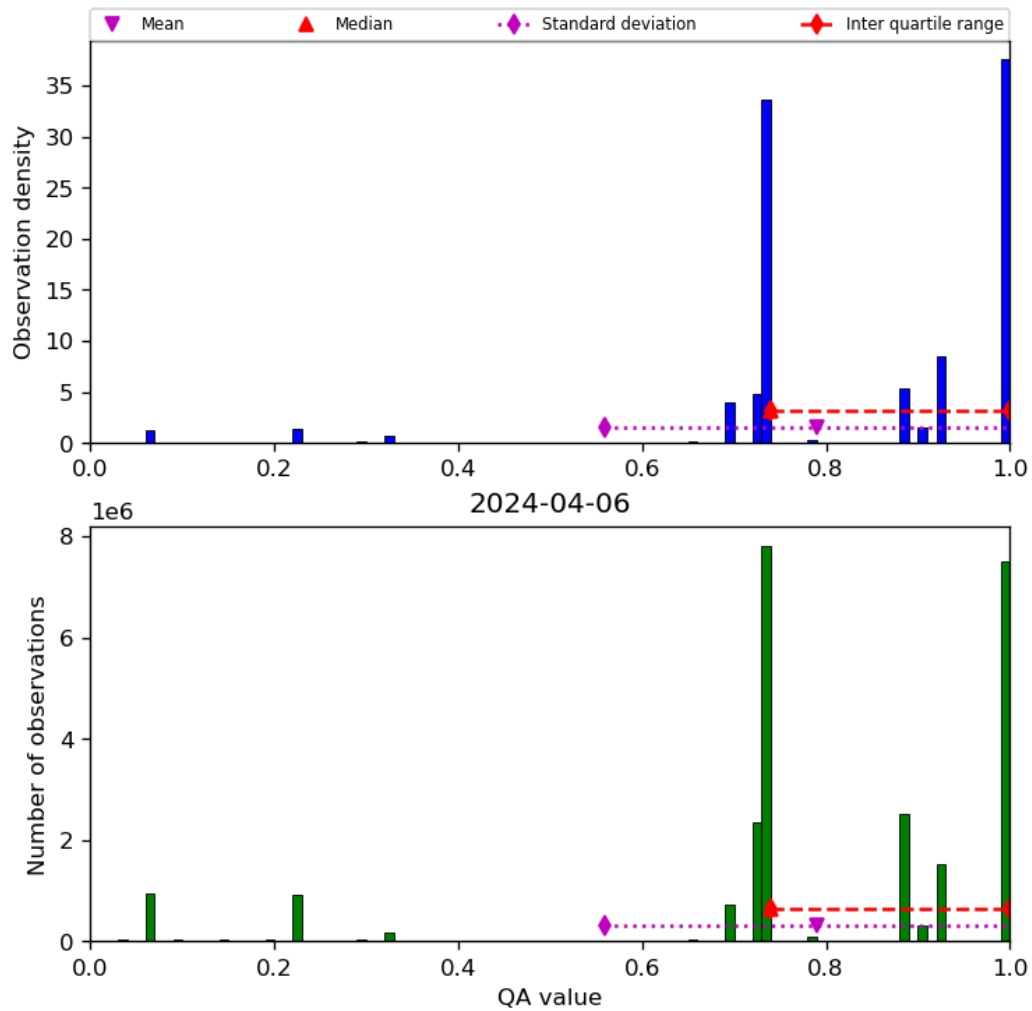
Figure 28: Histogram of “QA value” for 2024-04-05 to 2024-04-07
