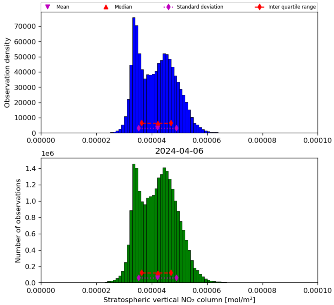
Figure 36: Histogram of “Stratospheric vertical NO 2 column” for 2024-04-05 to 2024-04-07
