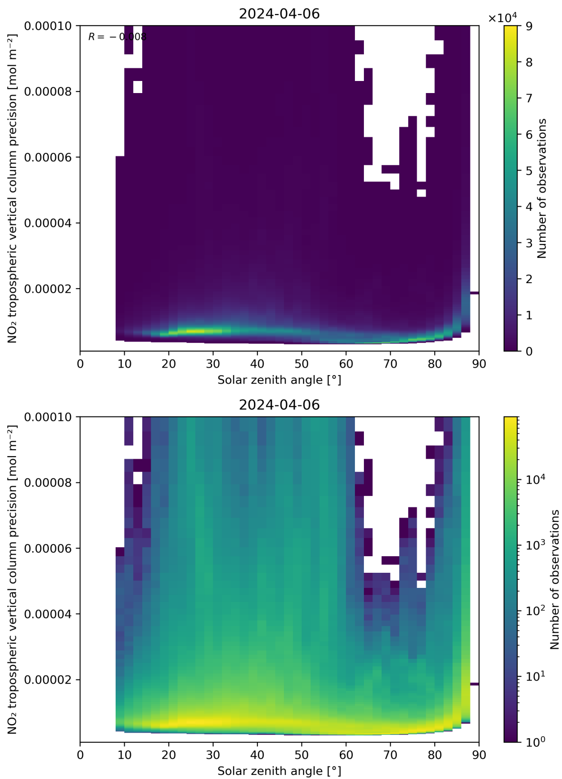
Figure 156: Scatter density plot of “Solar zenith angle” against “NO 2 tropospheric vertical column precision” for 2024-04-05 to 2024-04-07.
