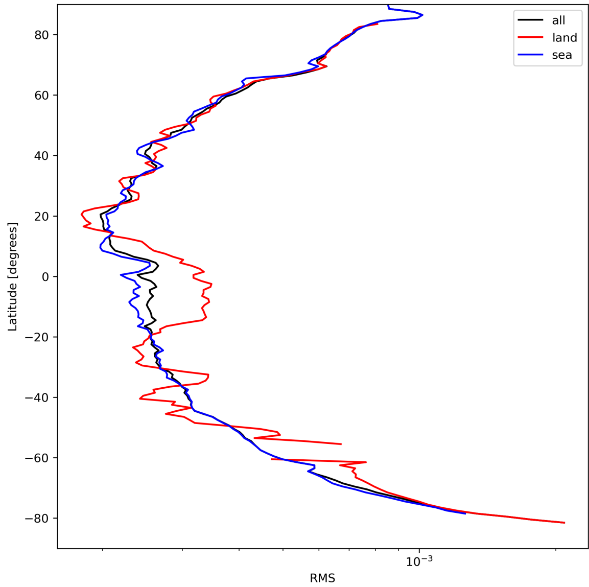
Figure 26: Zonal average of “RMS” for 2024-04-05 to 2024-04-07.
