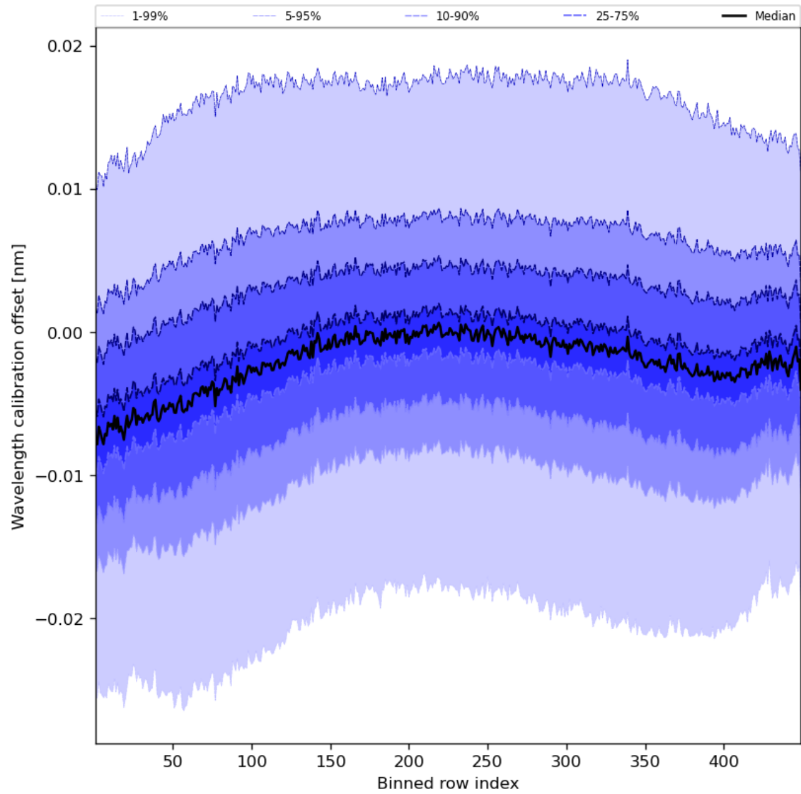
Figure 52: Along track statistics of “Wavelength calibration offset” for 2024-04-05 to 2024-04-07
