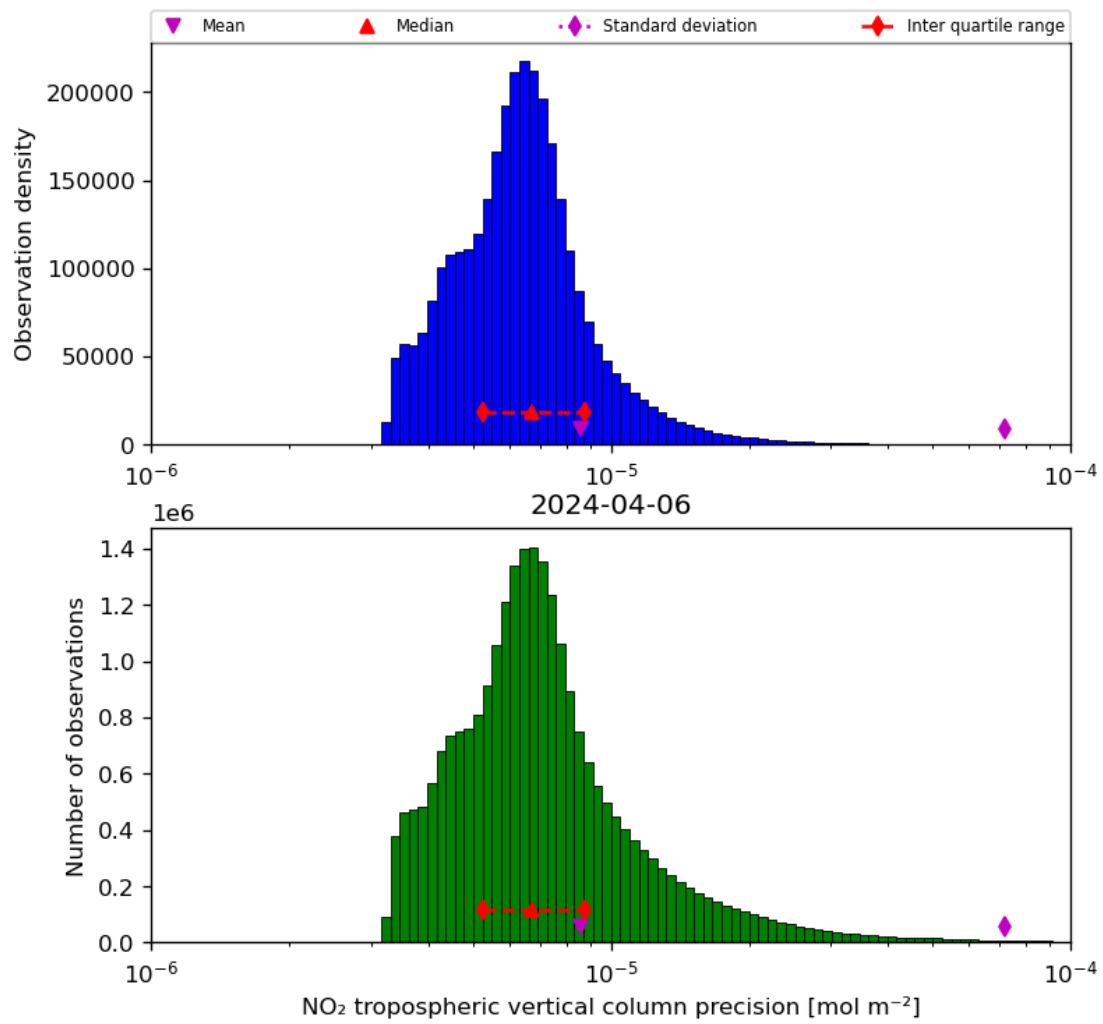
Figure 30: Histogram of “NO 2 tropospheric vertical column precision” for 2024-04-05 to 2024-04-07
