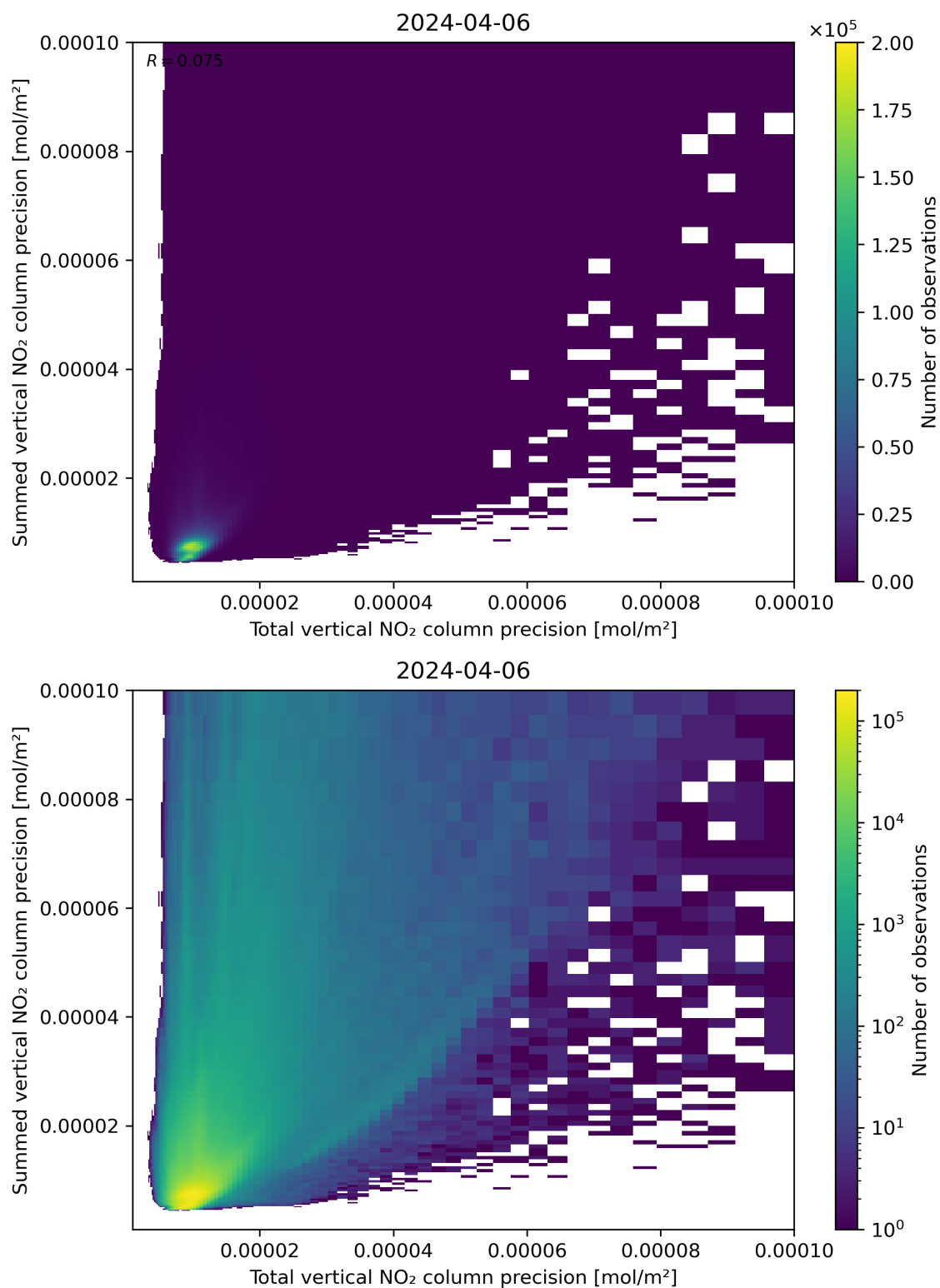
Figure 118: Scatter density plot of “Total vertical NO 2 column precision” against “Summed vertical NO 2 column precision” for 2024-04-05 to 2024-04-07.
