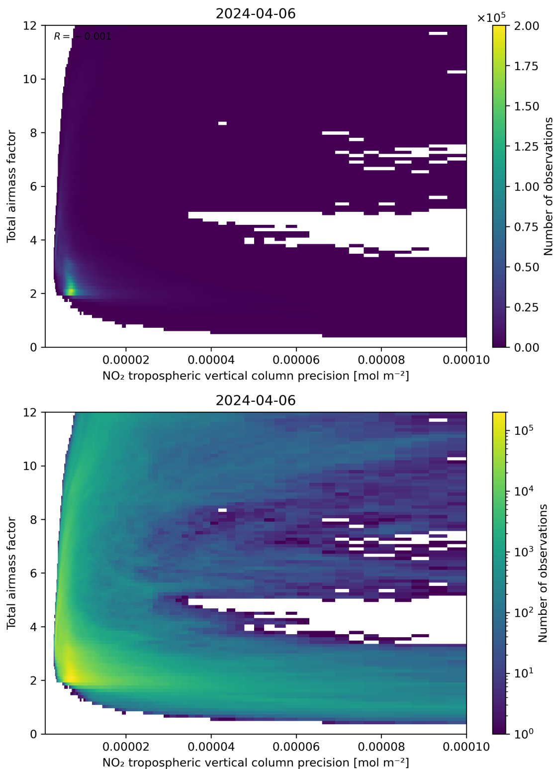
Figure 132: Scatter density plot of “NO 2 tropospheric vertical column precision” against “Total air mass factor” for 2024-04-05 to 2024-04-07.
