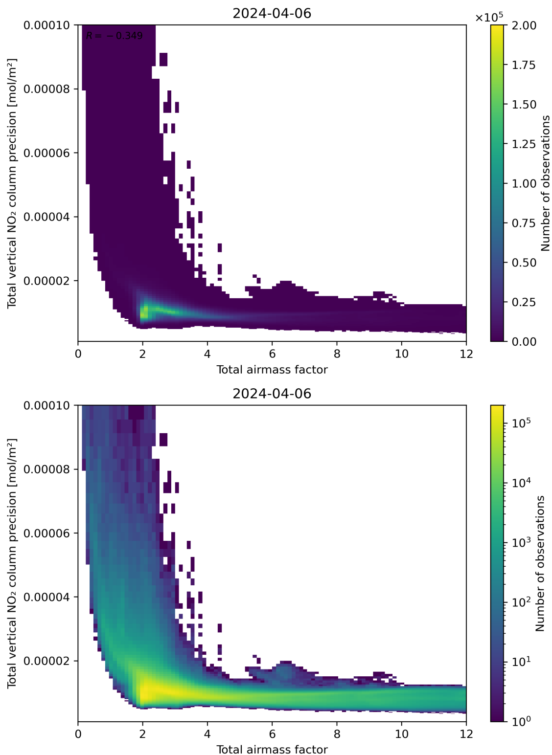
Figure 68: Scatter density plot of “Total airmass factor” against “Total vertical NO 2 column precision” for 2024-04-05 to 2024-04-07.
