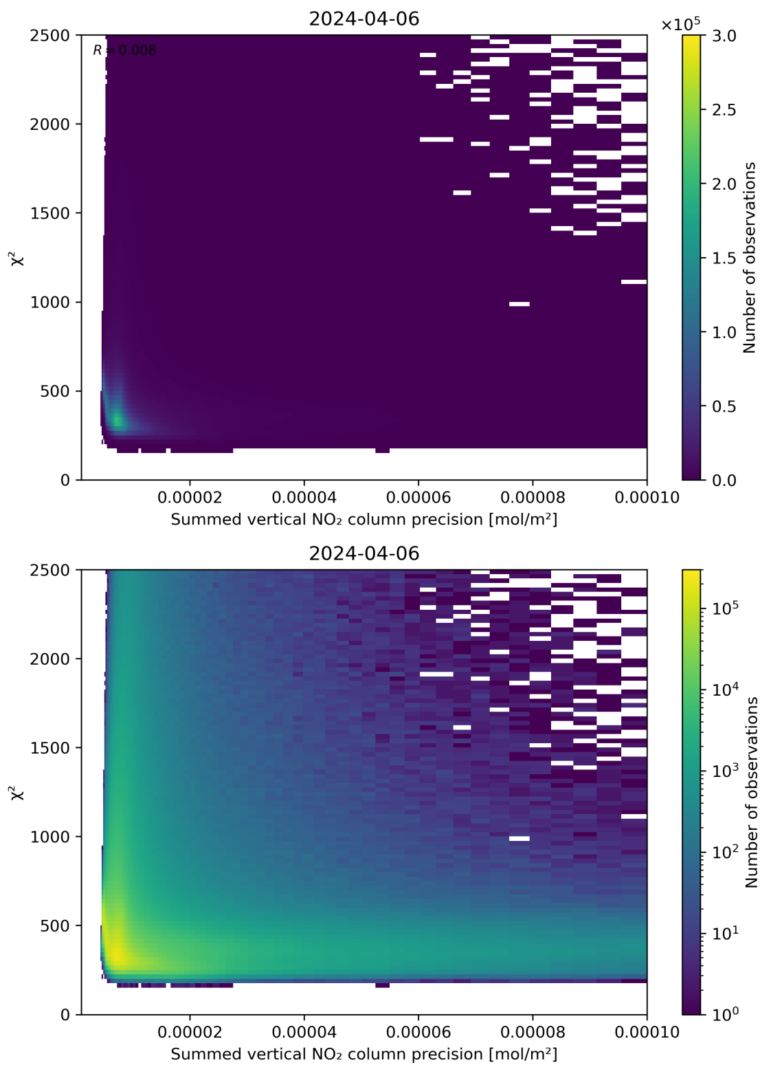
Figure 107: Scatter density plot of “Summed vertical NO 2 column precision” against “ \chi^2 ” for 2024-04-05 to 2024-04-07.
