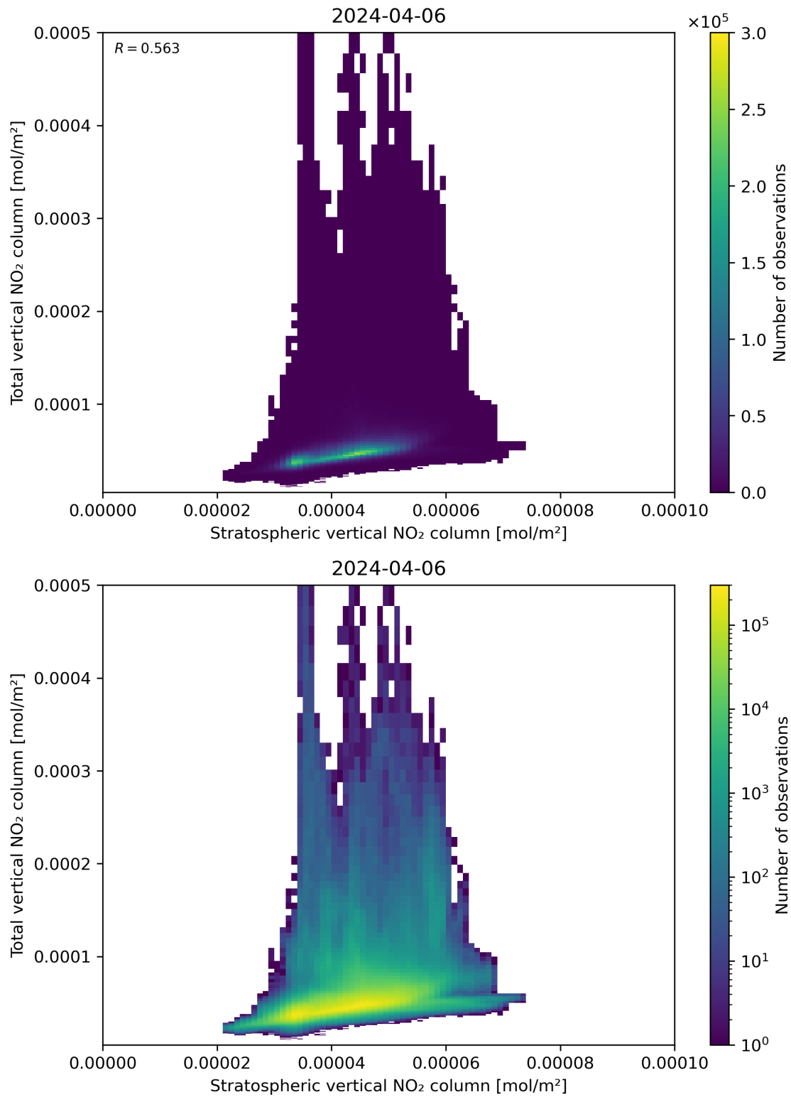
Figure 100: Scatter density plot of “Stratospheric vertical NO 2 column” against “Total vertical NO 2 column” for 2024-04-05 to 2024-04-07.
