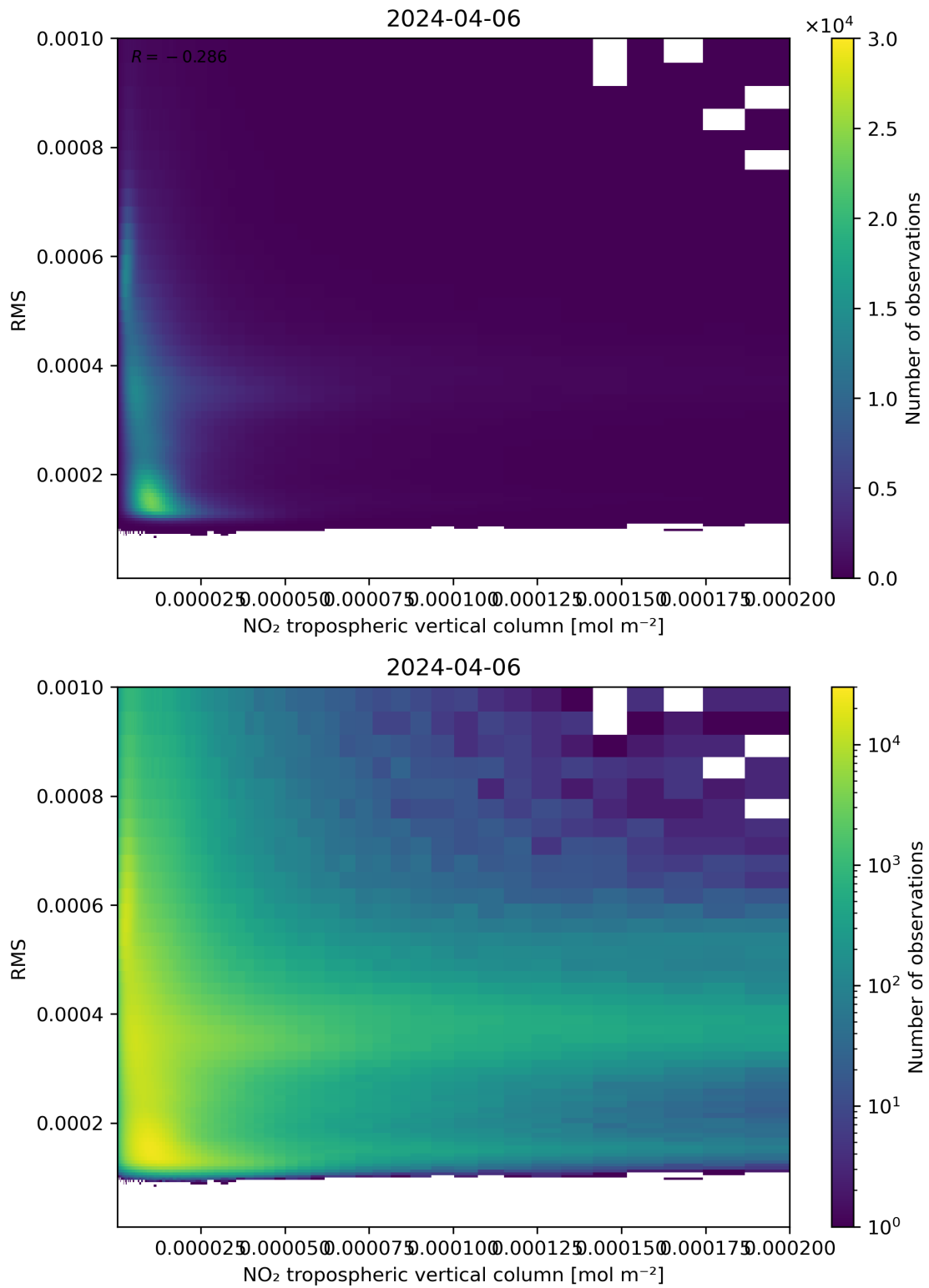
Figure 142: Scatter density plot of “NO 2 tropospheric vertical column” against “RMS” for 2024-04-05 to 2024-04-07.
