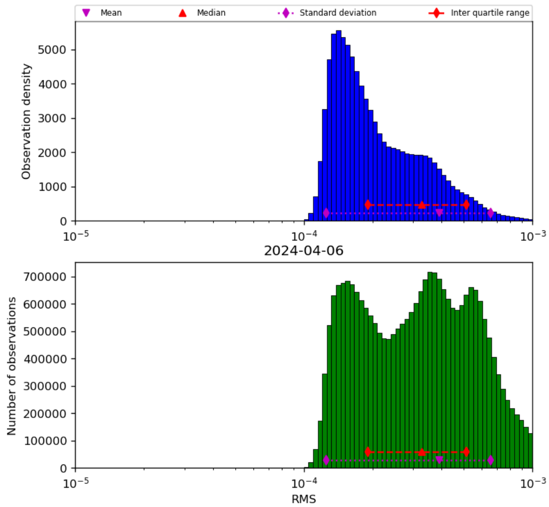
Figure 43: Histogram of “RMS” for 2024-04-05 to 2024-04-07
