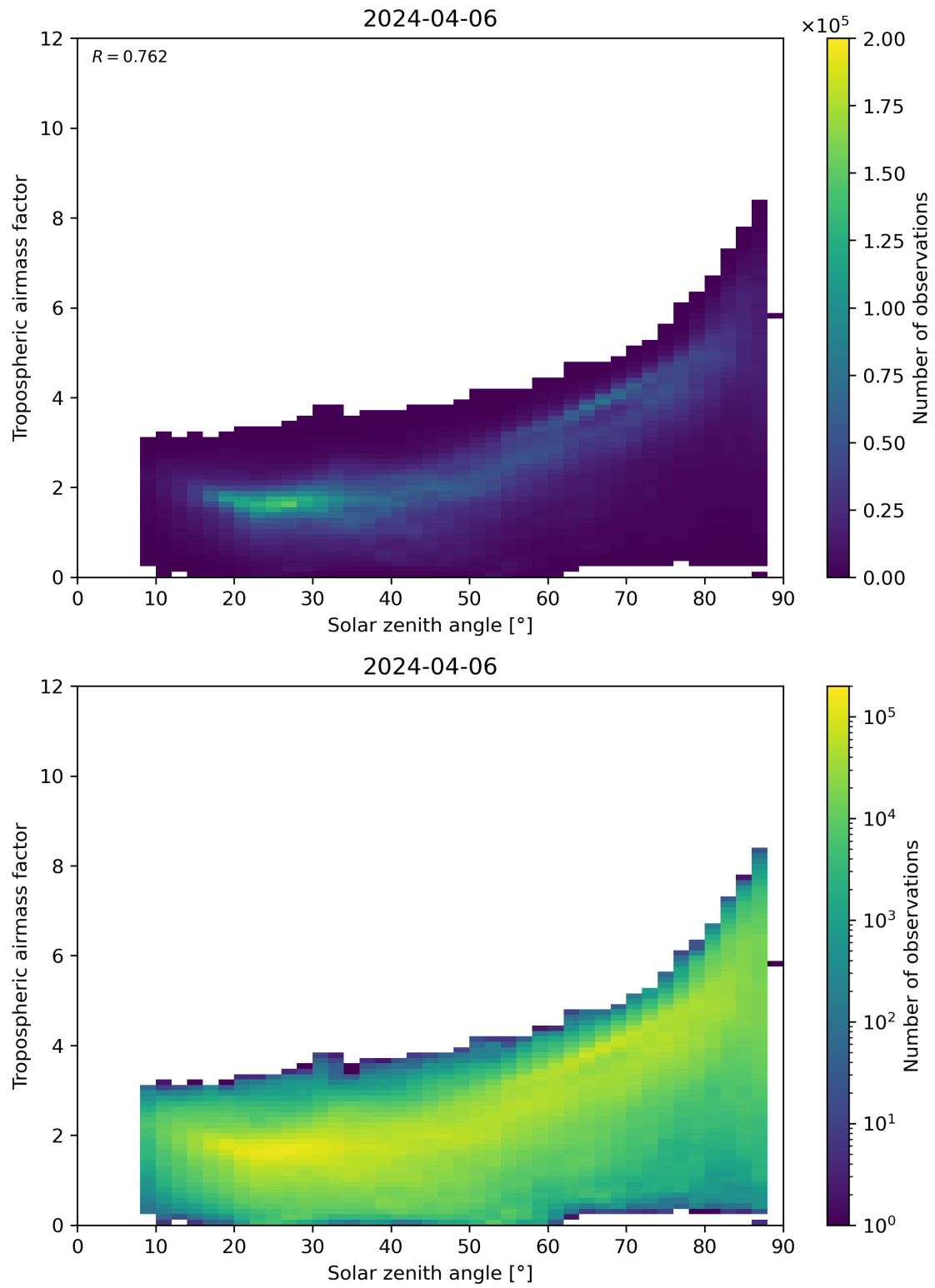
Figure 147: Scatter density plot of “Solar zenith angle” against “Tropospheric airmass factor” for 2024-04-05 to 2024-04-07.
