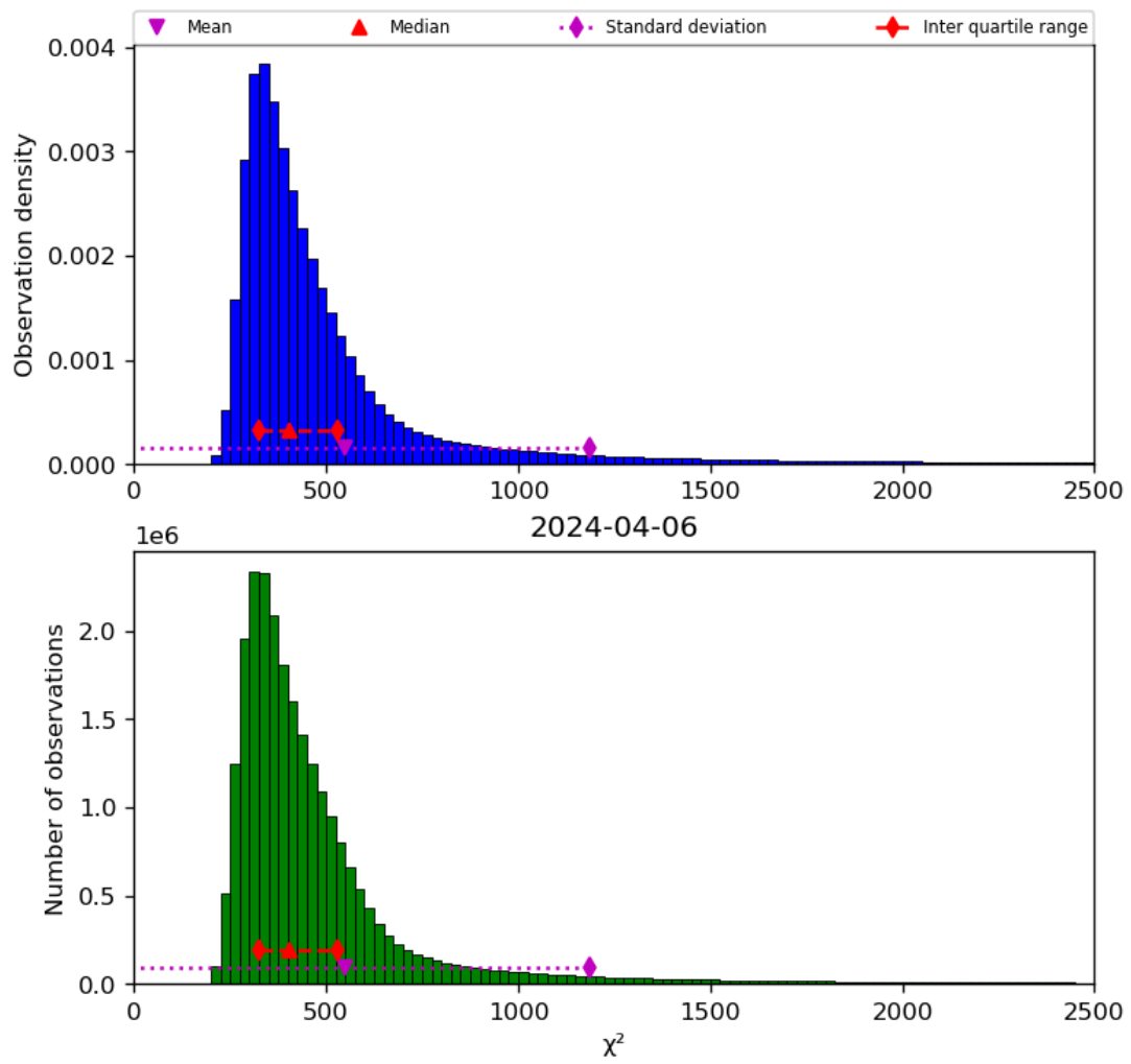
Figure 42: Histogram of “ \chi^2 ” for 2024-04-05 to 2024-04-07
