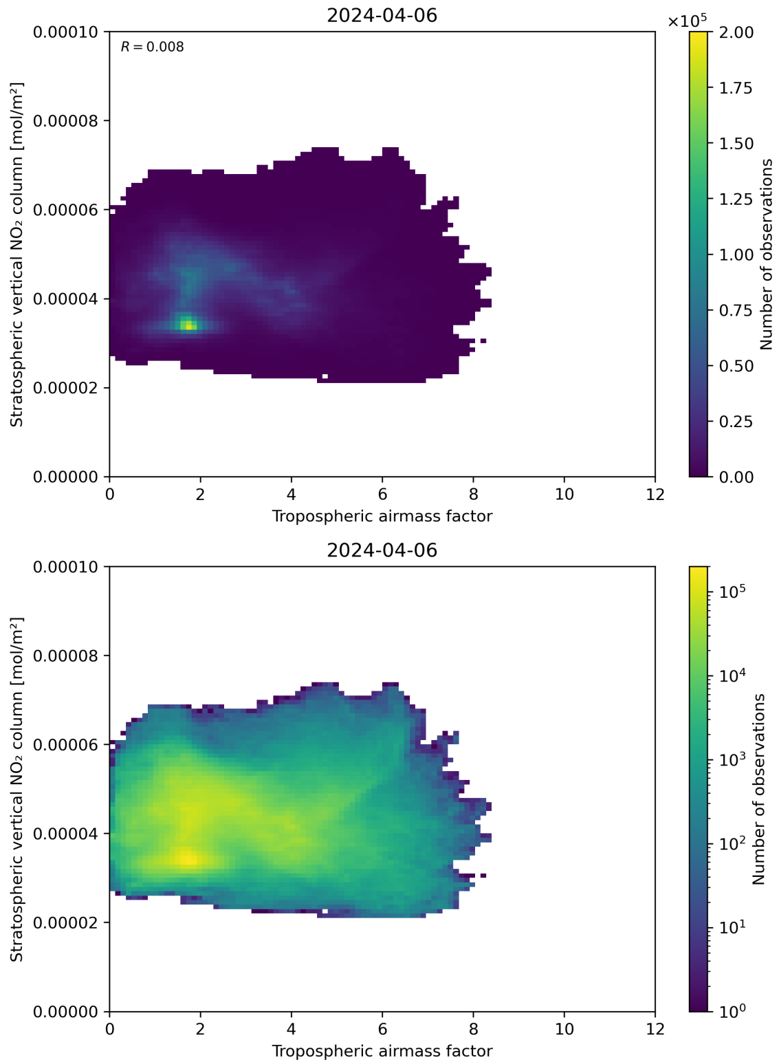
Figure 74: Scatter density plot of “Tropospheric air mass factor” against “Stratospheric vertical NO 2 column” for 2024-04-05 to 2024-04-07.
