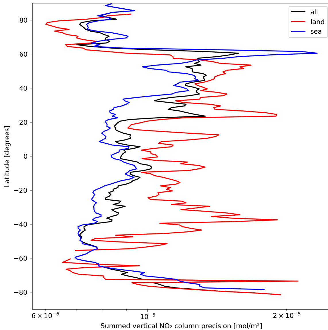
Figure 24: Zonal average of “Summed vertical NO 2 column precision” for 2024-04-05 to 2024-04-07.
