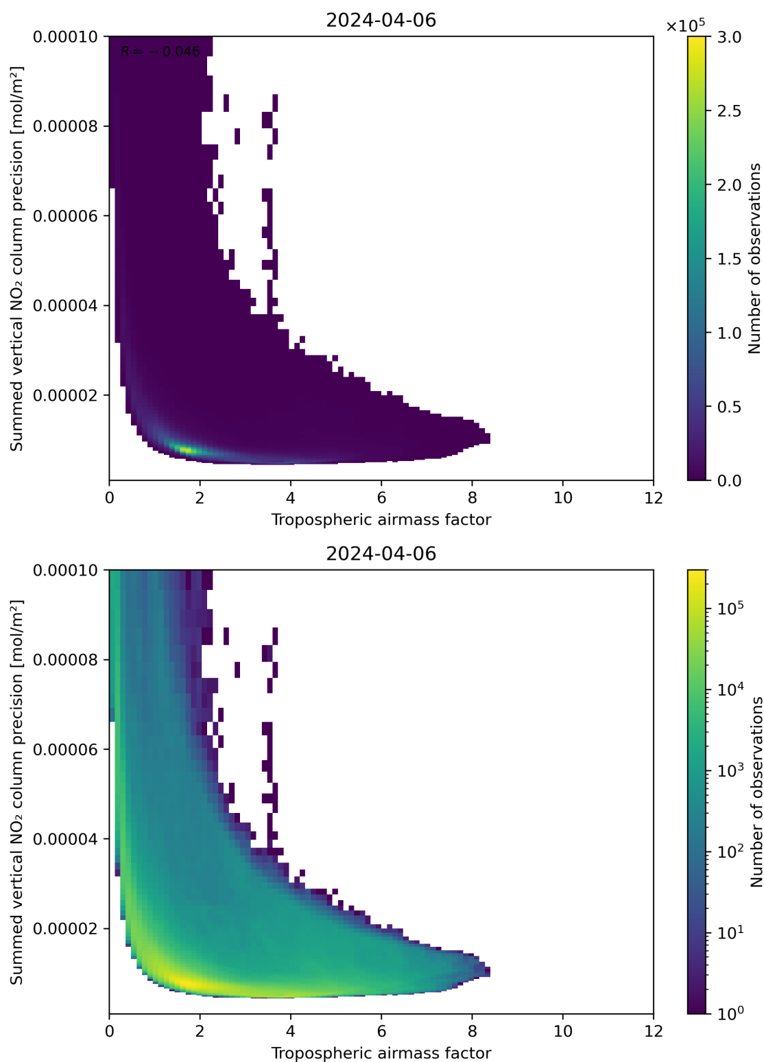
Figure 76: Scatter density plot of “Tropospheric air mass factor” against “Summed vertical NO 2 column precision” for 2024-04-05 to 2024-04-07.
