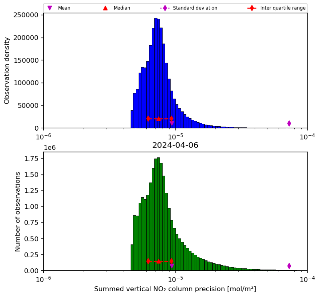
Figure 41: Histogram of "Summed vertical NO 2 column precision" for 2024-04-05 to 2024-04-07
