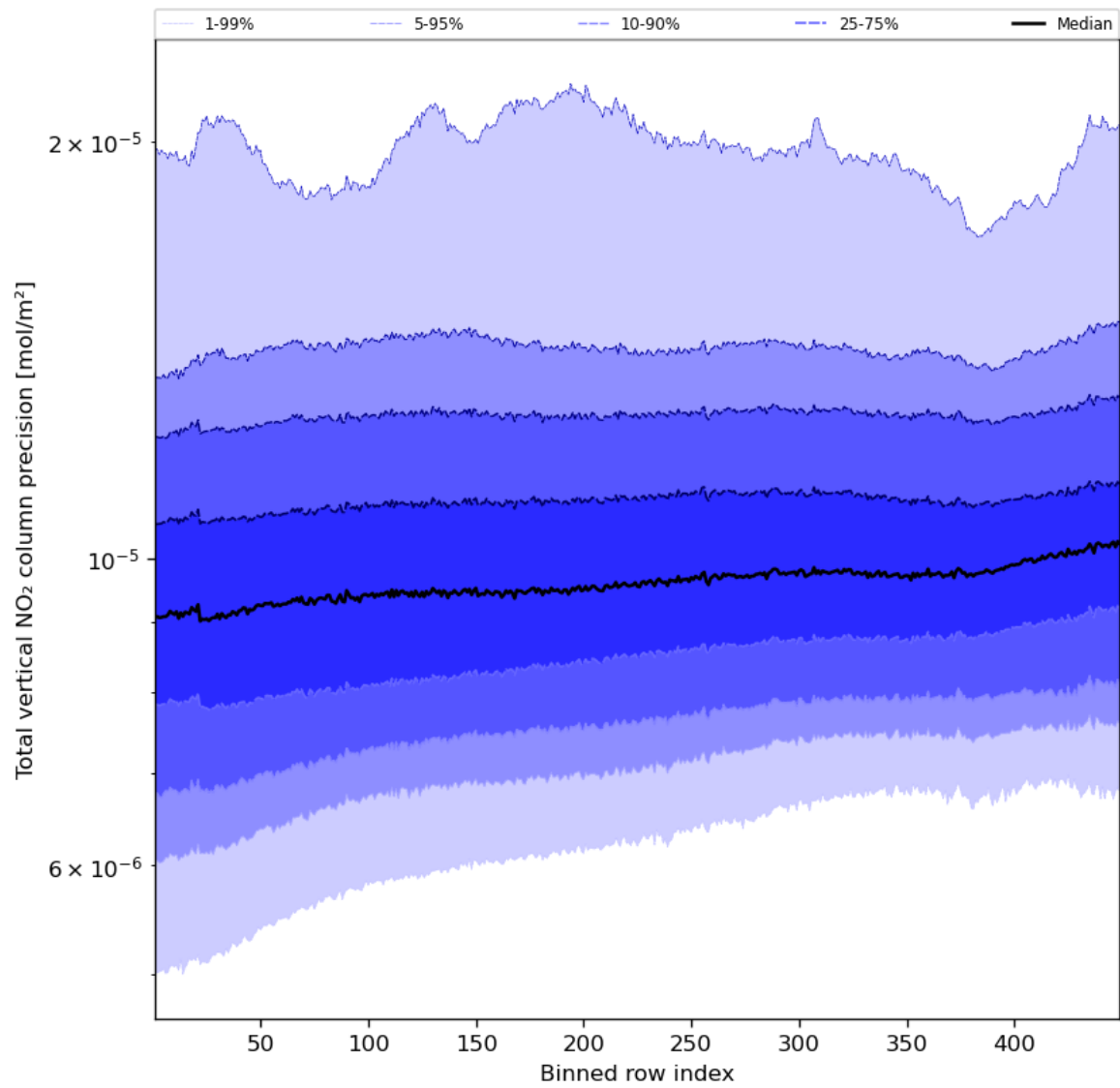
Figure 56: Along track statistics of "Total vertical NO 2 column precision" for 2024-04-05 to 2024-04-07
