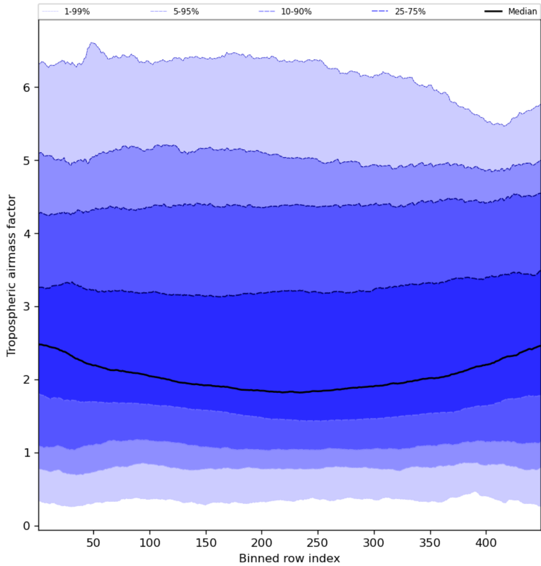
Figure 48: Along track statistics of “Tropospheric air mass factor” for 2024-04-05 to 2024-04-07
