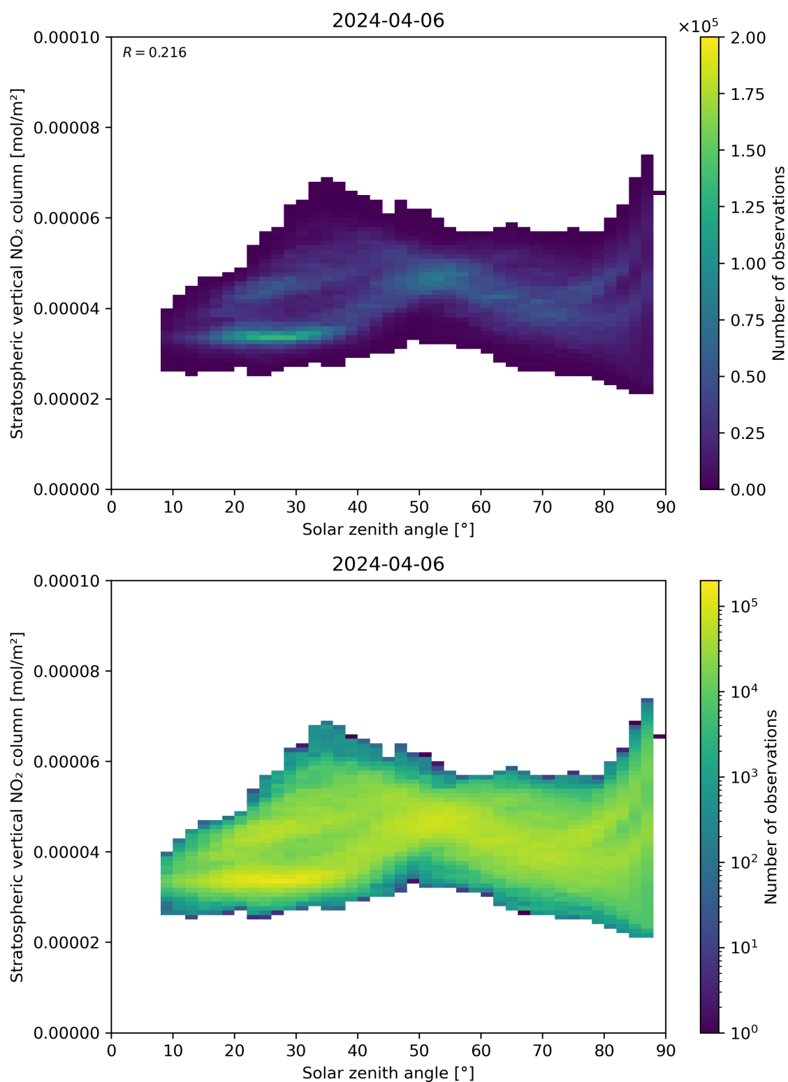
Figure 150: Scatter density plot of “Solar zenith angle” against “Stratospheric vertical NO 2 column” for 2024-04-05 to 2024-04-07.
