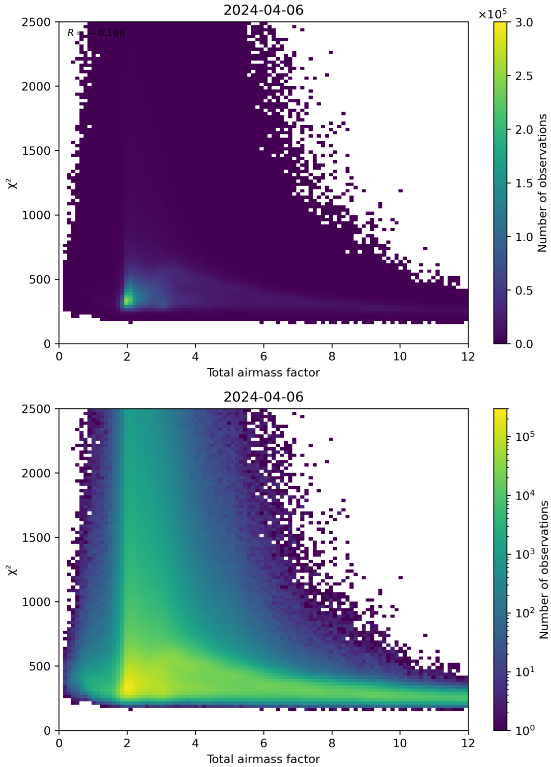
Figure 63: Scatter density plot of “Total airmass factor” against “ \chi^2 ” for 2024-04-05 to 2024-04-07.
