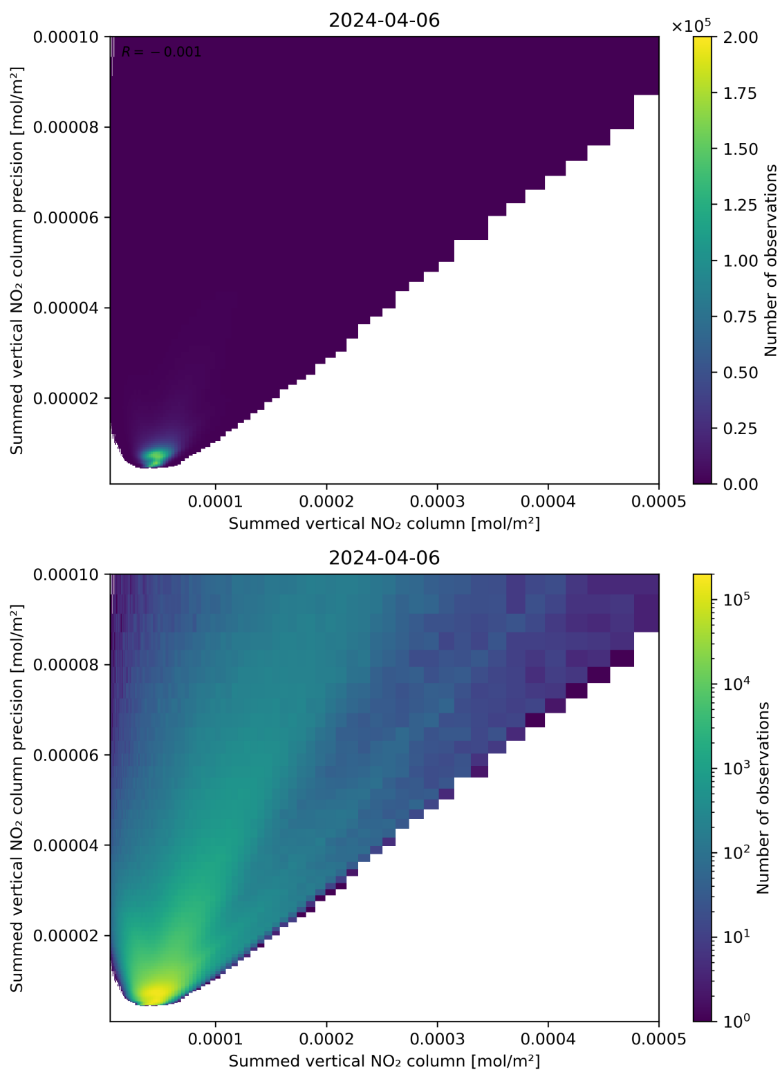
Figure 105: Scatter density plot of “Summed vertical NO 2 column” against “Summed vertical NO 2 column precision” for 2024-04-05 to 2024-04-07.
