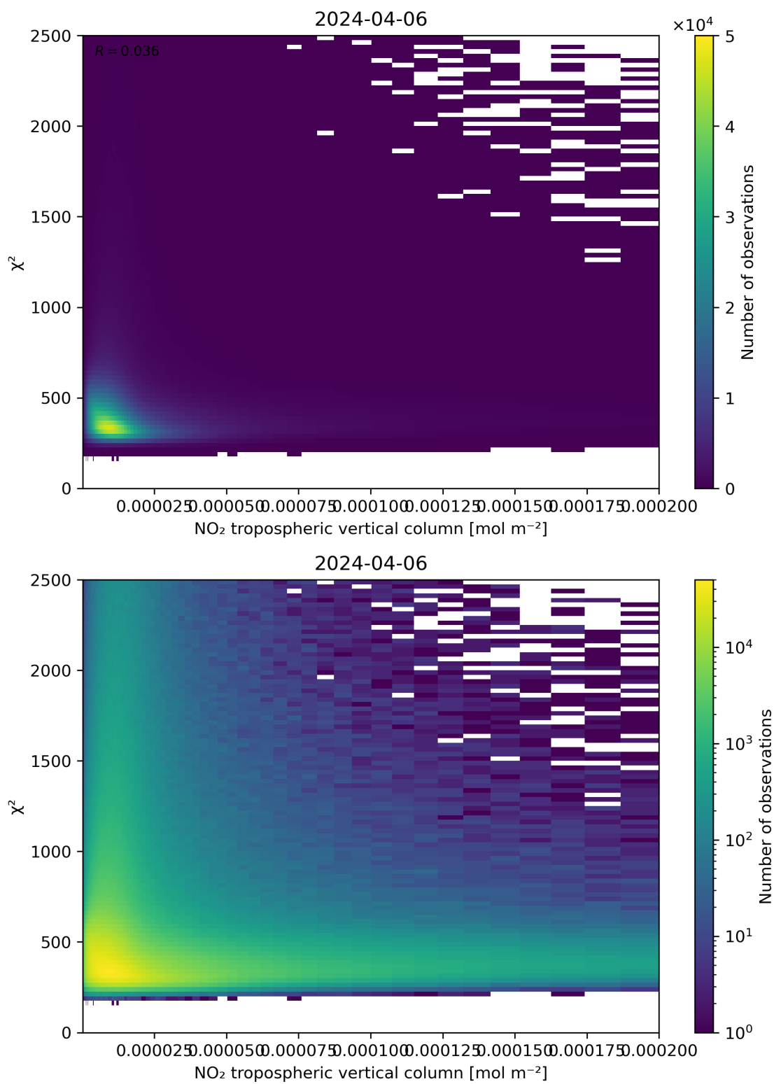
Figure 124: Scatter density plot of “NO 2 tropospheric vertical column” against “ \chi^2 ” for 2024-04-05 to 2024-04-07.
