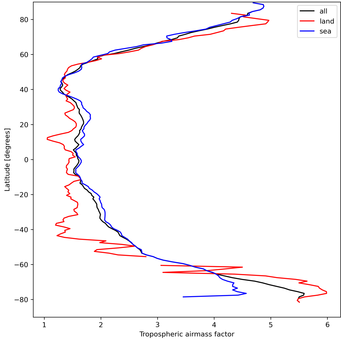
Figure 14: Zonal average of “Tropospheric air mass factor” for 2024-04-05 to 2024-04-07.
