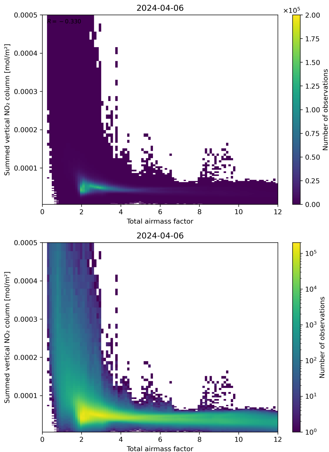
Figure 65: Scatter density plot of “Total airmass factor” against “Summed vertical NO 2 column” for 2024-04-05 to 2024-04-07.
