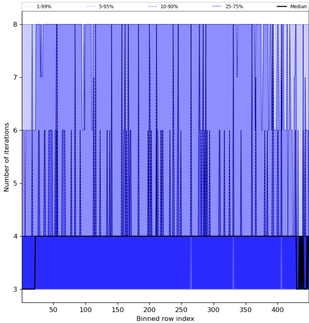
Figure 51: Along track statistics of “Number of iterations” for 2024-04-05 to 2024-04-07
