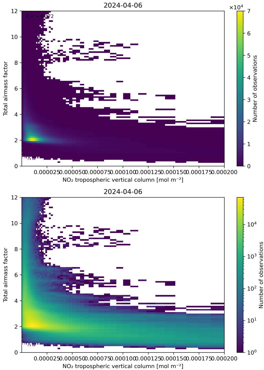
Figure 122: Scatter density plot of “NO 2 tropospheric vertical column” against “Total air mass factor” for 2024-04-05 to 2024-04-07.
