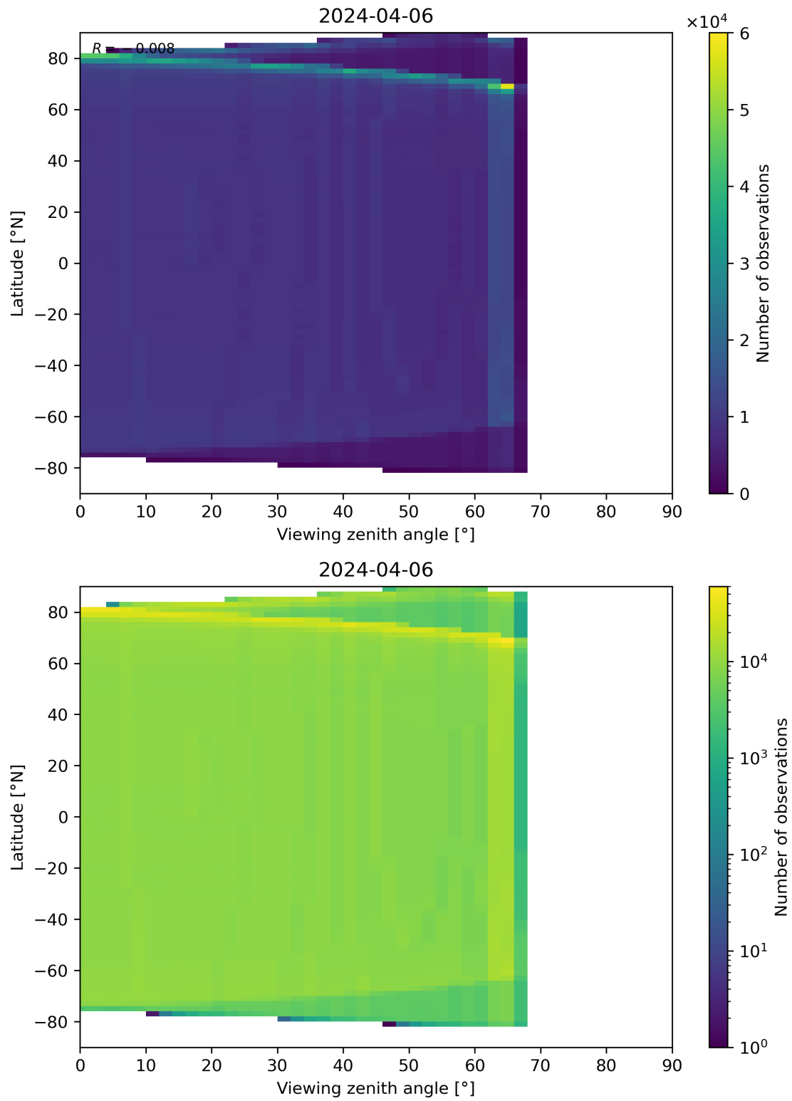
Figure 163: Scatter density plot of “Viewing zenith angle” against “Latitude” for 2024-04-05 to 2024-04-07.
