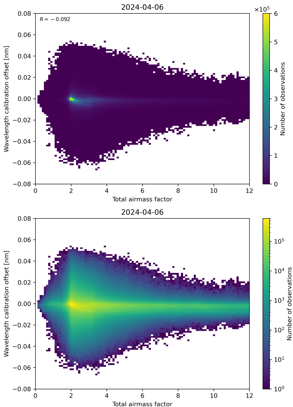
Figure 70: Scatter density plot of “Total airmass factor” against “Wavelength calibration offset” for 2024-04-05 to 2024-04-07.
