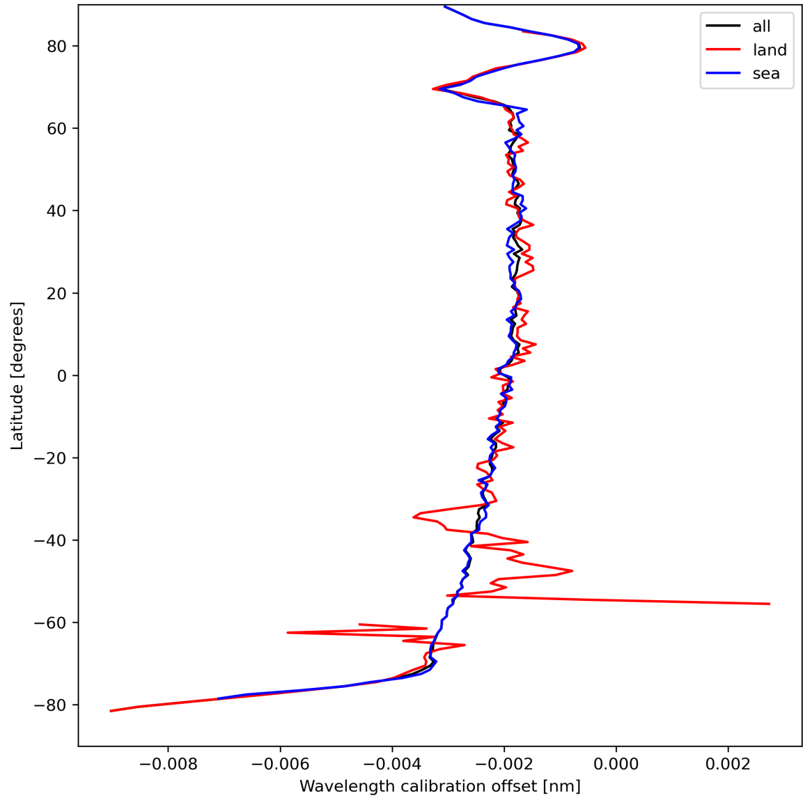
Figure 18: Zonal average of “Wavelength calibration offset” for 2024-04-05 to 2024-04-07.
