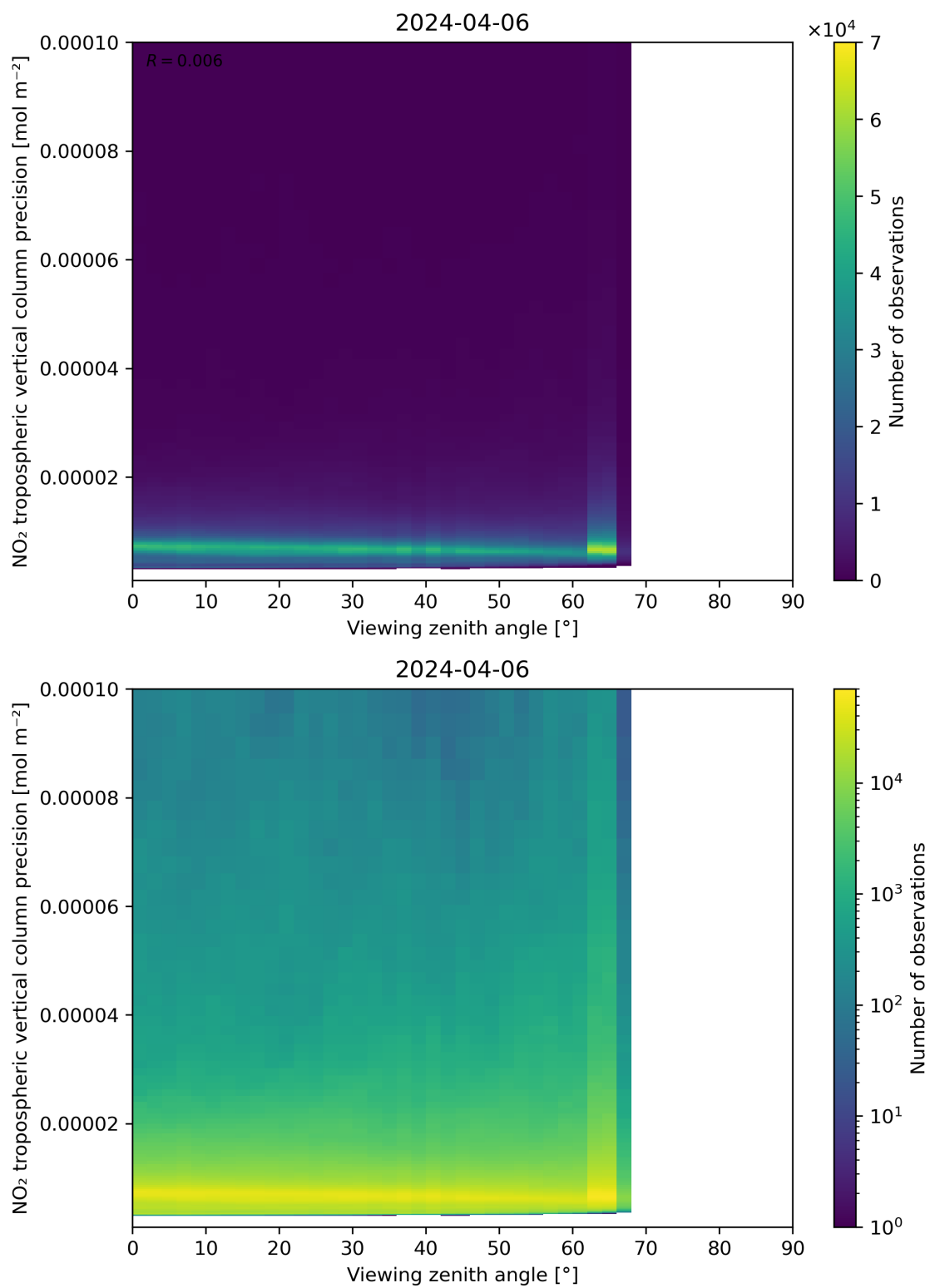
Figure 170: Scatter density plot of “Viewing zenith angle” against “NO 2 tropospheric vertical column precision” for 2024-04-05 to 2024-04-07.
