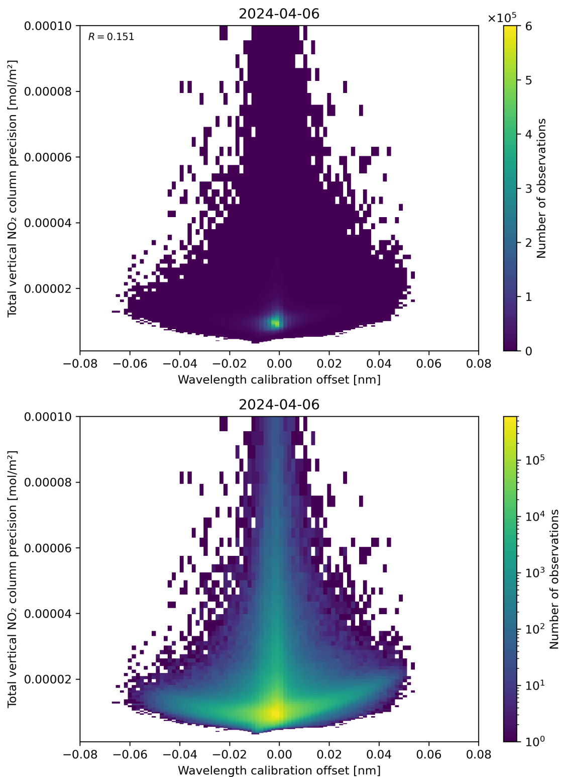
Figure 180: Scatter density plot of “Wavelength calibration offset” against “Total vertical NO 2 column precision” for 2024-04-05 to 2024-04-07.
