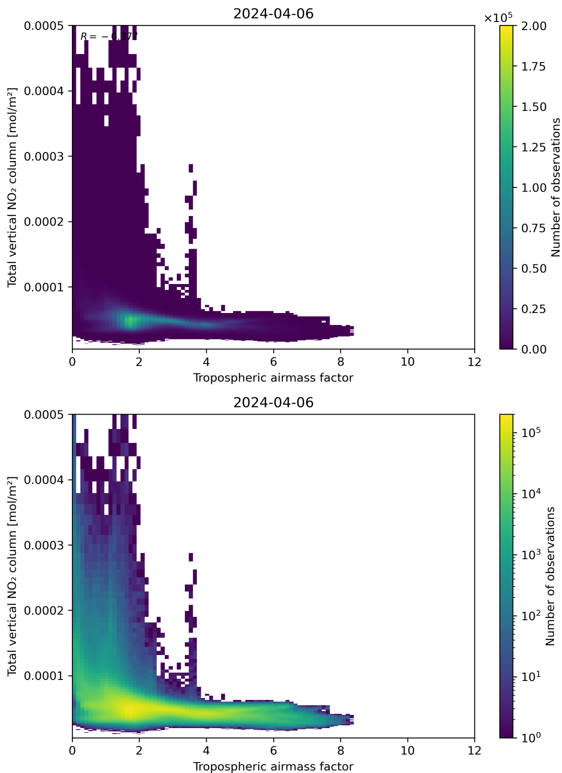
Figure 77: Scatter density plot of “Tropospheric airmass factor” against “Total vertical NO 2 column” for 2024-04-05 to 2024-04-07.
