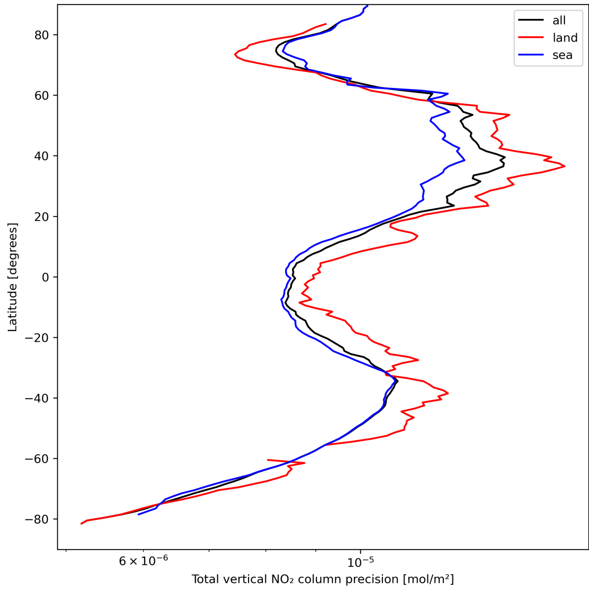
Figure 22: Zonal average of “Total vertical NO 2 column precision” for 2024-04-05 to 2024-04-07.
