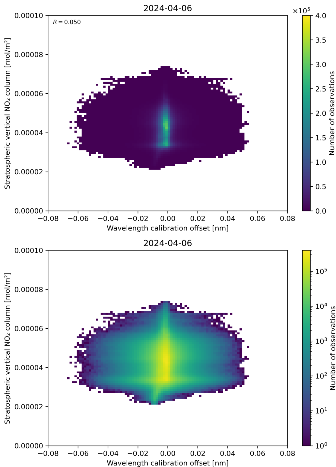
Figure 176: Scatter density plot of “Wavelength calibration offset” against “Stratospheric vertical NO 2 column” for 2024-04-05 to 2024-04-07.
