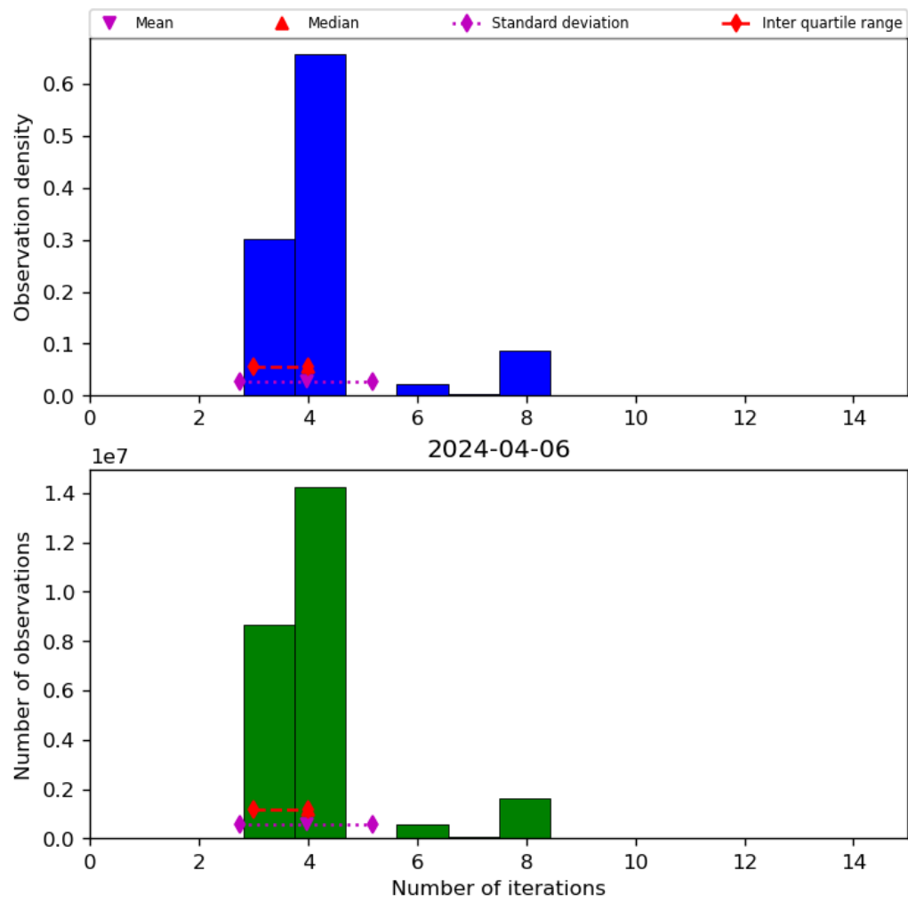
Figure 34: Histogram of “Number of iterations” for 2024-04-05 to 2024-04-07
