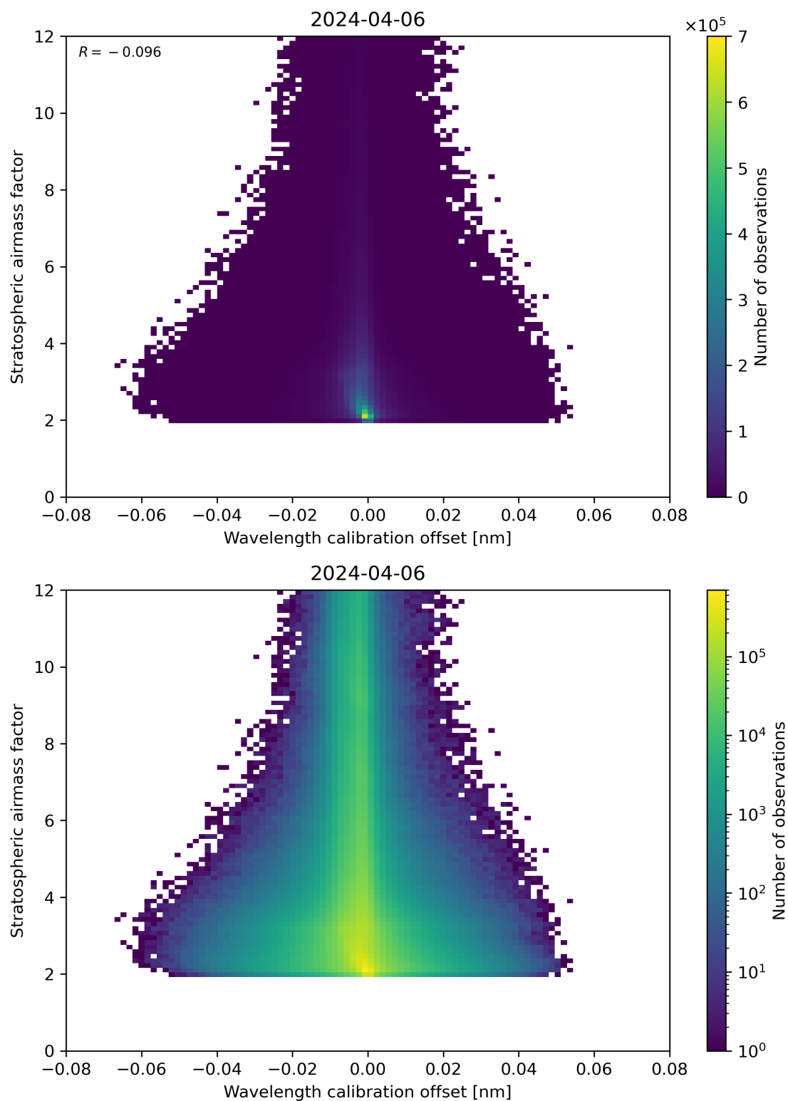
Figure 174: Scatter density plot of “Wavelength calibration offset” against “Stratospheric airmass factor” for 2024-04-05 to 2024-04-07.
