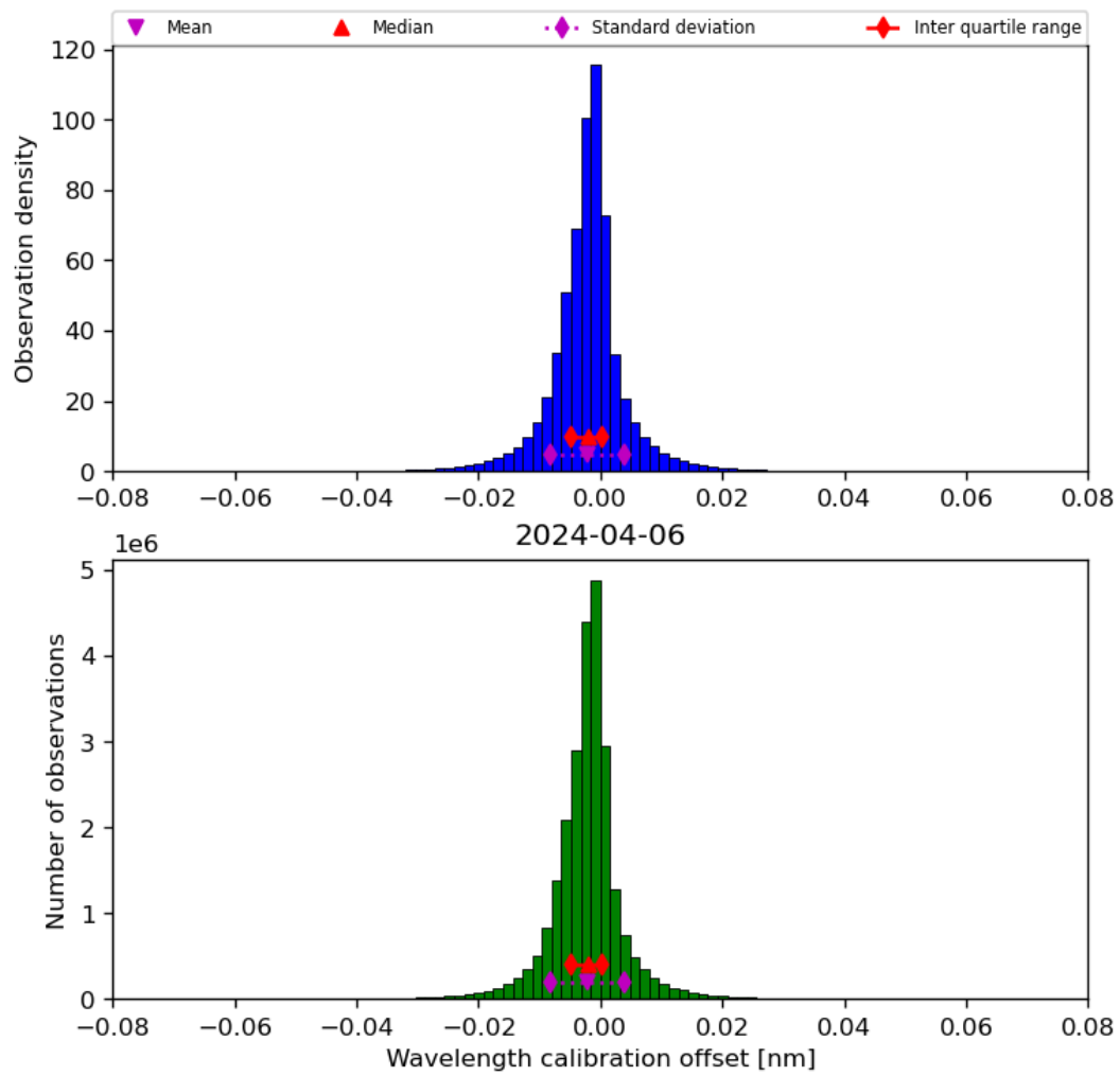
Figure 35: Histogram of “Wavelength calibration offset” for 2024-04-05 to 2024-04-07
