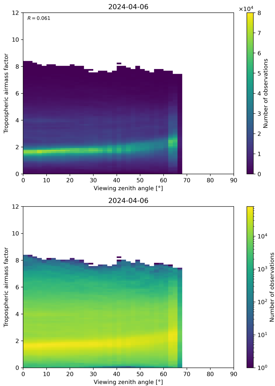
Figure 161: Scatter density plot of “Viewing zenith angle” against “Tropospheric airmass factor” for 2024-04-05 to 2024-04-07.
