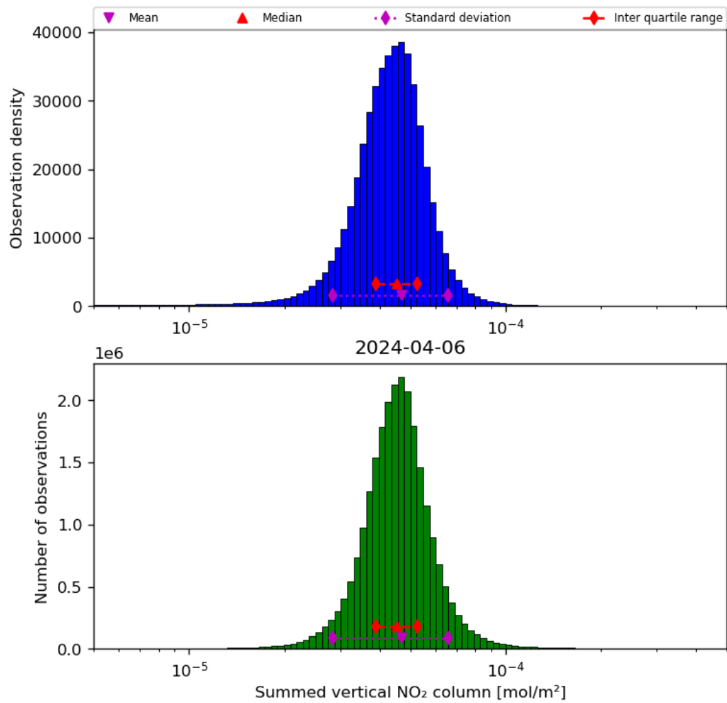
Figure 40: Histogram of “Summed vertical NO 2 column” for 2024-04-05 to 2024-04-07
