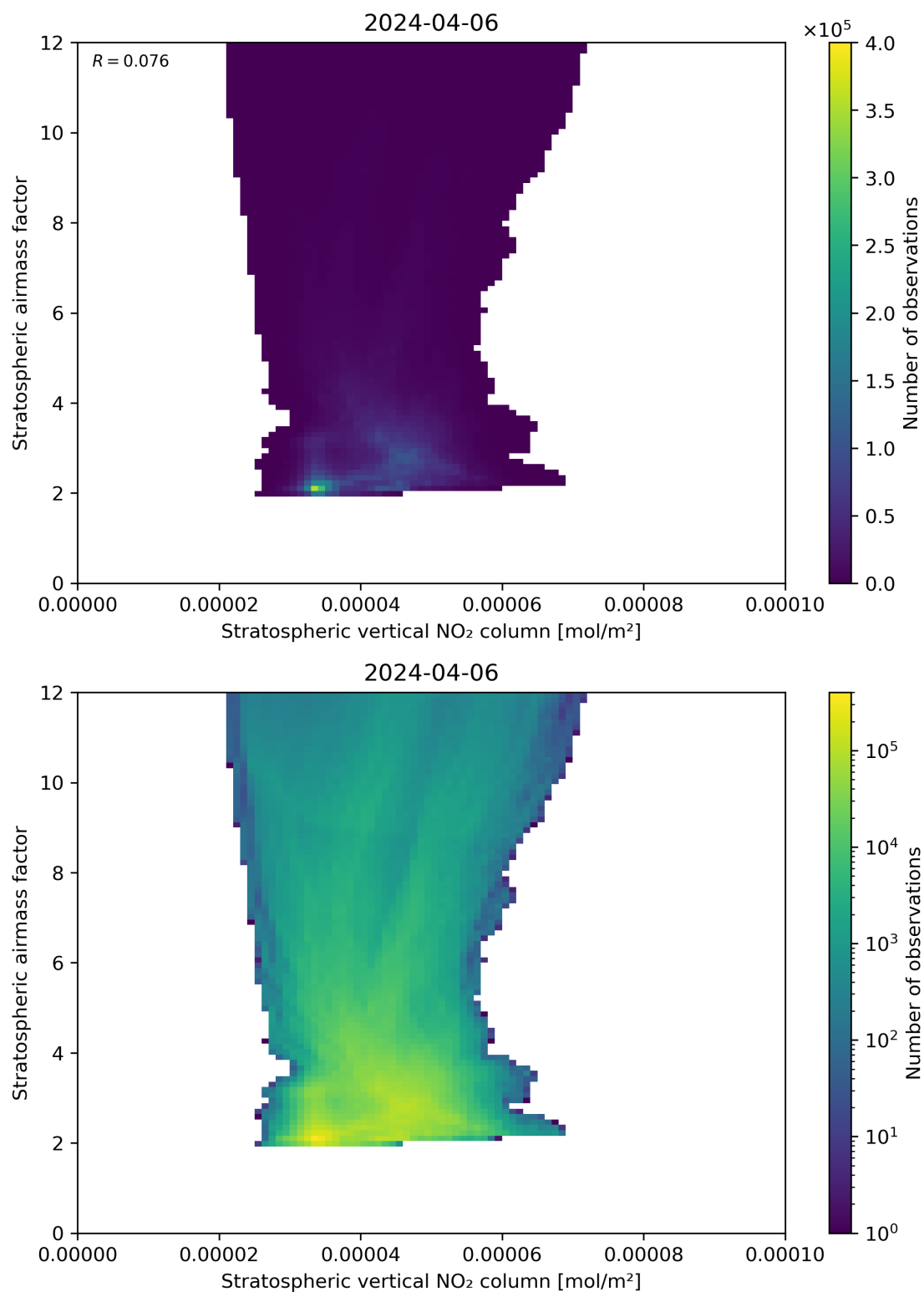
Figure 96: Scatter density plot of “Stratospheric vertical NO 2 column” against “Stratospheric airmass factor” for 2024-04-05 to 2024-04-07.
