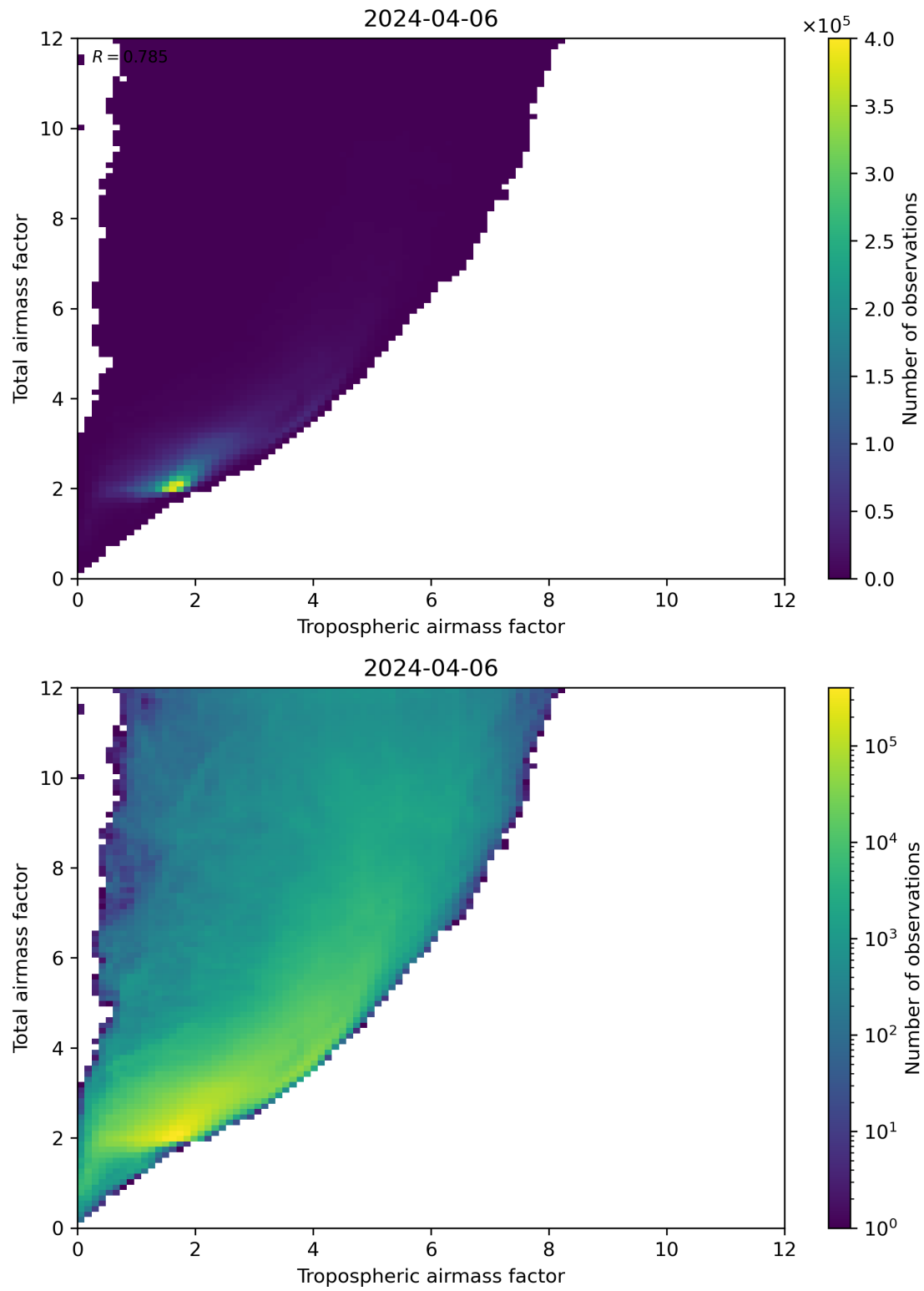
Figure 72: Scatter density plot of “Tropospheric airmass factor” against “Total airmass factor” for 2024-04-05 to 2024-04-07.
