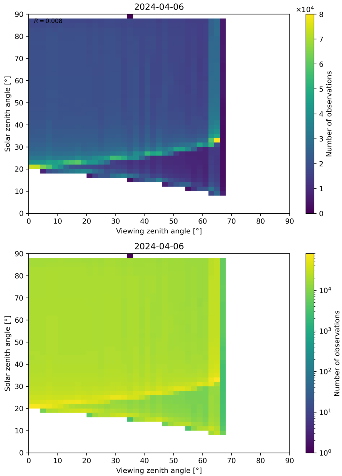
Figure 172: Scatter density plot of “Viewing zenith angle” against “Solar zenith angle” for 2024-04-05 to 2024-04-07.
