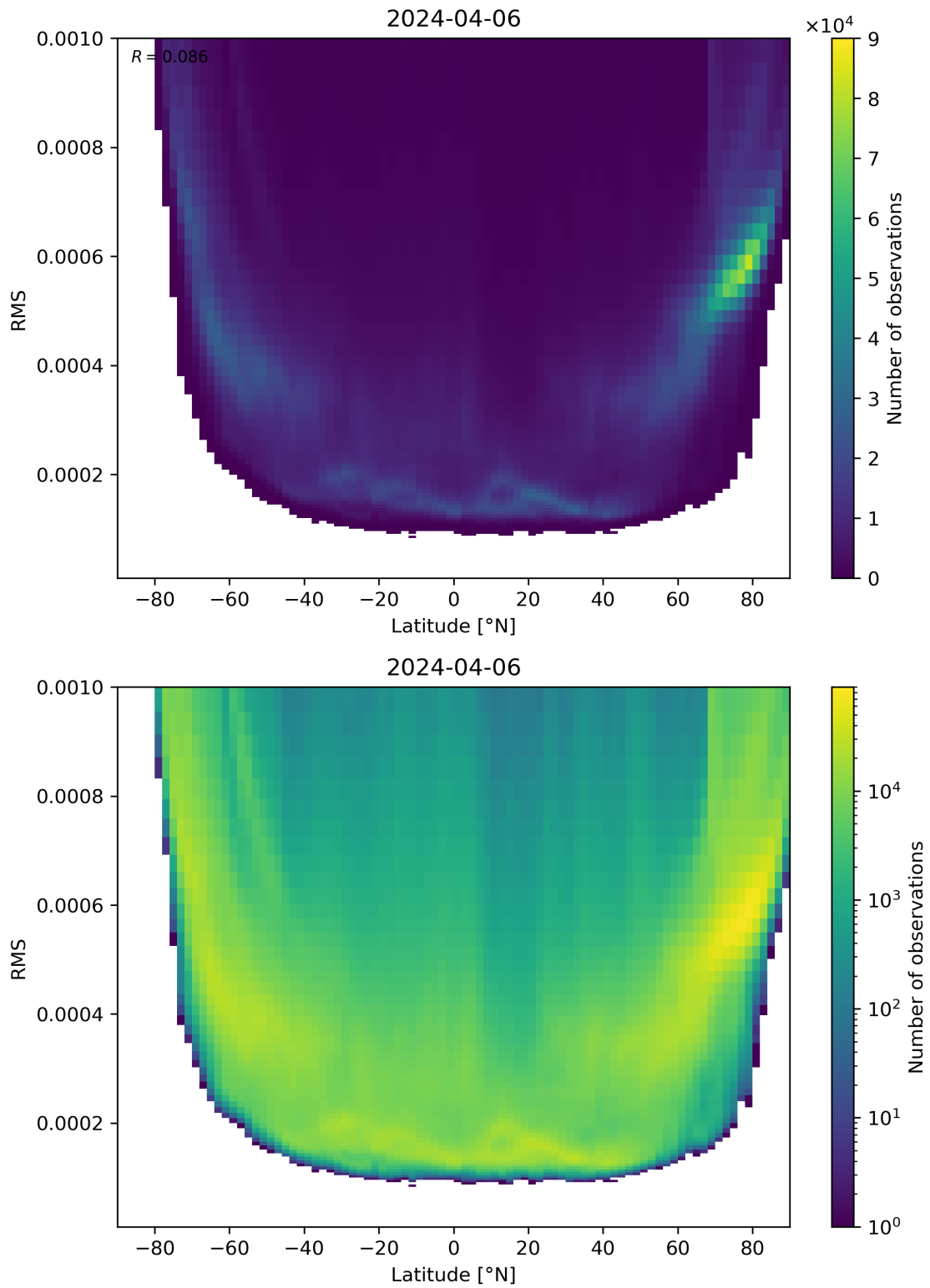
Figure 94: Scatter density plot of “Latitude” against “RMS” for 2024-04-05 to 2024-04-07.
