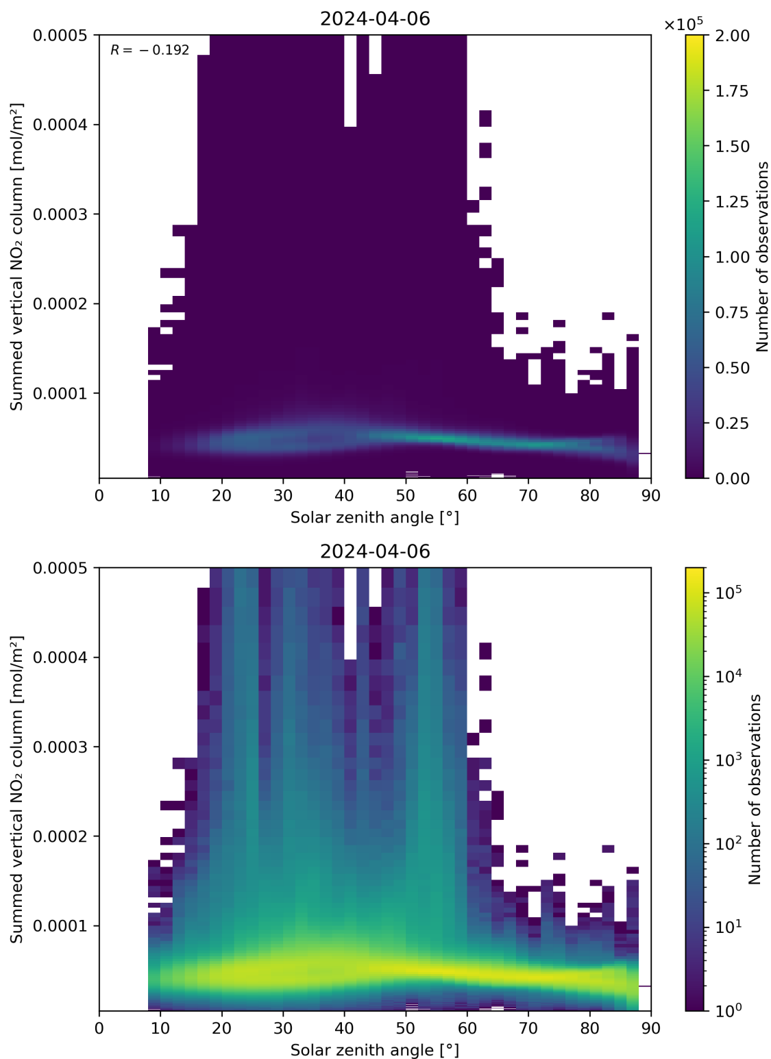
Figure 151: Scatter density plot of “Solar zenith angle” against “Summed vertical NO 2 column” for 2024-04-05 to 2024-04-07.
