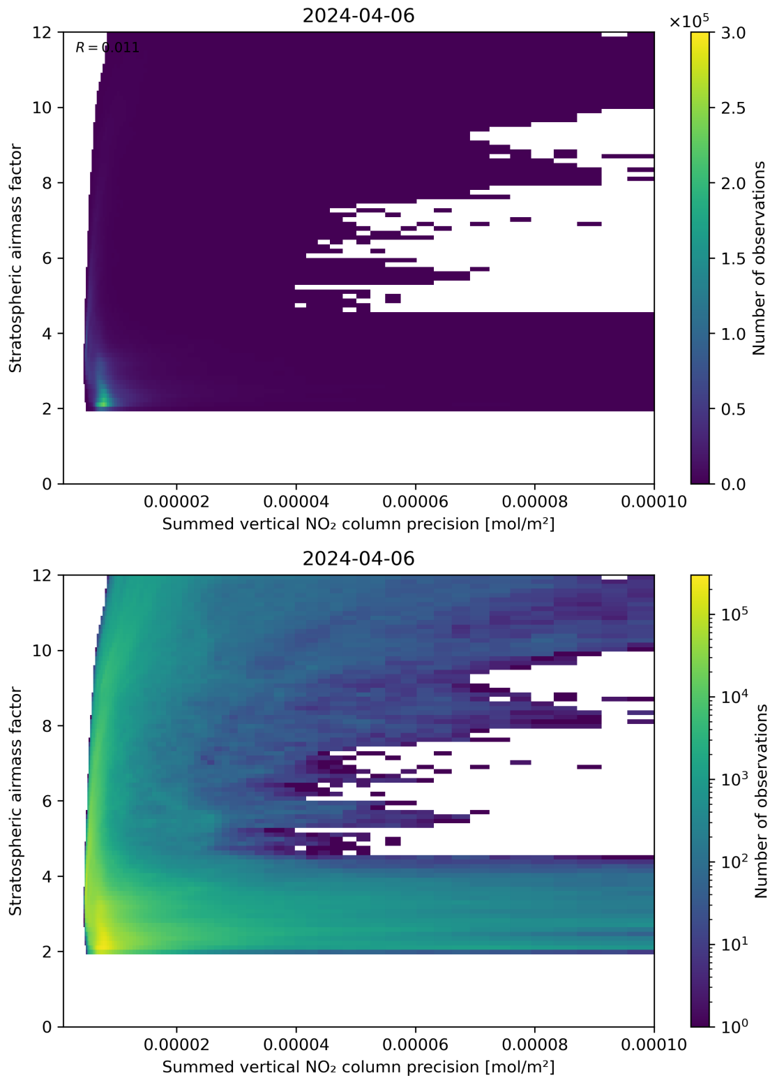
Figure 106: Scatter density plot of “Summed vertical NO 2 column precision” against “Stratospheric airmass factor” for 2024-04-05 to 2024-04-07.
