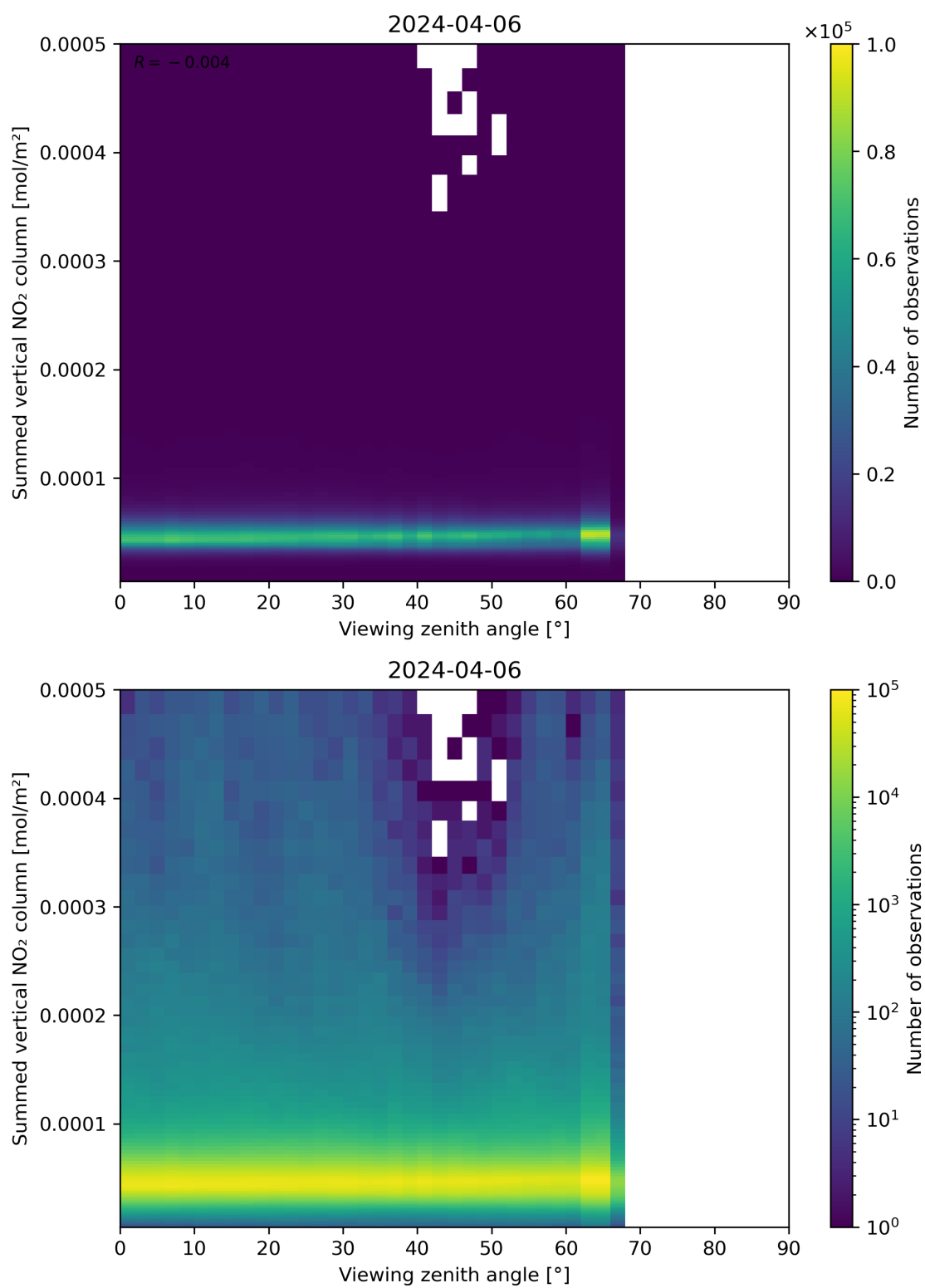
Figure 165: Scatter density plot of “Viewing zenith angle” against “Summed vertical NO 2 column” for 2024-04-05 to 2024-04-07.
