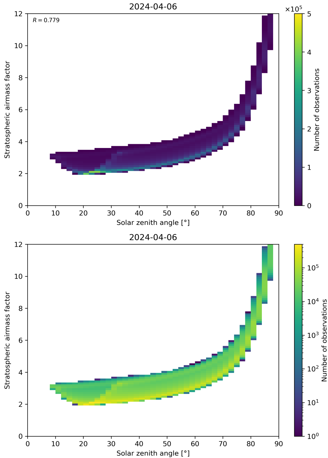
Figure 145: Scatter density plot of “Solar zenith angle” against “Stratospheric airmass factor” for 2024-04-05 to 2024-04-07.
