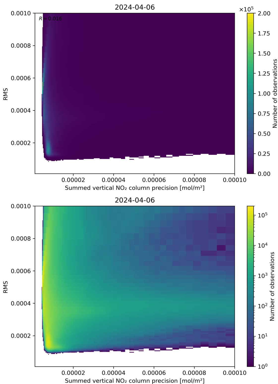
Figure 108: Scatter density plot of “Summed vertical NO 2 column precision” against “RMS” for 2024-04-05 to 2024-04-07.
