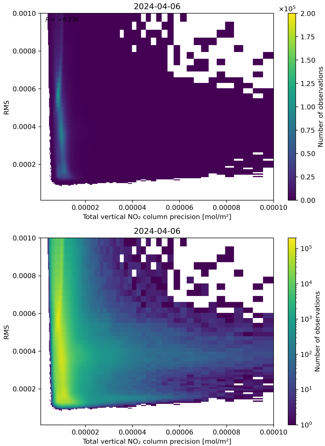
Figure 119: Scatter density plot of “Total vertical NO 2 column precision” against “RMS” for 2024-04-05 to 2024-04-07.
