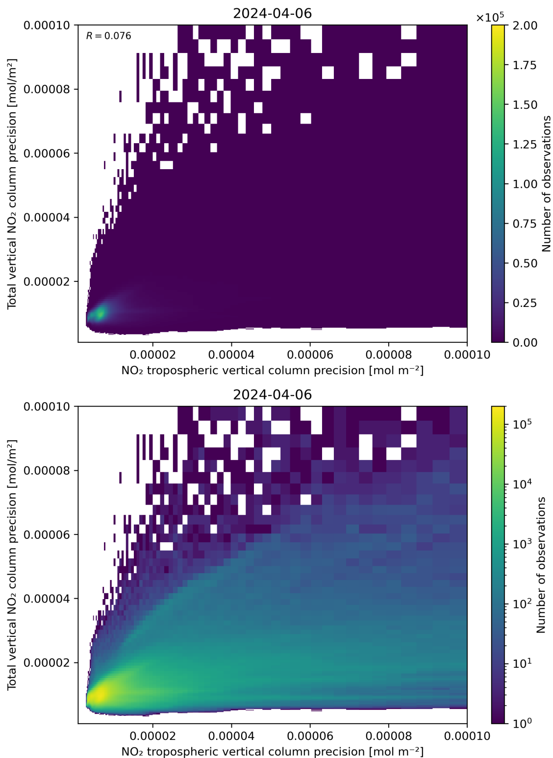
Figure 139: Scatter density plot of “NO 2 tropospheric vertical column precision” against “Total vertical NO 2 column precision” for 2024-04-05 to 2024-04-07.
