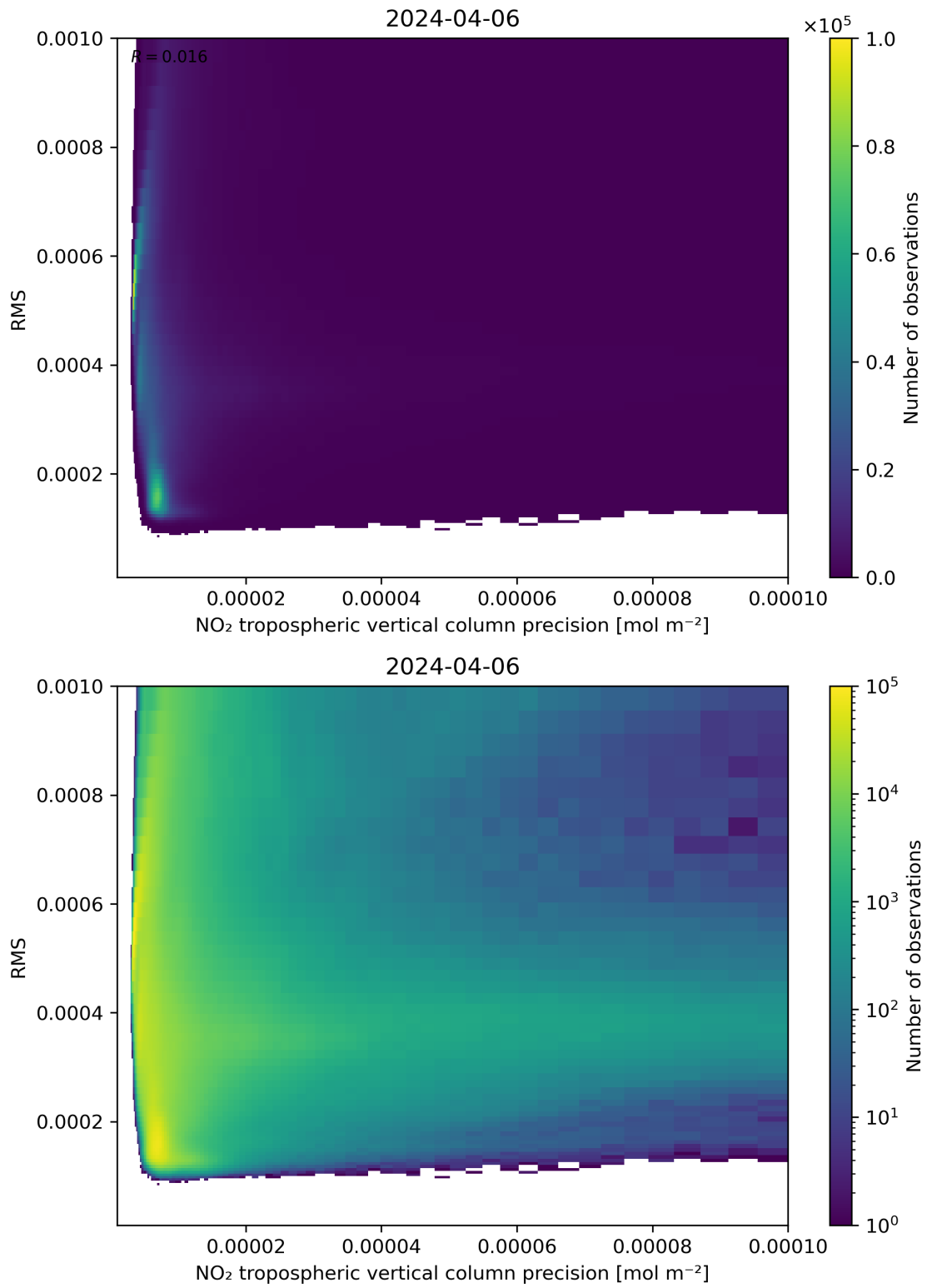
Figure 140: Scatter density plot of “NO 2 tropospheric vertical column precision” against “RMS” for 2024-04-05 to 2024-04-07.
