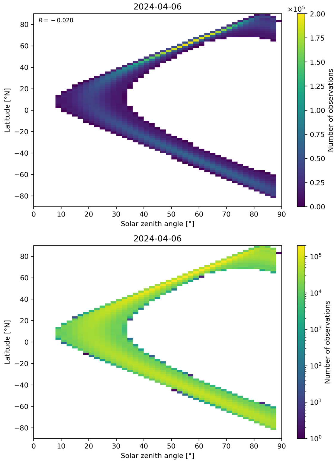
Figure 149: Scatter density plot of “Solar zenith angle” against “Latitude” for 2024-04-05 to 2024-04-07.
