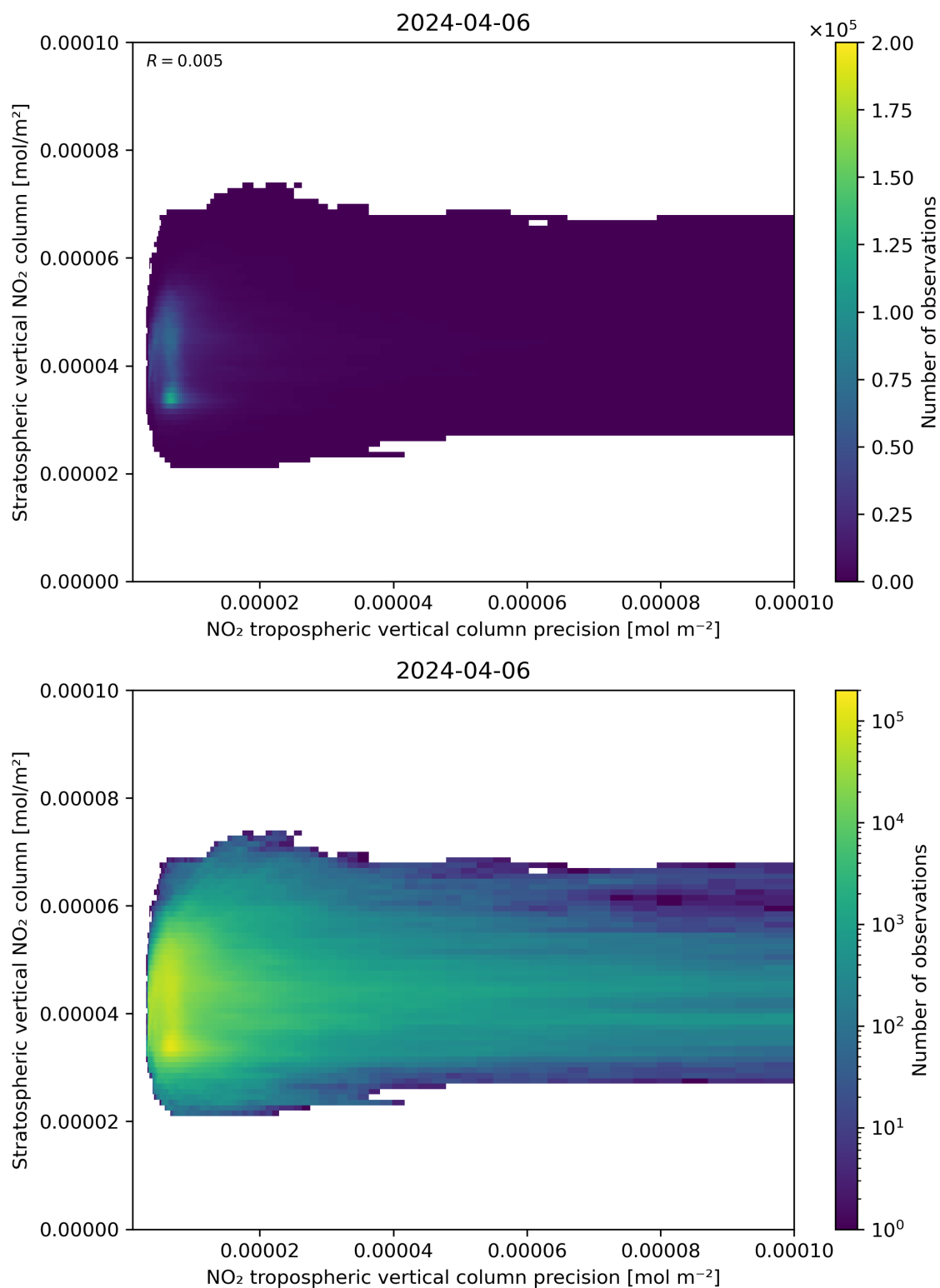
Figure 135: Scatter density plot of “NO 2 tropospheric vertical column precision” against “Stratospheric vertical NO 2 column” for 2024-04-05 to 2024-04-07.
