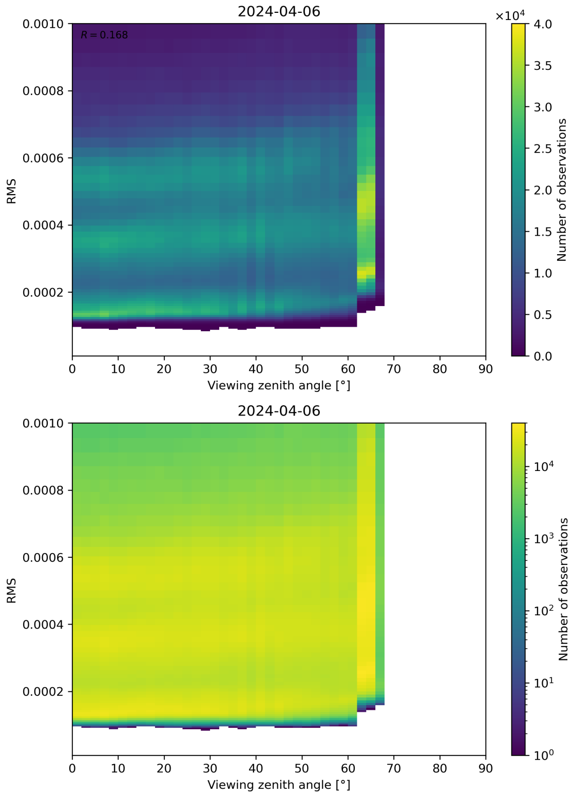
Figure 171: Scatter density plot of “Viewing zenith angle” against “RMS” for 2024-04-05 to 2024-04-07.
