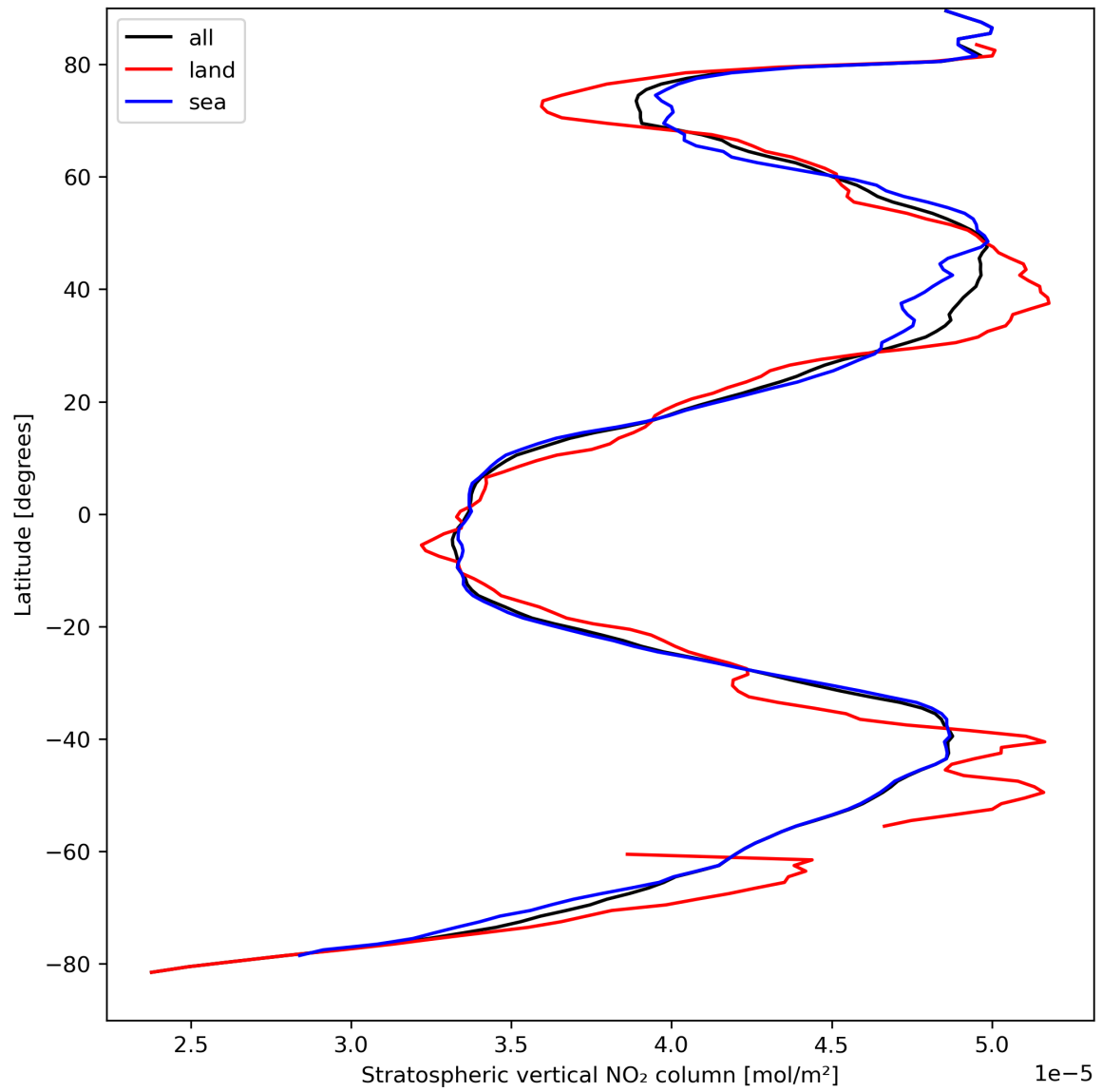
Figure 19: Zonal average of “Stratospheric vertical NO 2 column” for 2024-04-05 to 2024-04-07.
