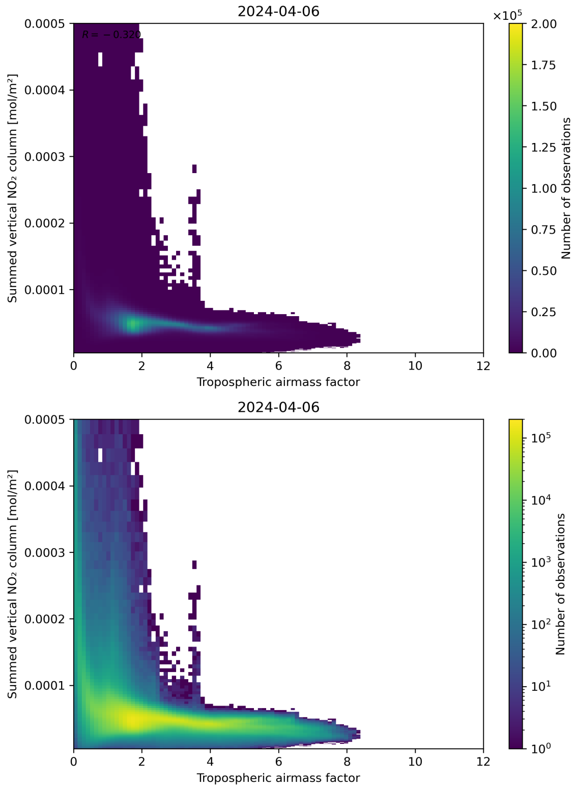
Figure 75: Scatter density plot of “Tropospheric air mass factor” against “Summed vertical NO 2 column” for 2024-04-05 to 2024-04-07.
