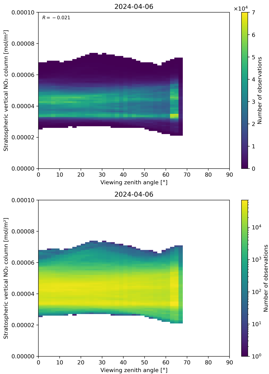
Figure 164: Scatter density plot of “Viewing zenith angle” against “Stratospheric vertical NO 2 column” for 2024-04-05 to 2024-04-07.
