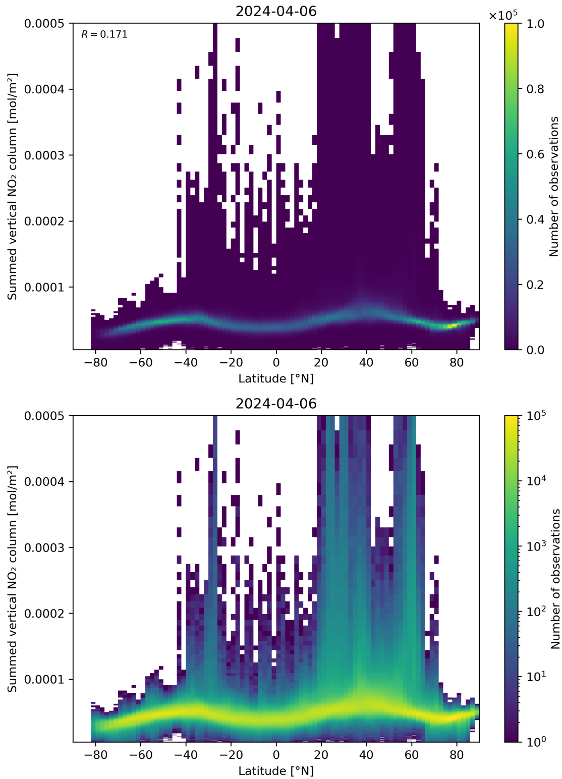
Figure 88: Scatter density plot of “Latitude” against “Summed vertical NO 2 column” for 2024-04-05 to 2024-04-07.
