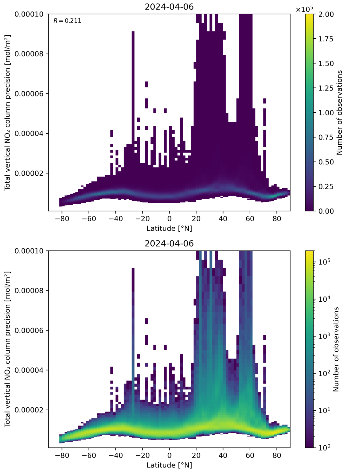
Figure 91: Scatter density plot of “Latitude” against “Total vertical NO 2 column precision” for 2024-04-05 to 2024-04-07.
