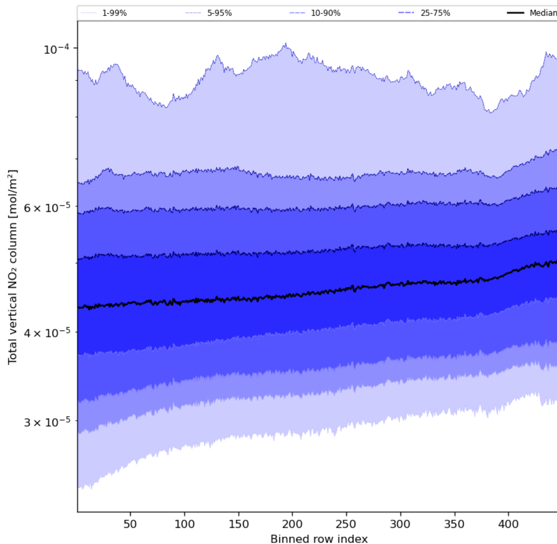
Figure 55: Along track statistics of “Total vertical NO 2 column” for 2024-04-05 to 2024-04-07
