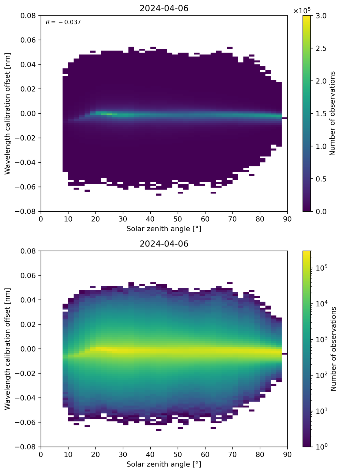
Figure 158: Scatter density plot of “Solar zenith angle” against “Wavelength calibration offset” for 2024-04-05 to 2024-04-07.
