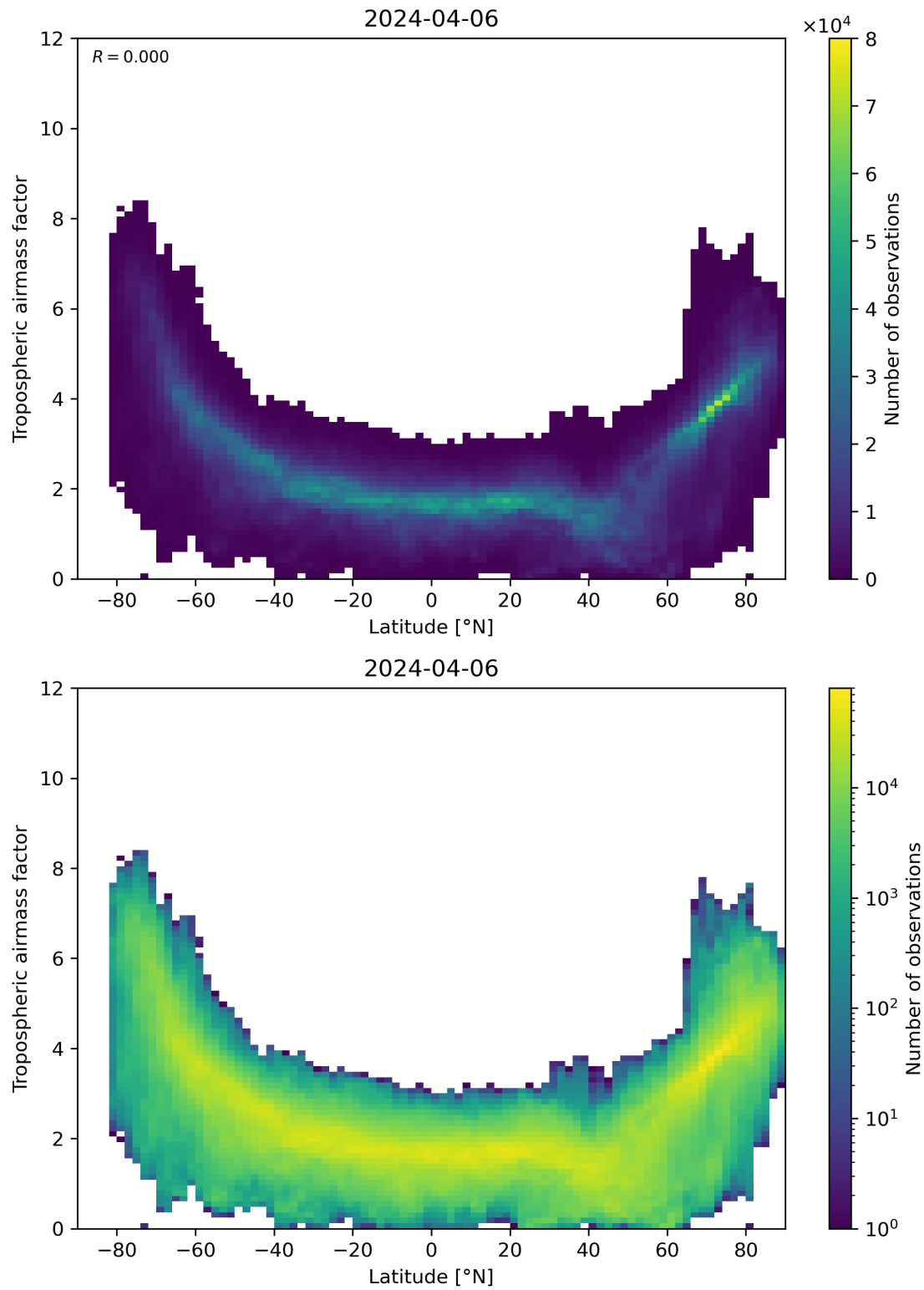
Figure 85: Scatter density plot of “Latitude” against “Tropospheric airmass factor” for 2024-04-05 to 2024-04-07.
