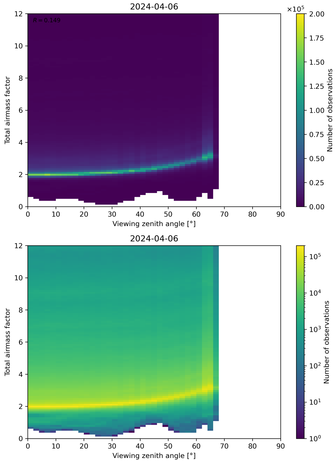
Figure 160: Scatter density plot of “Viewing zenith angle” against “Total airmass factor” for 2024-04-05 to 2024-04-07.
