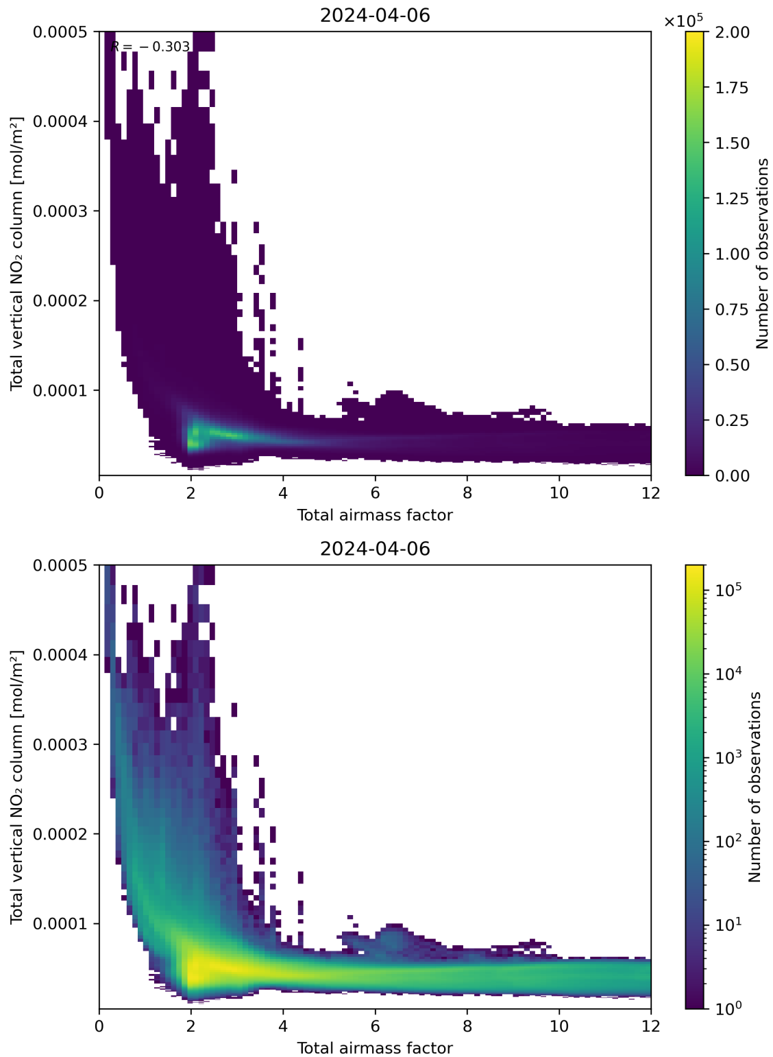
Figure 67: Scatter density plot of “Total airmass factor” against “Total vertical NO 2 column” for 2024-04-05 to 2024-04-07.
