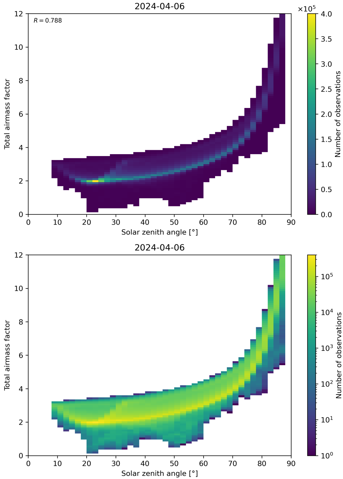
Figure 146: Scatter density plot of “Solar zenith angle” against “Total air mass factor” for 2024-04-05 to 2024-04-07.
