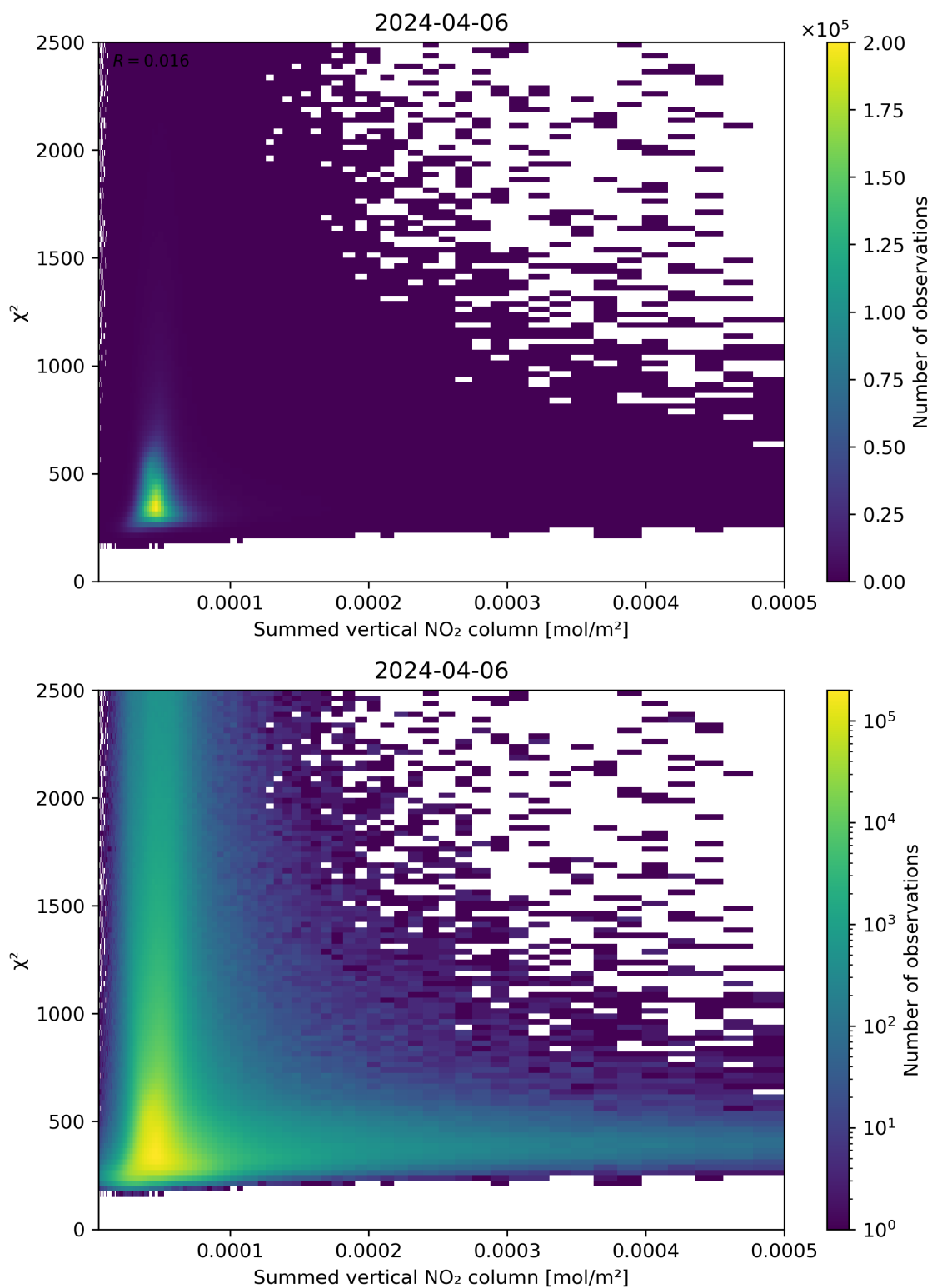
Figure 104: Scatter density plot of “Summed vertical NO 2 column” against “ \chi^2 ” for 2024-04-05 to 2024-04-07.
