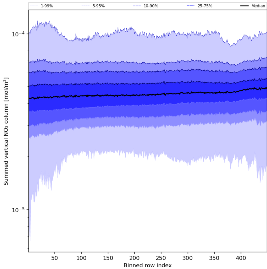
Figure 57: Along track statistics of “Summed vertical NO 2 column” for 2024-04-05 to 2024-04-07
