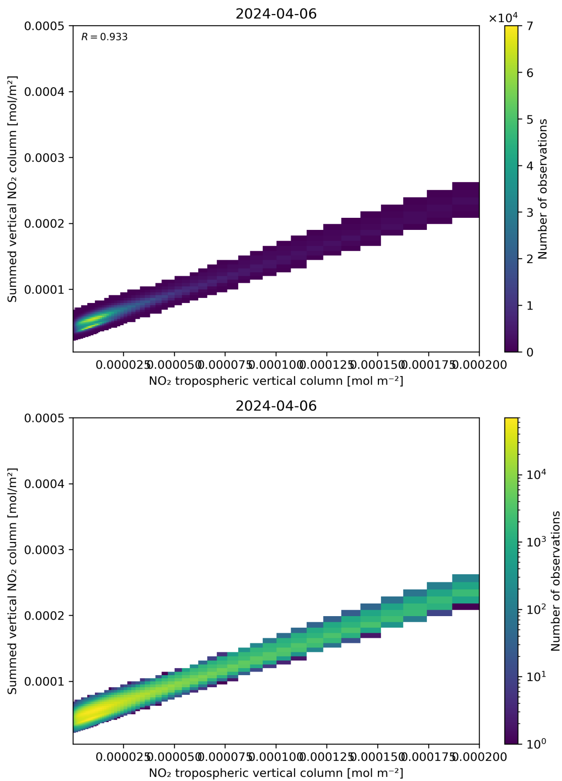
Figure 126: Scatter density plot of “NO 2 tropospheric vertical column” against “Summed vertical NO 2 column” for 2024-04-05 to 2024-04-07.
