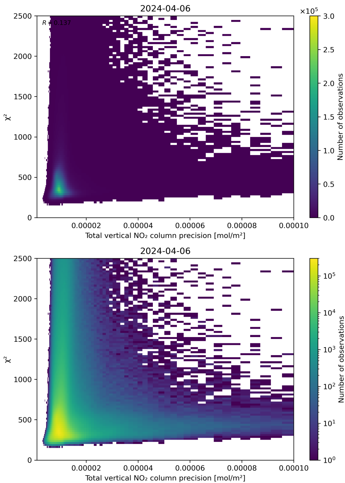
Figure 116: Scatter density plot of “Total vertical NO 2 column precision” against “ \chi^2 ” for 2024-04-05 to 2024-04-07.
