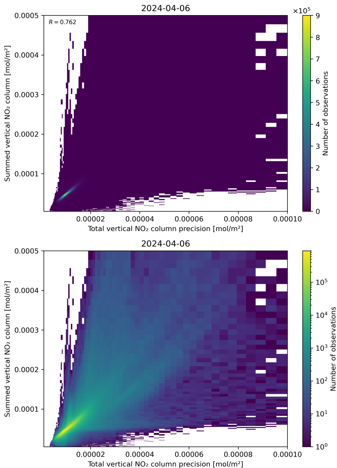
Figure 117: Scatter density plot of “Total vertical NO 2 column precision” against “Summed vertical NO 2 column” for 2024-04-05 to 2024-04-07.
