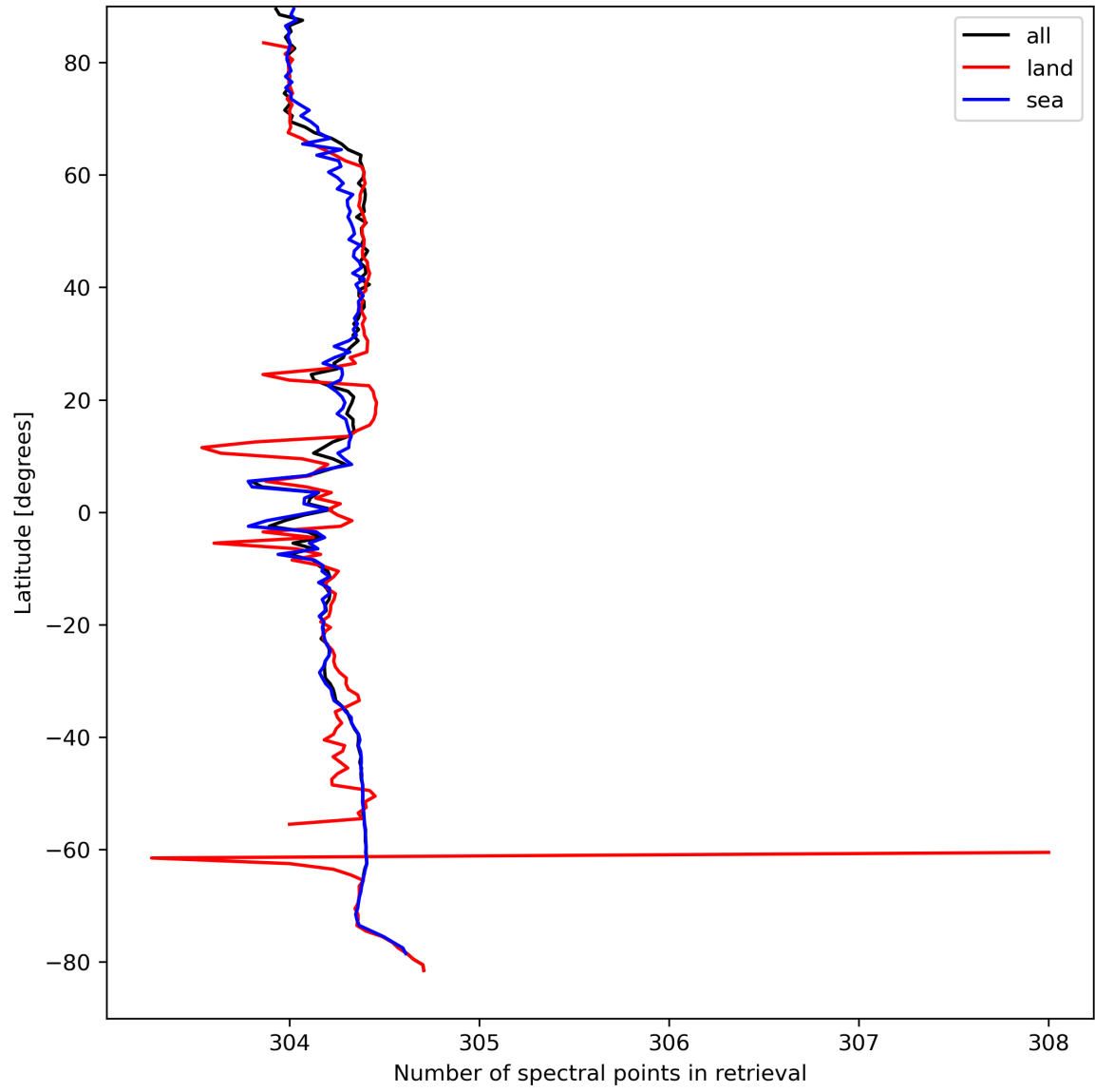
Figure 16: Zonal average of “Number of spectral points in retrieval” for 2024-04-05 to 2024-04-07.
