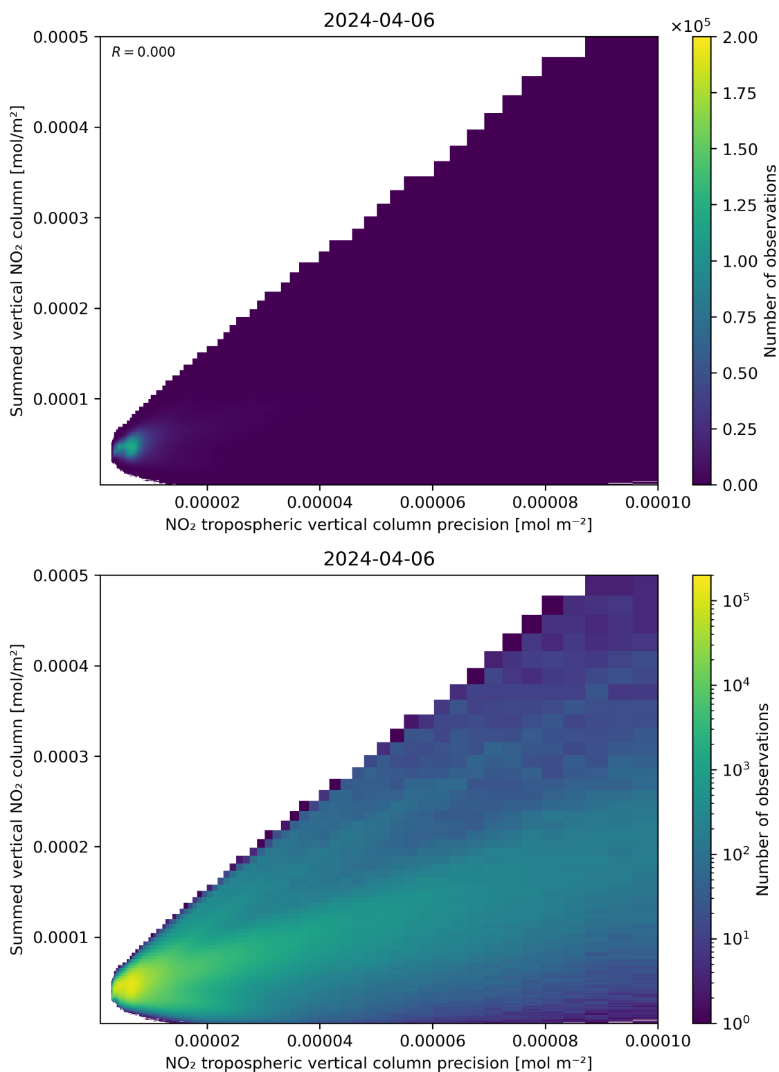
Figure 136: Scatter density plot of “NO 2 tropospheric vertical column precision” against “Summed vertical NO 2 column” for 2024-04-05 to 2024-04-07.
