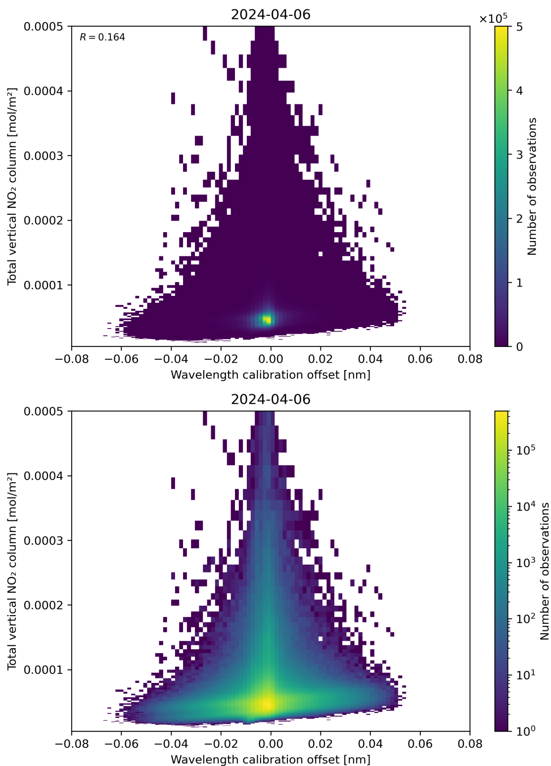
Figure 179: Scatter density plot of “Wavelength calibration offset” against “Total vertical NO 2 column” for 2024-04-05 to 2024-04-07.
