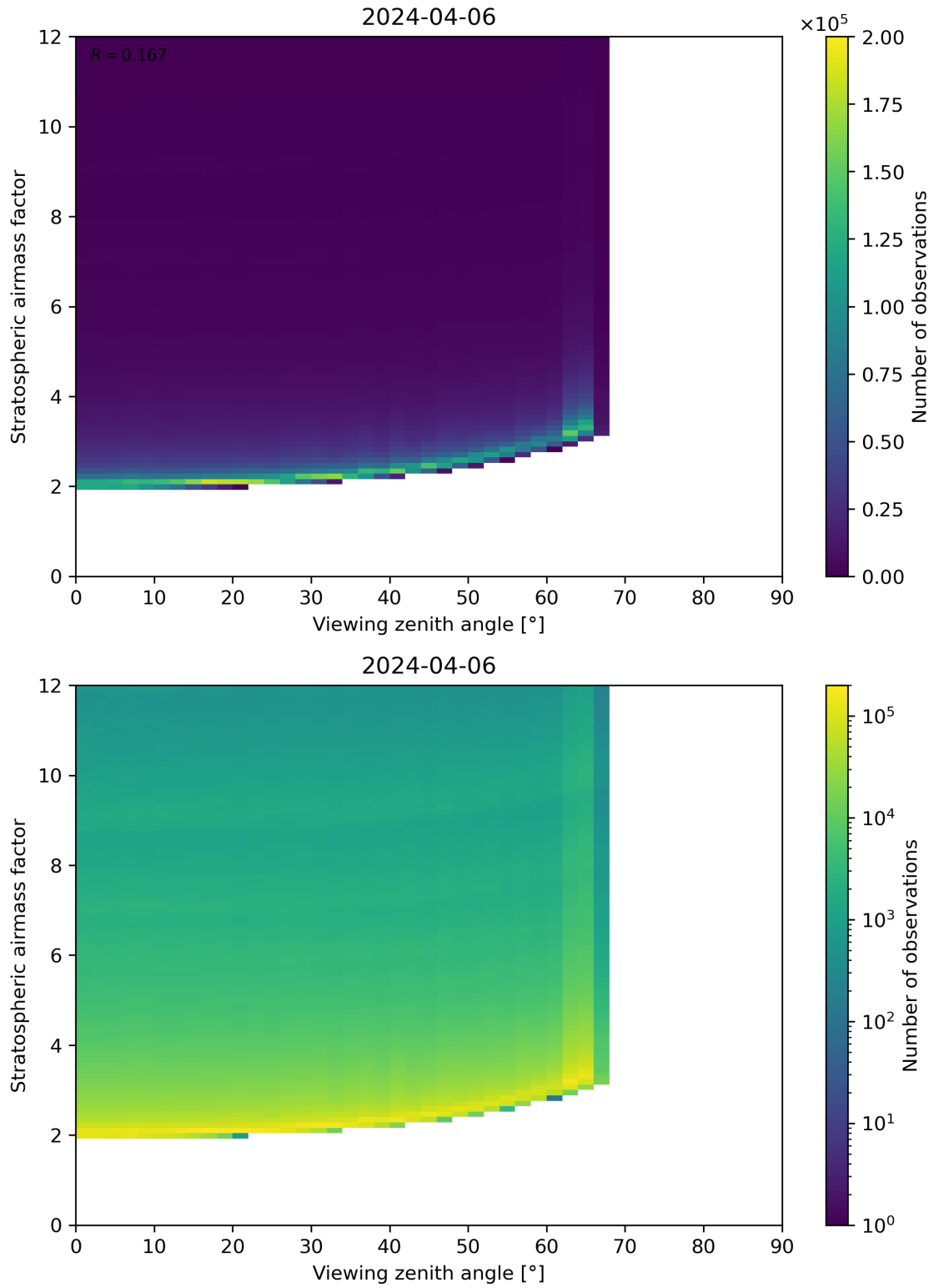
Figure 159: Scatter density plot of “Viewing zenith angle” against “Stratospheric airmass factor” for 2024-04-05 to 2024-04-07.
