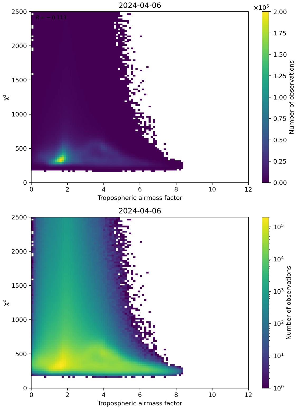
Figure 73: Scatter density plot of “Tropospheric airmass factor” against “ \chi^2 ” for 2024-04-05 to 2024-04-07.
