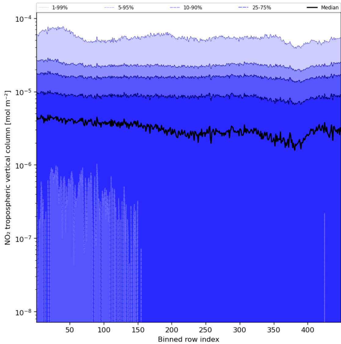
Figure 46: Along track statistics of “NO 2 tropospheric vertical column” for 2024-04-05 to 2024-04-07
