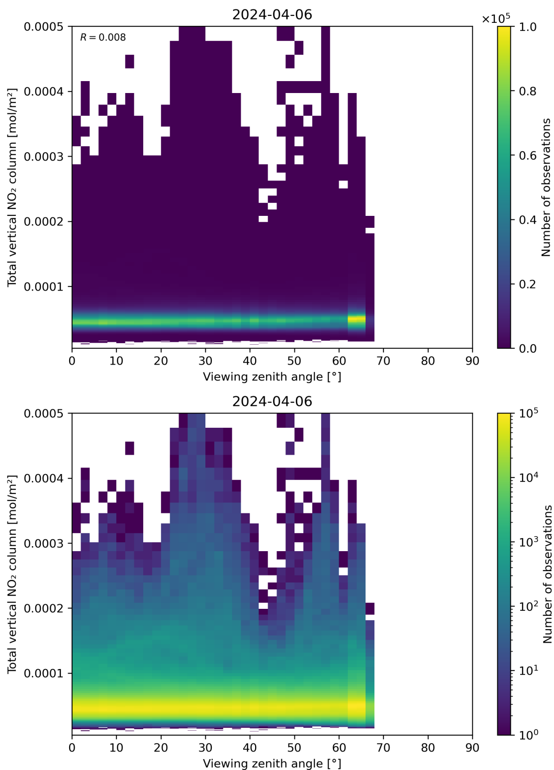
Figure 167: Scatter density plot of “Viewing zenith angle” against “Total vertical NO 2 column” for 2024-04-05 to 2024-04-07.
