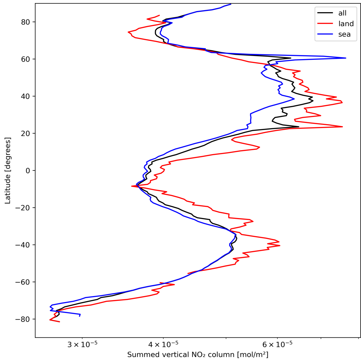
Figure 23: Zonal average of “Summed vertical NO 2 column” for 2024-04-05 to 2024-04-07.
