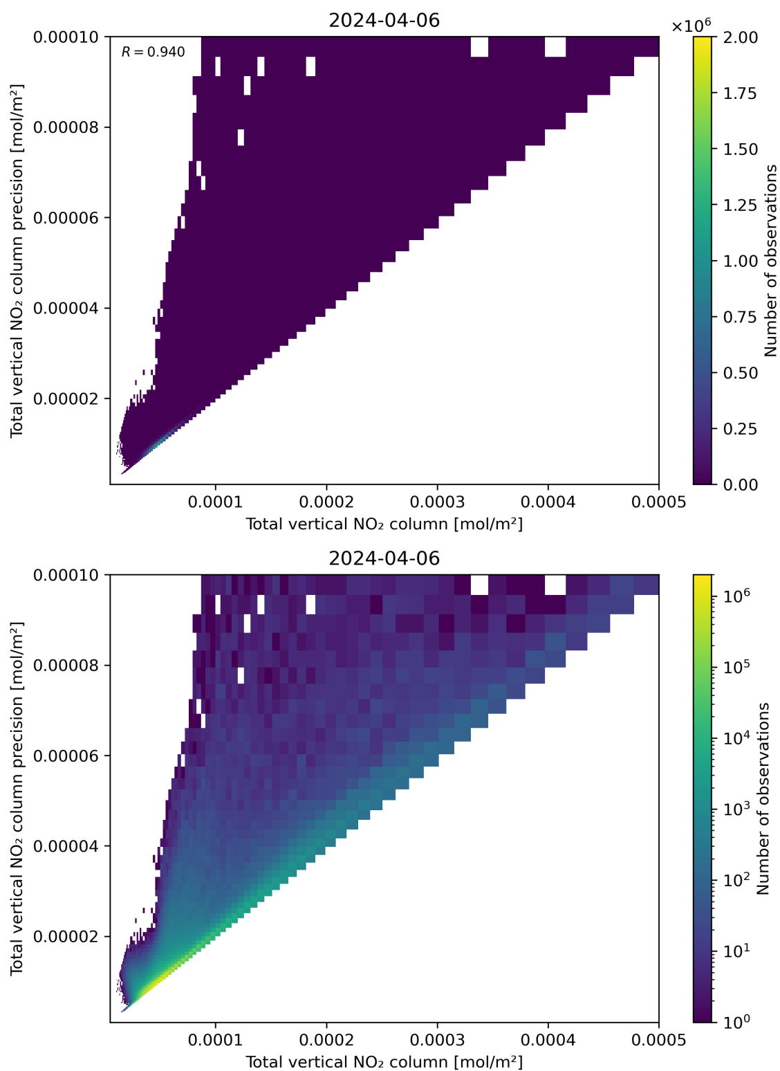
Figure 114: Scatter density plot of “Total vertical NO 2 column” against “Total vertical NO 2 column precision” for 2024-04-05 to 2024-04-07.
