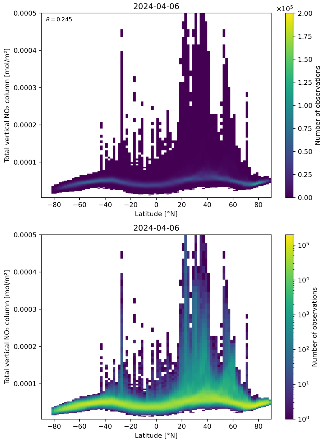
Figure 90: Scatter density plot of “Latitude” against “Total vertical NO 2 column” for 2024-04-05 to 2024-04-07.
