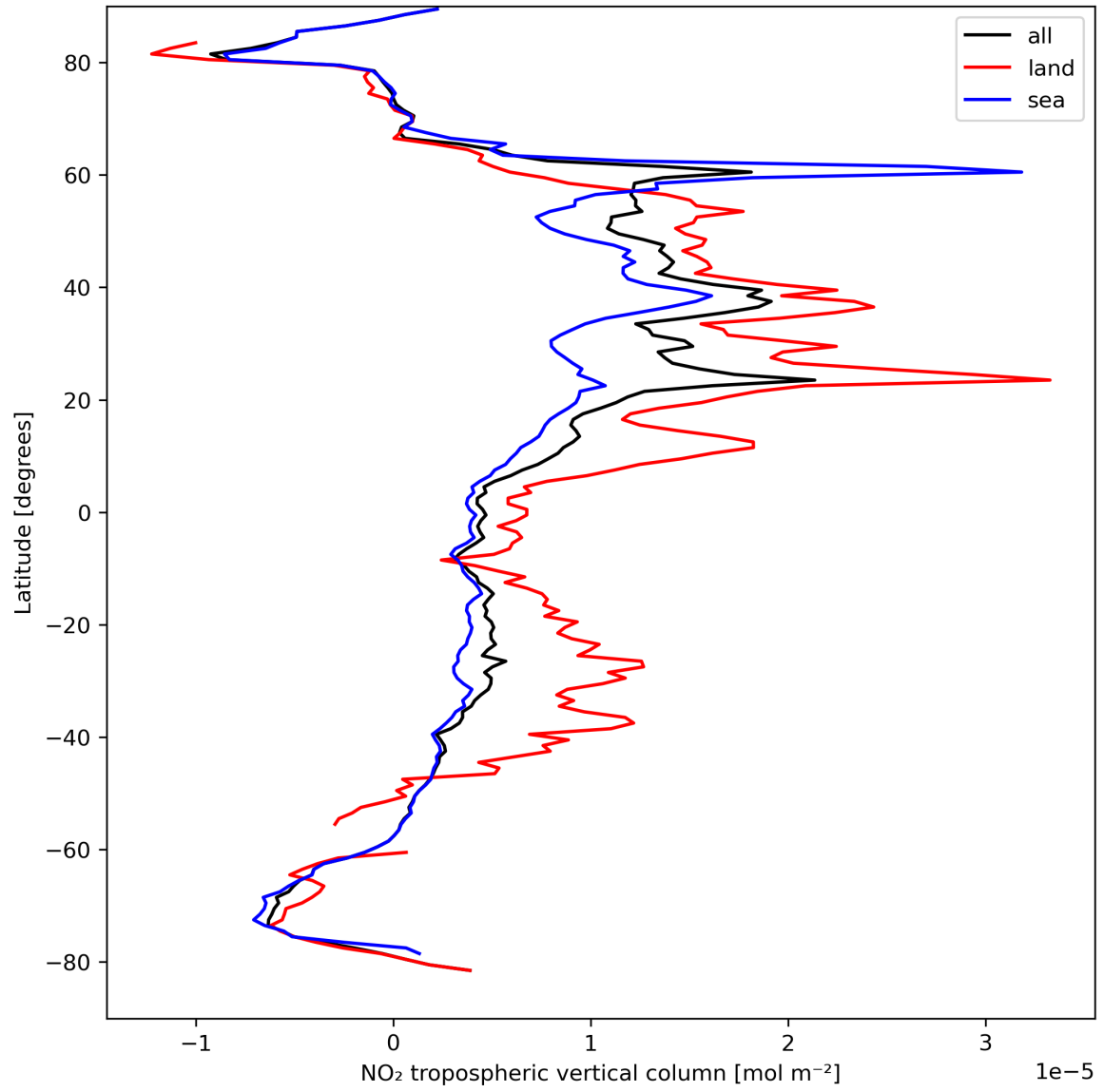
Figure 12: Zonal average of “NO 2 tropospheric vertical column” for 2024-04-05 to 2024-04-07.
