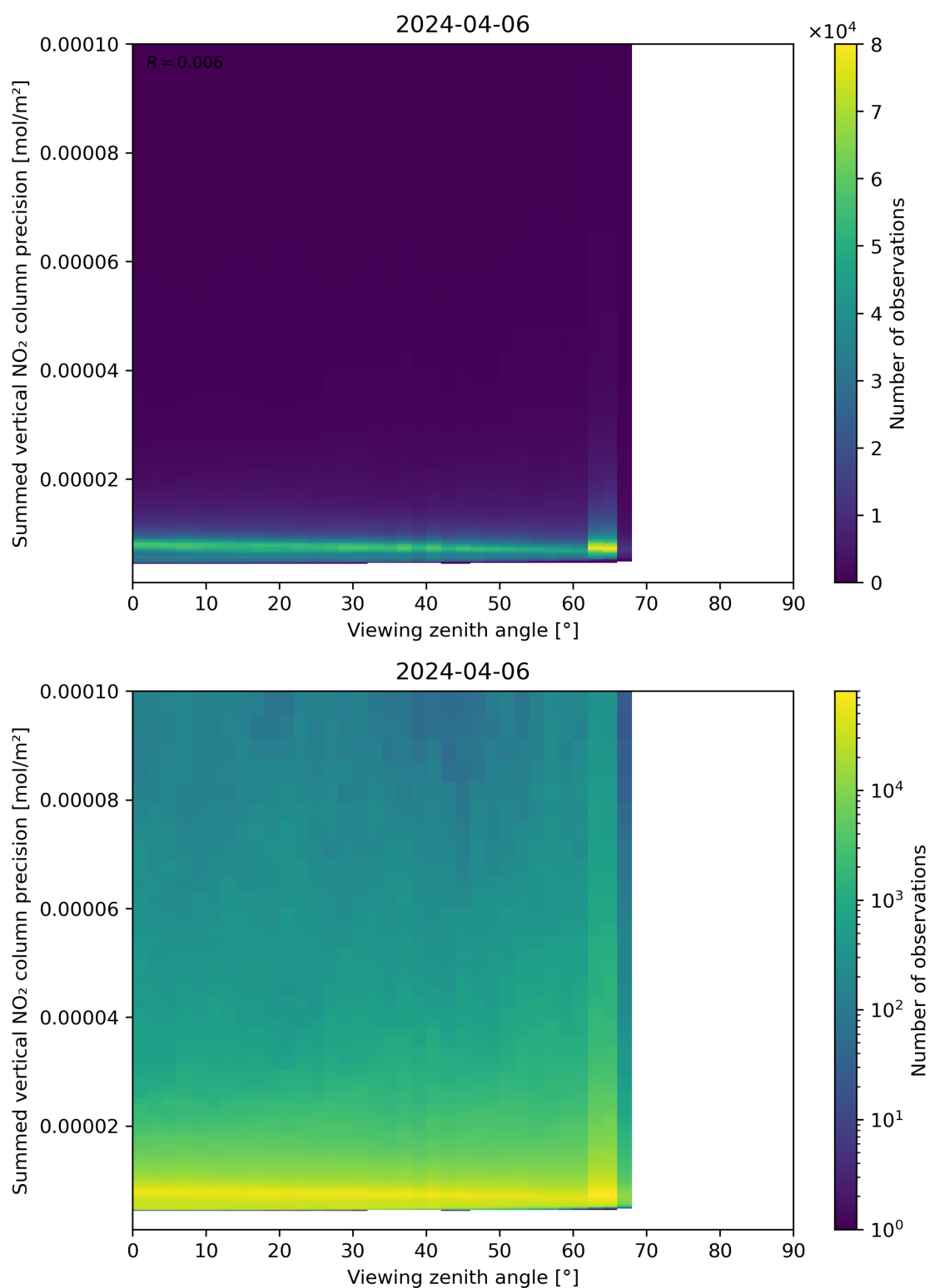
Figure 166: Scatter density plot of “Viewing zenith angle” against “Summed vertical NO 2 column precision” for 2024-04-05 to 2024-04-07.
