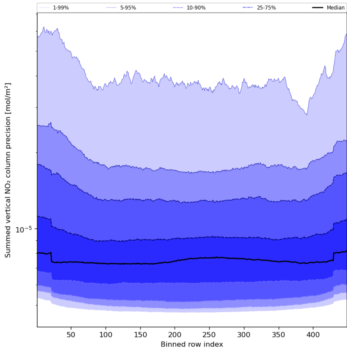
Figure 58: Along track statistics of “Summed vertical NO 2 column precision” for 2024-04-05 to 2024-04-07
