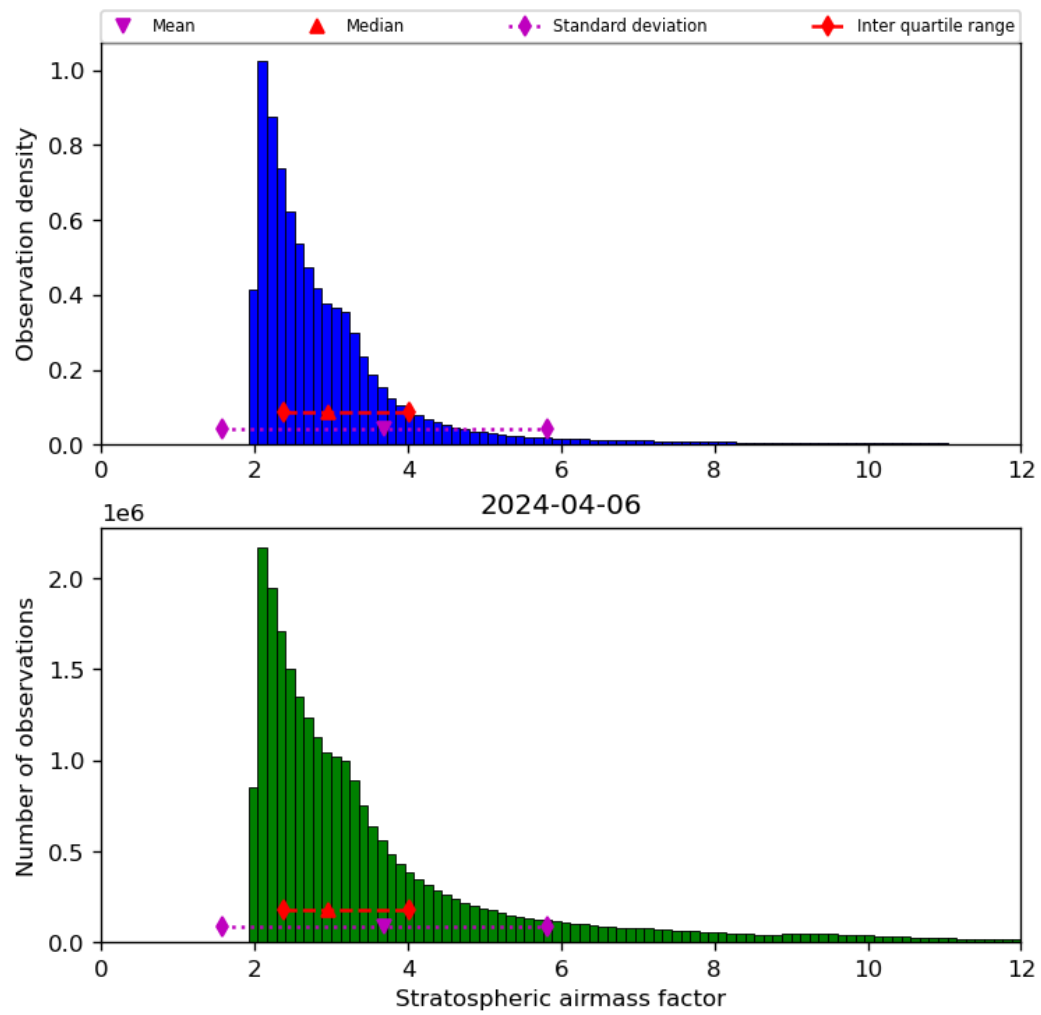
Figure 44: Histogram of “Stratospheric airmass factor” for 2024-04-05 to 2024-04-07
