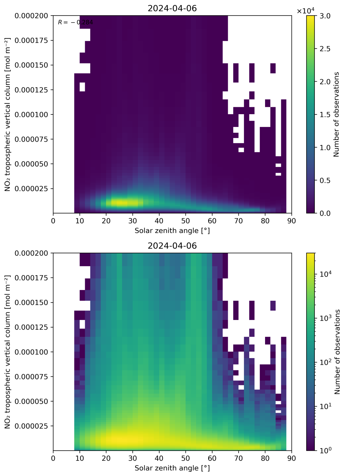
Figure 155: Scatter density plot of “Solar zenith angle” against “NO 2 tropospheric vertical column” for 2024-04-05 to 2024-04-07.
