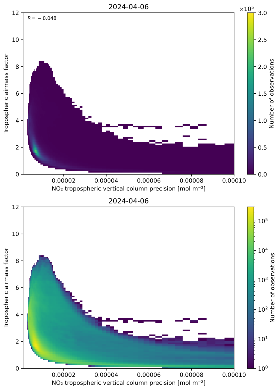
Figure 133: Scatter density plot of “NO 2 tropospheric vertical column precision” against “Tropospheric airmass factor” for 2024-04-05 to 2024-04-07.
