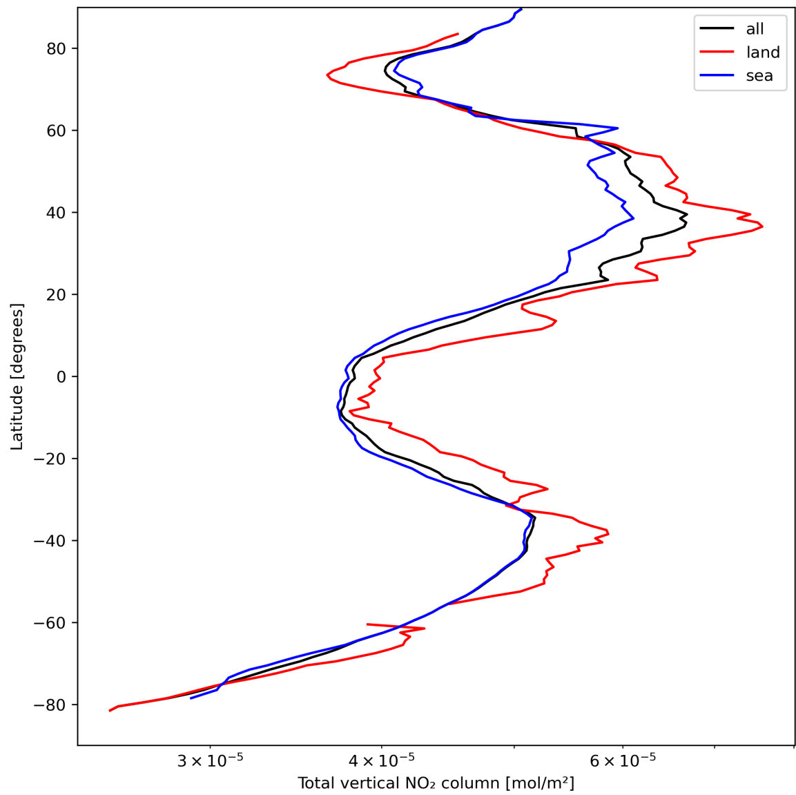
Figure 21: Zonal average of “Total vertical NO 2 column” for 2024-04-05 to 2024-04-07.
