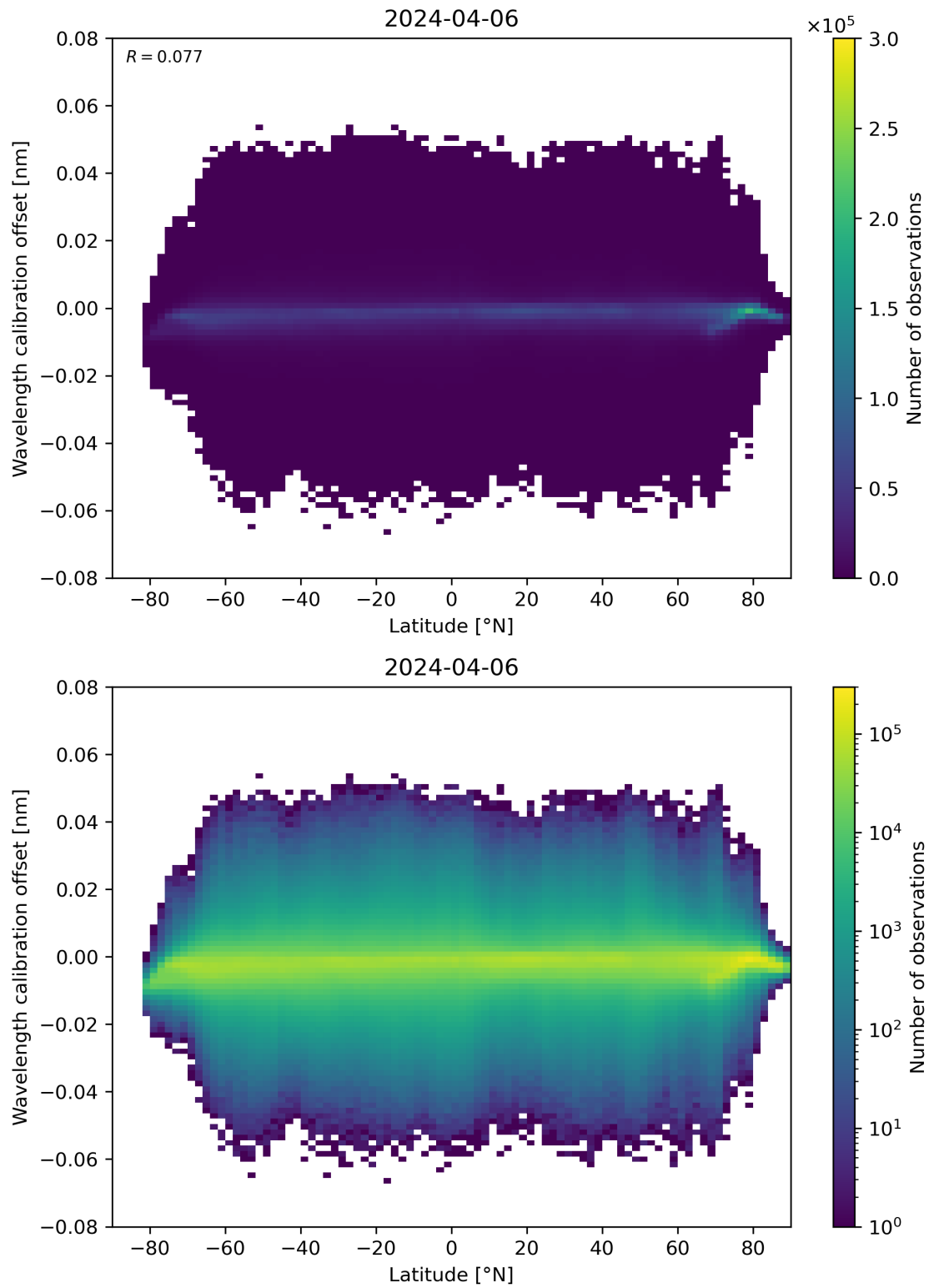
Figure 95: Scatter density plot of “Latitude” against “Wavelength calibration offset” for 2024-04-05 to 2024-04-07.
