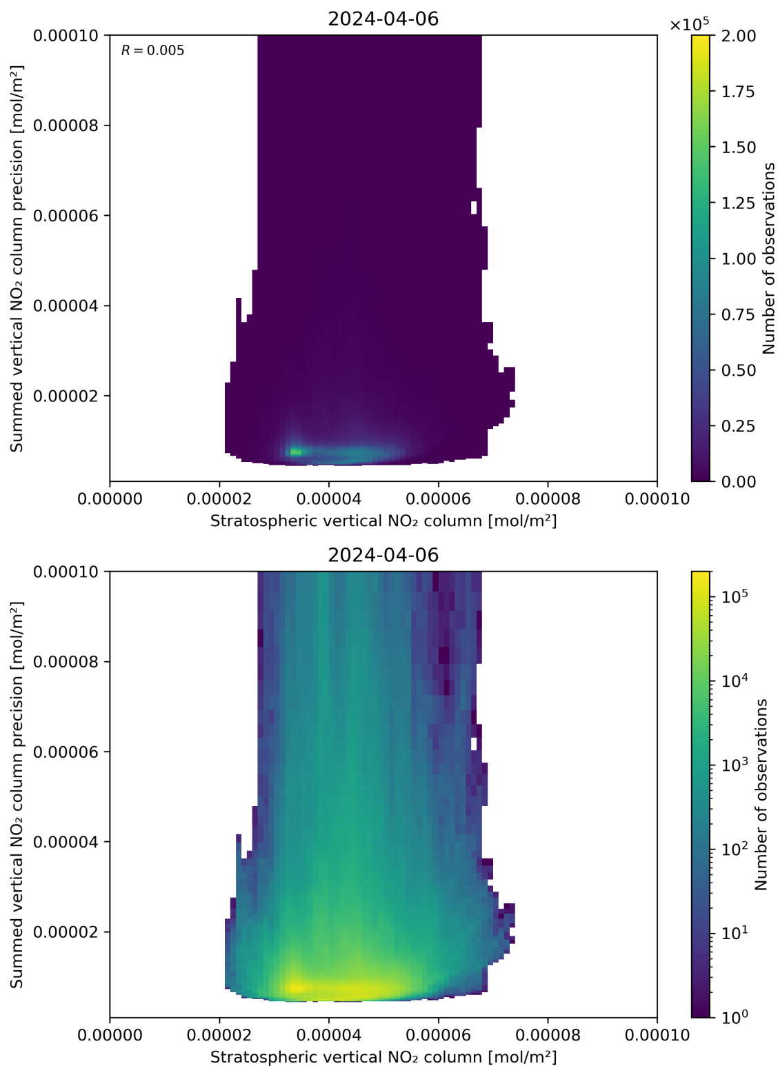
Figure 99: Scatter density plot of “Stratospheric vertical NO 2 column” against “Summed vertical NO 2 column precision” for 2024-04-05 to 2024-04-07.
