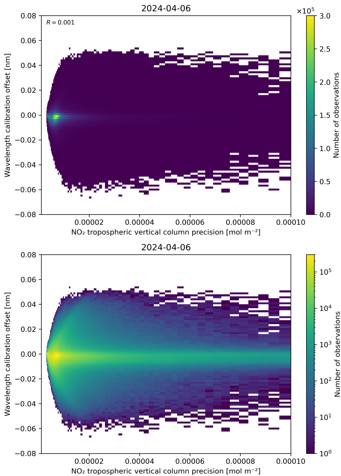
Figure 141: Scatter density plot of “NO 2 tropospheric vertical column precision” against “Wavelength calibration offset” for 2024-04-05 to 2024-04-07.
