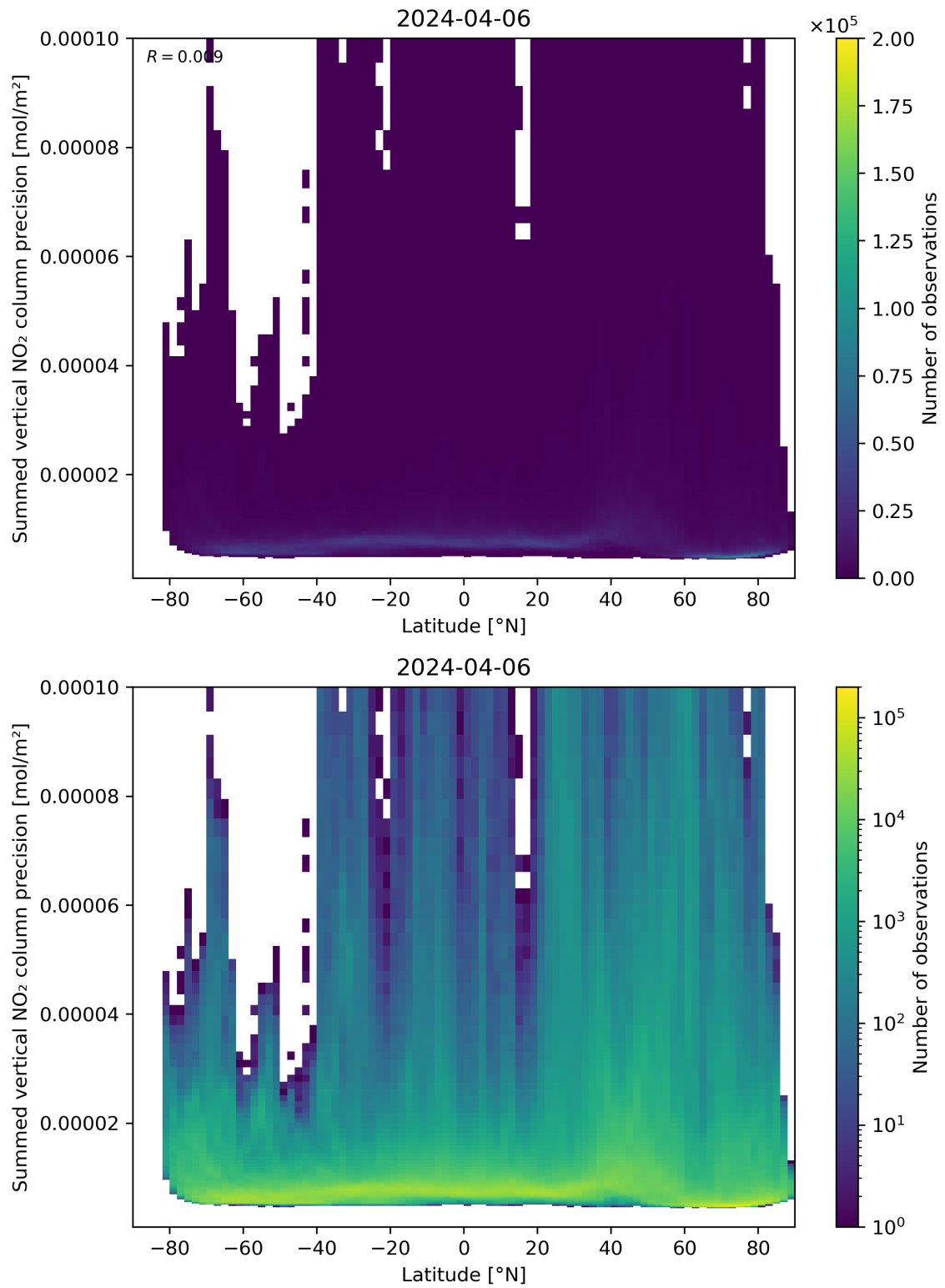
Figure 89: Scatter density plot of “Latitude” against “Summed vertical NO 2 column precision” for 2024-04-05 to 2024-04-07.
