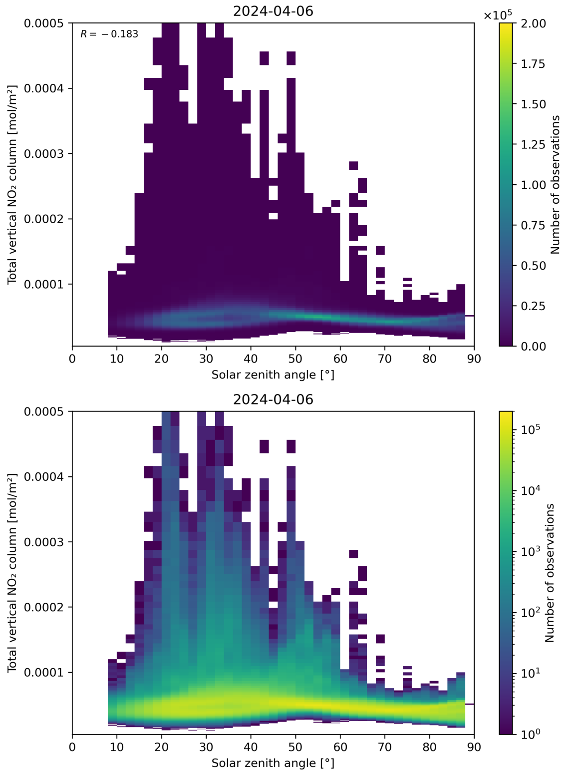
Figure 153: Scatter density plot of “Solar zenith angle” against “Total vertical NO 2 column” for 2024-04-05 to 2024-04-07.
