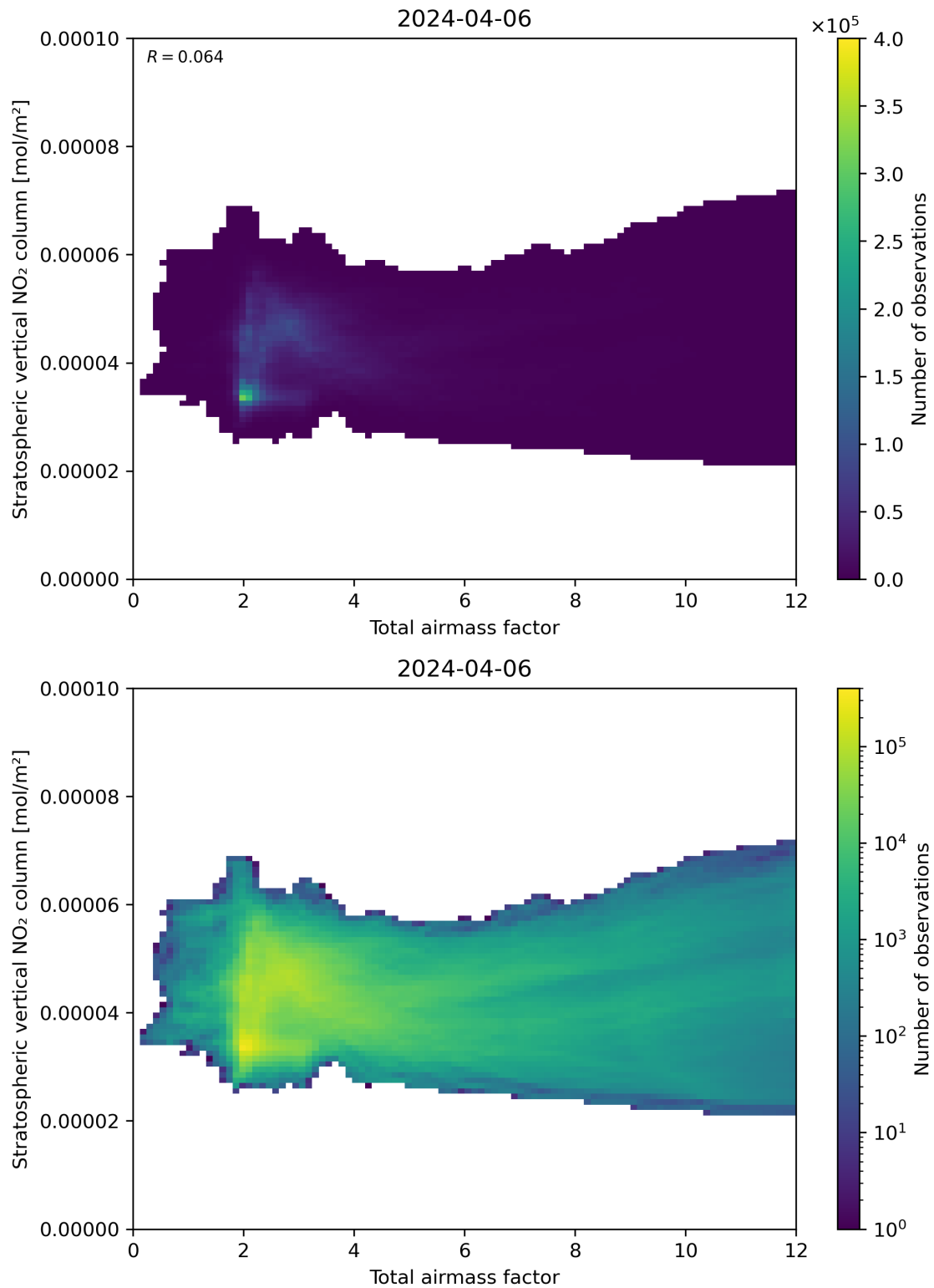
Figure 64: Scatter density plot of “Total airmass factor” against “Stratospheric vertical NO 2 column” for 2024-04-05 to 2024-04-07.
