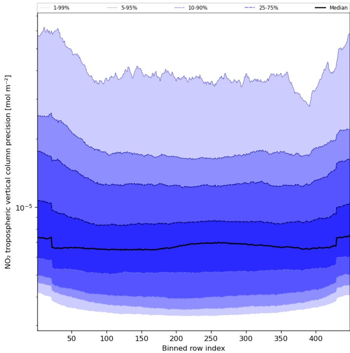
Figure 47: Along track statistics of “NO 2 tropospheric vertical column precision” for 2024-04-05 to 2024-04-07
