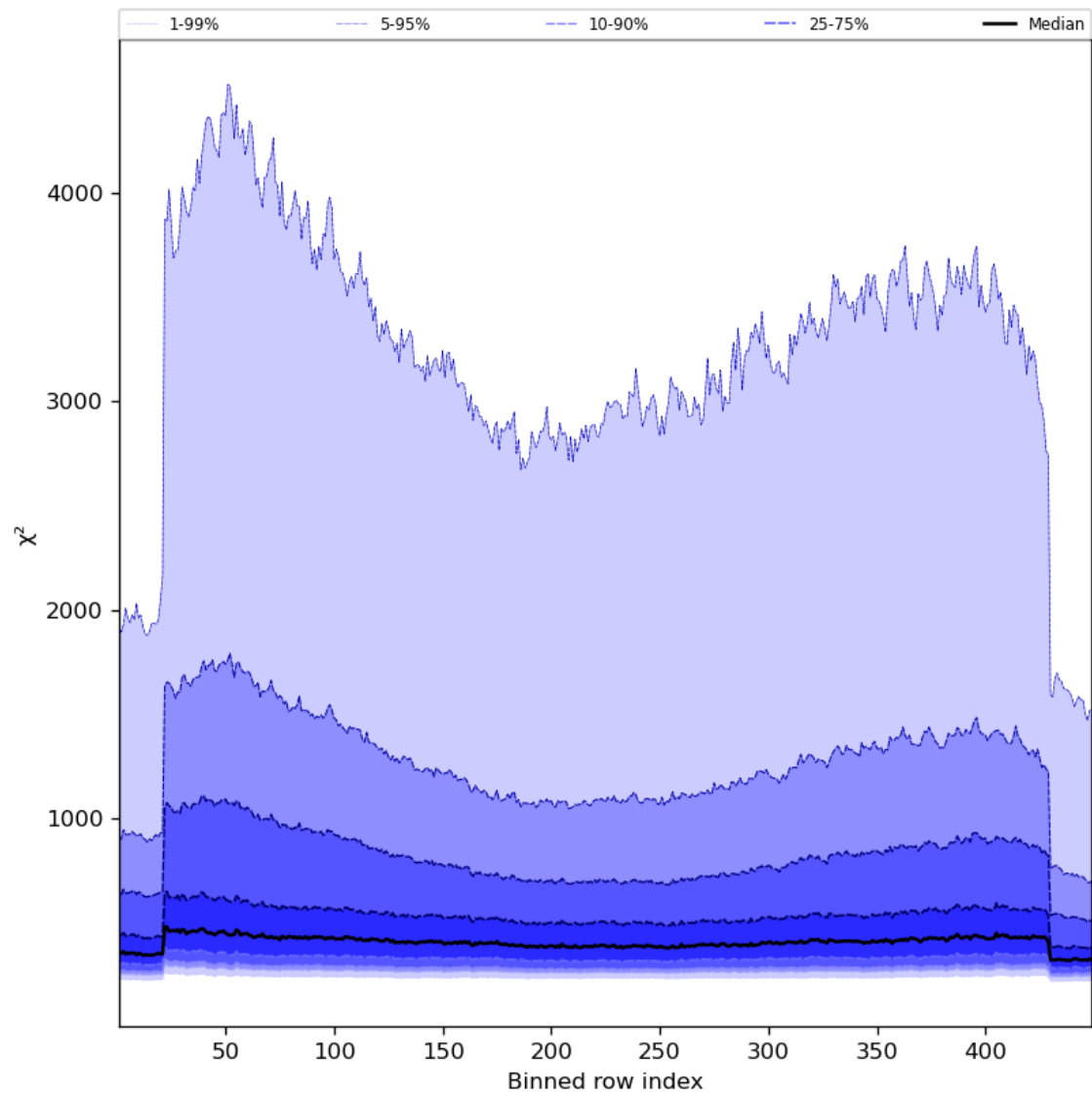
Figure 59: Along track statistics of “ \chi^2 ” for 2024-04-05 to 2024-04-07
