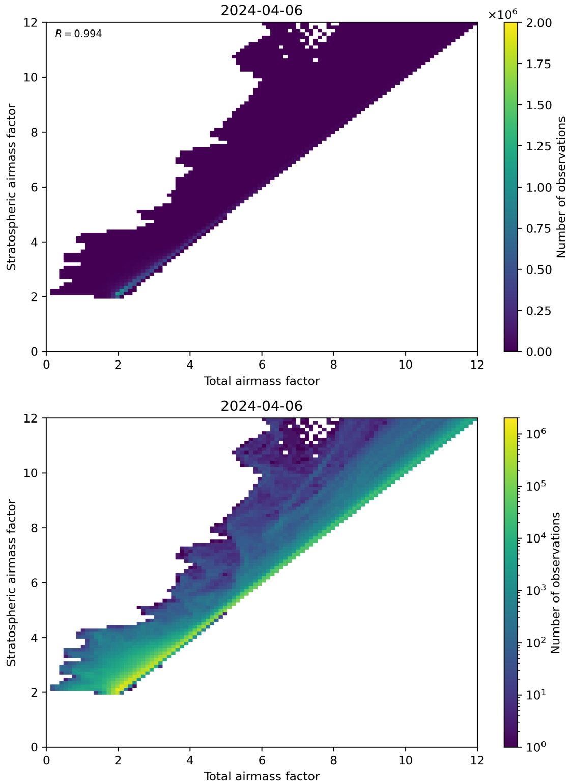
Figure 62: Scatter density plot of “Total air mass factor” against “Stratospheric air mass factor” for 2024-04-05 to 2024-04-07.
