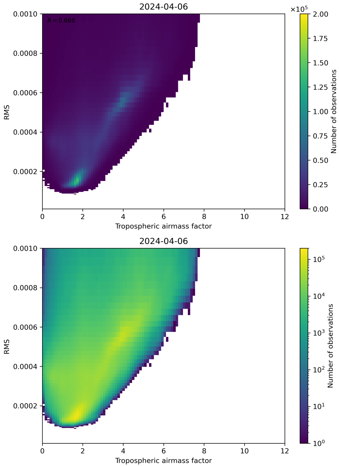
Figure 79: Scatter density plot of “Tropospheric airmass factor” against “RMS” for 2024-04-05 to 2024-04-07.
