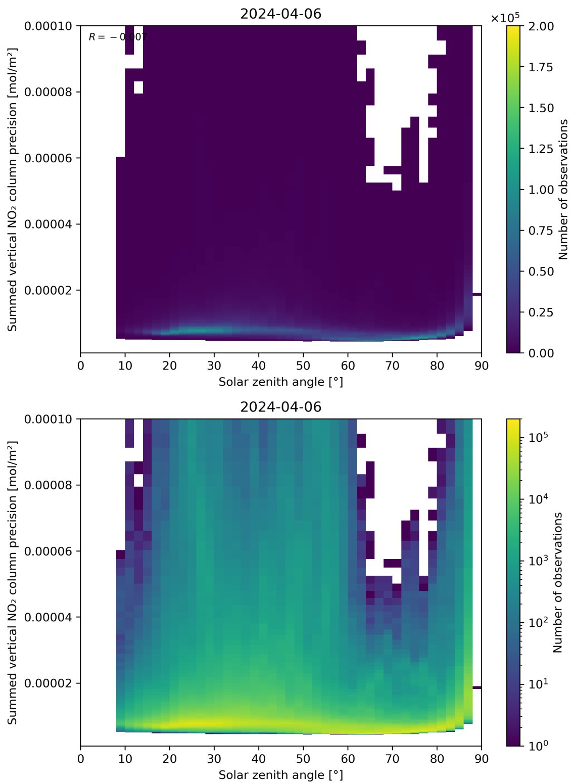
Figure 152: Scatter density plot of “Solar zenith angle” against “Summed vertical NO 2 column precision” for 2024-04-05 to 2024-04-07.
