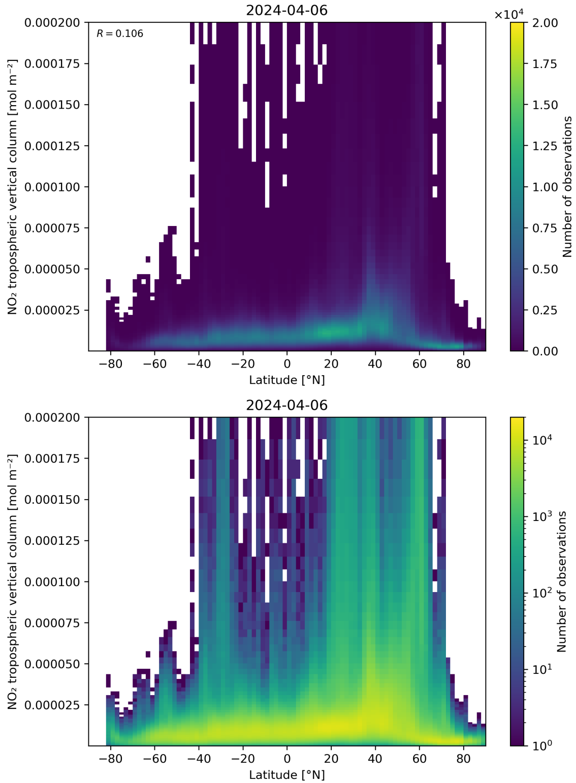
Figure 92: Scatter density plot of “Latitude” against “NO 2 tropospheric vertical column” for 2024-04-05 to 2024-04-07.
