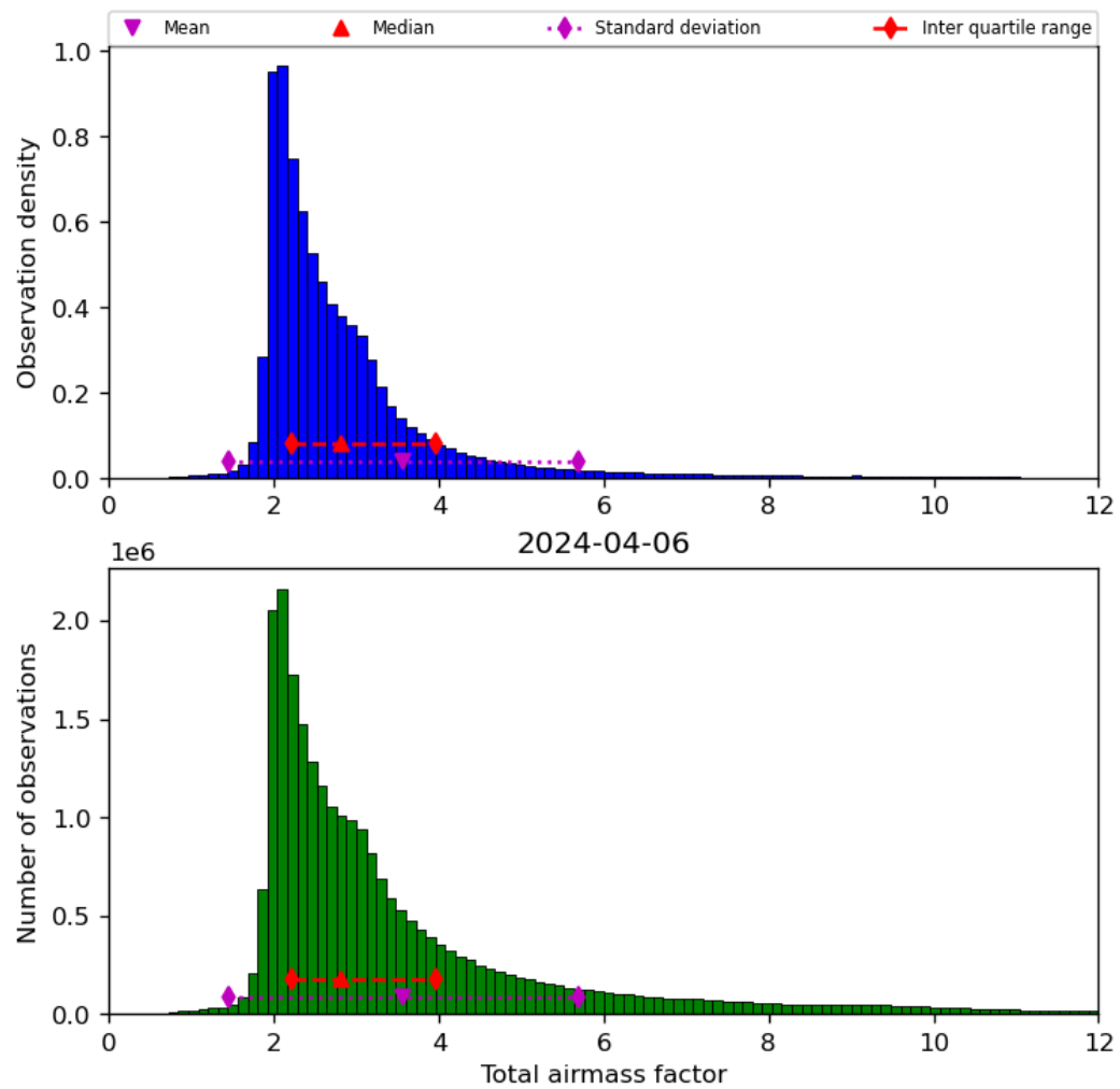
Figure 32: Histogram of “Total airmass factor” for 2024-04-05 to 2024-04-07
