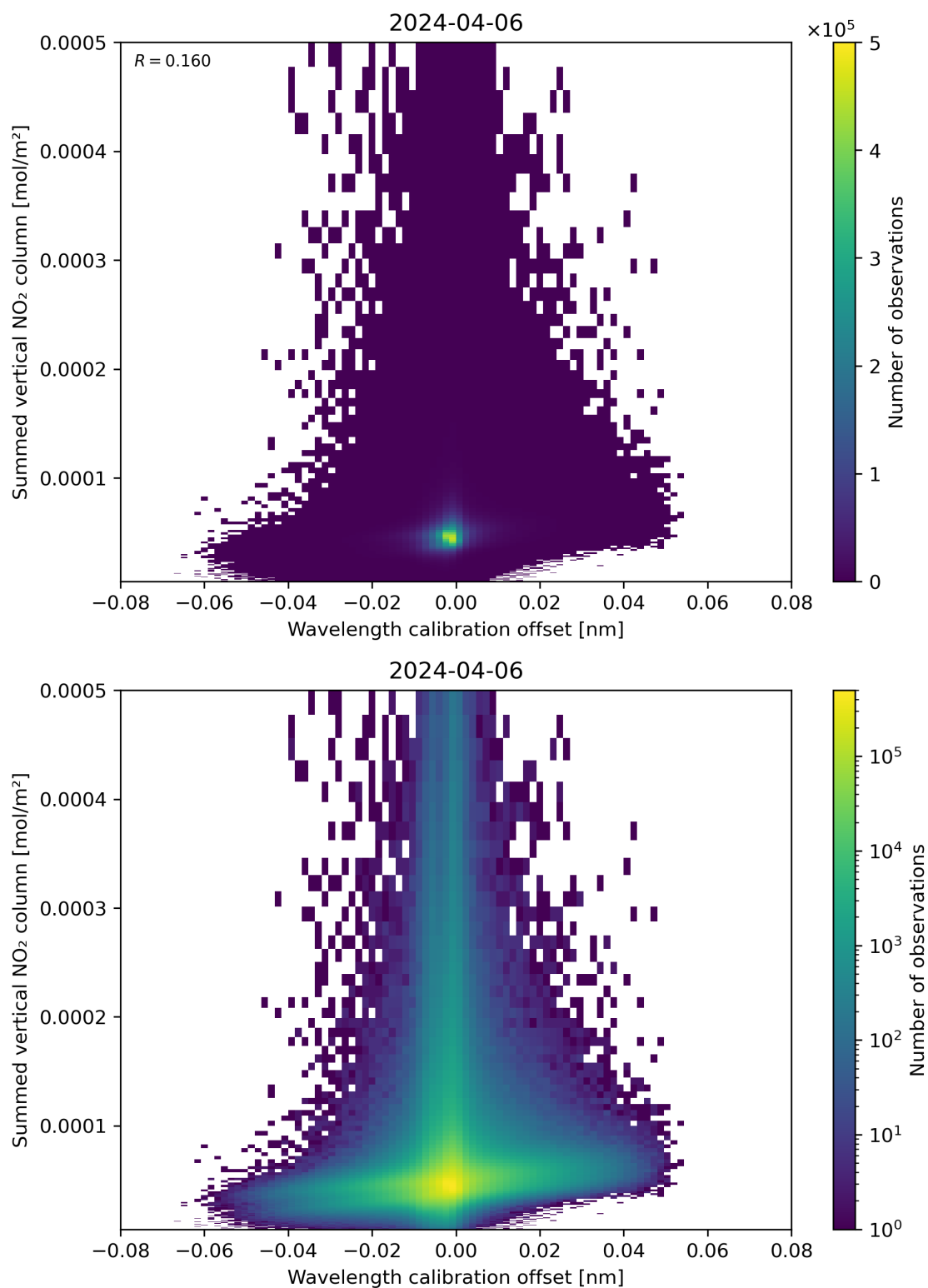
Figure 177: Scatter density plot of “Wavelength calibration offset” against “Summed vertical NO 2 column” for 2024-04-05 to 2024-04-07.
