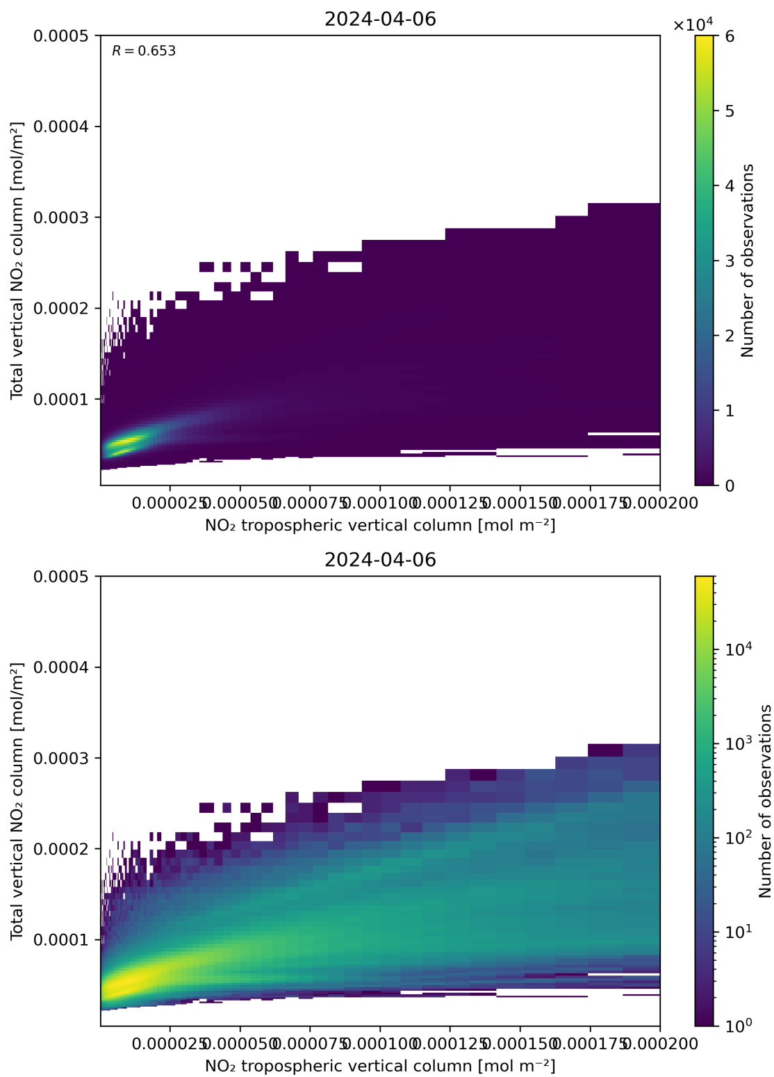
Figure 128: Scatter density plot of “NO 2 tropospheric vertical column” against “Total vertical NO 2 column” for 2024-04-05 to 2024-04-07.
