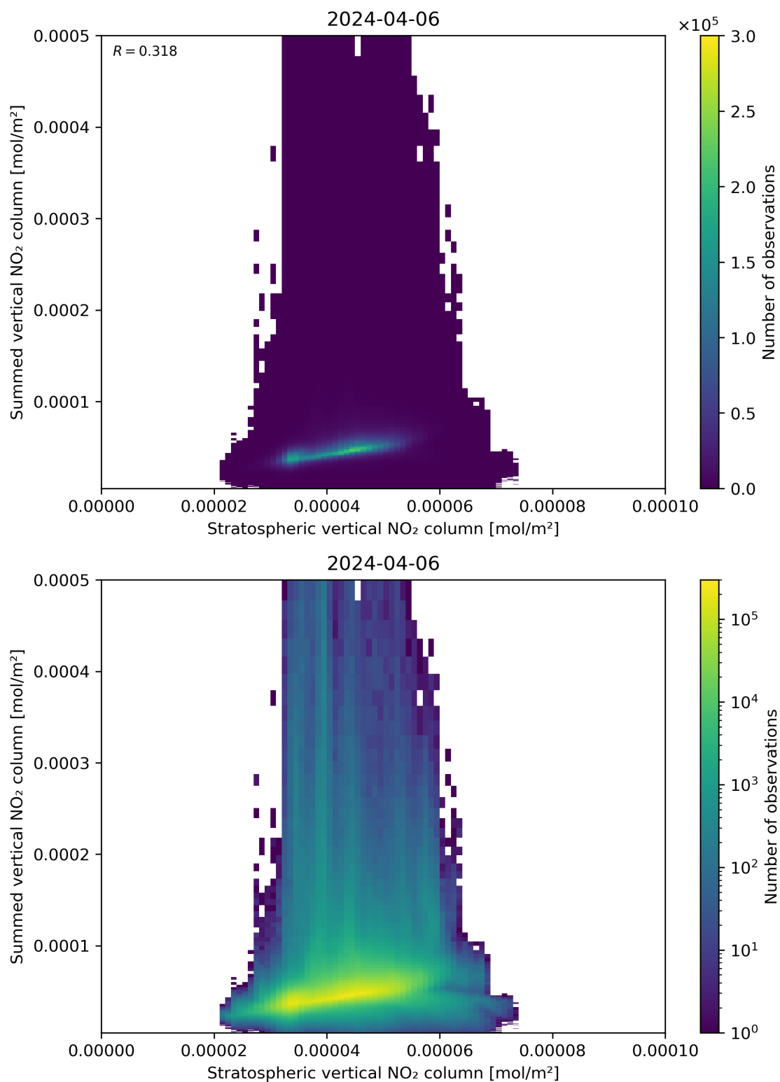
Figure 98: Scatter density plot of “Stratospheric vertical NO 2 column” against “Summed vertical NO 2 column” for 2024-04-05 to 2024-04-07.
