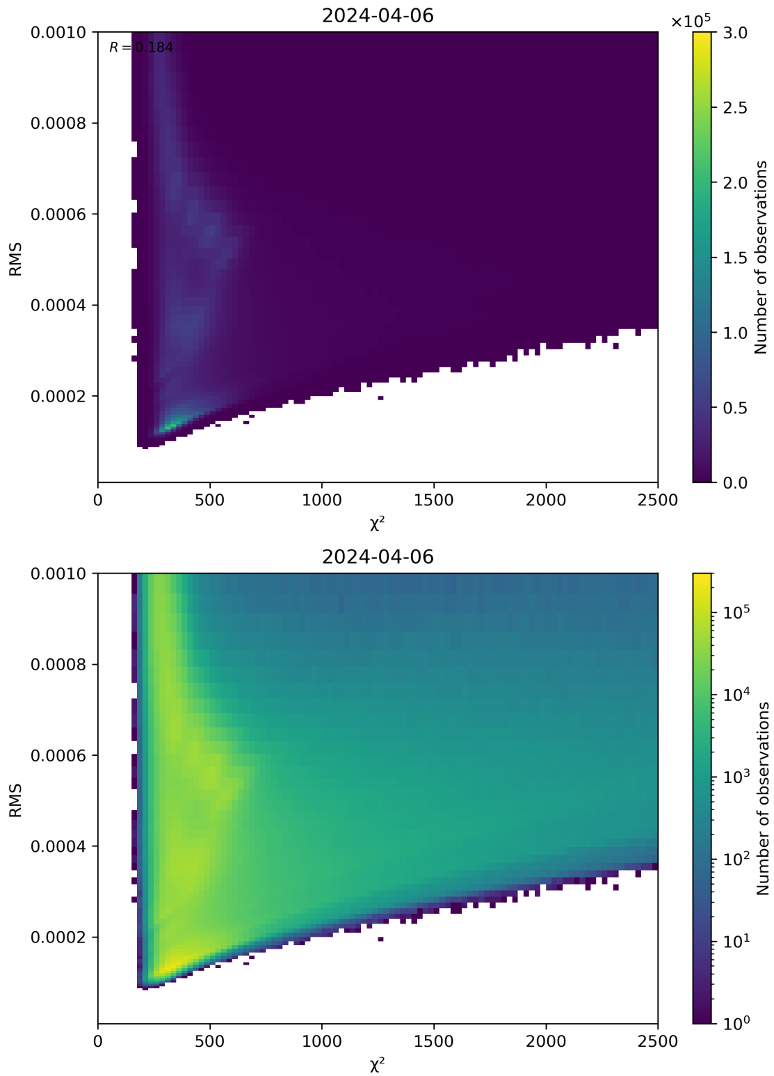
Figure 82: Scatter density plot of “ \chi^2 ” against “RMS” for 2024-04-05 to 2024-04-07.
