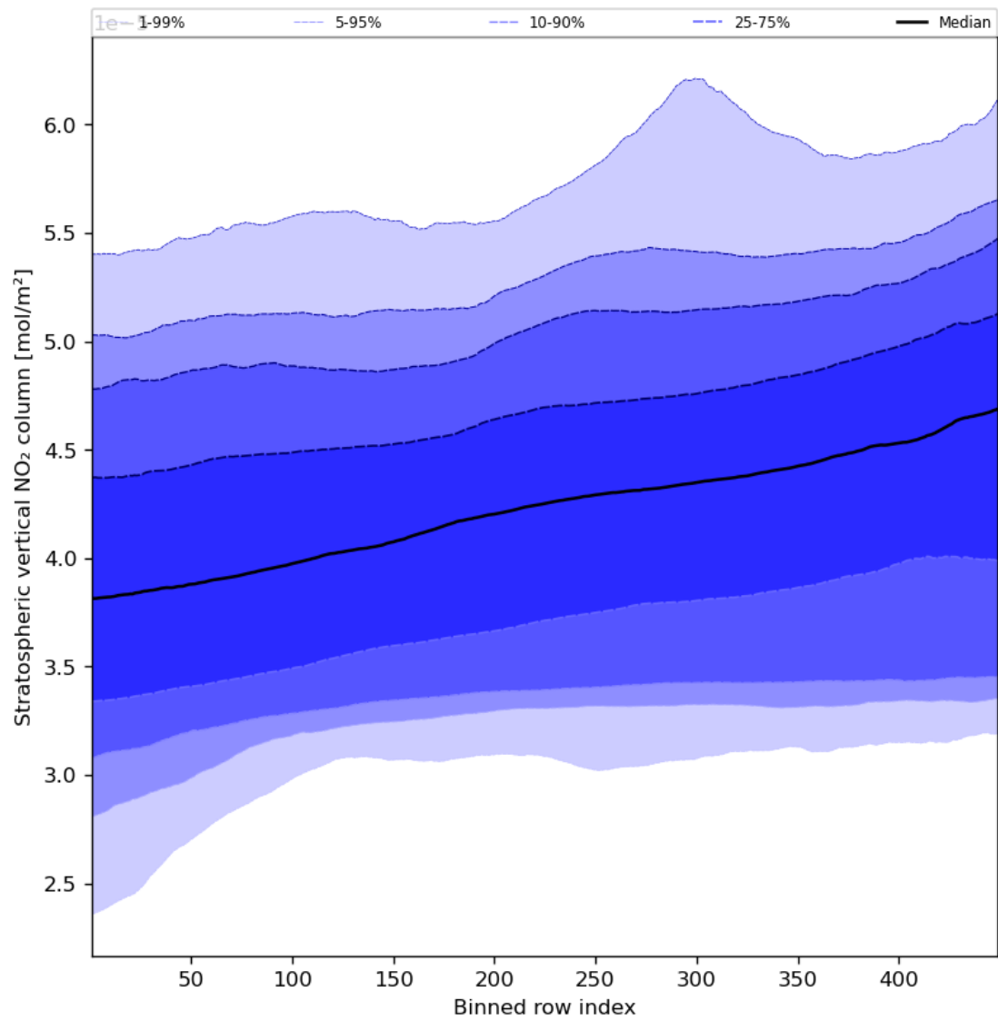
Figure 53: Along track statistics of “Stratospheric vertical NO 2 column” for 2024-04-05 to 2024-04-07
