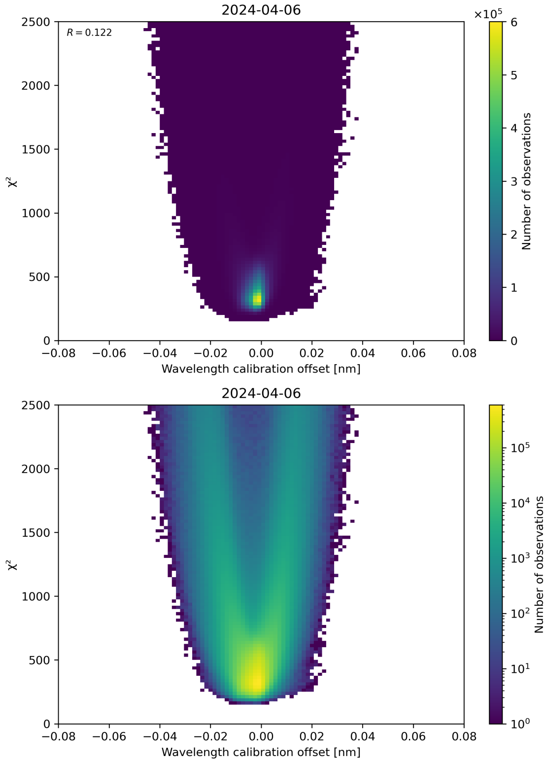
Figure 175: Scatter density plot of “Wavelength calibration offset” against “ \chi^2 ” for 2024-04-05 to 2024-04-07.
