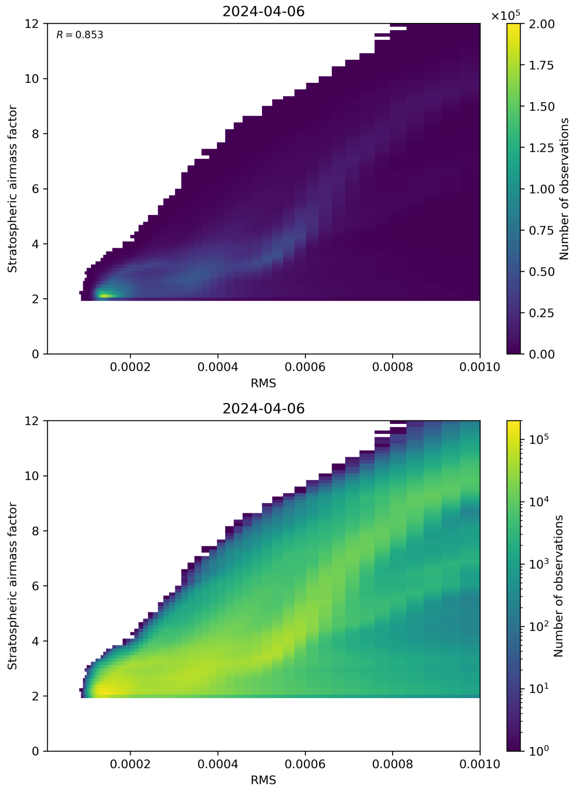
Figure 144: Scatter density plot of “RMS” against “Stratospheric airmass factor” for 2024-04-05 to 2024-04-07.
