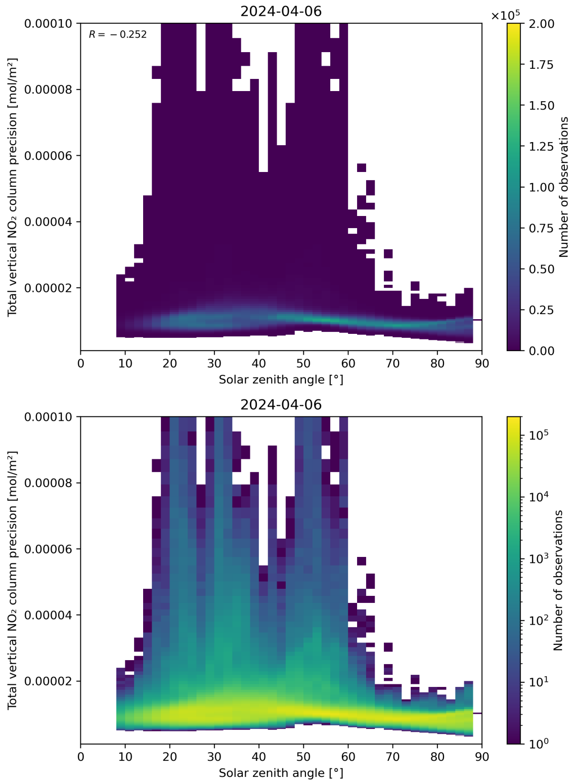
Figure 154: Scatter density plot of “Solar zenith angle” against “Total vertical NO 2 column precision” for 2024-04-05 to 2024-04-07.
