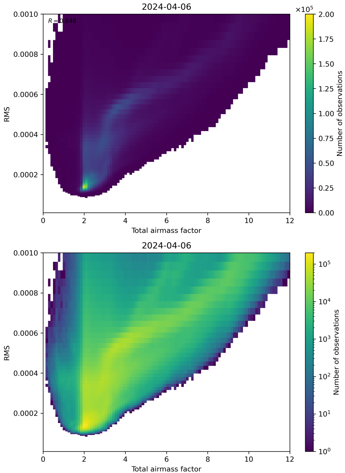
Figure 69: Scatter density plot of “Total airmass factor” against “RMS” for 2024-04-05 to 2024-04-07.
