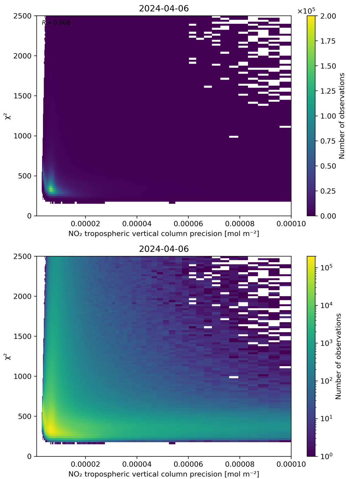
Figure 134: Scatter density plot of “NO 2 tropospheric vertical column precision” against “ \chi^2 ” for 2024-04-05 to 2024-04-07.
