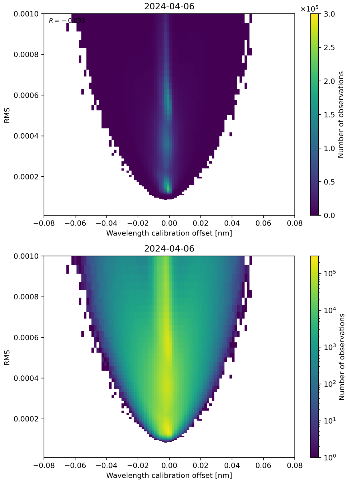
Figure 181: Scatter density plot of “Wavelength calibration offset” against “RMS” for 2024-04-05 to 2024-04-07.
