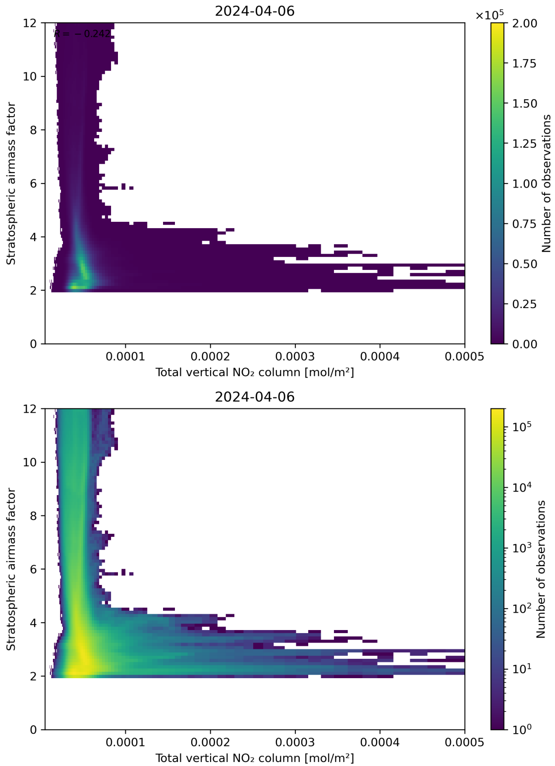
Figure 110: Scatter density plot of “Total vertical NO 2 column” against “Stratospheric airmass factor” for 2024-04-05 to 2024-04-07.
