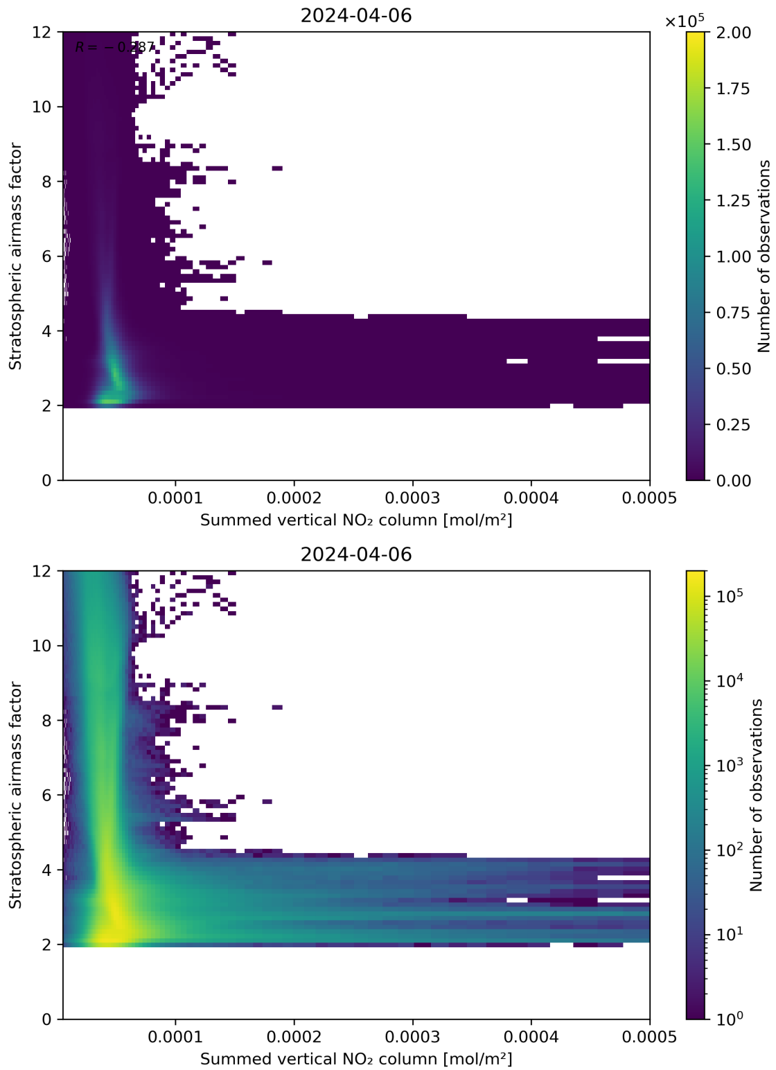
Figure 103: Scatter density plot of “Summed vertical NO 2 column” against “Stratospheric air mass factor” for 2024-04-05 to 2024-04-07.
