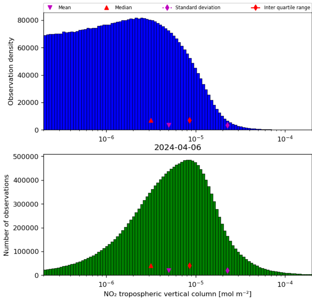
Figure 29: Histogram of “ \text{NO}_2 tropospheric vertical column” for 2024-04-05 to 2024-04-07
