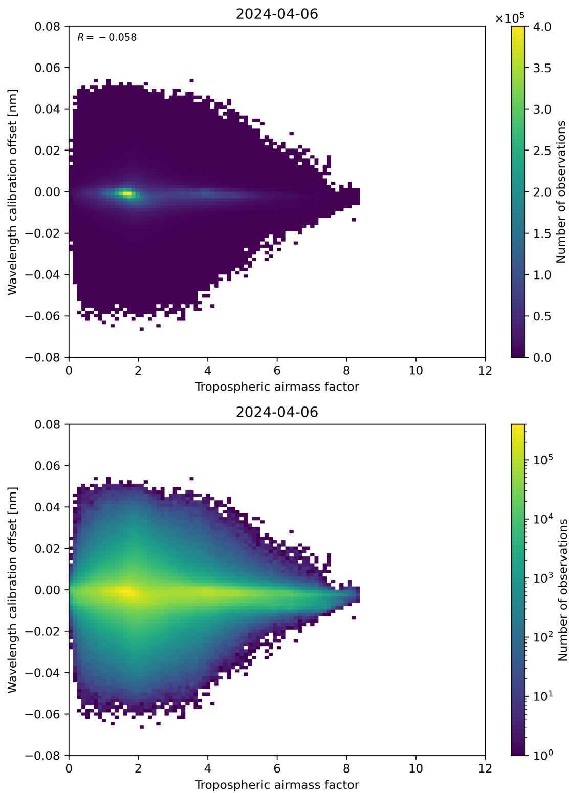
Figure 80: Scatter density plot of “Tropospheric air mass factor” against “Wavelength calibration offset” for 2024-04-05 to 2024-04-07.
