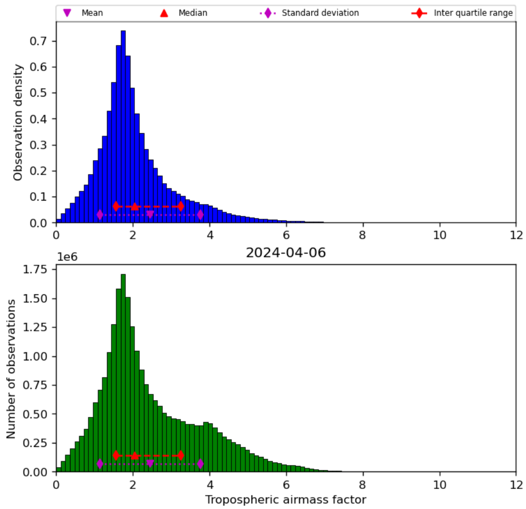
Figure 31: Histogram of “Tropospheric airmass factor” for 2024-04-05 to 2024-04-07
