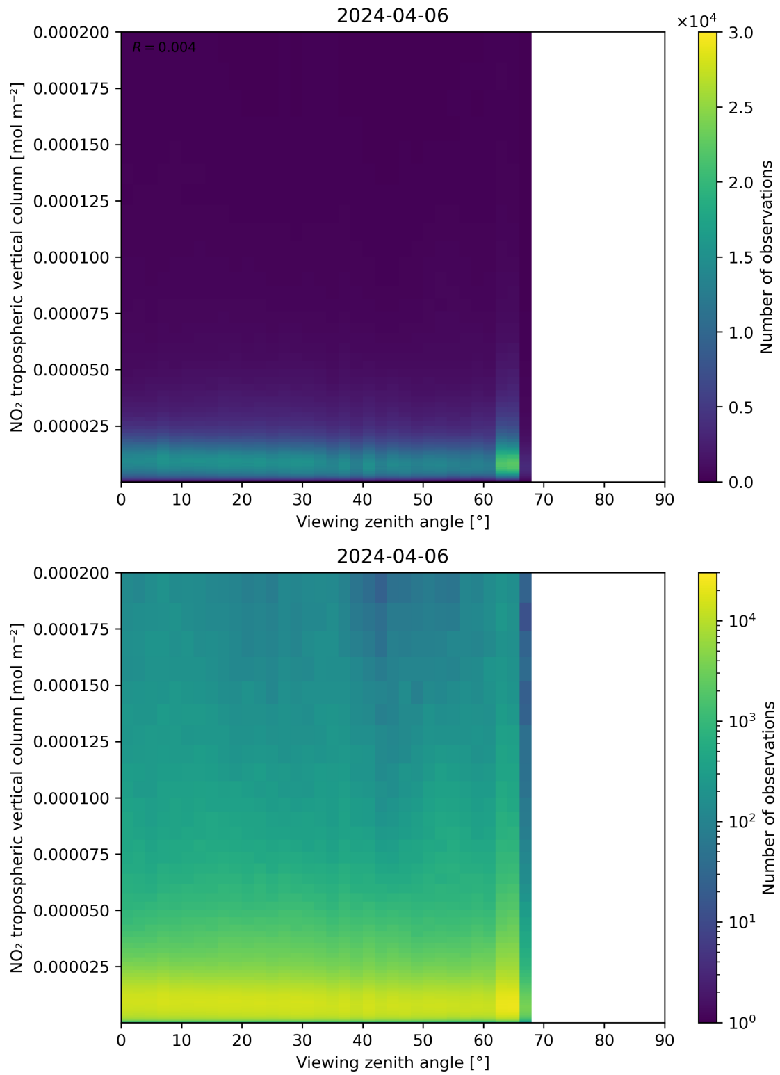
Figure 169: Scatter density plot of “Viewing zenith angle” against “NO 2 tropospheric vertical column” for 2024-04-05 to 2024-04-07.
