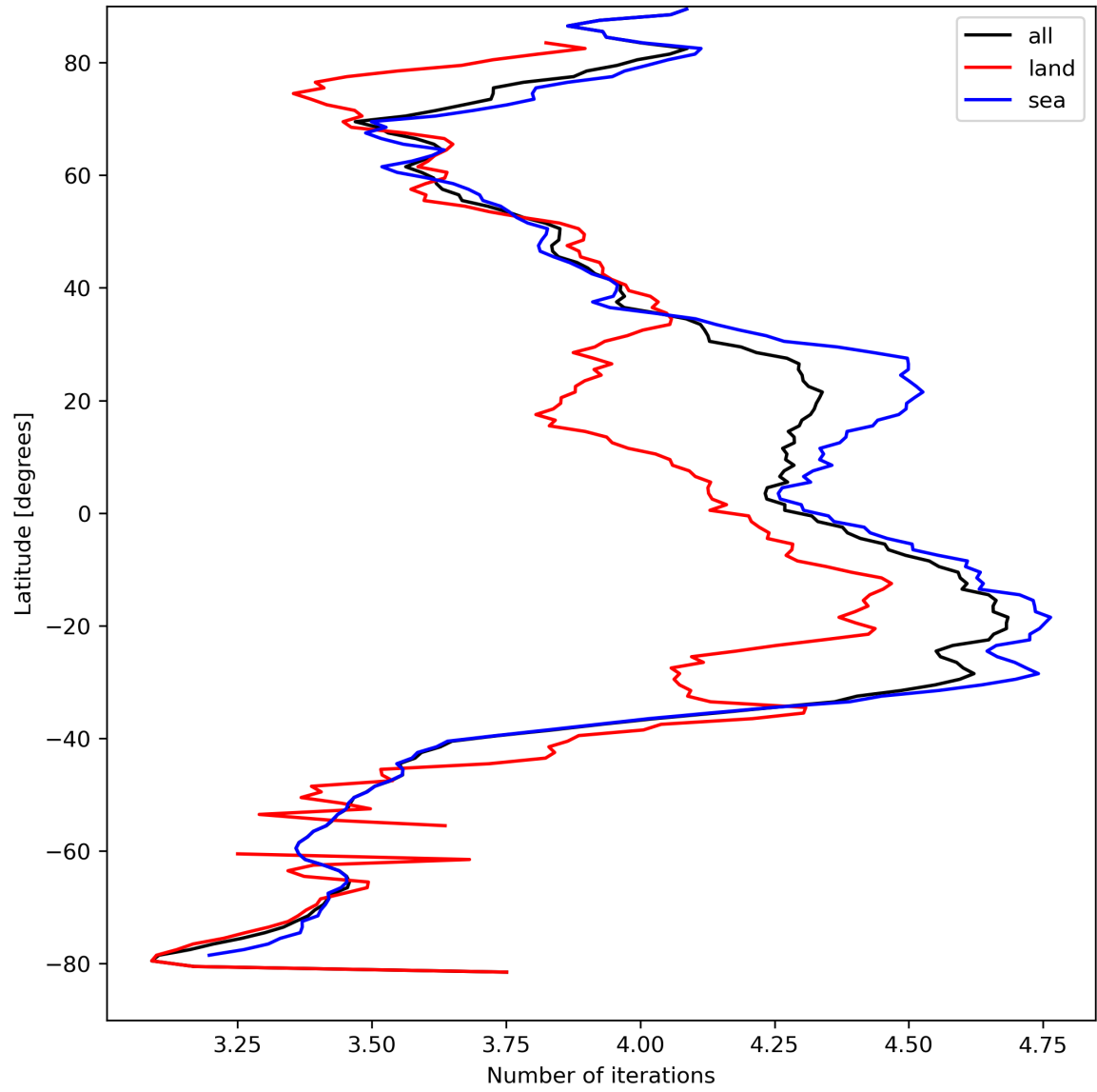
Figure 17: Zonal average of “Number of iterations” for 2024-04-05 to 2024-04-07.
