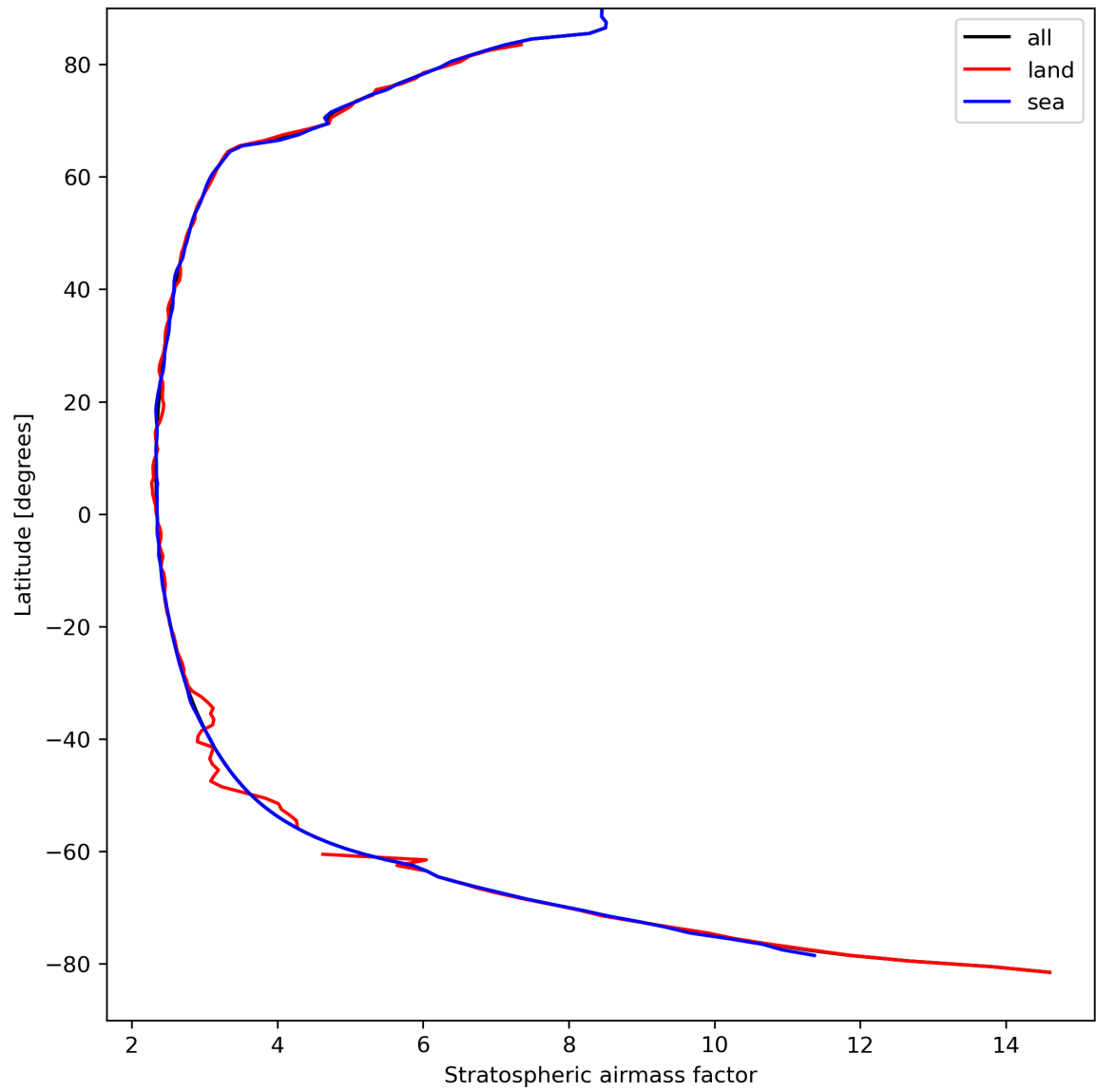
Figure 27: Zonal average of “Stratospheric air mass factor” for 2024-04-05 to 2024-04-07.
