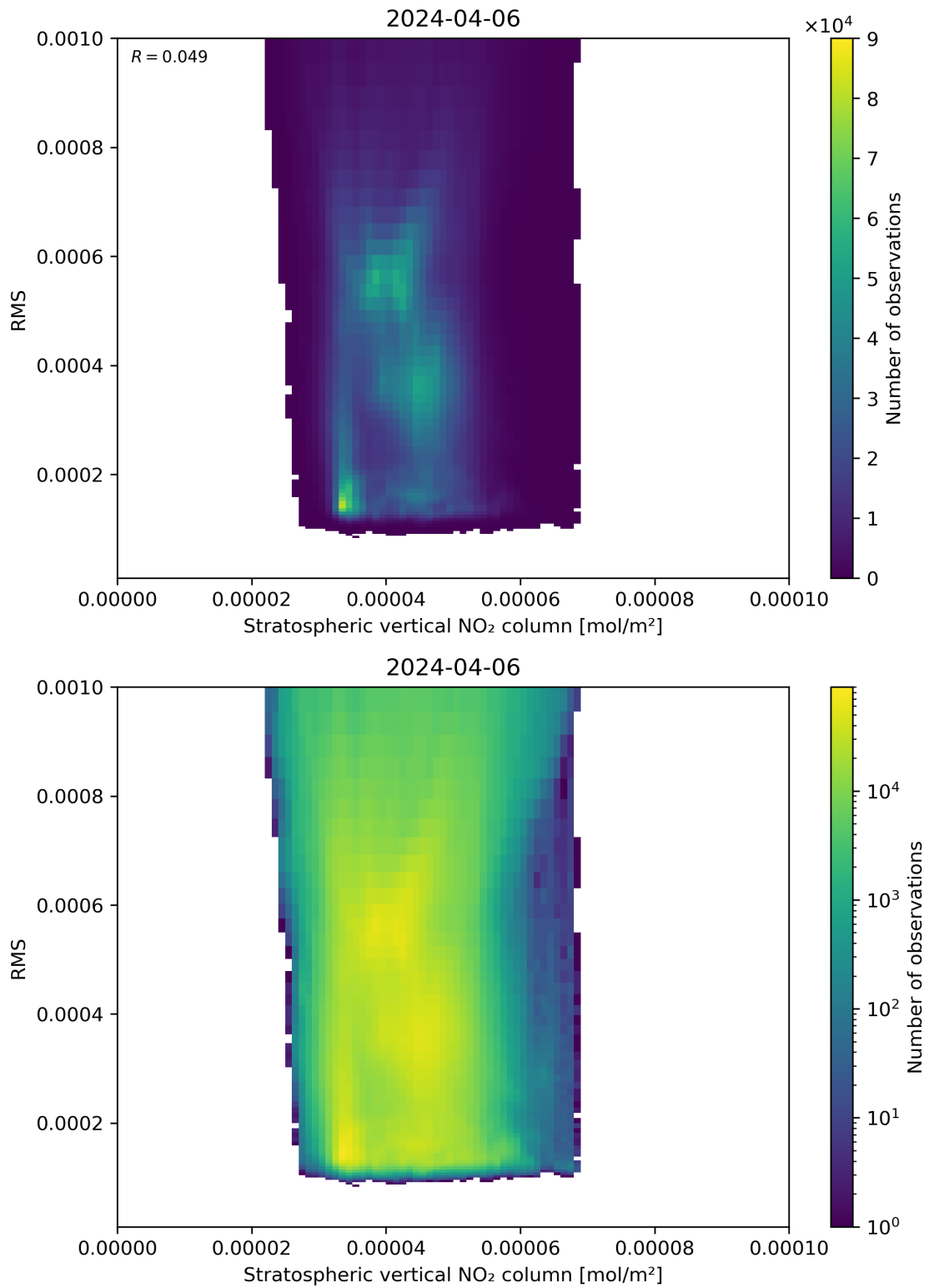
Figure 102: Scatter density plot of “Stratospheric vertical NO 2 column” against “RMS” for 2024-04-05 to 2024-04-07.
