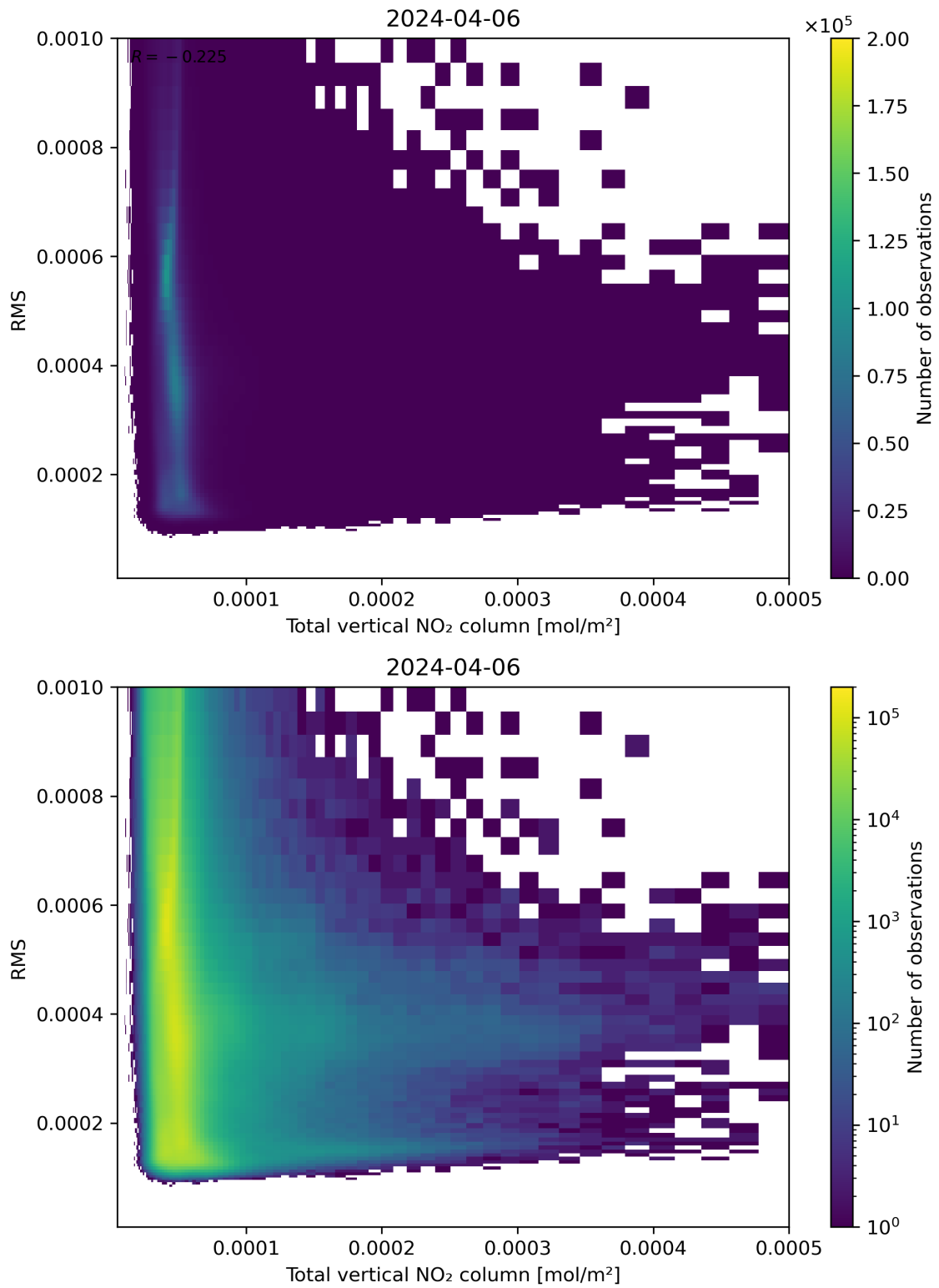
Figure 120: Scatter density plot of “Total vertical NO 2 column” against “RMS” for 2024-04-05 to 2024-04-07.
