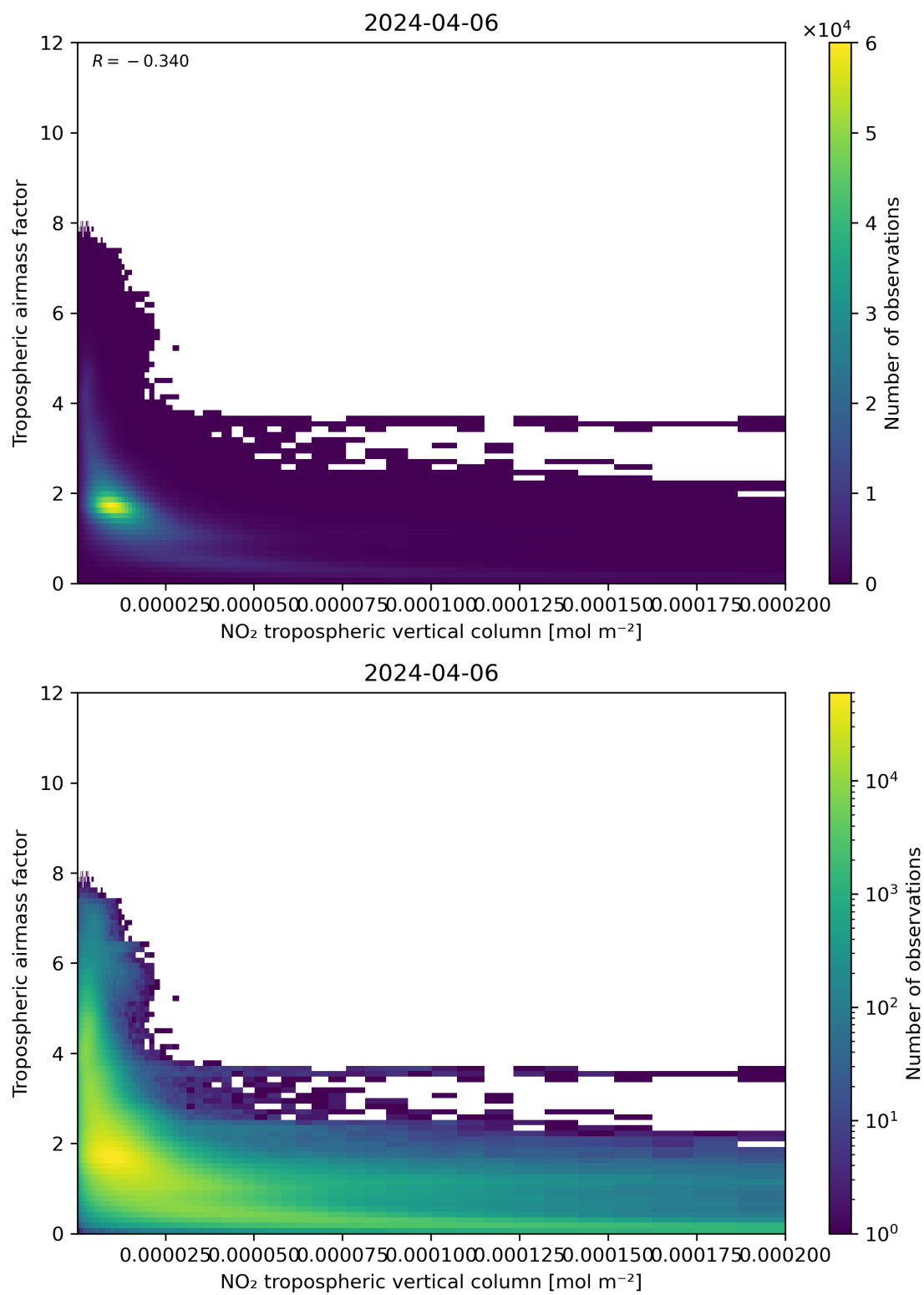
Figure 123: Scatter density plot of “NO 2 tropospheric vertical column” against “Tropospheric air mass factor” for 2024-04-05 to 2024-04-07.
