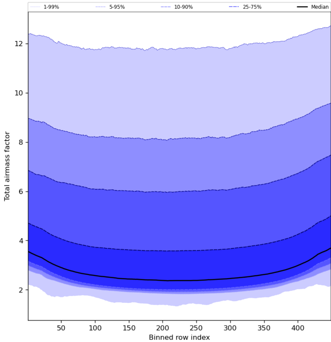
Figure 49: Along track statistics of “Total airmass factor” for 2024-04-05 to 2024-04-07
