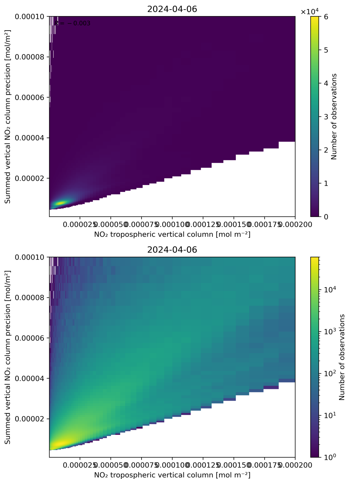
Figure 127: Scatter density plot of “NO 2 tropospheric vertical column” against “Summed vertical NO 2 column precision” for 2024-04-05 to 2024-04-07.
