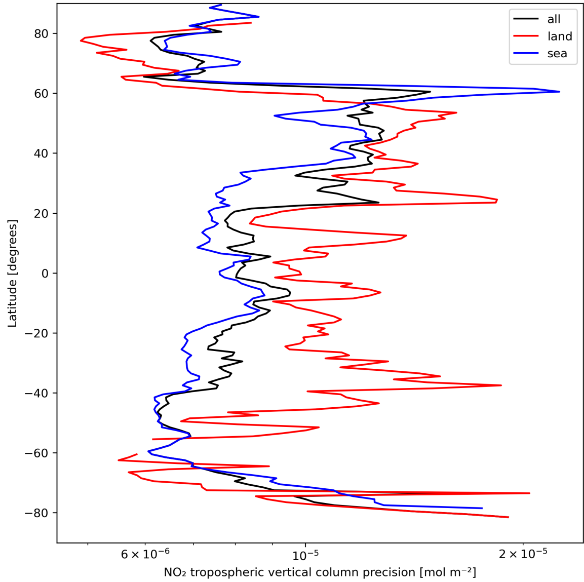
Figure 13: Zonal average of “NO 2 tropospheric vertical column precision” for 2024-04-05 to 2024-04-07.
