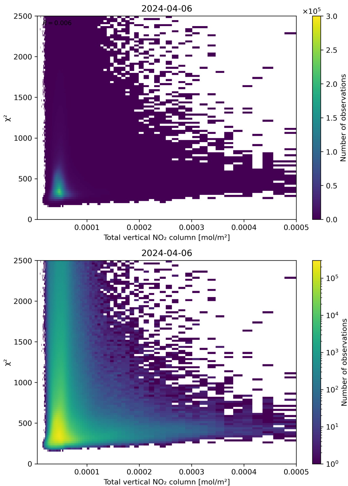
Figure 111: Scatter density plot of “Total vertical NO 2 column” against “ \chi^2 ” for 2024-04-05 to 2024-04-07.
