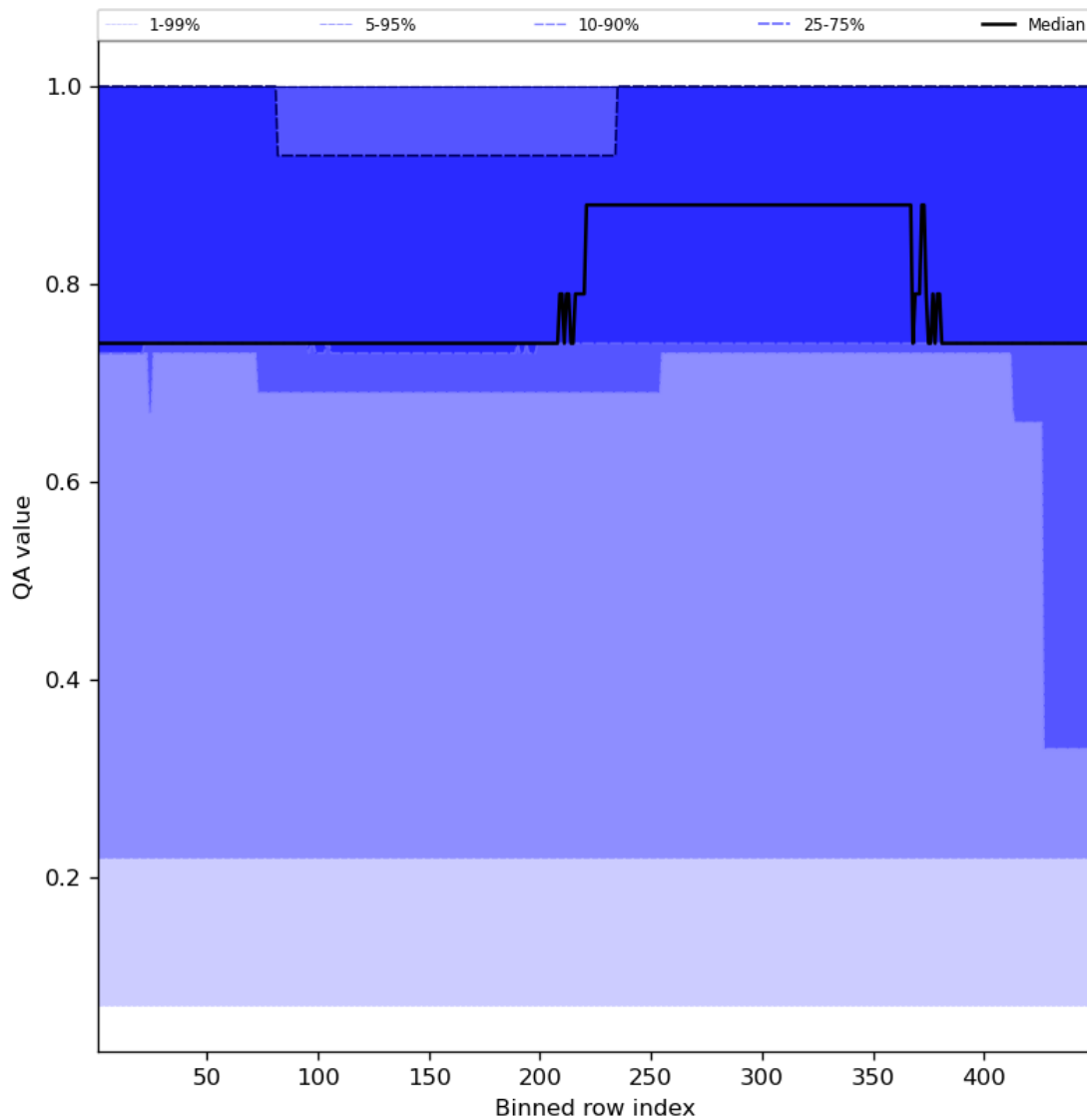
Figure 45: Along track statistics of “QA value” for 2024-04-05 to 2024-04-07
