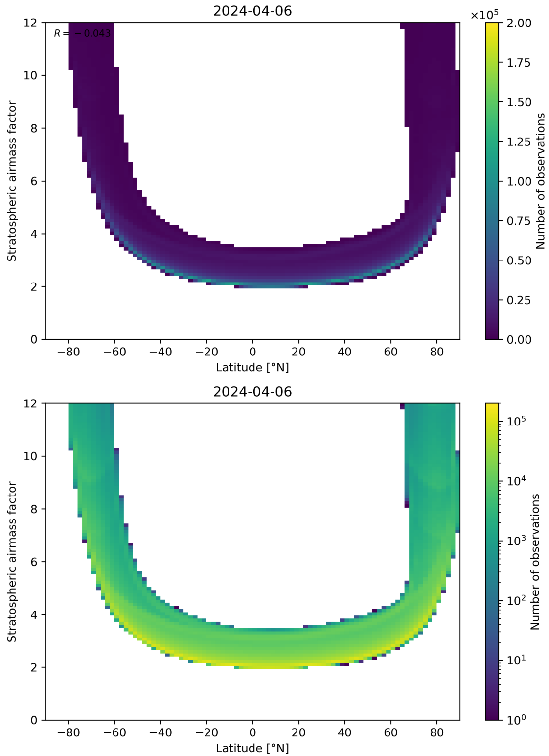
Figure 83: Scatter density plot of “Latitude” against “Stratospheric air mass factor” for 2024-04-05 to 2024-04-07.
