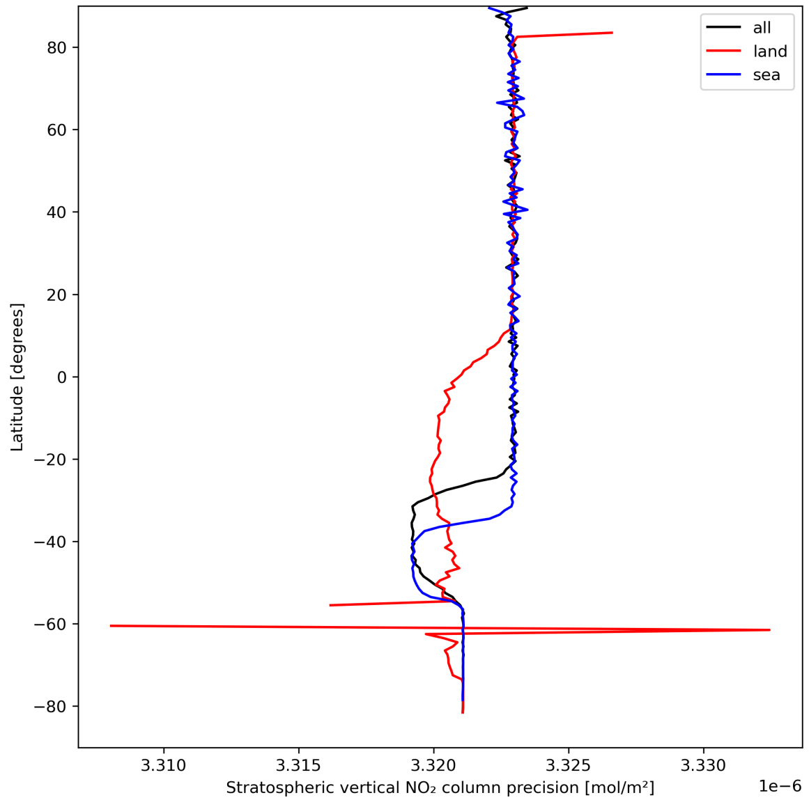
Figure 20: Zonal average of “Stratospheric vertical NO 2 column precision” for 2024-04-05 to 2024-04-07.
