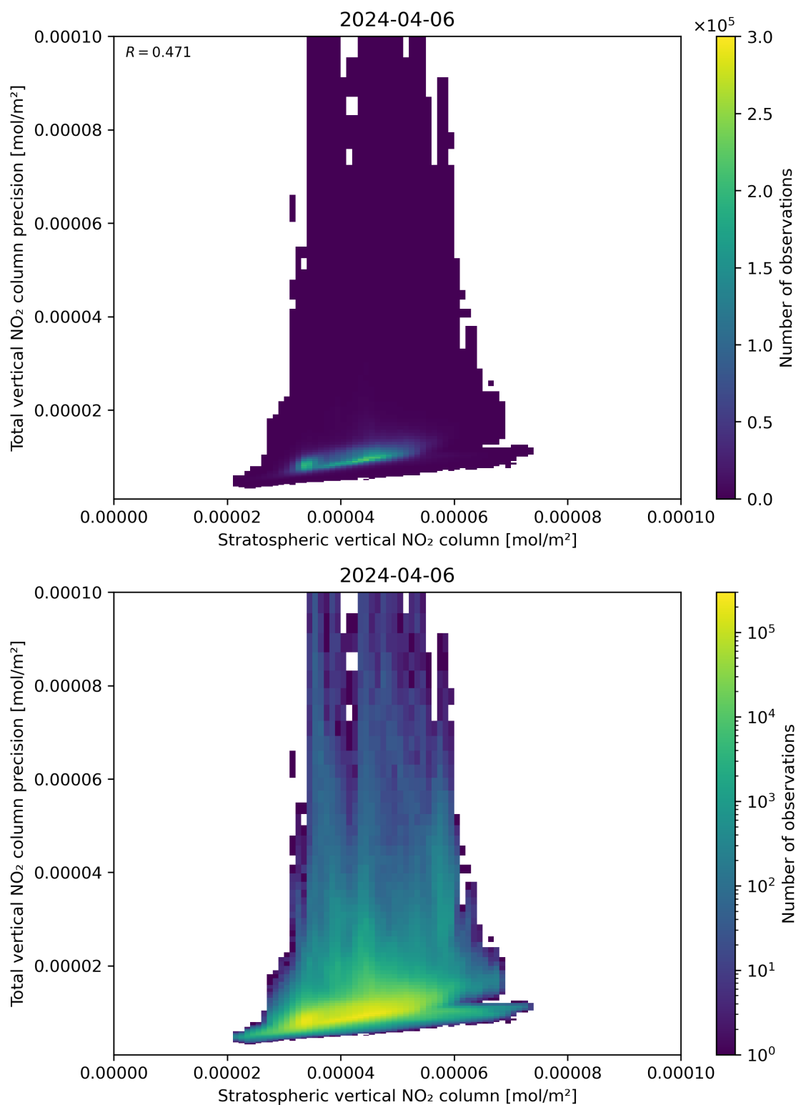
Figure 101: Scatter density plot of “Stratospheric vertical NO 2 column” against “Total vertical NO 2 column precision” for 2024-04-05 to 2024-04-07.
