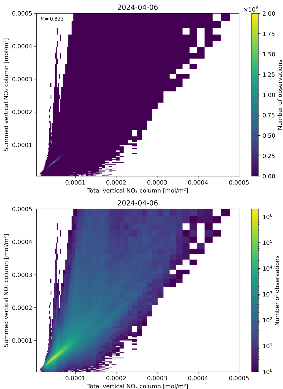
Figure 112: Scatter density plot of “Total vertical NO 2 column” against “Summed vertical NO 2 column” for 2024-04-05 to 2024-04-07.
