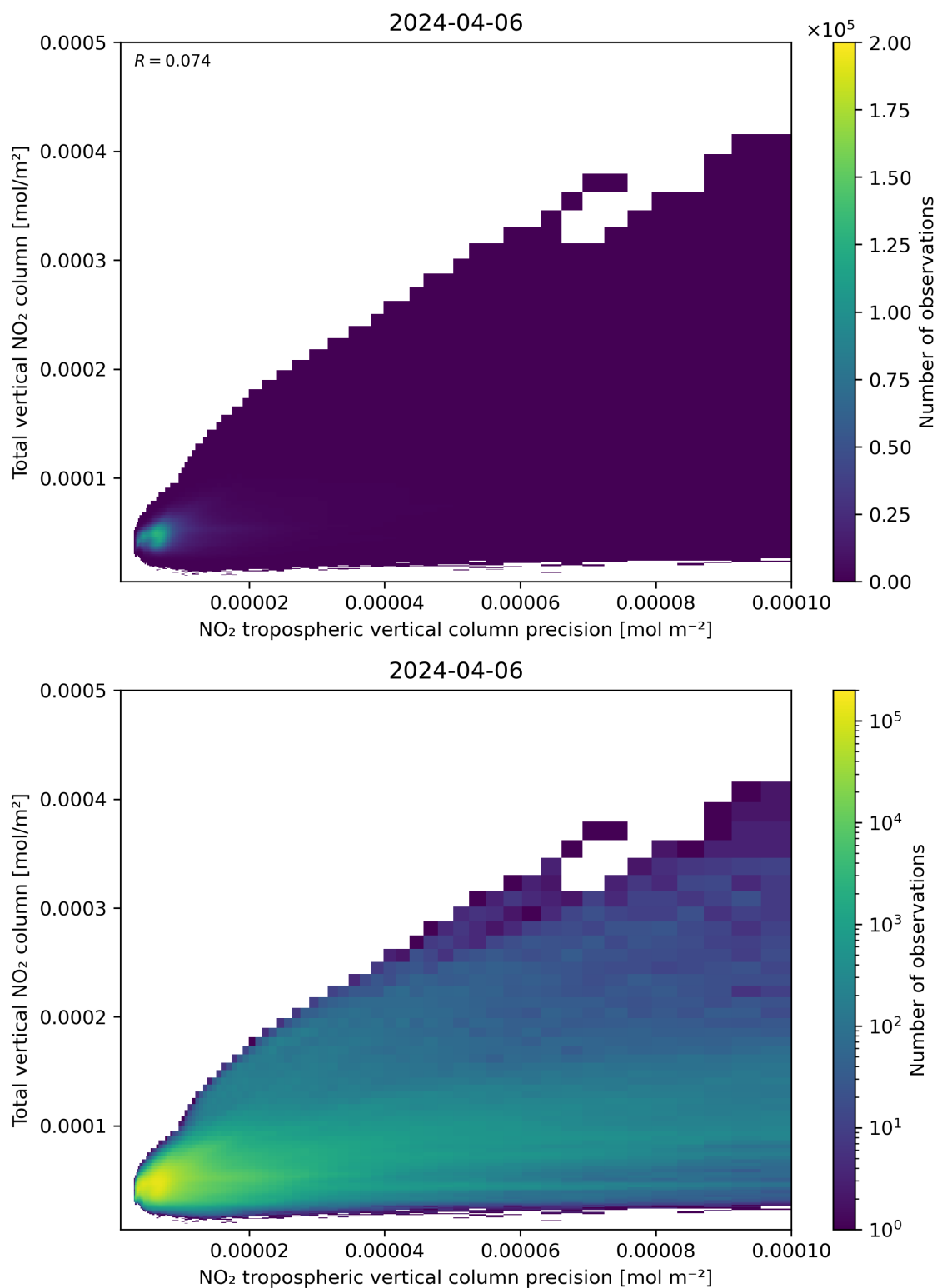
Figure 138: Scatter density plot of “NO 2 tropospheric vertical column precision” against “Total vertical NO 2 column” for 2024-04-05 to 2024-04-07.
