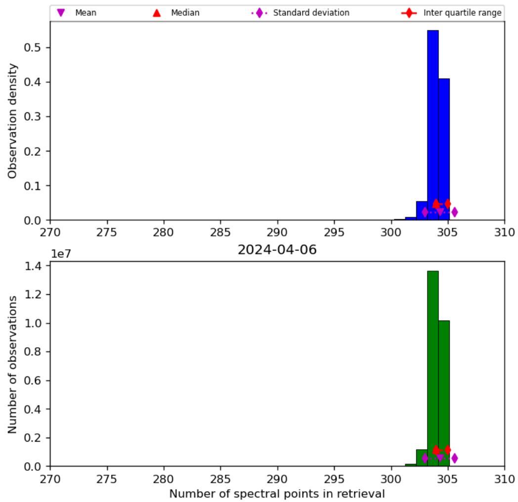
Figure 33: Histogram of “Number of spectral points in retrieval” for 2024-04-05 to 2024-04-07
