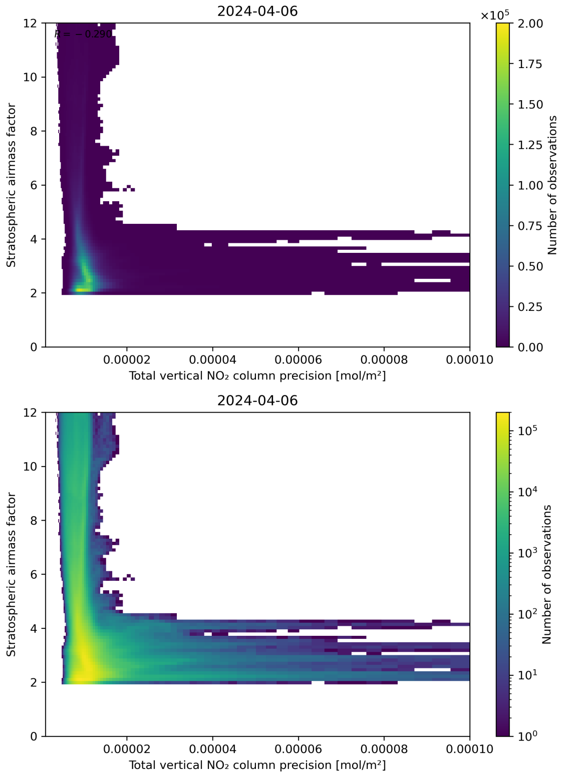
Figure 115: Scatter density plot of “Total vertical NO 2 column precision” against “Stratospheric air mass factor” for 2024-04-05 to 2024-04-07.
