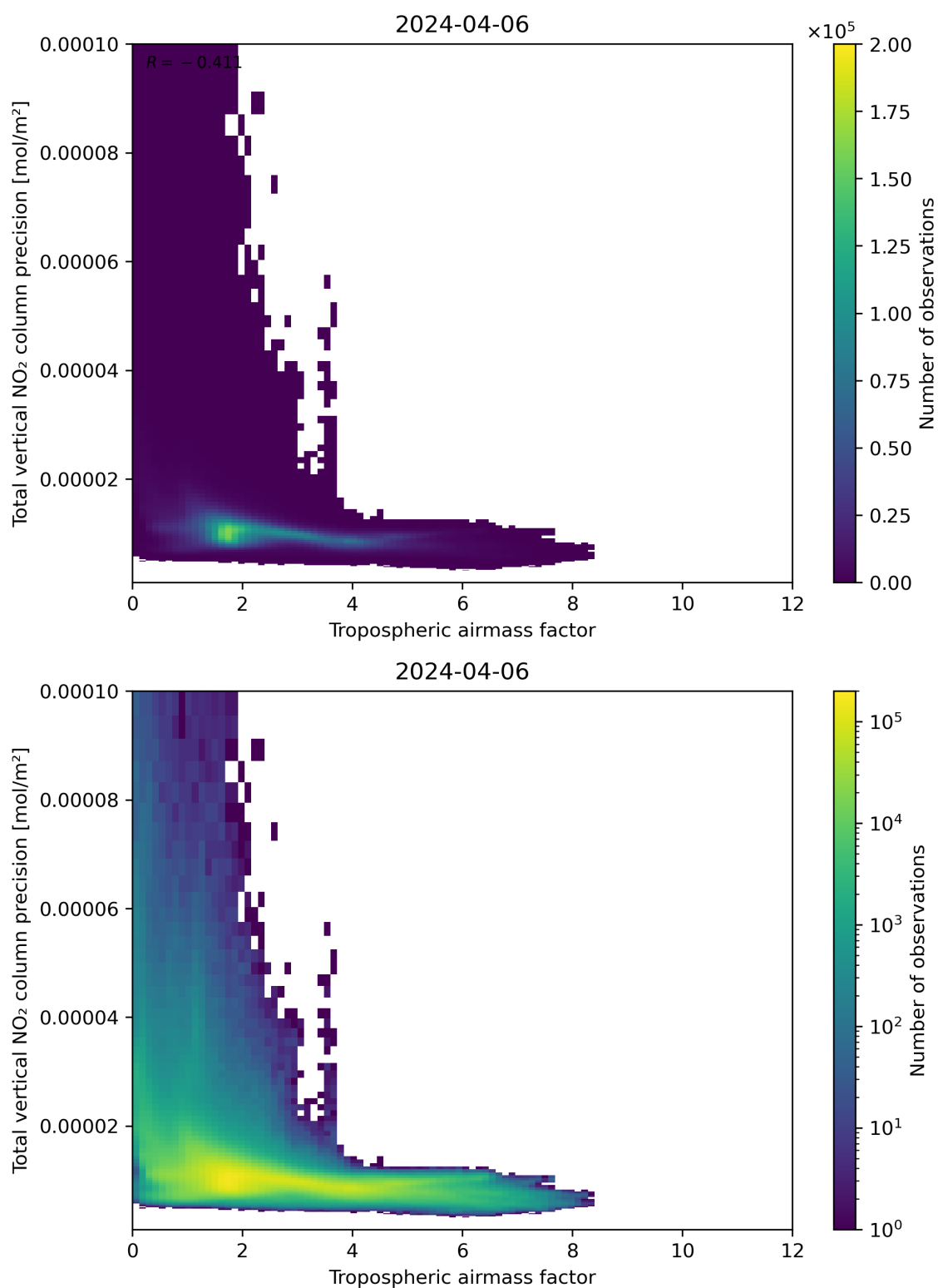
Figure 78: Scatter density plot of “Tropospheric air mass factor” against “Total vertical NO 2 column precision” for 2024-04-05 to 2024-04-07.
