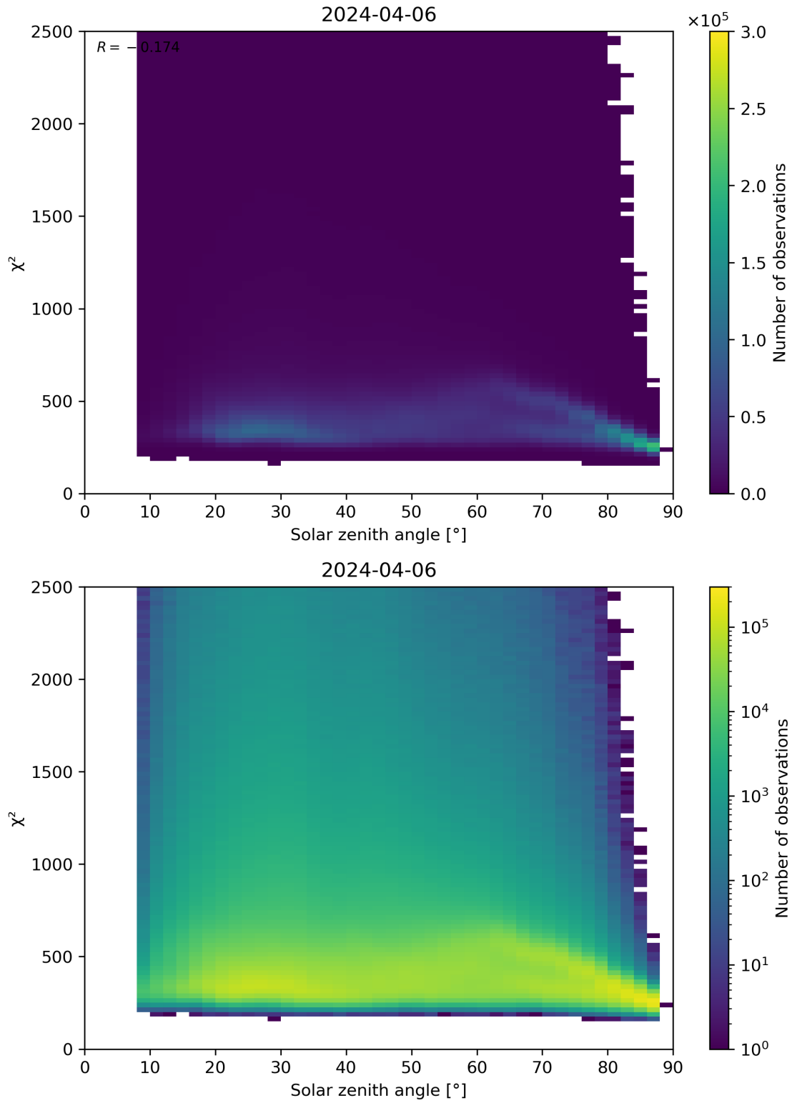
Figure 148: Scatter density plot of “Solar zenith angle” against “ \chi^2 ” for 2024-04-05 to 2024-04-07.
