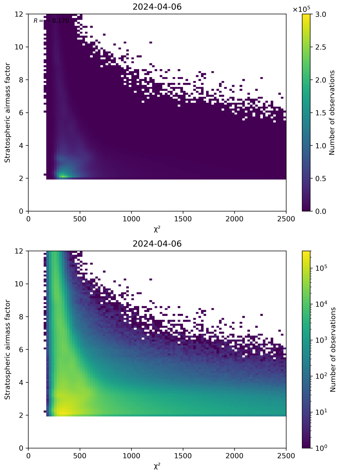
Figure 81: Scatter density plot of “ \chi^2 ” against “Stratospheric airmass factor” for 2024-04-05 to 2024-04-07.
