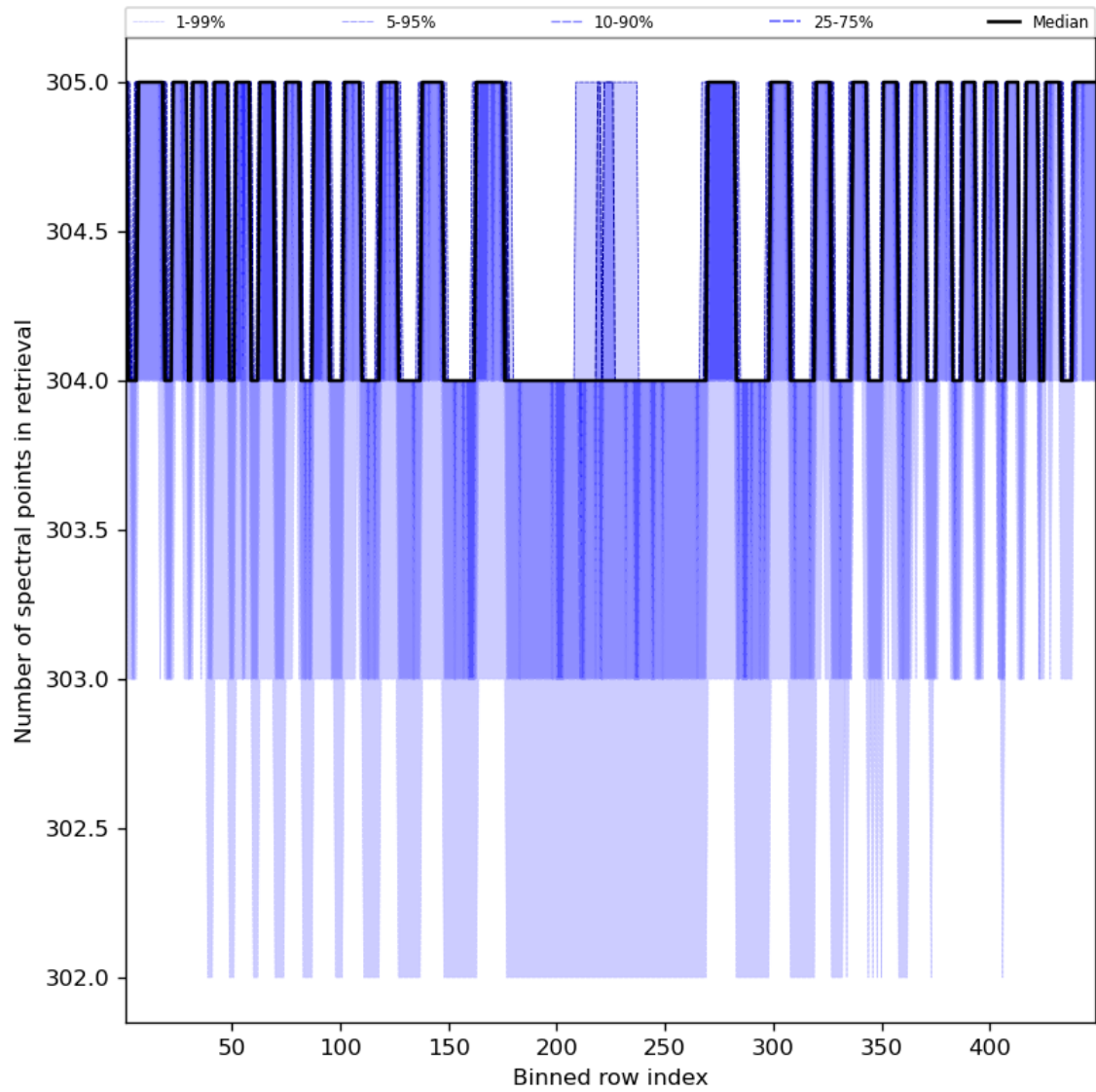
Figure 50: Along track statistics of “Number of spectral points in retrieval” for 2024-04-05 to 2024-04-07
