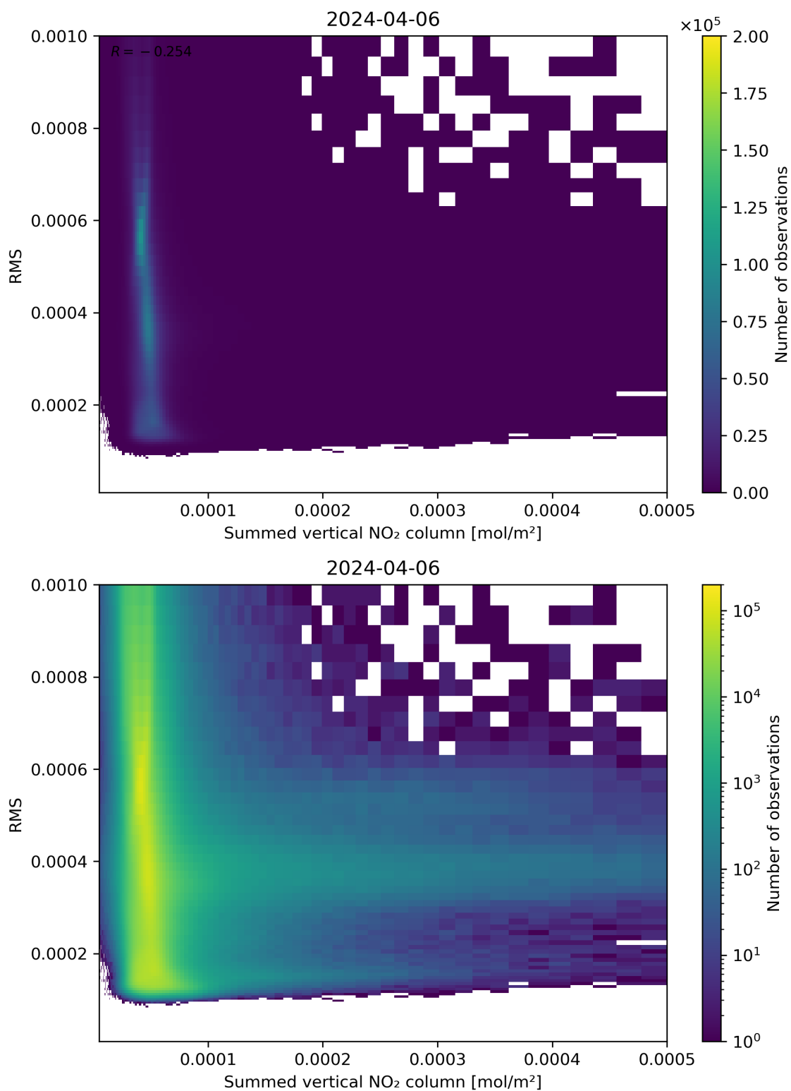
Figure 109: Scatter density plot of “Summed vertical NO 2 column” against “RMS” for 2024-04-05 to 2024-04-07.
