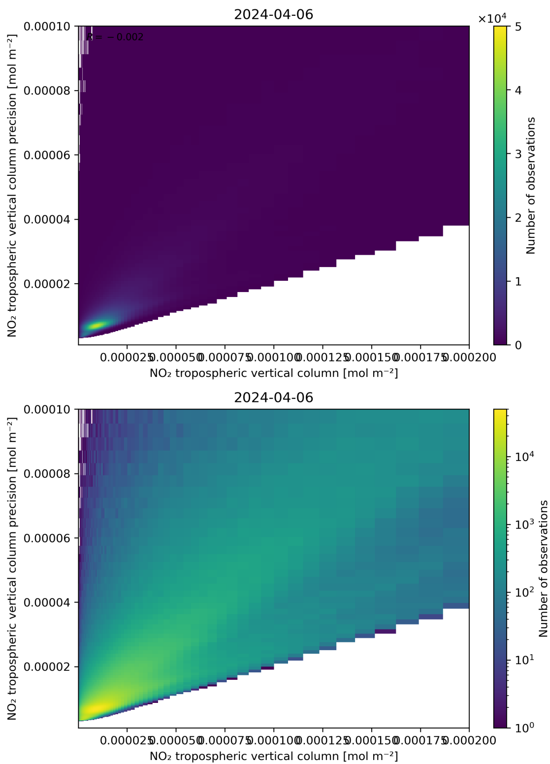
Figure 130: Scatter density plot of “NO 2 tropospheric vertical column” against “NO 2 tropospheric vertical column precision” for 2024-04-05 to 2024-04-07.
