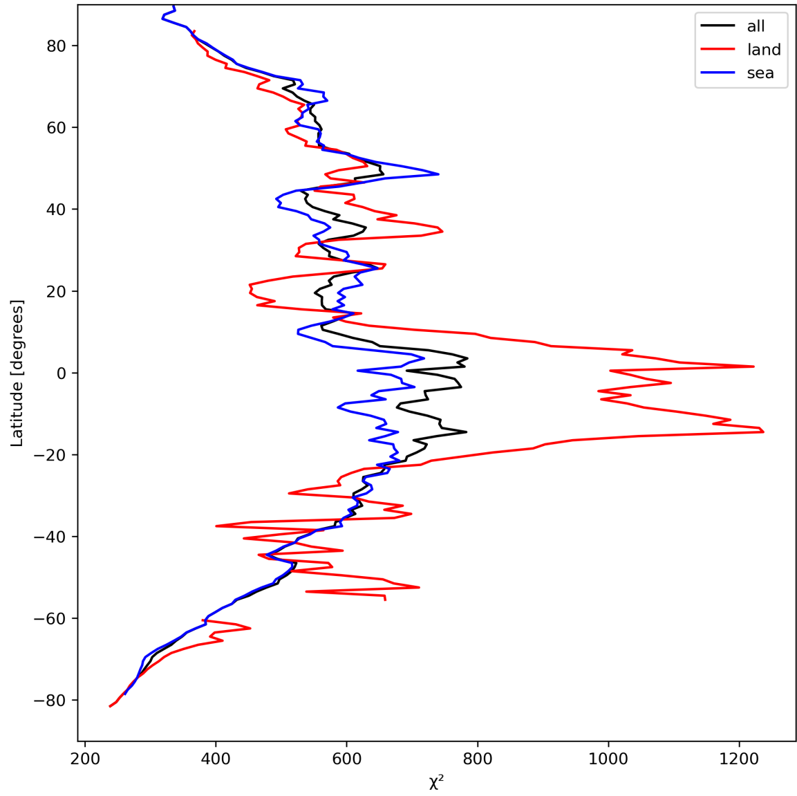
Figure 25: Zonal average of “ \chi^2 ” for 2024-04-05 to 2024-04-07.
