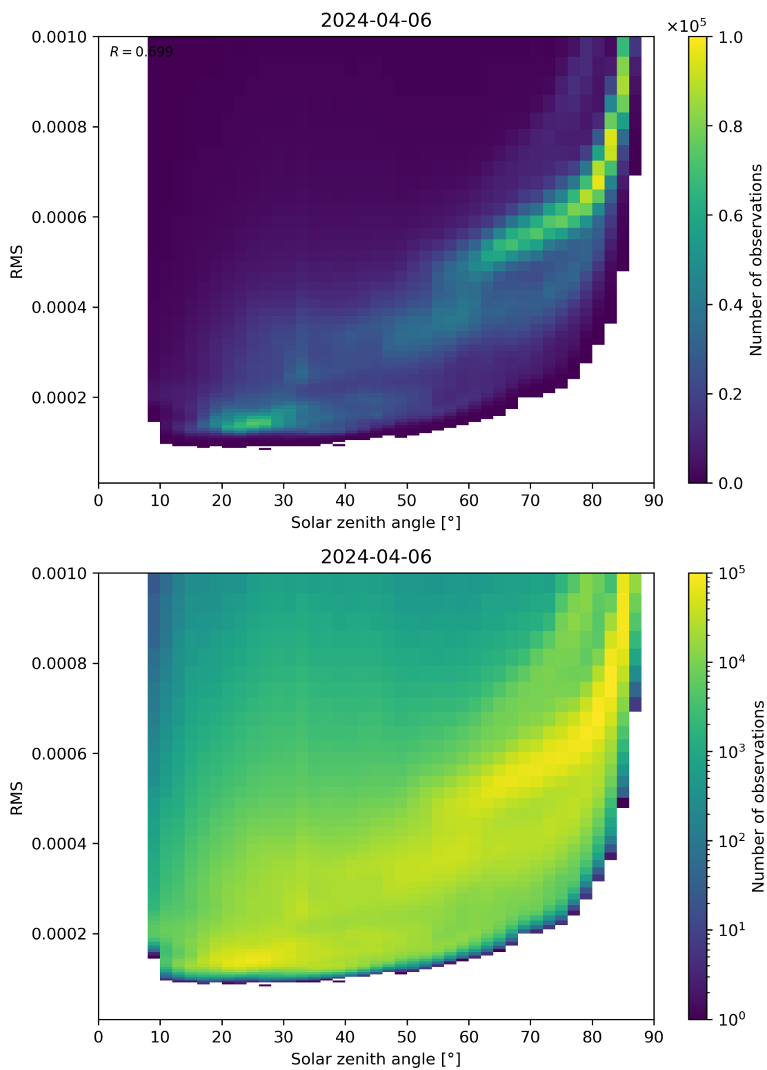
Figure 157: Scatter density plot of “Solar zenith angle” against “RMS” for 2024-04-05 to 2024-04-07.
