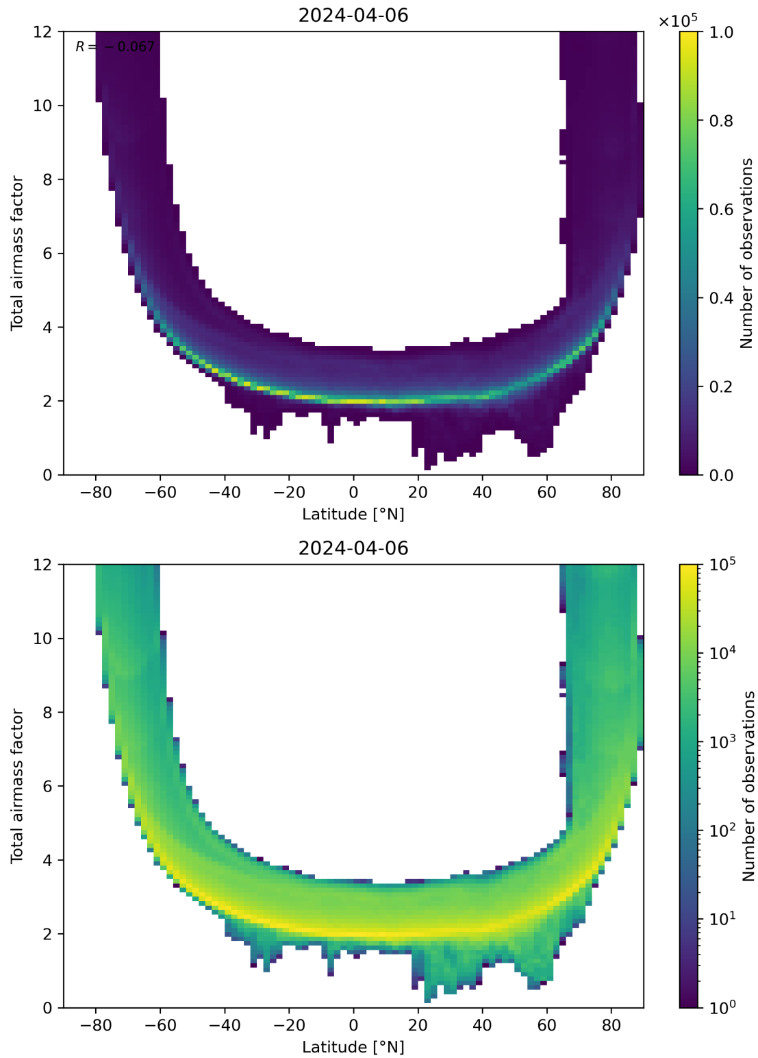
Figure 84: Scatter density plot of “Latitude” against “Total airmass factor” for 2024-04-05 to 2024-04-07.
