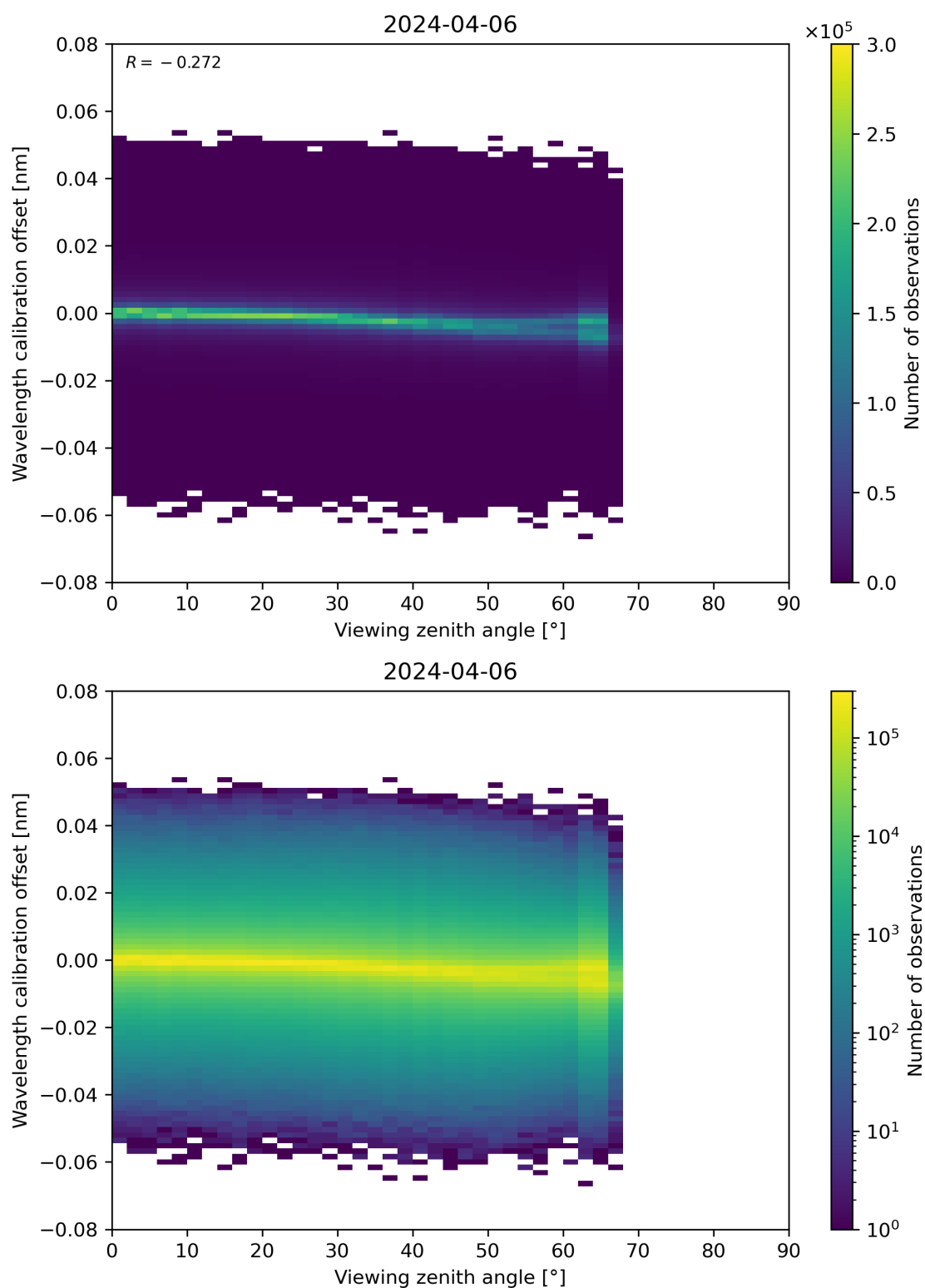
Figure 173: Scatter density plot of “Viewing zenith angle” against “Wavelength calibration offset” for 2024-04-05 to 2024-04-07.
