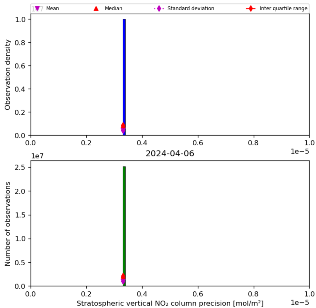
Figure 37: Histogram of “Stratospheric vertical NO 2 column precision” for 2024-04-05 to 2024-04-07
