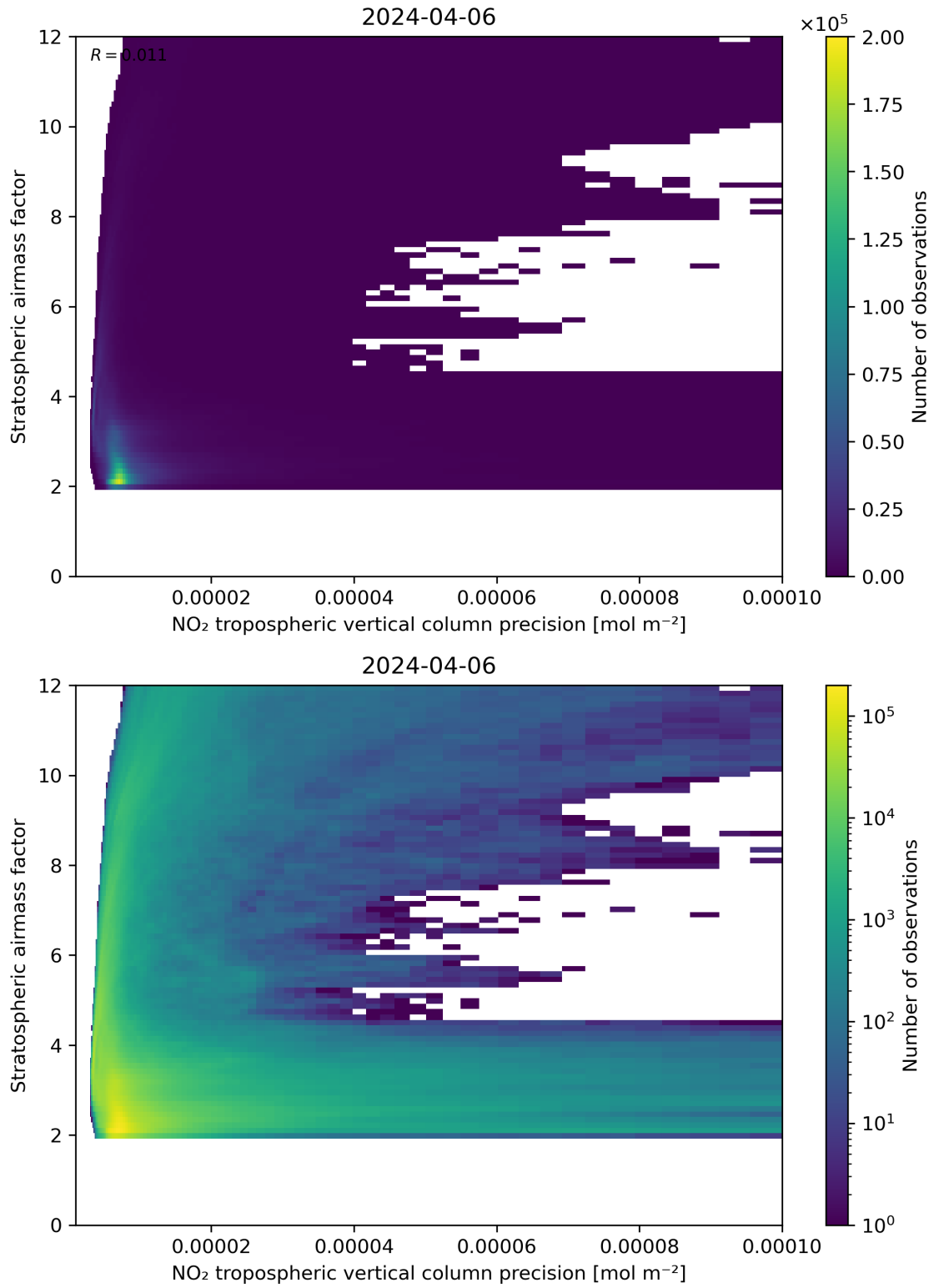
Figure 131: Scatter density plot of “NO 2 tropospheric vertical column precision” against “Stratospheric airmass factor” for 2024-04-05 to 2024-04-07.
