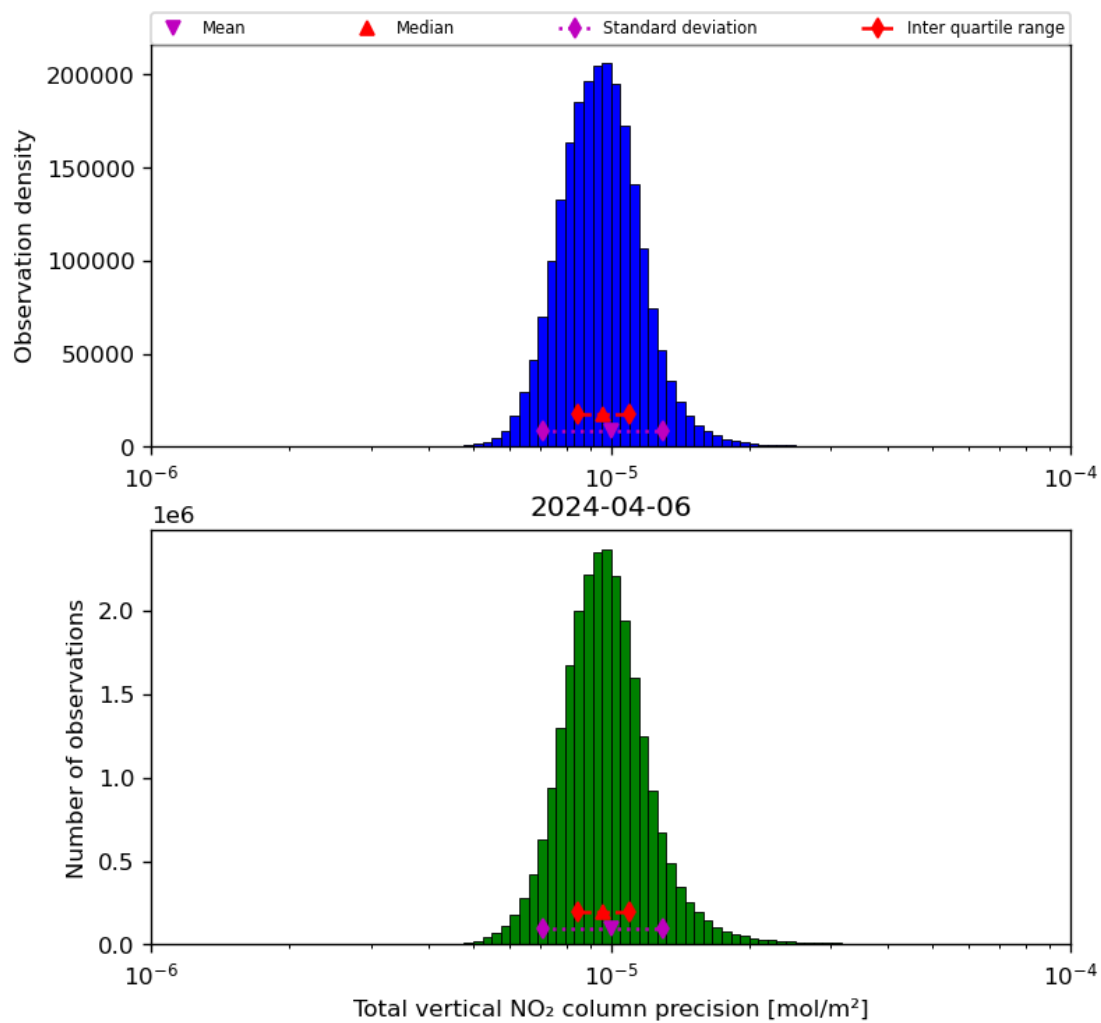
Figure 39: Histogram of “Total vertical NO 2 column precision” for 2024-04-05 to 2024-04-07
