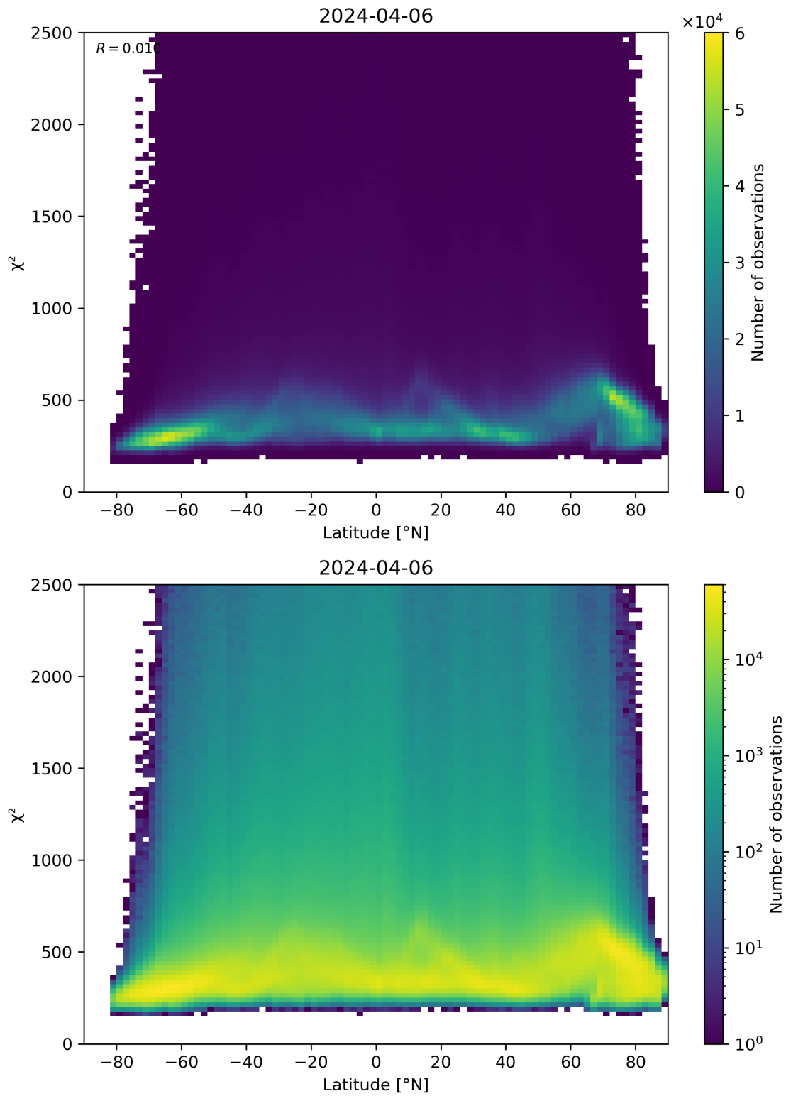
Figure 86: Scatter density plot of “Latitude” against “ \chi^2 ” for 2024-04-05 to 2024-04-07.
