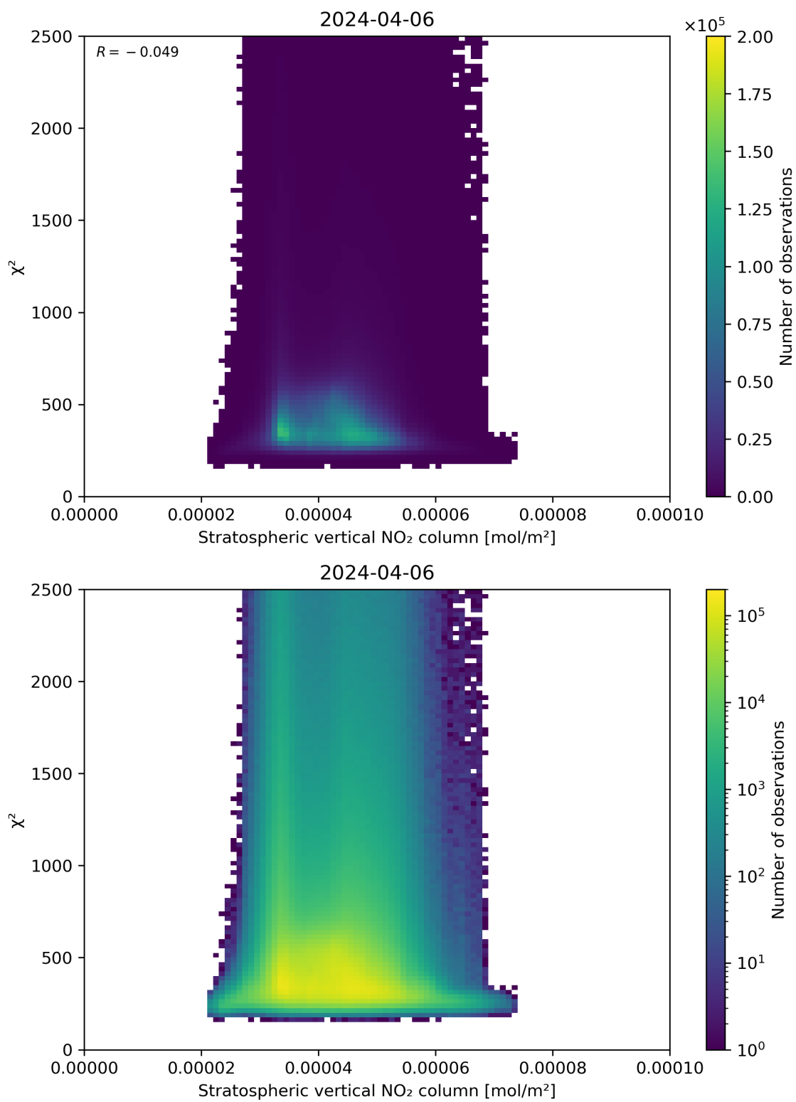
Figure 97: Scatter density plot of “Stratospheric vertical NO 2 column” against “ \chi^2 ” for 2024-04-05 to 2024-04-07.
