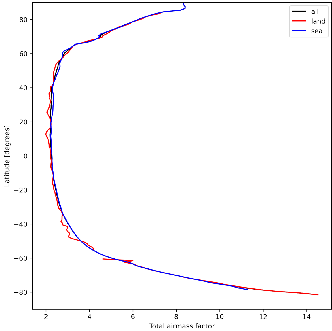
Figure 15: Zonal average of “Total airmass factor” for 2024-04-05 to 2024-04-07.
