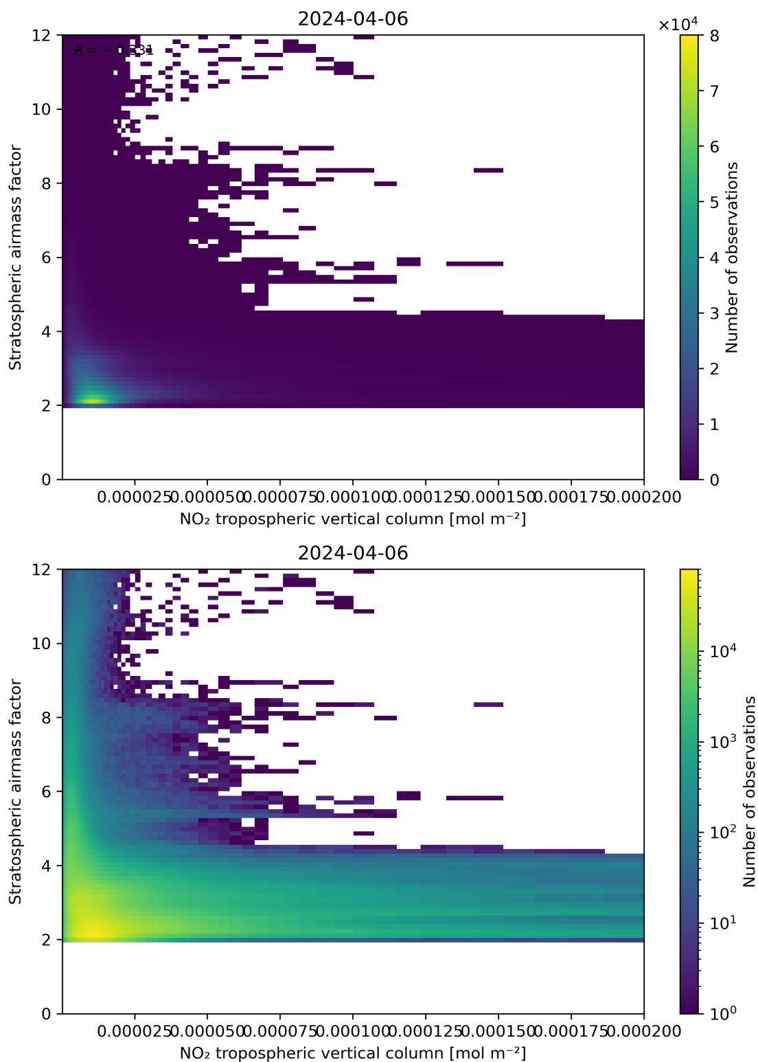
Figure 121: Scatter density plot of “NO 2 tropospheric vertical column” against “Stratospheric air mass factor” for 2024-04-05 to 2024-04-07.
