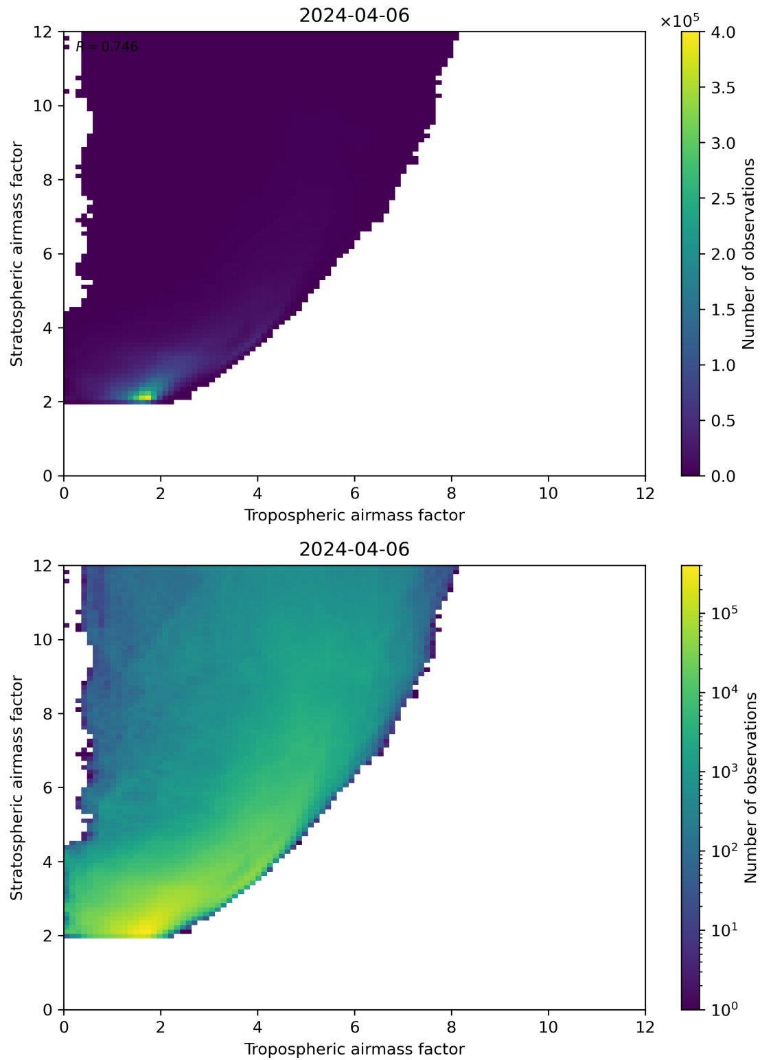
Figure 71: Scatter density plot of “Tropospheric airmass factor” against “Stratospheric airmass factor” for 2024-04-05 to 2024-04-07.
