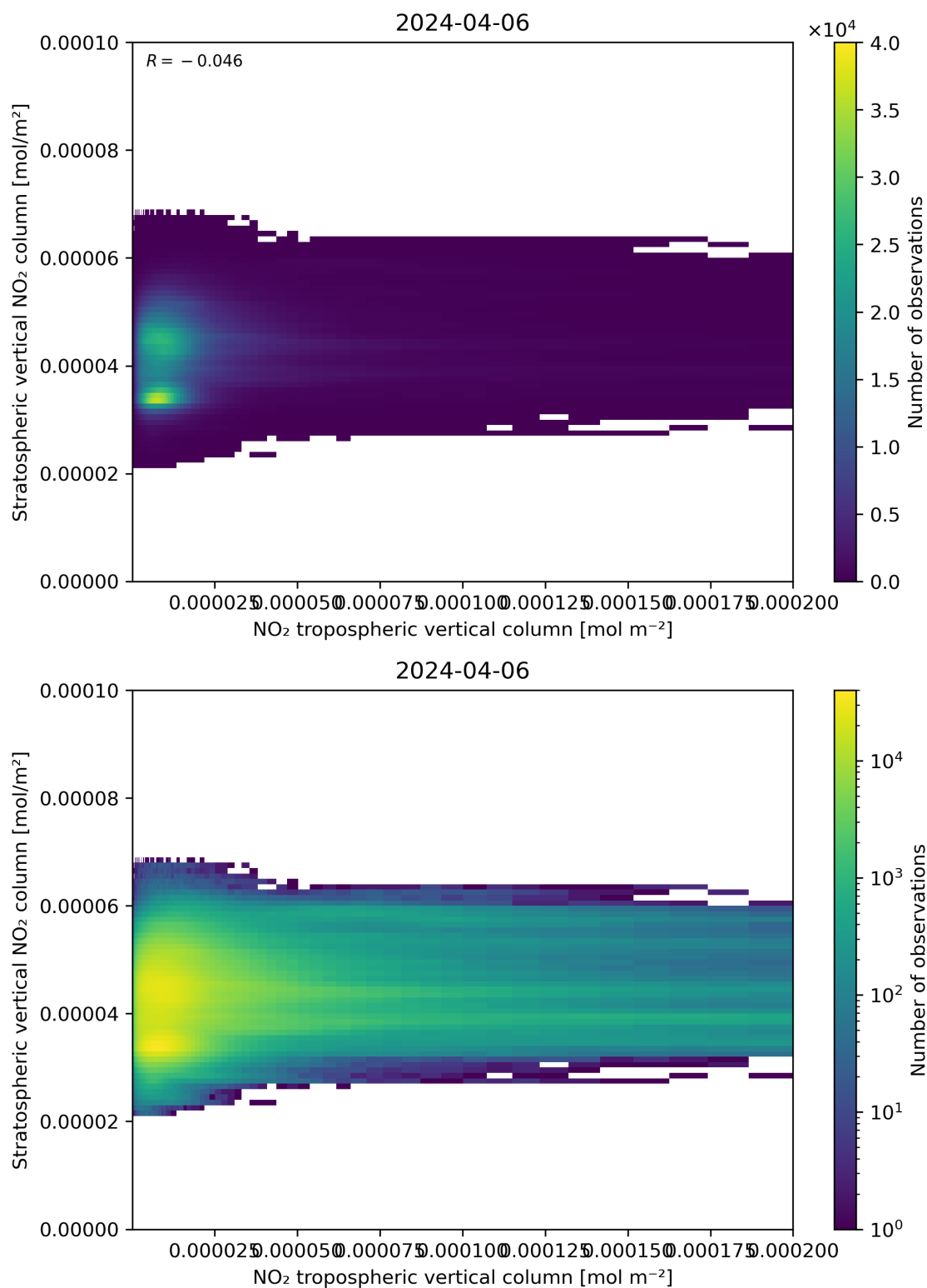
Figure 125: Scatter density plot of “NO 2 tropospheric vertical column” against “Stratospheric vertical NO 2 column” for 2024-04-05 to 2024-04-07.
