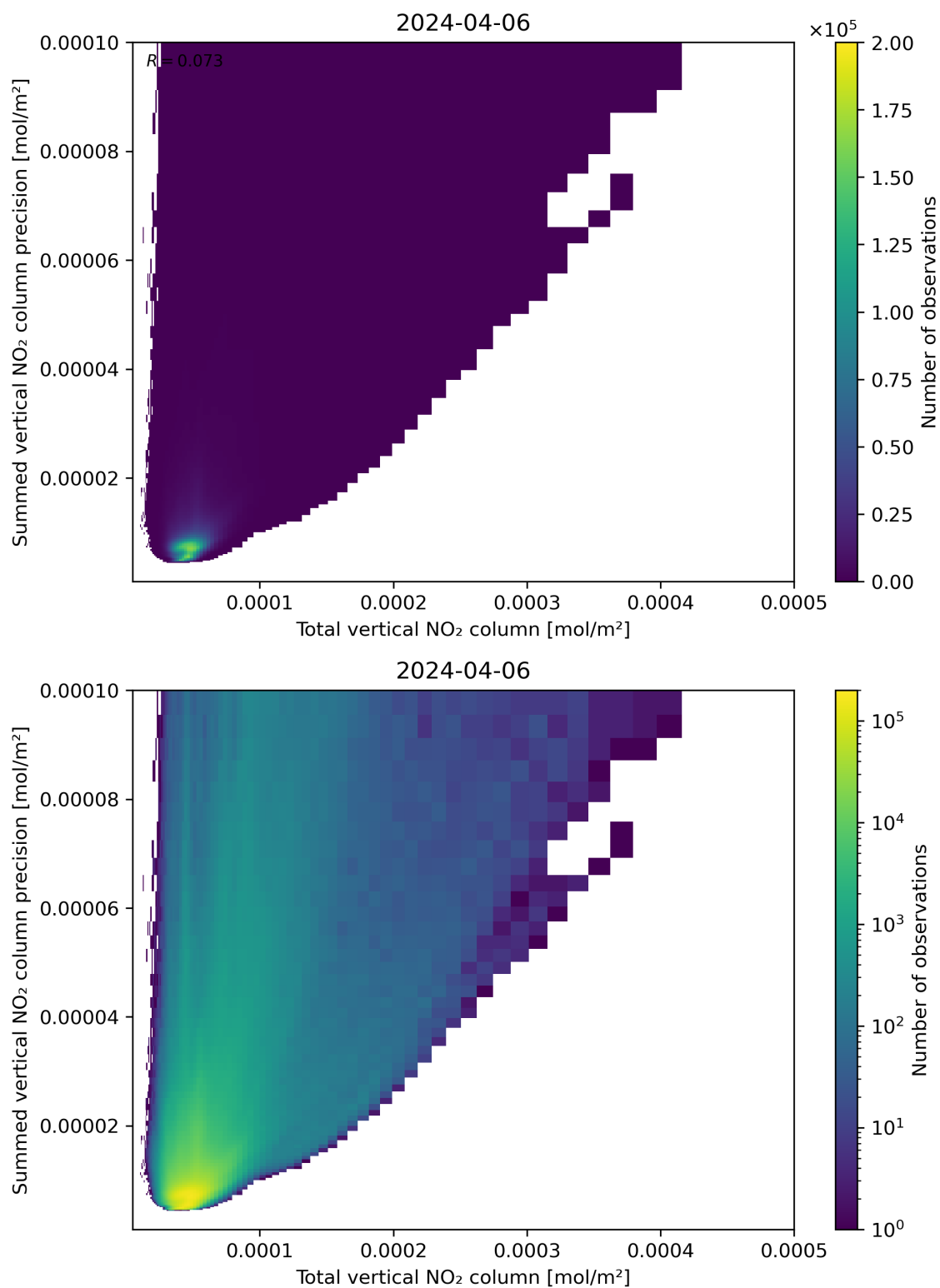
Figure 113: Scatter density plot of “Total vertical NO 2 column” against “Summed vertical NO 2 column precision” for 2024-04-05 to 2024-04-07.
