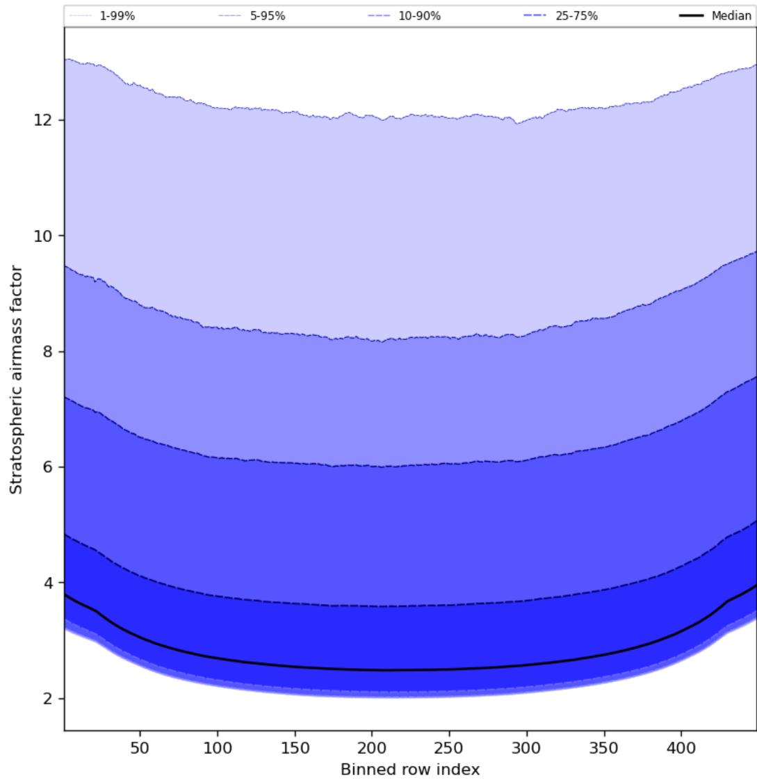
Figure 61: Along track statistics of “Stratospheric airmass factor” for 2024-04-05 to 2024-04-07
