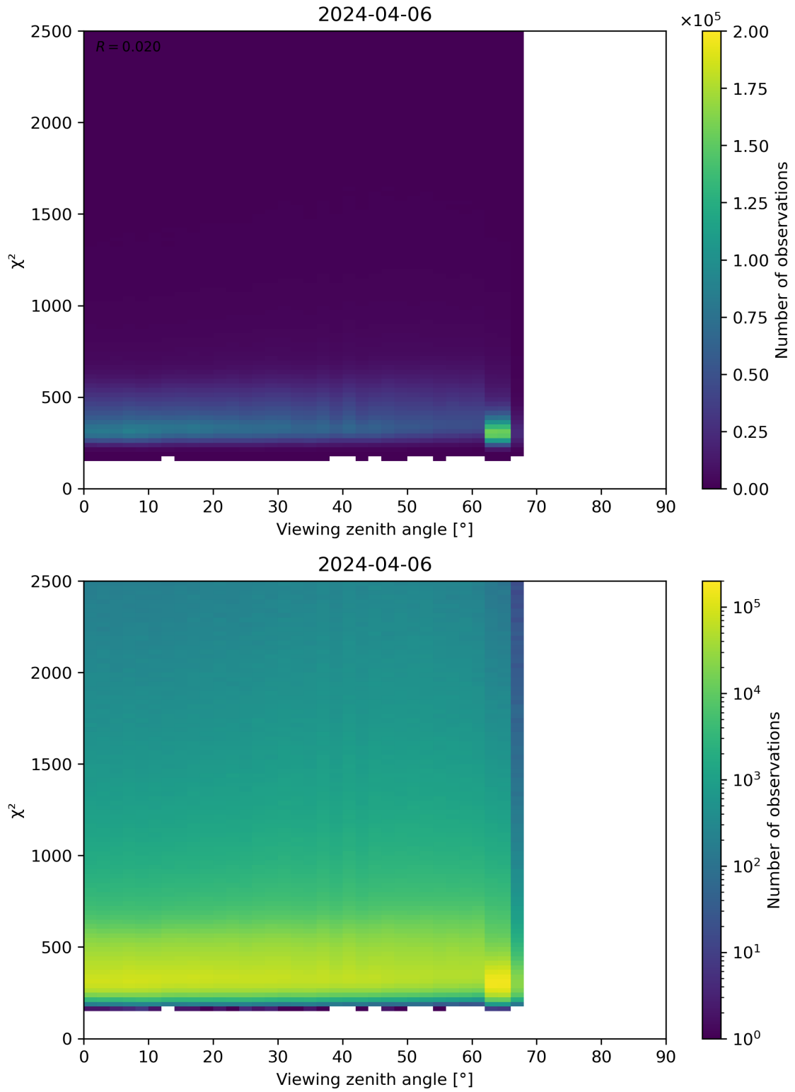
Figure 162: Scatter density plot of “Viewing zenith angle” against “ \chi^2 ” for 2024-04-05 to 2024-04-07.
