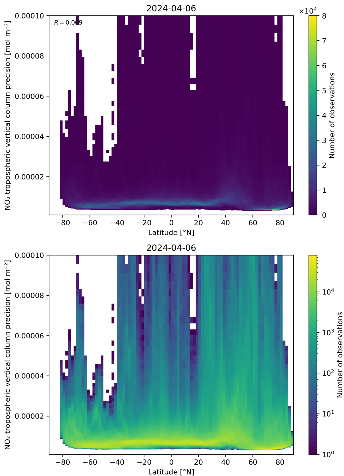
Figure 93: Scatter density plot of “Latitude” against “NO 2 tropospheric vertical column precision” for 2024-04-05 to 2024-04-07.
