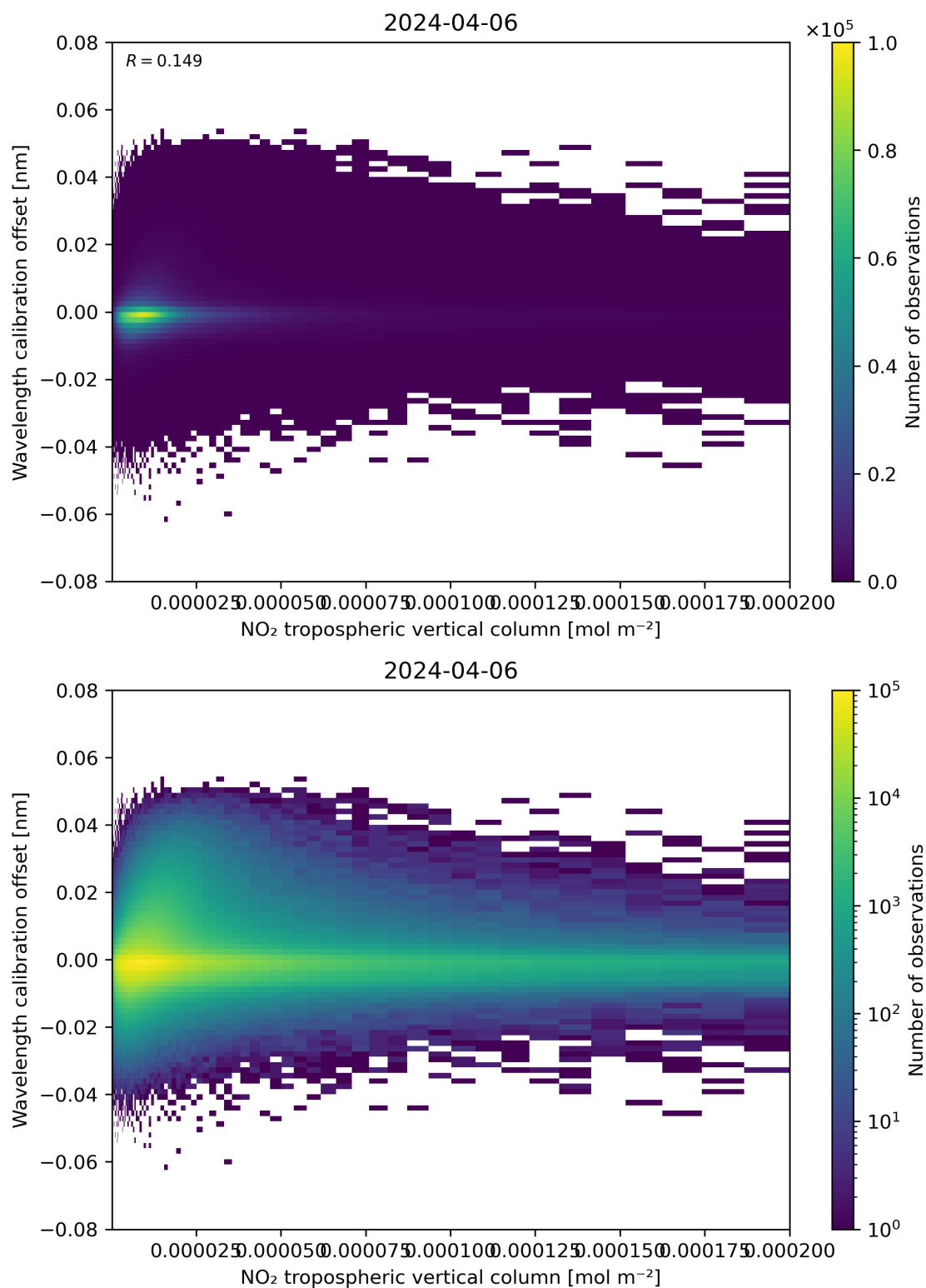
Figure 143: Scatter density plot of “NO 2 tropospheric vertical column” against “Wavelength calibration offset” for 2024-04-05 to 2024-04-07.
