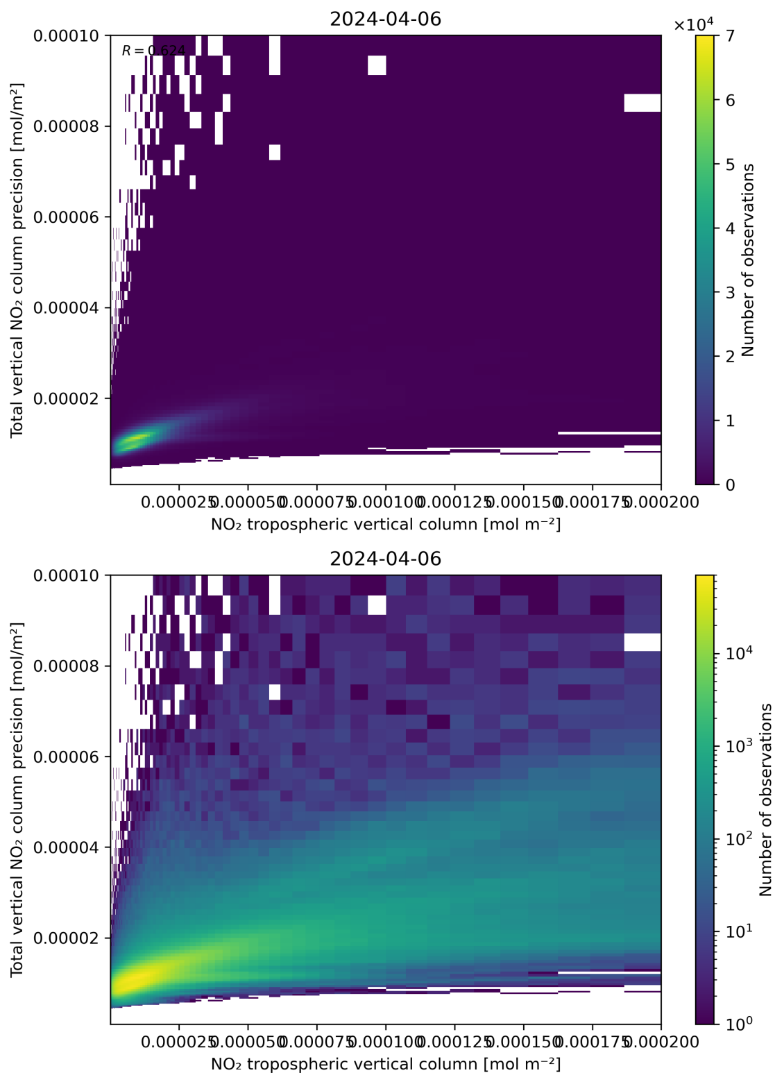
Figure 129: Scatter density plot of “NO 2 tropospheric vertical column” against “Total vertical NO 2 column precision” for 2024-04-05 to 2024-04-07.
