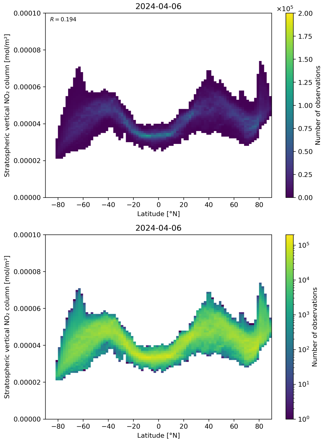
Figure 87: Scatter density plot of “Latitude” against “Stratospheric vertical NO 2 column” for 2024-04-05 to 2024-04-07.
