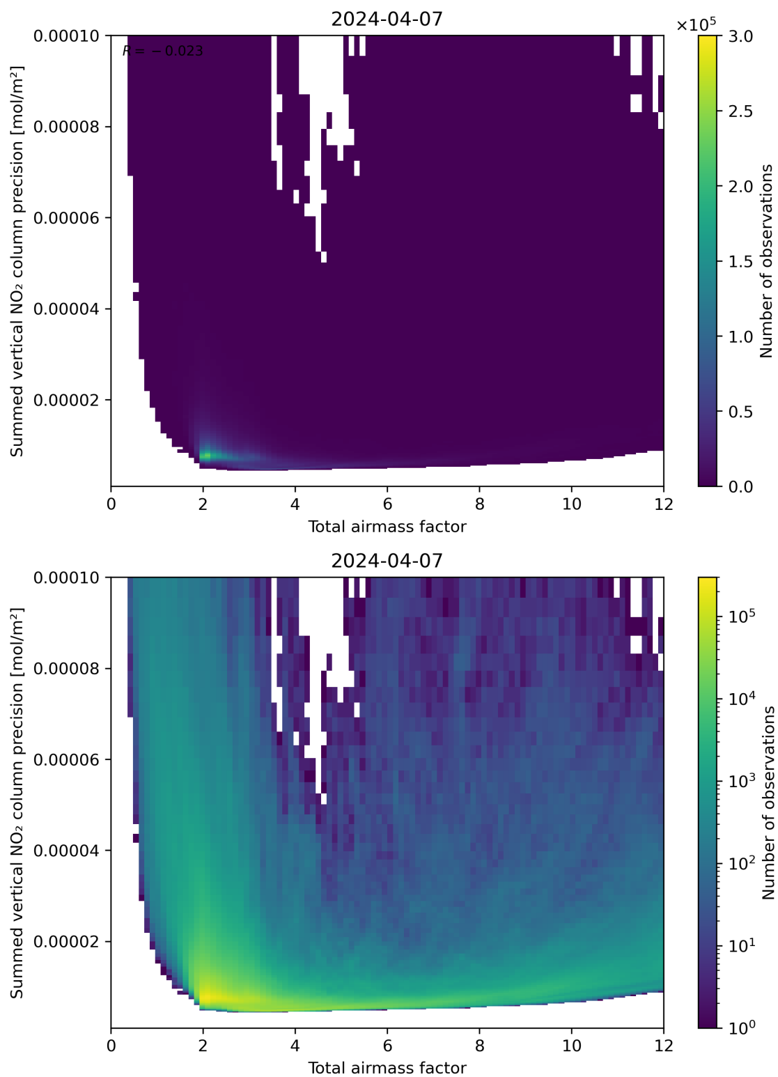
Figure 66: Scatter density plot of “Total airmass factor” against “Summed vertical NO 2 column precision” for 2024-04-06 to 2024-04-08.
