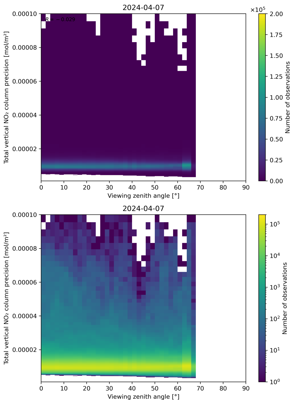
Figure 168: Scatter density plot of “Viewing zenith angle” against “Total vertical NO 2 column precision” for 2024-04-06 to 2024-04-08.
