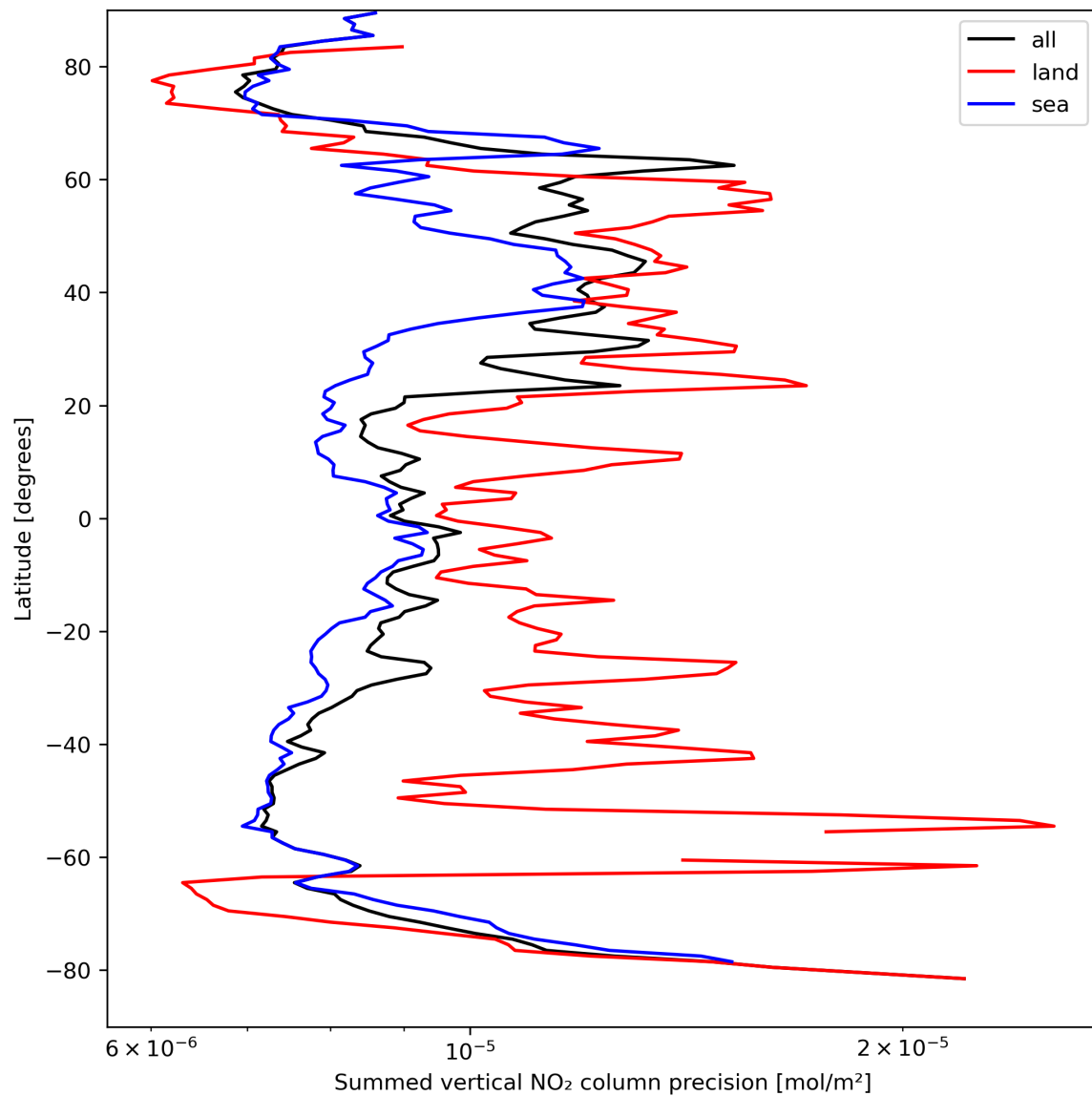
Figure 24: Zonal average of “Summed vertical NO 2 column precision” for 2024-04-06 to 2024-04-08.
