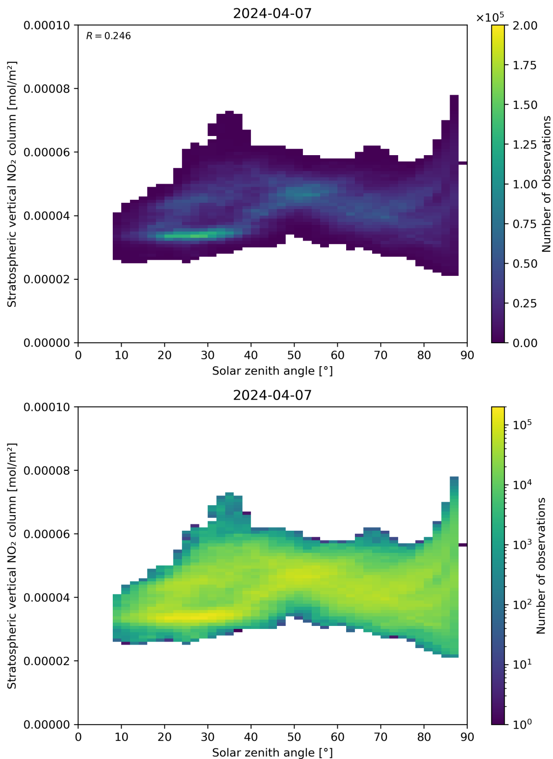
Figure 150: Scatter density plot of “Solar zenith angle” against “Stratospheric vertical NO 2 column” for 2024-04-06 to 2024-04-08.
