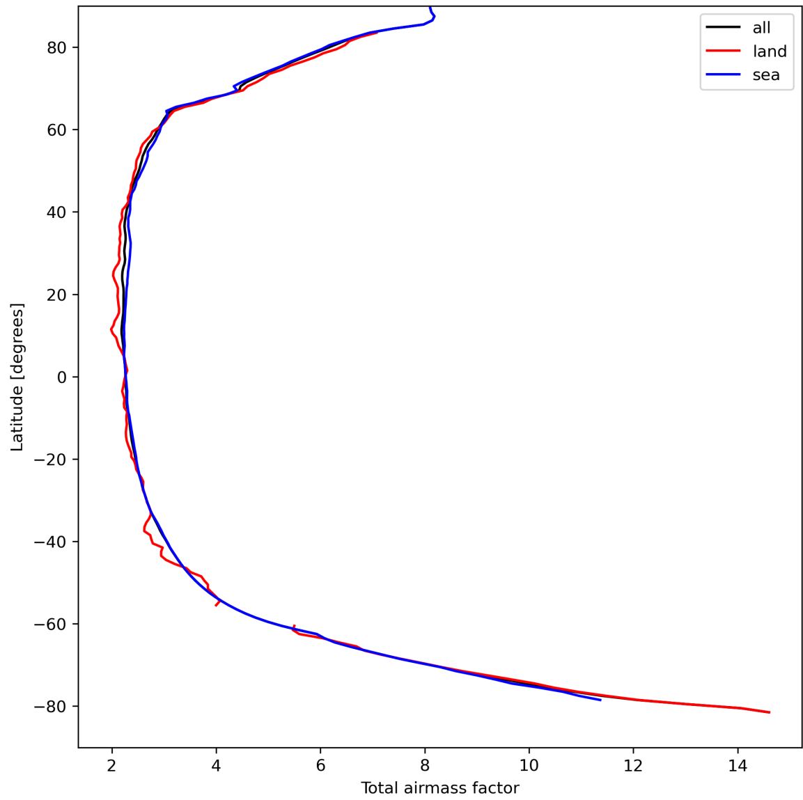
Figure 15: Zonal average of “Total airmass factor” for 2024-04-06 to 2024-04-08.
