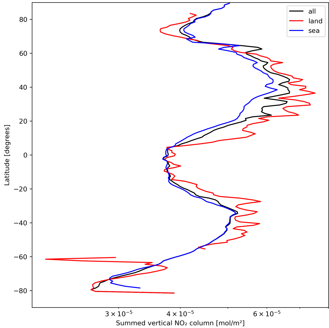
Figure 23: Zonal average of “Summed vertical NO 2 column” for 2024-04-06 to 2024-04-08.
