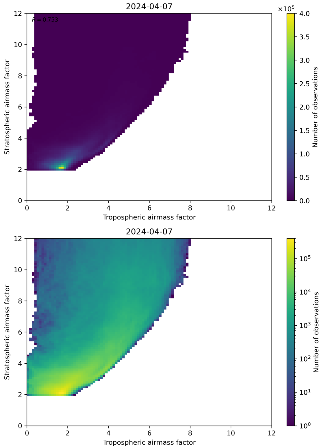
Figure 71: Scatter density plot of “Tropospheric airmass factor” against “Stratospheric airmass factor” for 2024-04-06 to 2024-04-08.
