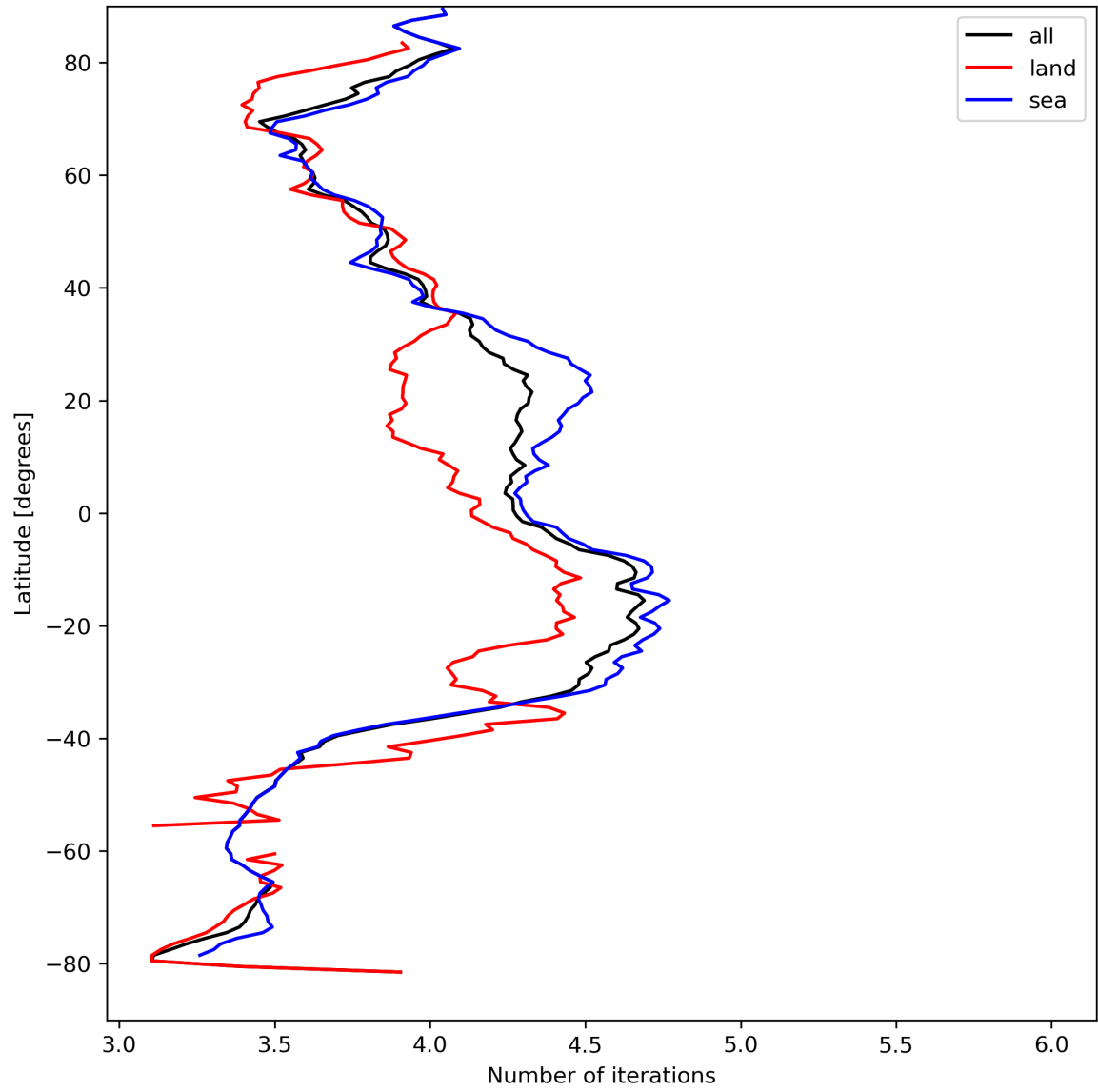
Figure 17: Zonal average of “Number of iterations” for 2024-04-06 to 2024-04-08.
