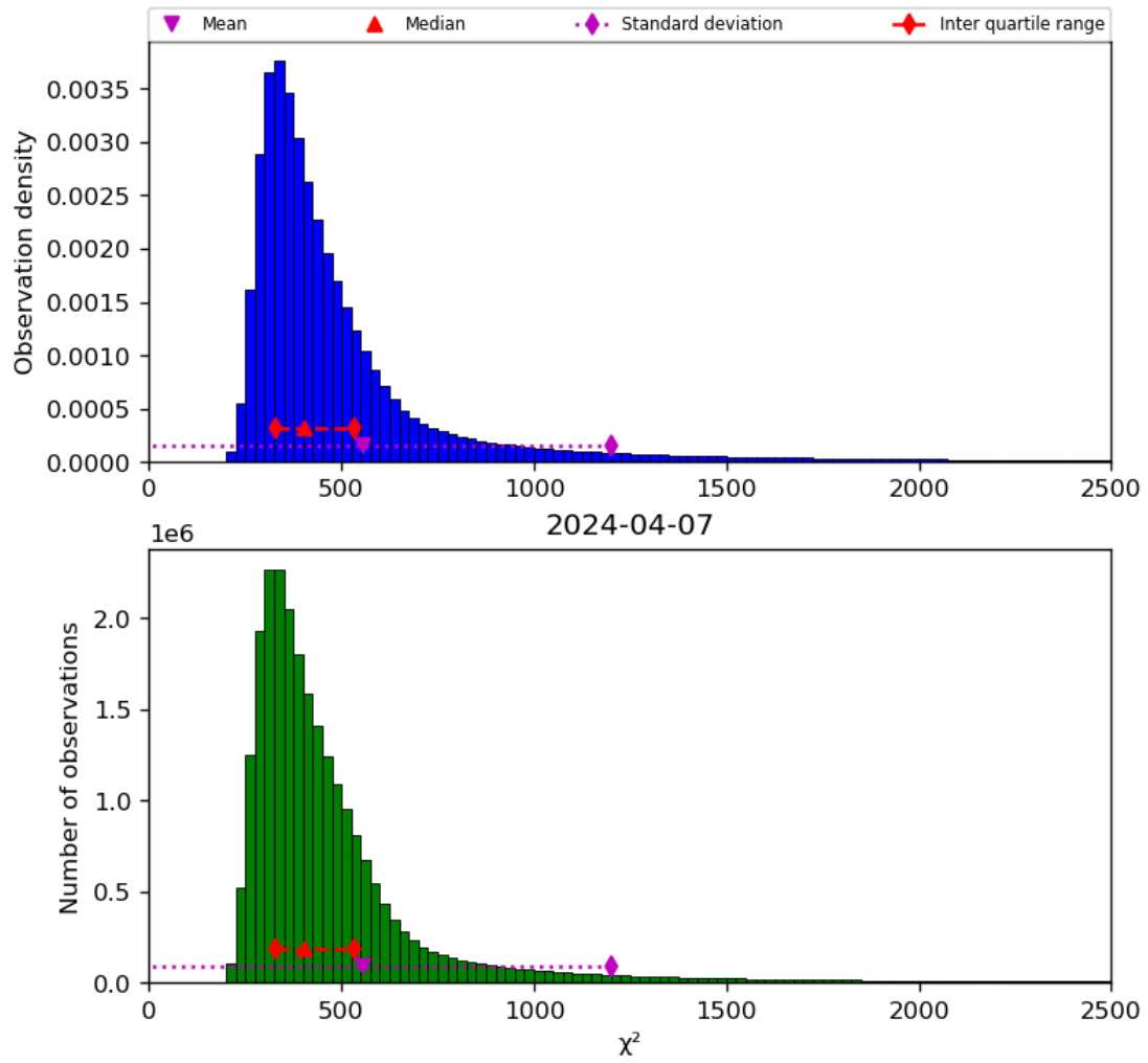
Figure 42: Histogram of “ \chi^2 ” for 2024-04-06 to 2024-04-08
