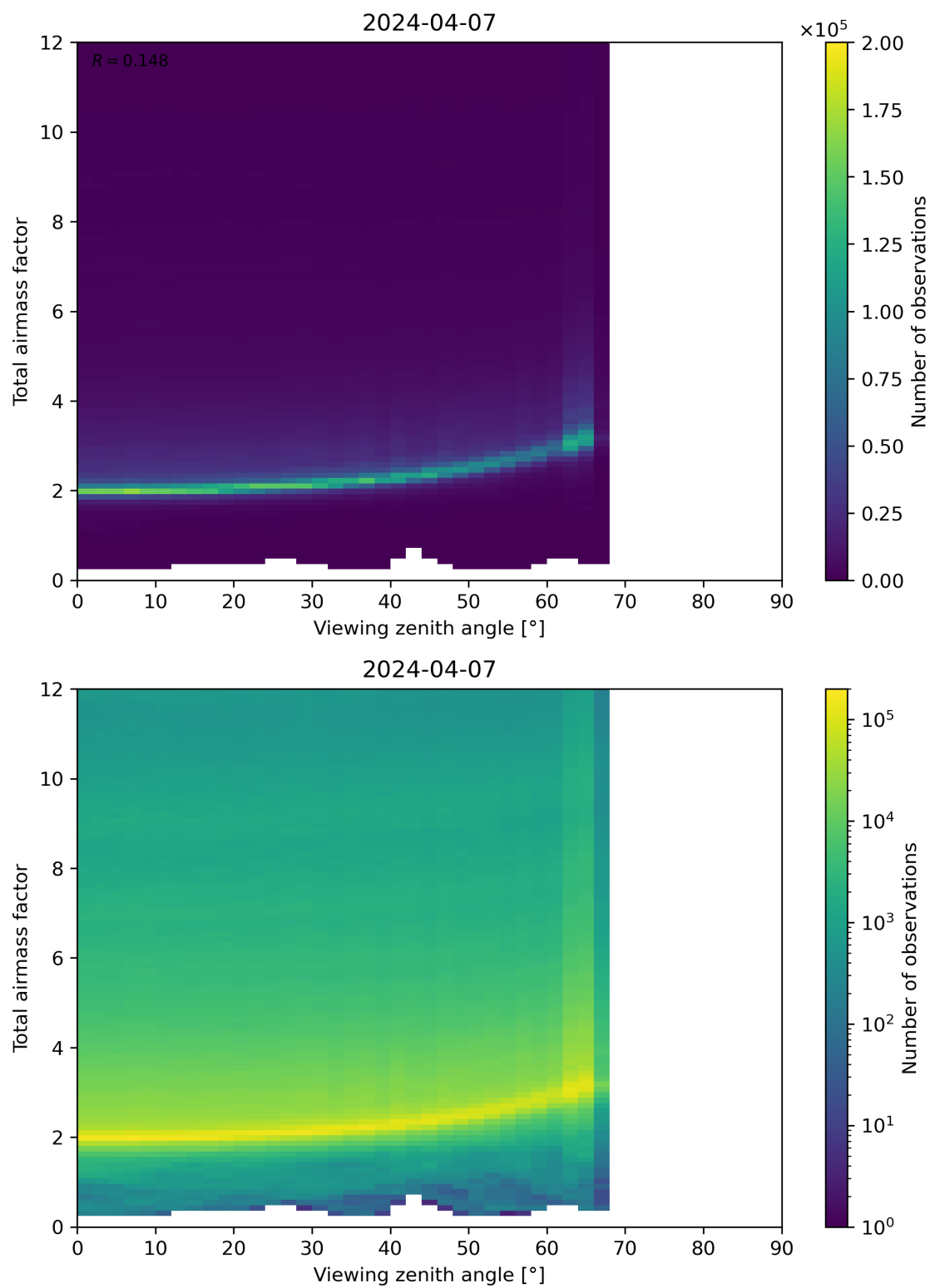
Figure 160: Scatter density plot of “Viewing zenith angle” against “Total airmass factor” for 2024-04-06 to 2024-04-08.
