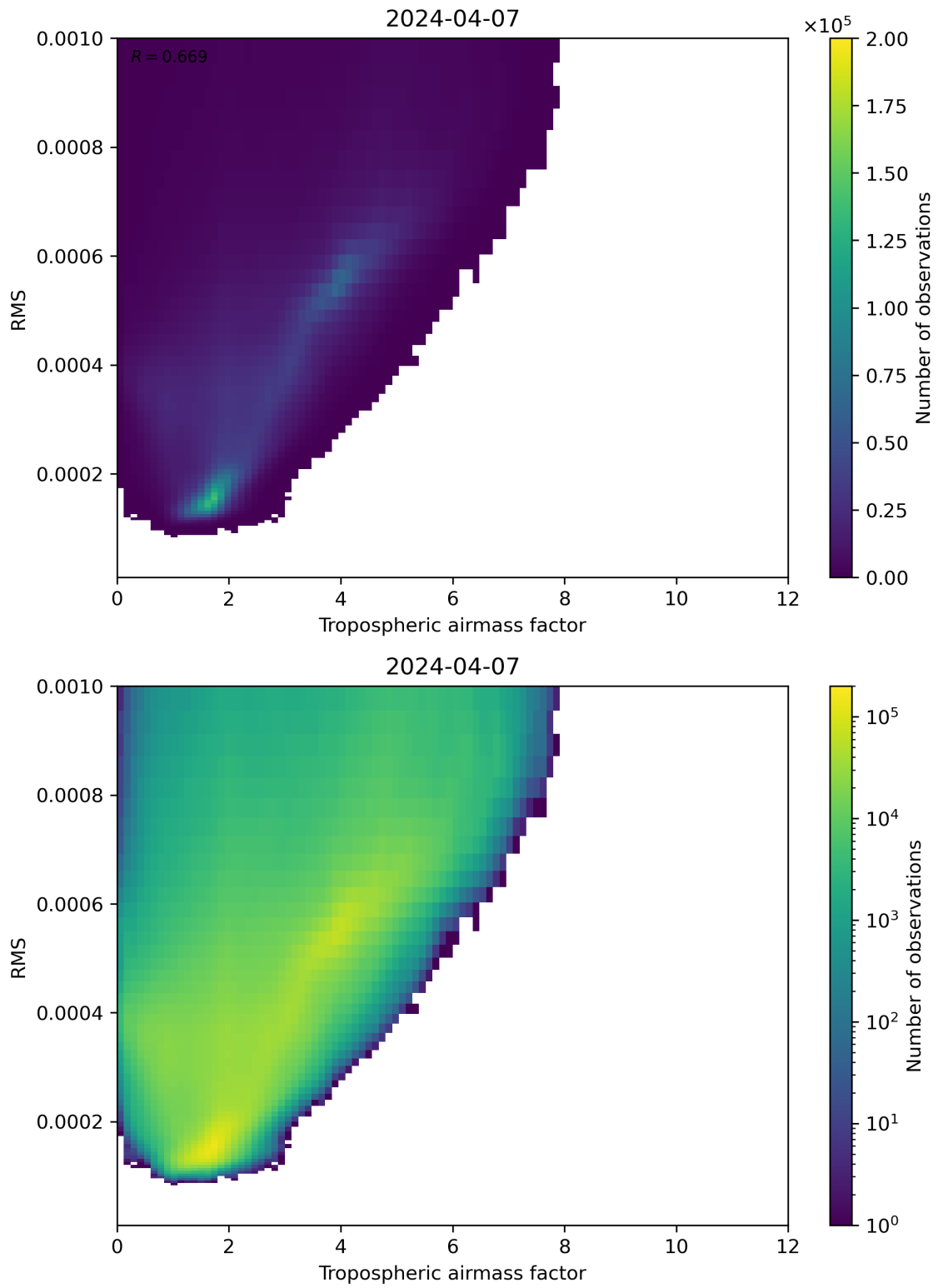
Figure 79: Scatter density plot of “Tropospheric airmass factor” against “RMS” for 2024-04-06 to 2024-04-08.
