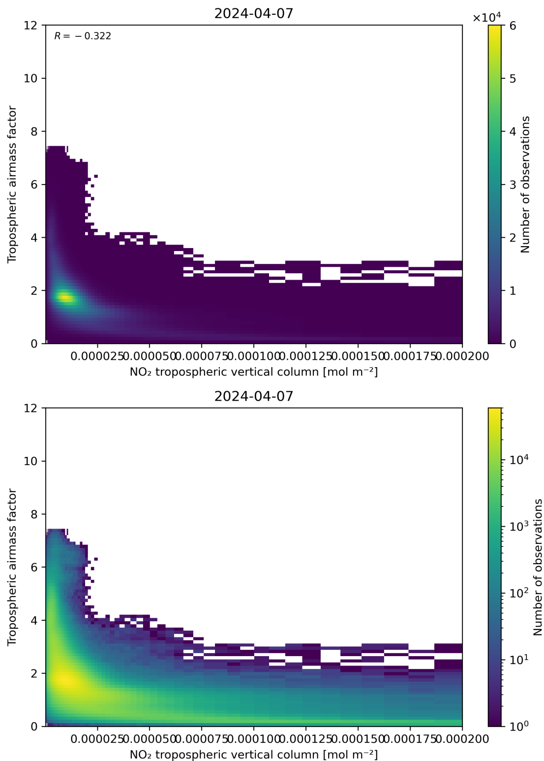
Figure 123: Scatter density plot of “NO 2 tropospheric vertical column” against “Tropospheric airmass factor” for 2024-04-06 to 2024-04-08.
