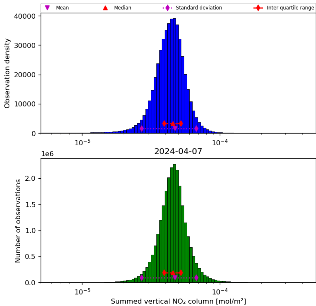
Figure 40: Histogram of “Summed vertical NO 2 column” for 2024-04-06 to 2024-04-08
