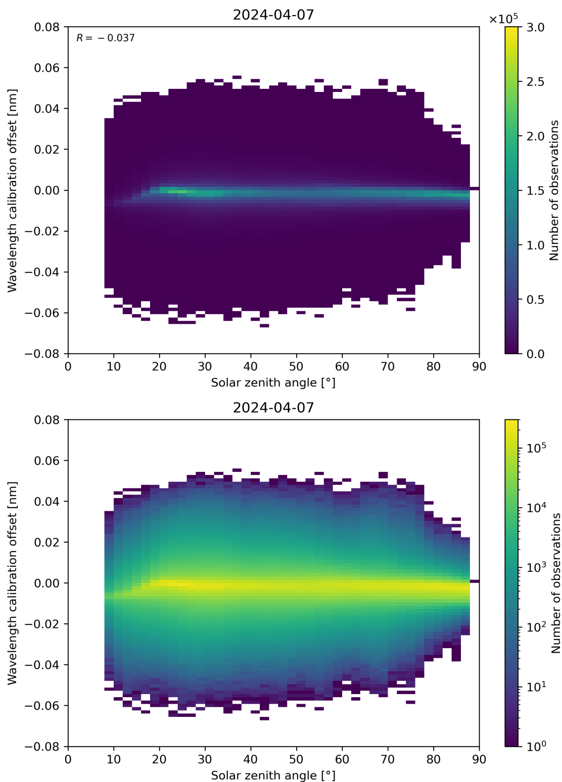
Figure 158: Scatter density plot of “Solar zenith angle” against “Wavelength calibration offset” for 2024-04-06 to 2024-04-08.
