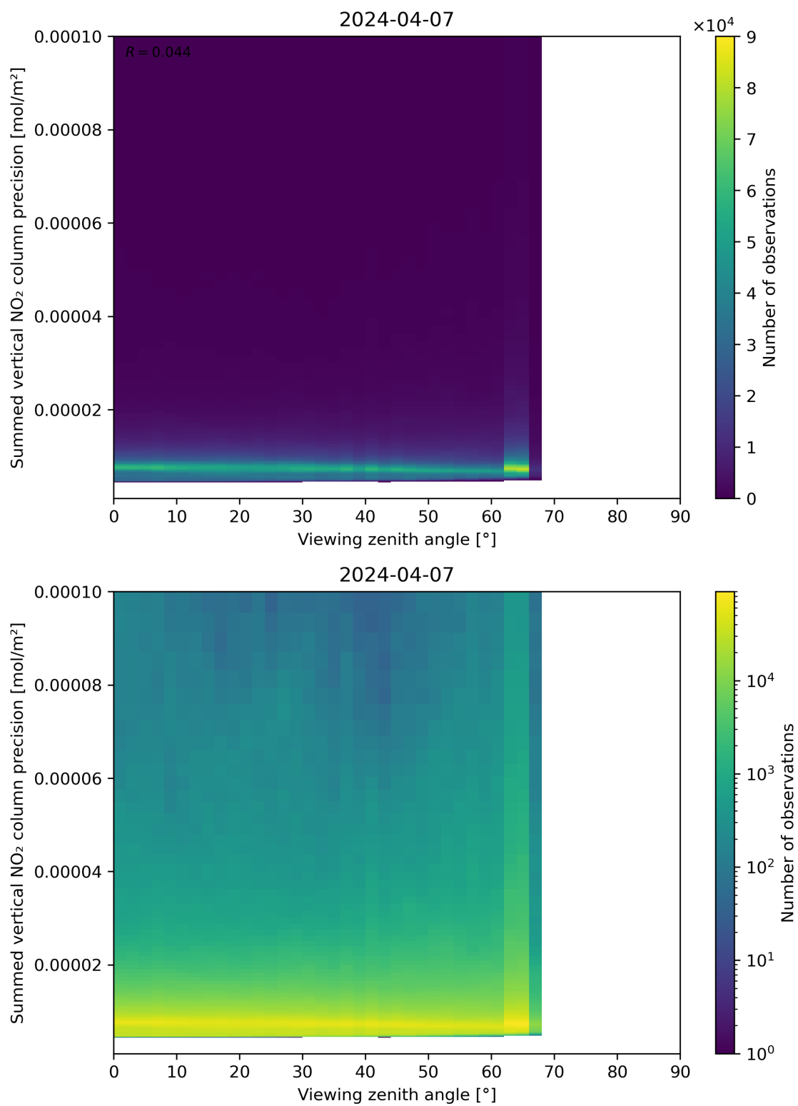
Figure 166: Scatter density plot of “Viewing zenith angle” against “Summed vertical NO 2 column precision” for 2024-04-06 to 2024-04-08.
