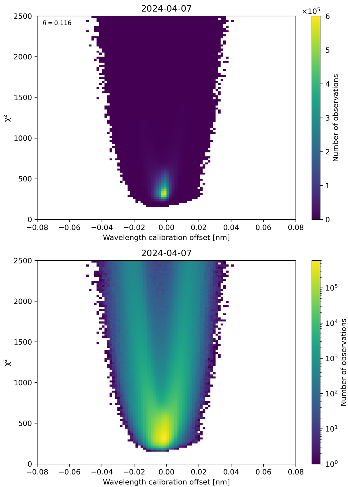
Figure 175: Scatter density plot of “Wavelength calibration offset” against “ \chi^2 ” for 2024-04-06 to 2024-04-08.
