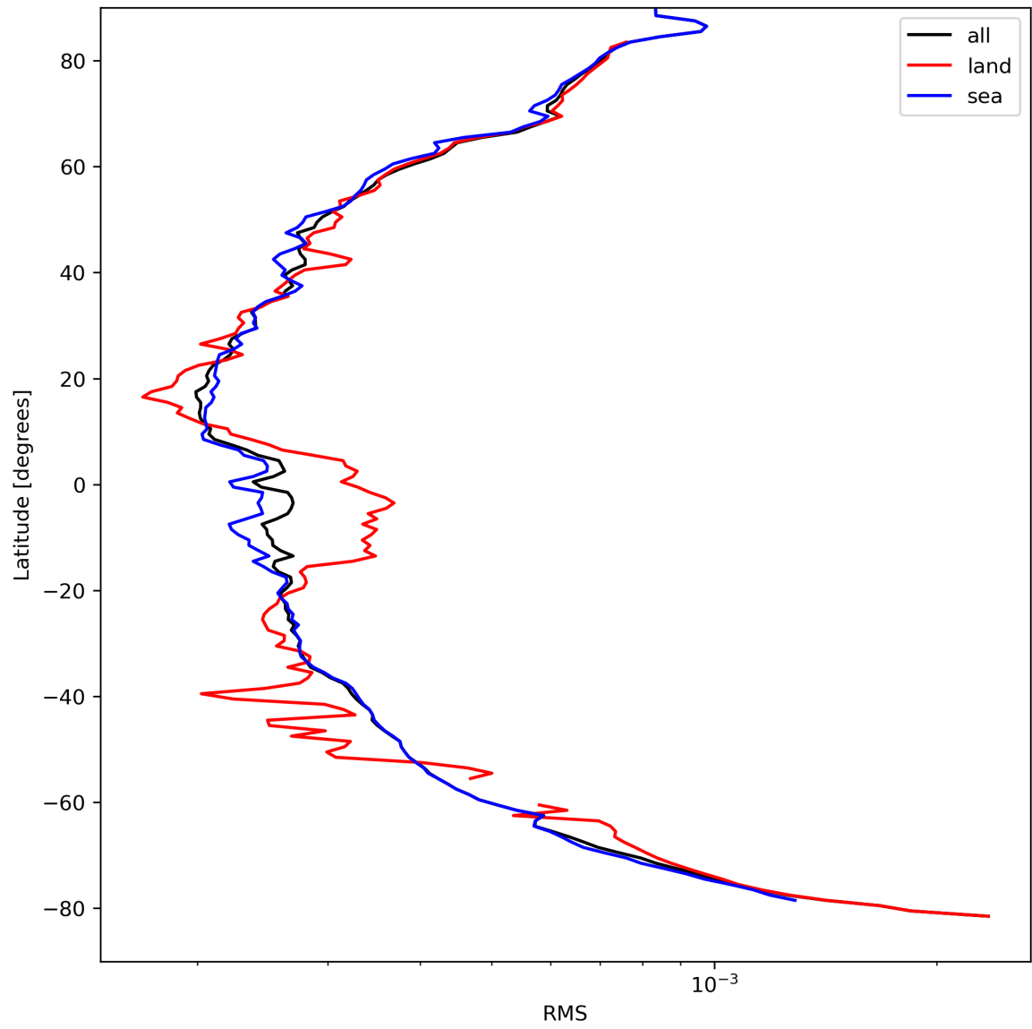
Figure 26: Zonal average of “RMS” for 2024-04-06 to 2024-04-08.
