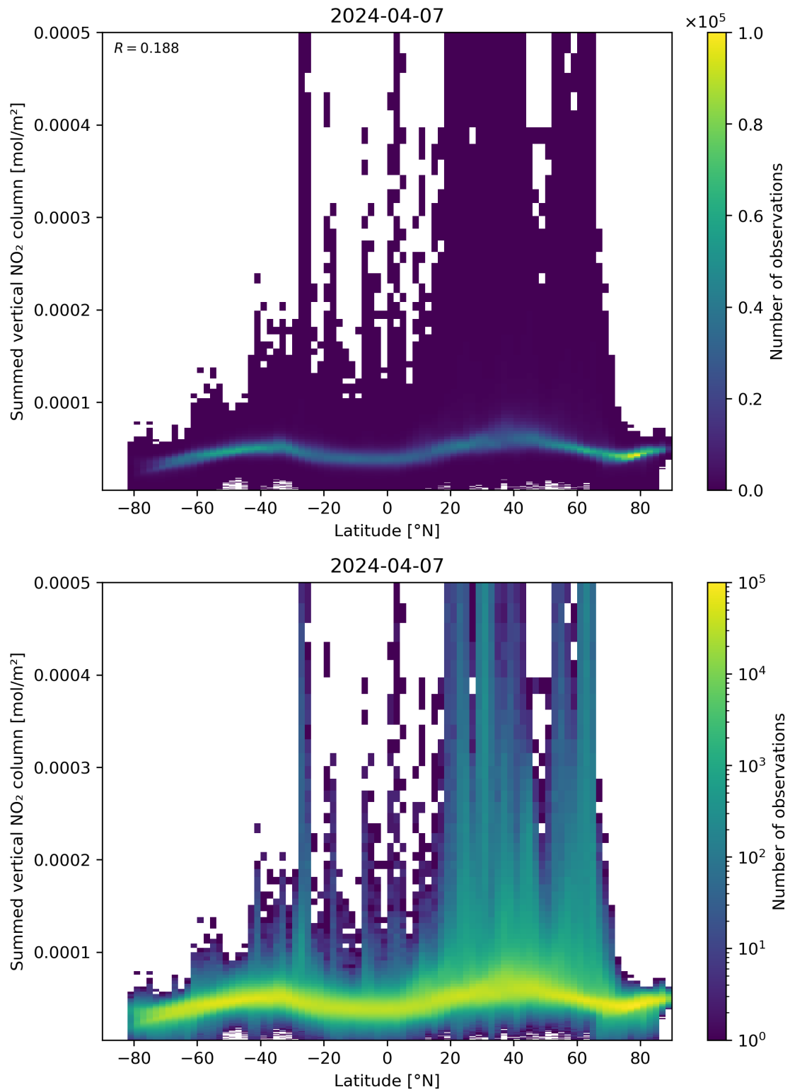
Figure 88: Scatter density plot of “Latitude” against “Summed vertical NO 2 column” for 2024-04-06 to 2024-04-08.
