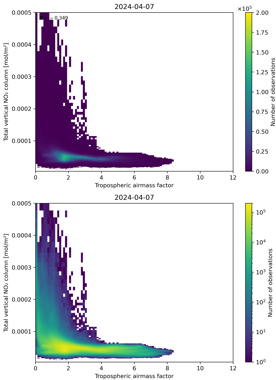
Figure 77: Scatter density plot of “Tropospheric airmass factor” against “Total vertical NO 2 column” for 2024-04-06 to 2024-04-08.
