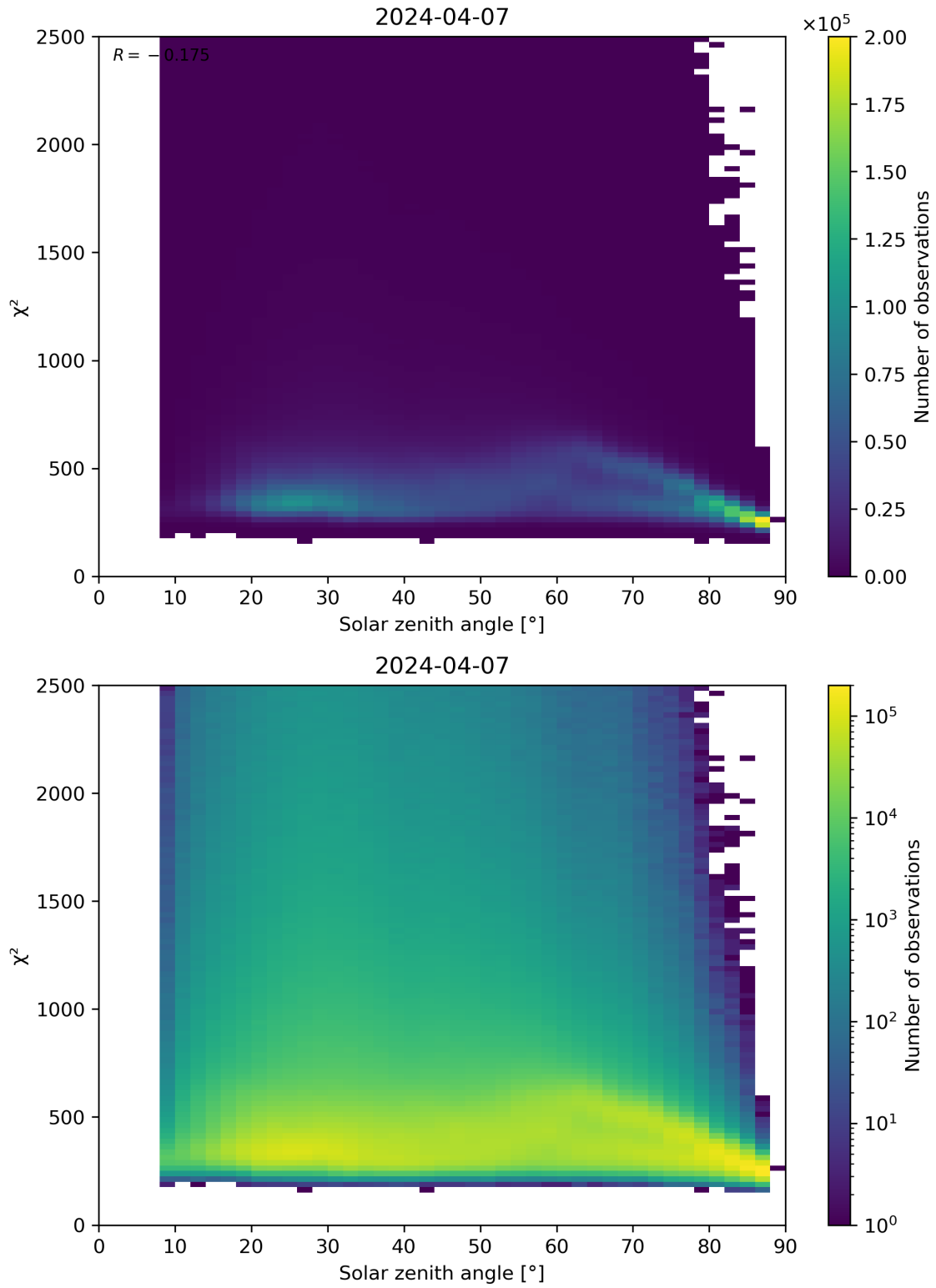
Figure 148: Scatter density plot of “Solar zenith angle” against “ \chi^2 ” for 2024-04-06 to 2024-04-08.
