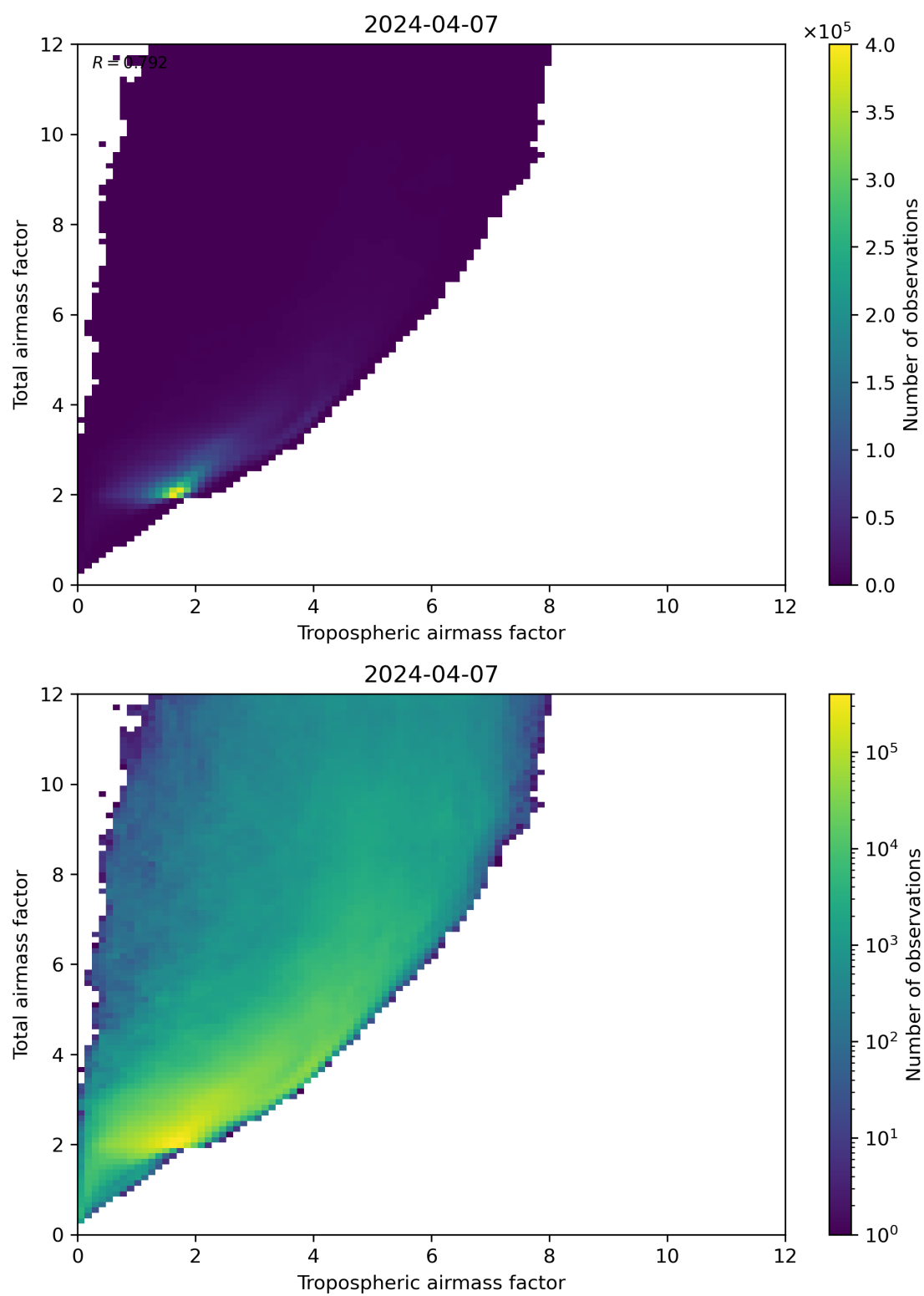
Figure 72: Scatter density plot of “Tropospheric airmass factor” against “Total airmass factor” for 2024-04-06 to 2024-04-08.
