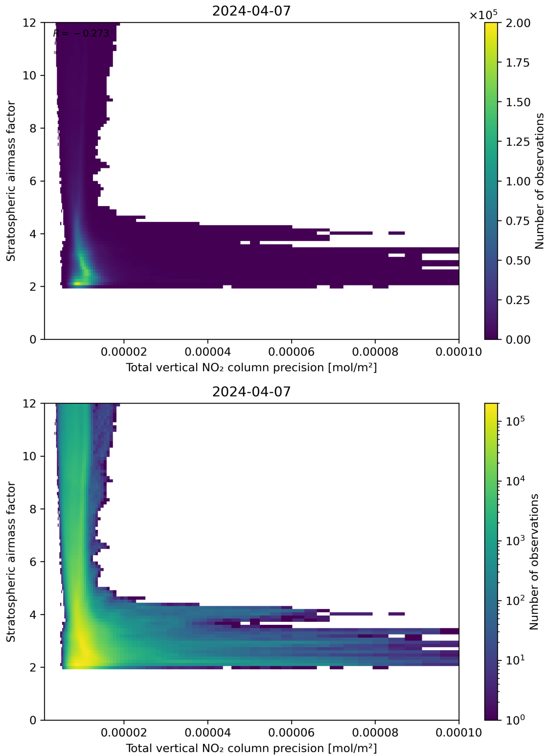
Figure 115: Scatter density plot of “Total vertical NO 2 column precision” against “Stratospheric airmass factor” for 2024-04-06 to 2024-04-08.
