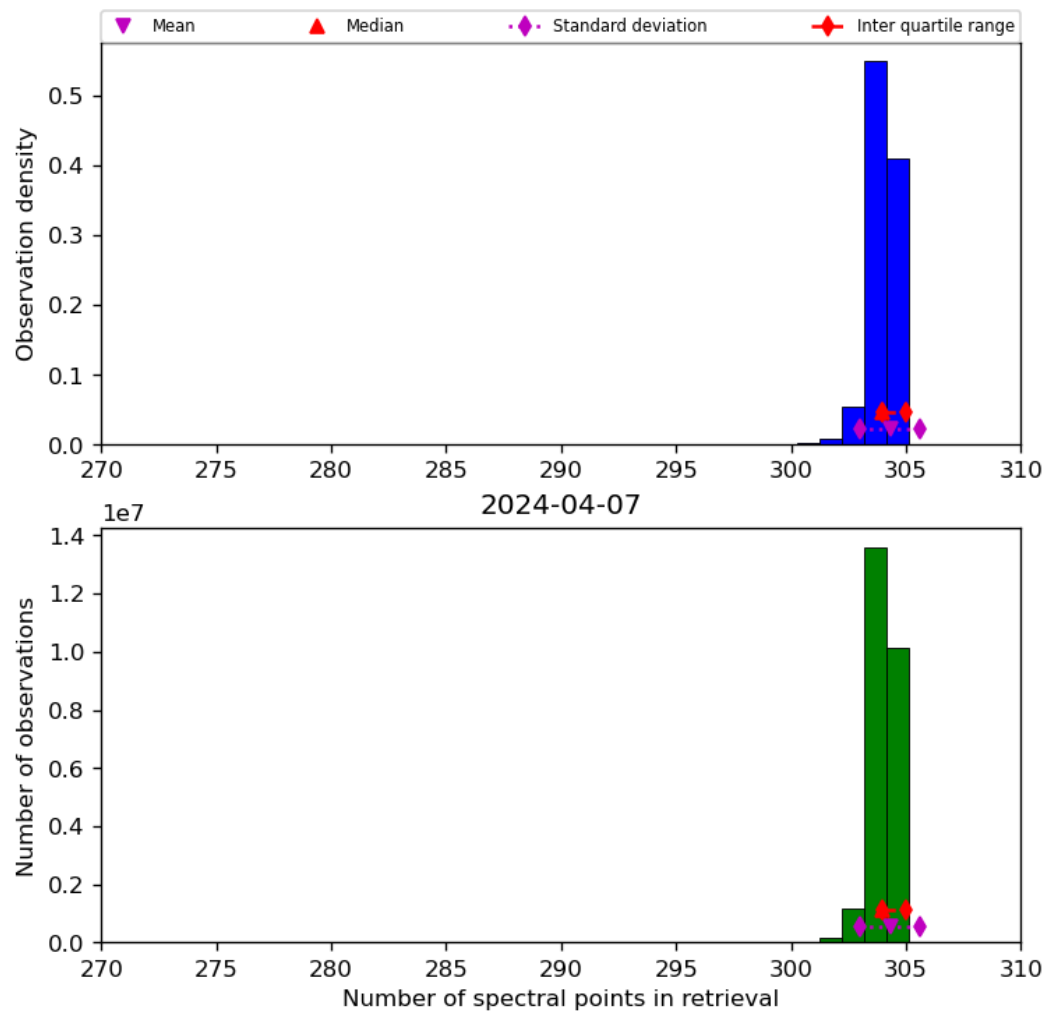
Figure 33: Histogram of “Number of spectral points in retrieval” for 2024-04-06 to 2024-04-08
