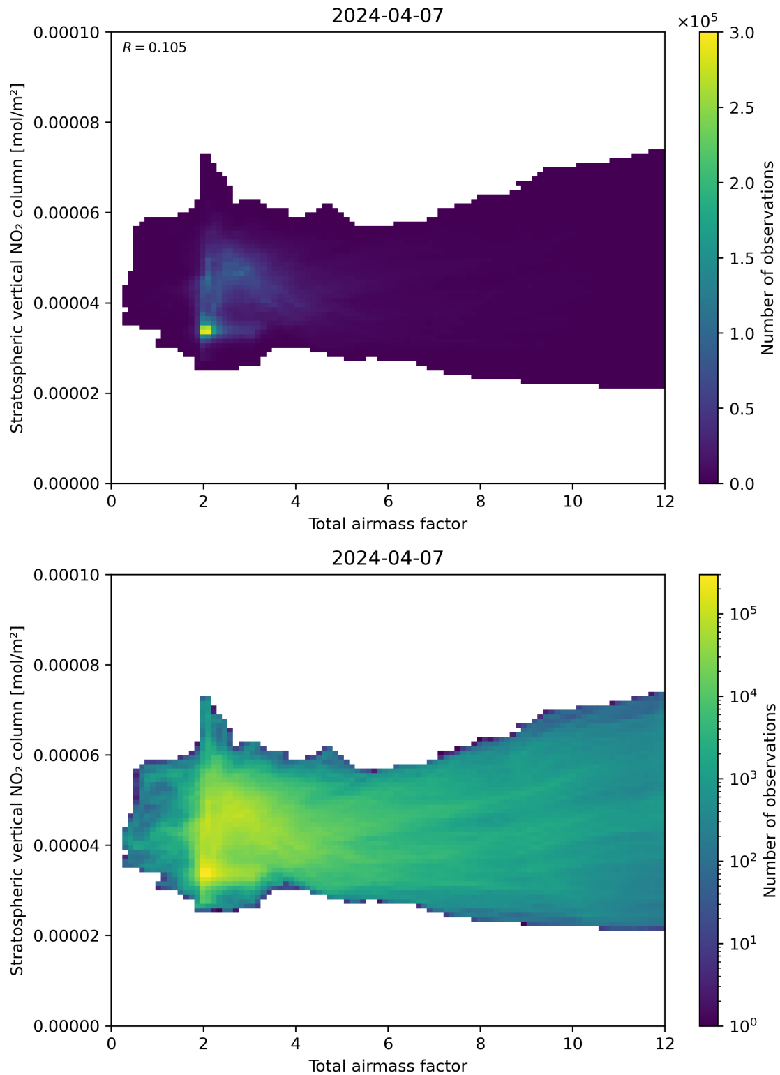
Figure 64: Scatter density plot of “Total airmass factor” against “Stratospheric vertical NO 2 column” for 2024-04-06 to 2024-04-08.
