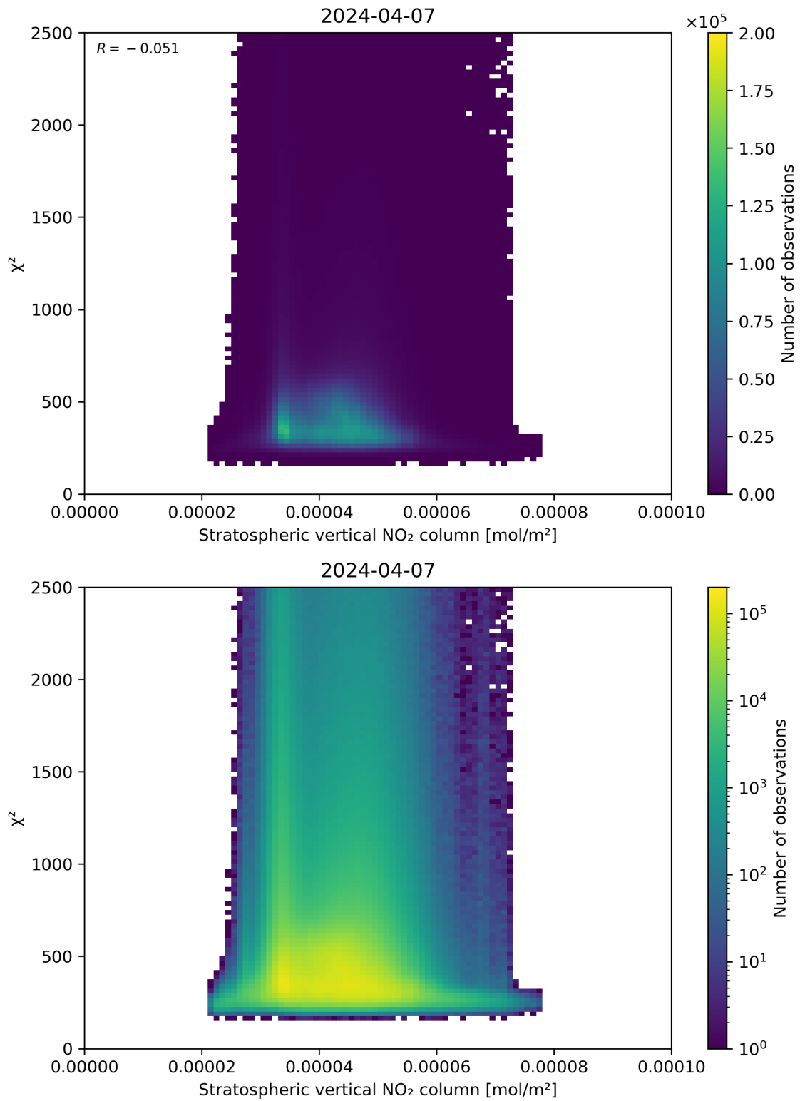
Figure 97: Scatter density plot of “Stratospheric vertical NO 2 column” against “ \chi^2 ” for 2024-04-06 to 2024-04-08.
