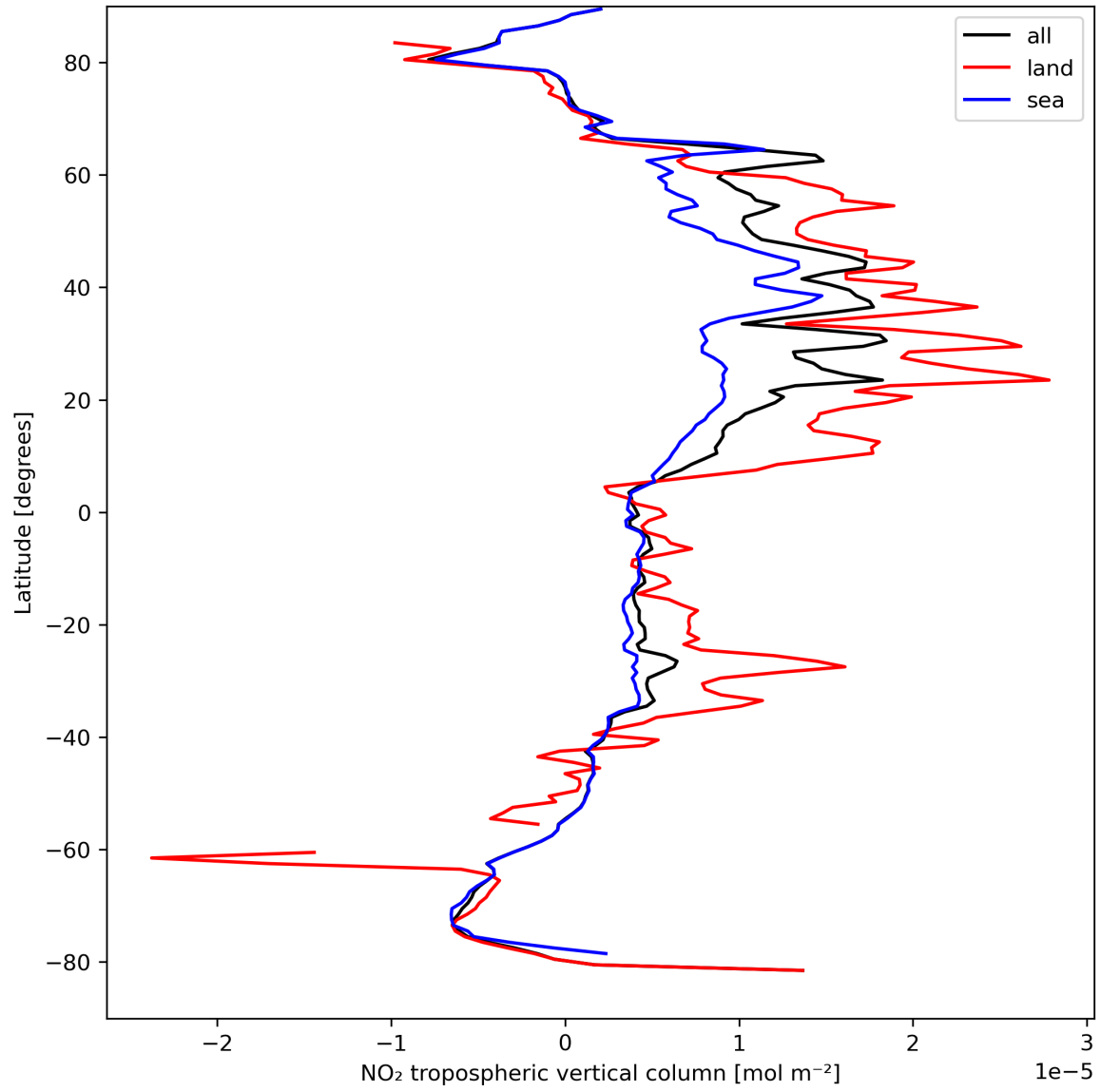
Figure 12: Zonal average of “NO 2 tropospheric vertical column” for 2024-04-06 to 2024-04-08.
