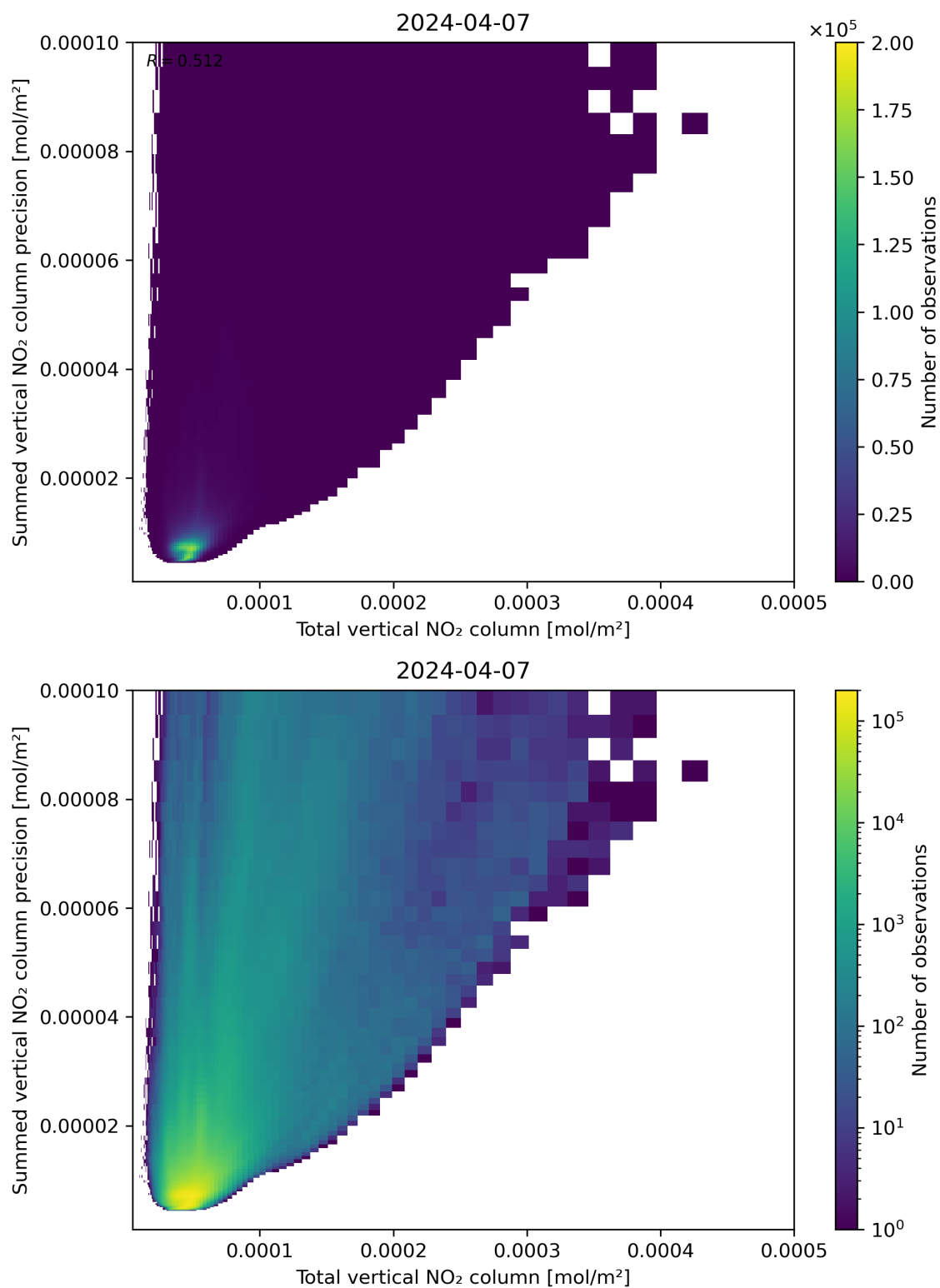
Figure 113: Scatter density plot of “Total vertical NO 2 column” against “Summed vertical NO 2 column precision” for 2024-04-06 to 2024-04-08.
