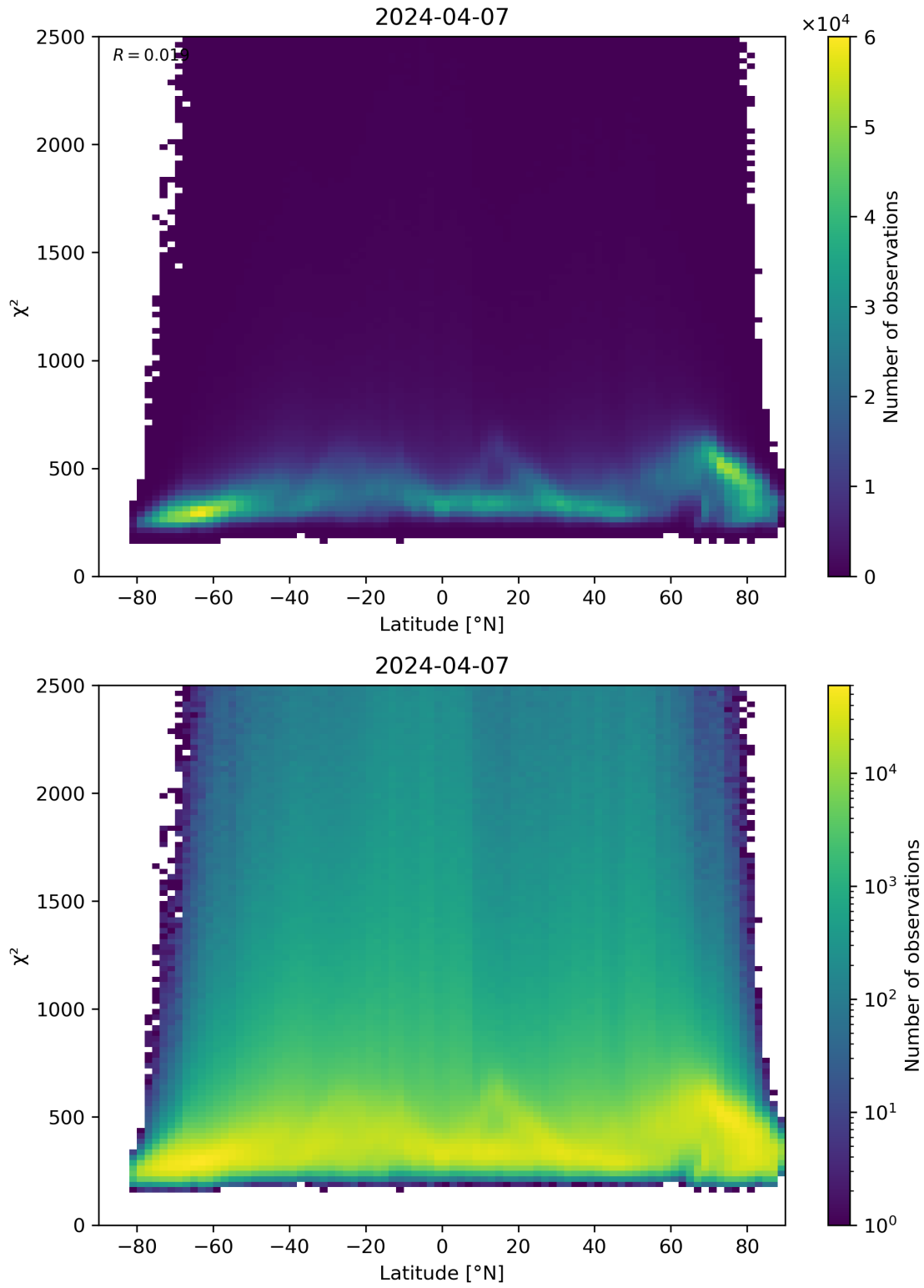
Figure 86: Scatter density plot of “Latitude” against “ \chi^2 ” for 2024-04-06 to 2024-04-08.
