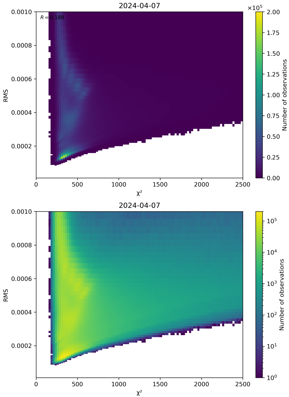
Figure 82: Scatter density plot of “ \chi^2 ” against “RMS” for 2024-04-06 to 2024-04-08.
