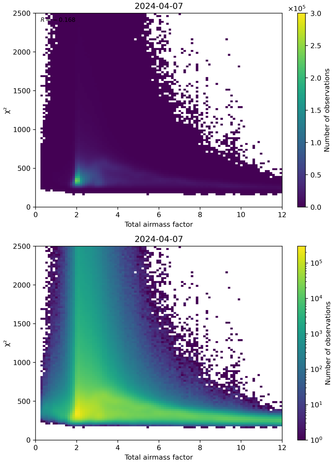
Figure 63: Scatter density plot of “Total airmass factor” against “ \chi^2 ” for 2024-04-06 to 2024-04-08.
