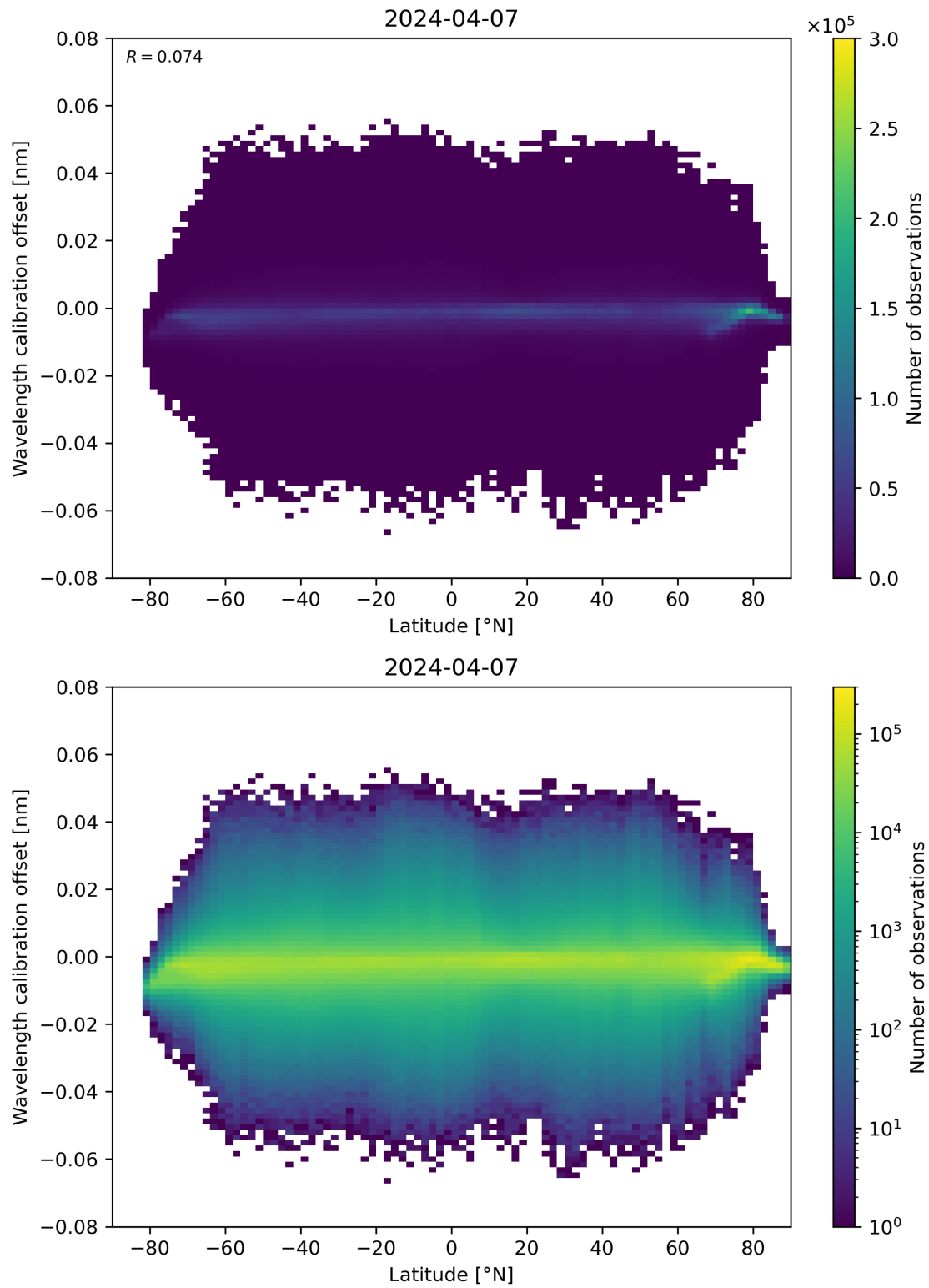
Figure 95: Scatter density plot of “Latitude” against “Wavelength calibration offset” for 2024-04-06 to 2024-04-08.
