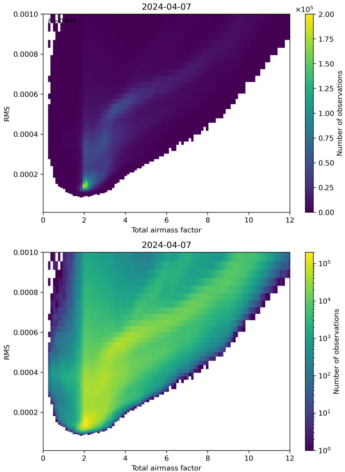
Figure 69: Scatter density plot of “Total airmass factor” against “RMS” for 2024-04-06 to 2024-04-08.
