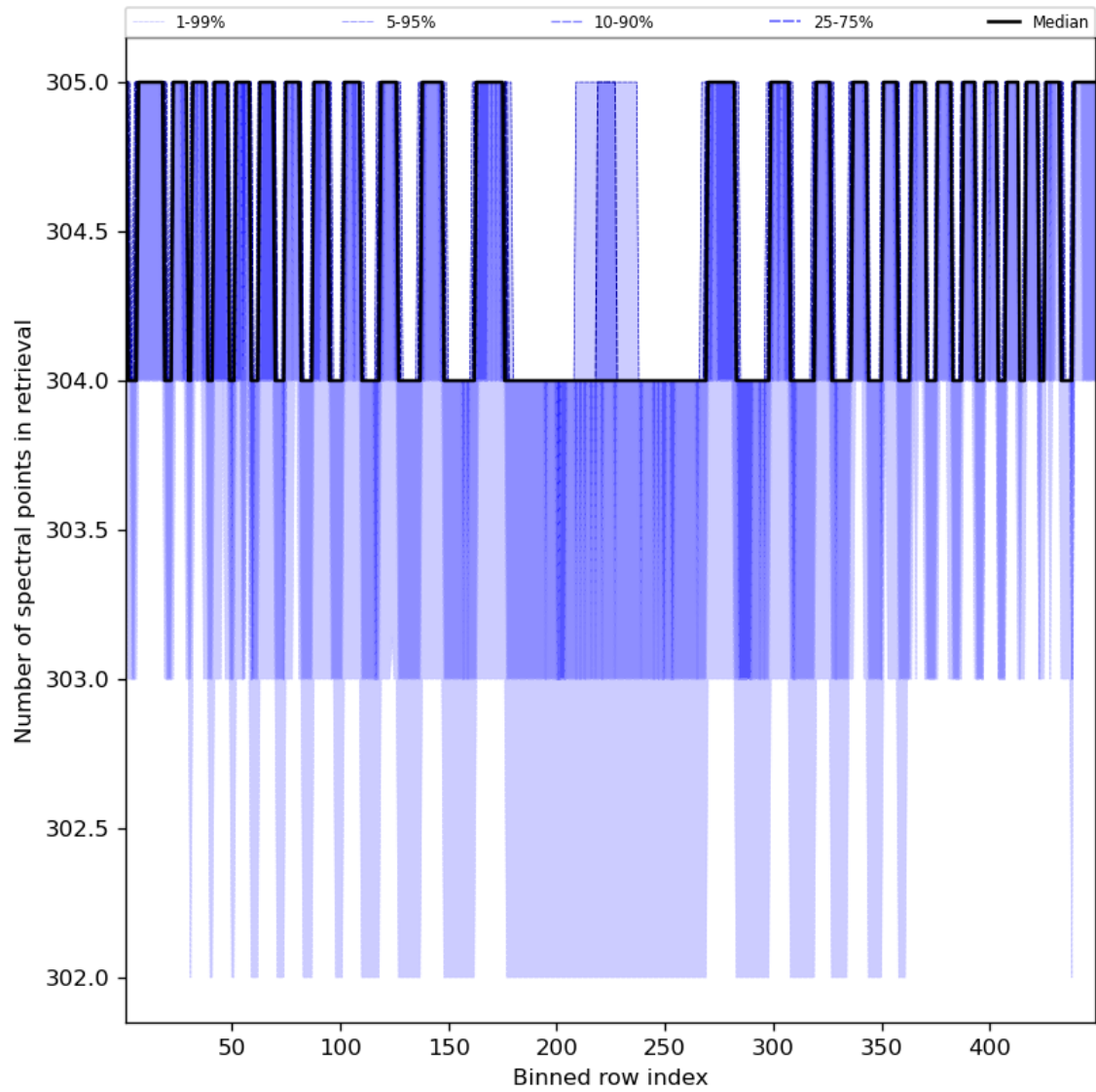
Figure 50: Along track statistics of “Number of spectral points in retrieval” for 2024-04-06 to 2024-04-08
