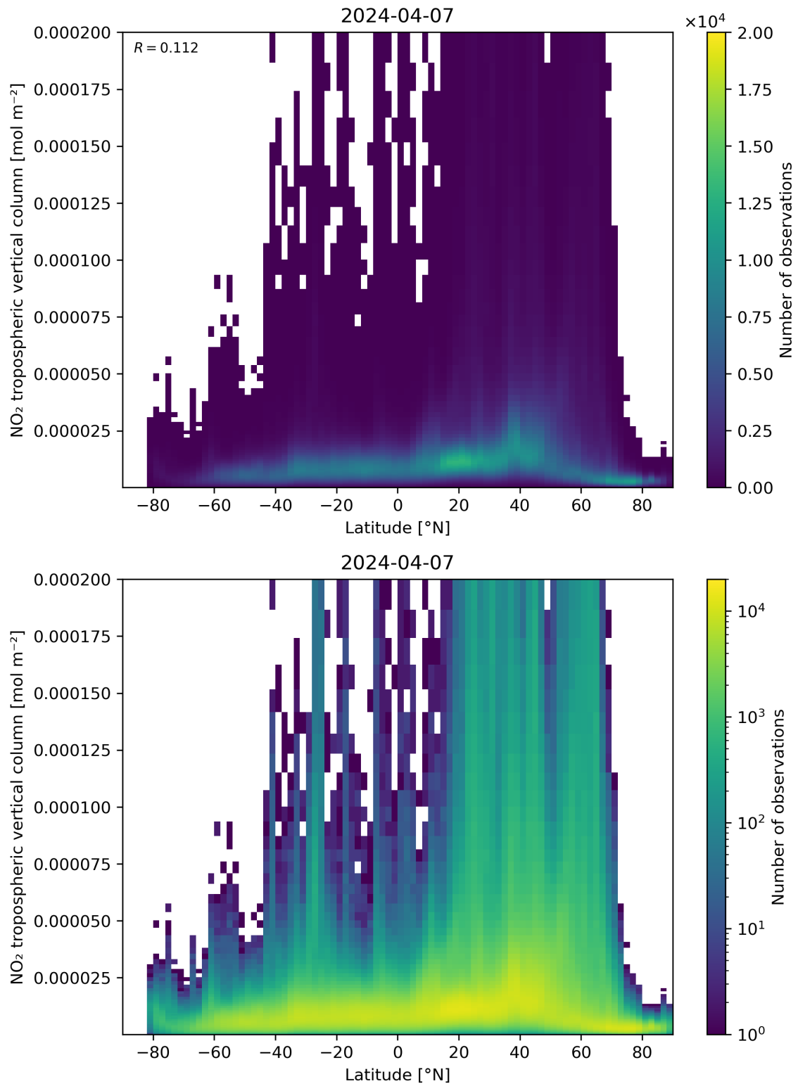
Figure 92: Scatter density plot of “Latitude” against “NO 2 tropospheric vertical column” for 2024-04-06 to 2024-04-08.
