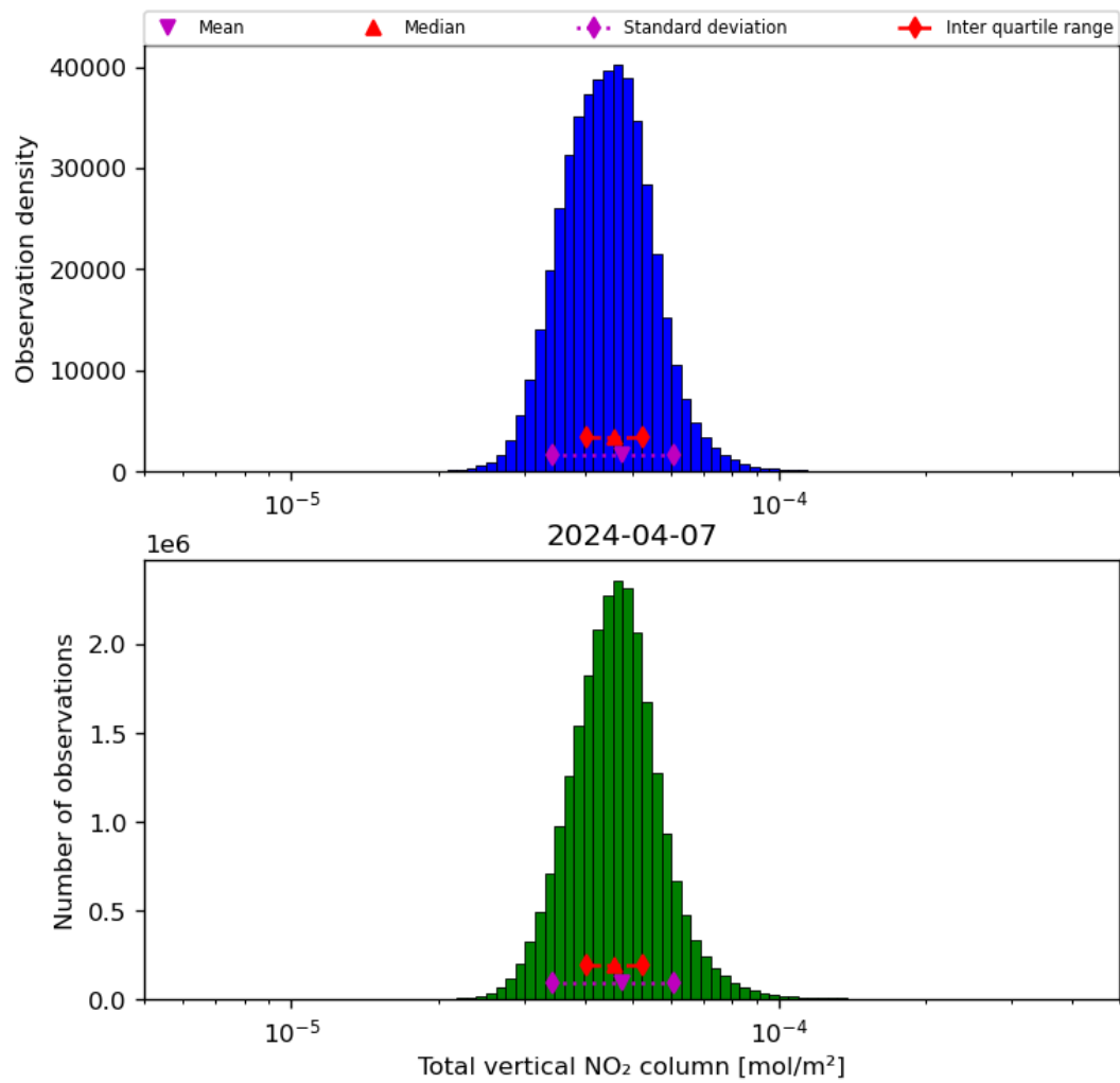
Figure 38: Histogram of “Total vertical NO 2 column” for 2024-04-06 to 2024-04-08
