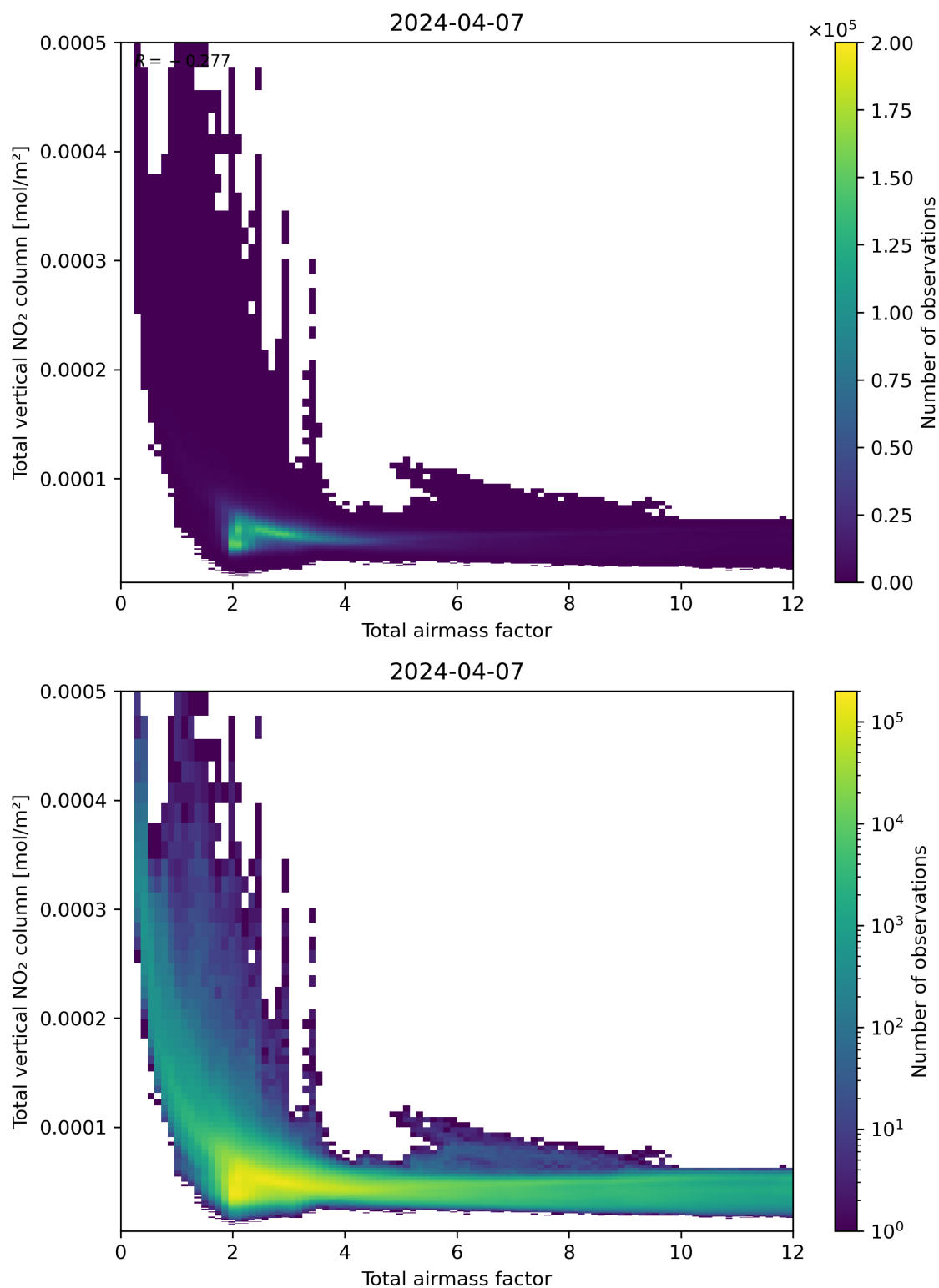
Figure 67: Scatter density plot of “Total airmass factor” against “Total vertical NO 2 column” for 2024-04-06 to 2024-04-08.
