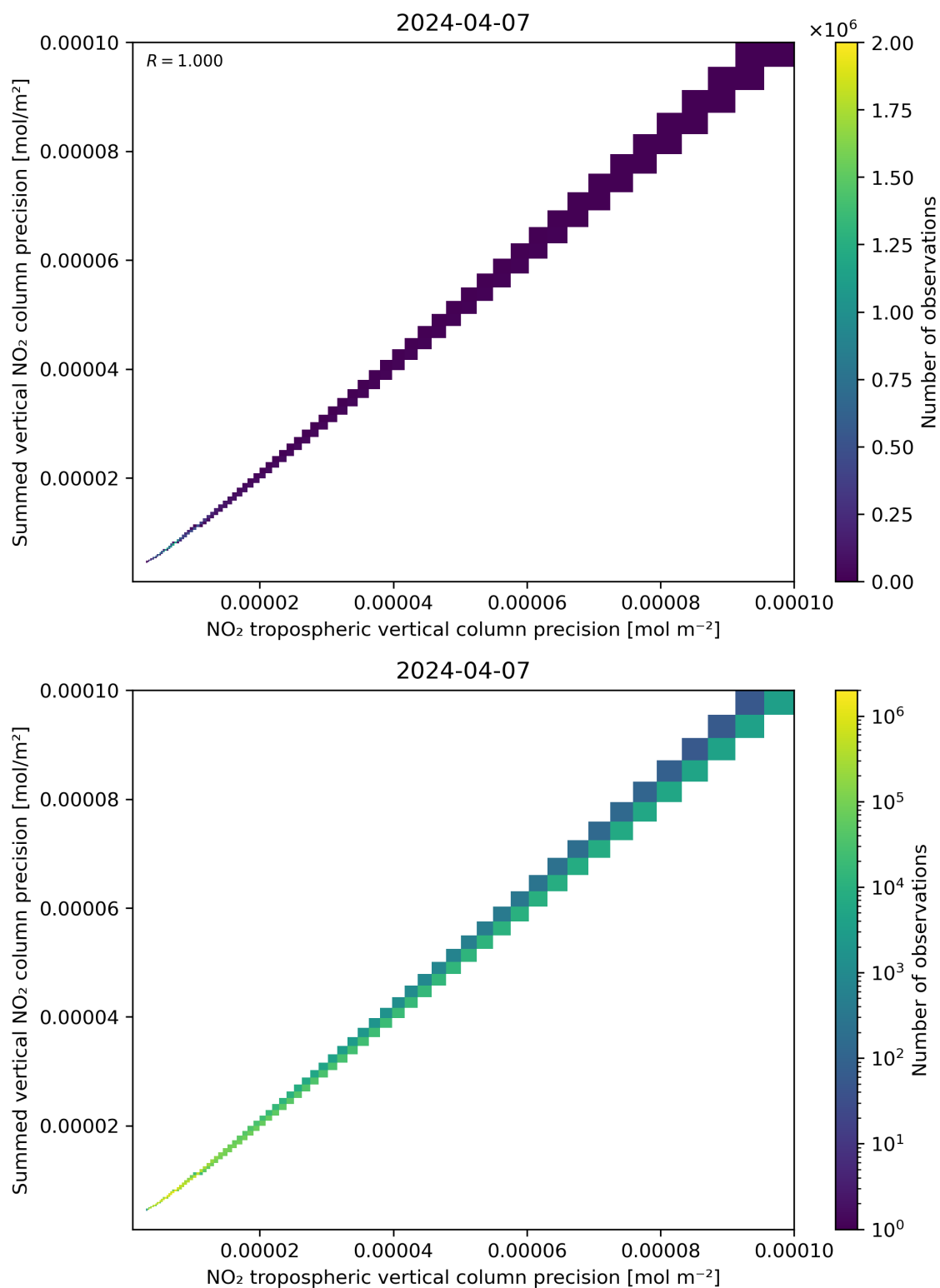
Figure 137: Scatter density plot of “NO 2 tropospheric vertical column precision” against “Summed vertical NO 2 column precision” for 2024-04-06 to 2024-04-08.
