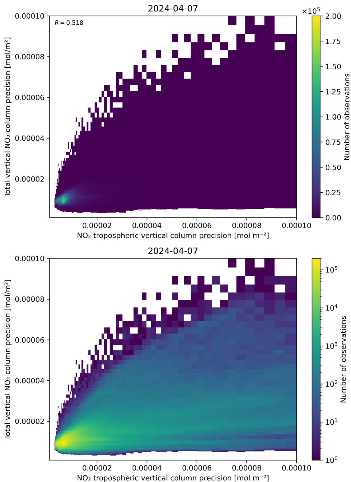
Figure 139: Scatter density plot of “NO 2 tropospheric vertical column precision” against “Total vertical NO 2 column precision” for 2024-04-06 to 2024-04-08.
