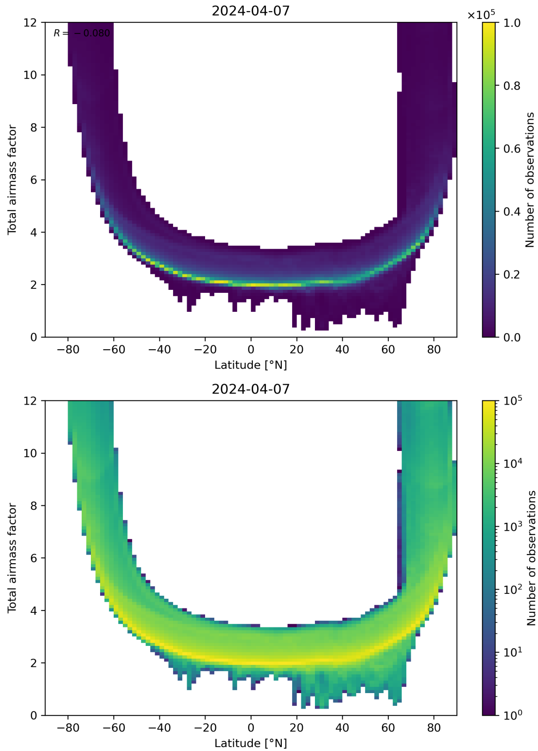
Figure 84: Scatter density plot of “Latitude” against “Total airmass factor” for 2024-04-06 to 2024-04-08.
