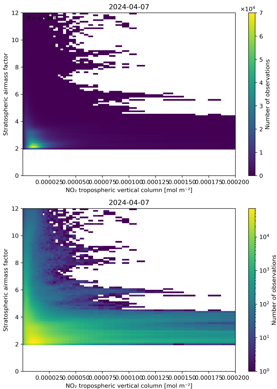
Figure 121: Scatter density plot of “NO 2 tropospheric vertical column” against “Stratospheric air mass factor” for 2024-04-06 to 2024-04-08.
