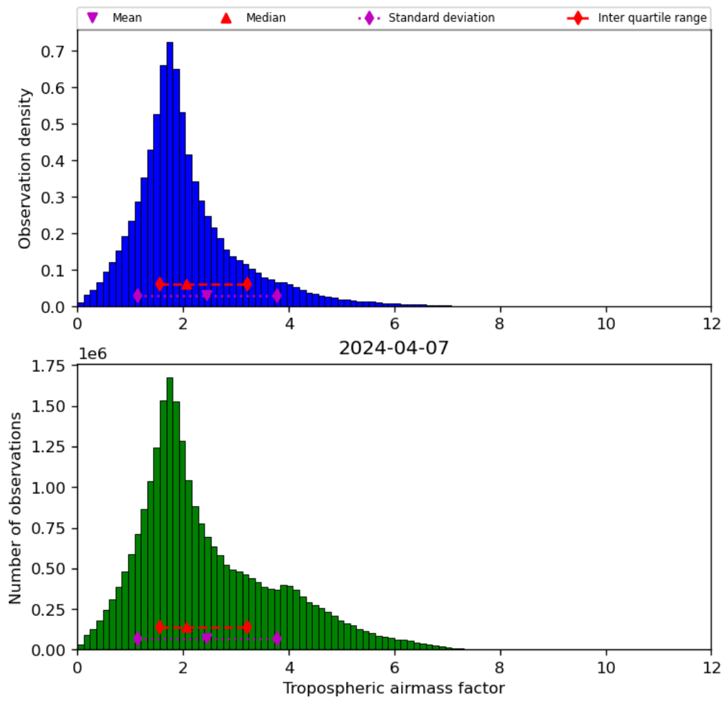
Figure 31: Histogram of “Tropospheric airmass factor” for 2024-04-06 to 2024-04-08
