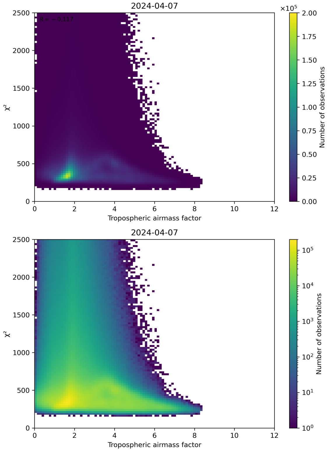
Figure 73: Scatter density plot of “Tropospheric airmass factor” against “ \chi^2 ” for 2024-04-06 to 2024-04-08.
