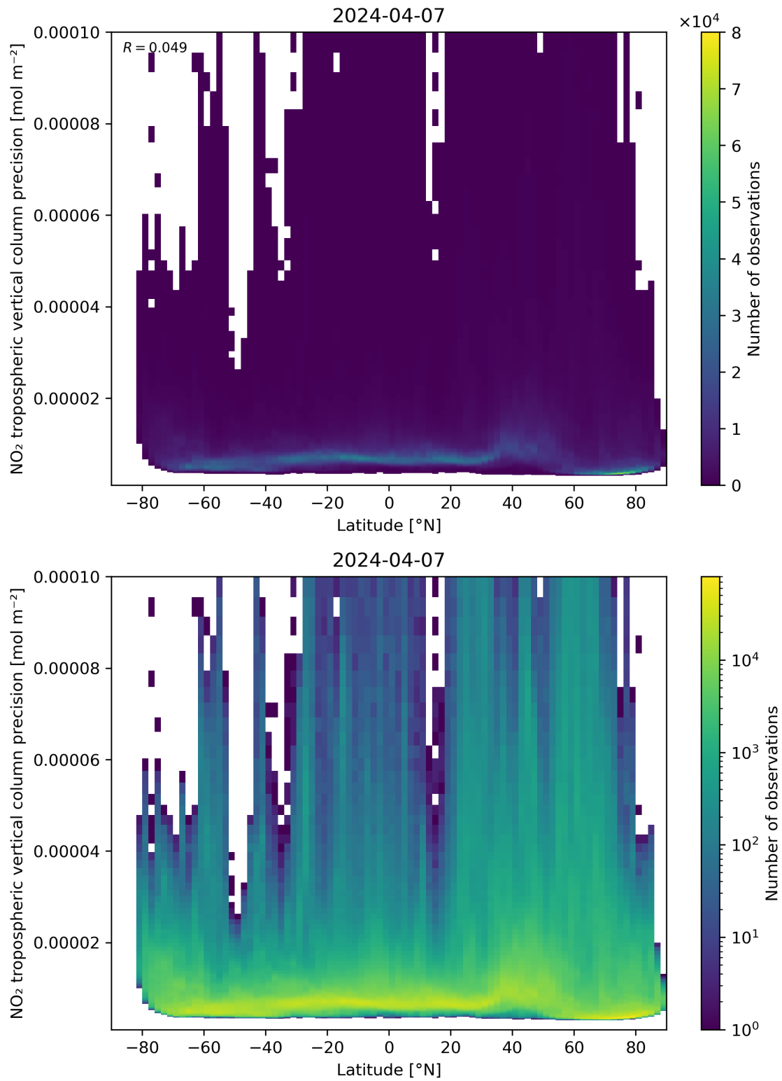
Figure 93: Scatter density plot of “Latitude” against “NO 2 tropospheric vertical column precision” for 2024-04-06 to 2024-04-08.
