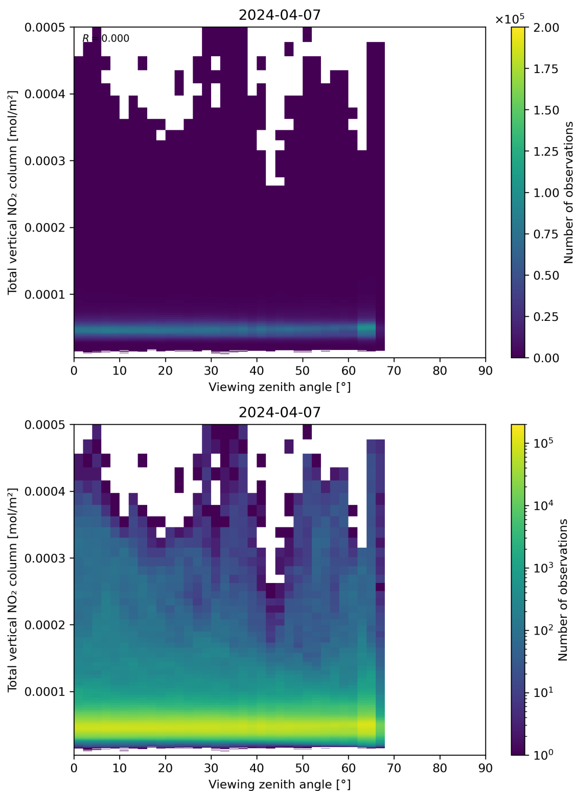
Figure 167: Scatter density plot of “Viewing zenith angle” against “Total vertical NO 2 column” for 2024-04-06 to 2024-04-08.
