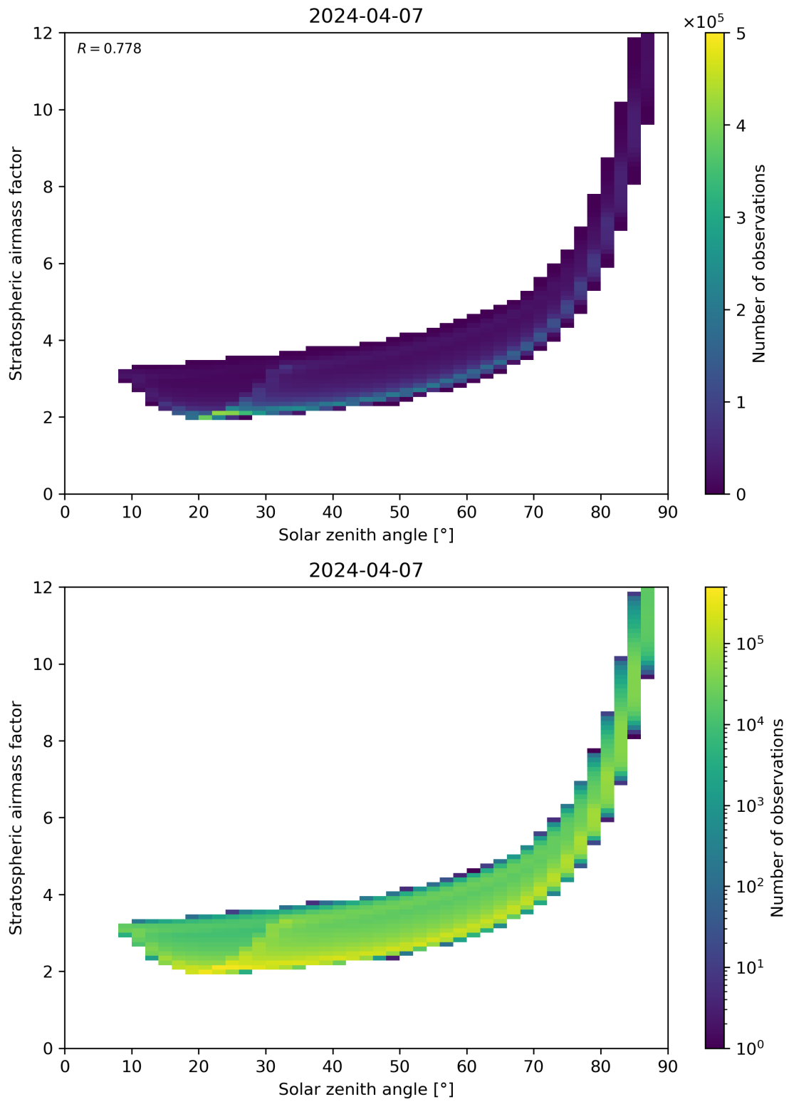
Figure 145: Scatter density plot of “Solar zenith angle” against “Stratospheric airmass factor” for 2024-04-06 to 2024-04-08.
