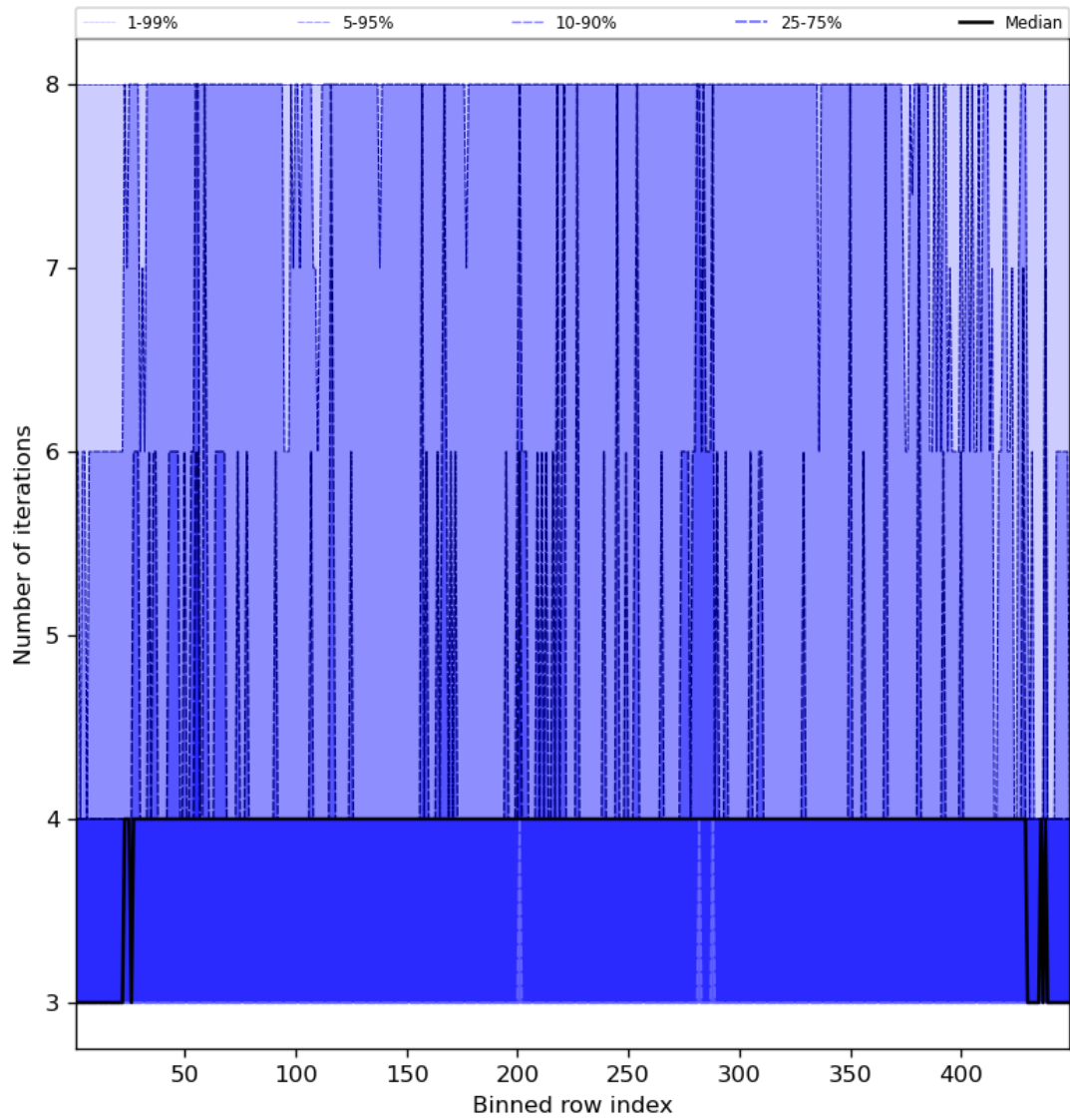
Figure 51: Along track statistics of “Number of iterations” for 2024-04-06 to 2024-04-08
