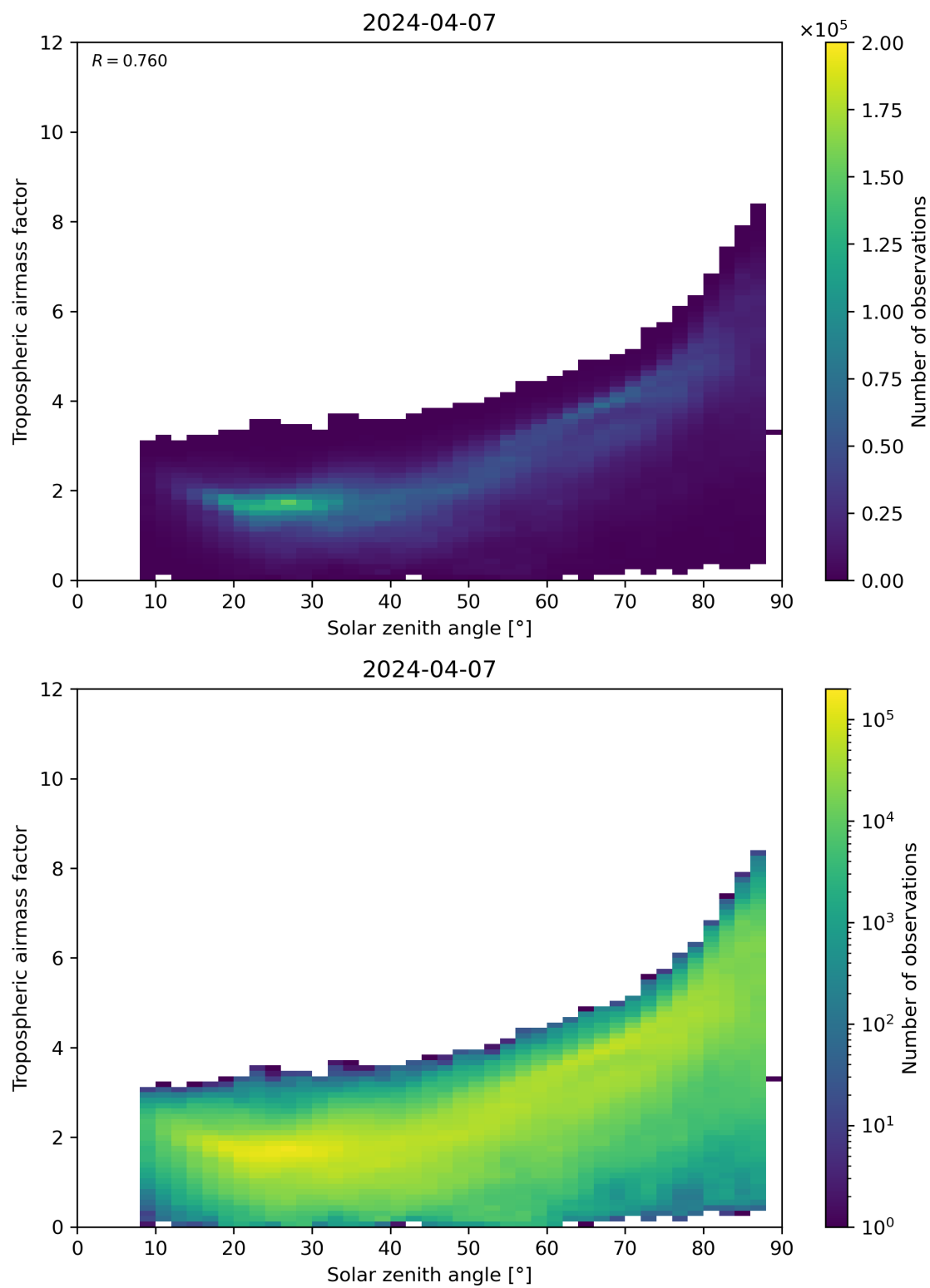
Figure 147: Scatter density plot of “Solar zenith angle” against “Tropospheric airmass factor” for 2024-04-06 to 2024-04-08.
