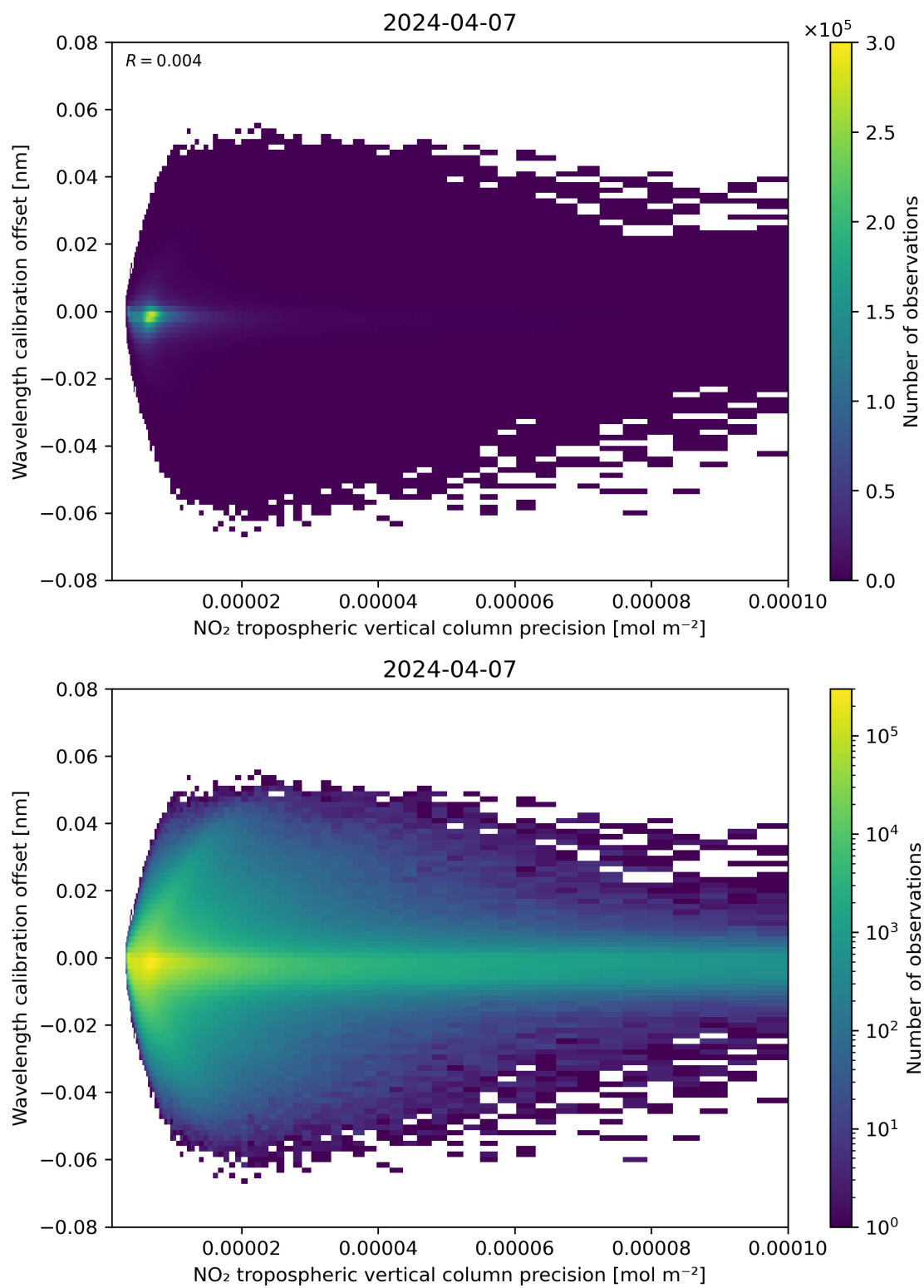
Figure 141: Scatter density plot of “NO 2 tropospheric vertical column precision” against “Wavelength calibration offset” for 2024-04-06 to 2024-04-08.
