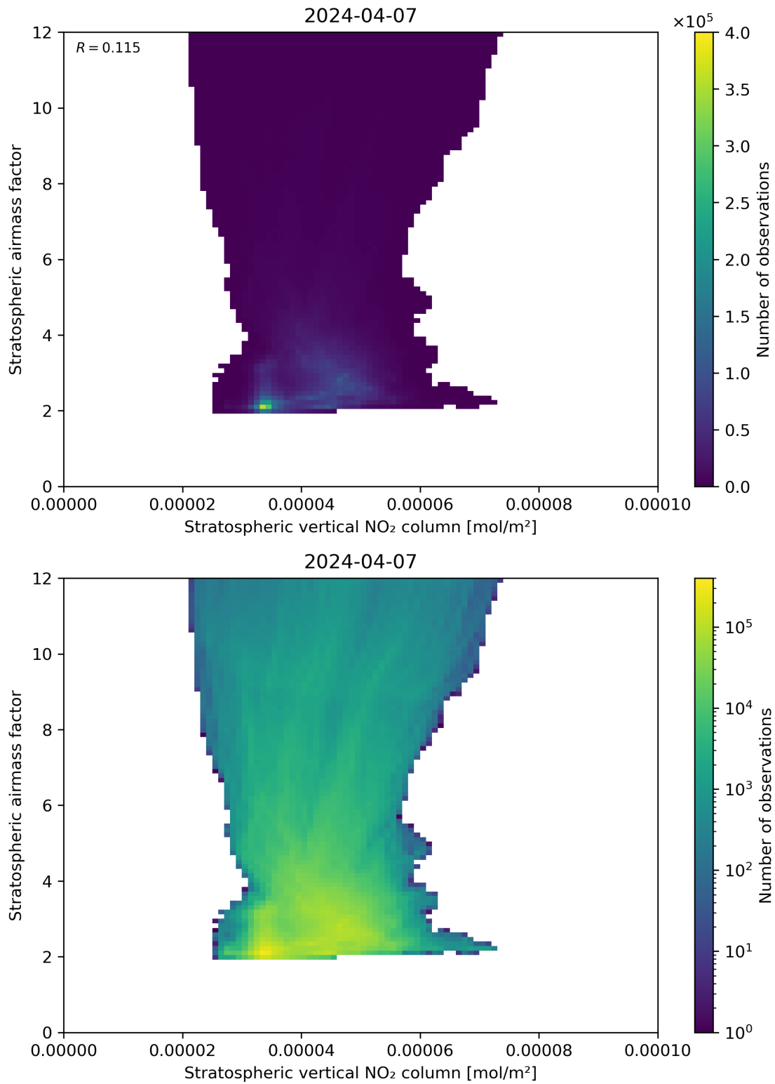
Figure 96: Scatter density plot of “Stratospheric vertical NO 2 column” against “Stratospheric airmass factor” for 2024-04-06 to 2024-04-08.
