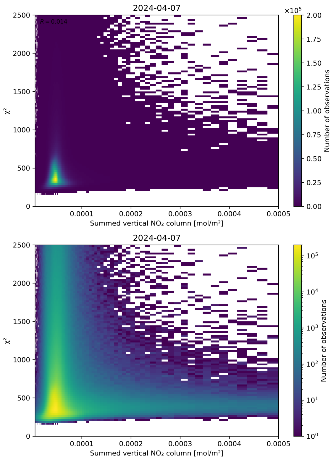
Figure 104: Scatter density plot of “Summed vertical NO 2 column” against “ \chi^2 ” for 2024-04-06 to 2024-04-08.
