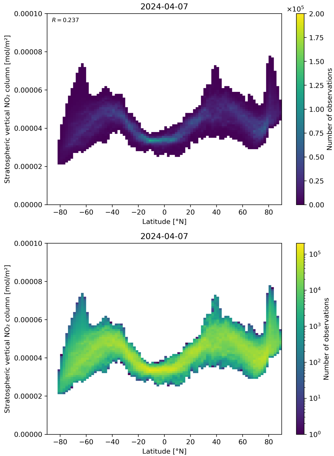
Figure 87: Scatter density plot of “Latitude” against “Stratospheric vertical NO 2 column” for 2024-04-06 to 2024-04-08.
