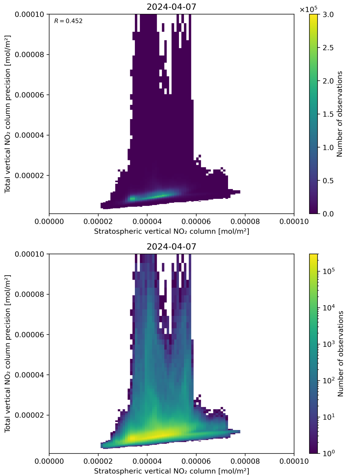
Figure 101: Scatter density plot of “Stratospheric vertical NO 2 column” against “Total vertical NO 2 column precision” for 2024-04-06 to 2024-04-08.
