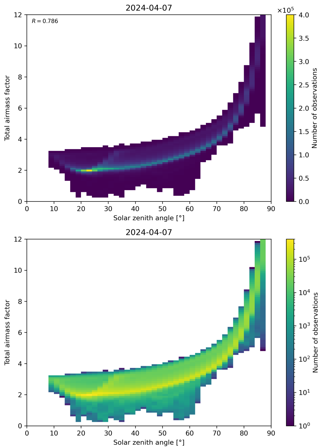
Figure 146: Scatter density plot of “Solar zenith angle” against “Total airmass factor” for 2024-04-06 to 2024-04-08.
