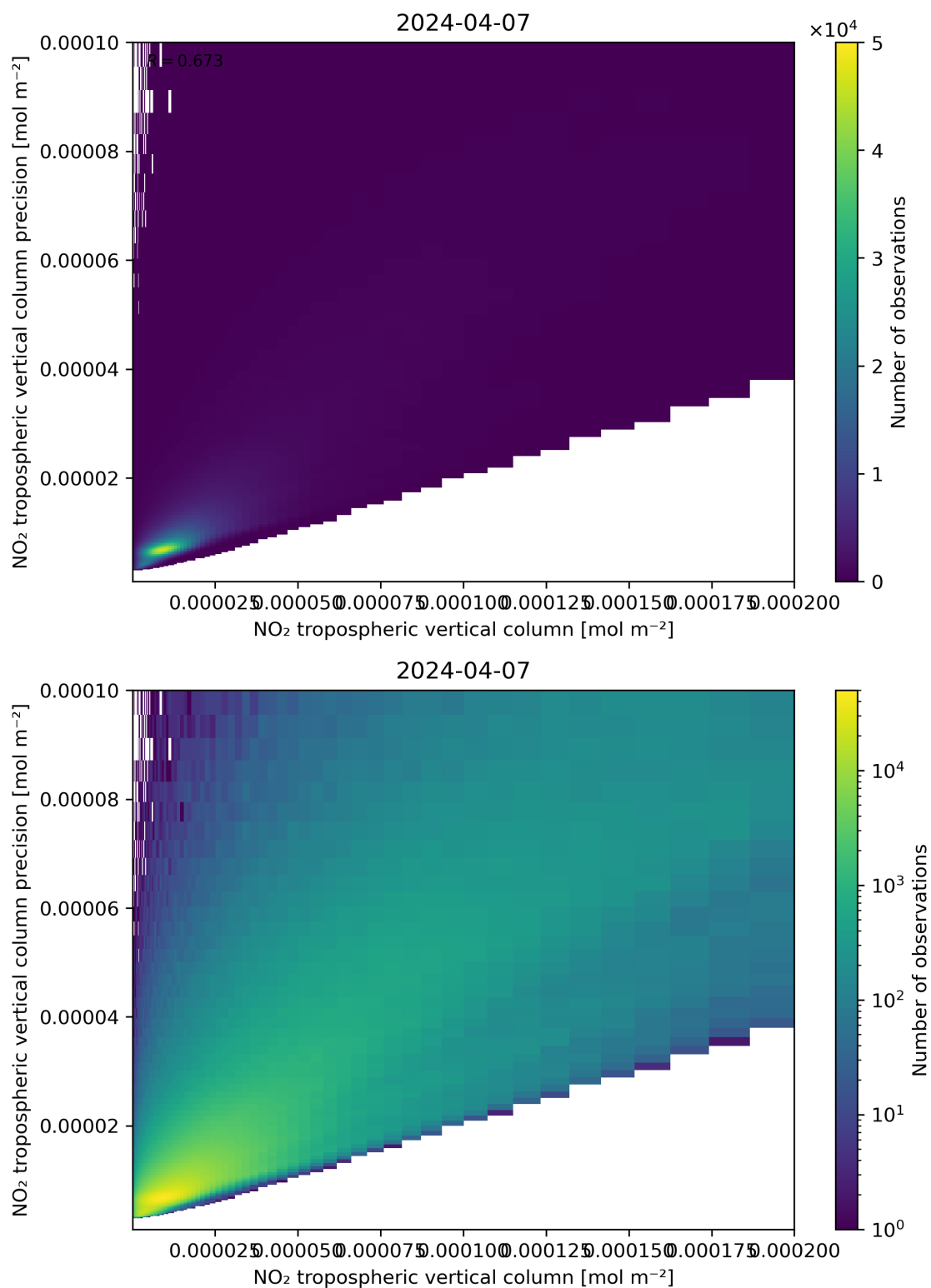
Figure 130: Scatter density plot of “NO 2 tropospheric vertical column” against “NO 2 tropospheric vertical column precision” for 2024-04-06 to 2024-04-08.
