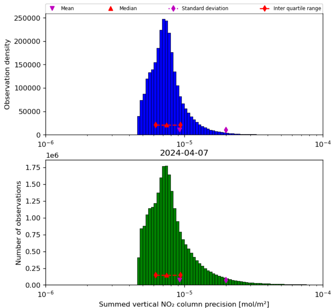
Figure 41: Histogram of “Summed vertical NO 2 column precision” for 2024-04-06 to 2024-04-08
