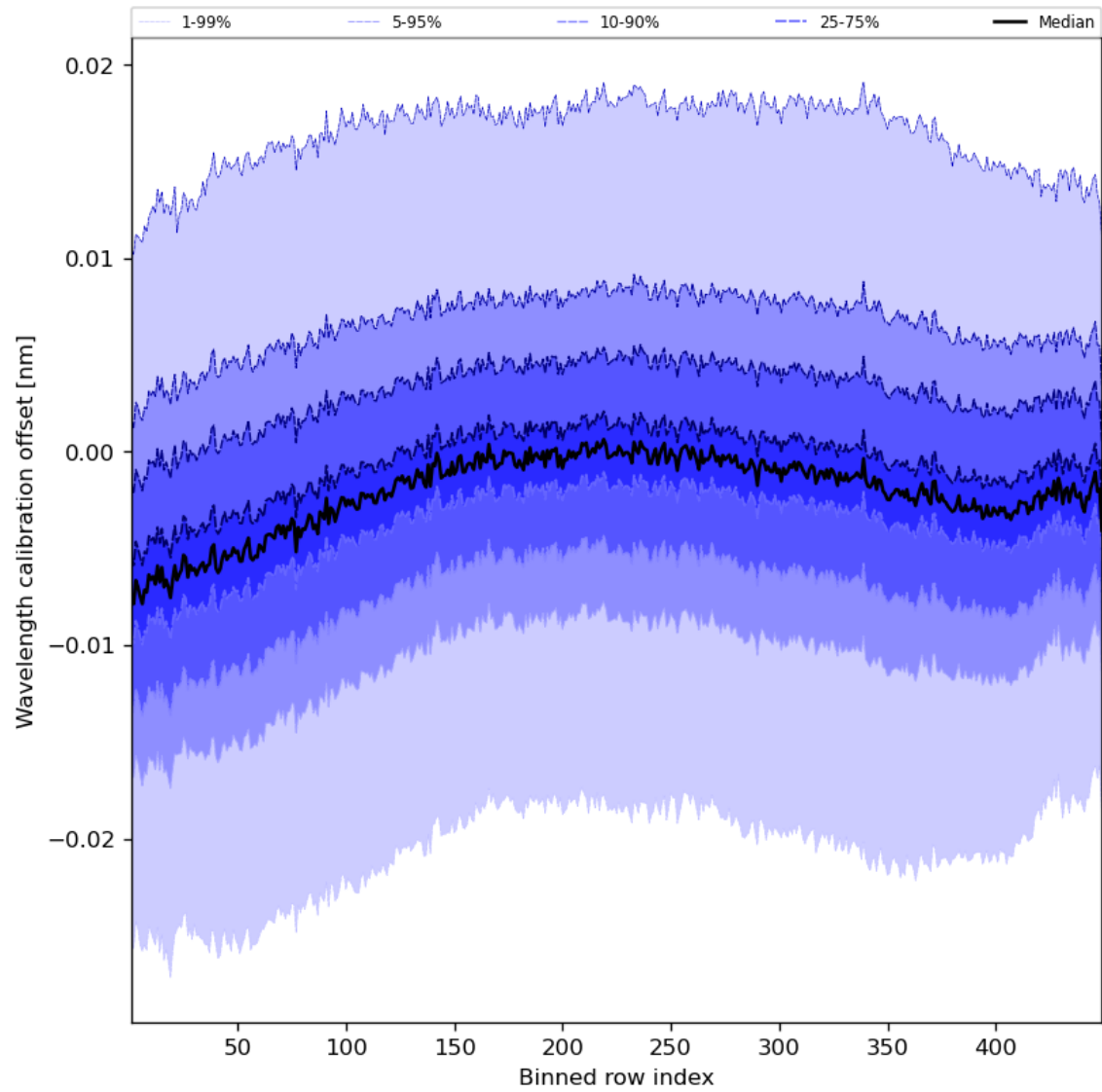
Figure 52: Along track statistics of “Wavelength calibration offset” for 2024-04-06 to 2024-04-08
