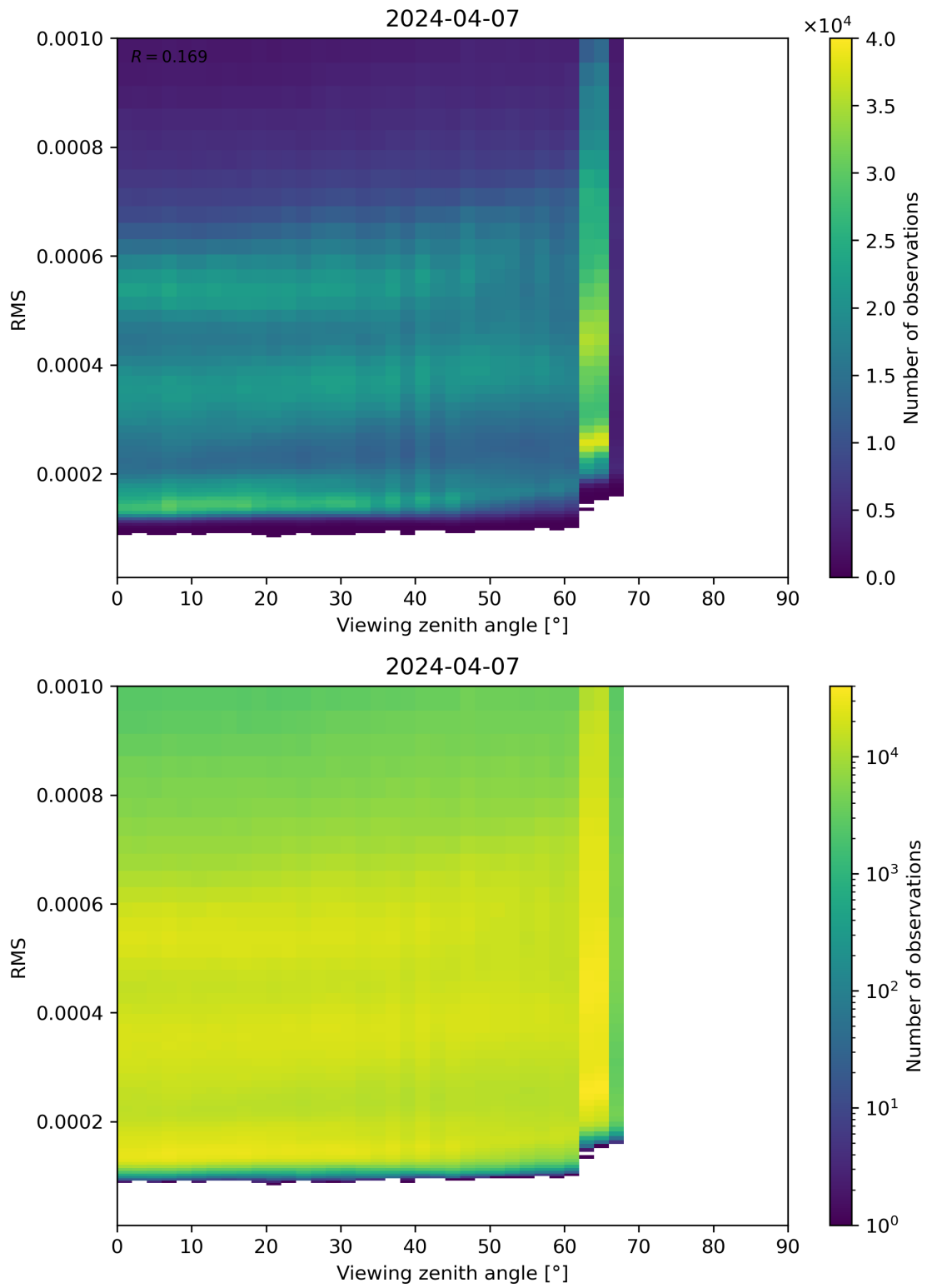
Figure 171: Scatter density plot of “Viewing zenith angle” against “RMS” for 2024-04-06 to 2024-04-08.
