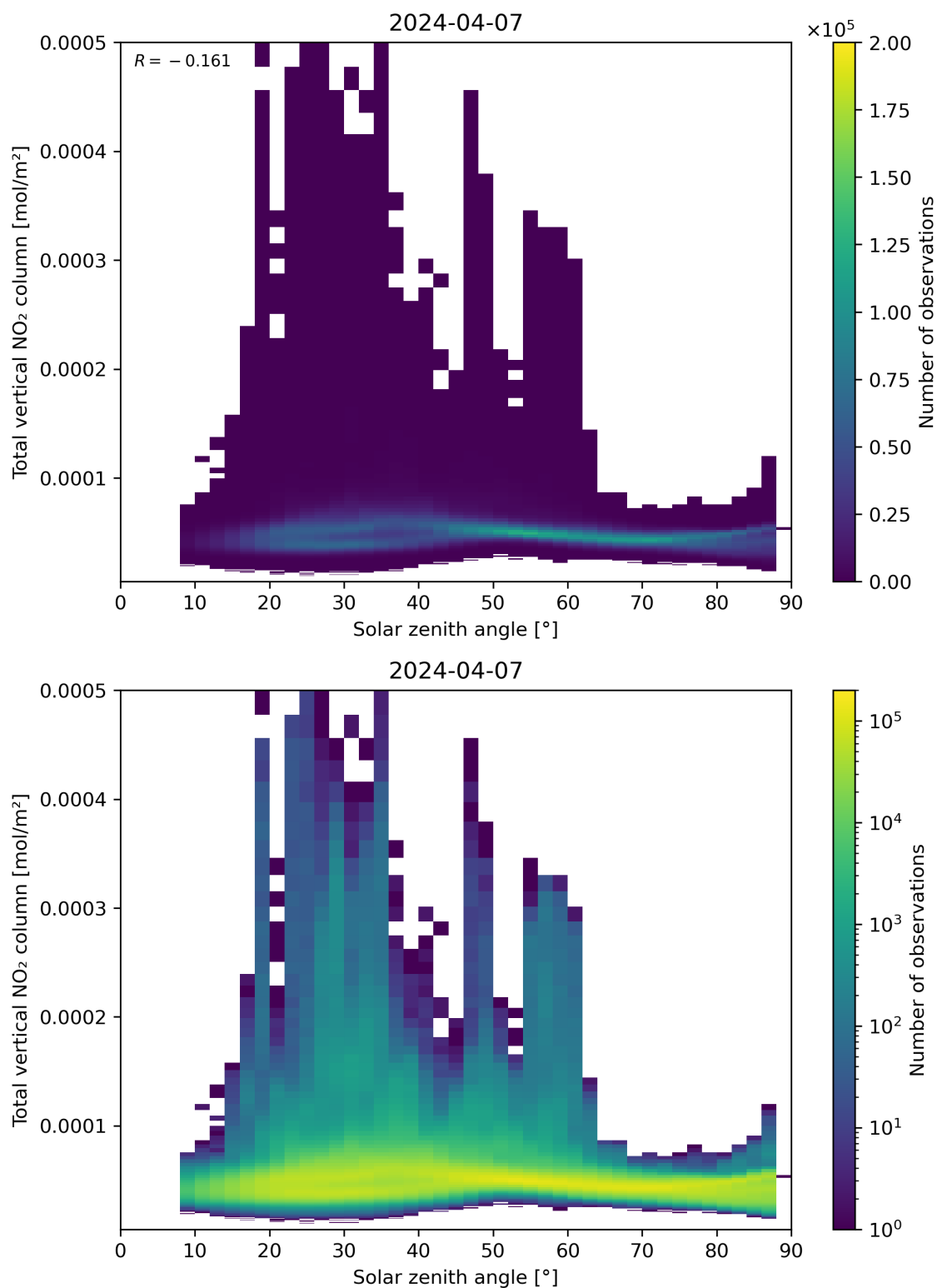
Figure 153: Scatter density plot of “Solar zenith angle” against “Total vertical NO 2 column” for 2024-04-06 to 2024-04-08.
