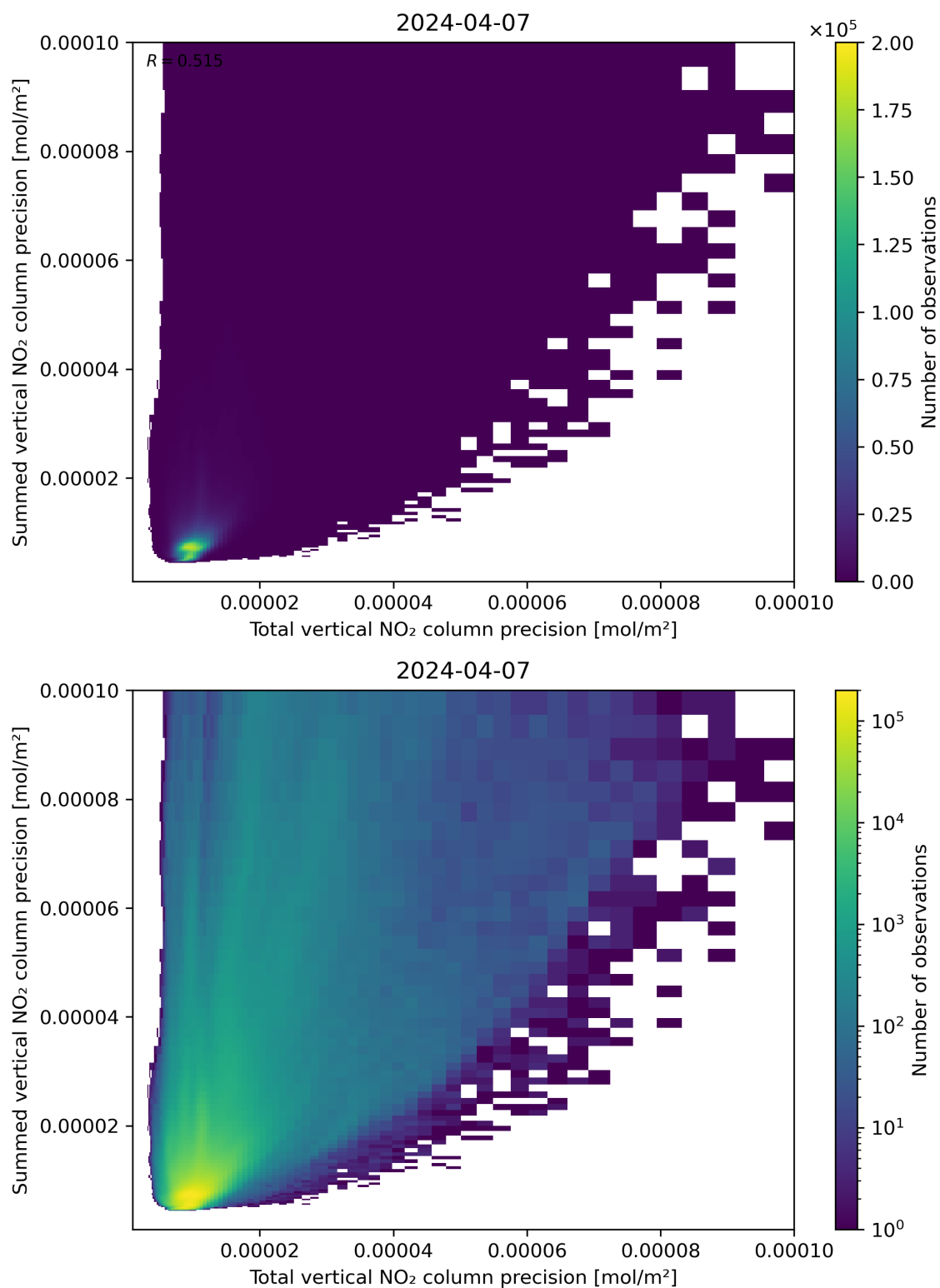
Figure 118: Scatter density plot of “Total vertical NO 2 column precision” against “Summed vertical NO 2 column precision” for 2024-04-06 to 2024-04-08.
