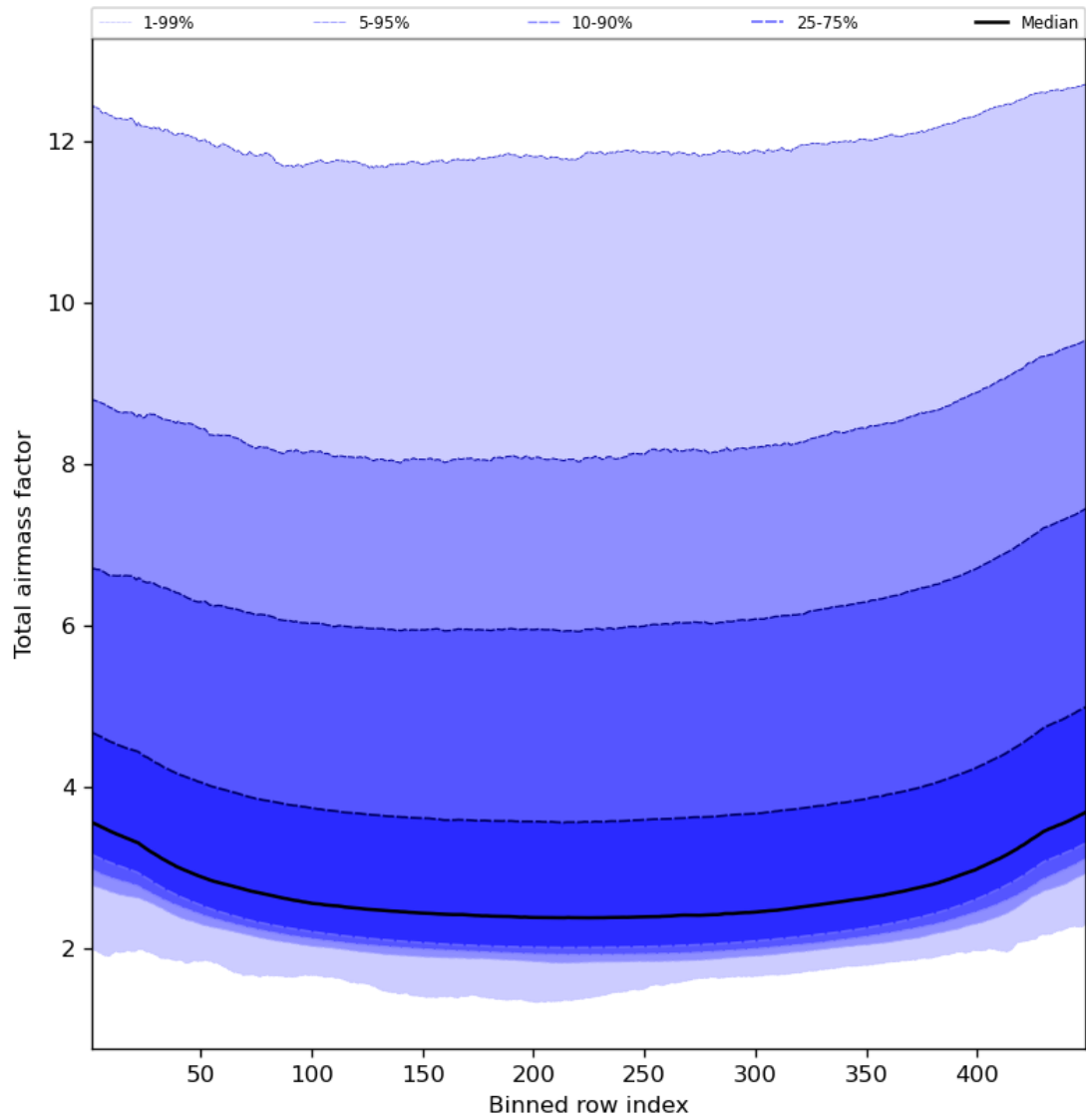
Figure 49: Along track statistics of “Total airmass factor” for 2024-04-06 to 2024-04-08
