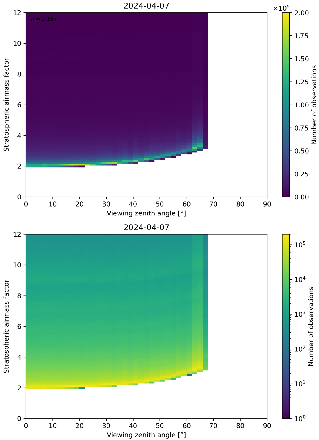
Figure 159: Scatter density plot of “Viewing zenith angle” against “Stratospheric airmass factor” for 2024-04-06 to 2024-04-08.
