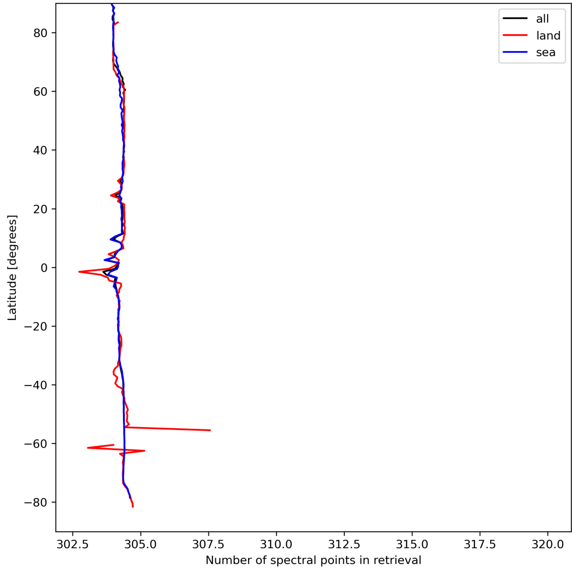
Figure 16: Zonal average of “Number of spectral points in retrieval” for 2024-04-06 to 2024-04-08.
