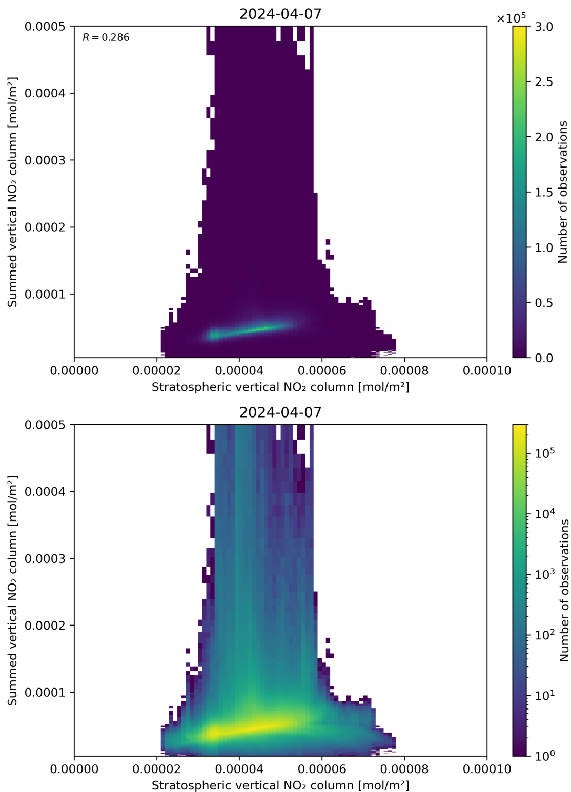
Figure 98: Scatter density plot of “Stratospheric vertical NO 2 column” against “Summed vertical NO 2 column” for 2024-04-06 to 2024-04-08.
