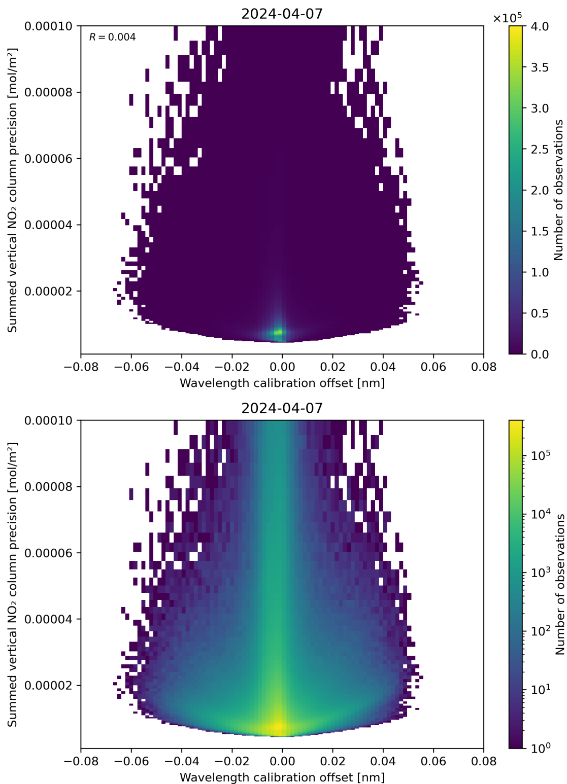
Figure 178: Scatter density plot of “Wavelength calibration offset” against “Summed vertical NO 2 column precision” for 2024-04-06 to 2024-04-08.
