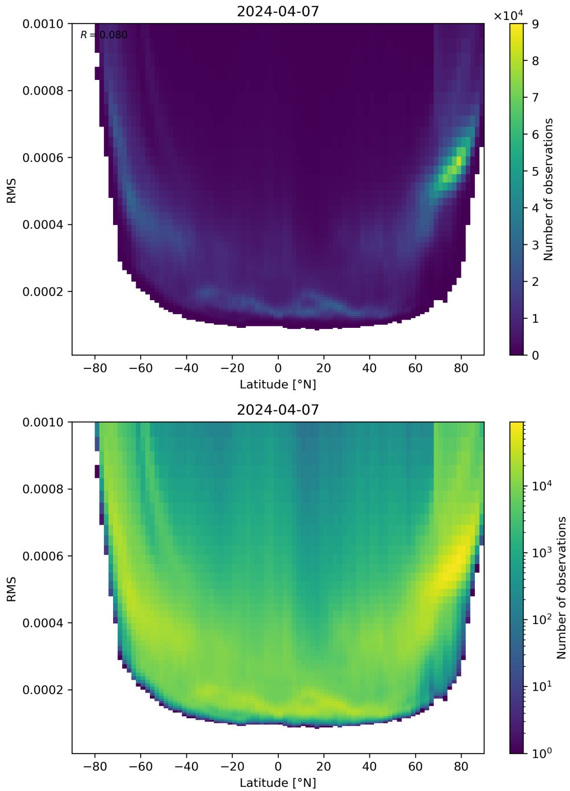
Figure 94: Scatter density plot of “Latitude” against “RMS” for 2024-04-06 to 2024-04-08.
