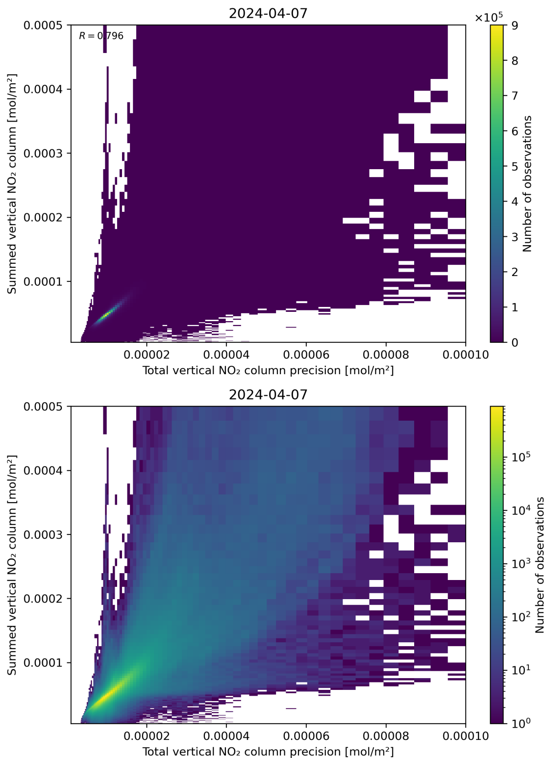
Figure 117: Scatter density plot of “Total vertical NO 2 column precision” against “Summed vertical NO 2 column” for 2024-04-06 to 2024-04-08.
