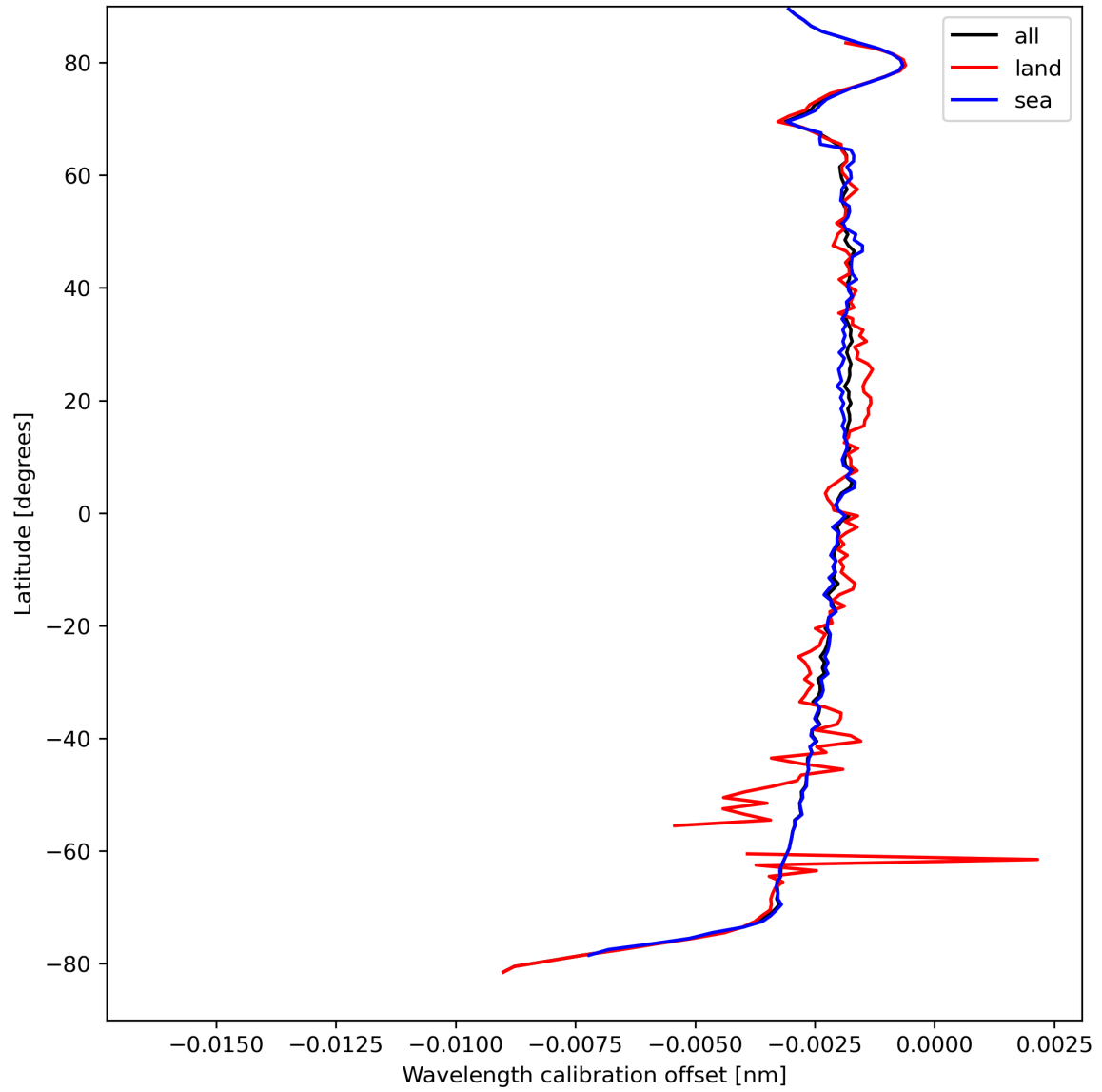
Figure 18: Zonal average of “Wavelength calibration offset” for 2024-04-06 to 2024-04-08.
