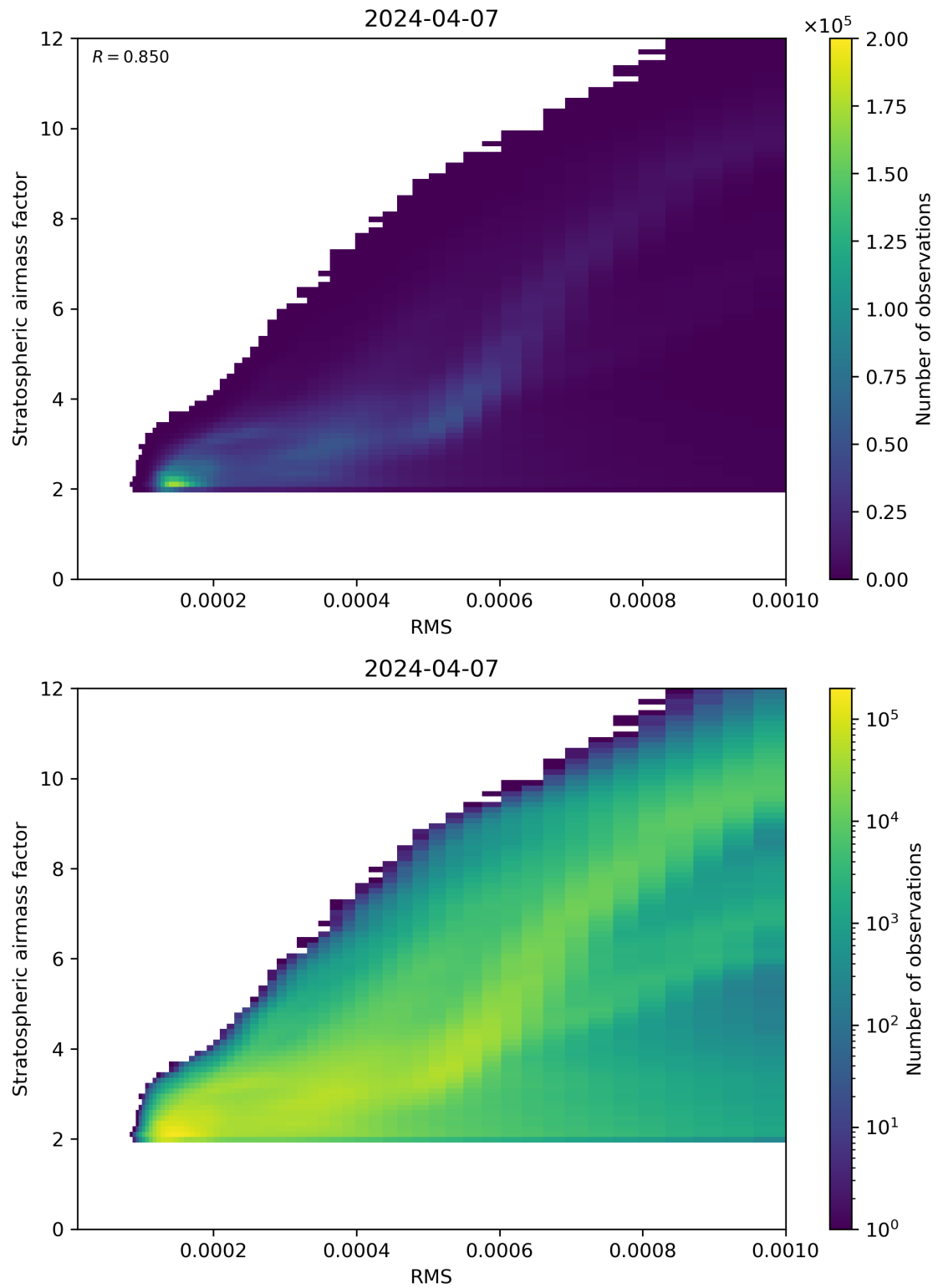
Figure 144: Scatter density plot of “RMS” against “Stratospheric airmass factor” for 2024-04-06 to 2024-04-08.
