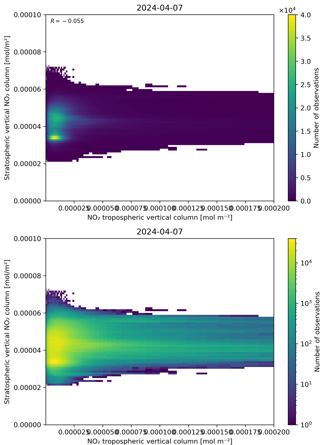
Figure 125: Scatter density plot of “NO 2 tropospheric vertical column” against “Stratospheric vertical NO 2 column” for 2024-04-06 to 2024-04-08.
