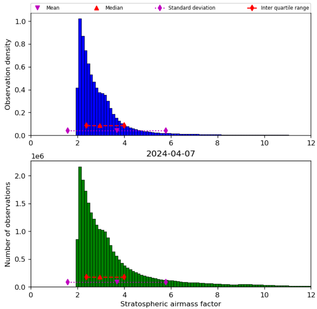
Figure 44: Histogram of “Stratospheric airmass factor” for 2024-04-06 to 2024-04-08
