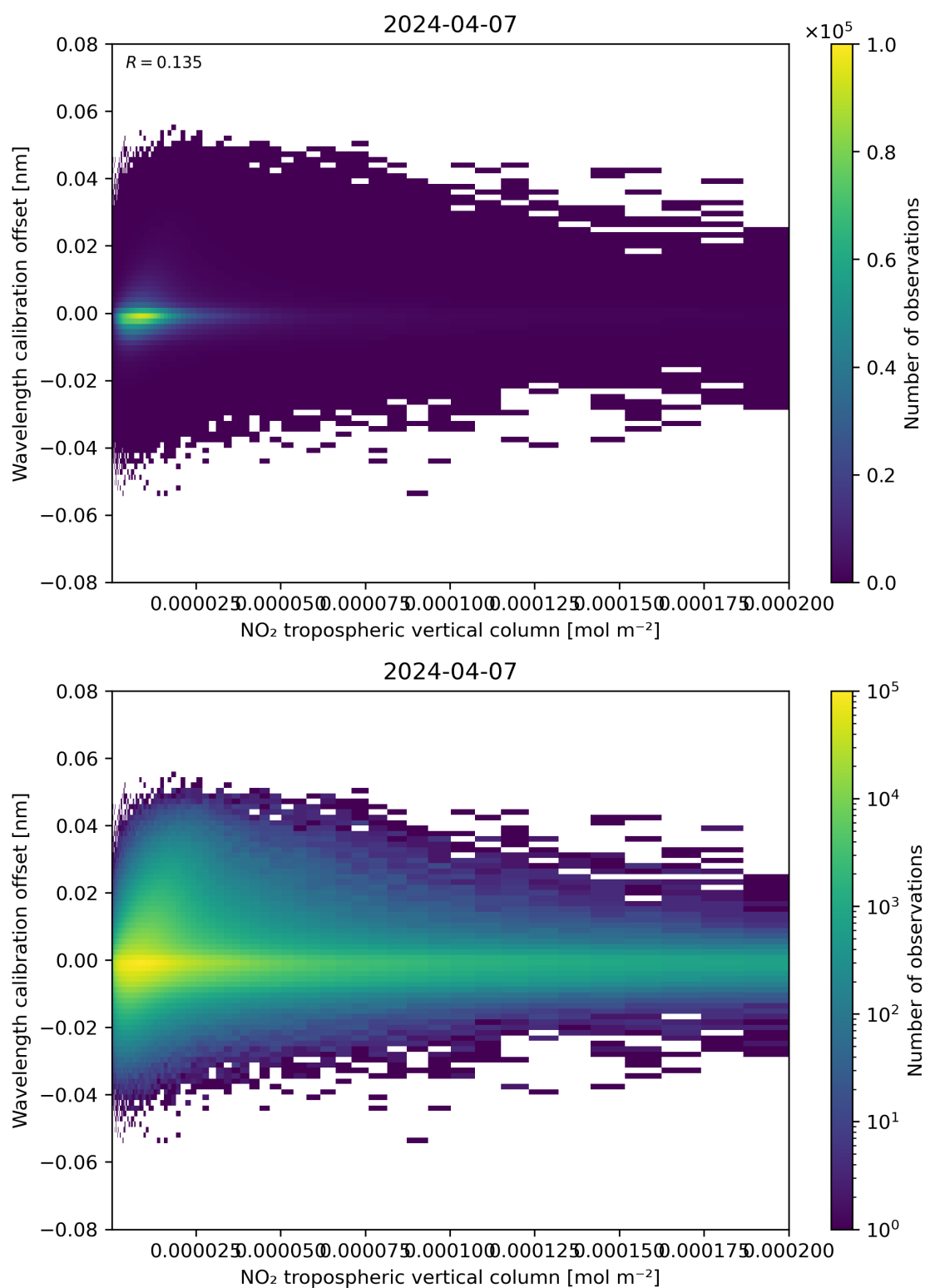
Figure 143: Scatter density plot of “NO 2 tropospheric vertical column” against “Wavelength calibration offset” for 2024-04-06 to 2024-04-08.
