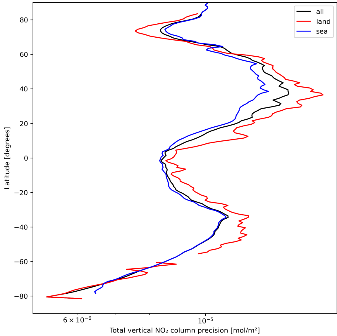
Figure 22: Zonal average of “Total vertical NO 2 column precision” for 2024-04-06 to 2024-04-08.
