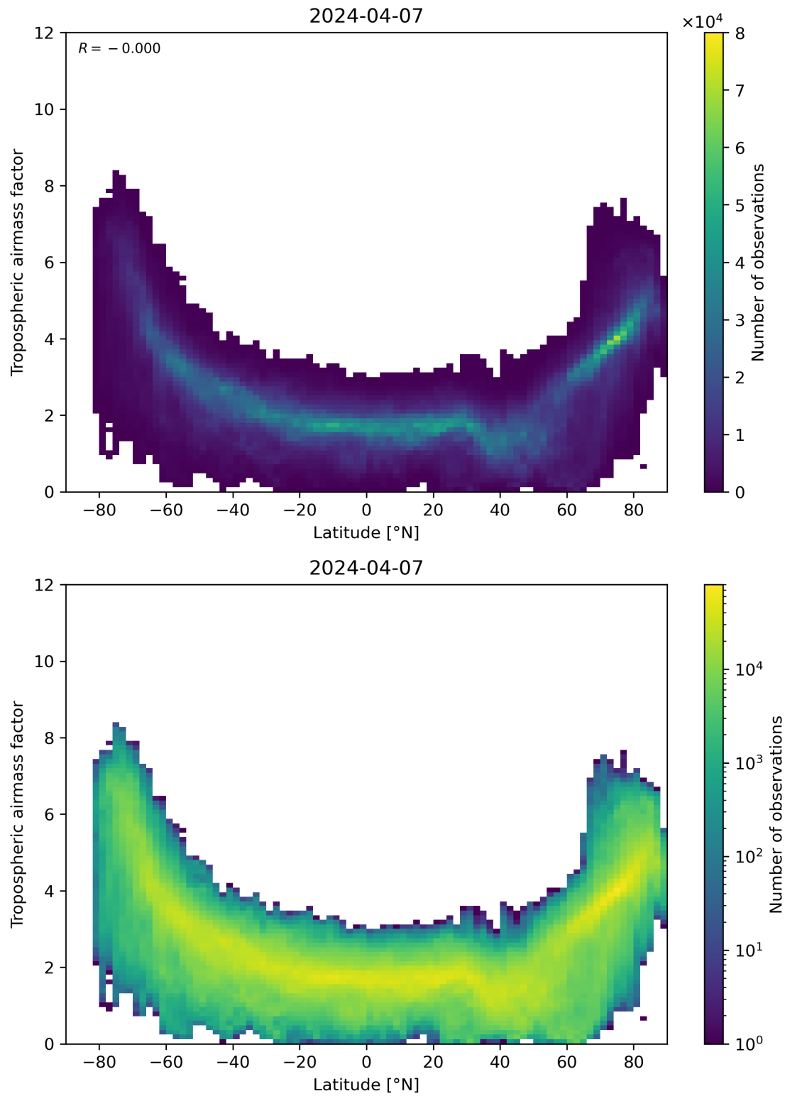
Figure 85: Scatter density plot of “Latitude” against “Tropospheric air mass factor” for 2024-04-06 to 2024-04-08.
