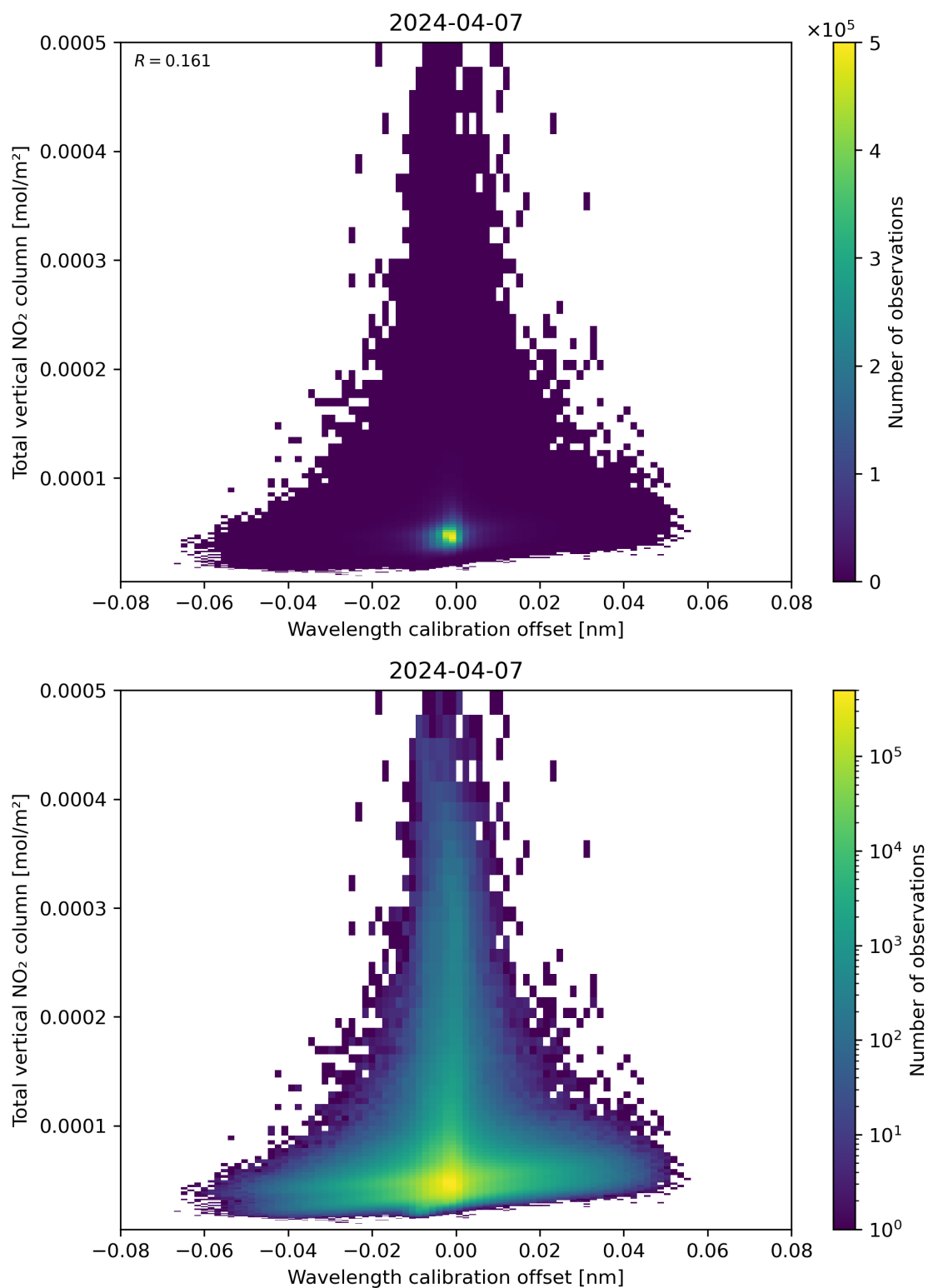
Figure 179: Scatter density plot of “Wavelength calibration offset” against “Total vertical NO 2 column” for 2024-04-06 to 2024-04-08.
