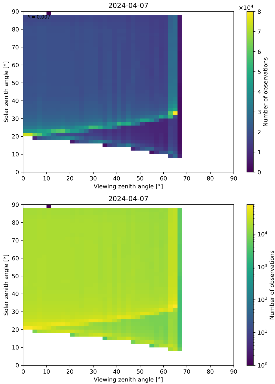
Figure 172: Scatter density plot of “Viewing zenith angle” against “Solar zenith angle” for 2024-04-06 to 2024-04-08.
