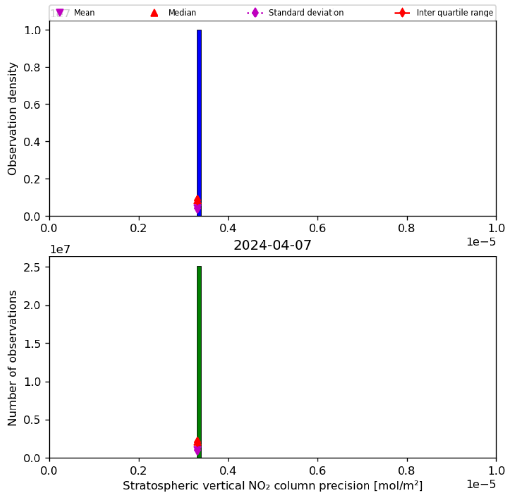
Figure 37: Histogram of “Stratospheric vertical NO 2 column precision” for 2024-04-06 to 2024-04-08
