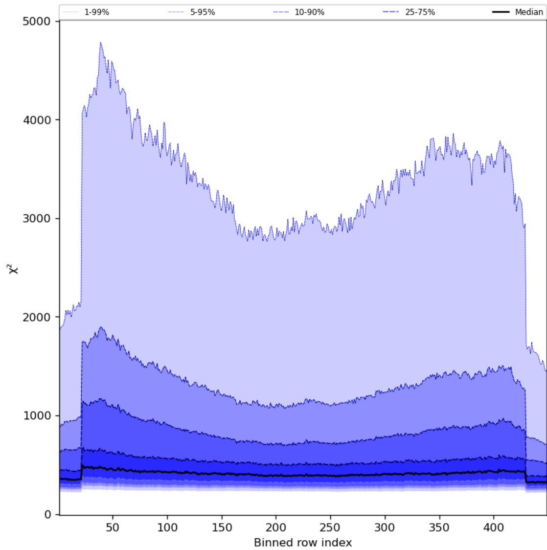
Figure 59: Along track statistics of “ \chi^2 ” for 2024-04-06 to 2024-04-08
