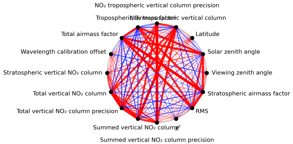
Figure 1: Map of correlation graph for 2024-04-06 to 2024-04-08.
