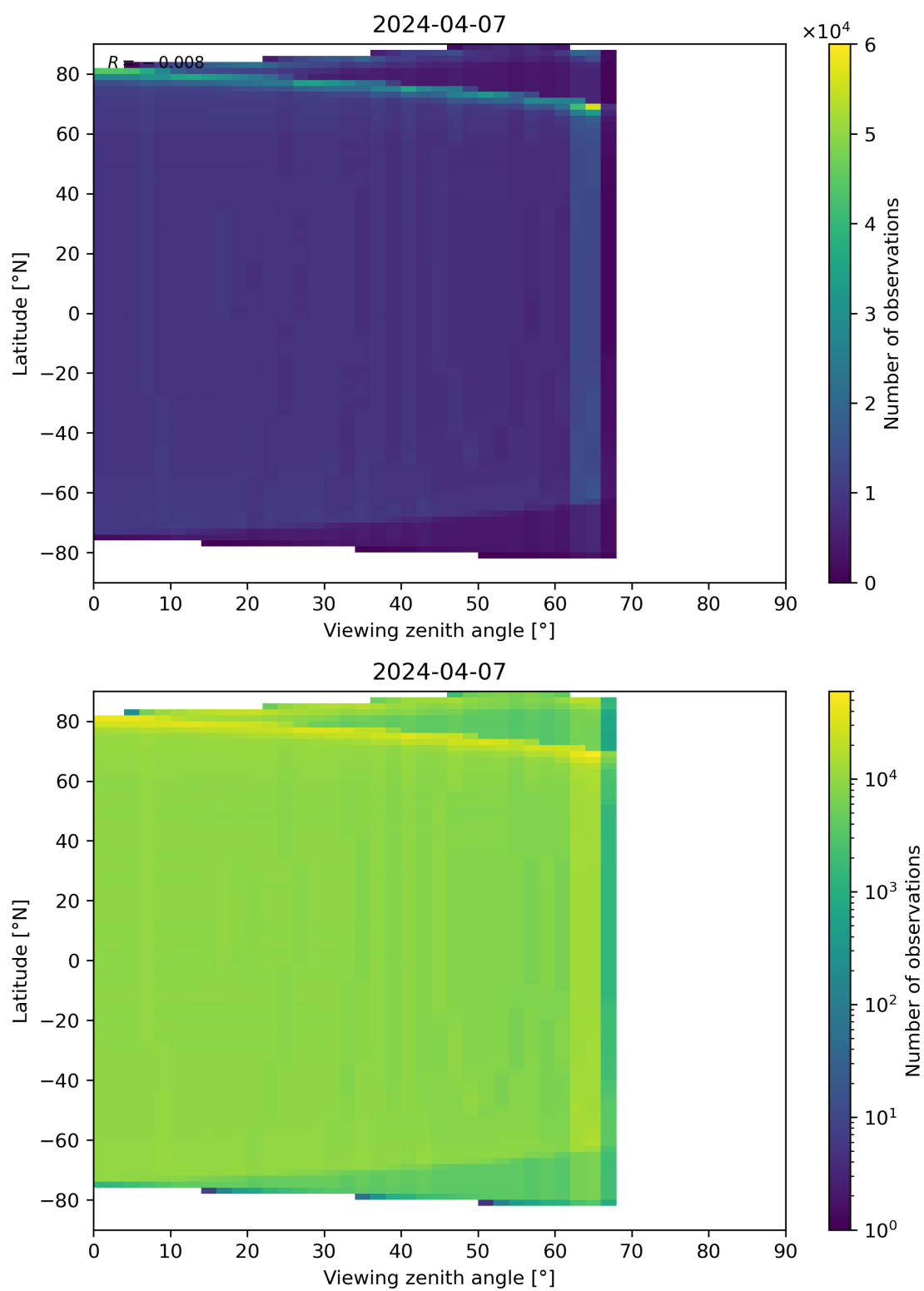
Figure 163: Scatter density plot of “Viewing zenith angle” against “Latitude” for 2024-04-06 to 2024-04-08.
