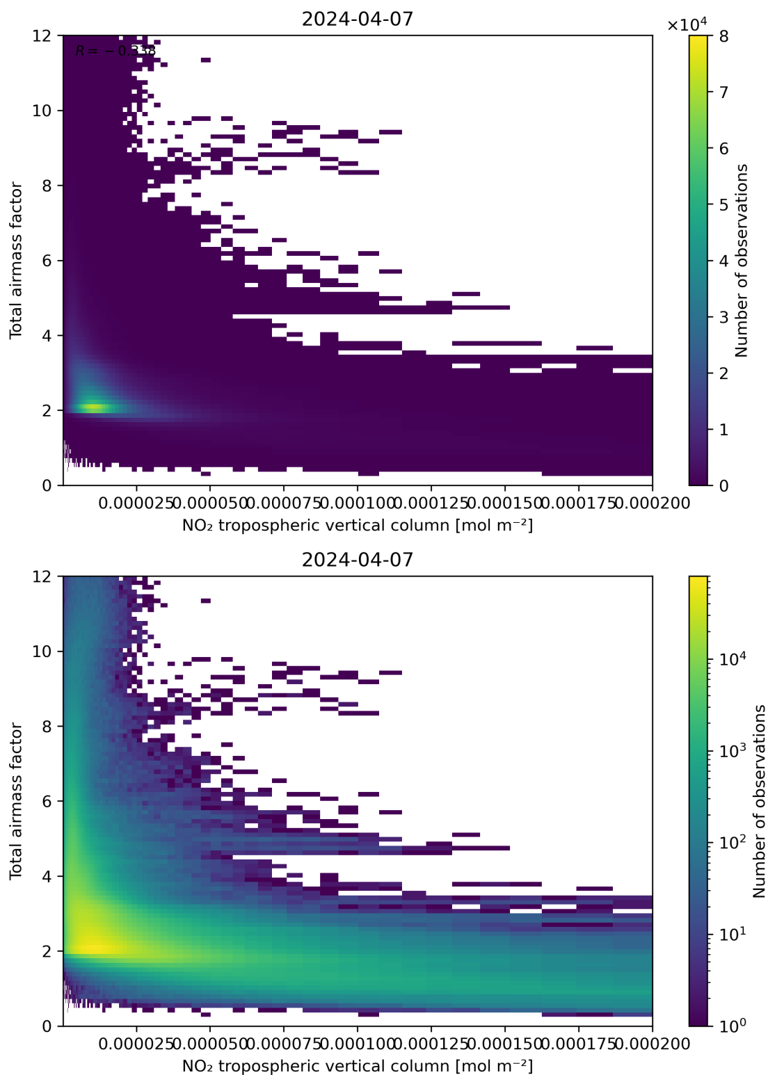
Figure 122: Scatter density plot of “NO 2 tropospheric vertical column” against “Total air mass factor” for 2024-04-06 to 2024-04-08.
