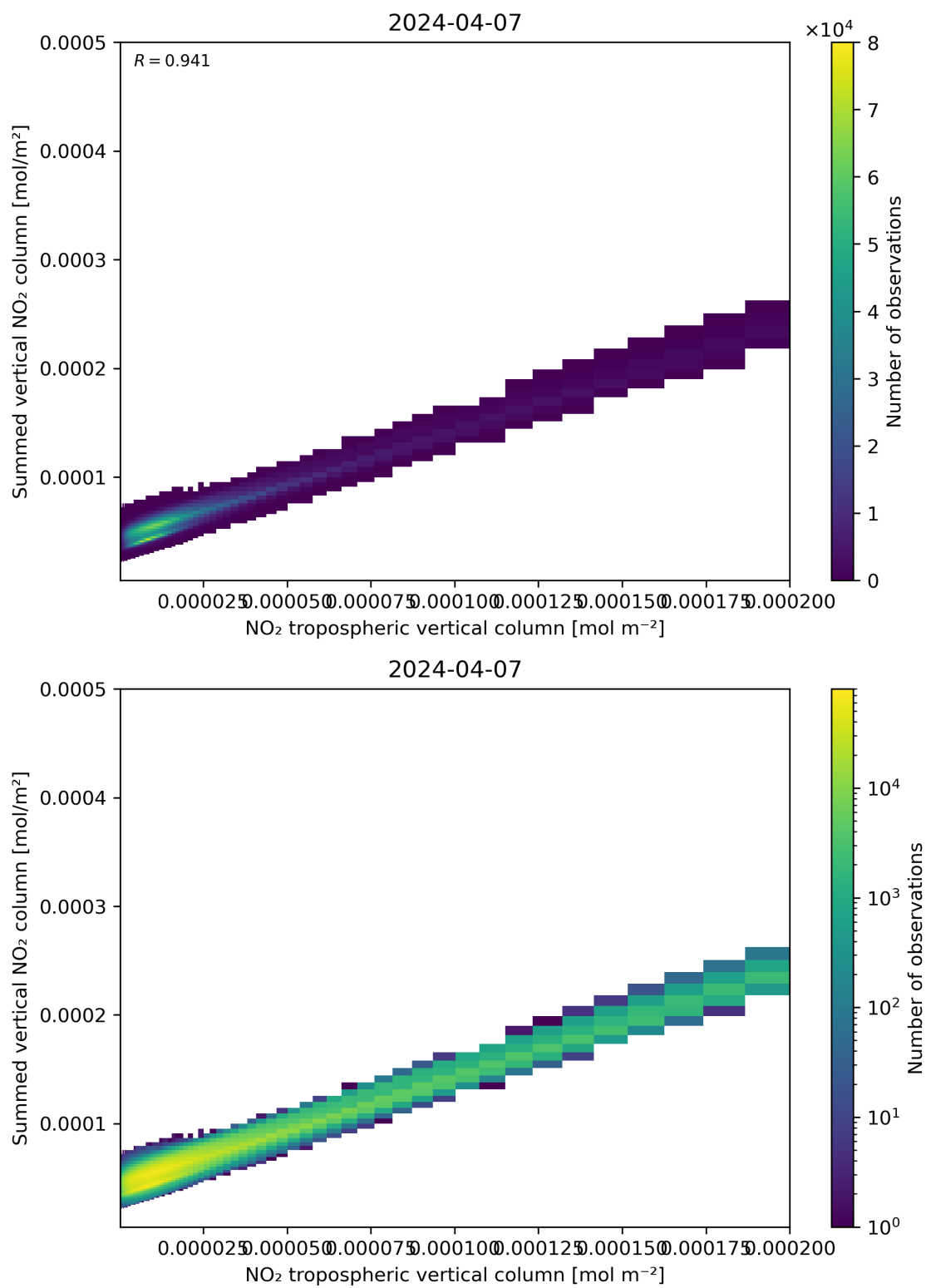
Figure 126: Scatter density plot of “NO 2 tropospheric vertical column” against “Summed vertical NO 2 column” for 2024-04-06 to 2024-04-08.
