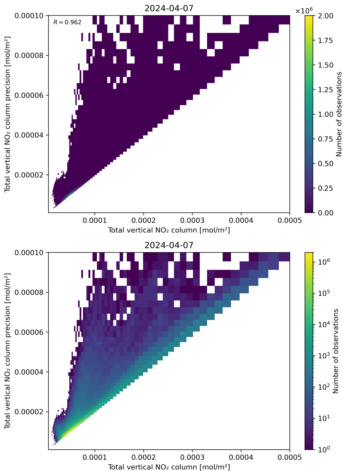
Figure 114: Scatter density plot of “Total vertical NO 2 column” against “Total vertical NO 2 column precision” for 2024-04-06 to 2024-04-08.
