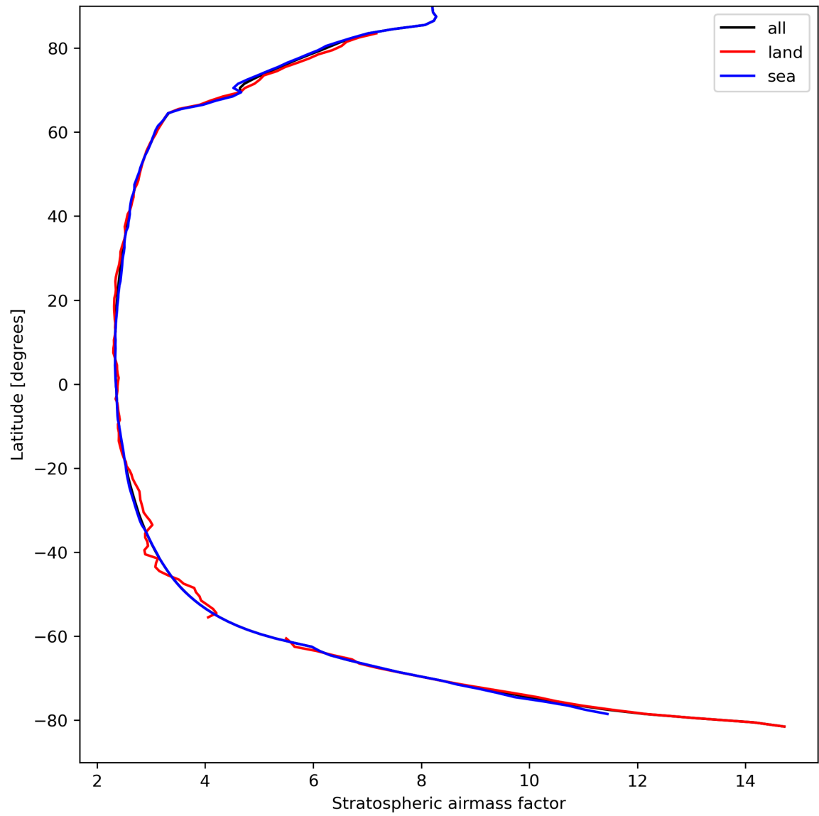
Figure 27: Zonal average of “Stratospheric air mass factor” for 2024-04-06 to 2024-04-08.
