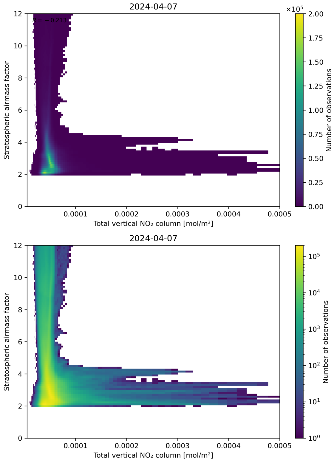
Figure 110: Scatter density plot of “Total vertical NO 2 column” against “Stratospheric airmass factor” for 2024-04-06 to 2024-04-08.
