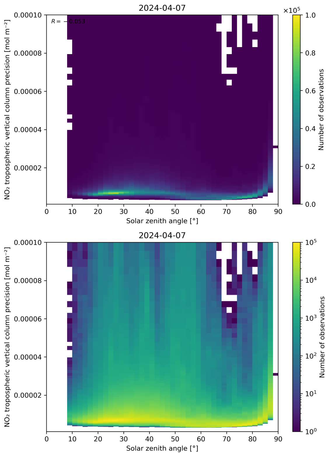
Figure 156: Scatter density plot of “Solar zenith angle” against “NO 2 tropospheric vertical column precision” for 2024-04-06 to 2024-04-08.
