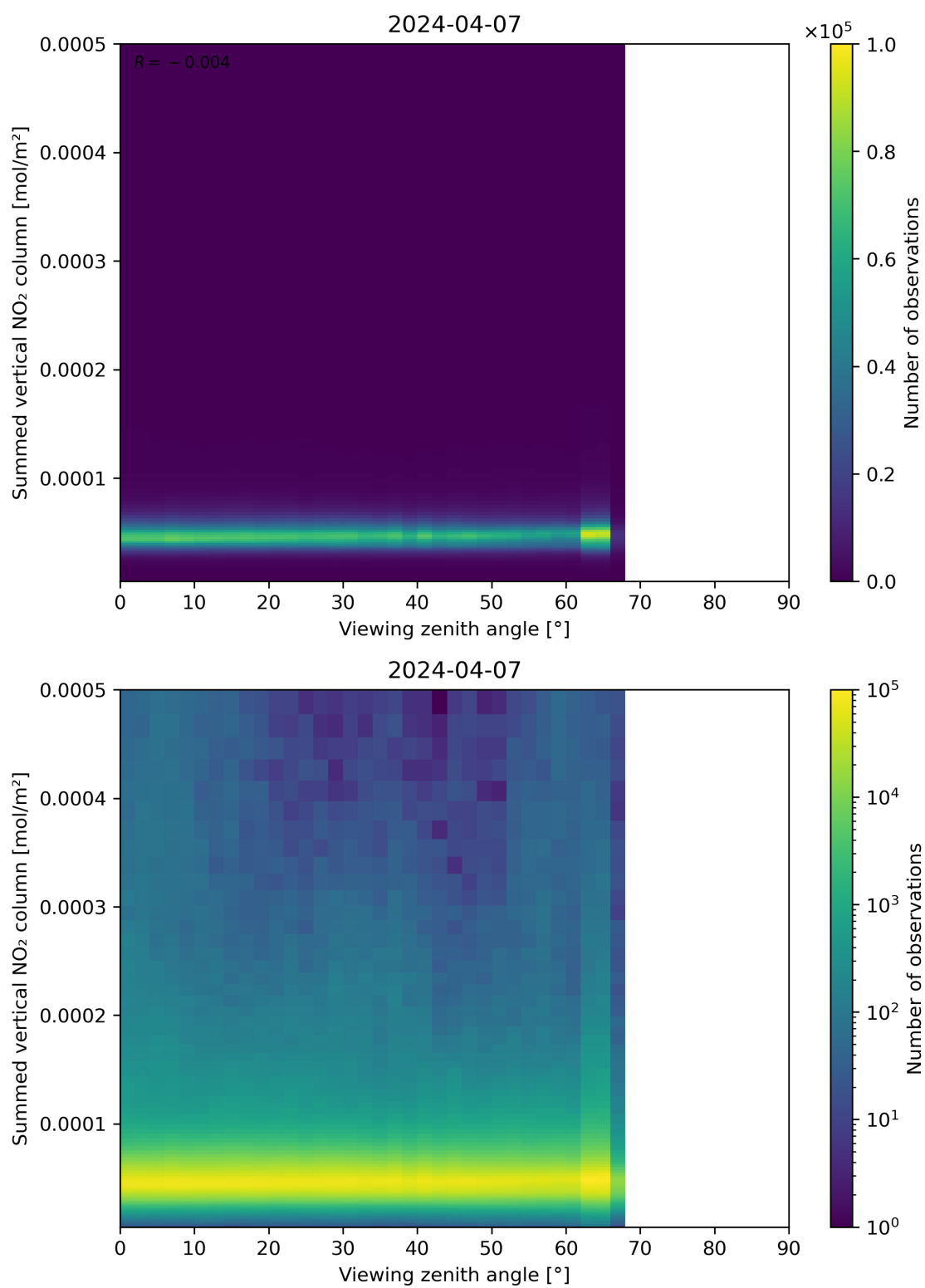
Figure 165: Scatter density plot of “Viewing zenith angle” against “Summed vertical NO 2 column” for 2024-04-06 to 2024-04-08.
