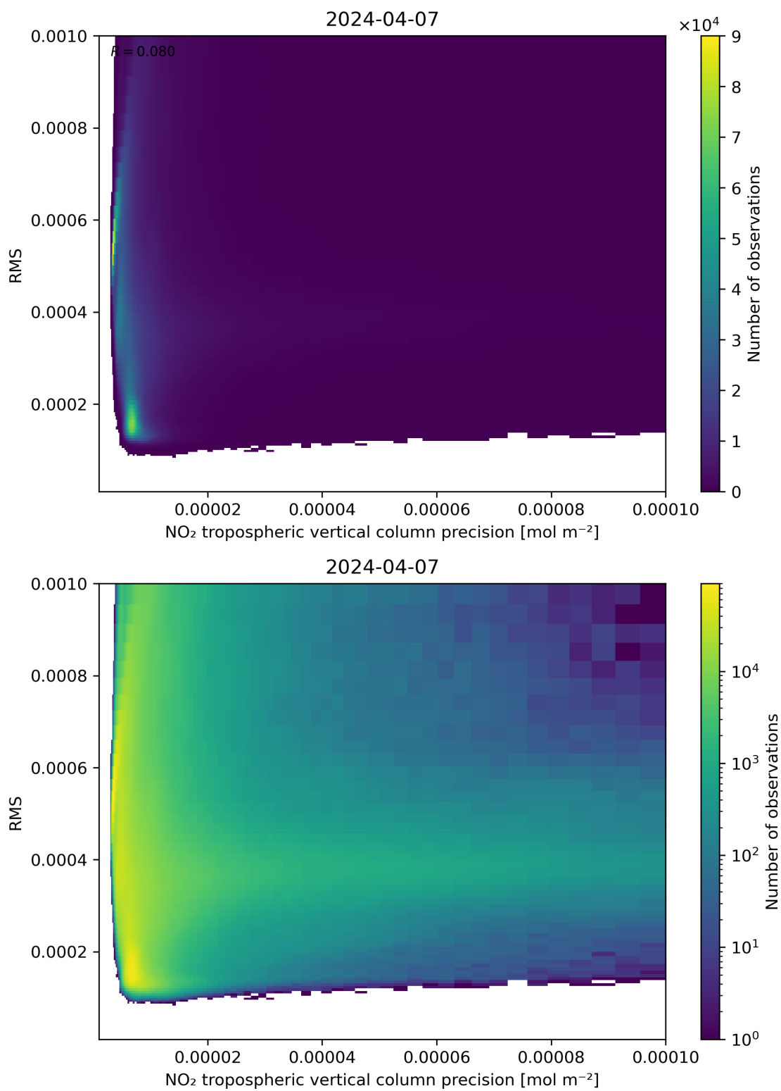
Figure 140: Scatter density plot of “NO 2 tropospheric vertical column precision” against “RMS” for 2024-04-06 to 2024-04-08.
