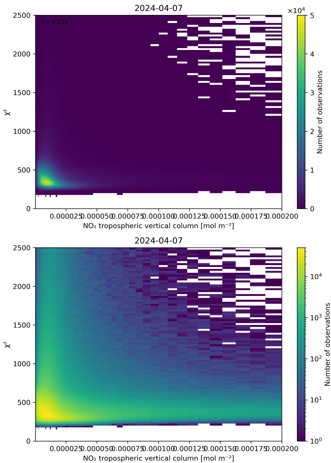
Figure 124: Scatter density plot of “NO 2 tropospheric vertical column” against “ \chi^2 ” for 2024-04-06 to 2024-04-08.
