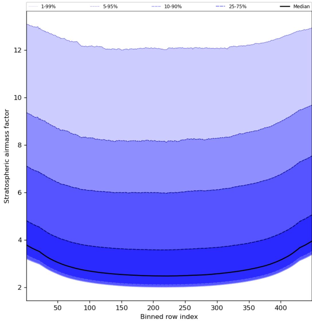
Figure 61: Along track statistics of “Stratospheric airmass factor” for 2024-04-06 to 2024-04-08
