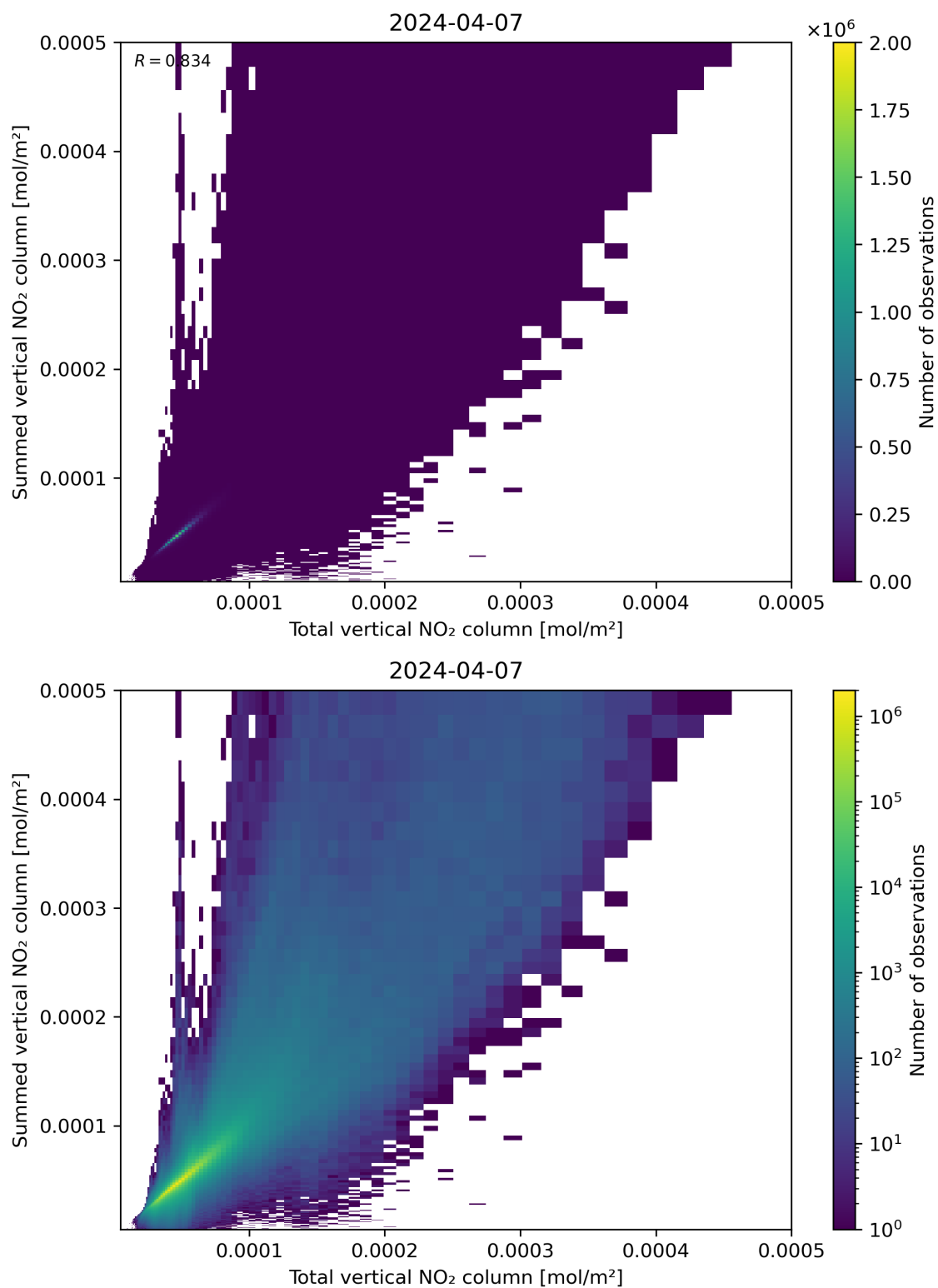
Figure 112: Scatter density plot of “Total vertical NO 2 column” against “Summed vertical NO 2 column” for 2024-04-06 to 2024-04-08.
