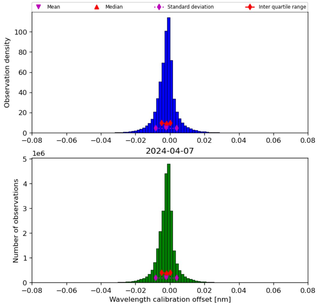
Figure 35: Histogram of “Wavelength calibration offset” for 2024-04-06 to 2024-04-08
