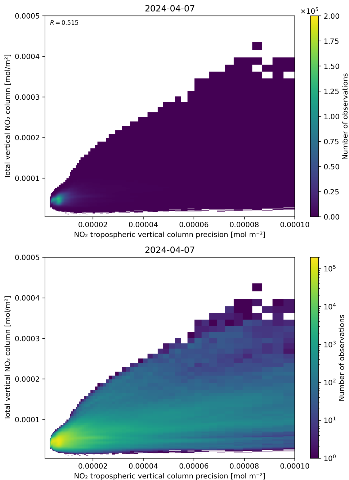
Figure 138: Scatter density plot of “NO 2 tropospheric vertical column precision” against “Total vertical NO 2 column” for 2024-04-06 to 2024-04-08.
