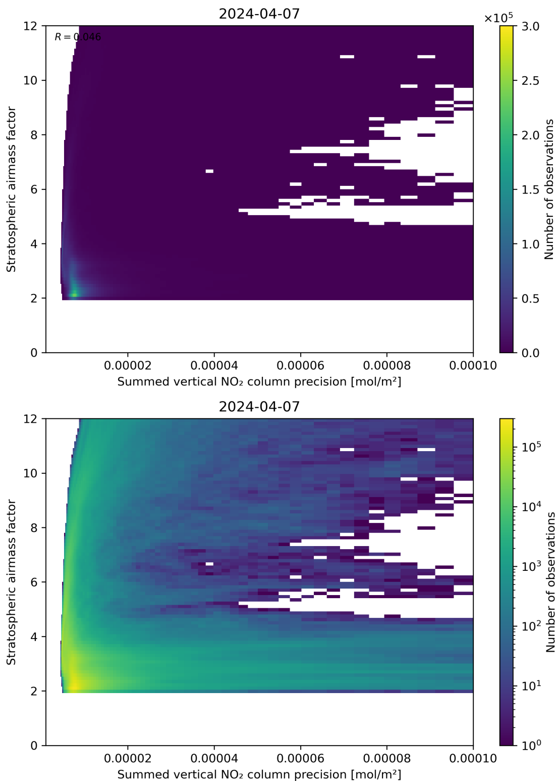
Figure 106: Scatter density plot of “Summed vertical NO 2 column precision” against “Stratospheric airmass factor” for 2024-04-06 to 2024-04-08.
