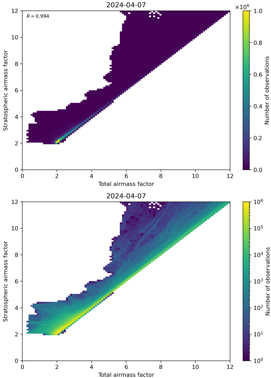
Figure 62: Scatter density plot of “Total airmass factor” against “Stratospheric airmass factor” for 2024-04-06 to 2024-04-08.
