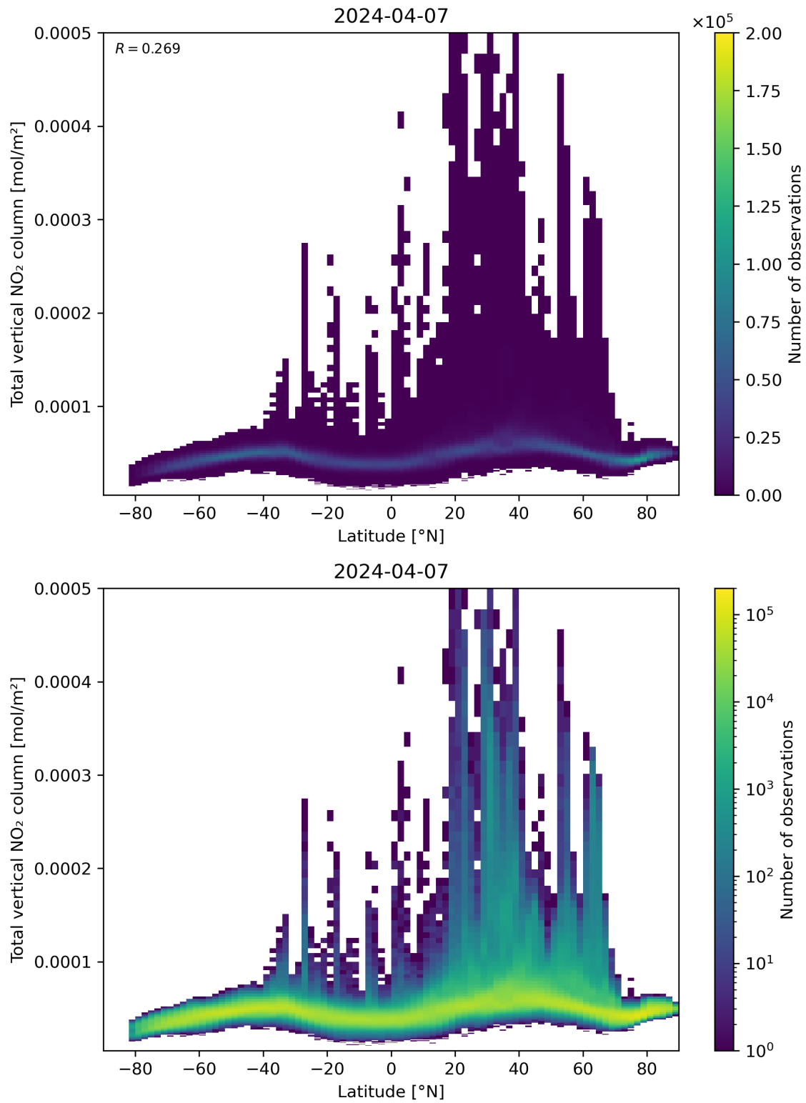
Figure 90: Scatter density plot of “Latitude” against “Total vertical NO 2 column” for 2024-04-06 to 2024-04-08.
