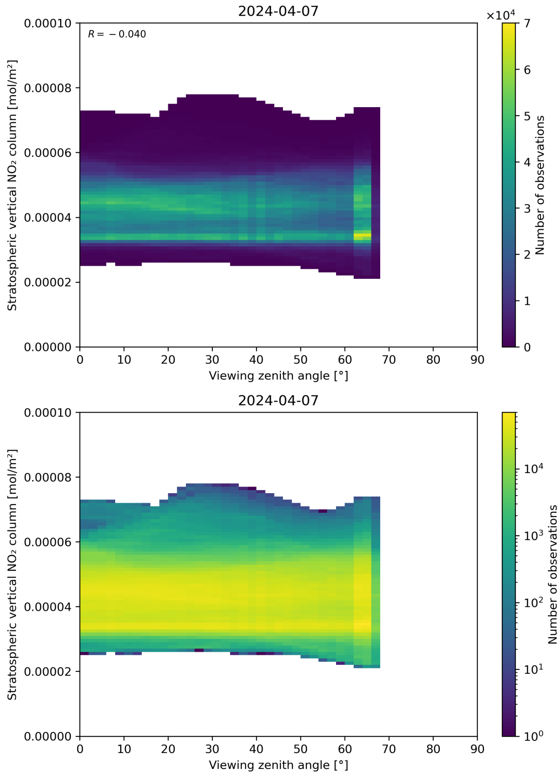
Figure 164: Scatter density plot of “Viewing zenith angle” against “Stratospheric vertical NO 2 column” for 2024-04-06 to 2024-04-08.
