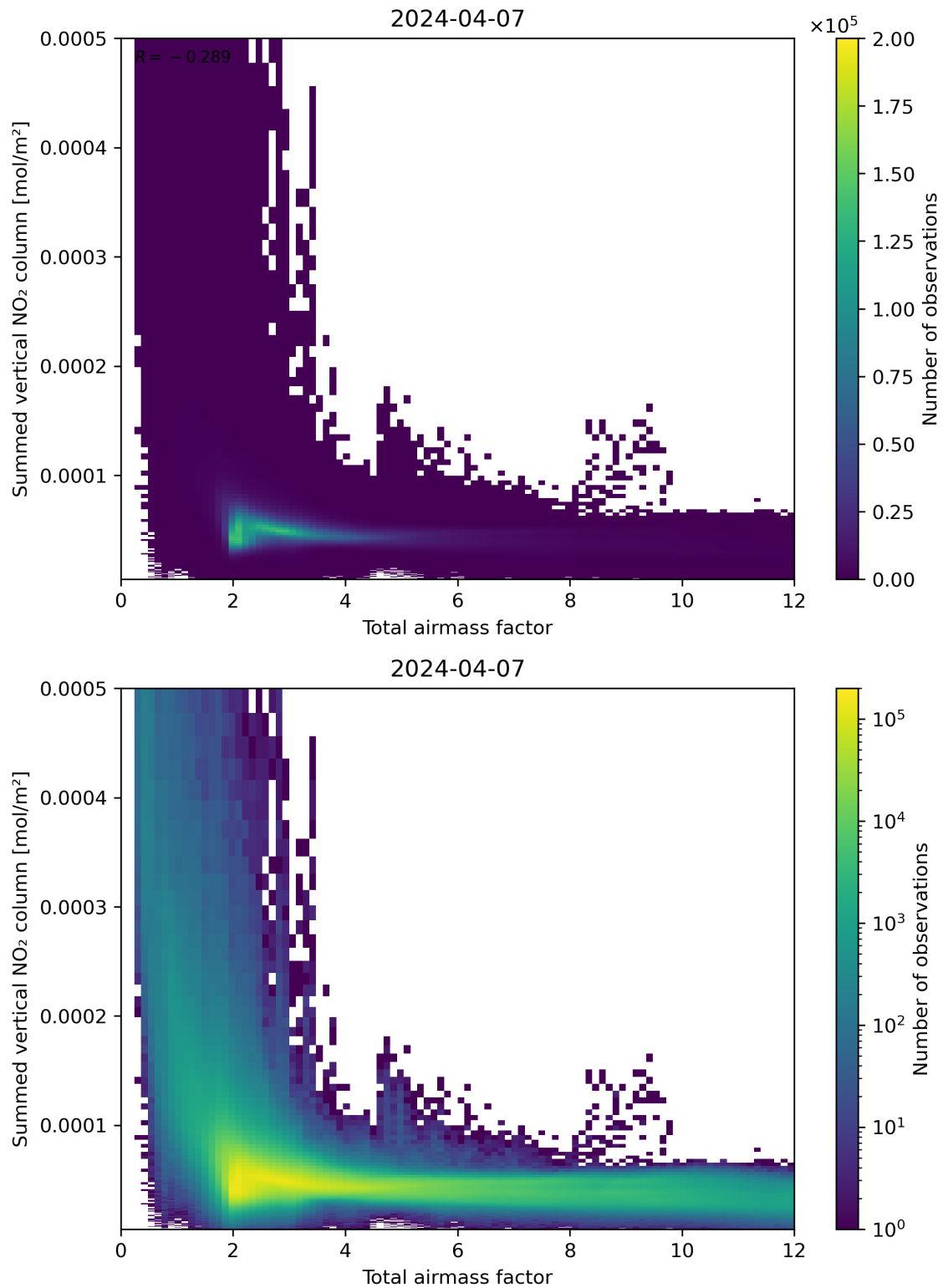
Figure 65: Scatter density plot of “Total airmass factor” against “Summed vertical NO 2 column” for 2024-04-06 to 2024-04-08.
