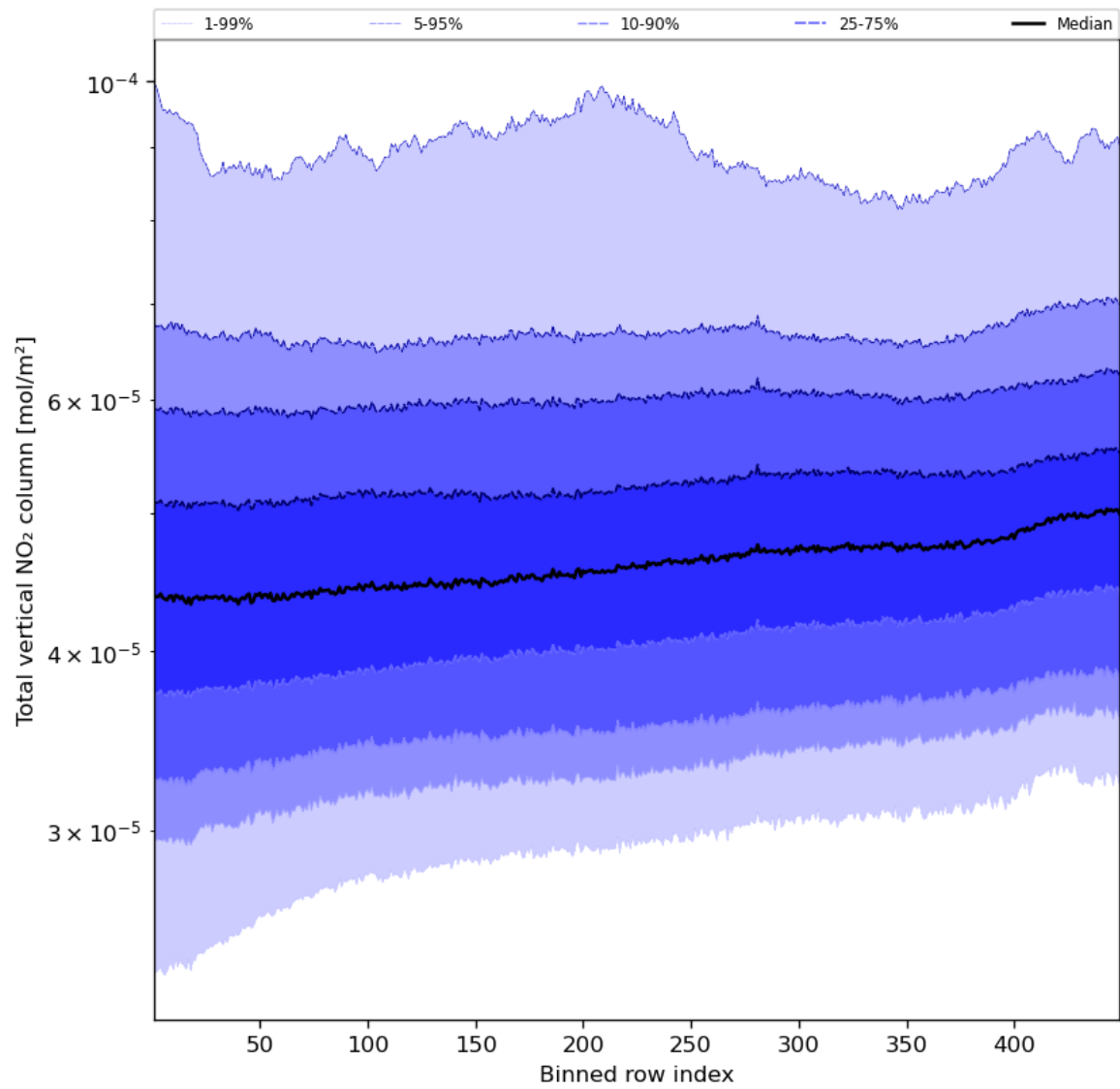
Figure 55: Along track statistics of “Total vertical NO 2 column” for 2024-04-06 to 2024-04-08
