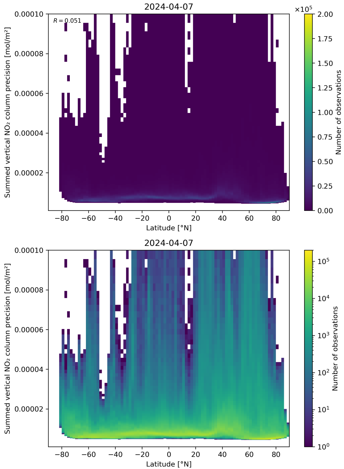
Figure 89: Scatter density plot of “Latitude” against “Summed vertical NO 2 column precision” for 2024-04-06 to 2024-04-08.
