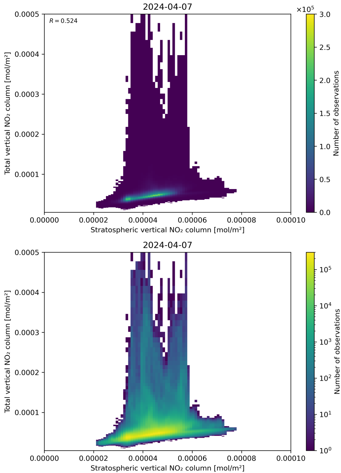
Figure 100: Scatter density plot of “Stratospheric vertical NO 2 column” against “Total vertical NO 2 column” for 2024-04-06 to 2024-04-08.
