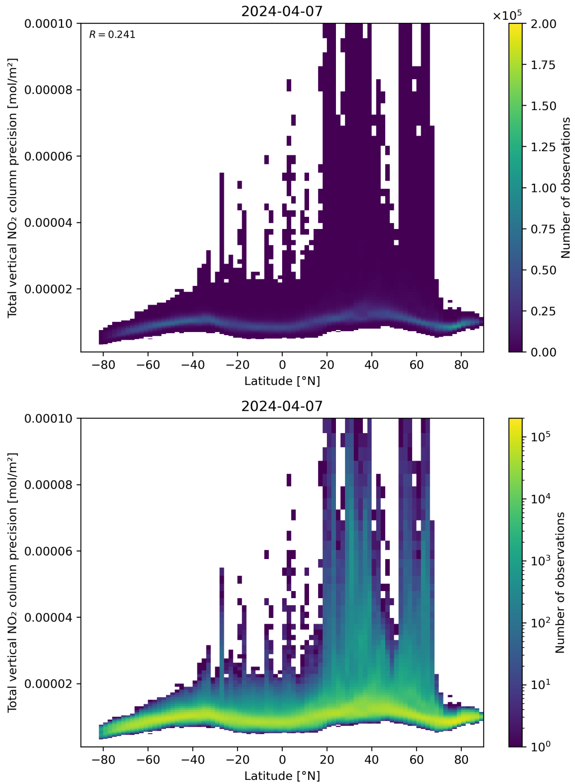
Figure 91: Scatter density plot of “Latitude” against “Total vertical NO 2 column precision” for 2024-04-06 to 2024-04-08.
