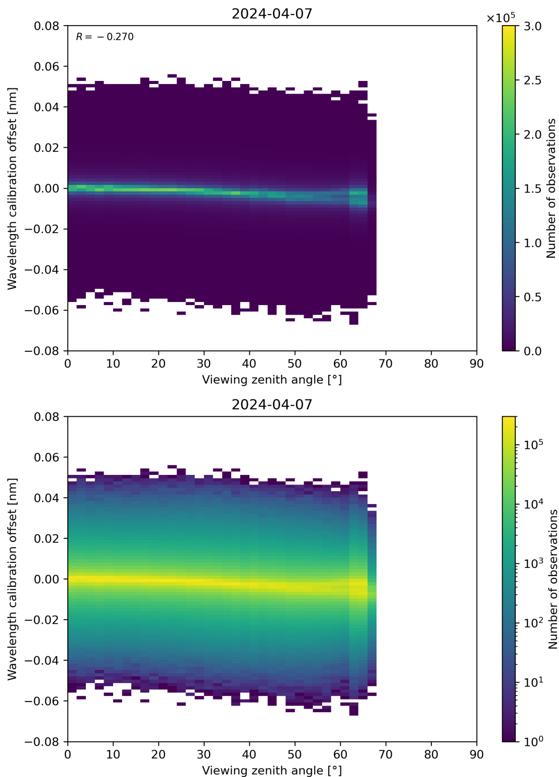
Figure 173: Scatter density plot of “Viewing zenith angle” against “Wavelength calibration offset” for 2024-04-06 to 2024-04-08.
