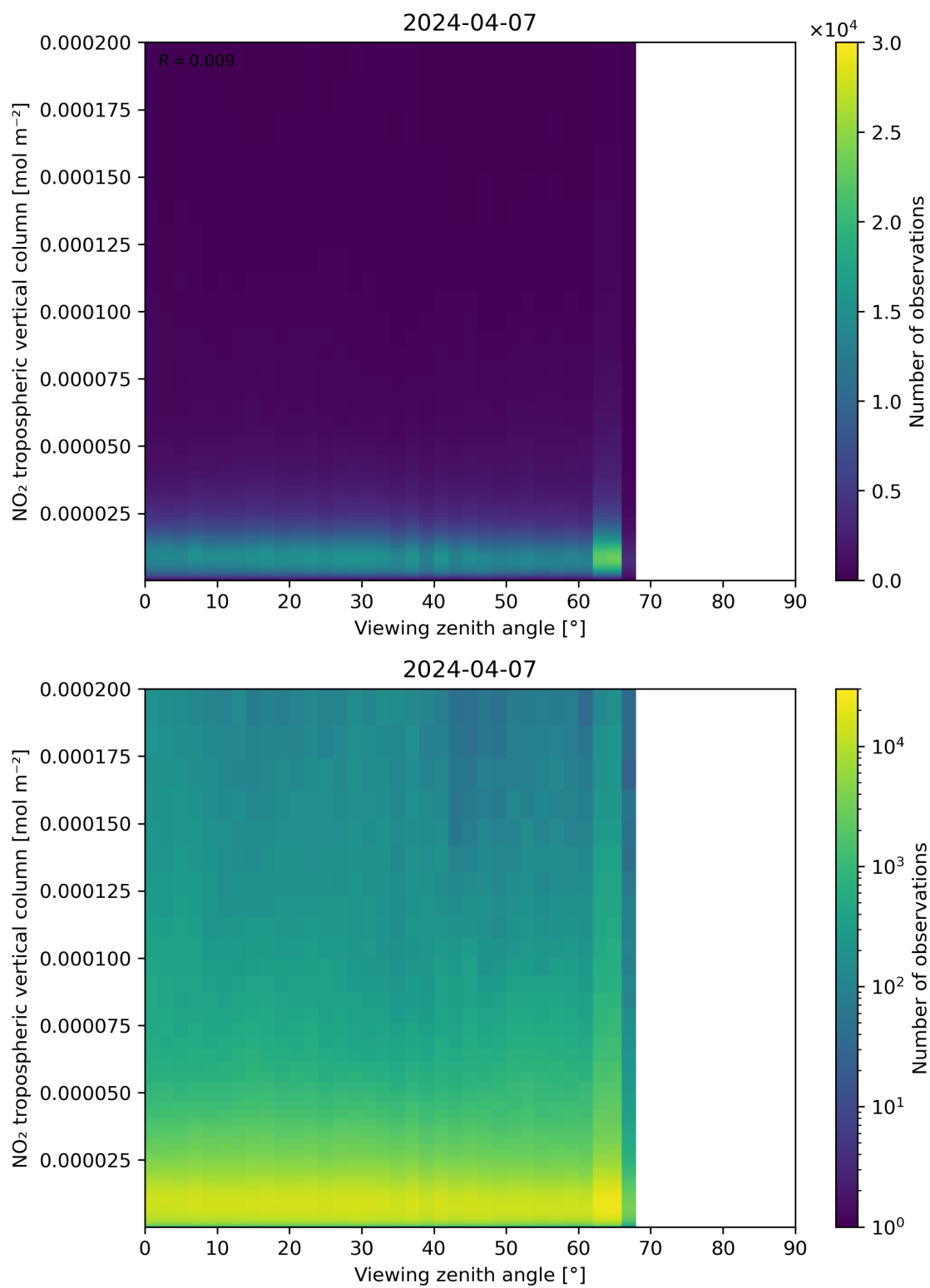
Figure 169: Scatter density plot of “Viewing zenith angle” against “NO 2 tropospheric vertical column” for 2024-04-06 to 2024-04-08.
