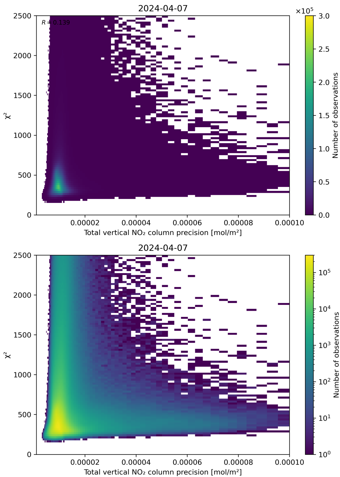
Figure 116: Scatter density plot of “Total vertical NO 2 column precision” against “ \chi^2 ” for 2024-04-06 to 2024-04-08.
