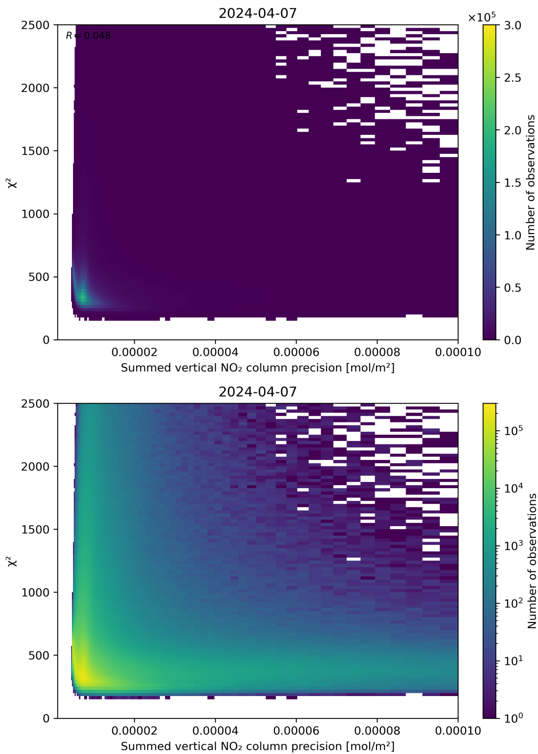
Figure 107: Scatter density plot of “Summed vertical NO 2 column precision” against “ \chi^2 ” for 2024-04-06 to 2024-04-08.
