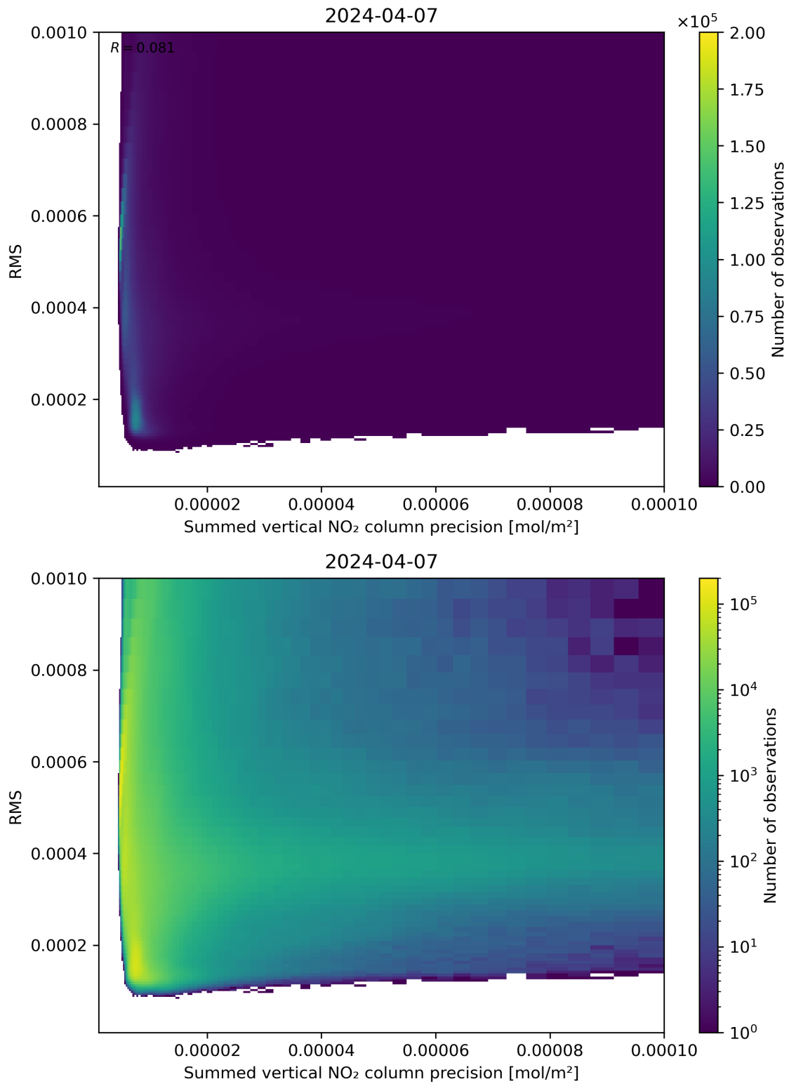
Figure 108: Scatter density plot of “Summed vertical NO 2 column precision” against “RMS” for 2024-04-06 to 2024-04-08.
