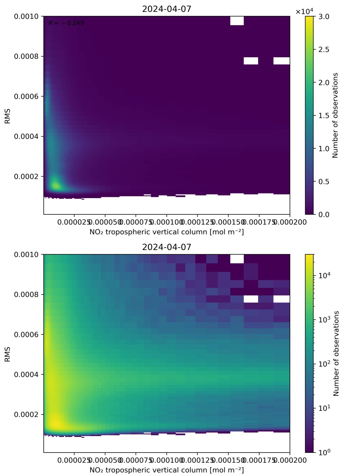
Figure 142: Scatter density plot of “NO 2 tropospheric vertical column” against “RMS” for 2024-04-06 to 2024-04-08.
