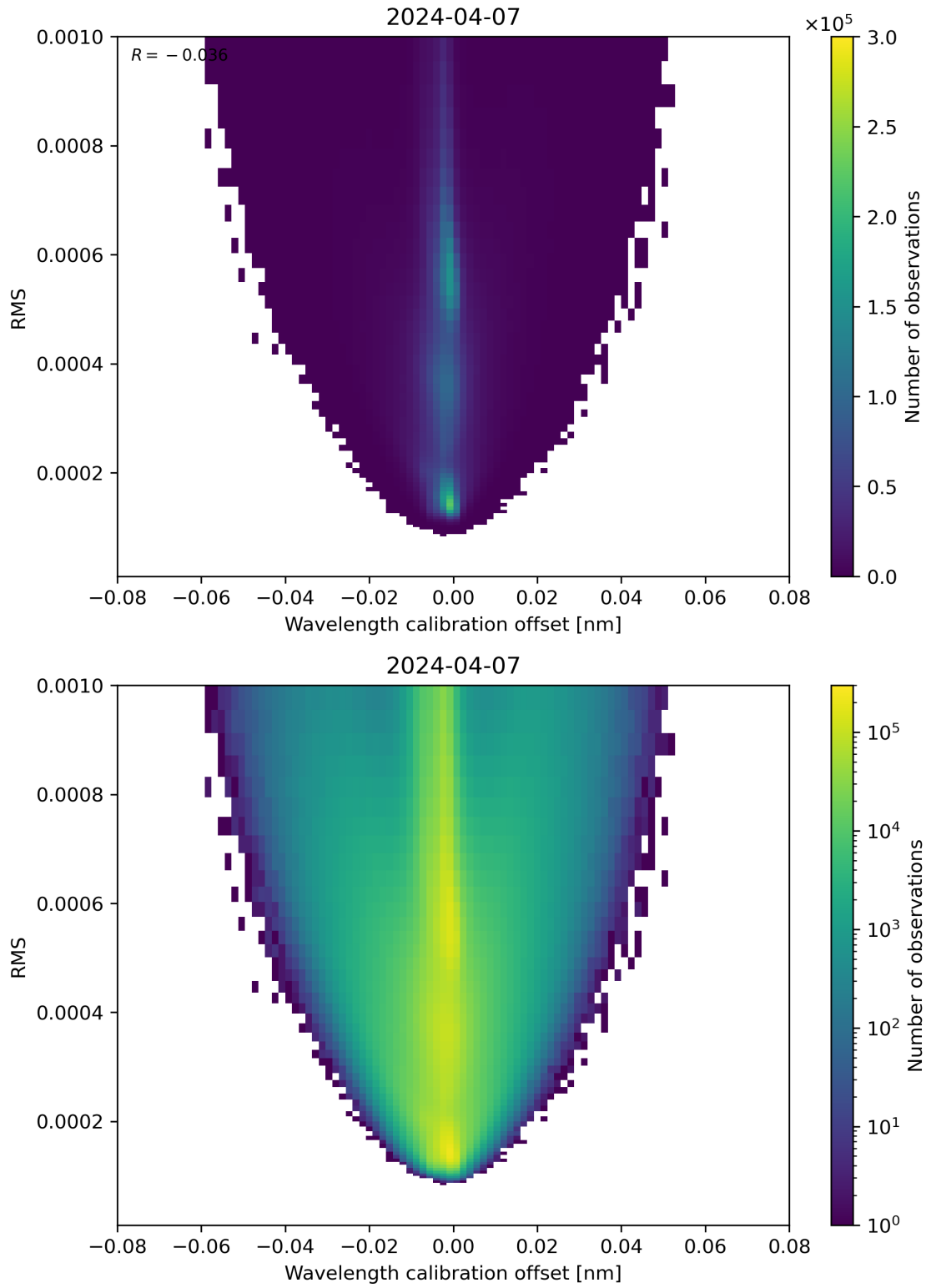
Figure 181: Scatter density plot of “Wavelength calibration offset” against “RMS” for 2024-04-06 to 2024-04-08.
