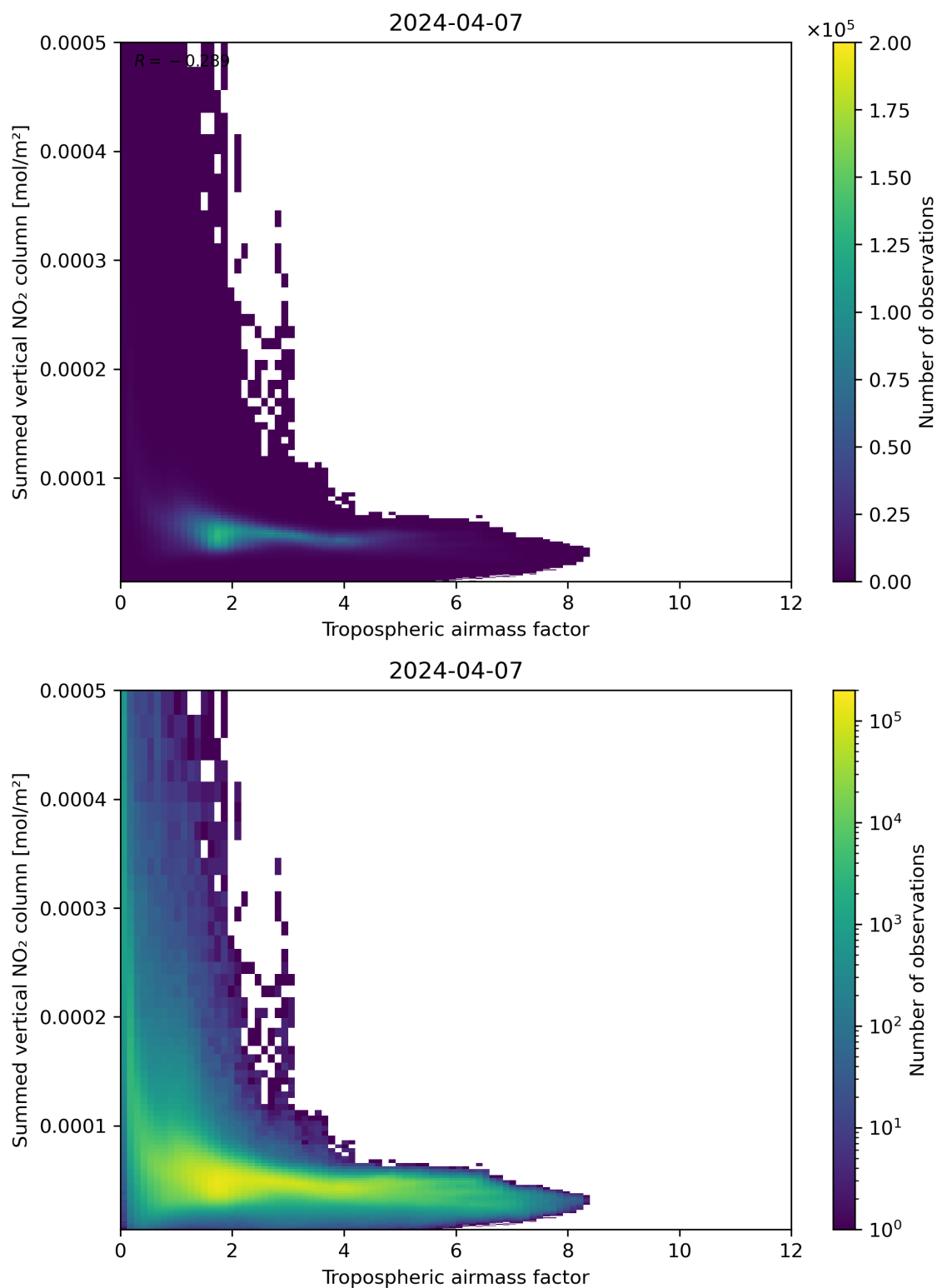
Figure 75: Scatter density plot of “Tropospheric air mass factor” against “Summed vertical NO 2 column” for 2024-04-06 to 2024-04-08.
