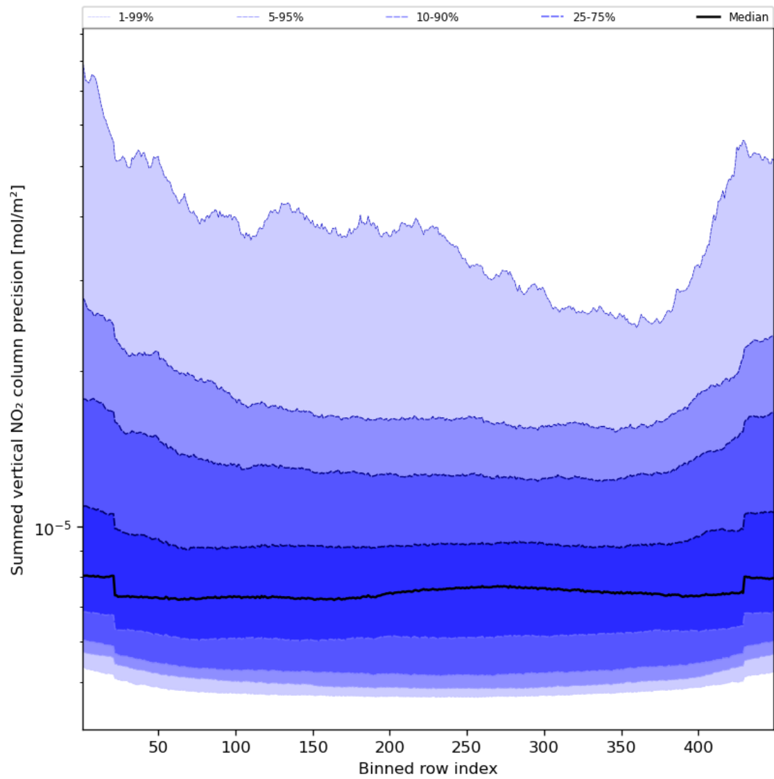
Figure 58: Along track statistics of “Summed vertical NO 2 column precision” for 2024-04-06 to 2024-04-08
