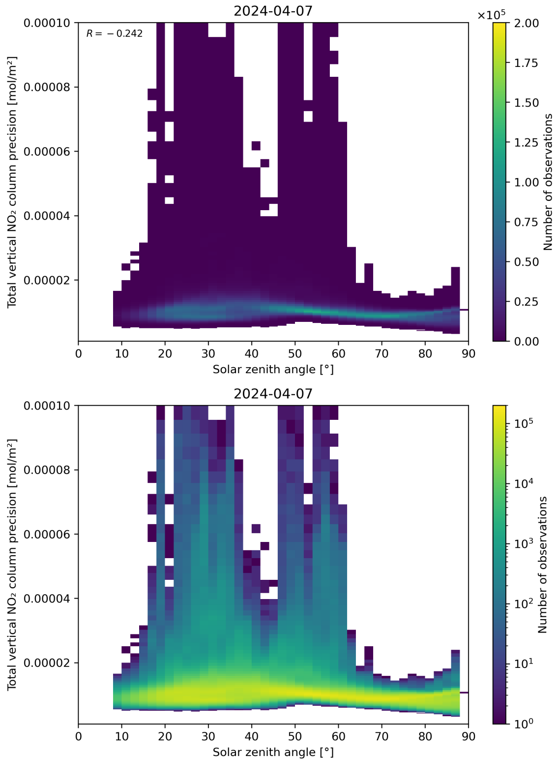
Figure 154: Scatter density plot of “Solar zenith angle” against “Total vertical NO 2 column precision” for 2024-04-06 to 2024-04-08.
