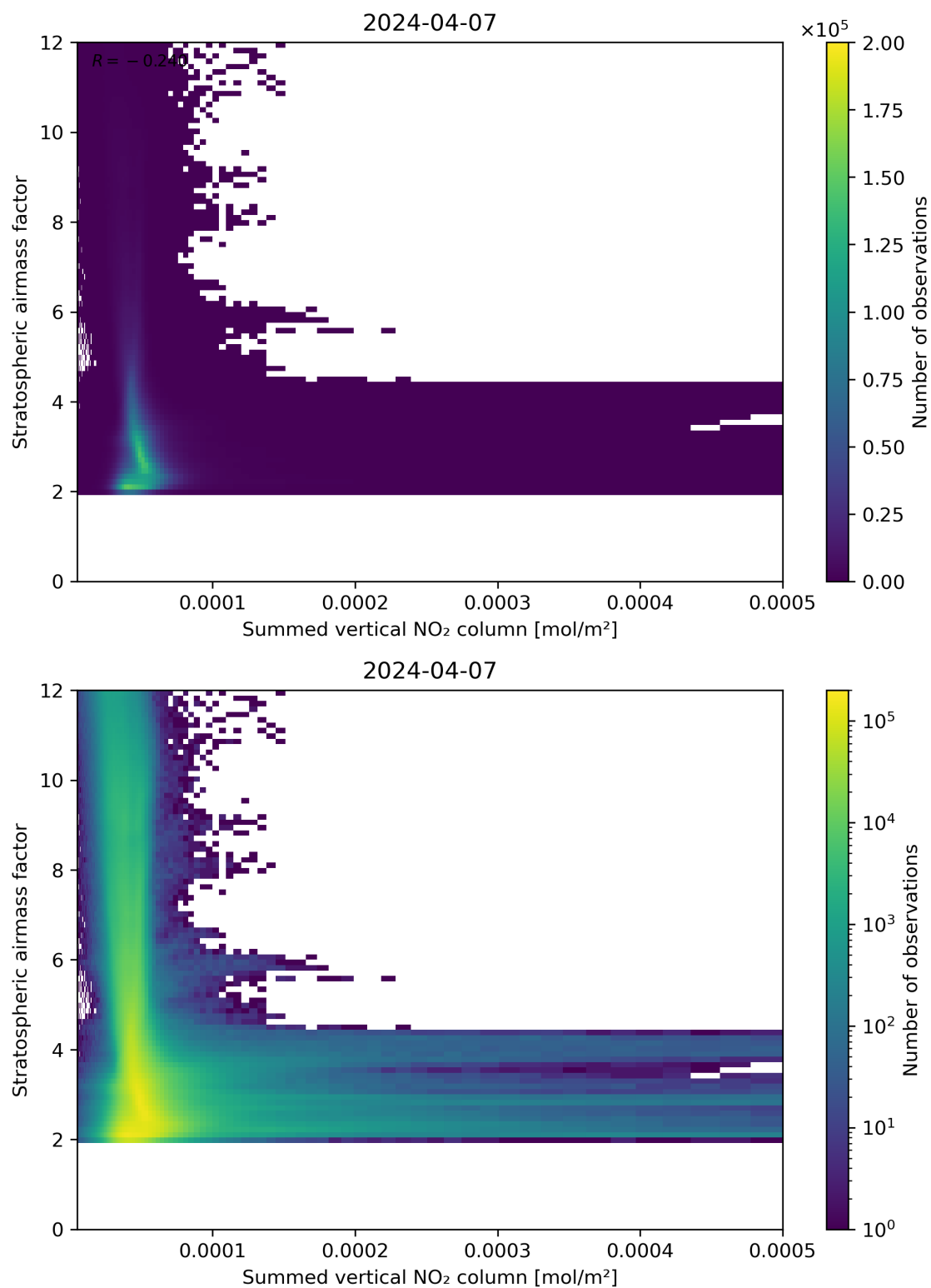
Figure 103: Scatter density plot of “Summed vertical NO 2 column” against “Stratospheric air mass factor” for 2024-04-06 to 2024-04-08.
