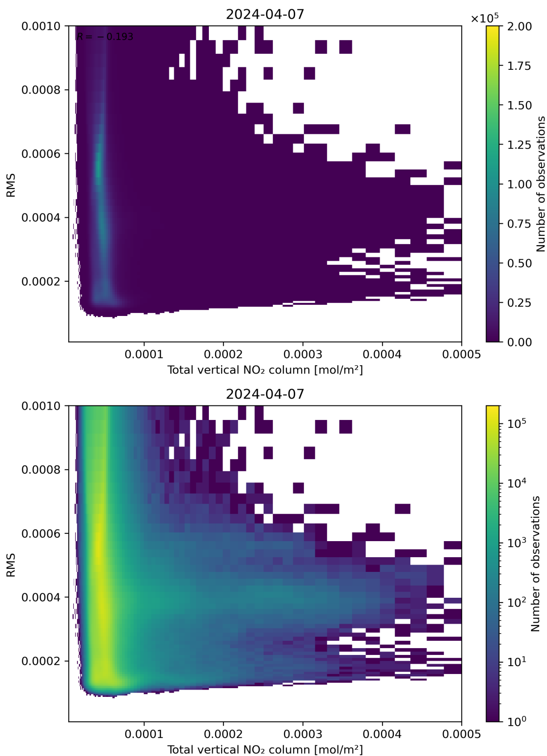
Figure 120: Scatter density plot of “Total vertical NO 2 column” against “RMS” for 2024-04-06 to 2024-04-08.
