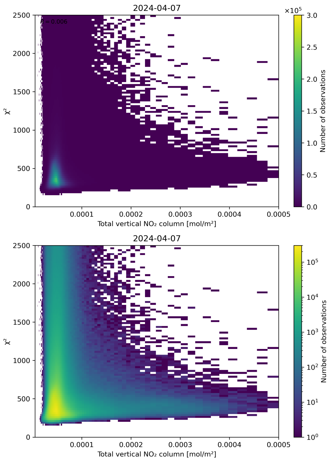
Figure 111: Scatter density plot of “Total vertical NO 2 column” against “ \chi^2 ” for 2024-04-06 to 2024-04-08.
