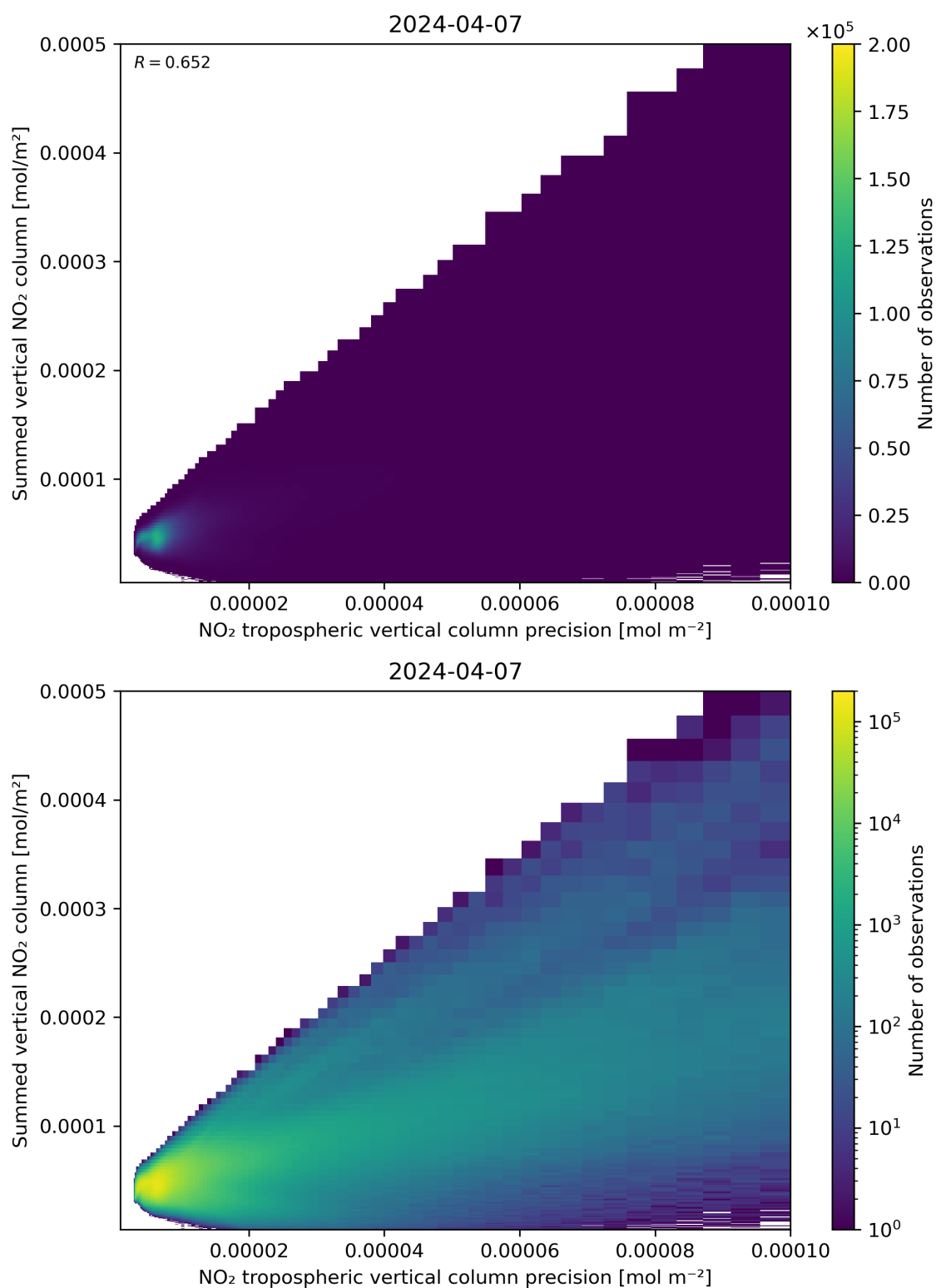
Figure 136: Scatter density plot of “NO 2 tropospheric vertical column precision” against “Summed vertical NO 2 column” for 2024-04-06 to 2024-04-08.
