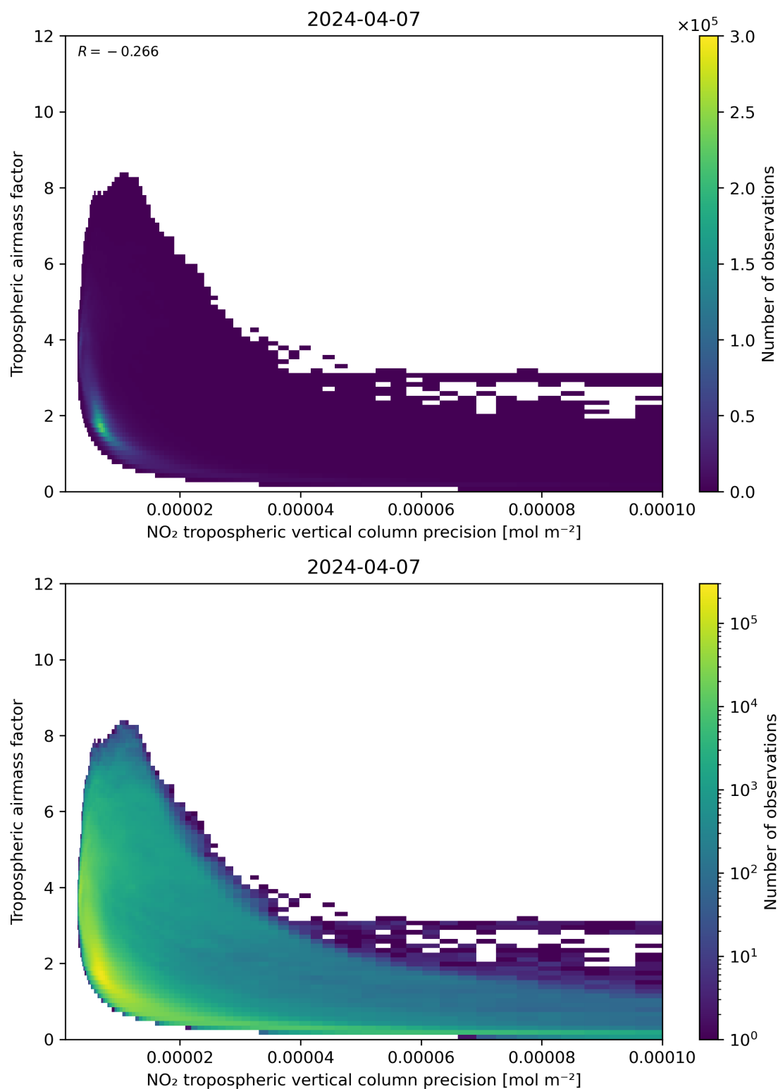
Figure 133: Scatter density plot of “NO 2 tropospheric vertical column precision” against “Tropospheric airmass factor” for 2024-04-06 to 2024-04-08.
