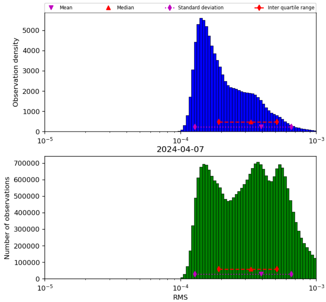
Figure 43: Histogram of “RMS” for 2024-04-06 to 2024-04-08
