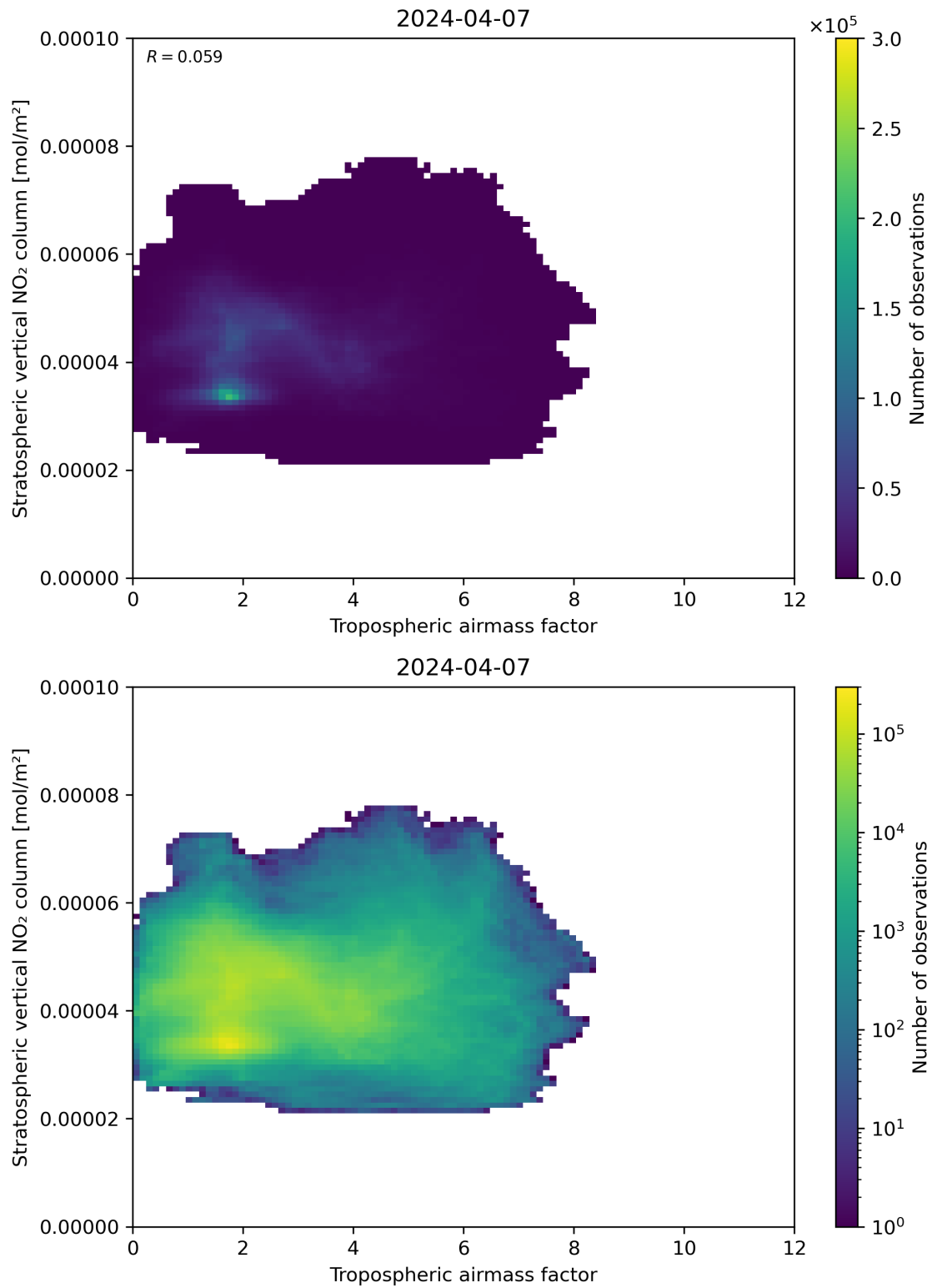
Figure 74: Scatter density plot of “Tropospheric air mass factor” against “Stratospheric vertical \text{NO}_2 column” for 2024-04-06 to 2024-04-08.
