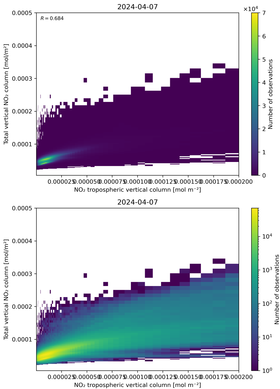
Figure 128: Scatter density plot of “NO 2 tropospheric vertical column” against “Total vertical NO 2 column” for 2024-04-06 to 2024-04-08.
