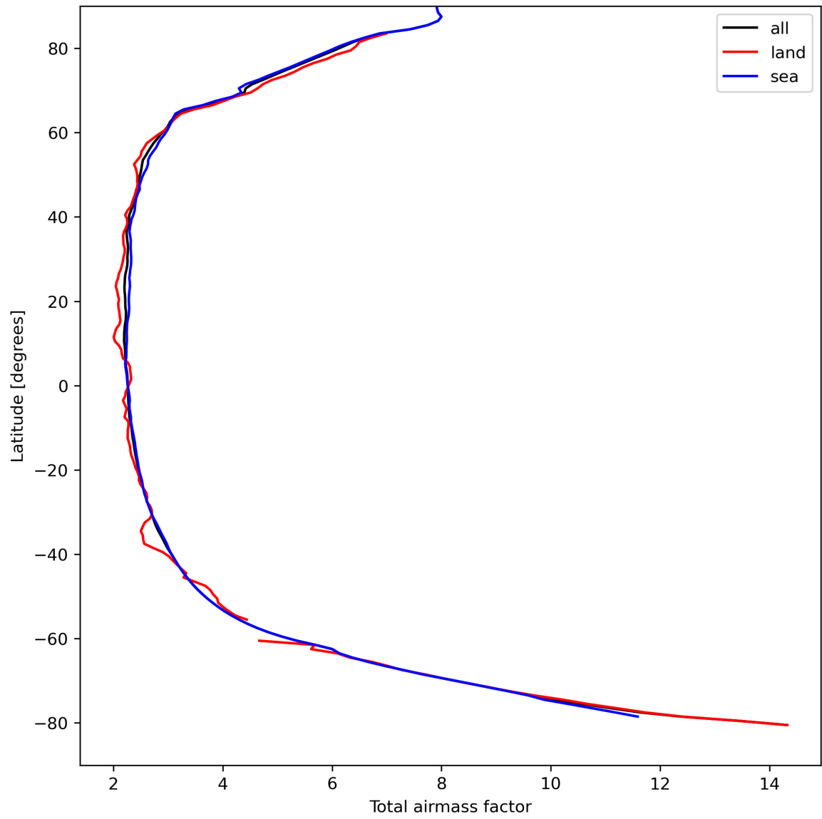
Figure 15: Zonal average of “Total airmass factor” for 2024-04-07 to 2024-04-09.
