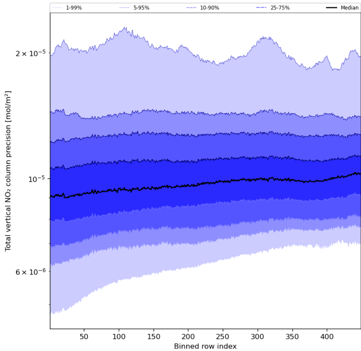
Figure 56: Along track statistics of "Total vertical NO 2 column precision" for 2024-04-07 to 2024-04-09
