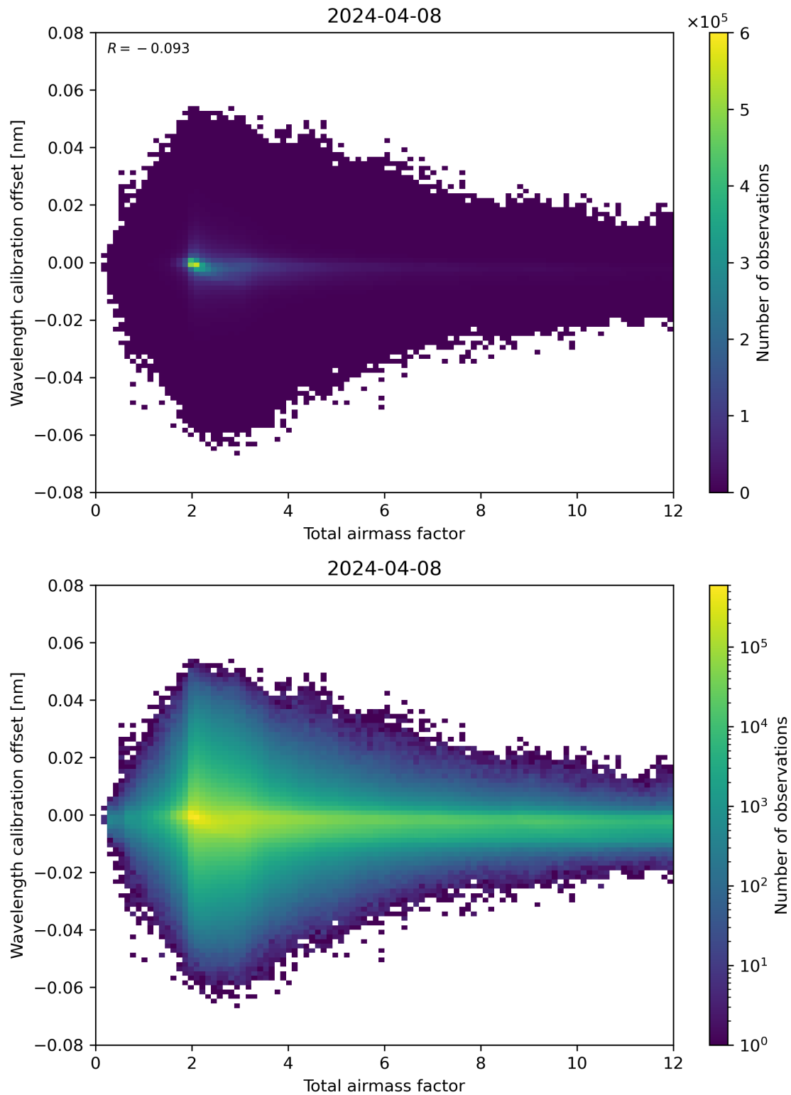
Figure 70: Scatter density plot of “Total airmass factor” against “Wavelength calibration offset” for 2024-04-07 to 2024-04-09.
