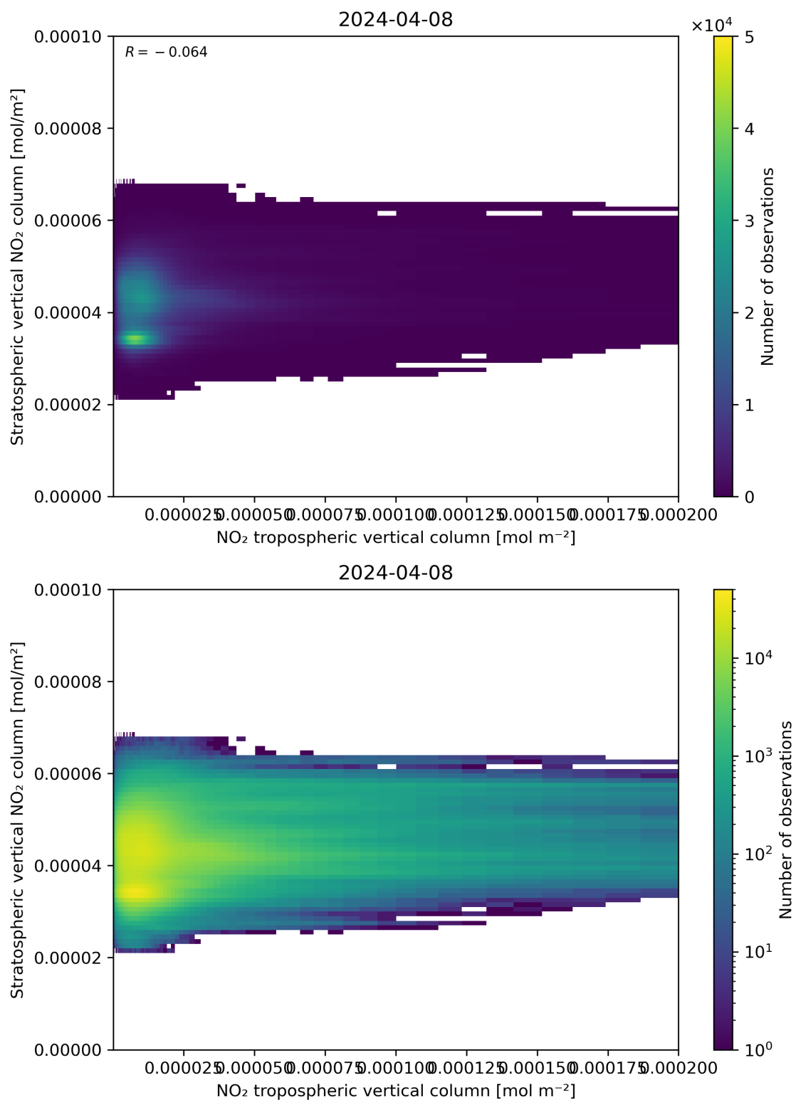
Figure 125: Scatter density plot of “NO 2 tropospheric vertical column” against “Stratospheric vertical NO 2 column” for 2024-04-07 to 2024-04-09.
