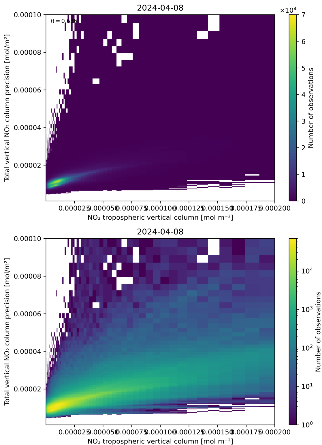
Figure 129: Scatter density plot of “NO 2 tropospheric vertical column” against “Total vertical NO 2 column precision” for 2024-04-07 to 2024-04-09.
