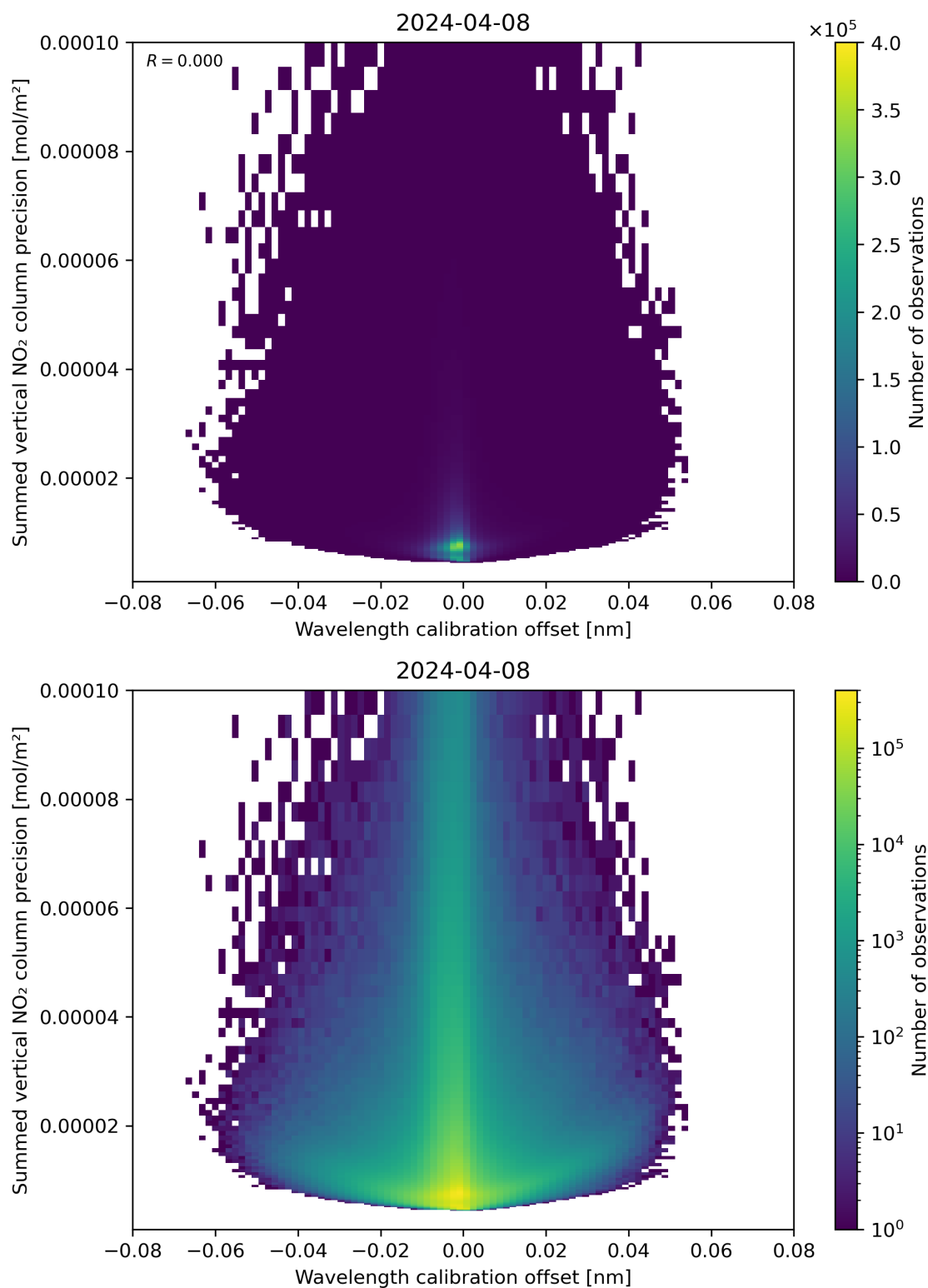
Figure 178: Scatter density plot of “Wavelength calibration offset” against “Summed vertical NO 2 column precision” for 2024-04-07 to 2024-04-09.
