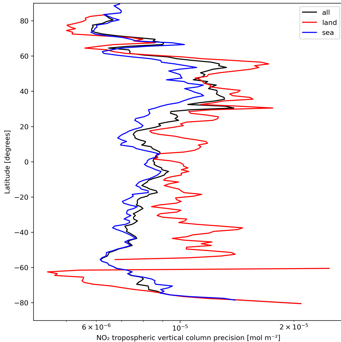
Figure 13: Zonal average of “NO 2 tropospheric vertical column precision” for 2024-04-07 to 2024-04-09.
