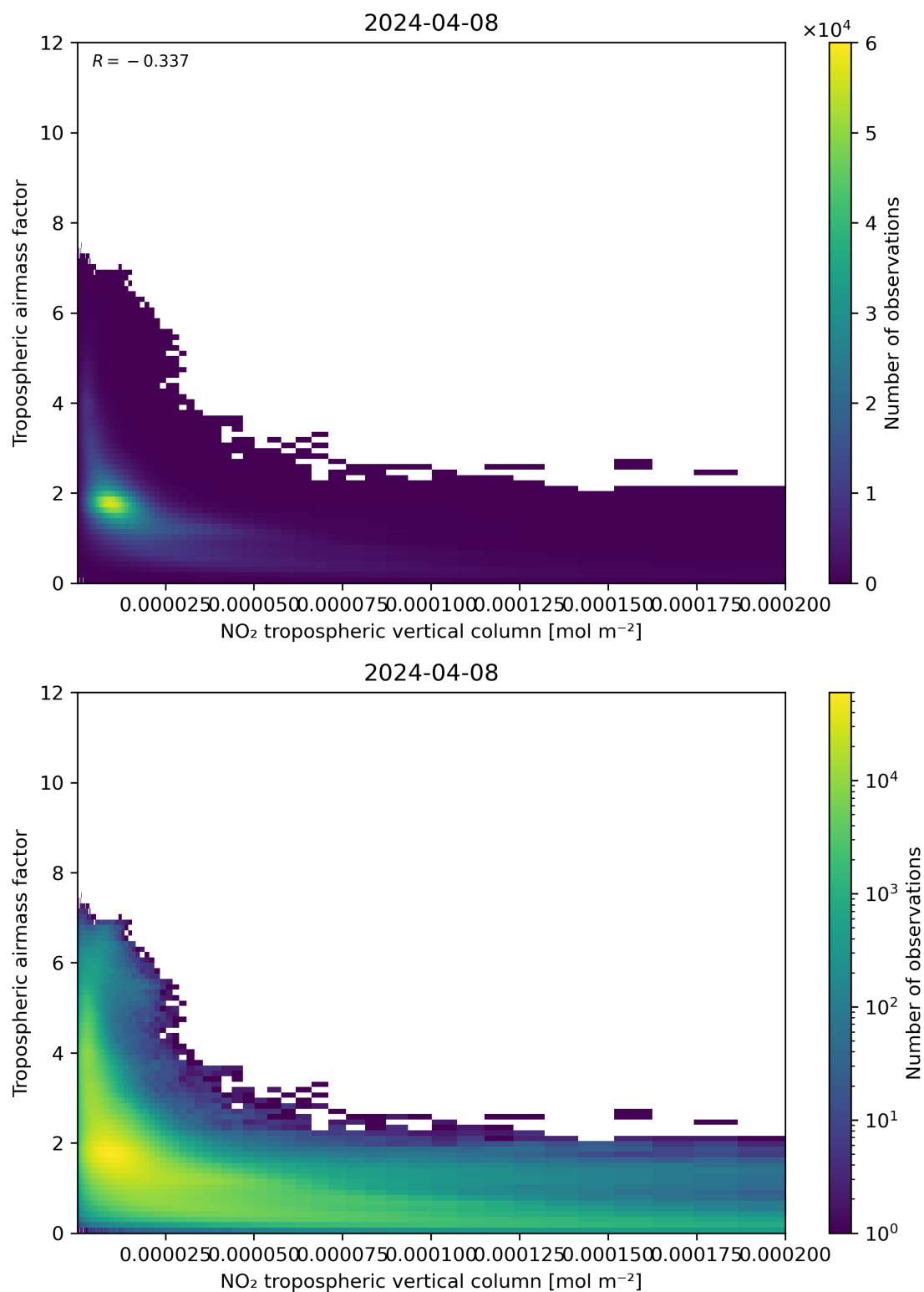
Figure 123: Scatter density plot of “NO 2 tropospheric vertical column” against “Tropospheric air mass factor” for 2024-04-07 to 2024-04-09.
