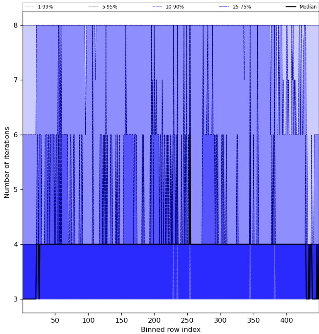
Figure 51: Along track statistics of “Number of iterations” for 2024-04-07 to 2024-04-09
