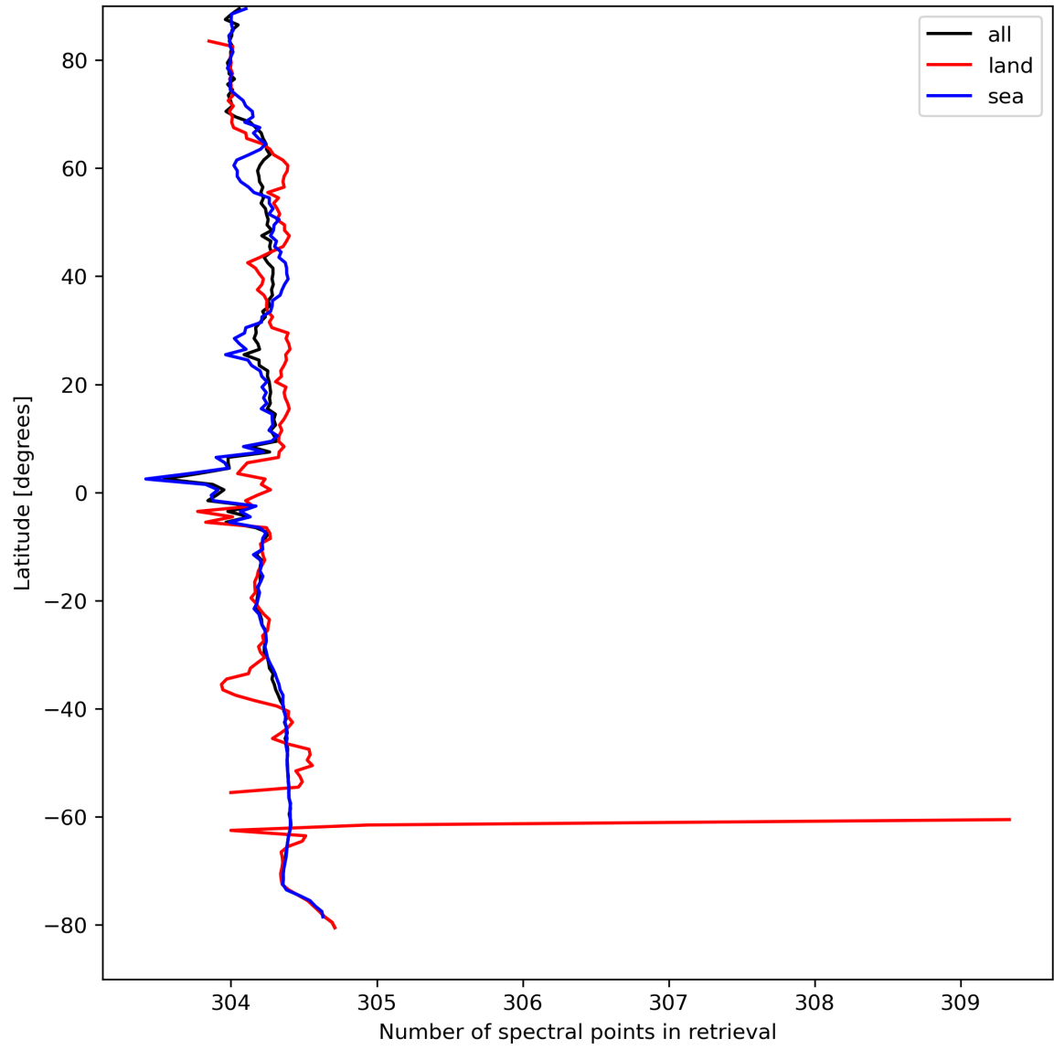
Figure 16: Zonal average of “Number of spectral points in retrieval” for 2024-04-07 to 2024-04-09.
