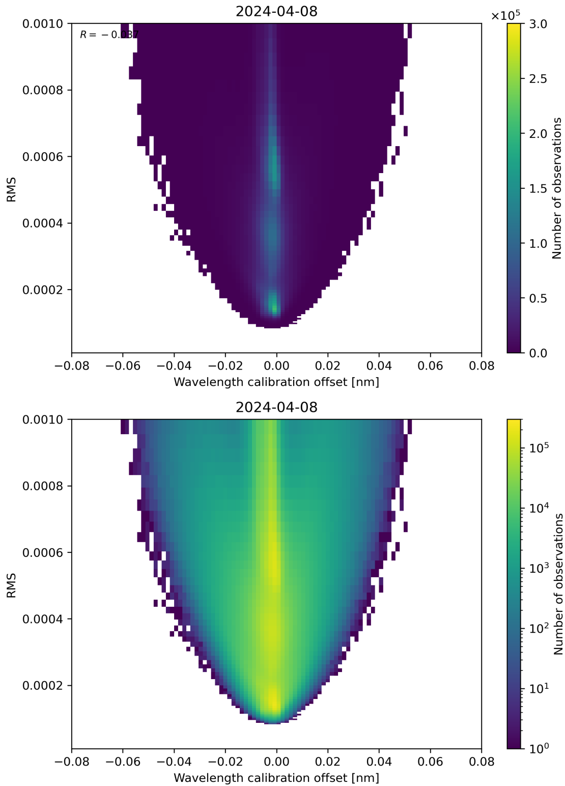
Figure 181: Scatter density plot of “Wavelength calibration offset” against “RMS” for 2024-04-07 to 2024-04-09.
