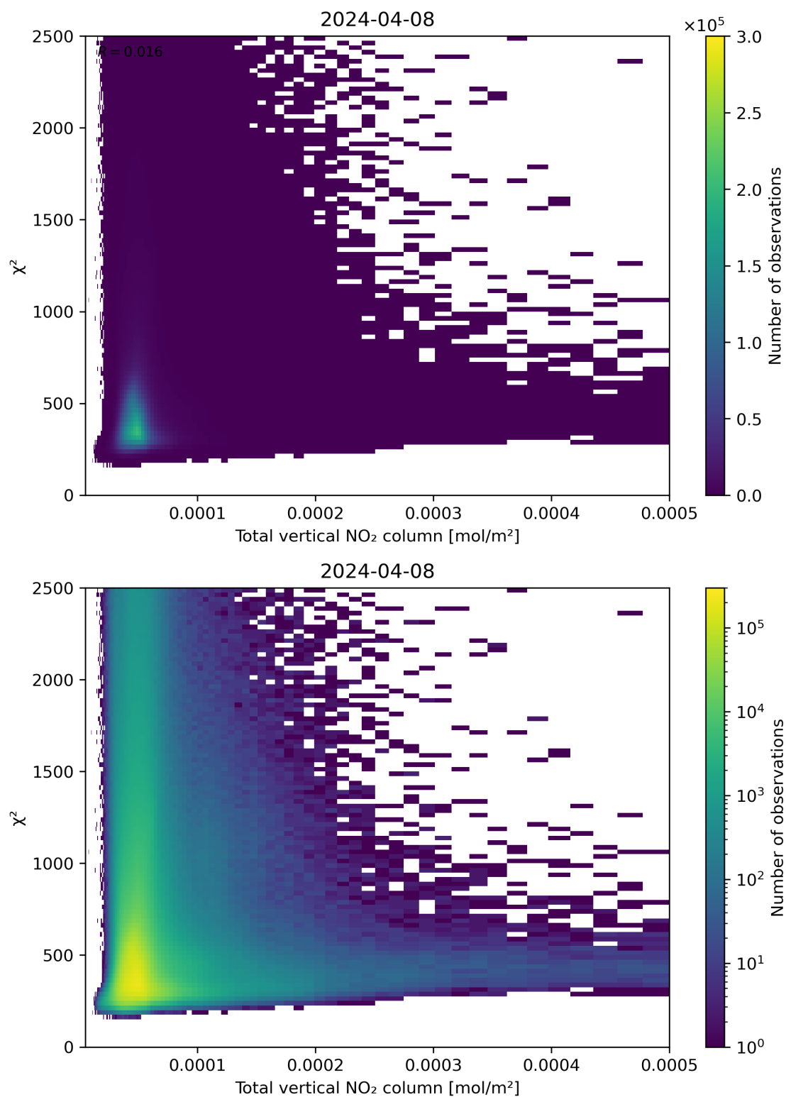
Figure 111: Scatter density plot of “Total vertical NO 2 column” against “ \chi^2 ” for 2024-04-07 to 2024-04-09.
