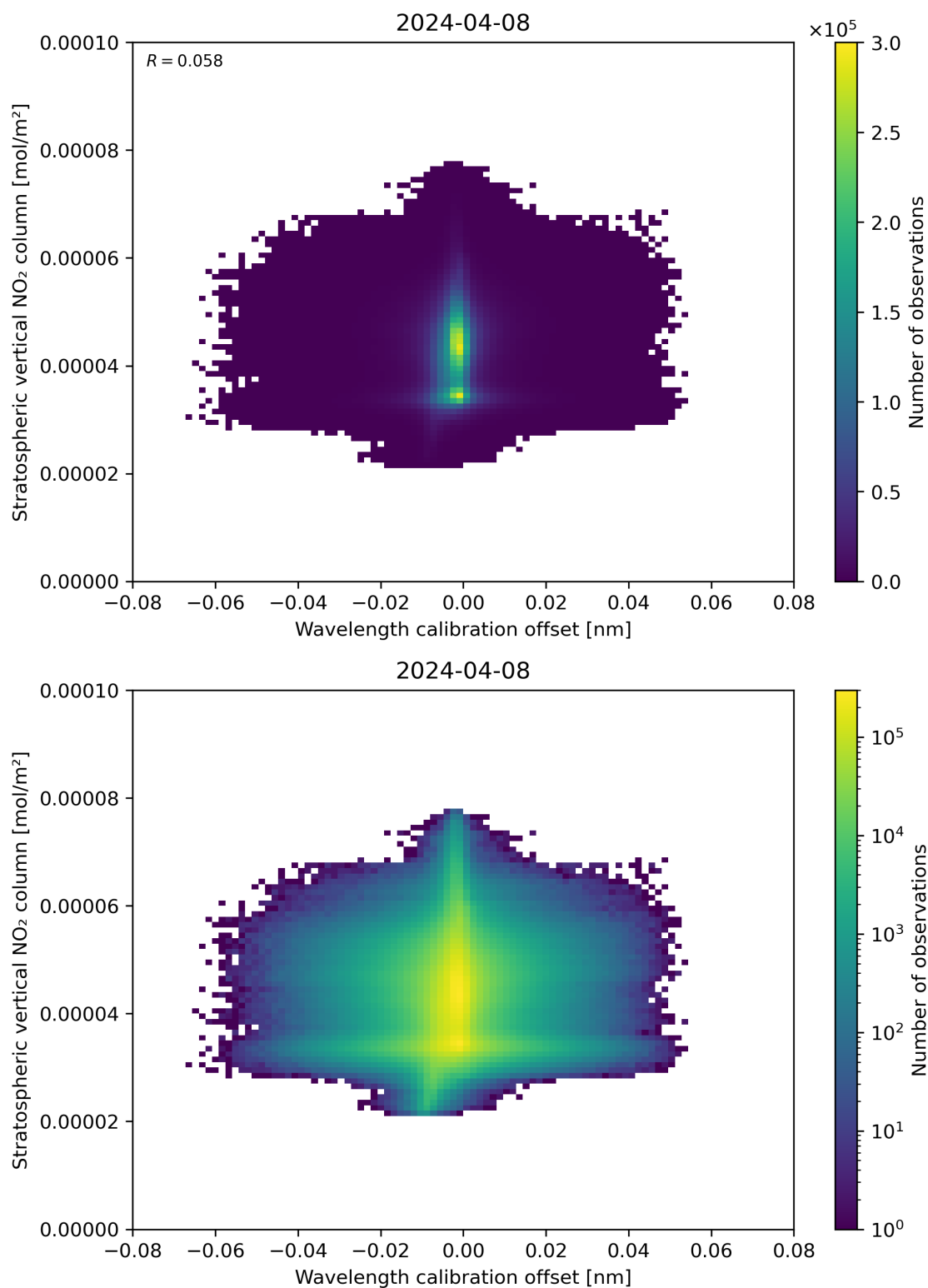
Figure 176: Scatter density plot of “Wavelength calibration offset” against “Stratospheric vertical NO 2 column” for 2024-04-07 to 2024-04-09.
