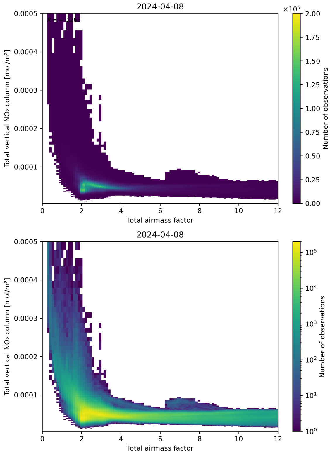
Figure 67: Scatter density plot of “Total airmass factor” against “Total vertical NO 2 column” for 2024-04-07 to 2024-04-09.
