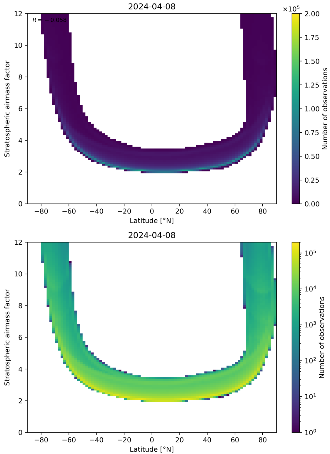
Figure 83: Scatter density plot of “Latitude” against “Stratospheric air mass factor” for 2024-04-07 to 2024-04-09.
