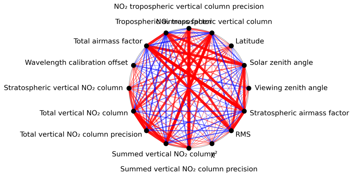
Figure 1: Map of correlation graph for 2024-04-07 to 2024-04-09.
