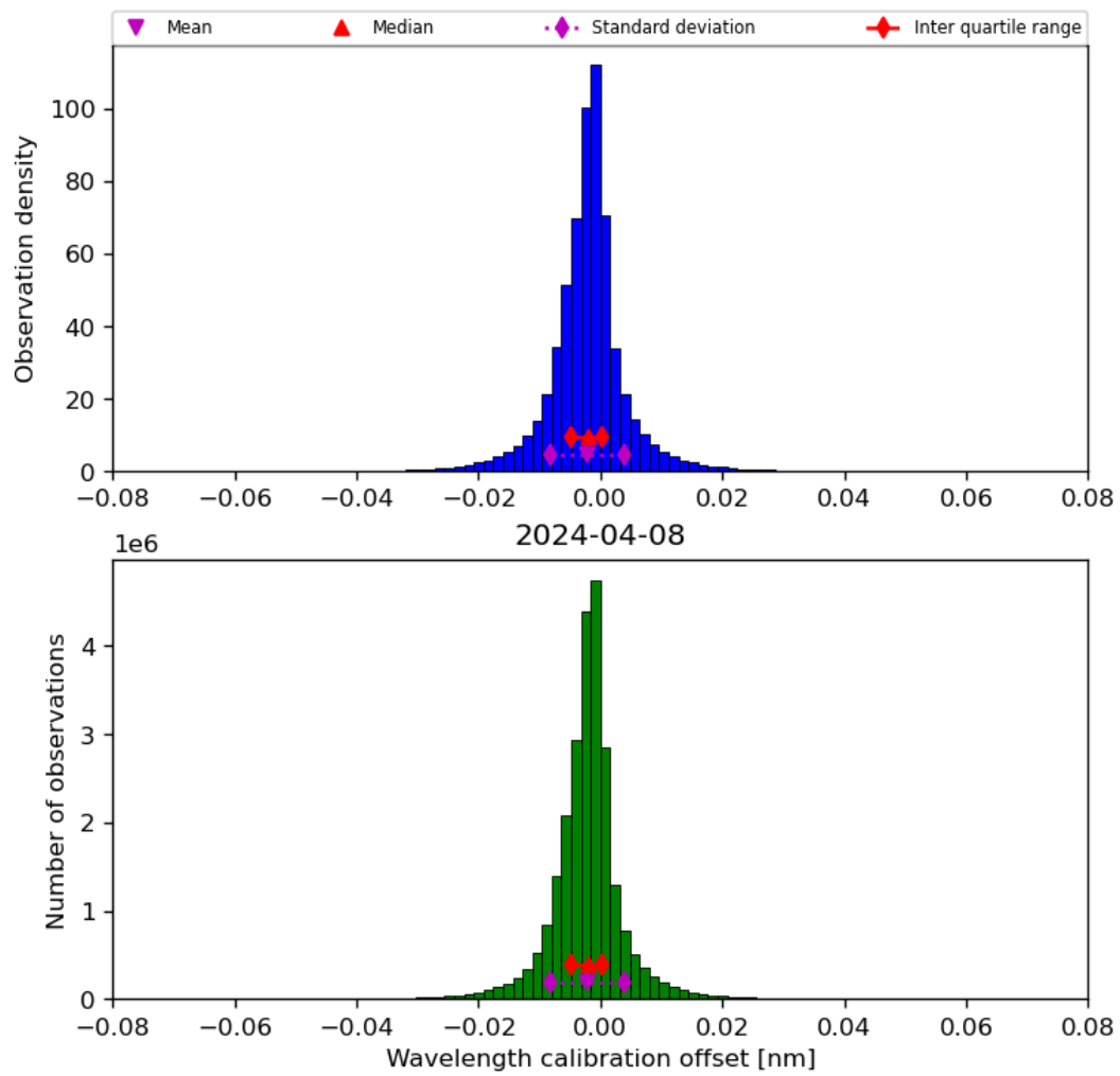
Figure 35: Histogram of “Wavelength calibration offset” for 2024-04-07 to 2024-04-09
