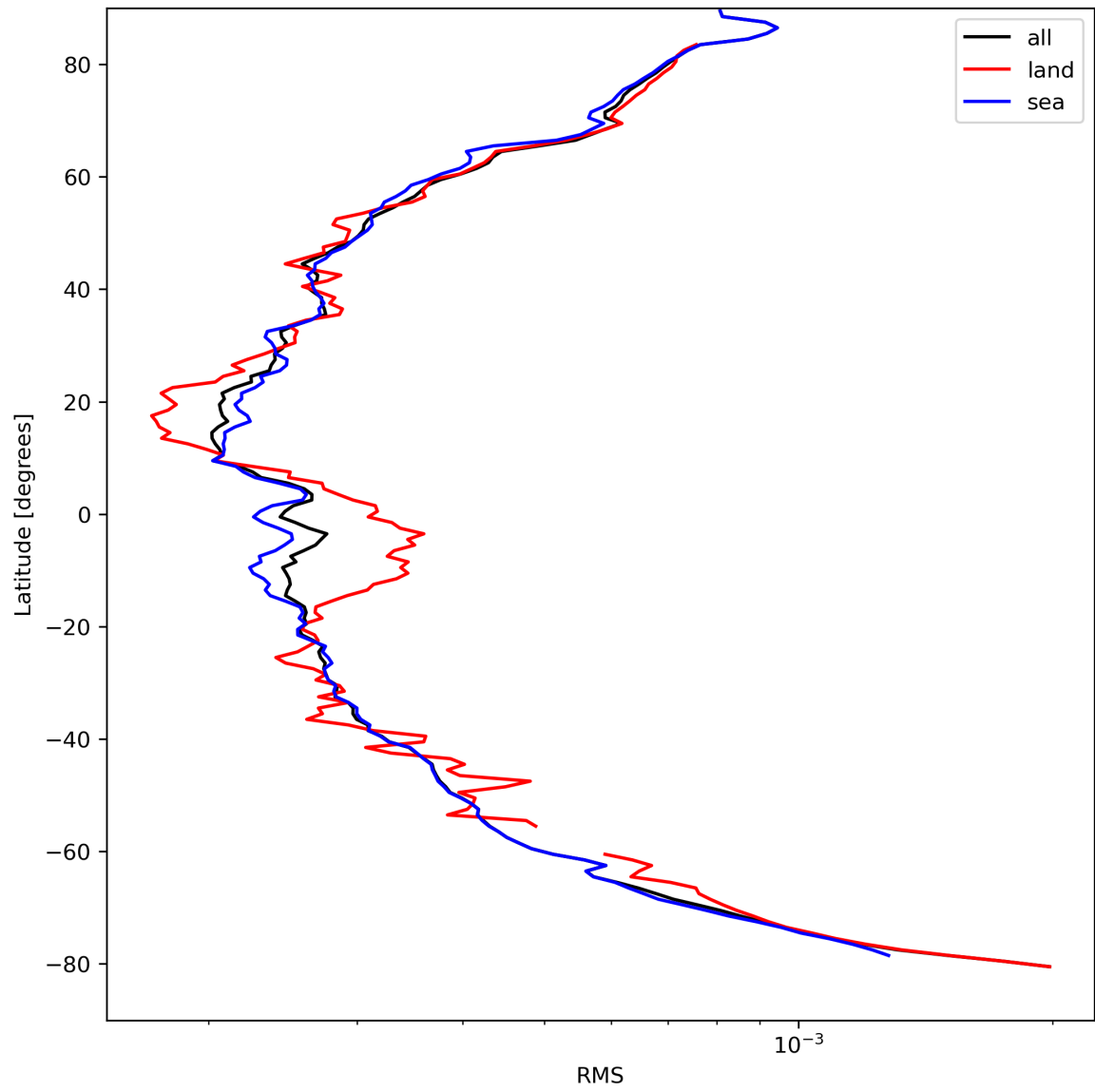
Figure 26: Zonal average of “RMS” for 2024-04-07 to 2024-04-09.
