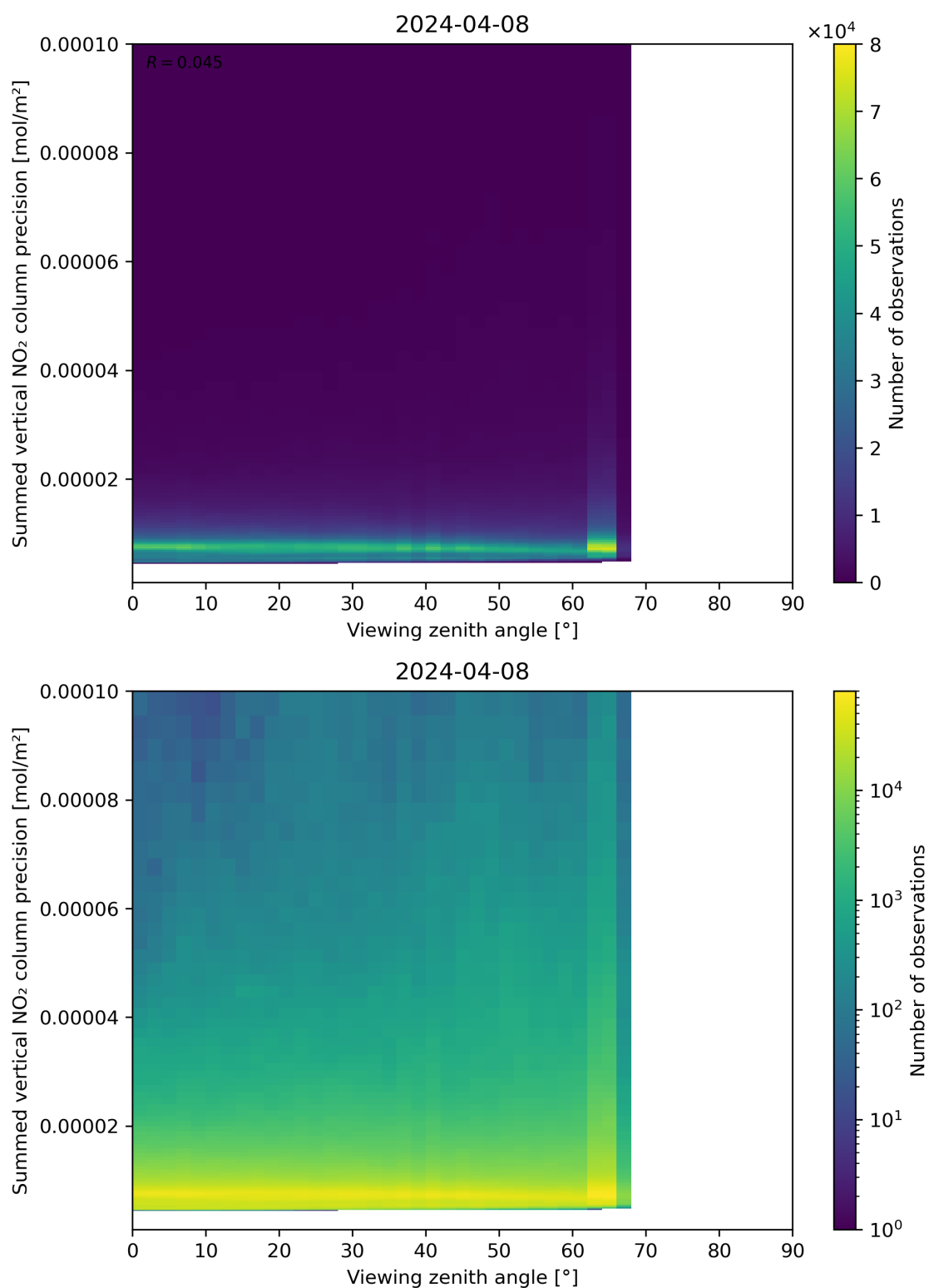
Figure 166: Scatter density plot of “Viewing zenith angle” against “Summed vertical NO 2 column precision” for 2024-04-07 to 2024-04-09.
