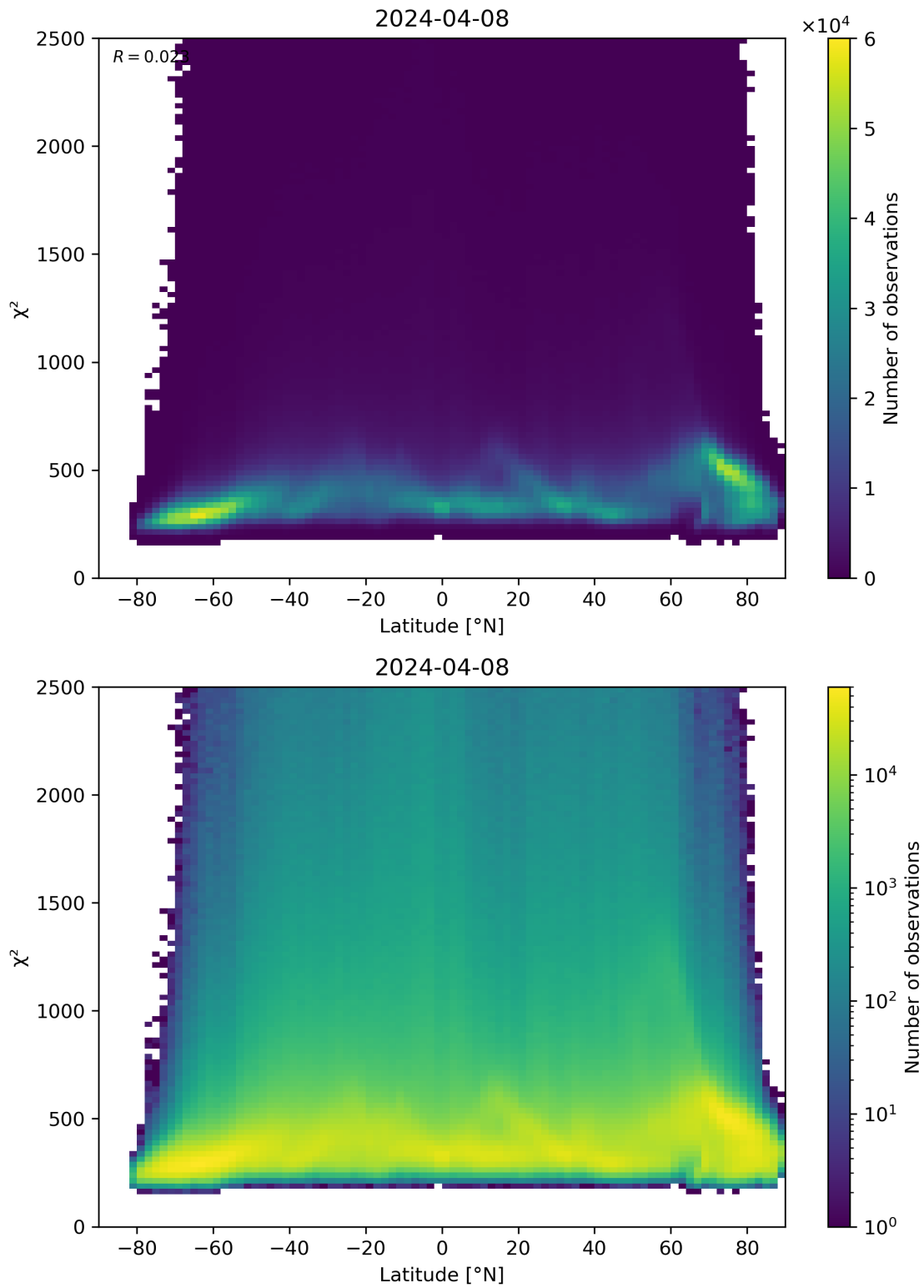
Figure 86: Scatter density plot of “Latitude” against “ \chi^2 ” for 2024-04-07 to 2024-04-09.
