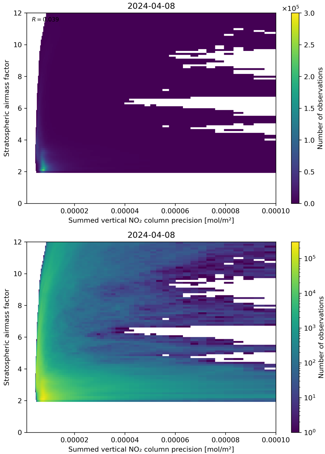
Figure 106: Scatter density plot of “Summed vertical NO 2 column precision” against “Stratospheric airmass factor” for 2024-04-07 to 2024-04-09.
