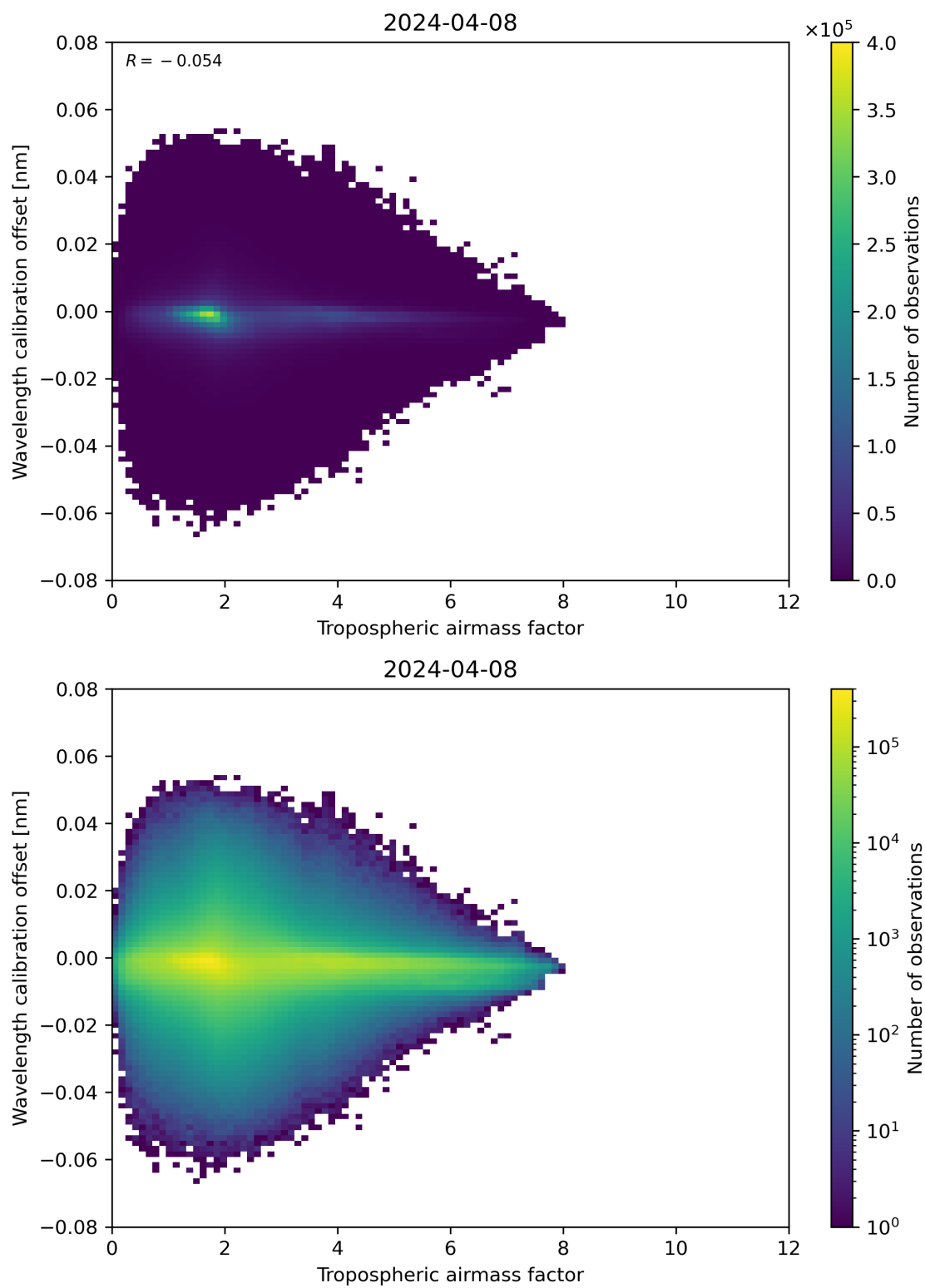
Figure 80: Scatter density plot of “Tropospheric airmass factor” against “Wavelength calibration offset” for 2024-04-07 to 2024-04-09.
