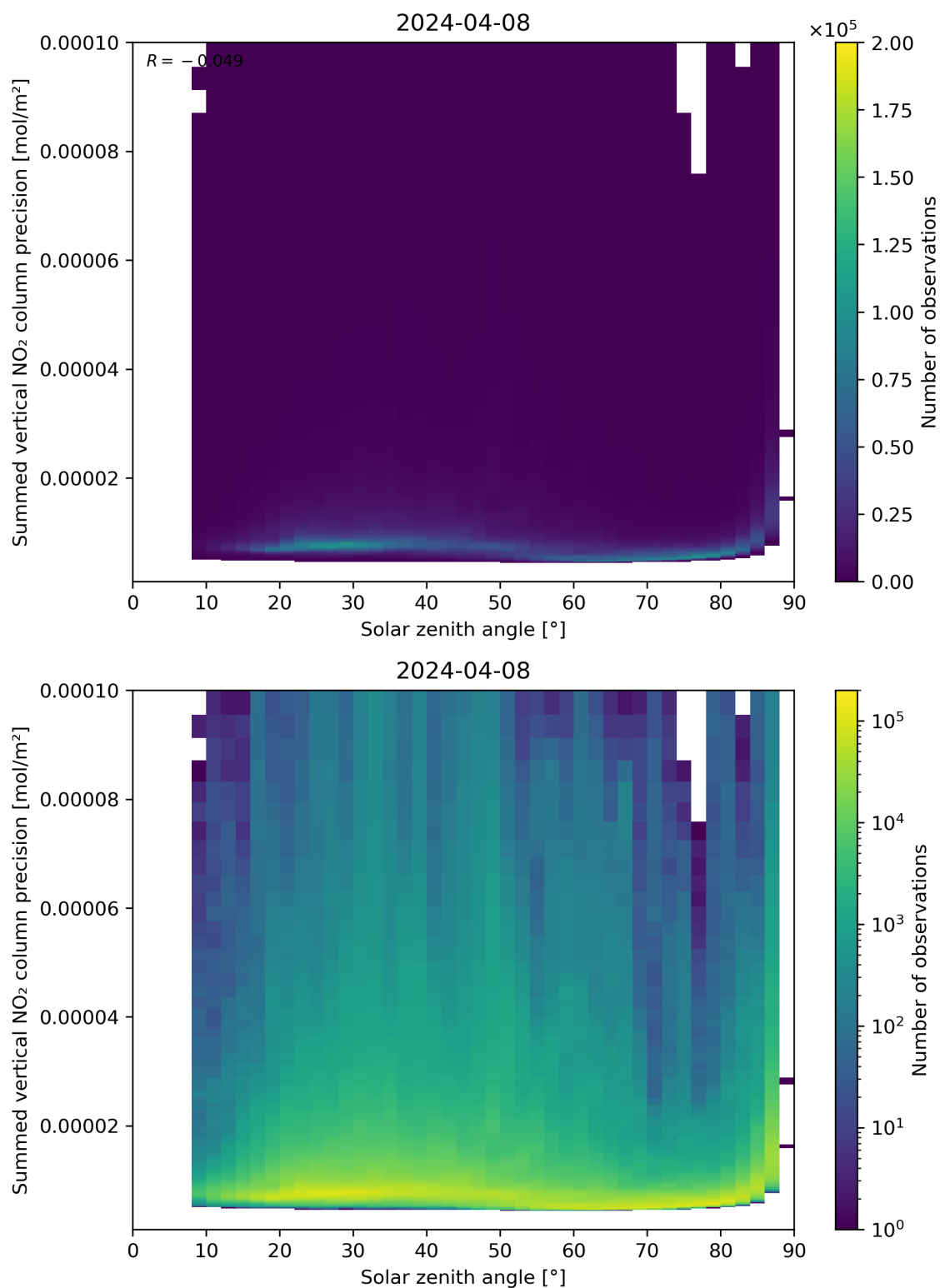
Figure 152: Scatter density plot of “Solar zenith angle” against “Summed vertical NO 2 column precision” for 2024-04-07 to 2024-04-09.
