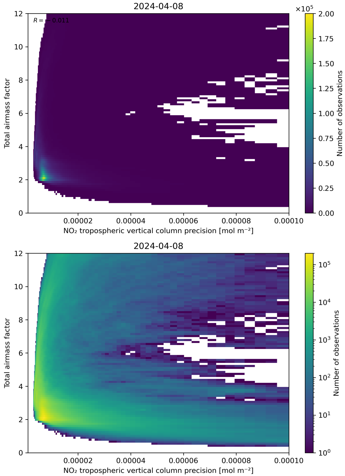
Figure 132: Scatter density plot of “NO 2 tropospheric vertical column precision” against “Total air mass factor” for 2024-04-07 to 2024-04-09.
