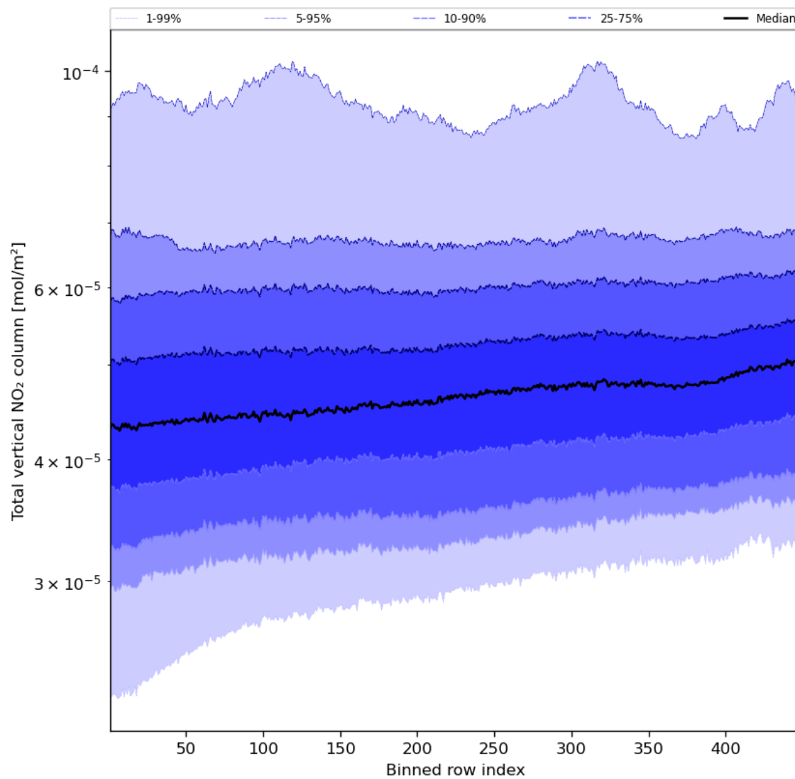
Figure 55: Along track statistics of “Total vertical NO 2 column” for 2024-04-07 to 2024-04-09
