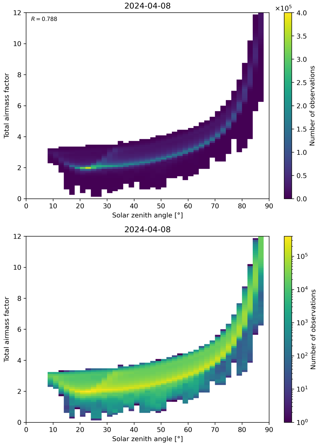
Figure 146: Scatter density plot of “Solar zenith angle” against “Total airmass factor” for 2024-04-07 to 2024-04-09.
