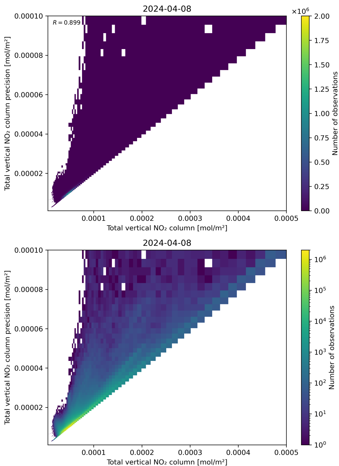
Figure 114: Scatter density plot of “Total vertical NO 2 column” against “Total vertical NO 2 column precision” for 2024-04-07 to 2024-04-09.
