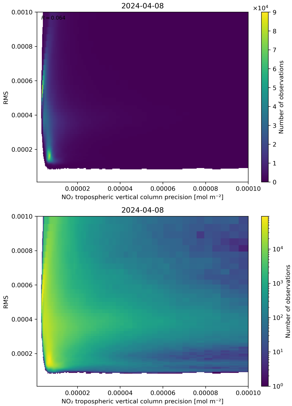
Figure 140: Scatter density plot of “NO 2 tropospheric vertical column precision” against “RMS” for 2024-04-07 to 2024-04-09.
