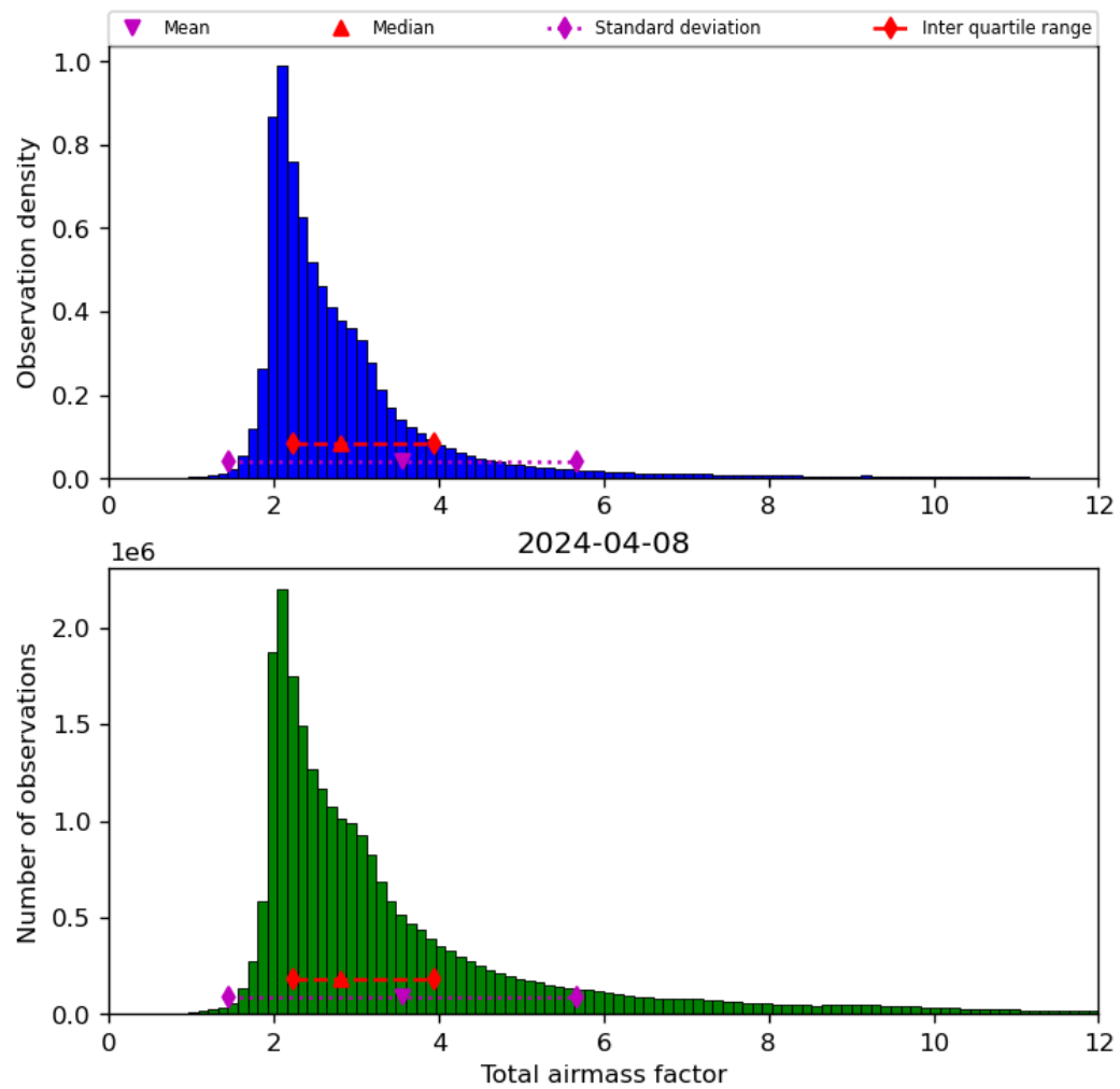
Figure 32: Histogram of “Total airmass factor” for 2024-04-07 to 2024-04-09
