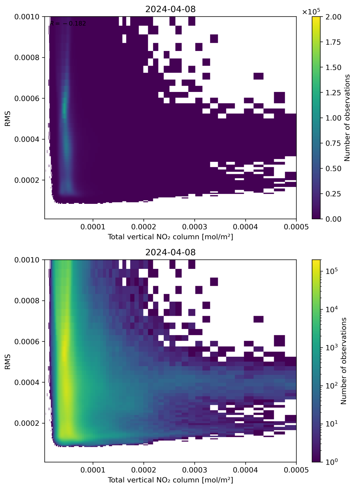
Figure 120: Scatter density plot of “Total vertical NO 2 column” against “RMS” for 2024-04-07 to 2024-04-09.
