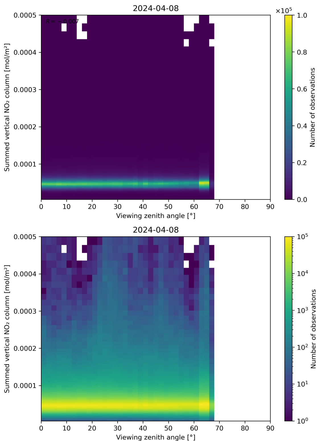
Figure 165: Scatter density plot of “Viewing zenith angle” against “Summed vertical NO 2 column” for 2024-04-07 to 2024-04-09.
