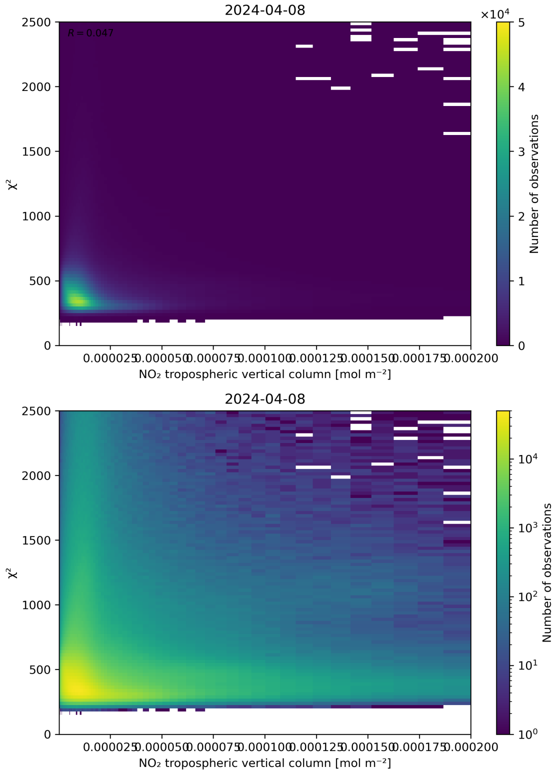
Figure 124: Scatter density plot of “NO 2 tropospheric vertical column” against “ \chi^2 ” for 2024-04-07 to 2024-04-09.
