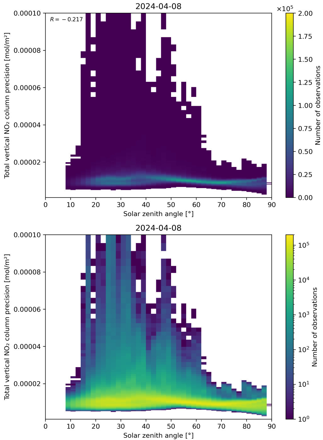
Figure 154: Scatter density plot of “Solar zenith angle” against “Total vertical NO 2 column precision” for 2024-04-07 to 2024-04-09.
