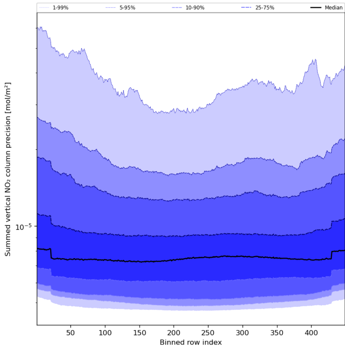
Figure 58: Along track statistics of “Summed vertical NO 2 column precision” for 2024-04-07 to 2024-04-09
