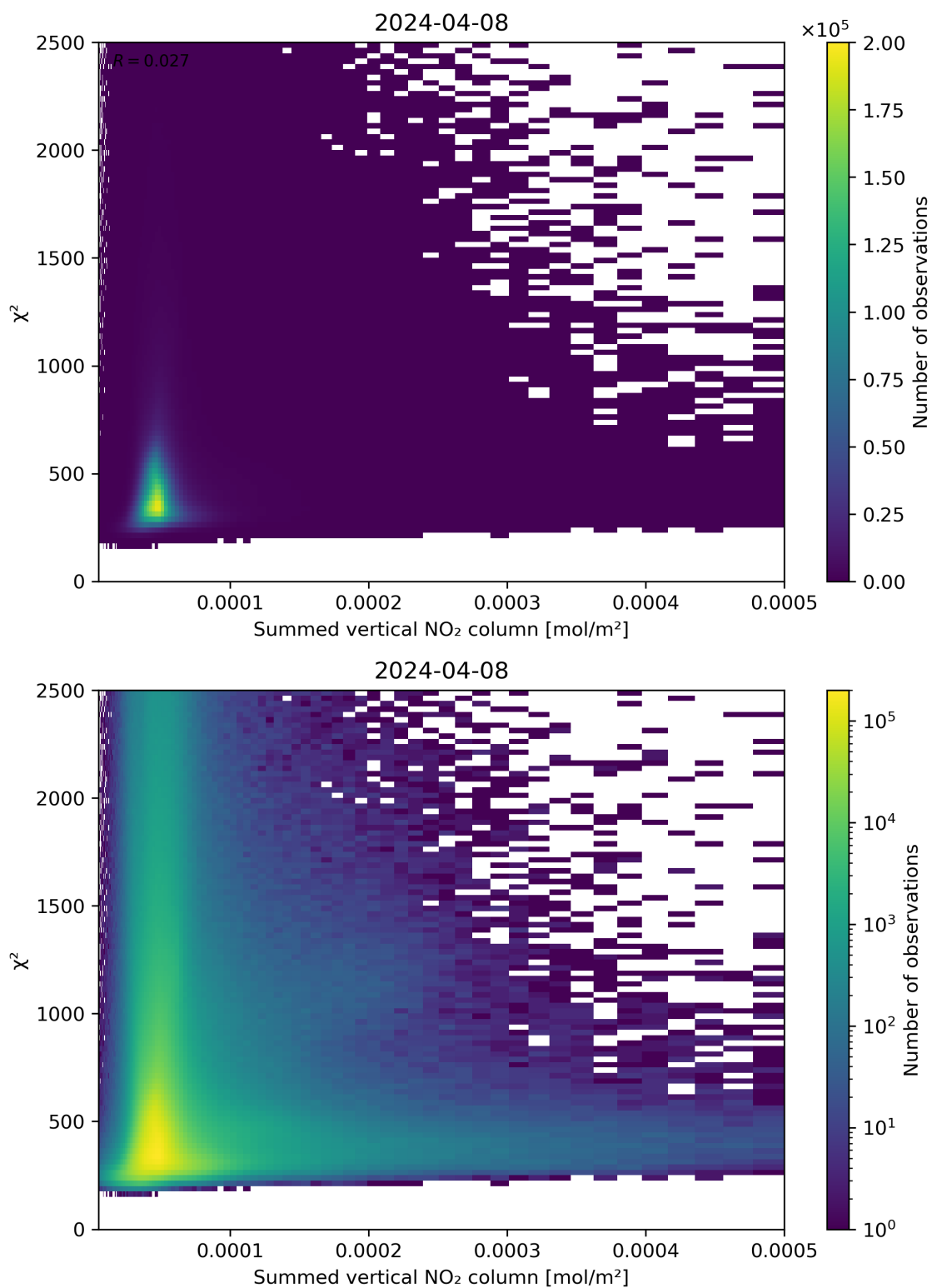
Figure 104: Scatter density plot of “Summed vertical NO 2 column” against “ \chi^2 ” for 2024-04-07 to 2024-04-09.
