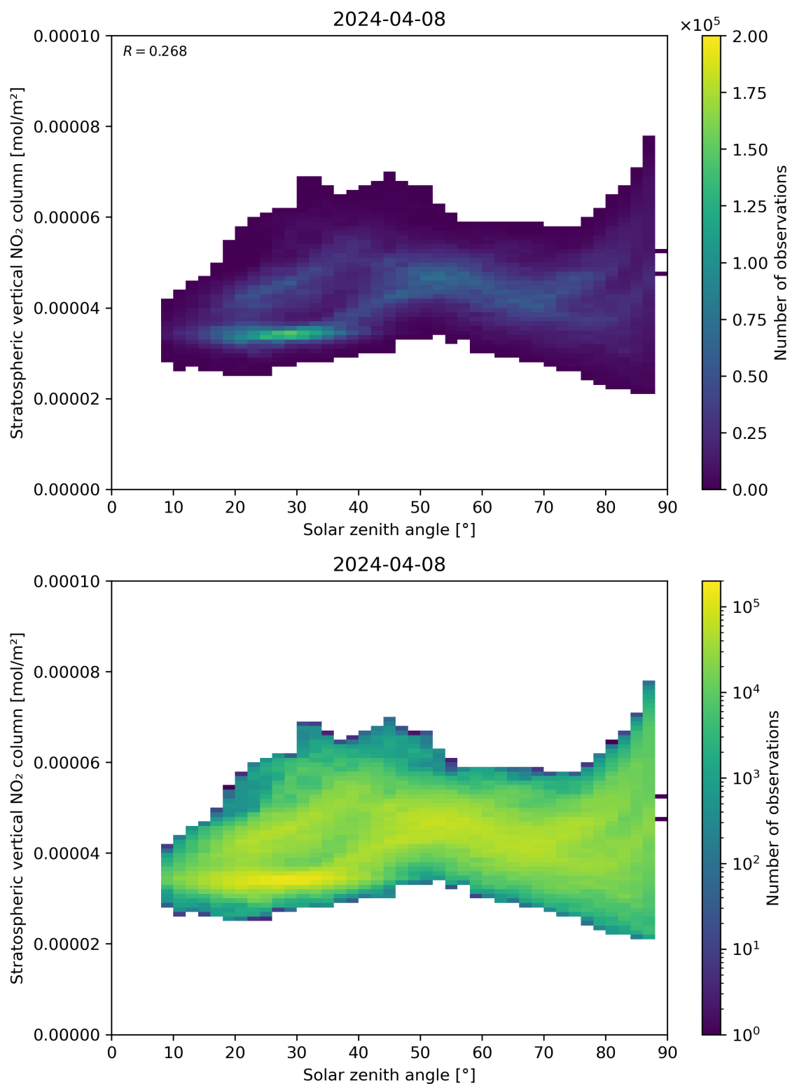
Figure 150: Scatter density plot of “Solar zenith angle” against “Stratospheric vertical NO 2 column” for 2024-04-07 to 2024-04-09.
