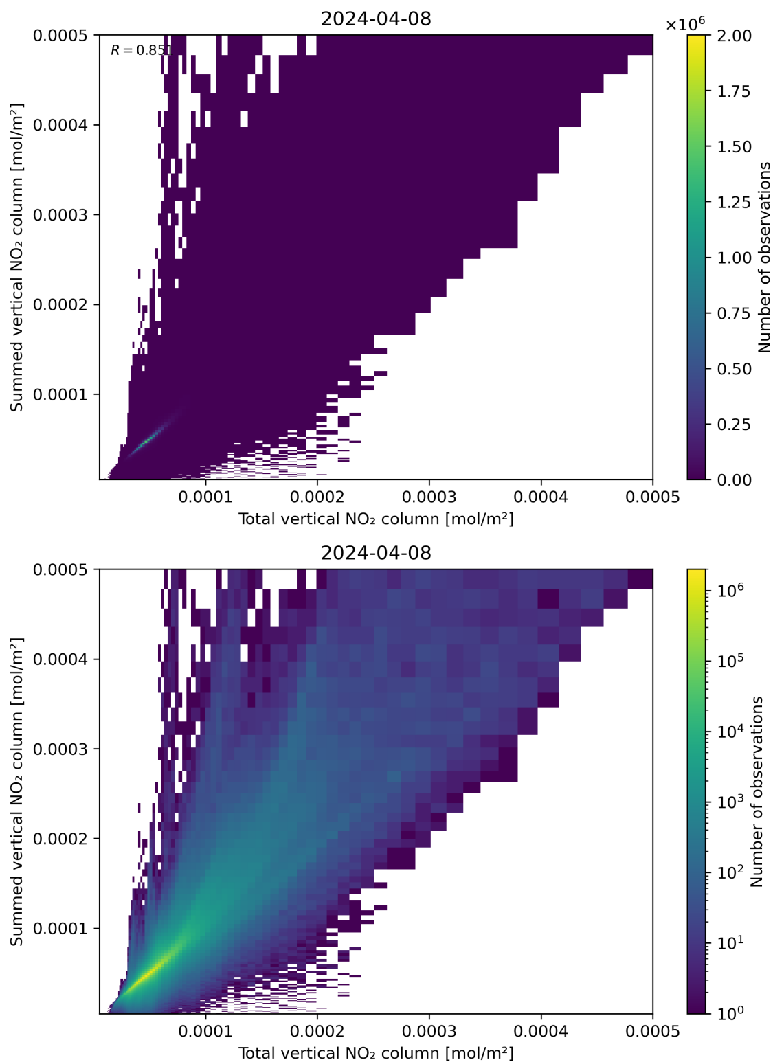
Figure 112: Scatter density plot of “Total vertical NO 2 column” against “Summed vertical NO 2 column” for 2024-04-07 to 2024-04-09.
