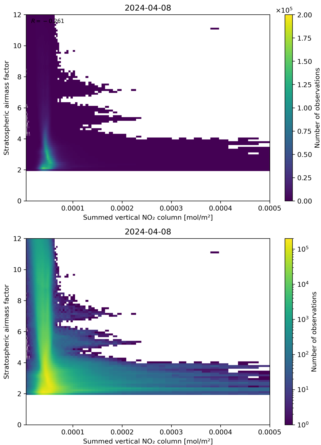
Figure 103: Scatter density plot of “Summed vertical NO 2 column” against “Stratospheric air mass factor” for 2024-04-07 to 2024-04-09.
