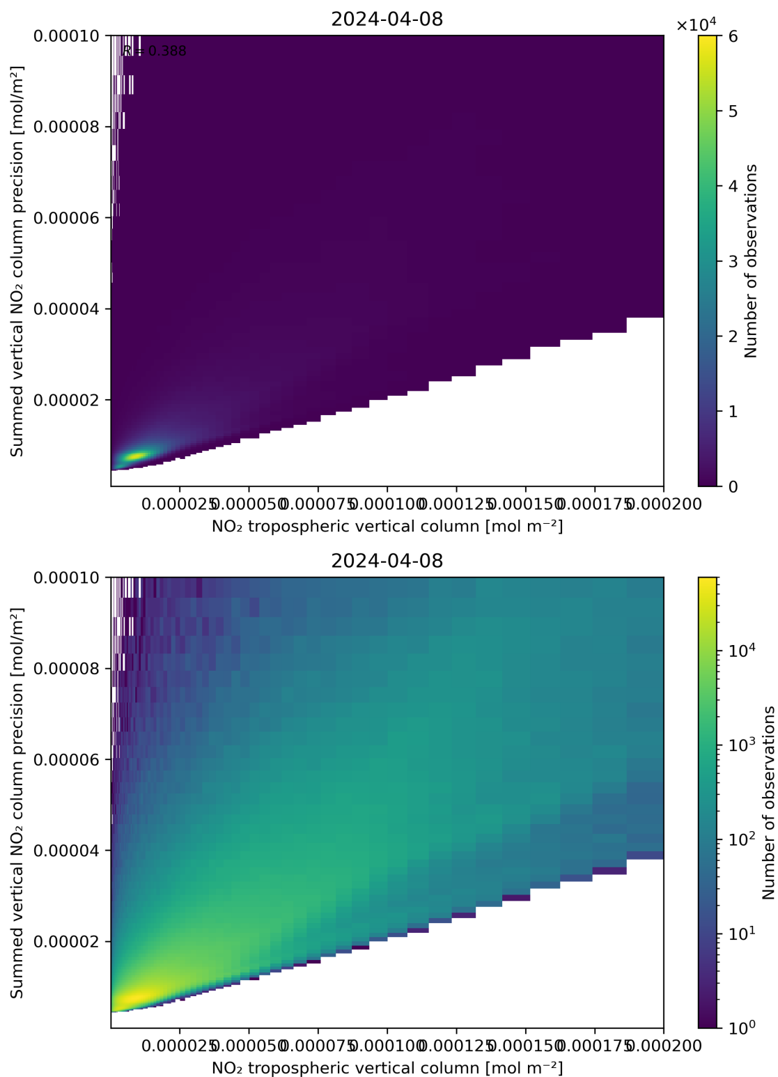
Figure 127: Scatter density plot of “NO 2 tropospheric vertical column” against “Summed vertical NO 2 column precision” for 2024-04-07 to 2024-04-09.
