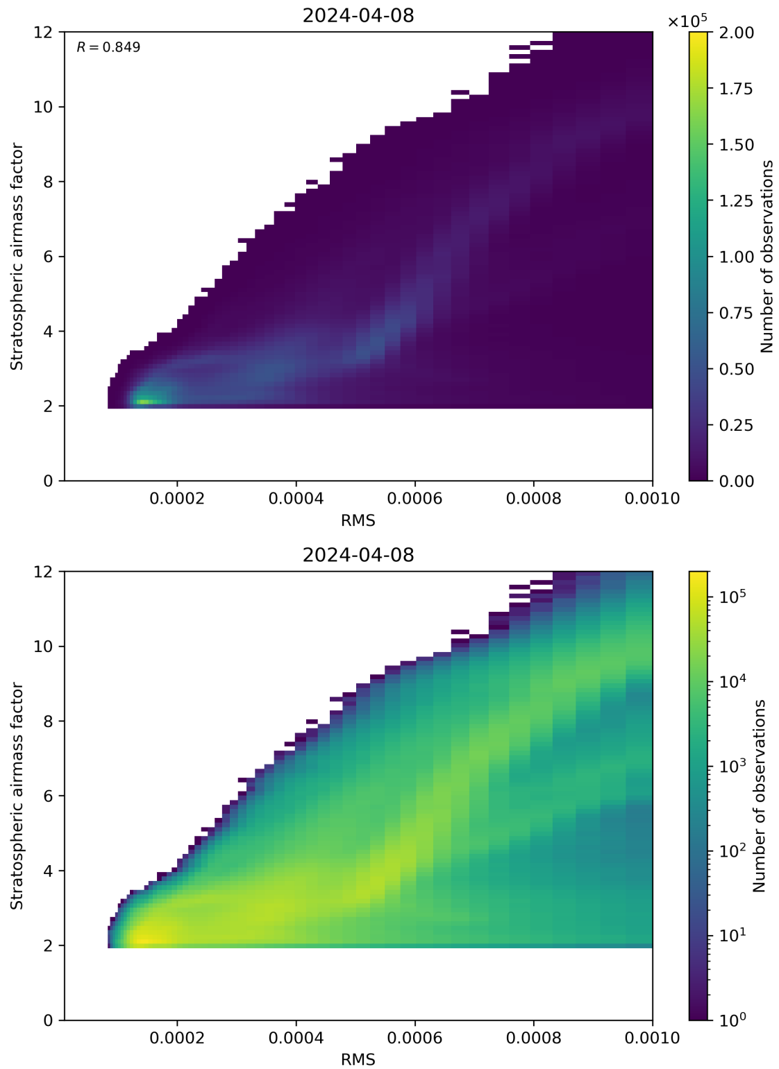
Figure 144: Scatter density plot of “RMS” against “Stratospheric airmass factor” for 2024-04-07 to 2024-04-09.
