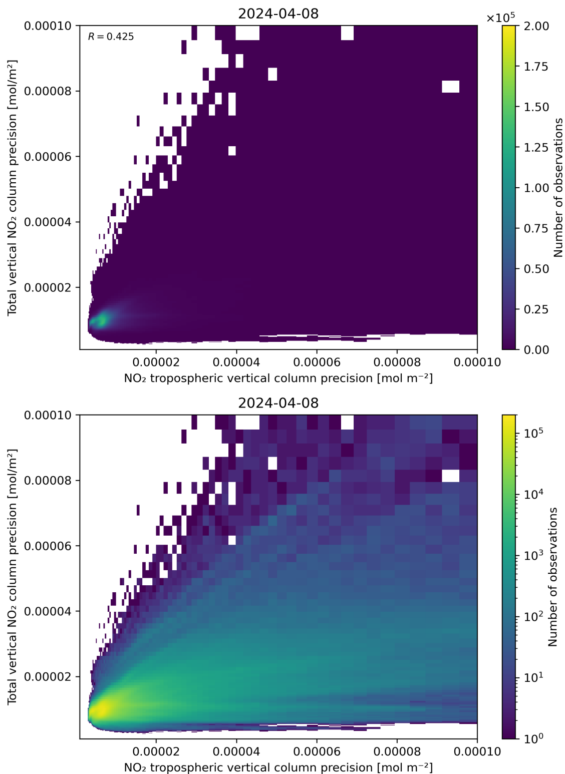
Figure 139: Scatter density plot of “NO 2 tropospheric vertical column precision” against “Total vertical NO 2 column precision” for 2024-04-07 to 2024-04-09.
