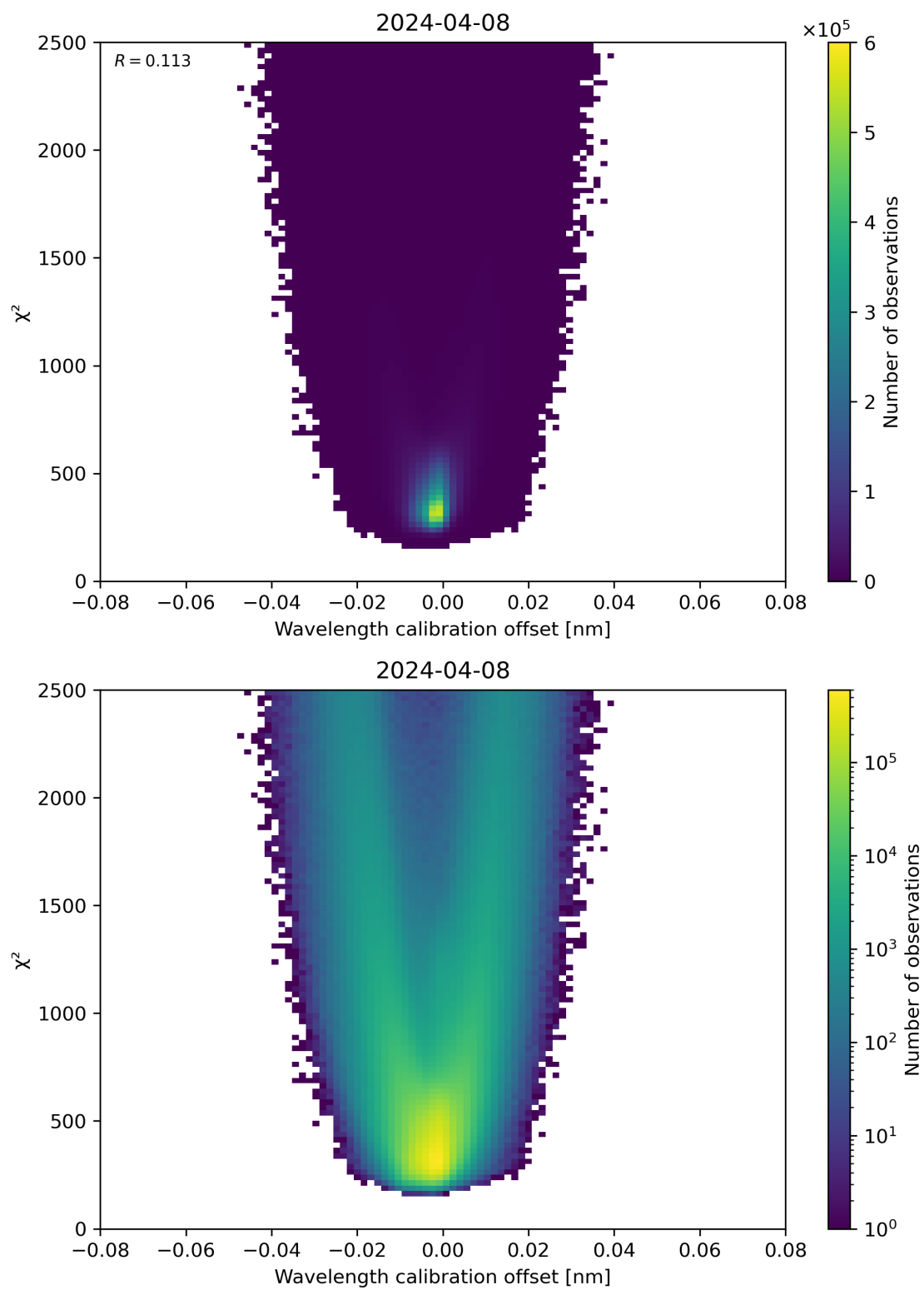
Figure 175: Scatter density plot of “Wavelength calibration offset” against “ \chi^2 ” for 2024-04-07 to 2024-04-09.
