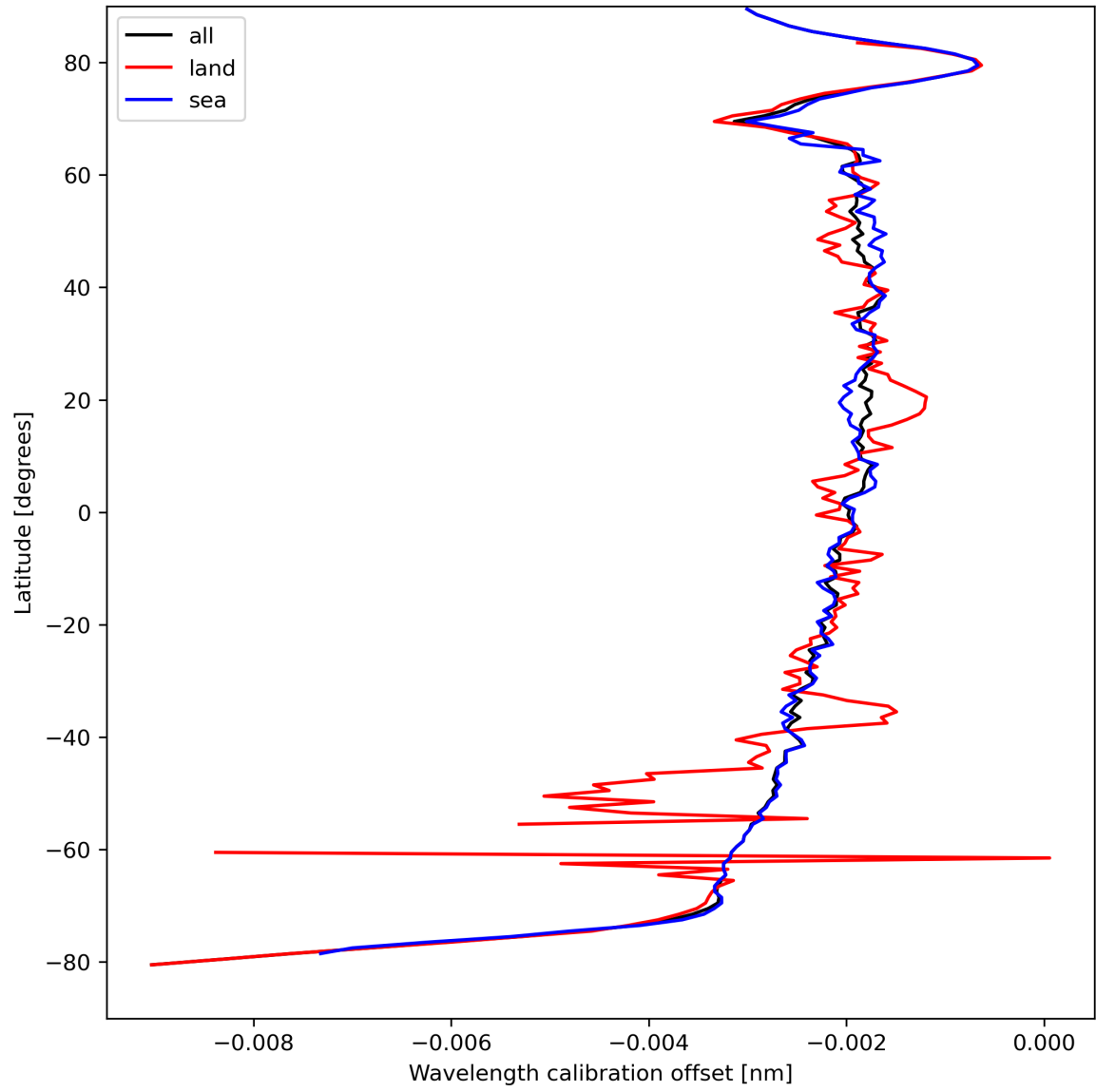
Figure 18: Zonal average of “Wavelength calibration offset” for 2024-04-07 to 2024-04-09.
