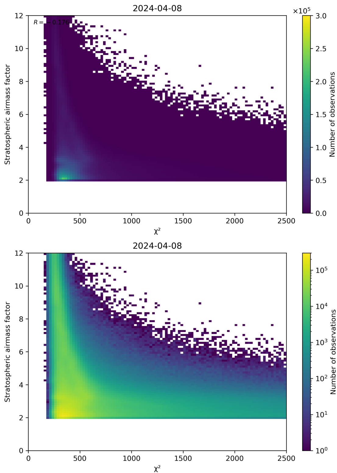
Figure 81: Scatter density plot of “ \chi^2 ” against “Stratospheric airmass factor” for 2024-04-07 to 2024-04-09.
