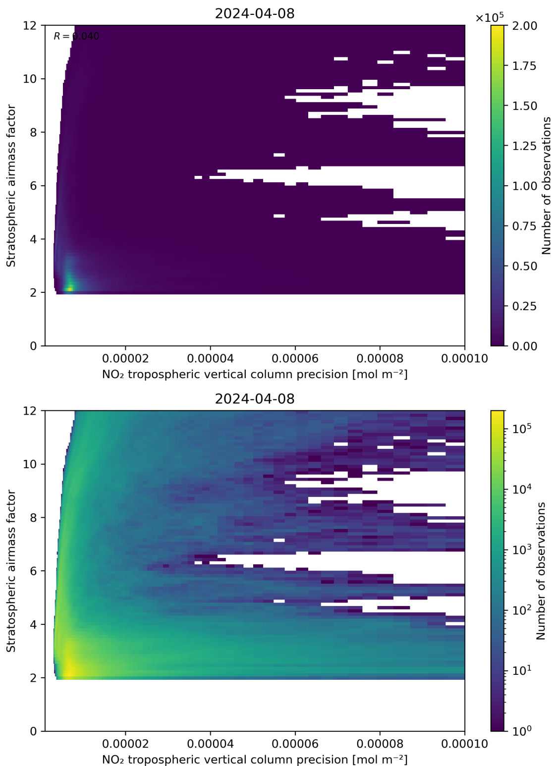
Figure 131: Scatter density plot of “NO 2 tropospheric vertical column precision” against “Stratospheric airmass factor” for 2024-04-07 to 2024-04-09.
