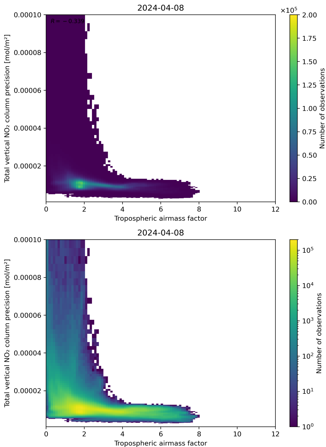
Figure 78: Scatter density plot of “Tropospheric air mass factor” against “Total vertical NO 2 column precision” for 2024-04-07 to 2024-04-09.
