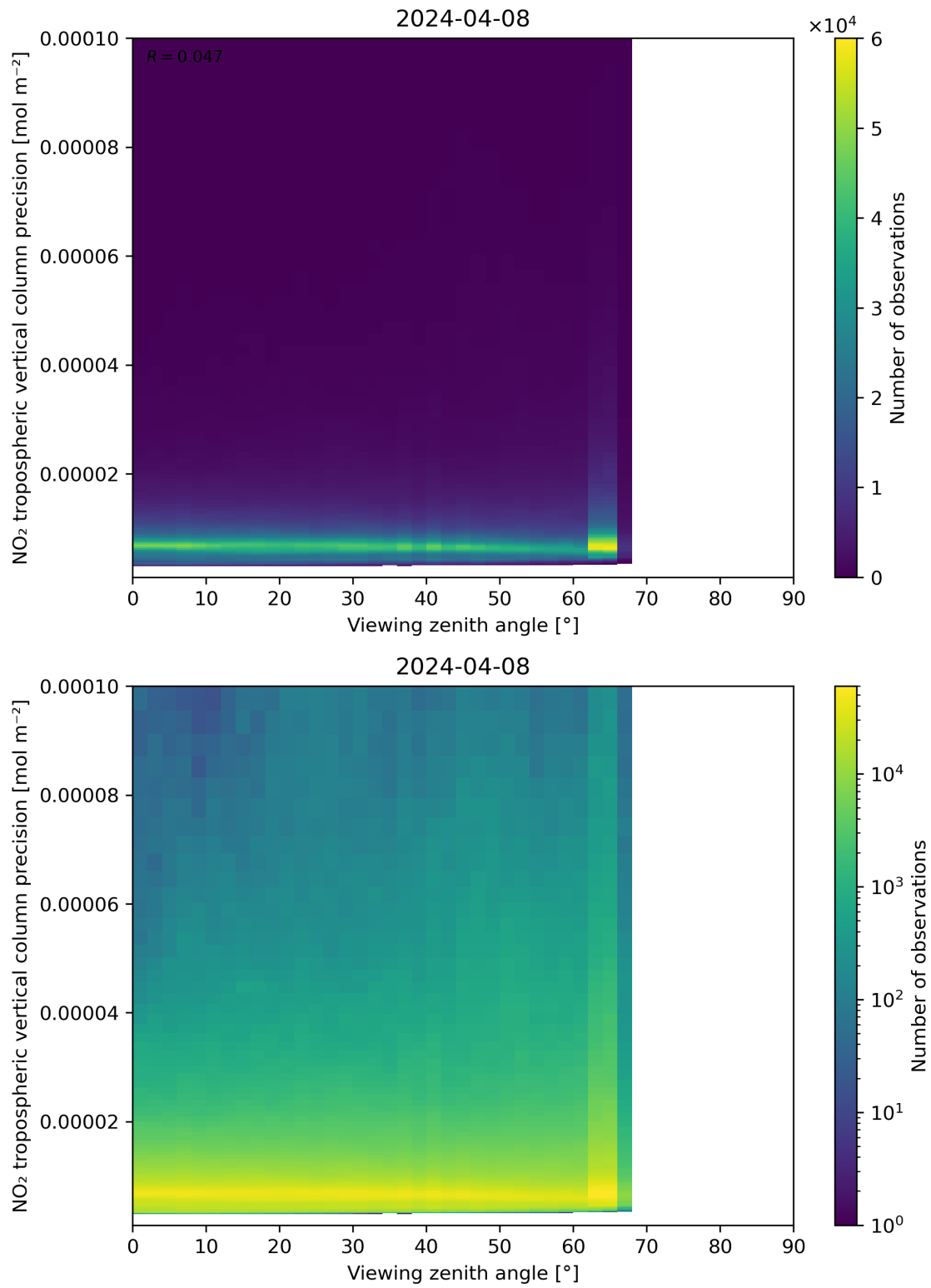
Figure 170: Scatter density plot of “Viewing zenith angle” against “NO 2 tropospheric vertical column precision” for 2024-04-07 to 2024-04-09.
