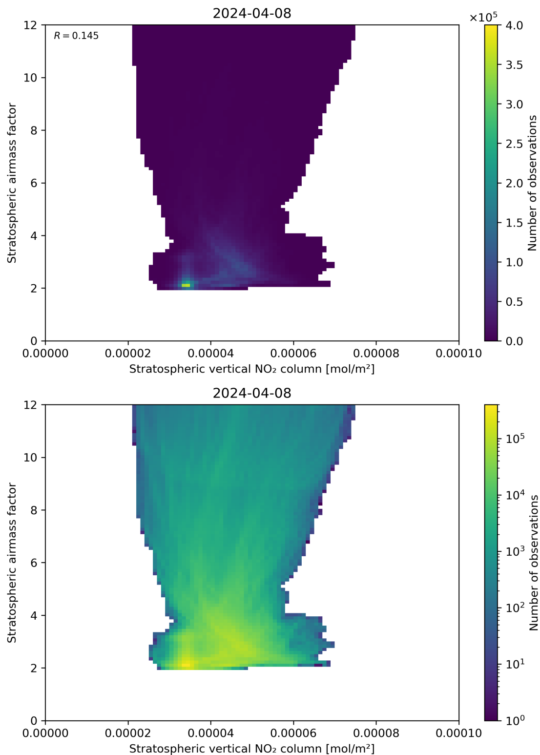
Figure 96: Scatter density plot of “Stratospheric vertical NO 2 column” against “Stratospheric airmass factor” for 2024-04-07 to 2024-04-09.
