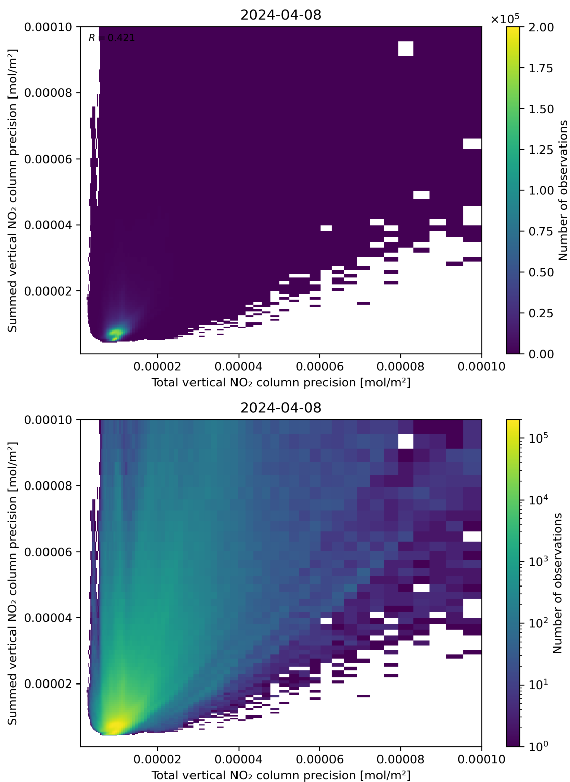
Figure 118: Scatter density plot of “Total vertical NO 2 column precision” against “Summed vertical NO 2 column precision” for 2024-04-07 to 2024-04-09.
