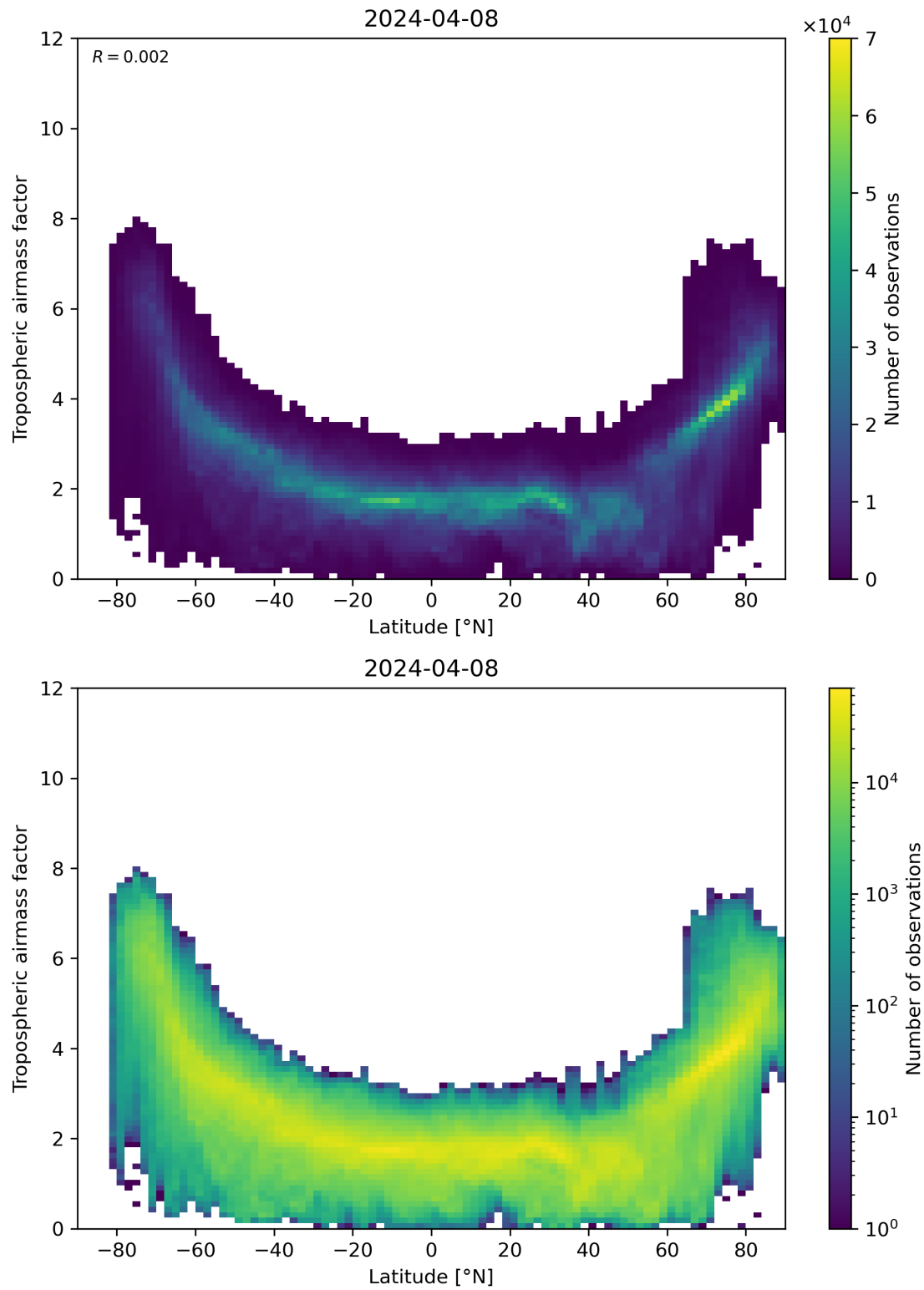
Figure 85: Scatter density plot of “Latitude” against “Tropospheric air mass factor” for 2024-04-07 to 2024-04-09.
