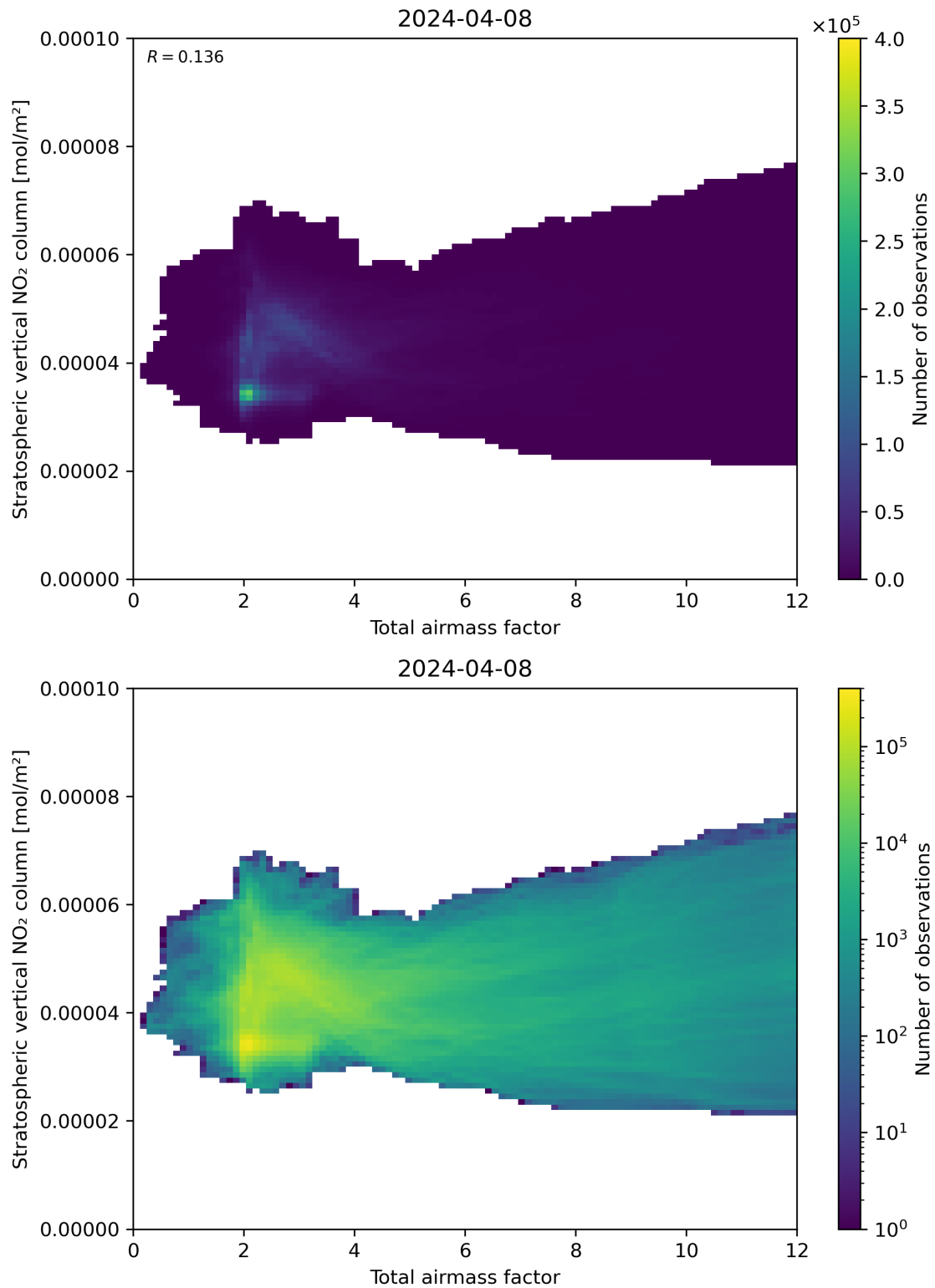
Figure 64: Scatter density plot of “Total airmass factor” against “Stratospheric vertical \text{NO}_2 column” for 2024-04-07 to 2024-04-09.
