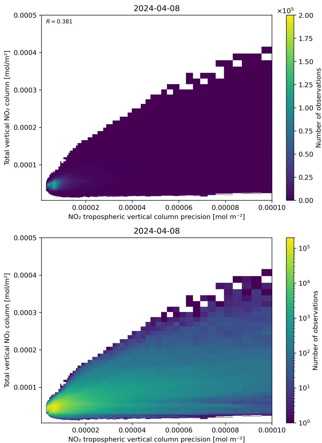
Figure 138: Scatter density plot of “NO 2 tropospheric vertical column precision” against “Total vertical NO 2 column” for 2024-04-07 to 2024-04-09.
