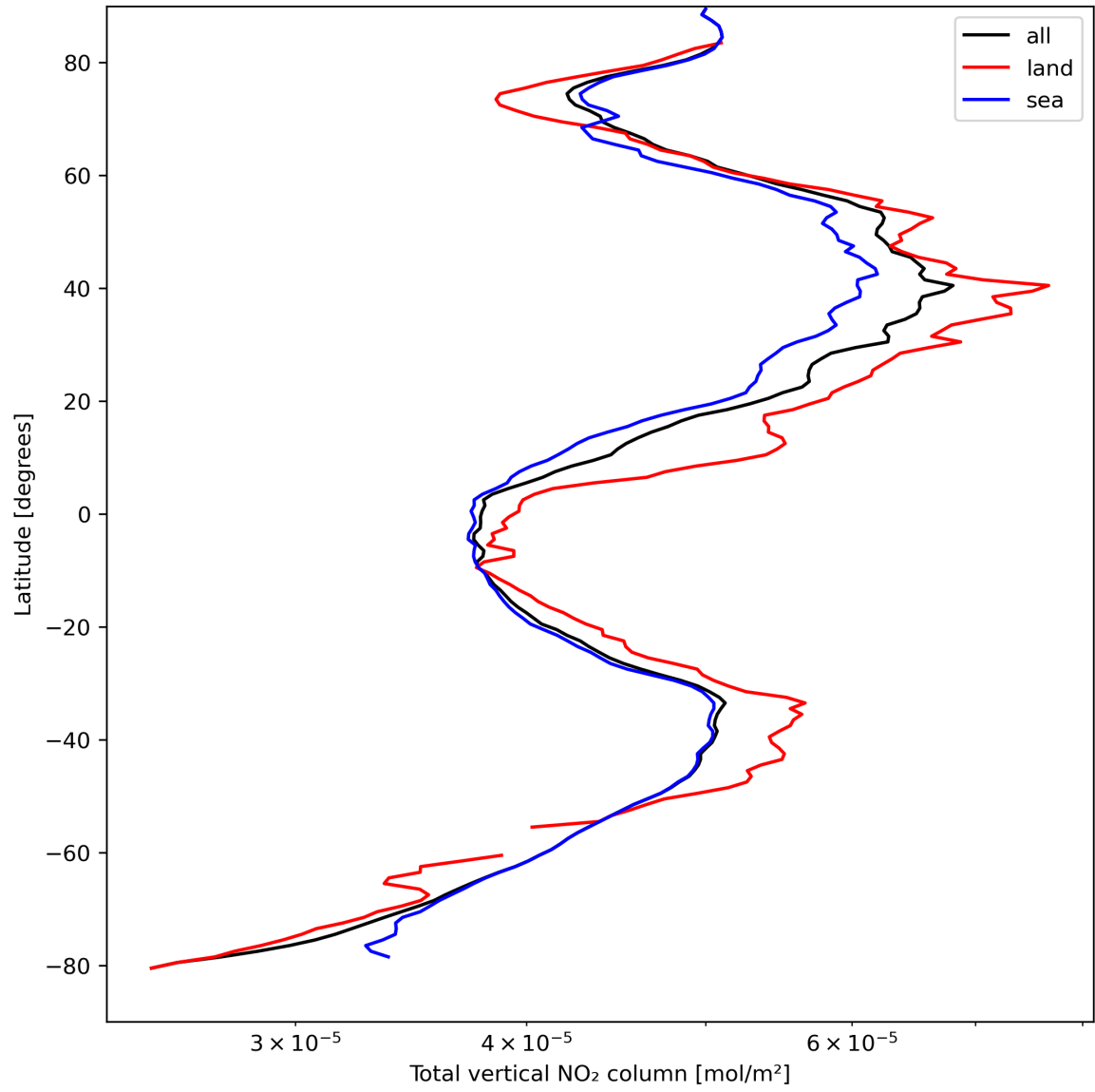
Figure 21: Zonal average of “Total vertical NO 2 column” for 2024-04-07 to 2024-04-09.
