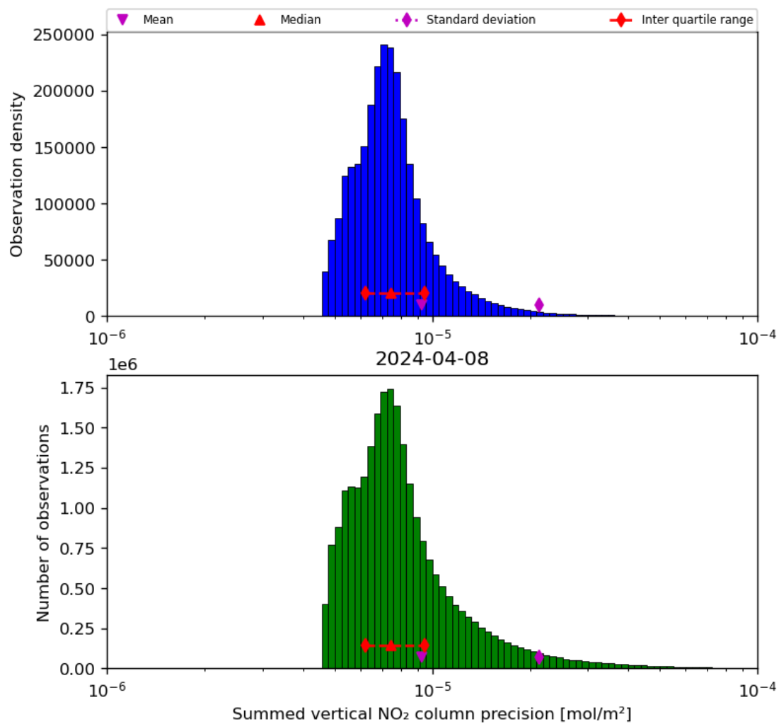
Figure 41: Histogram of “Summed vertical NO 2 column precision” for 2024-04-07 to 2024-04-09
