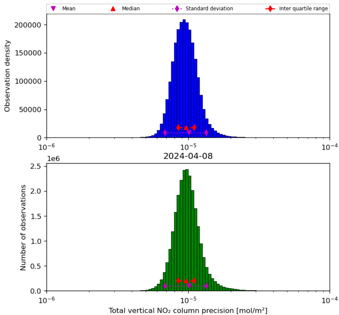
Figure 39: Histogram of “Total vertical NO 2 column precision” for 2024-04-07 to 2024-04-09
