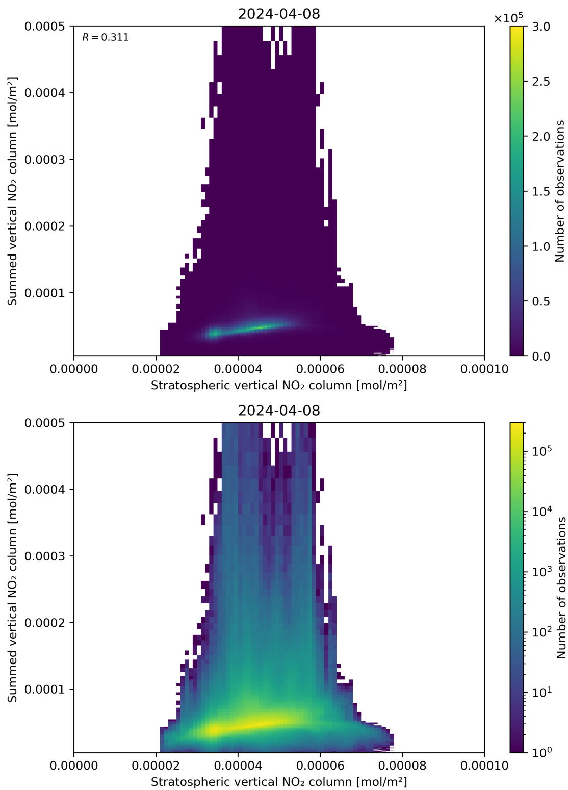
Figure 98: Scatter density plot of “Stratospheric vertical NO 2 column” against “Summed vertical NO 2 column” for 2024-04-07 to 2024-04-09.
