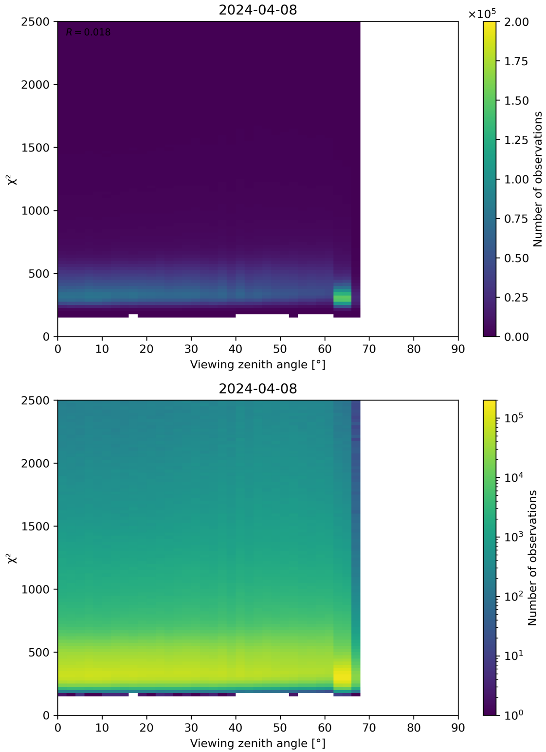
Figure 162: Scatter density plot of “Viewing zenith angle” against “ \chi^2 ” for 2024-04-07 to 2024-04-09.
