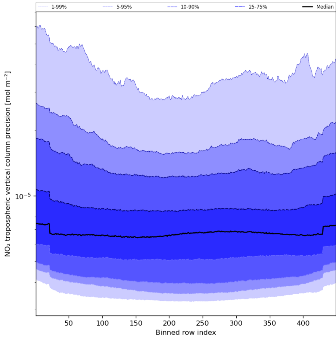
Figure 47: Along track statistics of “NO 2 tropospheric vertical column precision” for 2024-04-07 to 2024-04-09
