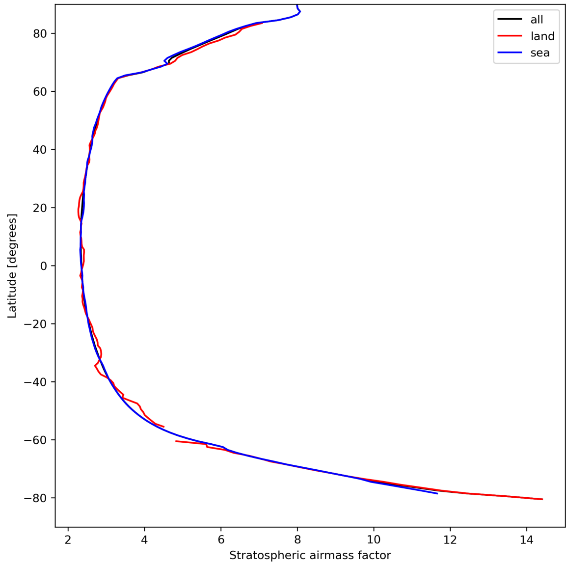
Figure 27: Zonal average of “Stratospheric air mass factor” for 2024-04-07 to 2024-04-09.
