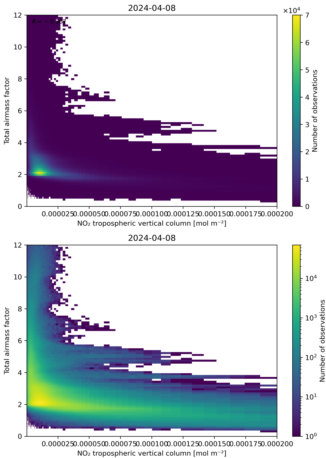
Figure 122: Scatter density plot of “NO 2 tropospheric vertical column” against “Total air mass factor” for 2024-04-07 to 2024-04-09.
