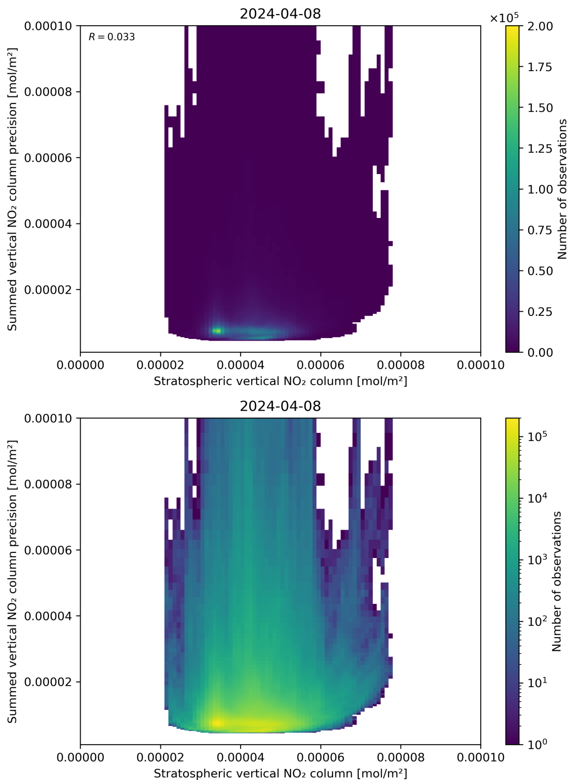
Figure 99: Scatter density plot of “Stratospheric vertical NO 2 column” against “Summed vertical NO 2 column precision” for 2024-04-07 to 2024-04-09.
