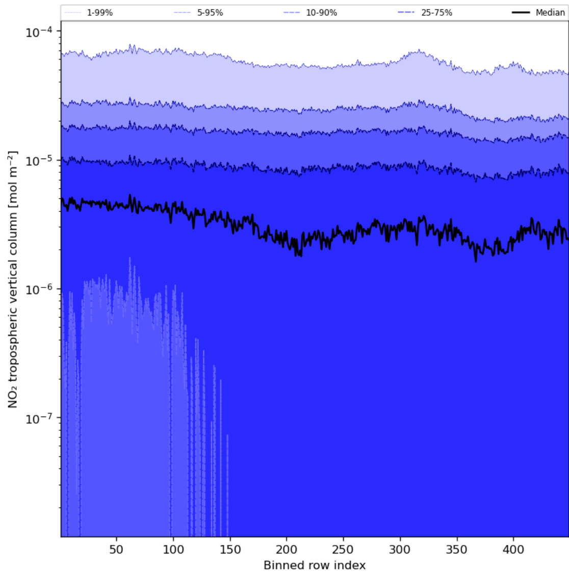
Figure 46: Along track statistics of “NO 2 tropospheric vertical column” for 2024-04-07 to 2024-04-09
