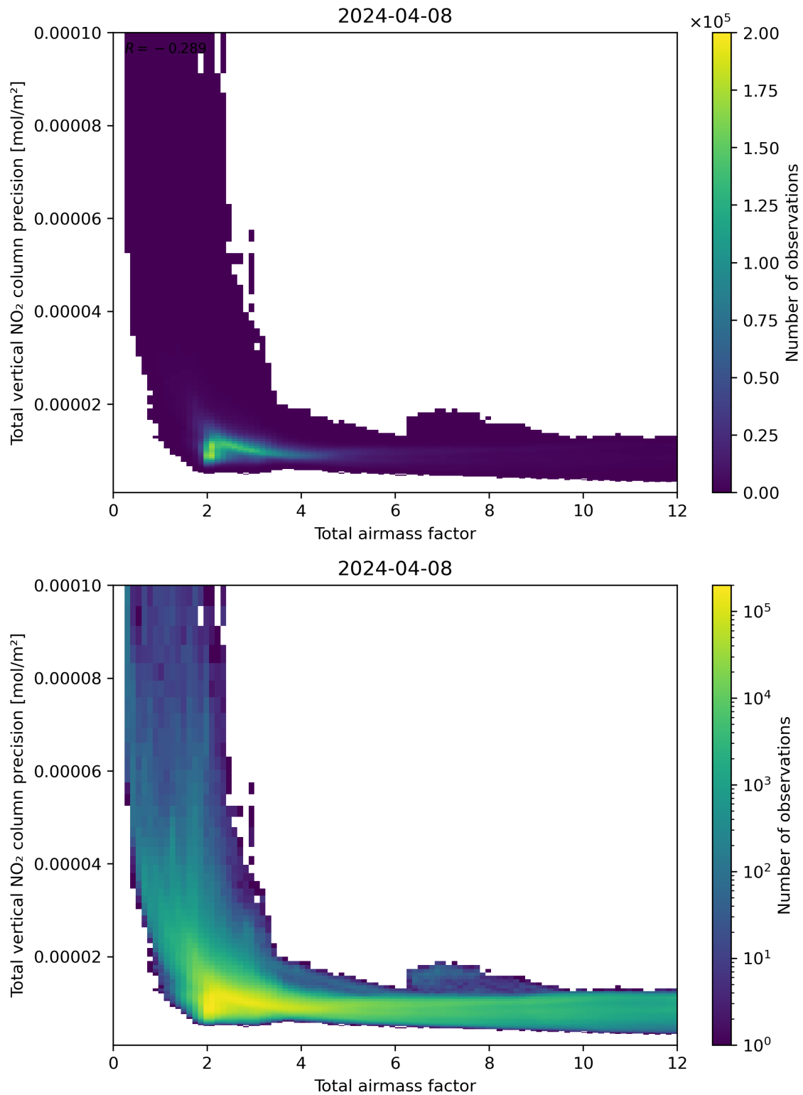
Figure 68: Scatter density plot of “Total airmass factor” against “Total vertical NO 2 column precision” for 2024-04-07 to 2024-04-09.
