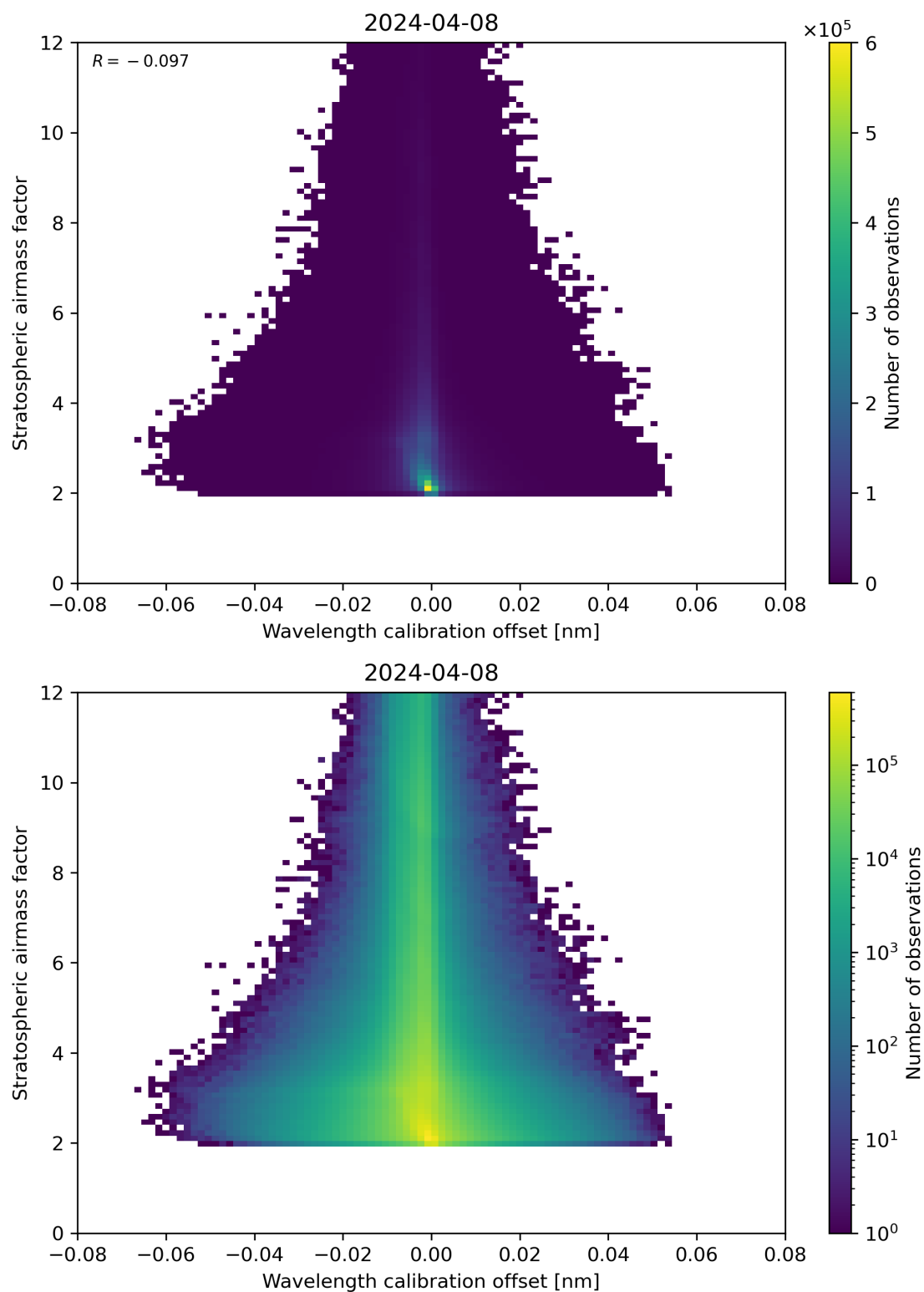
Figure 174: Scatter density plot of “Wavelength calibration offset” against “Stratospheric air mass factor” for 2024-04-07 to 2024-04-09.
