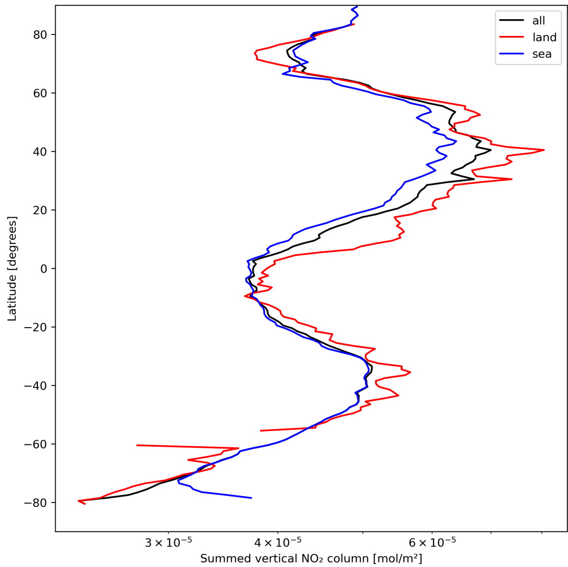
Figure 23: Zonal average of “Summed vertical NO 2 column” for 2024-04-07 to 2024-04-09.
