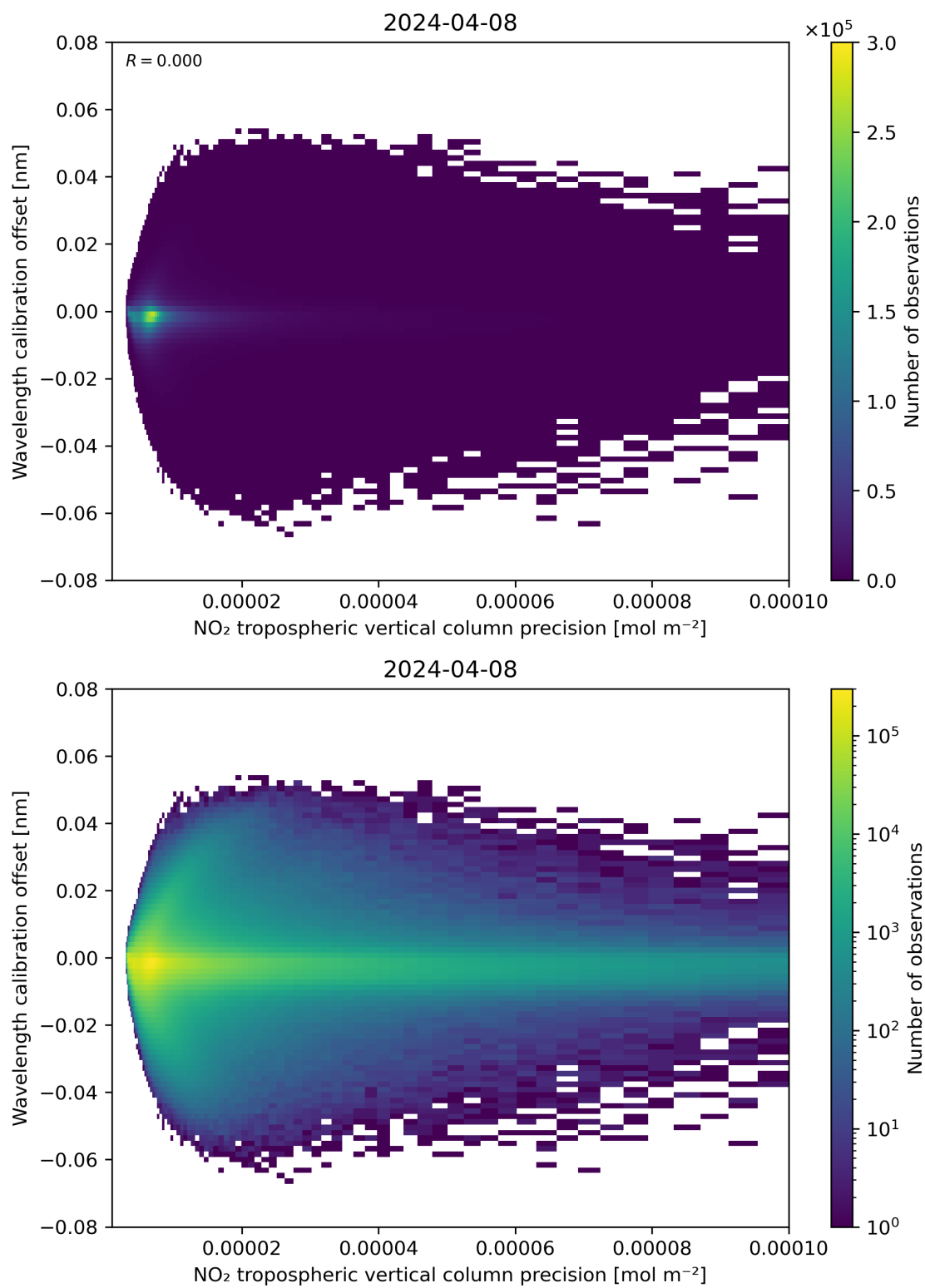
Figure 141: Scatter density plot of “NO 2 tropospheric vertical column precision” against “Wavelength calibration offset” for 2024-04-07 to 2024-04-09.
