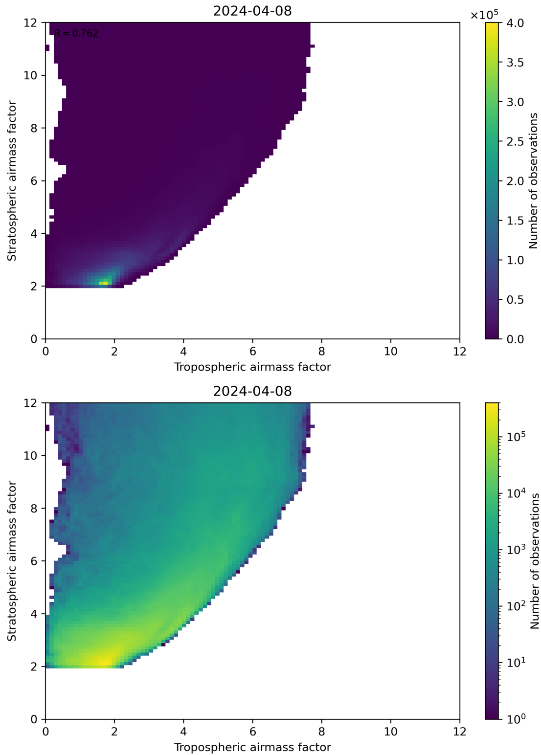
Figure 71: Scatter density plot of “Tropospheric airmass factor” against “Stratospheric airmass factor” for 2024-04-07 to 2024-04-09.
