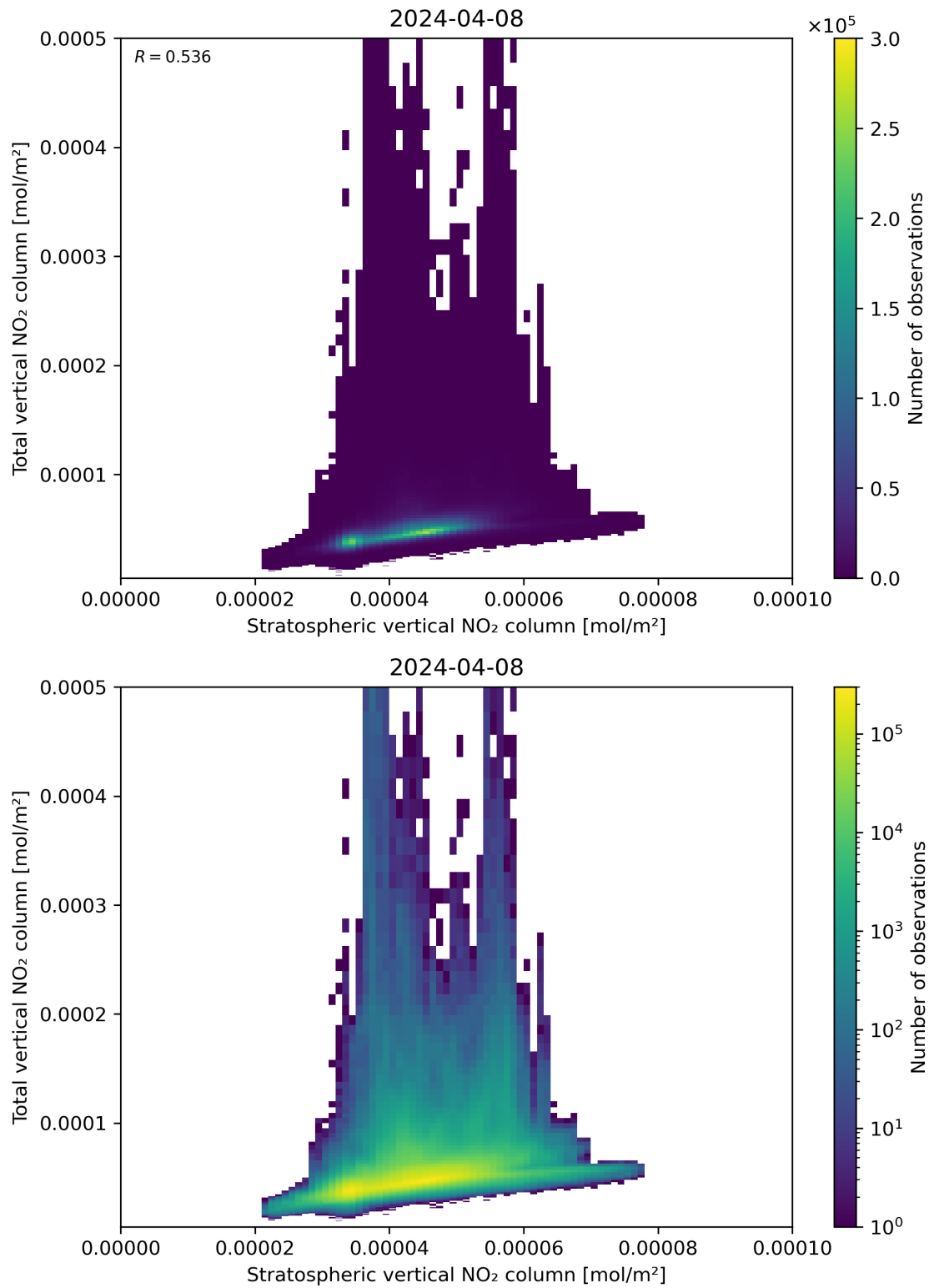
Figure 100: Scatter density plot of “Stratospheric vertical NO 2 column” against “Total vertical NO 2 column” for 2024-04-07 to 2024-04-09.
