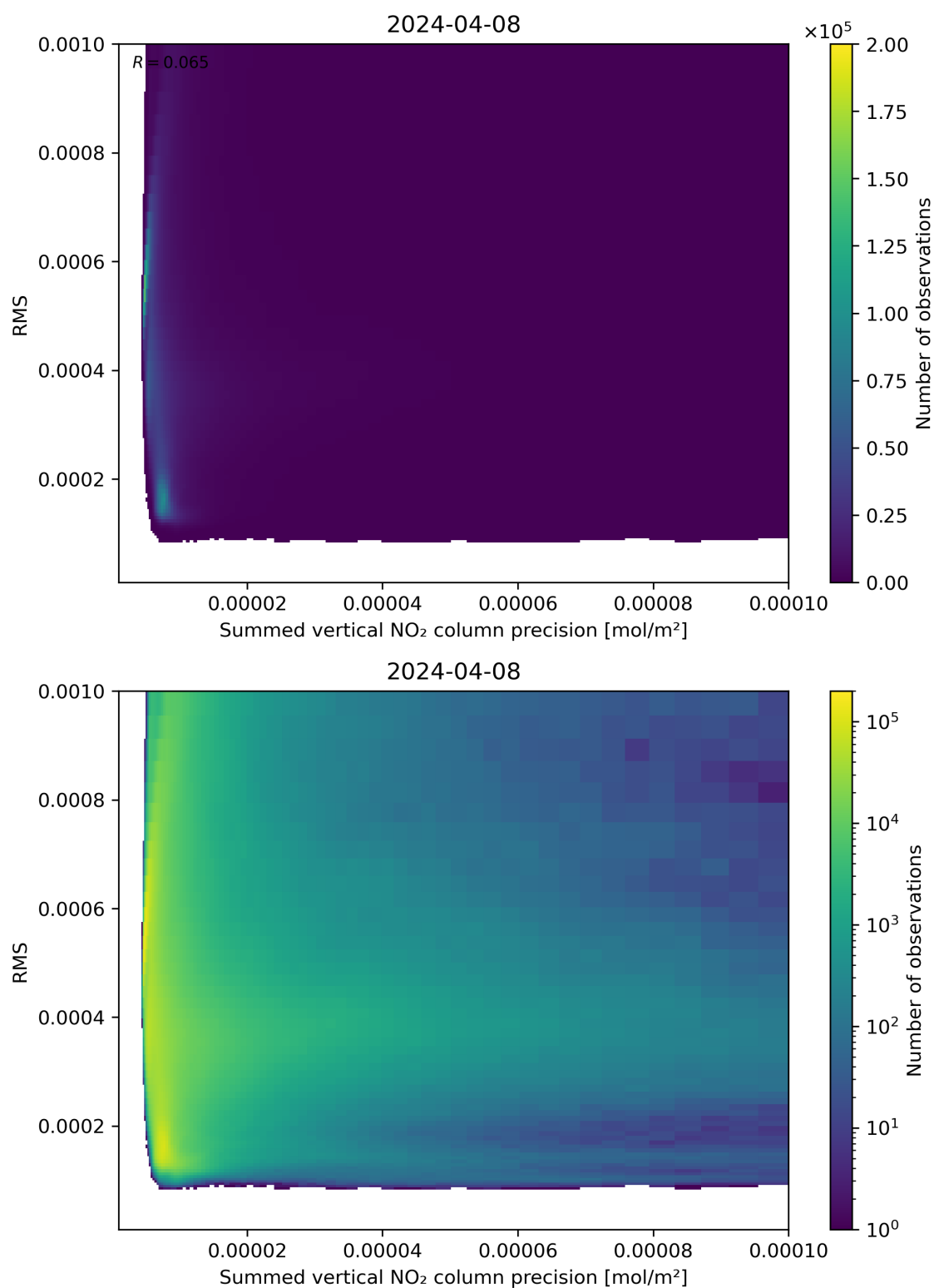
Figure 108: Scatter density plot of “Summed vertical NO 2 column precision” against “RMS” for 2024-04-07 to 2024-04-09.
