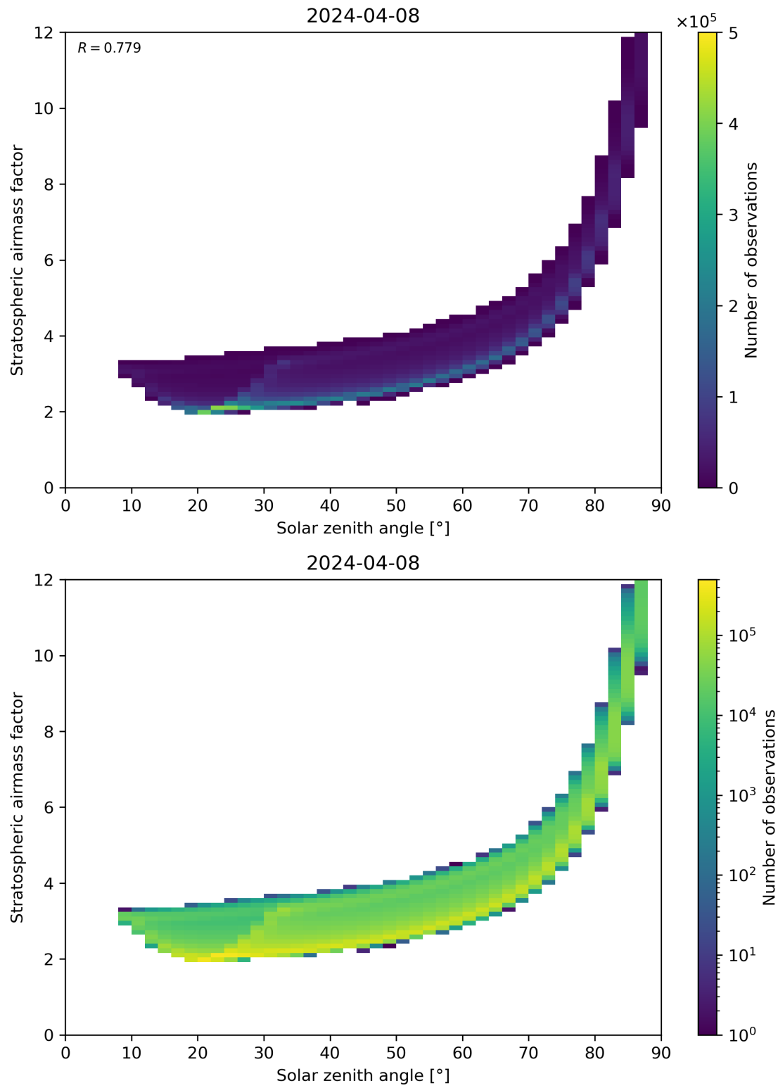
Figure 145: Scatter density plot of “Solar zenith angle” against “Stratospheric airmass factor” for 2024-04-07 to 2024-04-09.
