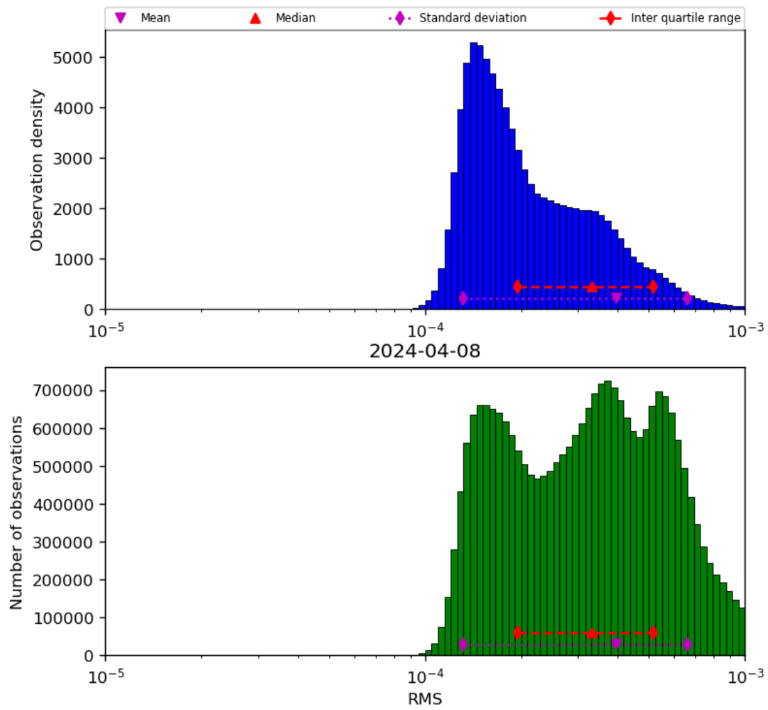
Figure 43: Histogram of “RMS” for 2024-04-07 to 2024-04-09
