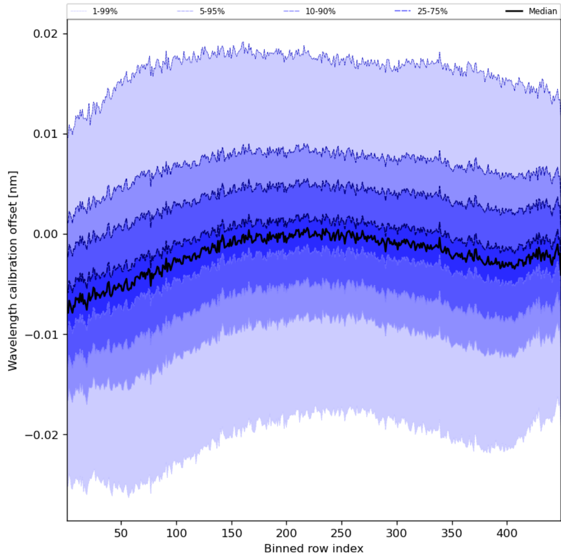
Figure 52: Along track statistics of “Wavelength calibration offset” for 2024-04-07 to 2024-04-09
