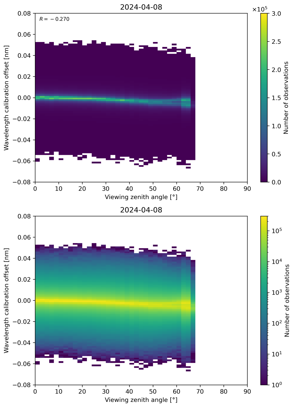
Figure 173: Scatter density plot of “Viewing zenith angle” against “Wavelength calibration offset” for 2024-04-07 to 2024-04-09.
