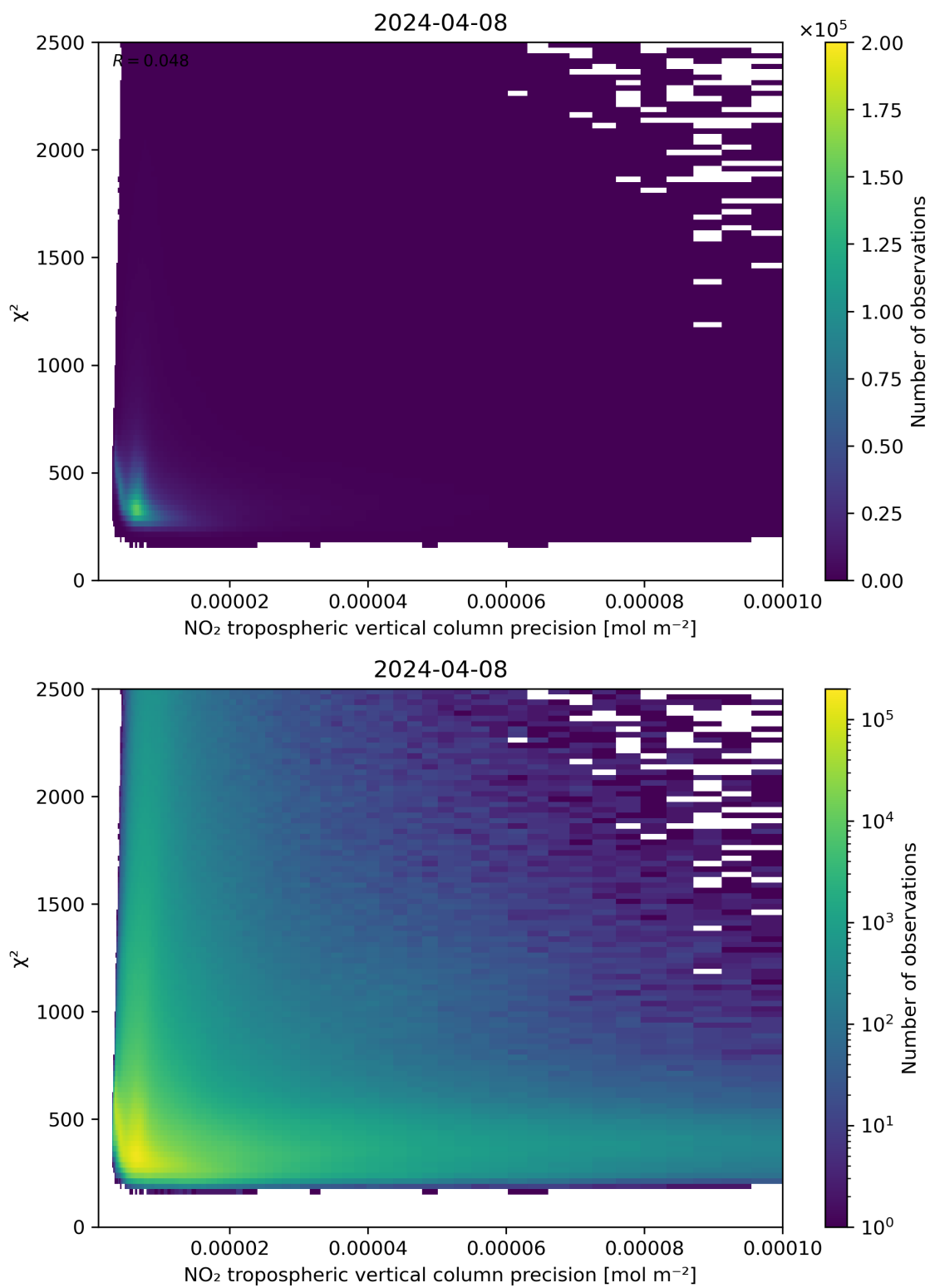
Figure 134: Scatter density plot of “NO 2 tropospheric vertical column precision” against “ \chi^2 ” for 2024-04-07 to 2024-04-09.
