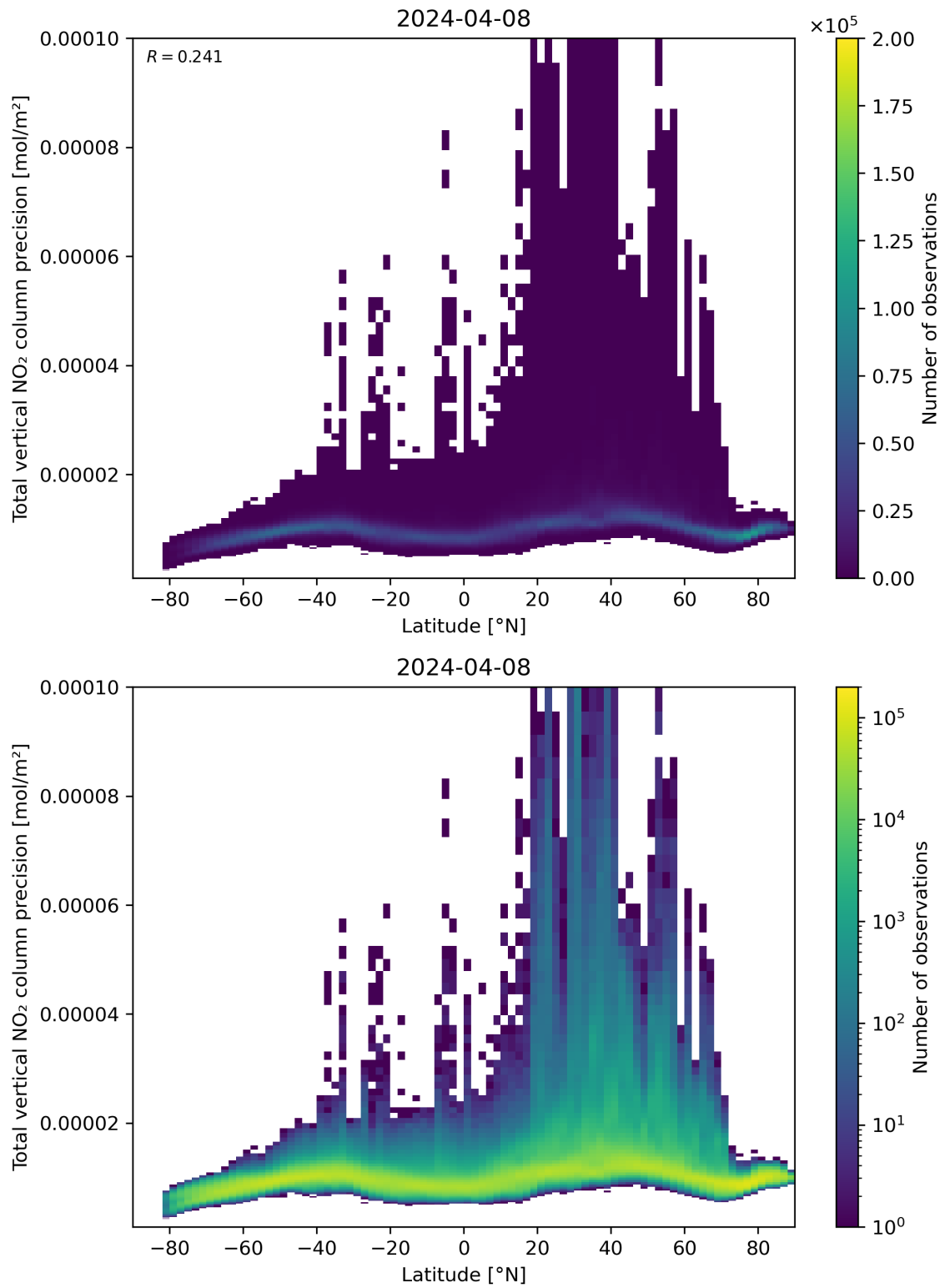
Figure 91: Scatter density plot of “Latitude” against “Total vertical NO 2 column precision” for 2024-04-07 to 2024-04-09.
