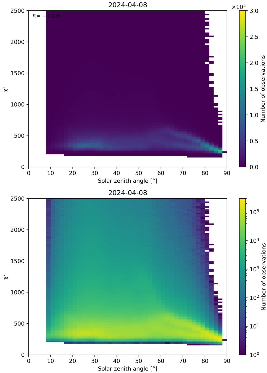
Figure 148: Scatter density plot of “Solar zenith angle” against “ \chi^2 ” for 2024-04-07 to 2024-04-09.
