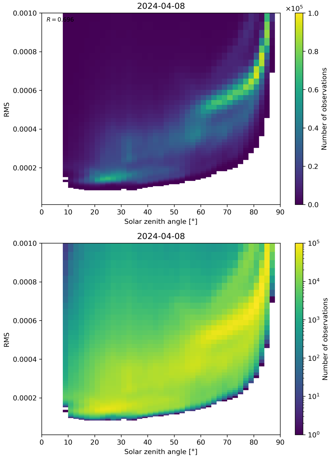
Figure 157: Scatter density plot of “Solar zenith angle” against “RMS” for 2024-04-07 to 2024-04-09.
