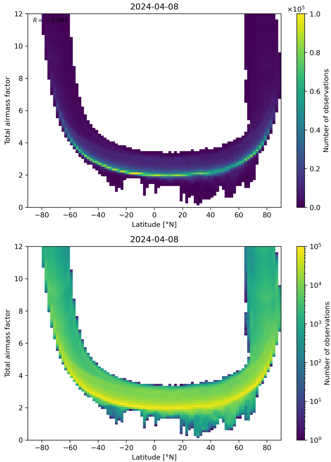
Figure 84: Scatter density plot of “Latitude” against “Total airmass factor” for 2024-04-07 to 2024-04-09.
