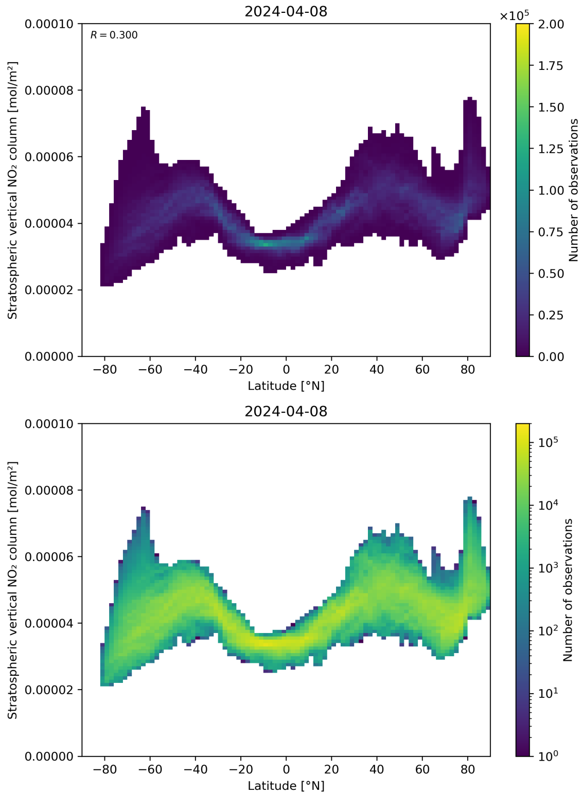
Figure 87: Scatter density plot of “Latitude” against “Stratospheric vertical NO 2 column” for 2024-04-07 to 2024-04-09.
