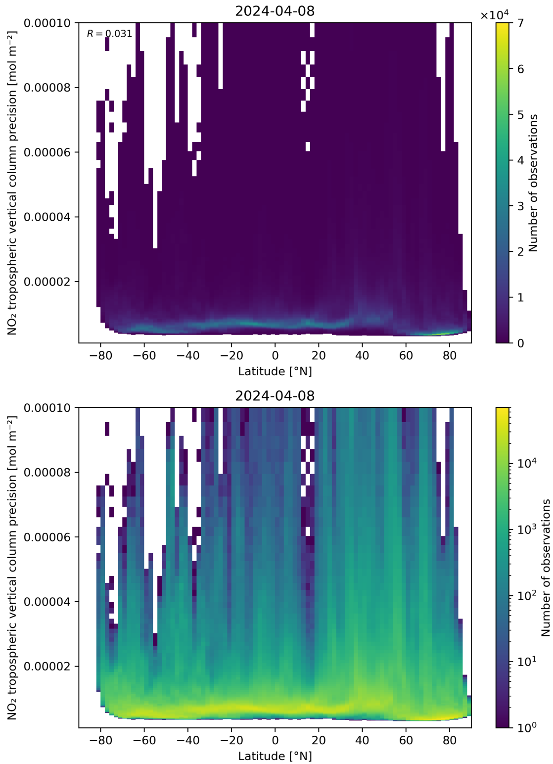
Figure 93: Scatter density plot of “Latitude” against “NO 2 tropospheric vertical column precision” for 2024-04-07 to 2024-04-09.
