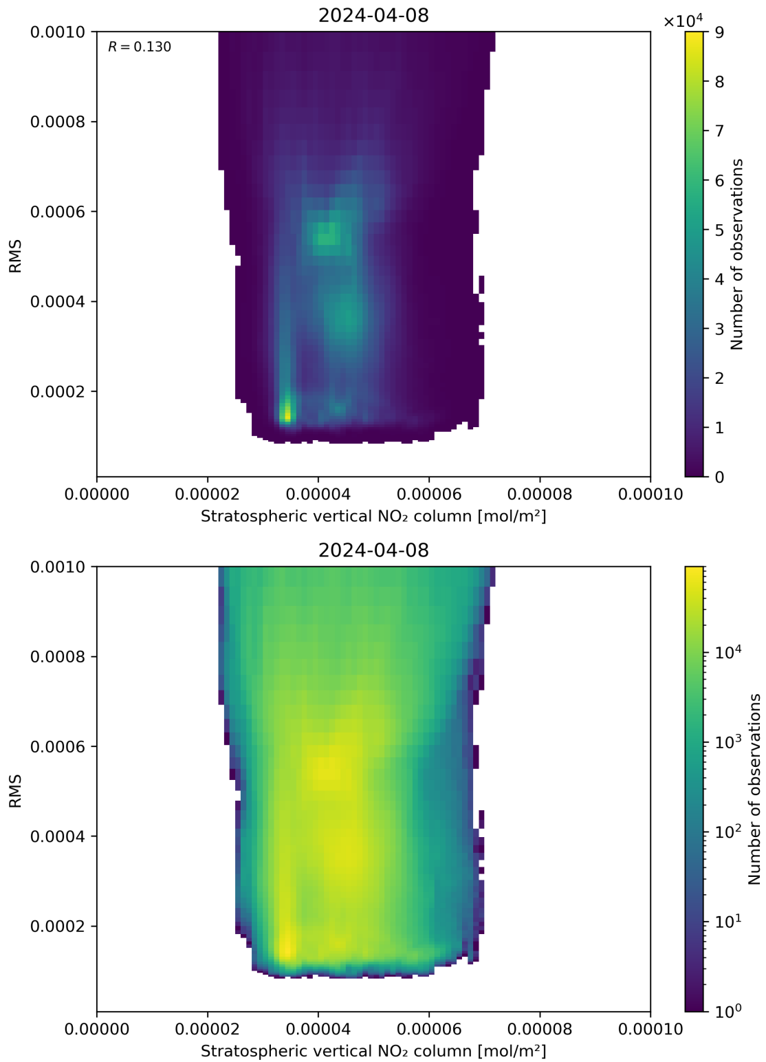
Figure 102: Scatter density plot of “Stratospheric vertical NO 2 column” against “RMS” for 2024-04-07 to 2024-04-09.
