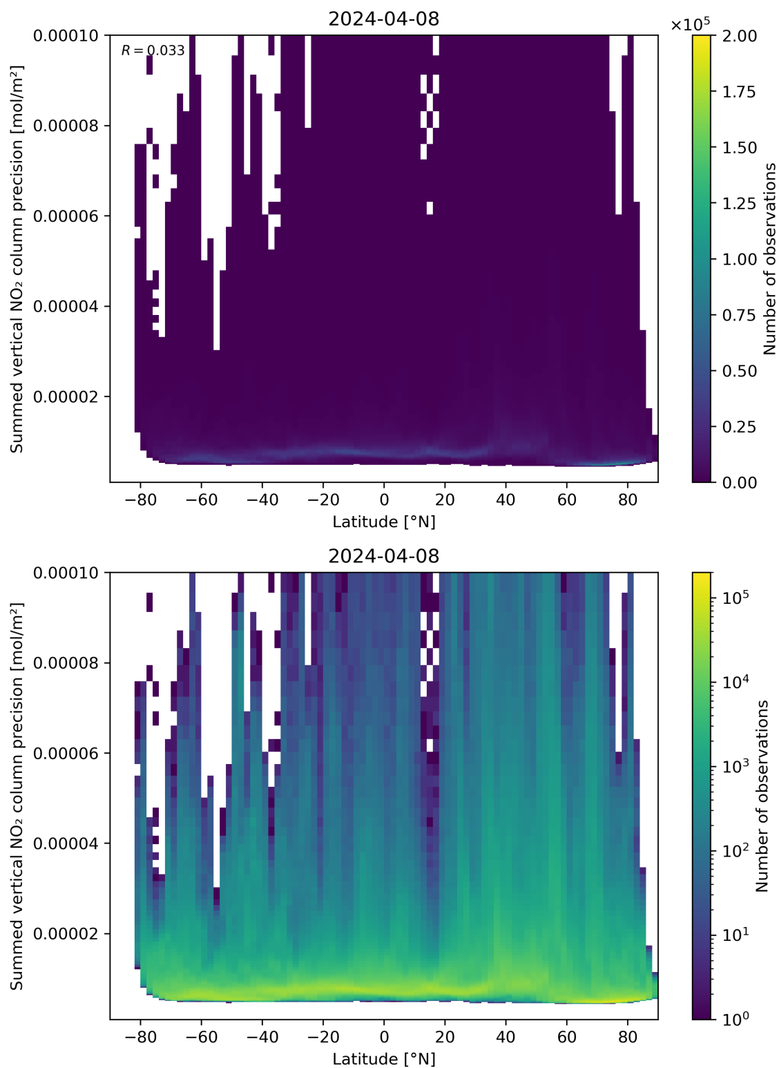
Figure 89: Scatter density plot of “Latitude” against “Summed vertical NO 2 column precision” for 2024-04-07 to 2024-04-09.
