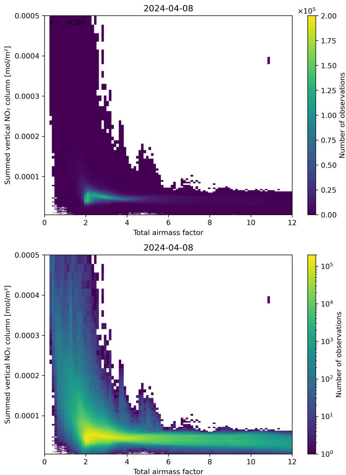
Figure 65: Scatter density plot of “Total airmass factor” against “Summed vertical NO 2 column” for 2024-04-07 to 2024-04-09.
