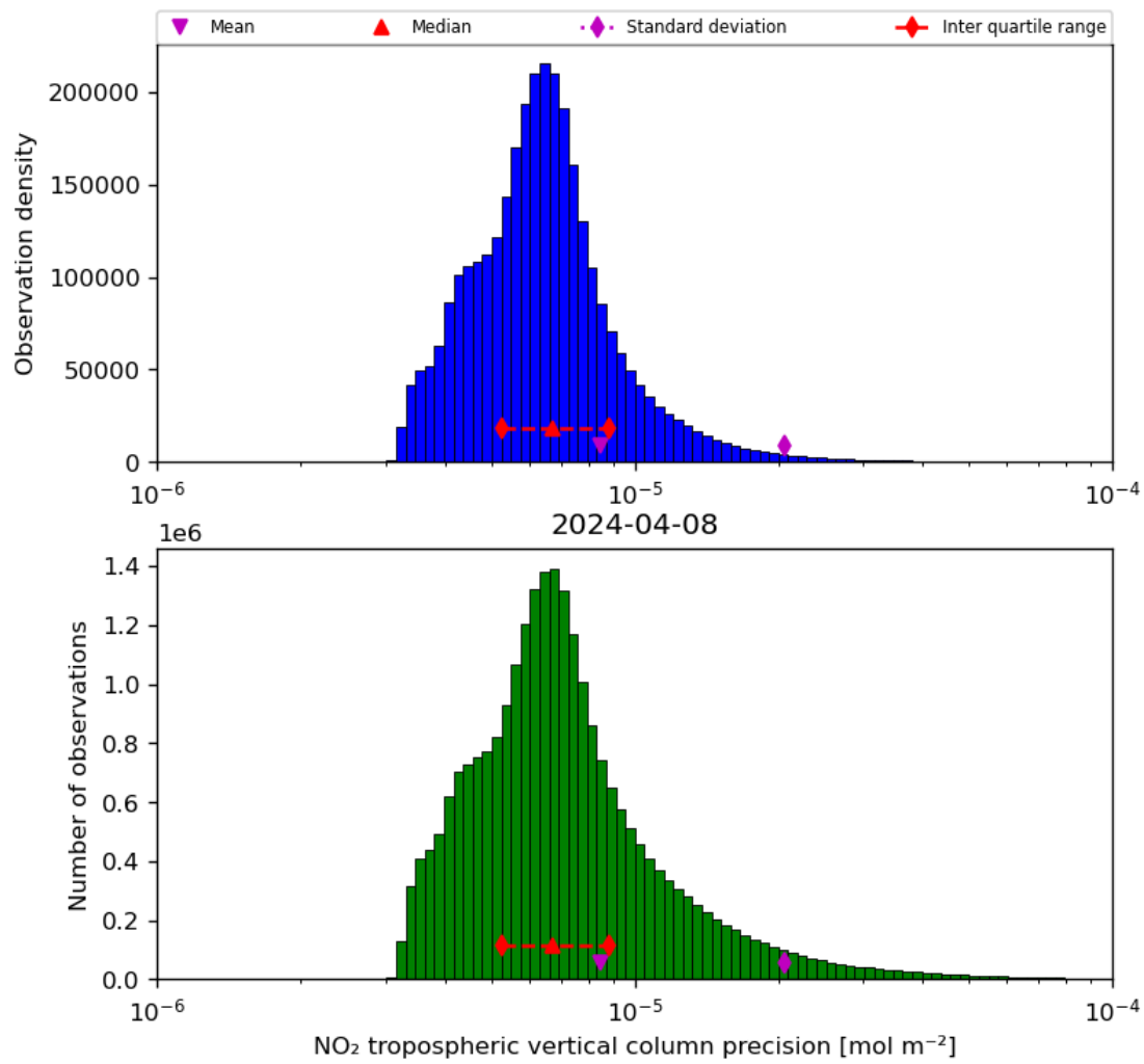
Figure 30: Histogram of “NO 2 tropospheric vertical column precision” for 2024-04-07 to 2024-04-09
