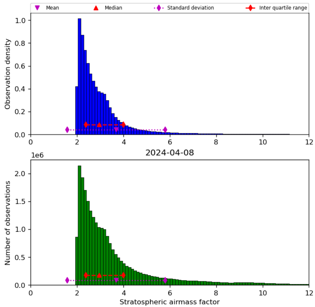
Figure 44: Histogram of “Stratospheric airmass factor” for 2024-04-07 to 2024-04-09
