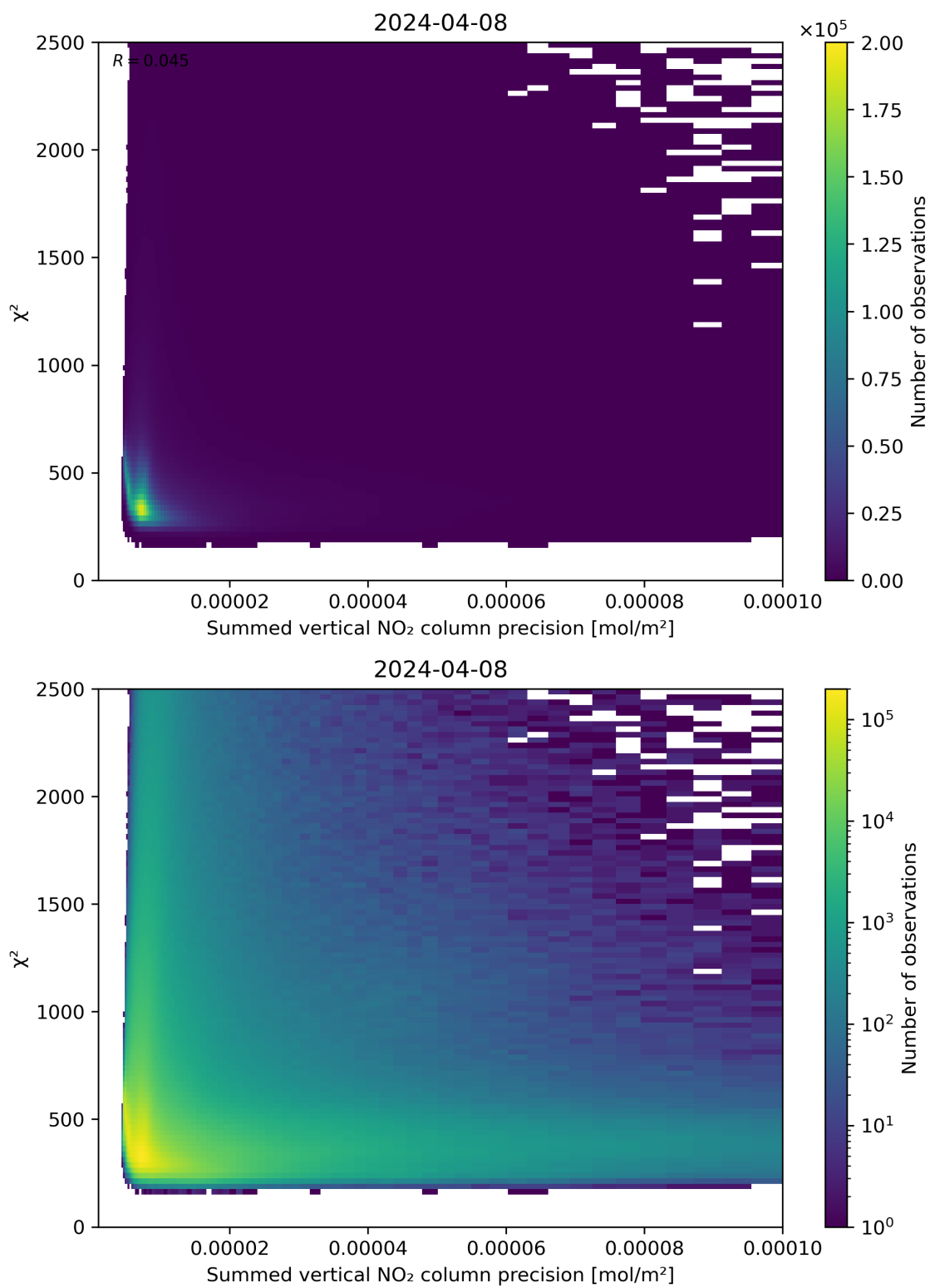
Figure 107: Scatter density plot of “Summed vertical NO 2 column precision” against “ \chi^2 ” for 2024-04-07 to 2024-04-09.
