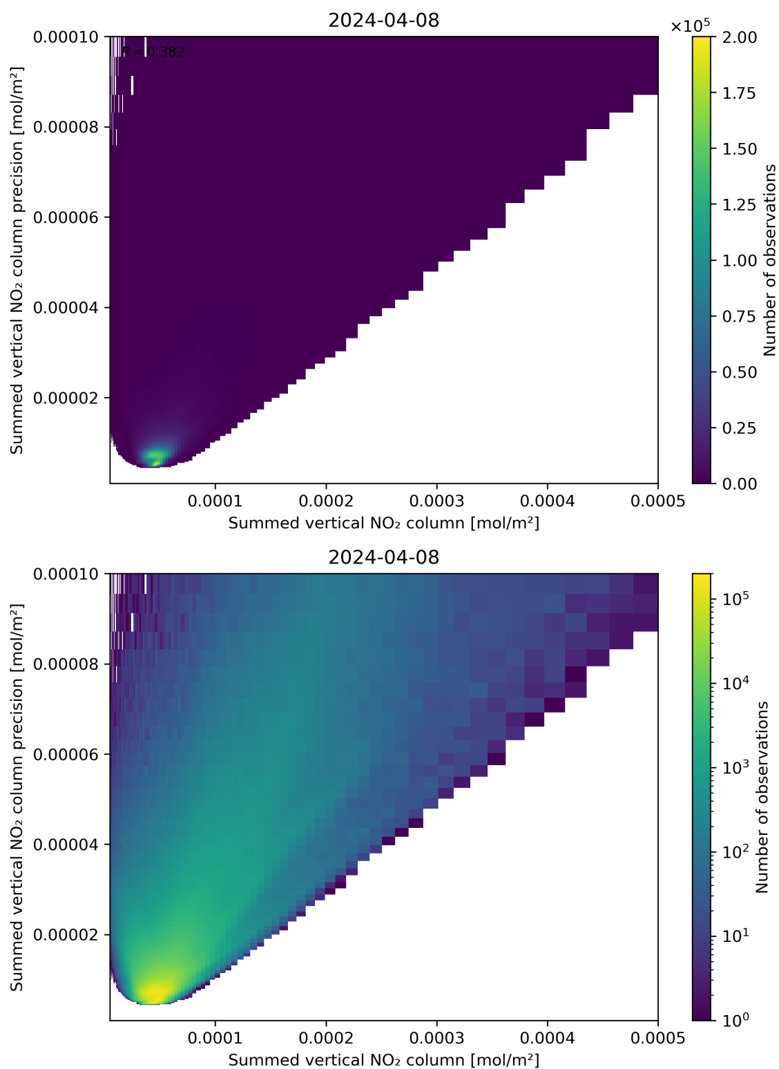
Figure 105: Scatter density plot of “Summed vertical NO 2 column” against “Summed vertical NO 2 column precision” for 2024-04-07 to 2024-04-09.
