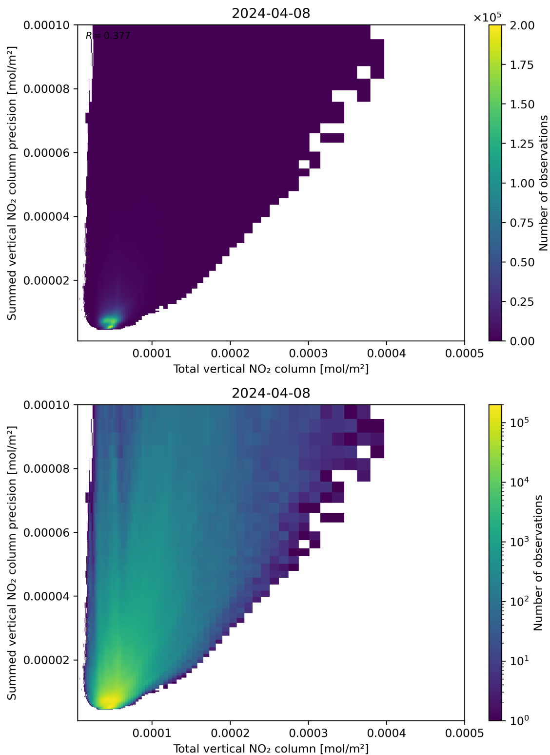
Figure 113: Scatter density plot of “Total vertical NO 2 column” against “Summed vertical NO 2 column precision” for 2024-04-07 to 2024-04-09.
