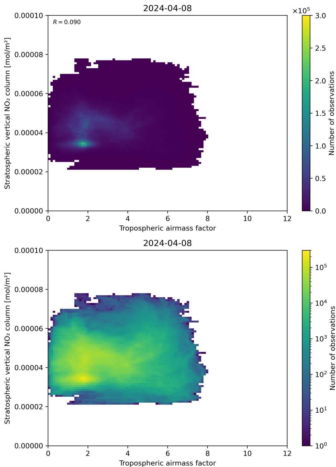
Figure 74: Scatter density plot of “Tropospheric airmass factor” against “Stratospheric vertical NO 2 column” for 2024-04-07 to 2024-04-09.
