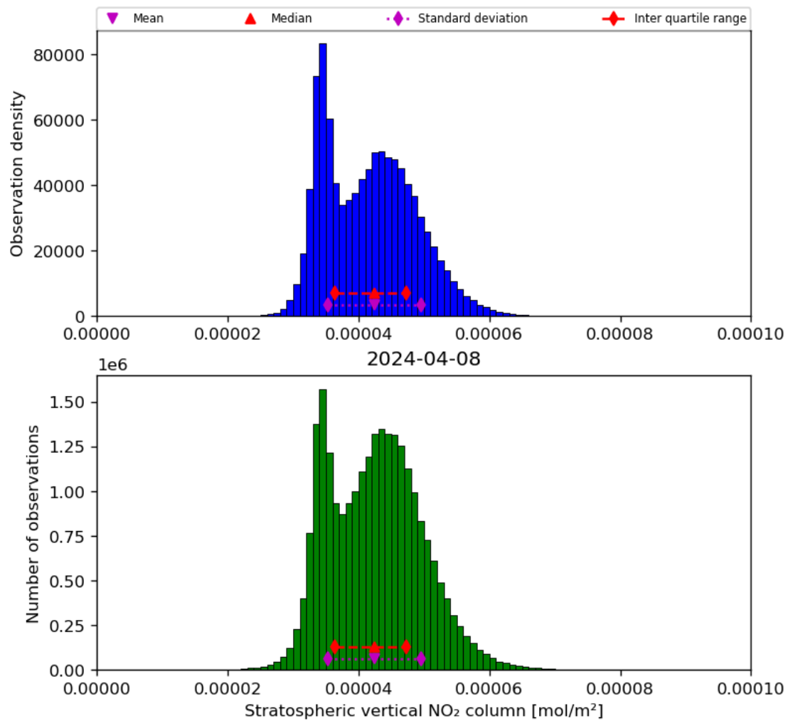
Figure 36: Histogram of “Stratospheric vertical NO 2 column” for 2024-04-07 to 2024-04-09
