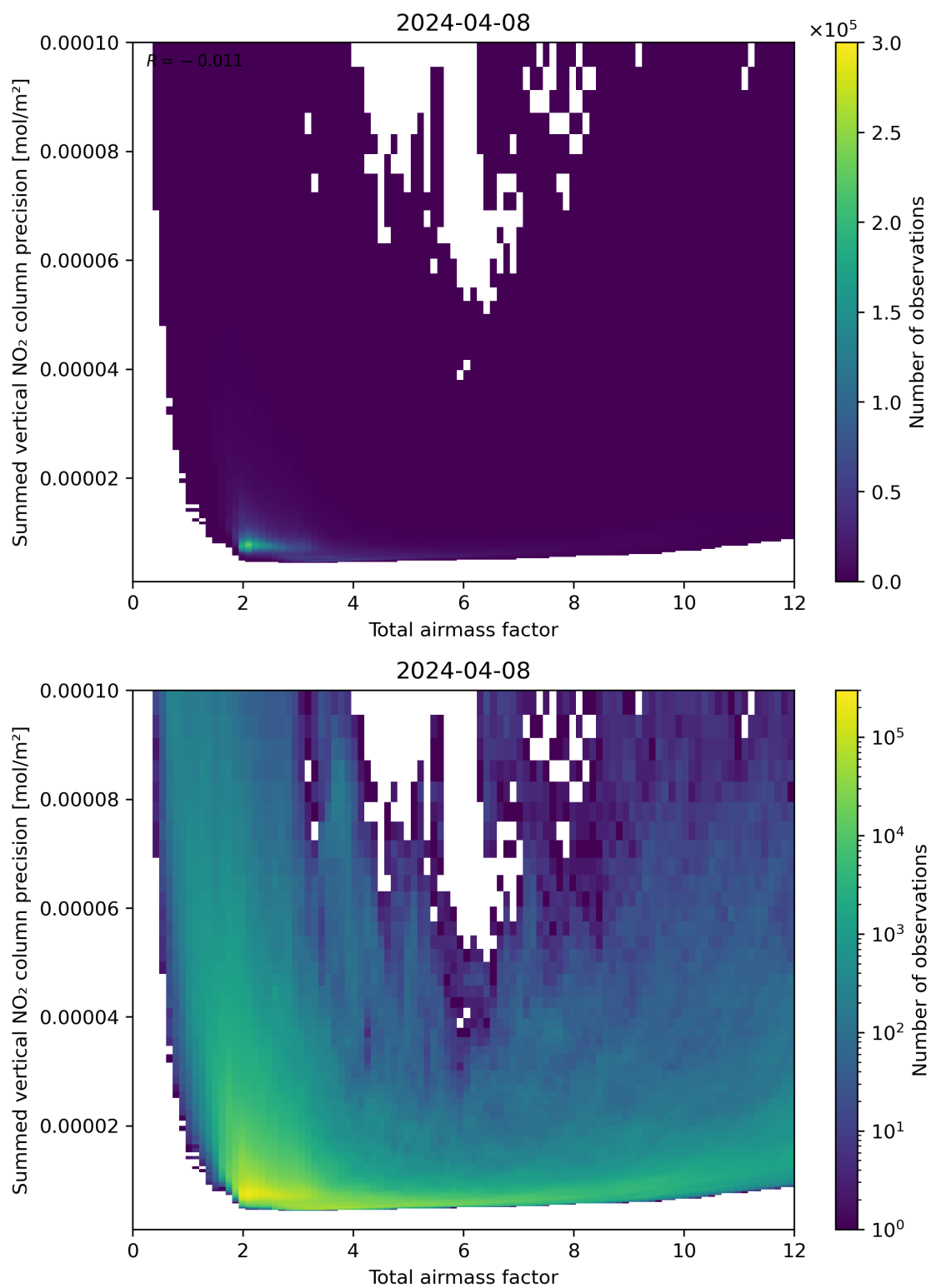
Figure 66: Scatter density plot of “Total airmass factor” against “Summed vertical NO 2 column precision” for 2024-04-07 to 2024-04-09.
