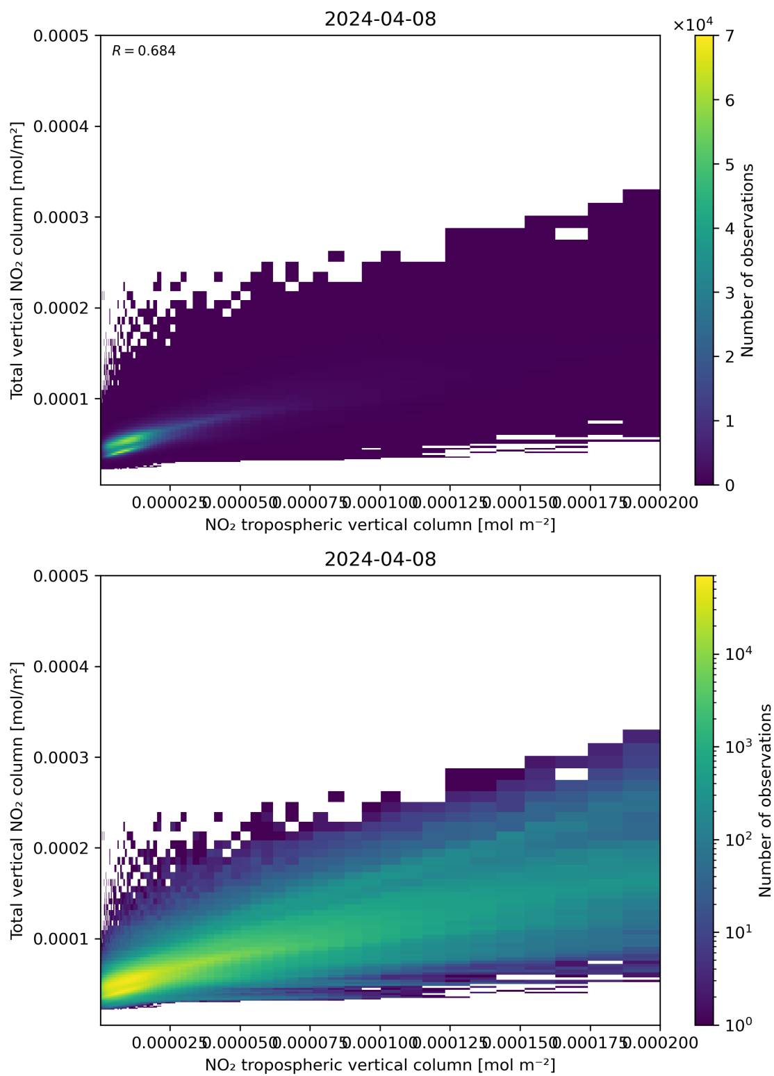
Figure 128: Scatter density plot of “NO 2 tropospheric vertical column” against “Total vertical NO 2 column” for 2024-04-07 to 2024-04-09.
