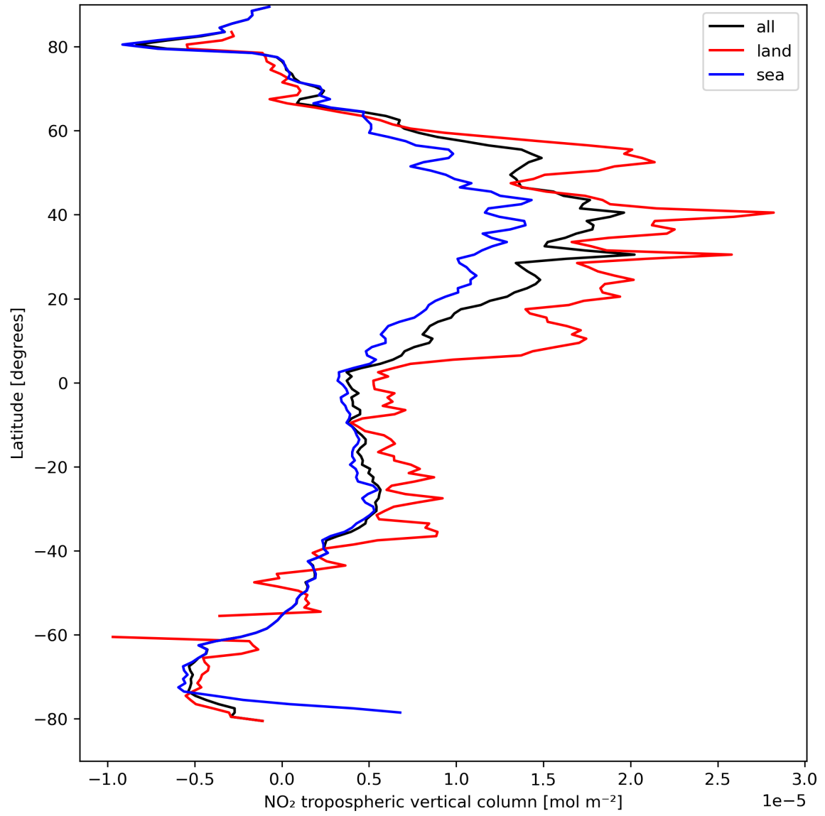
Figure 12: Zonal average of “NO 2 tropospheric vertical column” for 2024-04-07 to 2024-04-09.
