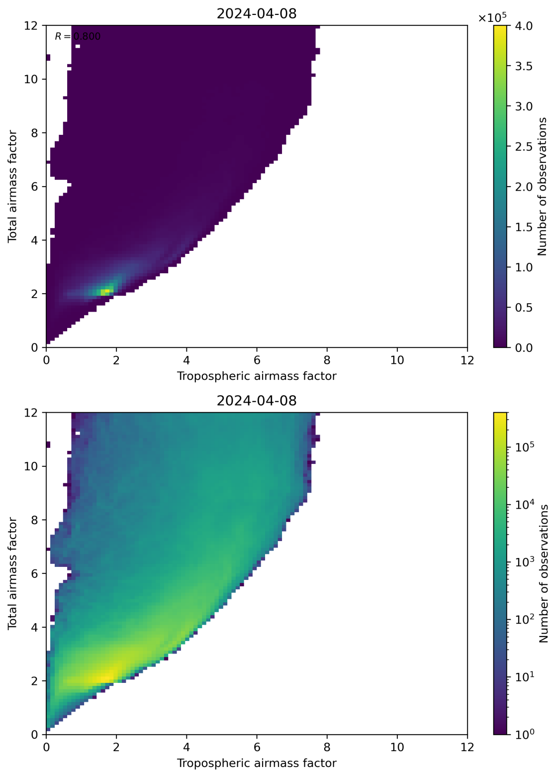
Figure 72: Scatter density plot of “Tropospheric airmass factor” against “Total airmass factor” for 2024-04-07 to 2024-04-09.
