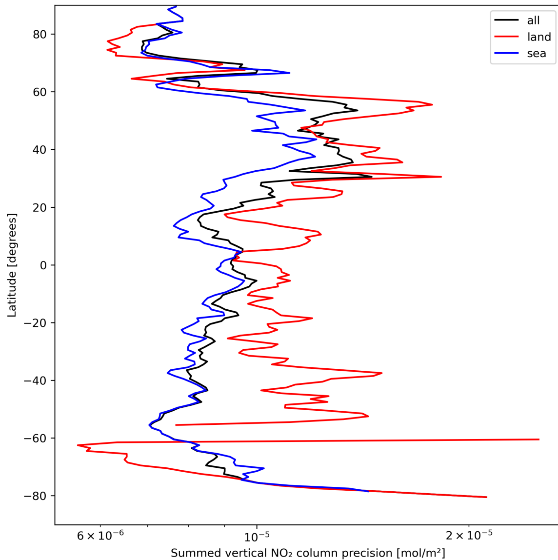
Figure 24: Zonal average of “Summed vertical NO 2 column precision” for 2024-04-07 to 2024-04-09.
