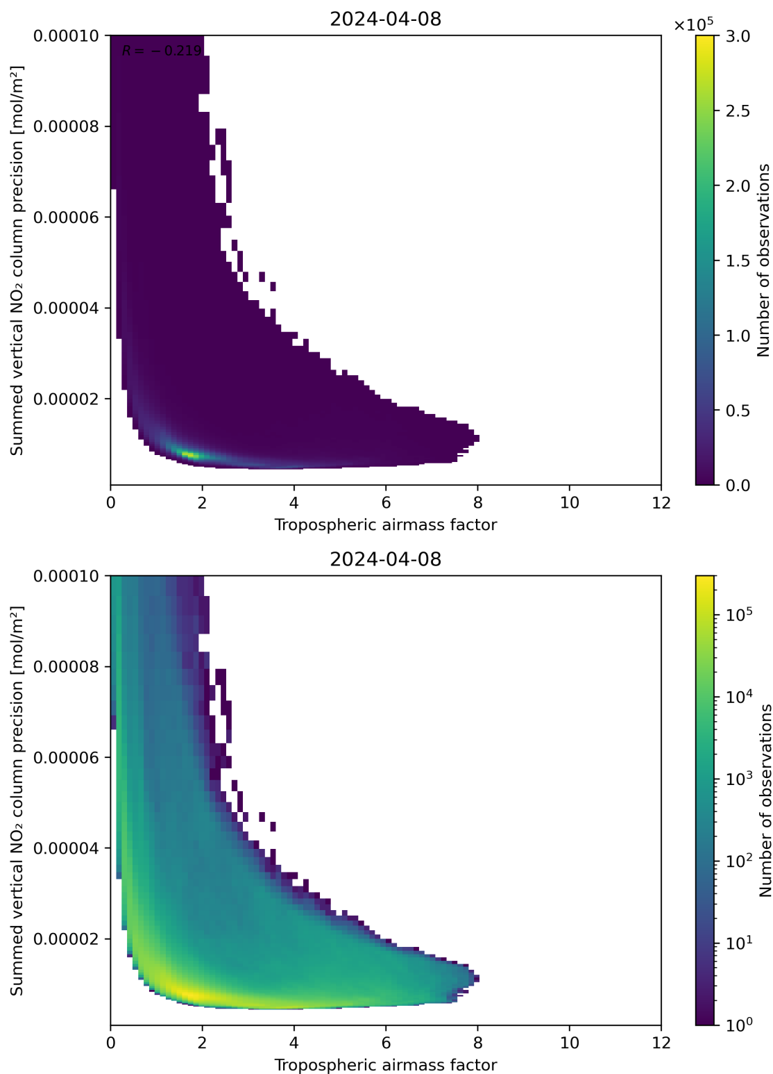
Figure 76: Scatter density plot of “Tropospheric air mass factor” against “Summed vertical NO 2 column precision” for 2024-04-07 to 2024-04-09.
