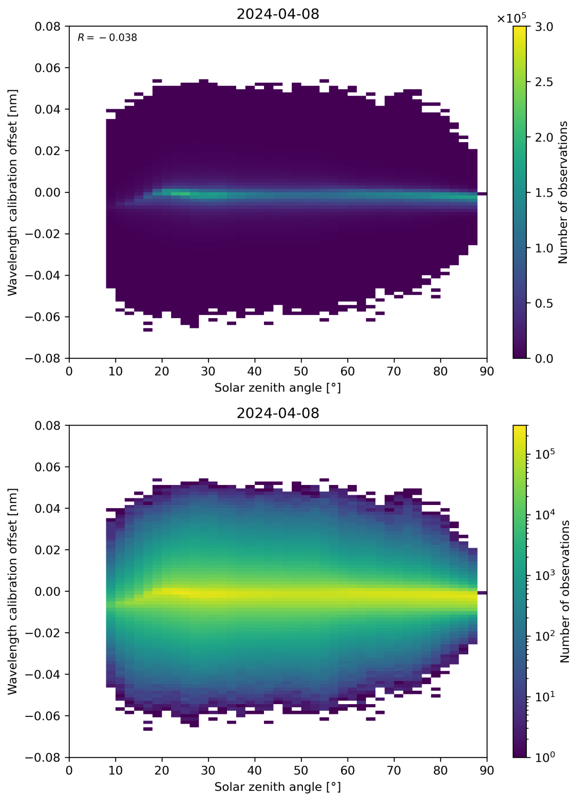
Figure 158: Scatter density plot of “Solar zenith angle” against “Wavelength calibration offset” for 2024-04-07 to 2024-04-09.
