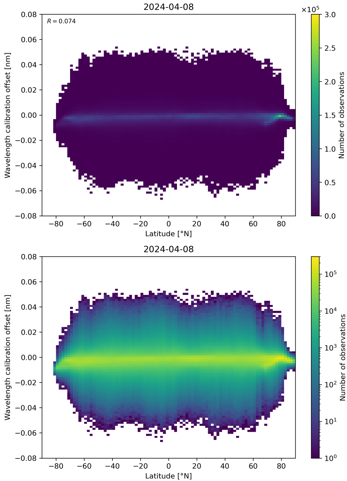
Figure 95: Scatter density plot of “Latitude” against “Wavelength calibration offset” for 2024-04-07 to 2024-04-09.
