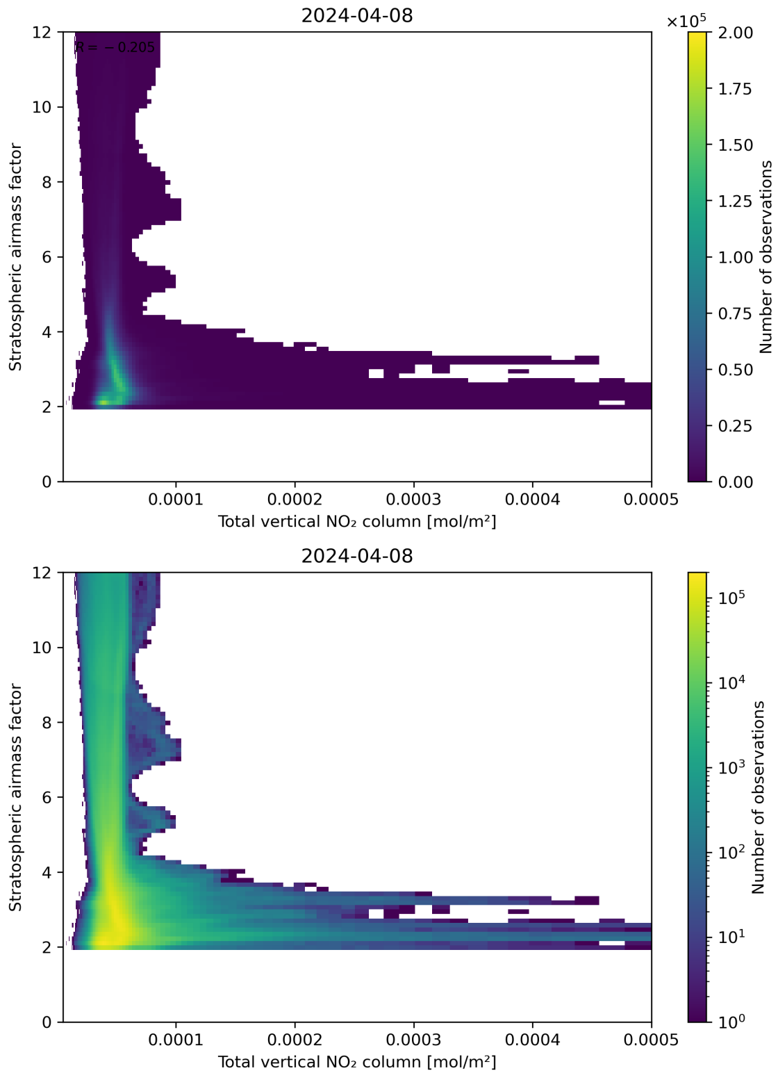
Figure 110: Scatter density plot of “Total vertical NO 2 column” against “Stratospheric airmass factor” for 2024-04-07 to 2024-04-09.
