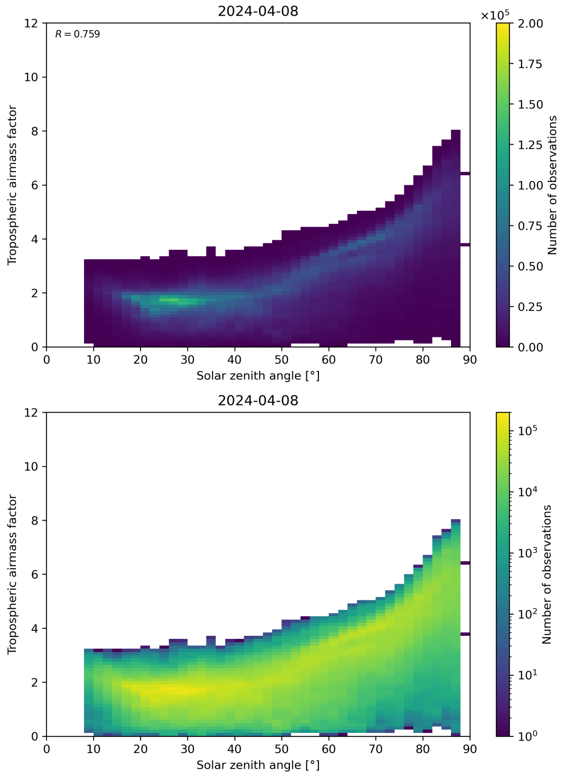
Figure 147: Scatter density plot of “Solar zenith angle” against “Tropospheric airmass factor” for 2024-04-07 to 2024-04-09.
