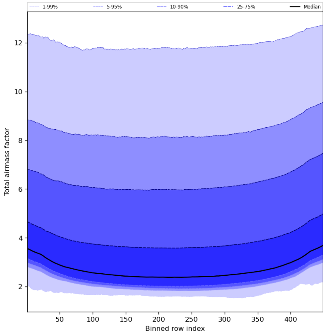
Figure 49: Along track statistics of “Total airmass factor” for 2024-04-07 to 2024-04-09
