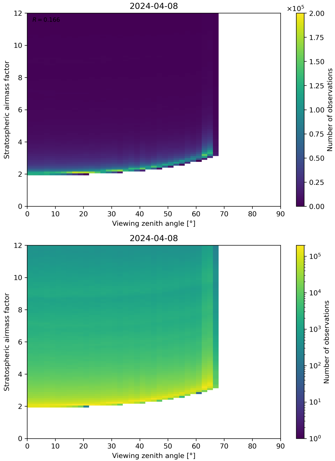
Figure 159: Scatter density plot of “Viewing zenith angle” against “Stratospheric airmass factor” for 2024-04-07 to 2024-04-09.
