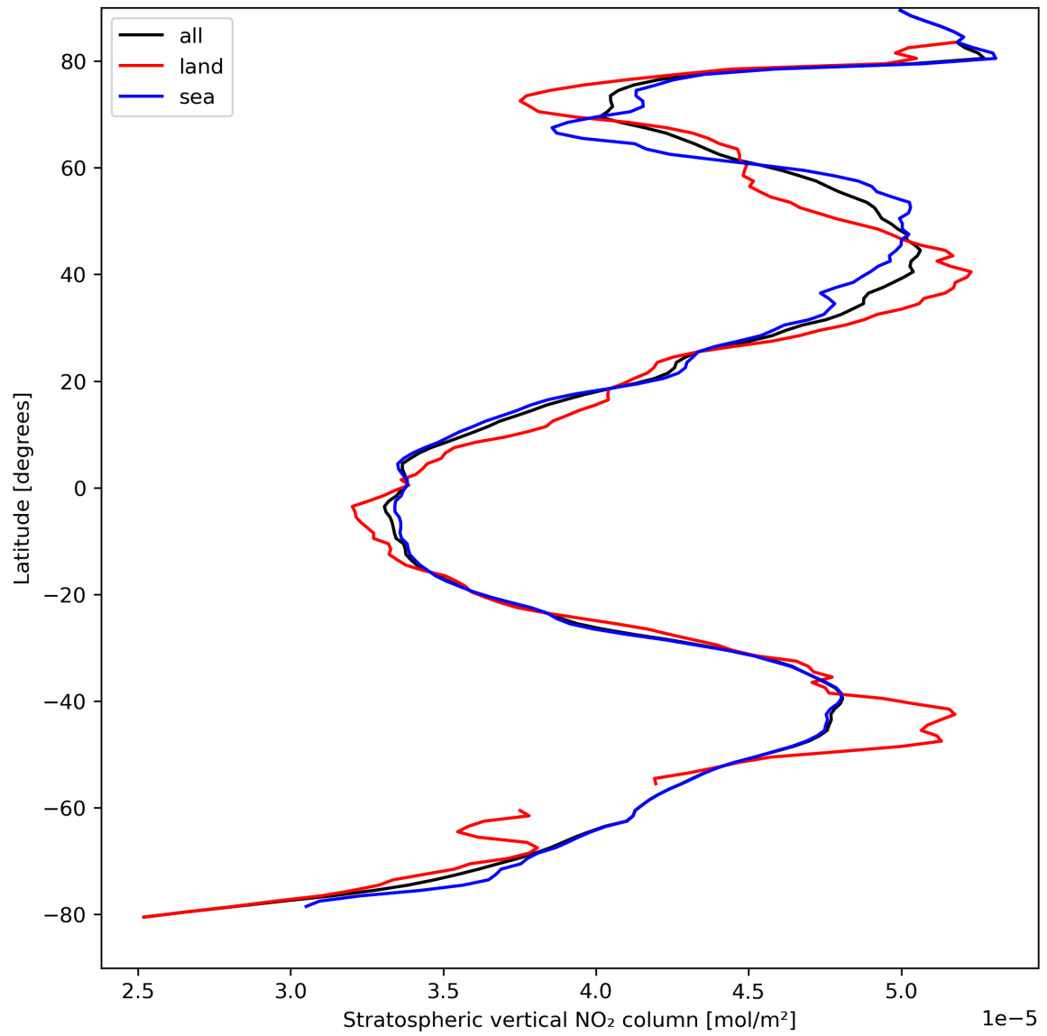
Figure 19: Zonal average of “Stratospheric vertical NO 2 column” for 2024-04-07 to 2024-04-09.
