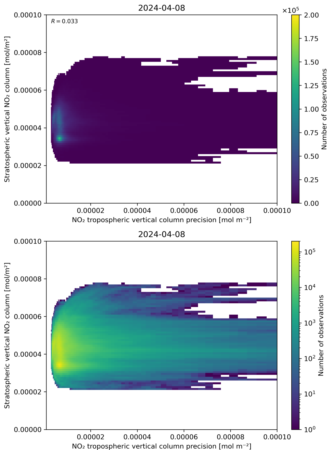
Figure 135: Scatter density plot of “NO 2 tropospheric vertical column precision” against “Stratospheric vertical NO 2 column” for 2024-04-07 to 2024-04-09.
