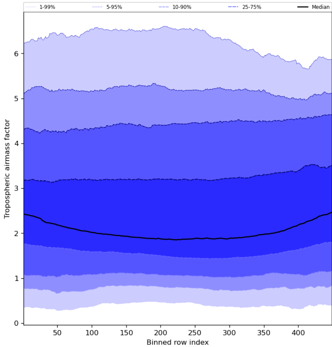
Figure 48: Along track statistics of “Tropospheric airmass factor” for 2024-04-07 to 2024-04-09
