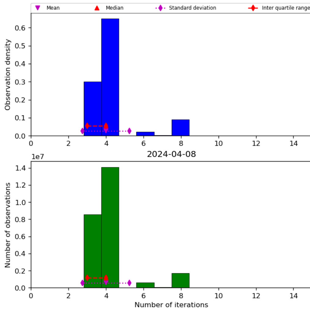
Figure 34: Histogram of “Number of iterations” for 2024-04-07 to 2024-04-09
