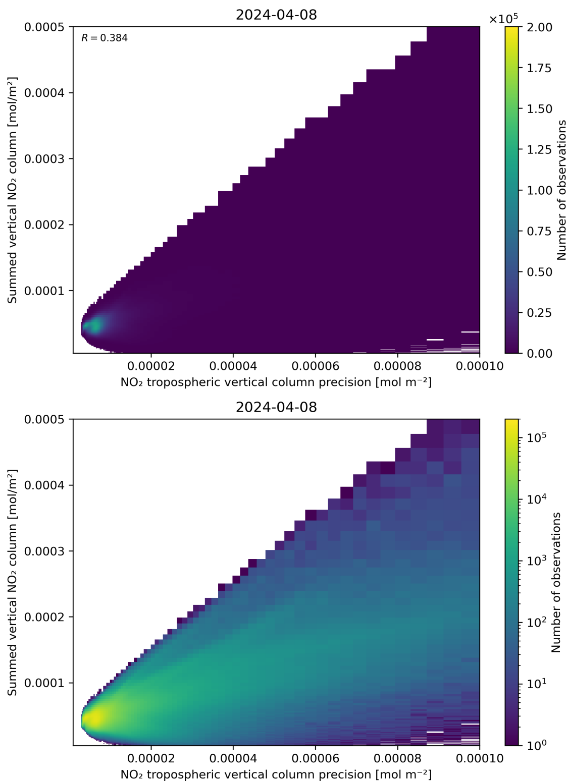
Figure 136: Scatter density plot of “NO 2 tropospheric vertical column precision” against “Summed vertical NO 2 column” for 2024-04-07 to 2024-04-09.
