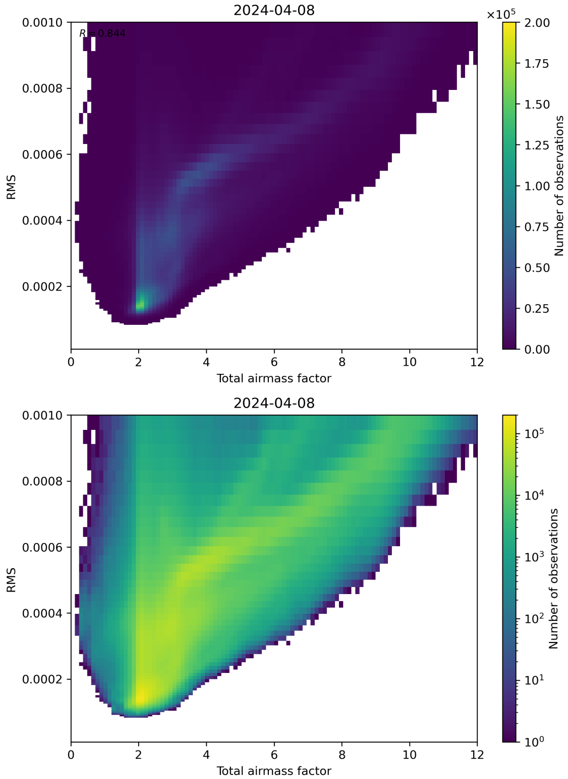
Figure 69: Scatter density plot of “Total airmass factor” against “RMS” for 2024-04-07 to 2024-04-09.
