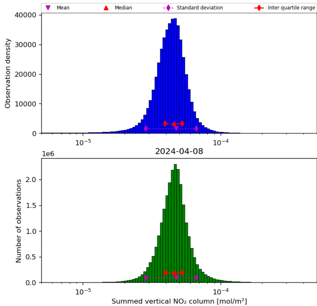
Figure 40: Histogram of “Summed vertical NO 2 column” for 2024-04-07 to 2024-04-09
