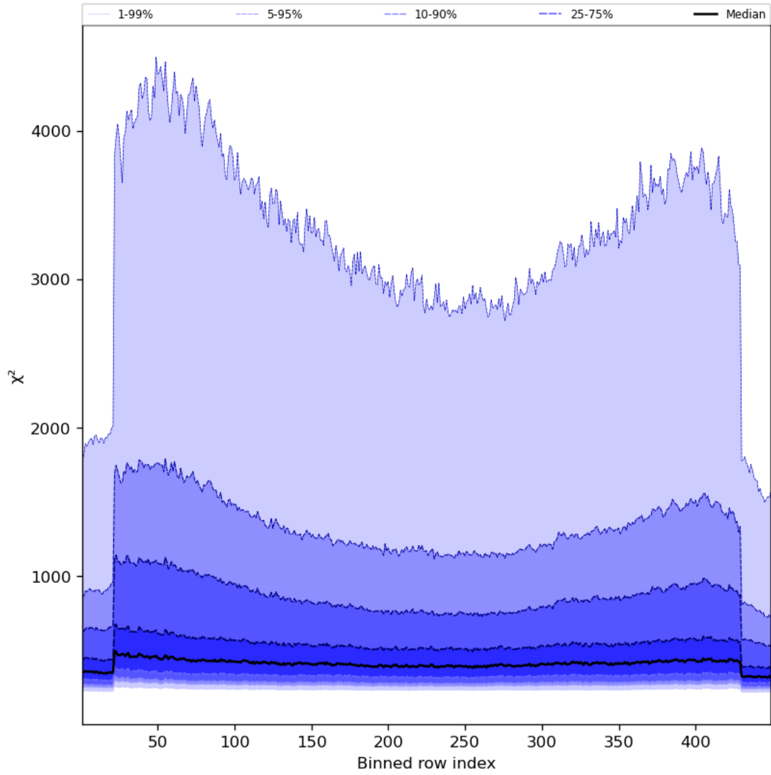
Figure 59: Along track statistics of “ \chi^2 ” for 2024-04-07 to 2024-04-09
