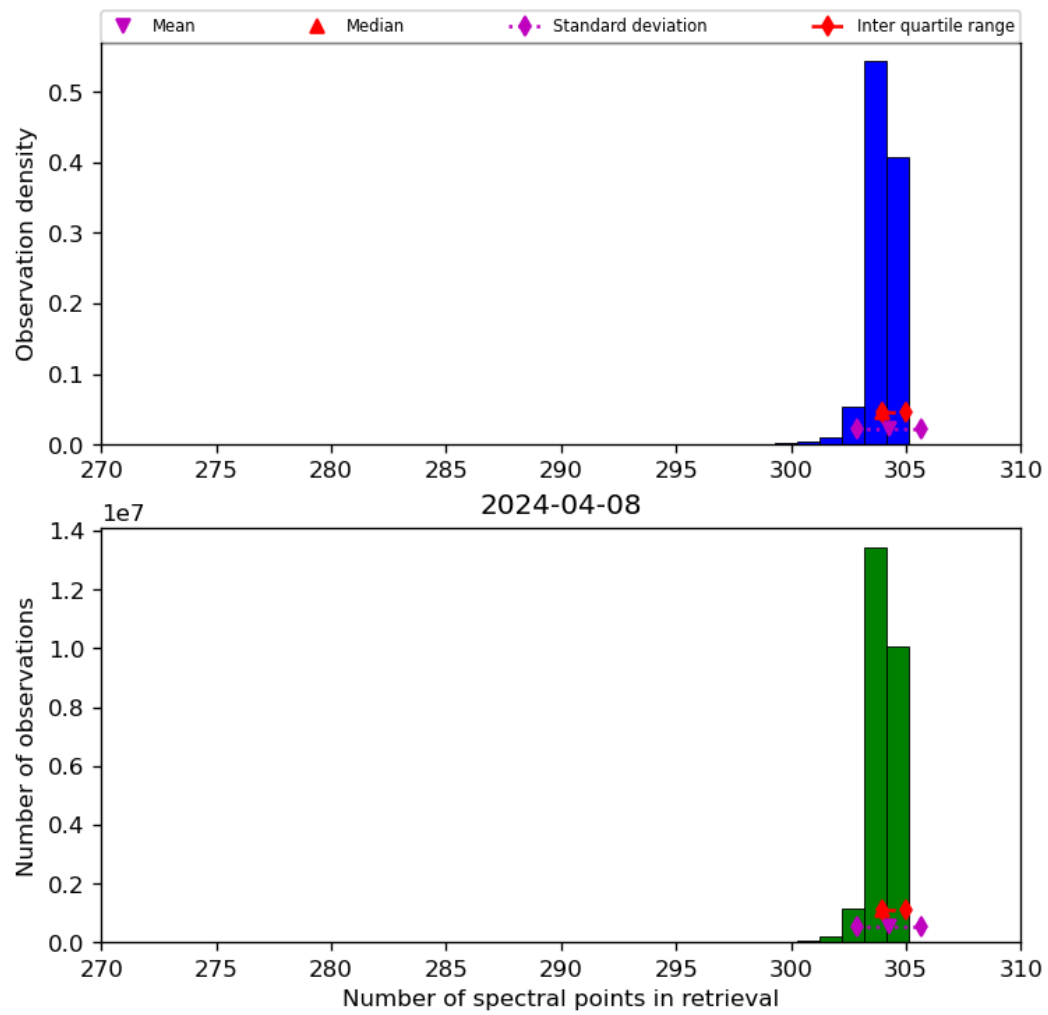
Figure 33: Histogram of “Number of spectral points in retrieval” for 2024-04-07 to 2024-04-09
