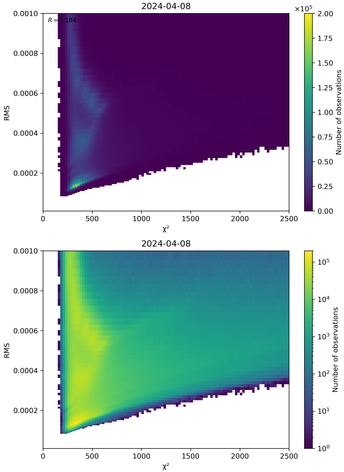
Figure 82: Scatter density plot of “ \chi^2 ” against “RMS” for 2024-04-07 to 2024-04-09.
