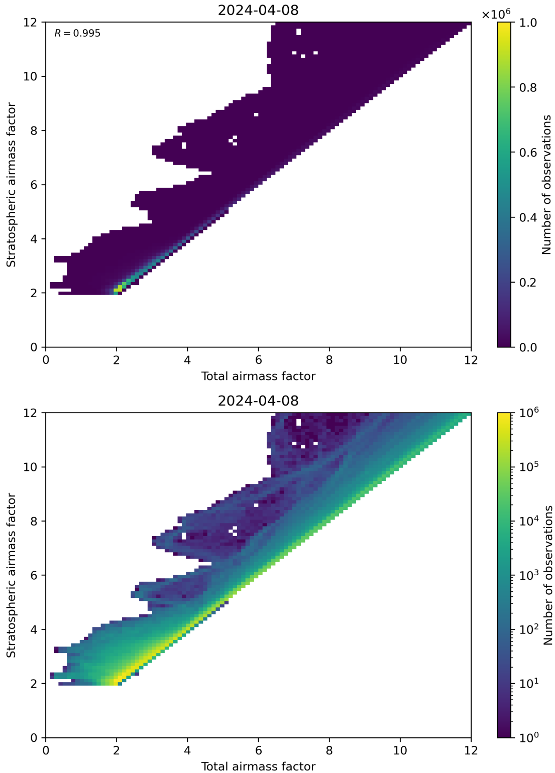
Figure 62: Scatter density plot of “Total airmass factor” against “Stratospheric airmass factor” for 2024-04-07 to 2024-04-09.
