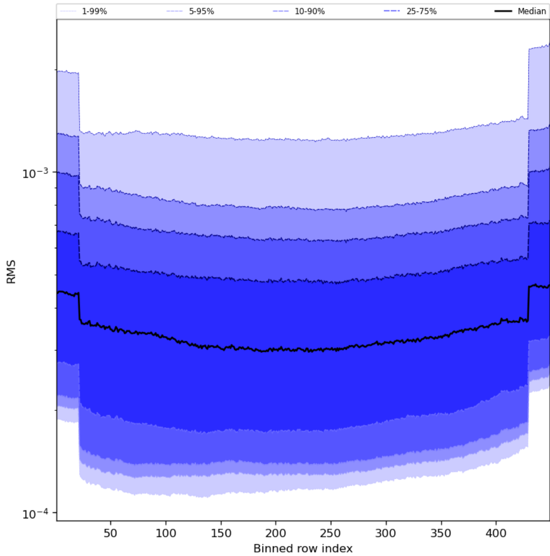
Figure 60: Along track statistics of “RMS” for 2024-04-07 to 2024-04-09
