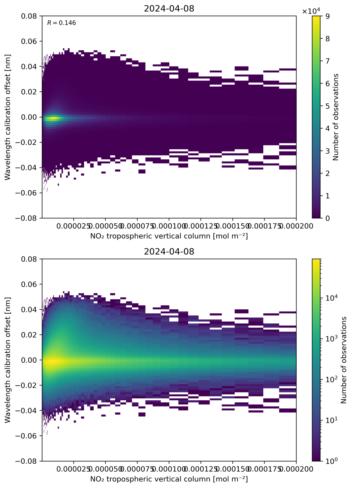
Figure 143: Scatter density plot of “NO 2 tropospheric vertical column” against “Wavelength calibration offset” for 2024-04-07 to 2024-04-09.
