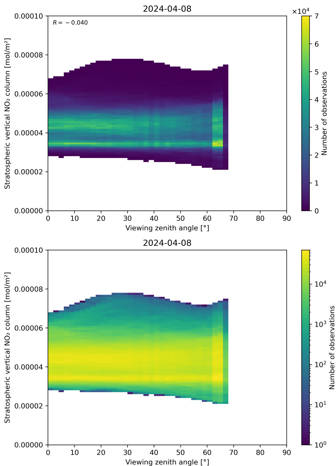
Figure 164: Scatter density plot of “Viewing zenith angle” against “Stratospheric vertical NO 2 column” for 2024-04-07 to 2024-04-09.
