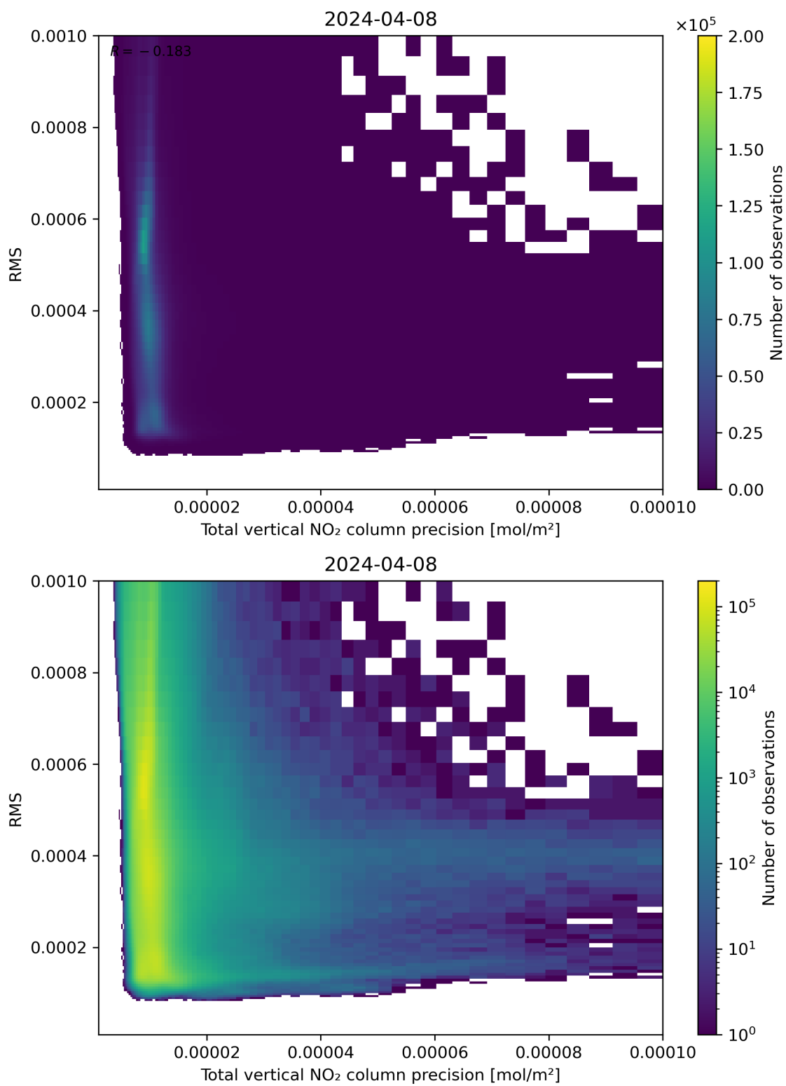
Figure 119: Scatter density plot of “Total vertical NO 2 column precision” against “RMS” for 2024-04-07 to 2024-04-09.
