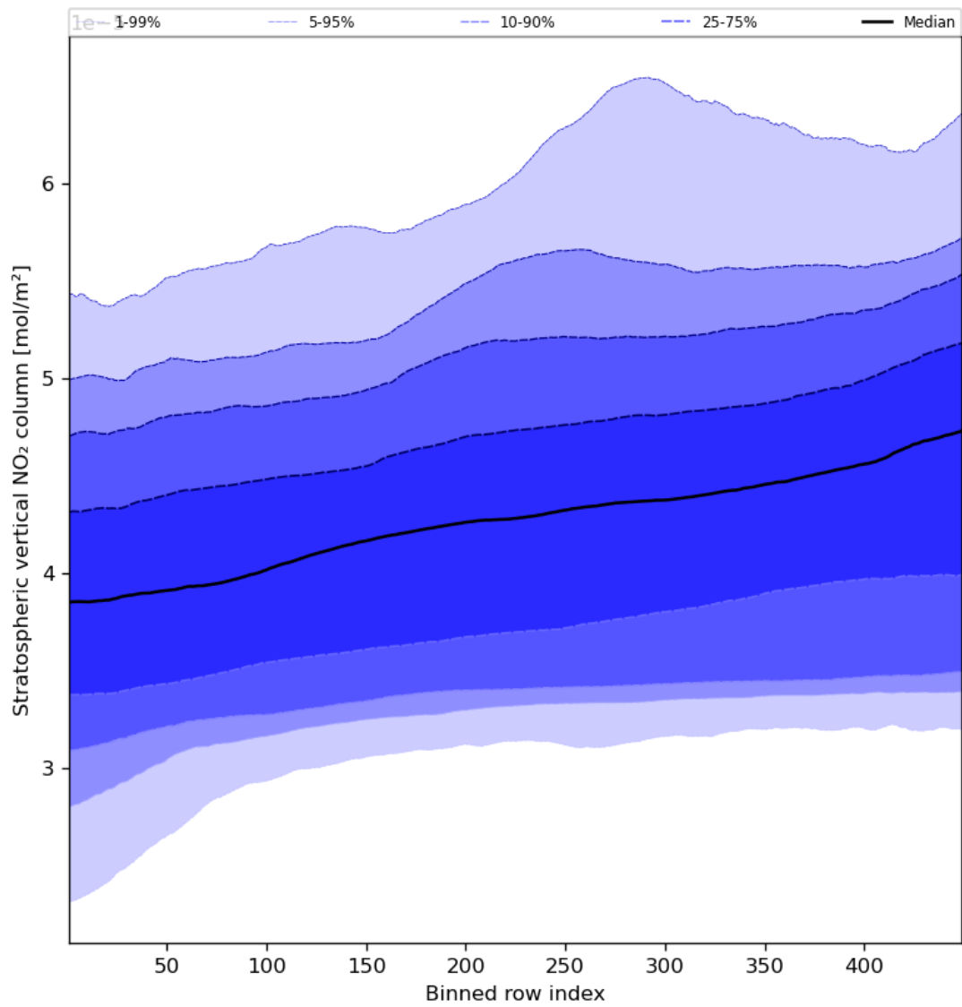
Figure 53: Along track statistics of “Stratospheric vertical NO 2 column” for 2024-04-07 to 2024-04-09
