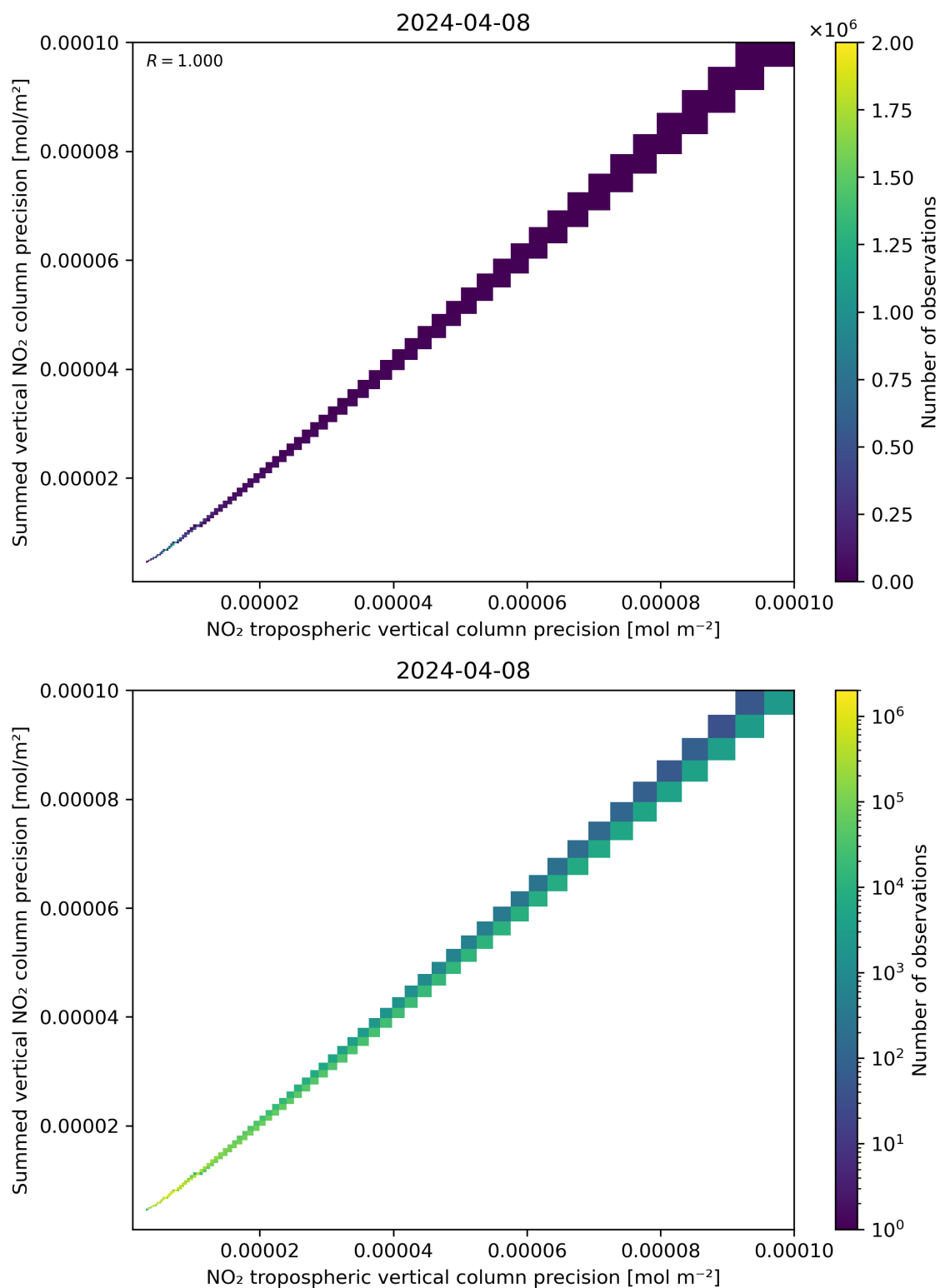
Figure 137: Scatter density plot of “NO 2 tropospheric vertical column precision” against “Summed vertical NO 2 column precision” for 2024-04-07 to 2024-04-09.
