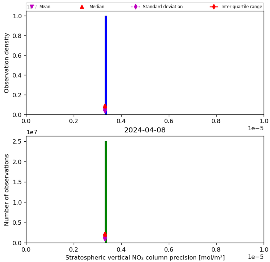
Figure 37: Histogram of “Stratospheric vertical NO 2 column precision” for 2024-04-07 to 2024-04-09
