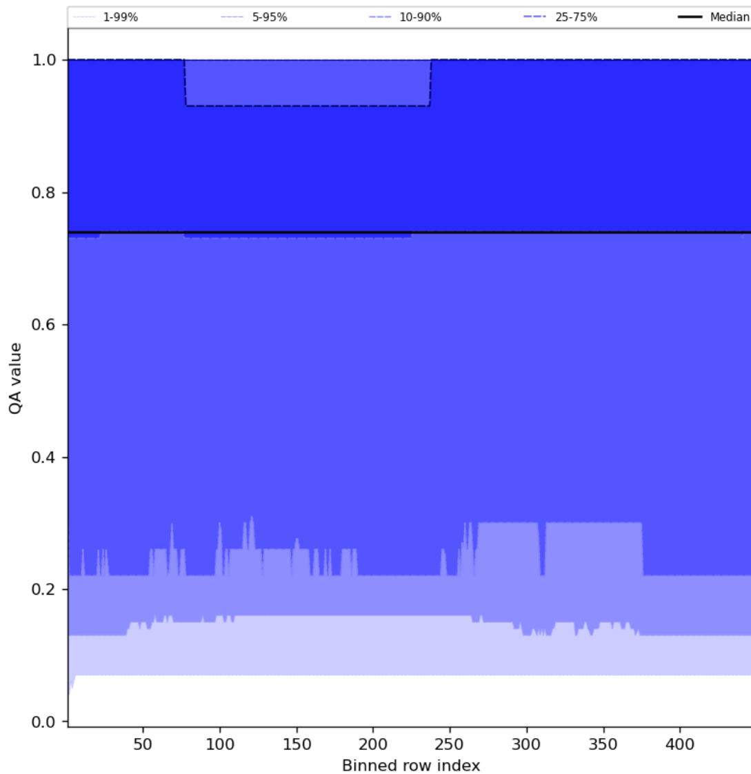
Figure 45: Along track statistics of “QA value” for 2024-04-07 to 2024-04-09
