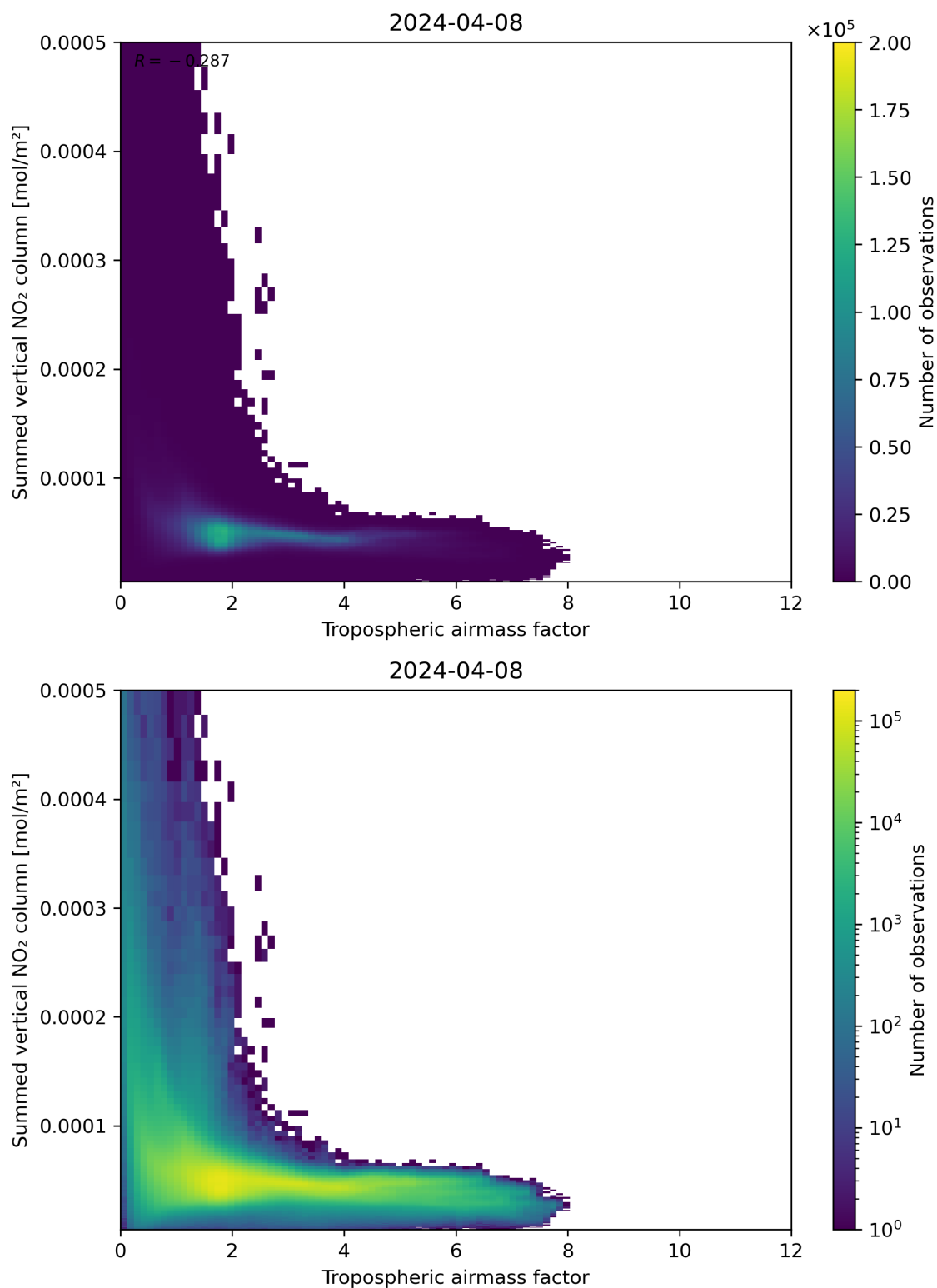
Figure 75: Scatter density plot of “Tropospheric airmass factor” against “Summed vertical NO 2 column” for 2024-04-07 to 2024-04-09.
