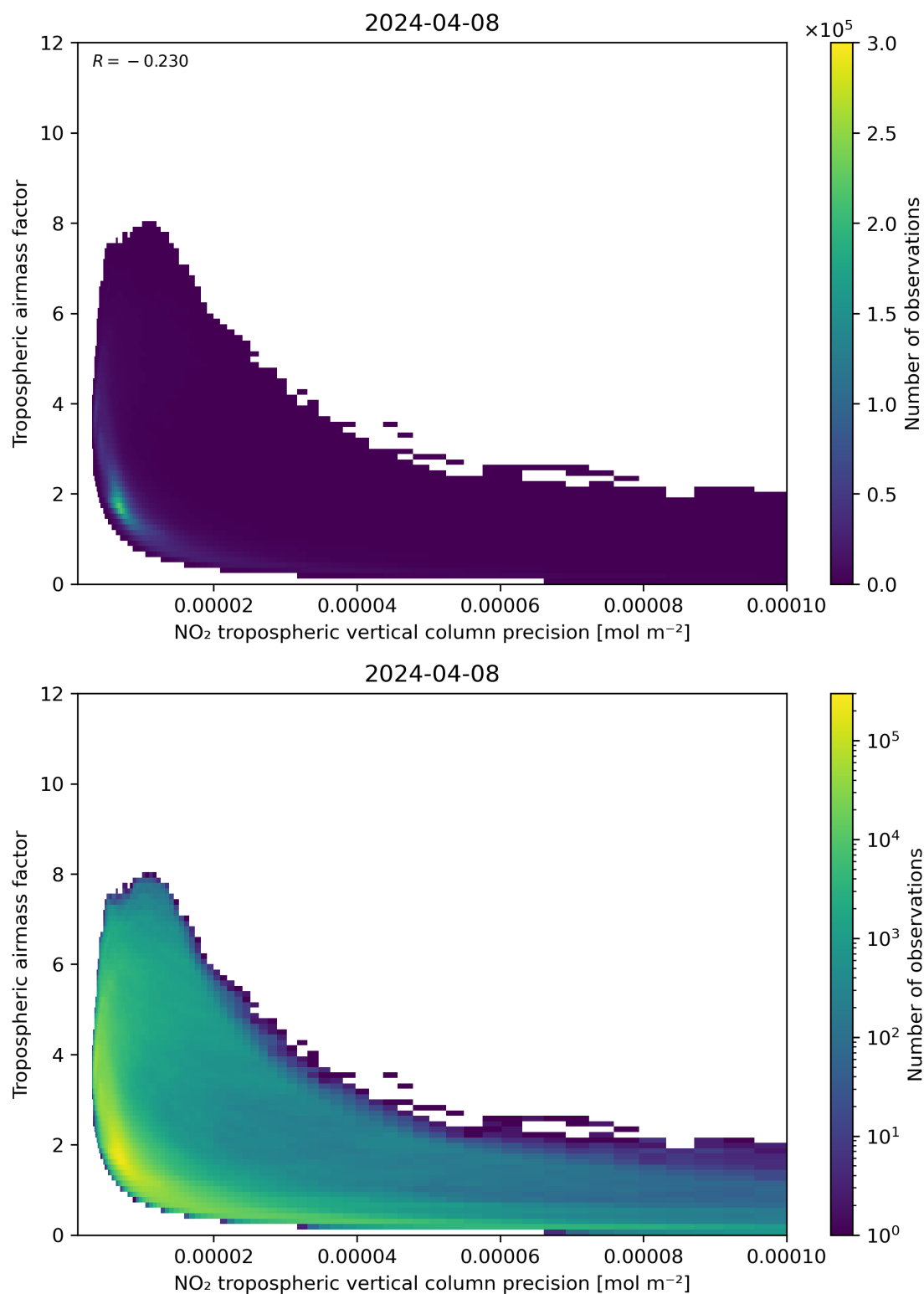
Figure 133: Scatter density plot of “NO 2 tropospheric vertical column precision” against “Tropospheric airmass factor” for 2024-04-07 to 2024-04-09.
