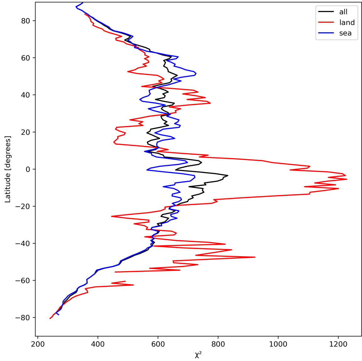
Figure 25: Zonal average of “ \chi^2 ” for 2024-04-07 to 2024-04-09.
