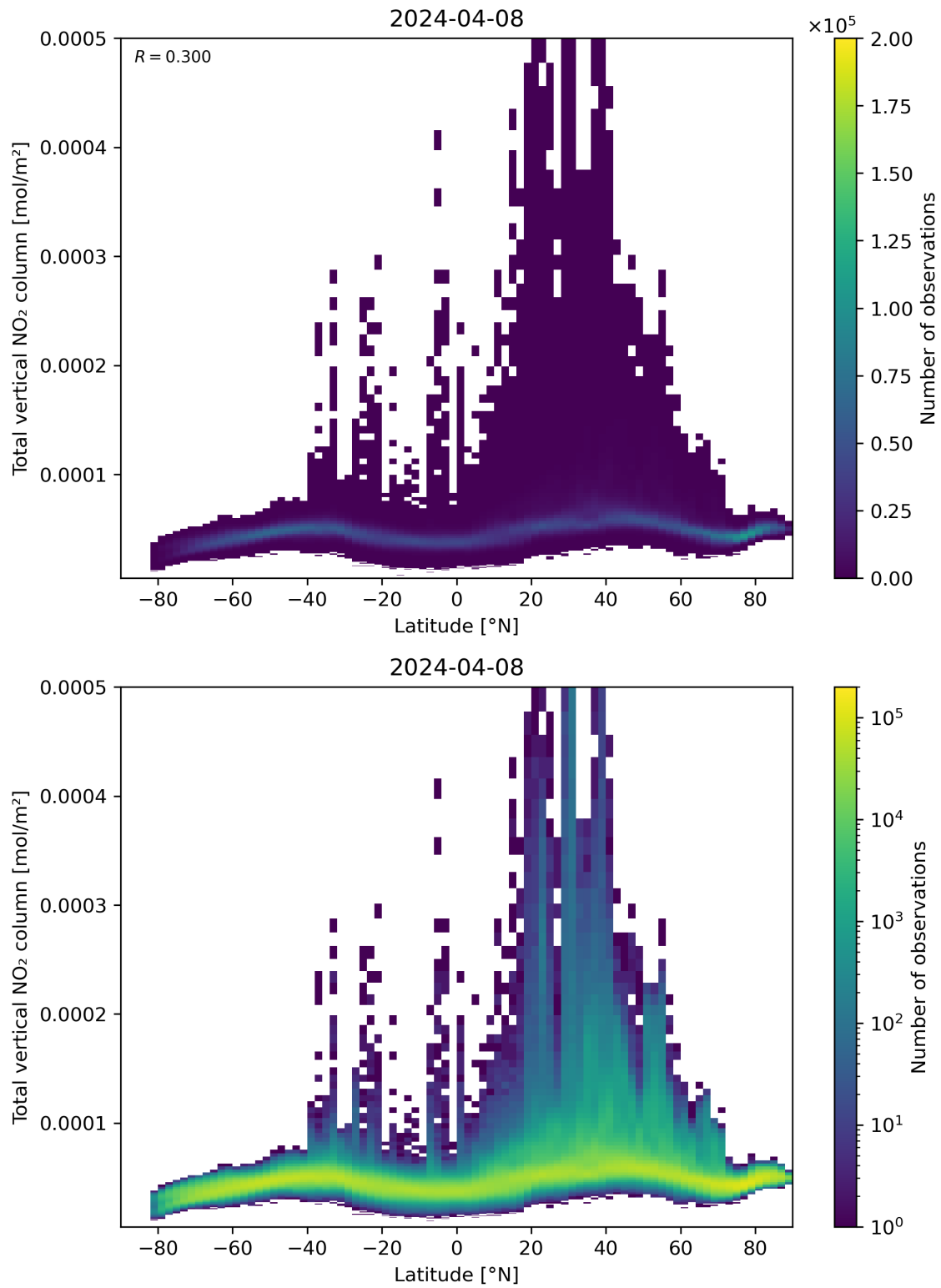
Figure 90: Scatter density plot of “Latitude” against “Total vertical NO 2 column” for 2024-04-07 to 2024-04-09.
