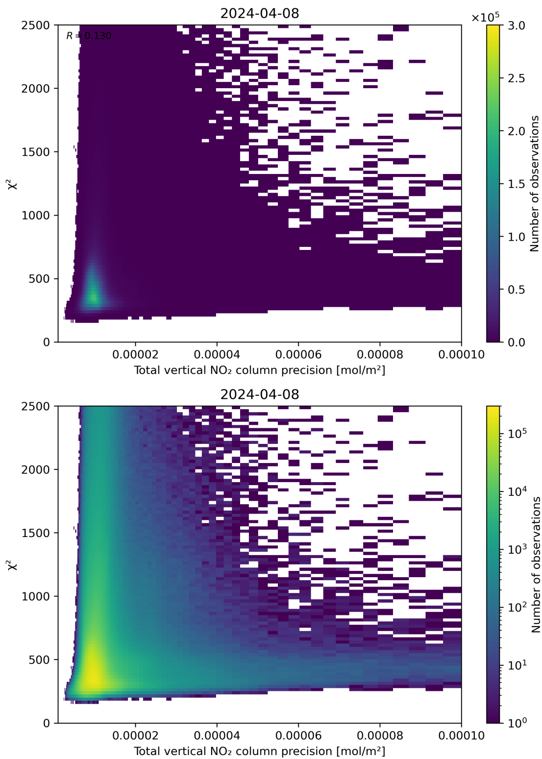
Figure 116: Scatter density plot of “Total vertical NO 2 column precision” against “ \chi^2 ” for 2024-04-07 to 2024-04-09.
