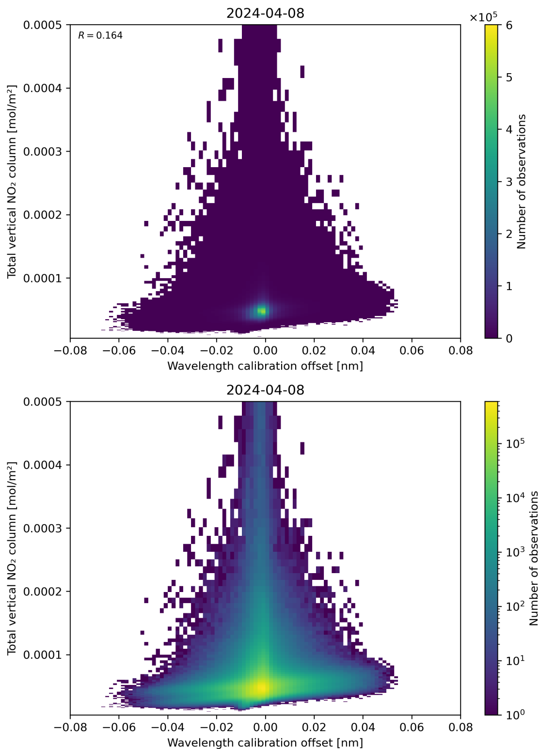
Figure 179: Scatter density plot of “Wavelength calibration offset” against “Total vertical NO 2 column” for 2024-04-07 to 2024-04-09.
