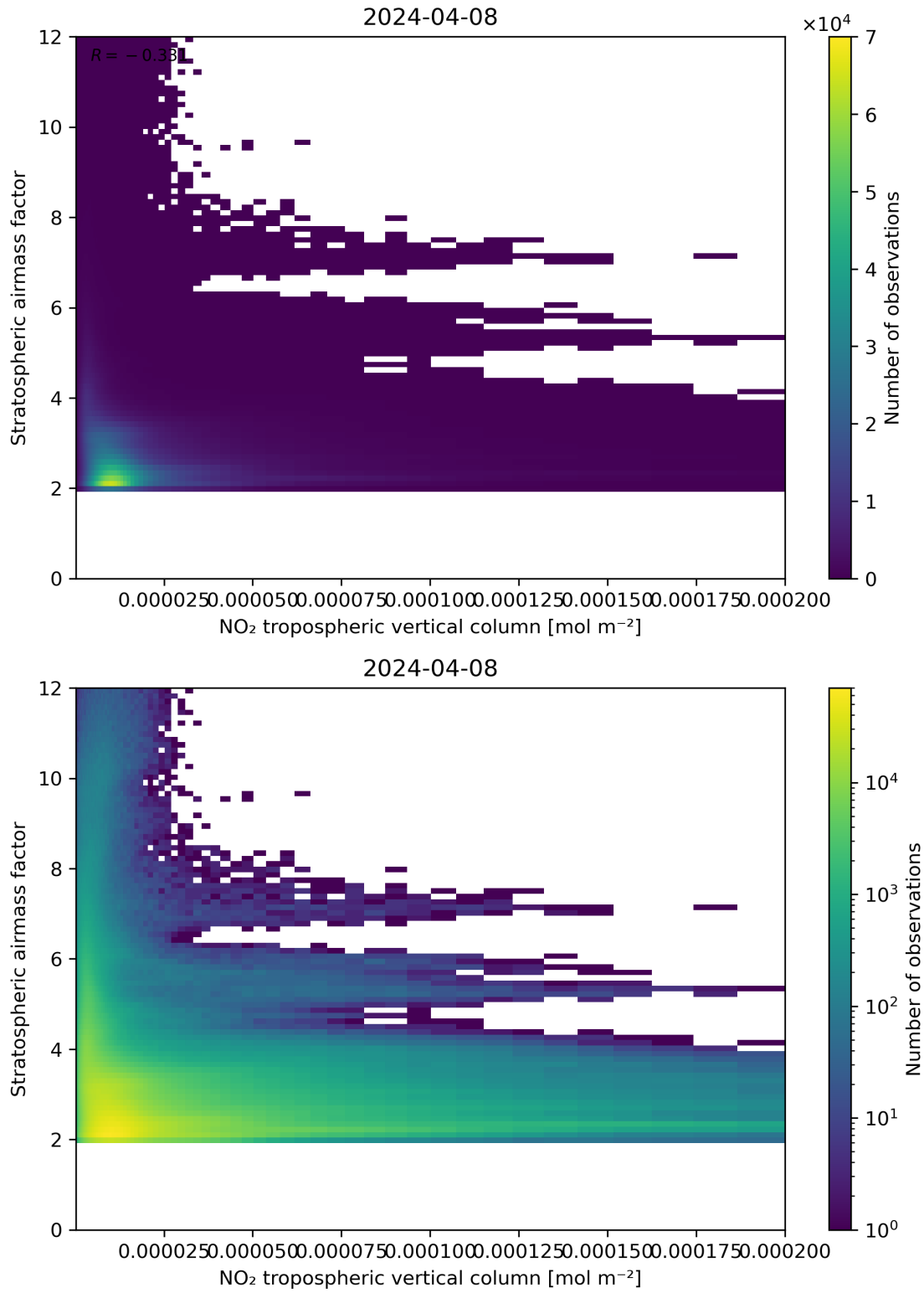
Figure 121: Scatter density plot of “NO 2 tropospheric vertical column” against “Stratospheric air mass factor” for 2024-04-07 to 2024-04-09.
