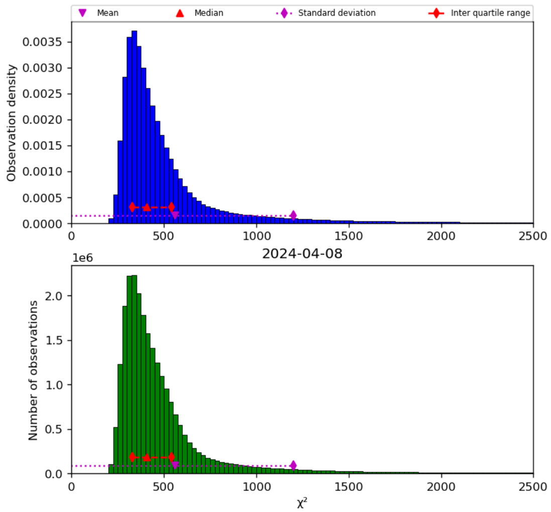
Figure 42: Histogram of “ \chi^2 ” for 2024-04-07 to 2024-04-09
