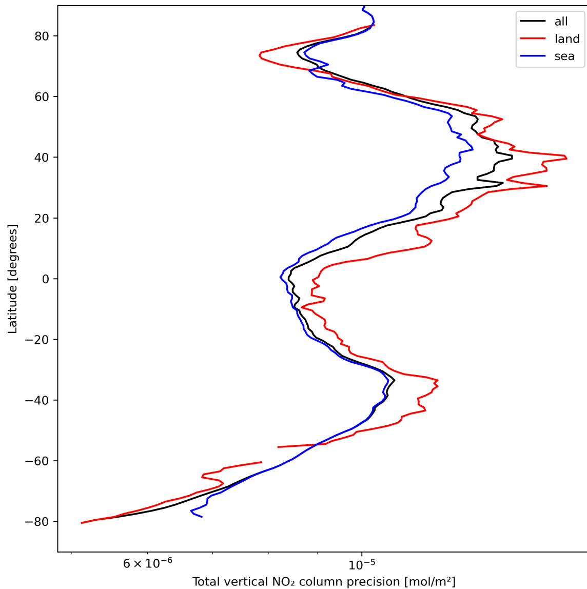
Figure 22: Zonal average of “Total vertical NO 2 column precision” for 2024-04-07 to 2024-04-09.
