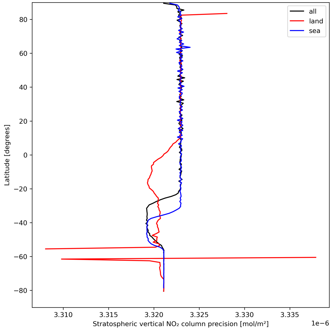
Figure 20: Zonal average of “Stratospheric vertical NO 2 column precision” for 2024-04-07 to 2024-04-09.
