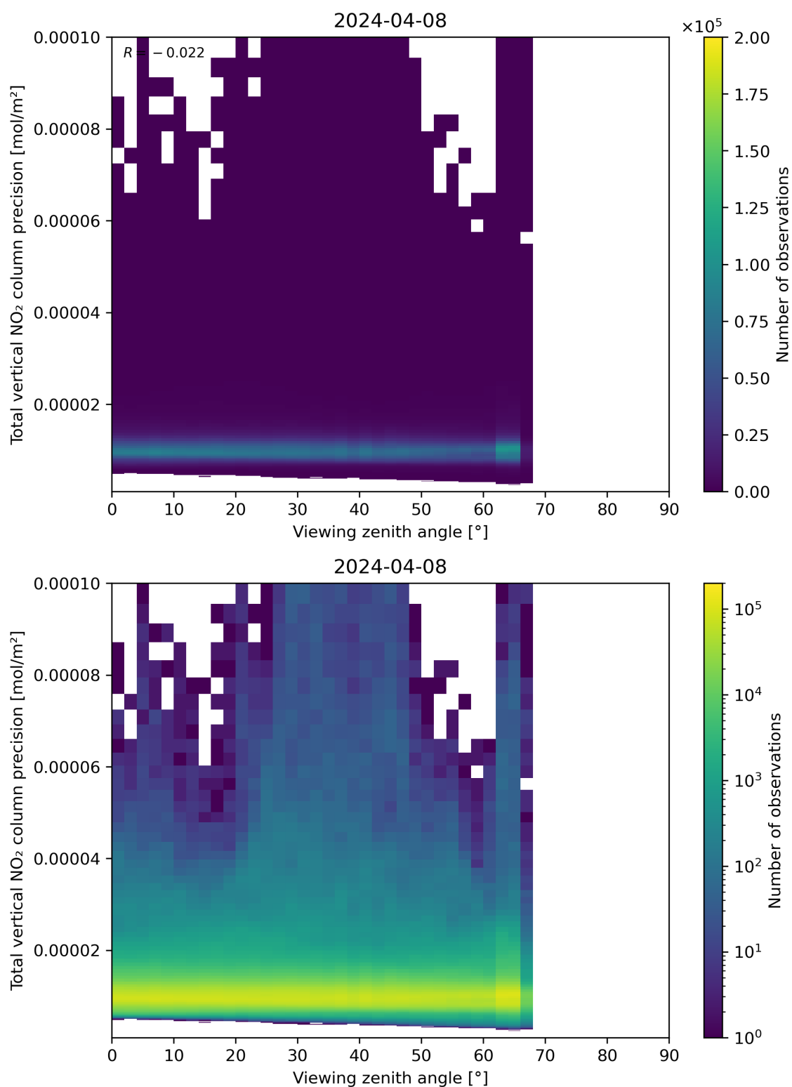
Figure 168: Scatter density plot of “Viewing zenith angle” against “Total vertical NO 2 column precision” for 2024-04-07 to 2024-04-09.
