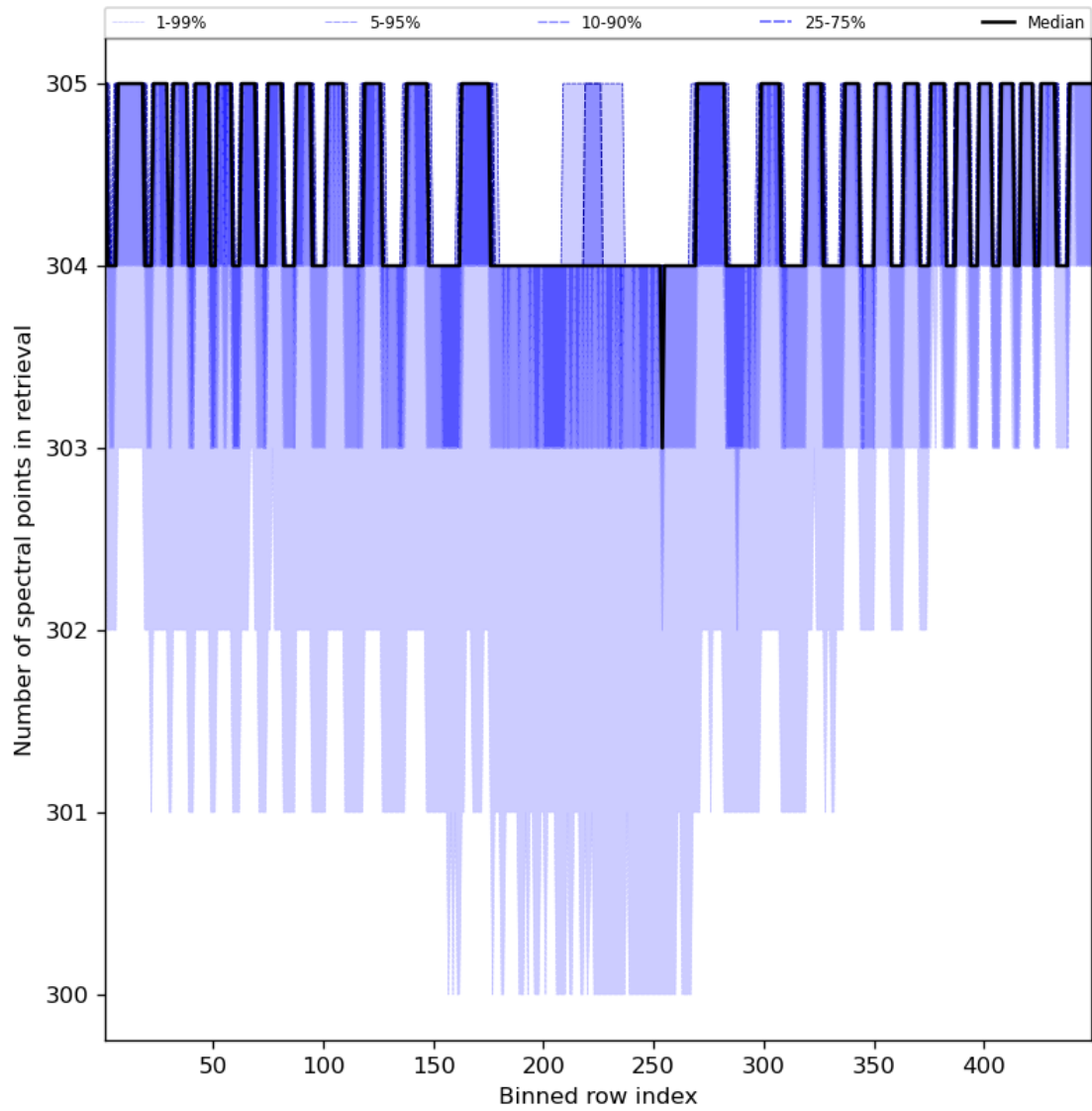
Figure 50: Along track statistics of “Number of spectral points in retrieval” for 2024-04-07 to 2024-04-09
