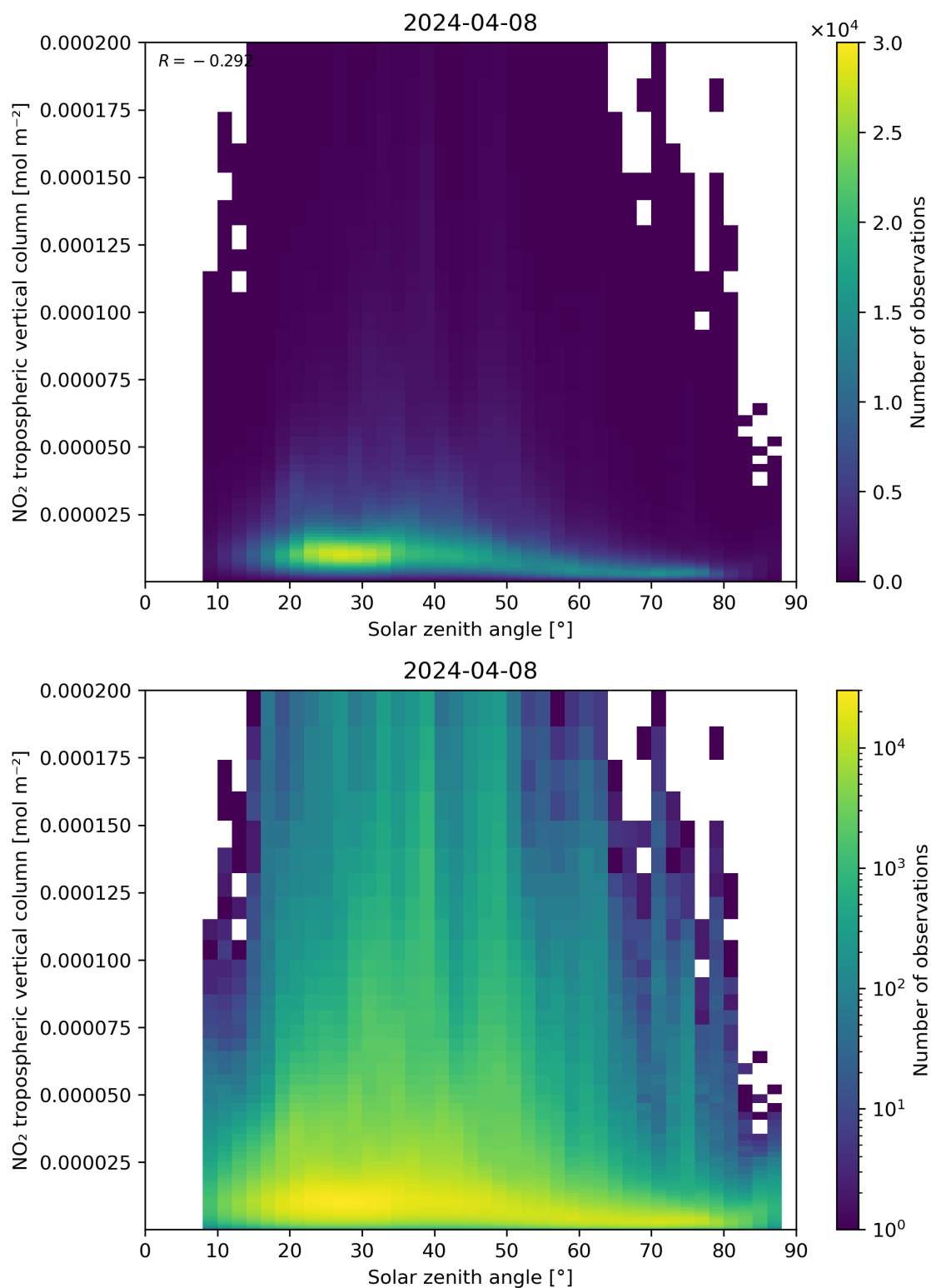
Figure 155: Scatter density plot of “Solar zenith angle” against “NO 2 tropospheric vertical column” for 2024-04-07 to 2024-04-09.
