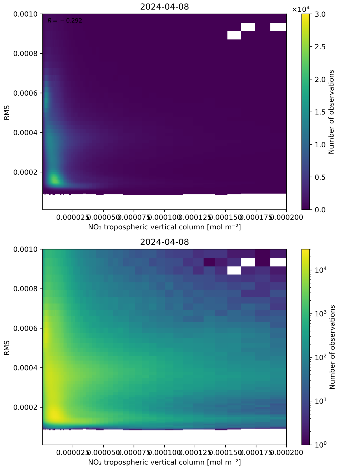
Figure 142: Scatter density plot of “NO 2 tropospheric vertical column” against “RMS” for 2024-04-07 to 2024-04-09.
