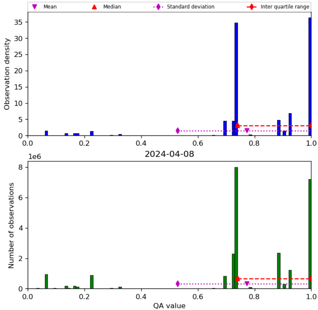
Figure 28: Histogram of “QA value” for 2024-04-07 to 2024-04-09
