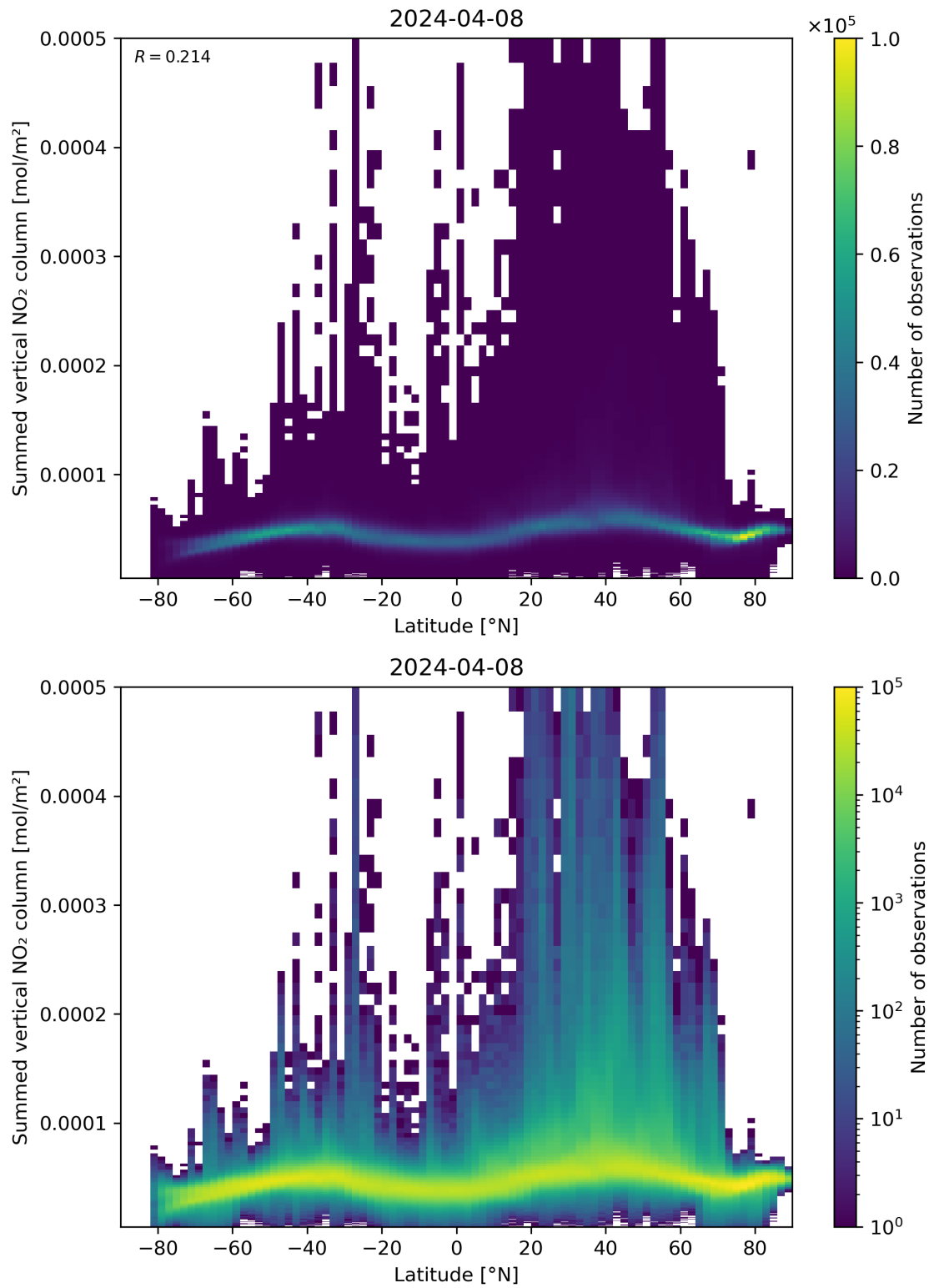
Figure 88: Scatter density plot of “Latitude” against “Summed vertical NO 2 column” for 2024-04-07 to 2024-04-09.
