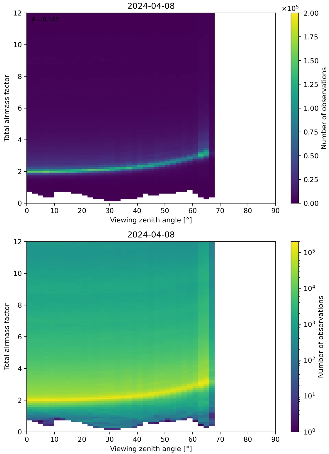
Figure 160: Scatter density plot of “Viewing zenith angle” against “Total airmass factor” for 2024-04-07 to 2024-04-09.
