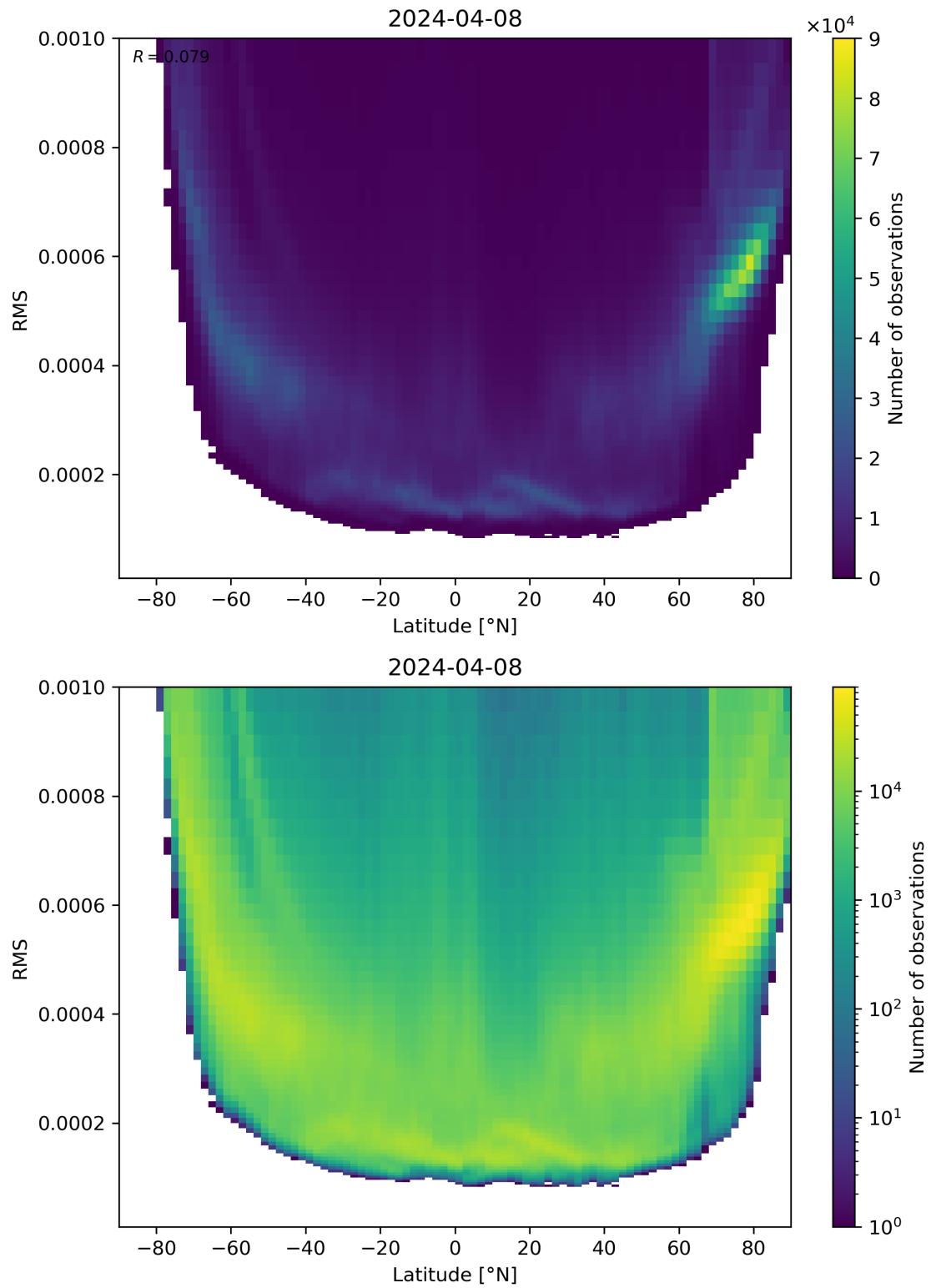
Figure 94: Scatter density plot of “Latitude” against “RMS” for 2024-04-07 to 2024-04-09.
