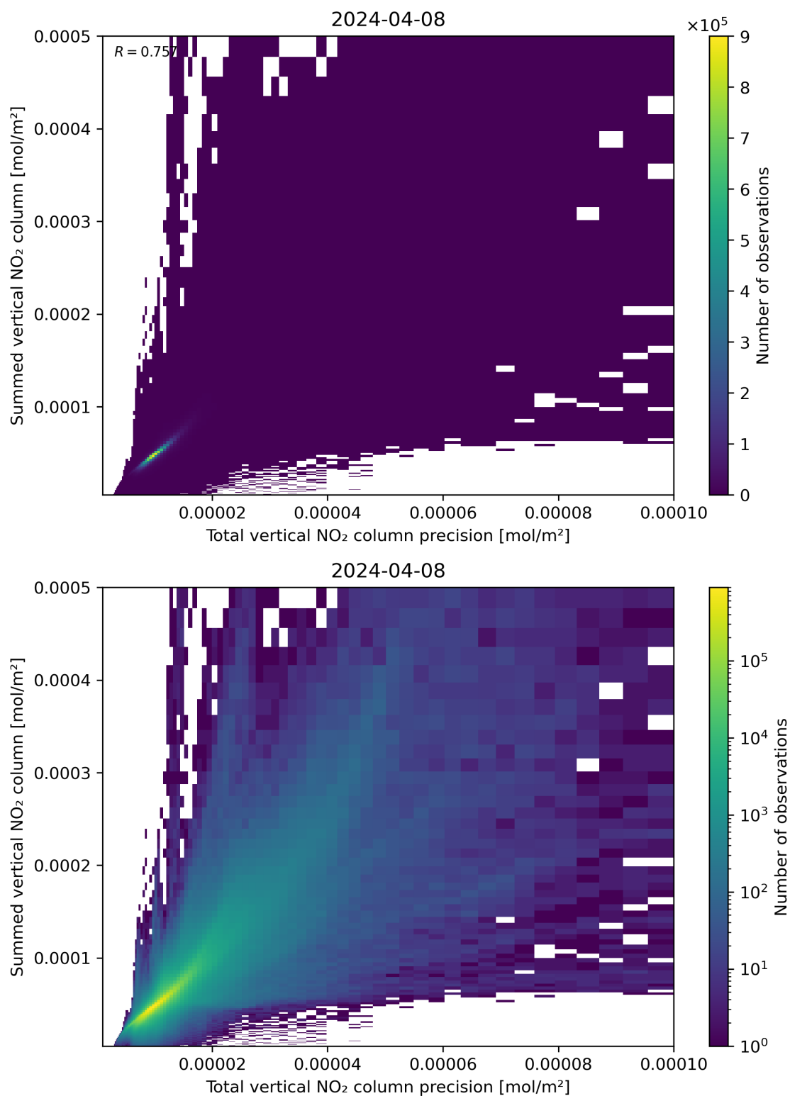
Figure 117: Scatter density plot of “Total vertical NO 2 column precision” against “Summed vertical NO 2 column” for 2024-04-07 to 2024-04-09.
