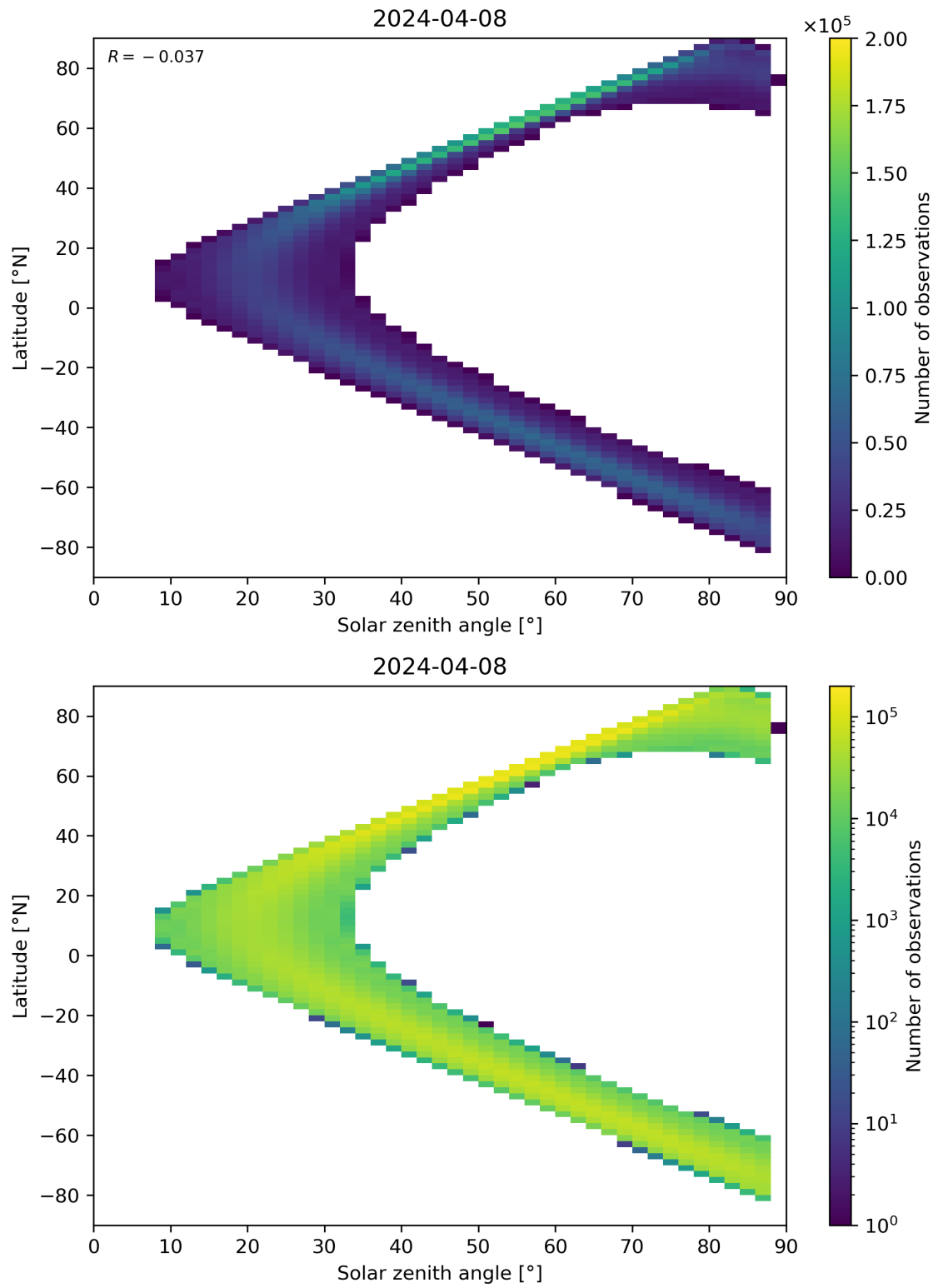
Figure 149: Scatter density plot of “Solar zenith angle” against “Latitude” for 2024-04-07 to 2024-04-09.
