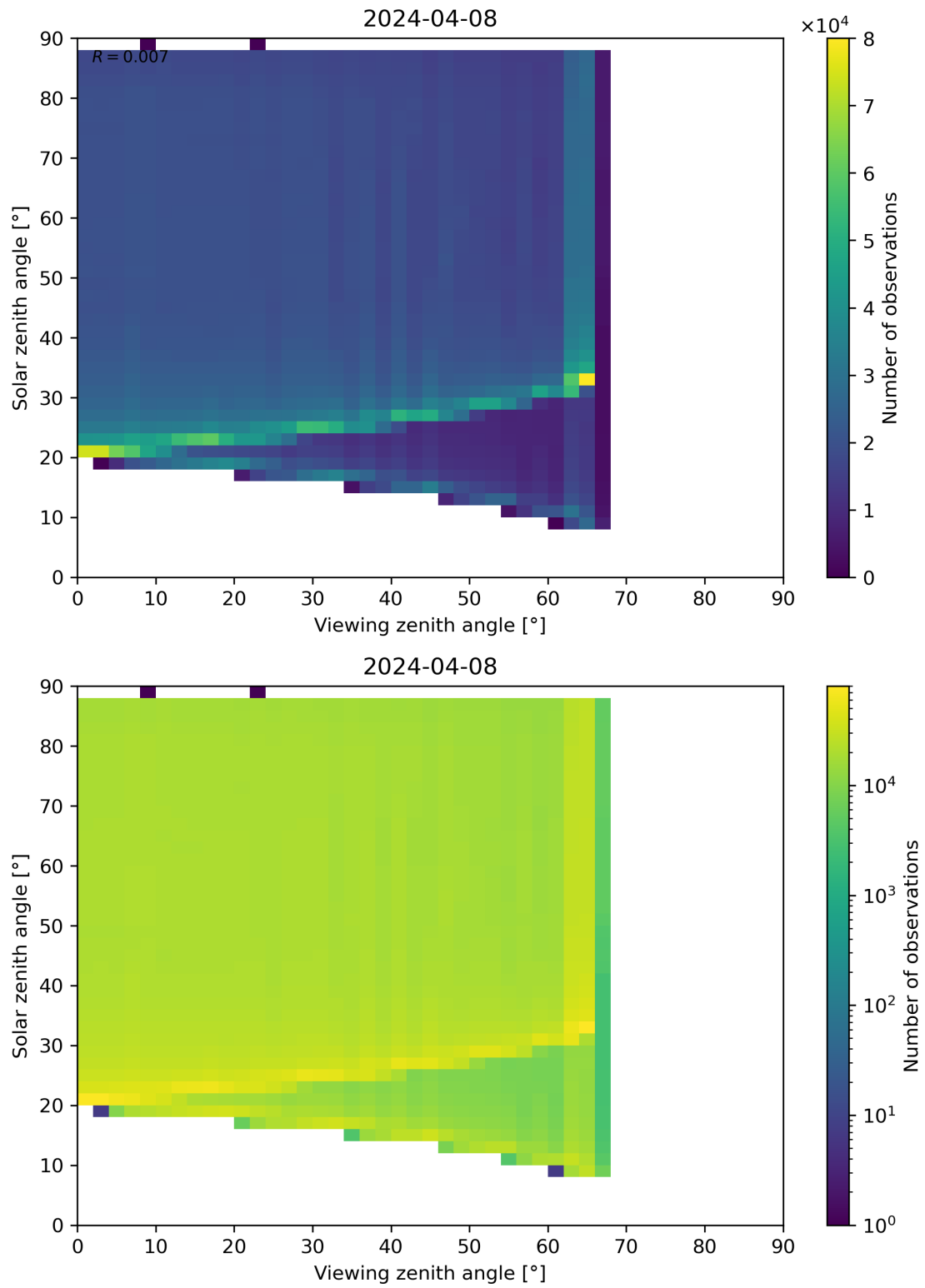
Figure 172: Scatter density plot of “Viewing zenith angle” against “Solar zenith angle” for 2024-04-07 to 2024-04-09.
