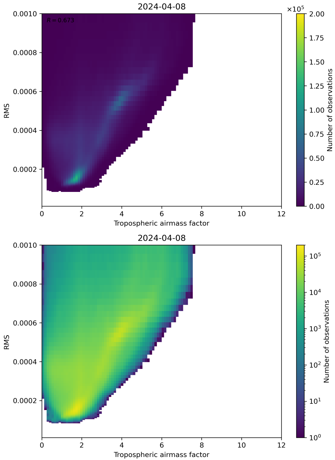
Figure 79: Scatter density plot of “Tropospheric airmass factor” against “RMS” for 2024-04-07 to 2024-04-09.
