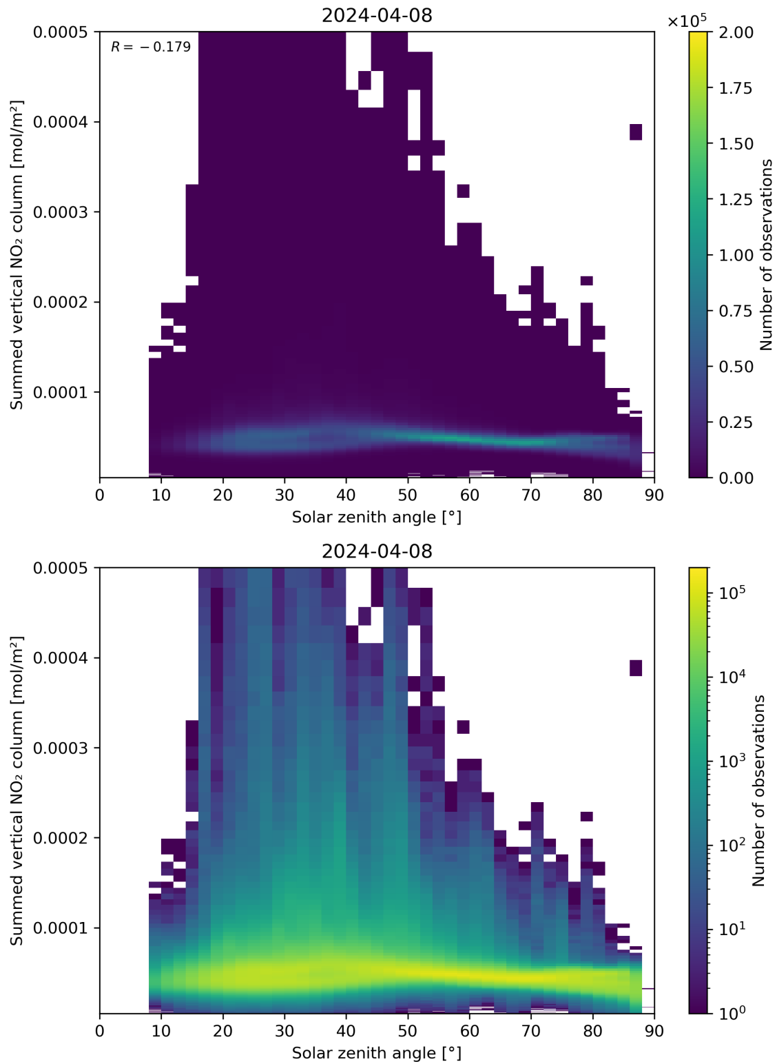
Figure 151: Scatter density plot of “Solar zenith angle” against “Summed vertical NO 2 column” for 2024-04-07 to 2024-04-09.
