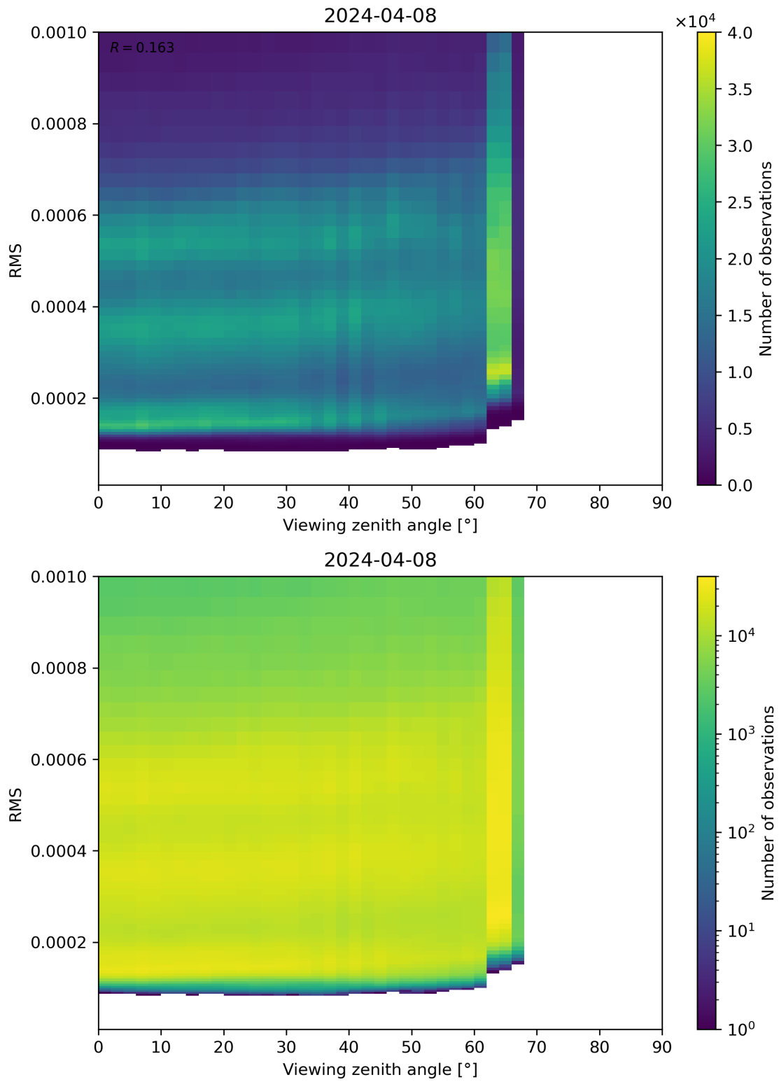
Figure 171: Scatter density plot of “Viewing zenith angle” against “RMS” for 2024-04-07 to 2024-04-09.
