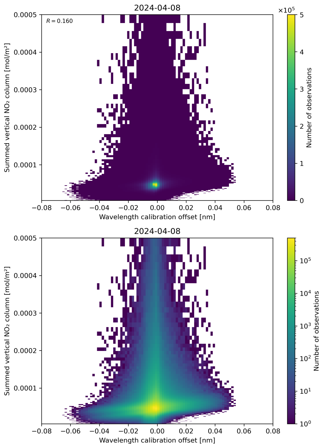
Figure 177: Scatter density plot of “Wavelength calibration offset” against “Summed vertical NO 2 column” for 2024-04-07 to 2024-04-09.
