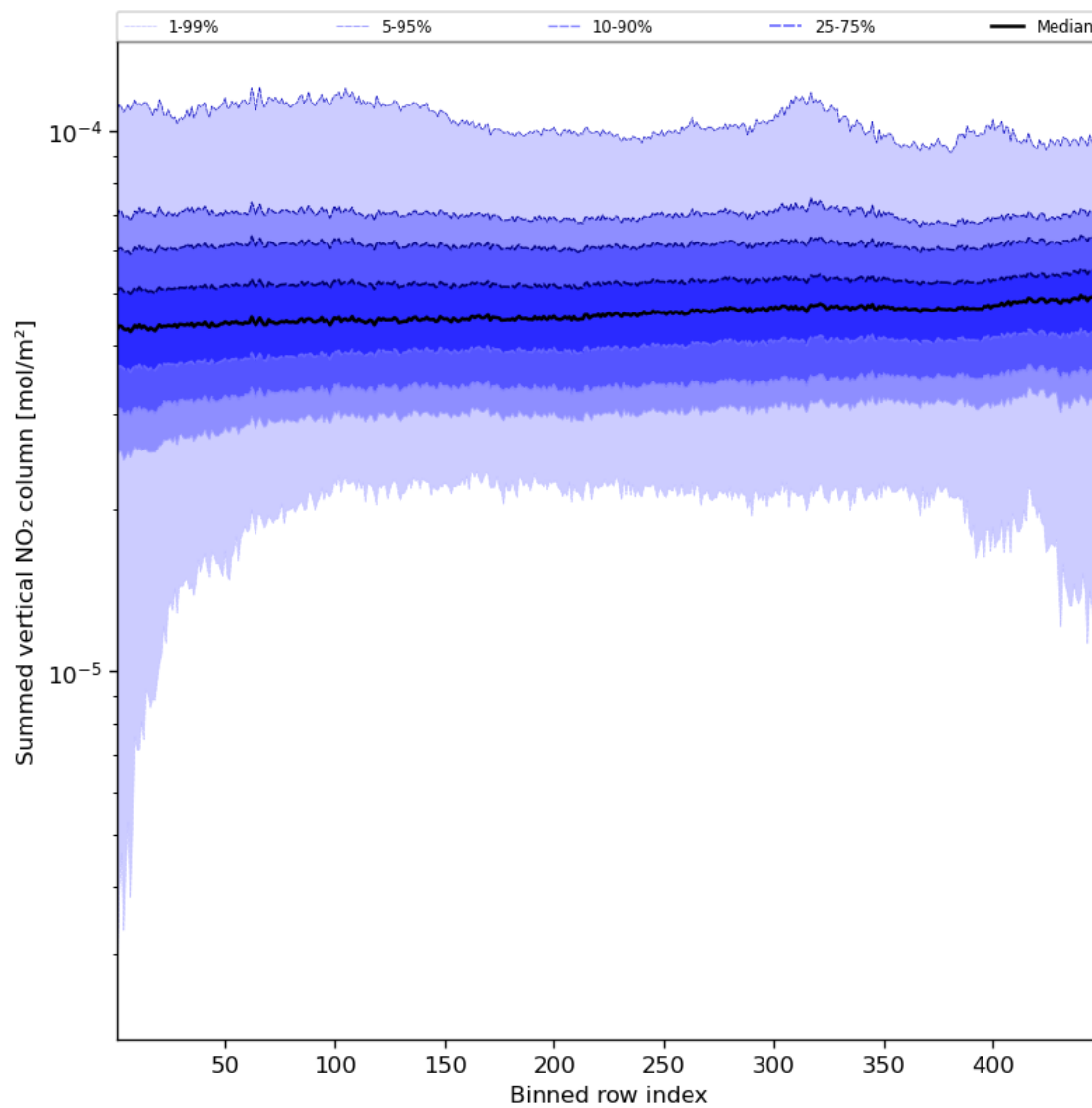
Figure 57: Along track statistics of “Summed vertical NO 2 column” for 2024-04-07 to 2024-04-09
