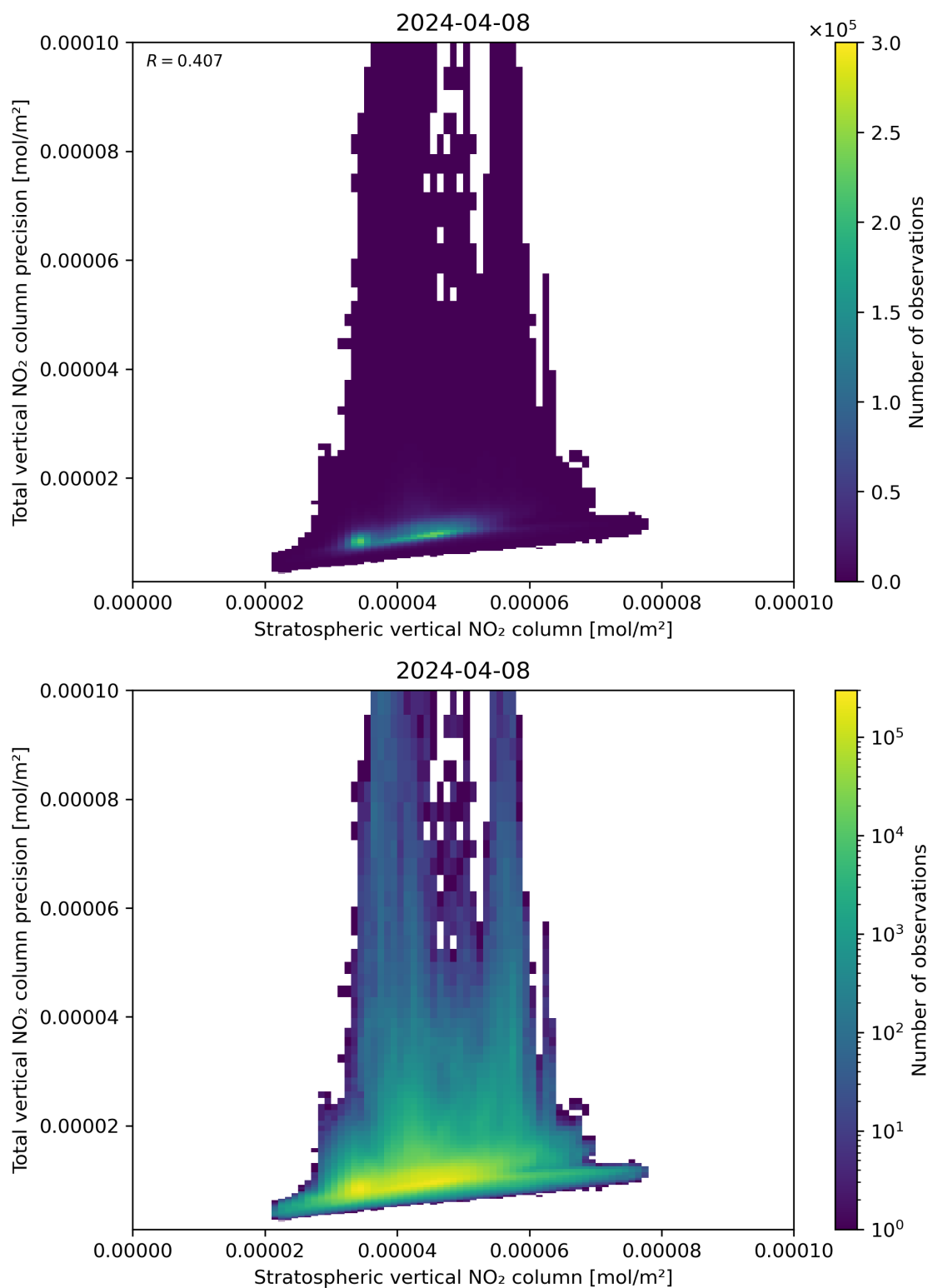
Figure 101: Scatter density plot of “Stratospheric vertical NO 2 column” against “Total vertical NO 2 column precision” for 2024-04-07 to 2024-04-09.
