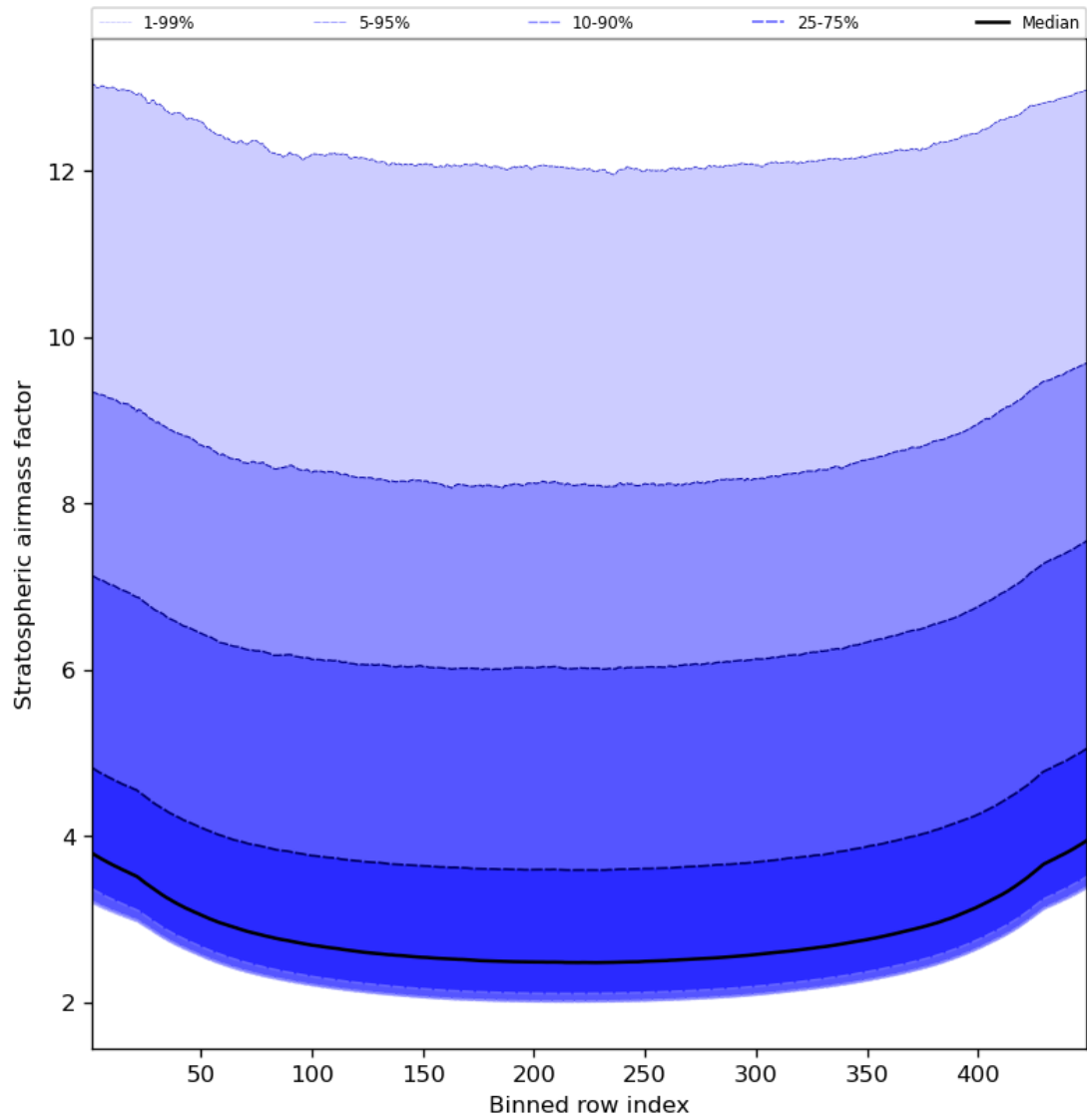
Figure 61: Along track statistics of “Stratospheric airmass factor” for 2024-04-07 to 2024-04-09
