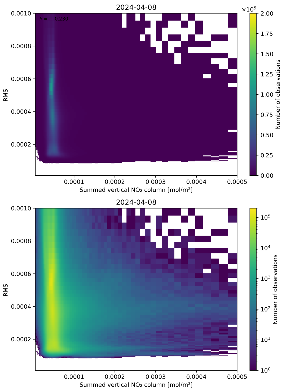
Figure 109: Scatter density plot of “Summed vertical NO 2 column” against “RMS” for 2024-04-07 to 2024-04-09.
