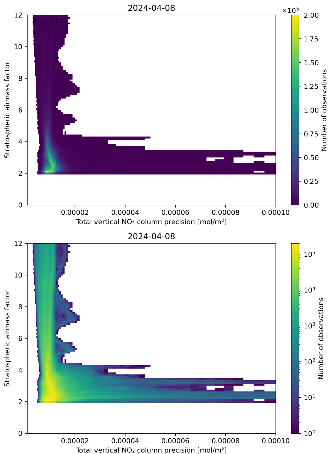
Figure 115: Scatter density plot of “Total vertical NO 2 column precision” against “Stratospheric air mass factor” for 2024-04-07 to 2024-04-09.
