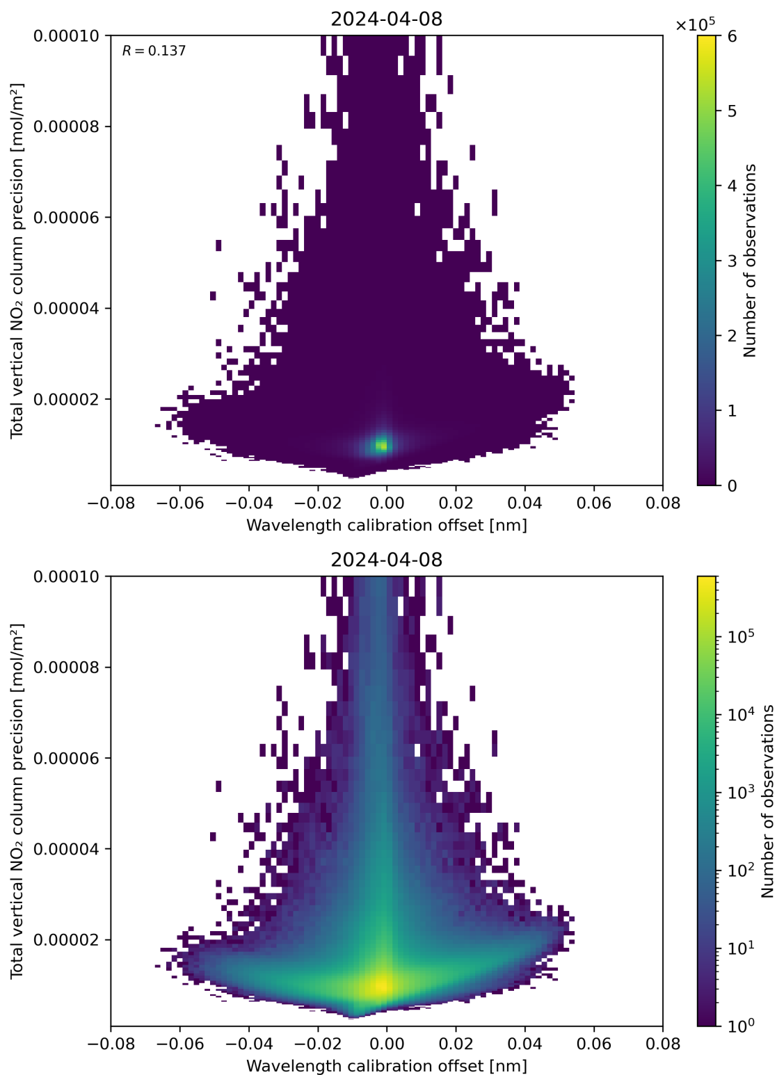
Figure 180: Scatter density plot of “Wavelength calibration offset” against “Total vertical NO 2 column precision” for 2024-04-07 to 2024-04-09.
