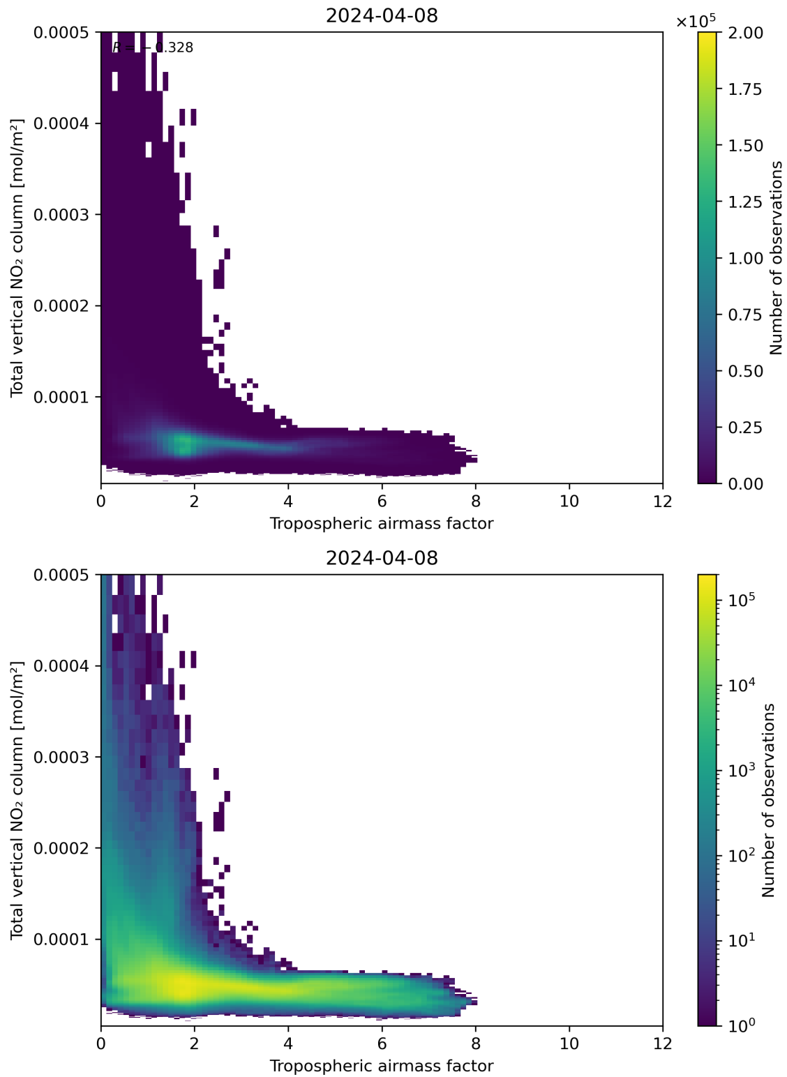
Figure 77: Scatter density plot of “Tropospheric airmass factor” against “Total vertical NO 2 column” for 2024-04-07 to 2024-04-09.
