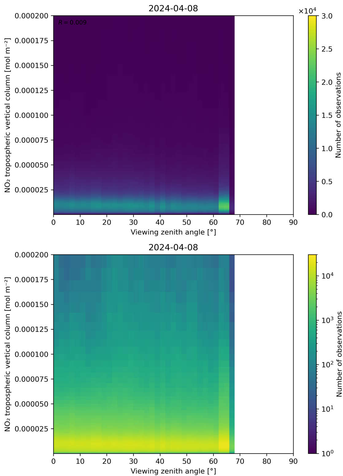
Figure 169: Scatter density plot of “Viewing zenith angle” against “NO 2 tropospheric vertical column” for 2024-04-07 to 2024-04-09.
