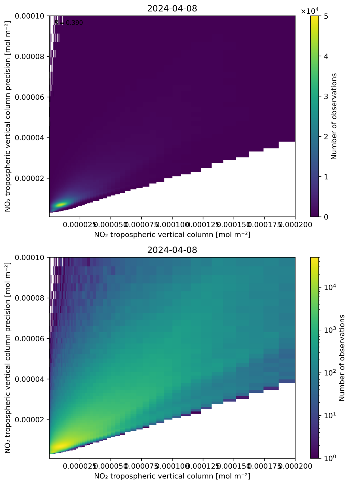
Figure 130: Scatter density plot of “NO 2 tropospheric vertical column” against “NO 2 tropospheric vertical column precision” for 2024-04-07 to 2024-04-09.
