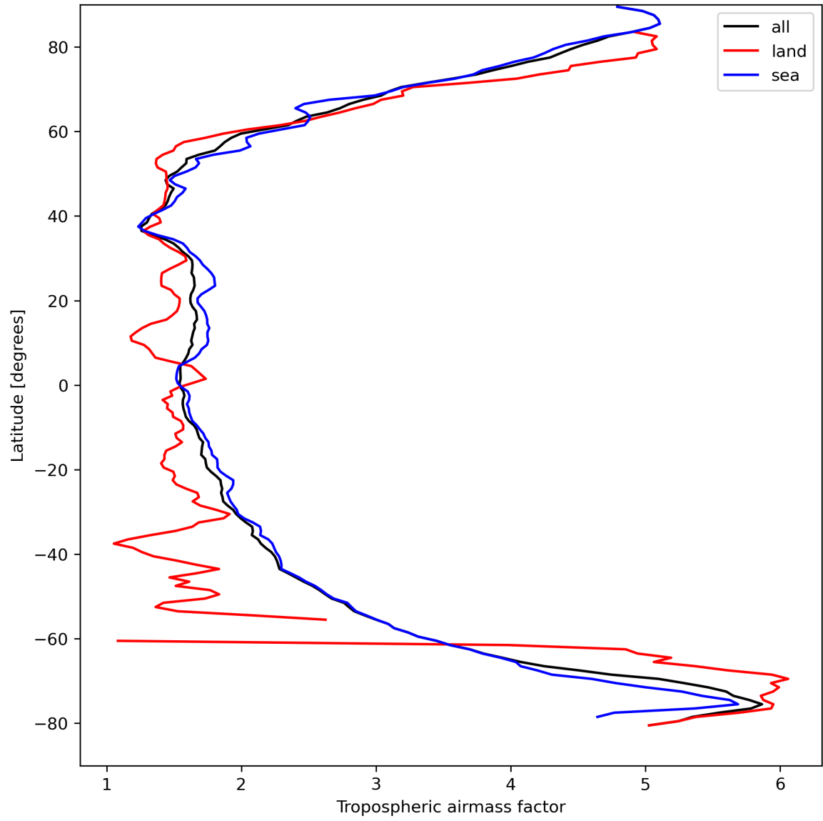
Figure 14: Zonal average of “Tropospheric air mass factor” for 2024-04-07 to 2024-04-09.
