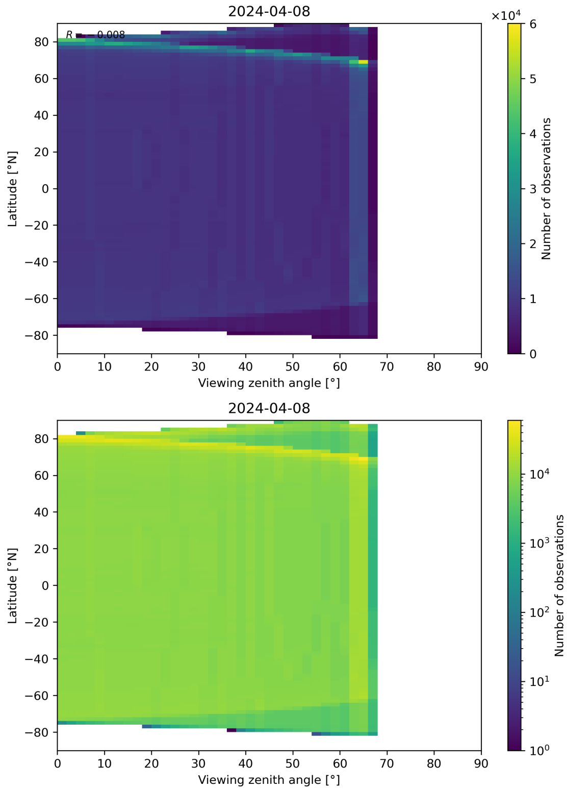
Figure 163: Scatter density plot of “Viewing zenith angle” against “Latitude” for 2024-04-07 to 2024-04-09.
