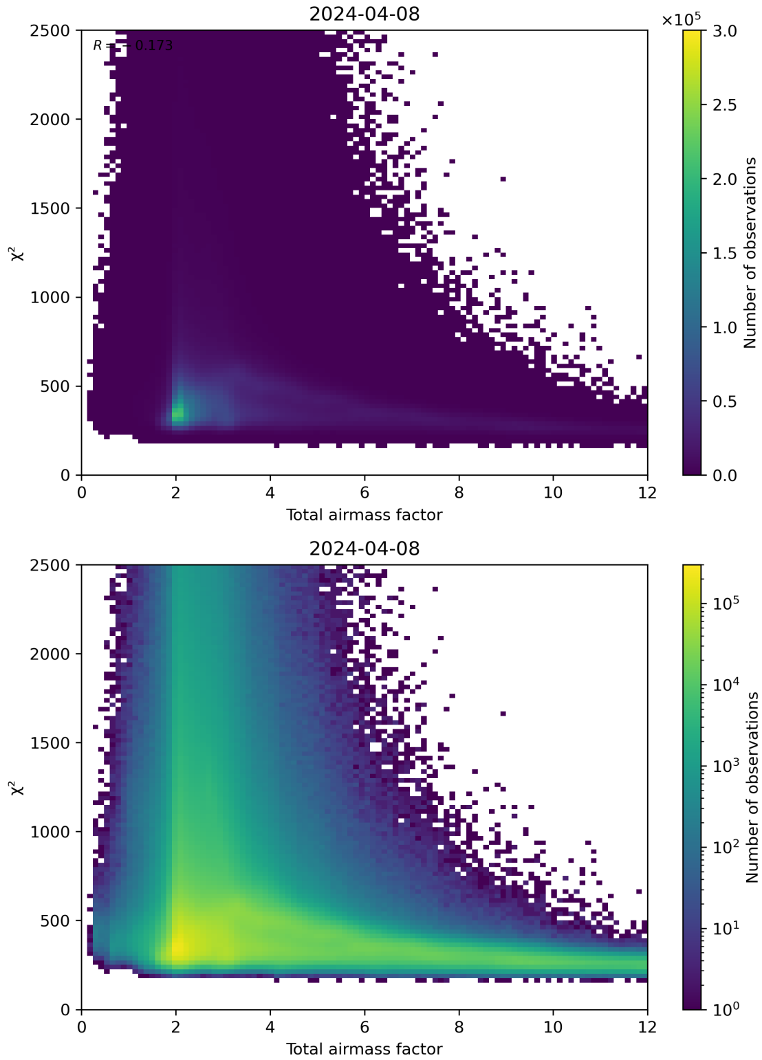
Figure 63: Scatter density plot of “Total airmass factor” against “ \chi^2 ” for 2024-04-07 to 2024-04-09.
