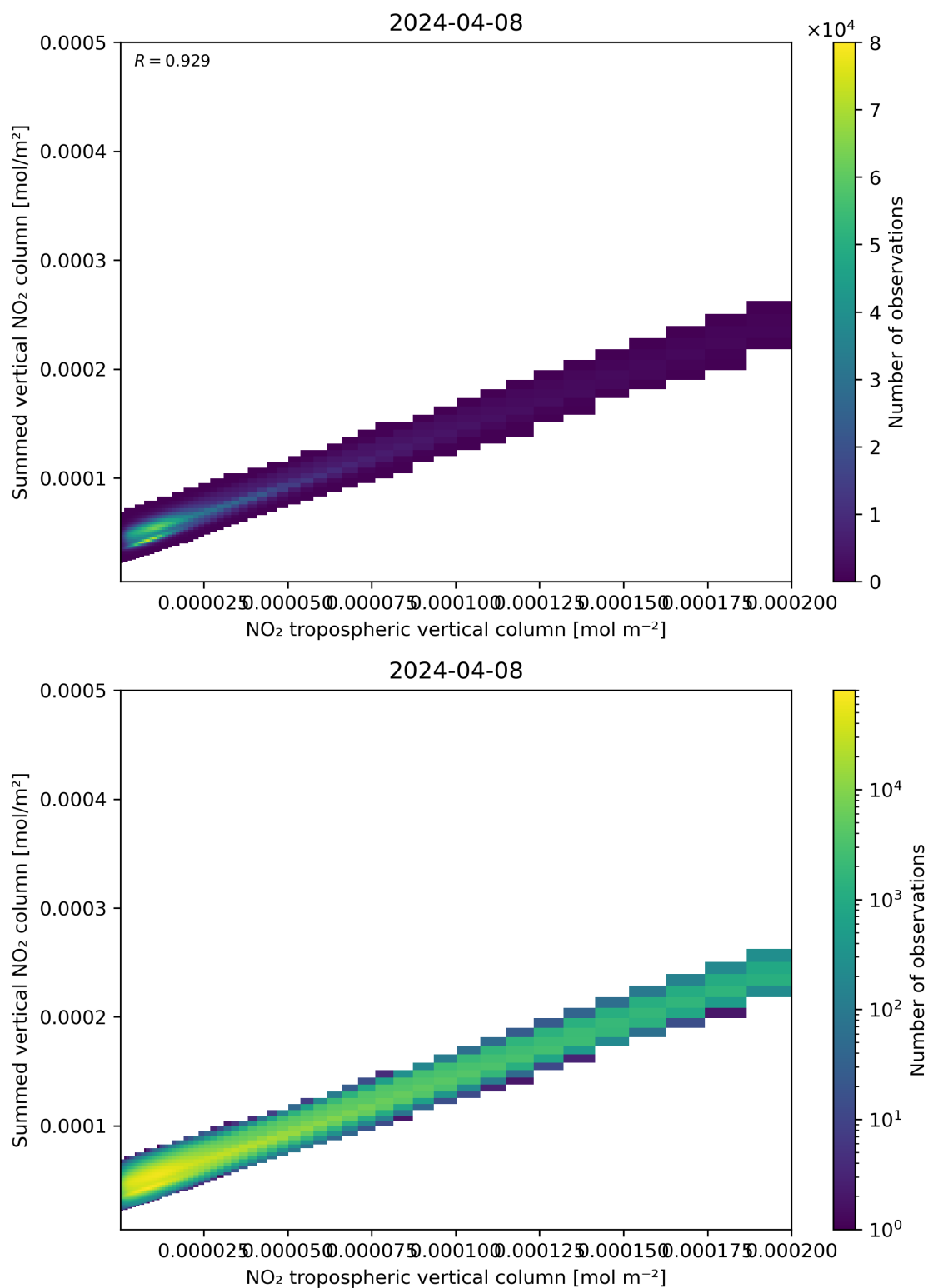
Figure 126: Scatter density plot of “NO 2 tropospheric vertical column” against “Summed vertical NO 2 column” for 2024-04-07 to 2024-04-09.
