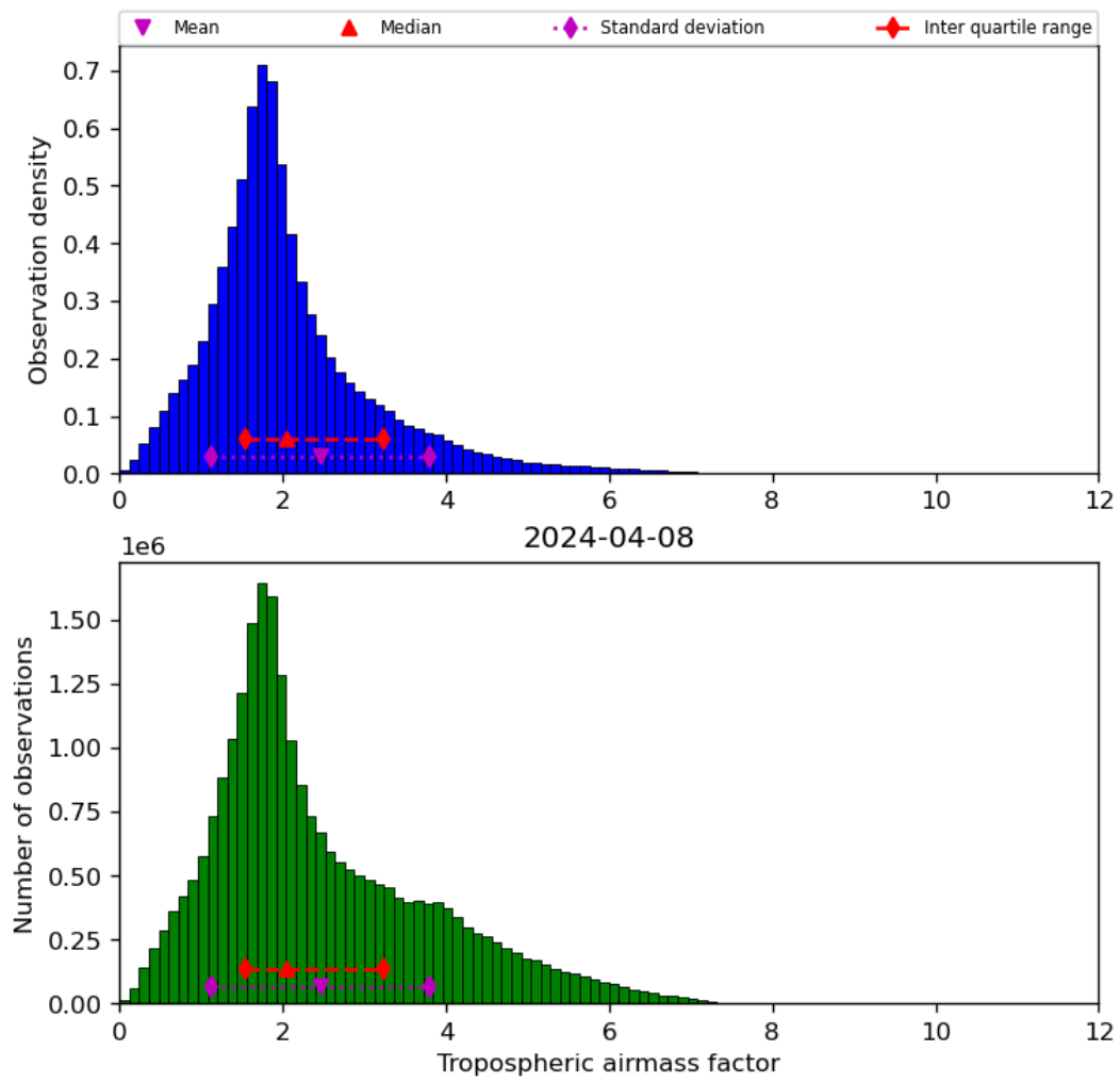
Figure 31: Histogram of “Tropospheric airmass factor” for 2024-04-07 to 2024-04-09
