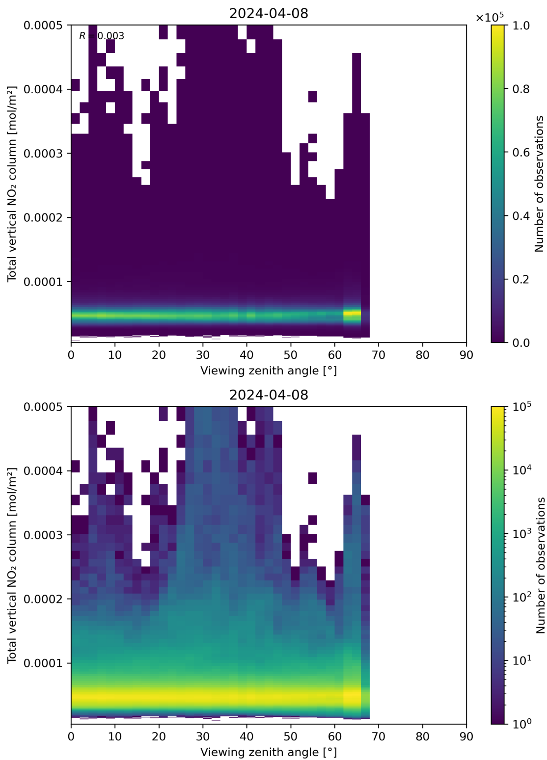
Figure 167: Scatter density plot of “Viewing zenith angle” against “Total vertical NO 2 column” for 2024-04-07 to 2024-04-09.
