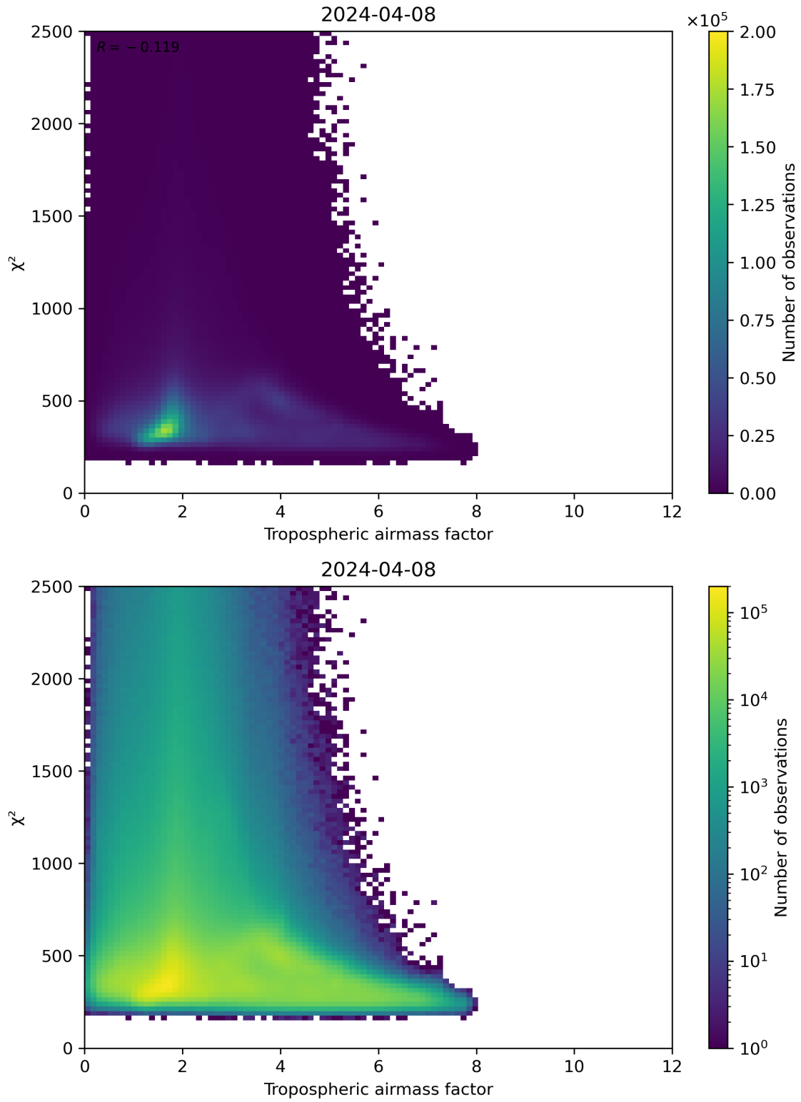
Figure 73: Scatter density plot of “Tropospheric airmass factor” against “ \chi^2 ” for 2024-04-07 to 2024-04-09.
