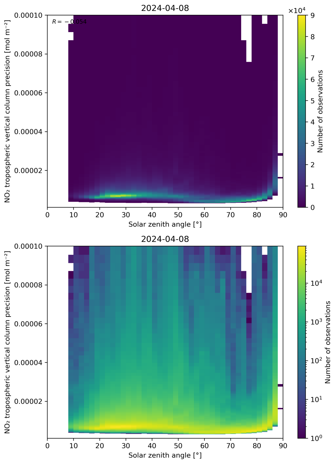
Figure 156: Scatter density plot of “Solar zenith angle” against “NO 2 tropospheric vertical column precision” for 2024-04-07 to 2024-04-09.
