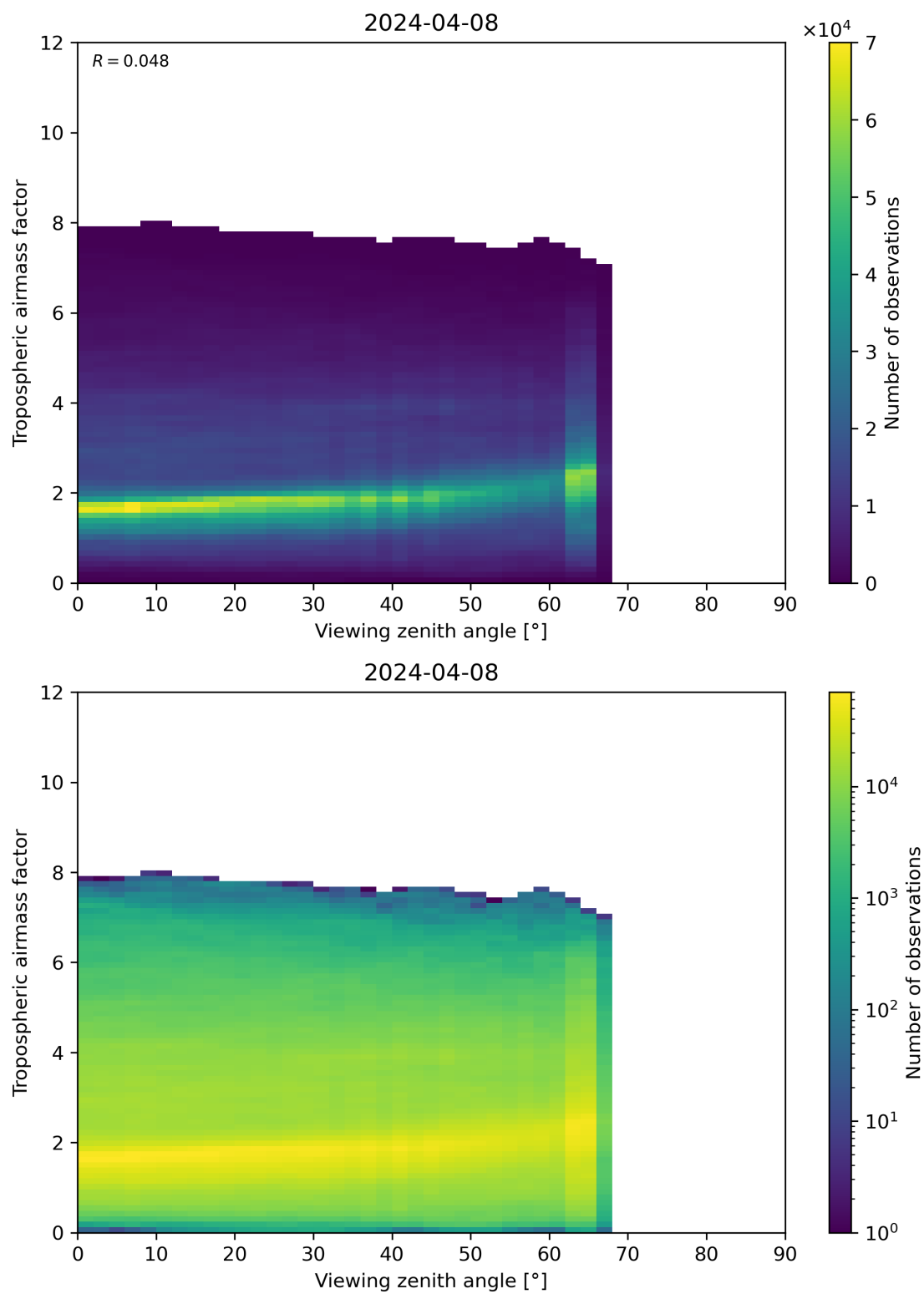
Figure 161: Scatter density plot of “Viewing zenith angle” against “Tropospheric airmass factor” for 2024-04-07 to 2024-04-09.
