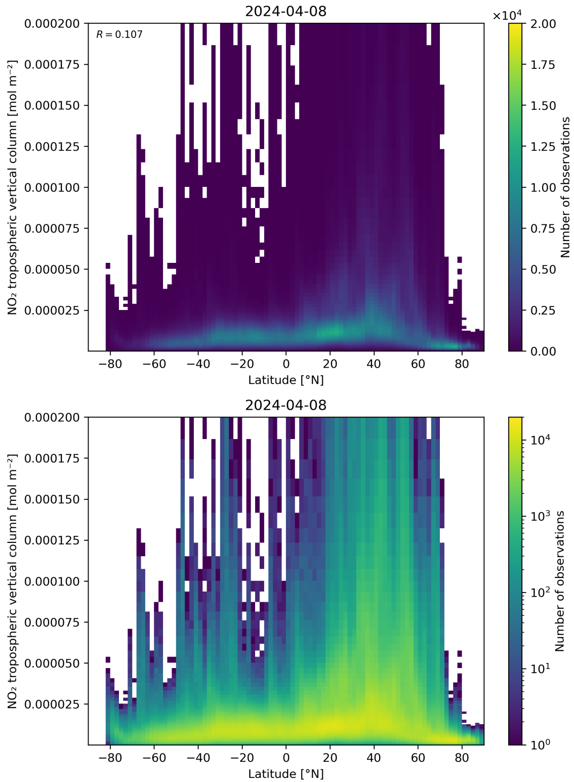
Figure 92: Scatter density plot of “Latitude” against “NO 2 tropospheric vertical column” for 2024-04-07 to 2024-04-09.
