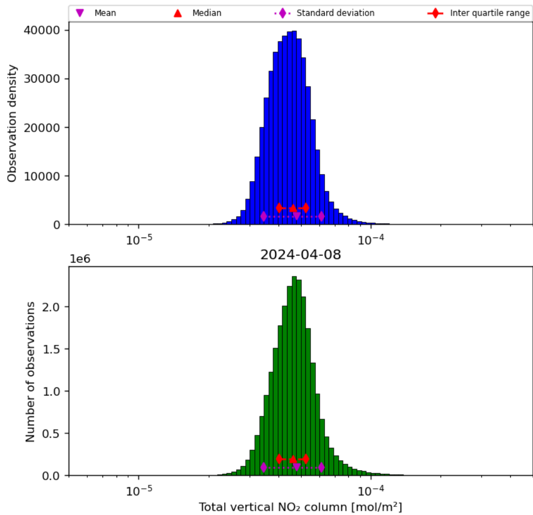
Figure 38: Histogram of "Total vertical NO 2 column" for 2024-04-07 to 2024-04-09
