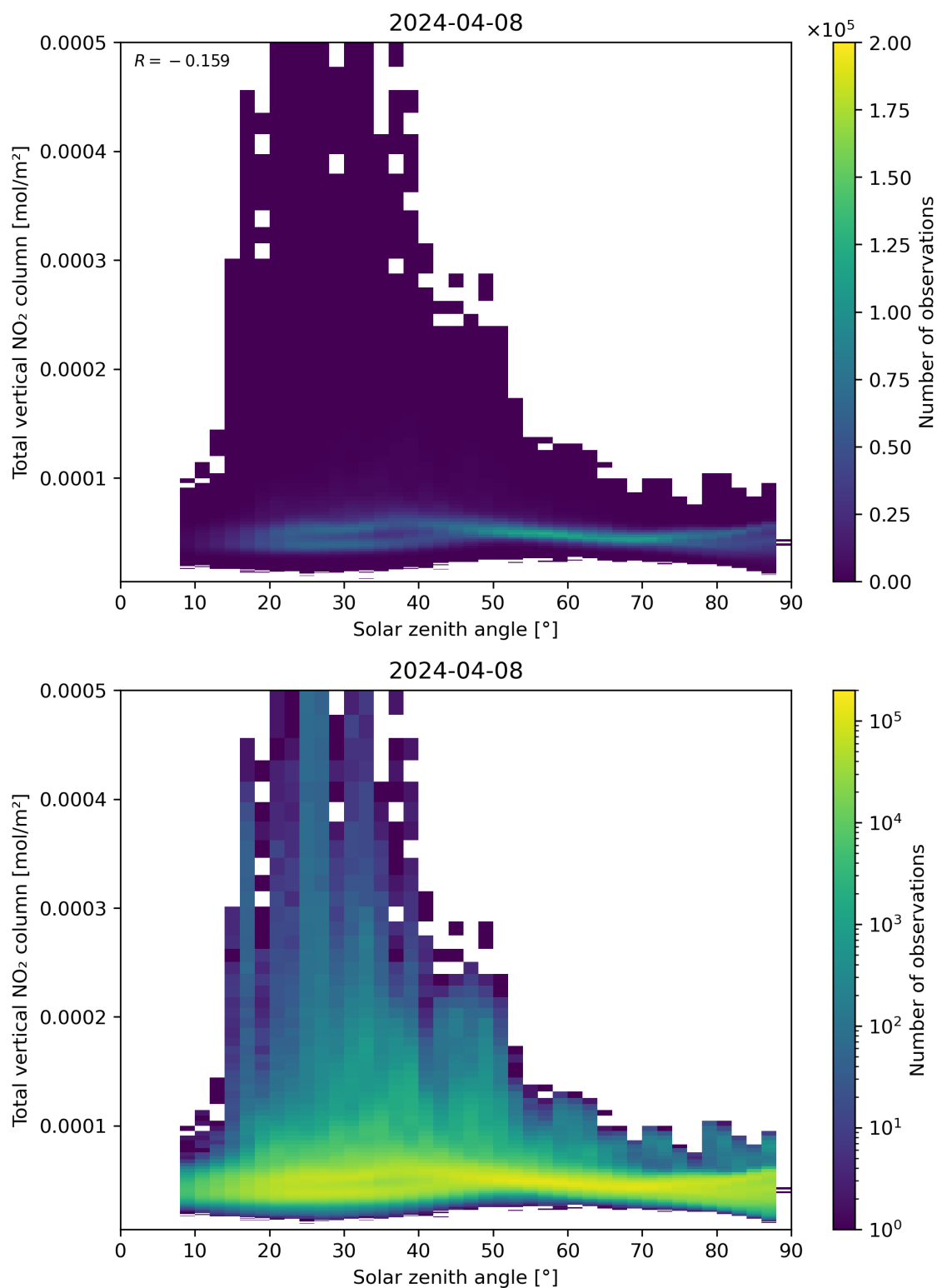
Figure 153: Scatter density plot of “Solar zenith angle” against “Total vertical NO 2 column” for 2024-04-07 to 2024-04-09.
