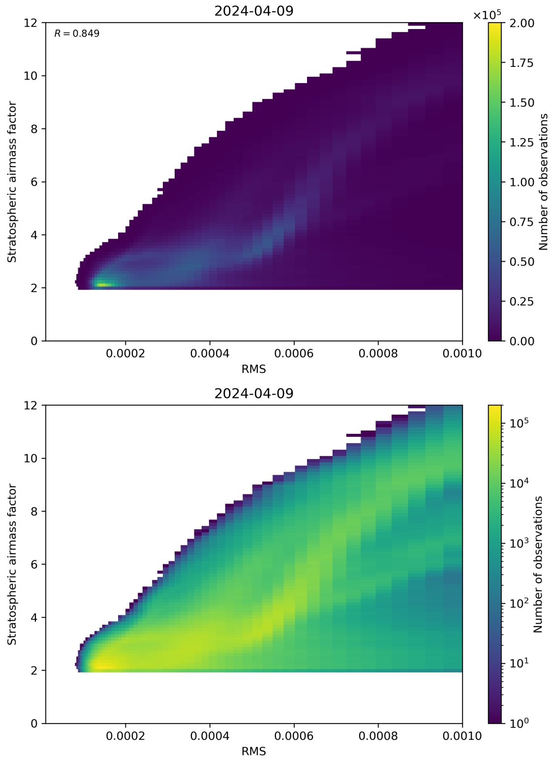
Figure 144: Scatter density plot of “RMS” against “Stratospheric airmass factor” for 2024-04-08 to 2024-04-10.
