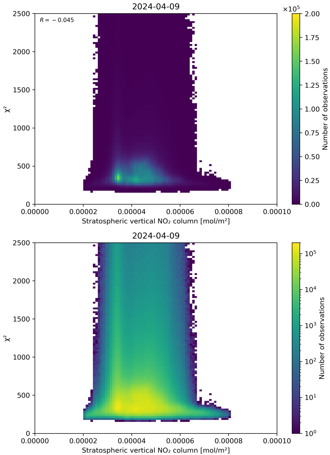
Figure 97: Scatter density plot of “Stratospheric vertical NO 2 column” against “ \chi^2 ” for 2024-04-08 to 2024-04-10.
