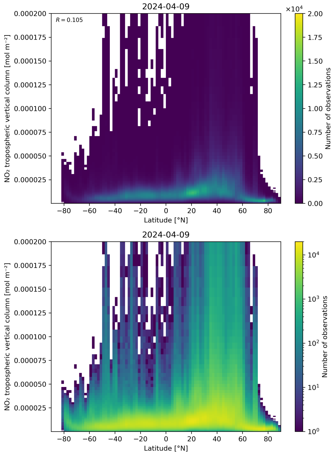
Figure 92: Scatter density plot of “Latitude” against “NO 2 tropospheric vertical column” for 2024-04-08 to 2024-04-10.
