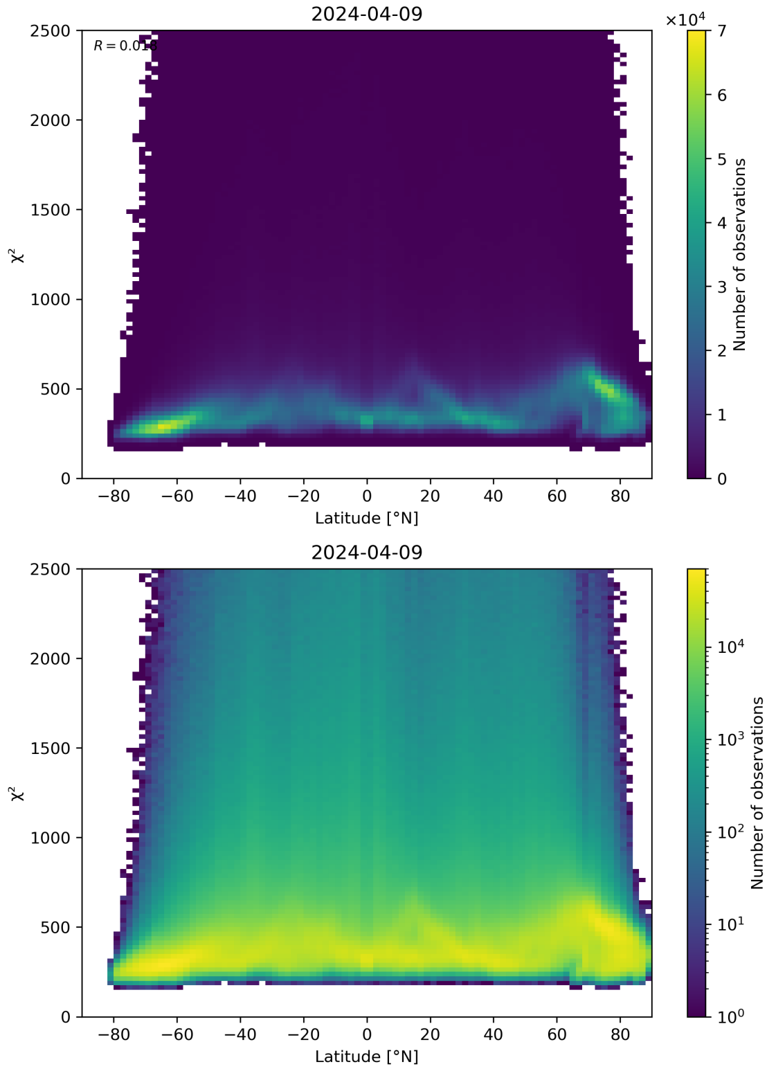
Figure 86: Scatter density plot of “Latitude” against “ \chi^2 ” for 2024-04-08 to 2024-04-10.
