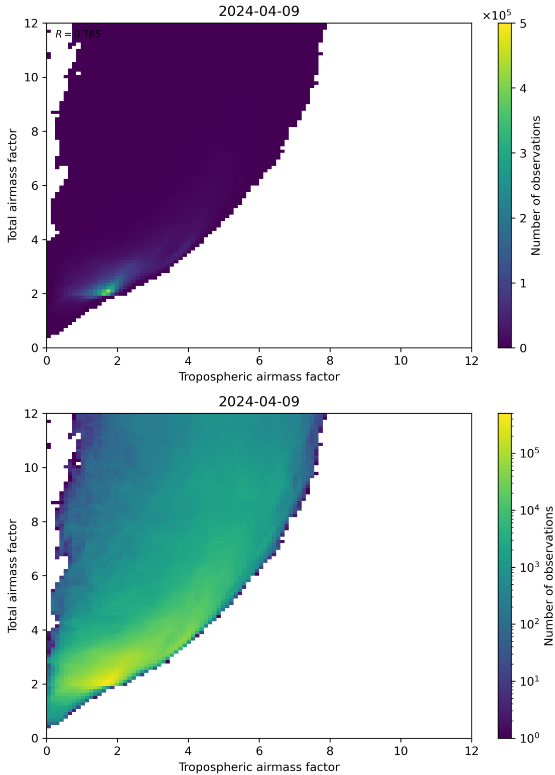
Figure 72: Scatter density plot of “Tropospheric airmass factor” against “Total airmass factor” for 2024-04-08 to 2024-04-10.
