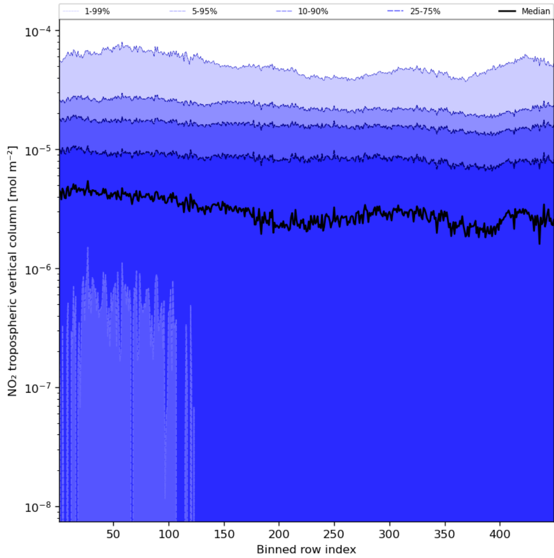
Figure 46: Along track statistics of “NO 2 tropospheric vertical column” for 2024-04-08 to 2024-04-10
