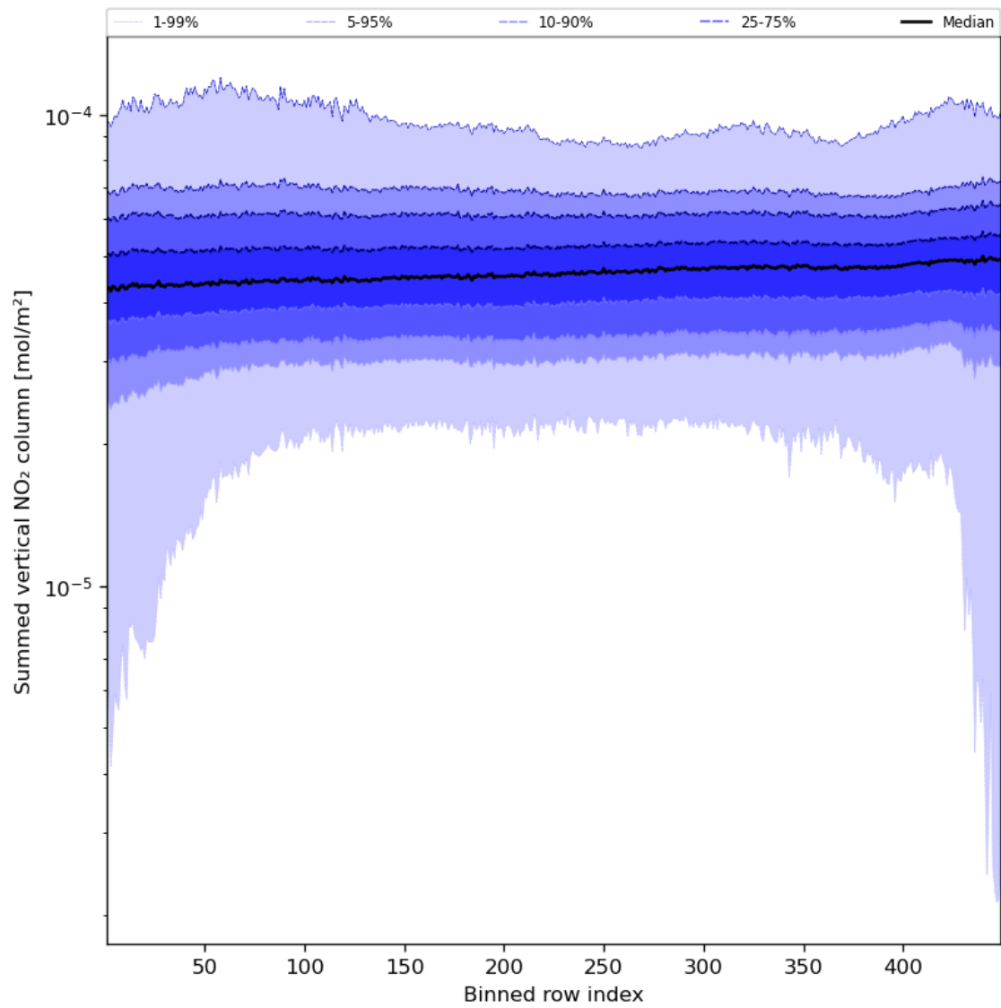
Figure 57: Along track statistics of “Summed vertical NO 2 column” for 2024-04-08 to 2024-04-10
