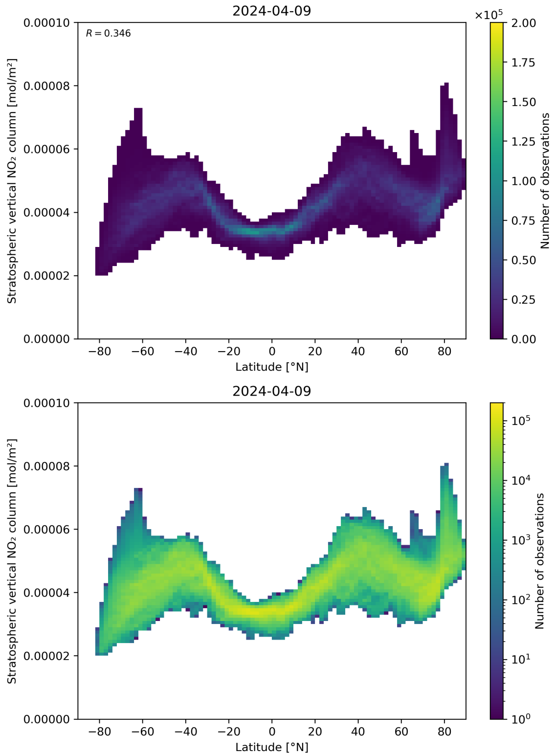
Figure 87: Scatter density plot of “Latitude” against “Stratospheric vertical NO 2 column” for 2024-04-08 to 2024-04-10.
