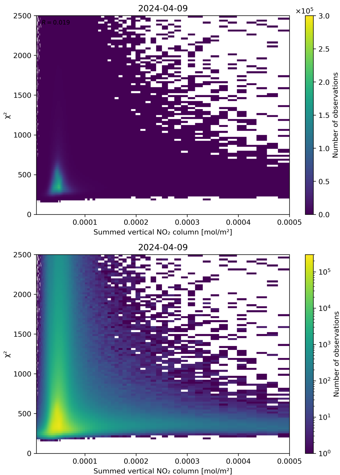
Figure 104: Scatter density plot of “Summed vertical NO 2 column” against “ \chi^2 ” for 2024-04-08 to 2024-04-10.
