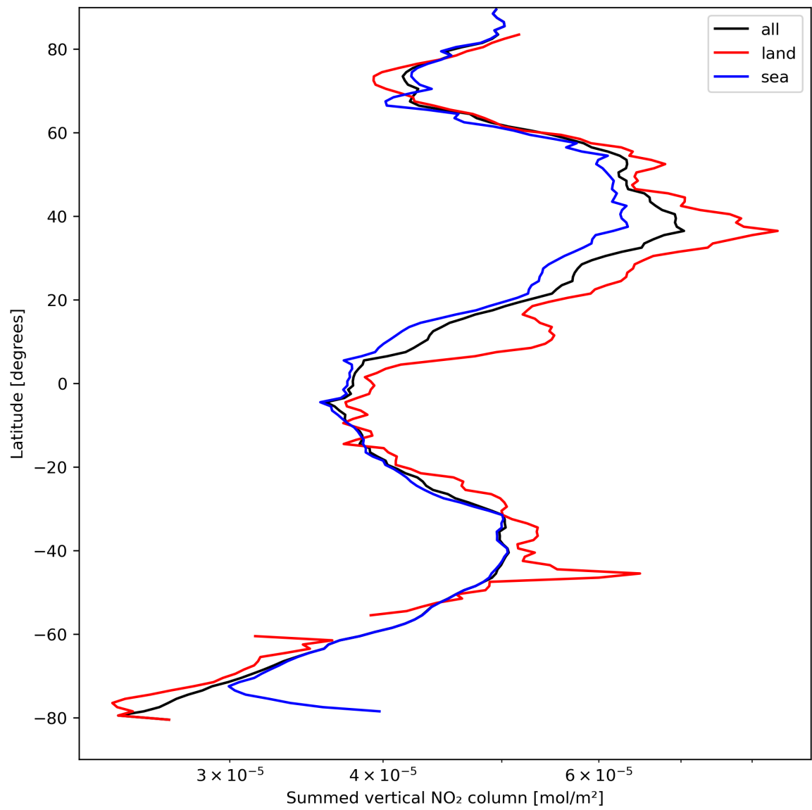
Figure 23: Zonal average of “Summed vertical NO 2 column” for 2024-04-08 to 2024-04-10.
