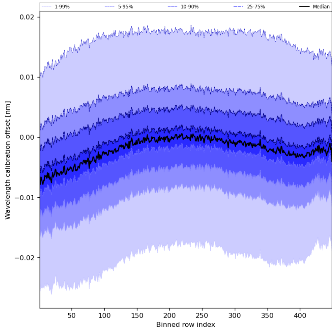
Figure 52: Along track statistics of “Wavelength calibration offset” for 2024-04-08 to 2024-04-10
