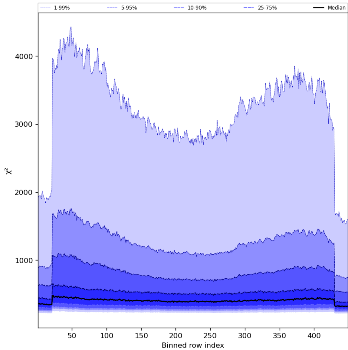
Figure 59: Along track statistics of “ \chi^2 ” for 2024-04-08 to 2024-04-10
