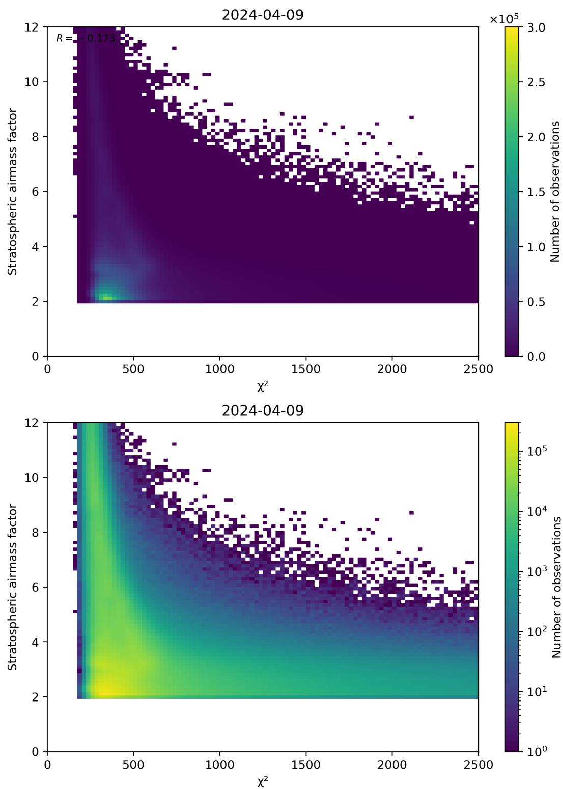
Figure 81: Scatter density plot of “ \chi^2 ” against “Stratospheric airmass factor” for 2024-04-08 to 2024-04-10.
