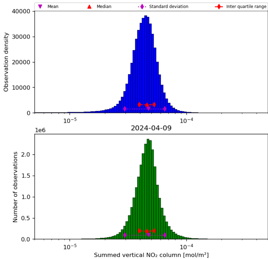
Figure 40: Histogram of “Summed vertical NO 2 column” for 2024-04-08 to 2024-04-10
