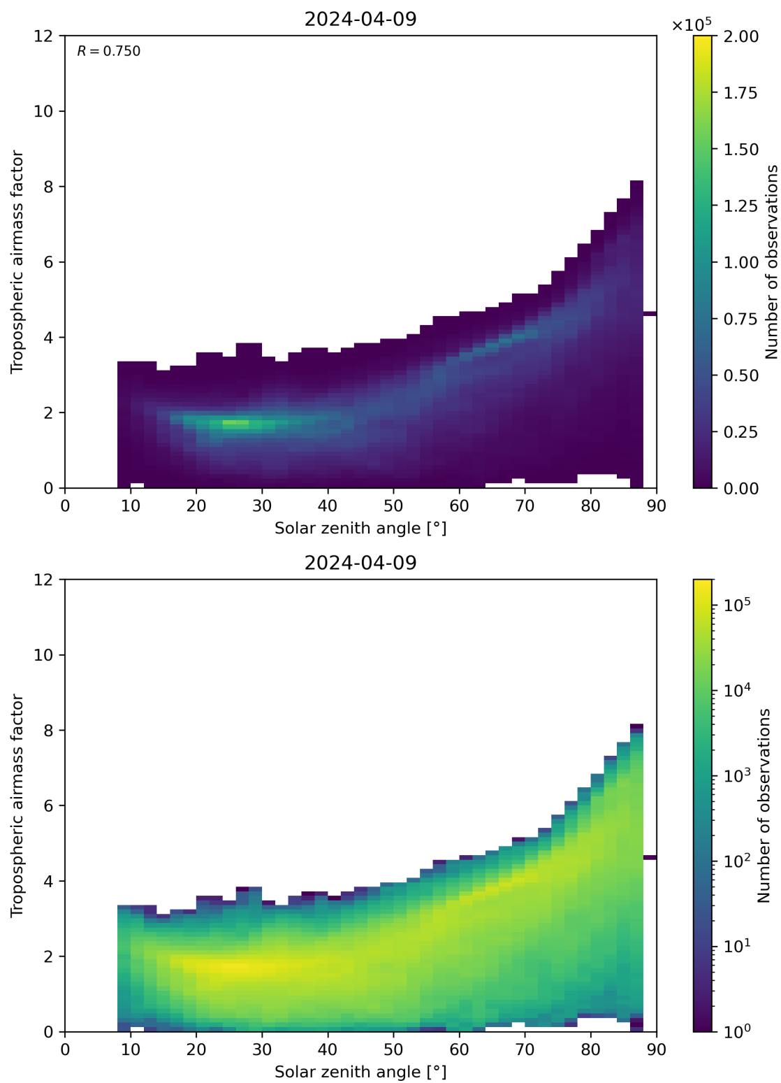
Figure 147: Scatter density plot of “Solar zenith angle” against “Tropospheric airmass factor” for 2024-04-08 to 2024-04-10.
