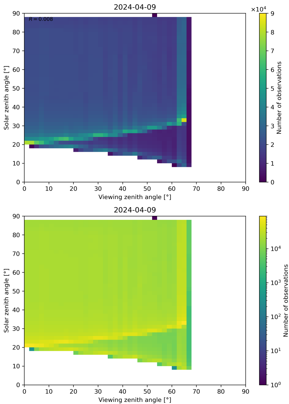
Figure 172: Scatter density plot of “Viewing zenith angle” against “Solar zenith angle” for 2024-04-08 to 2024-04-10.
