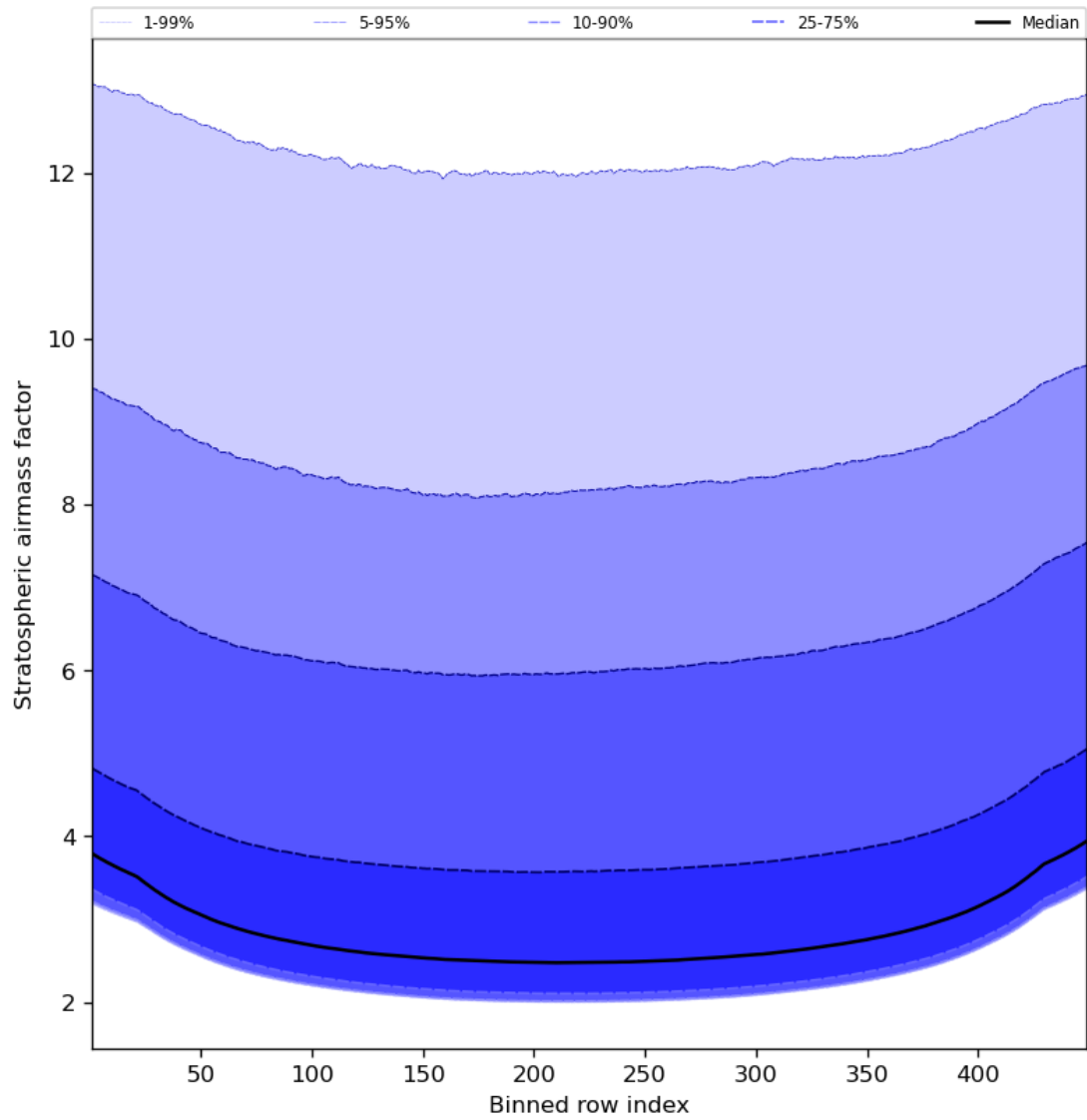
Figure 61: Along track statistics of “Stratospheric airmass factor” for 2024-04-08 to 2024-04-10
