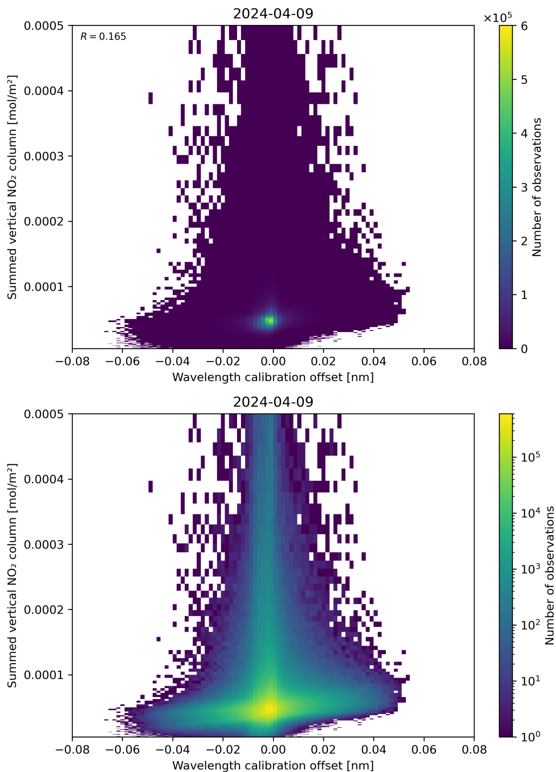
Figure 177: Scatter density plot of “Wavelength calibration offset” against “Summed vertical NO 2 column” for 2024-04-08 to 2024-04-10.
