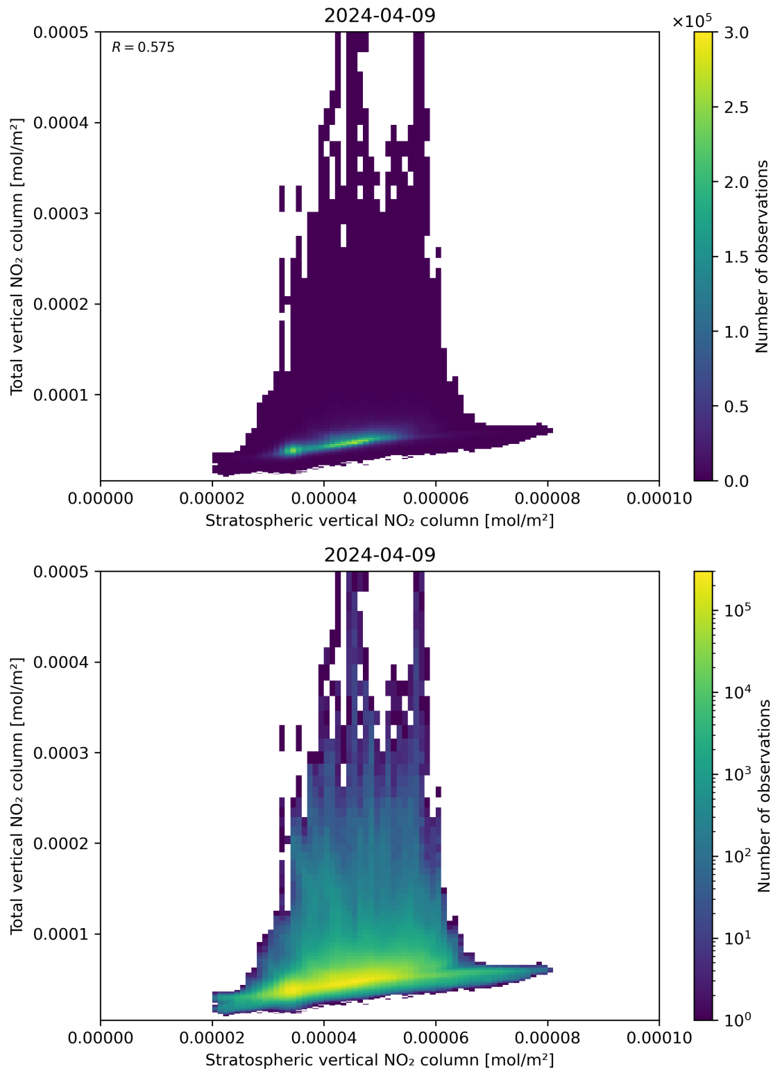
Figure 100: Scatter density plot of “Stratospheric vertical NO 2 column” against “Total vertical NO 2 column” for 2024-04-08 to 2024-04-10.
