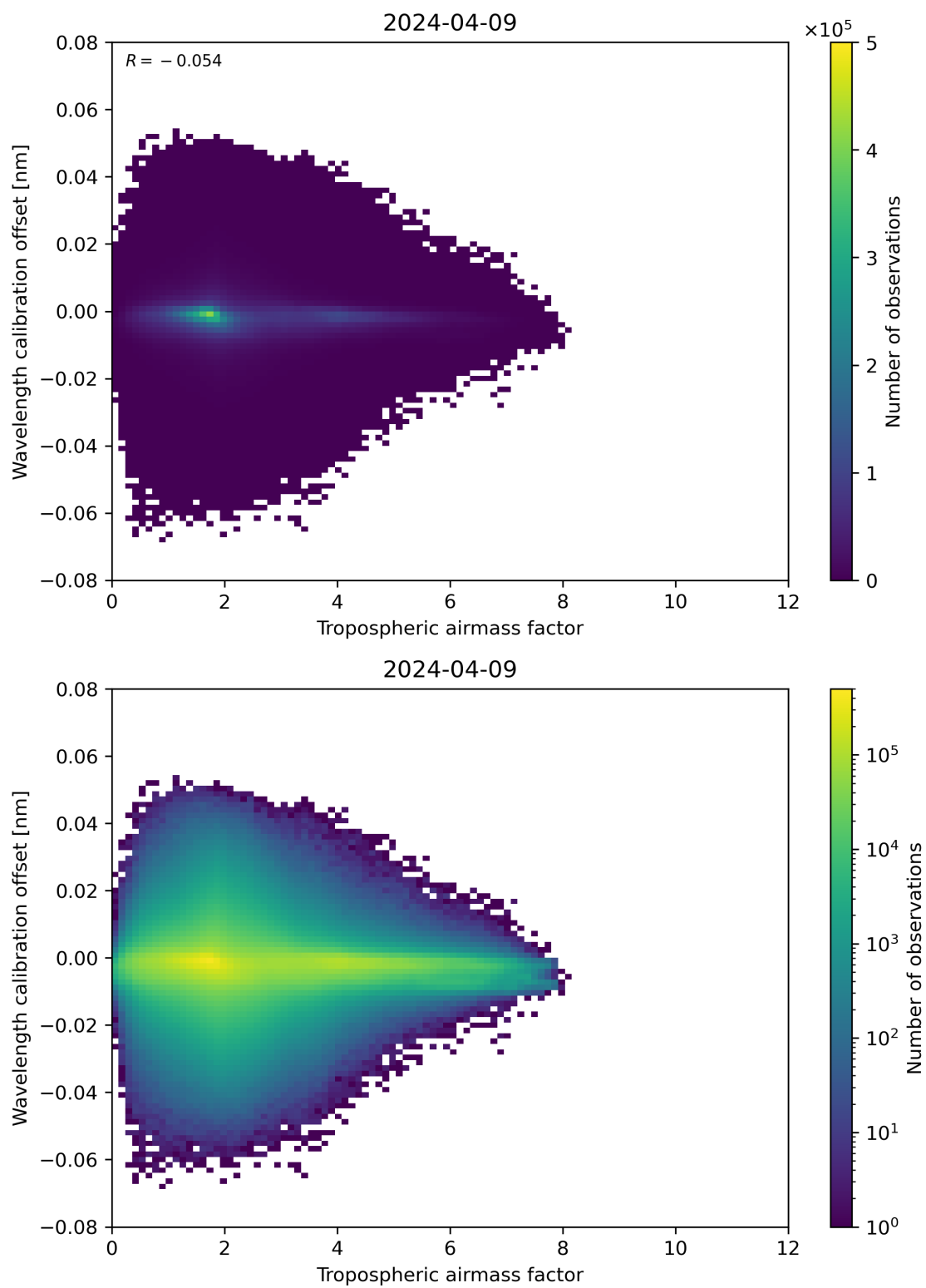
Figure 80: Scatter density plot of “Tropospheric airmass factor” against “Wavelength calibration offset” for 2024-04-08 to 2024-04-10.
