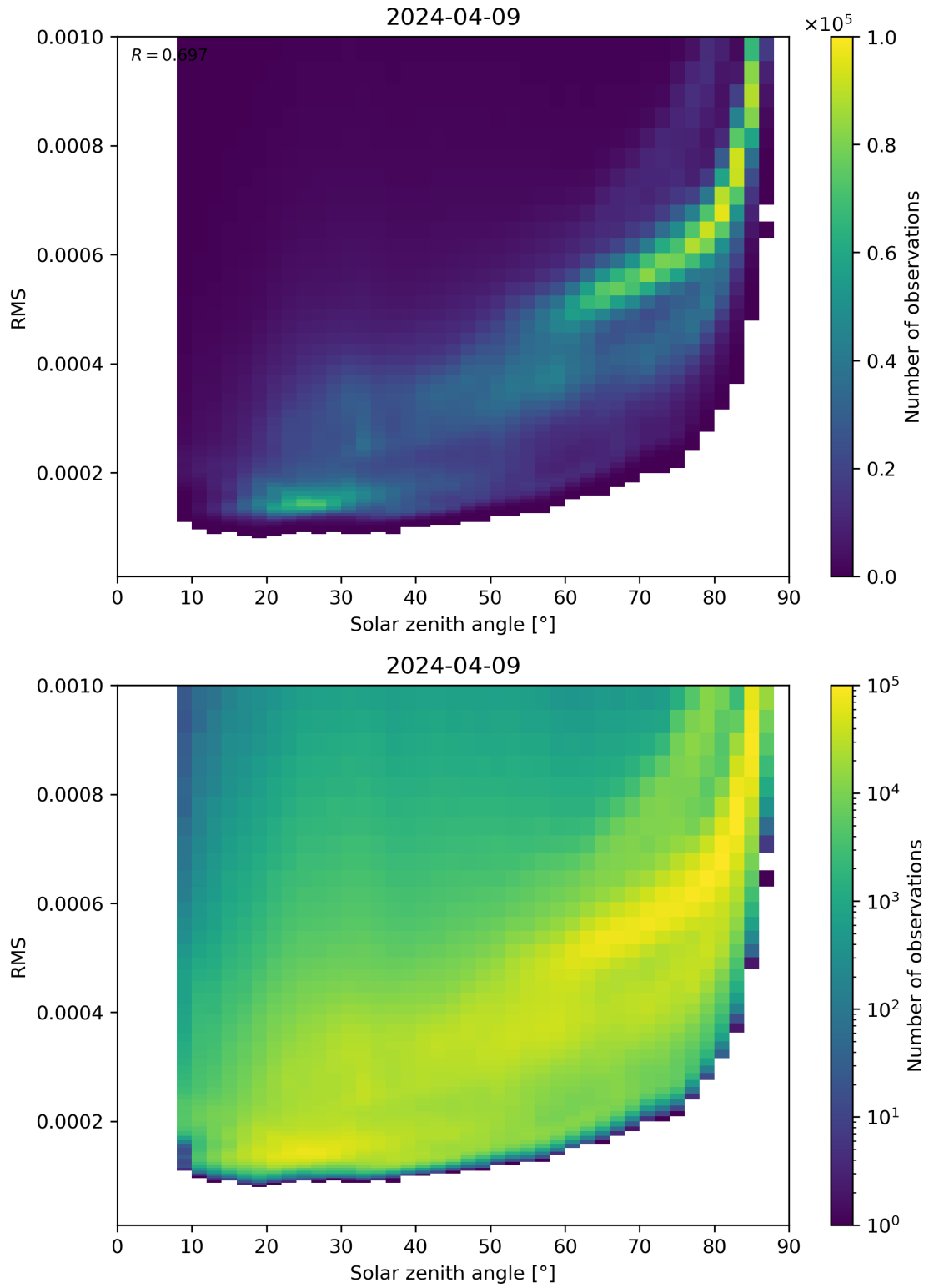
Figure 157: Scatter density plot of “Solar zenith angle” against “RMS” for 2024-04-08 to 2024-04-10.
