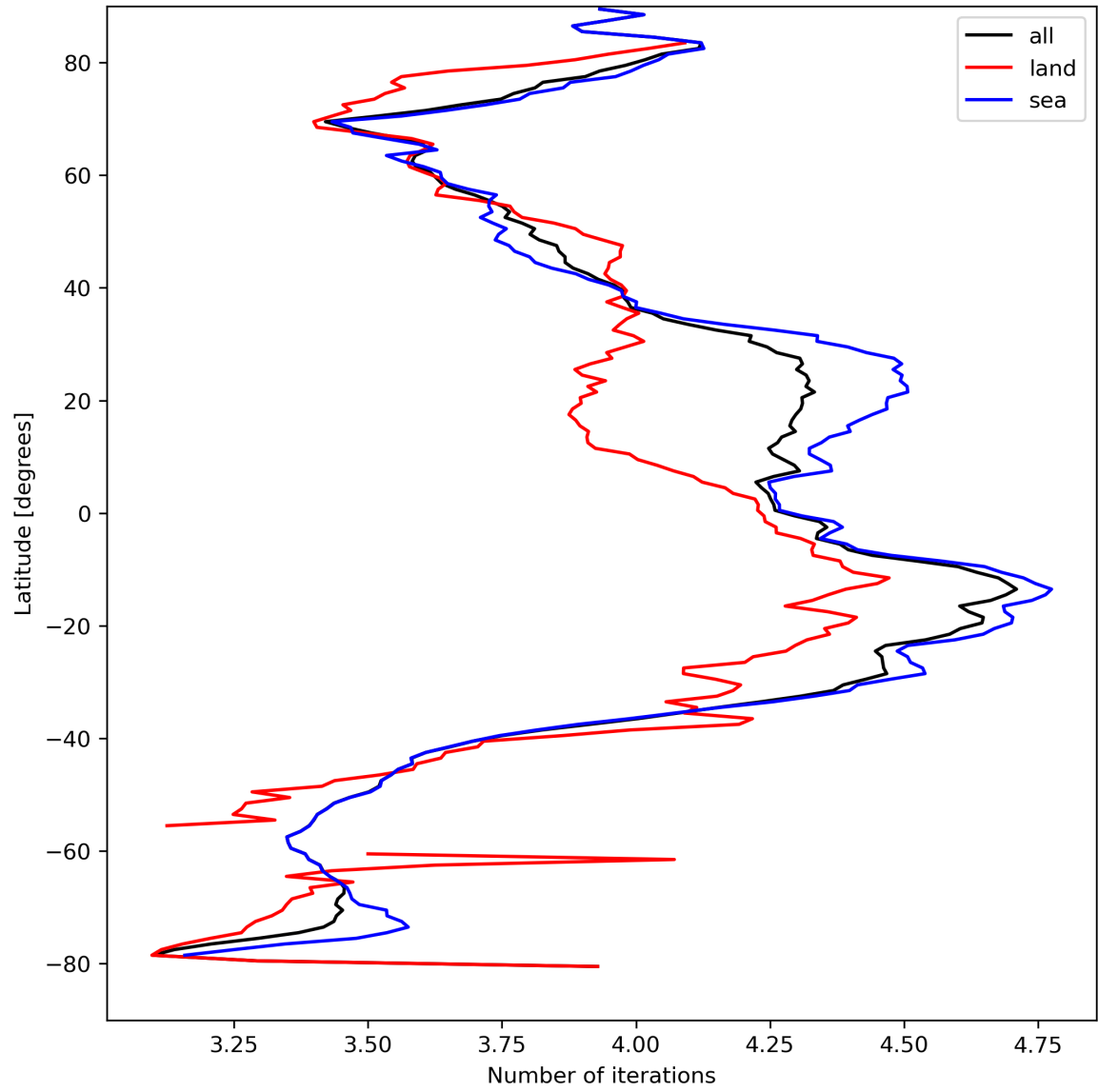
Figure 17: Zonal average of “Number of iterations” for 2024-04-08 to 2024-04-10.
