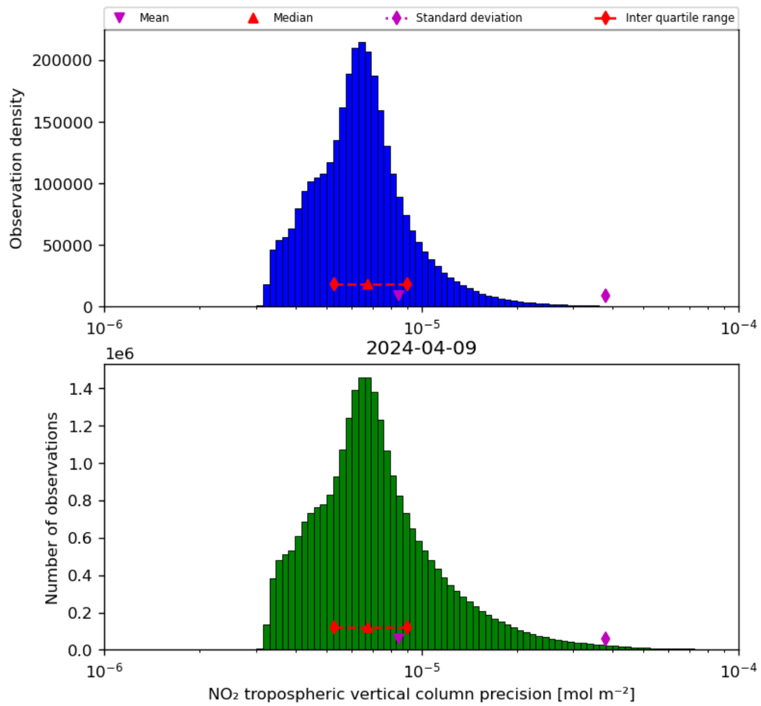
Figure 30: Histogram of “NO 2 tropospheric vertical column precision” for 2024-04-08 to 2024-04-10
