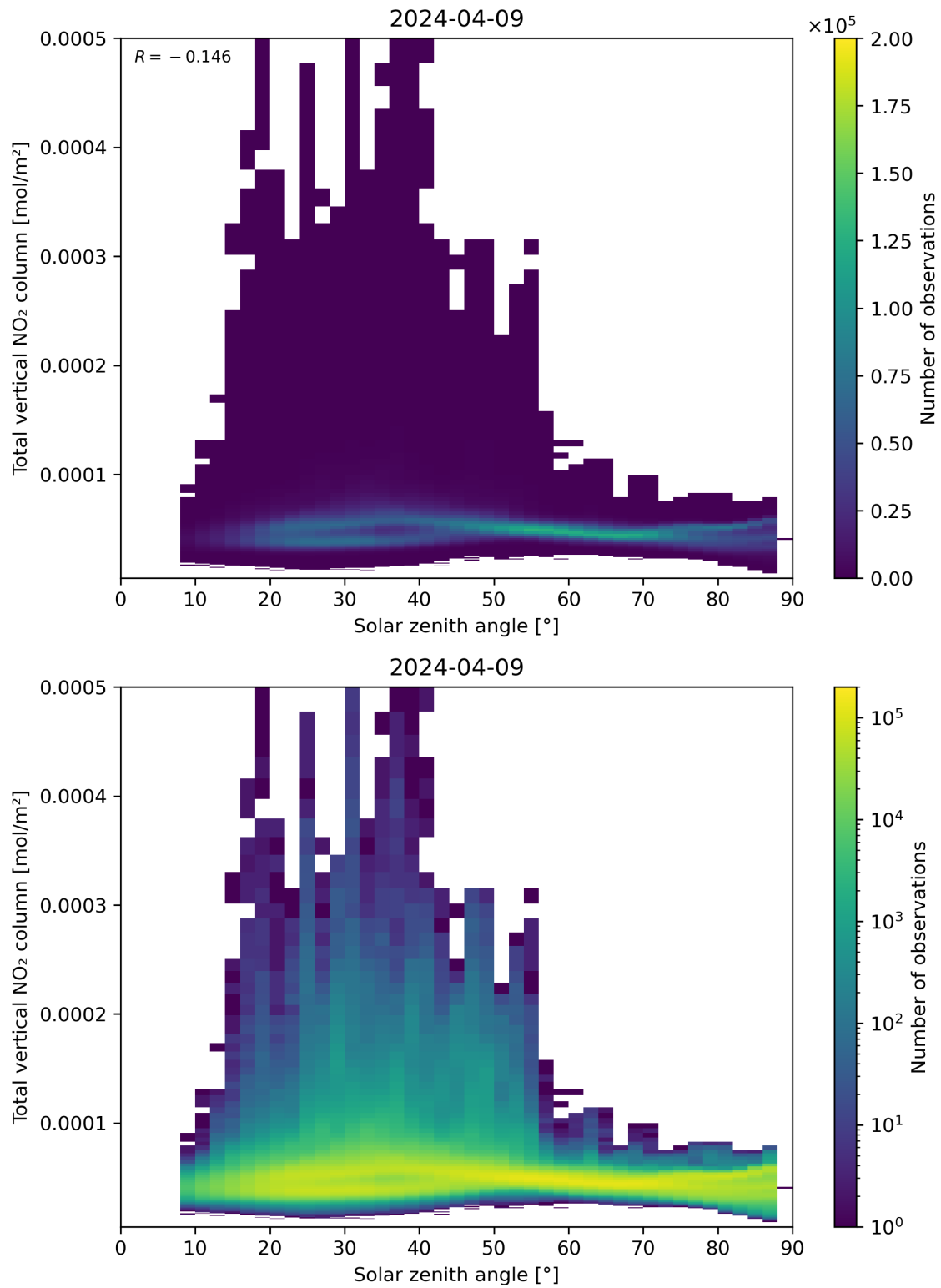
Figure 153: Scatter density plot of “Solar zenith angle” against “Total vertical NO 2 column” for 2024-04-08 to 2024-04-10.
