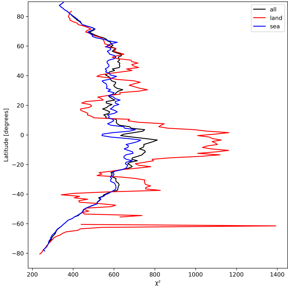
Figure 25: Zonal average of “ \chi^2 ” for 2024-04-08 to 2024-04-10.
