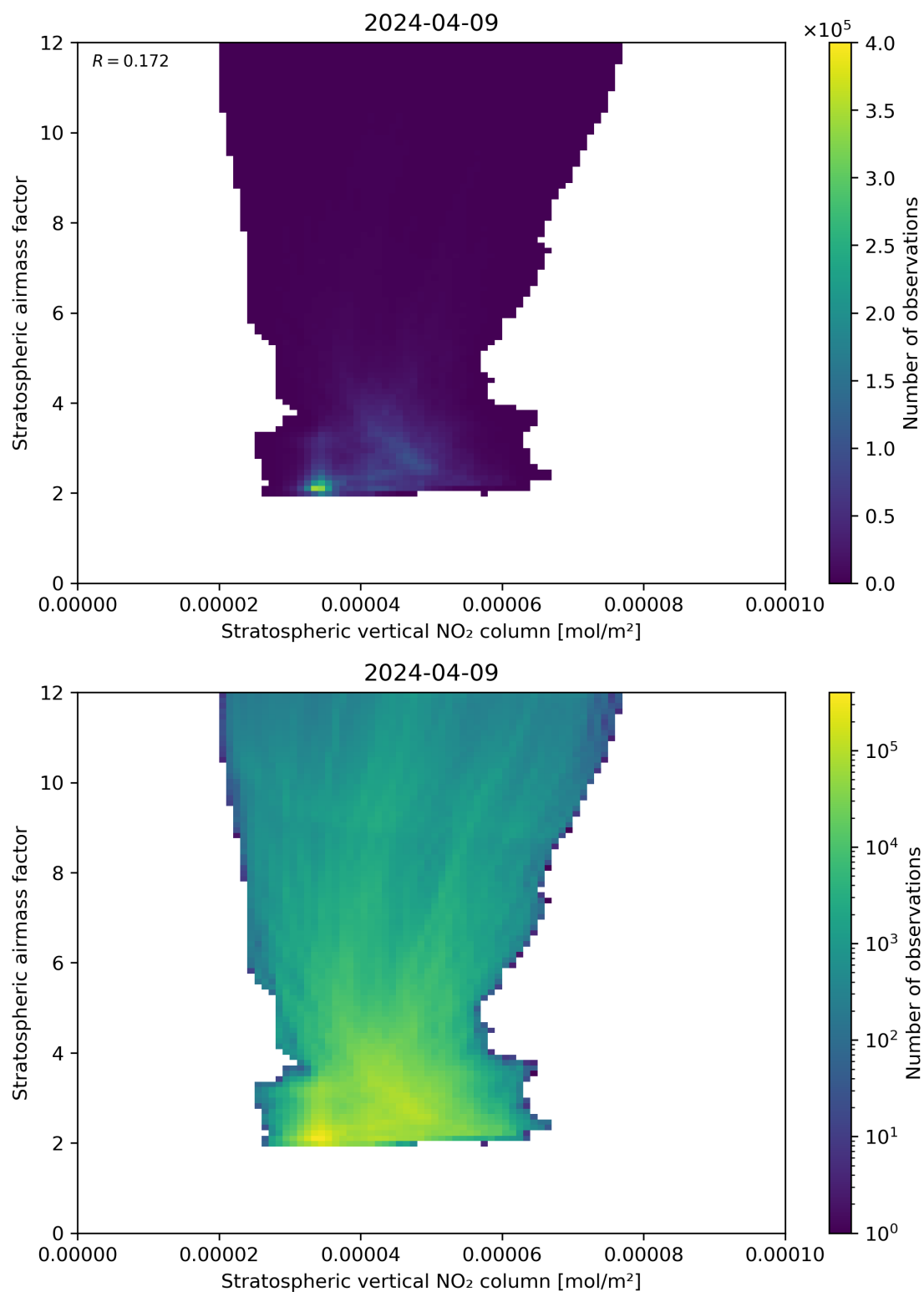
Figure 96: Scatter density plot of “Stratospheric vertical NO 2 column” against “Stratospheric airmass factor” for 2024-04-08 to 2024-04-10.
