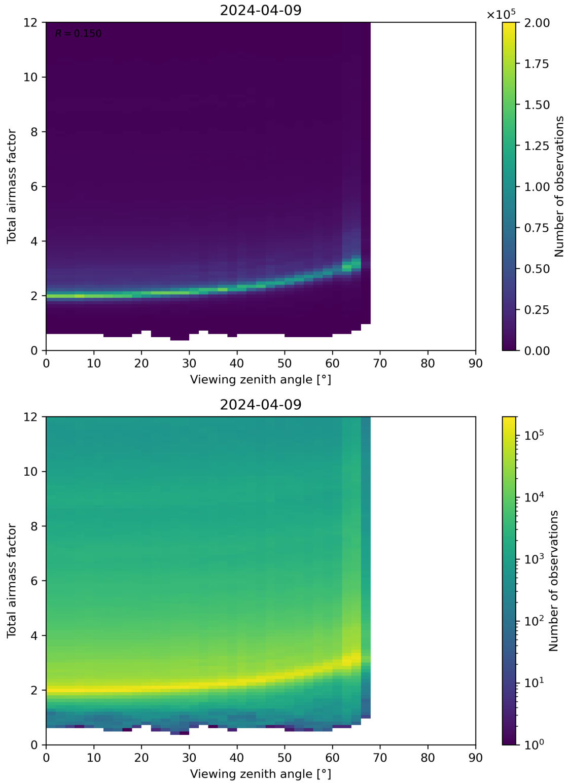
Figure 160: Scatter density plot of “Viewing zenith angle” against “Total airmass factor” for 2024-04-08 to 2024-04-10.
