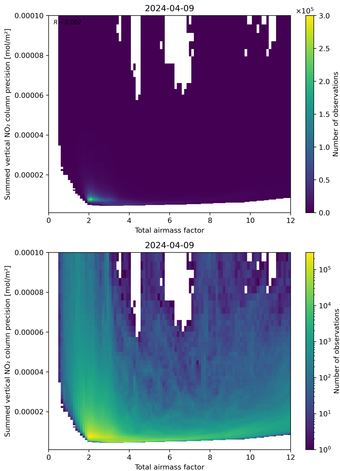
Figure 66: Scatter density plot of “Total airmass factor” against “Summed vertical NO 2 column precision” for 2024-04-08 to 2024-04-10.
