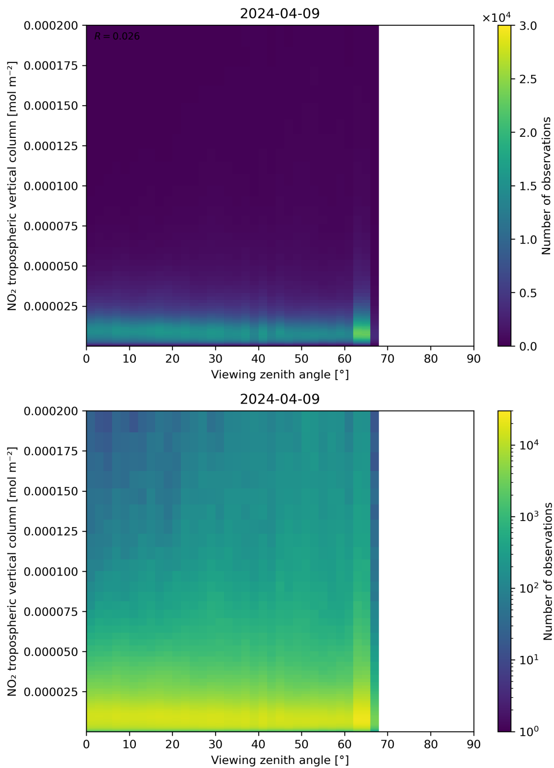
Figure 169: Scatter density plot of “Viewing zenith angle” against “NO 2 tropospheric vertical column” for 2024-04-08 to 2024-04-10.
