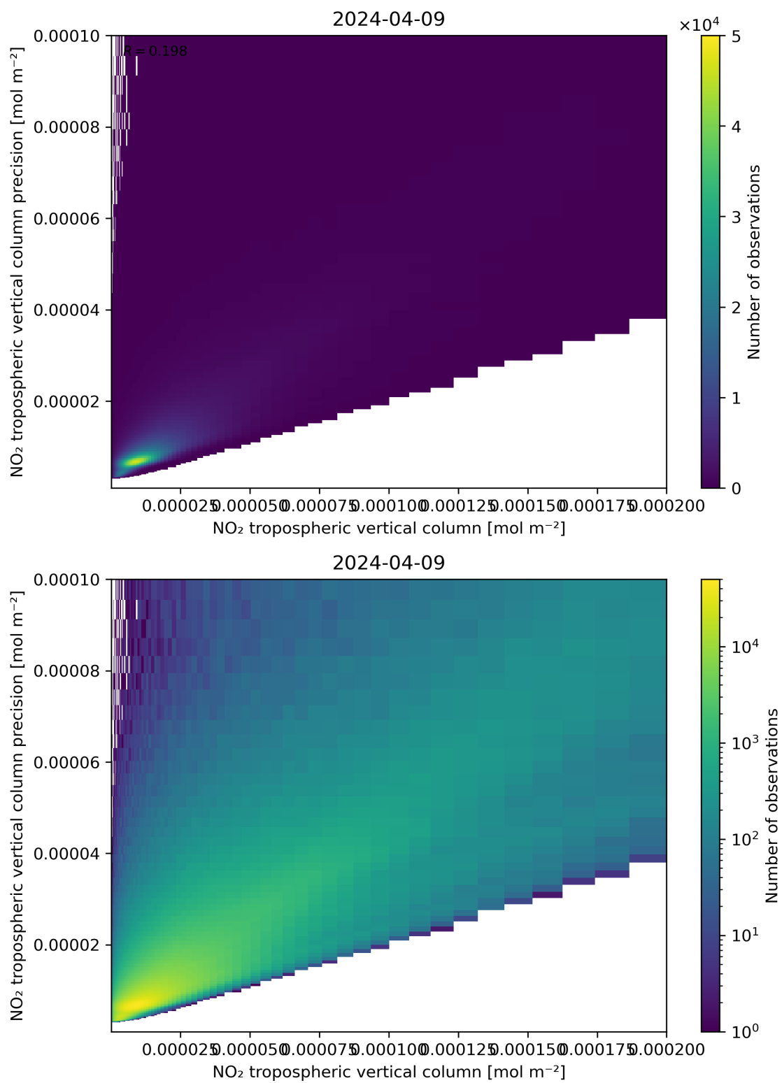
Figure 130: Scatter density plot of “NO 2 tropospheric vertical column” against “NO 2 tropospheric vertical column precision” for 2024-04-08 to 2024-04-10.
