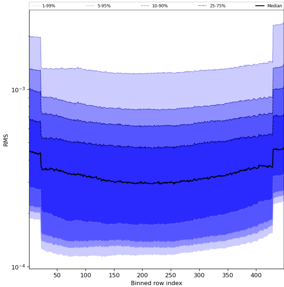
Figure 60: Along track statistics of “RMS” for 2024-04-08 to 2024-04-10
