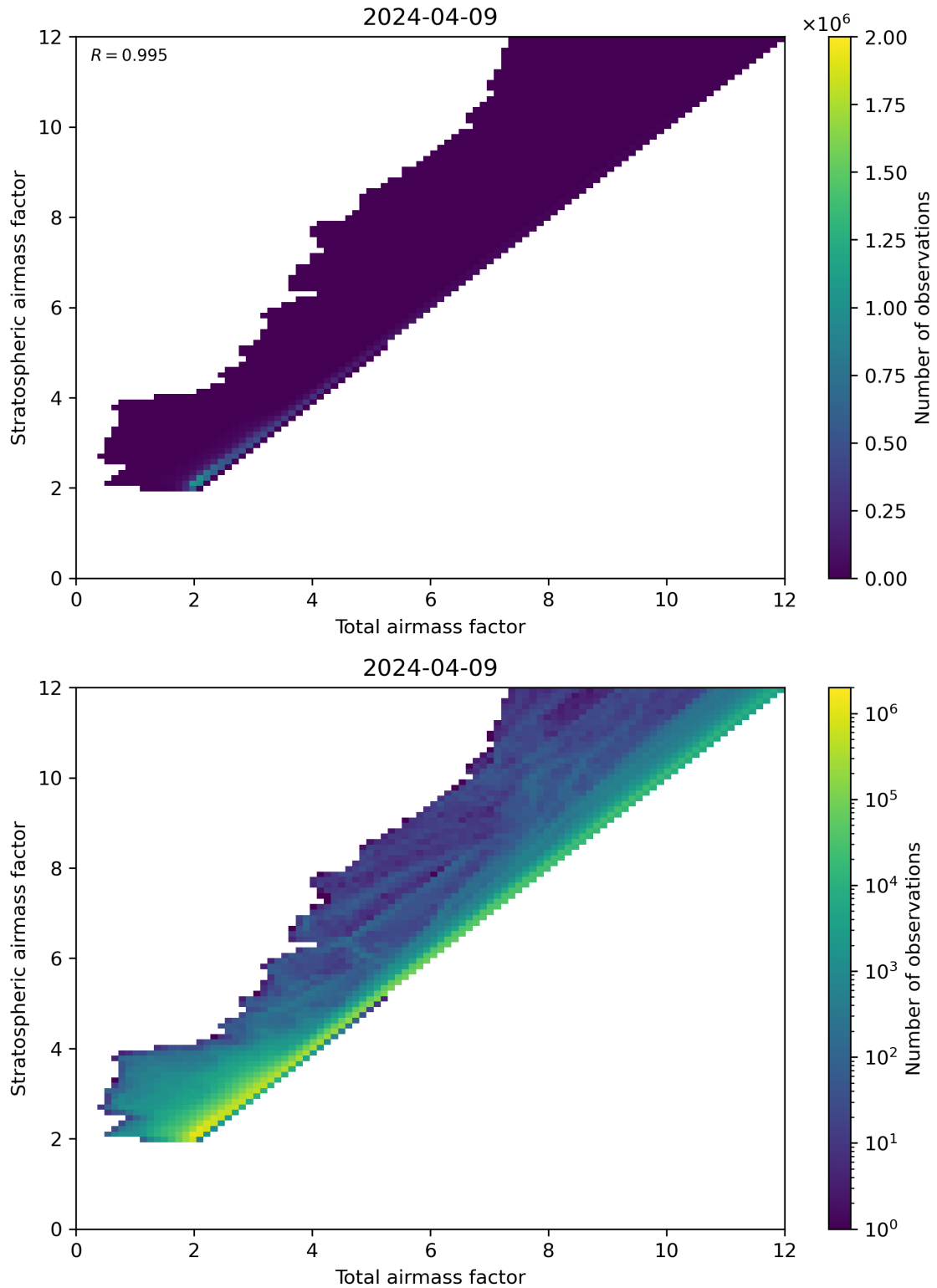
Figure 62: Scatter density plot of “Total airmass factor” against “Stratospheric airmass factor” for 2024-04-08 to 2024-04-10.
