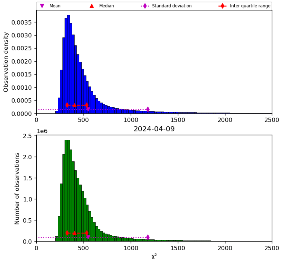
Figure 42: Histogram of “ \chi^2 ” for 2024-04-08 to 2024-04-10
