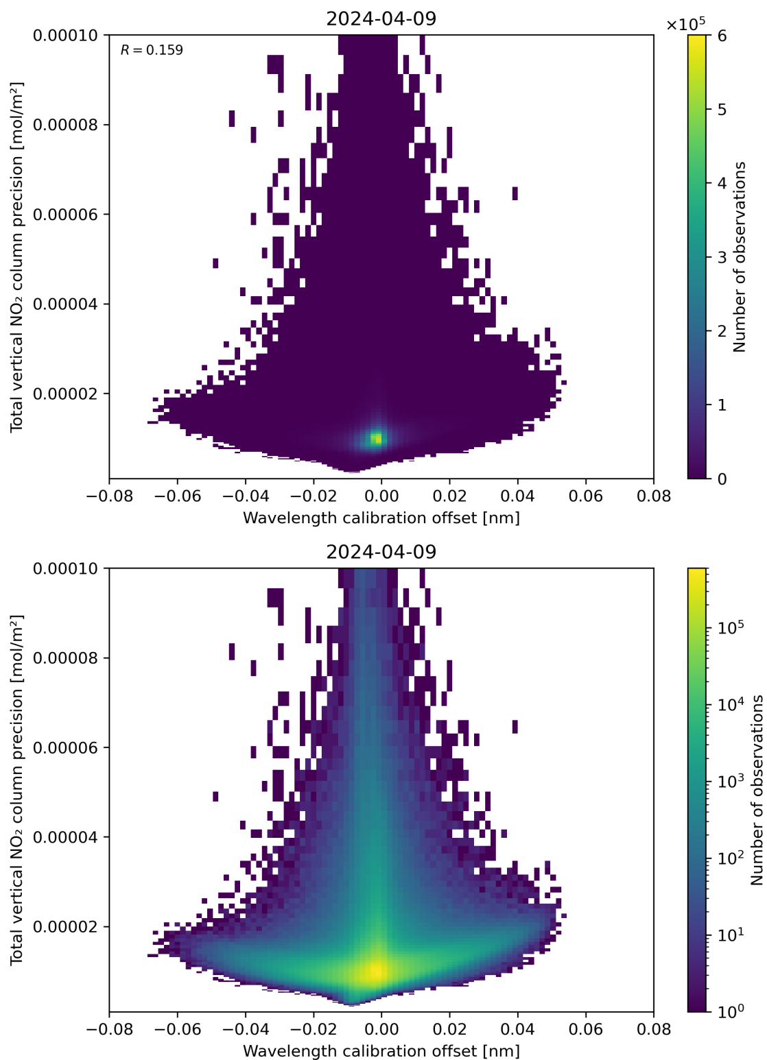
Figure 180: Scatter density plot of “Wavelength calibration offset” against “Total vertical NO 2 column precision” for 2024-04-08 to 2024-04-10.
