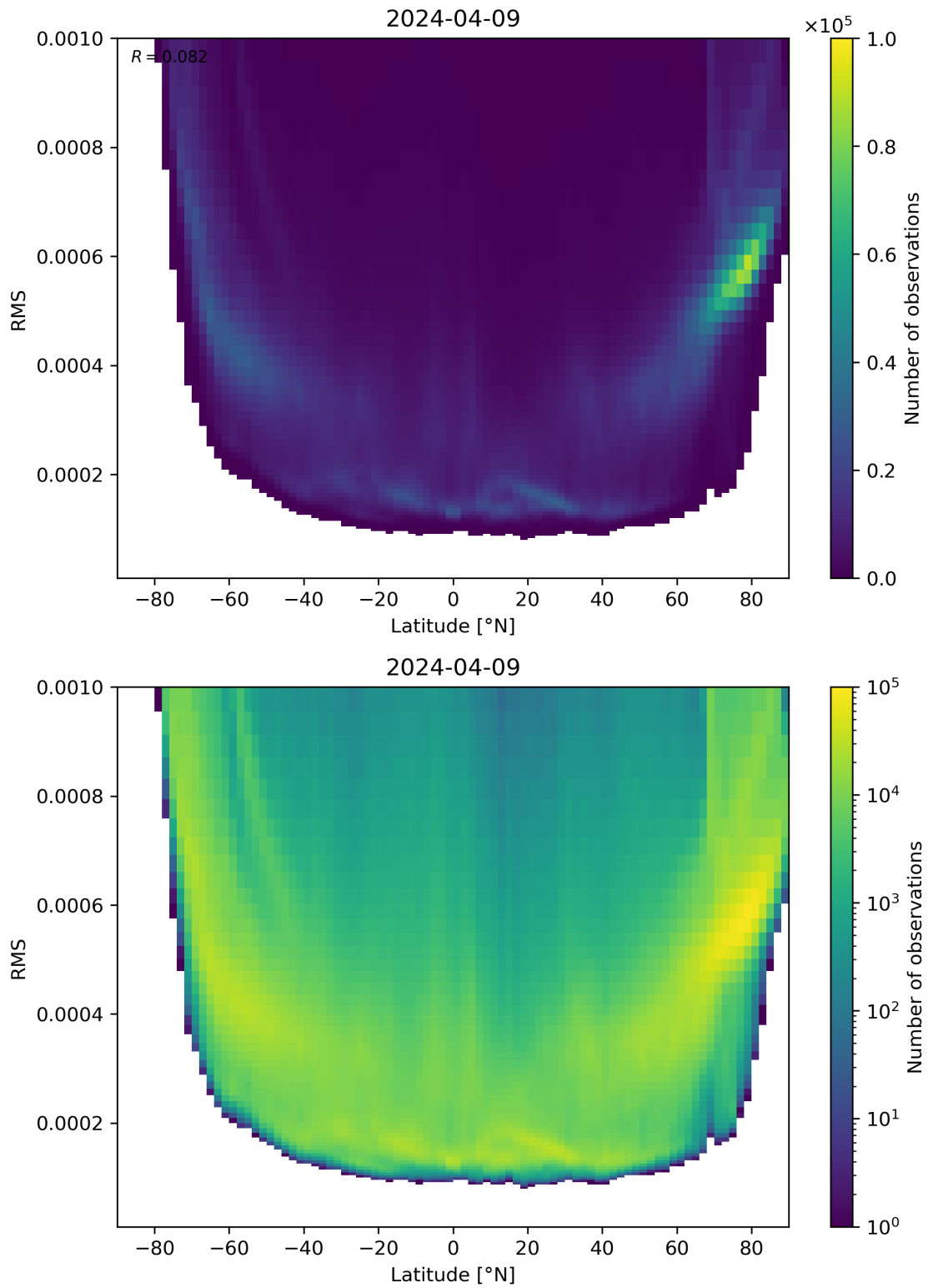
Figure 94: Scatter density plot of “Latitude” against “RMS” for 2024-04-08 to 2024-04-10.
