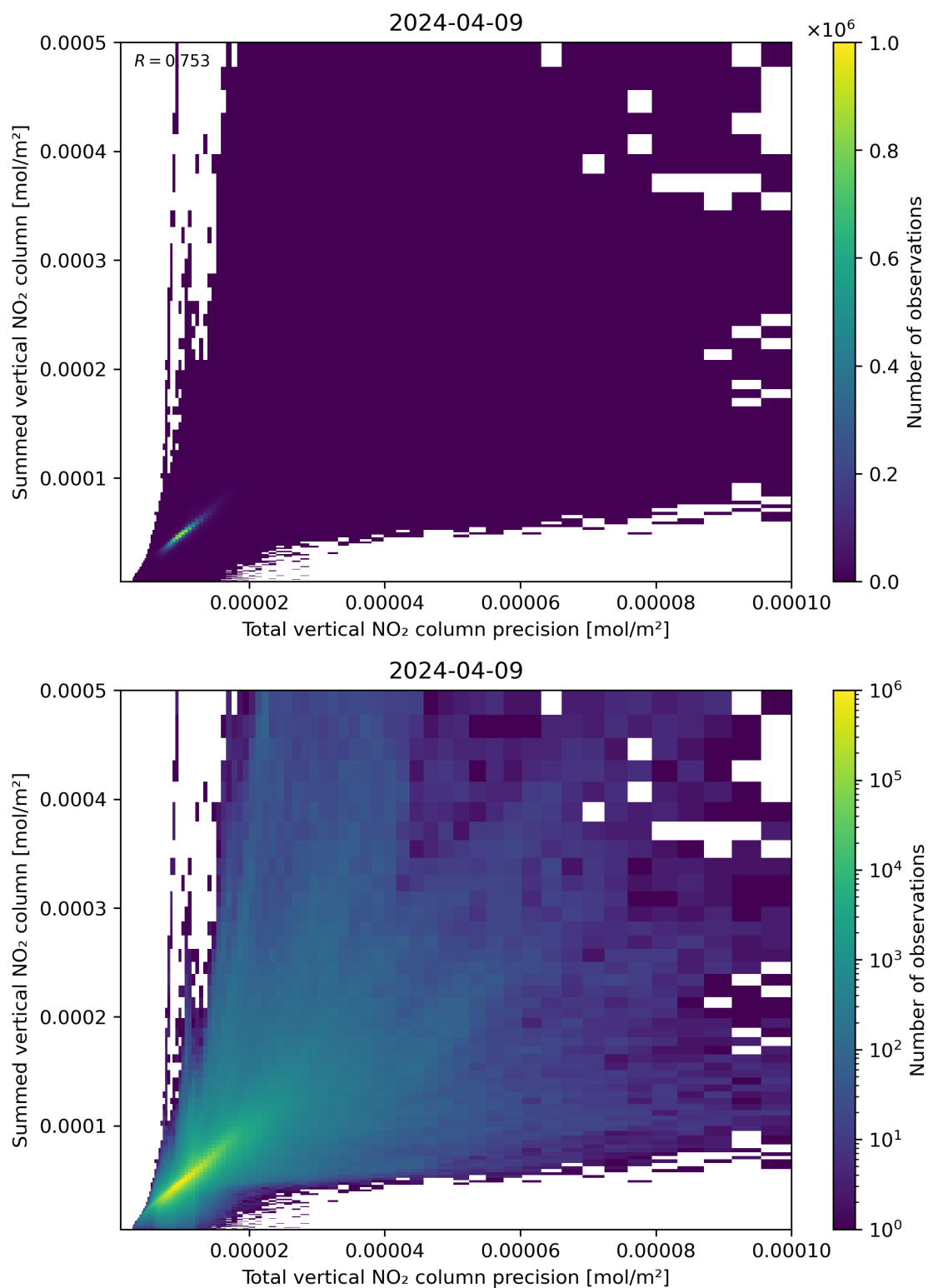
Figure 117: Scatter density plot of “Total vertical NO 2 column precision” against “Summed vertical NO 2 column” for 2024-04-08 to 2024-04-10.
