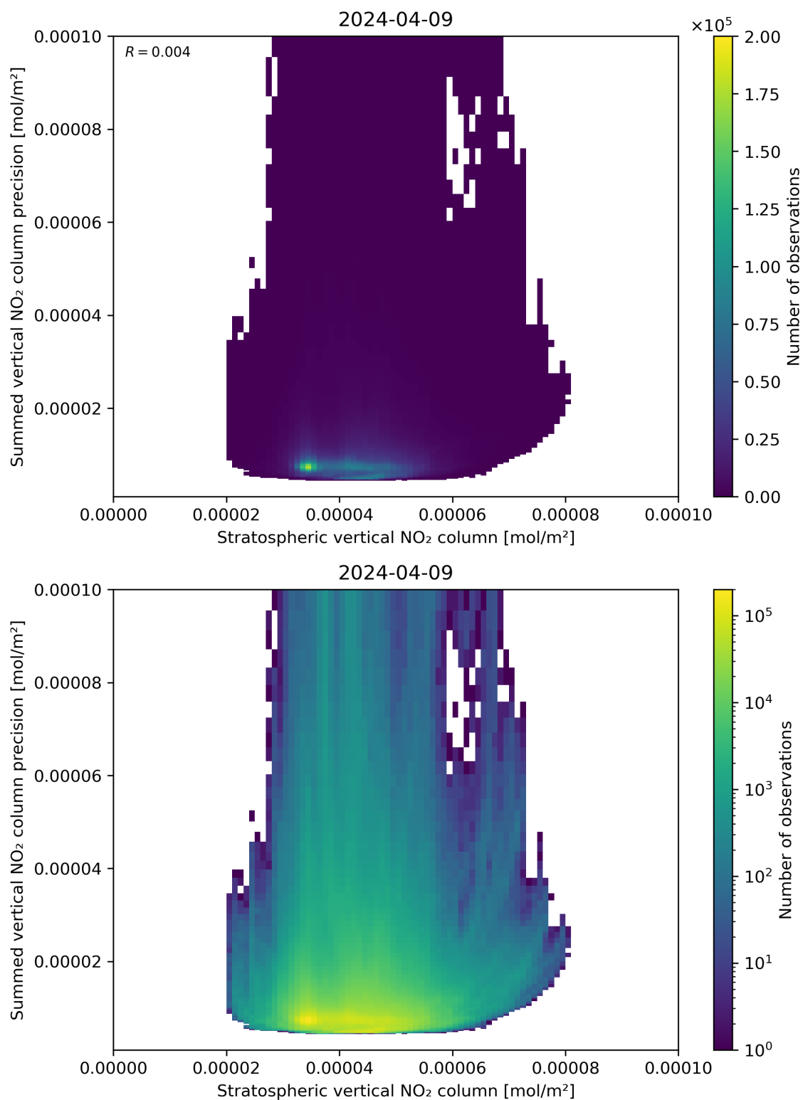
Figure 99: Scatter density plot of “Stratospheric vertical NO 2 column” against “Summed vertical NO 2 column precision” for 2024-04-08 to 2024-04-10.
