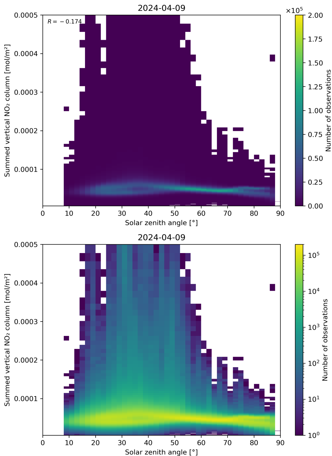
Figure 151: Scatter density plot of “Solar zenith angle” against “Summed vertical NO 2 column” for 2024-04-08 to 2024-04-10.
