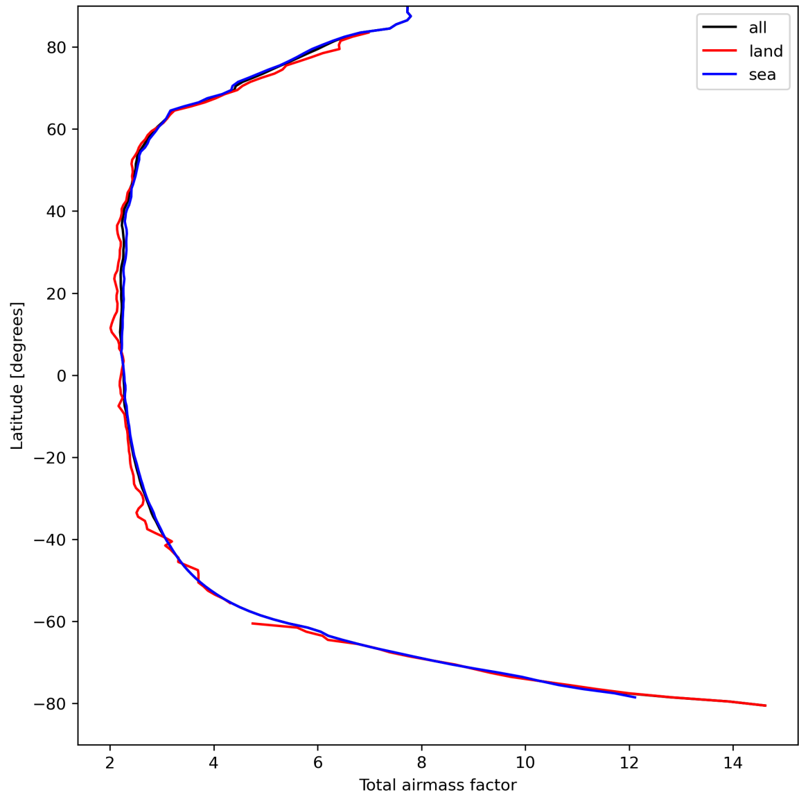
Figure 15: Zonal average of “Total airmass factor” for 2024-04-08 to 2024-04-10.
