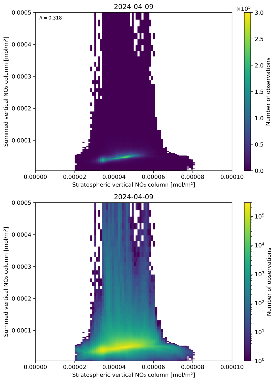
Figure 98: Scatter density plot of “Stratospheric vertical NO 2 column” against “Summed vertical NO 2 column” for 2024-04-08 to 2024-04-10.
