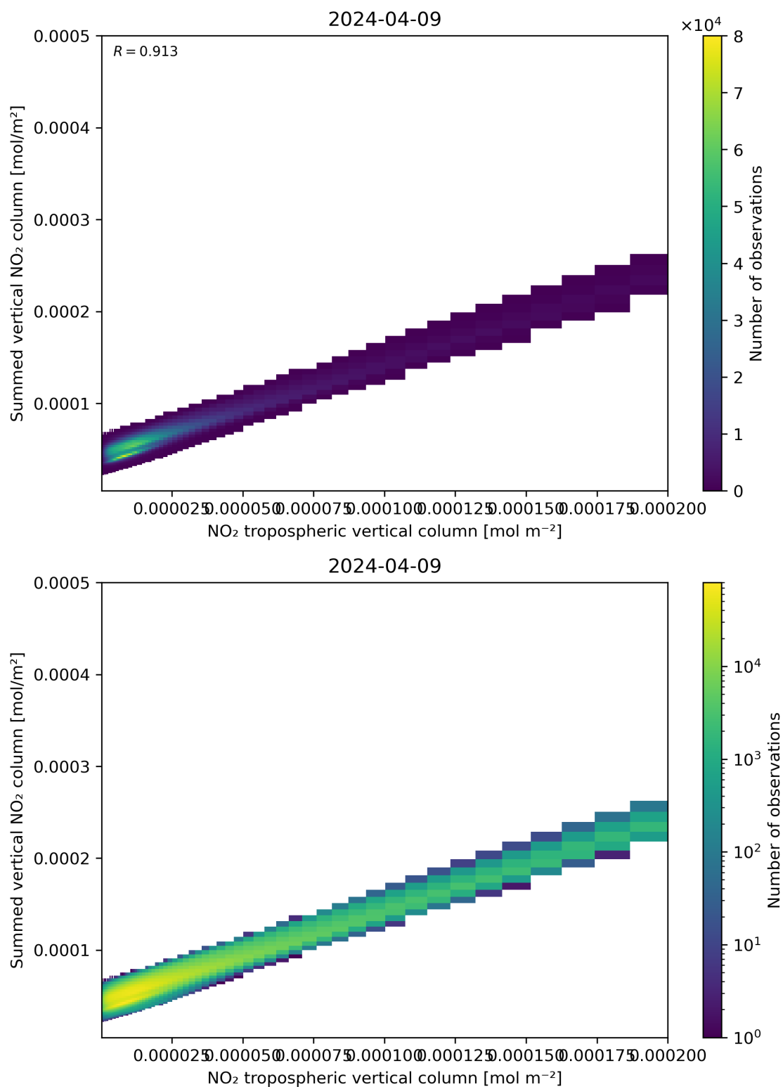
Figure 126: Scatter density plot of “NO 2 tropospheric vertical column” against “Summed vertical NO 2 column” for 2024-04-08 to 2024-04-10.
