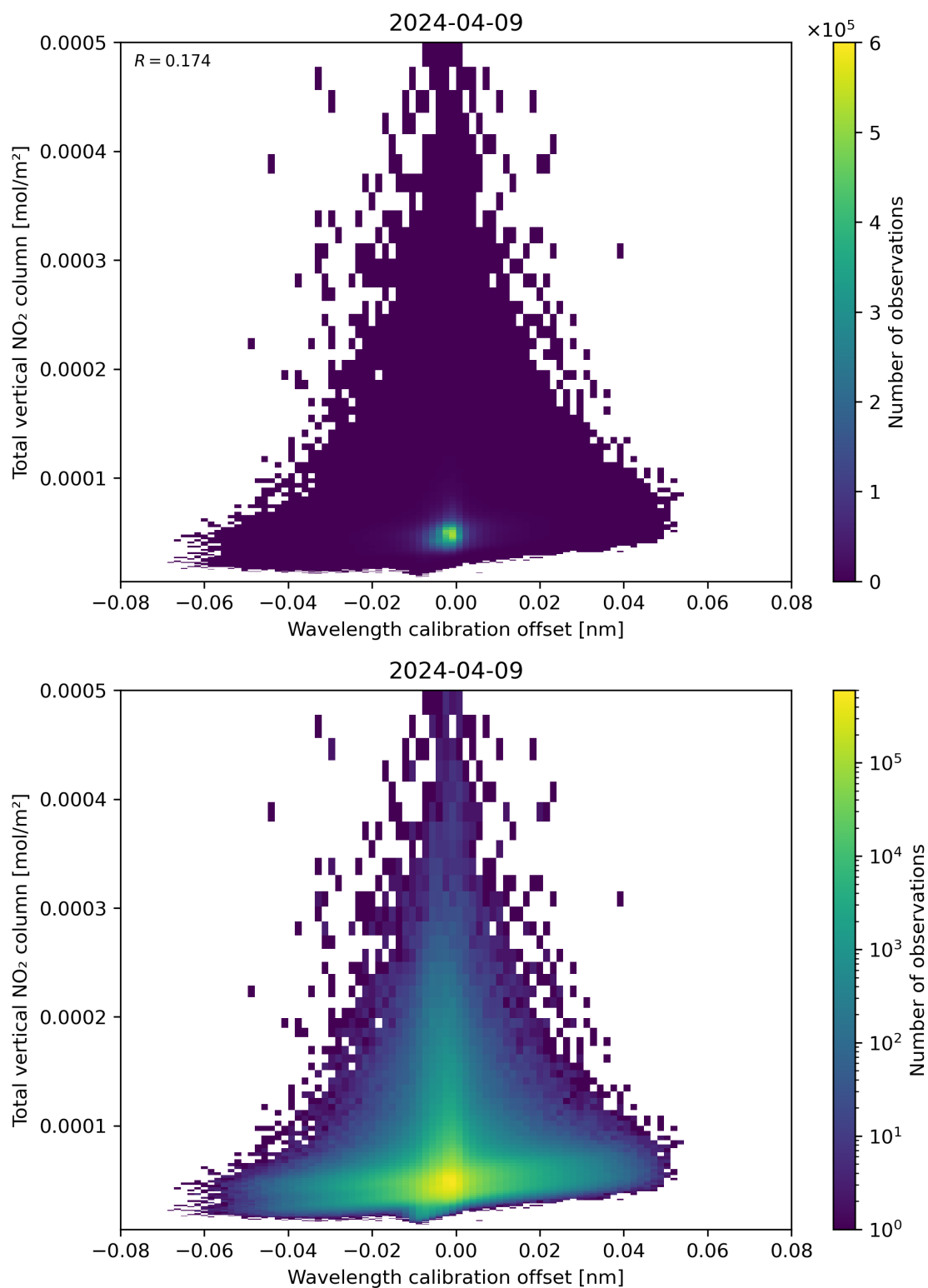
Figure 179: Scatter density plot of “Wavelength calibration offset” against “Total vertical NO 2 column” for 2024-04-08 to 2024-04-10.
