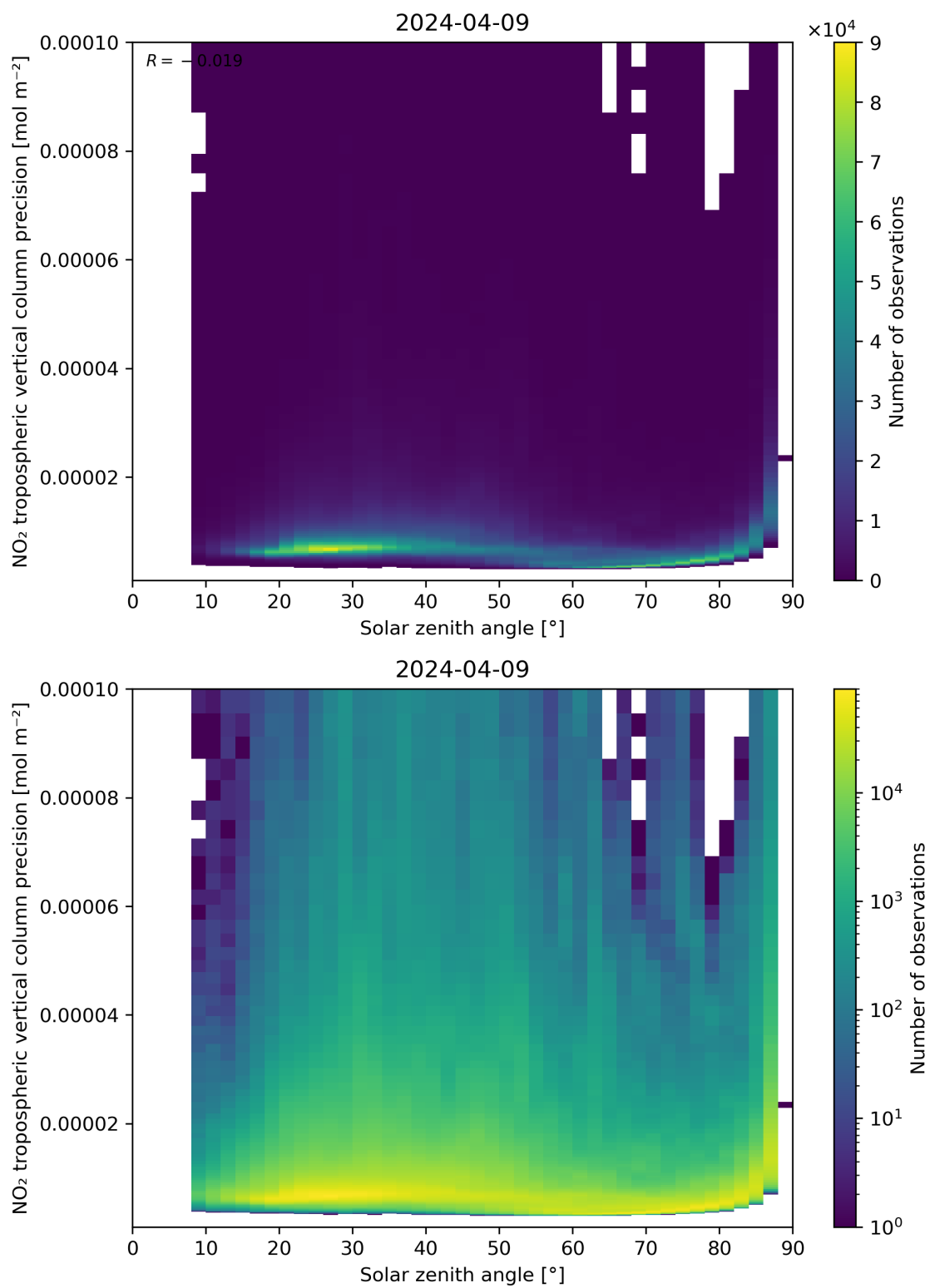
Figure 156: Scatter density plot of “Solar zenith angle” against “NO 2 tropospheric vertical column precision” for 2024-04-08 to 2024-04-10.
