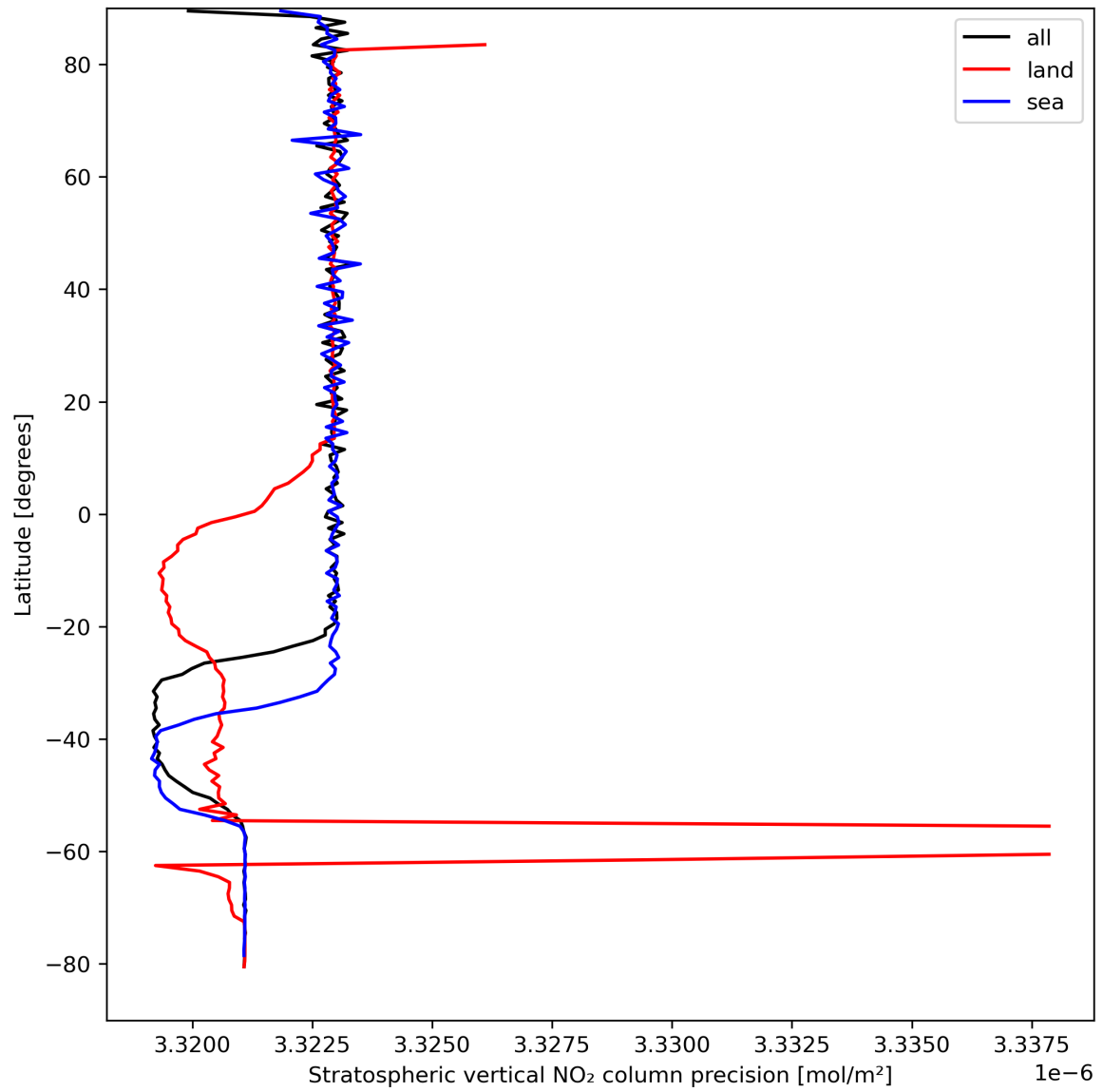
Figure 20: Zonal average of “Stratospheric vertical NO 2 column precision” for 2024-04-08 to 2024-04-10.
