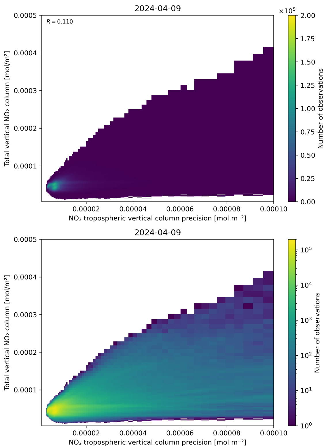
Figure 138: Scatter density plot of “NO 2 tropospheric vertical column precision” against “Total vertical NO 2 column” for 2024-04-08 to 2024-04-10.
