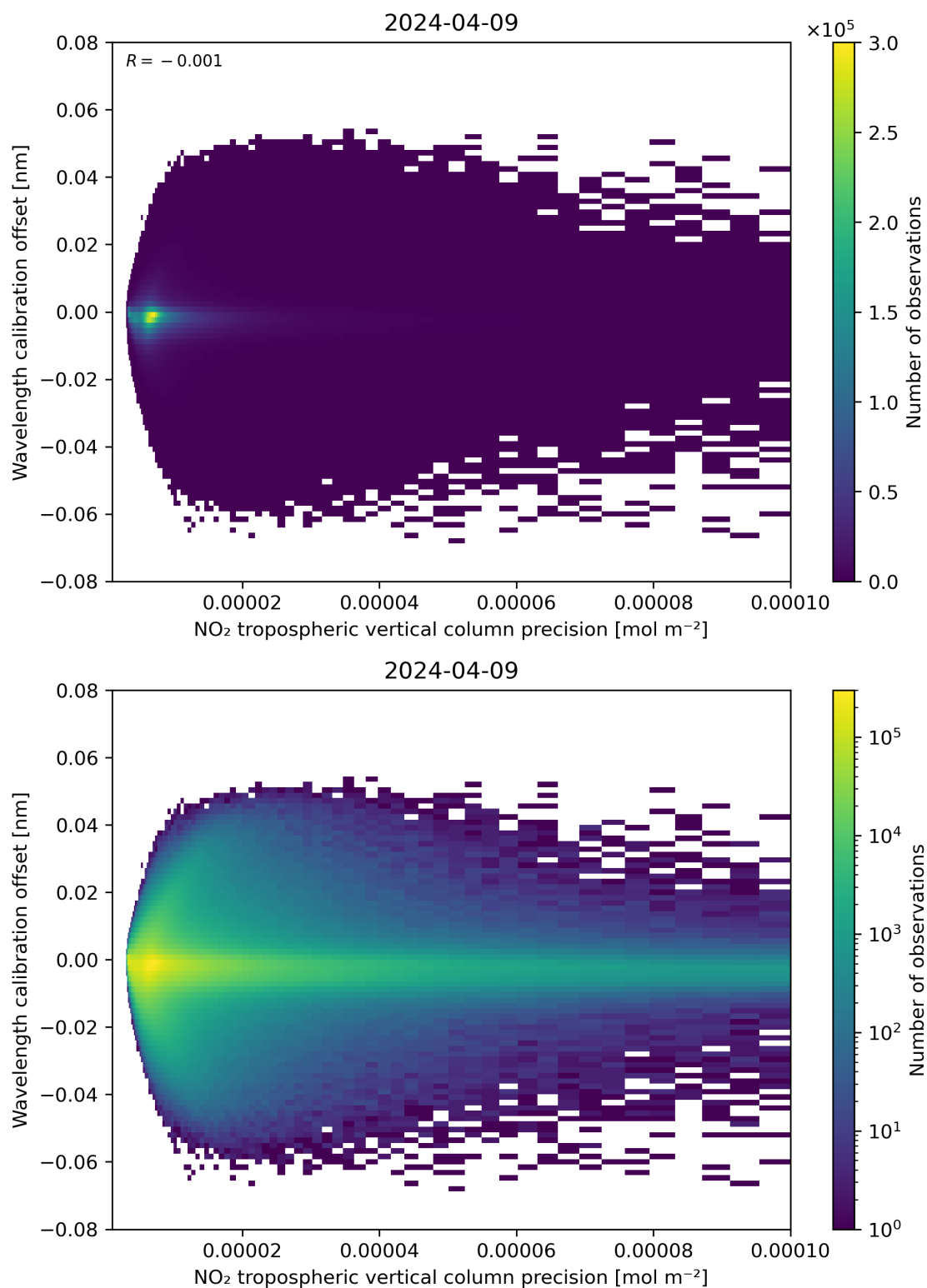
Figure 141: Scatter density plot of “NO 2 tropospheric vertical column precision” against “Wavelength calibration offset” for 2024-04-08 to 2024-04-10.
