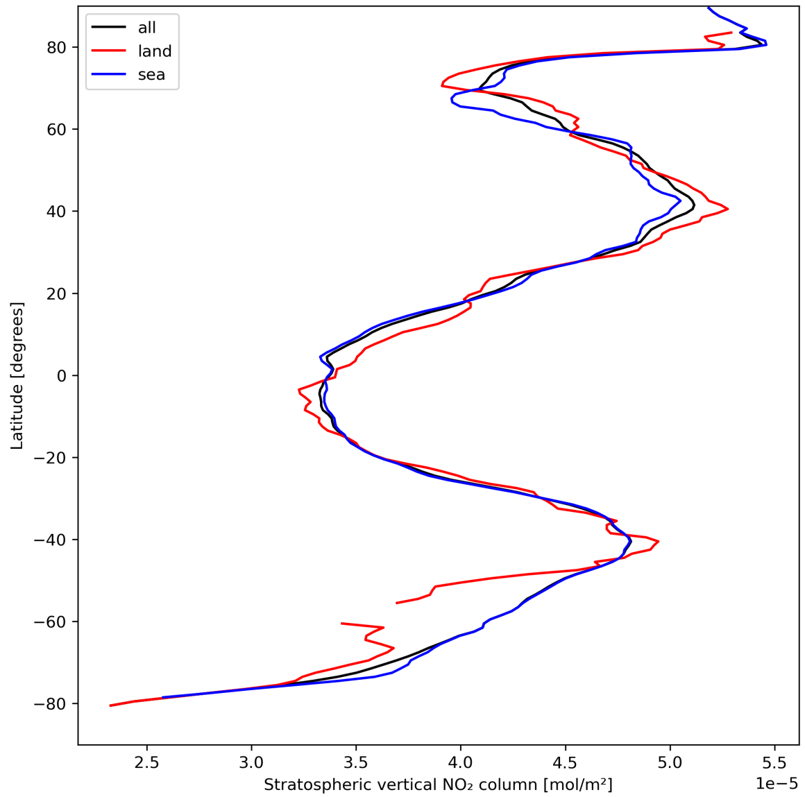
Figure 19: Zonal average of “Stratospheric vertical NO 2 column” for 2024-04-08 to 2024-04-10.
