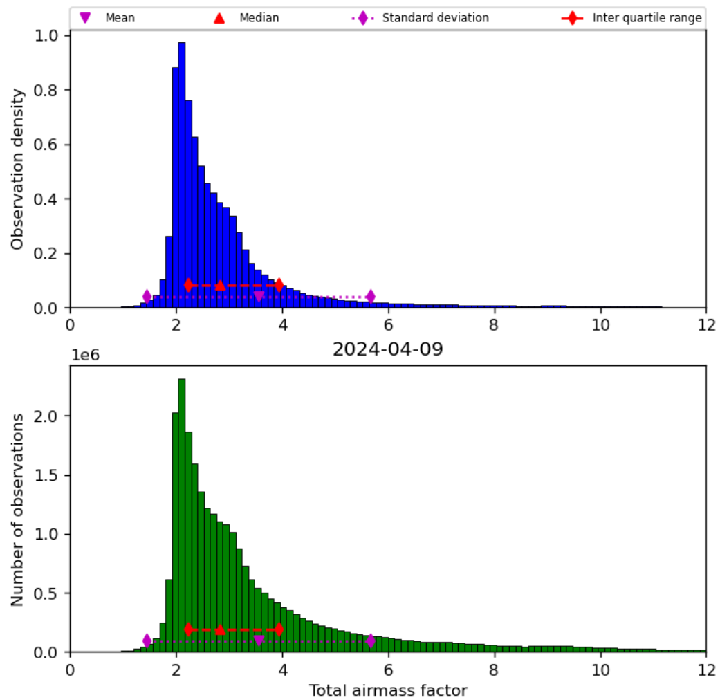
Figure 32: Histogram of “Total airmass factor” for 2024-04-08 to 2024-04-10
