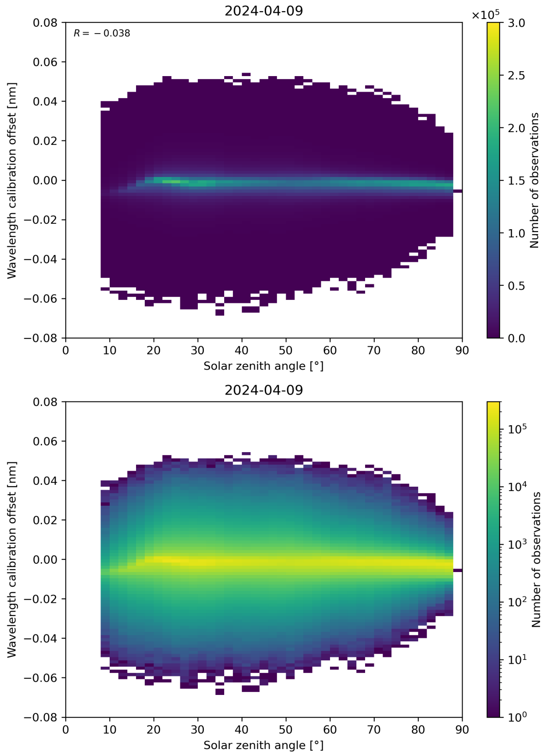
Figure 158: Scatter density plot of “Solar zenith angle” against “Wavelength calibration offset” for 2024-04-08 to 2024-04-10.
