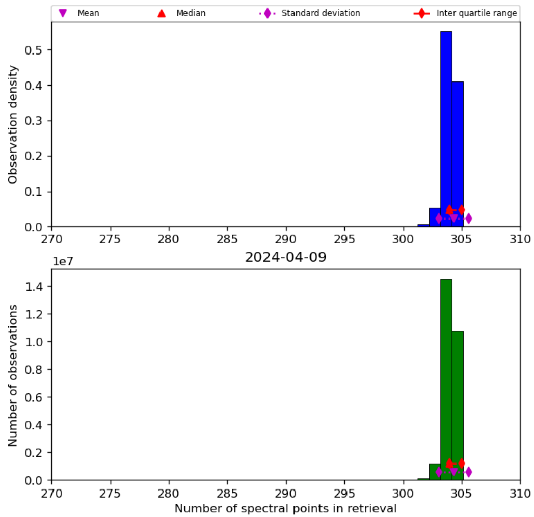
Figure 33: Histogram of “Number of spectral points in retrieval” for 2024-04-08 to 2024-04-10
