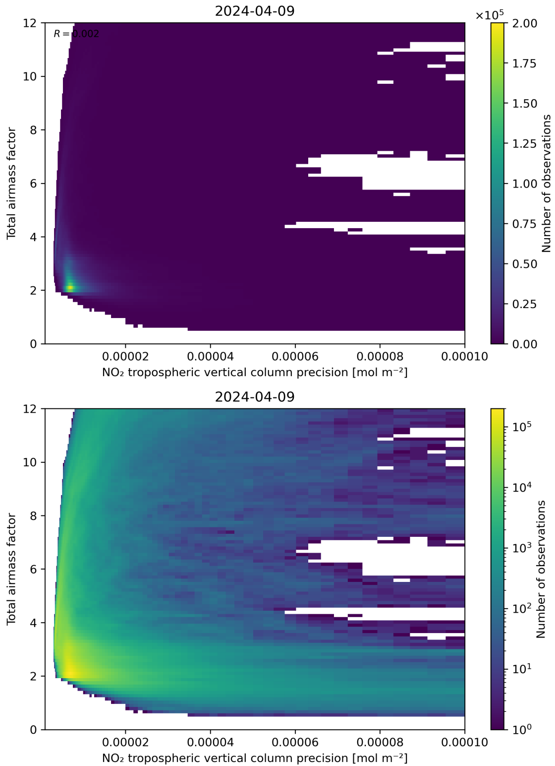
Figure 132: Scatter density plot of “NO 2 tropospheric vertical column precision” against “Total air mass factor” for 2024-04-08 to 2024-04-10.
