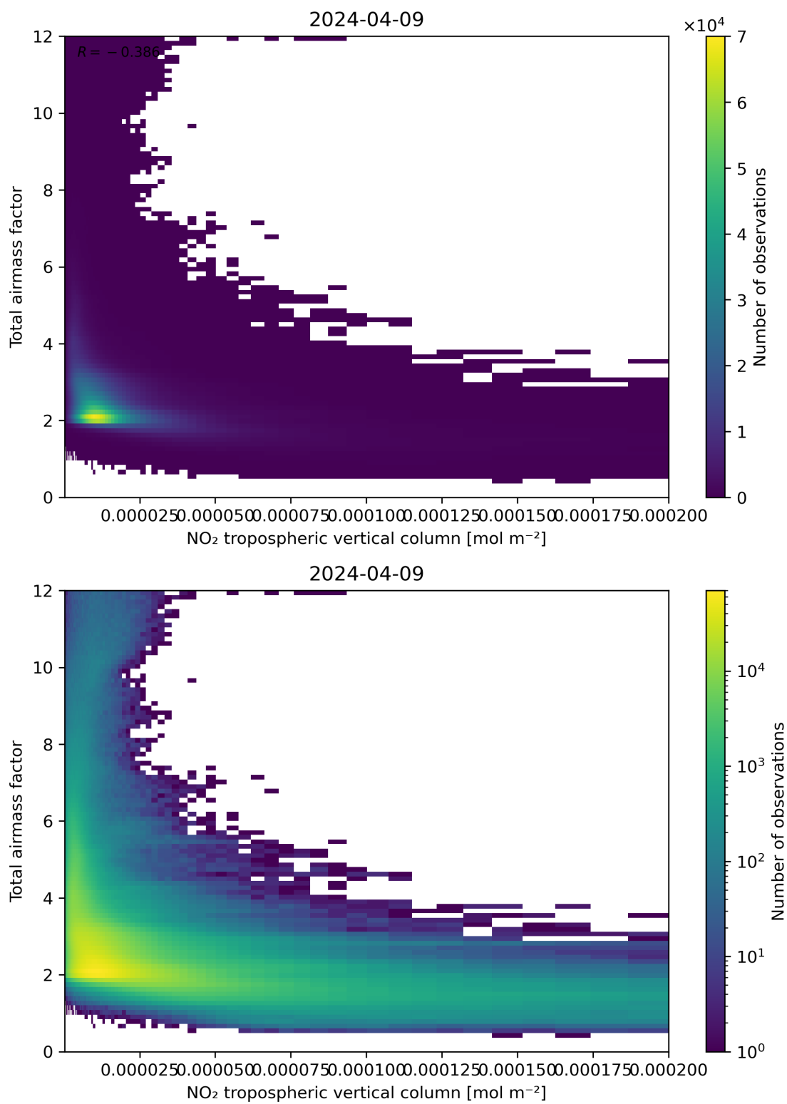
Figure 122: Scatter density plot of “NO 2 tropospheric vertical column” against “Total air mass factor” for 2024-04-08 to 2024-04-10.
