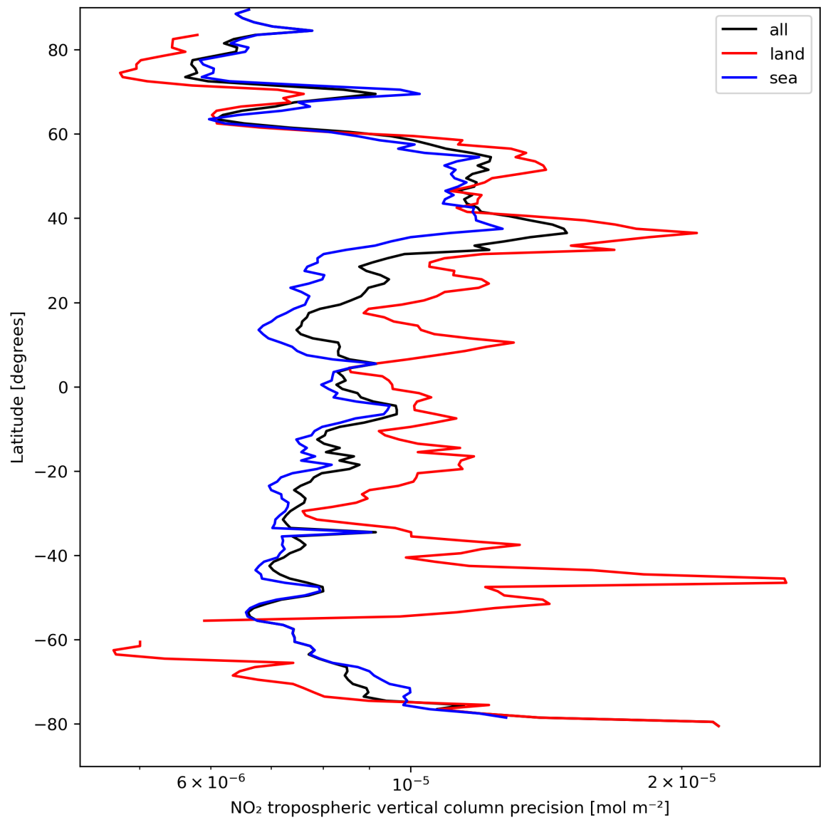
Figure 13: Zonal average of “NO 2 tropospheric vertical column precision” for 2024-04-08 to 2024-04-10.
