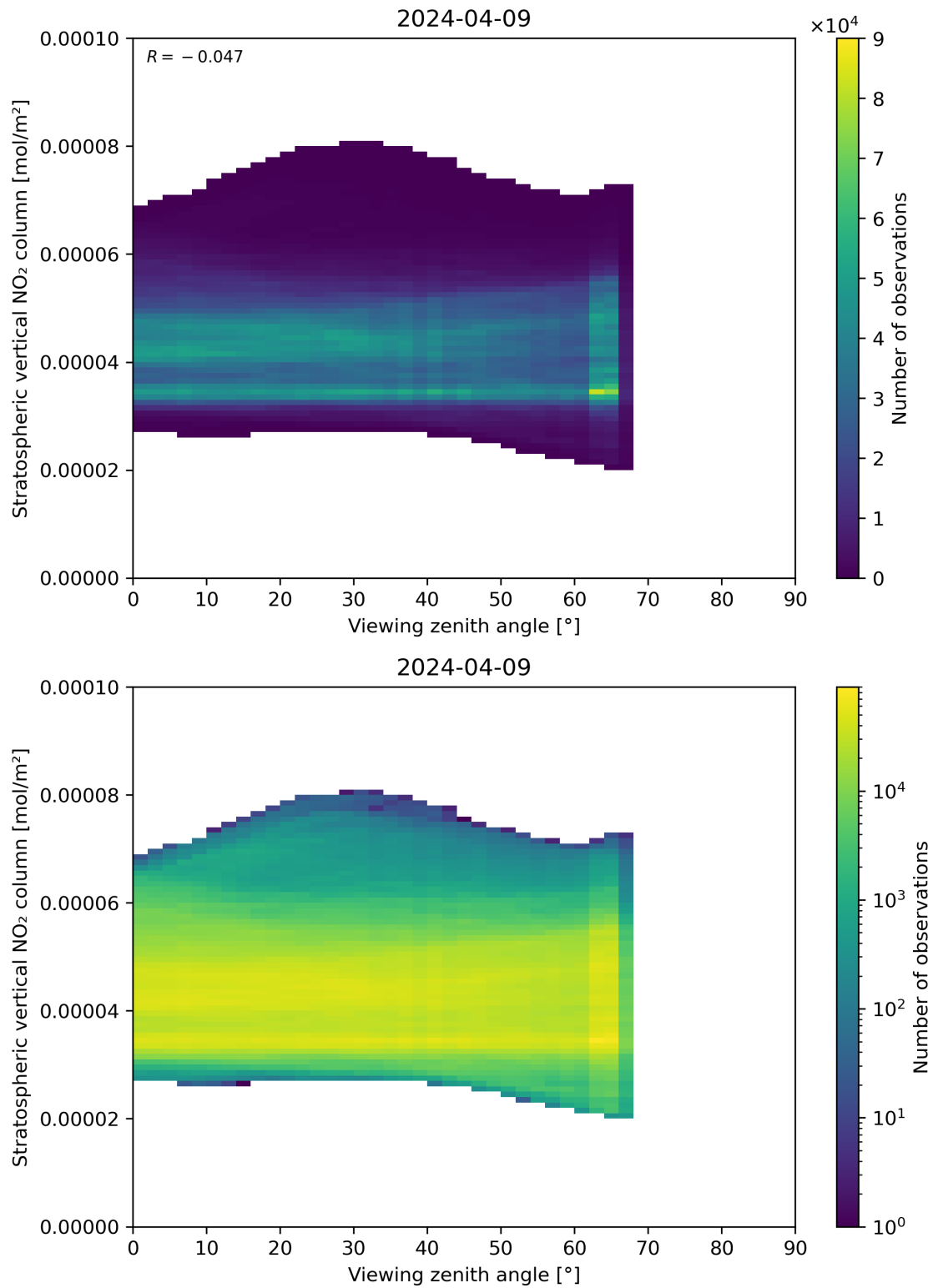
Figure 164: Scatter density plot of “Viewing zenith angle” against “Stratospheric vertical NO 2 column” for 2024-04-08 to 2024-04-10.
