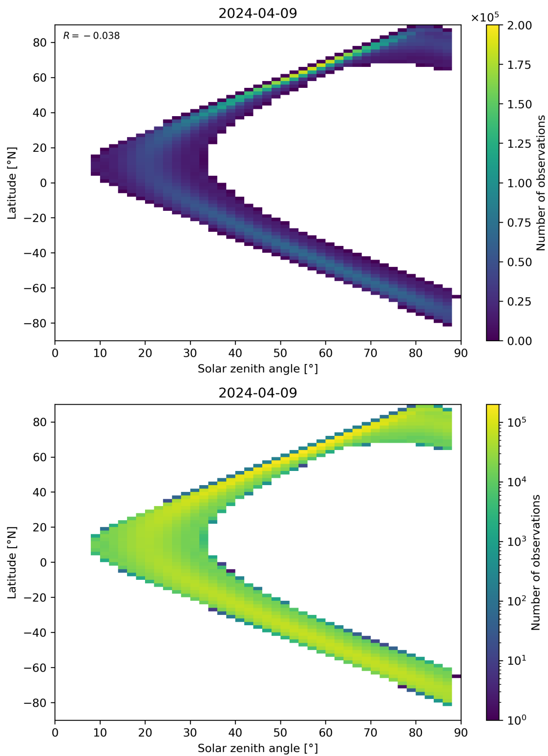
Figure 149: Scatter density plot of “Solar zenith angle” against “Latitude” for 2024-04-08 to 2024-04-10.
