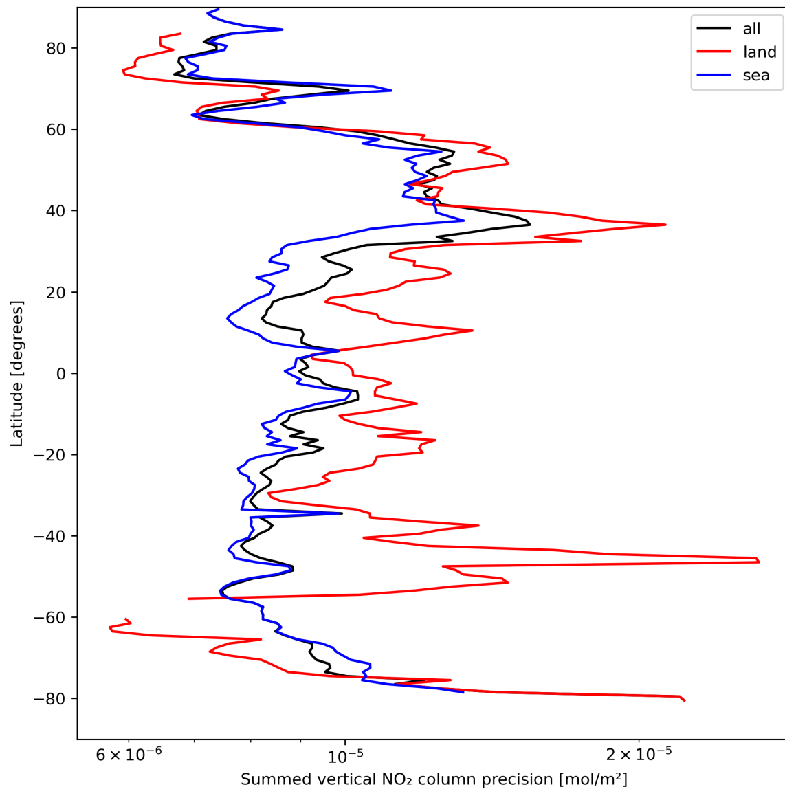
Figure 24: Zonal average of “Summed vertical NO 2 column precision” for 2024-04-08 to 2024-04-10.
