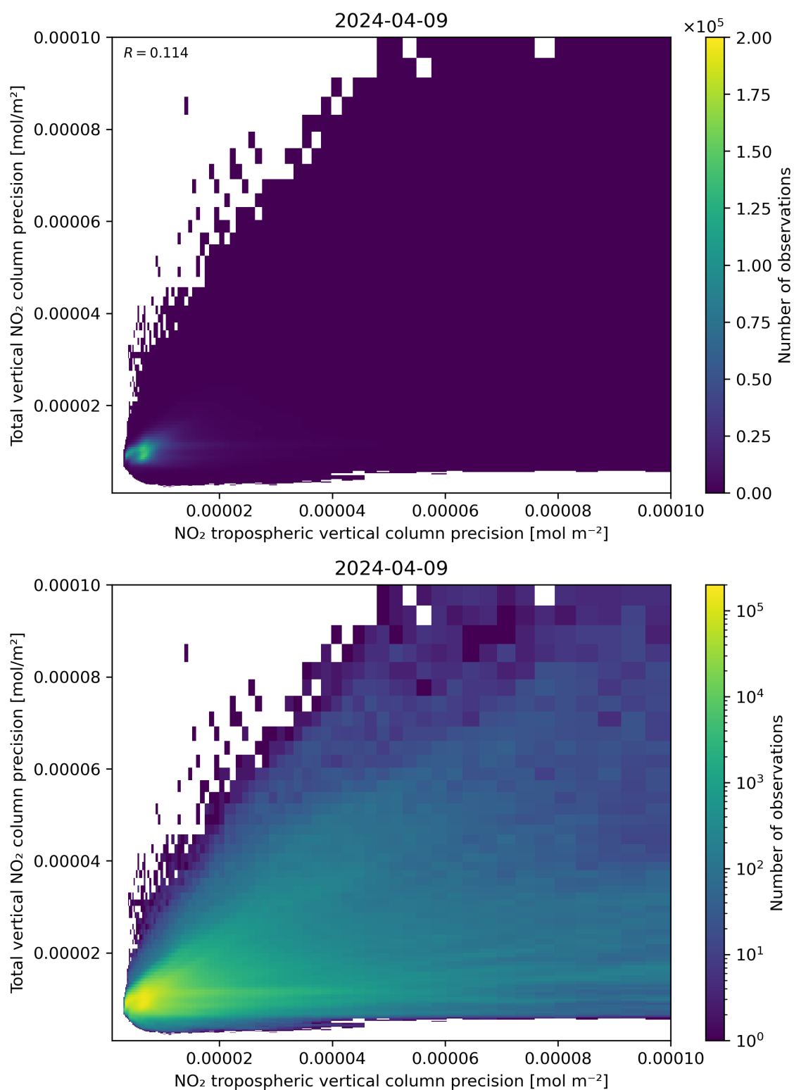
Figure 139: Scatter density plot of “NO 2 tropospheric vertical column precision” against “Total vertical NO 2 column precision” for 2024-04-08 to 2024-04-10.
