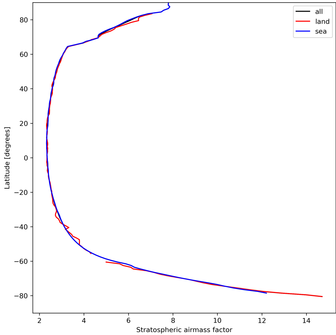
Figure 27: Zonal average of “Stratospheric airmass factor” for 2024-04-08 to 2024-04-10.
