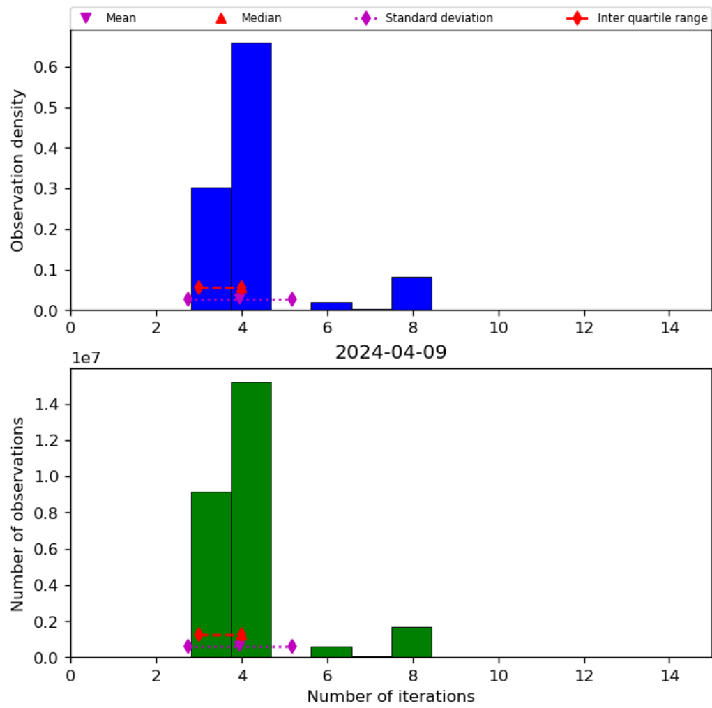
Figure 34: Histogram of “Number of iterations” for 2024-04-08 to 2024-04-10
