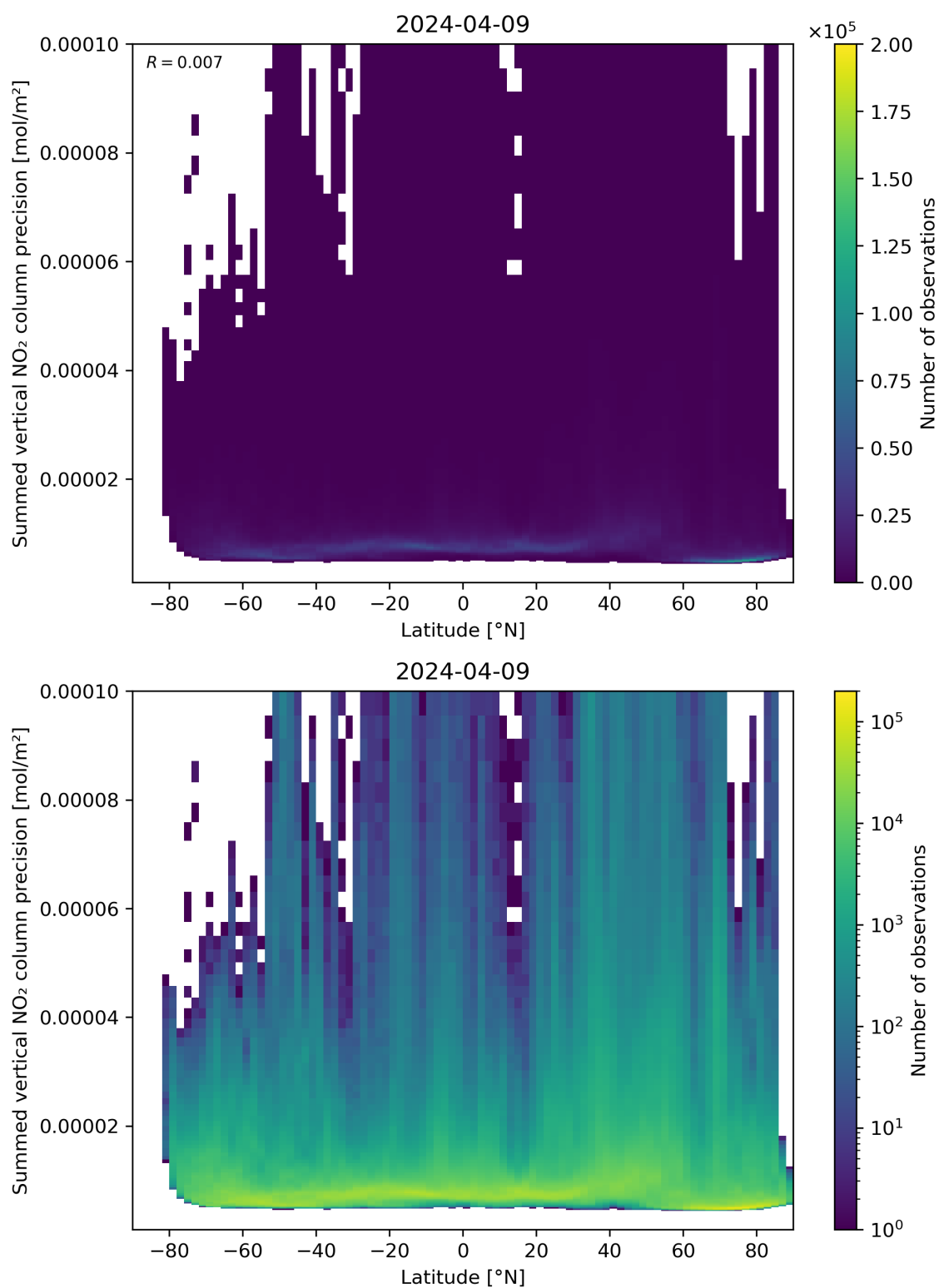
Figure 89: Scatter density plot of “Latitude” against “Summed vertical NO 2 column precision” for 2024-04-08 to 2024-04-10.
