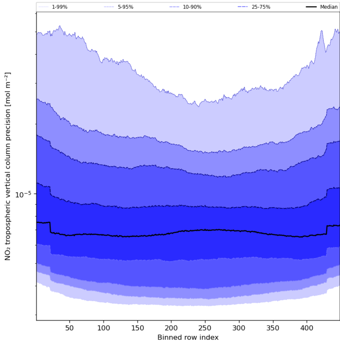
Figure 47: Along track statistics of “NO 2 tropospheric vertical column precision” for 2024-04-08 to 2024-04-10
