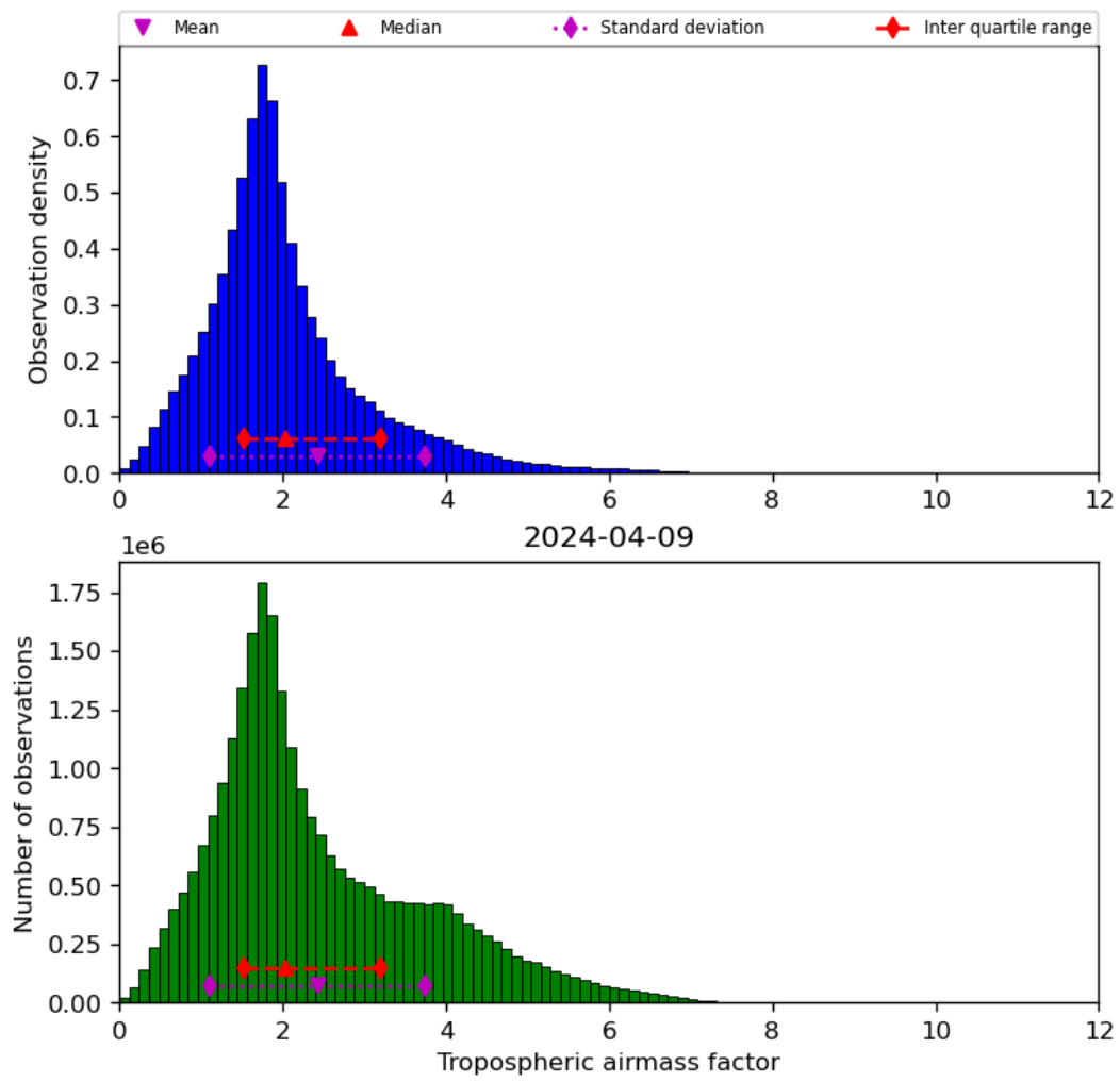
Figure 31: Histogram of “Tropospheric airmass factor” for 2024-04-08 to 2024-04-10
