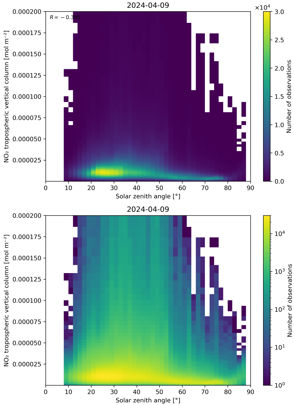
Figure 155: Scatter density plot of “Solar zenith angle” against “NO 2 tropospheric vertical column” for 2024-04-08 to 2024-04-10.
