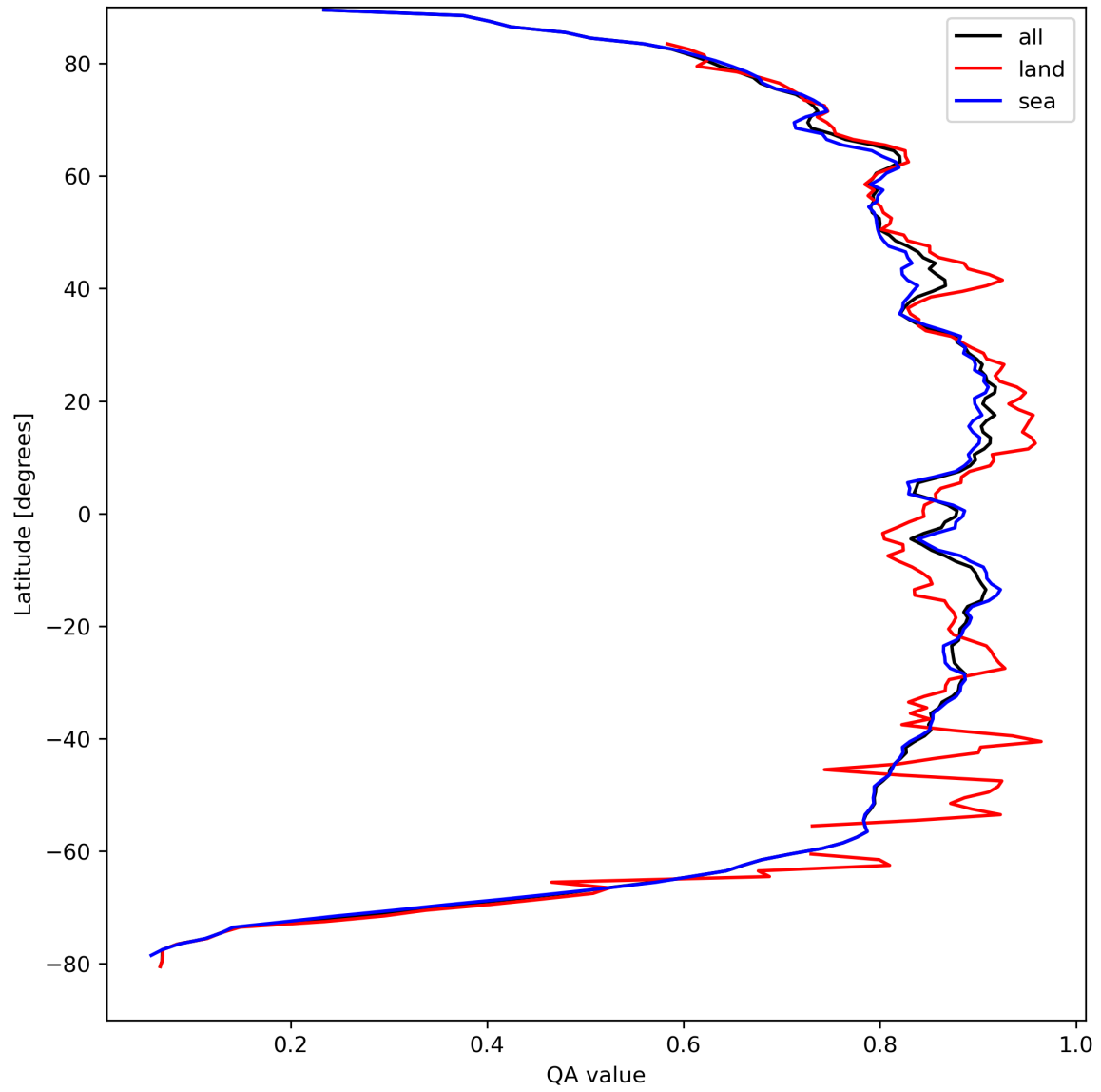
Figure 11: Zonal average of “QA value” for 2024-04-08 to 2024-04-10.
