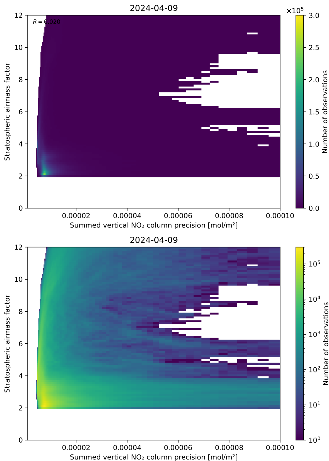
Figure 106: Scatter density plot of “Summed vertical NO 2 column precision” against “Stratospheric airmass factor” for 2024-04-08 to 2024-04-10.
