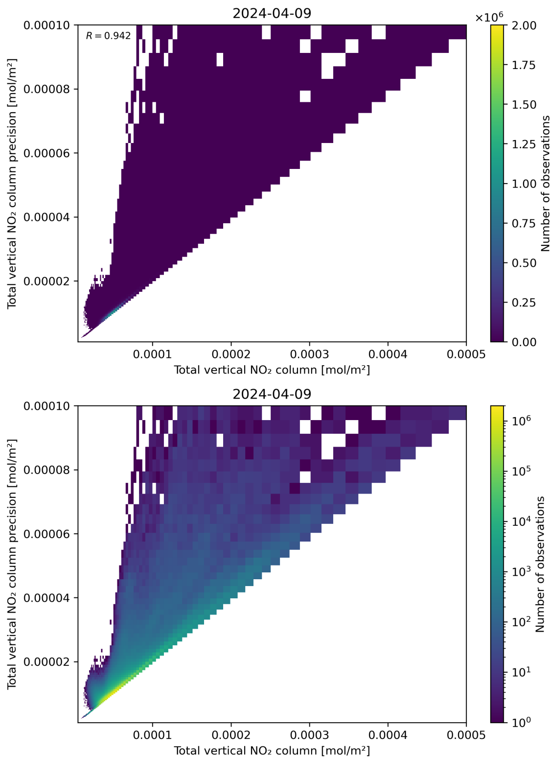
Figure 114: Scatter density plot of “Total vertical NO 2 column” against “Total vertical NO 2 column precision” for 2024-04-08 to 2024-04-10.
