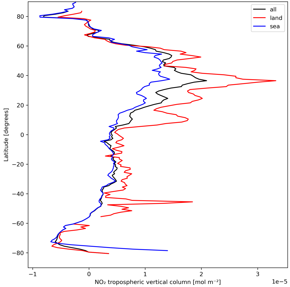
Figure 12: Zonal average of “NO 2 tropospheric vertical column” for 2024-04-08 to 2024-04-10.
