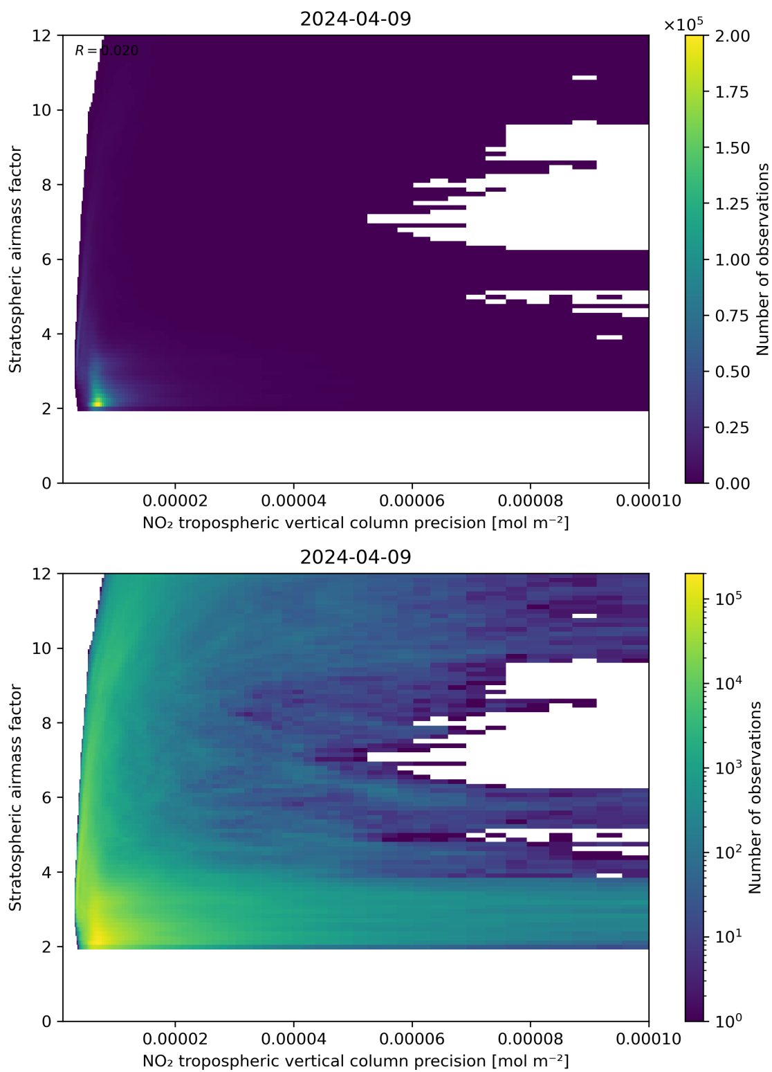
Figure 131: Scatter density plot of “NO 2 tropospheric vertical column precision” against “Stratospheric airmass factor” for 2024-04-08 to 2024-04-10.
