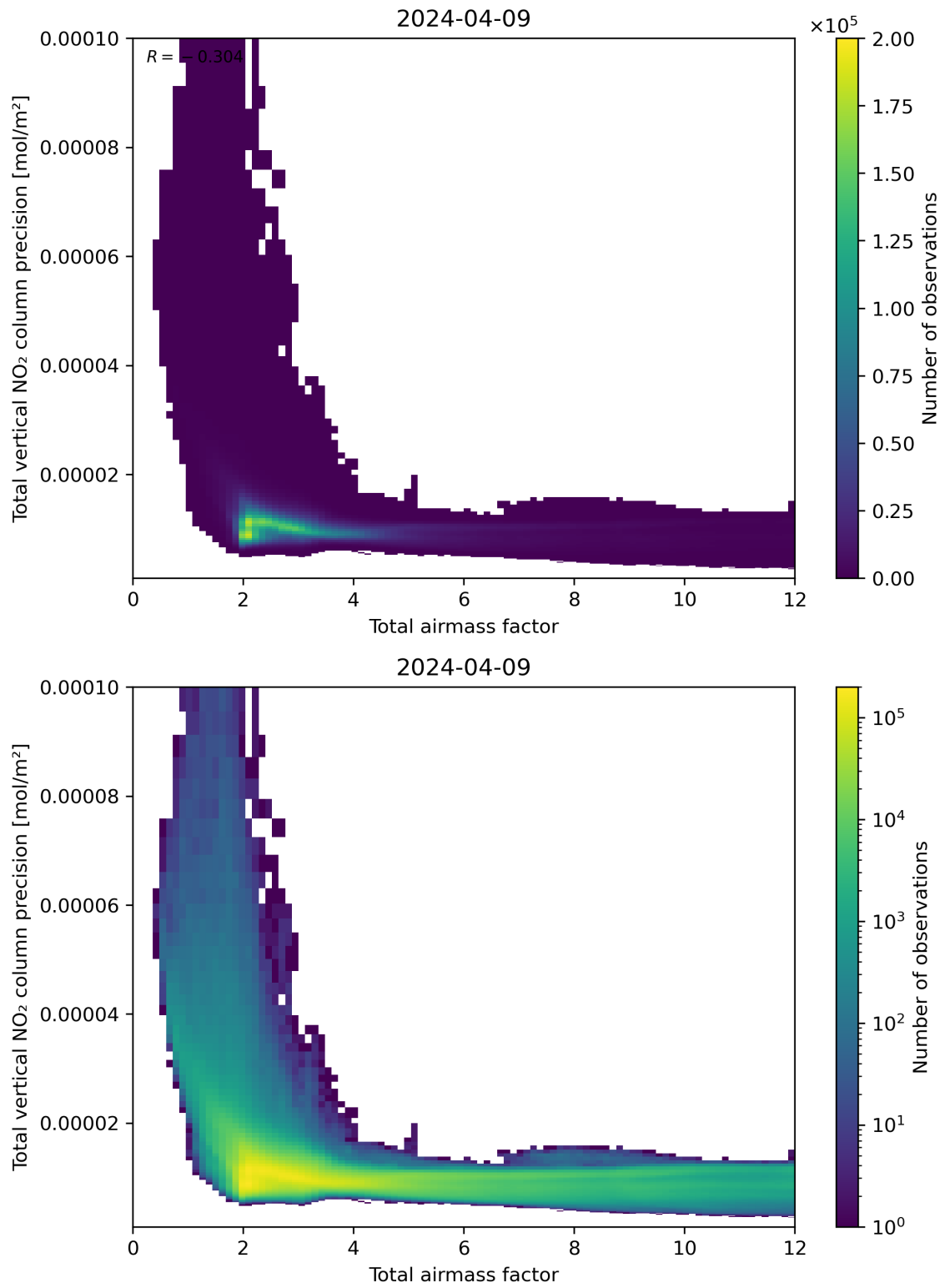
Figure 68: Scatter density plot of “Total airmass factor” against “Total vertical NO 2 column precision” for 2024-04-08 to 2024-04-10.
