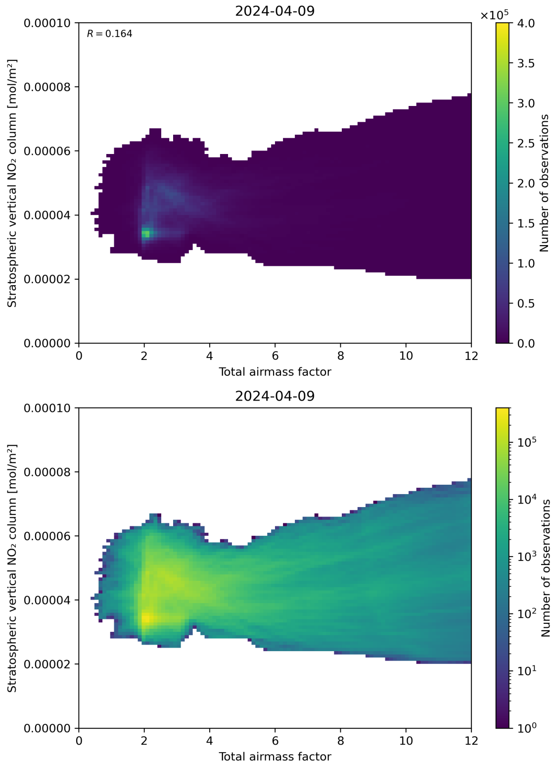
Figure 64: Scatter density plot of “Total airmass factor” against “Stratospheric vertical \text{NO}_2 column” for 2024-04-08 to 2024-04-10.
