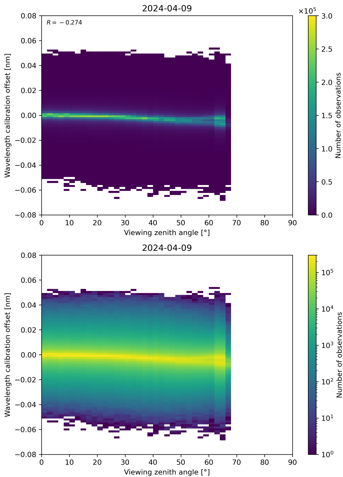
Figure 173: Scatter density plot of “Viewing zenith angle” against “Wavelength calibration offset” for 2024-04-08 to 2024-04-10.
