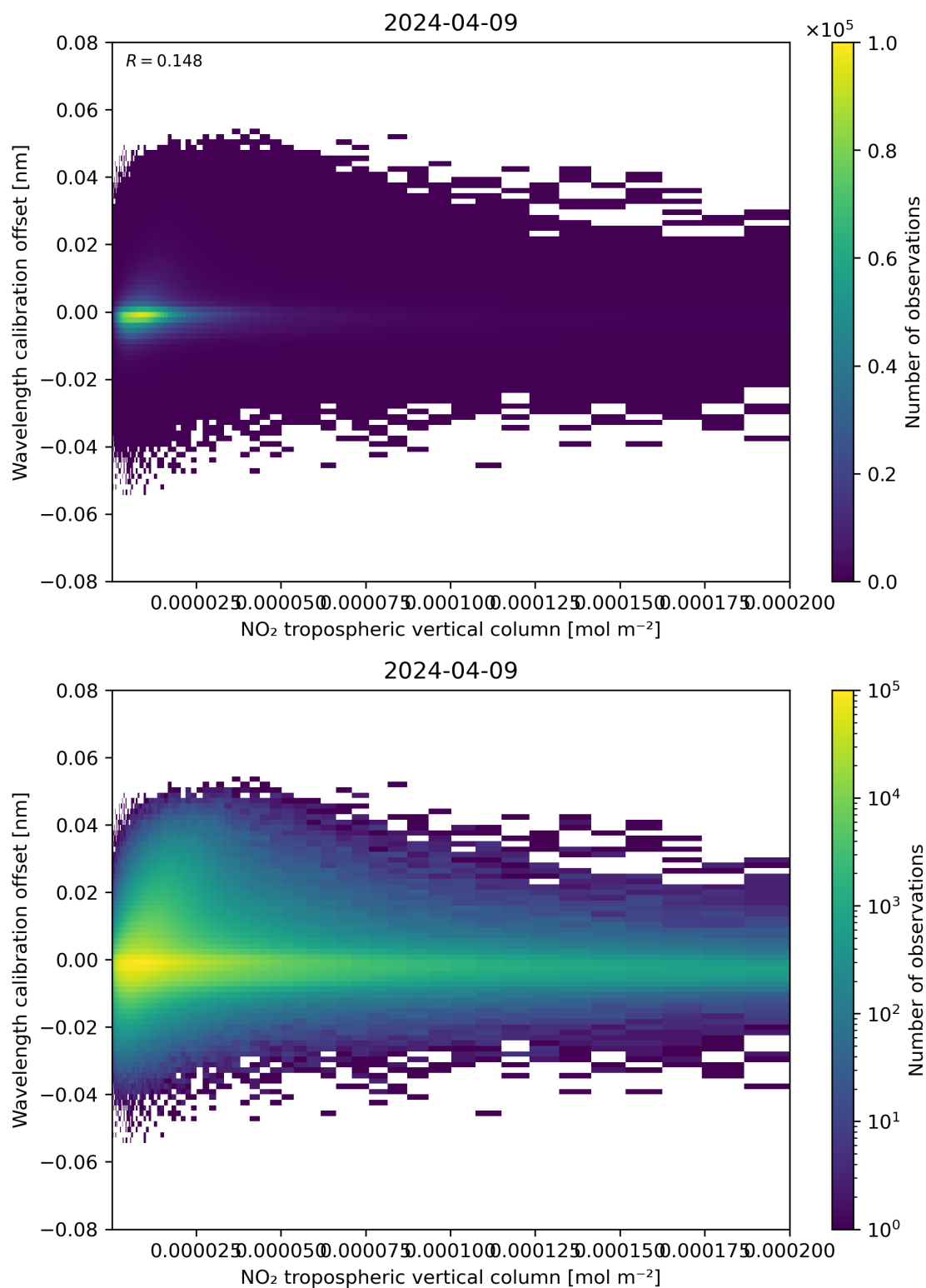
Figure 143: Scatter density plot of “NO 2 tropospheric vertical column” against “Wavelength calibration offset” for 2024-04-08 to 2024-04-10.
