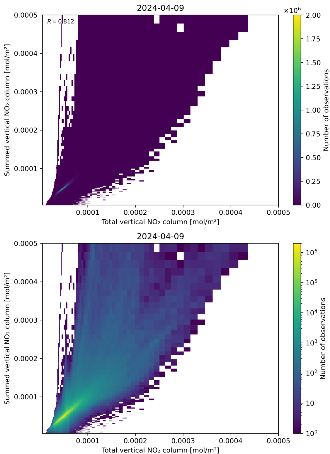
Figure 112: Scatter density plot of “Total vertical NO 2 column” against “Summed vertical NO 2 column” for 2024-04-08 to 2024-04-10.
