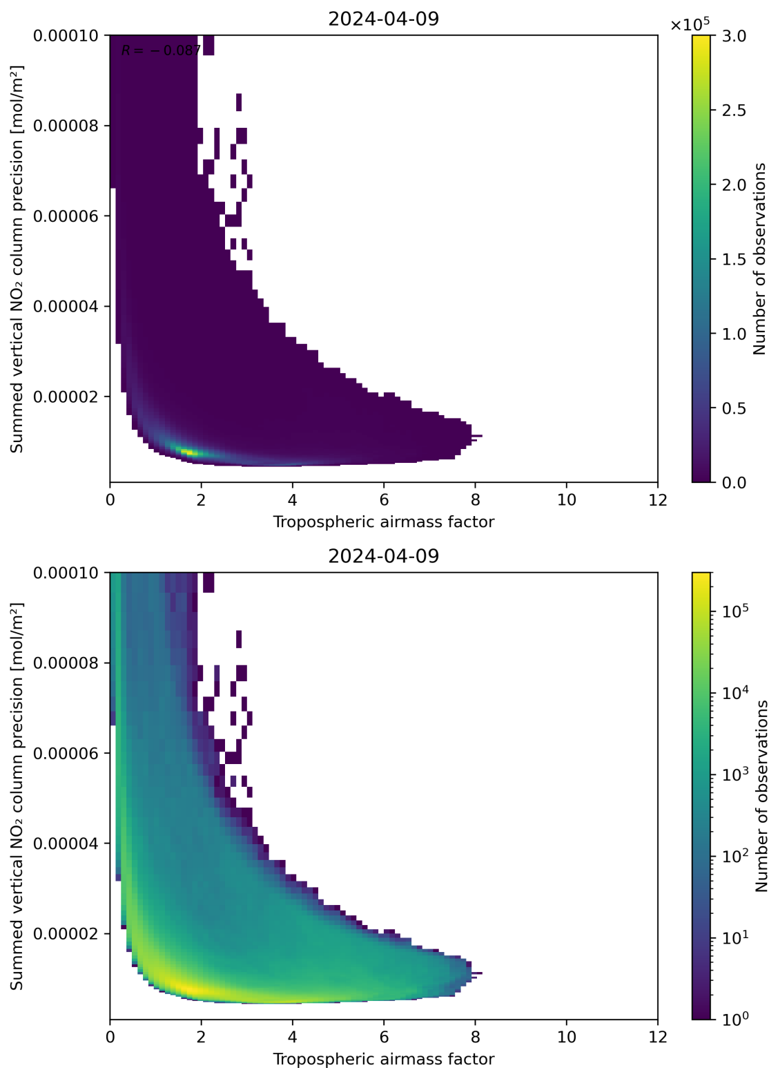
Figure 76: Scatter density plot of “Tropospheric air mass factor” against “Summed vertical NO 2 column precision” for 2024-04-08 to 2024-04-10.
