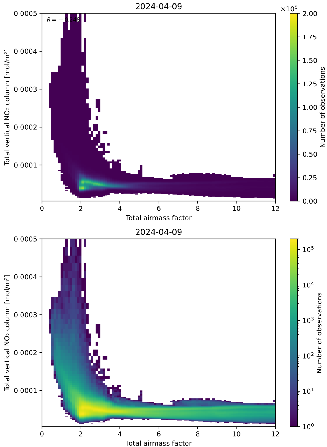
Figure 67: Scatter density plot of “Total airmass factor” against “Total vertical NO 2 column” for 2024-04-08 to 2024-04-10.
