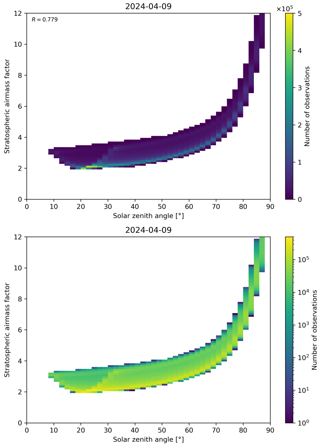
Figure 145: Scatter density plot of “Solar zenith angle” against “Stratospheric airmass factor” for 2024-04-08 to 2024-04-10.
