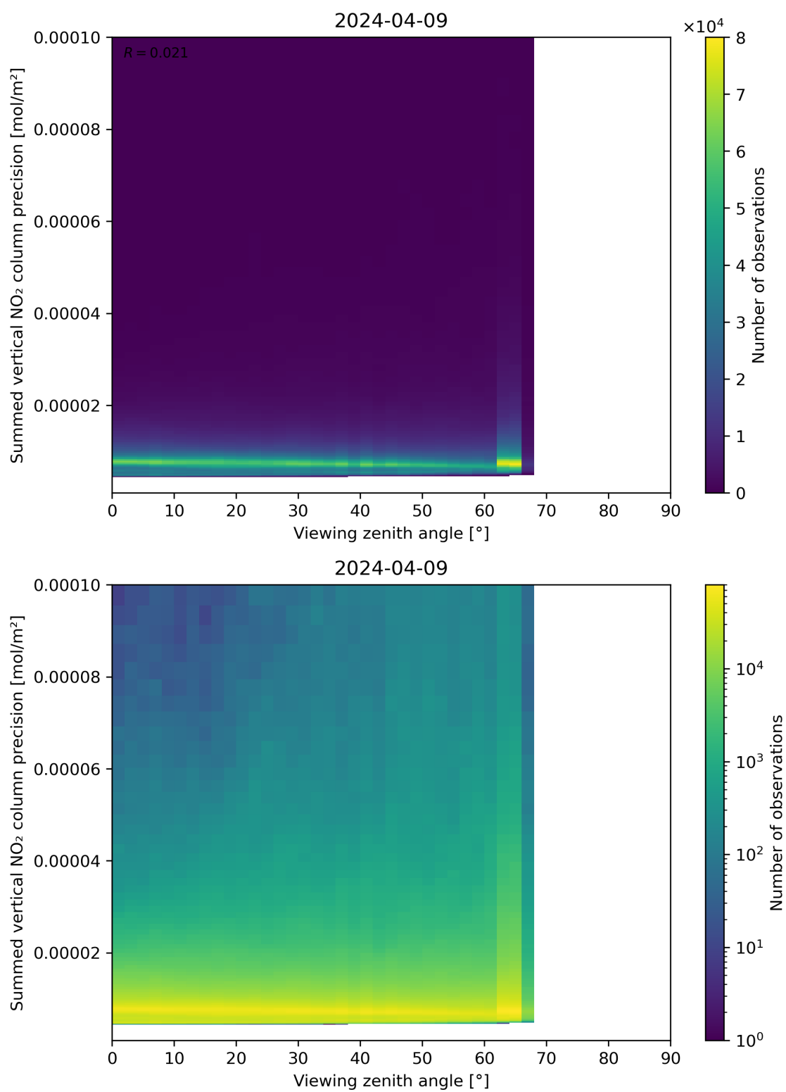
Figure 166: Scatter density plot of “Viewing zenith angle” against “Summed vertical NO 2 column precision” for 2024-04-08 to 2024-04-10.
