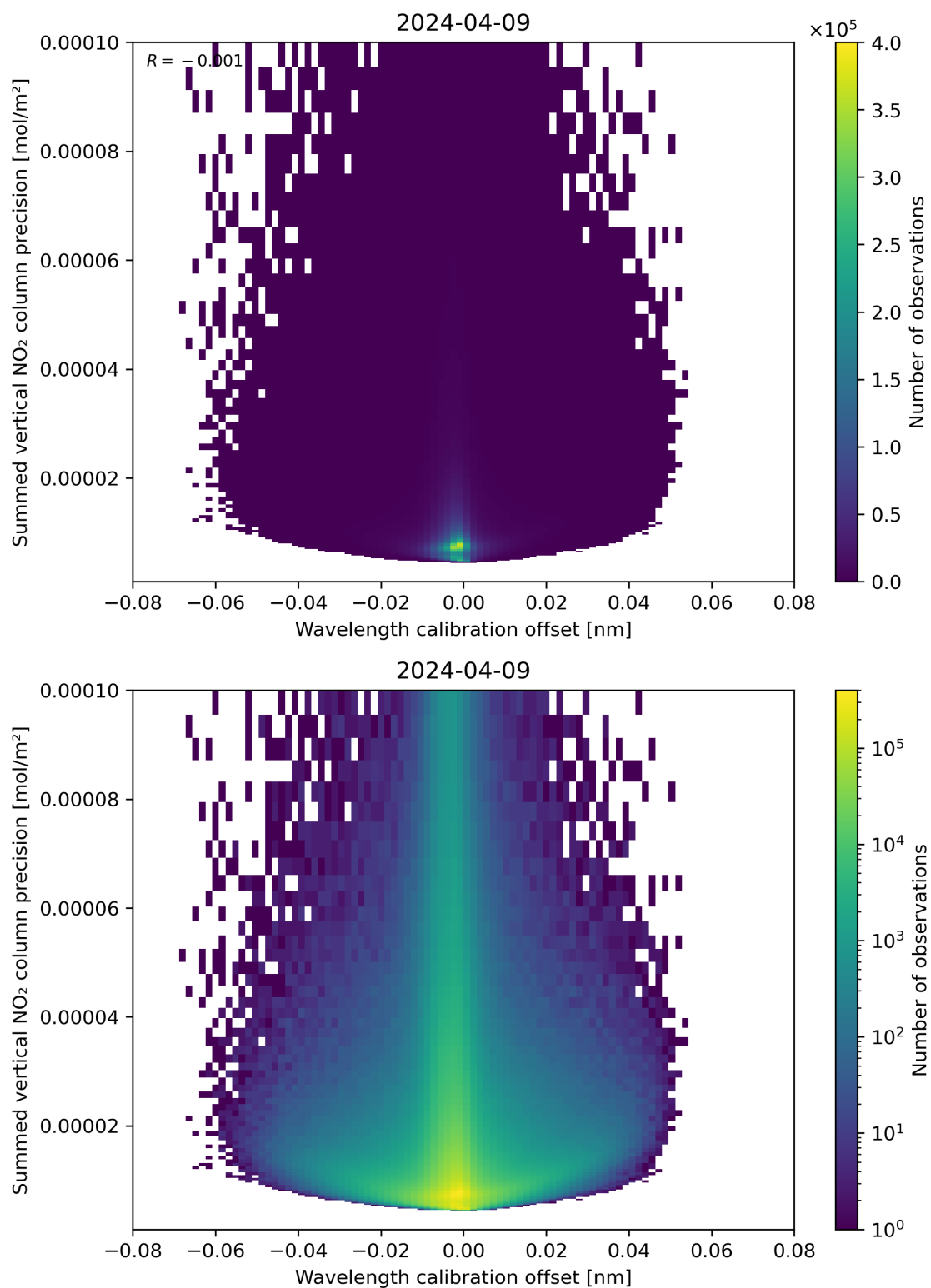
Figure 178: Scatter density plot of “Wavelength calibration offset” against “Summed vertical NO 2 column precision” for 2024-04-08 to 2024-04-10.
