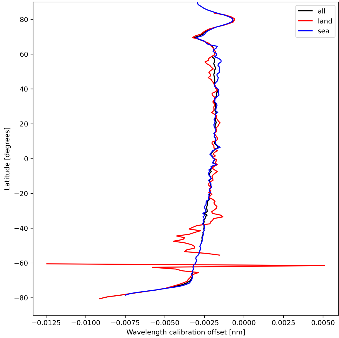
Figure 18: Zonal average of “Wavelength calibration offset” for 2024-04-08 to 2024-04-10.
