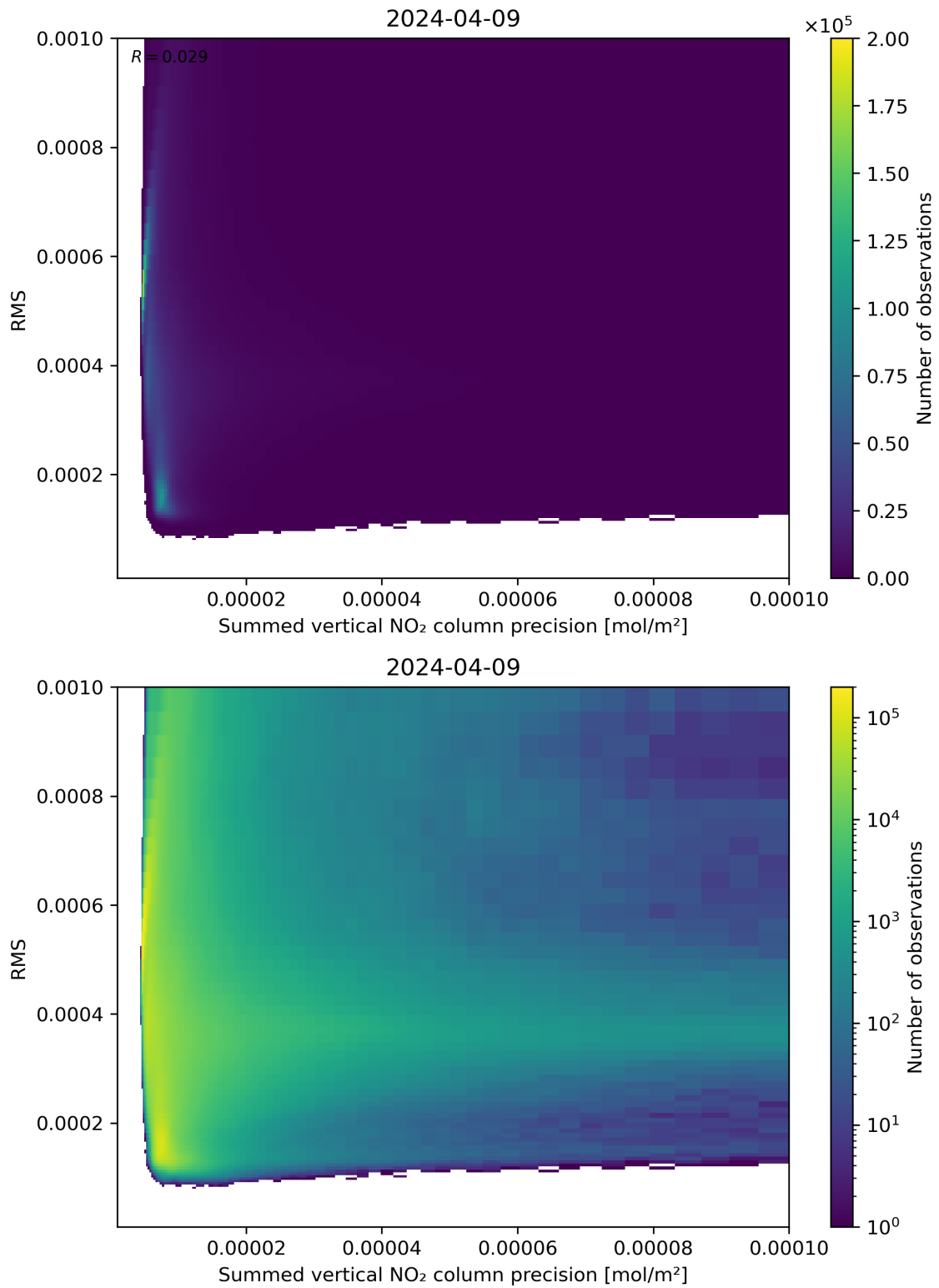
Figure 108: Scatter density plot of “Summed vertical NO 2 column precision” against “RMS” for 2024-04-08 to 2024-04-10.
