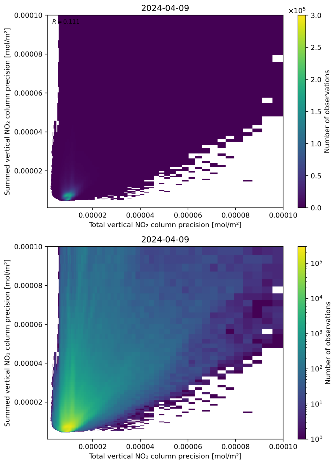
Figure 118: Scatter density plot of “Total vertical NO 2 column precision” against “Summed vertical NO 2 column precision” for 2024-04-08 to 2024-04-10.
