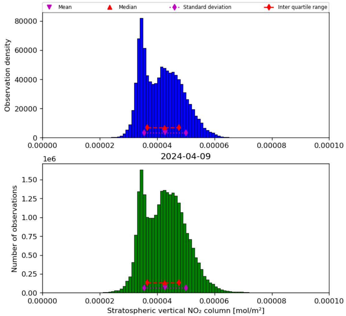
Figure 36: Histogram of “Stratospheric vertical NO 2 column” for 2024-04-08 to 2024-04-10
