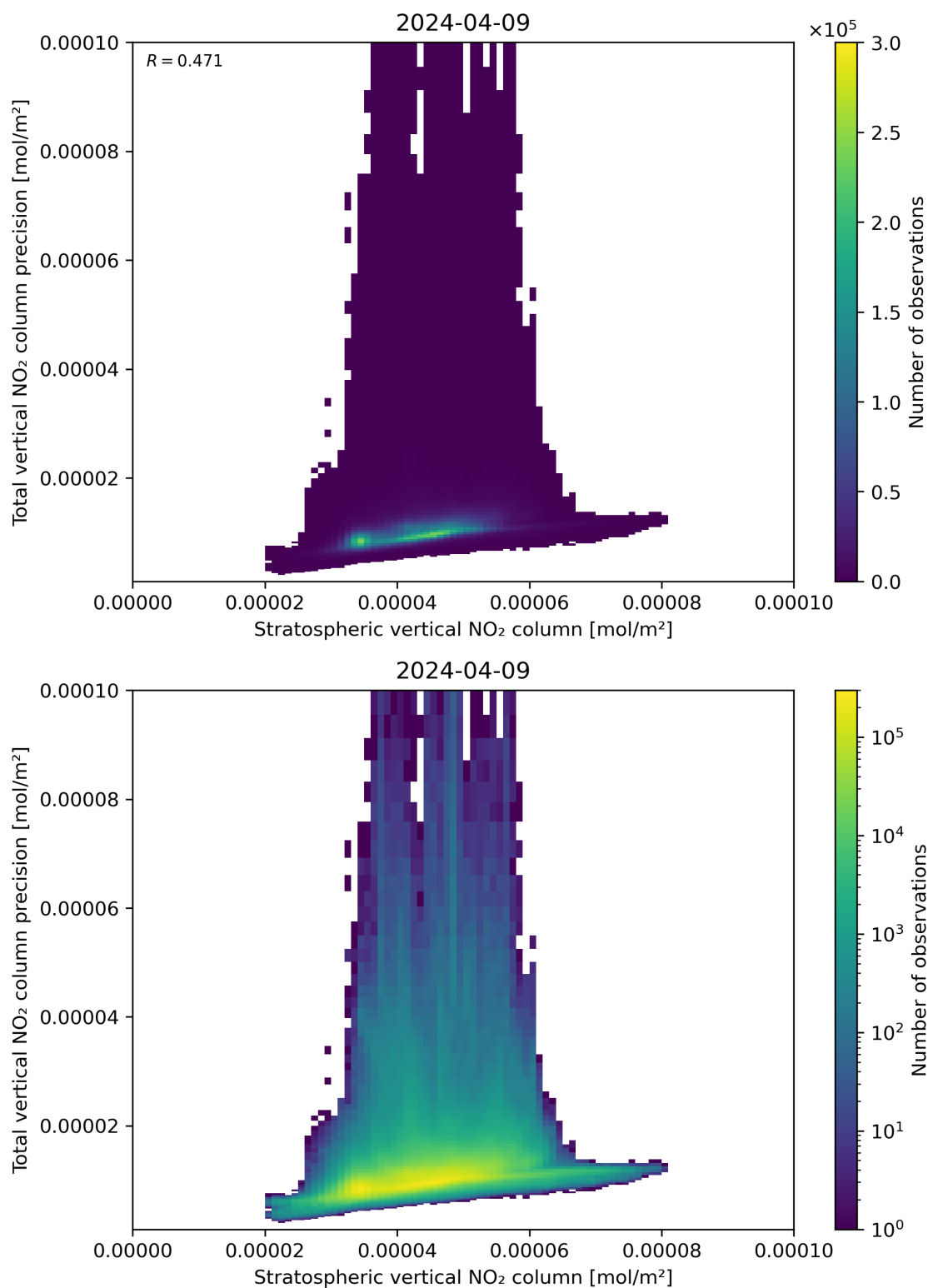
Figure 101: Scatter density plot of “Stratospheric vertical NO 2 column” against “Total vertical NO 2 column precision” for 2024-04-08 to 2024-04-10.
