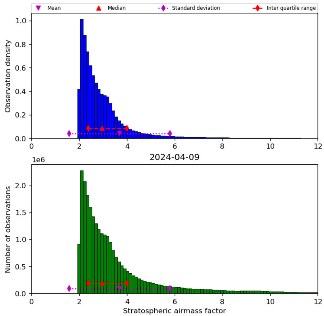
Figure 44: Histogram of “Stratospheric airmass factor” for 2024-04-08 to 2024-04-10
