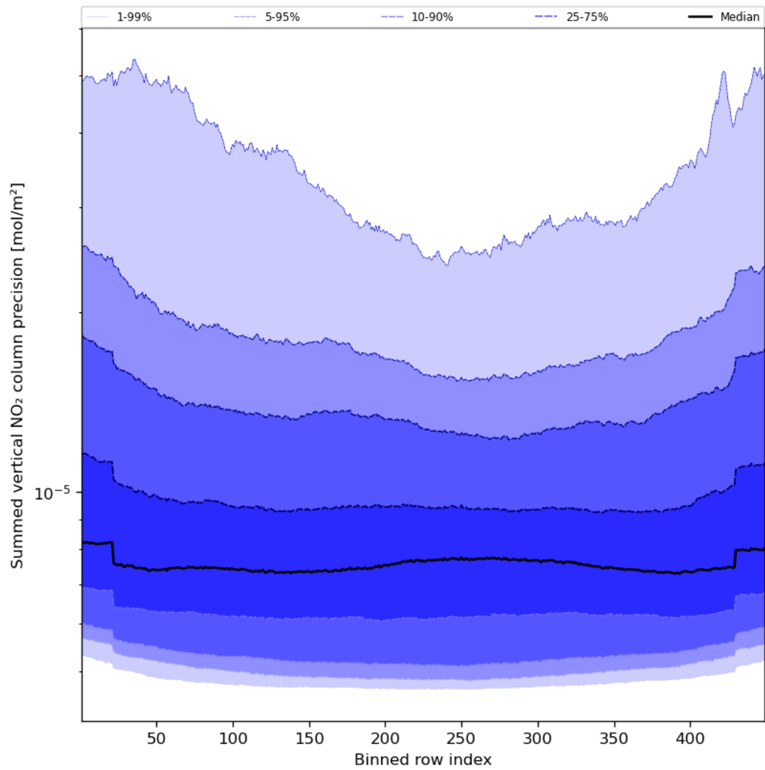
Figure 58: Along track statistics of “Summed vertical NO 2 column precision” for 2024-04-08 to 2024-04-10
