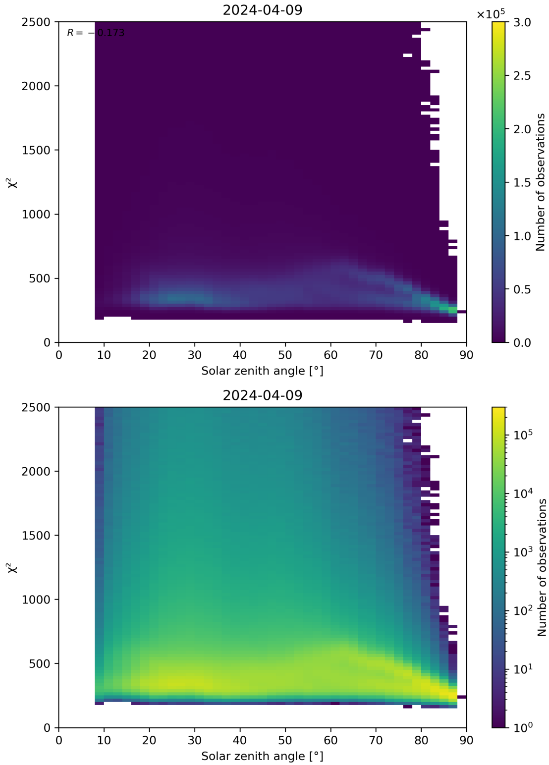
Figure 148: Scatter density plot of “Solar zenith angle” against “ \chi^2 ” for 2024-04-08 to 2024-04-10.
