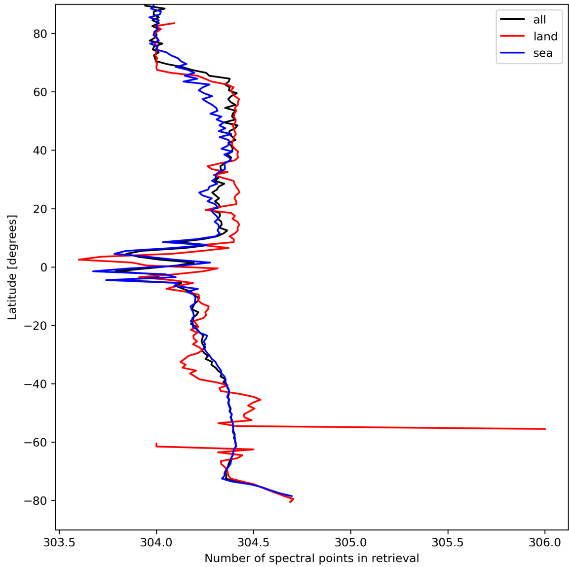
Figure 16: Zonal average of “Number of spectral points in retrieval” for 2024-04-08 to 2024-04-10.
