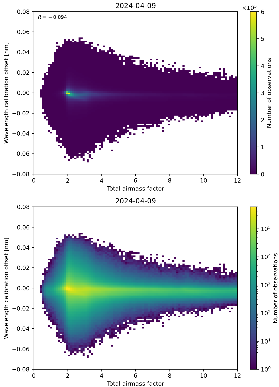
Figure 70: Scatter density plot of “Total airmass factor” against “Wavelength calibration offset” for 2024-04-08 to 2024-04-10.
