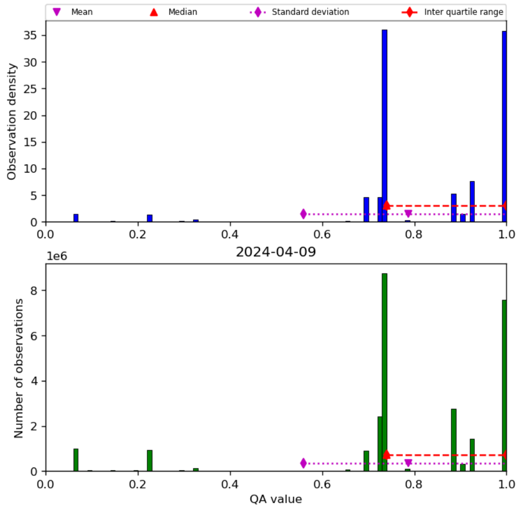
Figure 28: Histogram of “QA value” for 2024-04-08 to 2024-04-10
