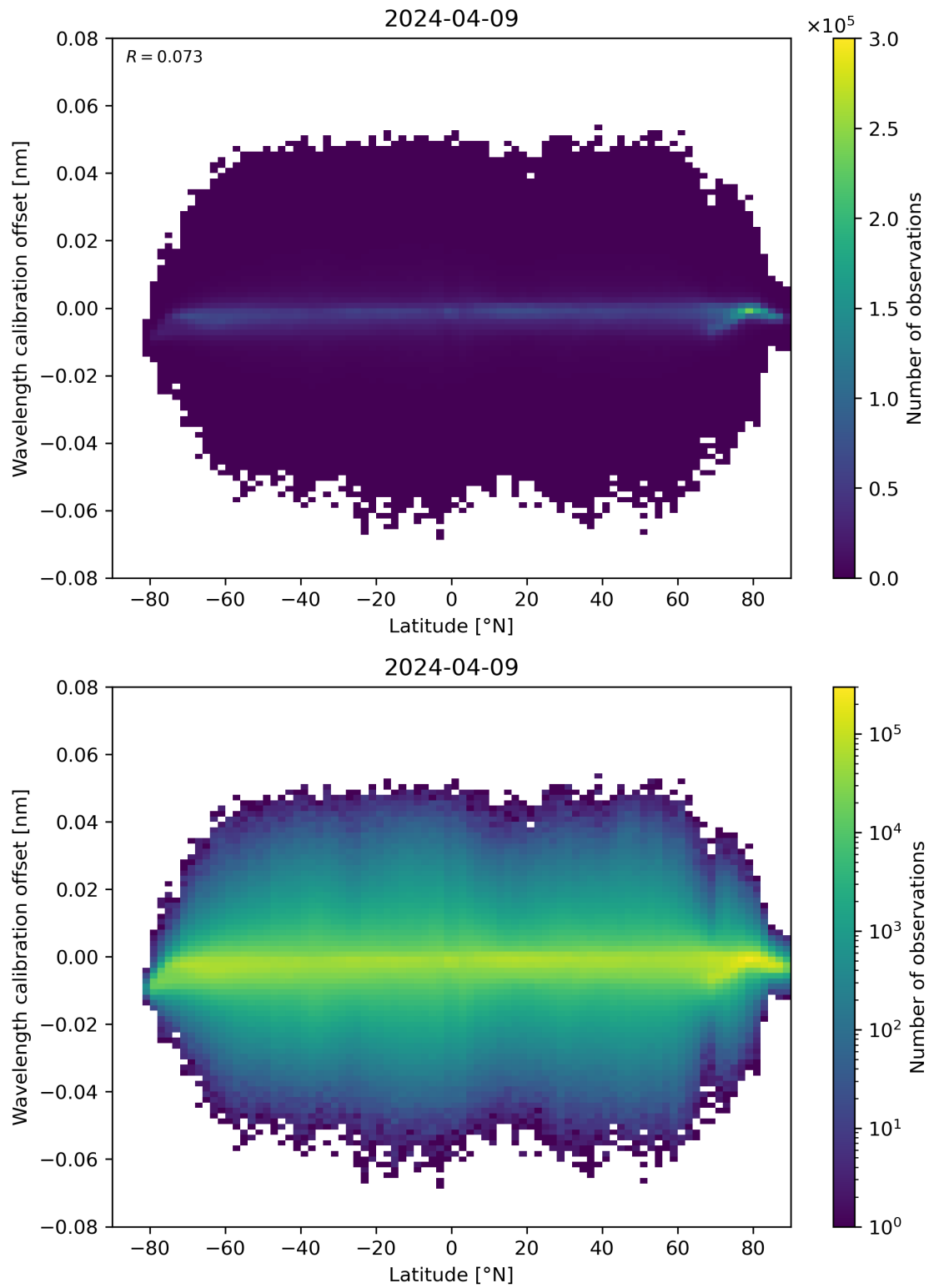
Figure 95: Scatter density plot of “Latitude” against “Wavelength calibration offset” for 2024-04-08 to 2024-04-10.
