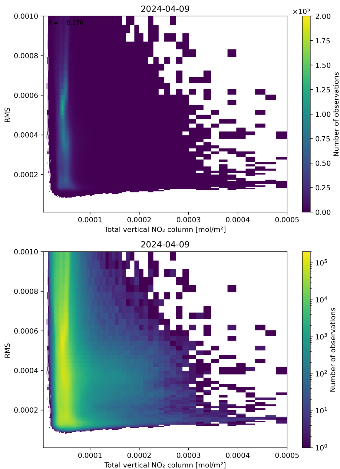
Figure 120: Scatter density plot of “Total vertical NO 2 column” against “RMS” for 2024-04-08 to 2024-04-10.
