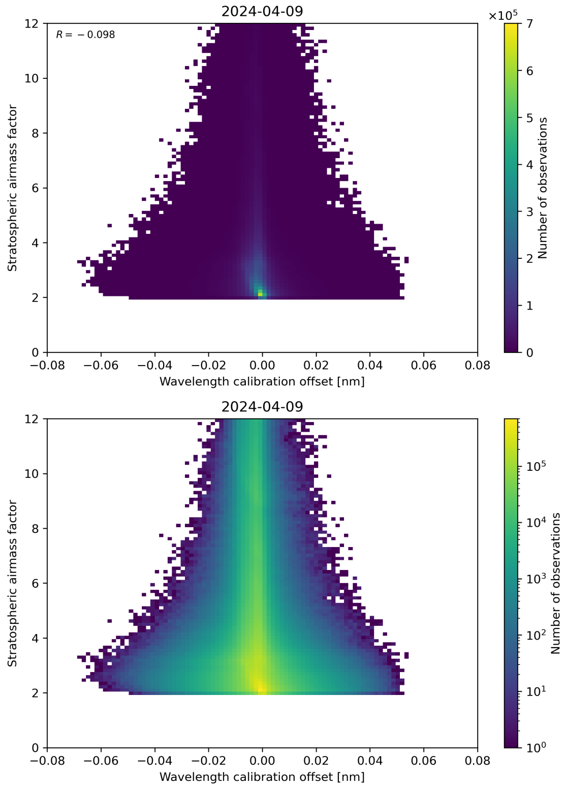
Figure 174: Scatter density plot of “Wavelength calibration offset” against “Stratospheric airmass factor” for 2024-04-08 to 2024-04-10.
