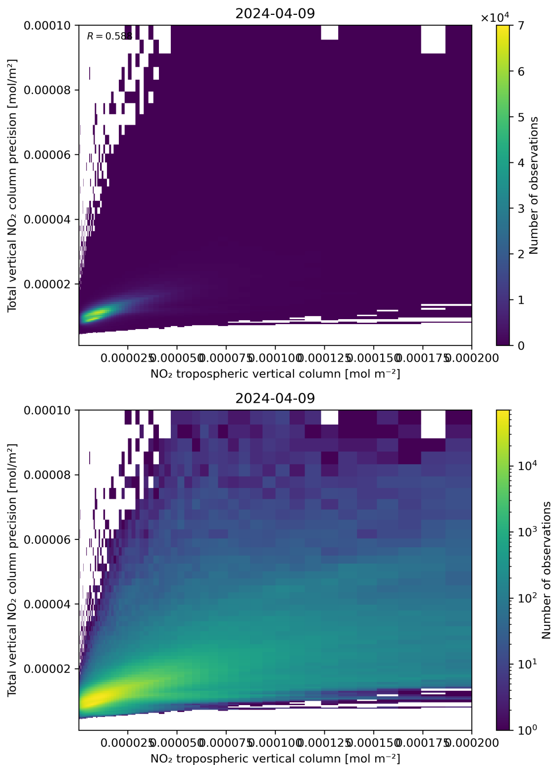
Figure 129: Scatter density plot of “NO 2 tropospheric vertical column” against “Total vertical NO 2 column precision” for 2024-04-08 to 2024-04-10.
