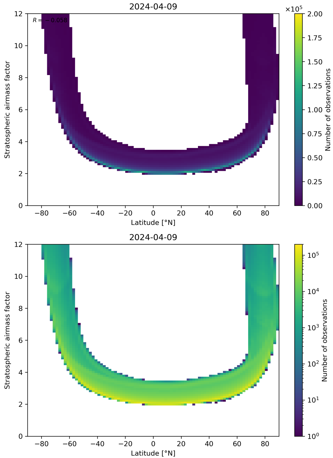
Figure 83: Scatter density plot of “Latitude” against “Stratospheric air mass factor” for 2024-04-08 to 2024-04-10.
