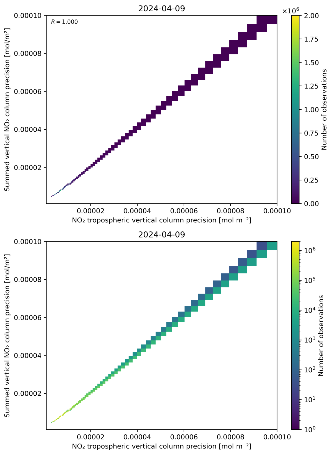
Figure 137: Scatter density plot of “NO 2 tropospheric vertical column precision” against “Summed vertical NO 2 column precision” for 2024-04-08 to 2024-04-10.
