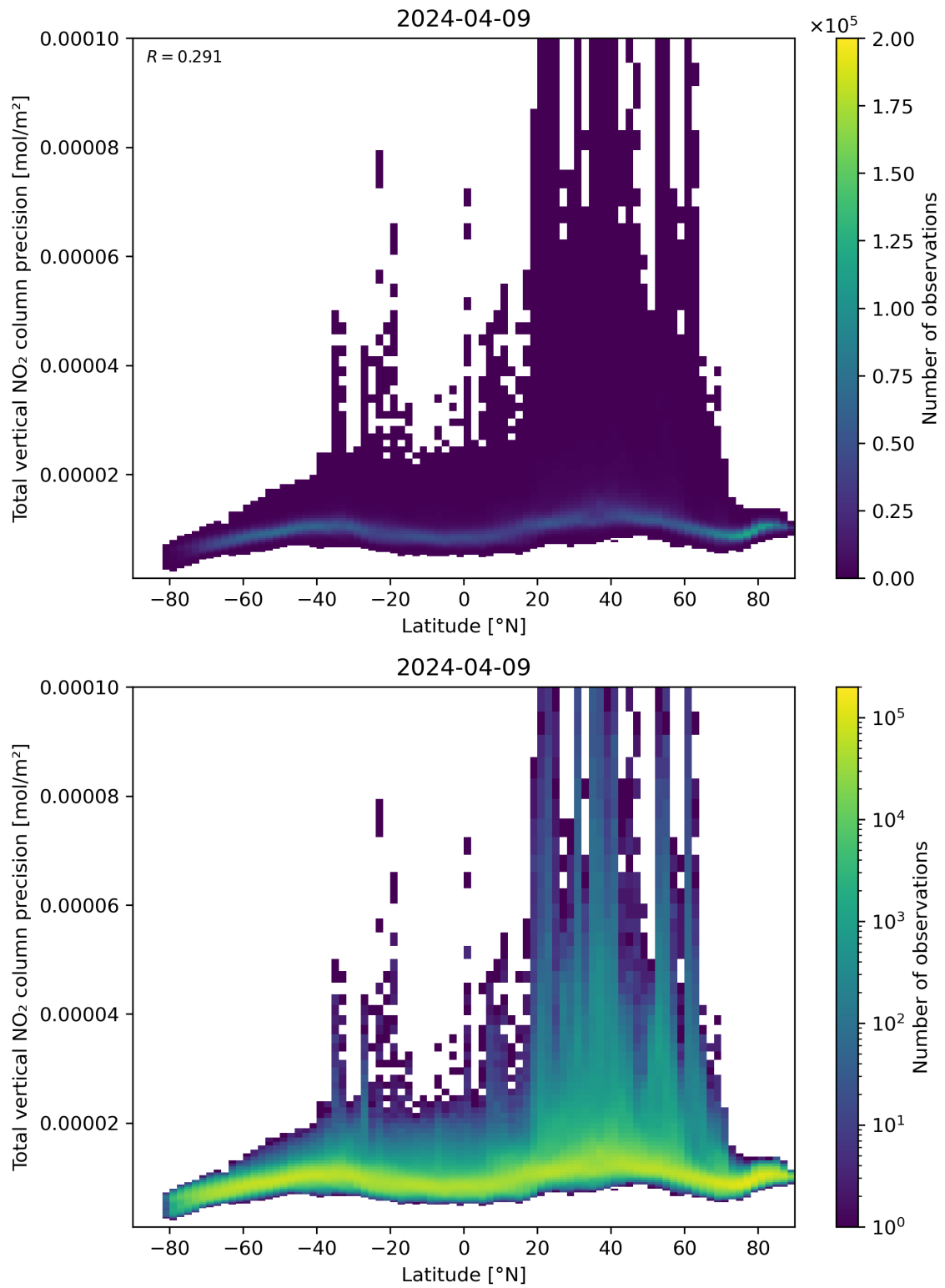
Figure 91: Scatter density plot of “Latitude” against “Total vertical NO 2 column precision” for 2024-04-08 to 2024-04-10.
