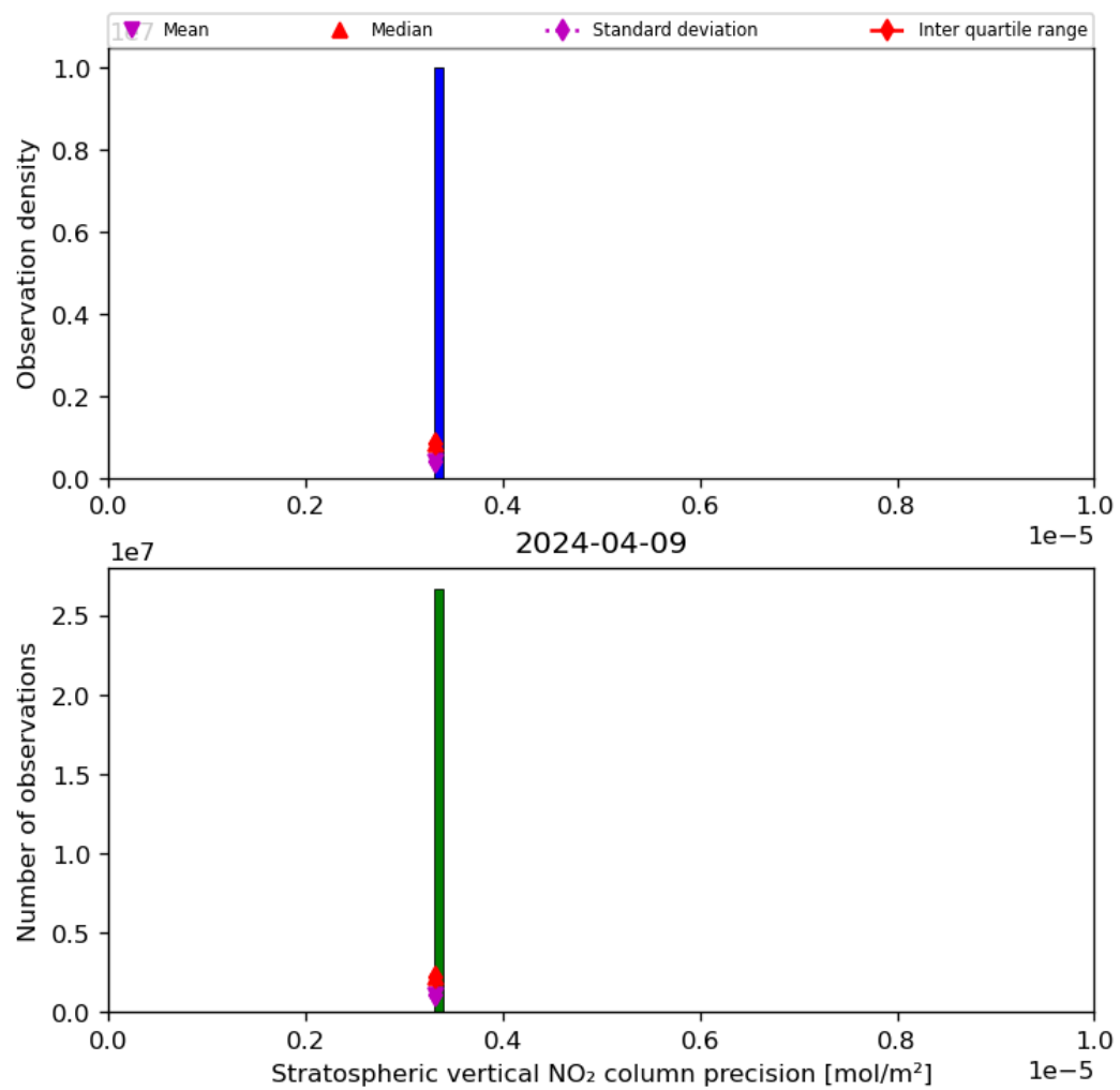
Figure 37: Histogram of “Stratospheric vertical NO 2 column precision” for 2024-04-08 to 2024-04-10
