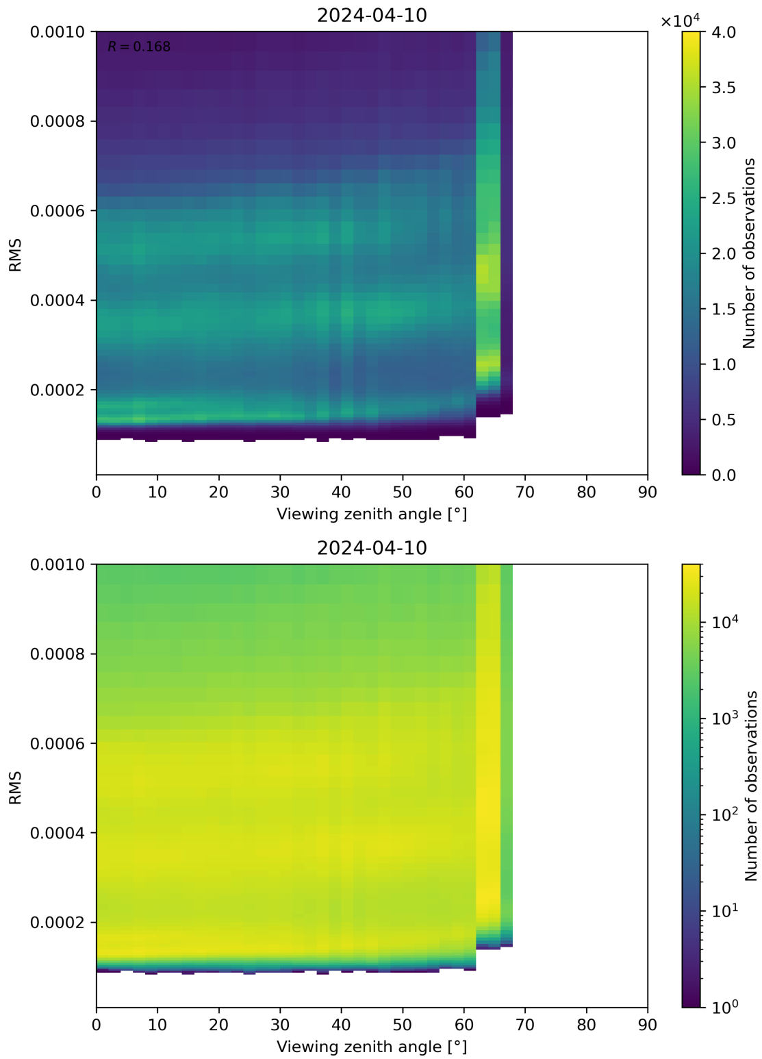
Figure 171: Scatter density plot of “Viewing zenith angle” against “RMS” for 2024-04-10 to 2024-04-11.
