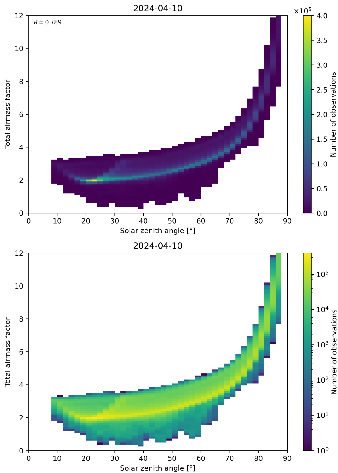
Figure 146: Scatter density plot of “Solar zenith angle” against “Total airmass factor” for 2024-04-10 to 2024-04-11.
