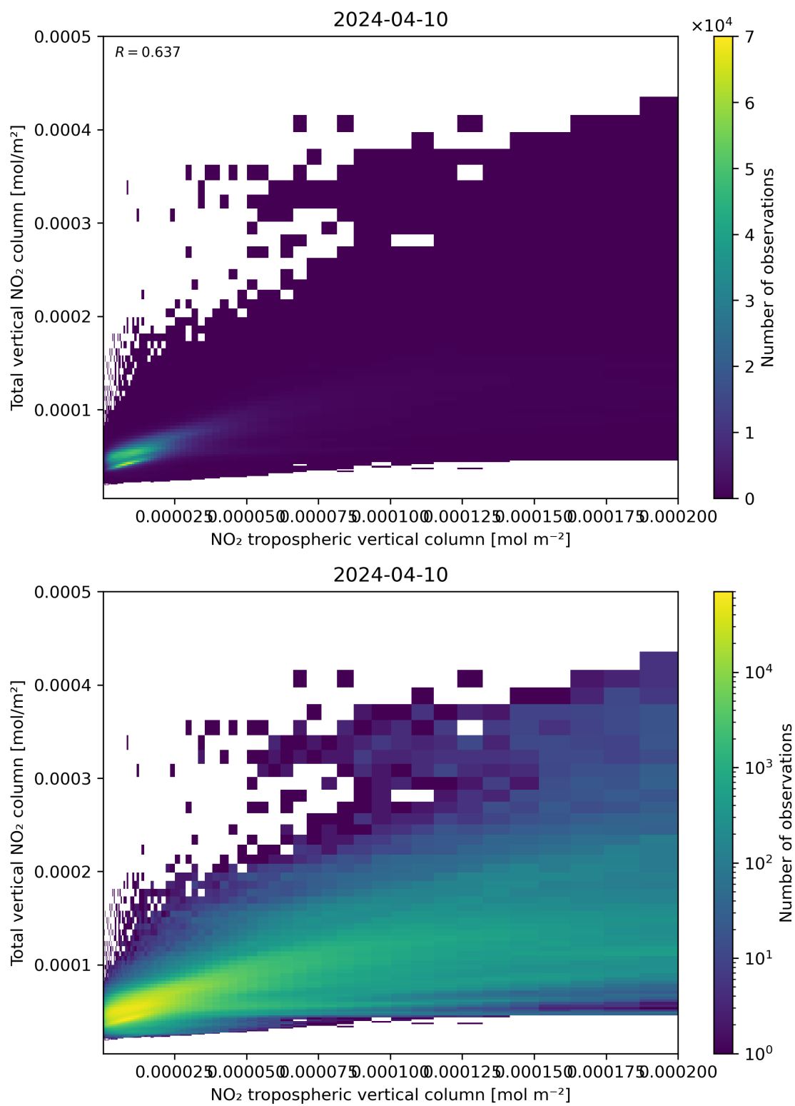
Figure 128: Scatter density plot of “NO 2 tropospheric vertical column” against “Total vertical NO 2 column” for 2024-04-10 to 2024-04-11.
