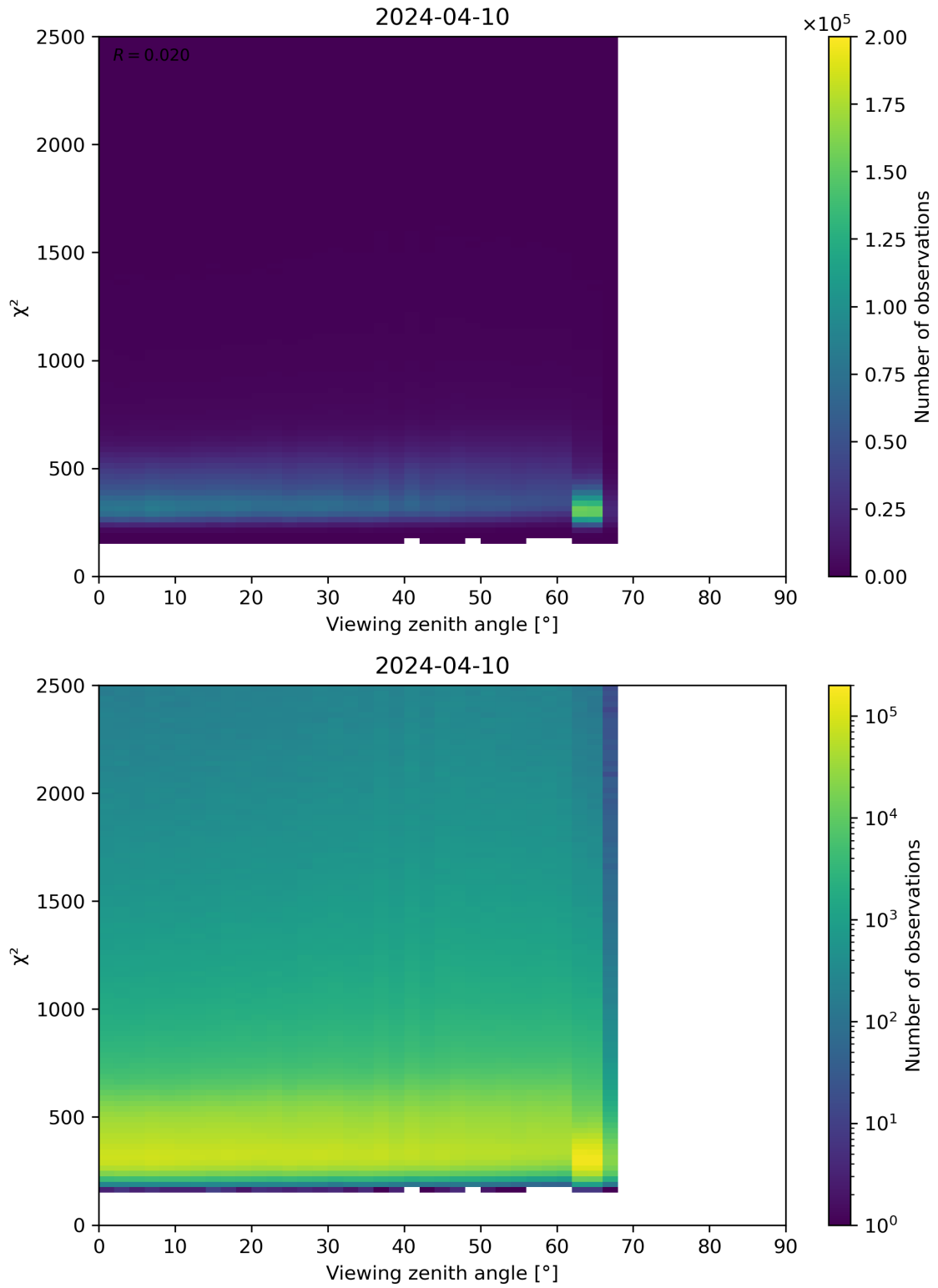
Figure 162: Scatter density plot of “Viewing zenith angle” against “ \chi^2 ” for 2024-04-10 to 2024-04-11.
