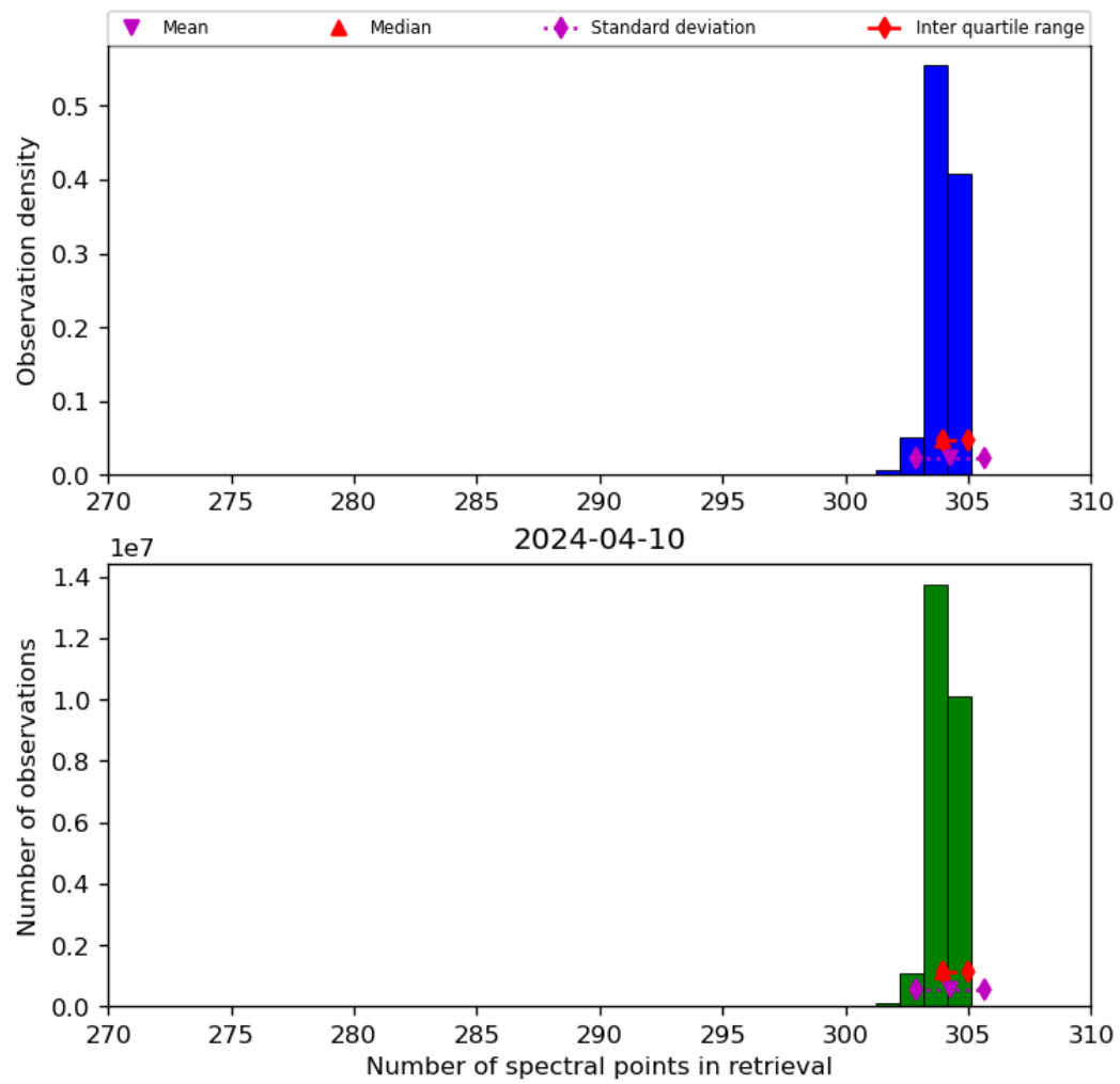
Figure 33: Histogram of “Number of spectral points in retrieval” for 2024-04-10 to 2024-04-11
