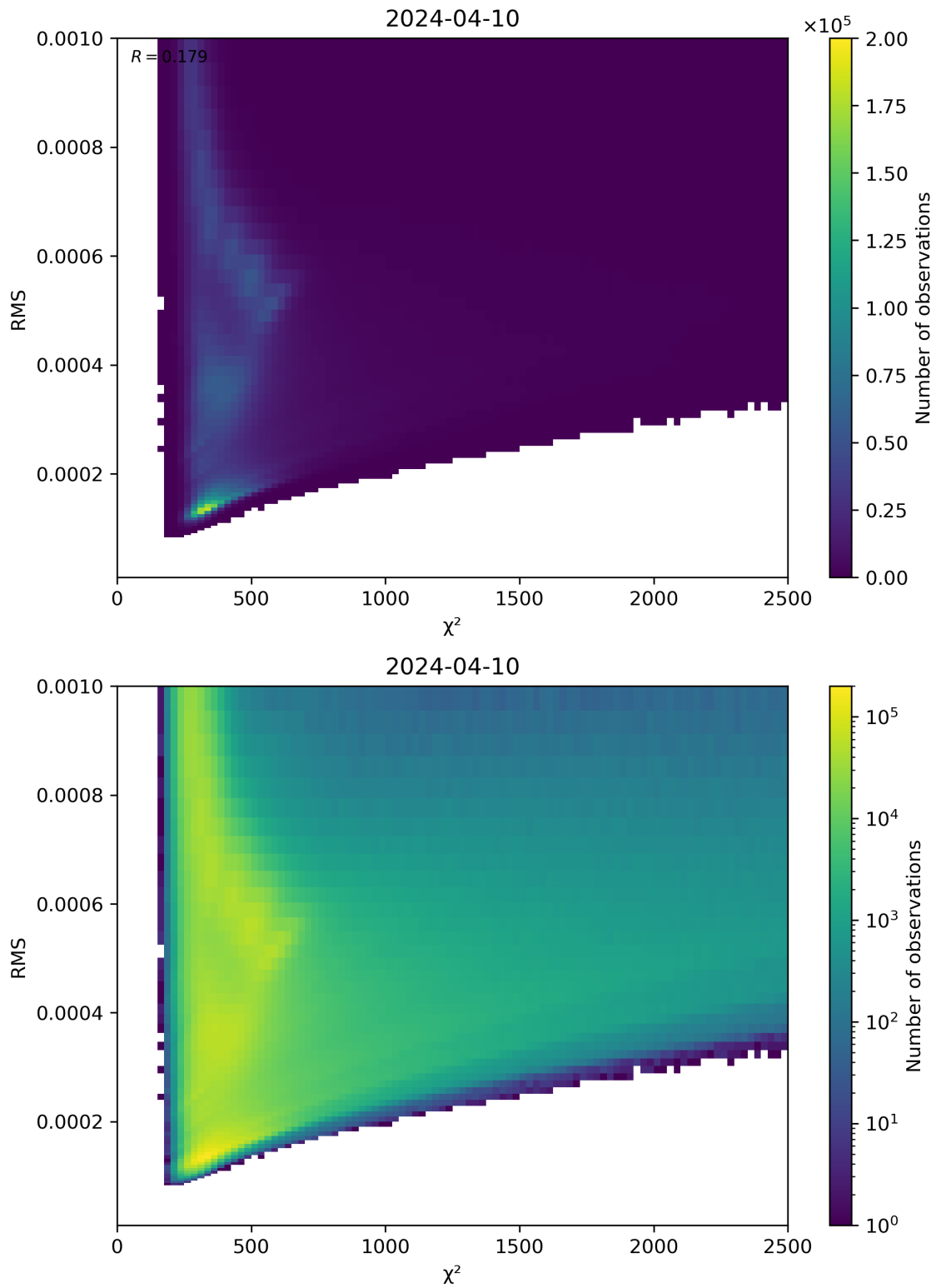
Figure 82: Scatter density plot of “ \chi^2 ” against “RMS” for 2024-04-10 to 2024-04-11.
