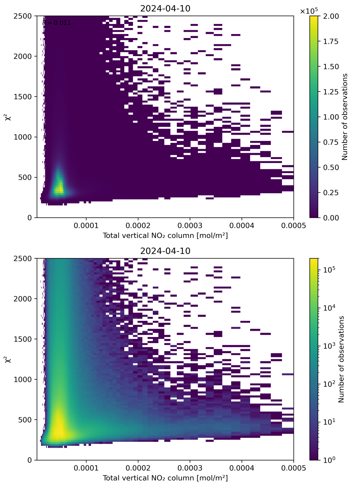
Figure 111: Scatter density plot of “Total vertical NO 2 column” against “ \chi^2 ” for 2024-04-10 to 2024-04-11.
