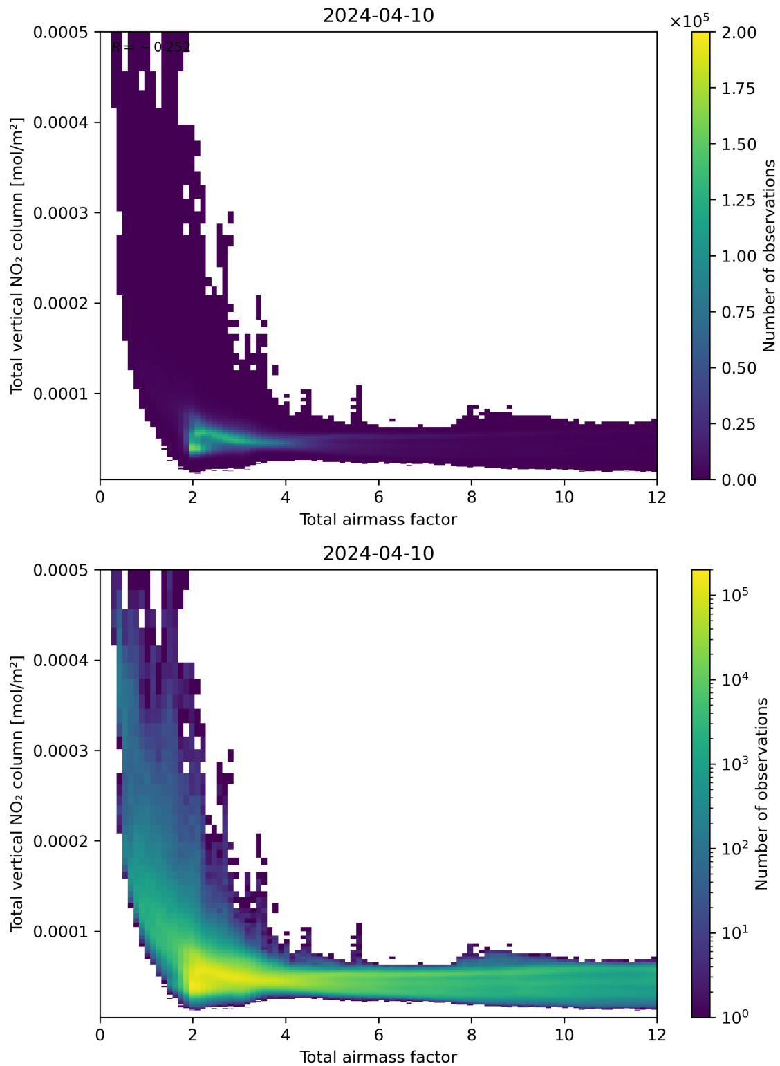
Figure 67: Scatter density plot of “Total airmass factor” against “Total vertical NO 2 column” for 2024-04-10 to 2024-04-11.
