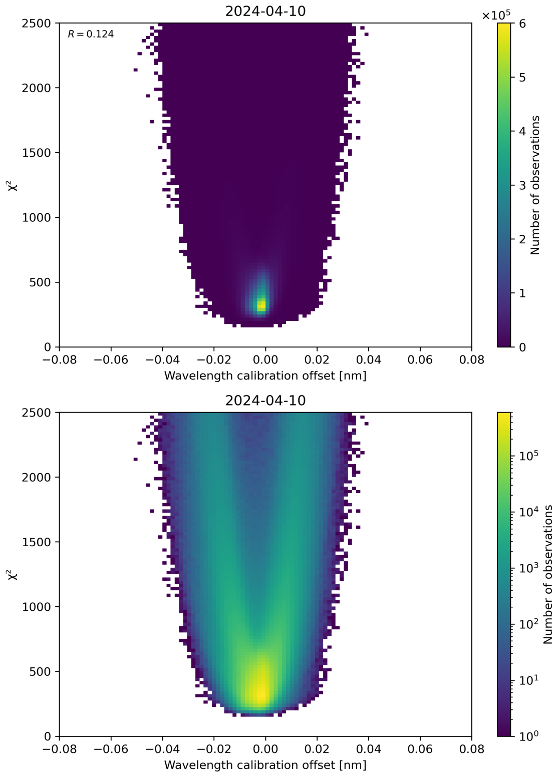
Figure 175: Scatter density plot of “Wavelength calibration offset” against “ \chi^2 ” for 2024-04-10 to 2024-04-11.
