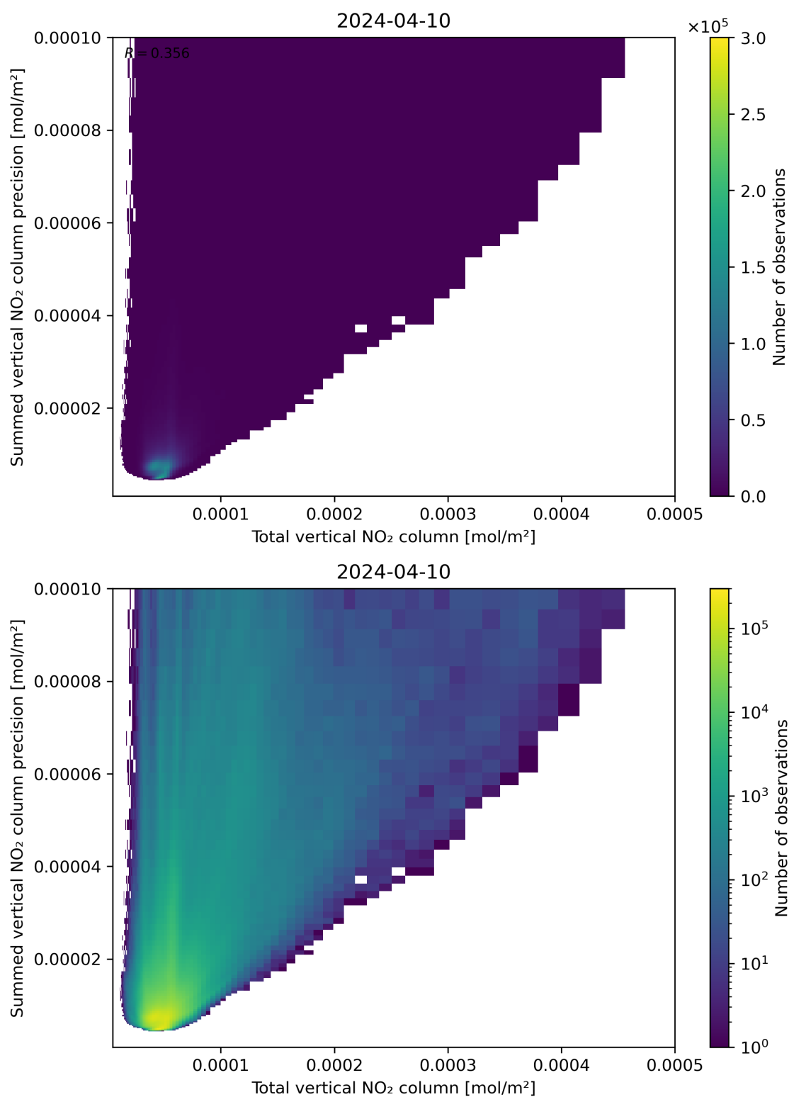
Figure 113: Scatter density plot of “Total vertical NO 2 column” against “Summed vertical NO 2 column precision” for 2024-04-10 to 2024-04-11.
