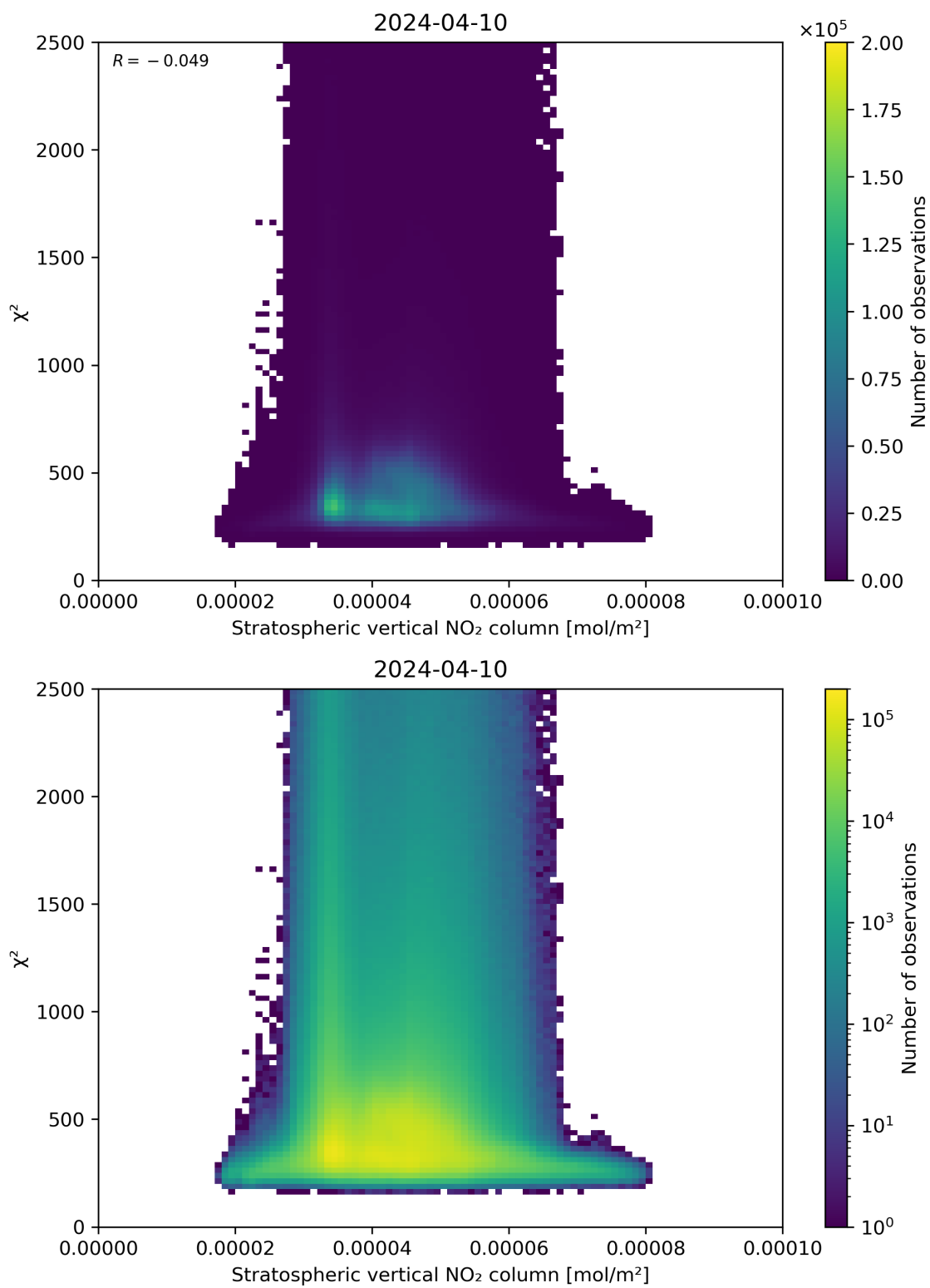
Figure 97: Scatter density plot of “Stratospheric vertical NO 2 column” against “ \chi^2 ” for 2024-04-10 to 2024-04-11.
