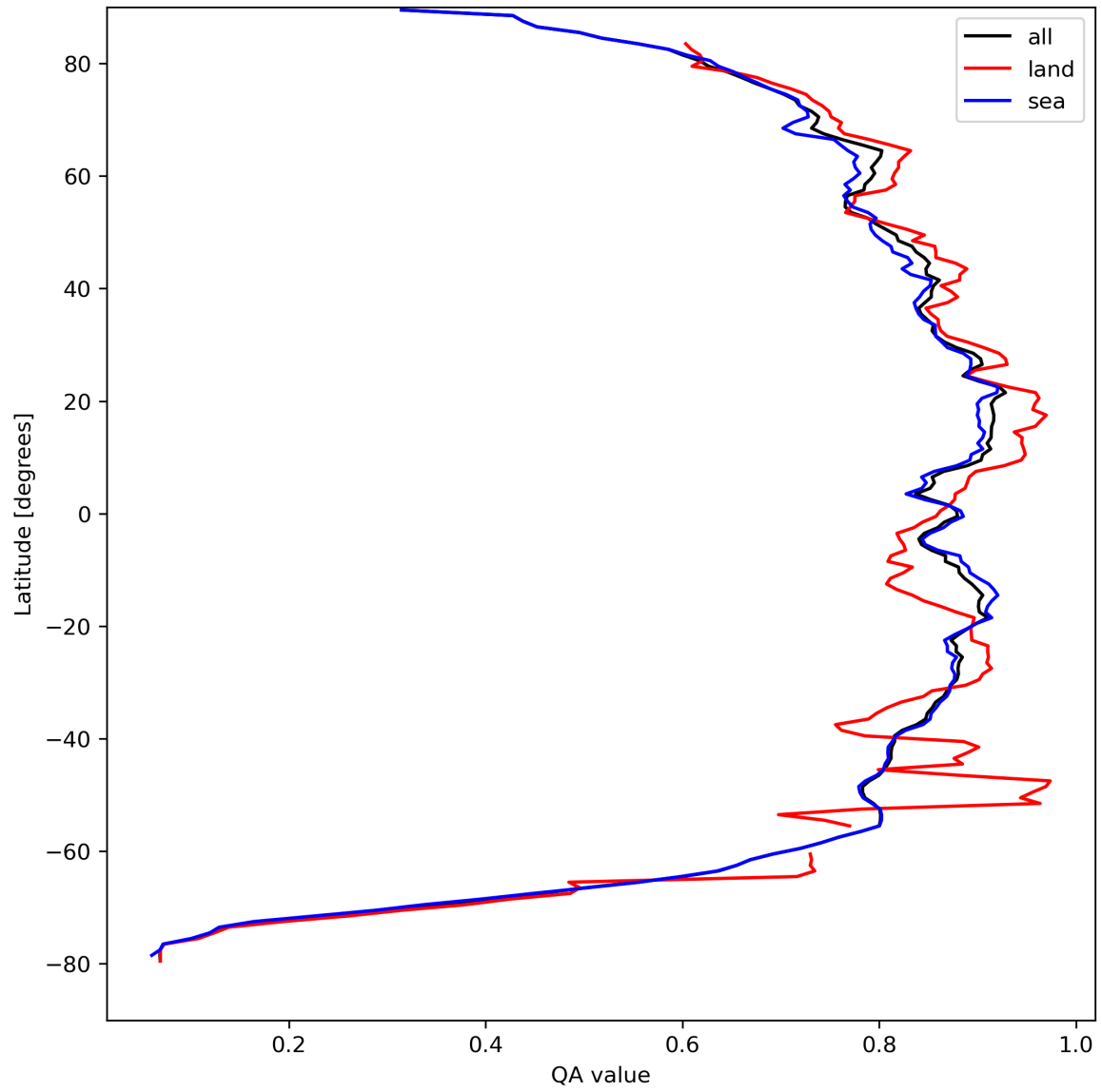
Figure 11: Zonal average of “QA value” for 2024-04-10 to 2024-04-11.
