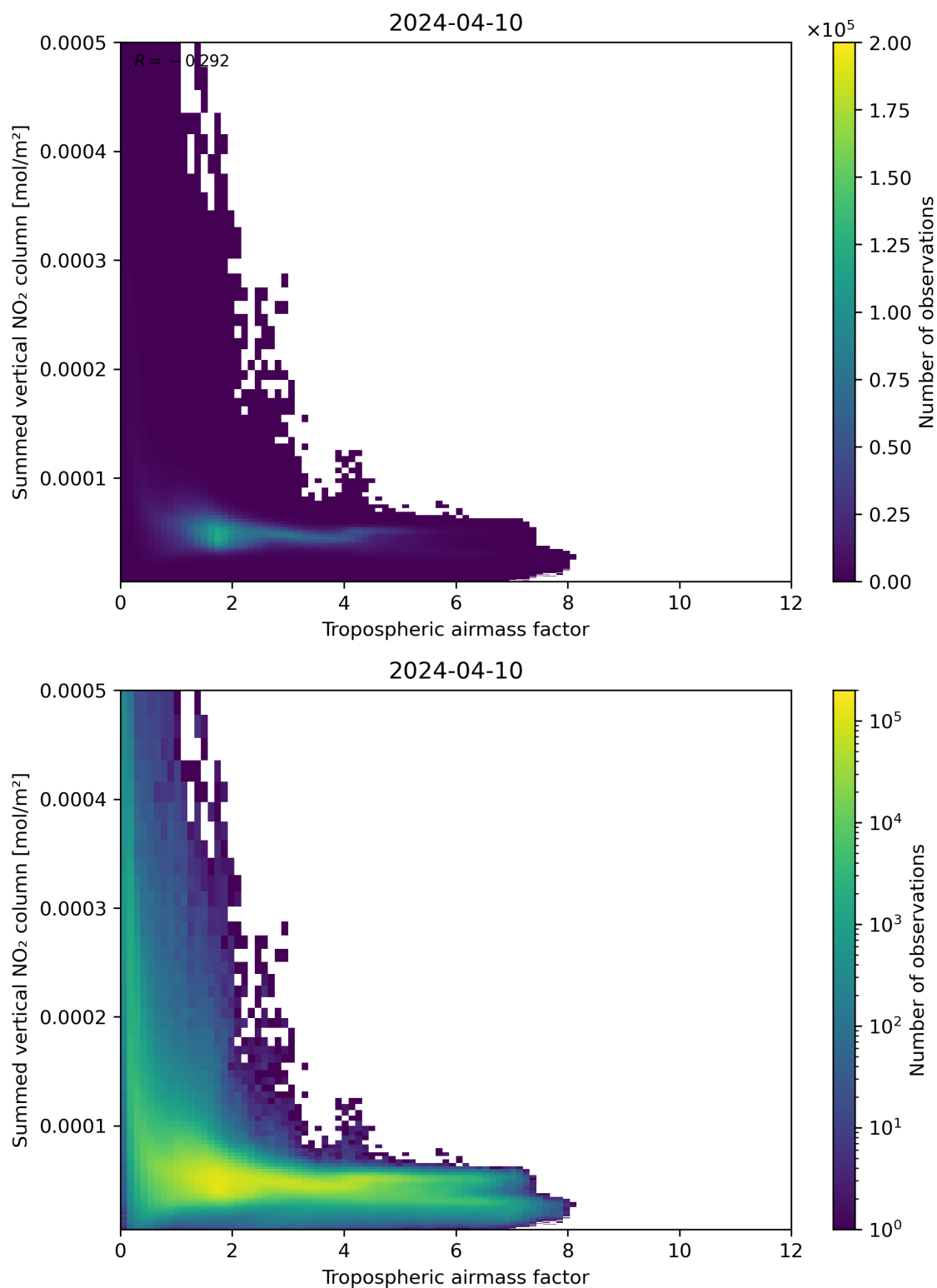
Figure 75: Scatter density plot of “Tropospheric airmass factor” against “Summed vertical NO 2 column” for 2024-04-10 to 2024-04-11.
