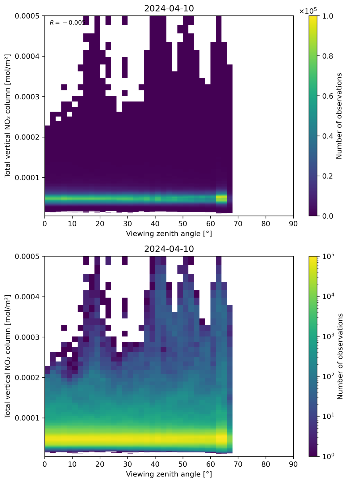
Figure 167: Scatter density plot of “Viewing zenith angle” against “Total vertical NO 2 column” for 2024-04-10 to 2024-04-11.
