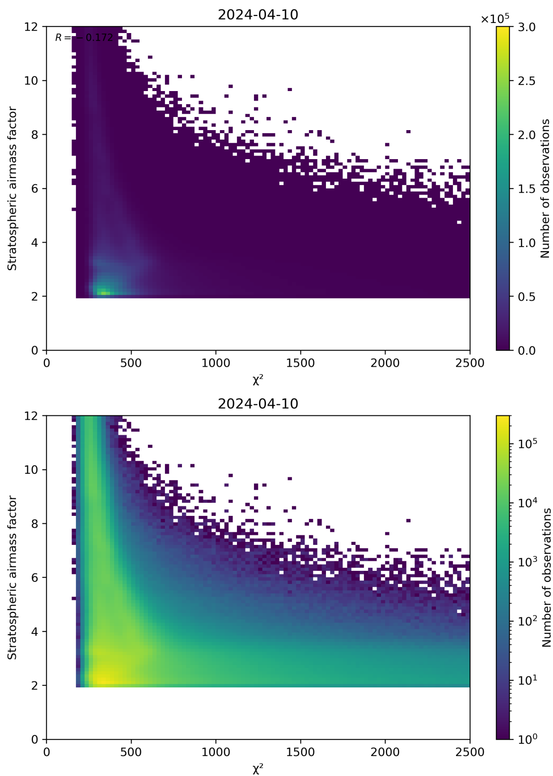
Figure 81: Scatter density plot of “ \chi^2 ” against “Stratospheric airmass factor” for 2024-04-10 to 2024-04-11.
