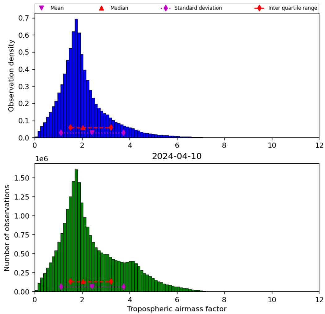
Figure 31: Histogram of “Tropospheric airmass factor” for 2024-04-10 to 2024-04-11
