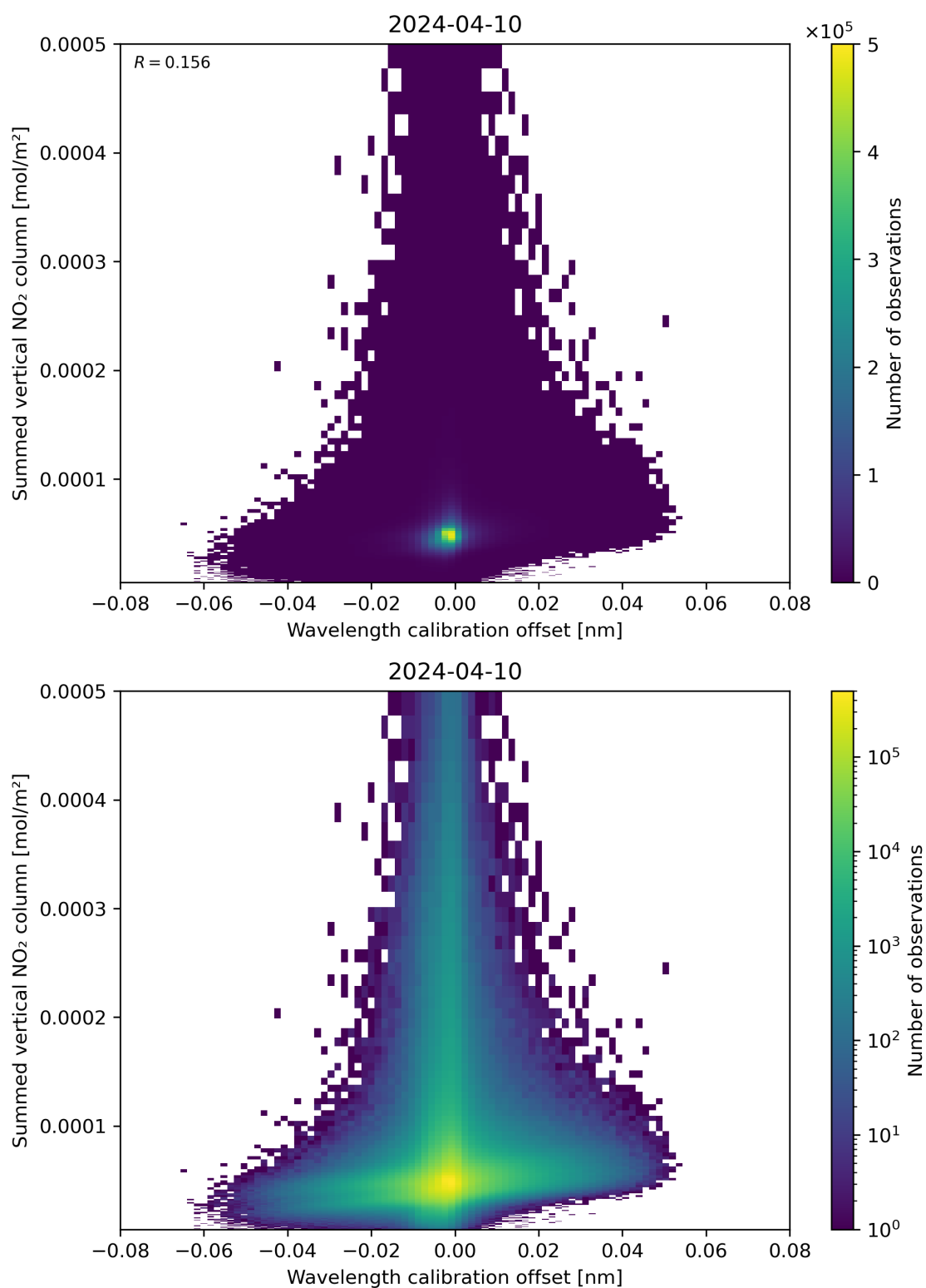
Figure 177: Scatter density plot of “Wavelength calibration offset” against “Summed vertical NO 2 column” for 2024-04-10 to 2024-04-11.
