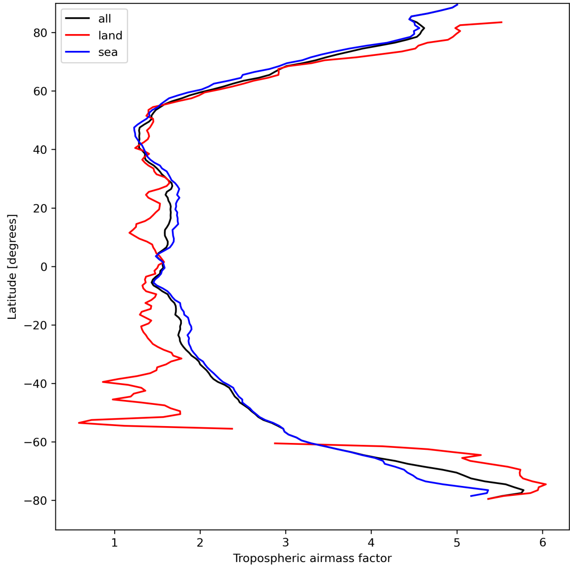
Figure 14: Zonal average of “Tropospheric airmass factor” for 2024-04-10 to 2024-04-11.
