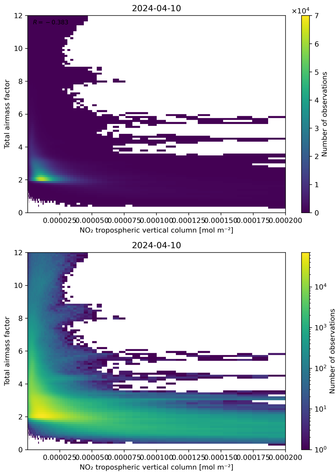
Figure 122: Scatter density plot of “NO 2 tropospheric vertical column” against “Total air mass factor” for 2024-04-10 to 2024-04-11.
