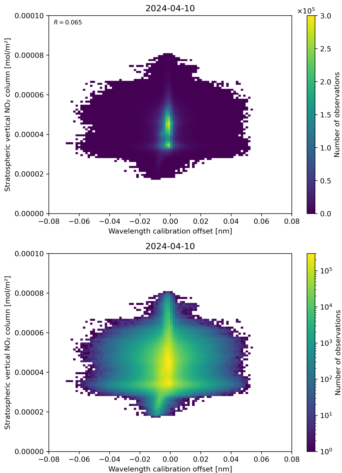
Figure 176: Scatter density plot of “Wavelength calibration offset” against “Stratospheric vertical NO 2 column” for 2024-04-10 to 2024-04-11.
