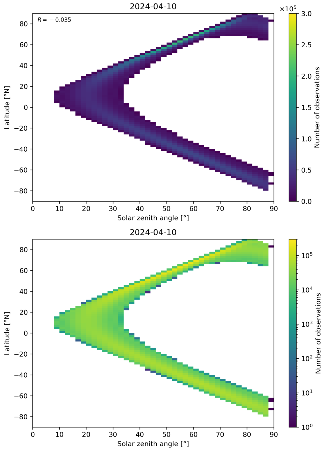
Figure 149: Scatter density plot of “Solar zenith angle” against “Latitude” for 2024-04-10 to 2024-04-11.
