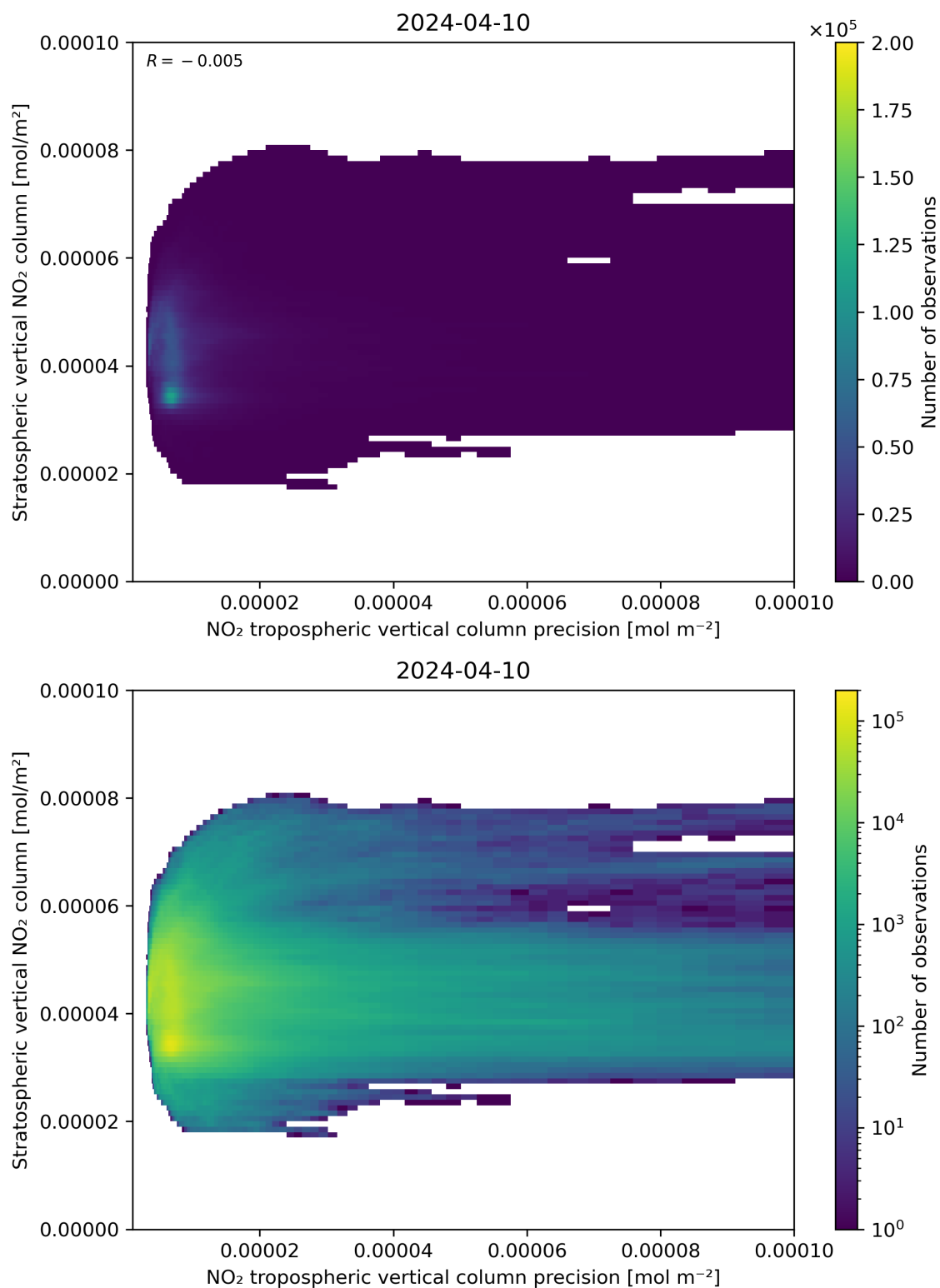
Figure 135: Scatter density plot of “NO 2 tropospheric vertical column precision” against “Stratospheric vertical NO 2 column” for 2024-04-10 to 2024-04-11.
