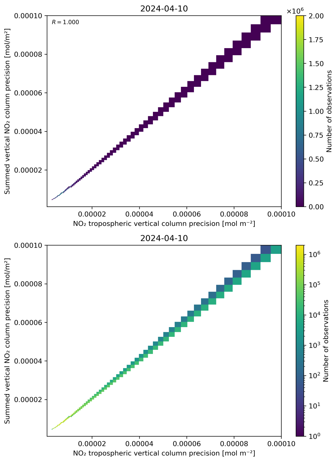
Figure 137: Scatter density plot of “NO 2 tropospheric vertical column precision” against “Summed vertical NO 2 column precision” for 2024-04-10 to 2024-04-11.
