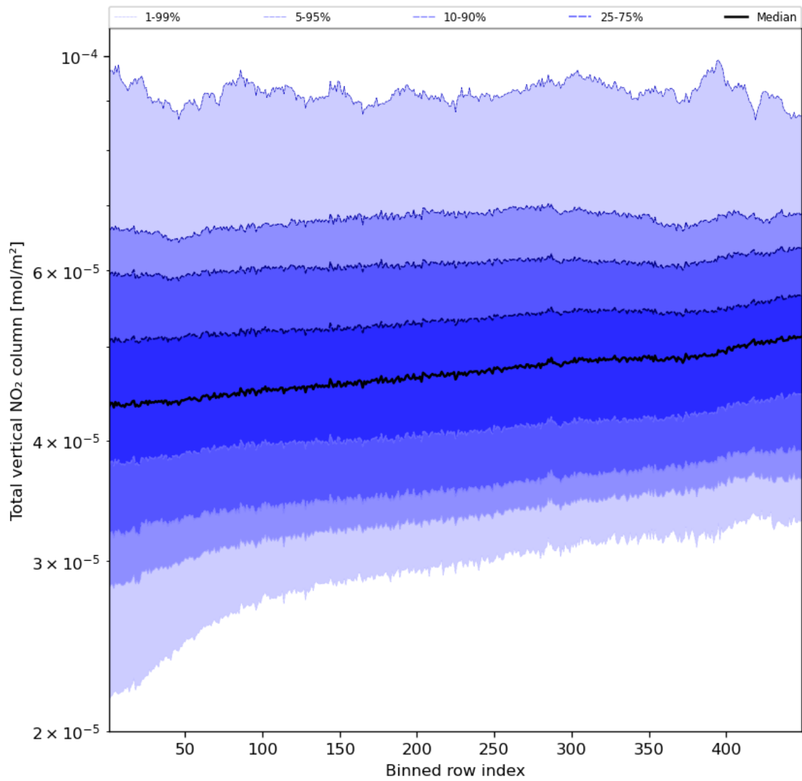
Figure 55: Along track statistics of “Total vertical NO 2 column” for 2024-04-10 to 2024-04-11
