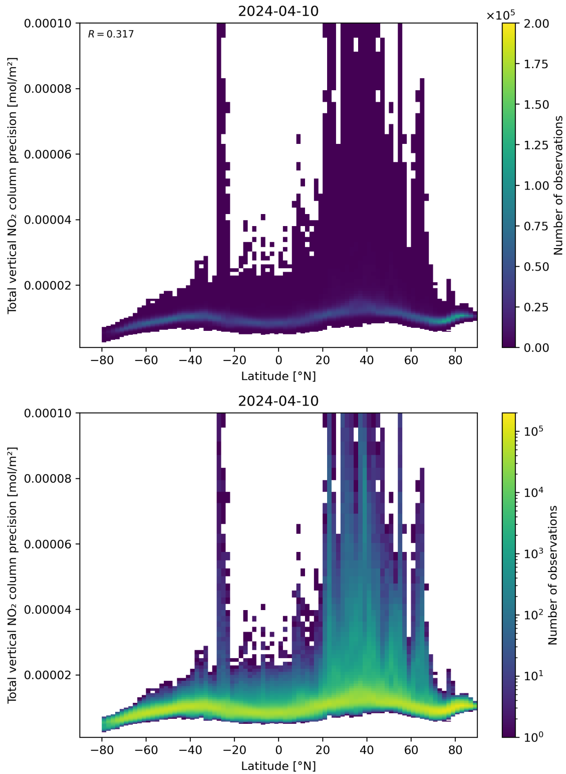
Figure 91: Scatter density plot of “Latitude” against “Total vertical NO 2 column precision” for 2024-04-10 to 2024-04-11.
