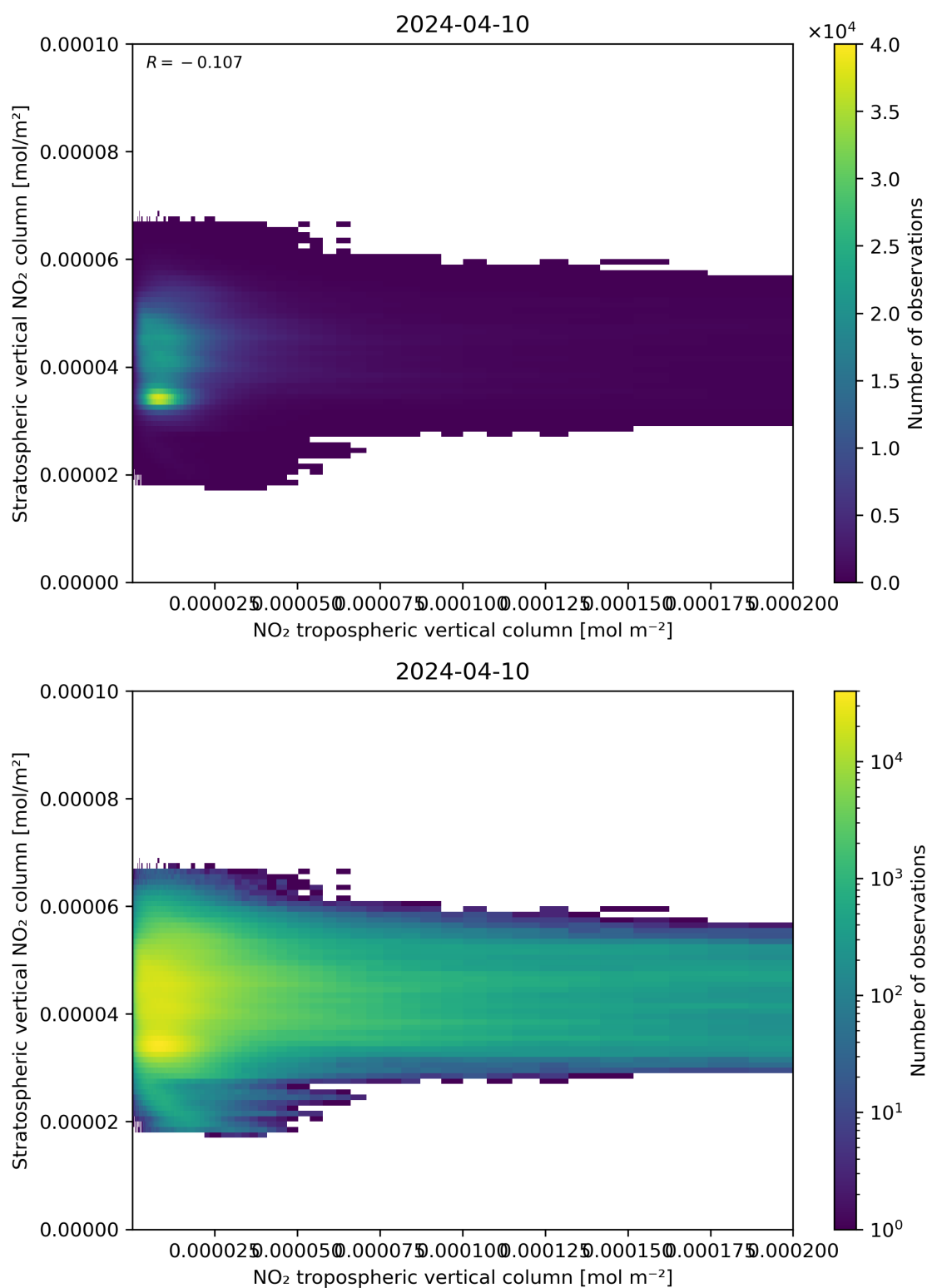
Figure 125: Scatter density plot of “NO 2 tropospheric vertical column” against “Stratospheric vertical NO 2 column” for 2024-04-10 to 2024-04-11.
