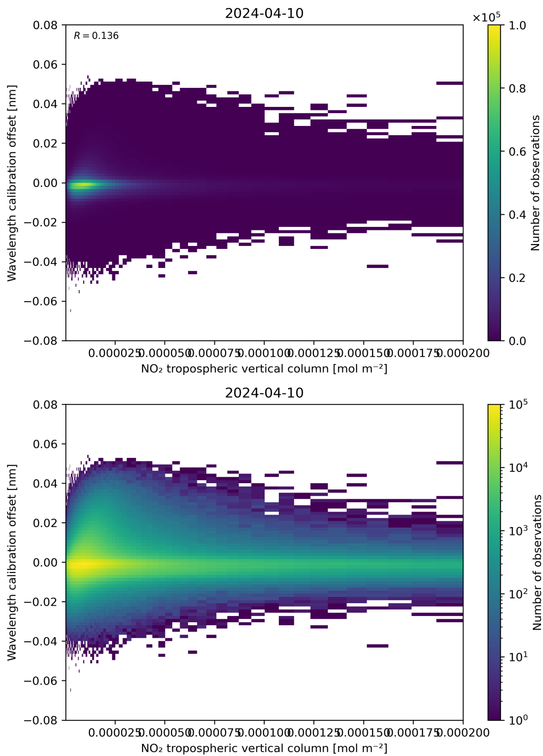
Figure 143: Scatter density plot of “NO 2 tropospheric vertical column” against “Wavelength calibration offset” for 2024-04-10 to 2024-04-11.
