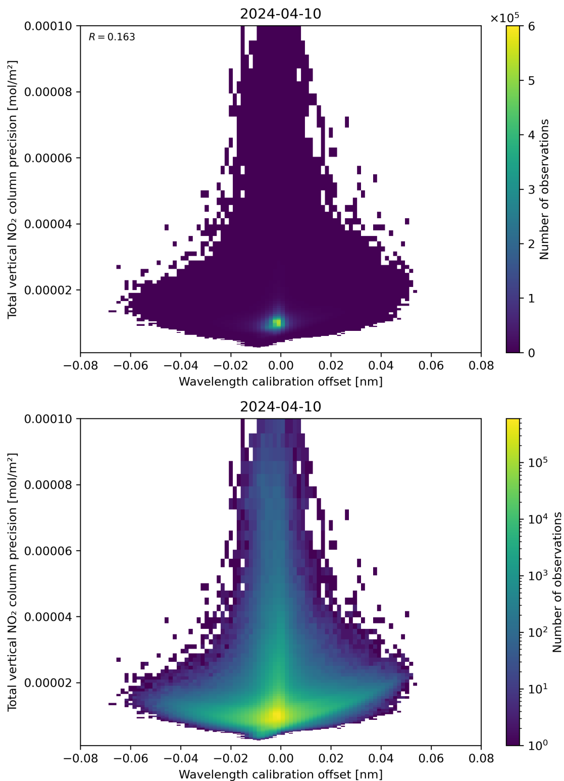
Figure 180: Scatter density plot of “Wavelength calibration offset” against “Total vertical NO 2 column precision” for 2024-04-10 to 2024-04-11.
