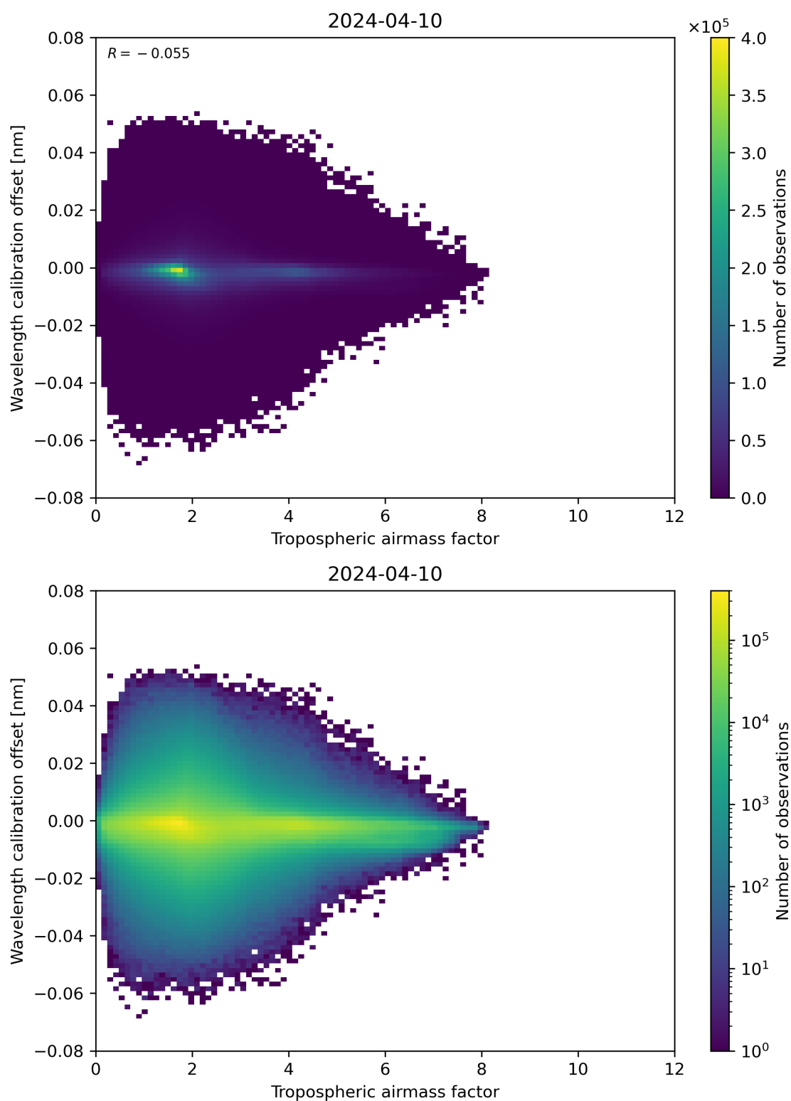
Figure 80: Scatter density plot of “Tropospheric airmass factor” against “Wavelength calibration offset” for 2024-04-10 to 2024-04-11.
