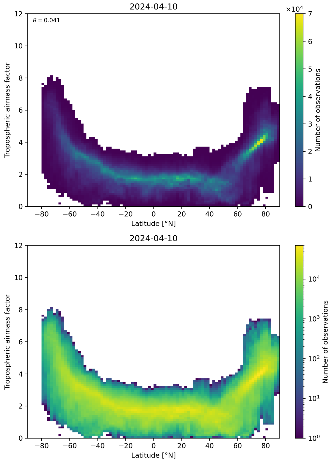
Figure 85: Scatter density plot of “Latitude” against “Tropospheric airmass factor” for 2024-04-10 to 2024-04-11.
