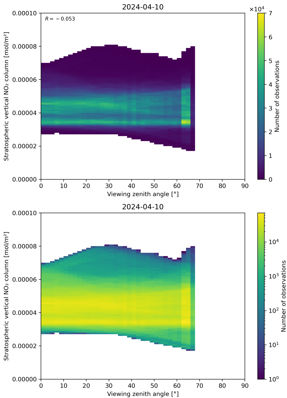
Figure 164: Scatter density plot of “Viewing zenith angle” against “Stratospheric vertical NO 2 column” for 2024-04-10 to 2024-04-11.
