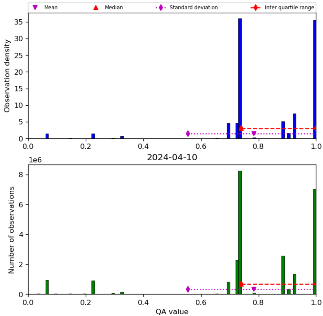
Figure 28: Histogram of “QA value” for 2024-04-10 to 2024-04-11
