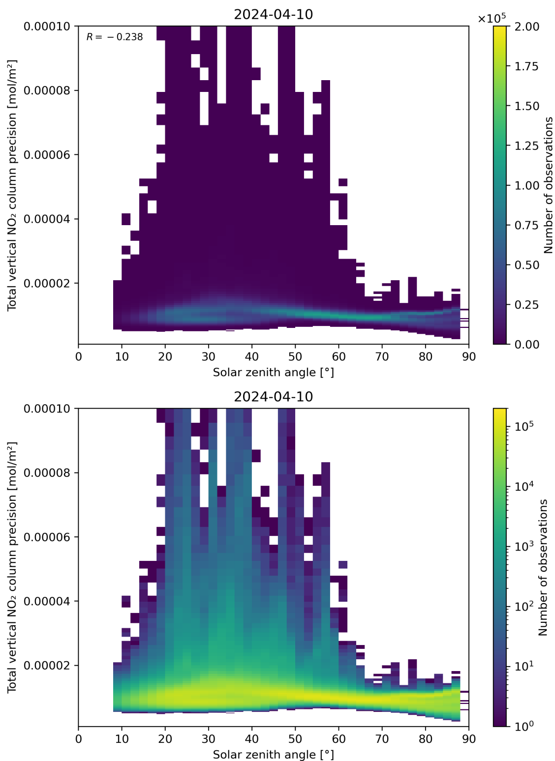
Figure 154: Scatter density plot of “Solar zenith angle” against “Total vertical NO 2 column precision” for 2024-04-10 to 2024-04-11.
