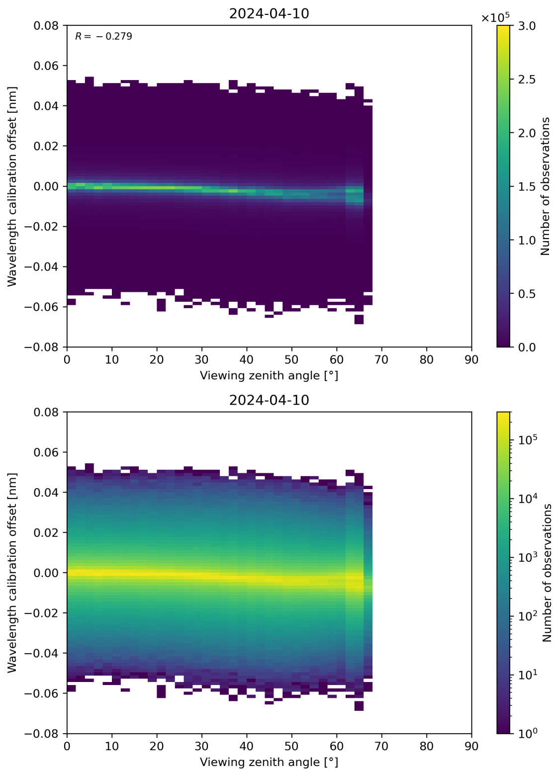
Figure 173: Scatter density plot of “Viewing zenith angle” against “Wavelength calibration offset” for 2024-04-10 to 2024-04-11.
