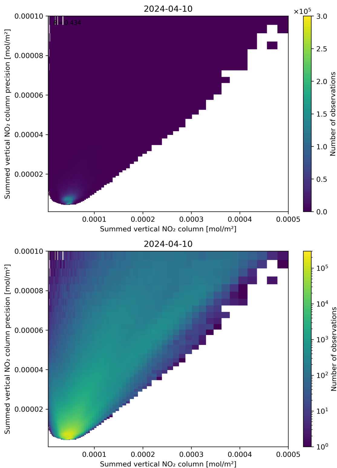
Figure 105: Scatter density plot of “Summed vertical NO 2 column” against “Summed vertical NO 2 column precision” for 2024-04-10 to 2024-04-11.
