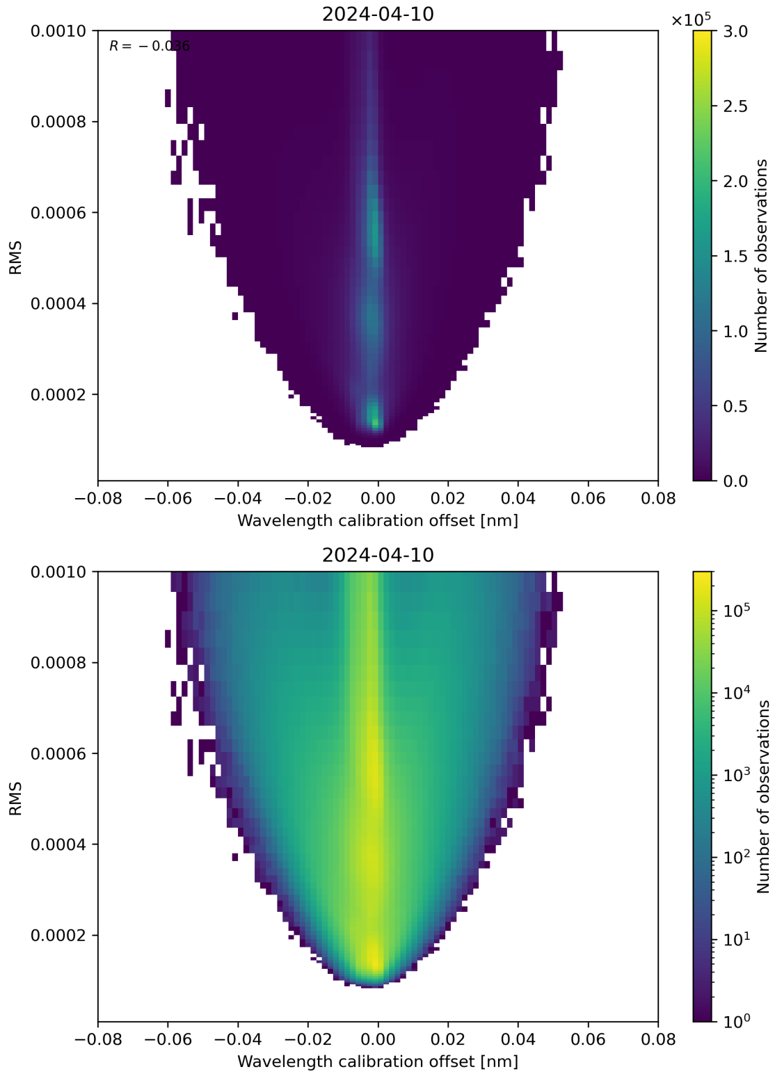
Figure 181: Scatter density plot of “Wavelength calibration offset” against “RMS” for 2024-04-10 to 2024-04-11.
