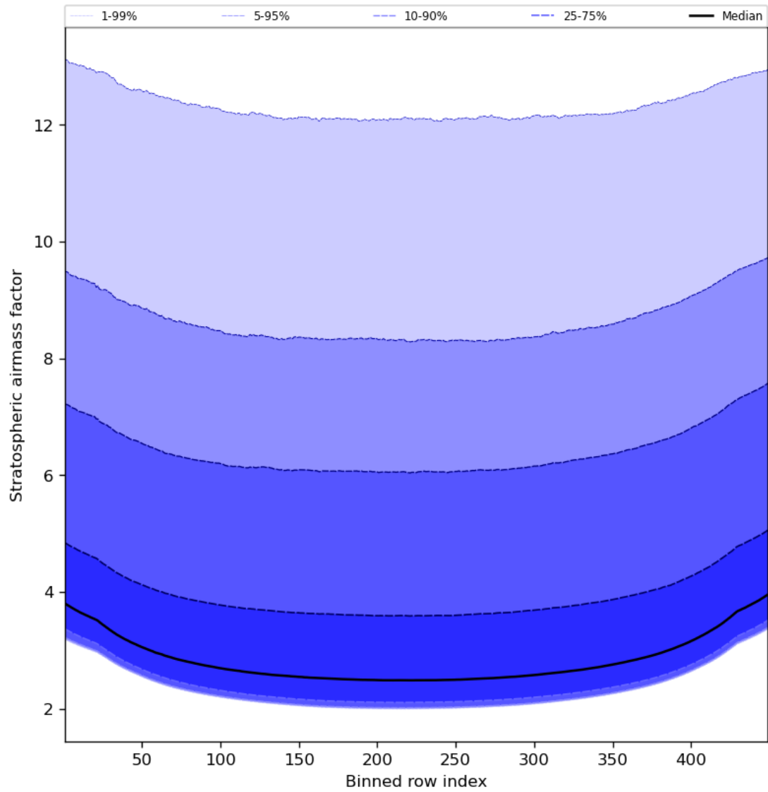
Figure 61: Along track statistics of “Stratospheric airmass factor” for 2024-04-10 to 2024-04-11
