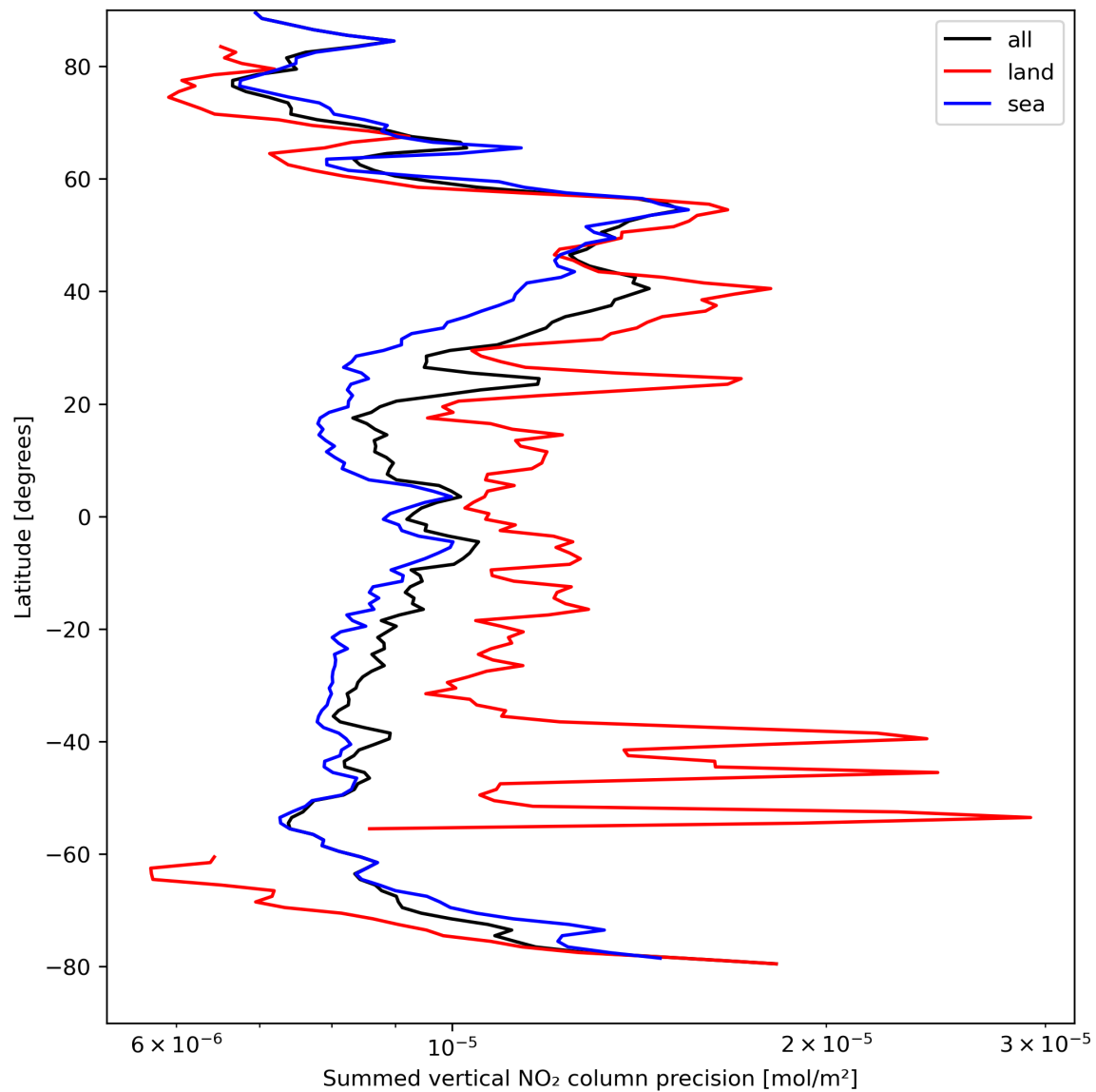
Figure 24: Zonal average of “Summed vertical NO 2 column precision” for 2024-04-10 to 2024-04-11.
