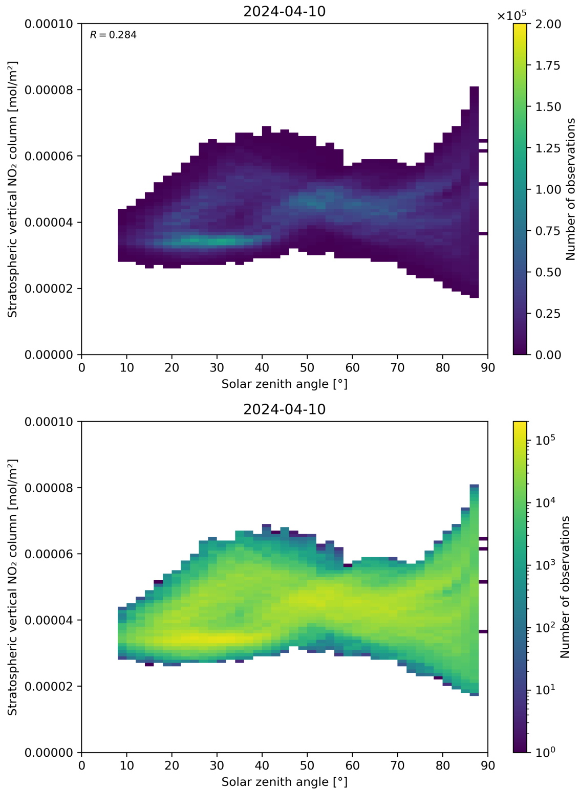
Figure 150: Scatter density plot of “Solar zenith angle” against “Stratospheric vertical NO 2 column” for 2024-04-10 to 2024-04-11.
