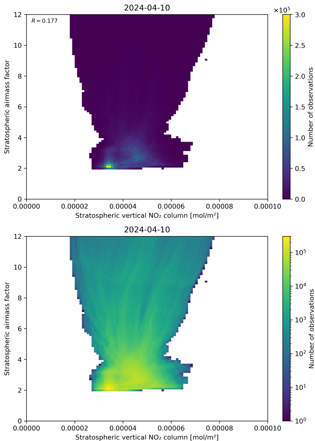
Figure 96: Scatter density plot of “Stratospheric vertical NO 2 column” against “Stratospheric airmass factor” for 2024-04-10 to 2024-04-11.
