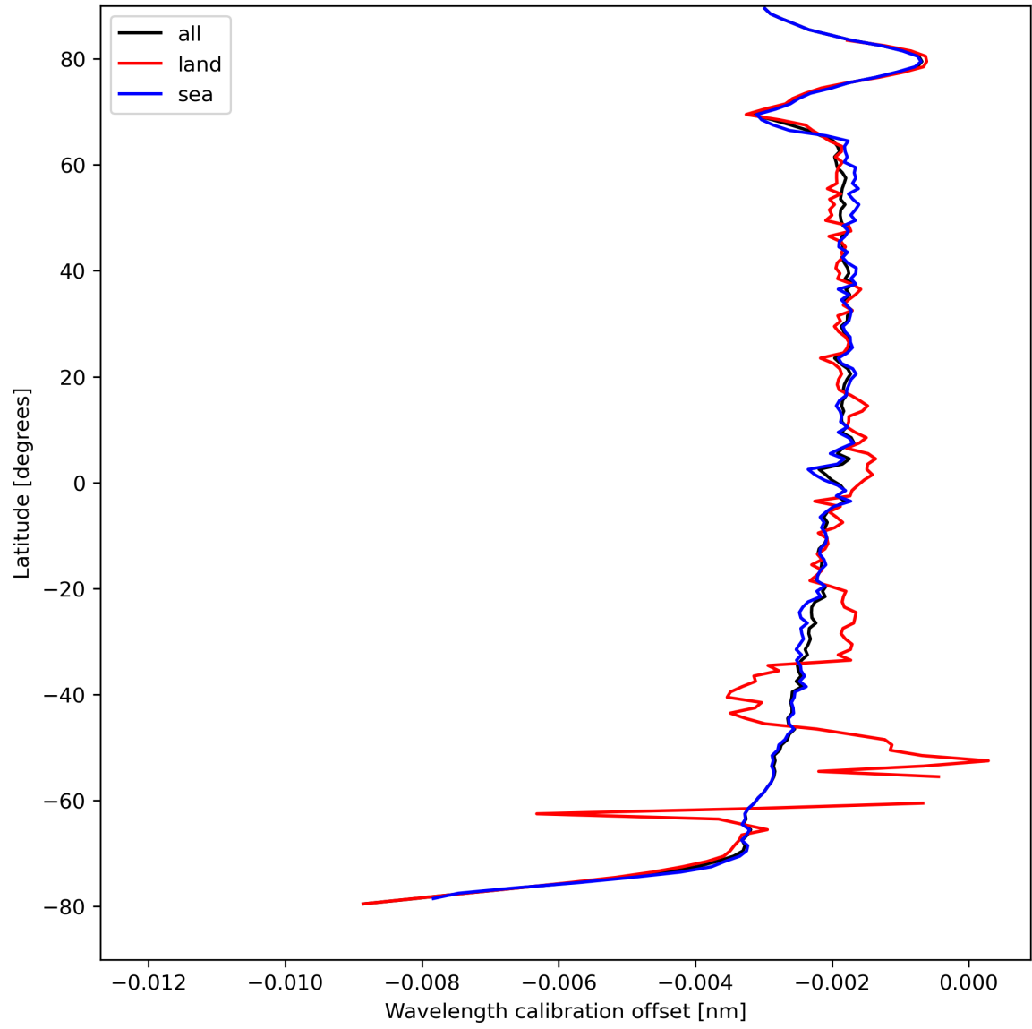
Figure 18: Zonal average of “Wavelength calibration offset” for 2024-04-10 to 2024-04-11.
