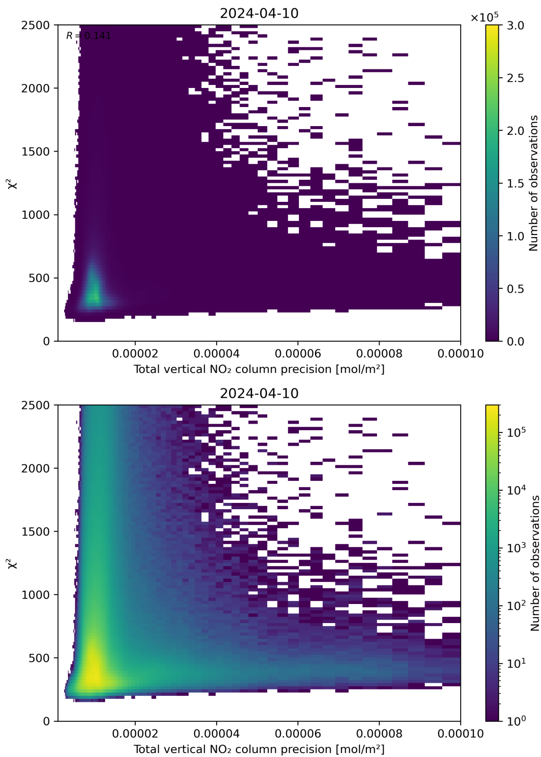
Figure 116: Scatter density plot of “Total vertical NO 2 column precision” against “ \chi^2 ” for 2024-04-10 to 2024-04-11.
