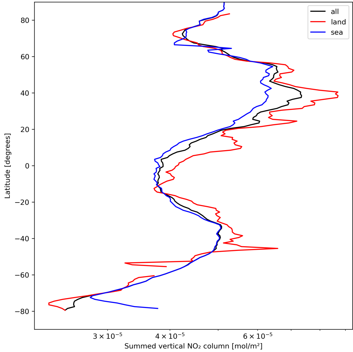
Figure 23: Zonal average of “Summed vertical NO 2 column” for 2024-04-10 to 2024-04-11.
