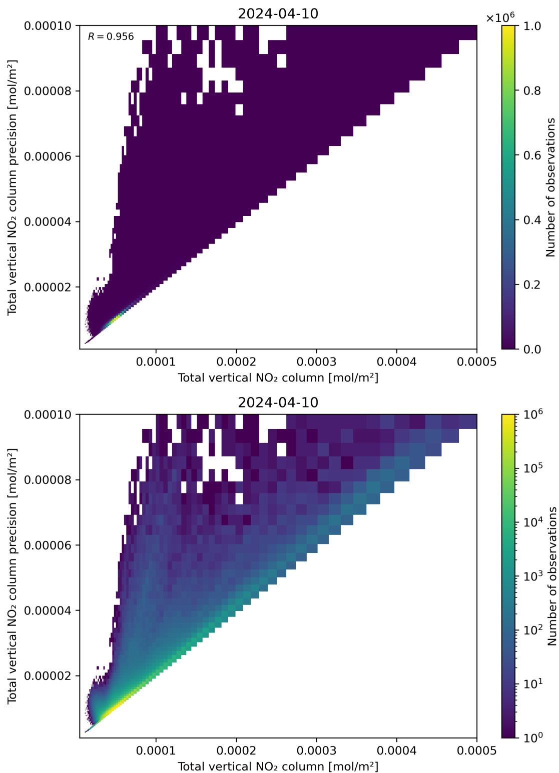
Figure 114: Scatter density plot of “Total vertical NO 2 column” against “Total vertical NO 2 column precision” for 2024-04-10 to 2024-04-11.
