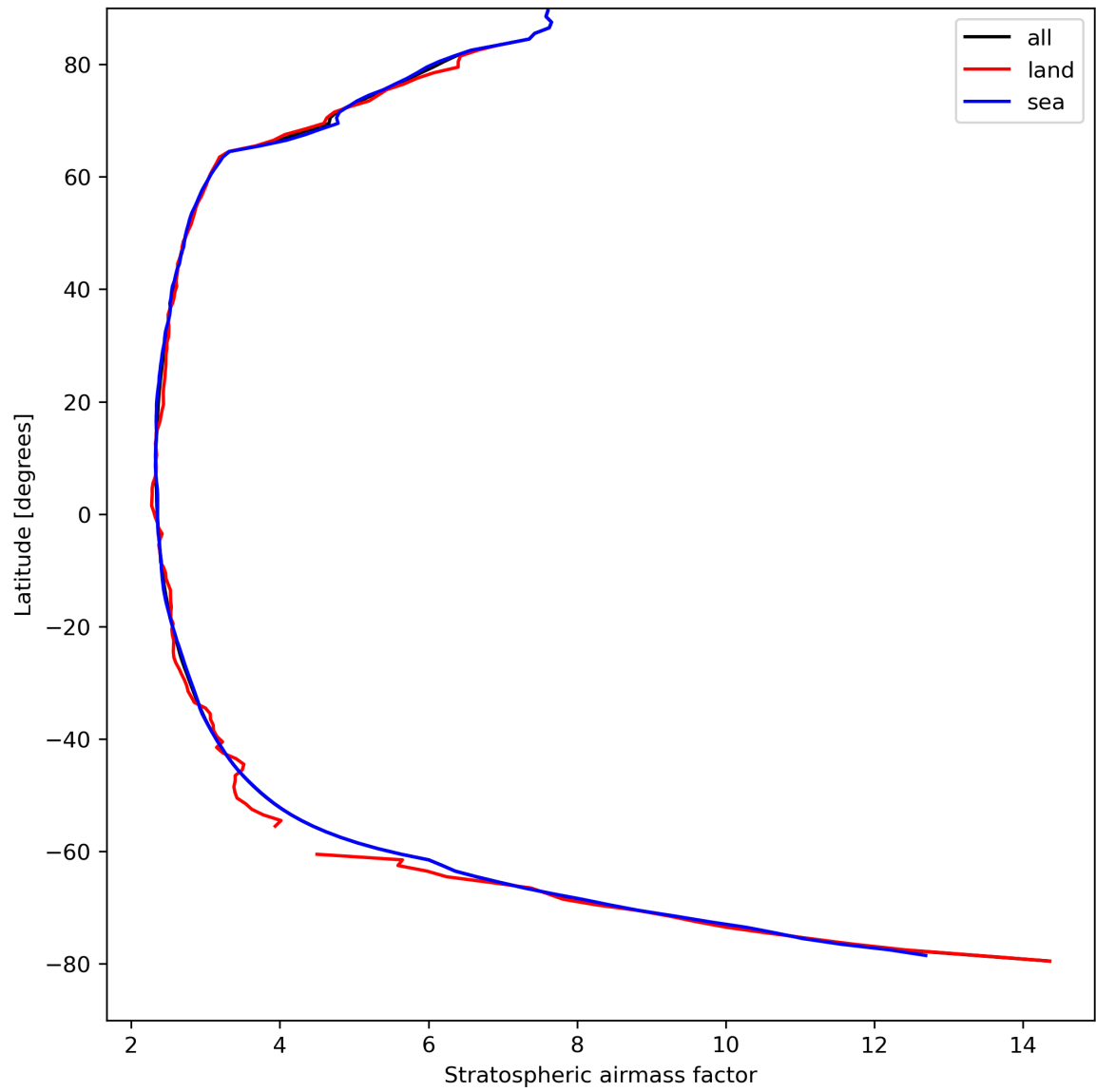
Figure 27: Zonal average of “Stratospheric air mass factor” for 2024-04-10 to 2024-04-11.
