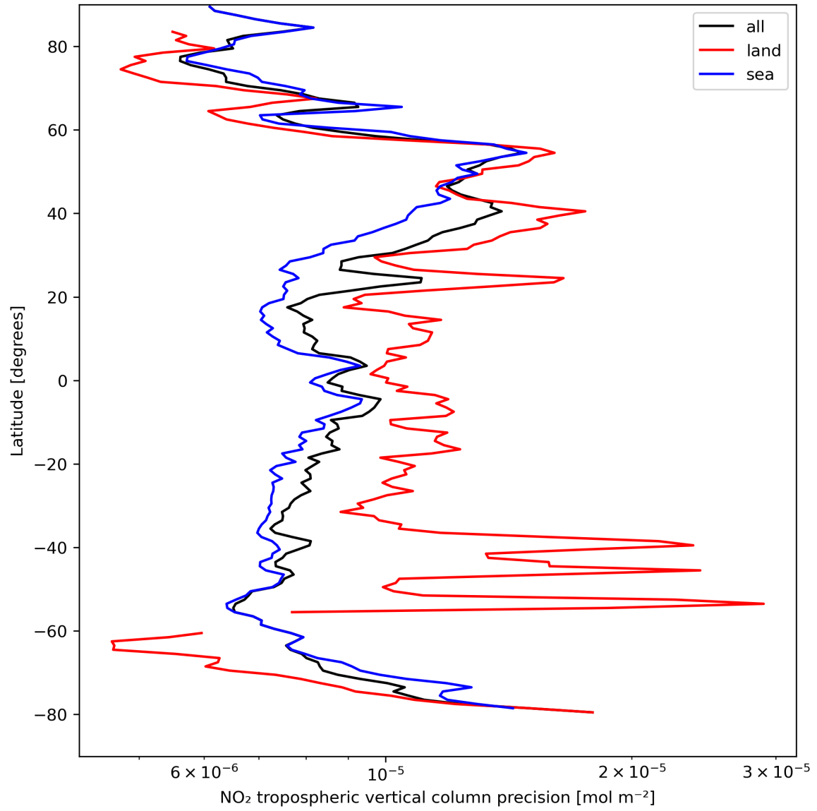
Figure 13: Zonal average of “NO 2 tropospheric vertical column precision” for 2024-04-10 to 2024-04-11.
