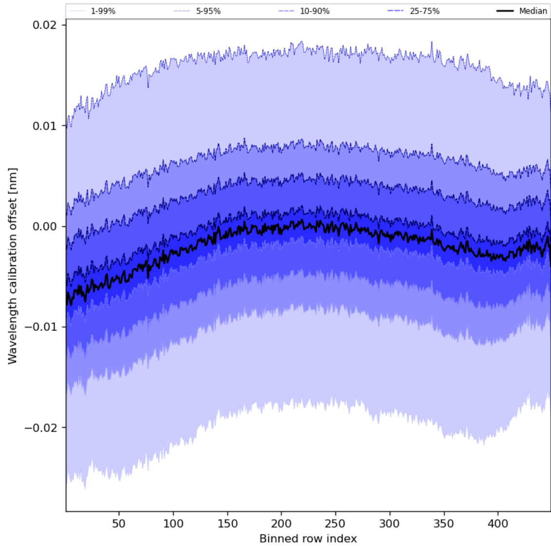
Figure 52: Along track statistics of “Wavelength calibration offset” for 2024-04-10 to 2024-04-11
