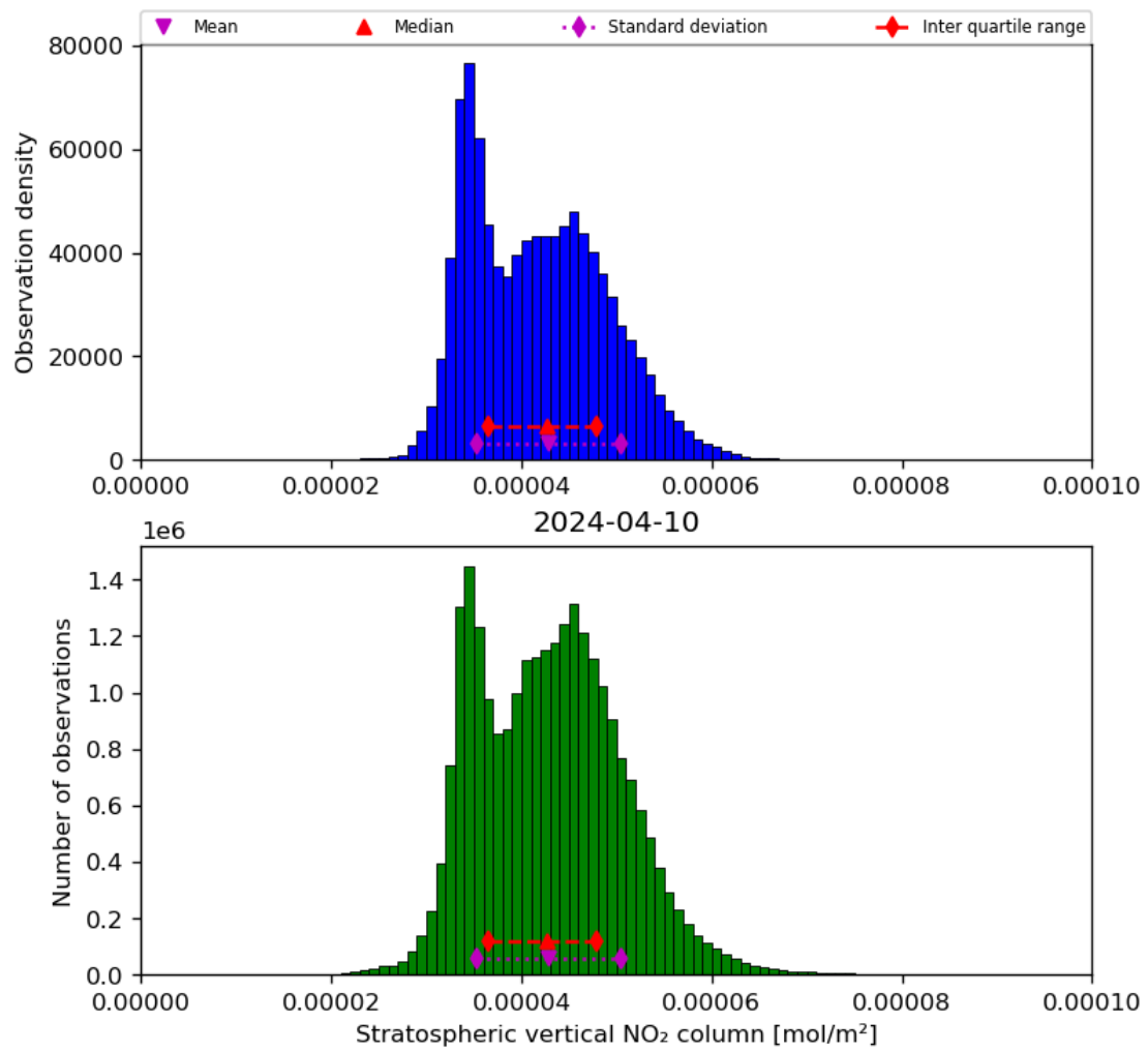
Figure 36: Histogram of “Stratospheric vertical NO 2 column” for 2024-04-10 to 2024-04-11
