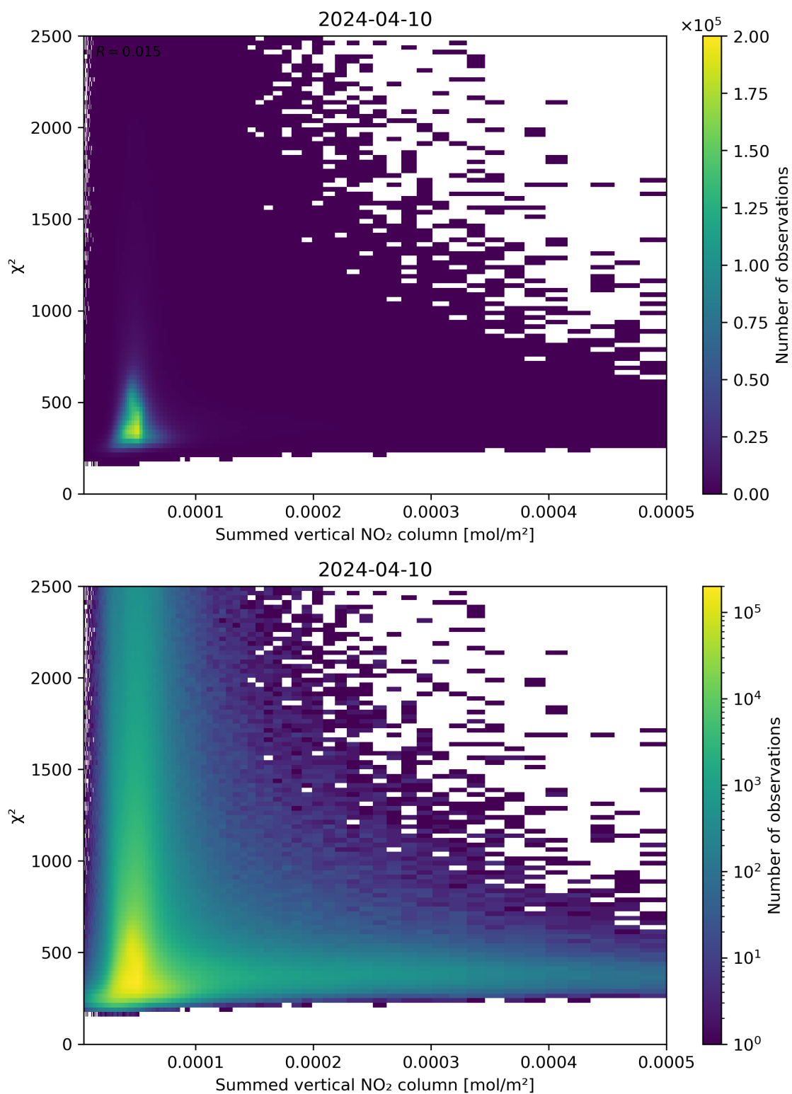
Figure 104: Scatter density plot of “Summed vertical NO 2 column” against “ \chi^2 ” for 2024-04-10 to 2024-04-11.
