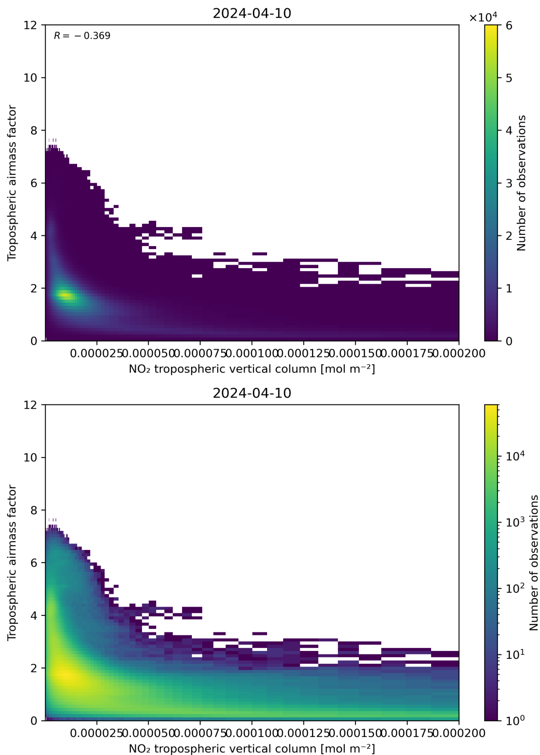
Figure 123: Scatter density plot of “NO 2 tropospheric vertical column” against “Tropospheric airmass factor” for 2024-04-10 to 2024-04-11.
