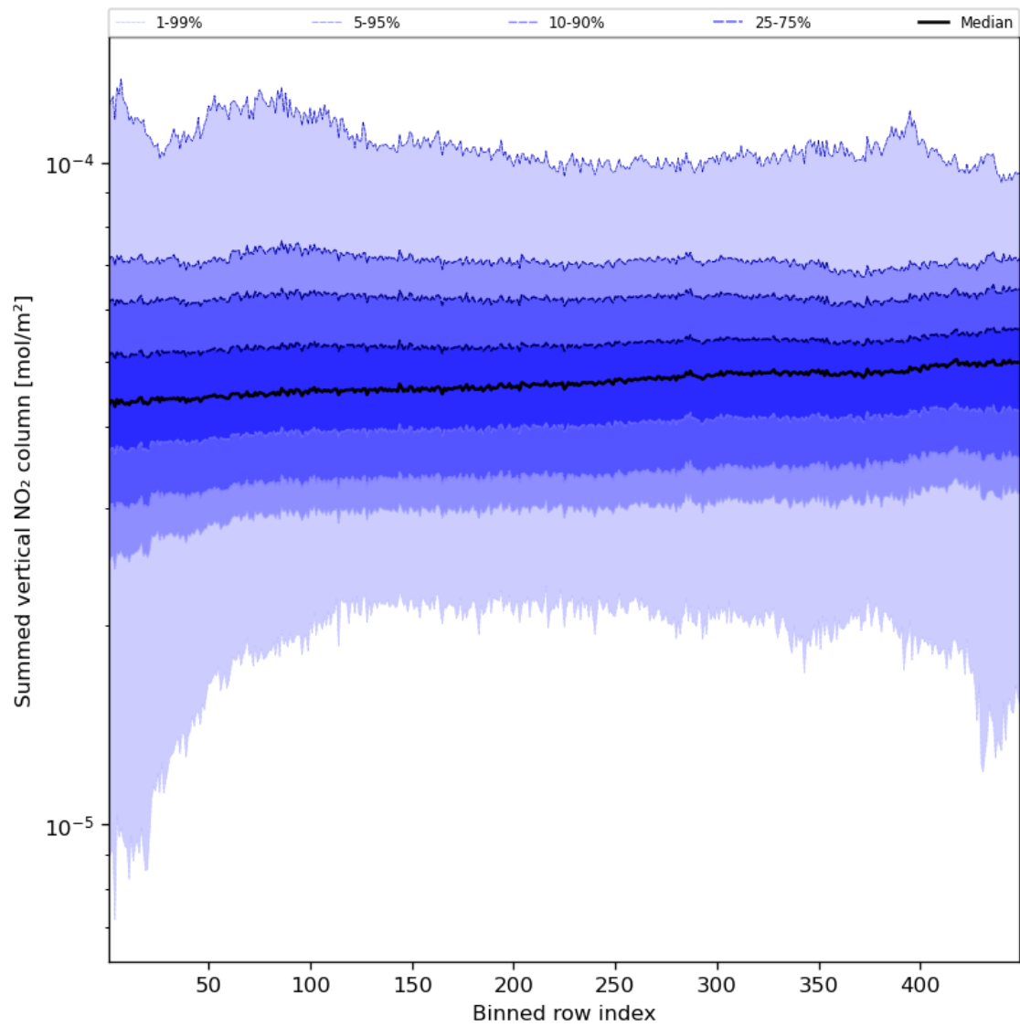
Figure 57: Along track statistics of “Summed vertical NO 2 column” for 2024-04-10 to 2024-04-11
