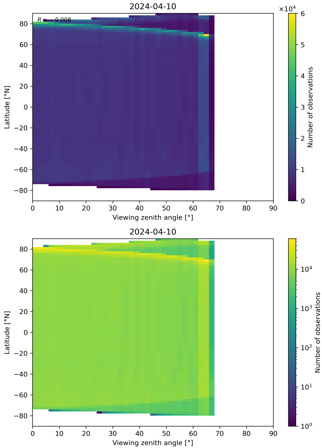
Figure 163: Scatter density plot of “Viewing zenith angle” against “Latitude” for 2024-04-10 to 2024-04-11.
