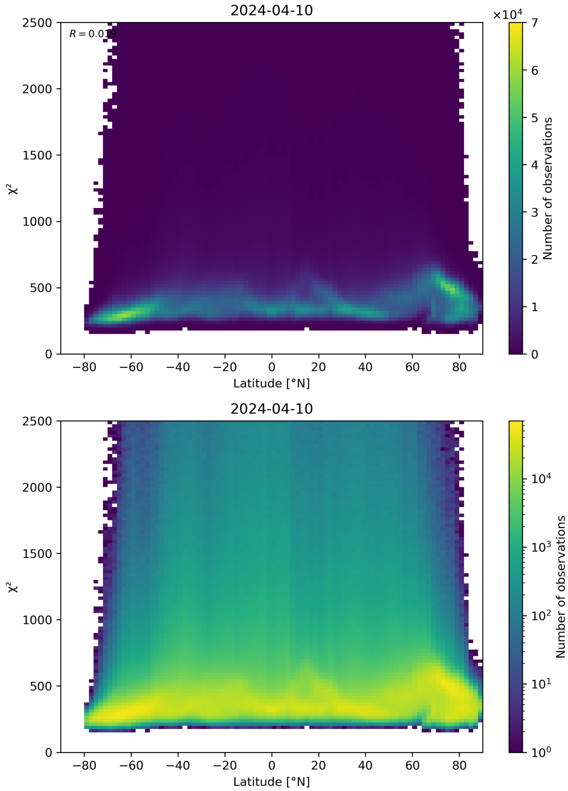
Figure 86: Scatter density plot of “Latitude” against “ \chi^2 ” for 2024-04-10 to 2024-04-11.
