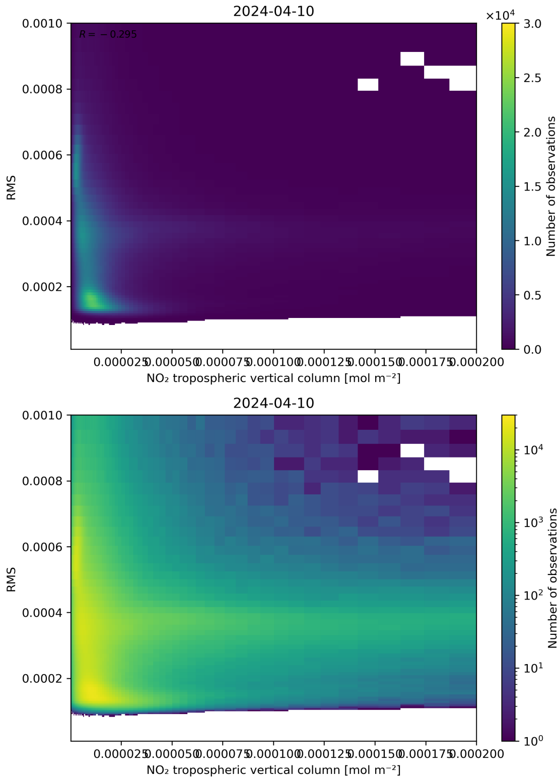
Figure 142: Scatter density plot of “NO 2 tropospheric vertical column” against “RMS” for 2024-04-10 to 2024-04-11.
