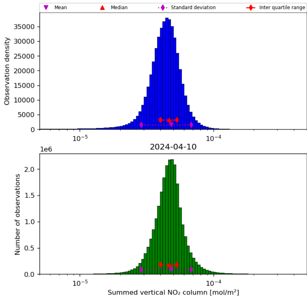
Figure 40: Histogram of “Summed vertical NO 2 column” for 2024-04-10 to 2024-04-11
