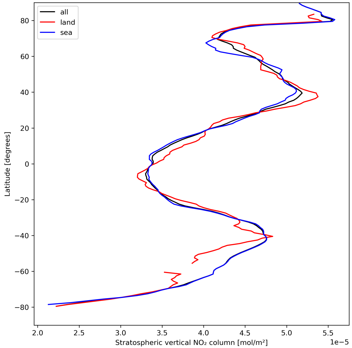
Figure 19: Zonal average of “Stratospheric vertical NO 2 column” for 2024-04-10 to 2024-04-11.
