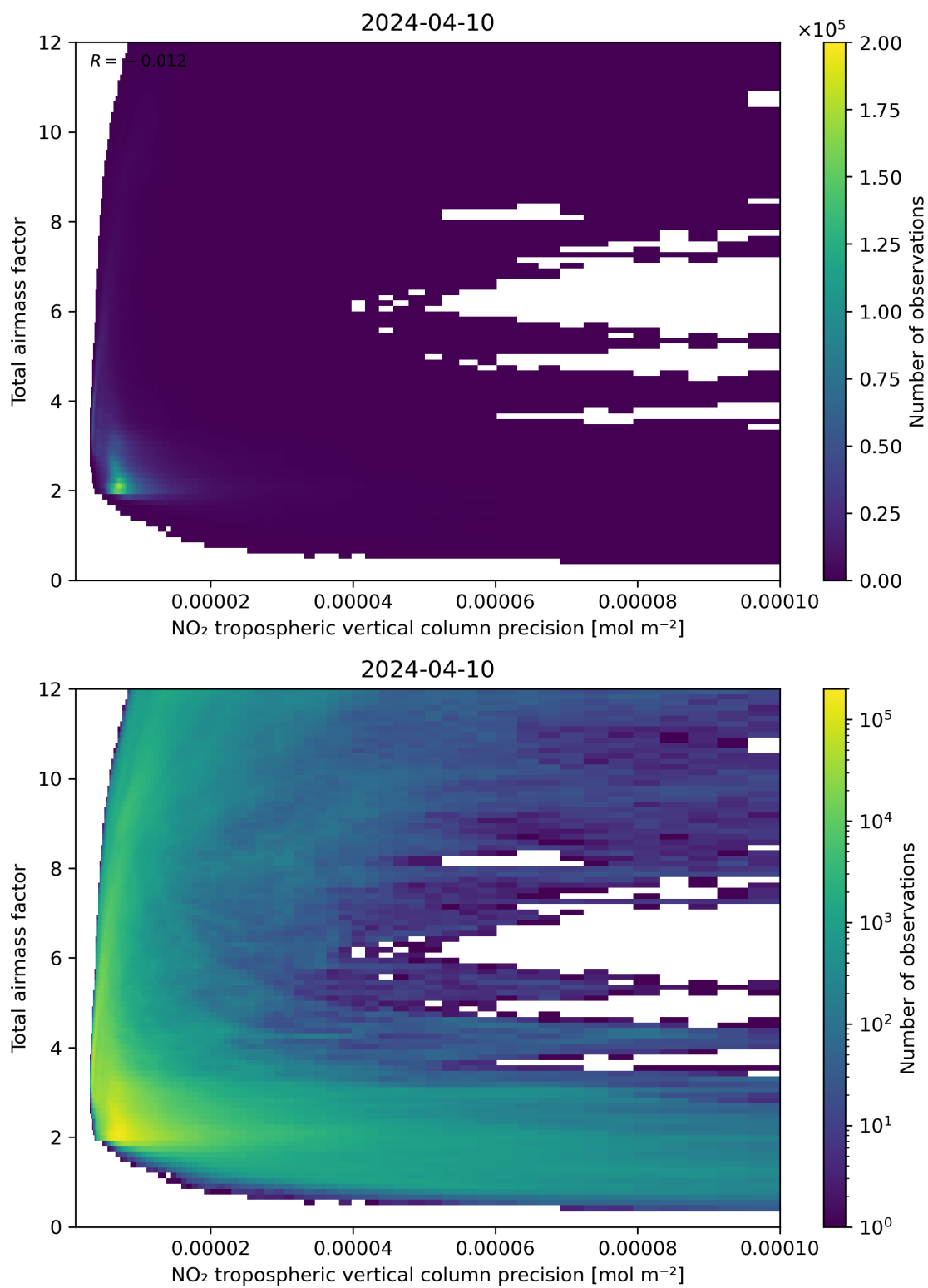
Figure 132: Scatter density plot of “NO 2 tropospheric vertical column precision” against “Total air mass factor” for 2024-04-10 to 2024-04-11.
