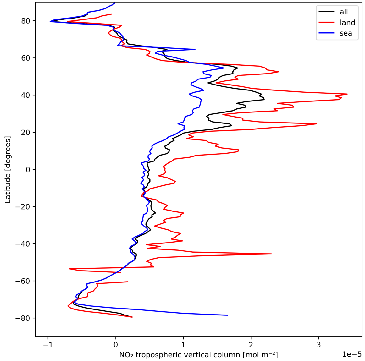
Figure 12: Zonal average of “NO 2 tropospheric vertical column” for 2024-04-10 to 2024-04-11.
