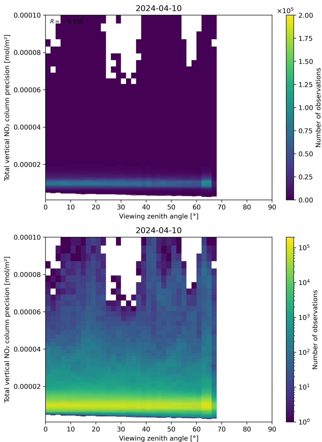
Figure 168: Scatter density plot of “Viewing zenith angle” against “Total vertical NO 2 column precision” for 2024-04-10 to 2024-04-11.
