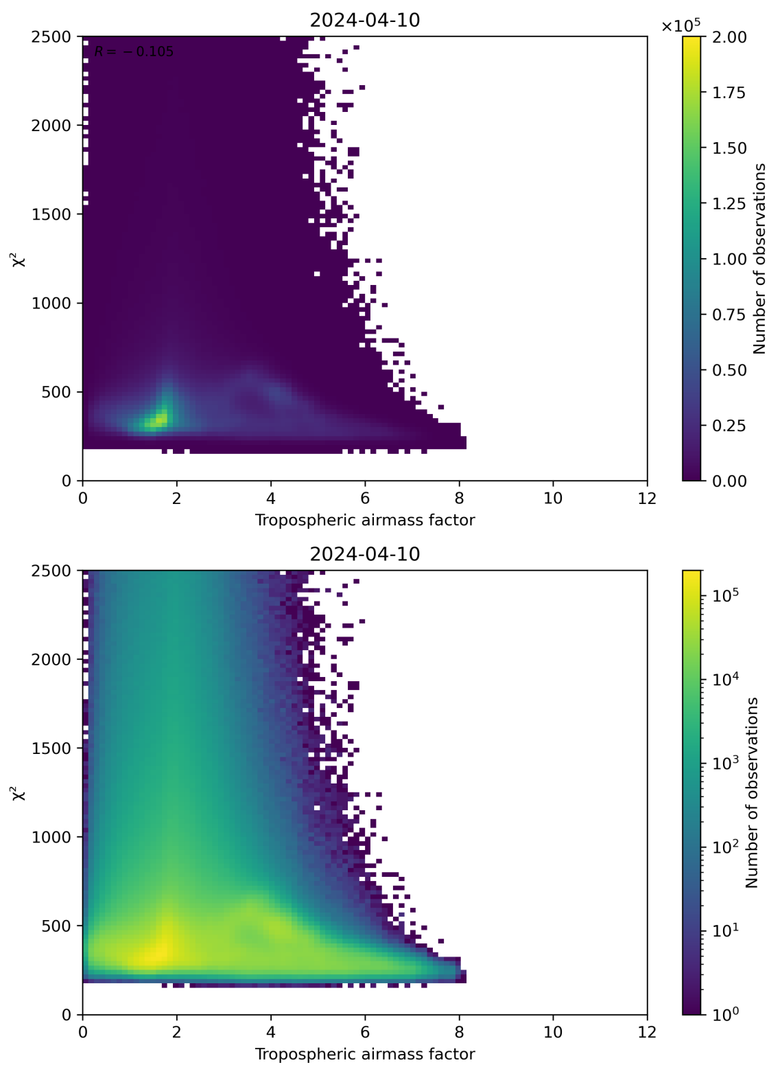
Figure 73: Scatter density plot of “Tropospheric airmass factor” against “ \chi^2 ” for 2024-04-10 to 2024-04-11.
