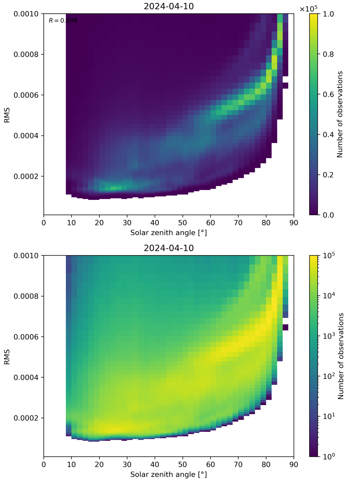
Figure 157: Scatter density plot of “Solar zenith angle” against “RMS” for 2024-04-10 to 2024-04-11.
