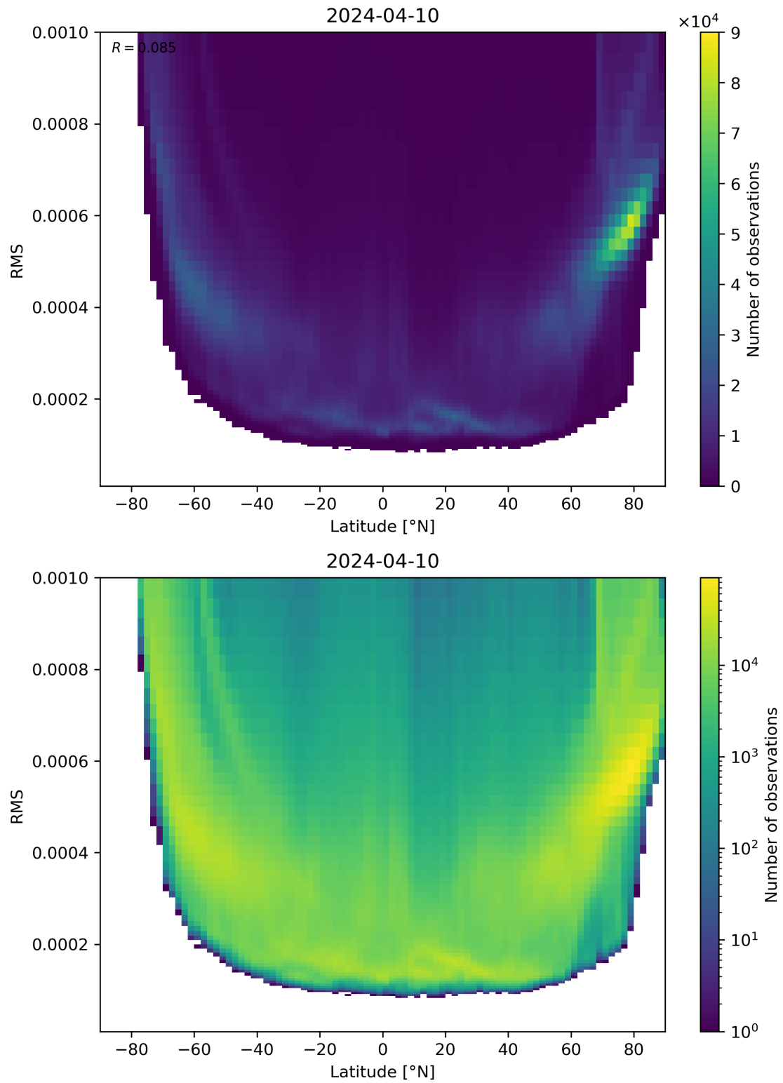
Figure 94: Scatter density plot of “Latitude” against “RMS” for 2024-04-10 to 2024-04-11.
