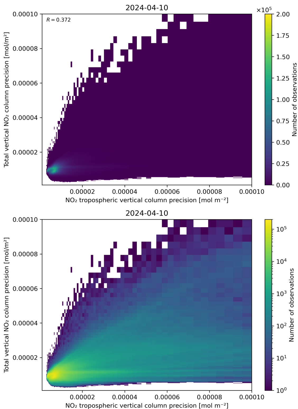
Figure 139: Scatter density plot of “NO 2 tropospheric vertical column precision” against “Total vertical NO 2 column precision” for 2024-04-10 to 2024-04-11.
