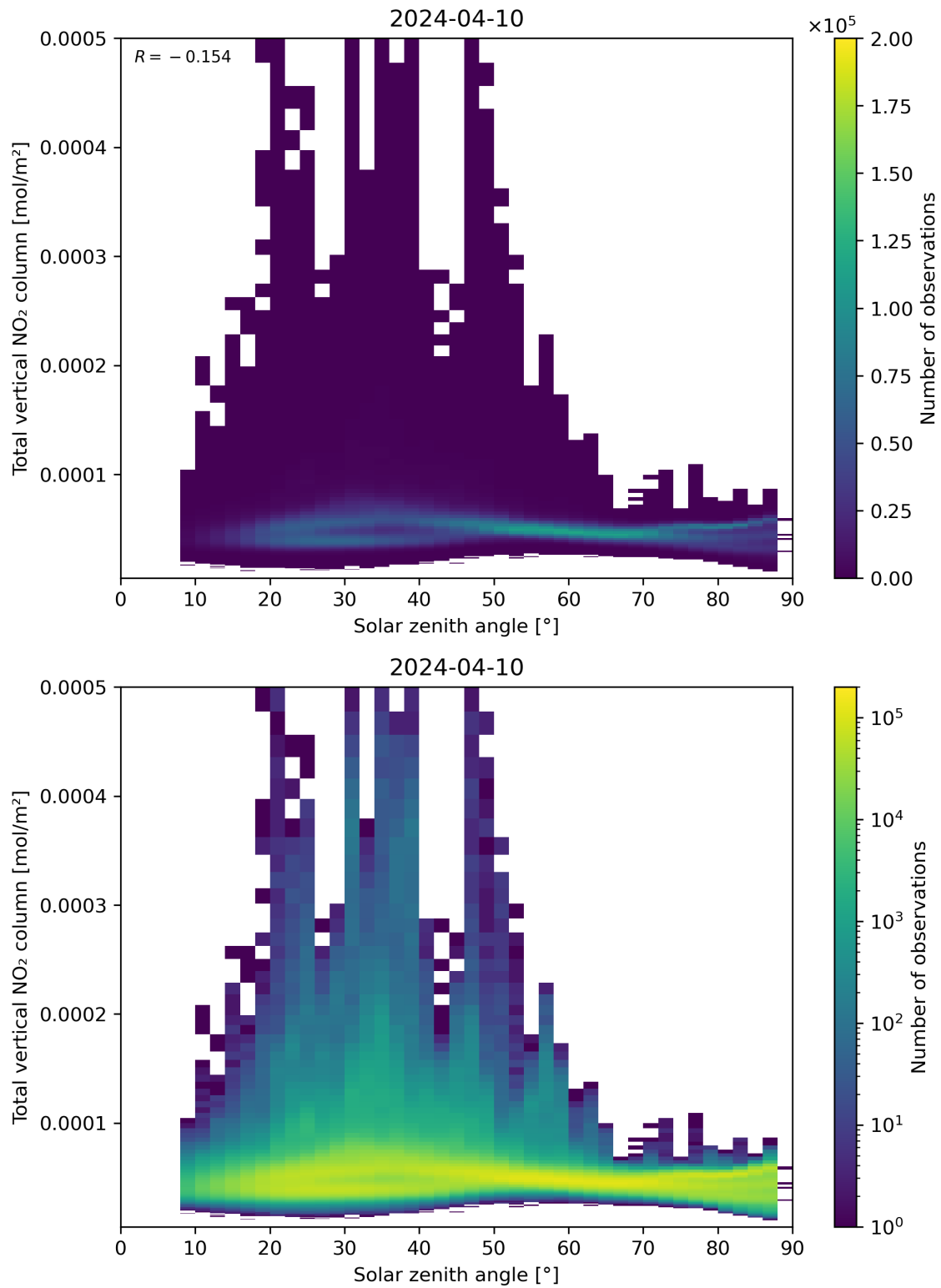
Figure 153: Scatter density plot of “Solar zenith angle” against “Total vertical NO 2 column” for 2024-04-10 to 2024-04-11.
