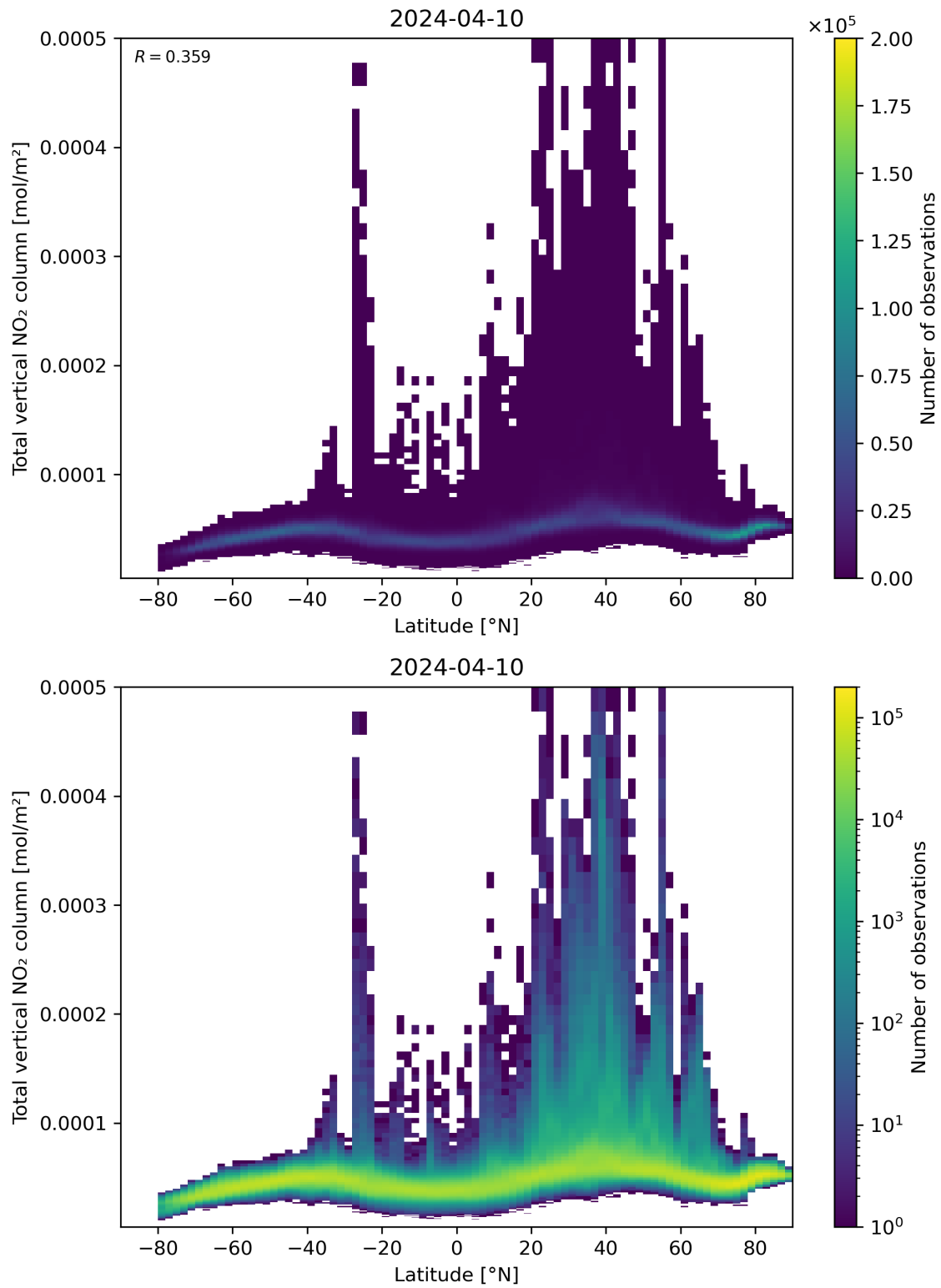
Figure 90: Scatter density plot of “Latitude” against “Total vertical NO 2 column” for 2024-04-10 to 2024-04-11.
