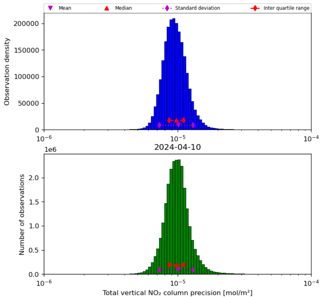
Figure 39: Histogram of “Total vertical NO 2 column precision” for 2024-04-10 to 2024-04-11
