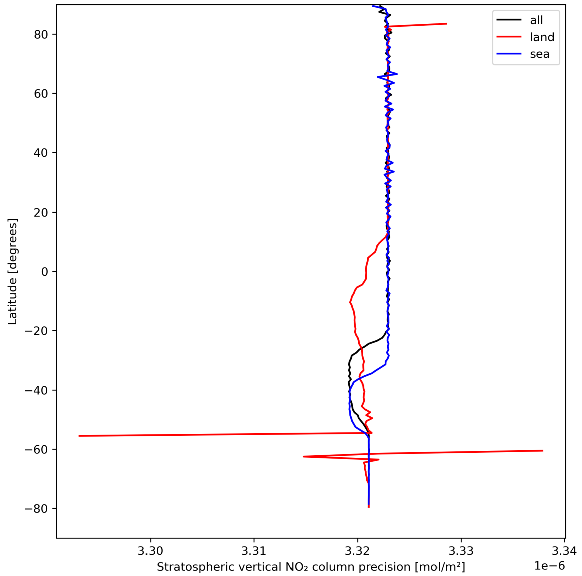
Figure 20: Zonal average of “Stratospheric vertical NO 2 column precision” for 2024-04-10 to 2024-04-11.
