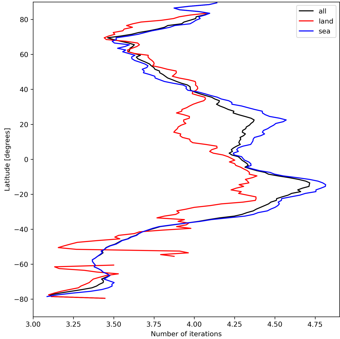
Figure 17: Zonal average of “Number of iterations” for 2024-04-10 to 2024-04-11.
