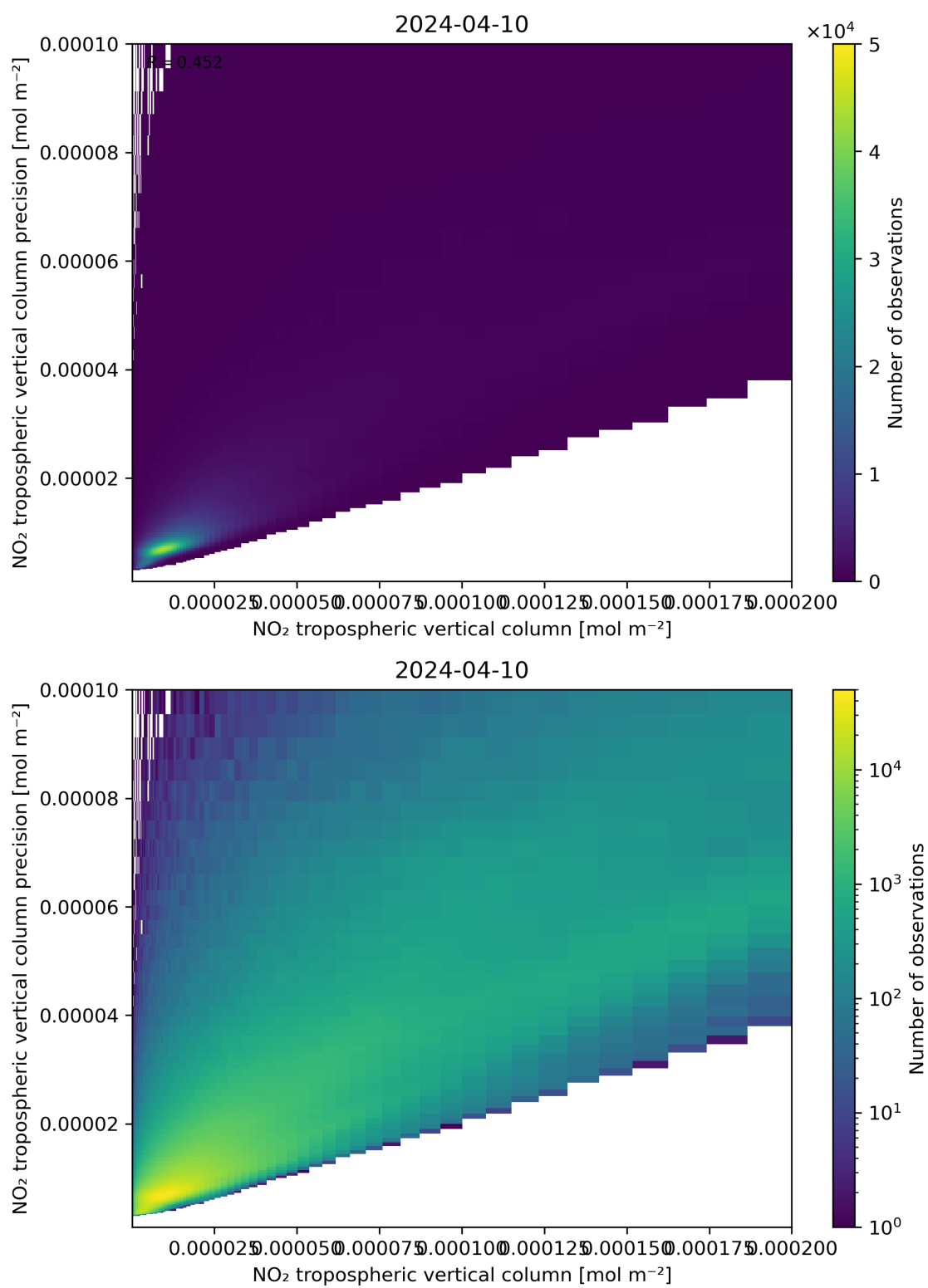
Figure 130: Scatter density plot of “NO 2 tropospheric vertical column” against “NO 2 tropospheric vertical column precision” for 2024-04-10 to 2024-04-11.
