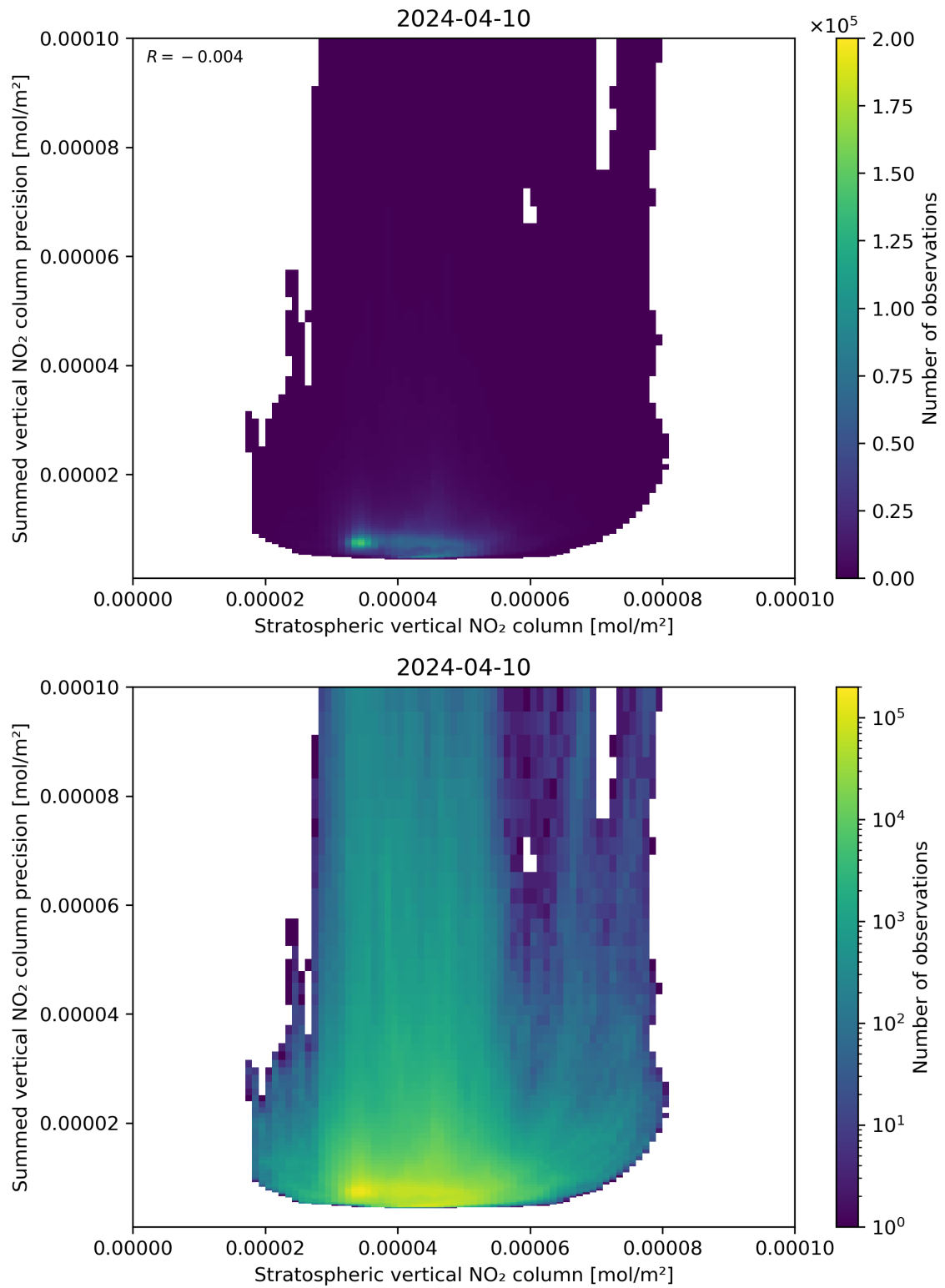
Figure 99: Scatter density plot of “Stratospheric vertical NO 2 column” against “Summed vertical NO 2 column precision” for 2024-04-10 to 2024-04-11.
