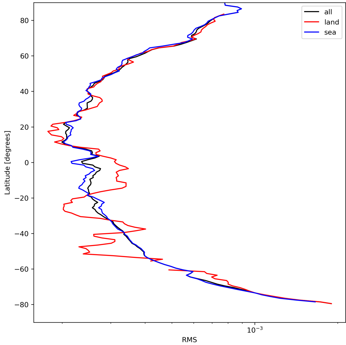
Figure 26: Zonal average of “RMS” for 2024-04-10 to 2024-04-11.
