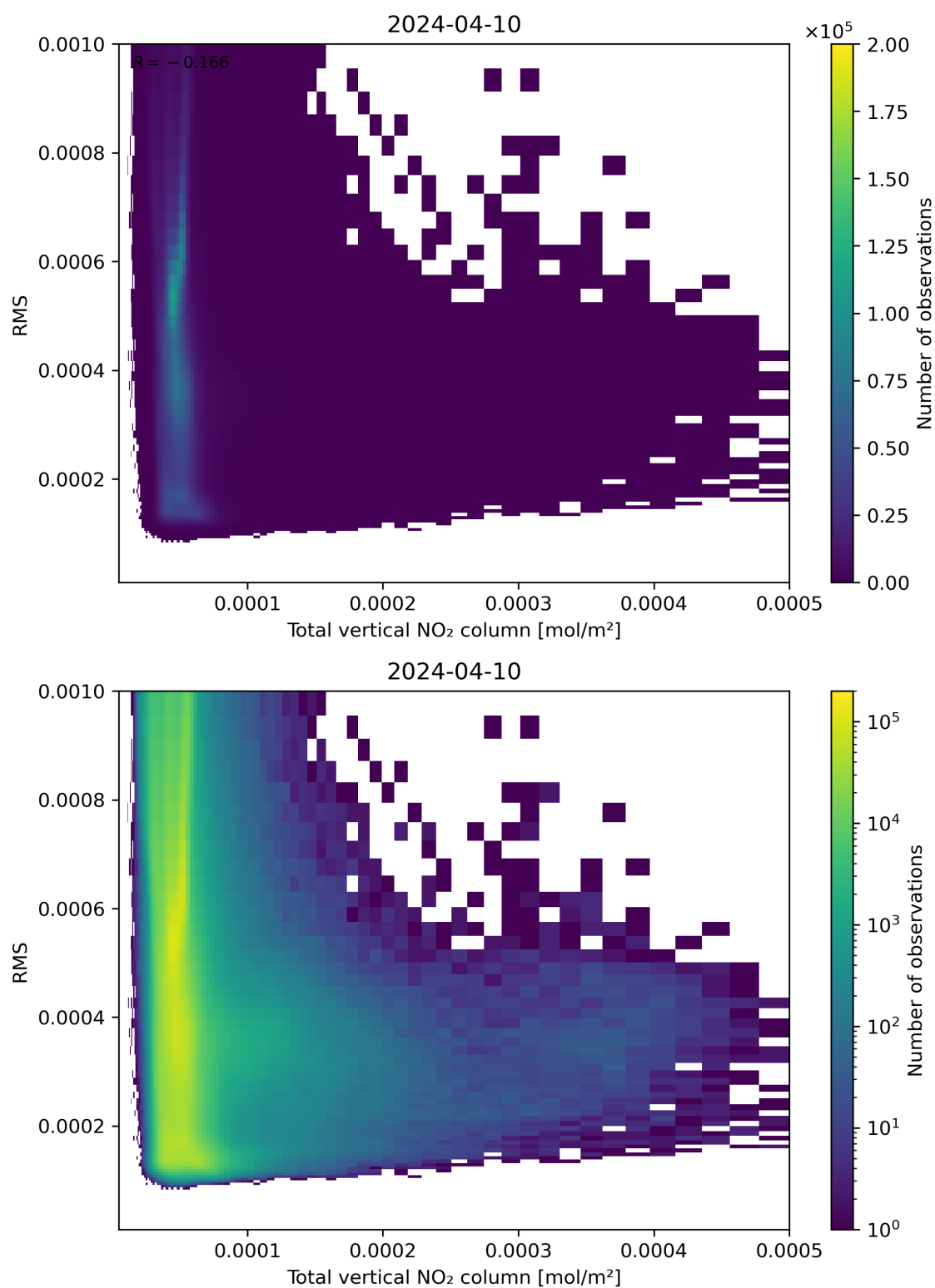
Figure 120: Scatter density plot of “Total vertical NO 2 column” against “RMS” for 2024-04-10 to 2024-04-11.
