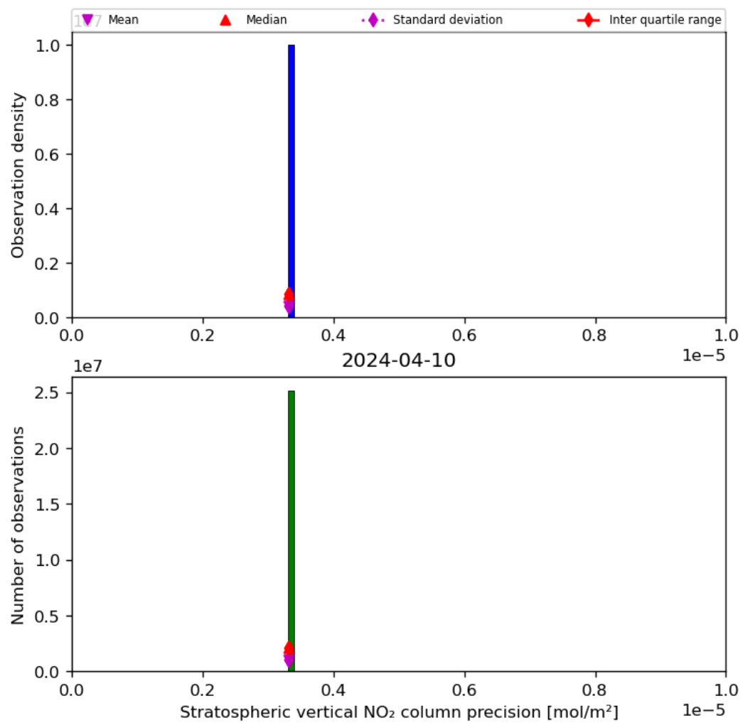
Figure 37: Histogram of “Stratospheric vertical NO 2 column precision” for 2024-04-10 to 2024-04-11
