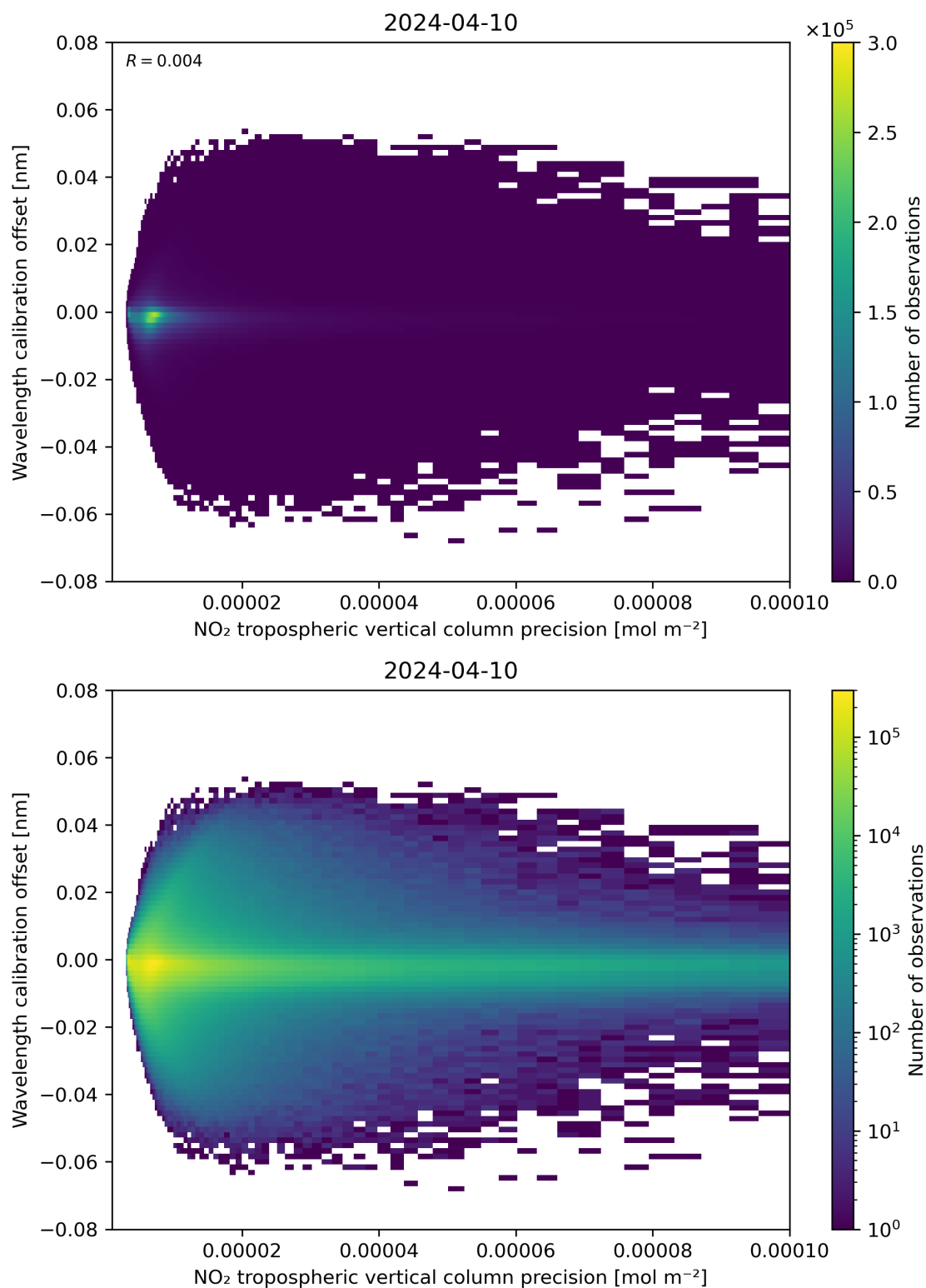
Figure 141: Scatter density plot of “NO 2 tropospheric vertical column precision” against “Wavelength calibration offset” for 2024-04-10 to 2024-04-11.
