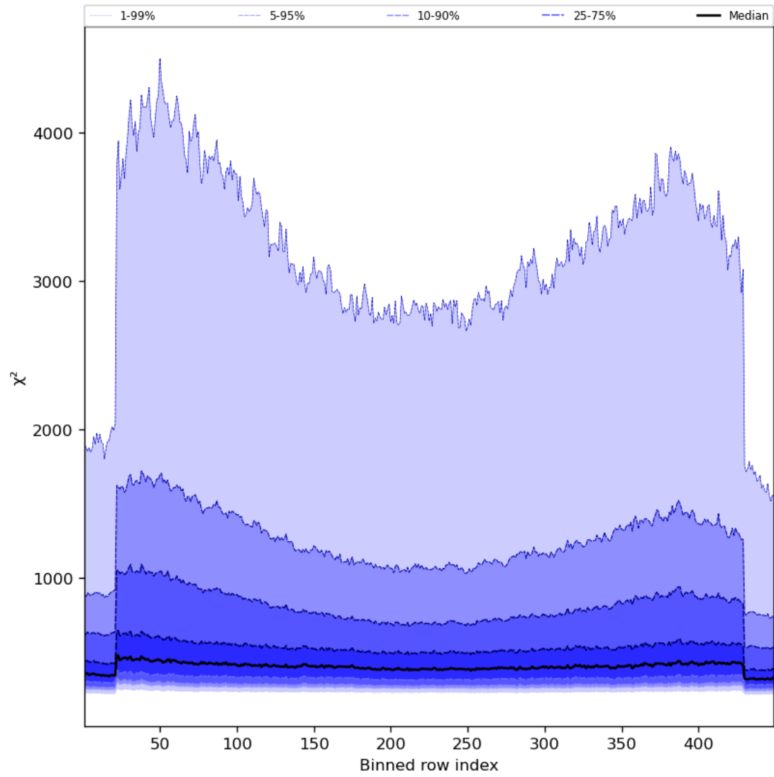
Figure 59: Along track statistics of “ \chi^2 ” for 2024-04-10 to 2024-04-11
