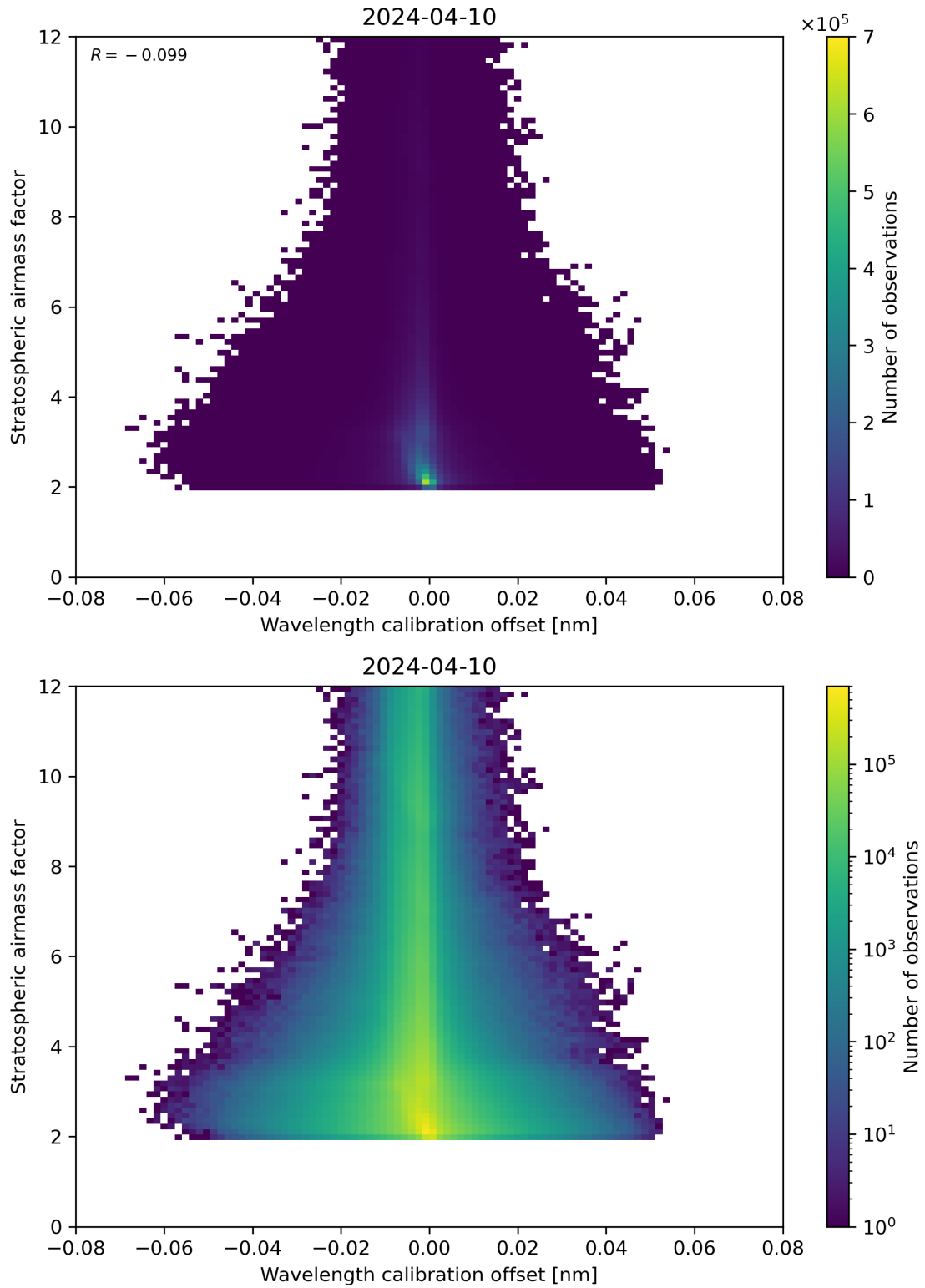
Figure 174: Scatter density plot of “Wavelength calibration offset” against “Stratospheric air mass factor” for 2024-04-10 to 2024-04-11.
