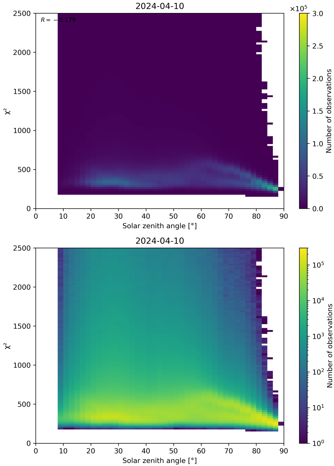
Figure 148: Scatter density plot of “Solar zenith angle” against “ \chi^2 ” for 2024-04-10 to 2024-04-11.
