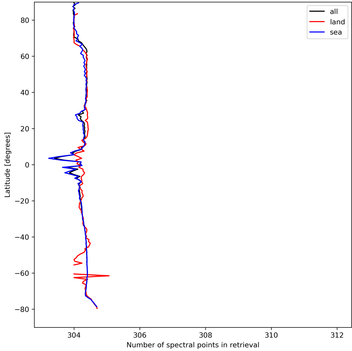
Figure 16: Zonal average of “Number of spectral points in retrieval” for 2024-04-10 to 2024-04-11.
