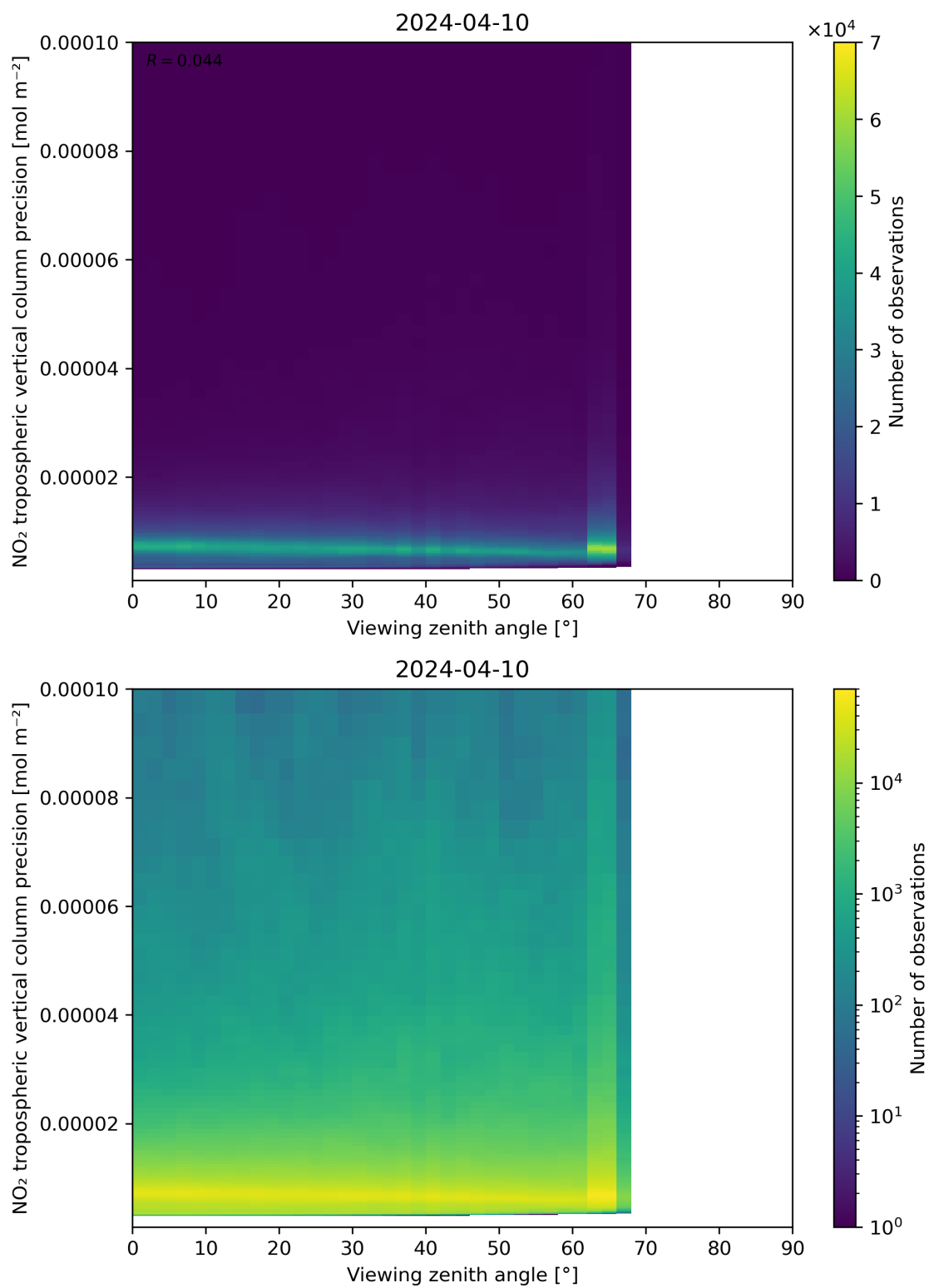
Figure 170: Scatter density plot of “Viewing zenith angle” against “NO 2 tropospheric vertical column precision” for 2024-04-10 to 2024-04-11.
