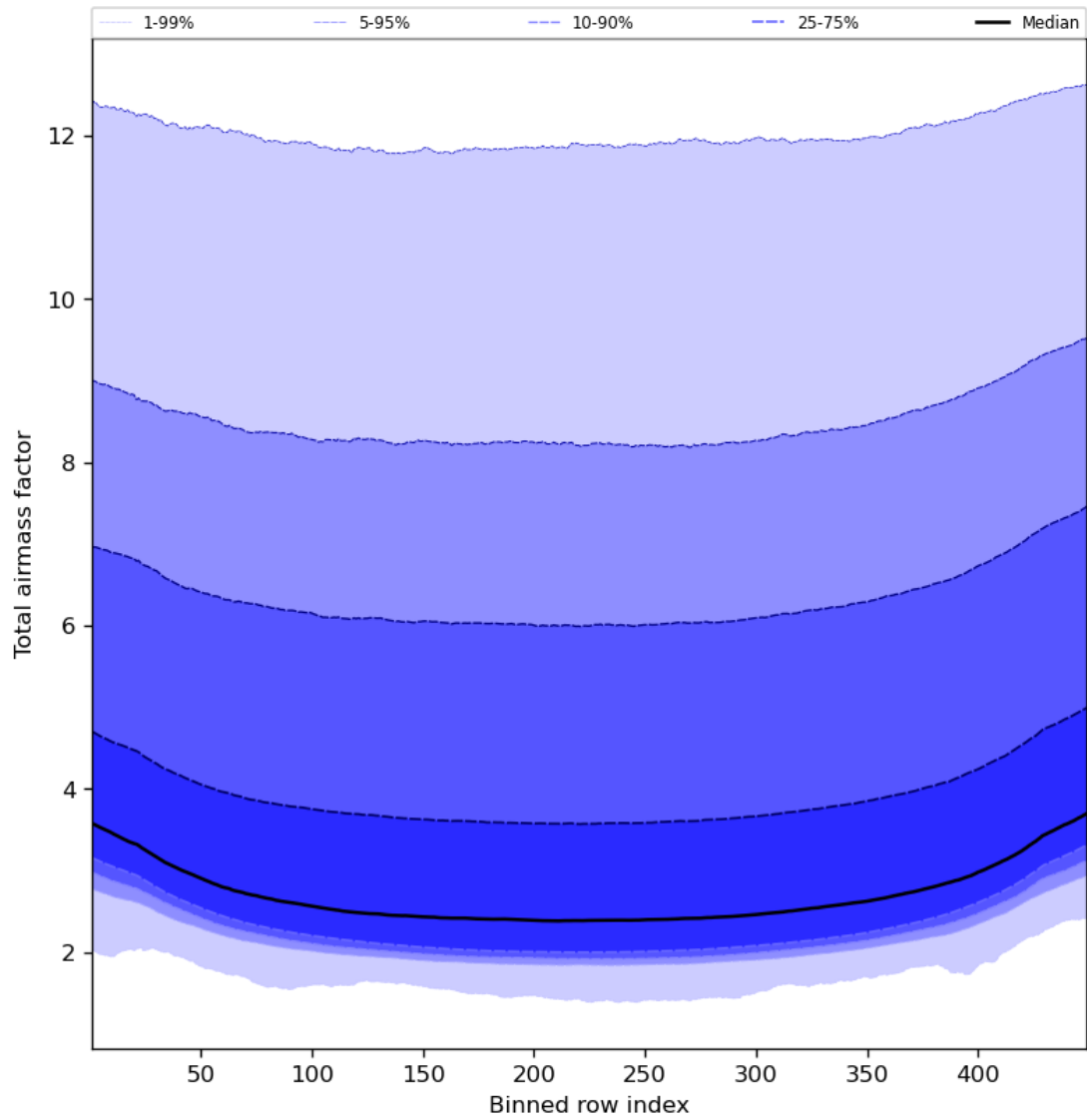
Figure 49: Along track statistics of “Total airmass factor” for 2024-04-10 to 2024-04-11
