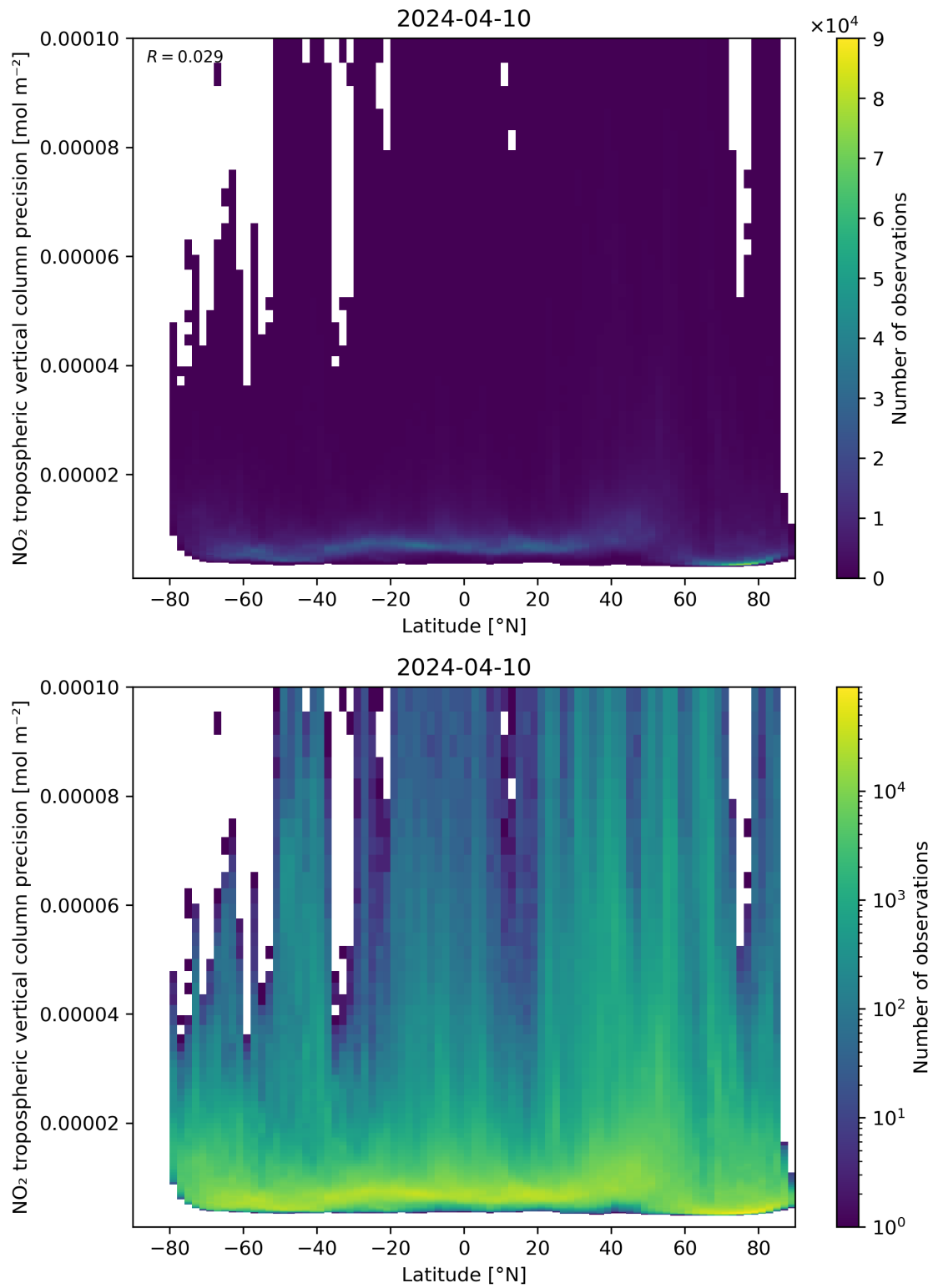
Figure 93: Scatter density plot of “Latitude” against “NO 2 tropospheric vertical column precision” for 2024-04-10 to 2024-04-11.
