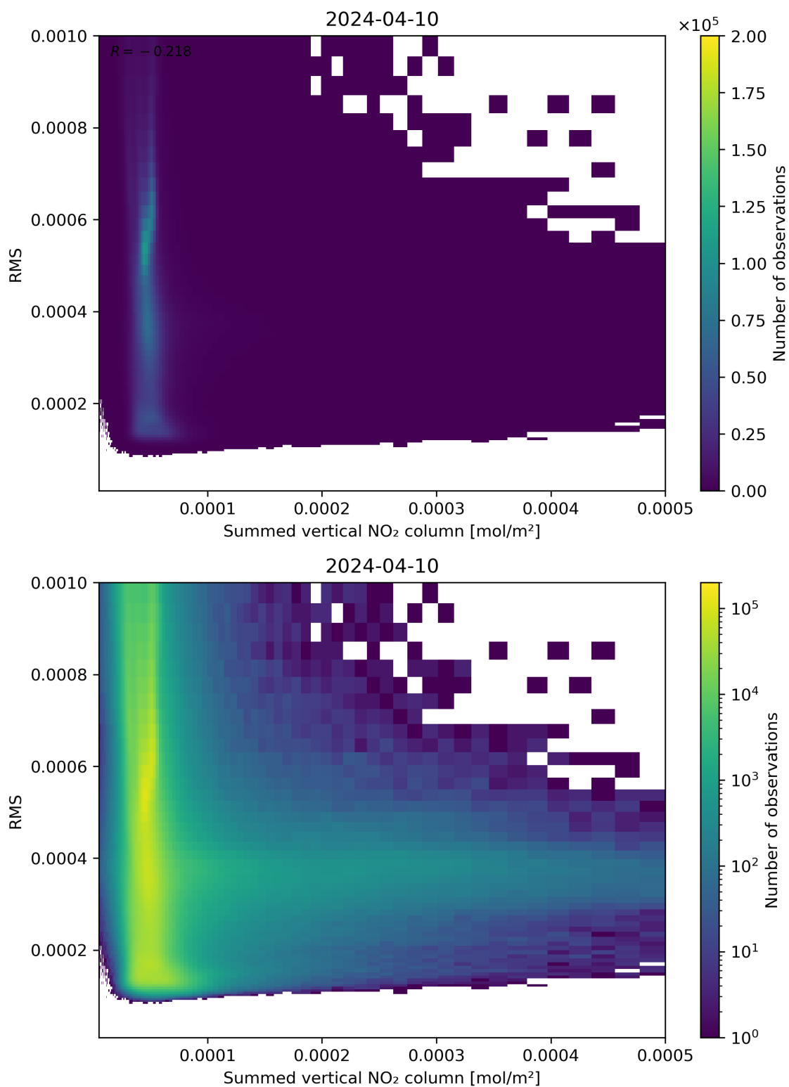
Figure 109: Scatter density plot of “Summed vertical NO 2 column” against “RMS” for 2024-04-10 to 2024-04-11.
