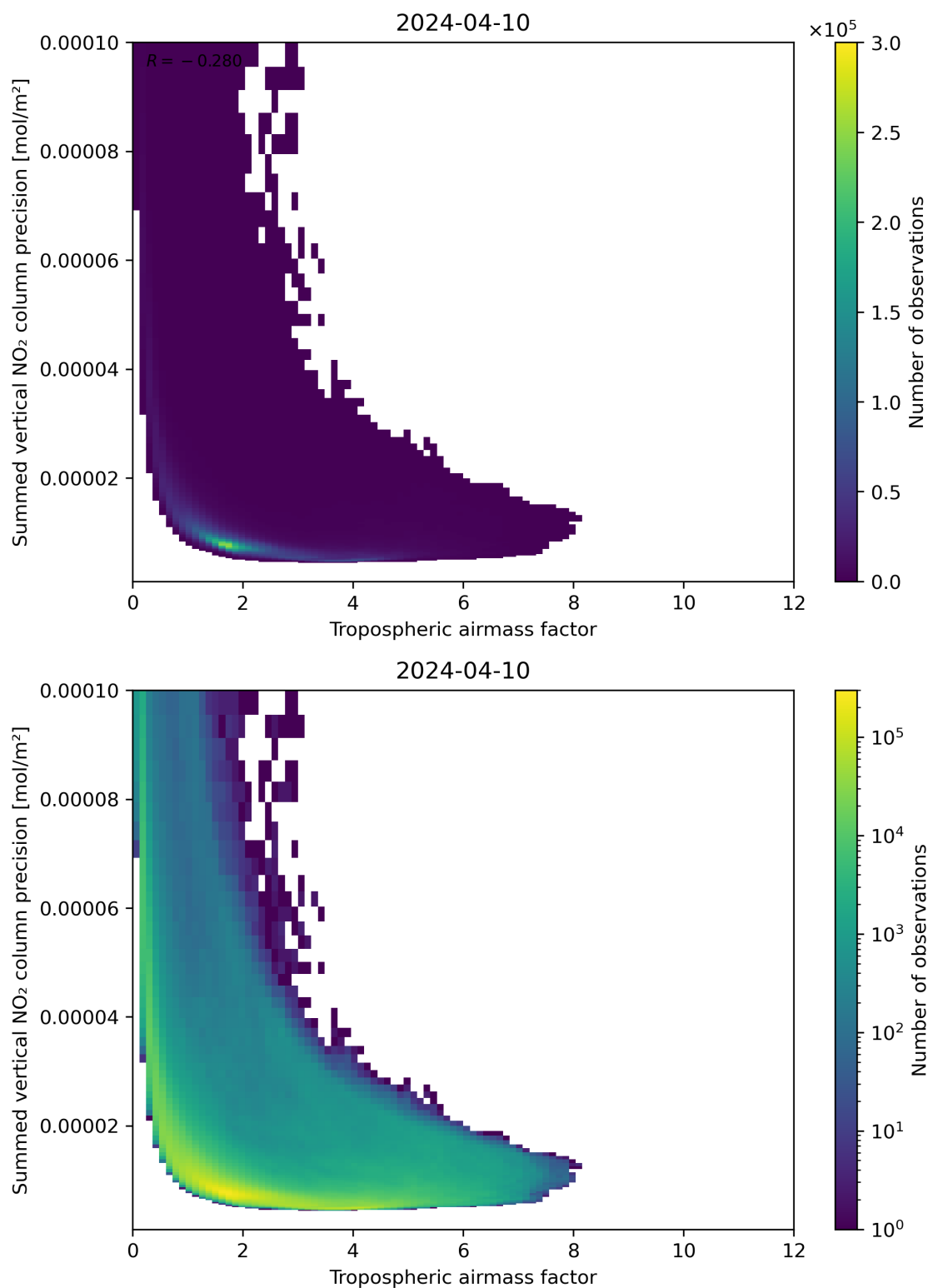
Figure 76: Scatter density plot of “Tropospheric air mass factor” against “Summed vertical NO 2 column precision” for 2024-04-10 to 2024-04-11.
