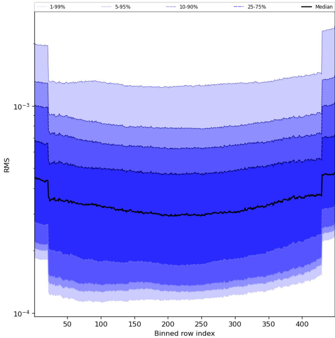
Figure 60: Along track statistics of “RMS” for 2024-04-10 to 2024-04-11
