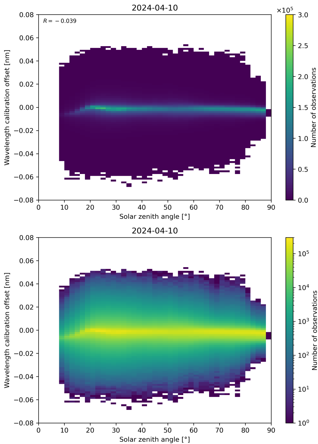
Figure 158: Scatter density plot of “Solar zenith angle” against “Wavelength calibration offset” for 2024-04-10 to 2024-04-11.
