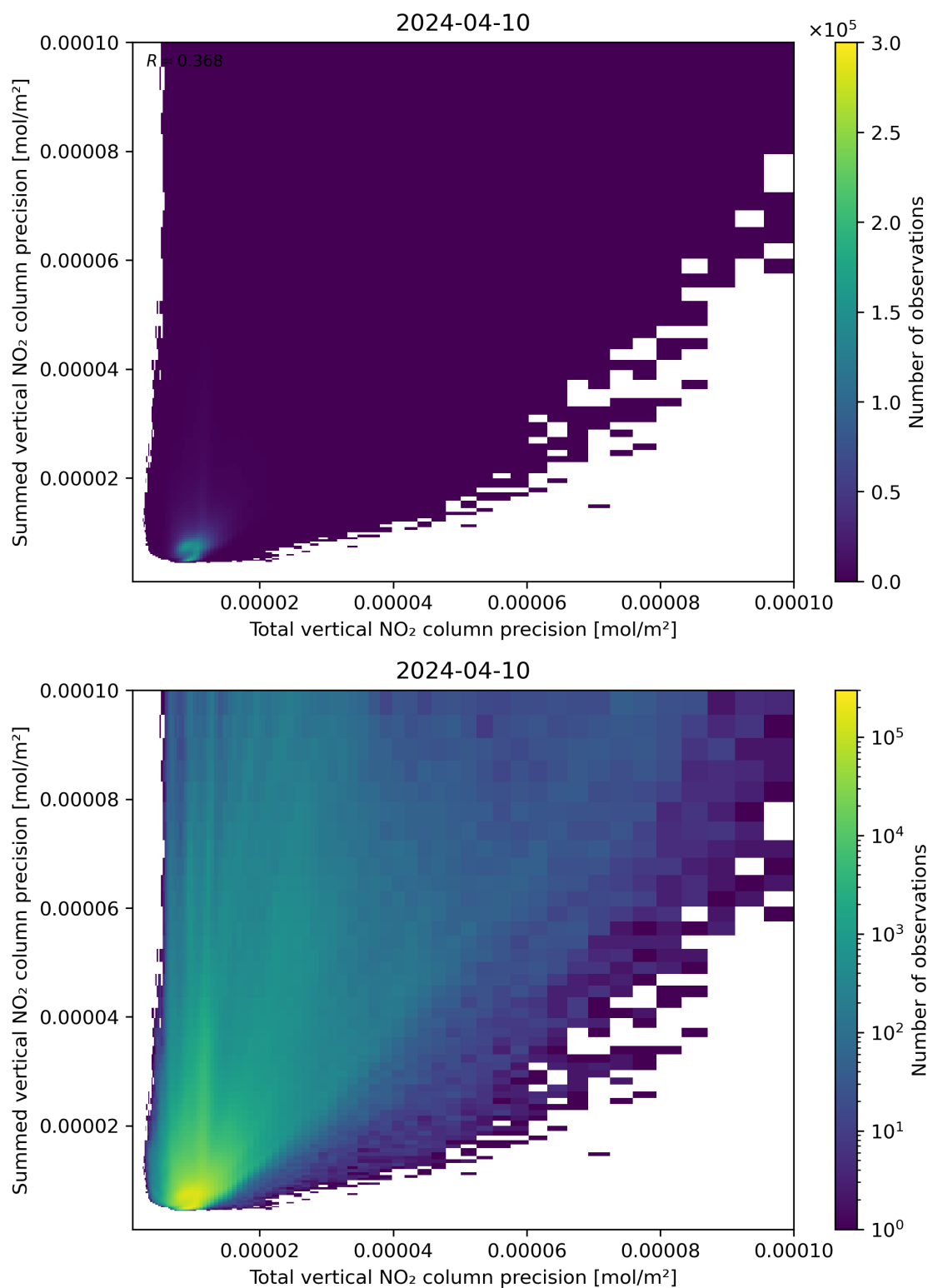
Figure 118: Scatter density plot of “Total vertical NO 2 column precision” against “Summed vertical NO 2 column precision” for 2024-04-10 to 2024-04-11.
