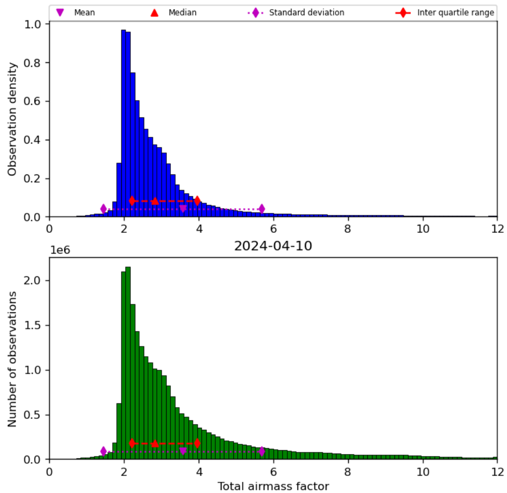
Figure 32: Histogram of “Total airmass factor” for 2024-04-10 to 2024-04-11
