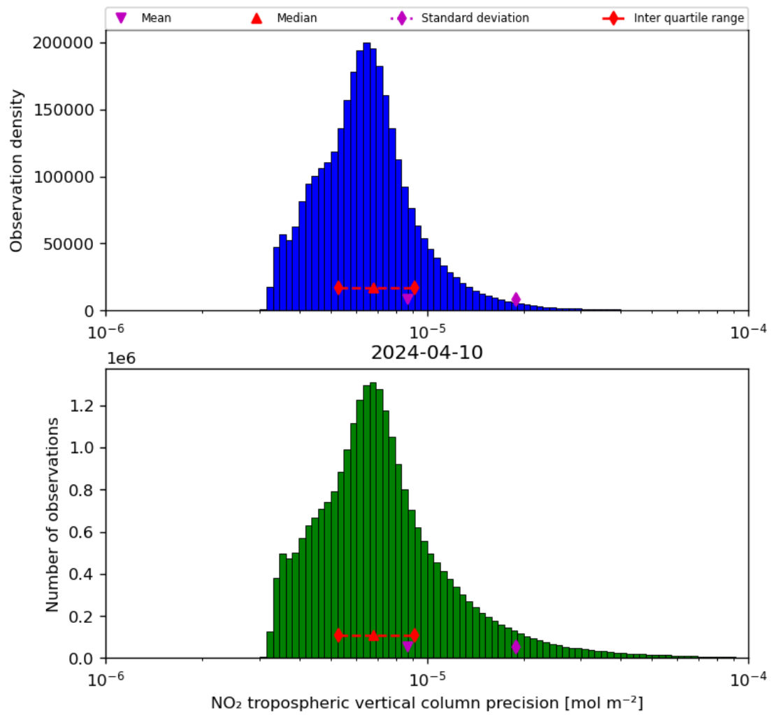
Figure 30: Histogram of “NO 2 tropospheric vertical column precision” for 2024-04-10 to 2024-04-11
