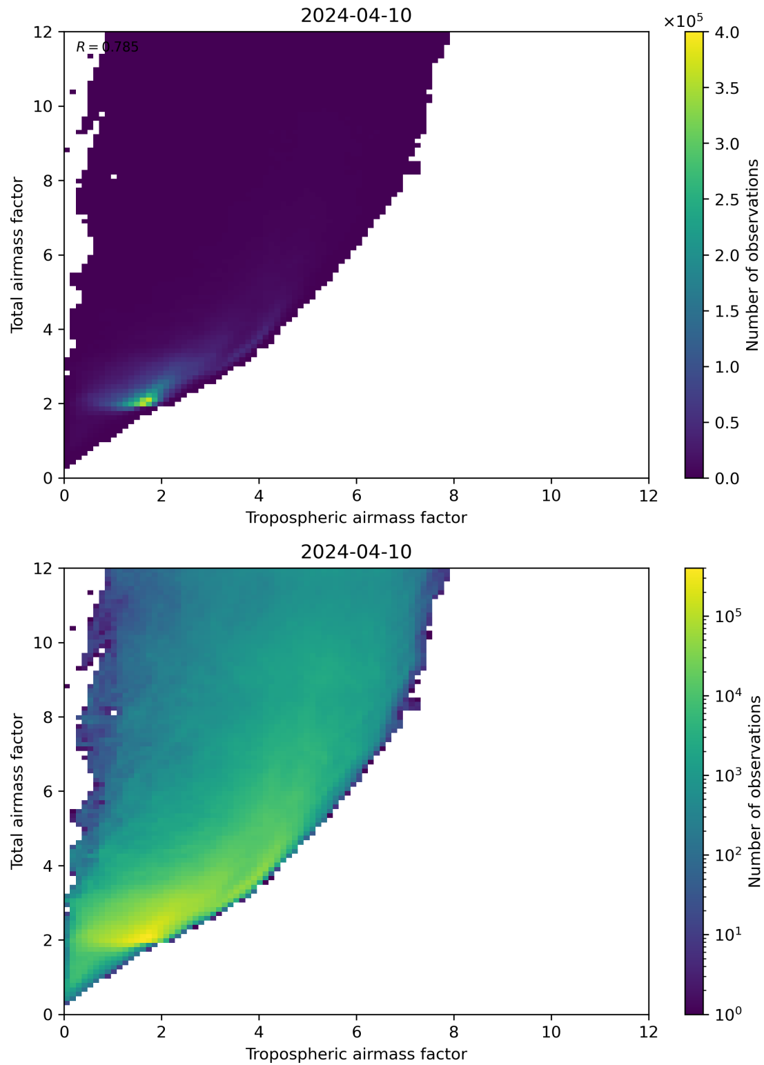
Figure 72: Scatter density plot of “Tropospheric airmass factor” against “Total airmass factor” for 2024-04-10 to 2024-04-11.
