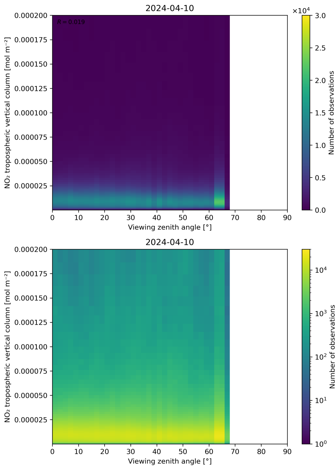
Figure 169: Scatter density plot of “Viewing zenith angle” against “NO 2 tropospheric vertical column” for 2024-04-10 to 2024-04-11.
