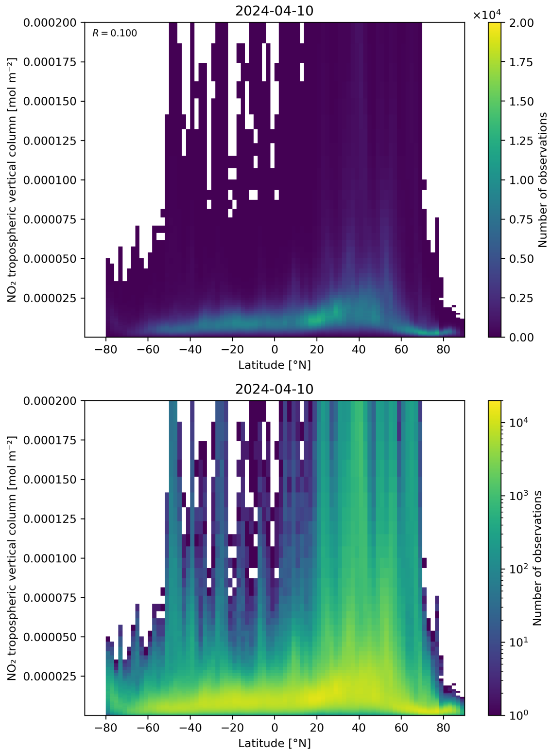
Figure 92: Scatter density plot of “Latitude” against “NO 2 tropospheric vertical column” for 2024-04-10 to 2024-04-11.
