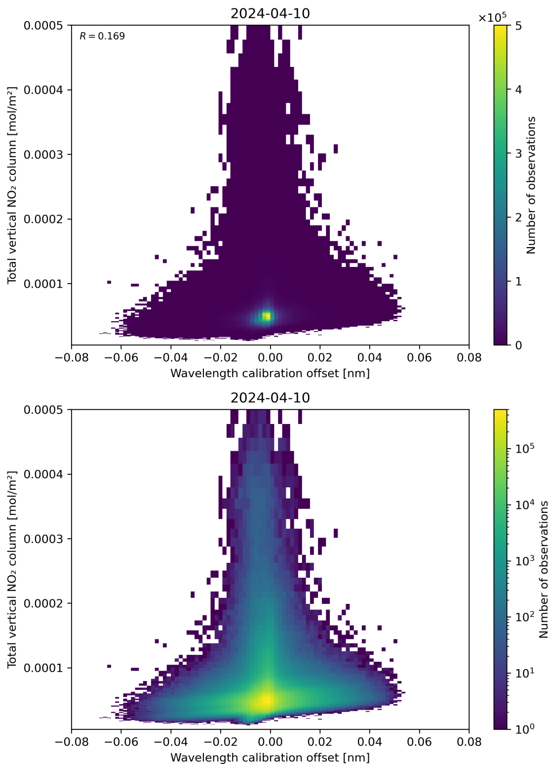
Figure 179: Scatter density plot of “Wavelength calibration offset” against “Total vertical NO 2 column” for 2024-04-10 to 2024-04-11.
