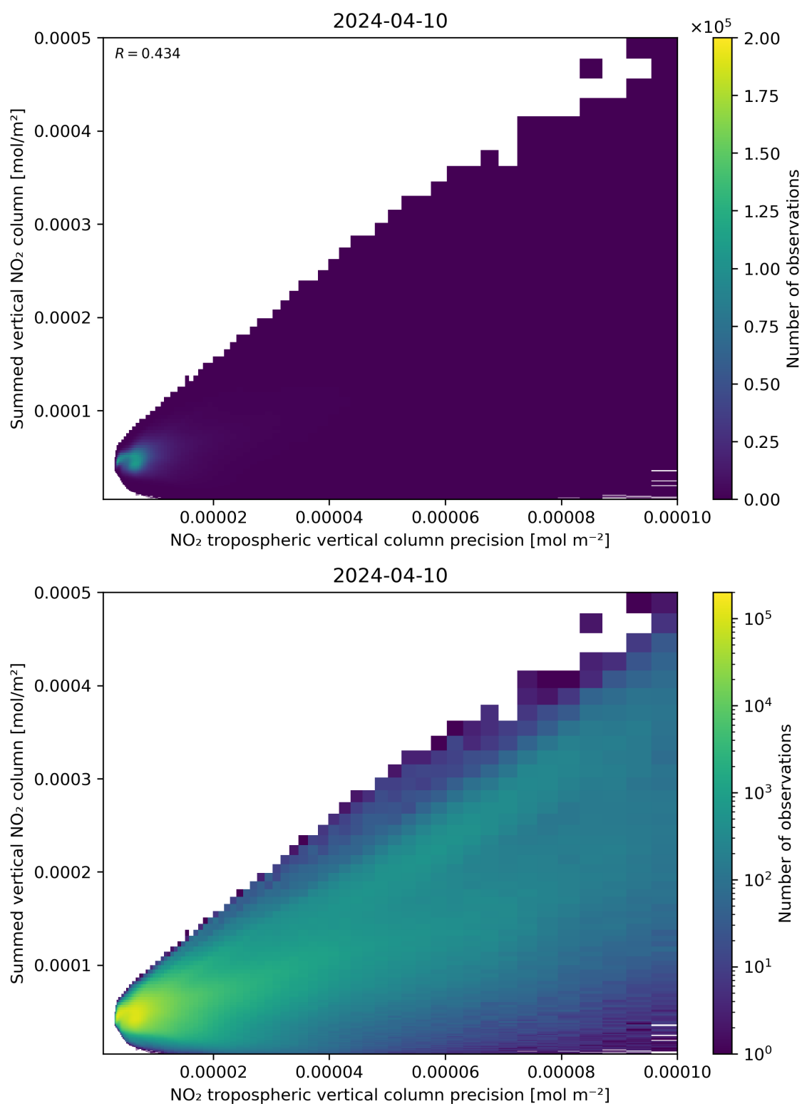
Figure 136: Scatter density plot of “NO 2 tropospheric vertical column precision” against “Summed vertical NO 2 column” for 2024-04-10 to 2024-04-11.
