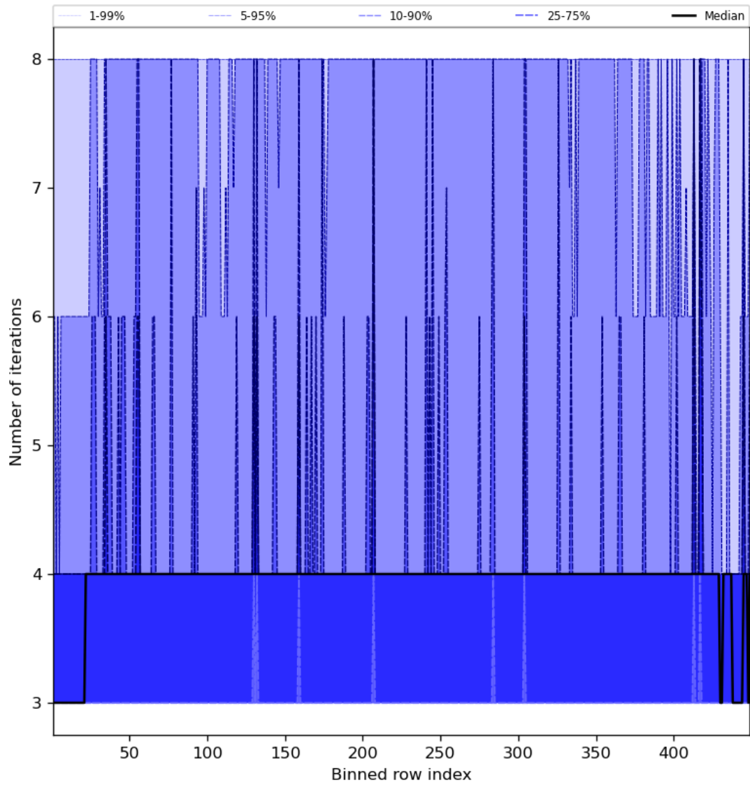
Figure 51: Along track statistics of “Number of iterations” for 2024-04-10 to 2024-04-11
