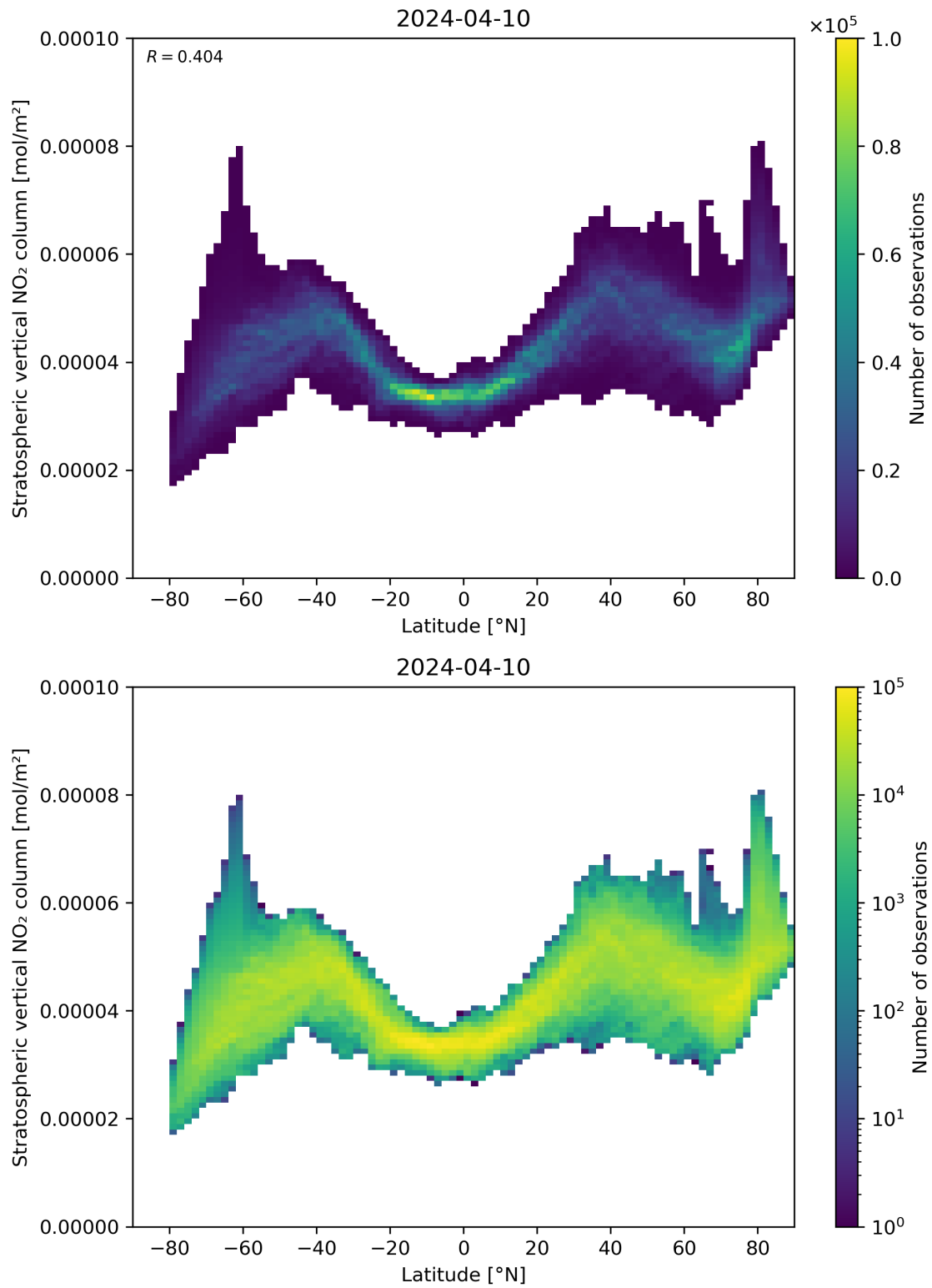
Figure 87: Scatter density plot of “Latitude” against “Stratospheric vertical NO 2 column” for 2024-04-10 to 2024-04-11.
