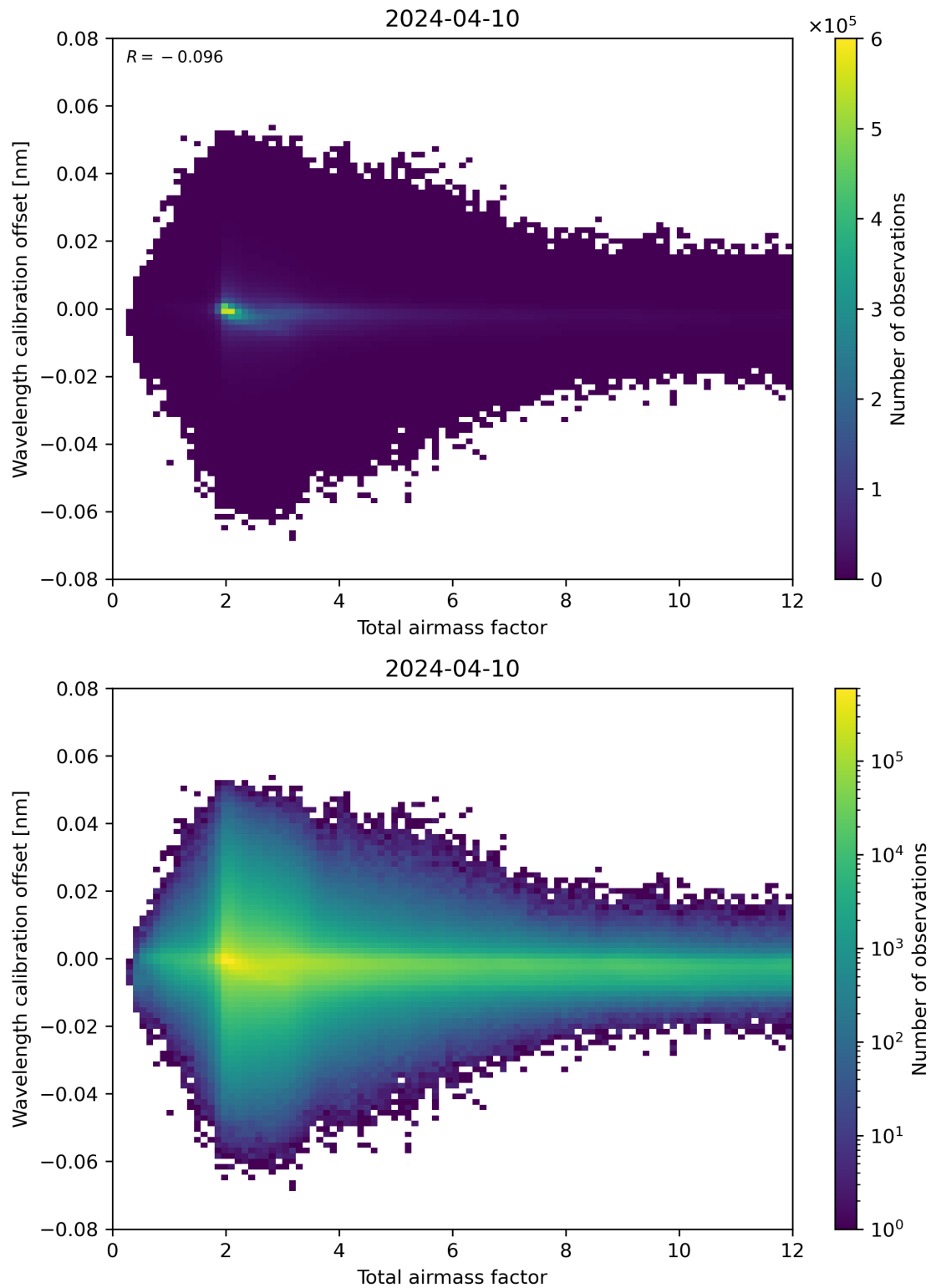
Figure 70: Scatter density plot of “Total airmass factor” against “Wavelength calibration offset” for 2024-04-10 to 2024-04-11.
