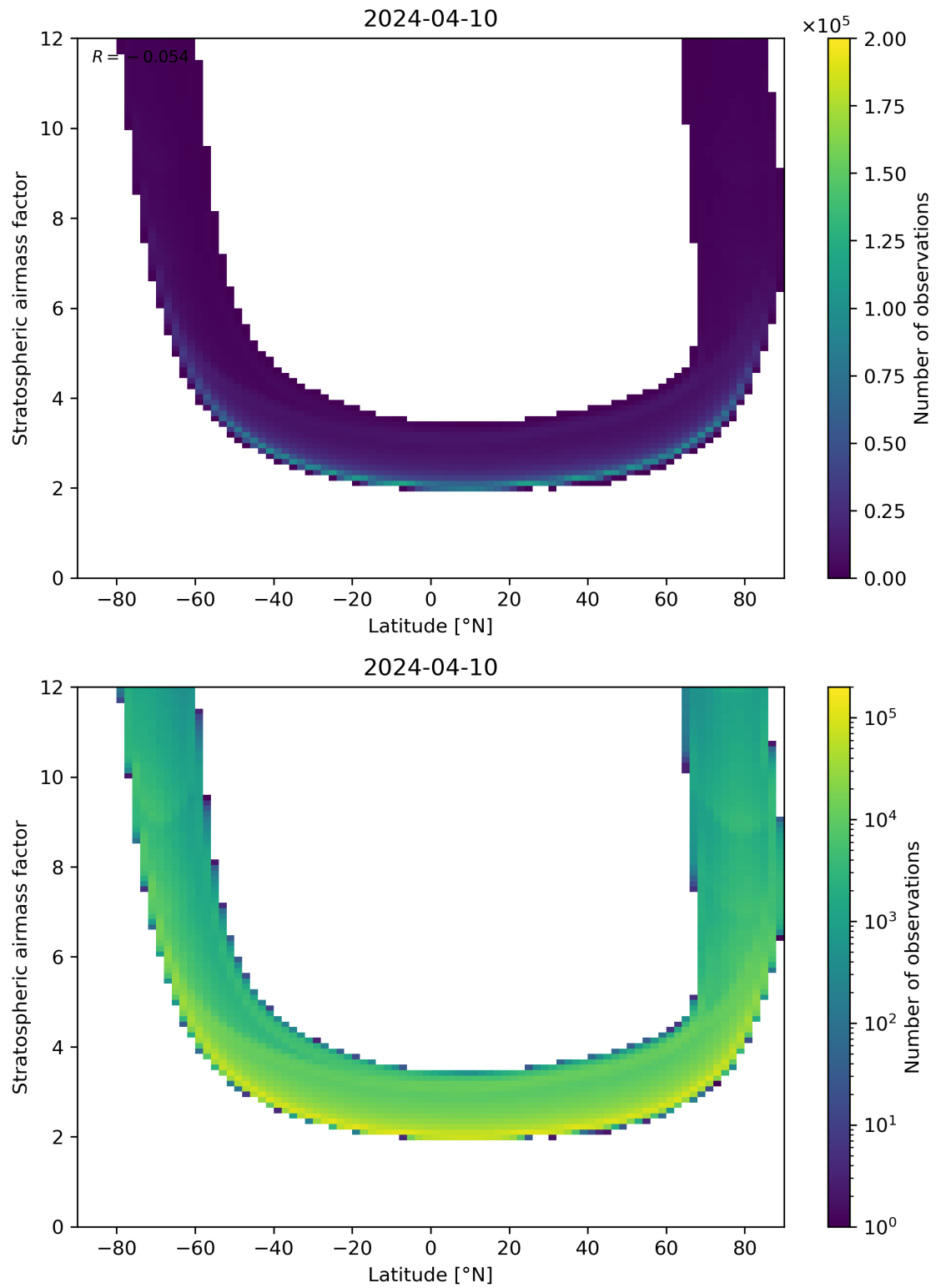
Figure 83: Scatter density plot of “Latitude” against “Stratospheric airmass factor” for 2024-04-10 to 2024-04-11.
