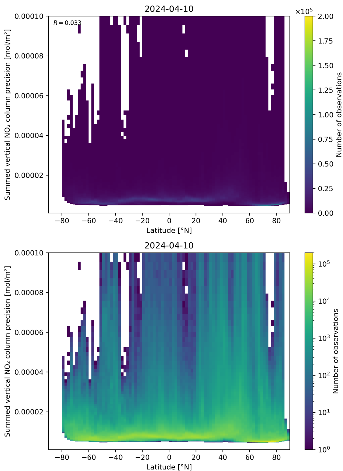
Figure 89: Scatter density plot of “Latitude” against “Summed vertical NO 2 column precision” for 2024-04-10 to 2024-04-11.
