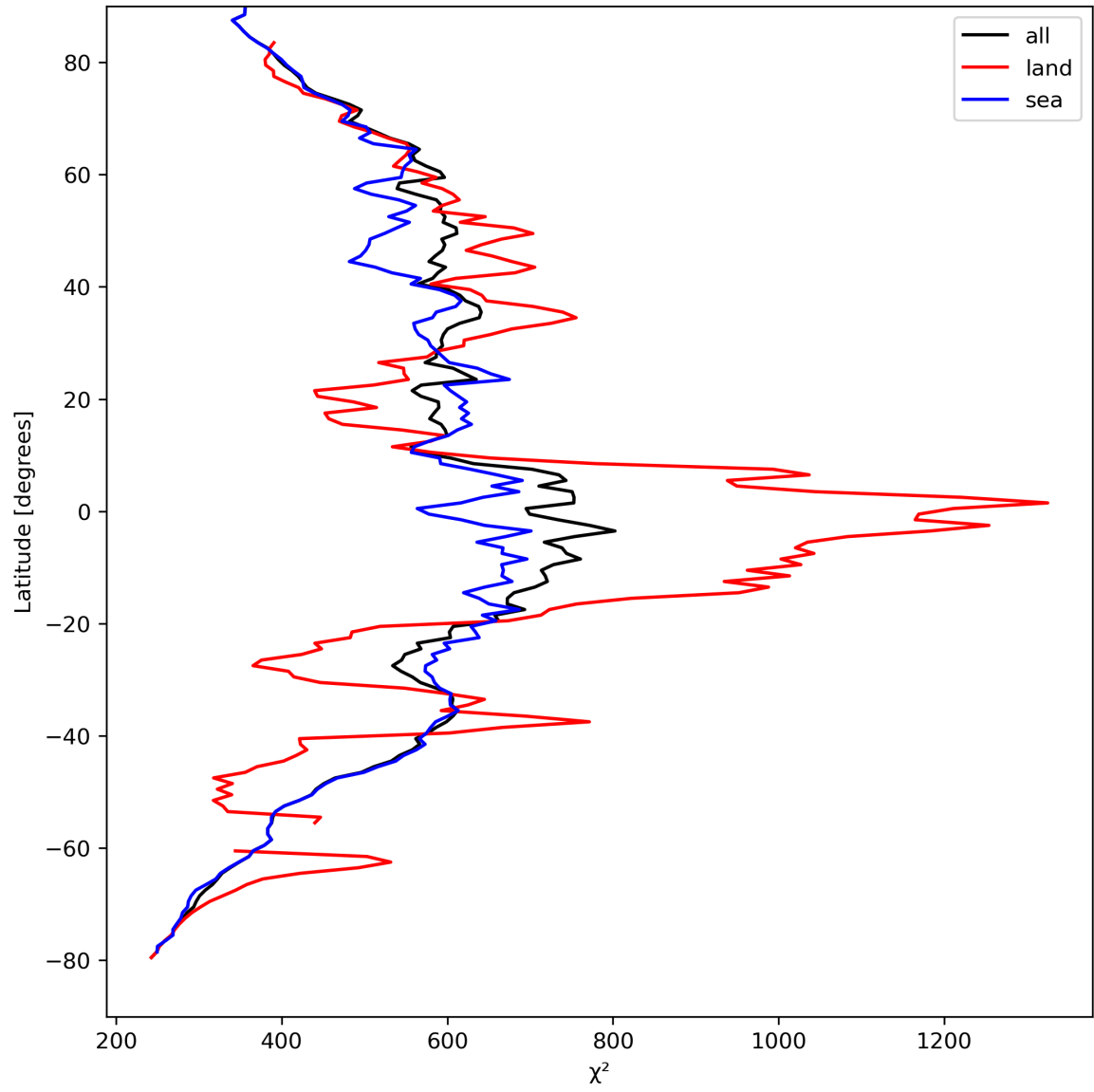
Figure 25: Zonal average of “ \chi^2 ” for 2024-04-10 to 2024-04-11.
