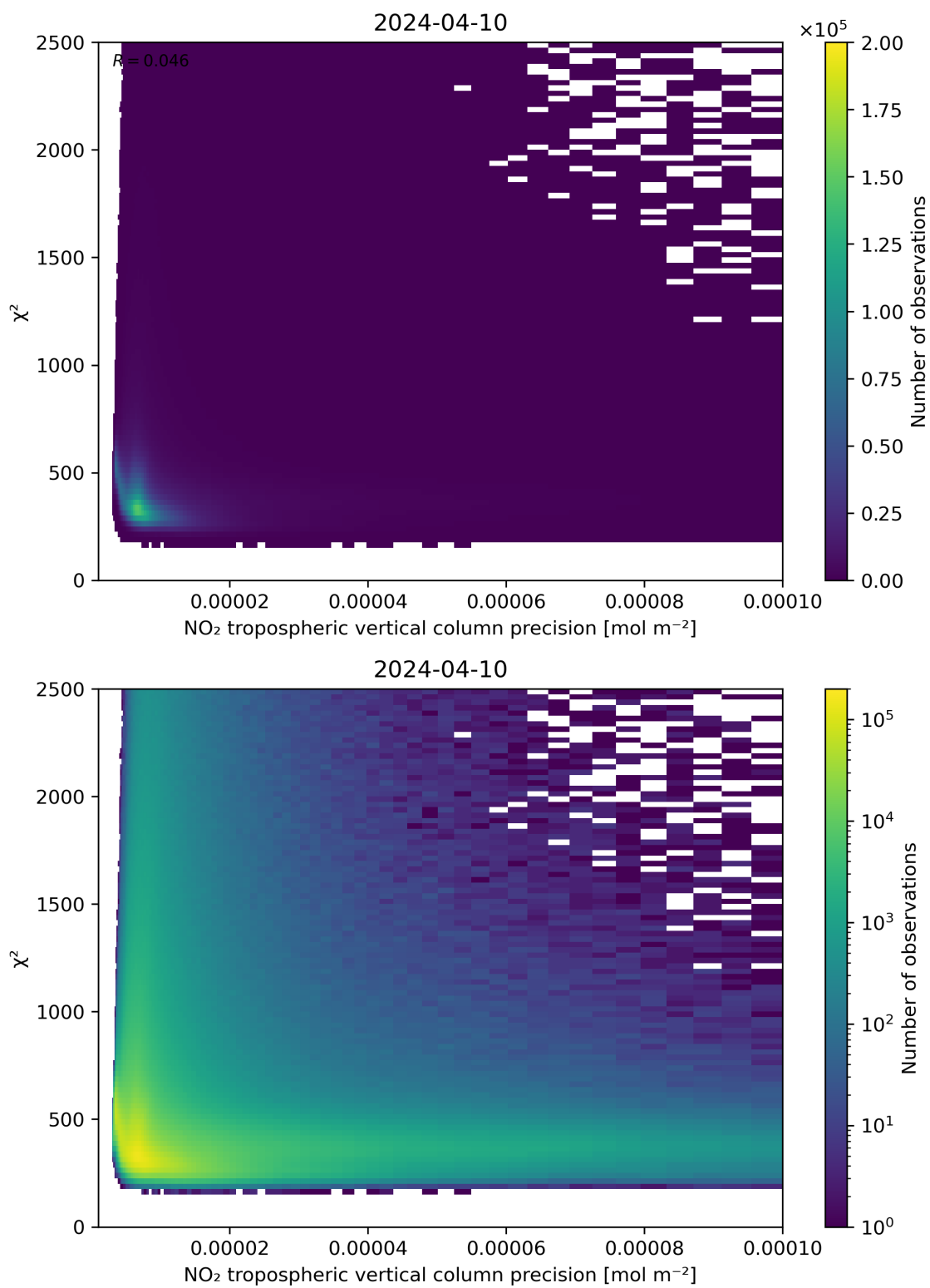
Figure 134: Scatter density plot of “NO 2 tropospheric vertical column precision” against “ \chi^2 ” for 2024-04-10 to 2024-04-11.
