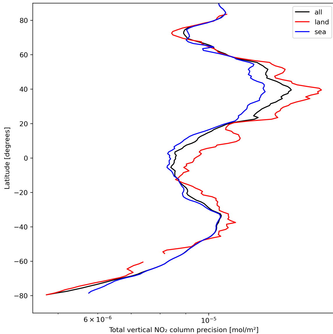
Figure 22: Zonal average of “Total vertical NO 2 column precision” for 2024-04-10 to 2024-04-11.
