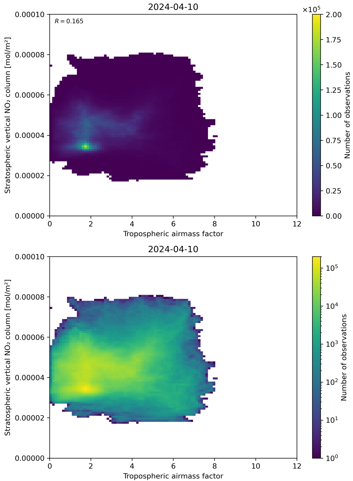
Figure 74: Scatter density plot of “Tropospheric air mass factor” against “Stratospheric vertical NO 2 column” for 2024-04-10 to 2024-04-11.
