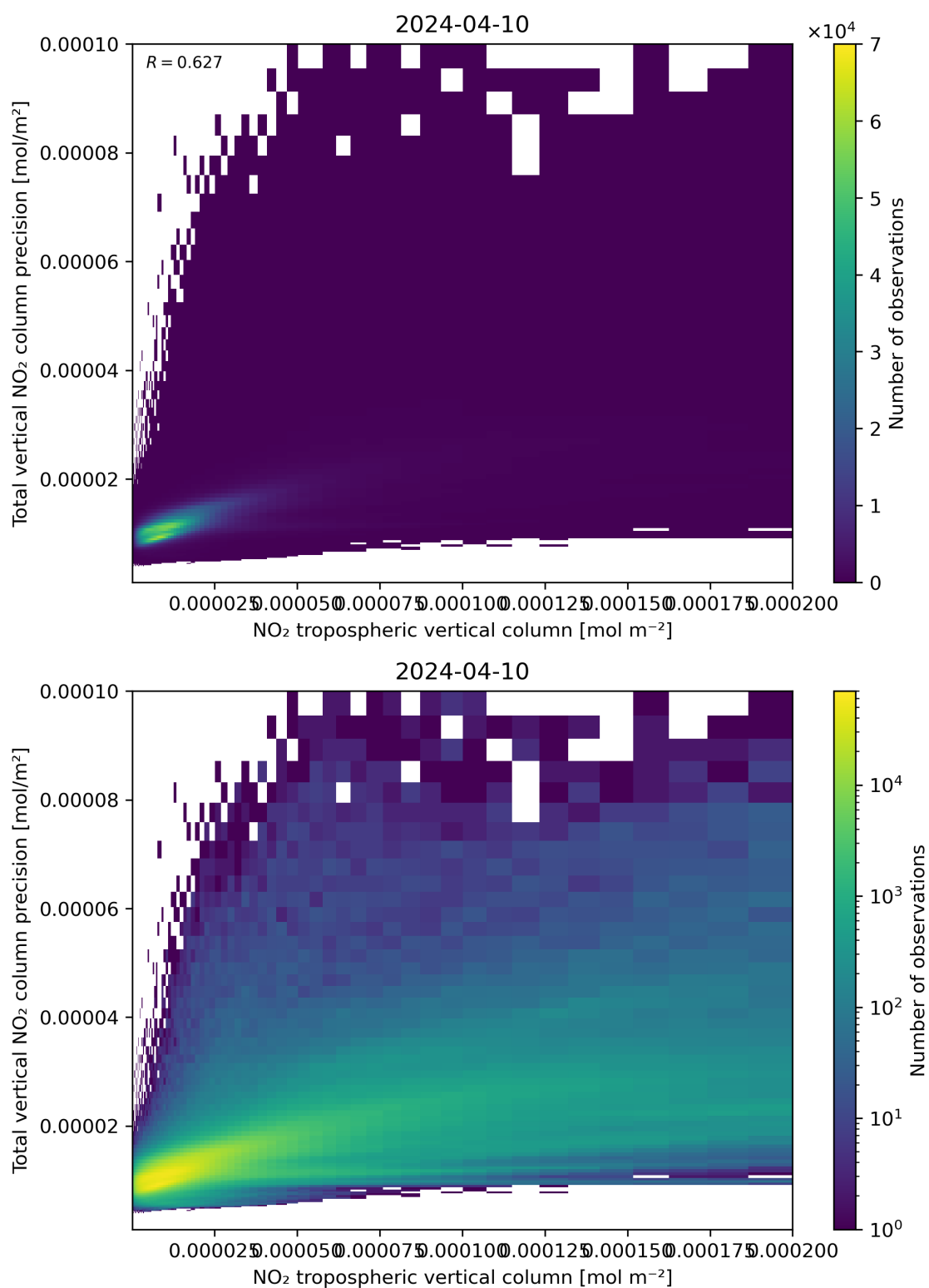
Figure 129: Scatter density plot of “NO 2 tropospheric vertical column” against “Total vertical NO 2 column precision” for 2024-04-10 to 2024-04-11.
