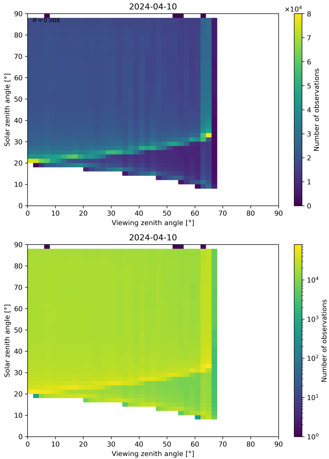
Figure 172: Scatter density plot of “Viewing zenith angle” against “Solar zenith angle” for 2024-04-10 to 2024-04-11.
