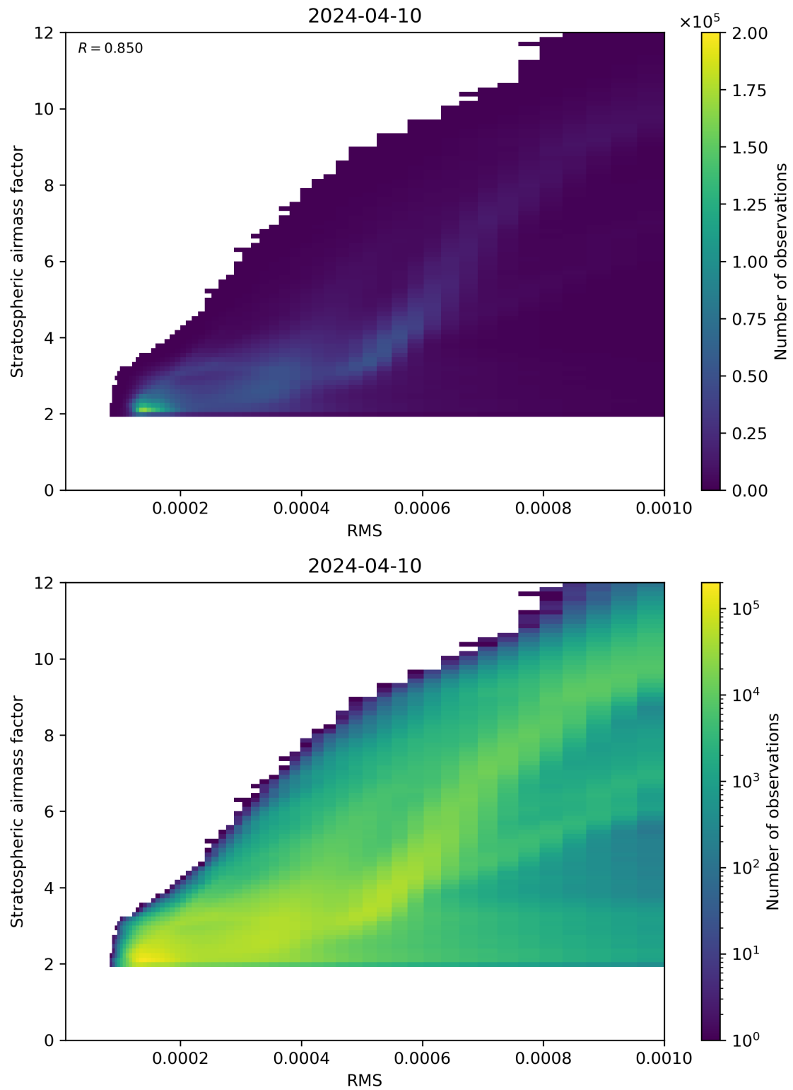
Figure 144: Scatter density plot of “RMS” against “Stratospheric airmass factor” for 2024-04-10 to 2024-04-11.
