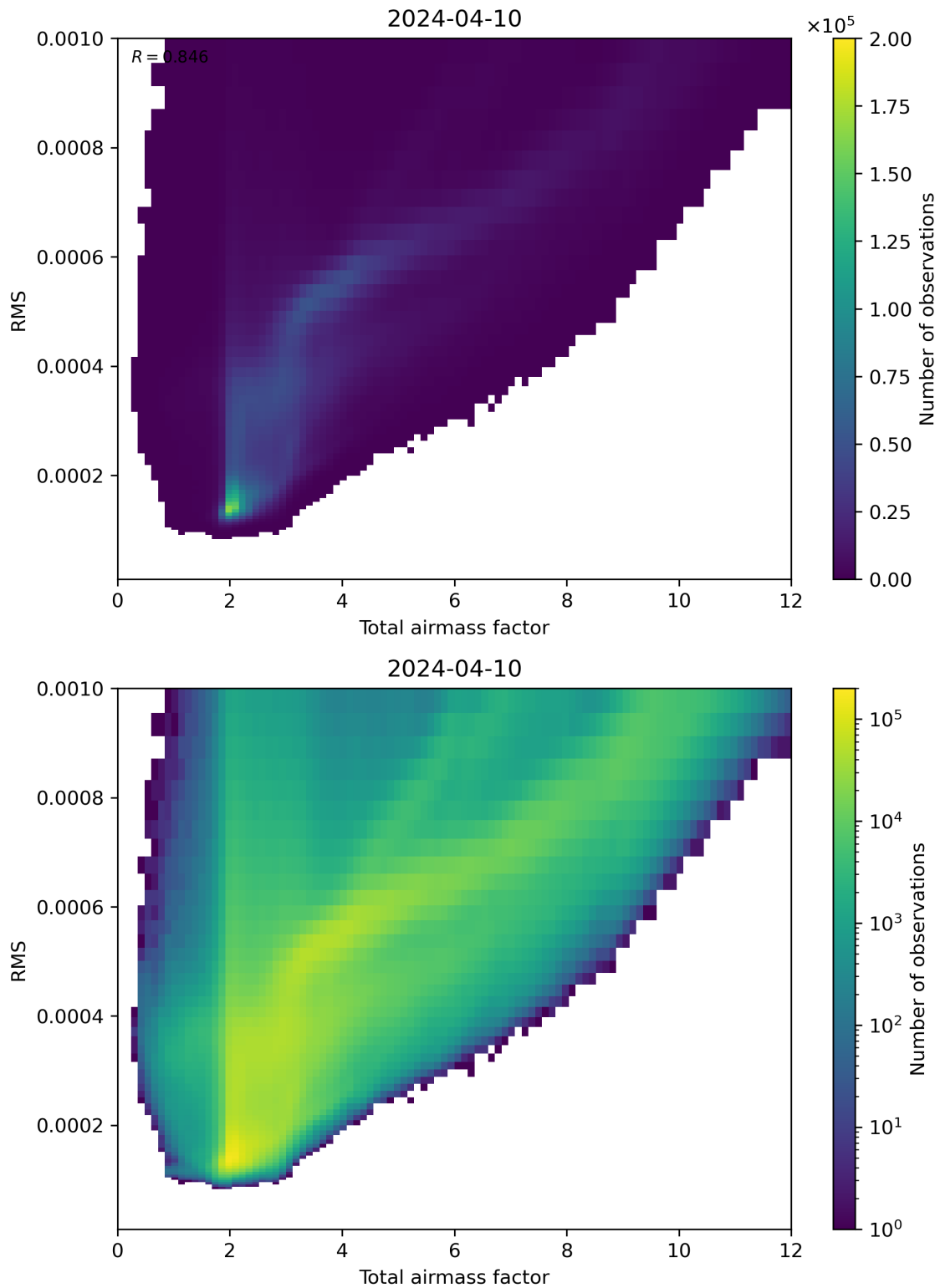
Figure 69: Scatter density plot of “Total airmass factor” against “RMS” for 2024-04-10 to 2024-04-11.
