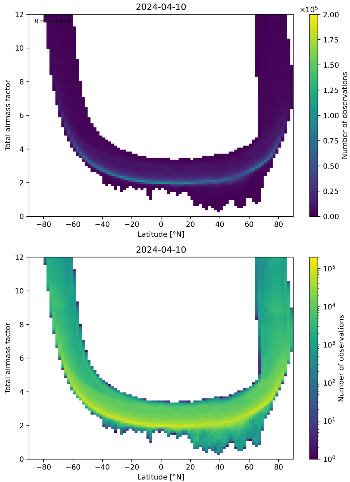
Figure 84: Scatter density plot of “Latitude” against “Total airmass factor” for 2024-04-10 to 2024-04-11.
