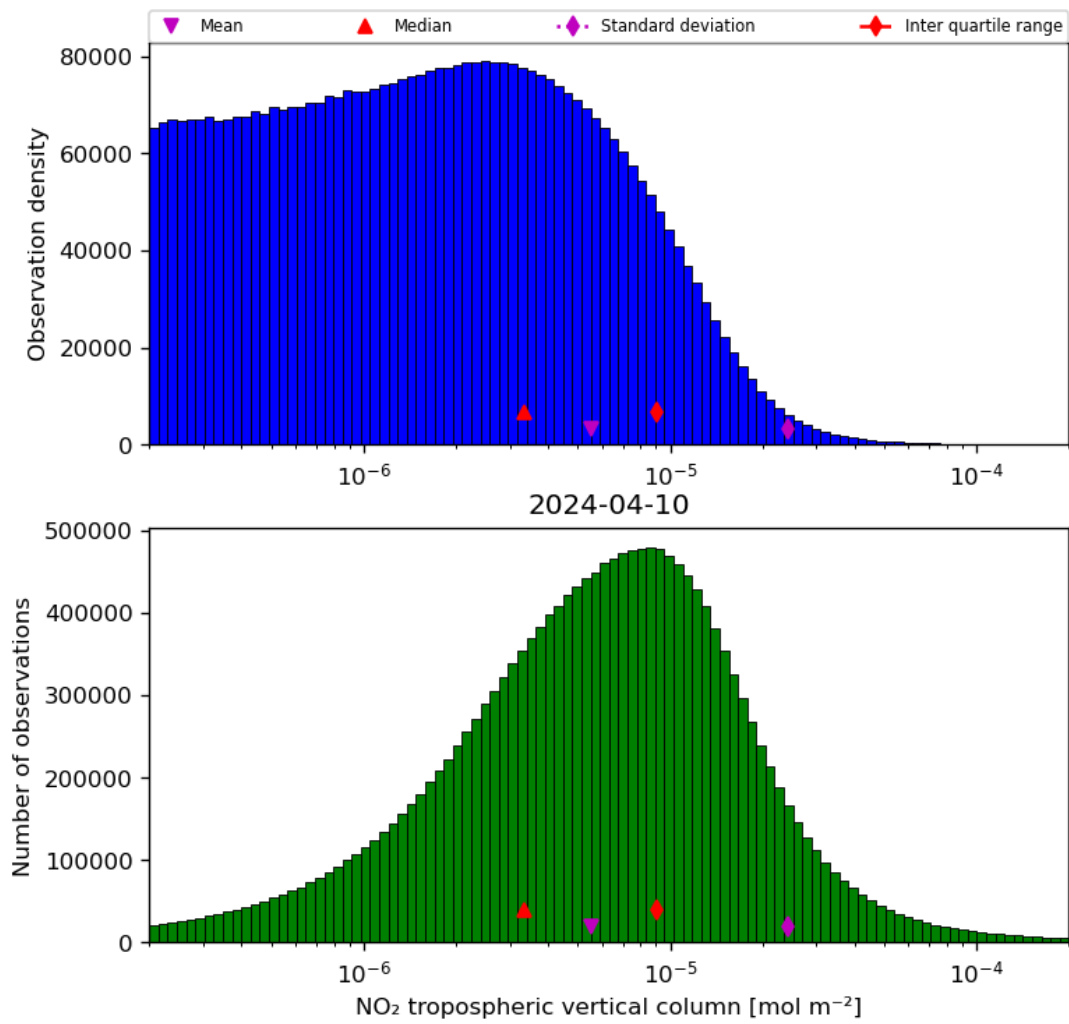
Figure 29: Histogram of “NO 2 tropospheric vertical column” for 2024-04-10 to 2024-04-11
