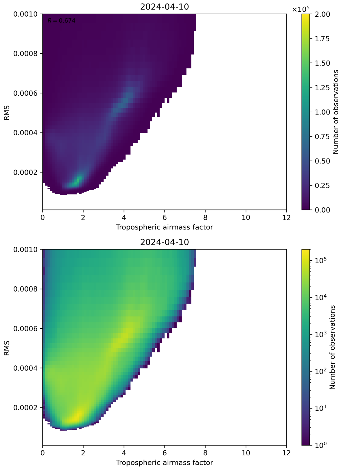
Figure 79: Scatter density plot of “Tropospheric airmass factor” against “RMS” for 2024-04-10 to 2024-04-11.
