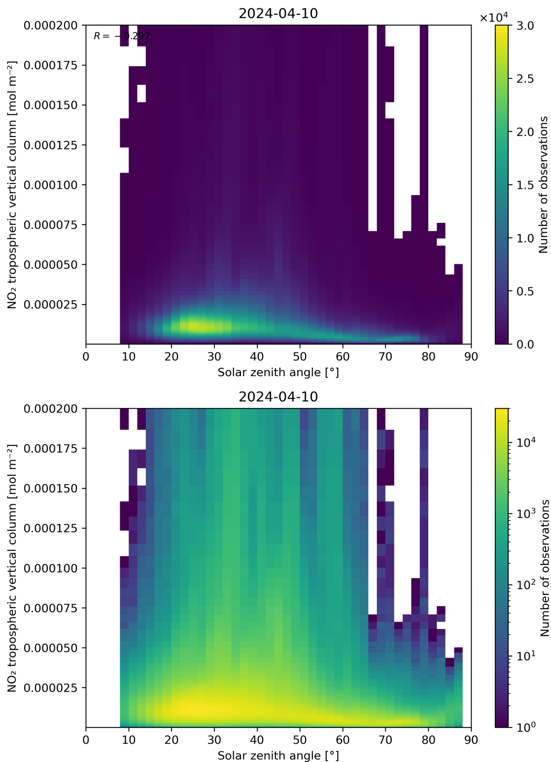
Figure 155: Scatter density plot of “Solar zenith angle” against “NO 2 tropospheric vertical column” for 2024-04-10 to 2024-04-11.
