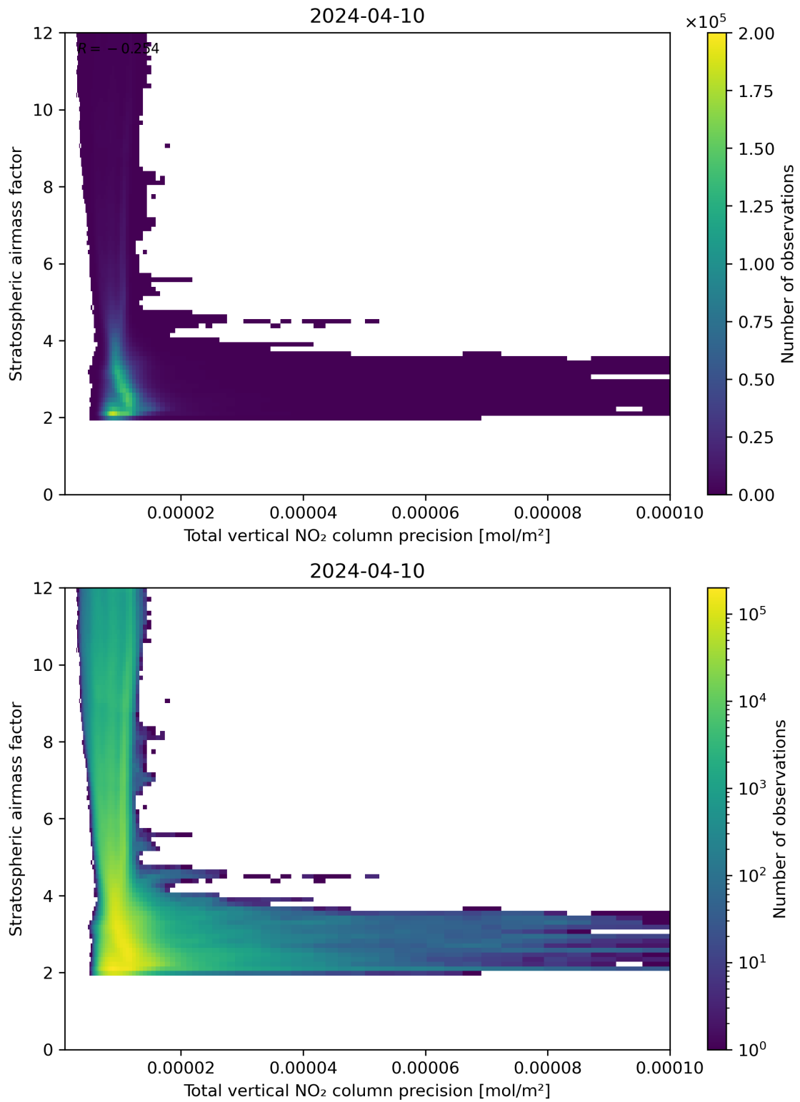
Figure 115: Scatter density plot of “Total vertical NO 2 column precision” against “Stratospheric air mass factor” for 2024-04-10 to 2024-04-11.
