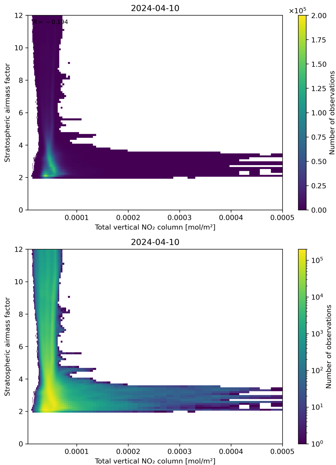
Figure 110: Scatter density plot of “Total vertical NO 2 column” against “Stratospheric airmass factor” for 2024-04-10 to 2024-04-11.
