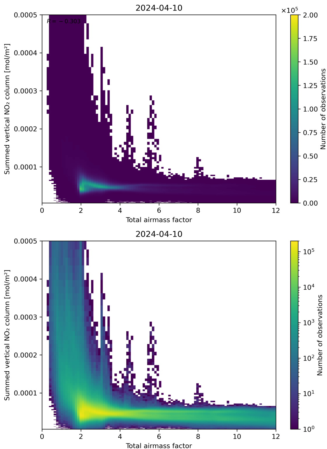
Figure 65: Scatter density plot of “Total airmass factor” against “Summed vertical NO 2 column” for 2024-04-10 to 2024-04-11.
