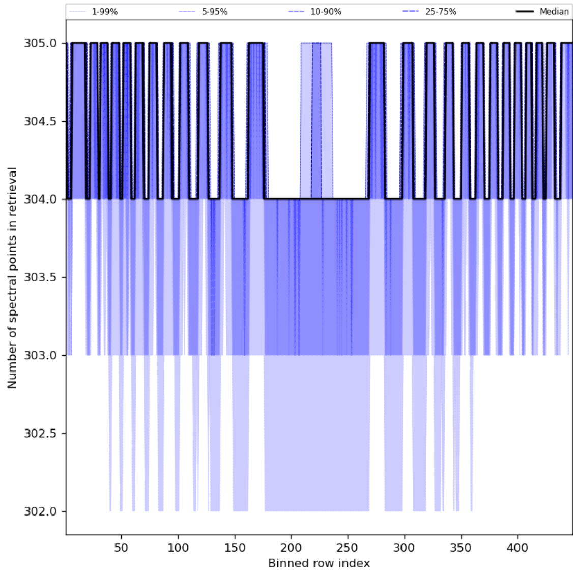
Figure 50: Along track statistics of “Number of spectral points in retrieval” for 2024-04-10 to 2024-04-11
