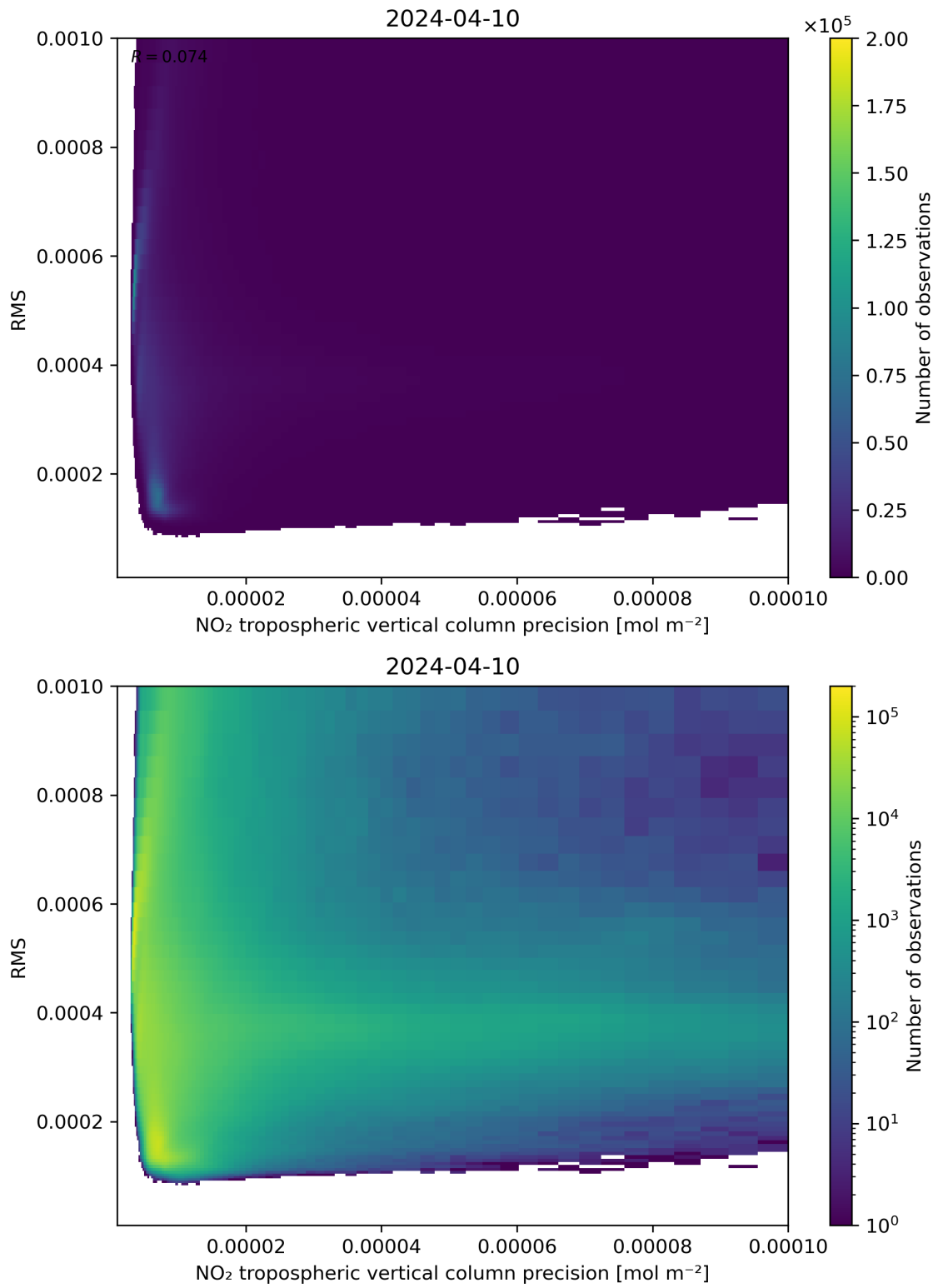
Figure 140: Scatter density plot of “NO 2 tropospheric vertical column precision” against “RMS” for 2024-04-10 to 2024-04-11.
