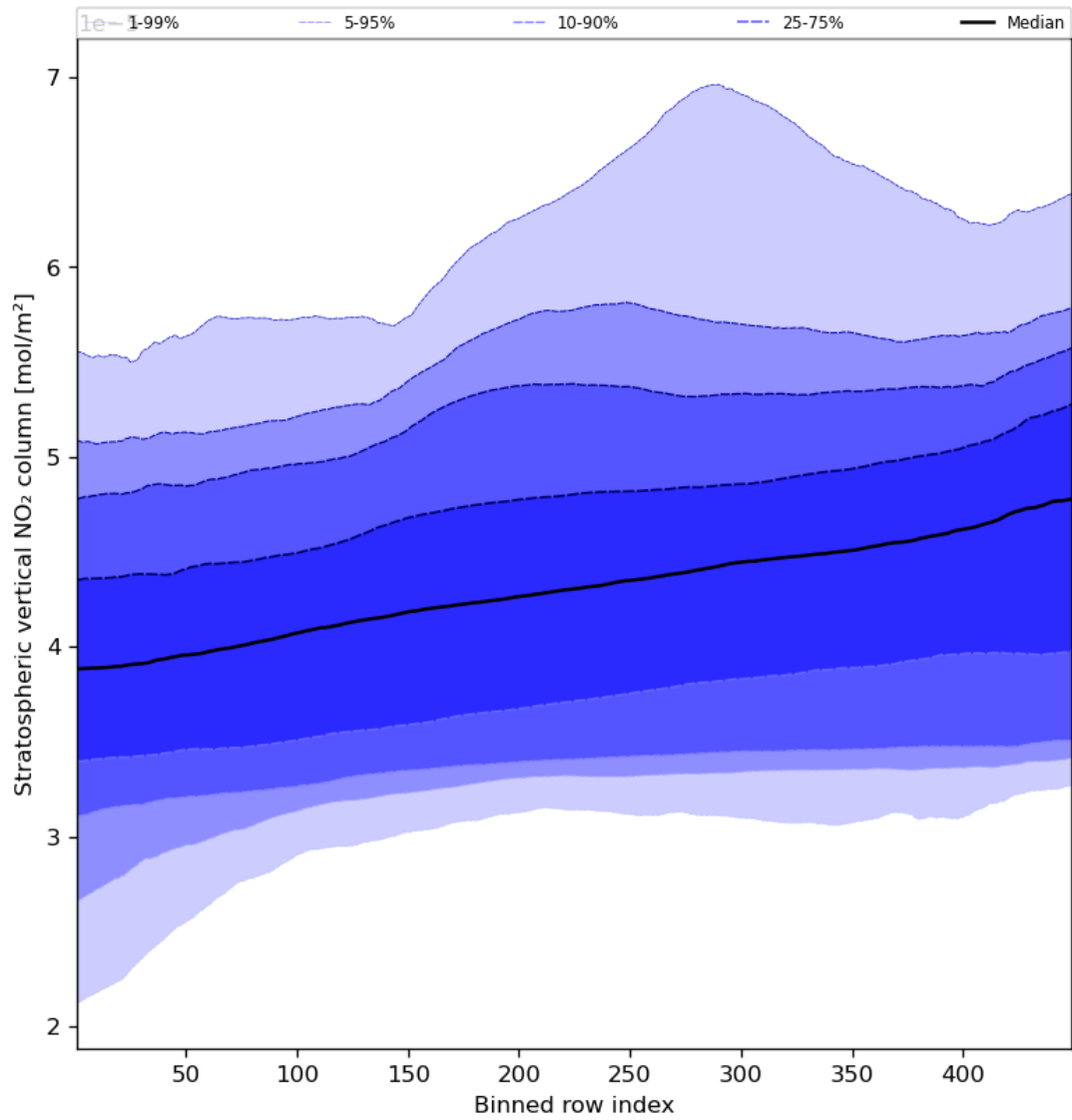
Figure 53: Along track statistics of “Stratospheric vertical NO 2 column” for 2024-04-10 to 2024-04-11
