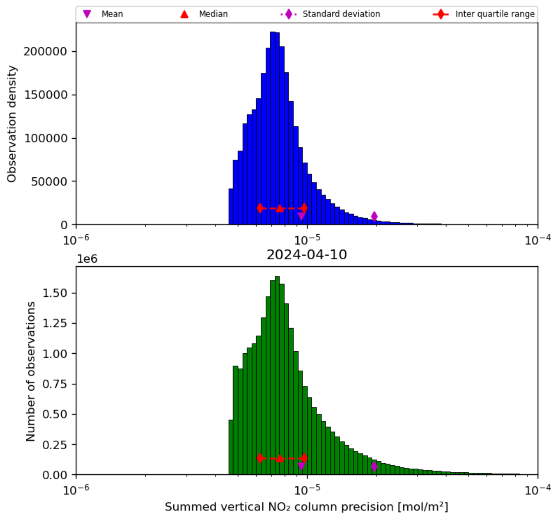
Figure 41: Histogram of “Summed vertical NO 2 column precision” for 2024-04-10 to 2024-04-11
