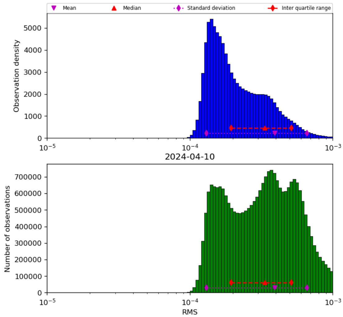
Figure 43: Histogram of “RMS” for 2024-04-10 to 2024-04-11
