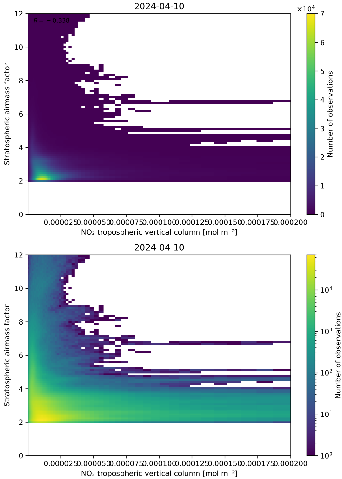
Figure 121: Scatter density plot of “NO 2 tropospheric vertical column” against “Stratospheric air mass factor” for 2024-04-10 to 2024-04-11.
