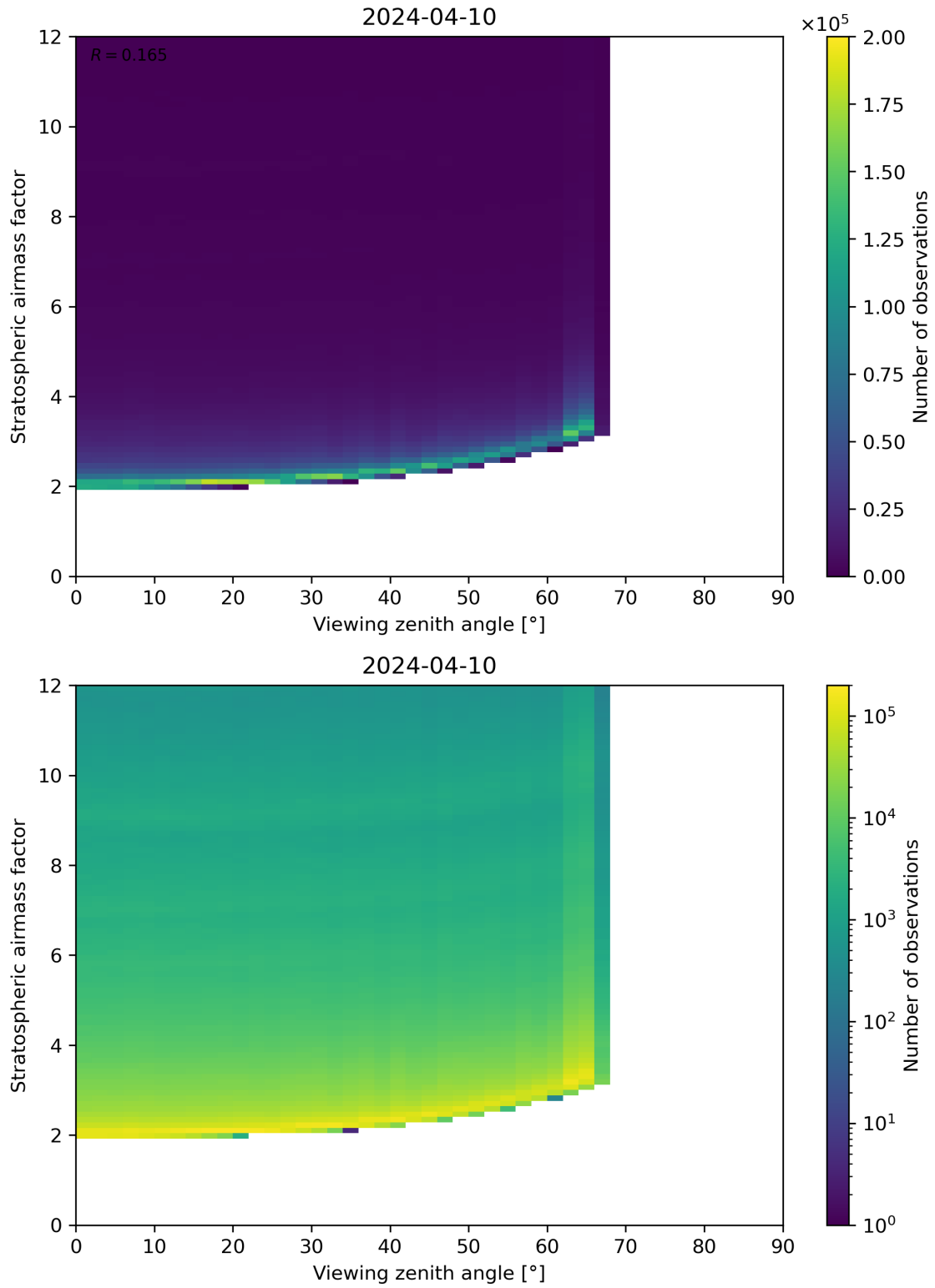
Figure 159: Scatter density plot of “Viewing zenith angle” against “Stratospheric airmass factor” for 2024-04-10 to 2024-04-11.
