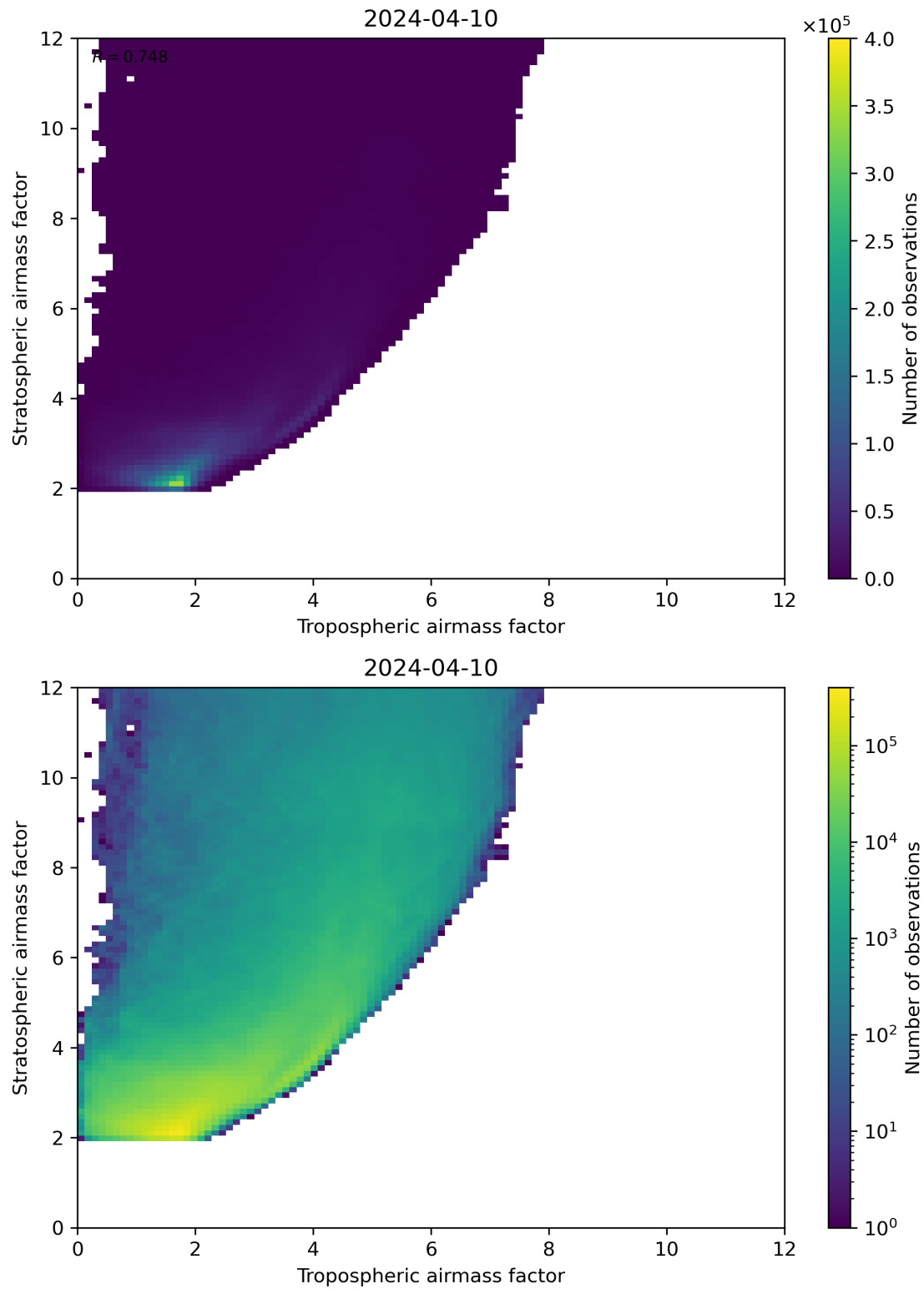
Figure 71: Scatter density plot of “Tropospheric airmass factor” against “Stratospheric airmass factor” for 2024-04-10 to 2024-04-11.
