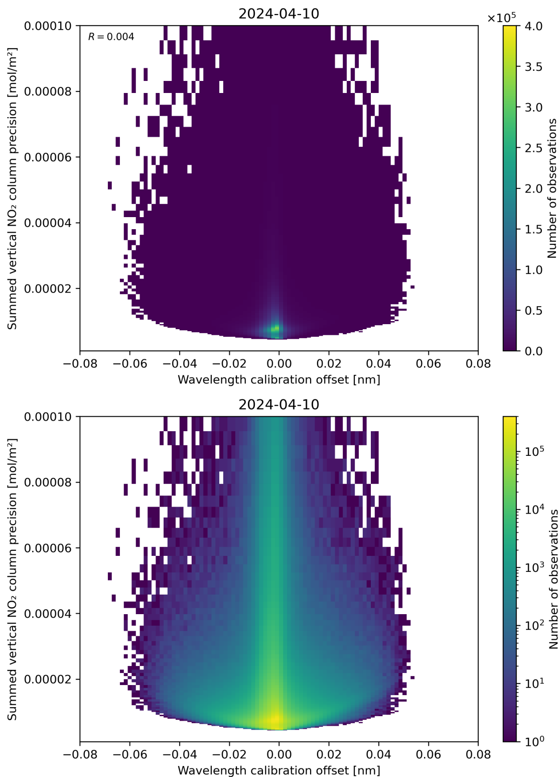
Figure 178: Scatter density plot of “Wavelength calibration offset” against “Summed vertical NO 2 column precision” for 2024-04-10 to 2024-04-11.
