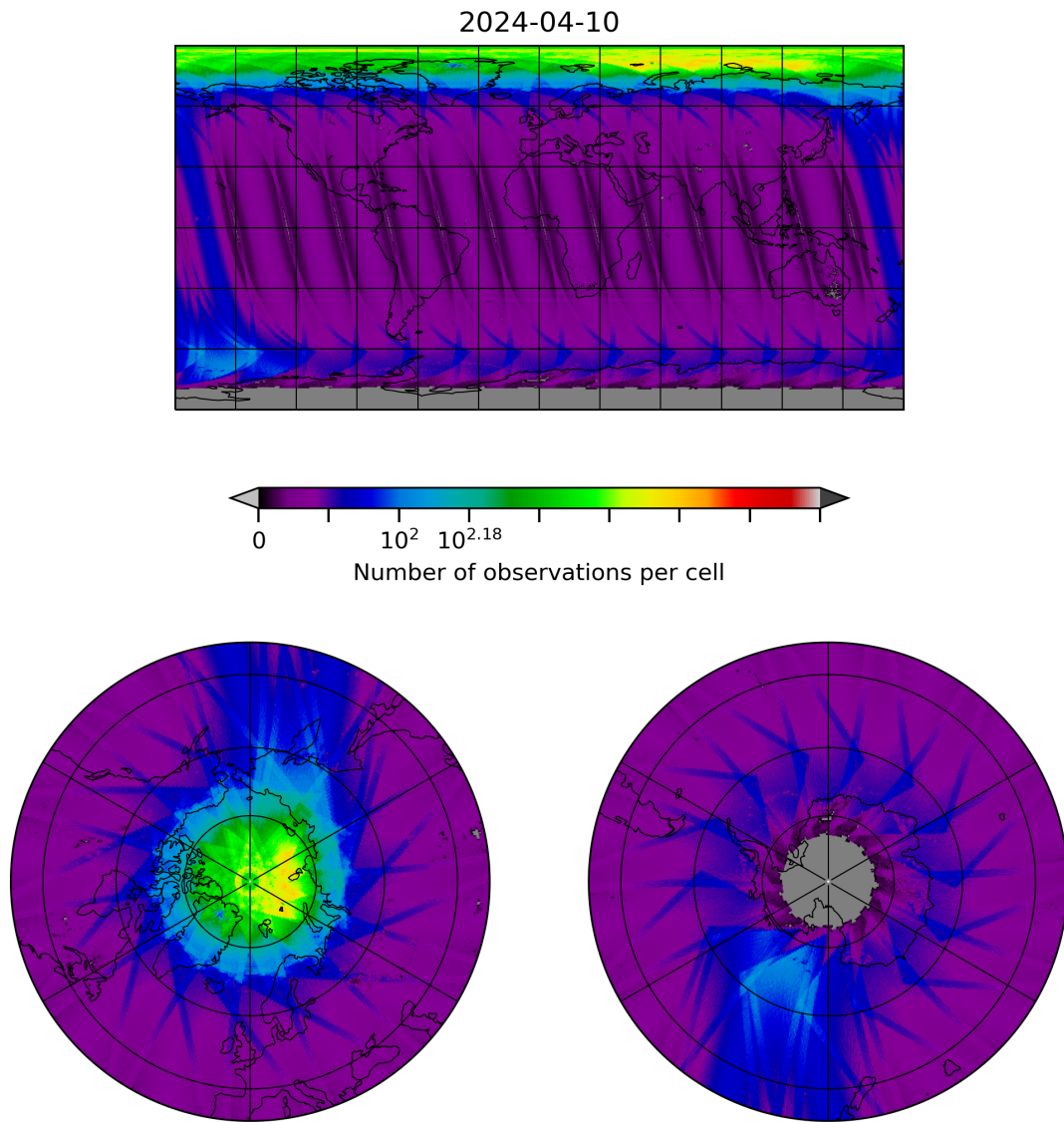
Figure 10: Map of the number of observations for 2024-04-10 to 2024-04-11
