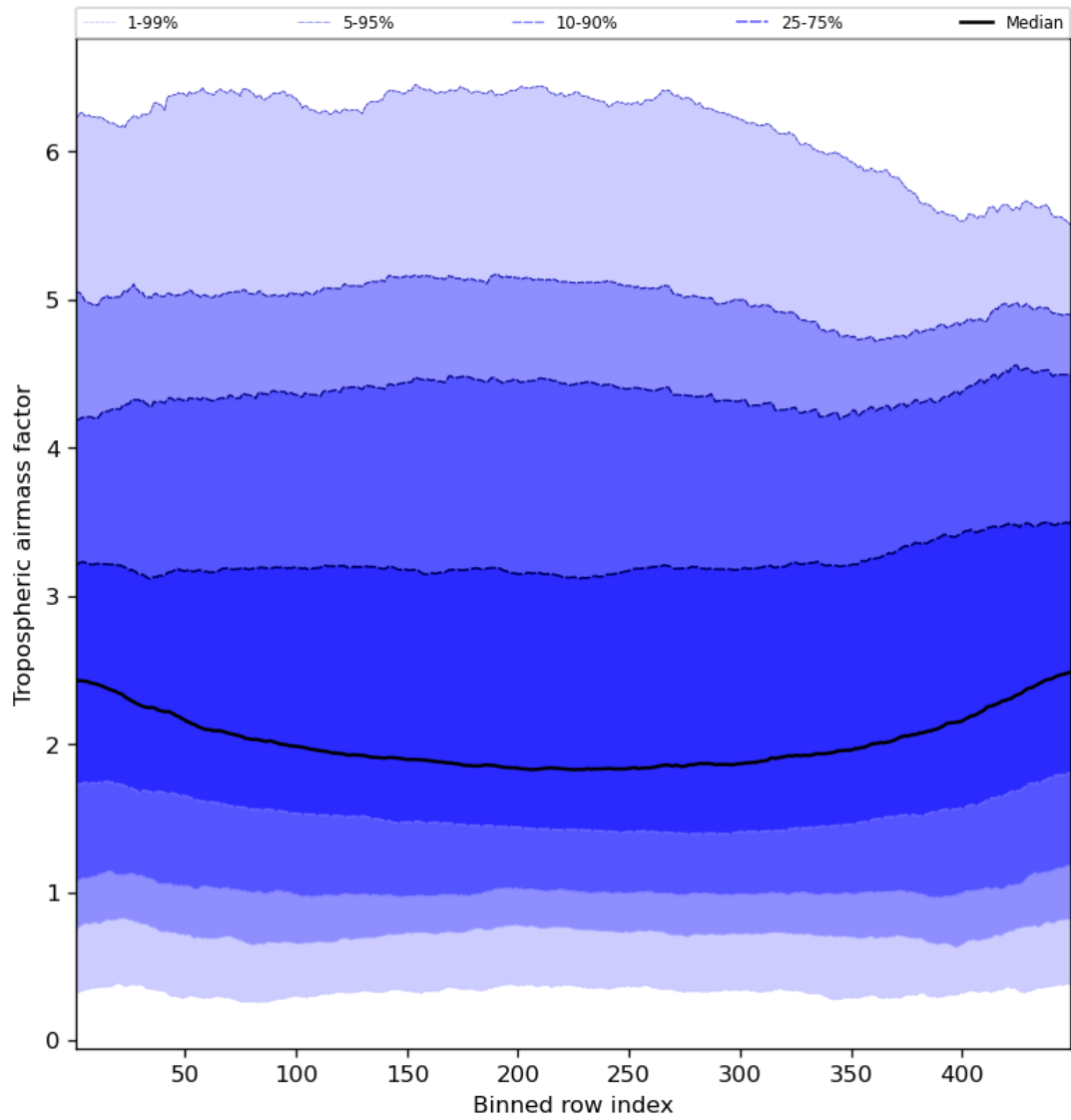
Figure 48: Along track statistics of “Tropospheric airmass factor” for 2024-04-10 to 2024-04-11
