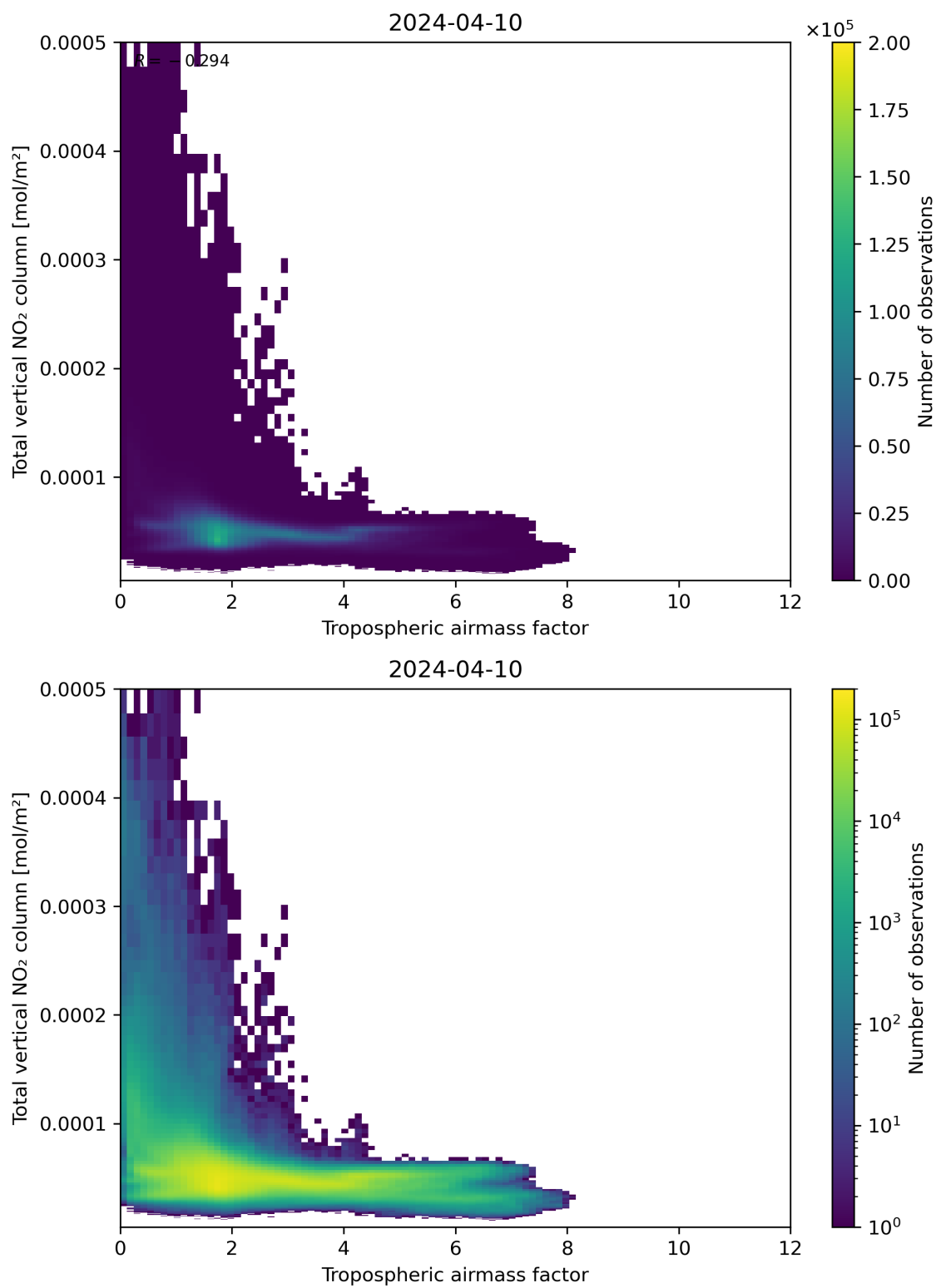
Figure 77: Scatter density plot of “Tropospheric airmass factor” against “Total vertical NO 2 column” for 2024-04-10 to 2024-04-11.
