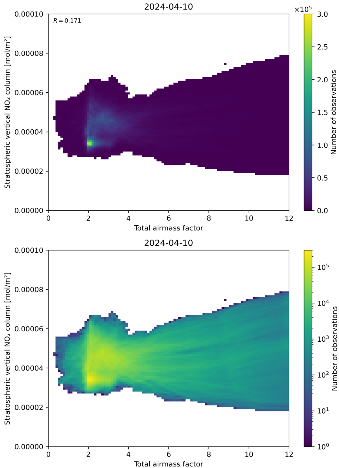
Figure 64: Scatter density plot of “Total airmass factor” against “Stratospheric vertical \text{NO}_2 column” for 2024-04-10 to 2024-04-11.
