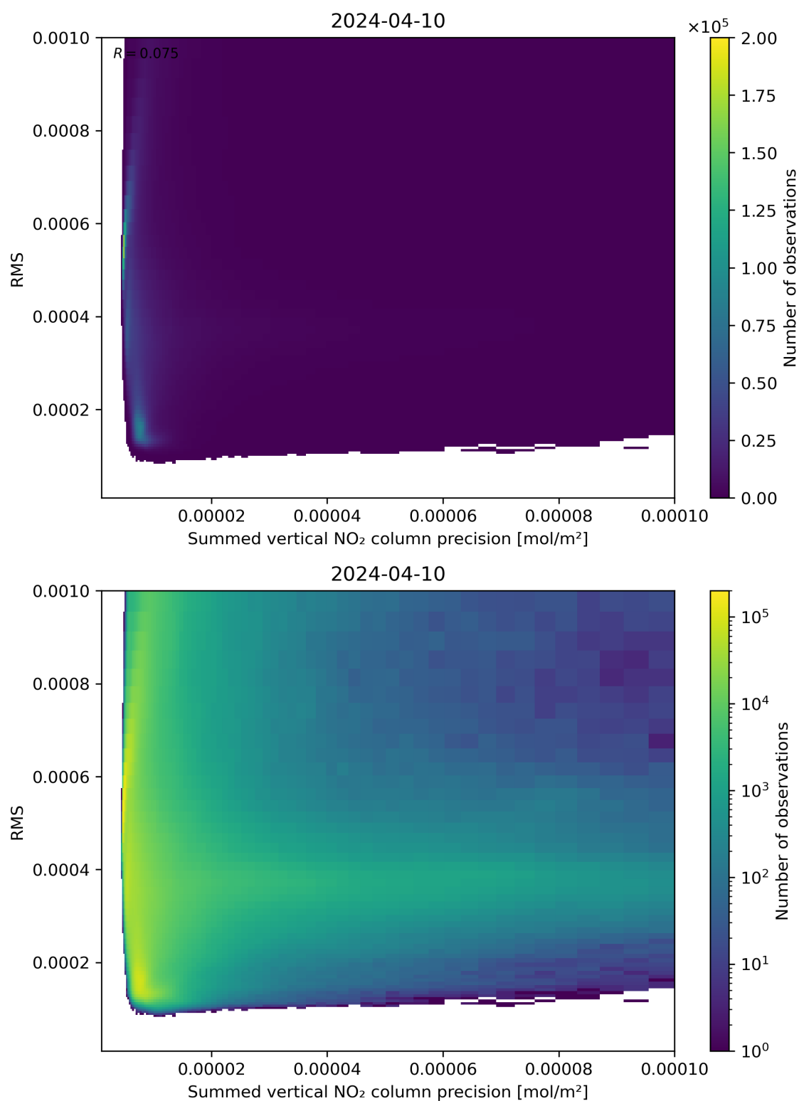
Figure 108: Scatter density plot of “Summed vertical NO 2 column precision” against “RMS” for 2024-04-10 to 2024-04-11.
