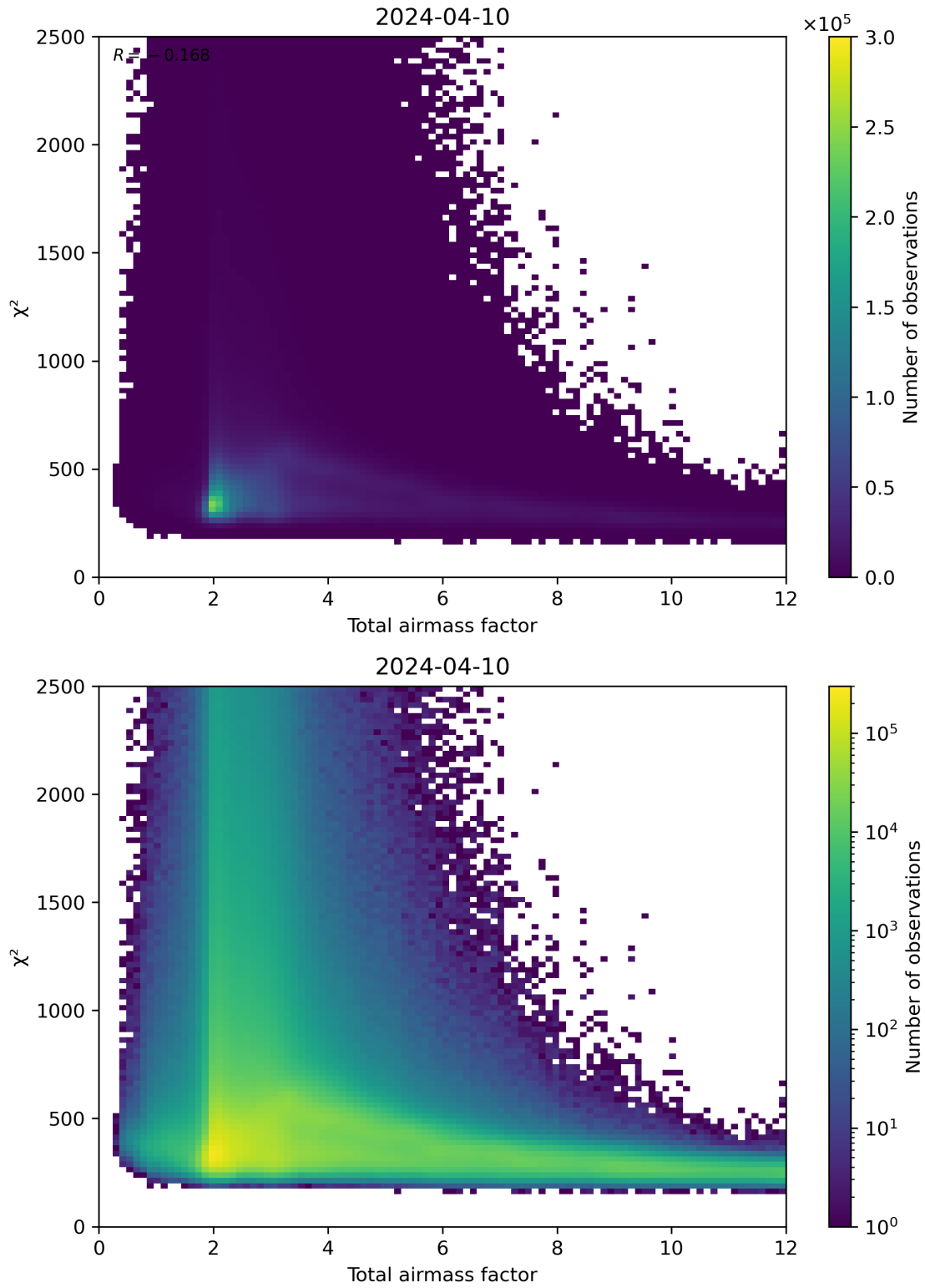
Figure 63: Scatter density plot of “Total airmass factor” against “ \chi^2 ” for 2024-04-10 to 2024-04-11.
