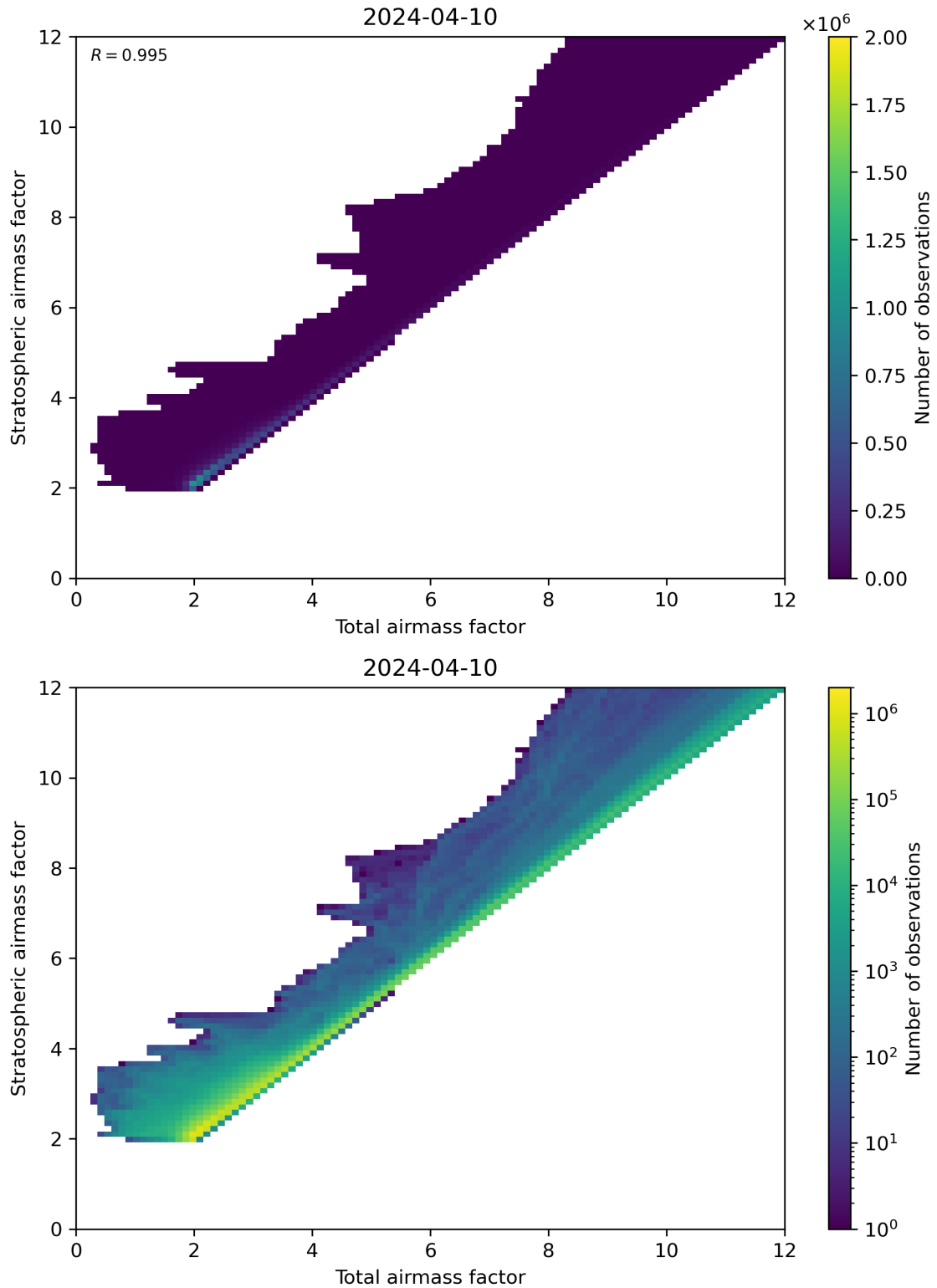
Figure 62: Scatter density plot of “Total airmass factor” against “Stratospheric airmass factor” for 2024-04-10 to 2024-04-11.
