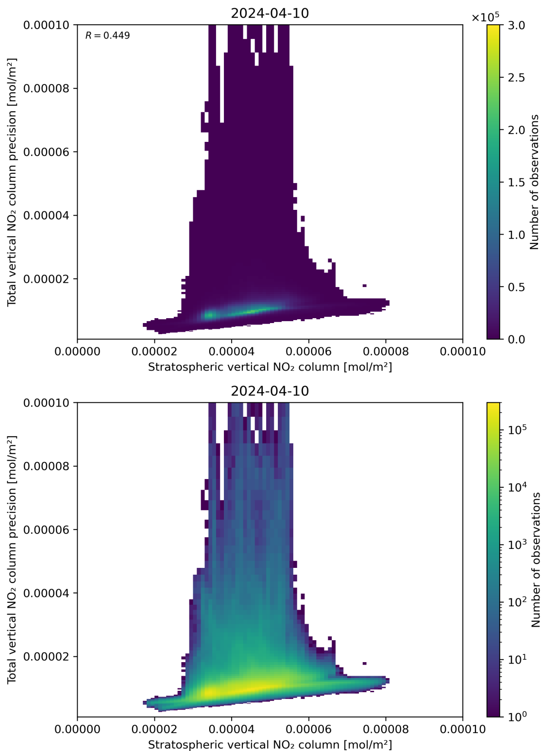
Figure 101: Scatter density plot of “Stratospheric vertical NO 2 column” against “Total vertical NO 2 column precision” for 2024-04-10 to 2024-04-11.
