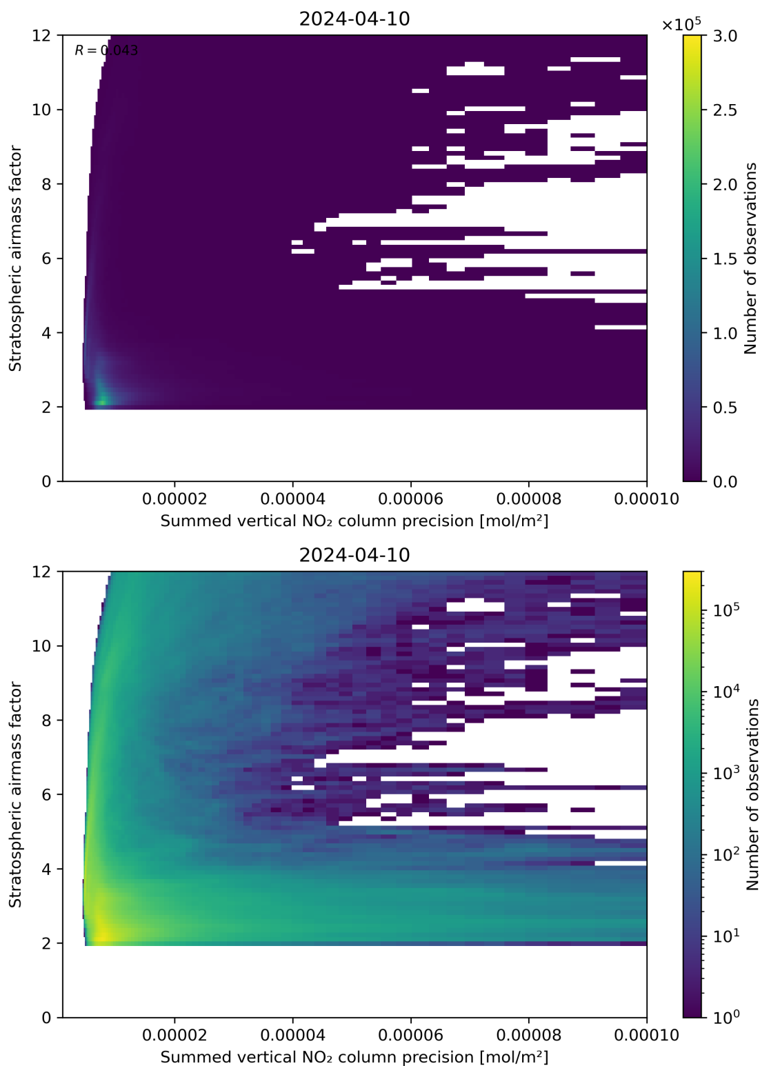
Figure 106: Scatter density plot of “Summed vertical NO 2 column precision” against “Stratospheric airmass factor” for 2024-04-10 to 2024-04-11.
