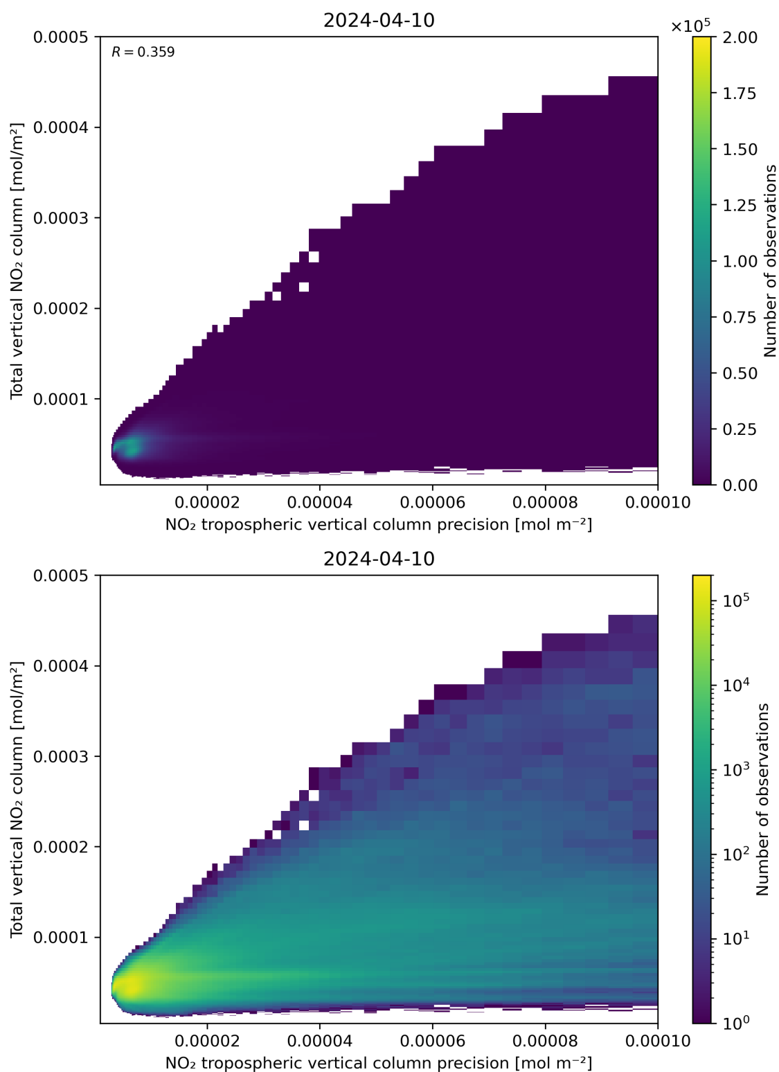
Figure 138: Scatter density plot of “NO 2 tropospheric vertical column precision” against “Total vertical NO 2 column” for 2024-04-10 to 2024-04-11.
