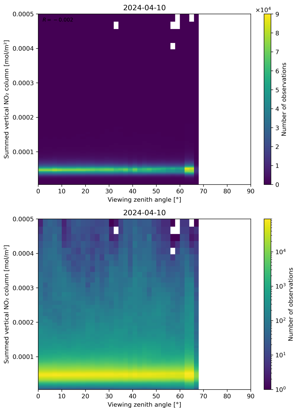
Figure 165: Scatter density plot of “Viewing zenith angle” against “Summed vertical NO 2 column” for 2024-04-10 to 2024-04-11.
