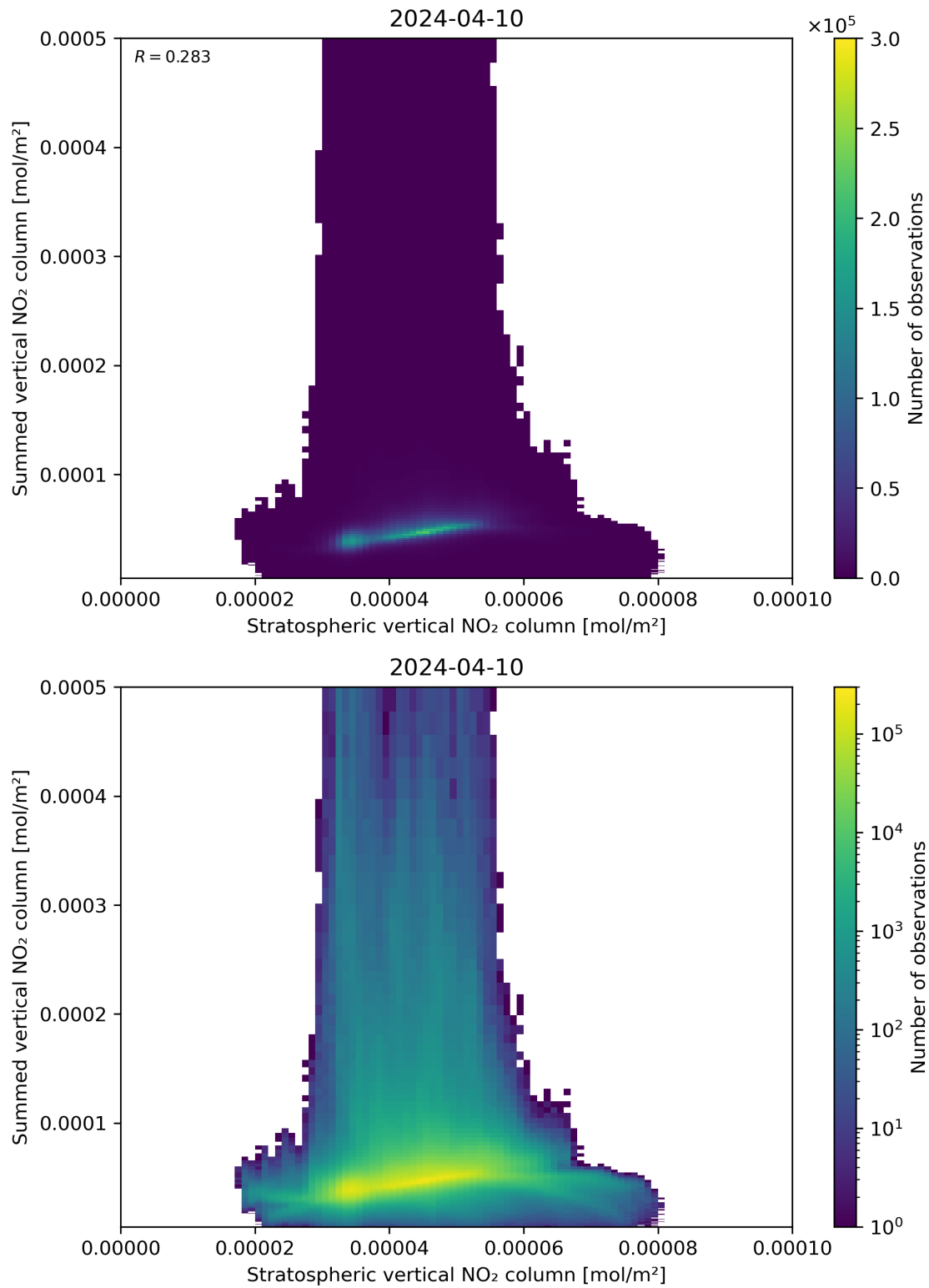
Figure 98: Scatter density plot of “Stratospheric vertical NO 2 column” against “Summed vertical NO 2 column” for 2024-04-10 to 2024-04-11.
