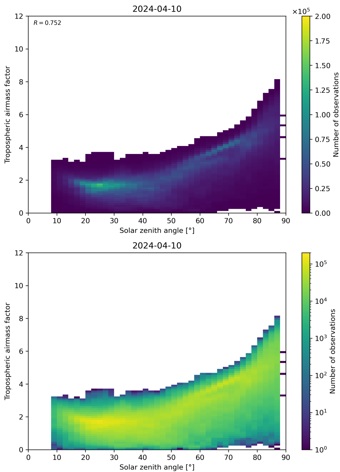
Figure 147: Scatter density plot of “Solar zenith angle” against “Tropospheric airmass factor” for 2024-04-10 to 2024-04-11.
