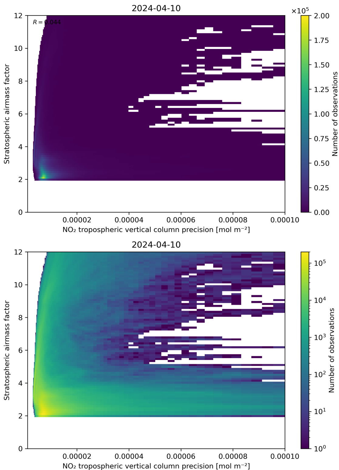
Figure 131: Scatter density plot of “NO 2 tropospheric vertical column precision” against “Stratospheric airmass factor” for 2024-04-10 to 2024-04-11.
