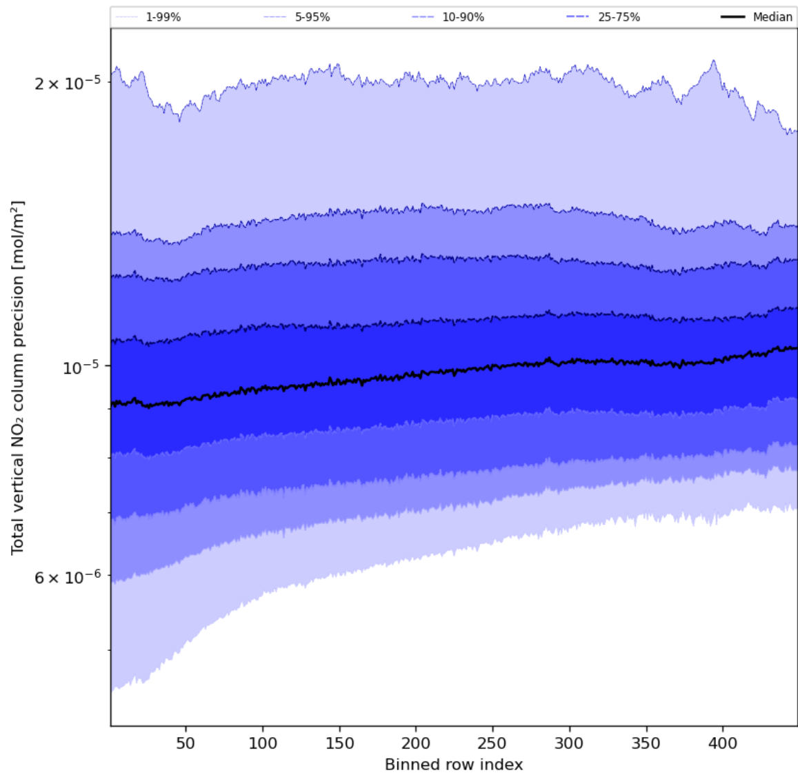
Figure 56: Along track statistics of “Total vertical NO 2 column precision” for 2024-04-10 to 2024-04-11
