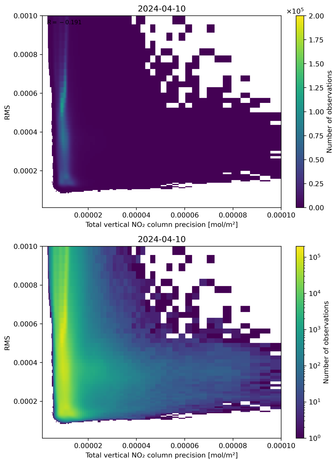
Figure 119: Scatter density plot of “Total vertical NO 2 column precision” against “RMS” for 2024-04-10 to 2024-04-11.
