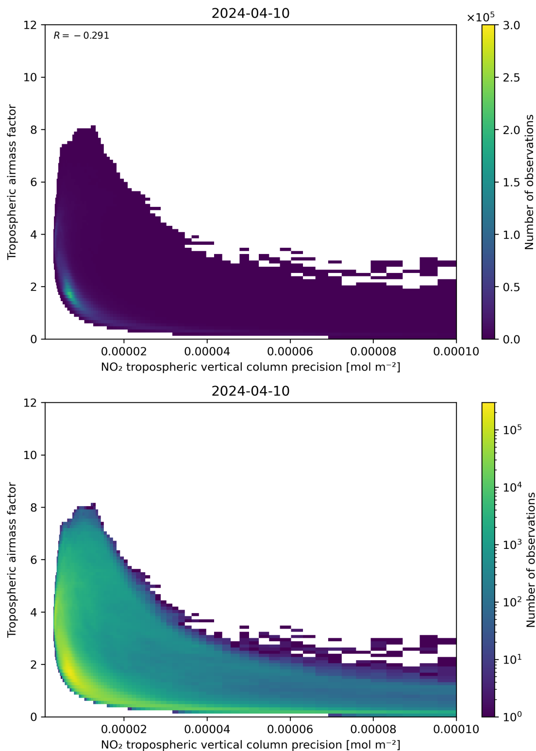
Figure 133: Scatter density plot of “NO 2 tropospheric vertical column precision” against “Tropospheric airmass factor” for 2024-04-10 to 2024-04-11.
