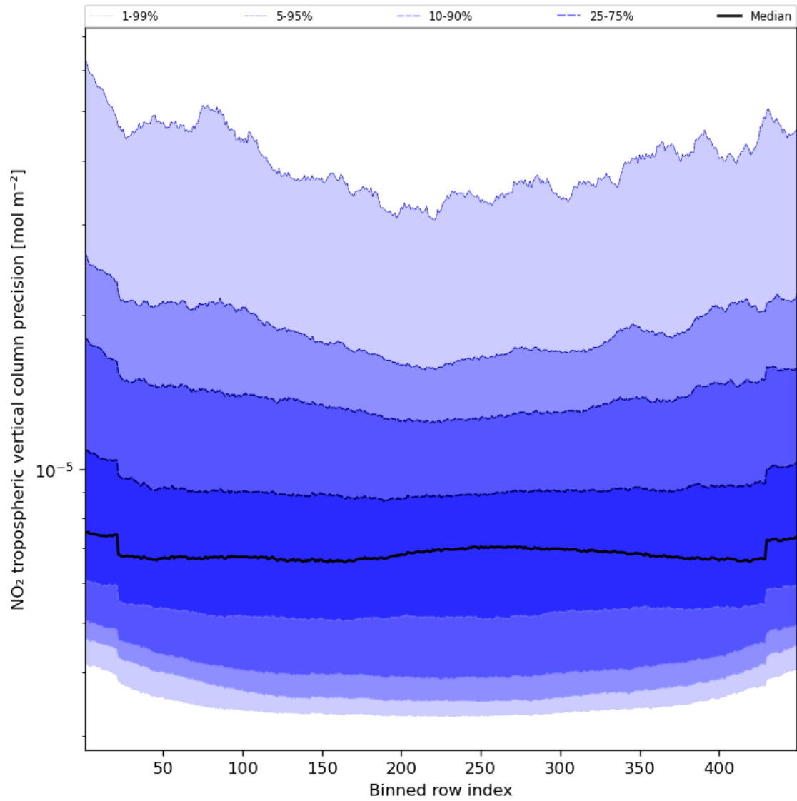
Figure 47: Along track statistics of “NO 2 tropospheric vertical column precision” for 2024-04-10 to 2024-04-11
