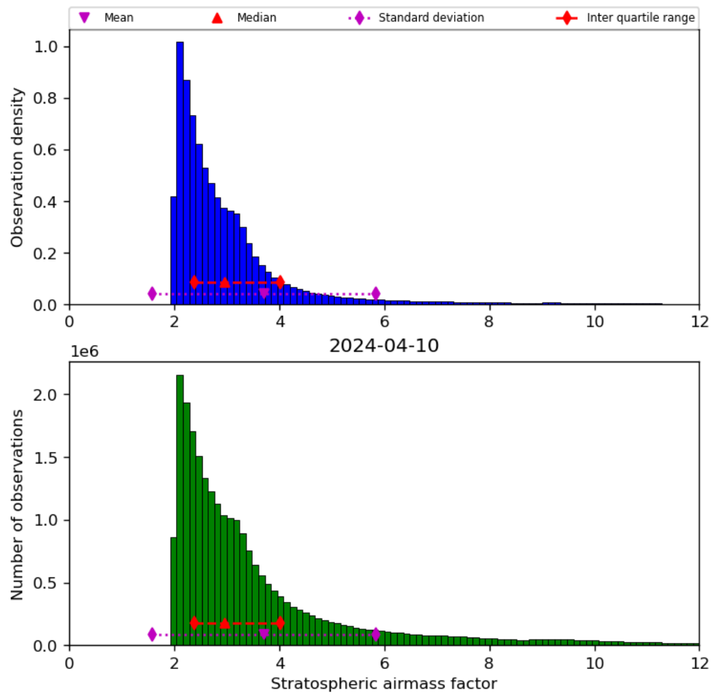
Figure 44: Histogram of “Stratospheric airmass factor” for 2024-04-10 to 2024-04-11
