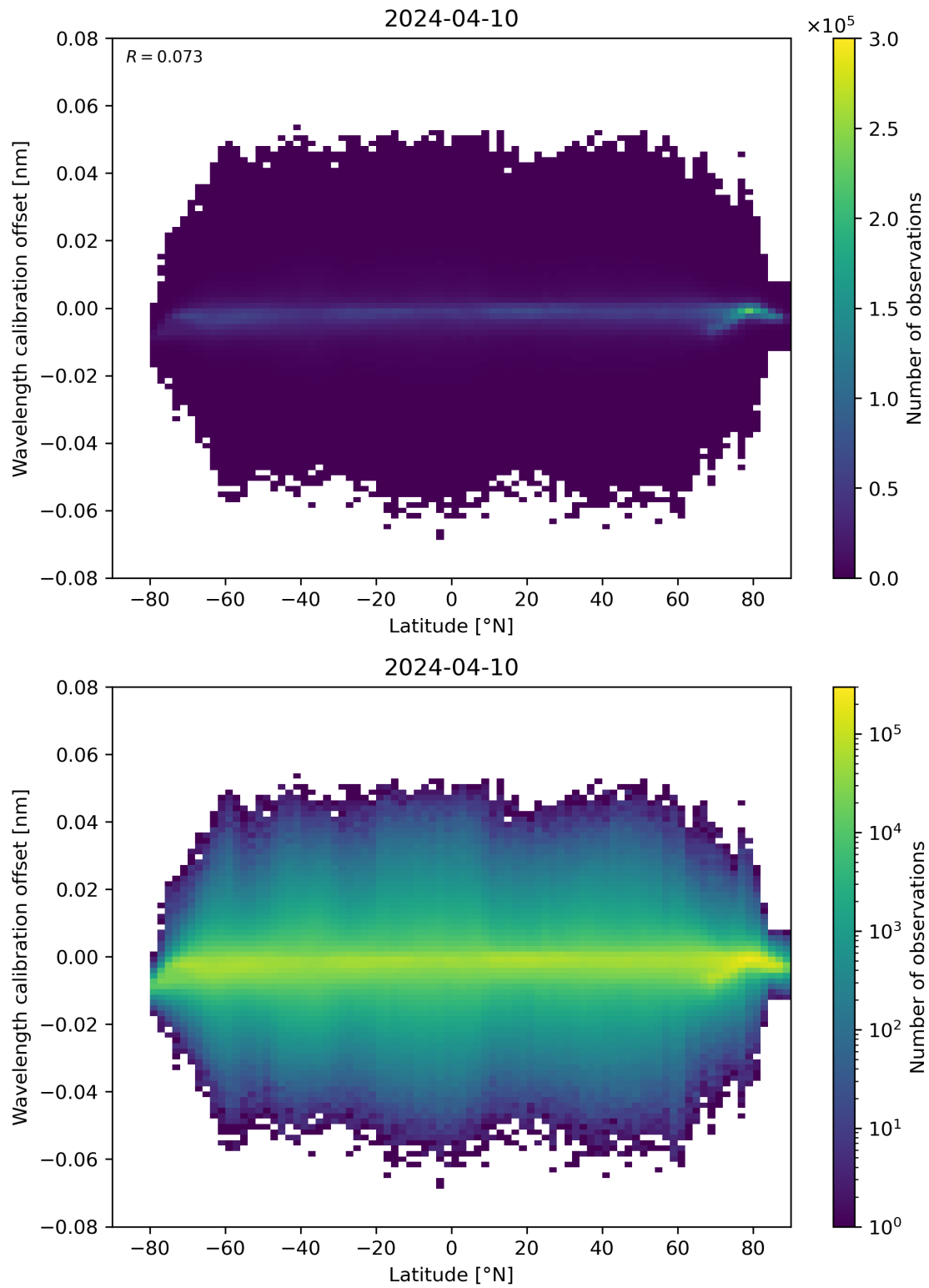
Figure 95: Scatter density plot of “Latitude” against “Wavelength calibration offset” for 2024-04-10 to 2024-04-11.
