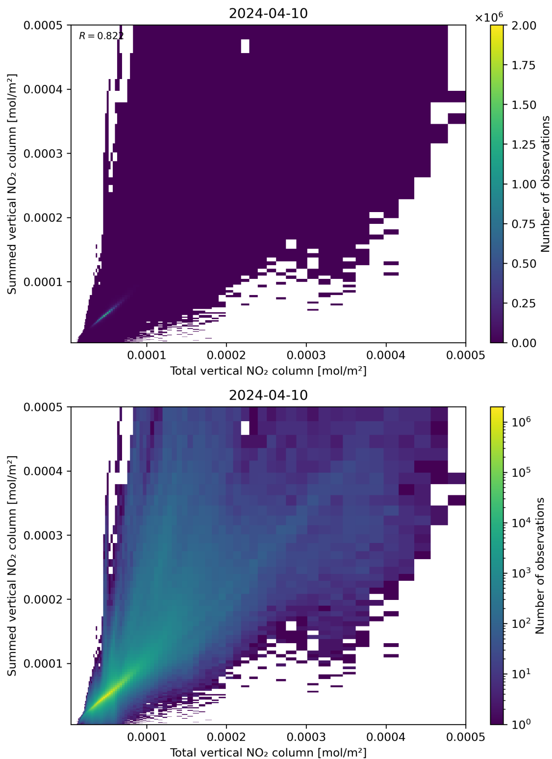
Figure 112: Scatter density plot of “Total vertical NO 2 column” against “Summed vertical NO 2 column” for 2024-04-10 to 2024-04-11.
