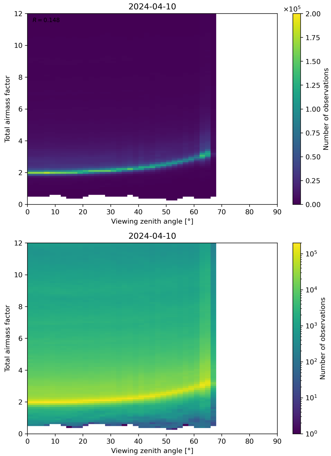
Figure 160: Scatter density plot of “Viewing zenith angle” against “Total airmass factor” for 2024-04-10 to 2024-04-11.
