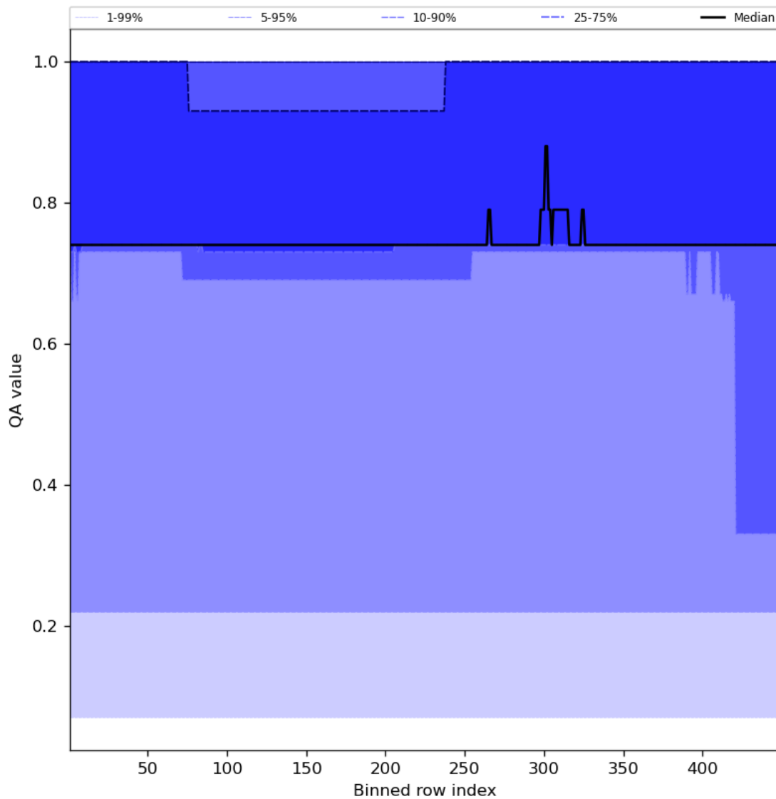
Figure 45: Along track statistics of “QA value” for 2024-04-10 to 2024-04-11
