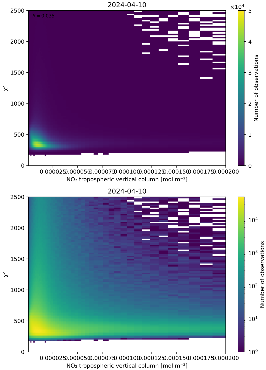
Figure 124: Scatter density plot of “NO 2 tropospheric vertical column” against “ \chi^2 ” for 2024-04-10 to 2024-04-11.
