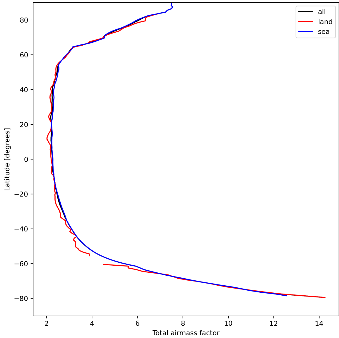
Figure 15: Zonal average of “Total airmass factor” for 2024-04-10 to 2024-04-11.
