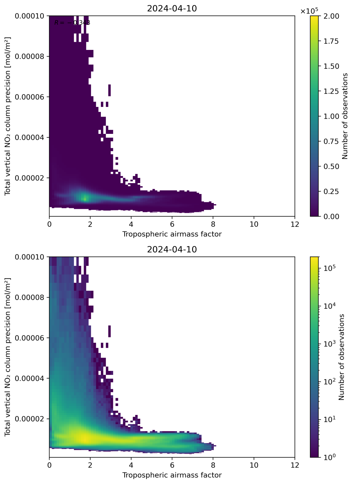
Figure 78: Scatter density plot of “Tropospheric air mass factor” against “Total vertical NO 2 column precision” for 2024-04-10 to 2024-04-11.
