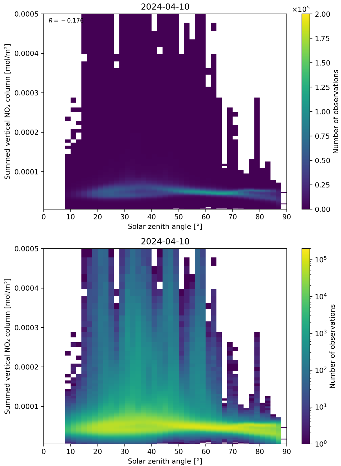
Figure 151: Scatter density plot of “Solar zenith angle” against “Summed vertical NO 2 column” for 2024-04-10 to 2024-04-11.
