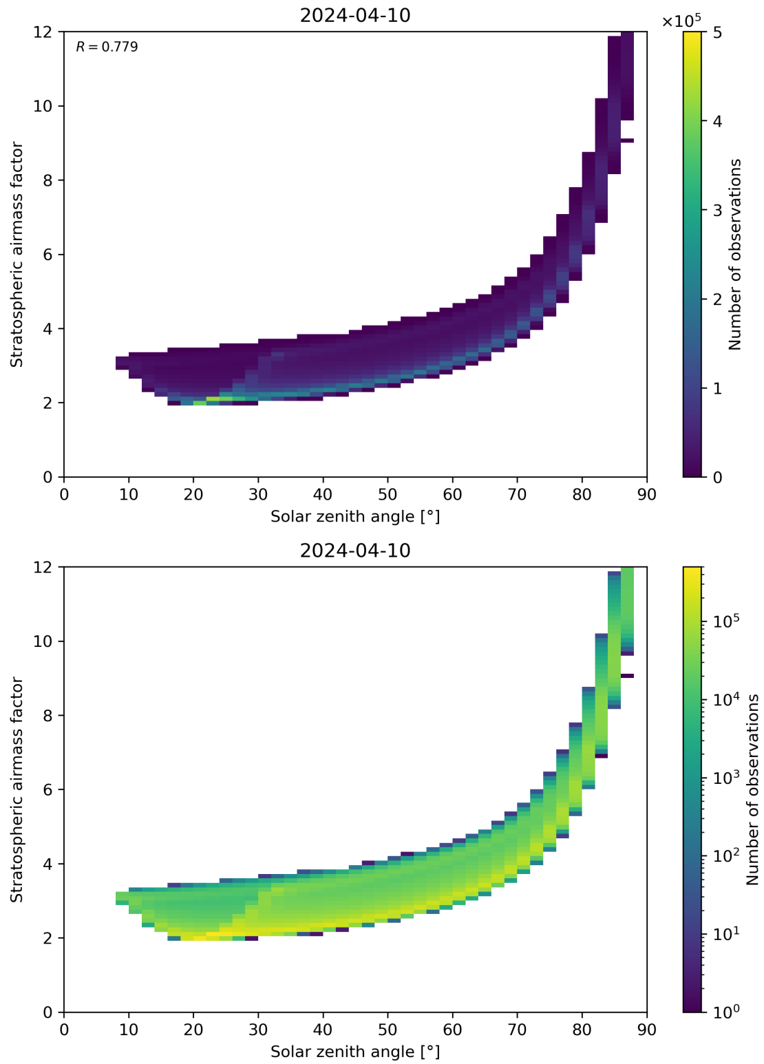
Figure 145: Scatter density plot of “Solar zenith angle” against “Stratospheric airmass factor” for 2024-04-10 to 2024-04-11.
