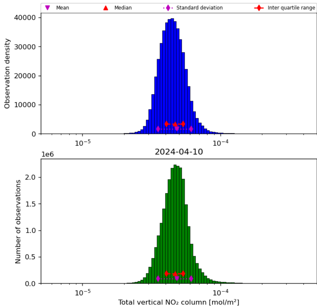
Figure 38: Histogram of "Total vertical NO 2 column" for 2024-04-10 to 2024-04-11
