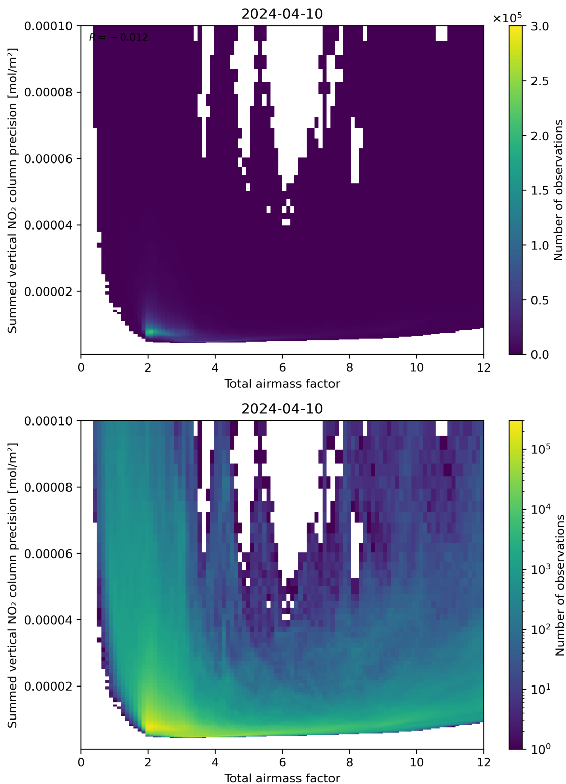
Figure 66: Scatter density plot of “Total airmass factor” against “Summed vertical NO 2 column precision” for 2024-04-10 to 2024-04-11.
