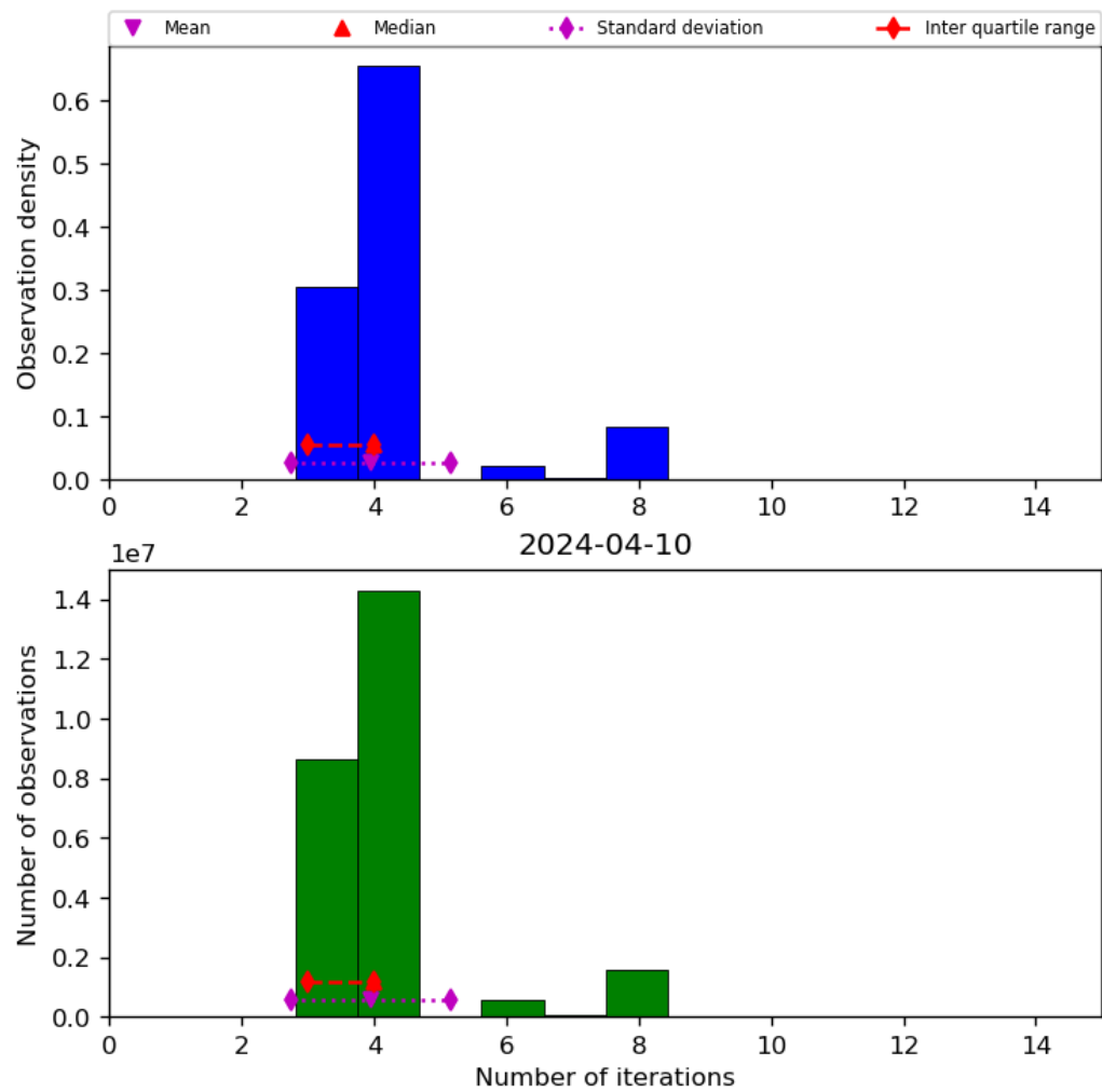
Figure 34: Histogram of “Number of iterations” for 2024-04-10 to 2024-04-11
