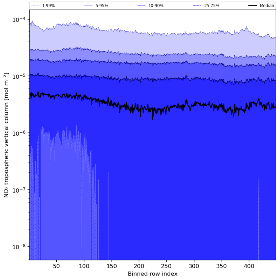
Figure 46: Along track statistics of “NO 2 tropospheric vertical column” for 2024-04-10 to 2024-04-11
