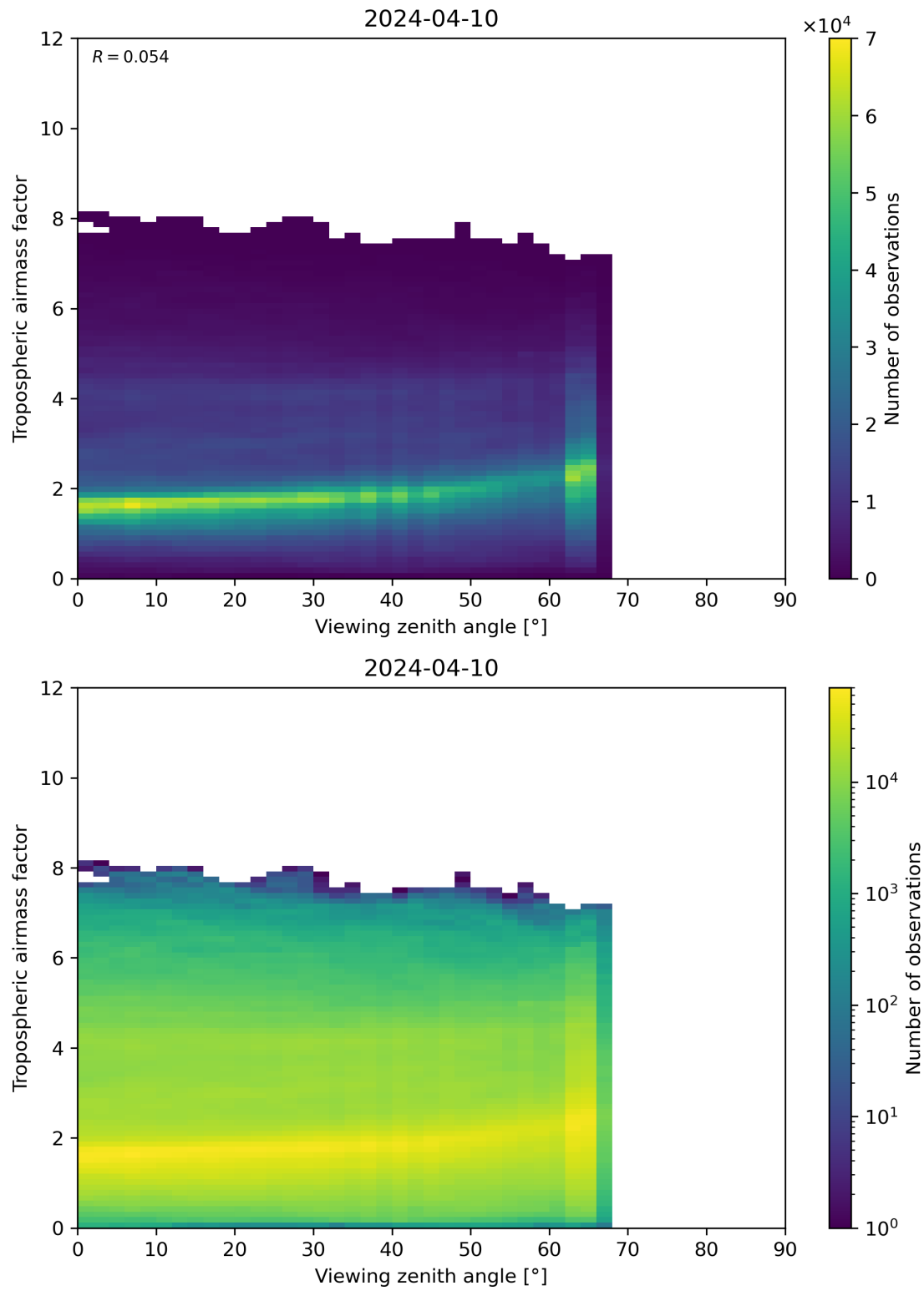
Figure 161: Scatter density plot of “Viewing zenith angle” against “Tropospheric airmass factor” for 2024-04-10 to 2024-04-11.
