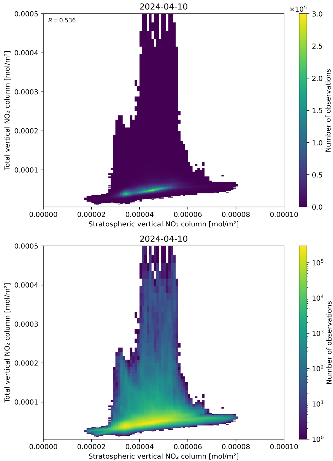
Figure 100: Scatter density plot of “Stratospheric vertical NO 2 column” against “Total vertical NO 2 column” for 2024-04-10 to 2024-04-11.
