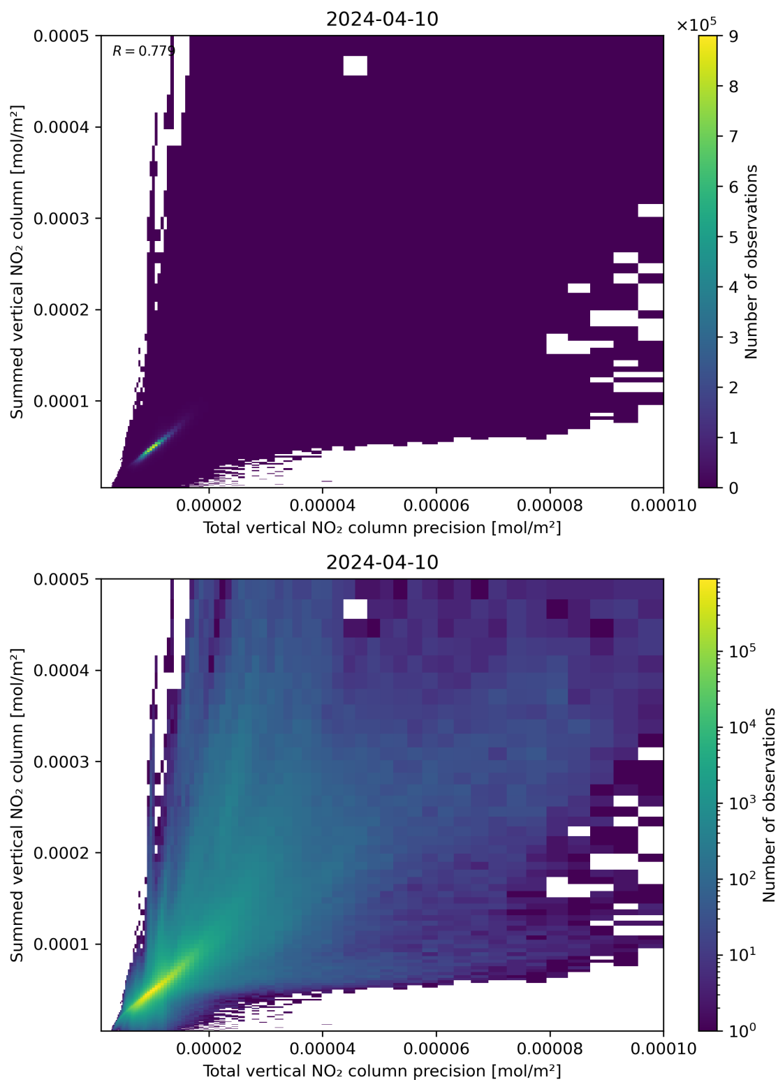
Figure 117: Scatter density plot of “Total vertical NO 2 column precision” against “Summed vertical NO 2 column” for 2024-04-10 to 2024-04-11.
