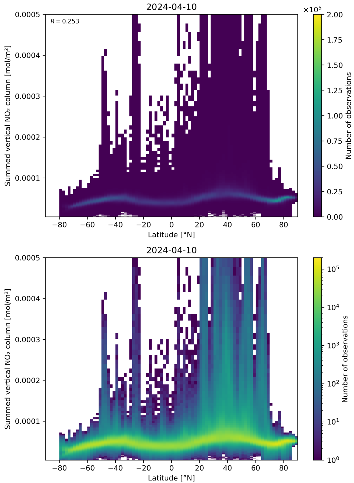
Figure 88: Scatter density plot of “Latitude” against “Summed vertical NO 2 column” for 2024-04-10 to 2024-04-11.
