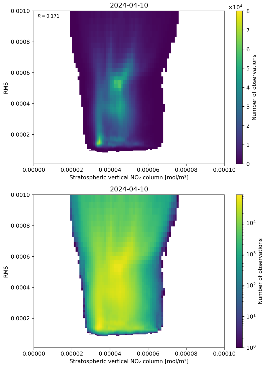
Figure 102: Scatter density plot of “Stratospheric vertical NO 2 column” against “RMS” for 2024-04-10 to 2024-04-11.
