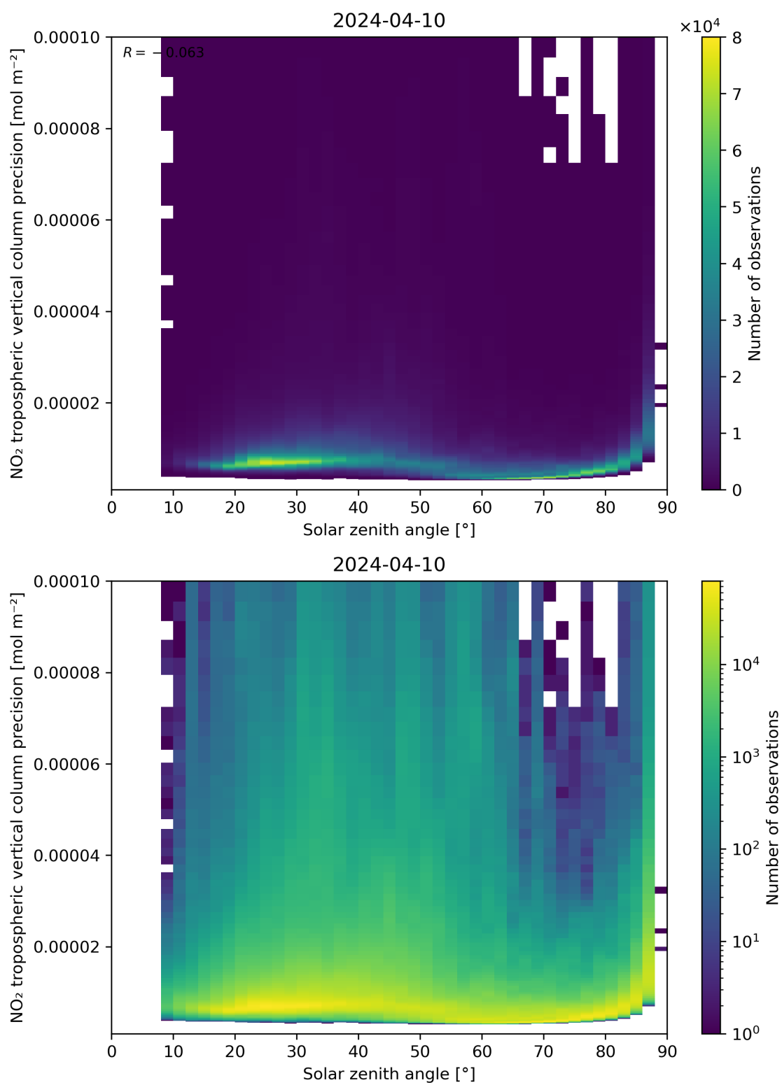
Figure 156: Scatter density plot of “Solar zenith angle” against “NO 2 tropospheric vertical column precision” for 2024-04-10 to 2024-04-11.
