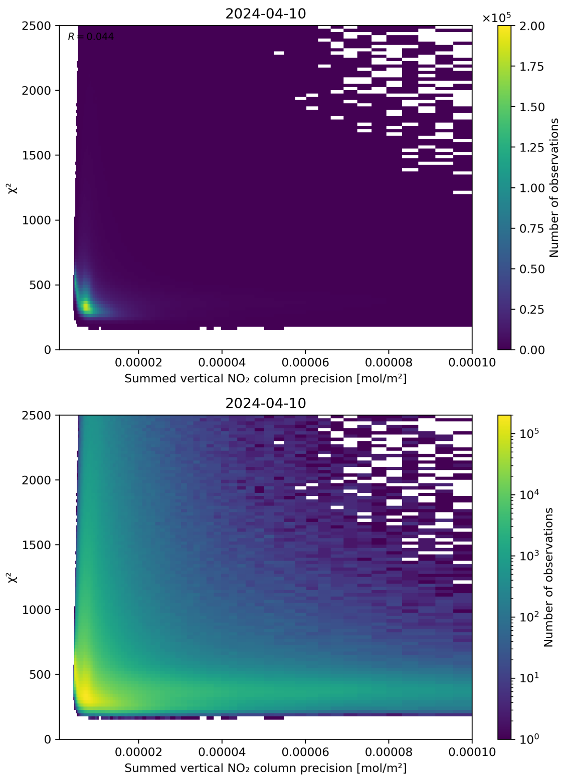
Figure 107: Scatter density plot of “Summed vertical NO 2 column precision” against “ \chi^2 ” for 2024-04-10 to 2024-04-11.
