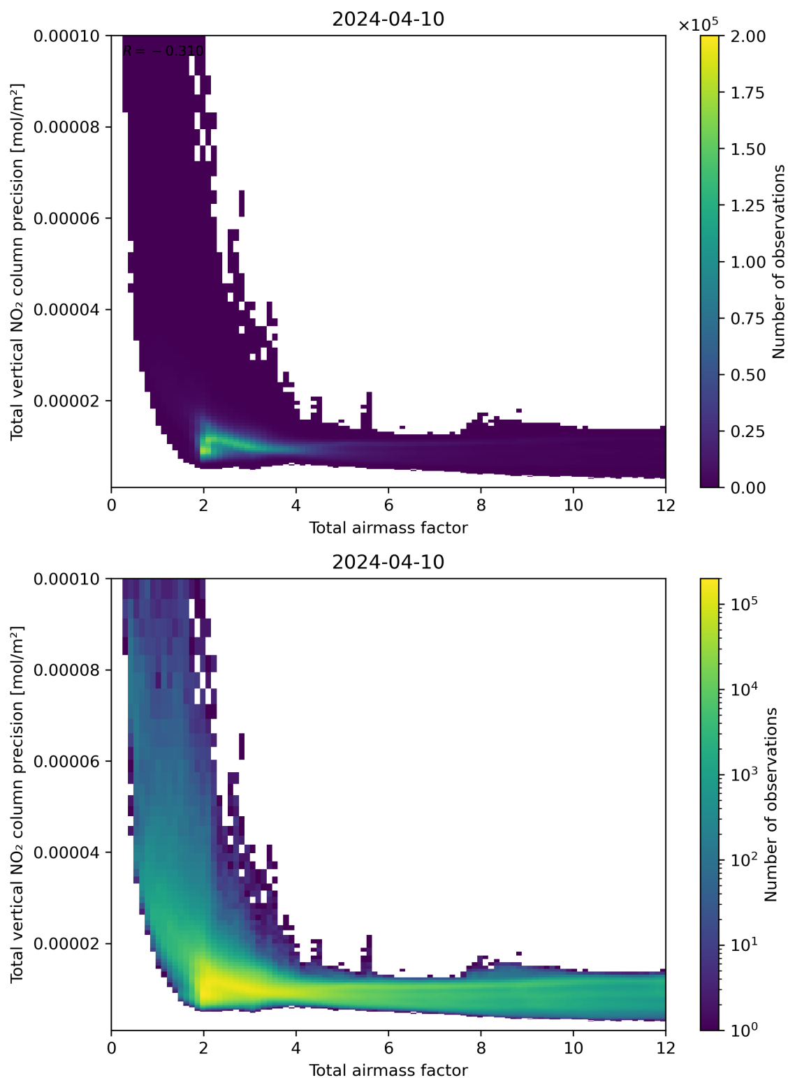
Figure 68: Scatter density plot of “Total airmass factor” against “Total vertical NO 2 column precision” for 2024-04-10 to 2024-04-11.
