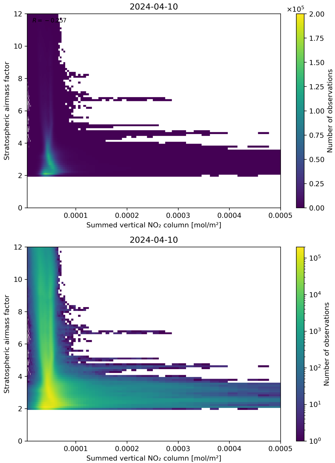
Figure 103: Scatter density plot of “Summed vertical NO 2 column” against “Stratospheric air mass factor” for 2024-04-10 to 2024-04-11.
