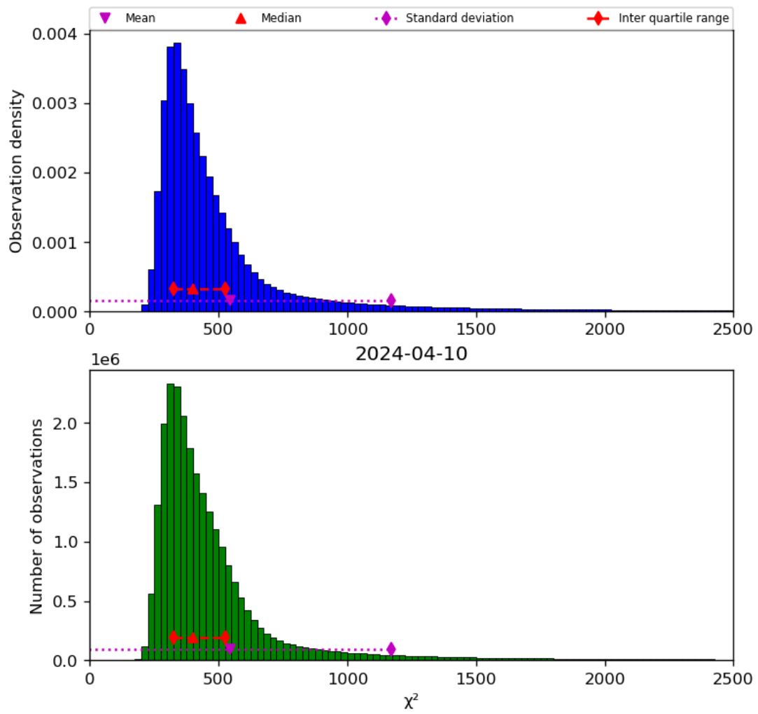
Figure 42: Histogram of “ \chi^2 ” for 2024-04-10 to 2024-04-11
