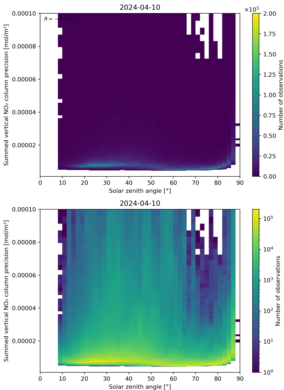
Figure 152: Scatter density plot of “Solar zenith angle” against “Summed vertical NO 2 column precision” for 2024-04-10 to 2024-04-11.
