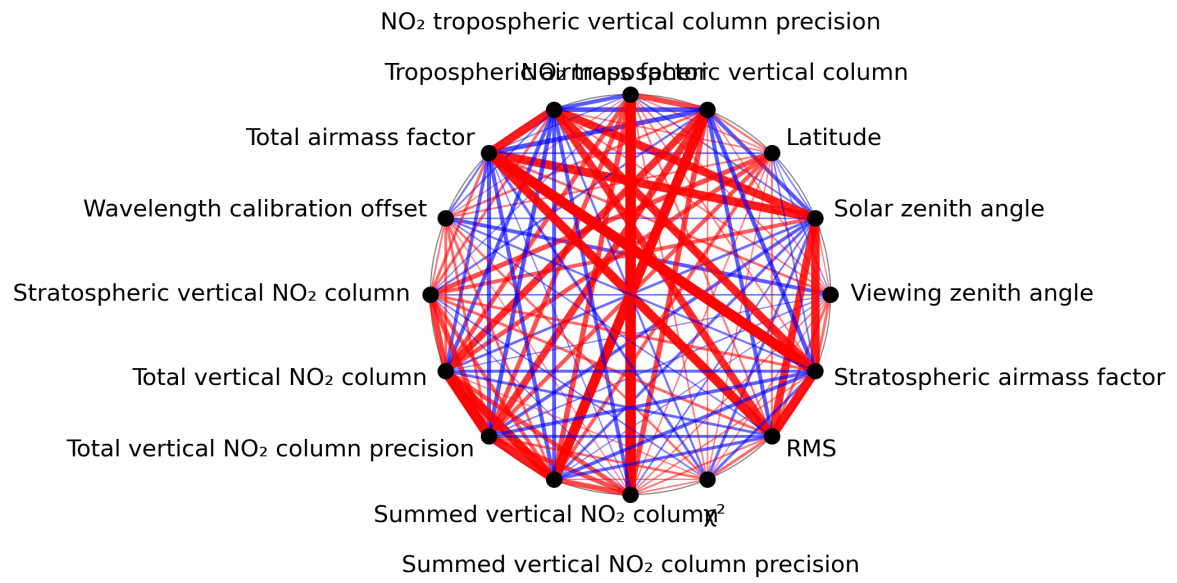
Figure 1: Map of correlation graph for 2024-04-10 to 2024-04-11.
