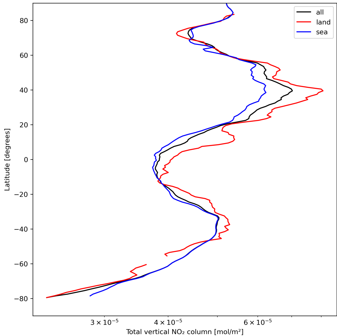
Figure 21: Zonal average of “Total vertical NO 2 column” for 2024-04-10 to 2024-04-11.
