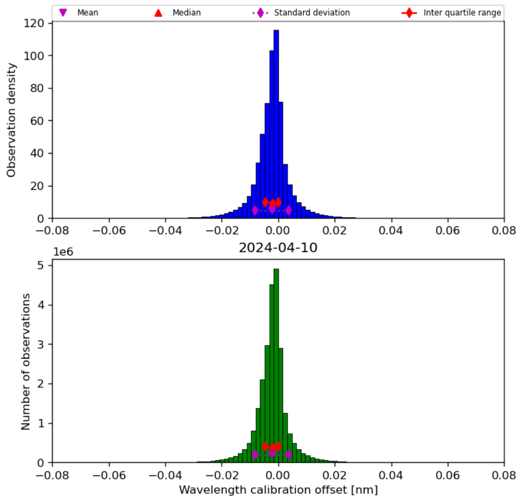
Figure 35: Histogram of “Wavelength calibration offset” for 2024-04-10 to 2024-04-11
