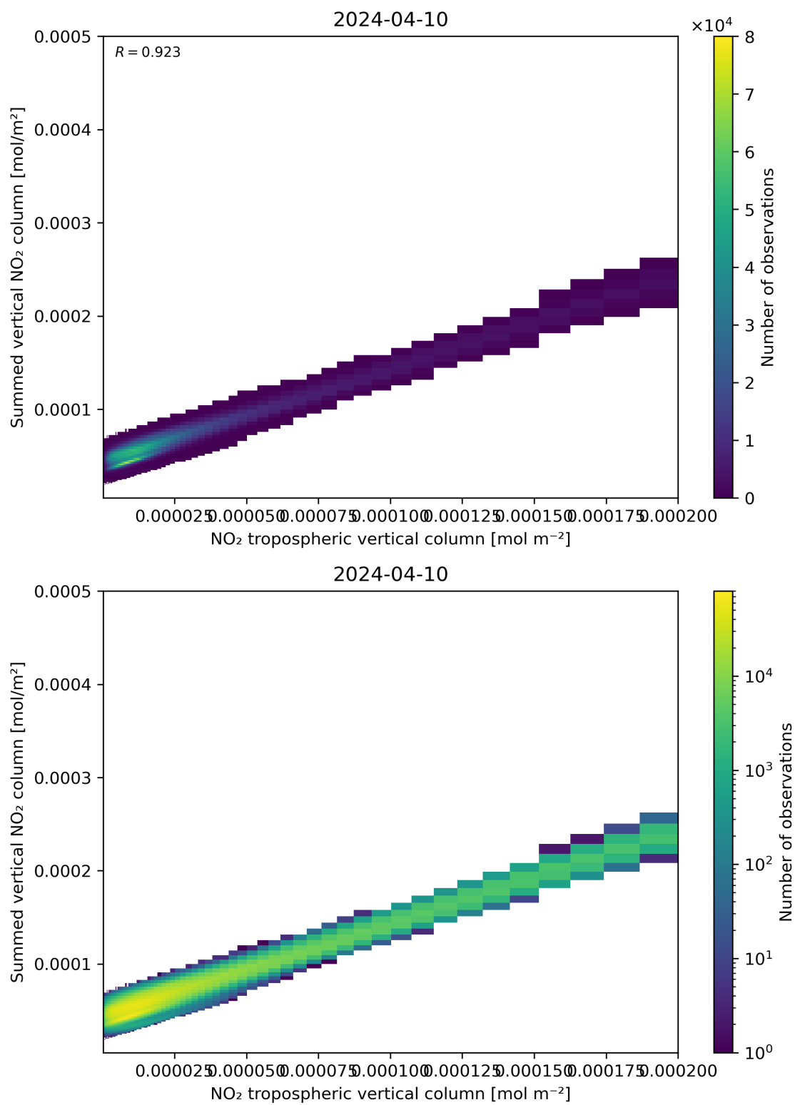
Figure 126: Scatter density plot of “NO 2 tropospheric vertical column” against “Summed vertical NO 2 column” for 2024-04-10 to 2024-04-11.
