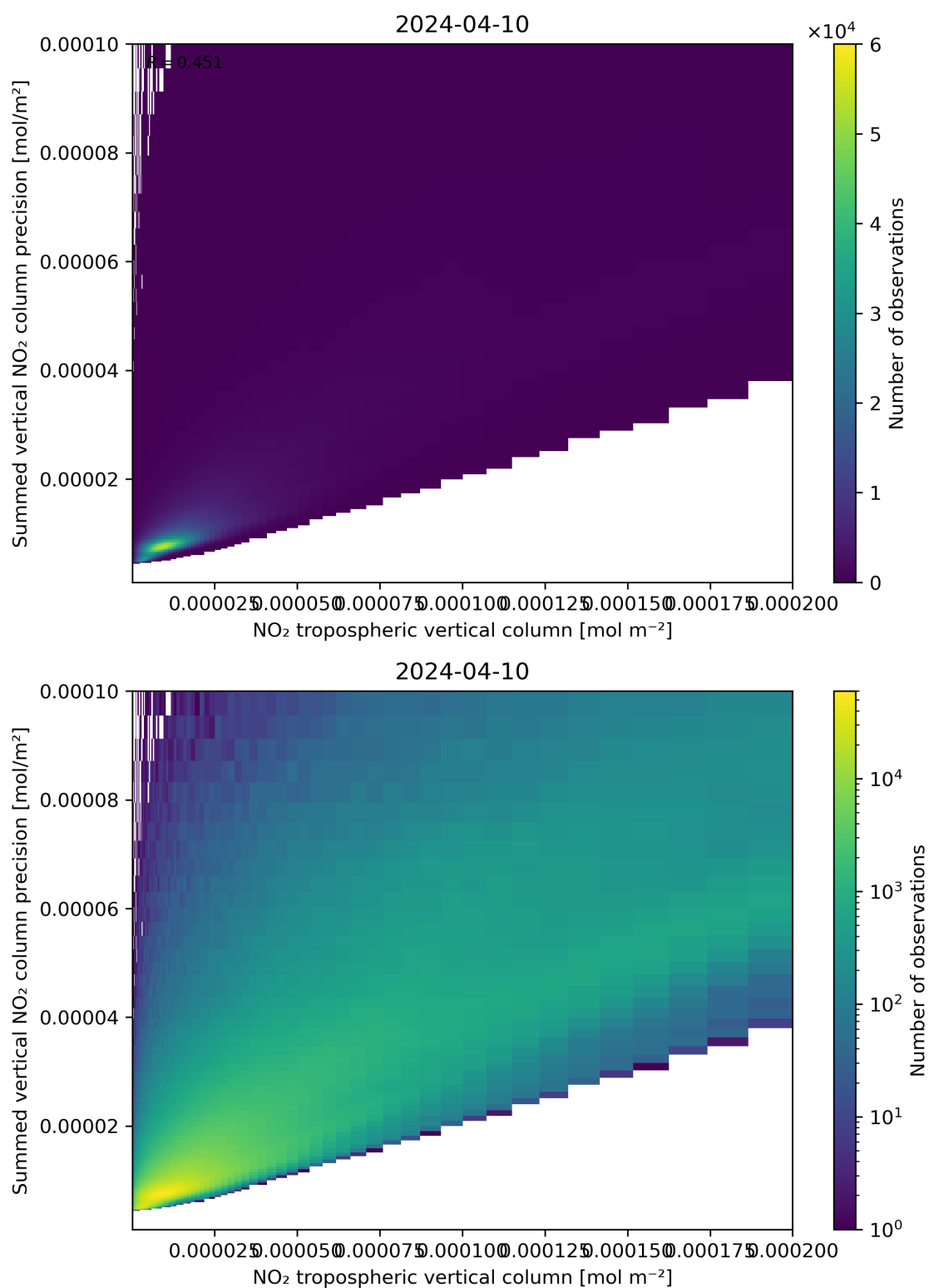
Figure 127: Scatter density plot of “NO 2 tropospheric vertical column” against “Summed vertical NO 2 column precision” for 2024-04-10 to 2024-04-11.
