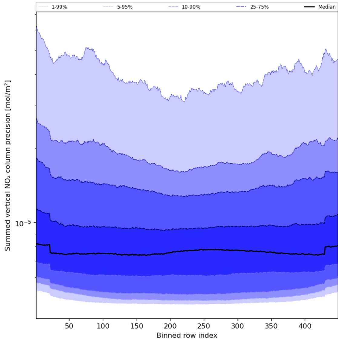
Figure 58: Along track statistics of “Summed vertical NO 2 column precision” for 2024-04-10 to 2024-04-11
