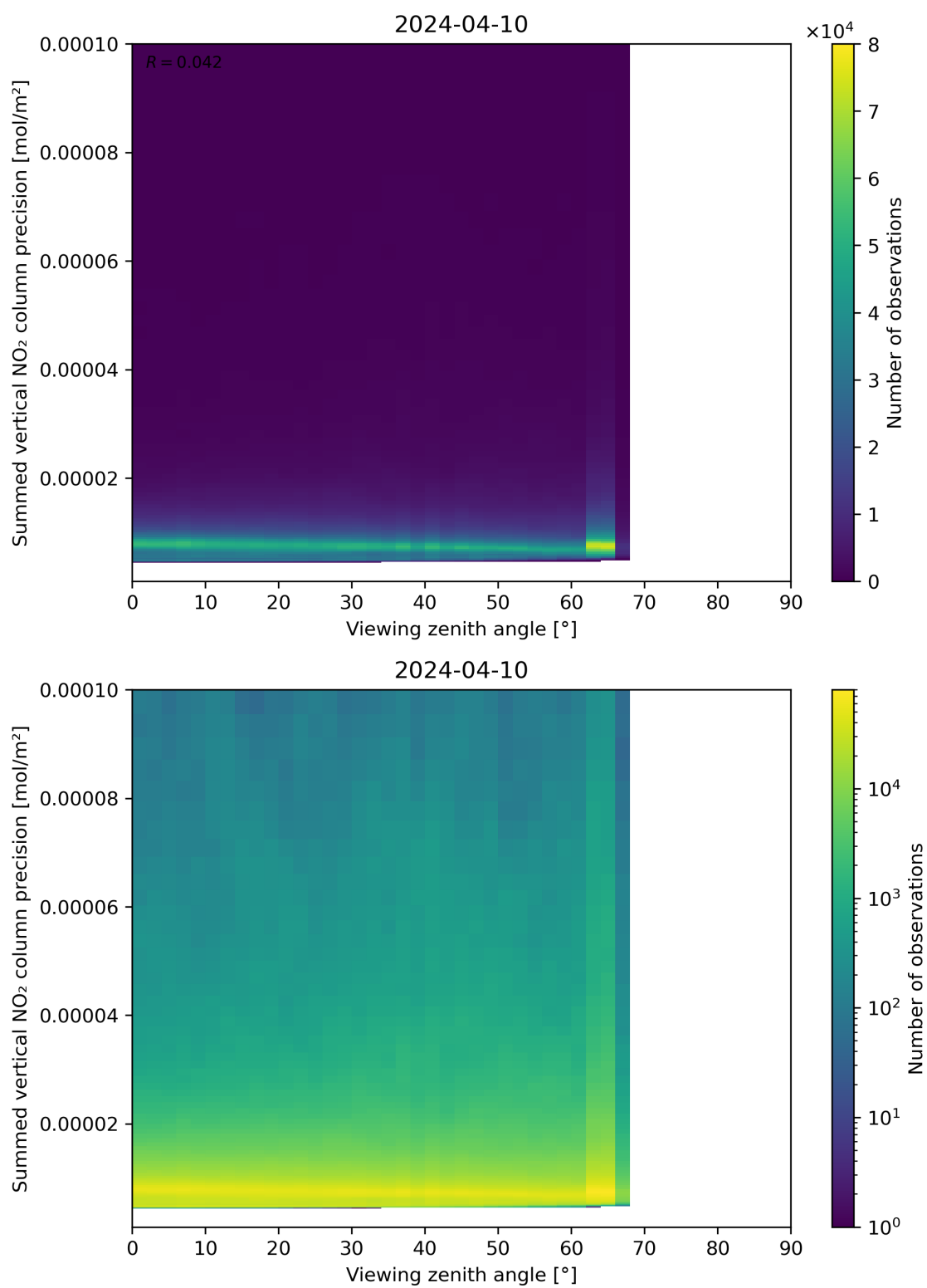
Figure 166: Scatter density plot of “Viewing zenith angle” against “Summed vertical NO 2 column precision” for 2024-04-10 to 2024-04-11.
