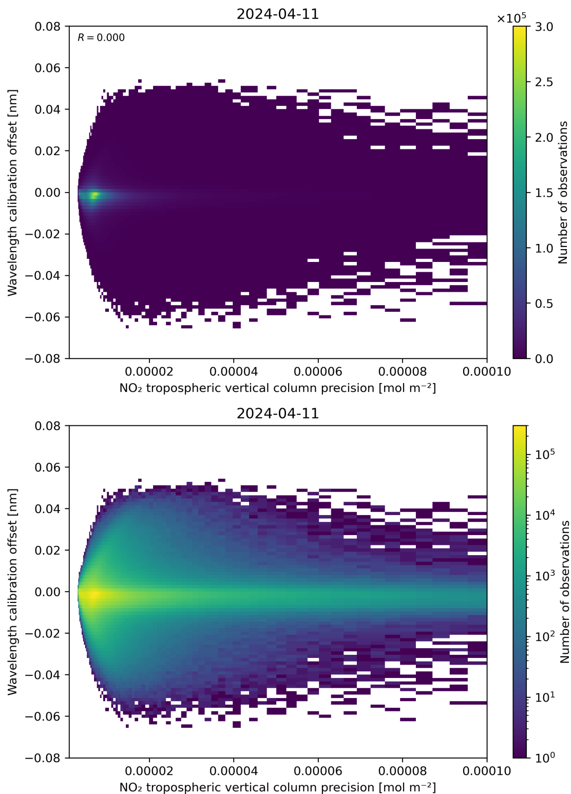
Figure 141: Scatter density plot of “NO 2 tropospheric vertical column precision” against “Wavelength calibration offset” for 2024-04-10 to 2024-04-12.
