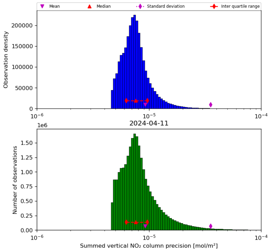
Figure 41: Histogram of “Summed vertical NO 2 column precision” for 2024-04-10 to 2024-04-12
