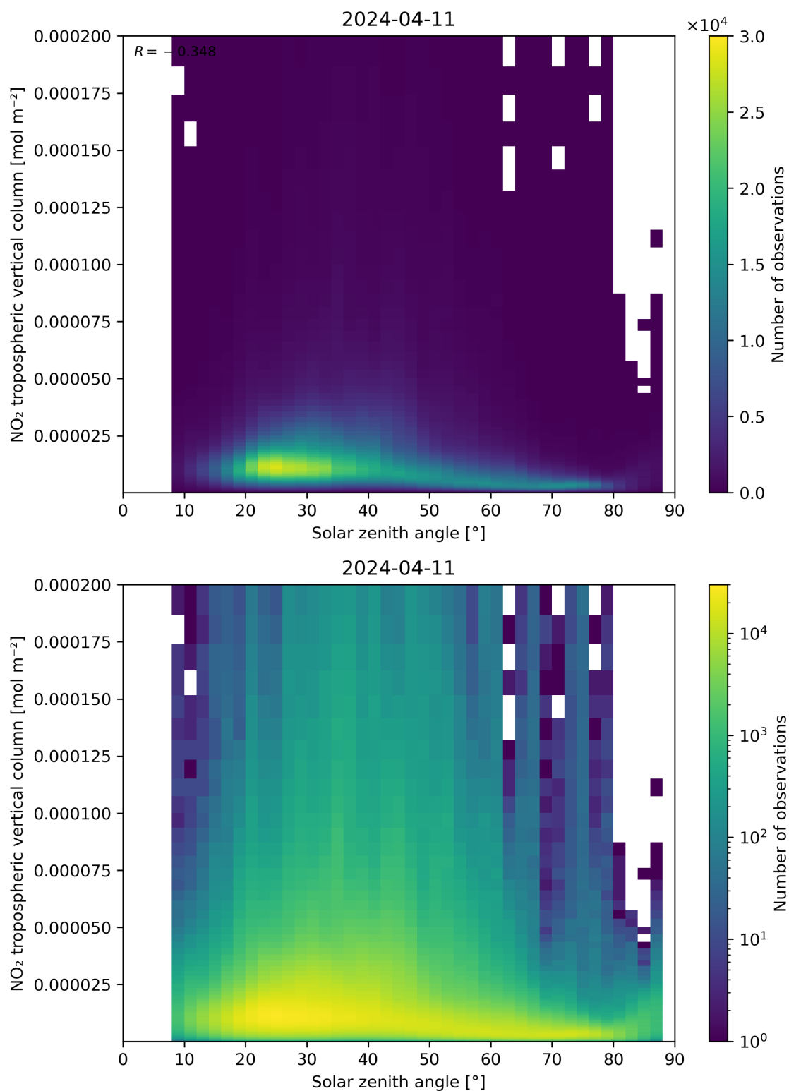
Figure 155: Scatter density plot of “Solar zenith angle” against “NO 2 tropospheric vertical column” for 2024-04-10 to 2024-04-12.
