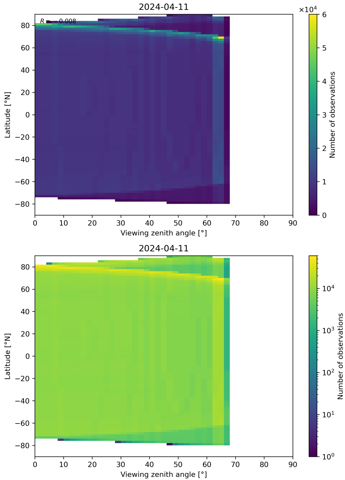
Figure 163: Scatter density plot of “Viewing zenith angle” against “Latitude” for 2024-04-10 to 2024-04-12.
