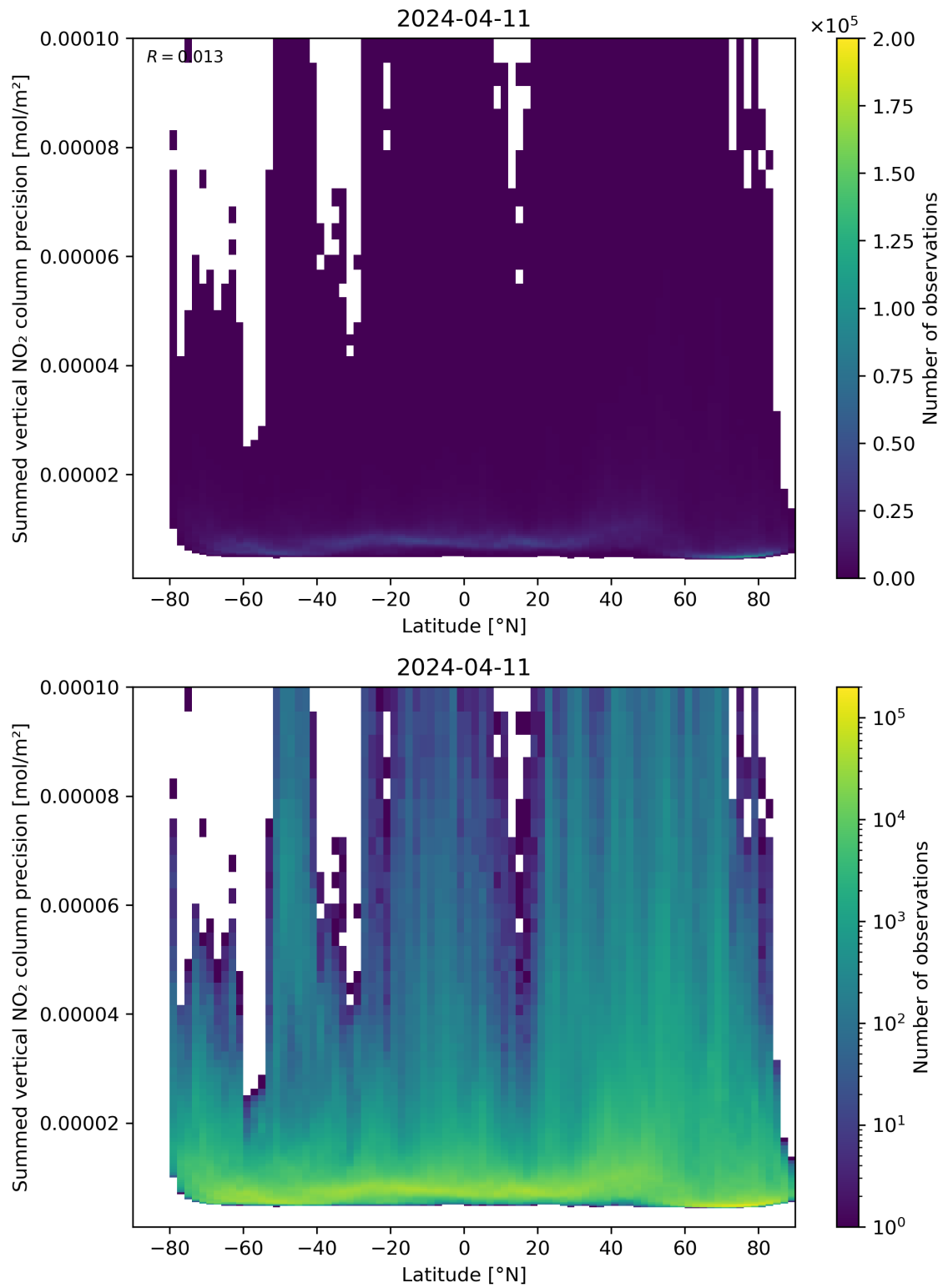
Figure 89: Scatter density plot of “Latitude” against “Summed vertical NO 2 column precision” for 2024-04-10 to 2024-04-12.
