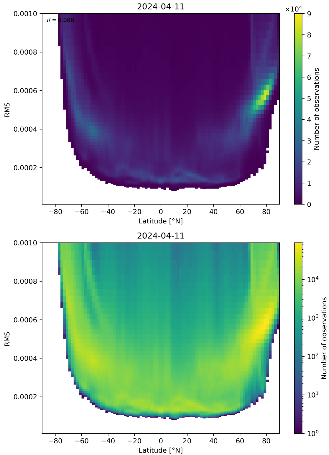
Figure 94: Scatter density plot of “Latitude” against “RMS” for 2024-04-10 to 2024-04-12.
