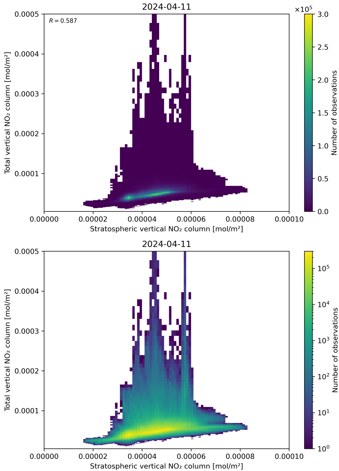
Figure 100: Scatter density plot of “Stratospheric vertical NO 2 column” against “Total vertical NO 2 column” for 2024-04-10 to 2024-04-12.
