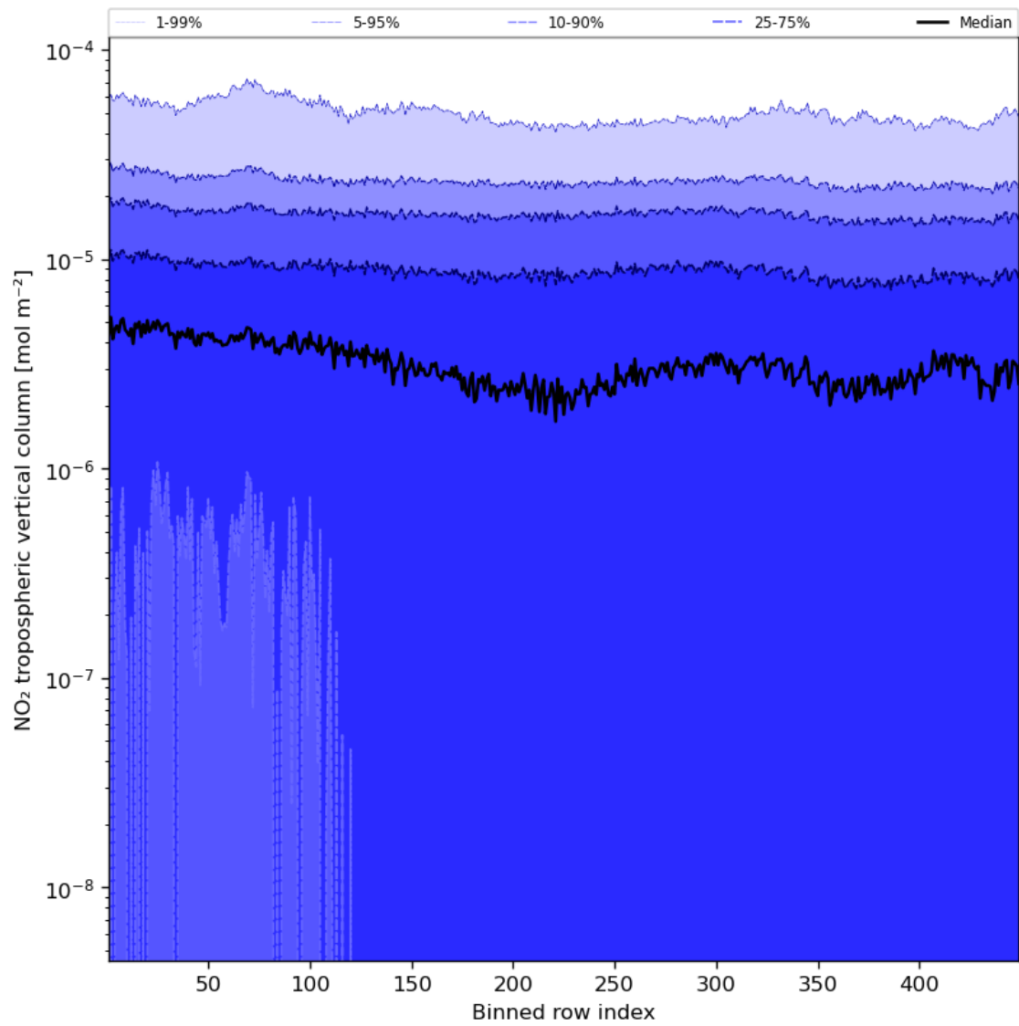
Figure 46: Along track statistics of “NO 2 tropospheric vertical column” for 2024-04-10 to 2024-04-12
