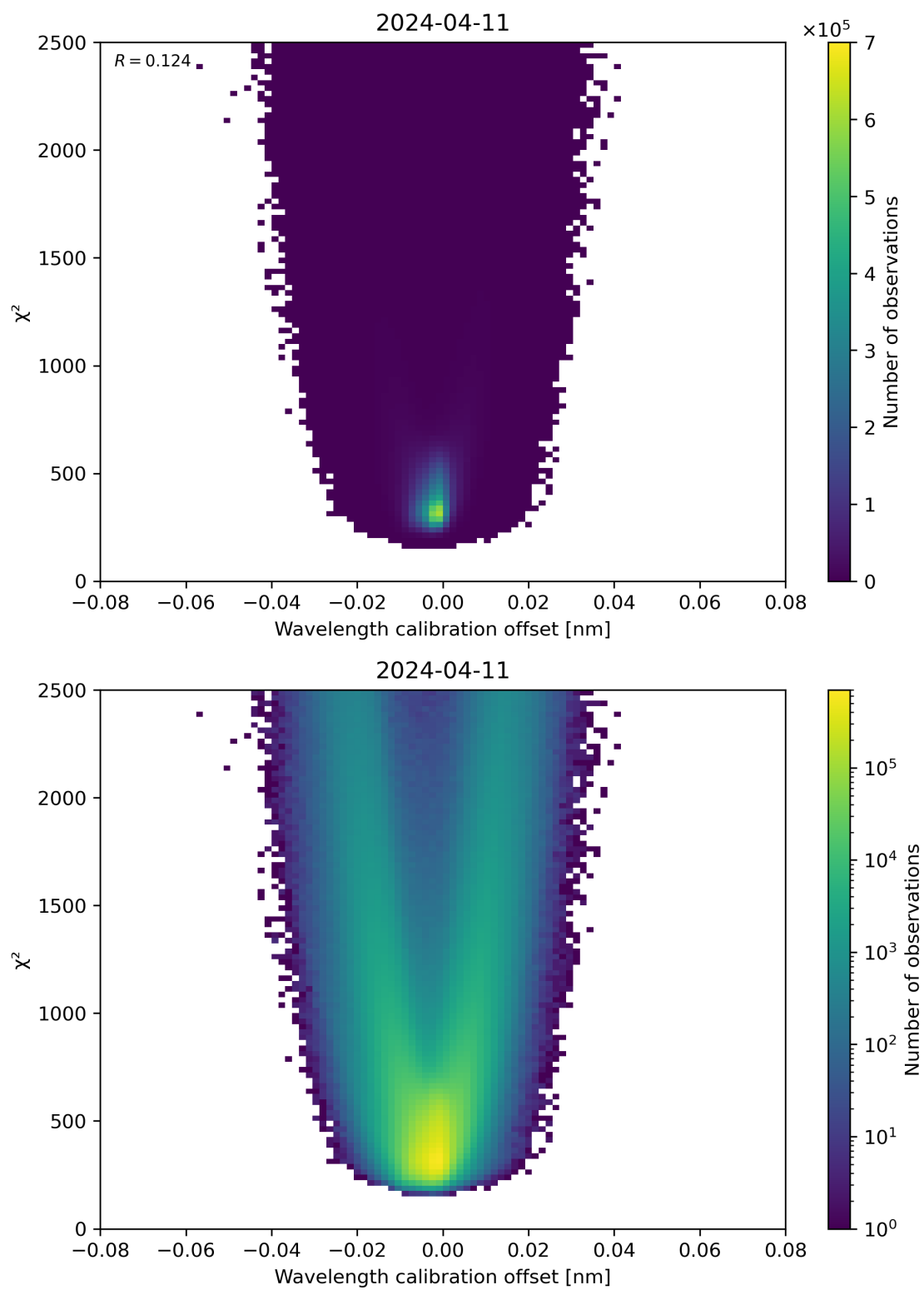
Figure 175: Scatter density plot of “Wavelength calibration offset” against “ \chi^2 ” for 2024-04-10 to 2024-04-12.
