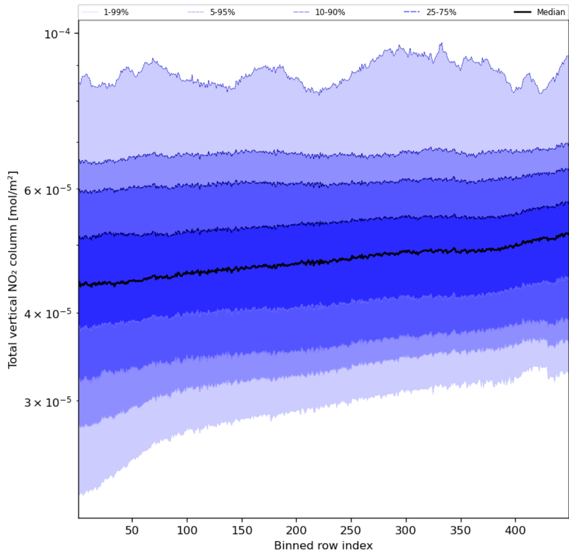
Figure 55: Along track statistics of “Total vertical NO 2 column” for 2024-04-10 to 2024-04-12
