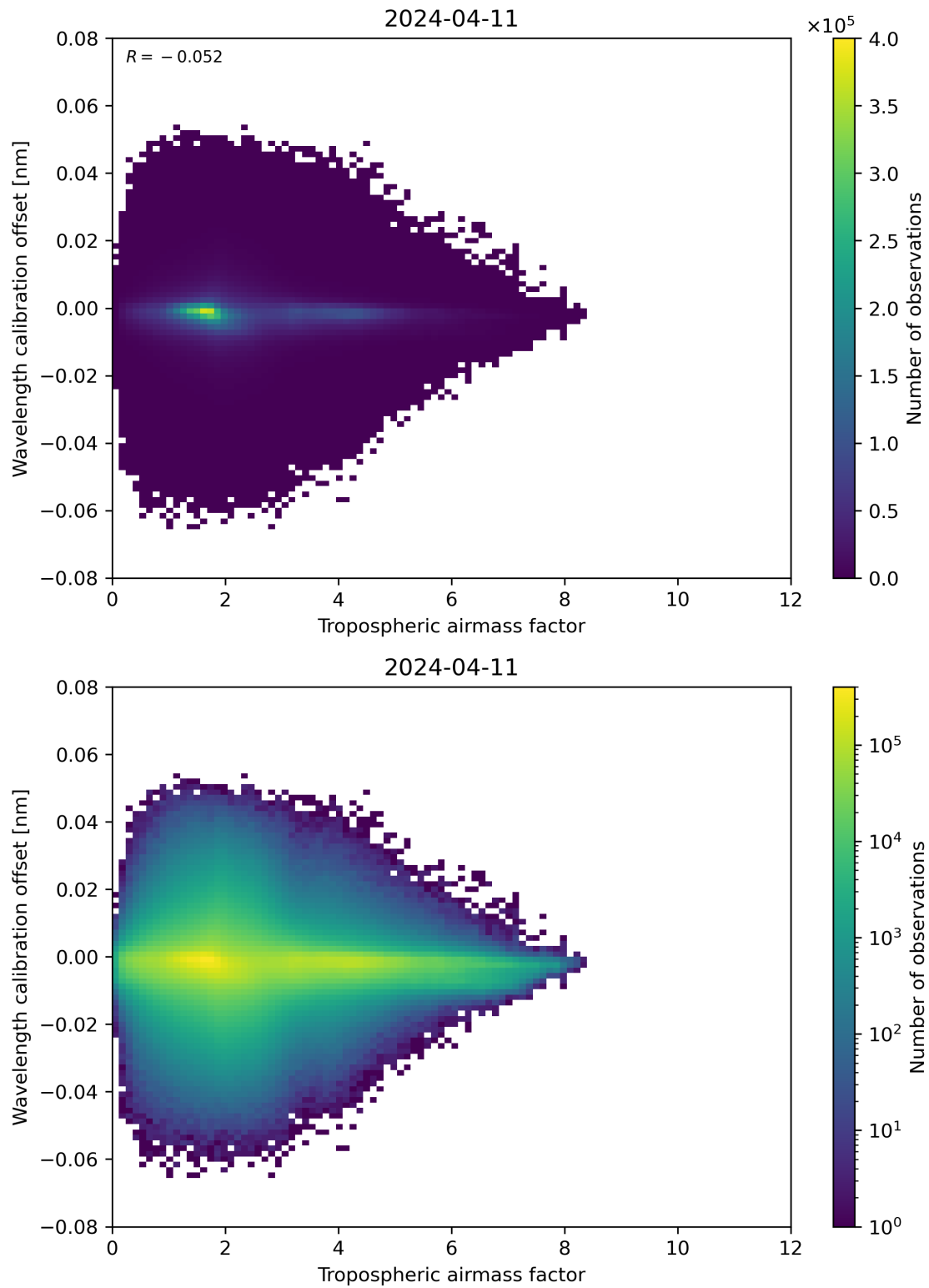
Figure 80: Scatter density plot of “Tropospheric airmass factor” against “Wavelength calibration offset” for 2024-04-10 to 2024-04-12.
