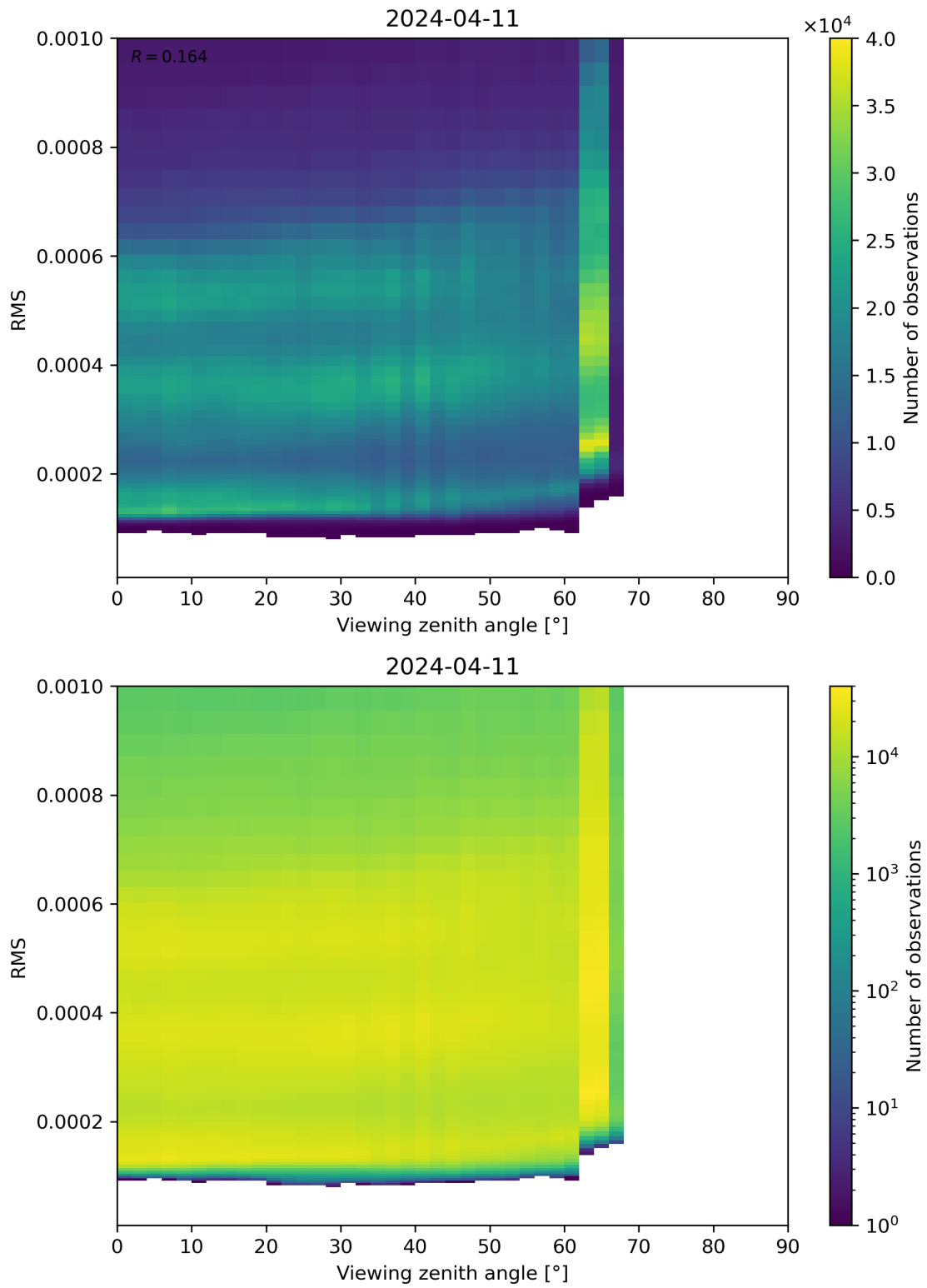
Figure 171: Scatter density plot of “Viewing zenith angle” against “RMS” for 2024-04-10 to 2024-04-12.
