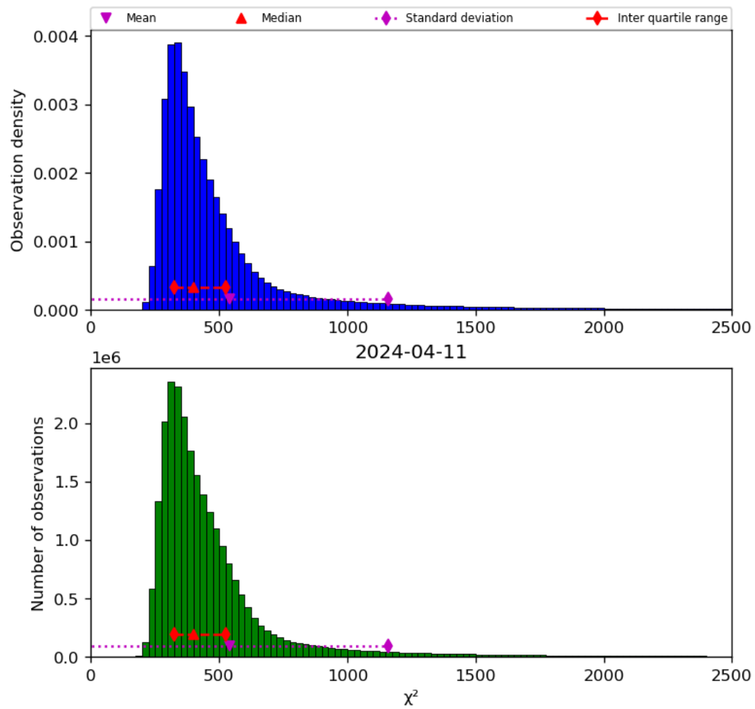
Figure 42: Histogram of “ \chi^2 ” for 2024-04-10 to 2024-04-12
