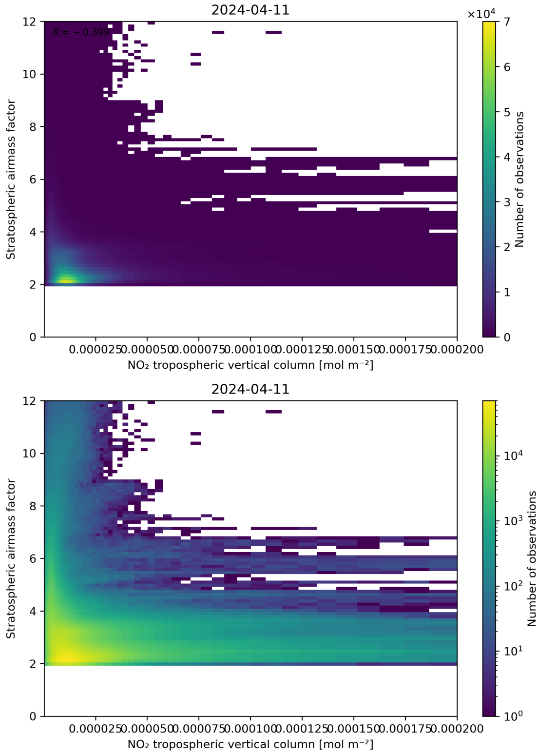
Figure 121: Scatter density plot of “NO 2 tropospheric vertical column” against “Stratospheric air mass factor” for 2024-04-10 to 2024-04-12.
