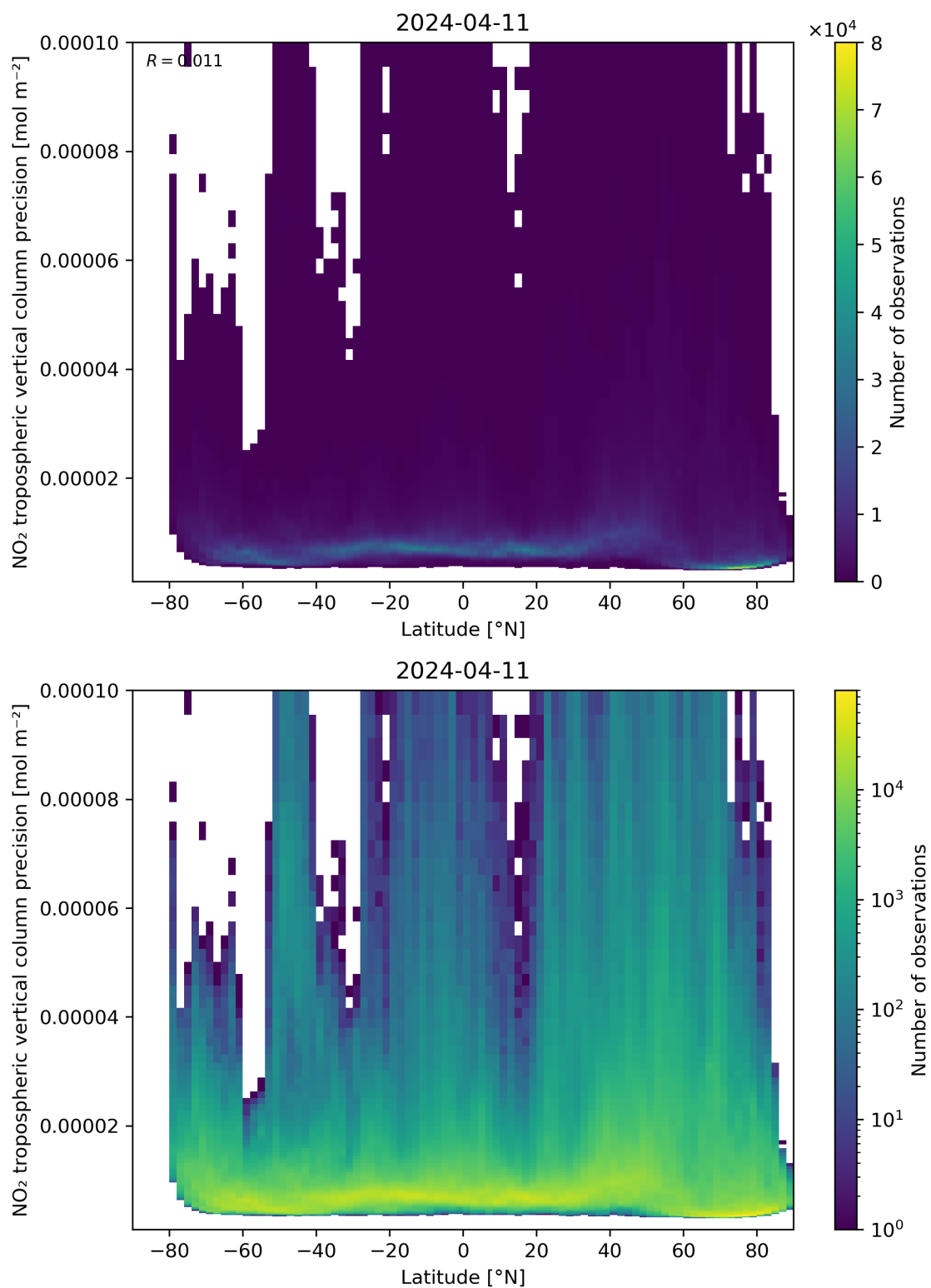
Figure 93: Scatter density plot of “Latitude” against “NO 2 tropospheric vertical column precision” for 2024-04-10 to 2024-04-12.
