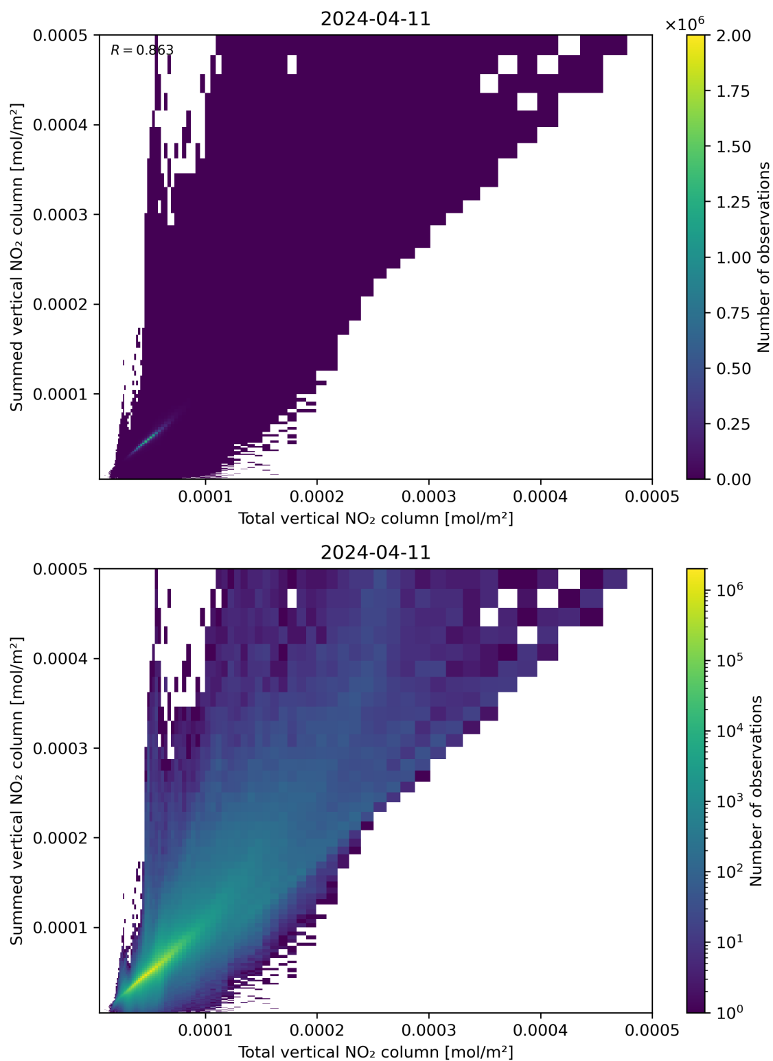
Figure 112: Scatter density plot of “Total vertical NO 2 column” against “Summed vertical NO 2 column” for 2024-04-10 to 2024-04-12.
