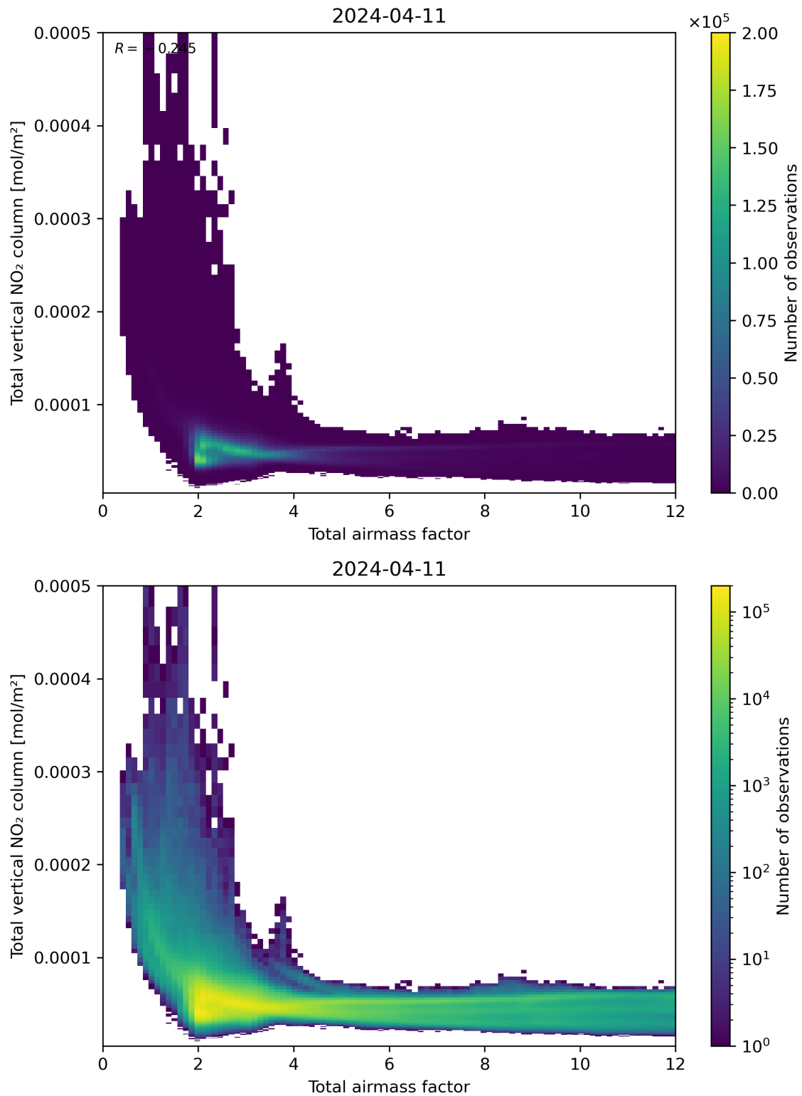
Figure 67: Scatter density plot of “Total airmass factor” against “Total vertical NO 2 column” for 2024-04-10 to 2024-04-12.
