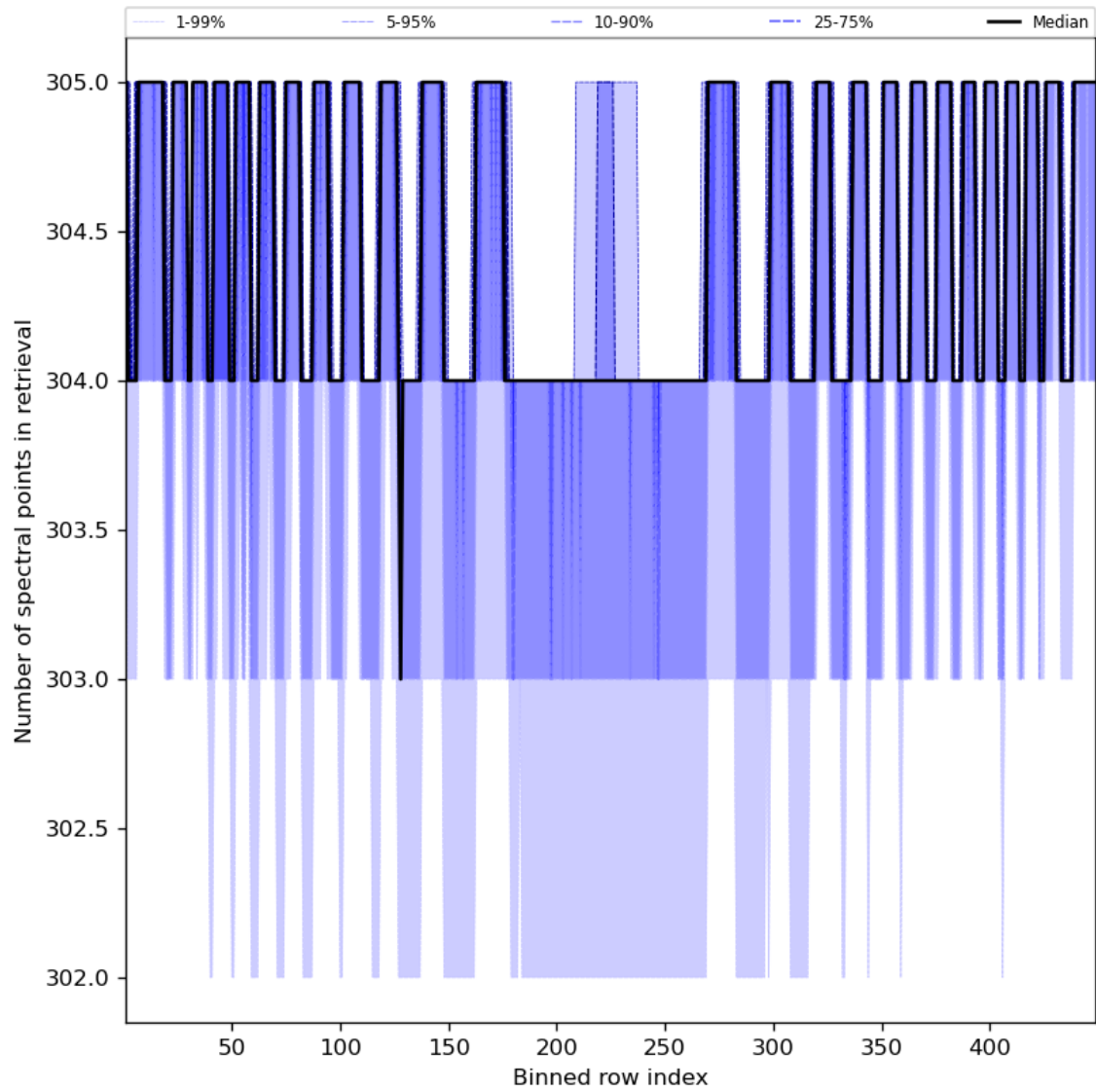
Figure 50: Along track statistics of “Number of spectral points in retrieval” for 2024-04-10 to 2024-04-12
