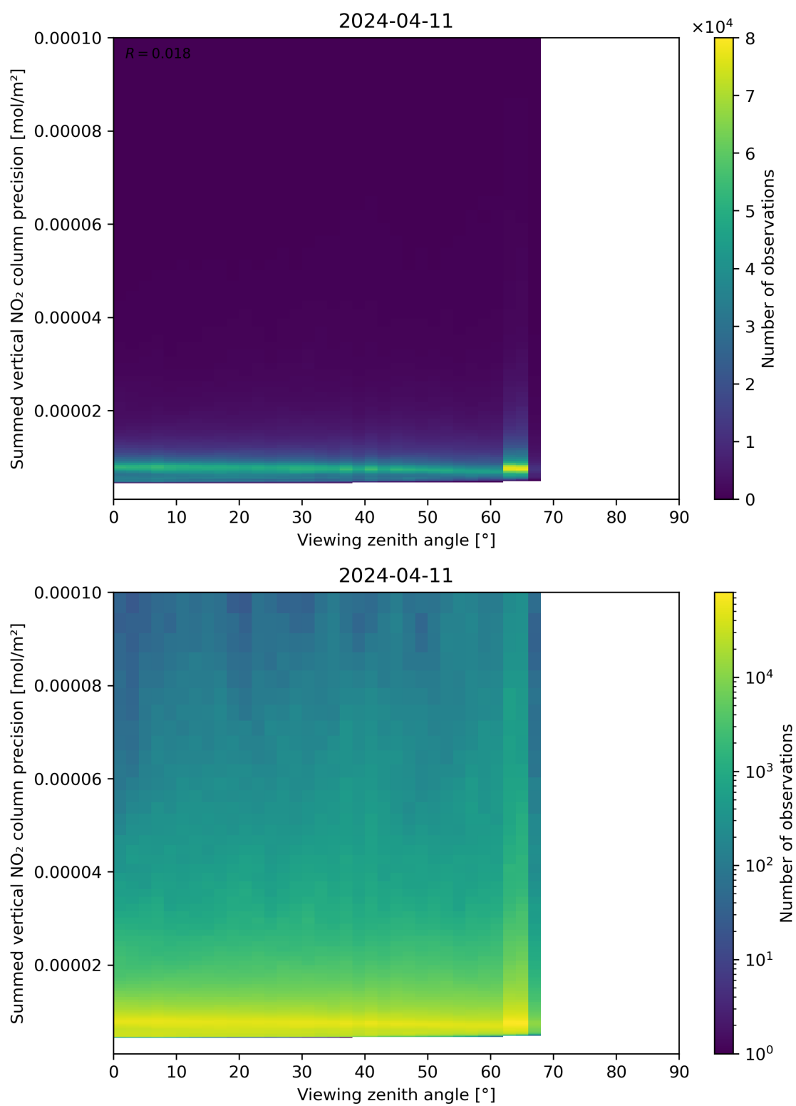
Figure 166: Scatter density plot of “Viewing zenith angle” against “Summed vertical NO 2 column precision” for 2024-04-10 to 2024-04-12.
