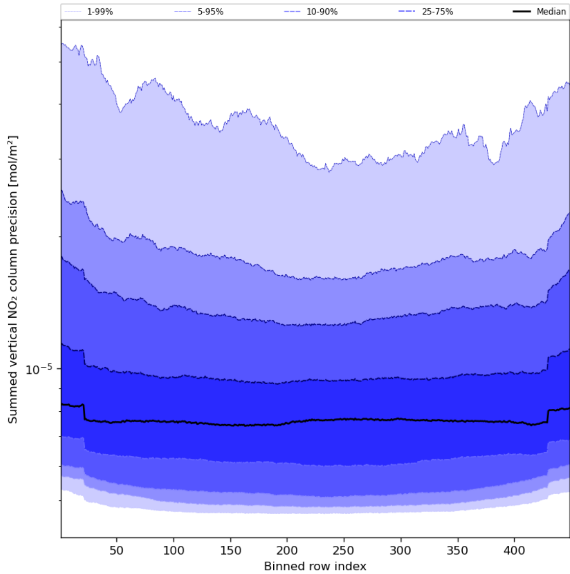
Figure 58: Along track statistics of “Summed vertical NO 2 column precision” for 2024-04-10 to 2024-04-12
