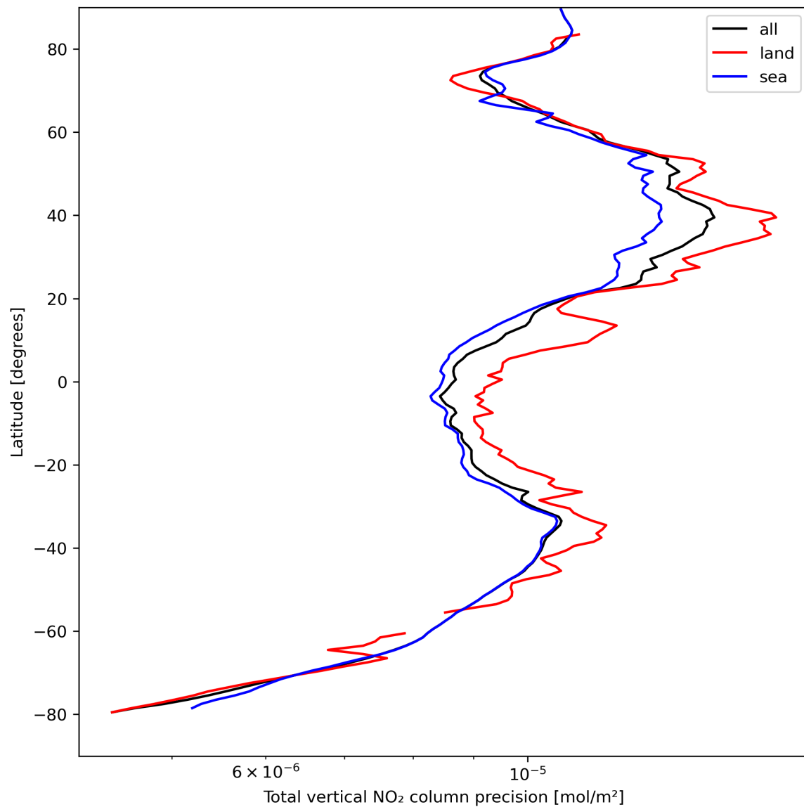
Figure 22: Zonal average of “Total vertical NO 2 column precision” for 2024-04-10 to 2024-04-12.
