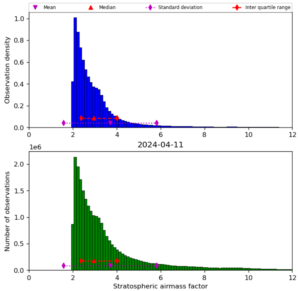
Figure 44: Histogram of “Stratospheric airmass factor” for 2024-04-10 to 2024-04-12
