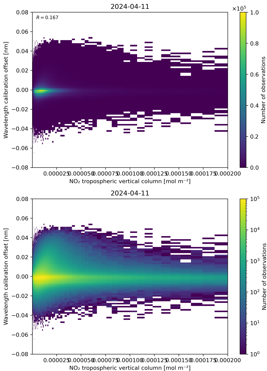
Figure 143: Scatter density plot of “NO 2 tropospheric vertical column” against “Wavelength calibration offset” for 2024-04-10 to 2024-04-12.
