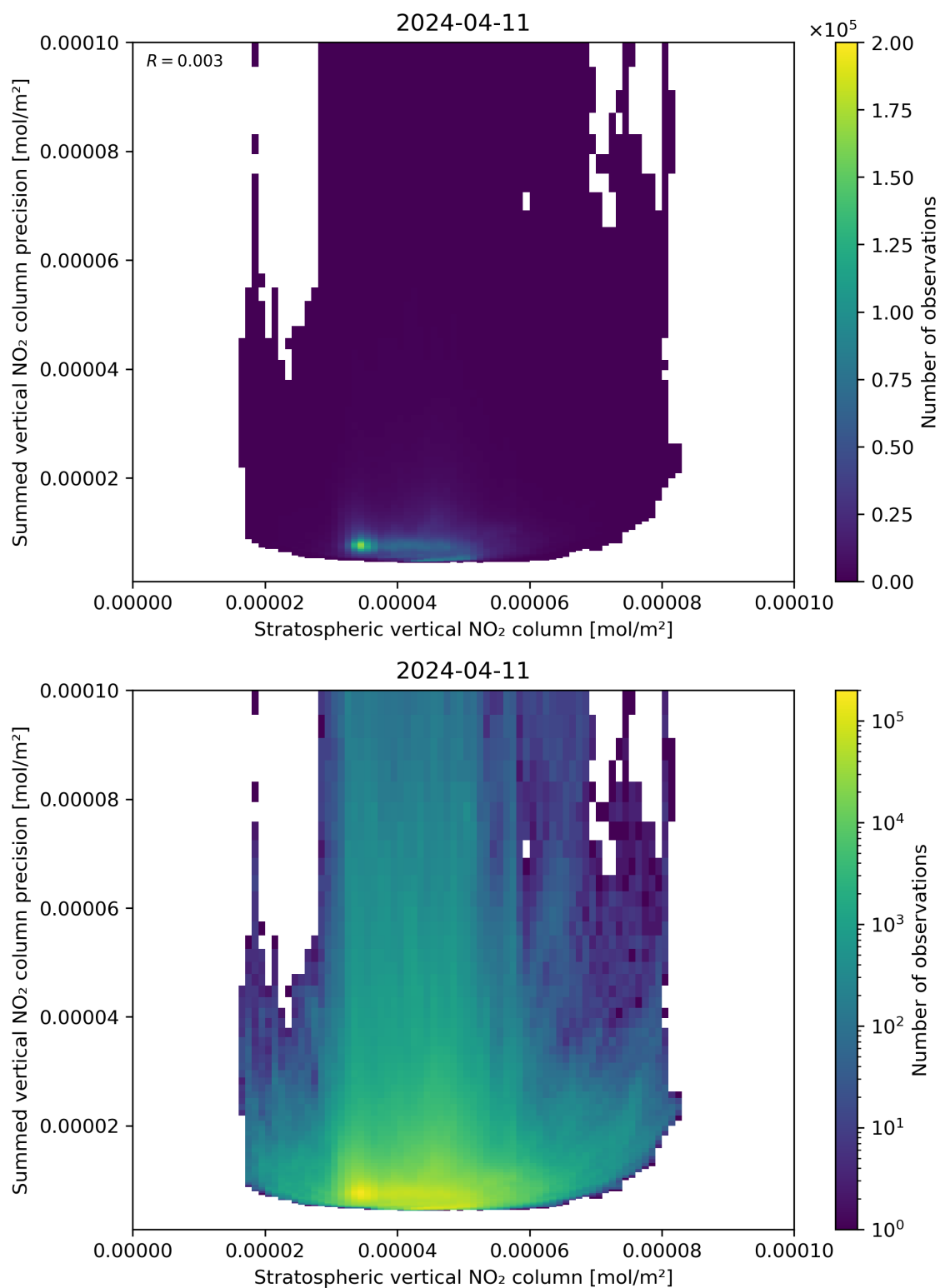
Figure 99: Scatter density plot of “Stratospheric vertical NO 2 column” against “Summed vertical NO 2 column precision” for 2024-04-10 to 2024-04-12.
