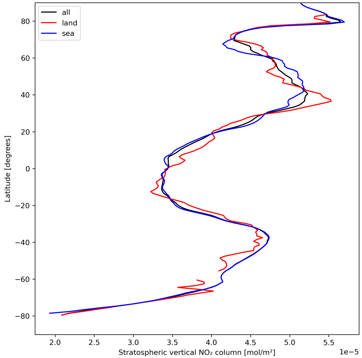
Figure 19: Zonal average of “Stratospheric vertical NO 2 column” for 2024-04-10 to 2024-04-12.
