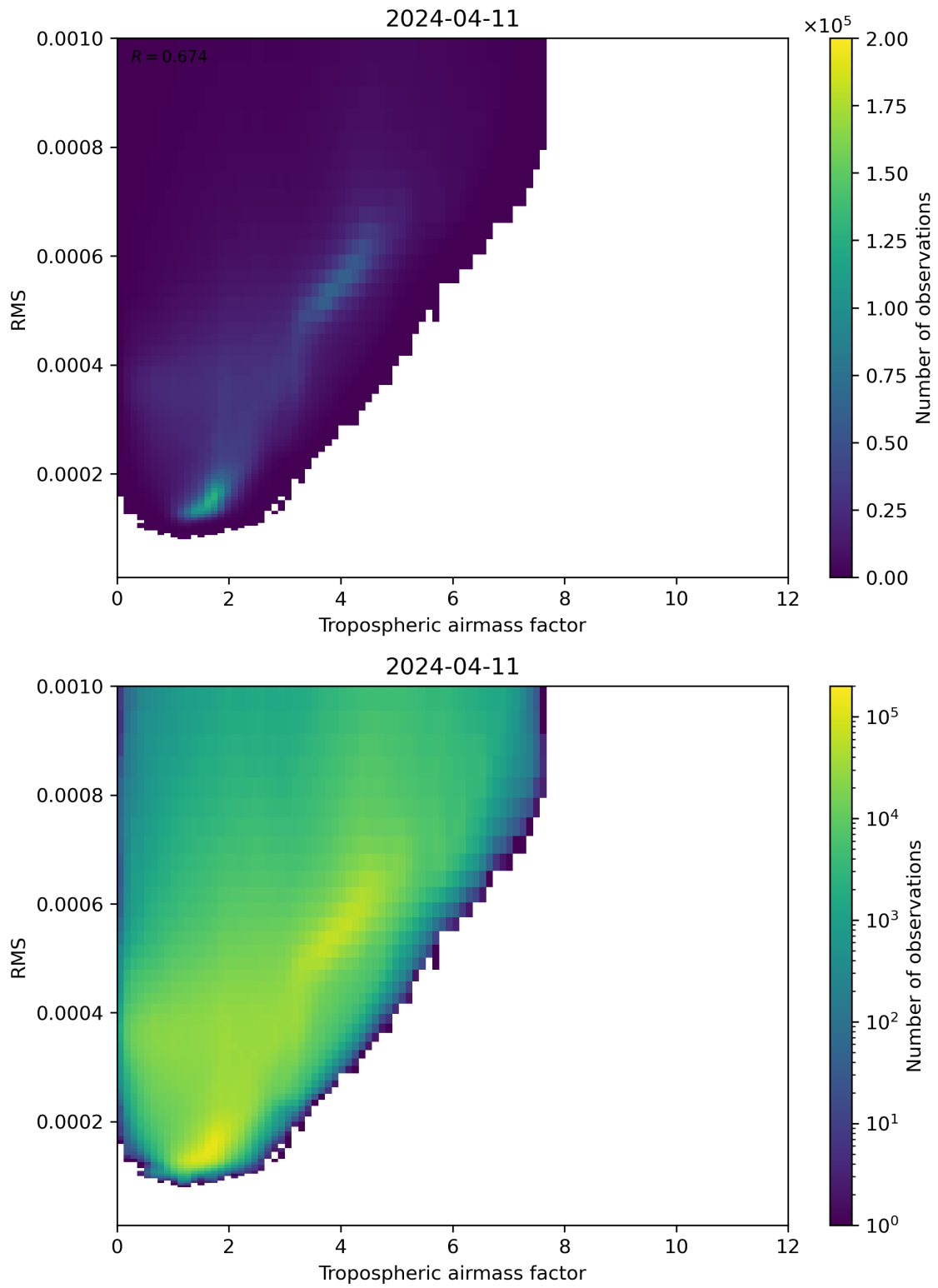
Figure 79: Scatter density plot of “Tropospheric airmass factor” against “RMS” for 2024-04-10 to 2024-04-12.
