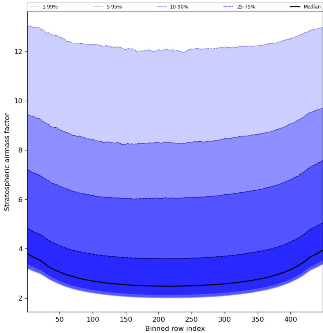
Figure 61: Along track statistics of “Stratospheric airmass factor” for 2024-04-10 to 2024-04-12
