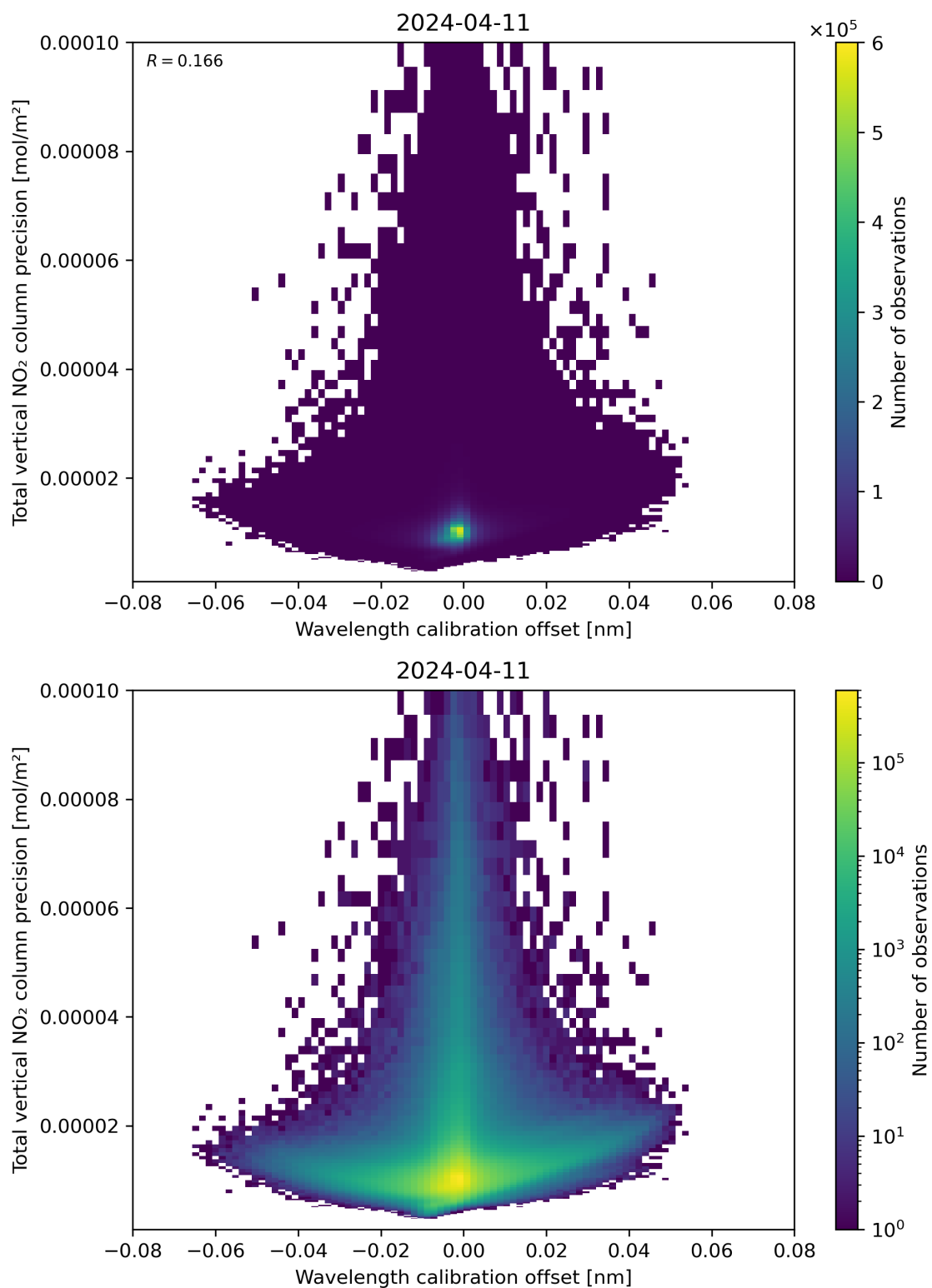
Figure 180: Scatter density plot of “Wavelength calibration offset” against “Total vertical NO 2 column precision” for 2024-04-10 to 2024-04-12.
