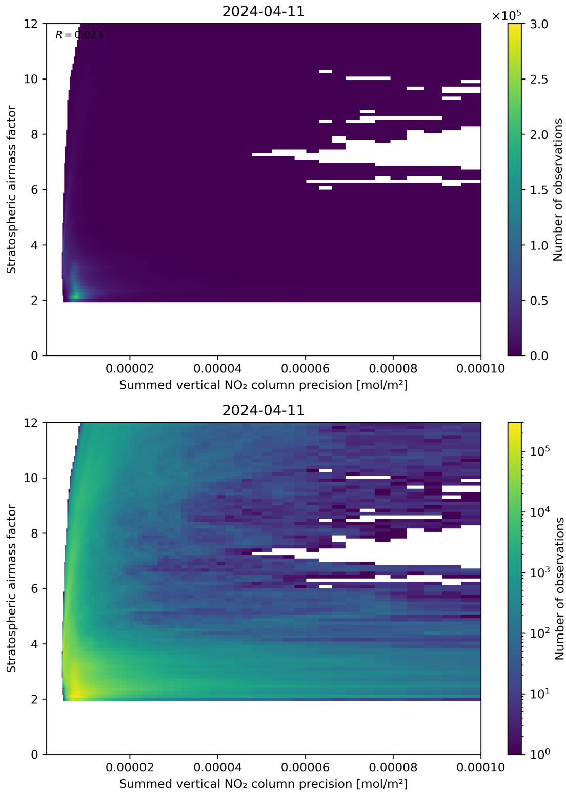
Figure 106: Scatter density plot of “Summed vertical NO 2 column precision” against “Stratospheric airmass factor” for 2024-04-10 to 2024-04-12.
