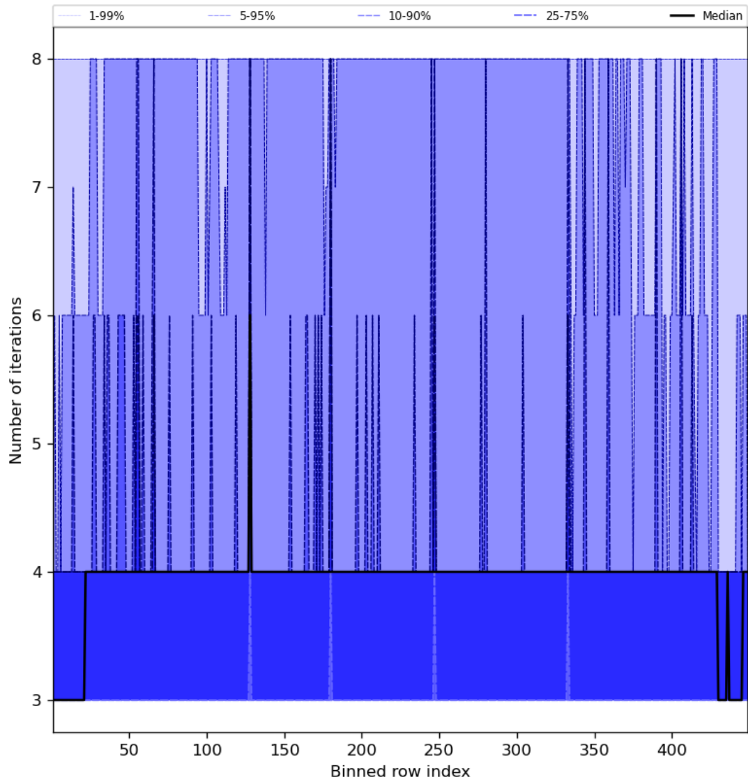
Figure 51: Along track statistics of “Number of iterations” for 2024-04-10 to 2024-04-12
