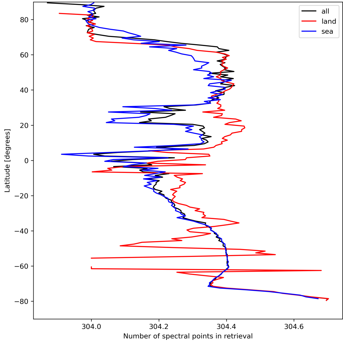
Figure 16: Zonal average of “Number of spectral points in retrieval” for 2024-04-10 to 2024-04-12.
