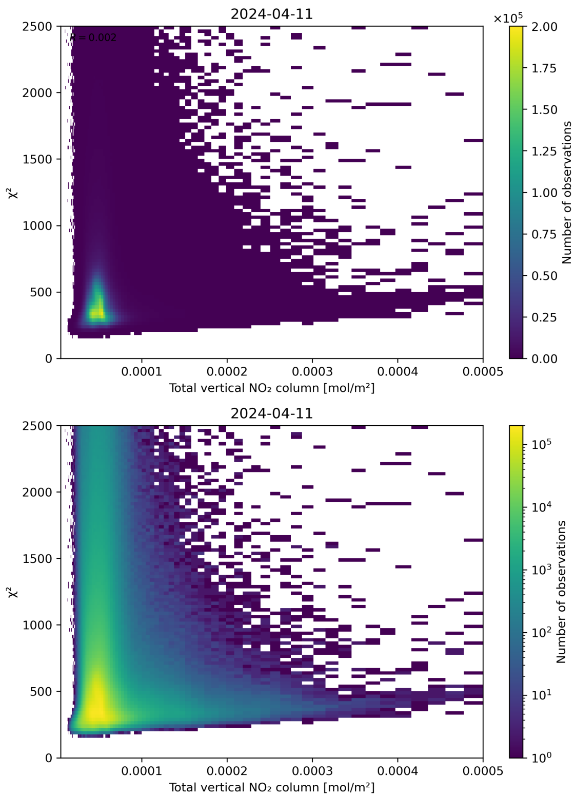
Figure 111: Scatter density plot of “Total vertical NO 2 column” against “ \chi^2 ” for 2024-04-10 to 2024-04-12.
