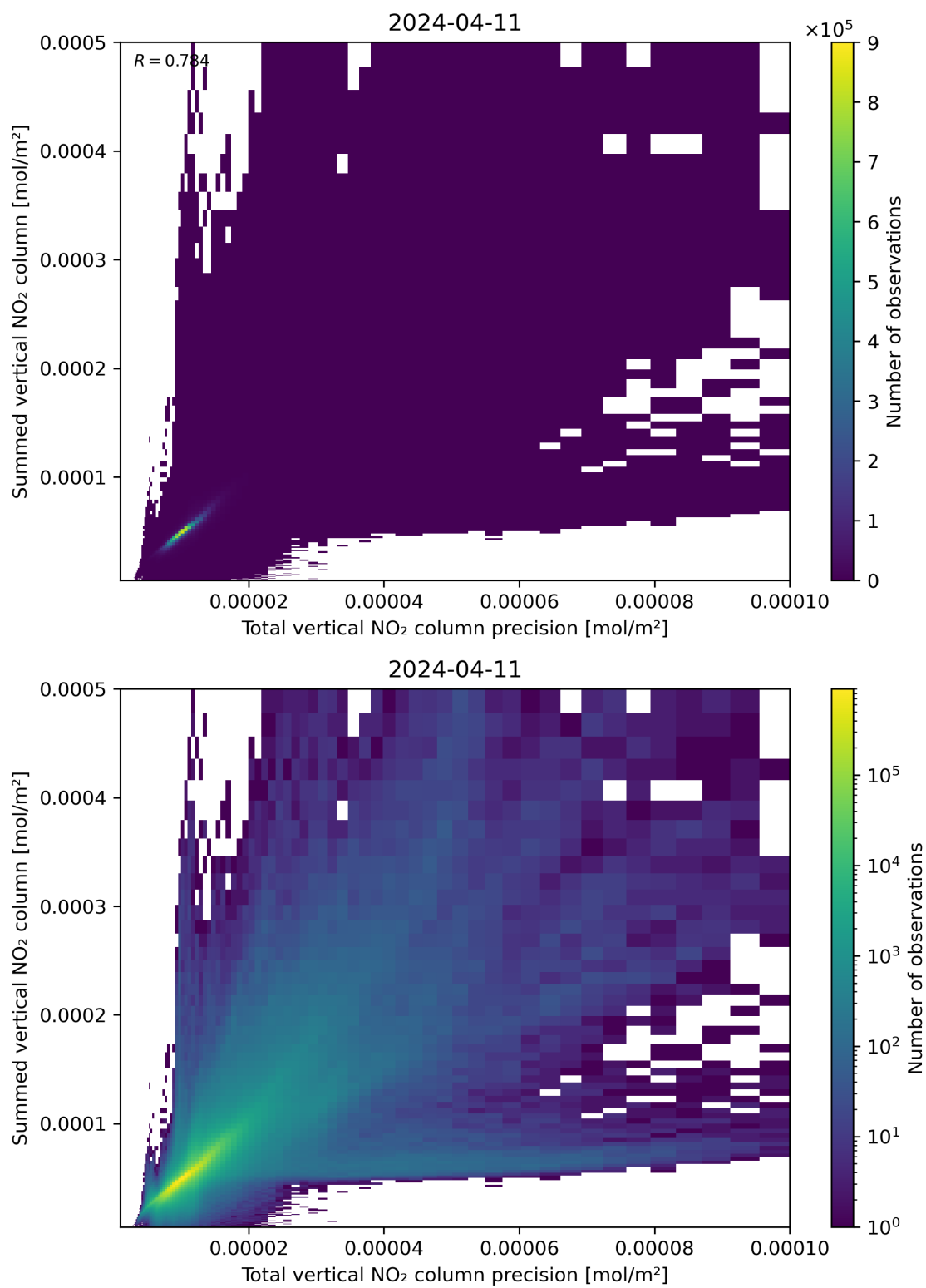
Figure 117: Scatter density plot of “Total vertical NO 2 column precision” against “Summed vertical NO 2 column” for 2024-04-10 to 2024-04-12.
