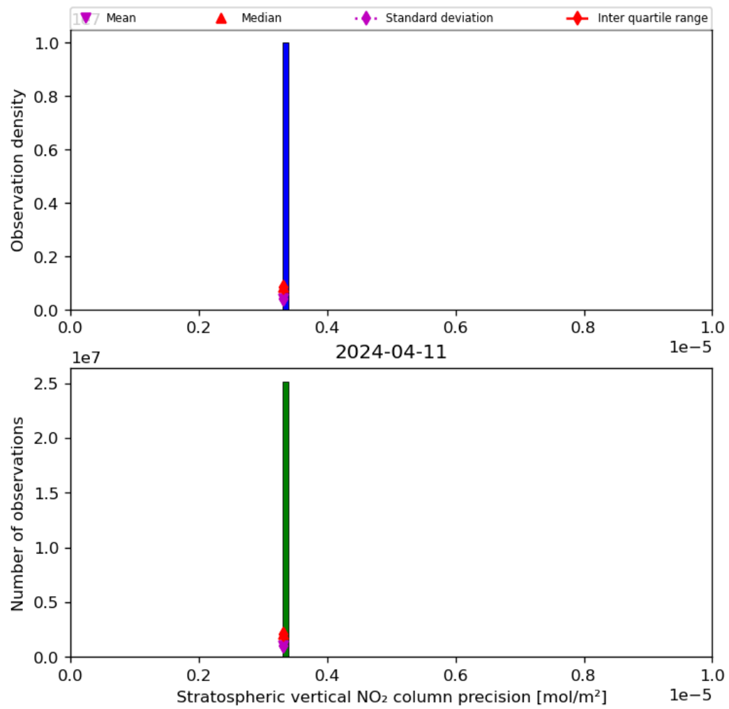
Figure 37: Histogram of “Stratospheric vertical NO 2 column precision” for 2024-04-10 to 2024-04-12
