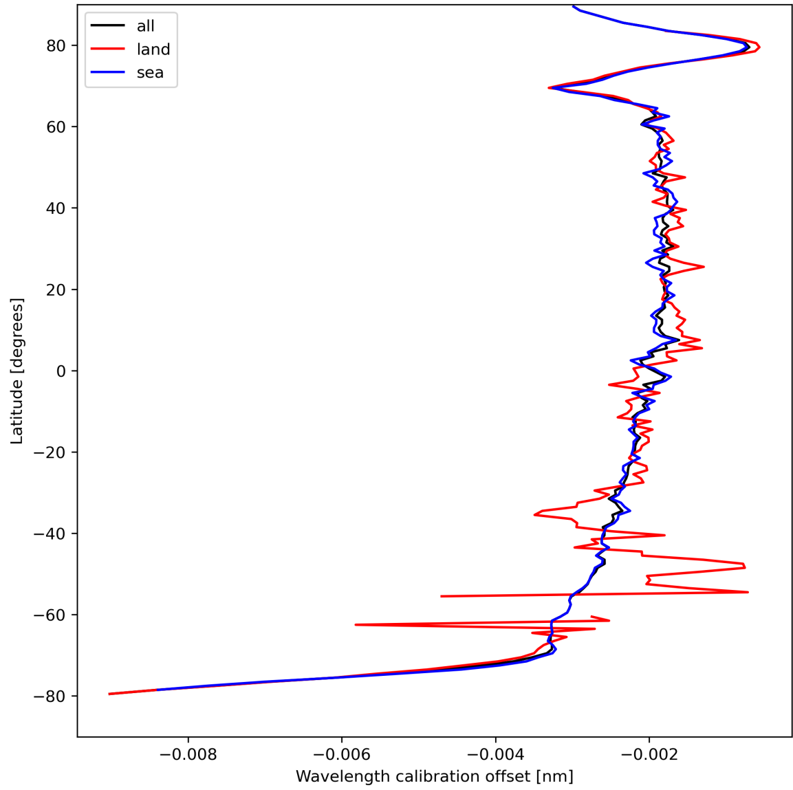
Figure 18: Zonal average of “Wavelength calibration offset” for 2024-04-10 to 2024-04-12.
