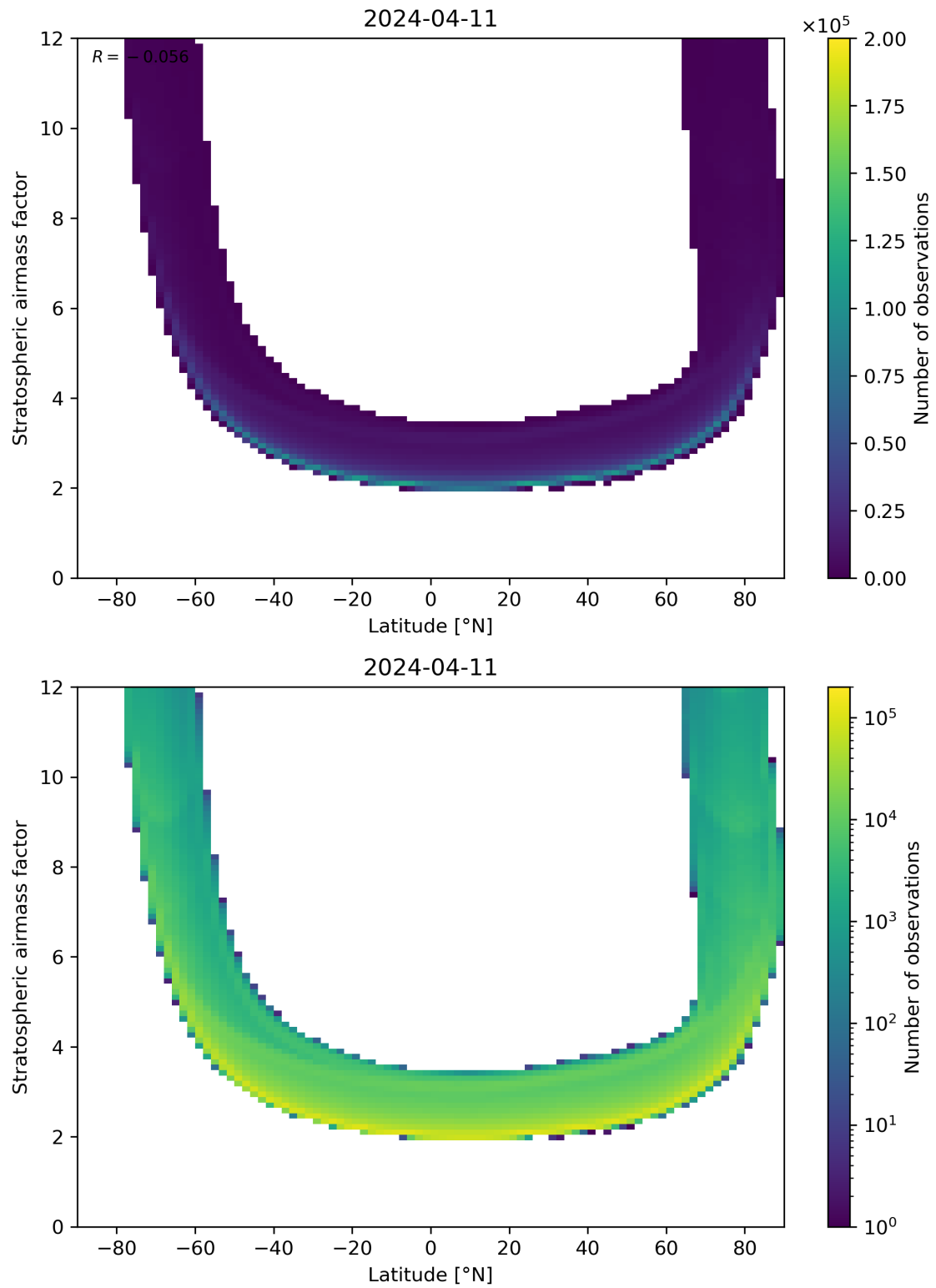
Figure 83: Scatter density plot of “Latitude” against “Stratospheric air mass factor” for 2024-04-10 to 2024-04-12.
