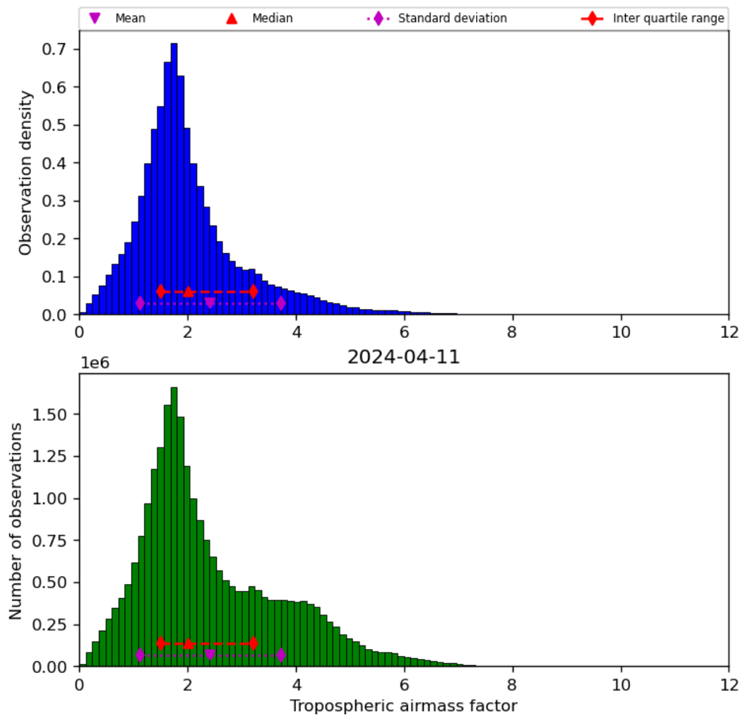
Figure 31: Histogram of “Tropospheric airmass factor” for 2024-04-10 to 2024-04-12
