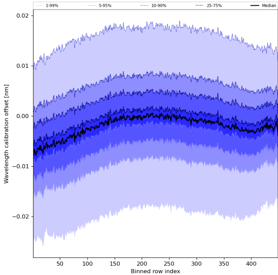
Figure 52: Along track statistics of “Wavelength calibration offset” for 2024-04-10 to 2024-04-12
