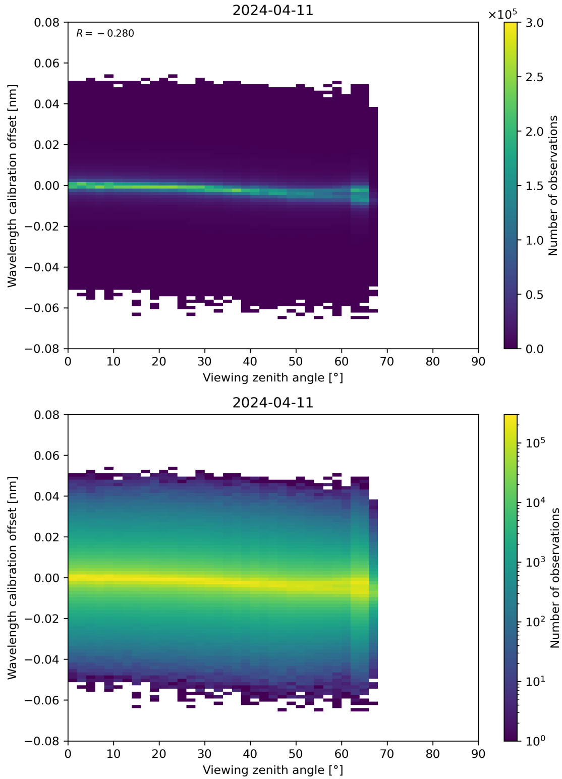
Figure 173: Scatter density plot of “Viewing zenith angle” against “Wavelength calibration offset” for 2024-04-10 to 2024-04-12.
