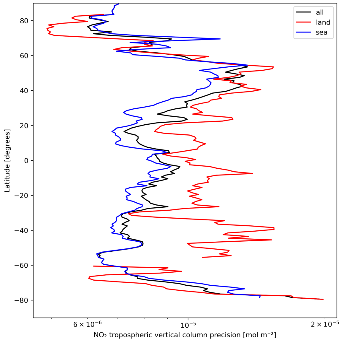
Figure 13: Zonal average of “NO 2 tropospheric vertical column precision” for 2024-04-10 to 2024-04-12.
