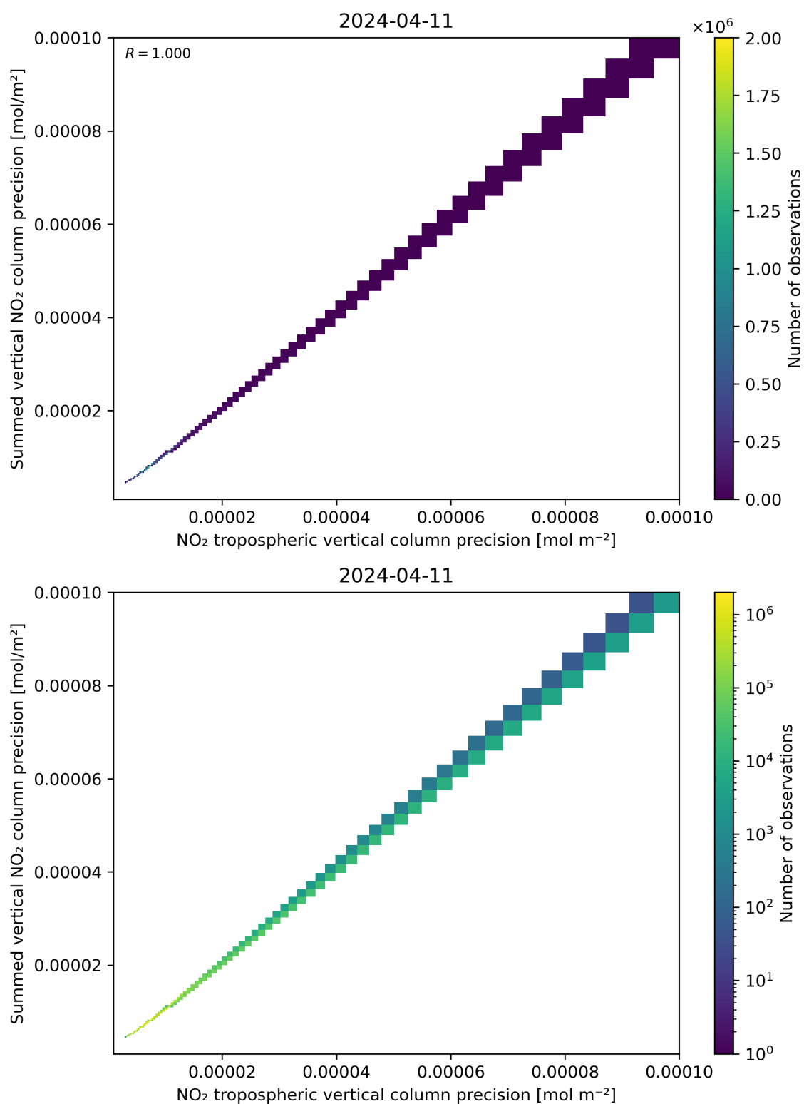
Figure 137: Scatter density plot of “NO 2 tropospheric vertical column precision” against “Summed vertical NO 2 column precision” for 2024-04-10 to 2024-04-12.
