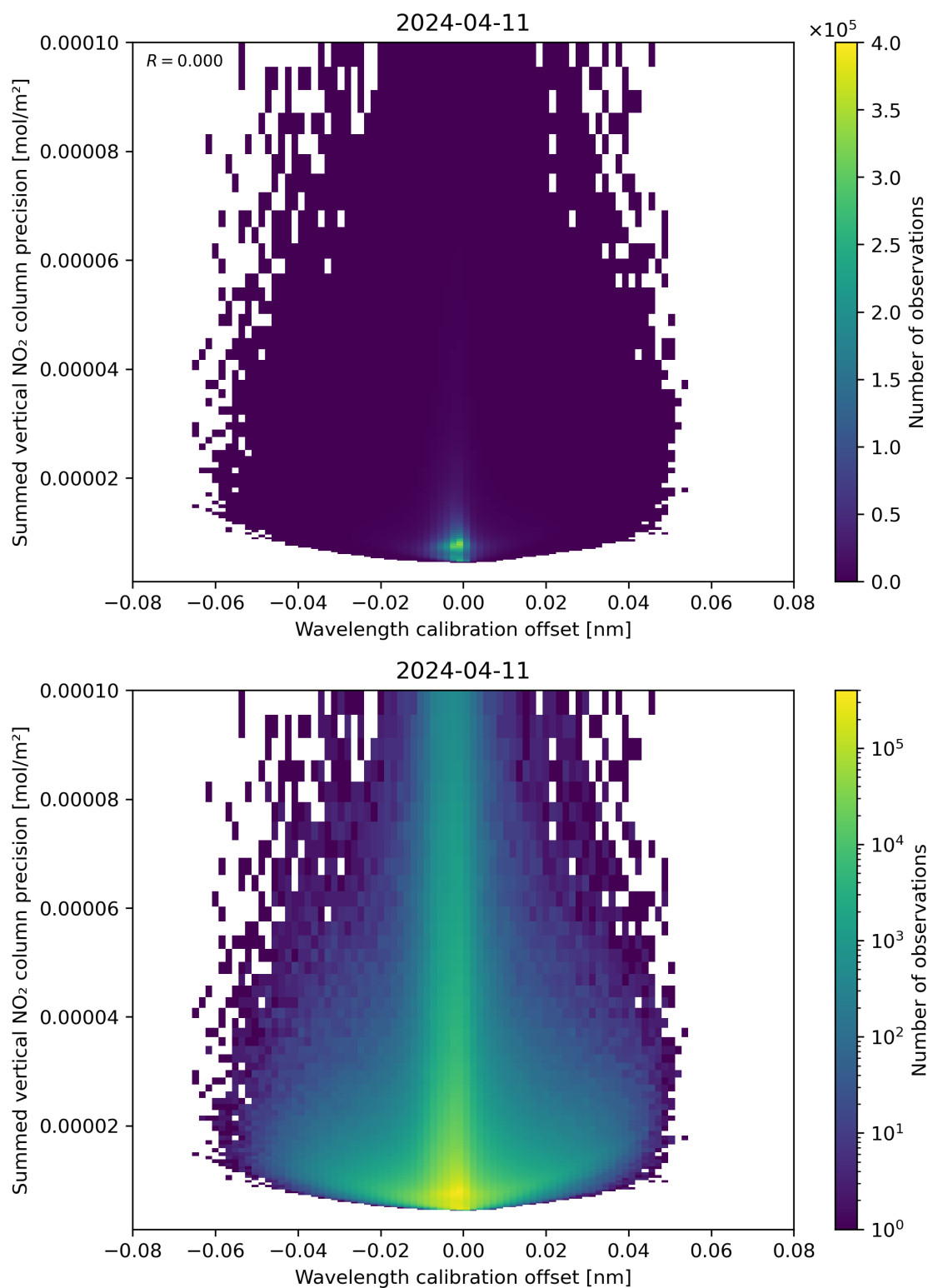
Figure 178: Scatter density plot of “Wavelength calibration offset” against “Summed vertical NO 2 column precision” for 2024-04-10 to 2024-04-12.
