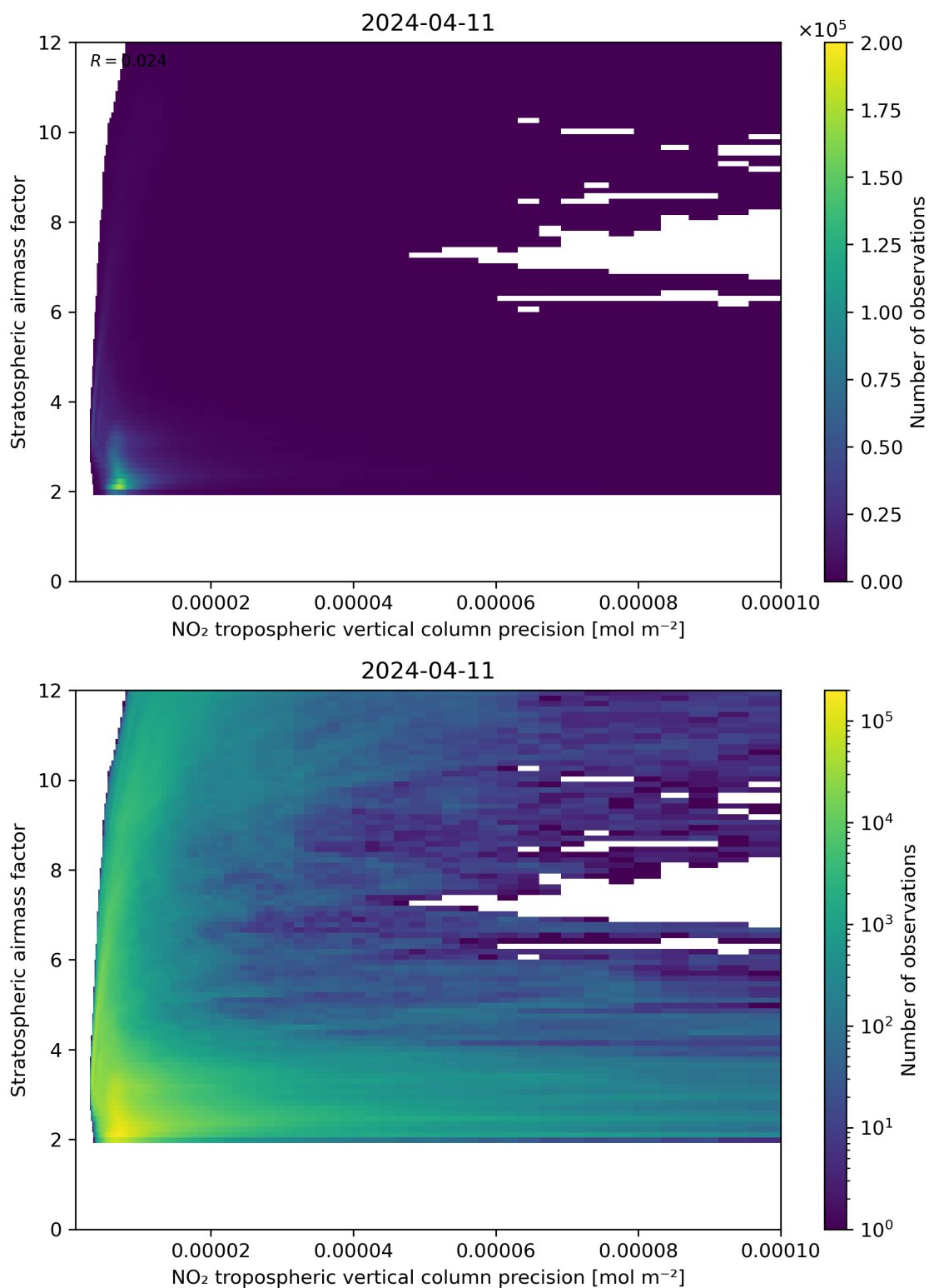
Figure 131: Scatter density plot of “NO 2 tropospheric vertical column precision” against “Stratospheric airmass factor” for 2024-04-10 to 2024-04-12.
