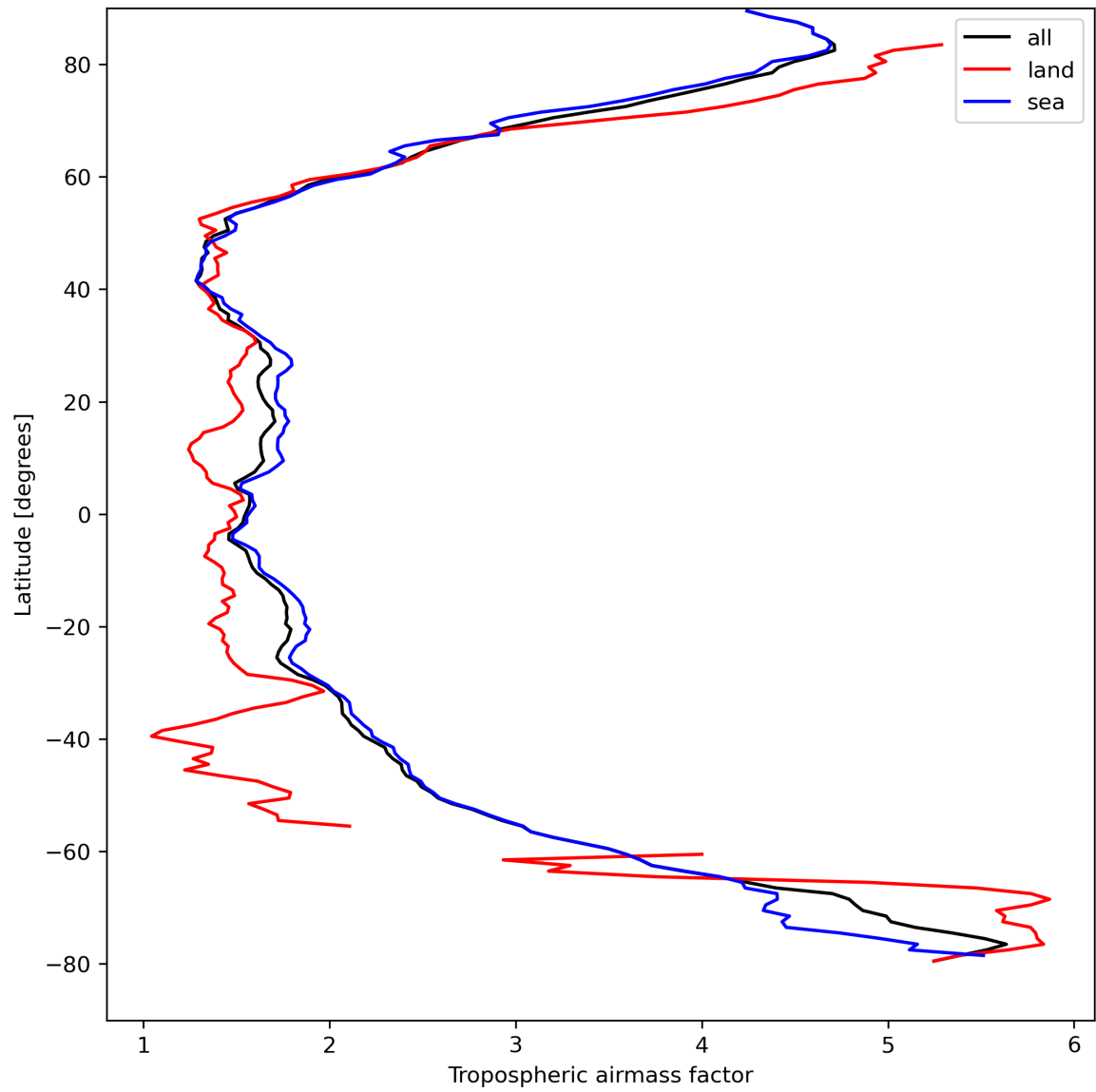
Figure 14: Zonal average of “Tropospheric airmass factor” for 2024-04-10 to 2024-04-12.
