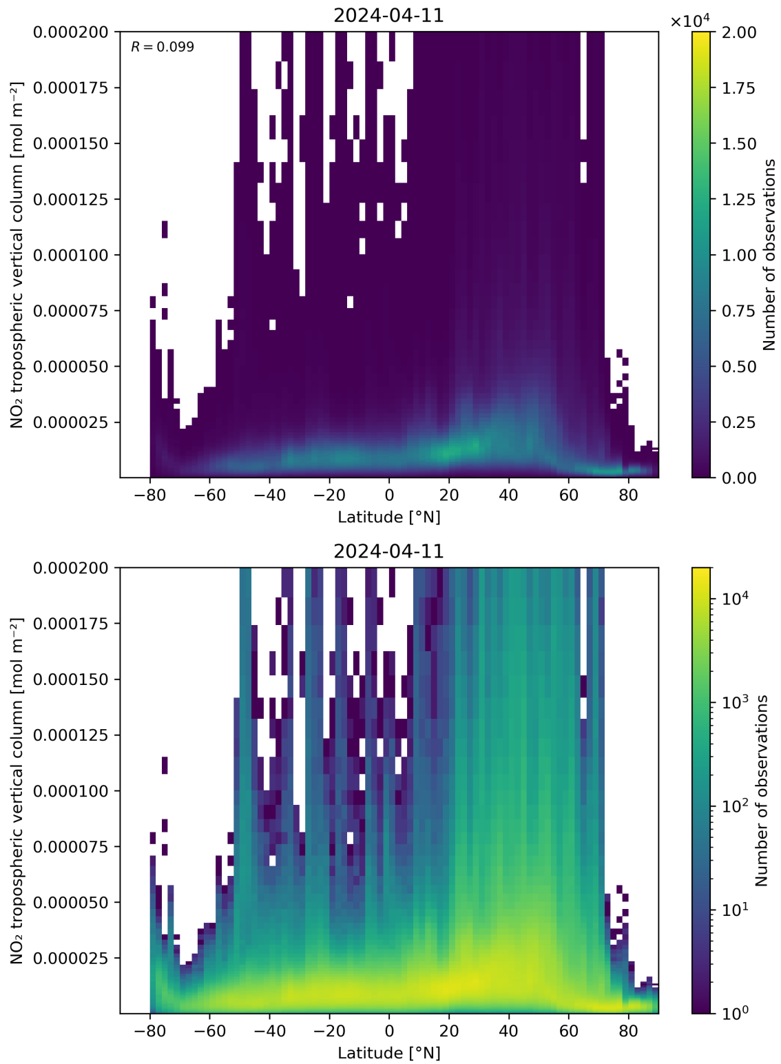
Figure 92: Scatter density plot of “Latitude” against “NO 2 tropospheric vertical column” for 2024-04-10 to 2024-04-12.
