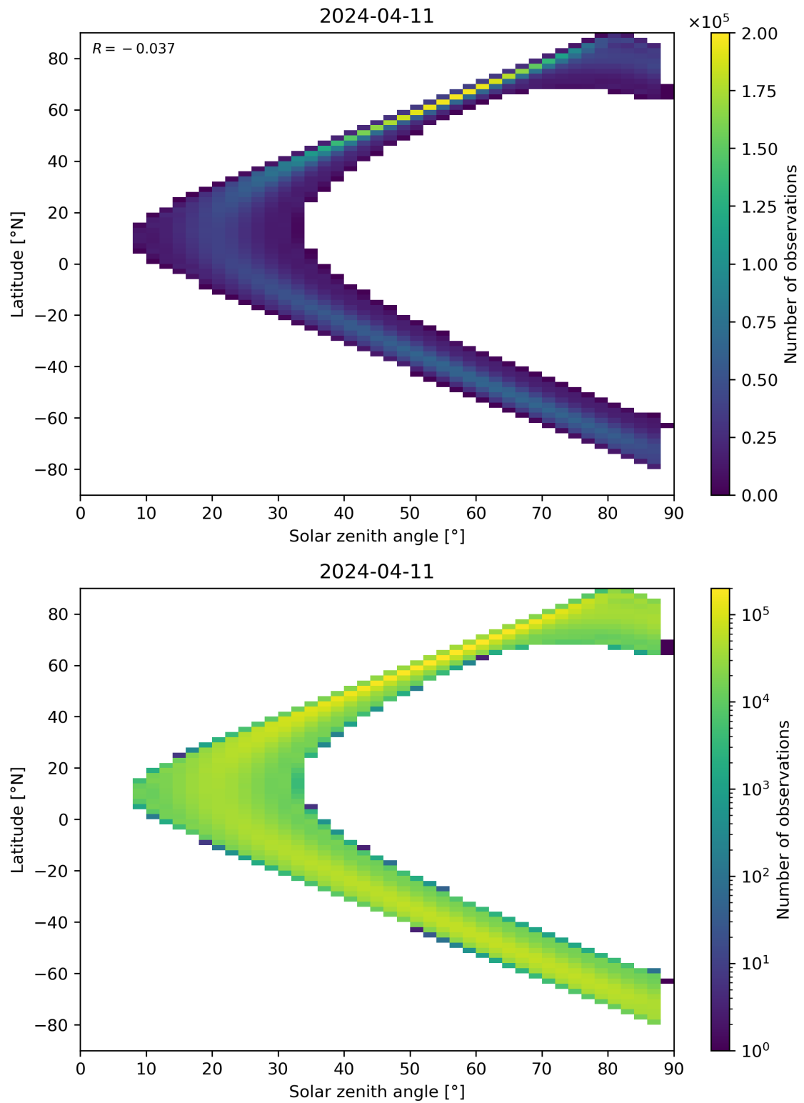
Figure 149: Scatter density plot of “Solar zenith angle” against “Latitude” for 2024-04-10 to 2024-04-12.
