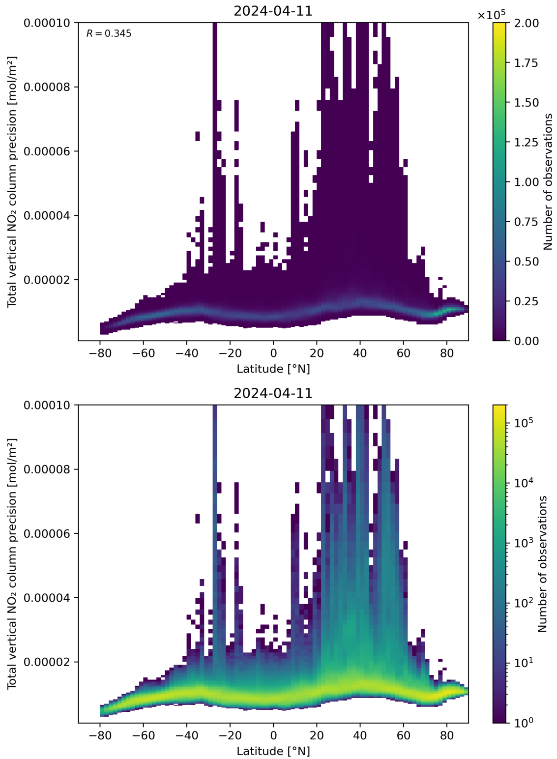
Figure 91: Scatter density plot of “Latitude” against “Total vertical NO 2 column precision” for 2024-04-10 to 2024-04-12.
