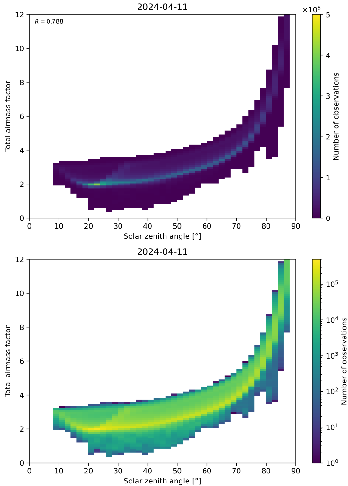
Figure 146: Scatter density plot of “Solar zenith angle” against “Total airmass factor” for 2024-04-10 to 2024-04-12.
