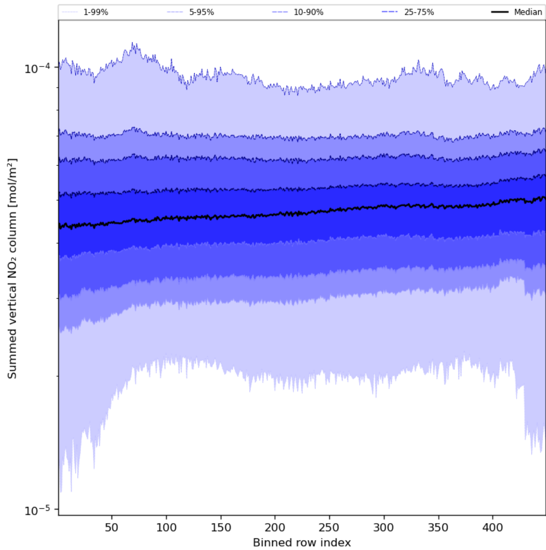
Figure 57: Along track statistics of “Summed vertical NO 2 column” for 2024-04-10 to 2024-04-12
