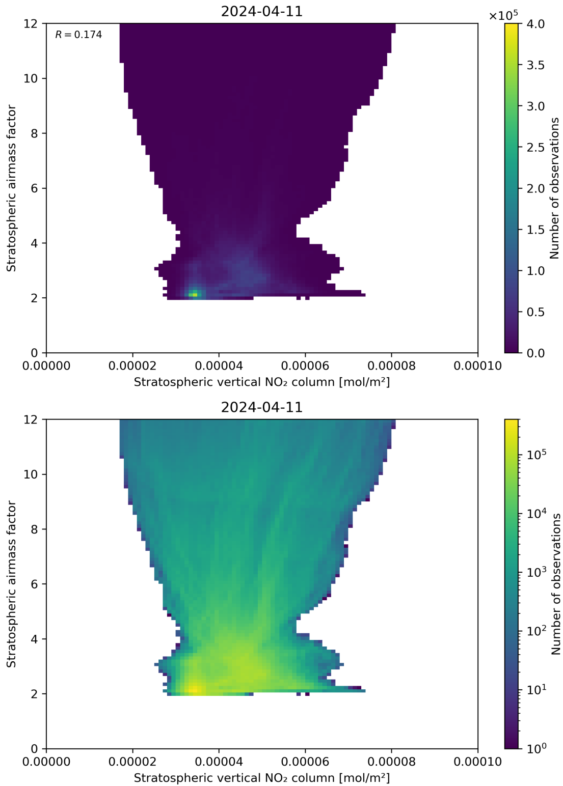
Figure 96: Scatter density plot of “Stratospheric vertical NO 2 column” against “Stratospheric airmass factor” for 2024-04-10 to 2024-04-12.
