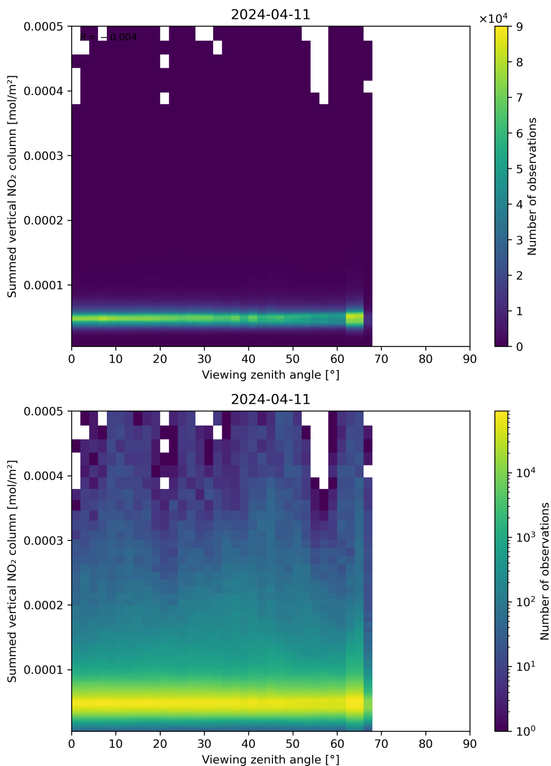
Figure 165: Scatter density plot of “Viewing zenith angle” against “Summed vertical NO 2 column” for 2024-04-10 to 2024-04-12.
