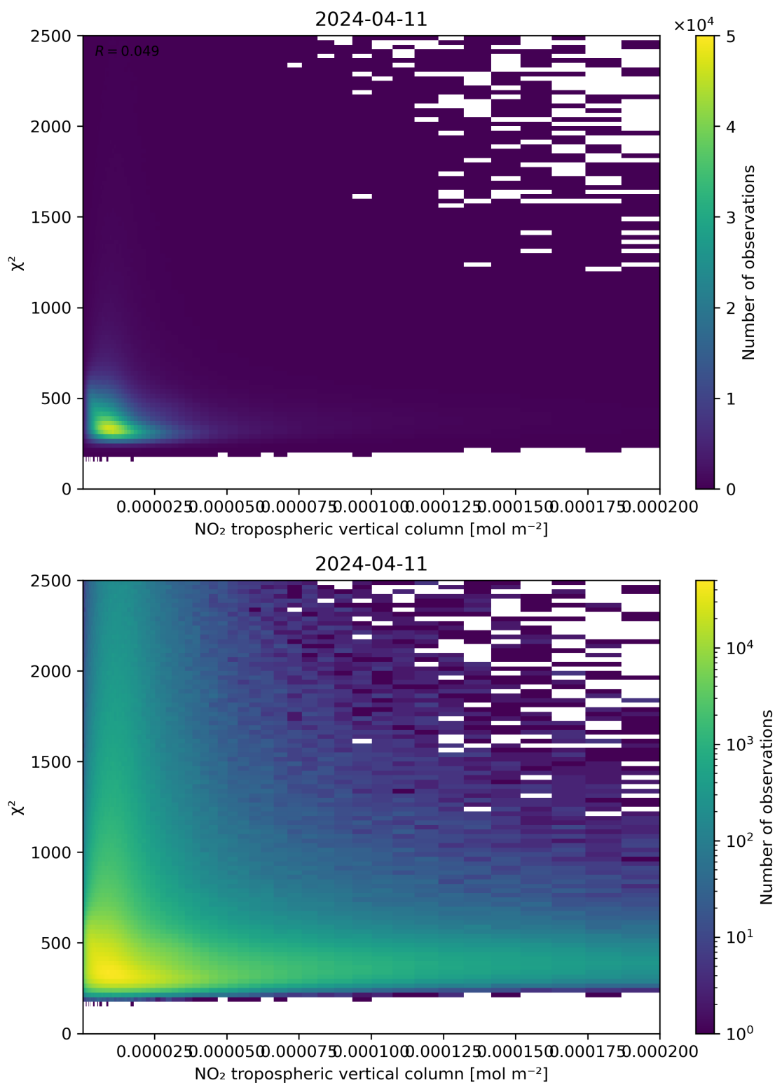
Figure 124: Scatter density plot of “NO 2 tropospheric vertical column” against “ \chi^2 ” for 2024-04-10 to 2024-04-12.
