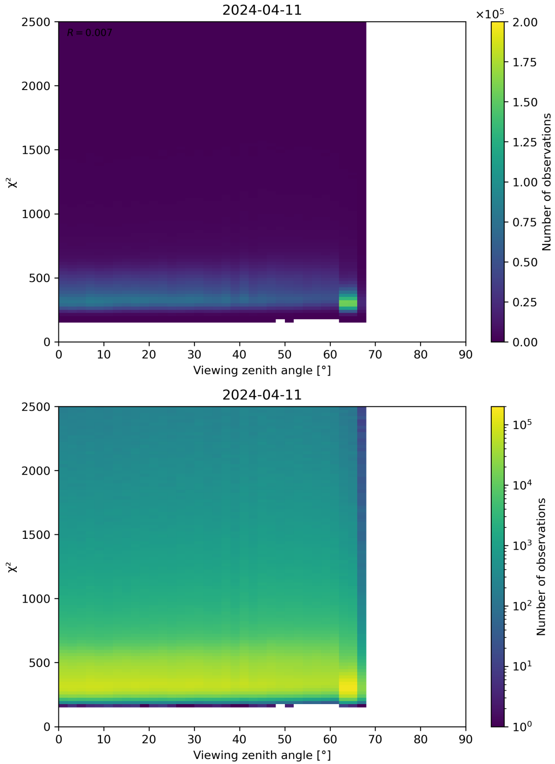
Figure 162: Scatter density plot of “Viewing zenith angle” against “ \chi^2 ” for 2024-04-10 to 2024-04-12.
