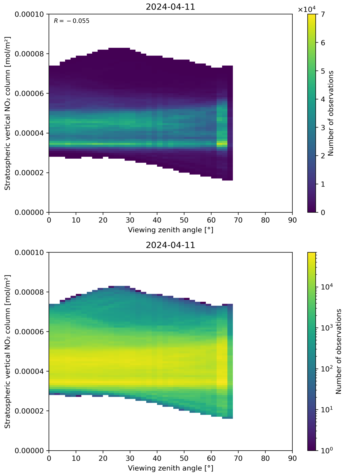
Figure 164: Scatter density plot of “Viewing zenith angle” against “Stratospheric vertical NO 2 column” for 2024-04-10 to 2024-04-12.
