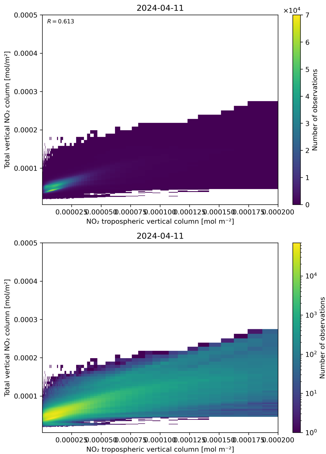
Figure 128: Scatter density plot of “NO 2 tropospheric vertical column” against “Total vertical NO 2 column” for 2024-04-10 to 2024-04-12.
