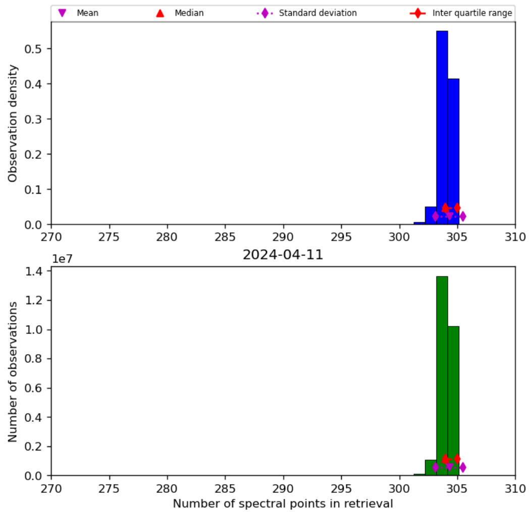
Figure 33: Histogram of “Number of spectral points in retrieval” for 2024-04-10 to 2024-04-12
