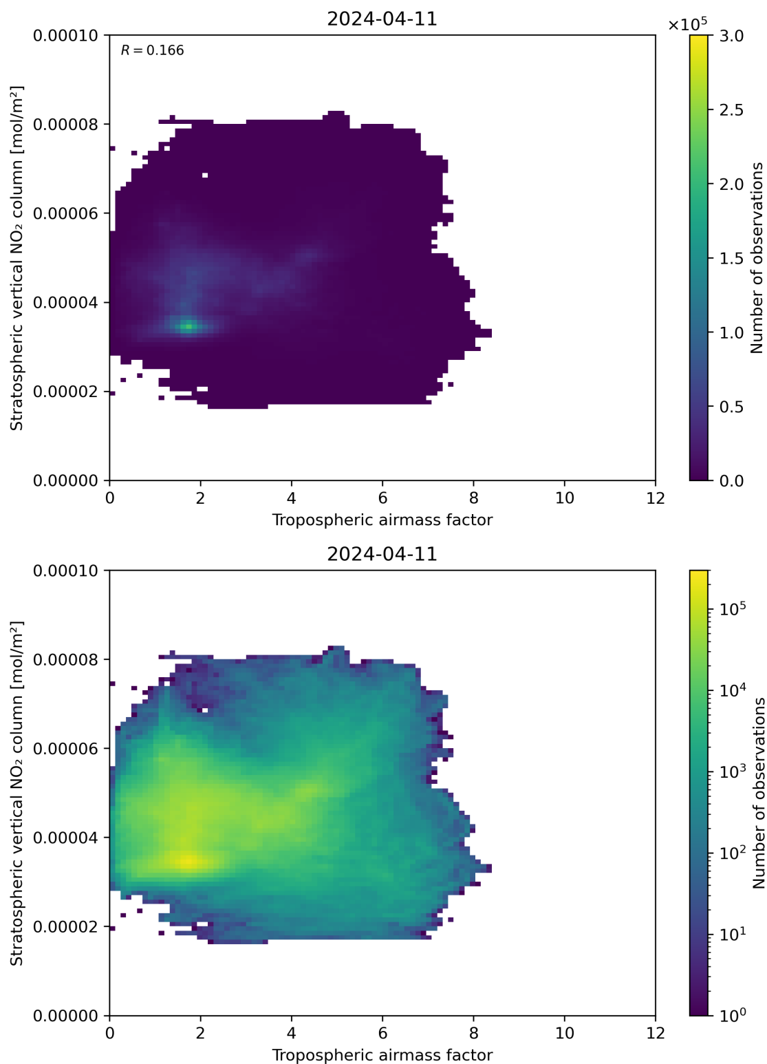
Figure 74: Scatter density plot of “Tropospheric air mass factor” against “Stratospheric vertical NO 2 column” for 2024-04-10 to 2024-04-12.
