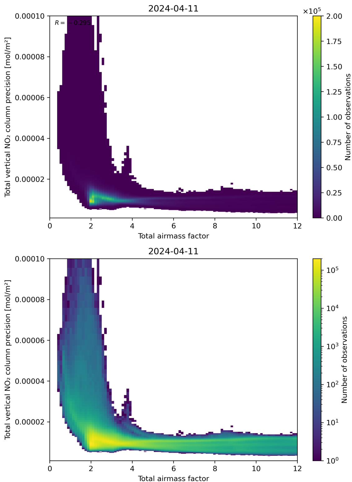
Figure 68: Scatter density plot of “Total airmass factor” against “Total vertical NO 2 column precision” for 2024-04-10 to 2024-04-12.
