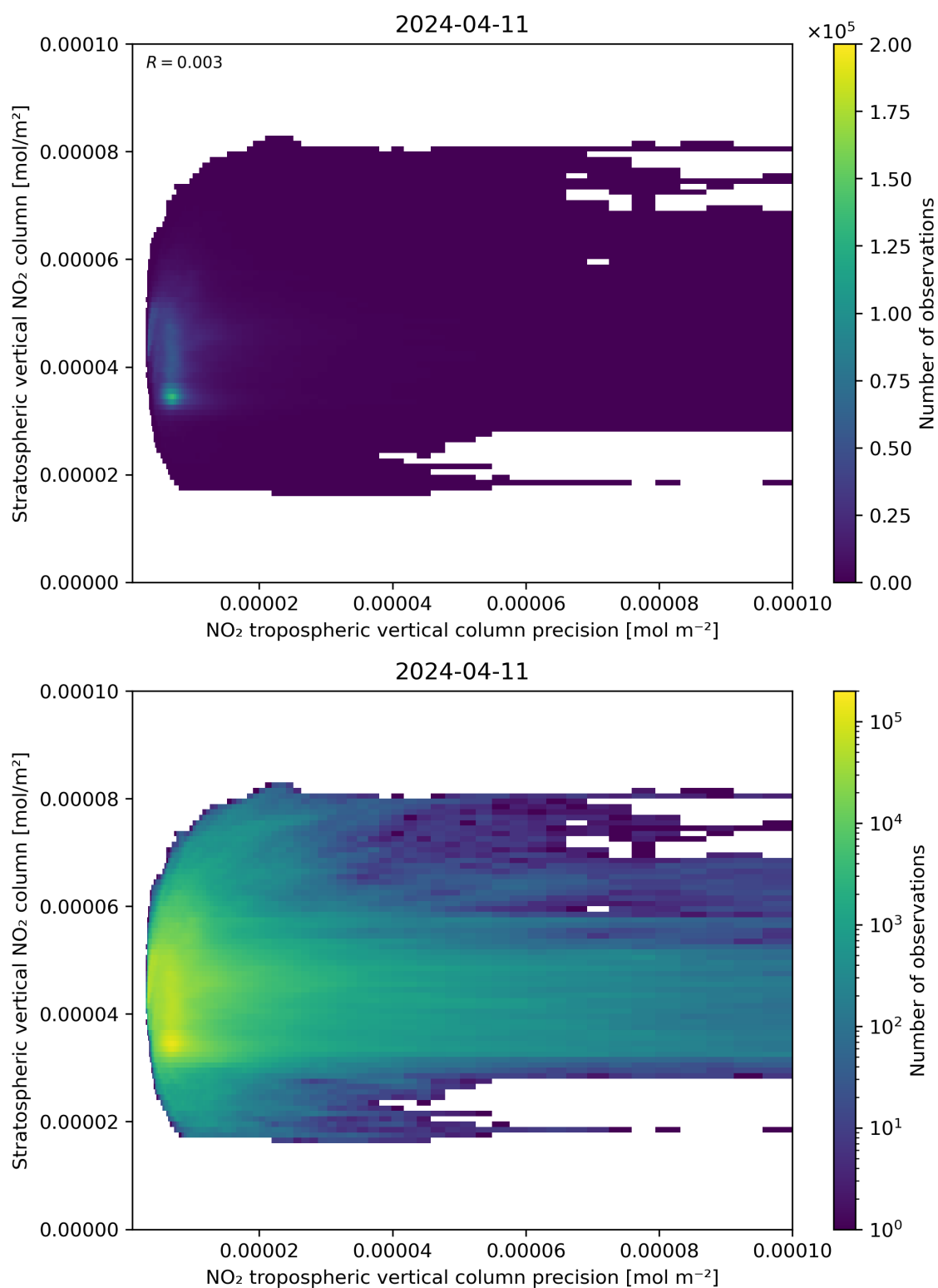
Figure 135: Scatter density plot of “NO 2 tropospheric vertical column precision” against “Stratospheric vertical NO 2 column” for 2024-04-10 to 2024-04-12.
