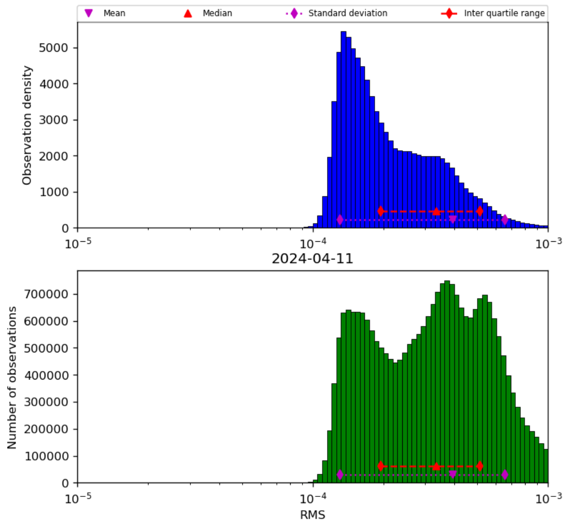
Figure 43: Histogram of “RMS” for 2024-04-10 to 2024-04-12
