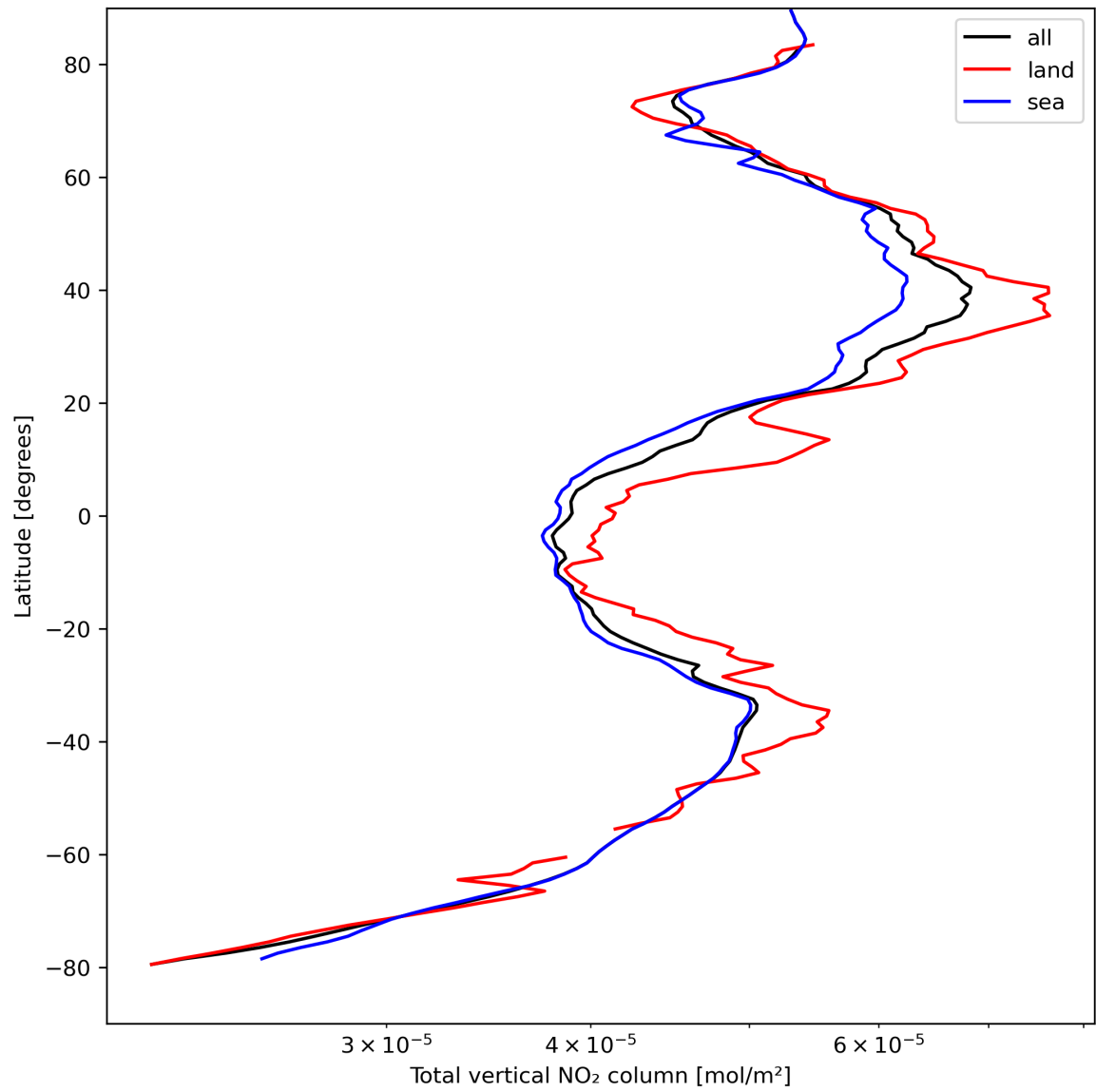
Figure 21: Zonal average of “Total vertical NO 2 column” for 2024-04-10 to 2024-04-12.
