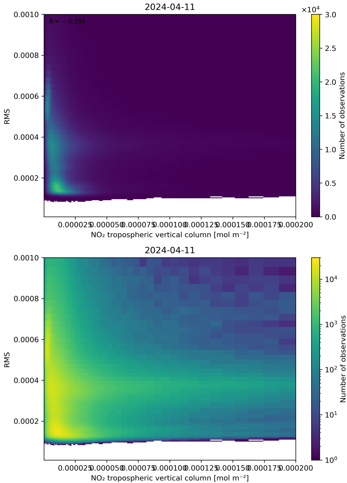
Figure 142: Scatter density plot of “NO 2 tropospheric vertical column” against “RMS” for 2024-04-10 to 2024-04-12.
