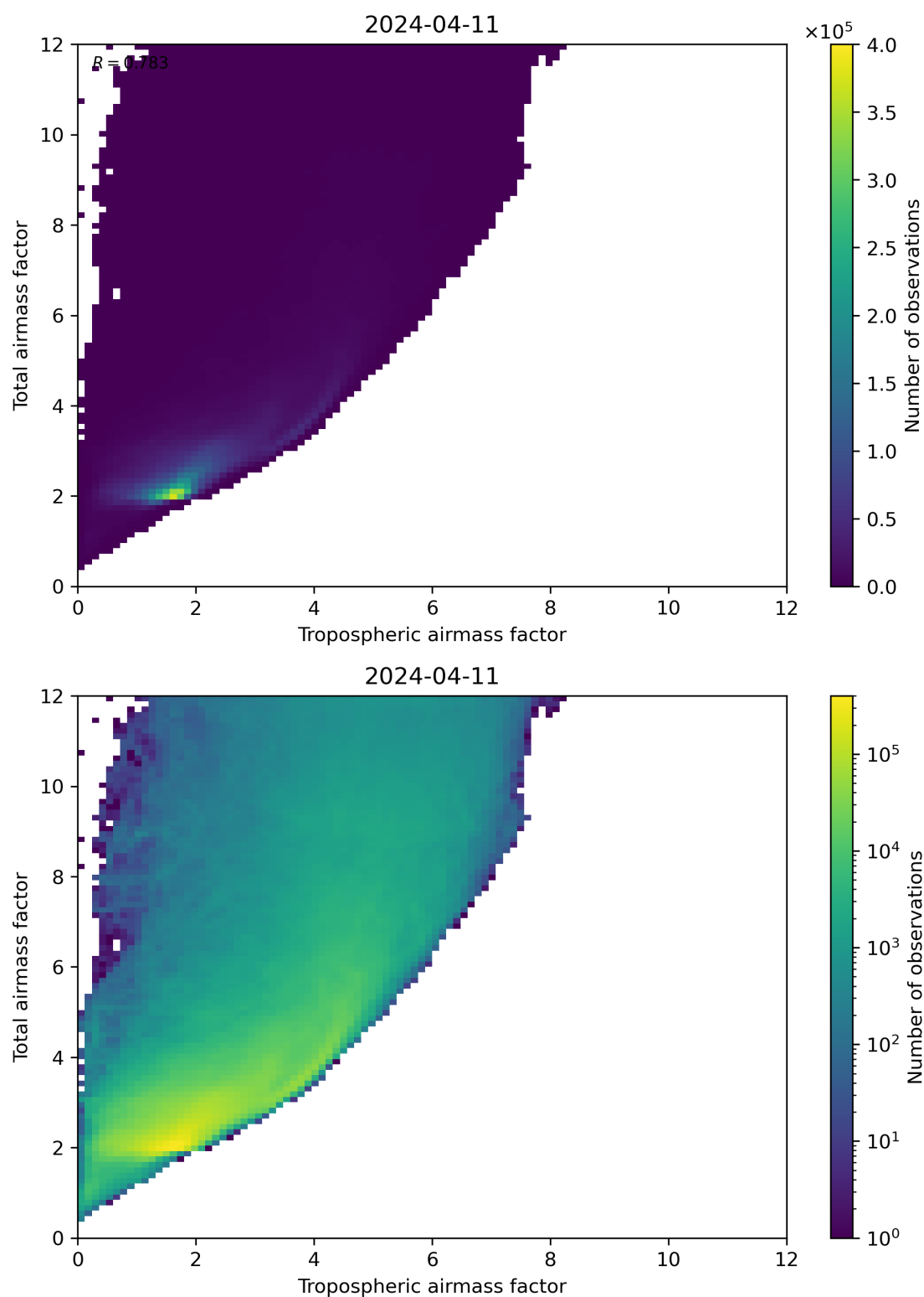
Figure 72: Scatter density plot of “Tropospheric airmass factor” against “Total airmass factor” for 2024-04-10 to 2024-04-12.
