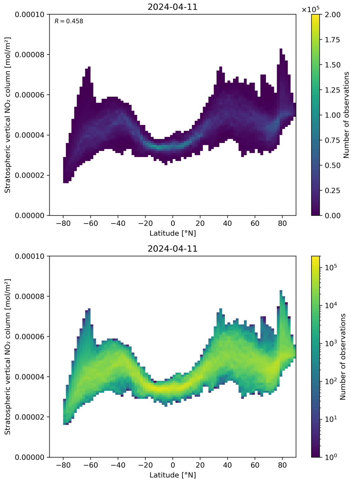
Figure 87: Scatter density plot of “Latitude” against “Stratospheric vertical NO 2 column” for 2024-04-10 to 2024-04-12.
