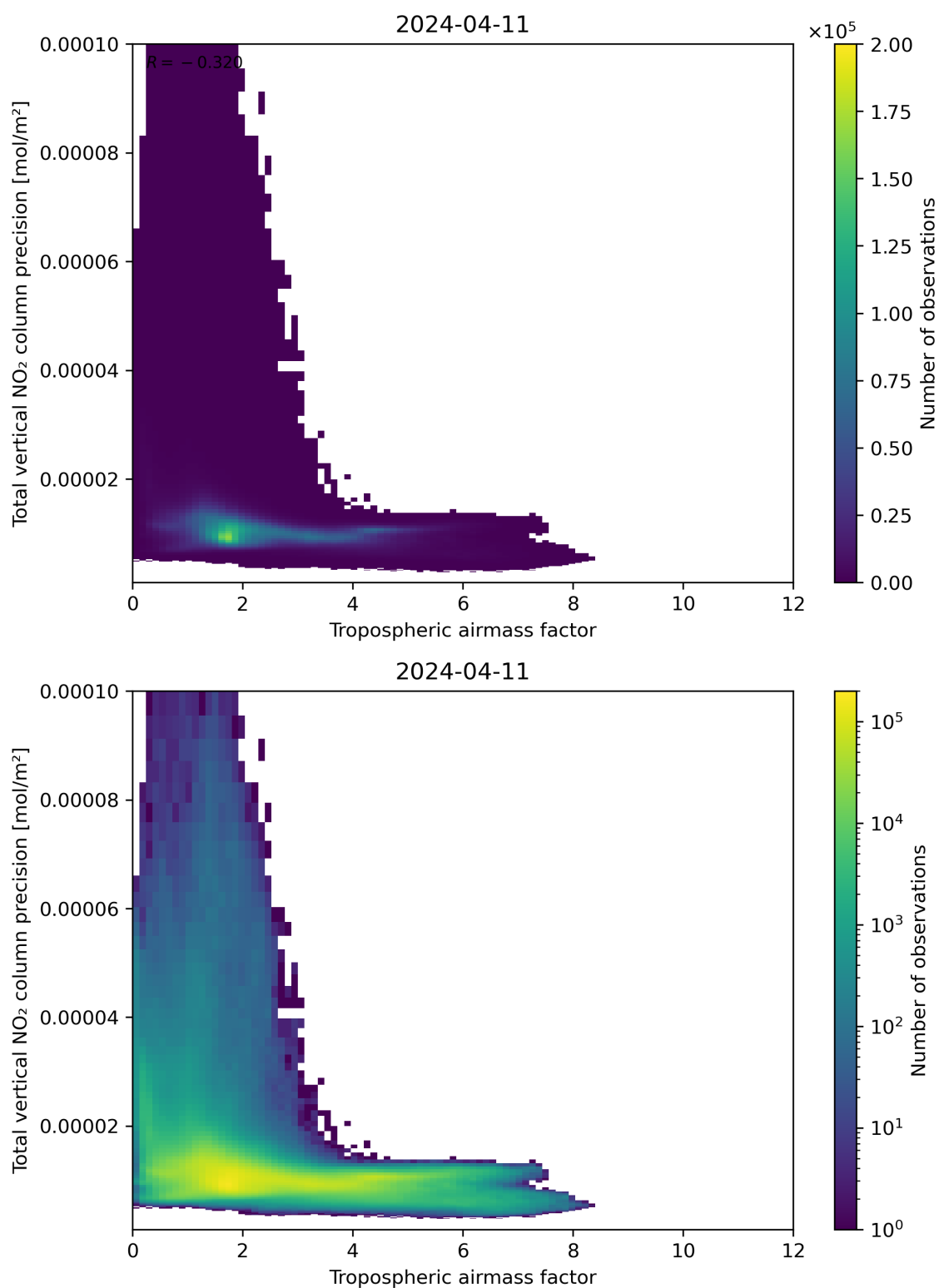
Figure 78: Scatter density plot of “Tropospheric air mass factor” against “Total vertical NO 2 column precision” for 2024-04-10 to 2024-04-12.
