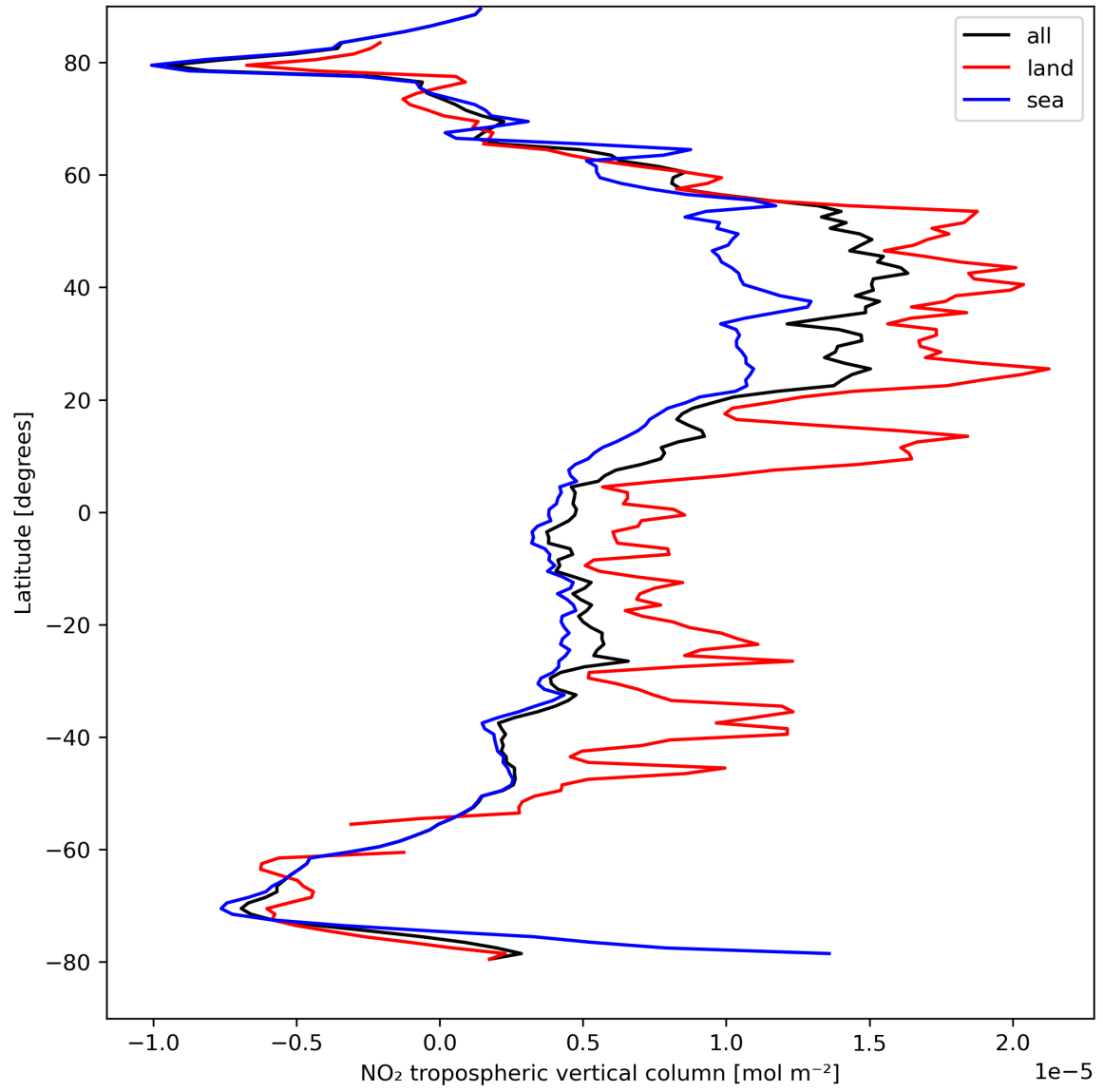
Figure 12: Zonal average of “NO 2 tropospheric vertical column” for 2024-04-10 to 2024-04-12.
