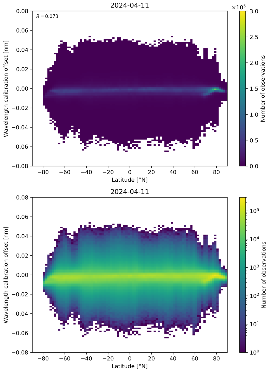
Figure 95: Scatter density plot of “Latitude” against “Wavelength calibration offset” for 2024-04-10 to 2024-04-12.
