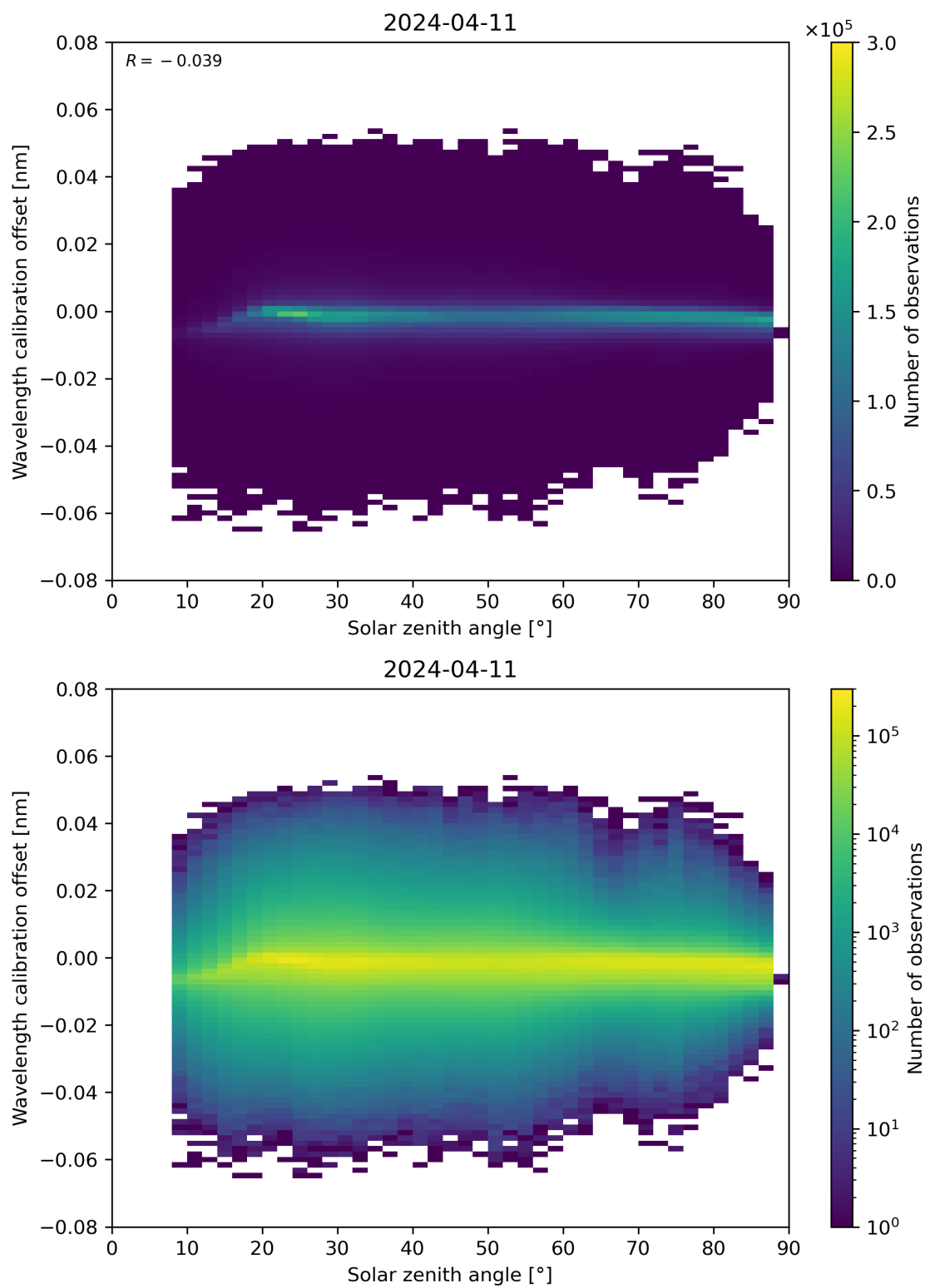
Figure 158: Scatter density plot of “Solar zenith angle” against “Wavelength calibration offset” for 2024-04-10 to 2024-04-12.
