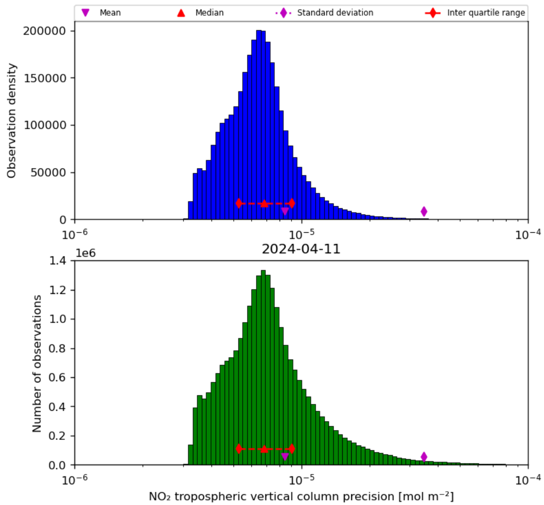
Figure 30: Histogram of "NO 2 tropospheric vertical column precision" for 2024-04-10 to 2024-04-12
