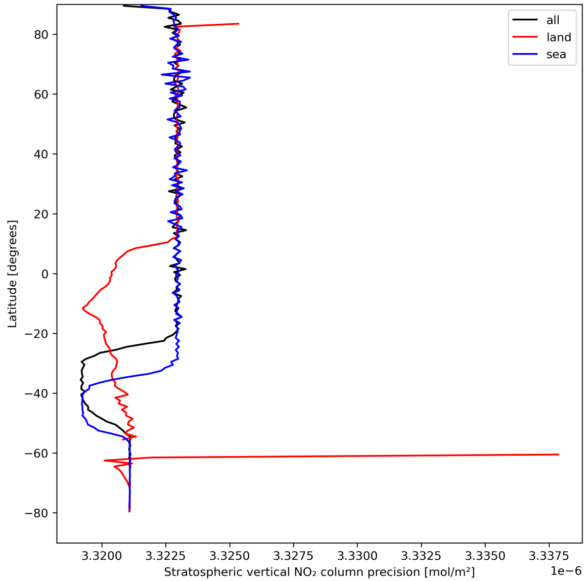
Figure 20: Zonal average of “Stratospheric vertical NO 2 column precision” for 2024-04-10 to 2024-04-12.
