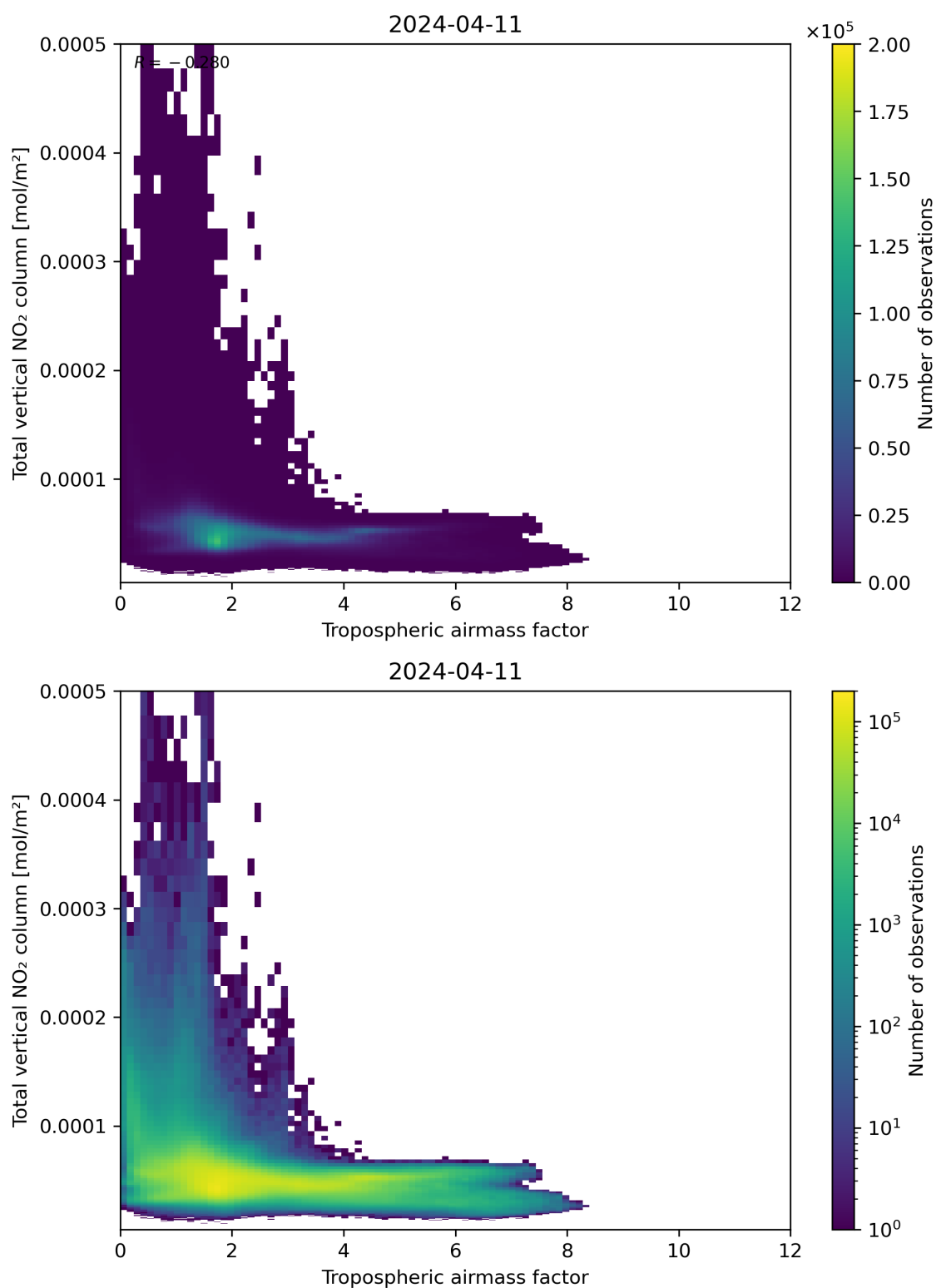
Figure 77: Scatter density plot of “Tropospheric airmass factor” against “Total vertical NO 2 column” for 2024-04-10 to 2024-04-12.
