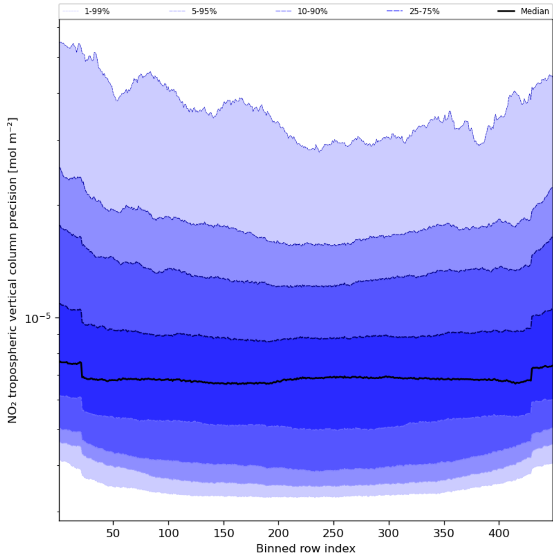
Figure 47: Along track statistics of “NO 2 tropospheric vertical column precision” for 2024-04-10 to 2024-04-12
