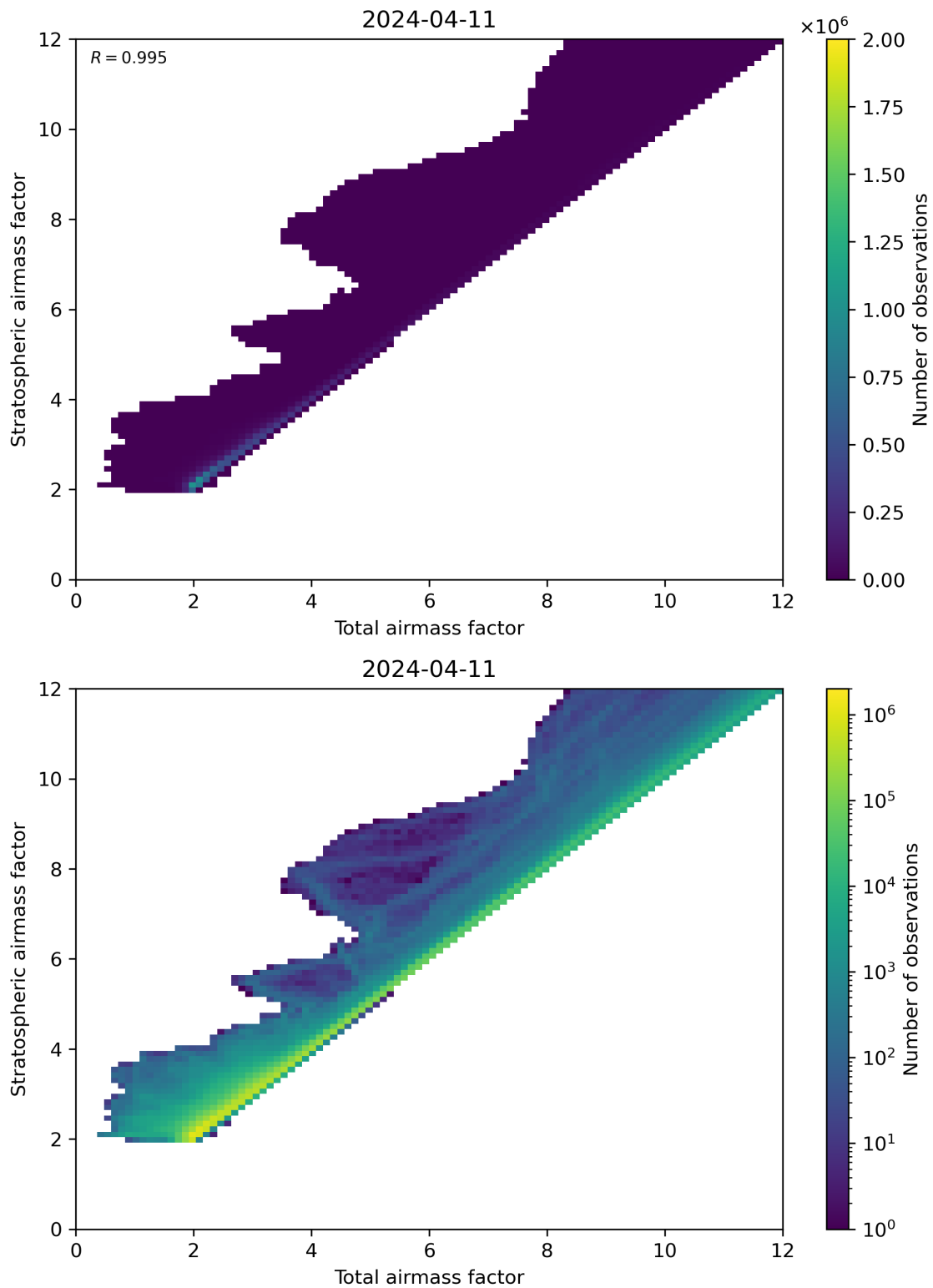
Figure 62: Scatter density plot of “Total airmass factor” against “Stratospheric airmass factor” for 2024-04-10 to 2024-04-12.
