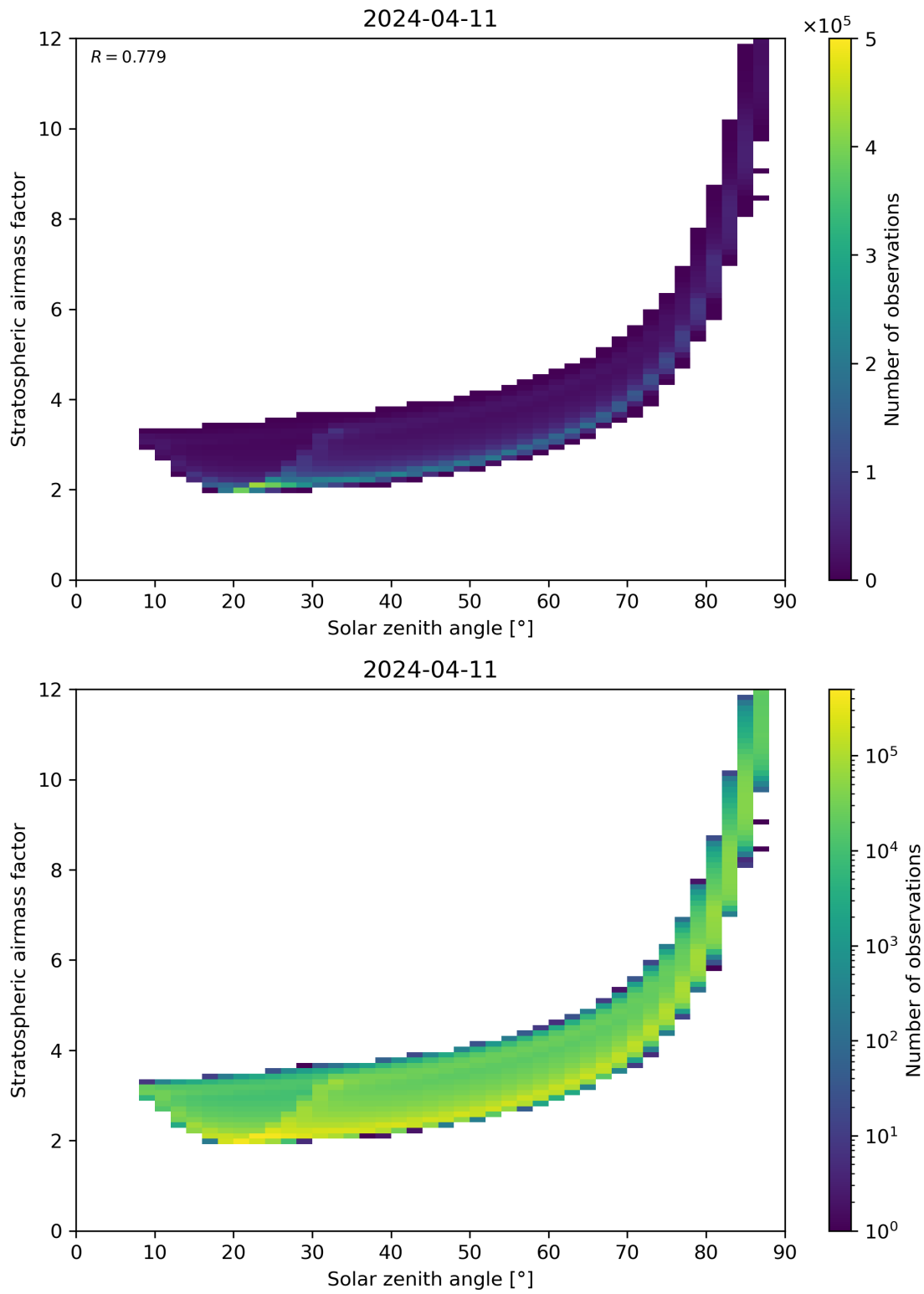
Figure 145: Scatter density plot of “Solar zenith angle” against “Stratospheric airmass factor” for 2024-04-10 to 2024-04-12.
