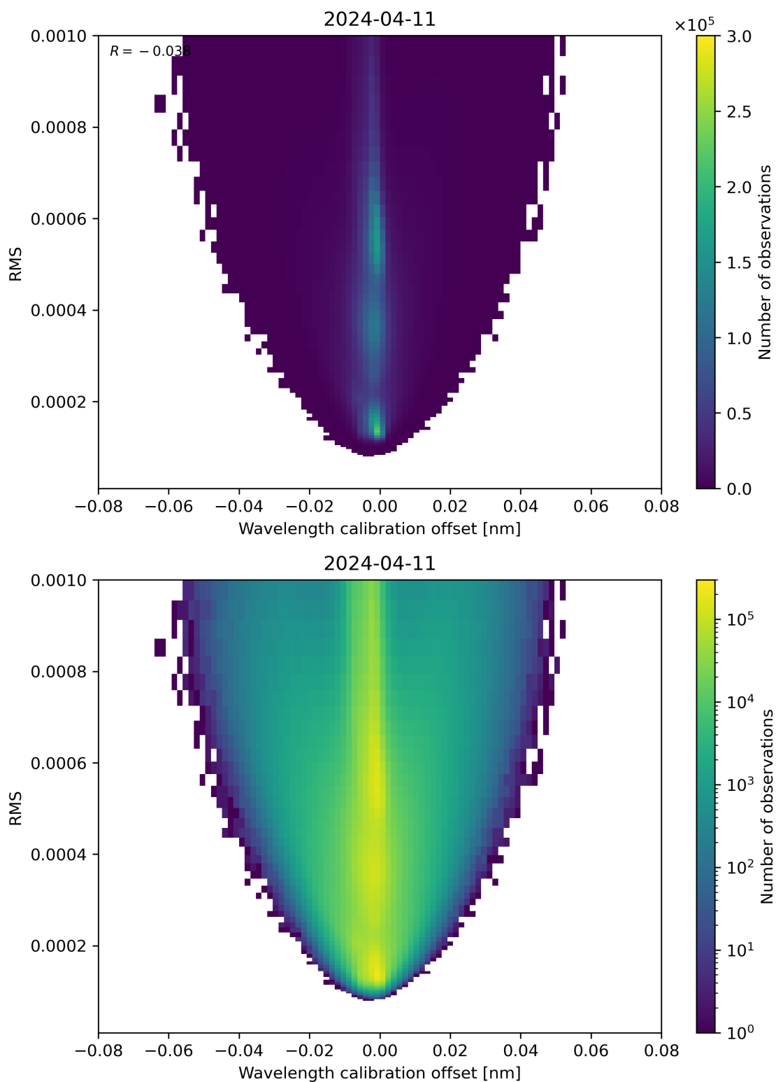
Figure 181: Scatter density plot of “Wavelength calibration offset” against “RMS” for 2024-04-10 to 2024-04-12.
