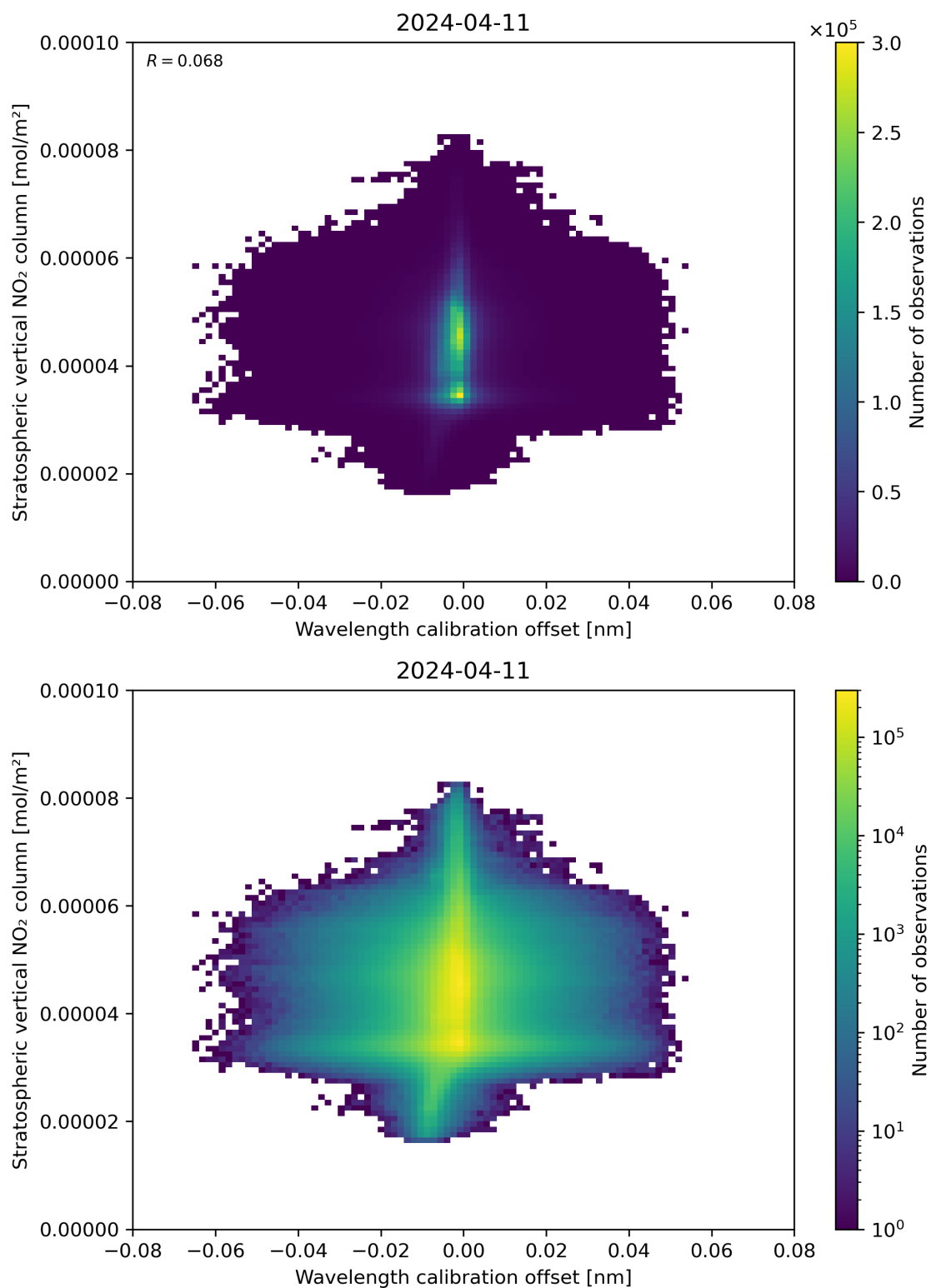
Figure 176: Scatter density plot of “Wavelength calibration offset” against “Stratospheric vertical NO 2 column” for 2024-04-10 to 2024-04-12.
