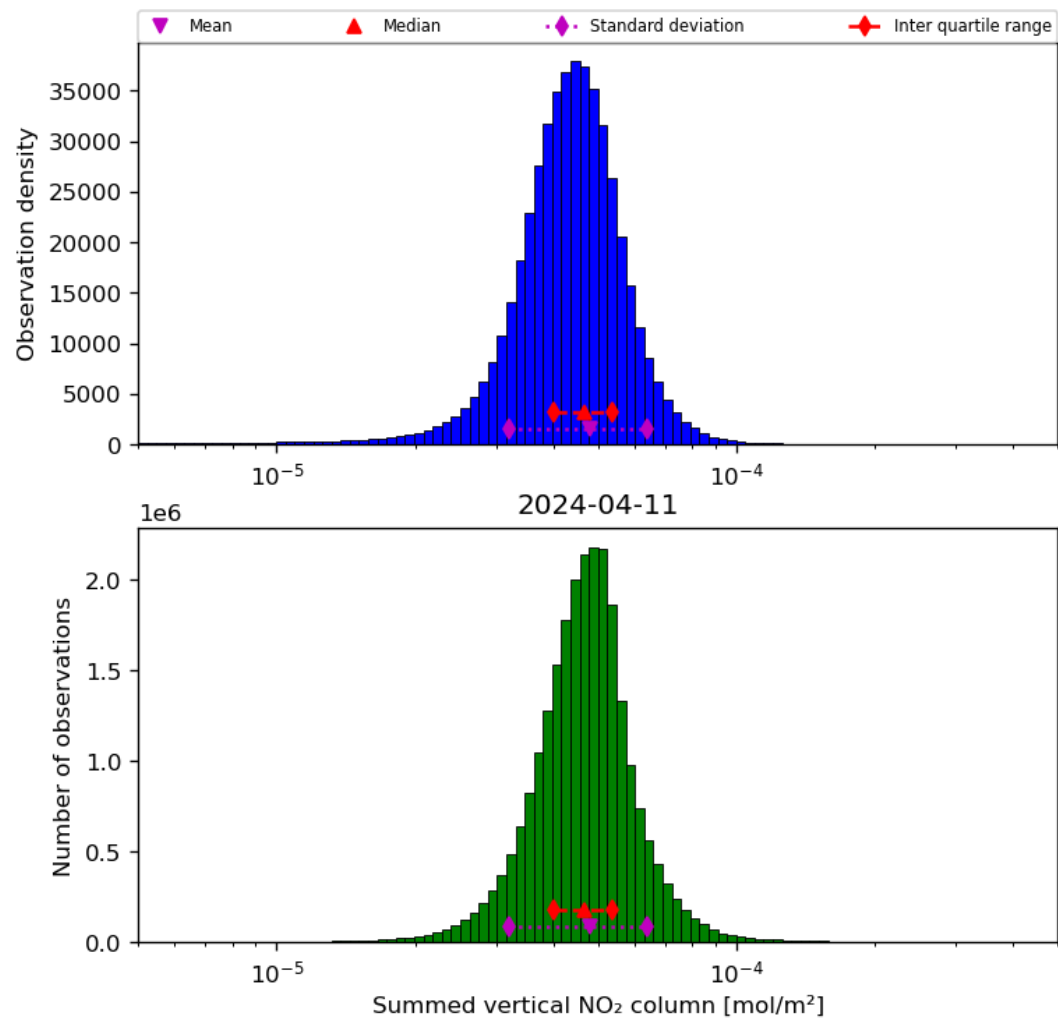
Figure 40: Histogram of “Summed vertical NO 2 column” for 2024-04-10 to 2024-04-12
