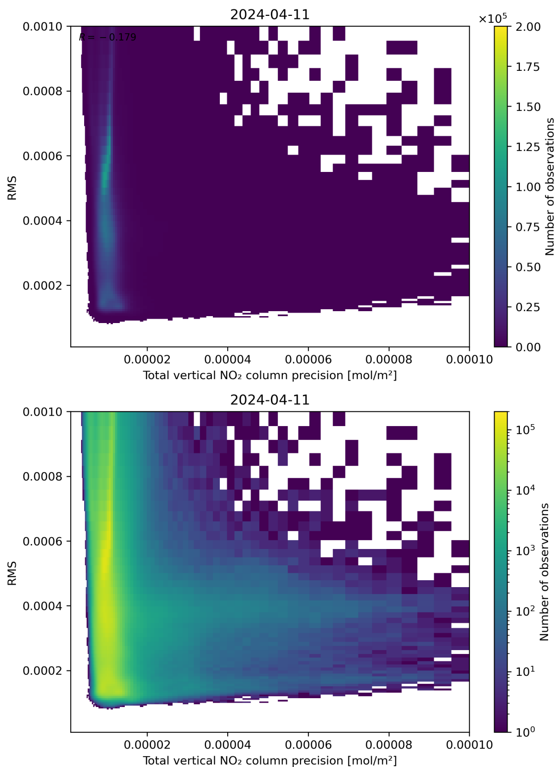
Figure 119: Scatter density plot of “Total vertical NO 2 column precision” against “RMS” for 2024-04-10 to 2024-04-12.
