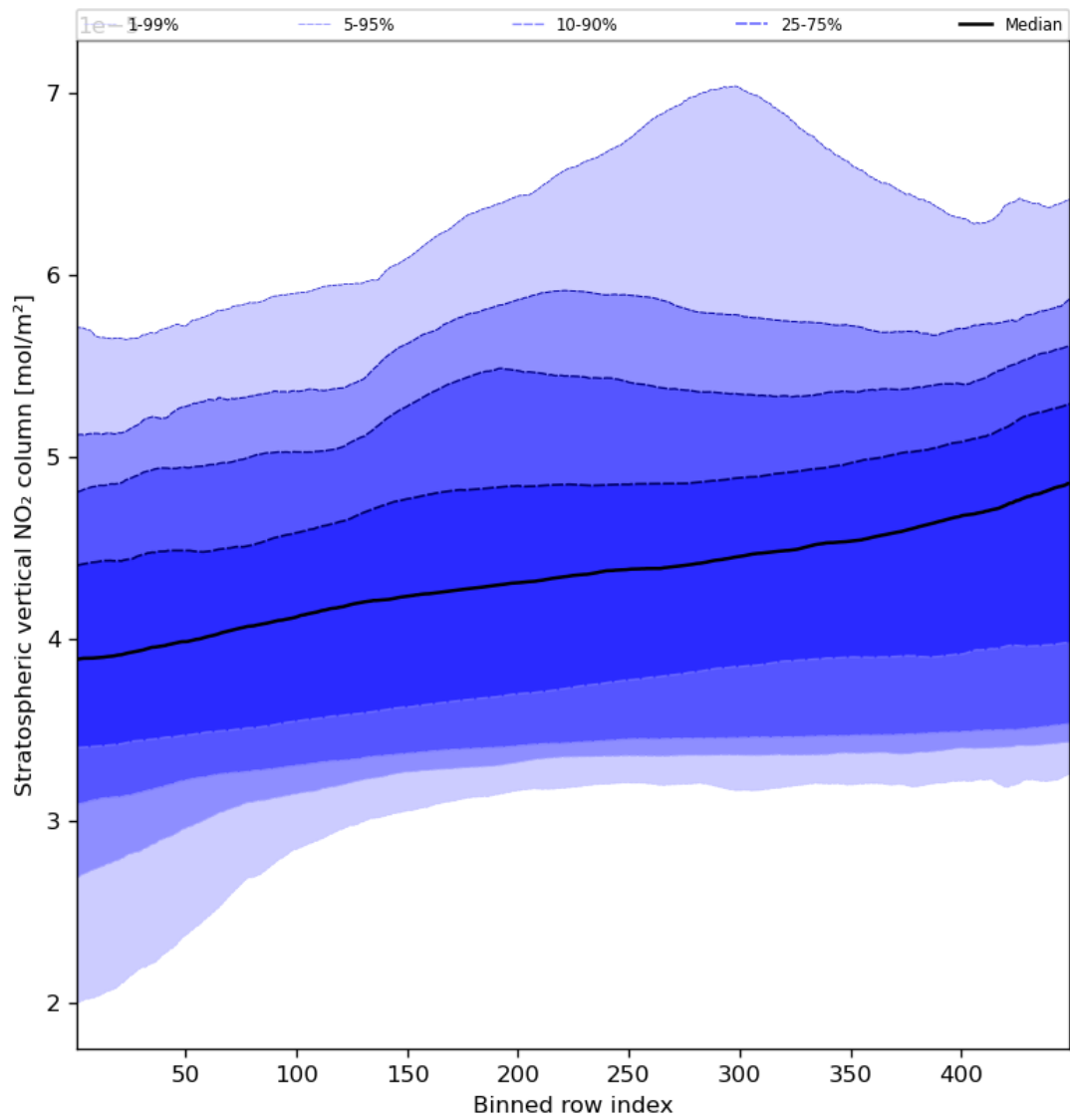
Figure 53: Along track statistics of “Stratospheric vertical NO 2 column” for 2024-04-10 to 2024-04-12
