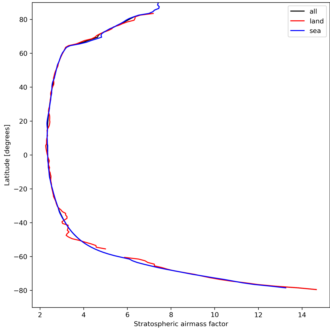
Figure 27: Zonal average of “Stratospheric air mass factor” for 2024-04-10 to 2024-04-12.
