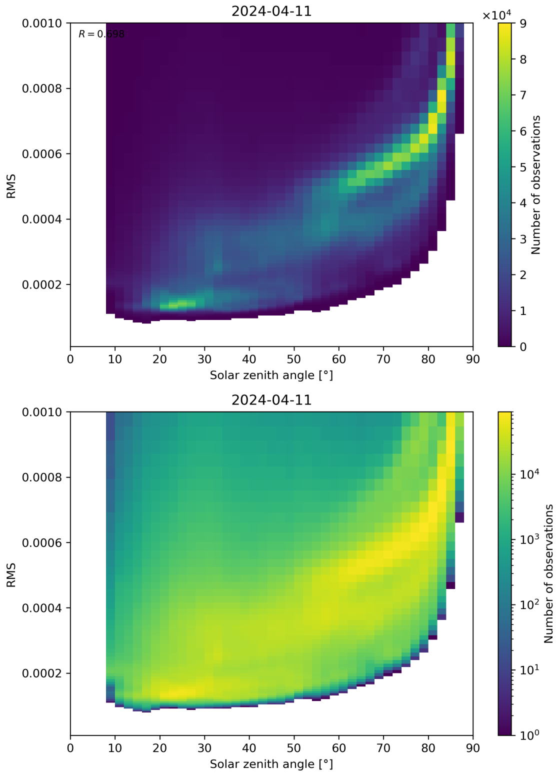
Figure 157: Scatter density plot of “Solar zenith angle” against “RMS” for 2024-04-10 to 2024-04-12.
