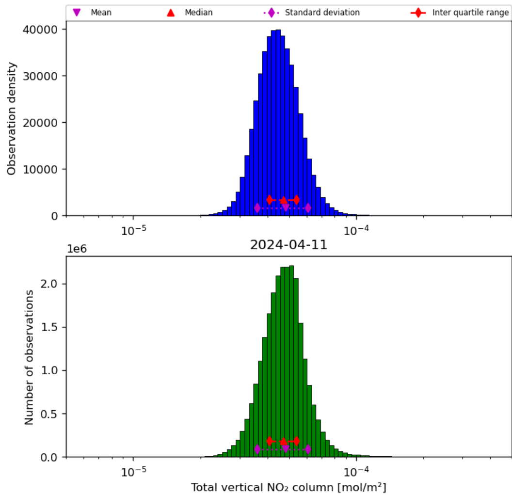
Figure 38: Histogram of “Total vertical NO 2 column” for 2024-04-10 to 2024-04-12
