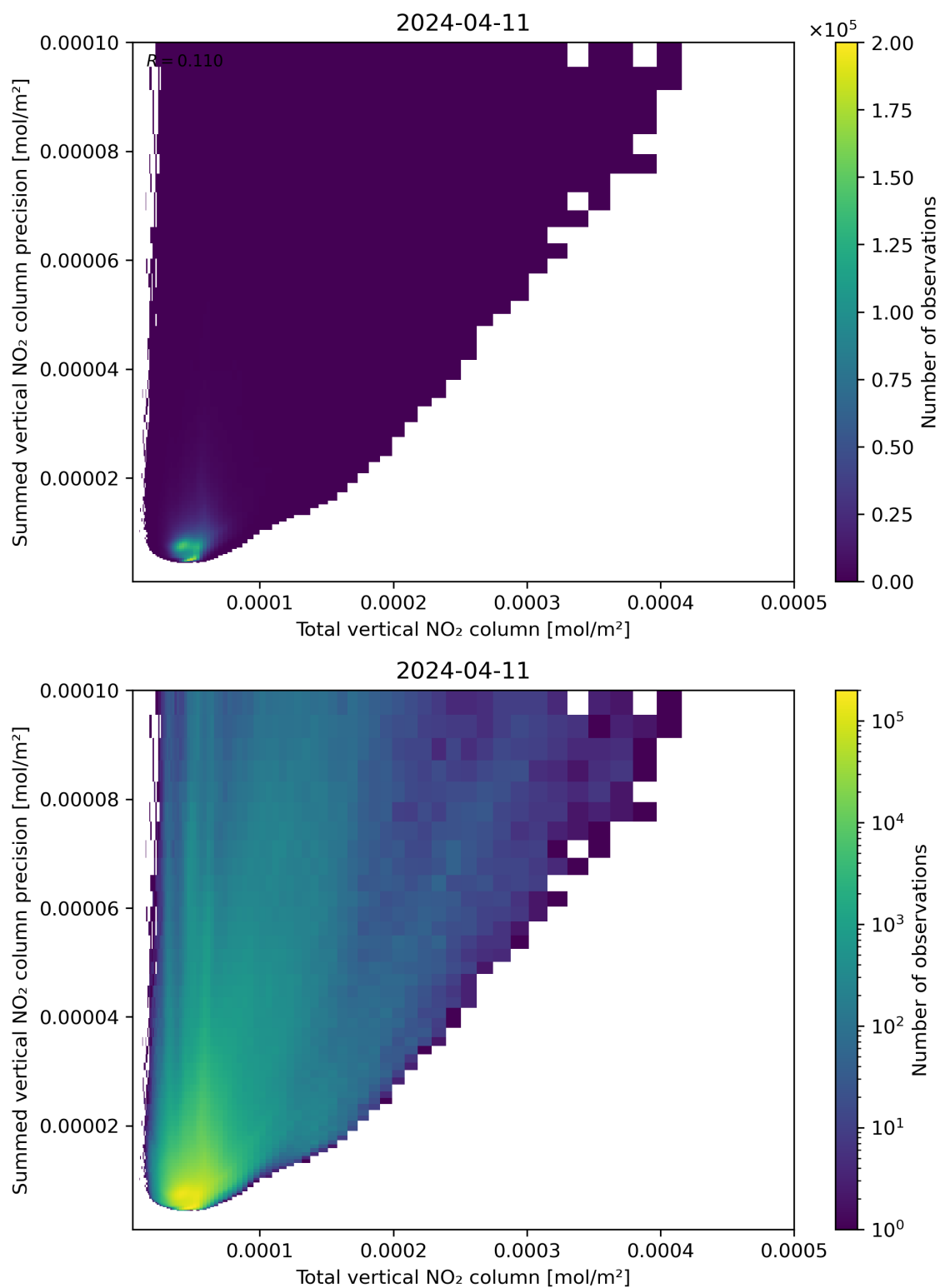
Figure 113: Scatter density plot of “Total vertical NO 2 column” against “Summed vertical NO 2 column precision” for 2024-04-10 to 2024-04-12.
