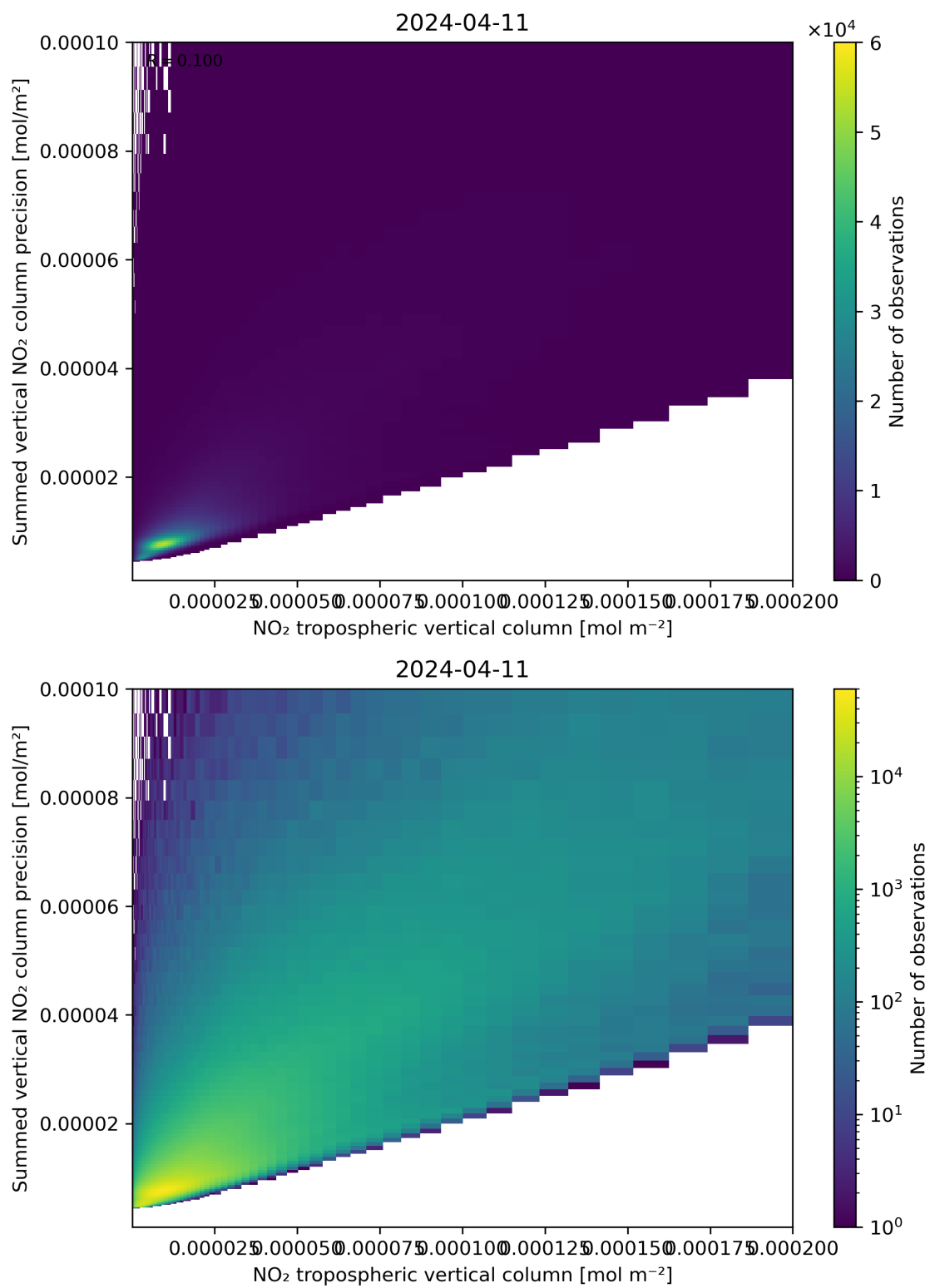
Figure 127: Scatter density plot of “NO 2 tropospheric vertical column” against “Summed vertical NO 2 column precision” for 2024-04-10 to 2024-04-12.
