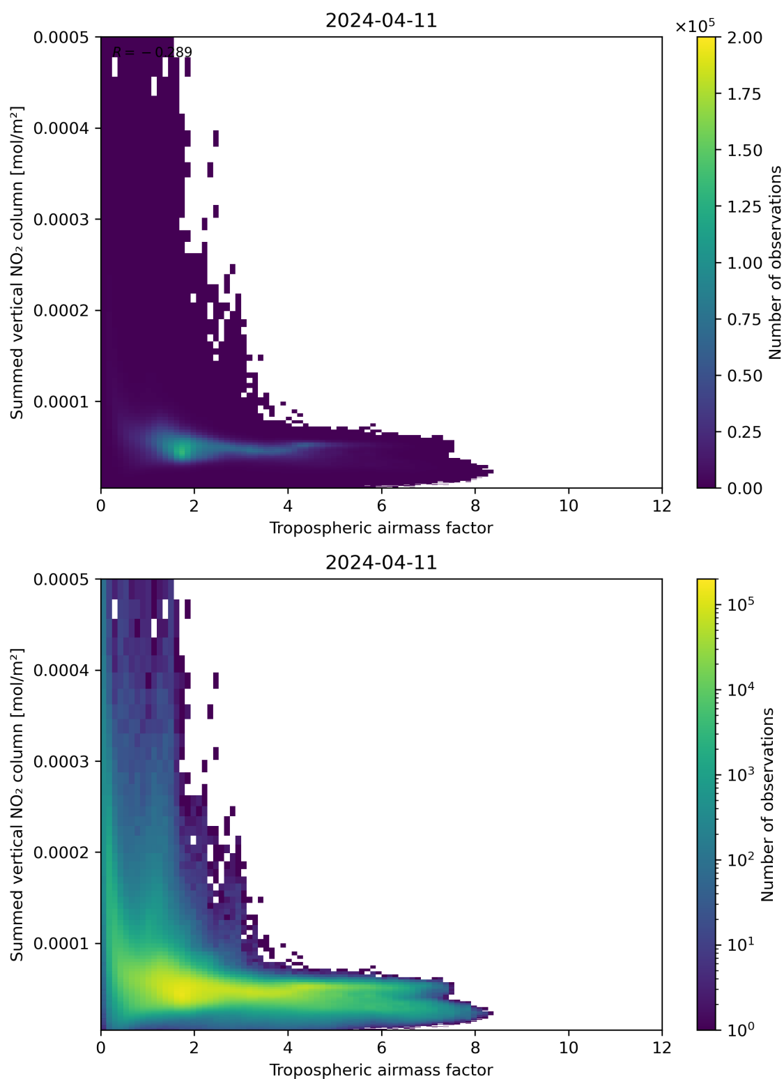
Figure 75: Scatter density plot of “Tropospheric air mass factor” against “Summed vertical NO 2 column” for 2024-04-10 to 2024-04-12.
