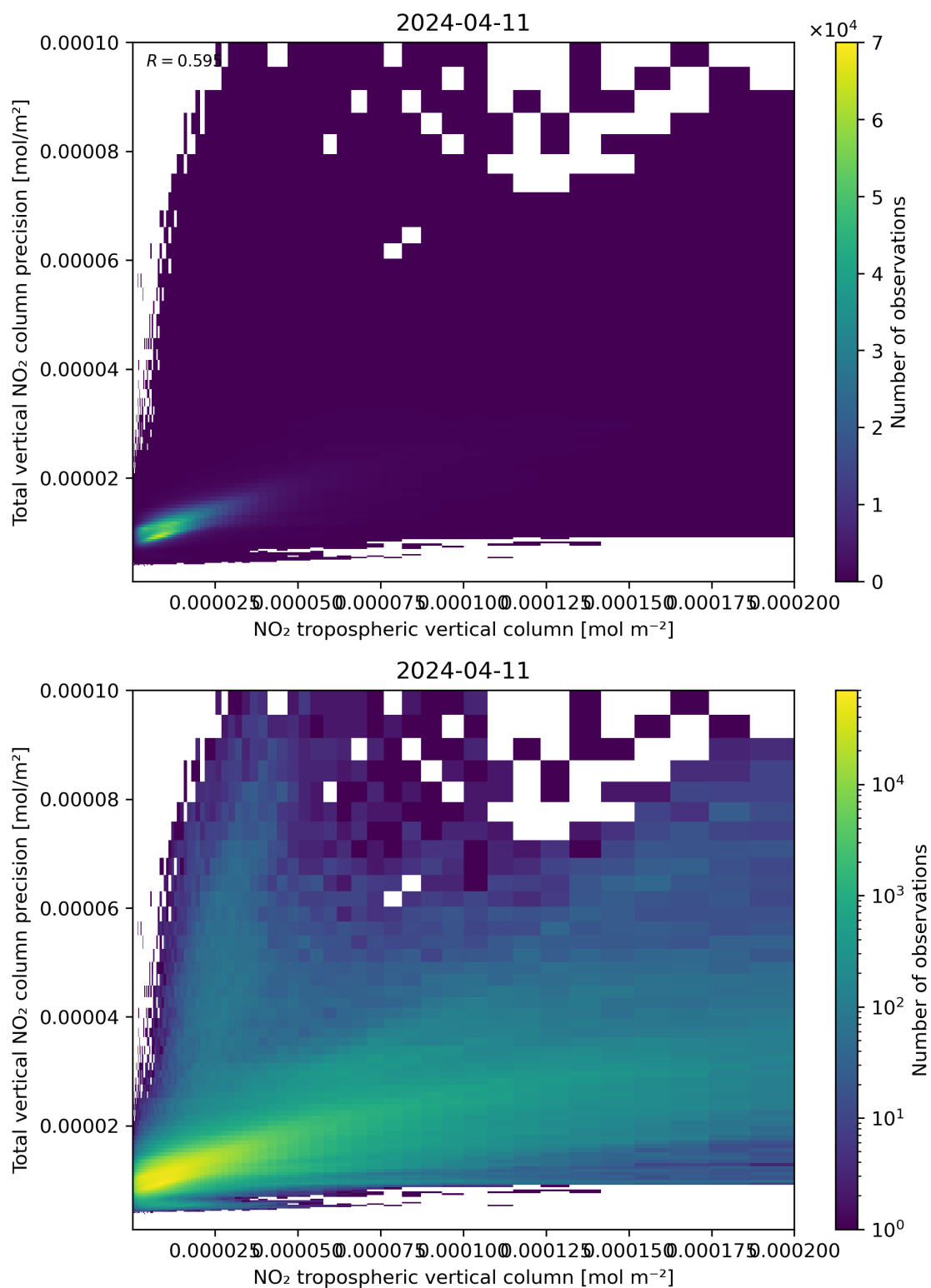
Figure 129: Scatter density plot of “NO 2 tropospheric vertical column” against “Total vertical NO 2 column precision” for 2024-04-10 to 2024-04-12.
