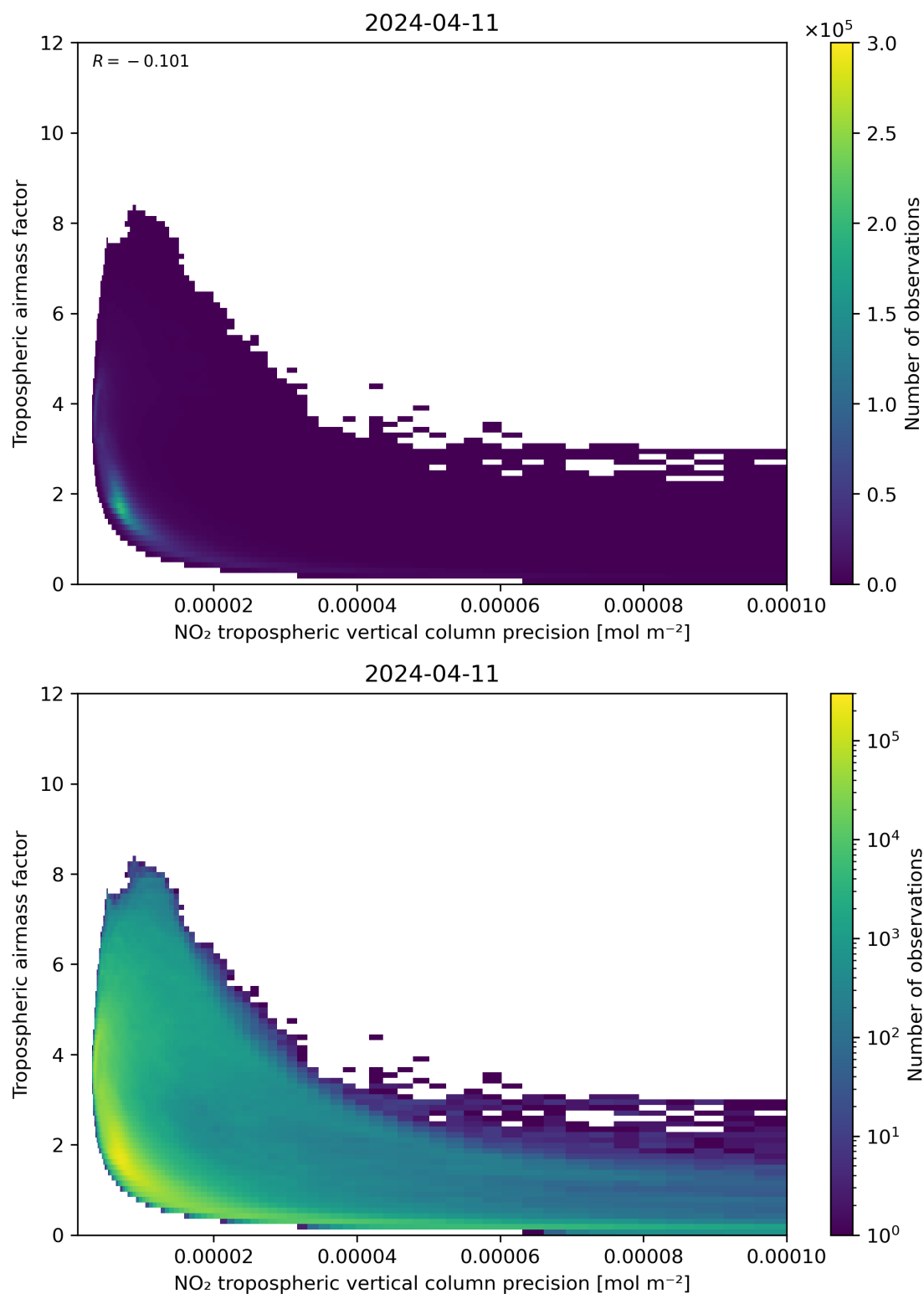
Figure 133: Scatter density plot of “NO 2 tropospheric vertical column precision” against “Tropospheric air mass factor” for 2024-04-10 to 2024-04-12.
