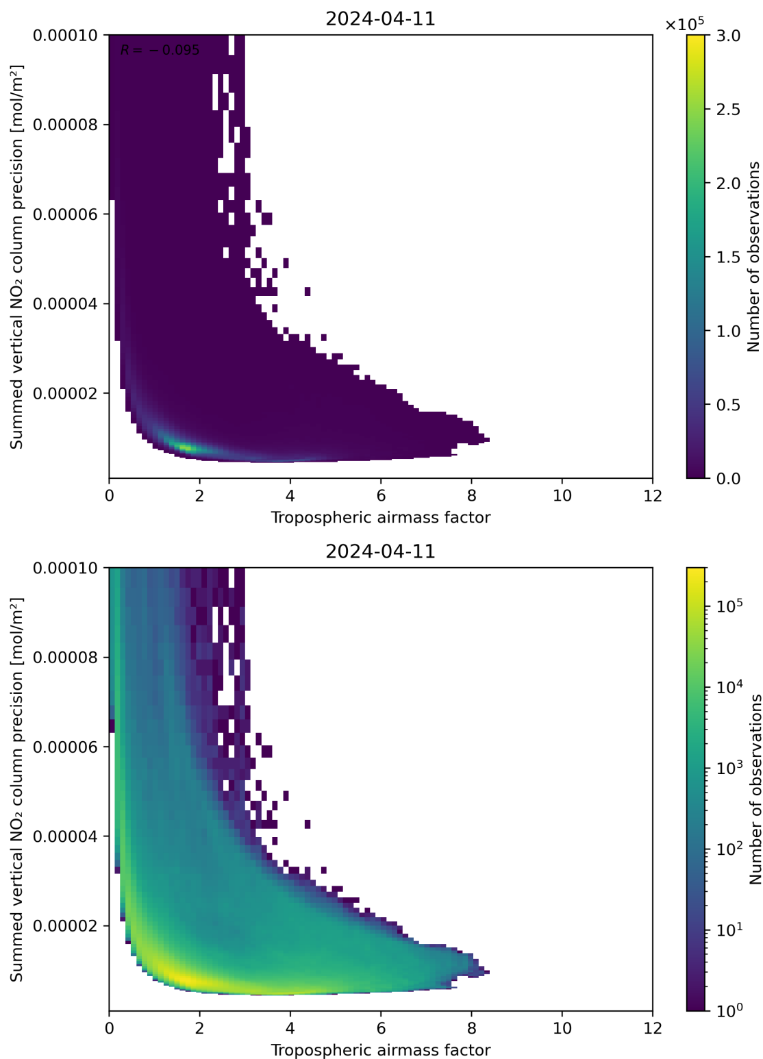
Figure 76: Scatter density plot of “Tropospheric air mass factor” against “Summed vertical NO 2 column precision” for 2024-04-10 to 2024-04-12.
