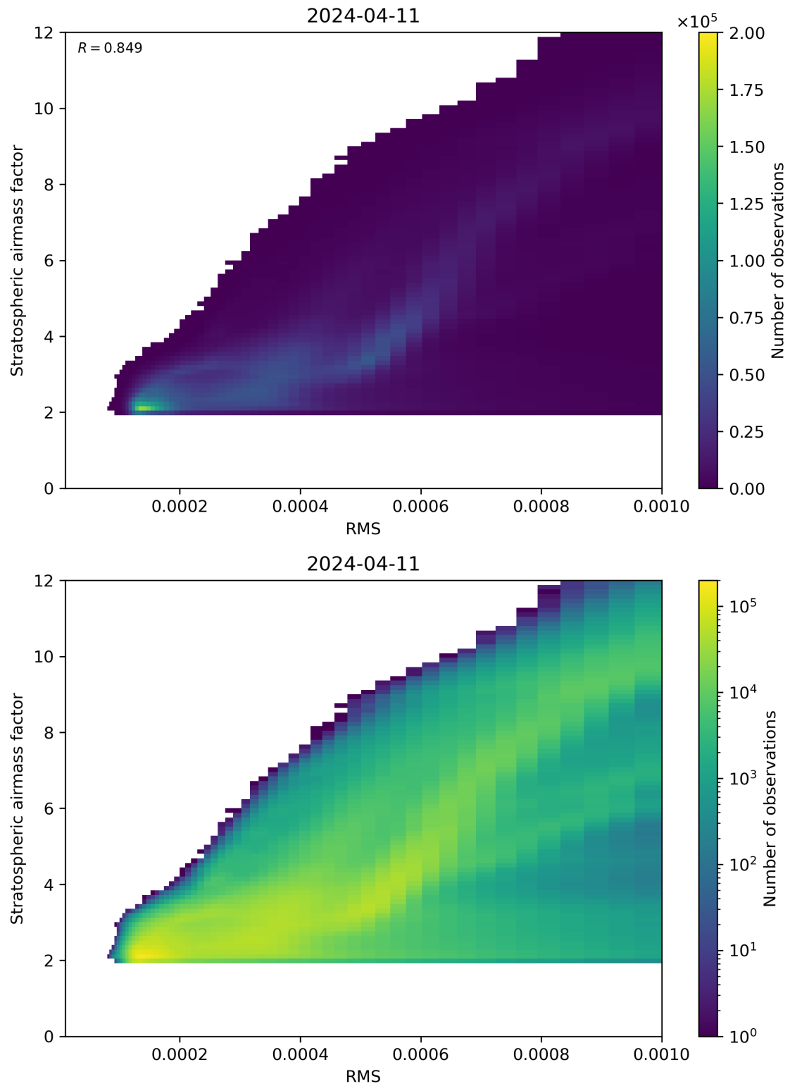
Figure 144: Scatter density plot of “RMS” against “Stratospheric airmass factor” for 2024-04-10 to 2024-04-12.
