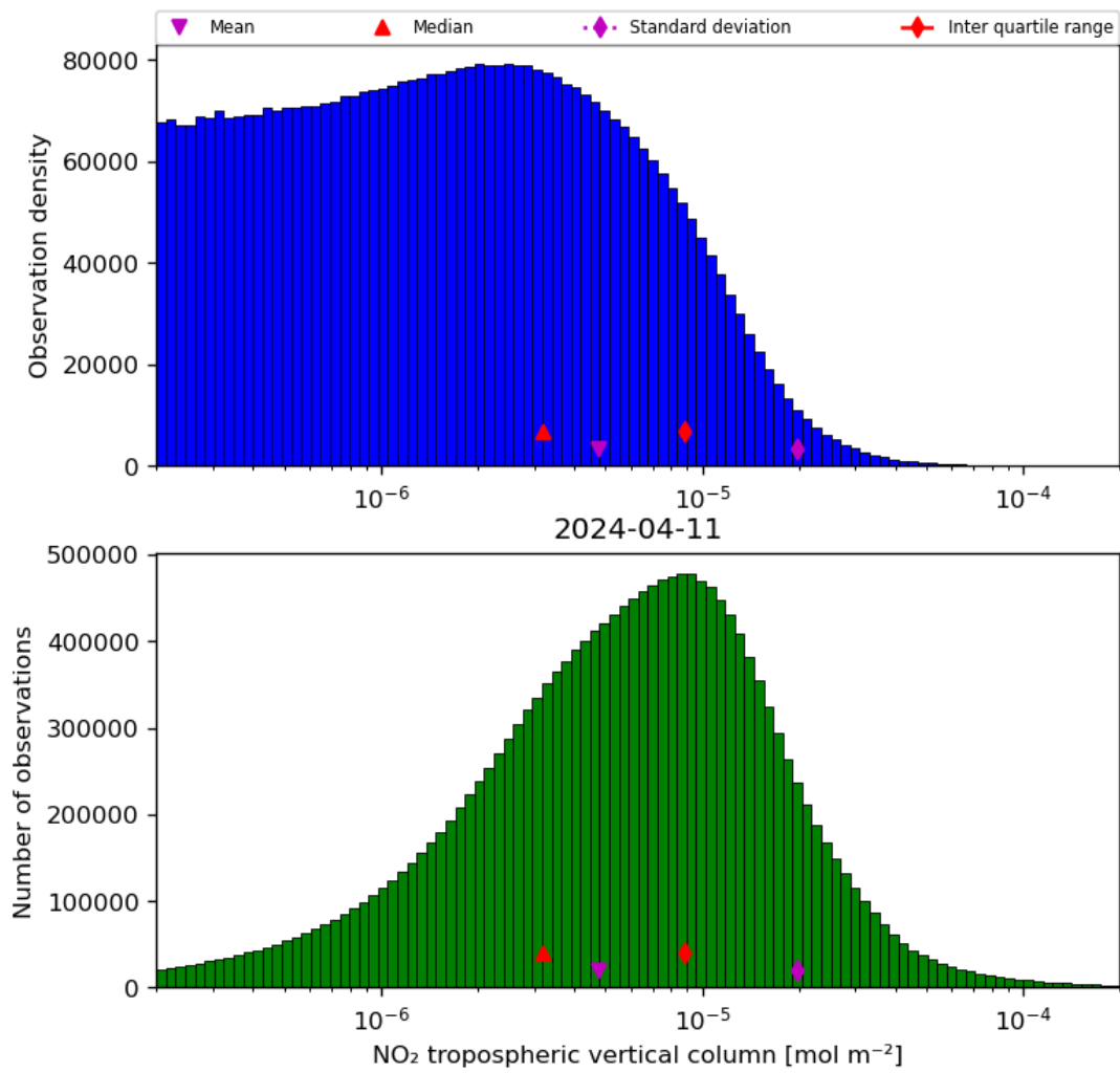
Figure 29: Histogram of “NO 2 tropospheric vertical column” for 2024-04-10 to 2024-04-12
