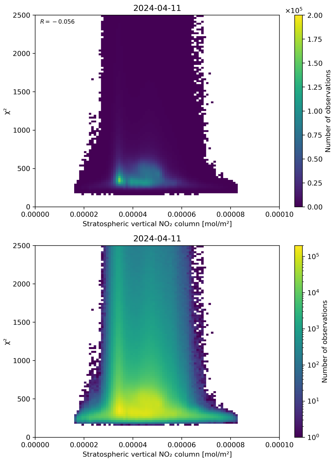
Figure 97: Scatter density plot of “Stratospheric vertical NO 2 column” against “ \chi^2 ” for 2024-04-10 to 2024-04-12.
