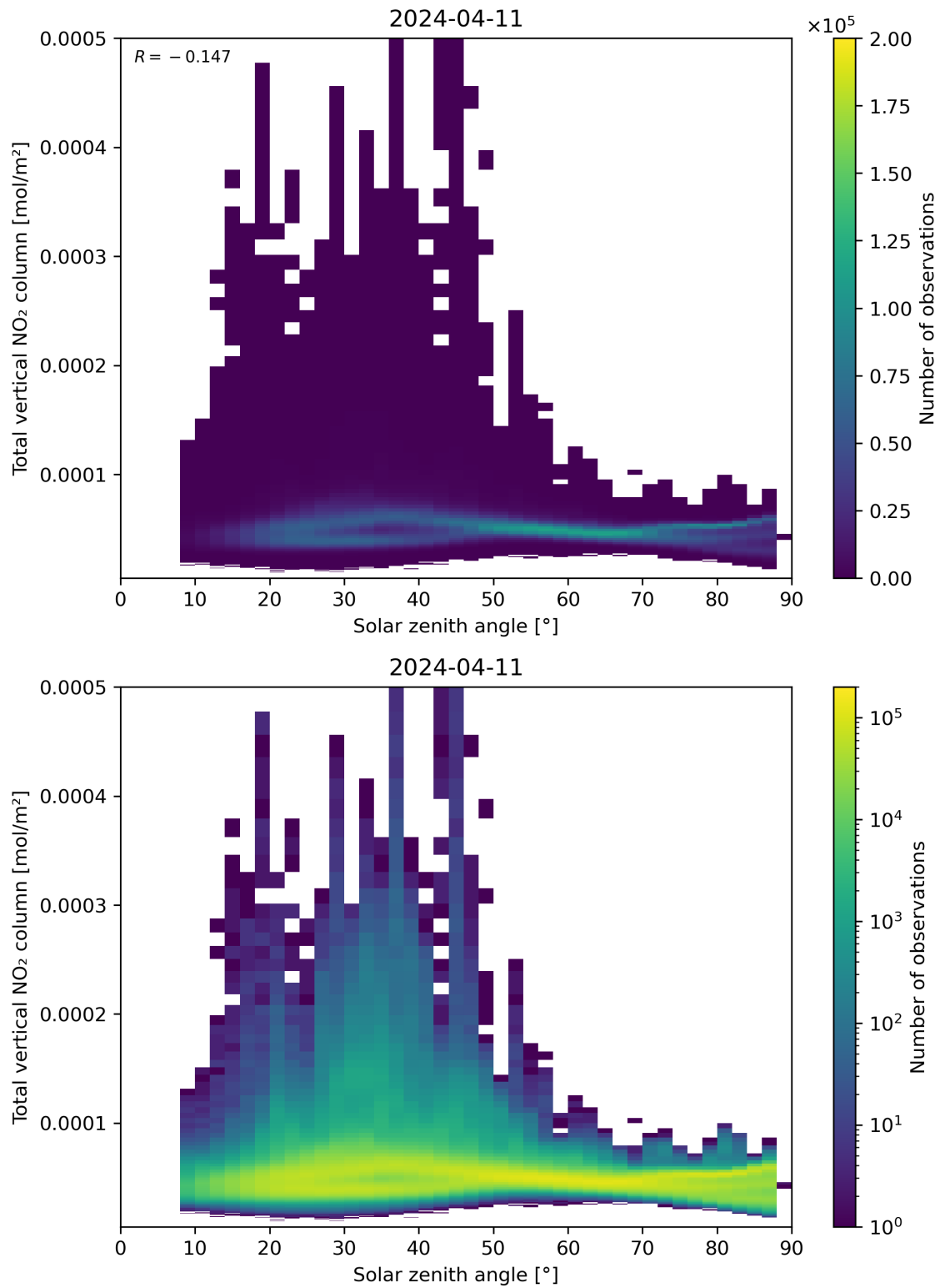
Figure 153: Scatter density plot of “Solar zenith angle” against “Total vertical NO 2 column” for 2024-04-10 to 2024-04-12.
