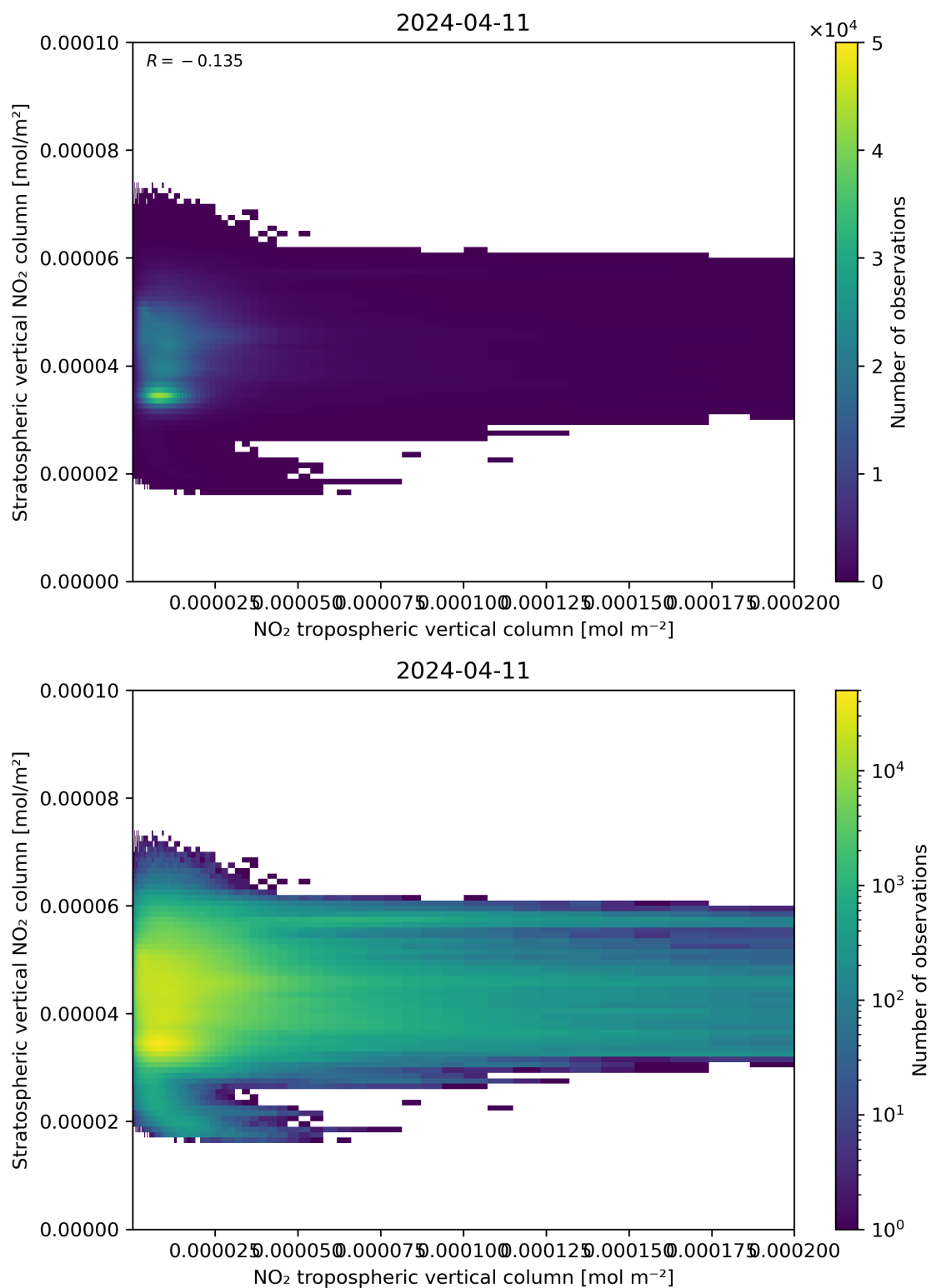
Figure 125: Scatter density plot of “NO 2 tropospheric vertical column” against “Stratospheric vertical NO 2 column” for 2024-04-10 to 2024-04-12.
