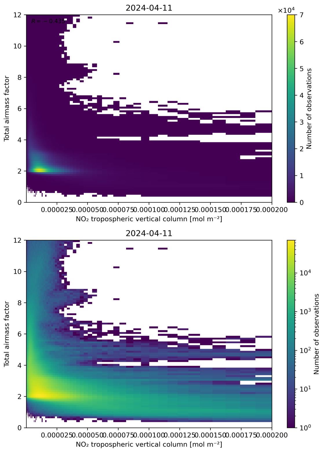
Figure 122: Scatter density plot of “NO 2 tropospheric vertical column” against “Total air mass factor” for 2024-04-10 to 2024-04-12.
