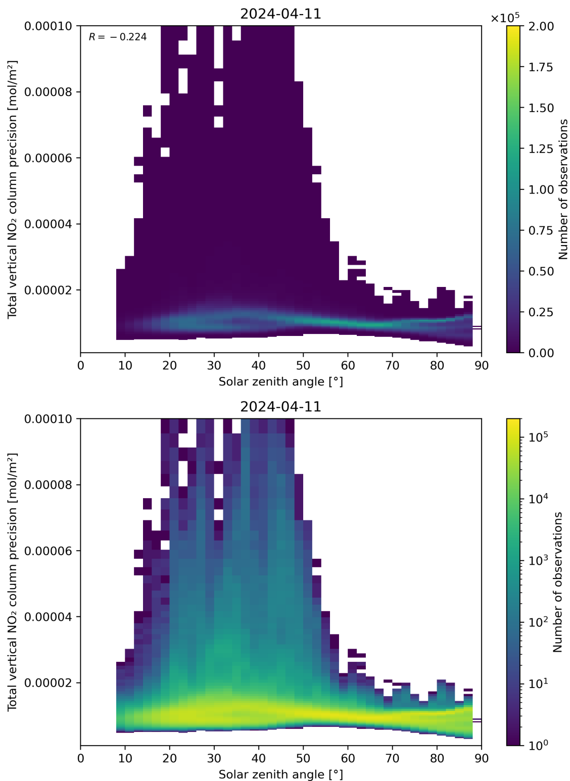
Figure 154: Scatter density plot of “Solar zenith angle” against “Total vertical NO 2 column precision” for 2024-04-10 to 2024-04-12.
