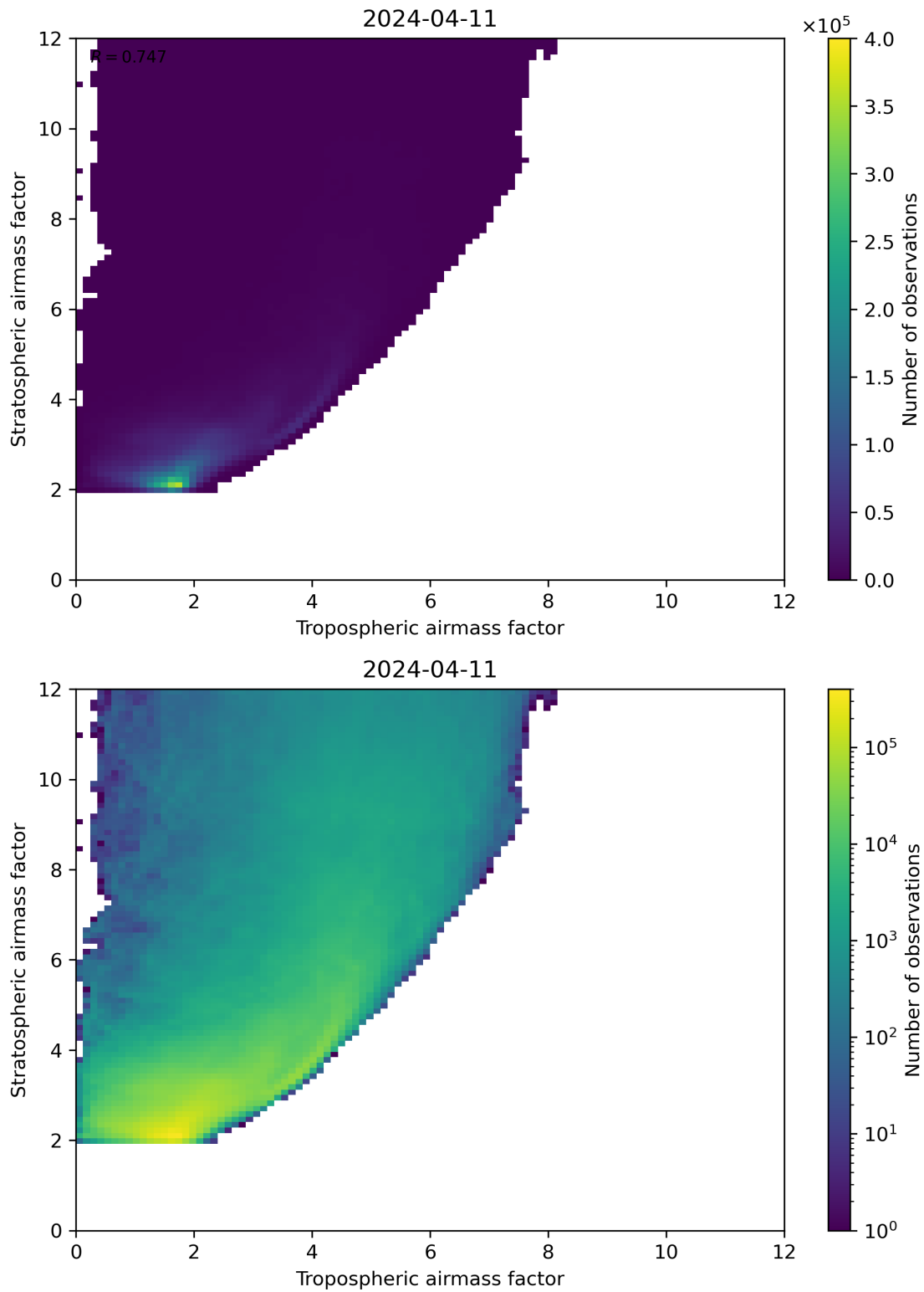
Figure 71: Scatter density plot of “Tropospheric airmass factor” against “Stratospheric airmass factor” for 2024-04-10 to 2024-04-12.
