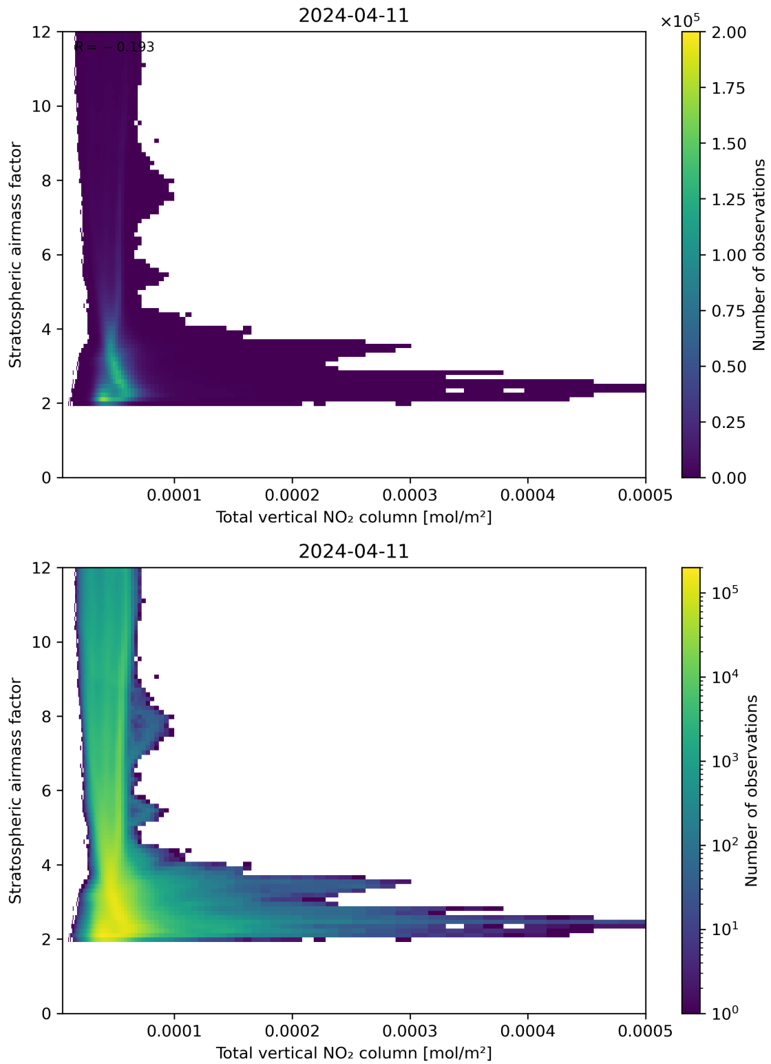
Figure 110: Scatter density plot of “Total vertical NO 2 column” against “Stratospheric airmass factor” for 2024-04-10 to 2024-04-12.
