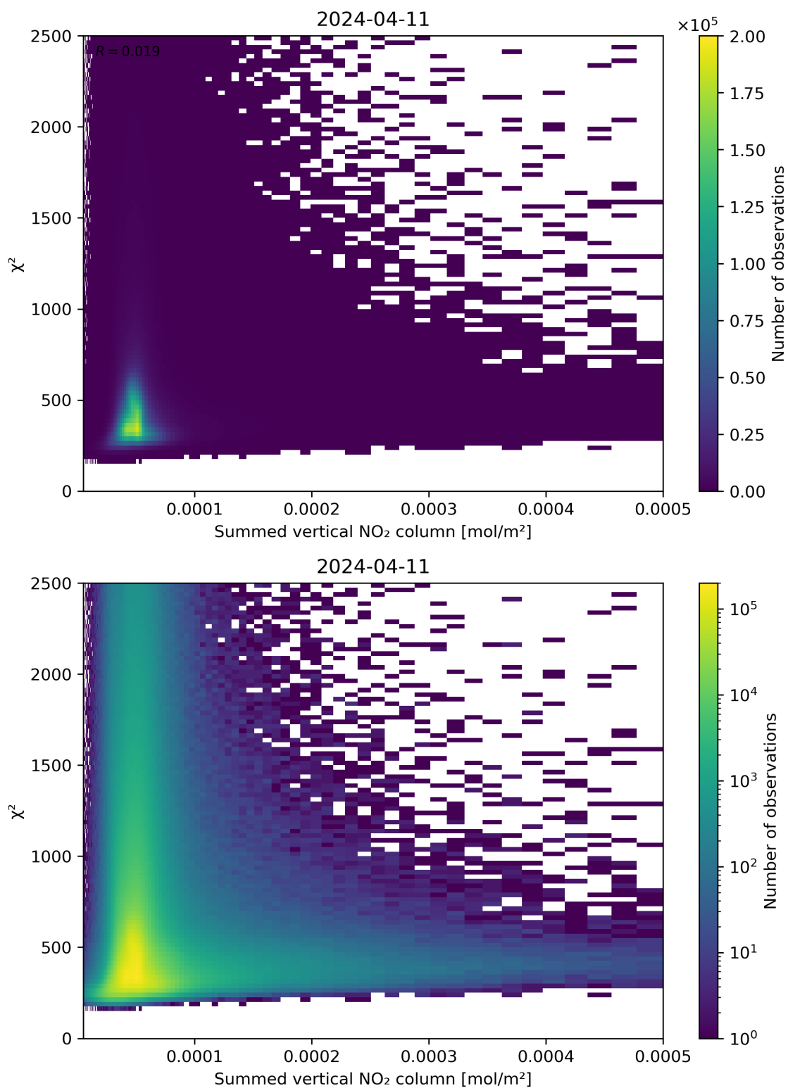
Figure 104: Scatter density plot of “Summed vertical NO 2 column” against “ \chi^2 ” for 2024-04-10 to 2024-04-12.
