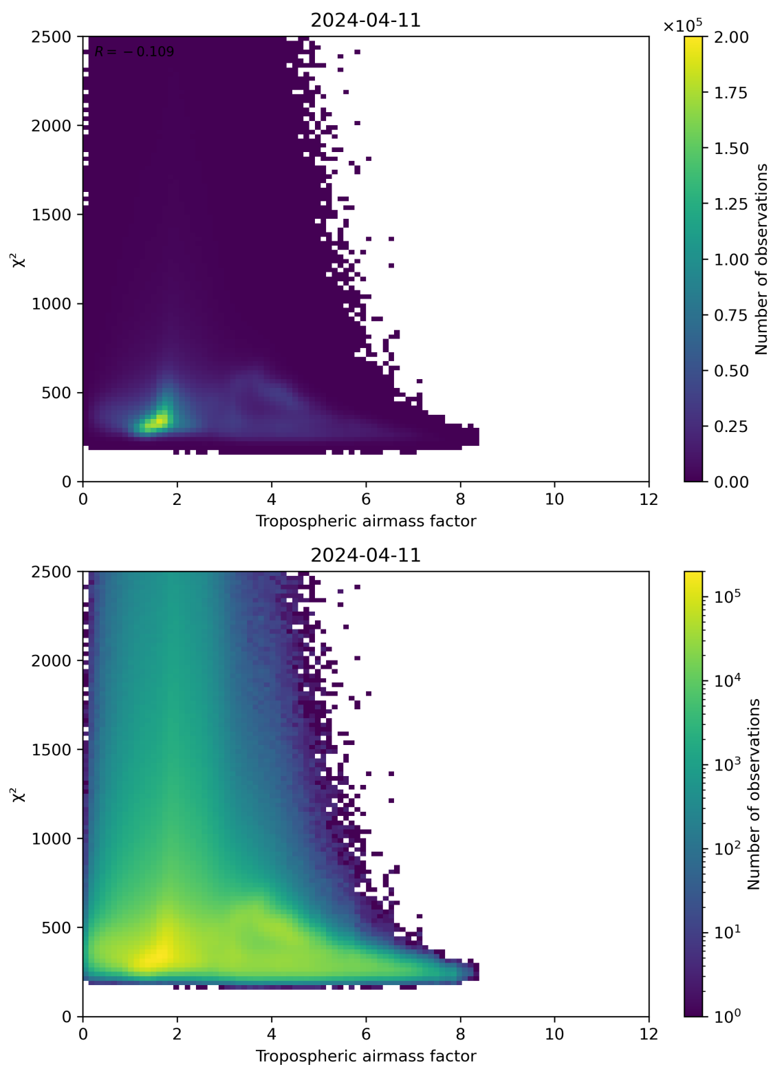
Figure 73: Scatter density plot of “Tropospheric airmass factor” against “ \chi^2 ” for 2024-04-10 to 2024-04-12.
