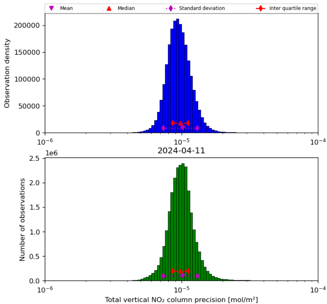
Figure 39: Histogram of "Total vertical NO 2 column precision" for 2024-04-10 to 2024-04-12
