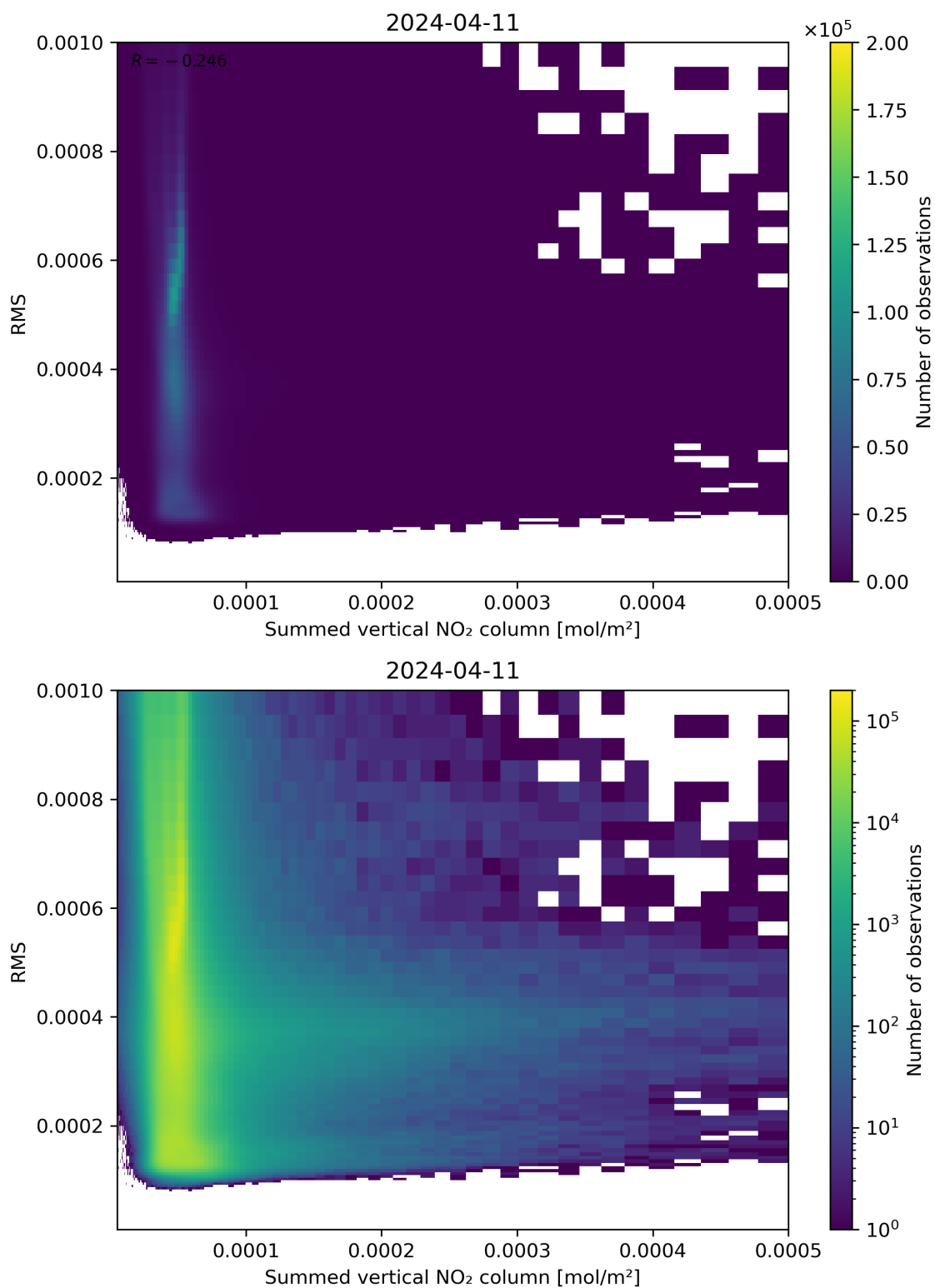
Figure 109: Scatter density plot of “Summed vertical NO 2 column” against “RMS” for 2024-04-10 to 2024-04-12.
