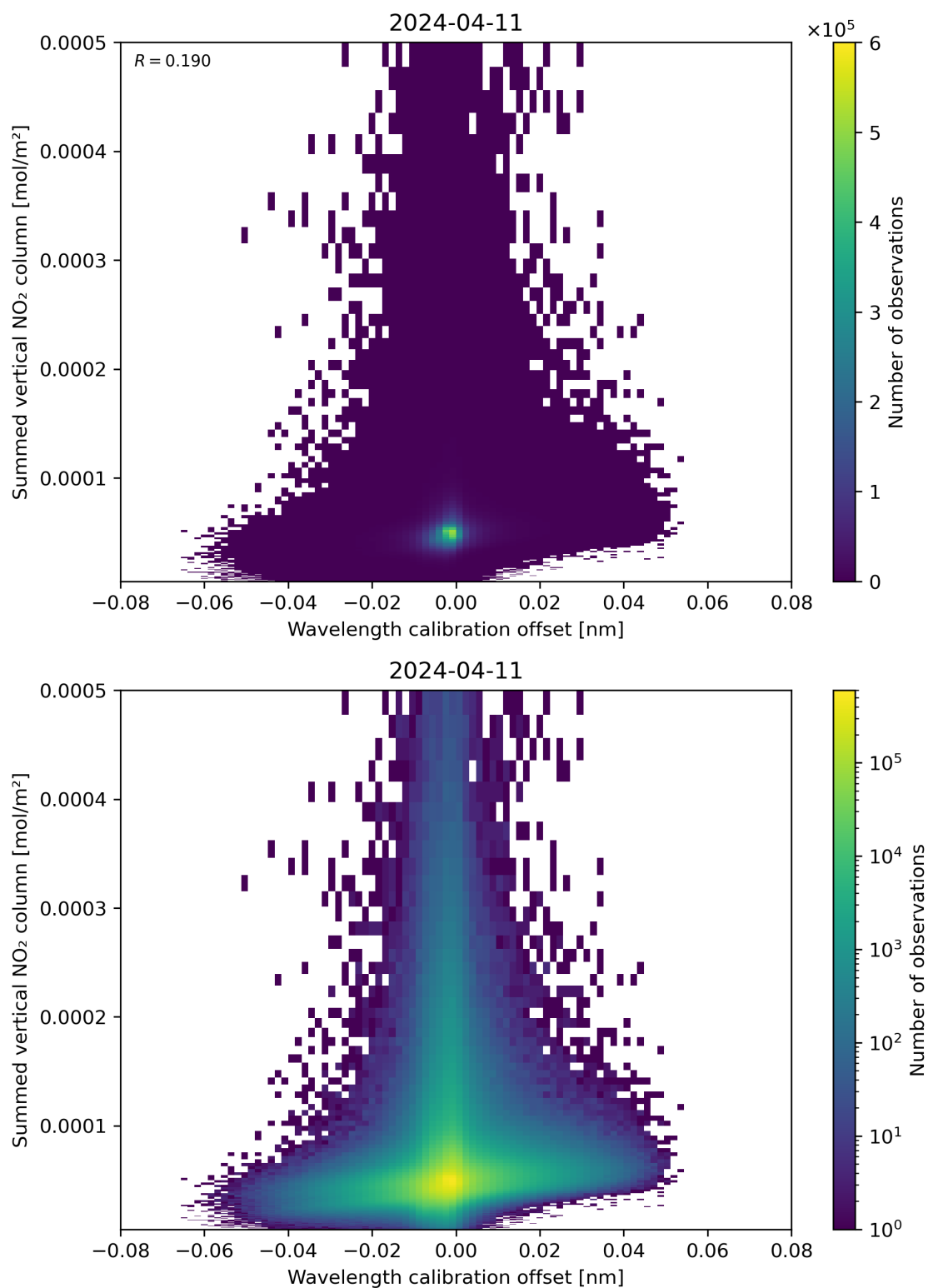
Figure 177: Scatter density plot of “Wavelength calibration offset” against “Summed vertical NO 2 column” for 2024-04-10 to 2024-04-12.
