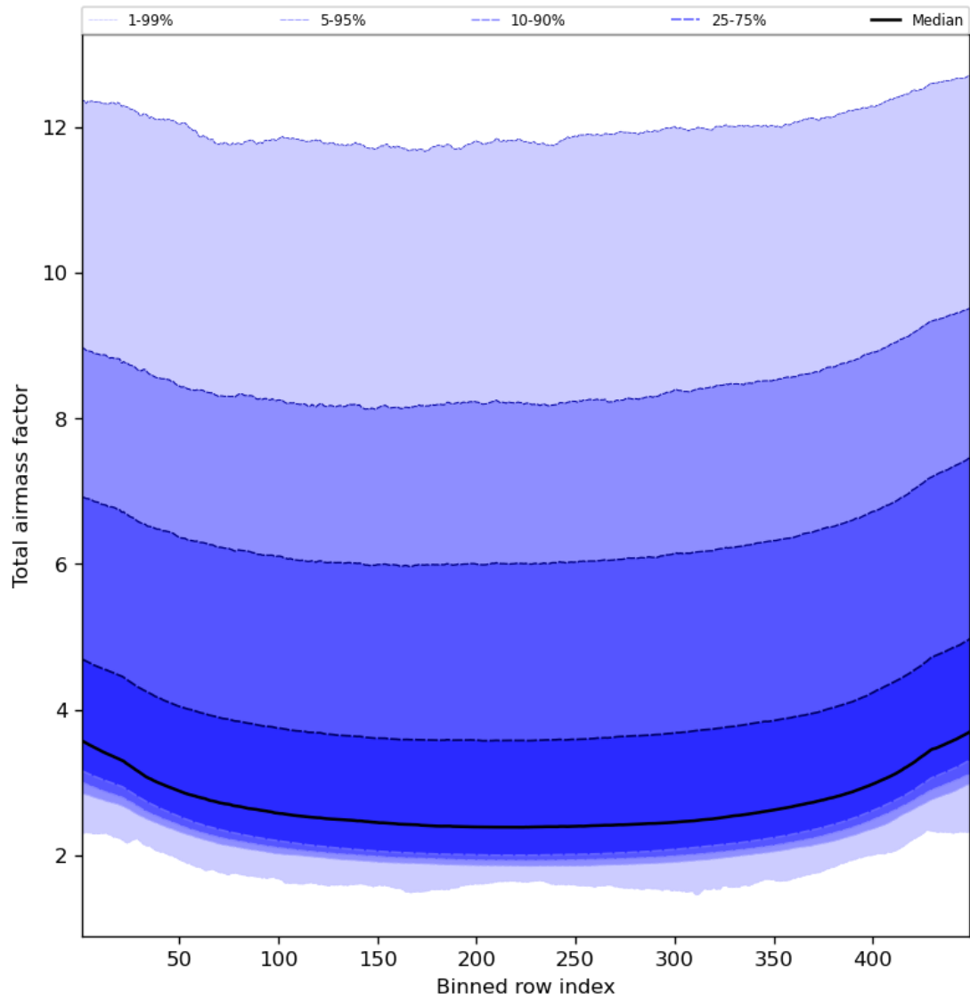
Figure 49: Along track statistics of “Total airmass factor” for 2024-04-10 to 2024-04-12
