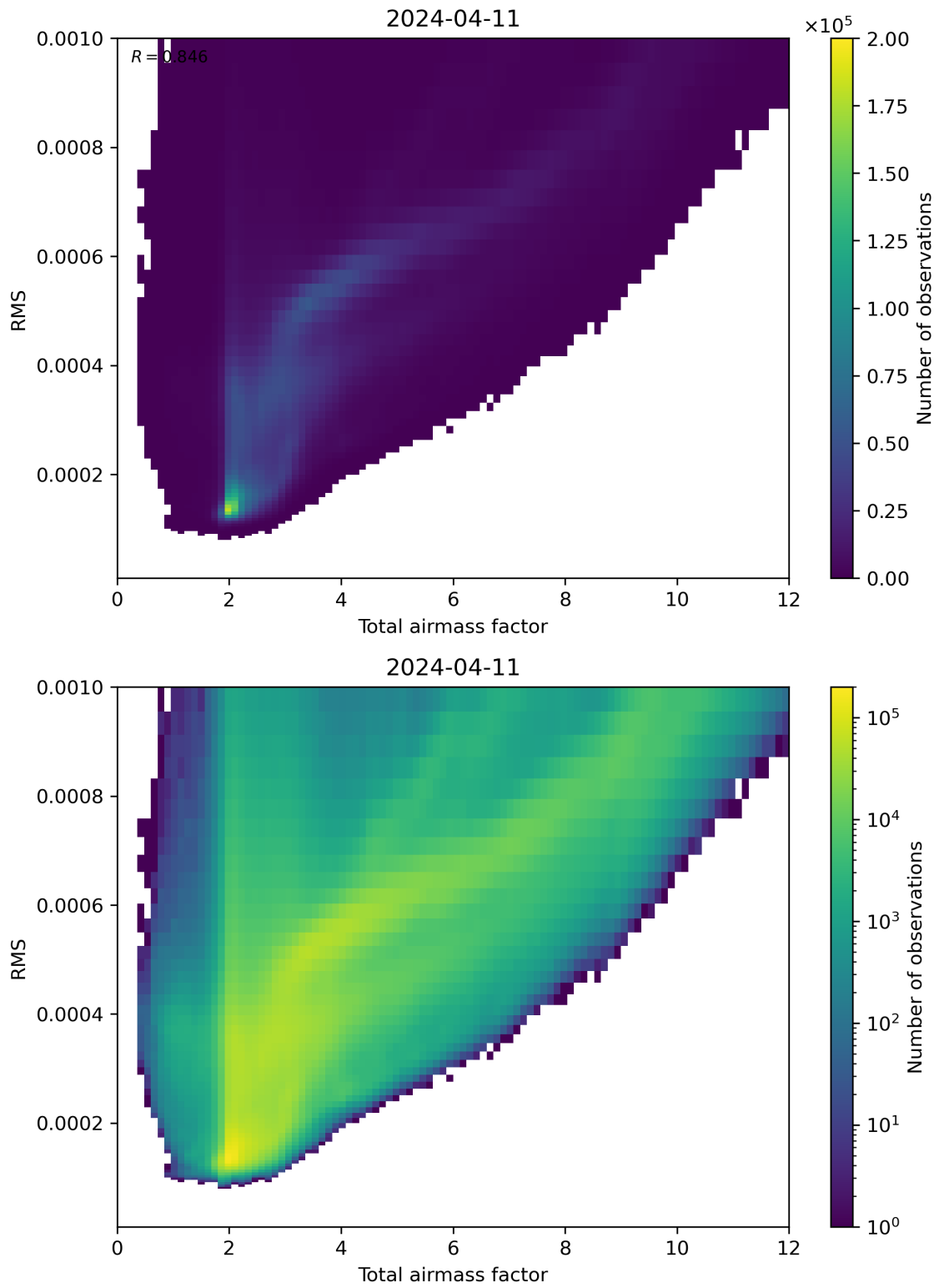
Figure 69: Scatter density plot of “Total airmass factor” against “RMS” for 2024-04-10 to 2024-04-12.
