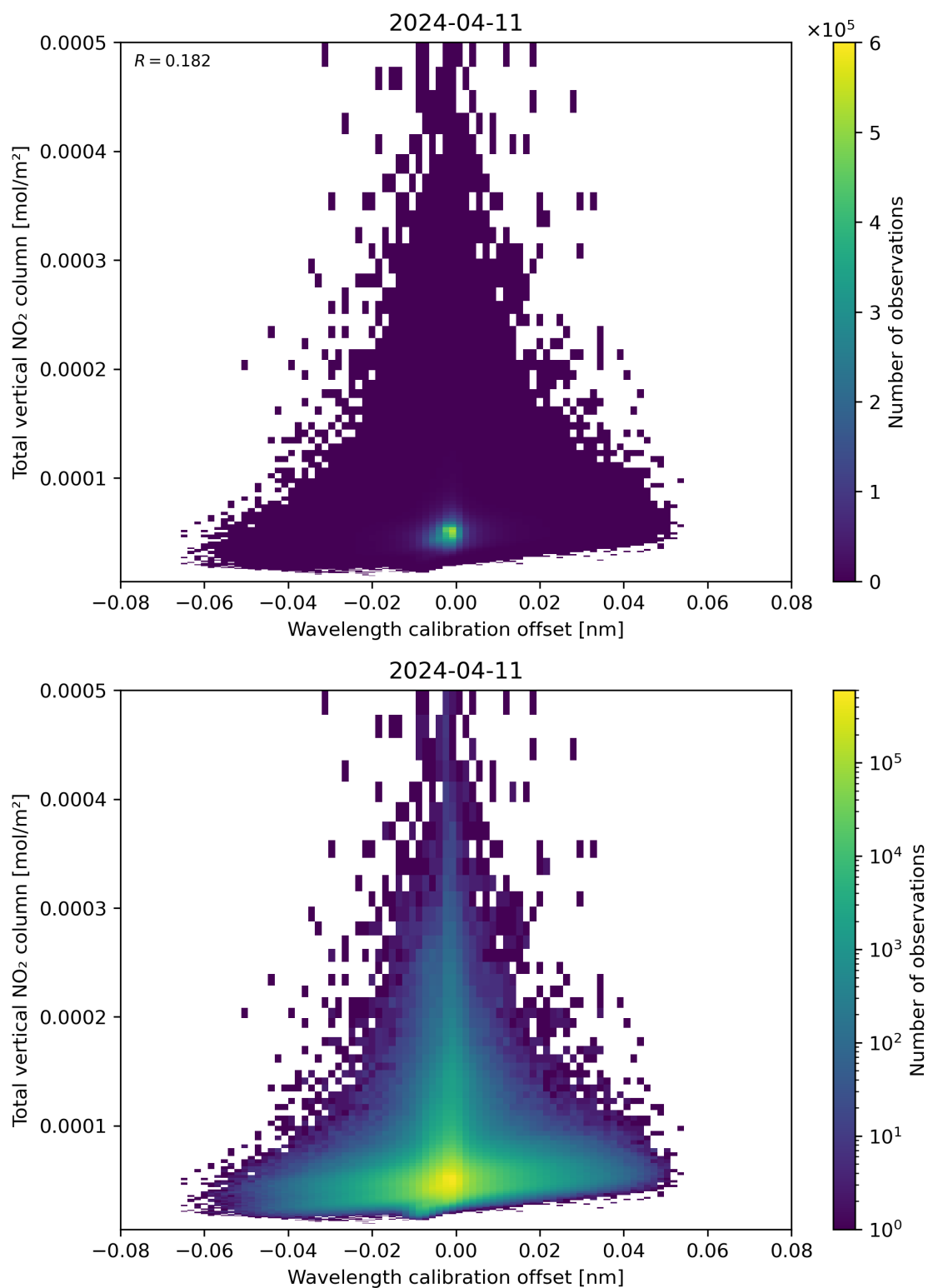
Figure 179: Scatter density plot of “Wavelength calibration offset” against “Total vertical NO 2 column” for 2024-04-10 to 2024-04-12.
