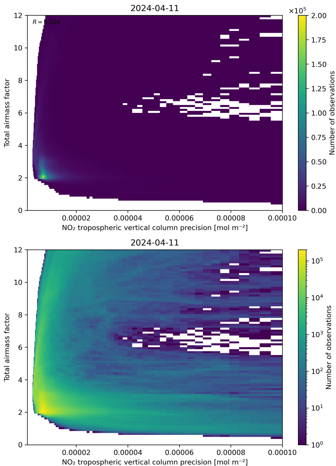
Figure 132: Scatter density plot of “NO 2 tropospheric vertical column precision” against “Total air mass factor” for 2024-04-10 to 2024-04-12.
