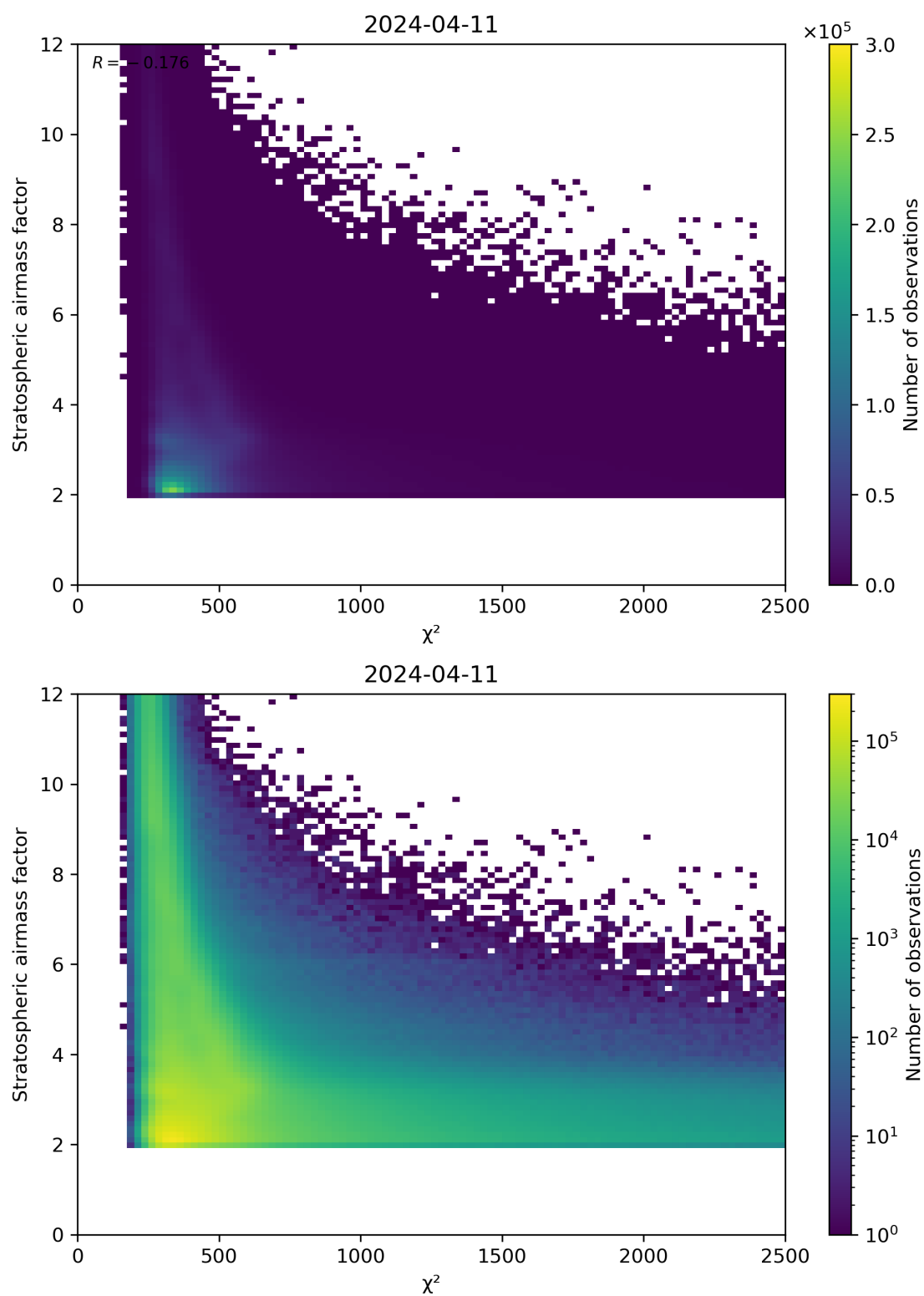
Figure 81: Scatter density plot of “ \chi^2 ” against “Stratospheric airmass factor” for 2024-04-10 to 2024-04-12.
