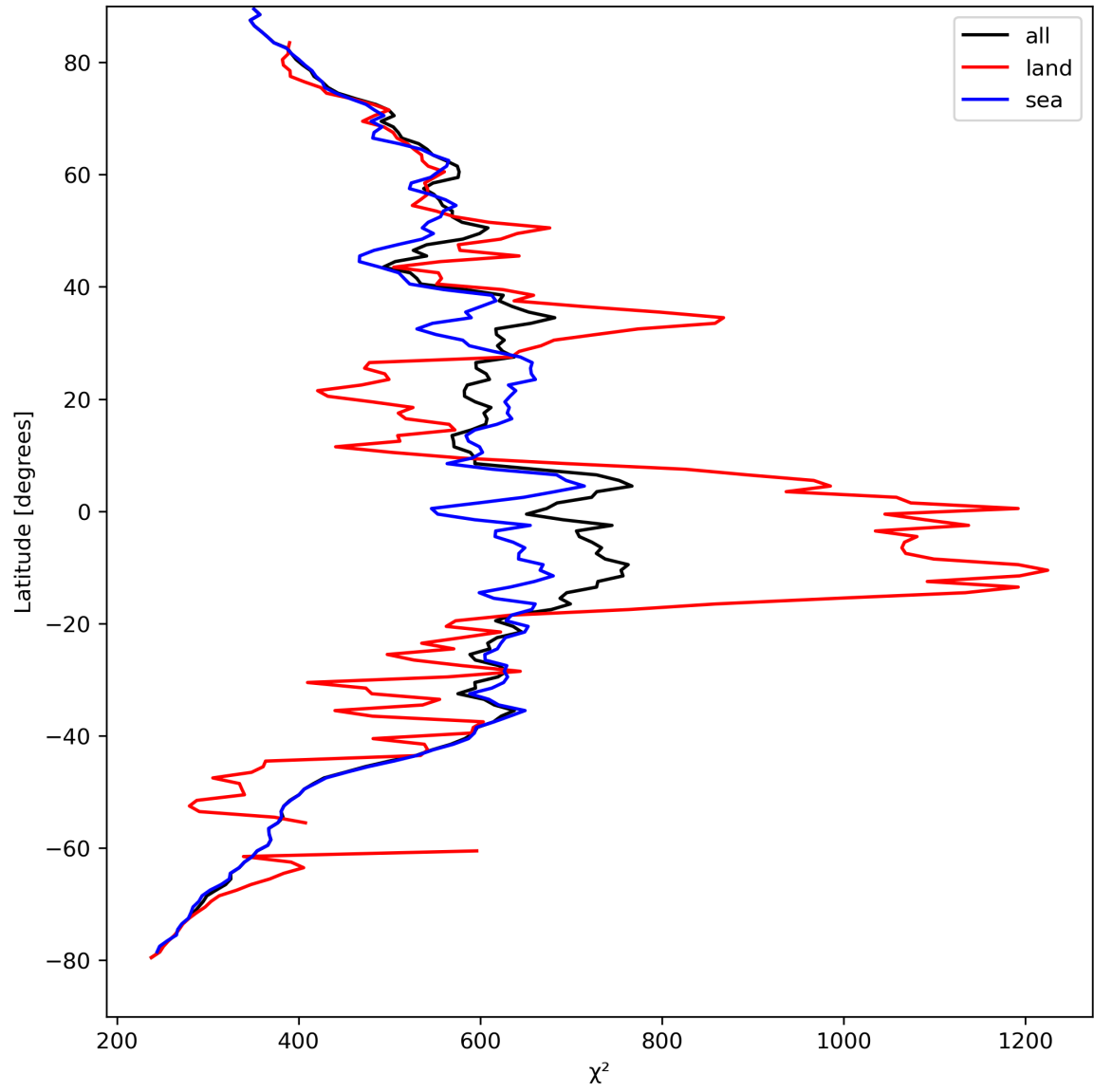
Figure 25: Zonal average of “ \chi^2 ” for 2024-04-10 to 2024-04-12.
