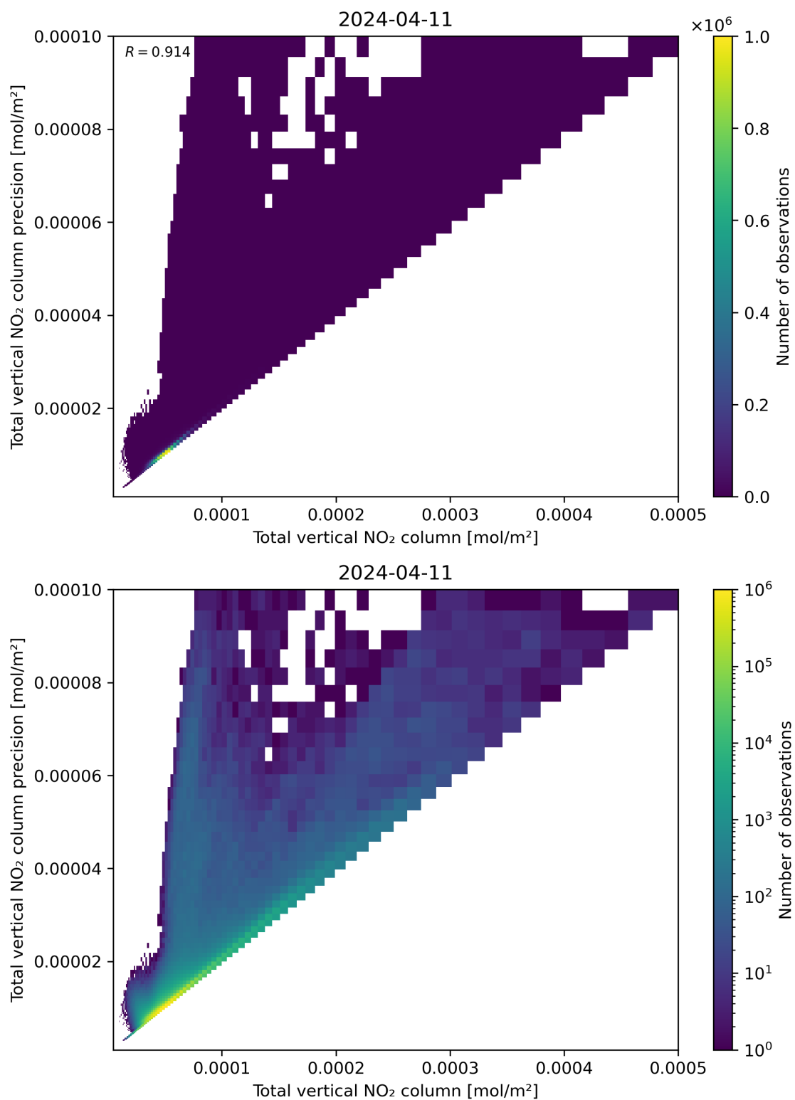
Figure 114: Scatter density plot of “Total vertical NO 2 column” against “Total vertical NO 2 column precision” for 2024-04-10 to 2024-04-12.
