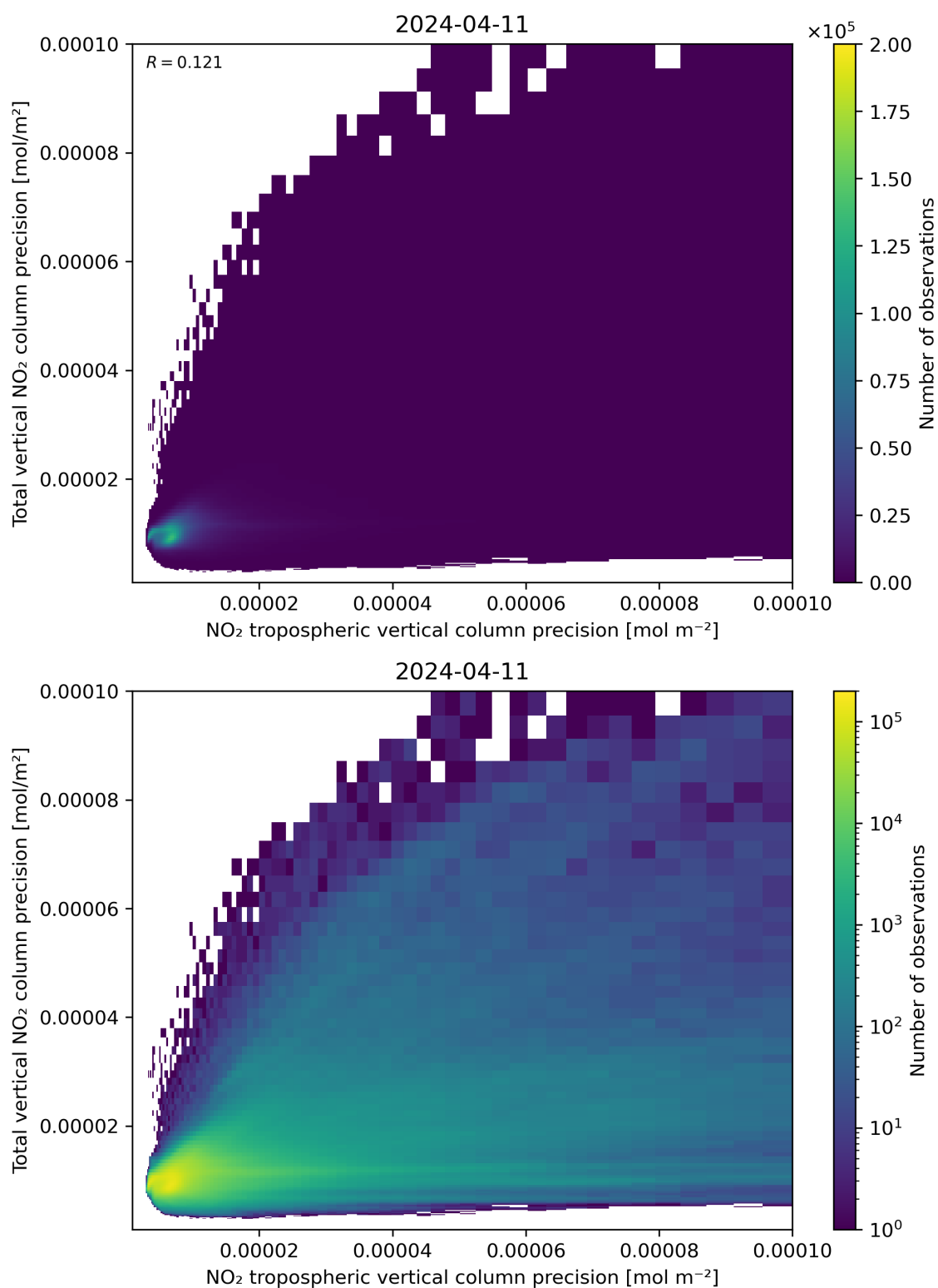
Figure 139: Scatter density plot of “NO 2 tropospheric vertical column precision” against “Total vertical NO 2 column precision” for 2024-04-10 to 2024-04-12.
