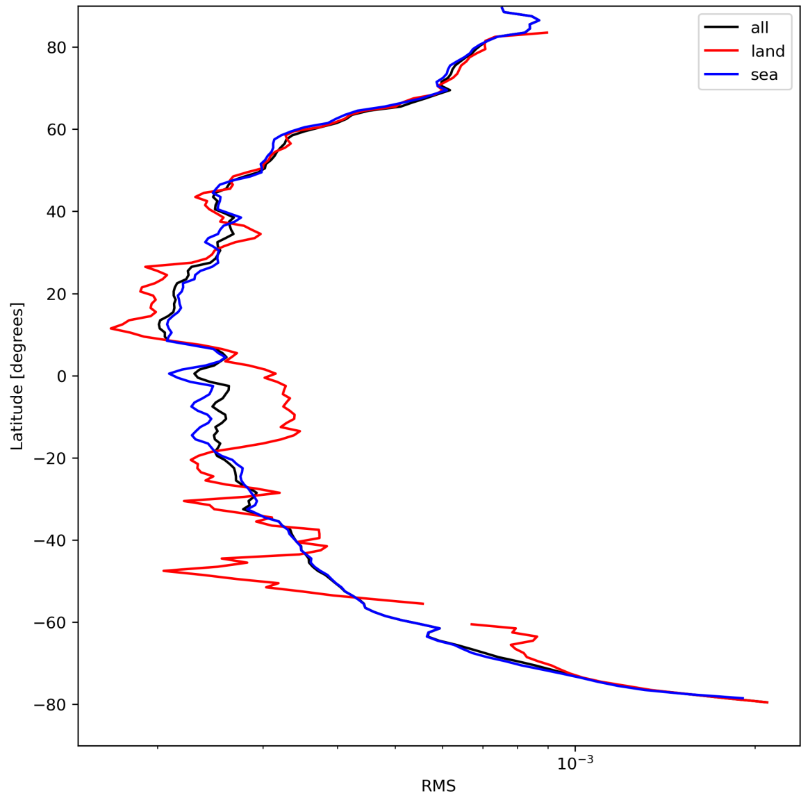
Figure 26: Zonal average of “RMS” for 2024-04-10 to 2024-04-12.
