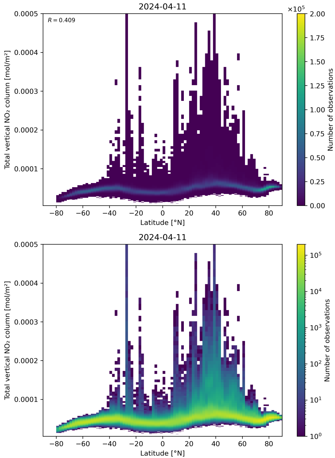
Figure 90: Scatter density plot of “Latitude” against “Total vertical NO 2 column” for 2024-04-10 to 2024-04-12.
