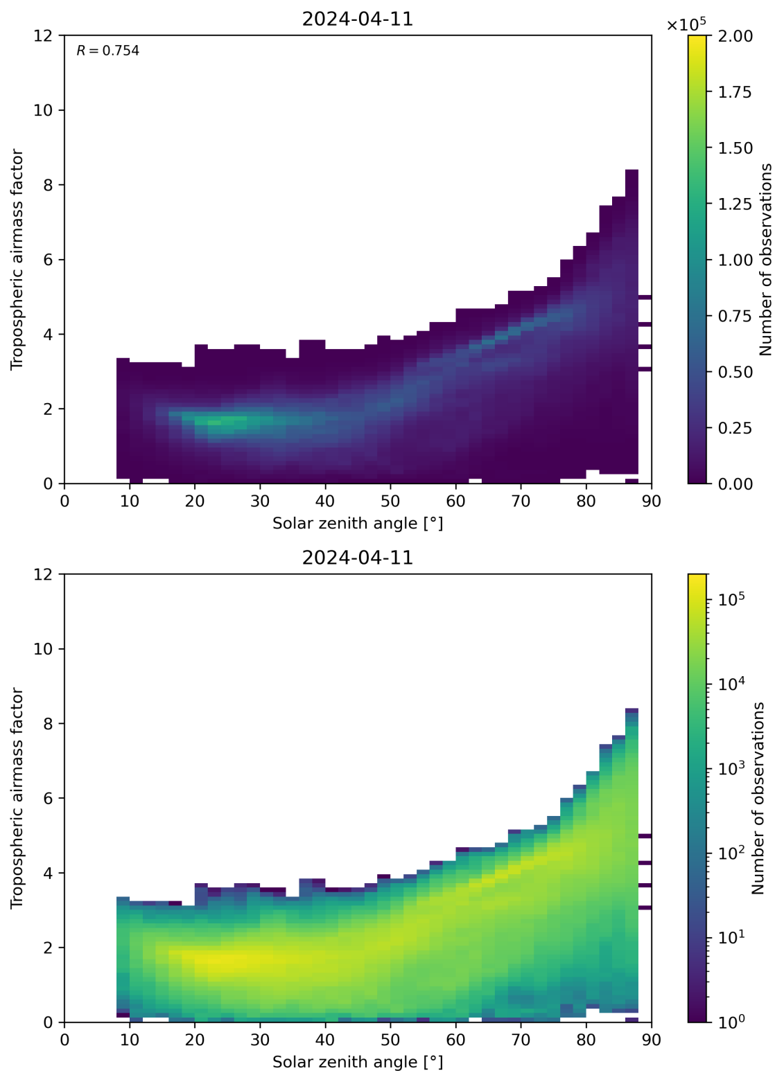
Figure 147: Scatter density plot of “Solar zenith angle” against “Tropospheric airmass factor” for 2024-04-10 to 2024-04-12.
