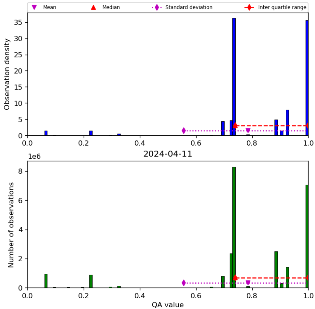
Figure 28: Histogram of “QA value” for 2024-04-10 to 2024-04-12
