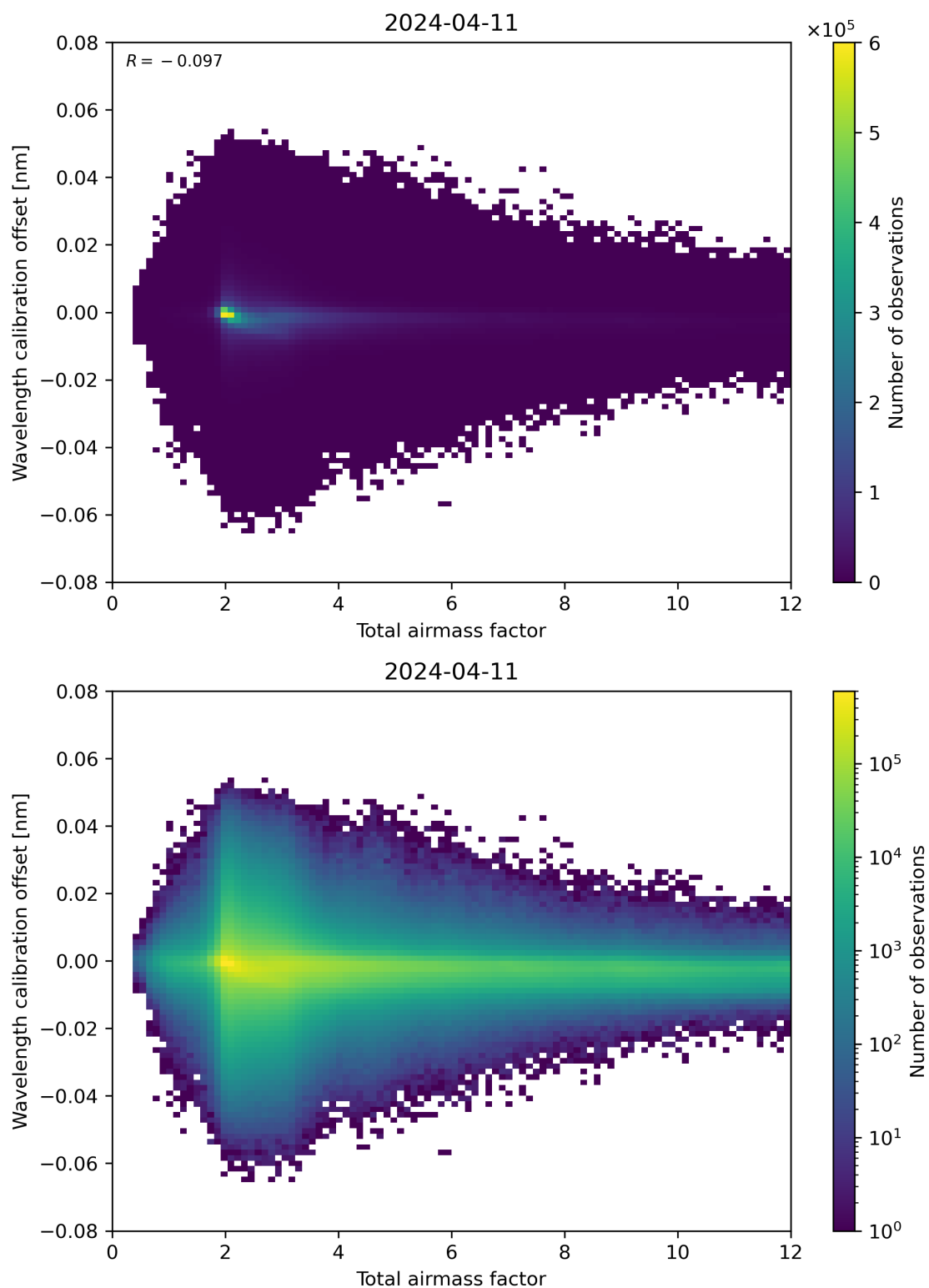
Figure 70: Scatter density plot of “Total airmass factor” against “Wavelength calibration offset” for 2024-04-10 to 2024-04-12.
