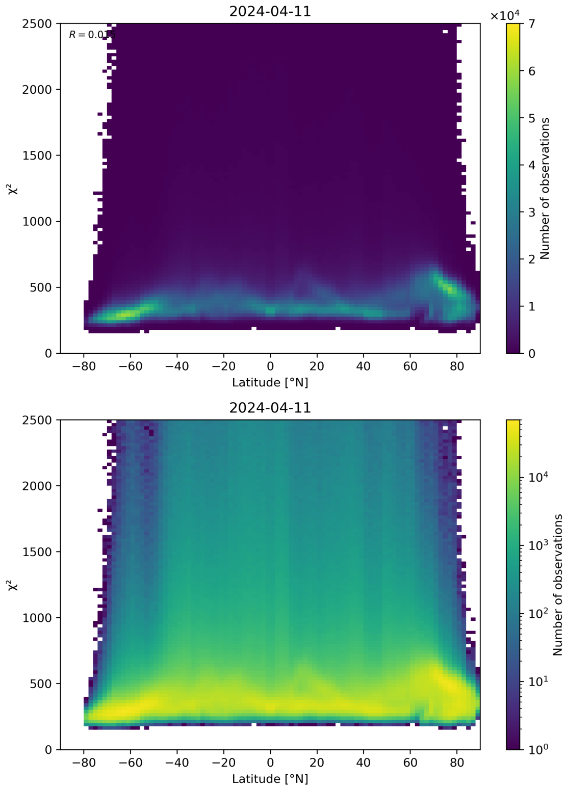
Figure 86: Scatter density plot of “Latitude” against “ \chi^2 ” for 2024-04-10 to 2024-04-12.
