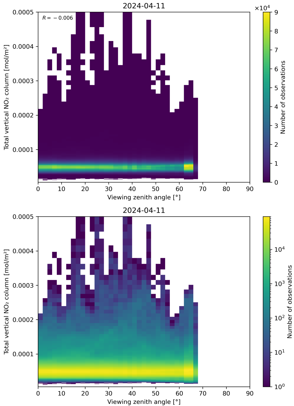
Figure 167: Scatter density plot of “Viewing zenith angle” against “Total vertical NO 2 column” for 2024-04-10 to 2024-04-12.
