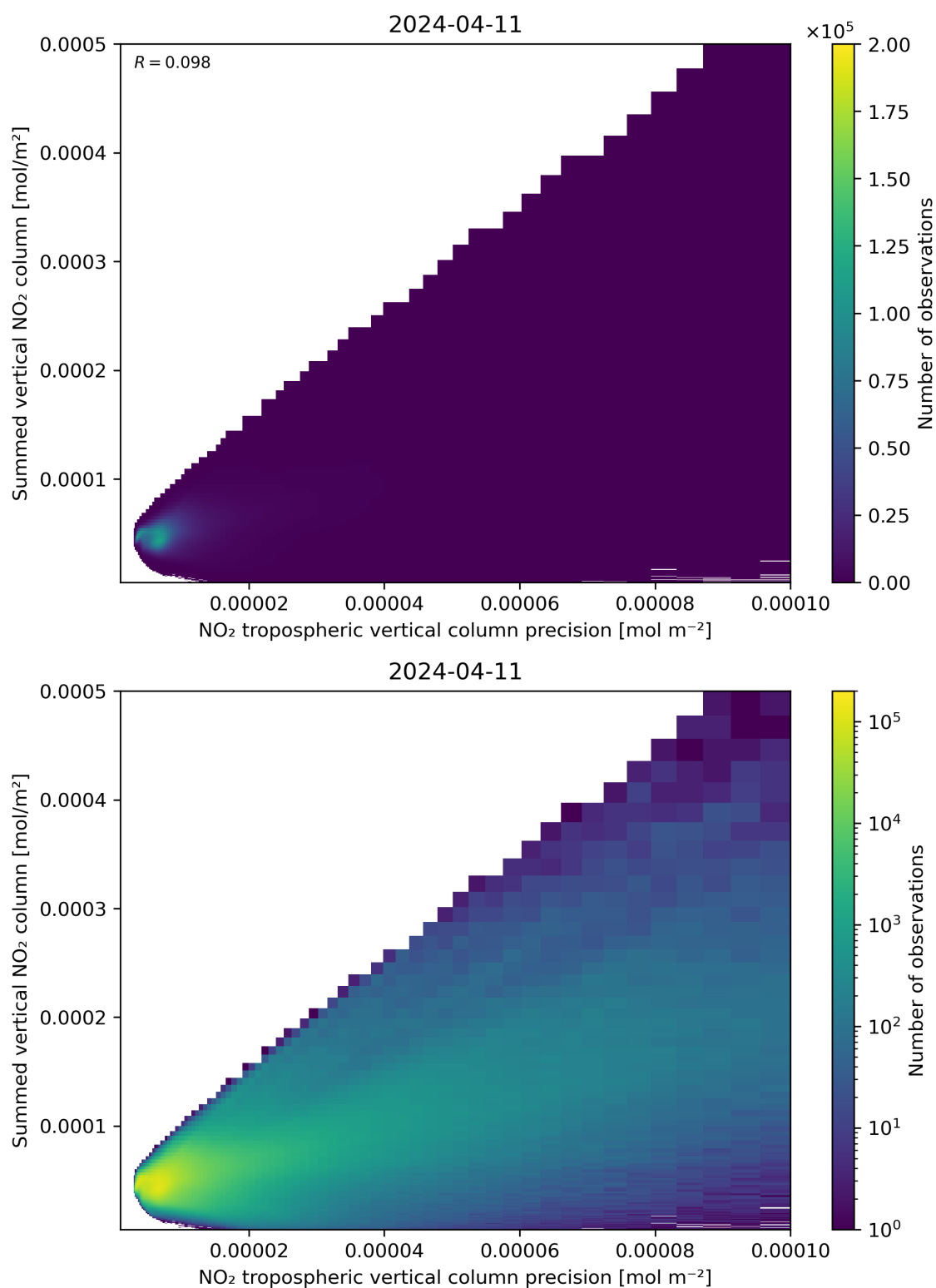
Figure 136: Scatter density plot of “NO 2 tropospheric vertical column precision” against “Summed vertical NO 2 column” for 2024-04-10 to 2024-04-12.
