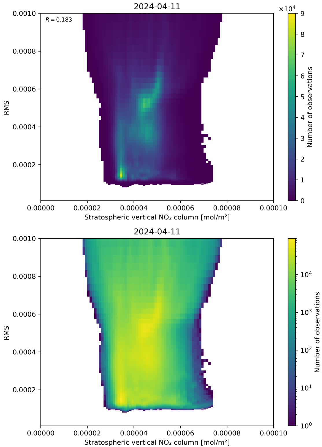
Figure 102: Scatter density plot of “Stratospheric vertical NO 2 column” against “RMS” for 2024-04-10 to 2024-04-12.
