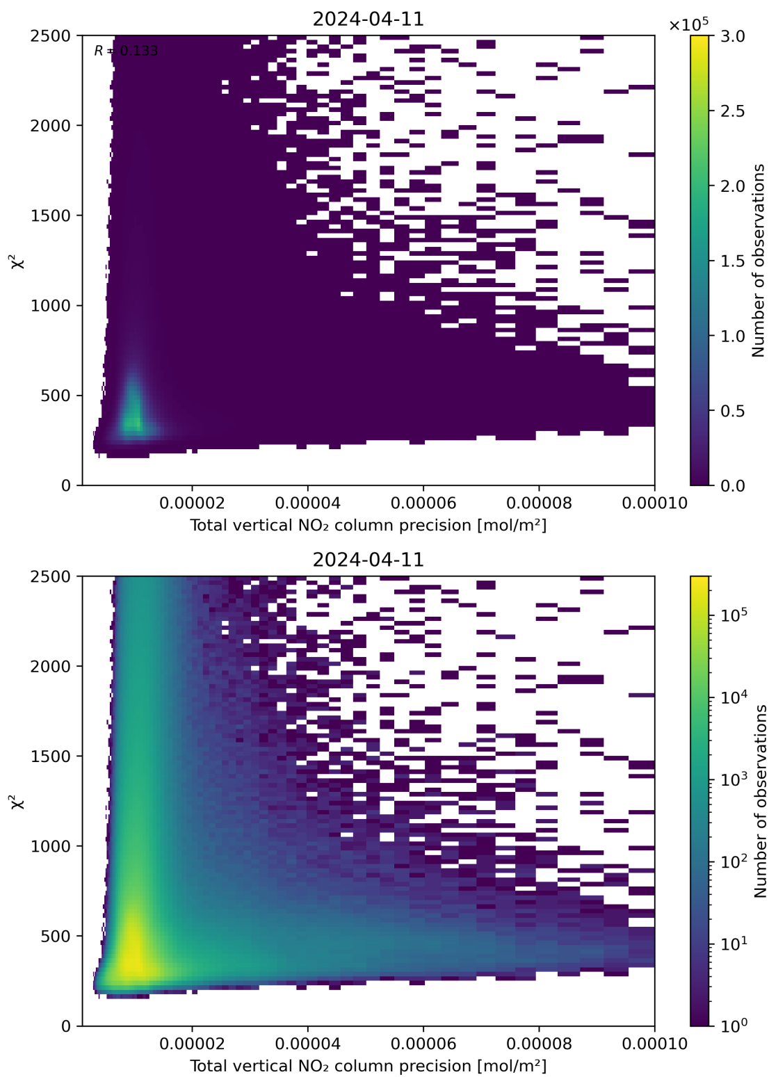
Figure 116: Scatter density plot of “Total vertical NO 2 column precision” against “ \chi^2 ” for 2024-04-10 to 2024-04-12.
