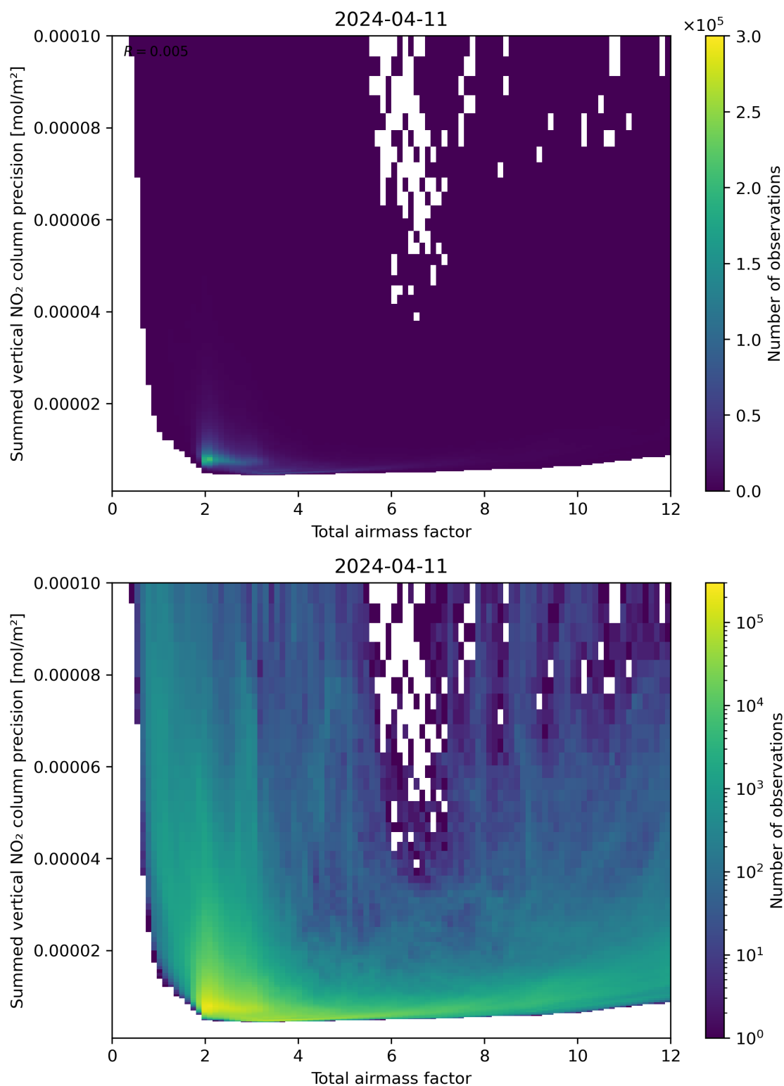
Figure 66: Scatter density plot of “Total airmass factor” against “Summed vertical NO 2 column precision” for 2024-04-10 to 2024-04-12.
