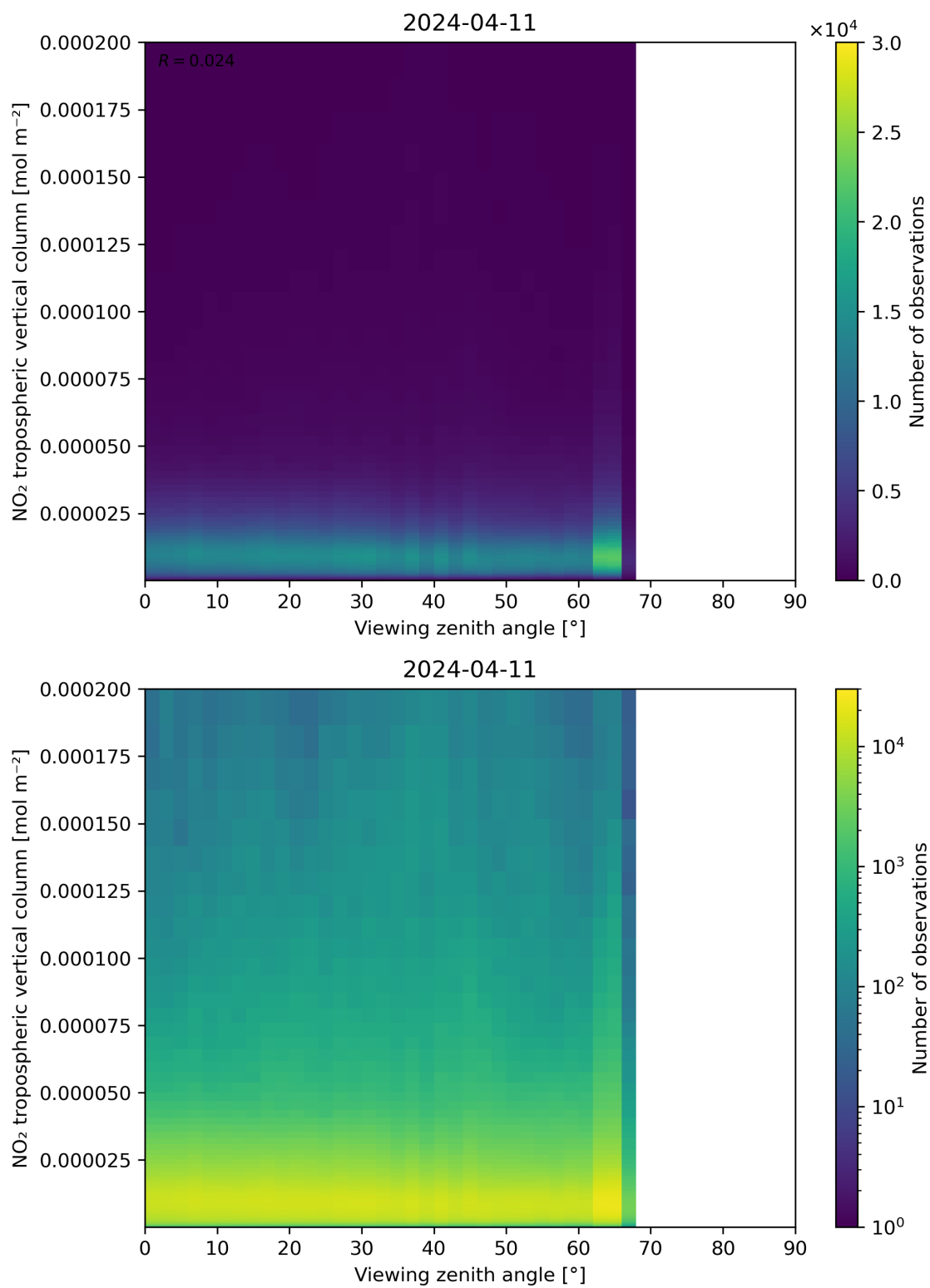
Figure 169: Scatter density plot of “Viewing zenith angle” against “NO 2 tropospheric vertical column” for 2024-04-10 to 2024-04-12.
