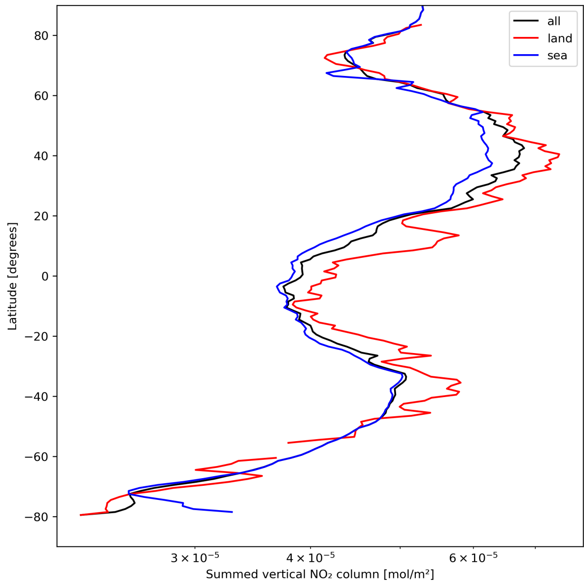
Figure 23: Zonal average of “Summed vertical NO 2 column” for 2024-04-10 to 2024-04-12.
