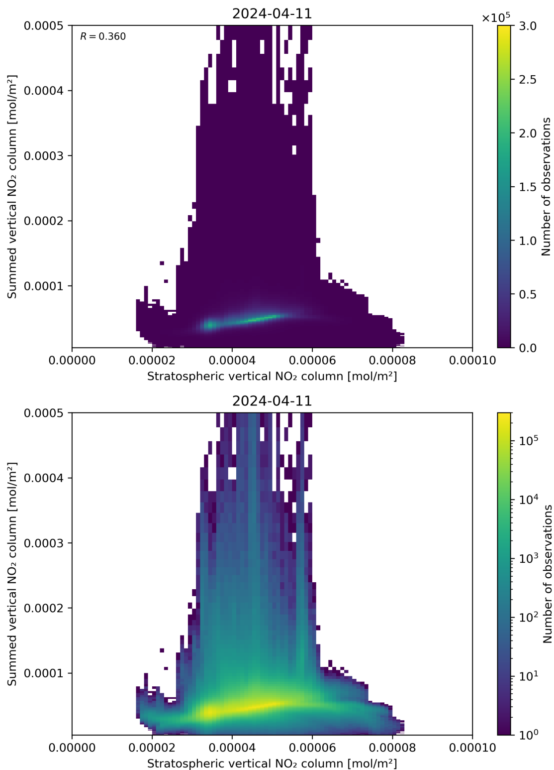
Figure 98: Scatter density plot of “Stratospheric vertical NO 2 column” against “Summed vertical NO 2 column” for 2024-04-10 to 2024-04-12.
