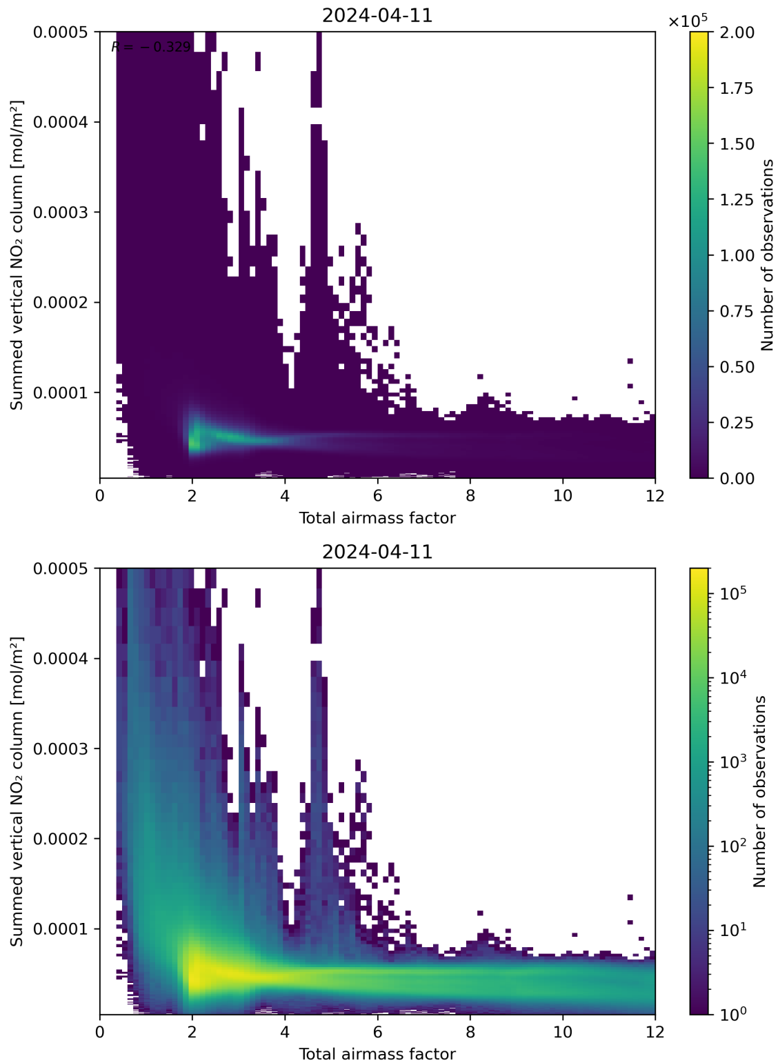
Figure 65: Scatter density plot of “Total airmass factor” against “Summed vertical NO 2 column” for 2024-04-10 to 2024-04-12.
