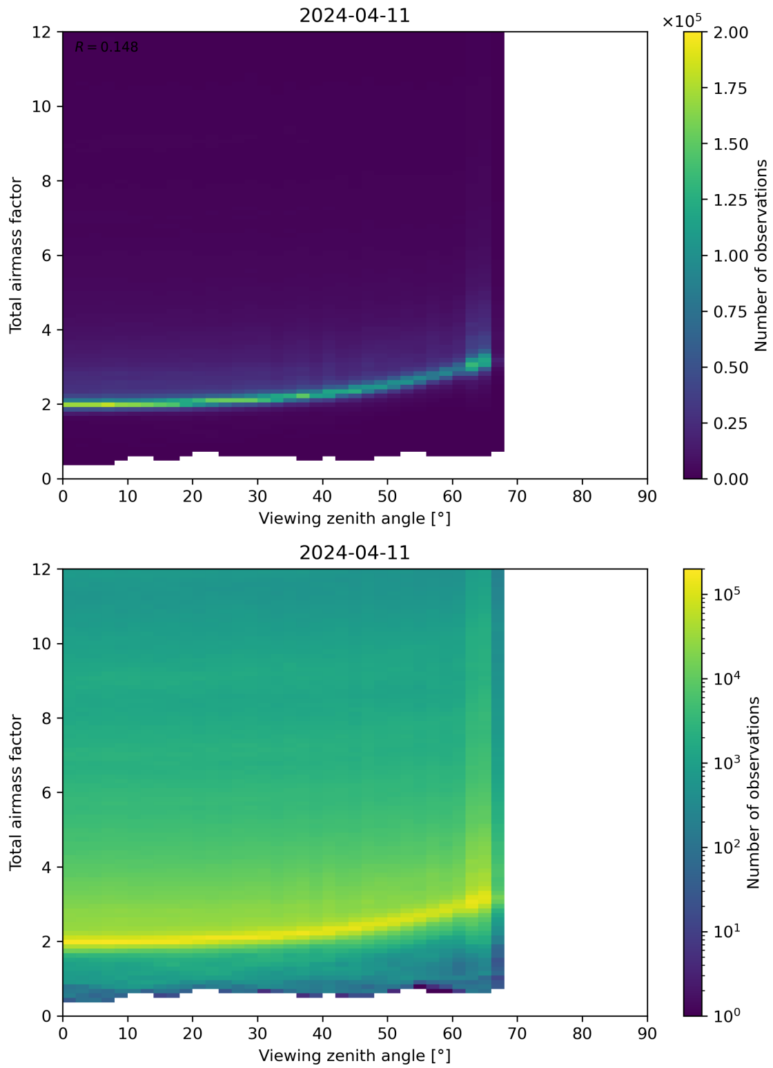
Figure 160: Scatter density plot of “Viewing zenith angle” against “Total airmass factor” for 2024-04-10 to 2024-04-12.
