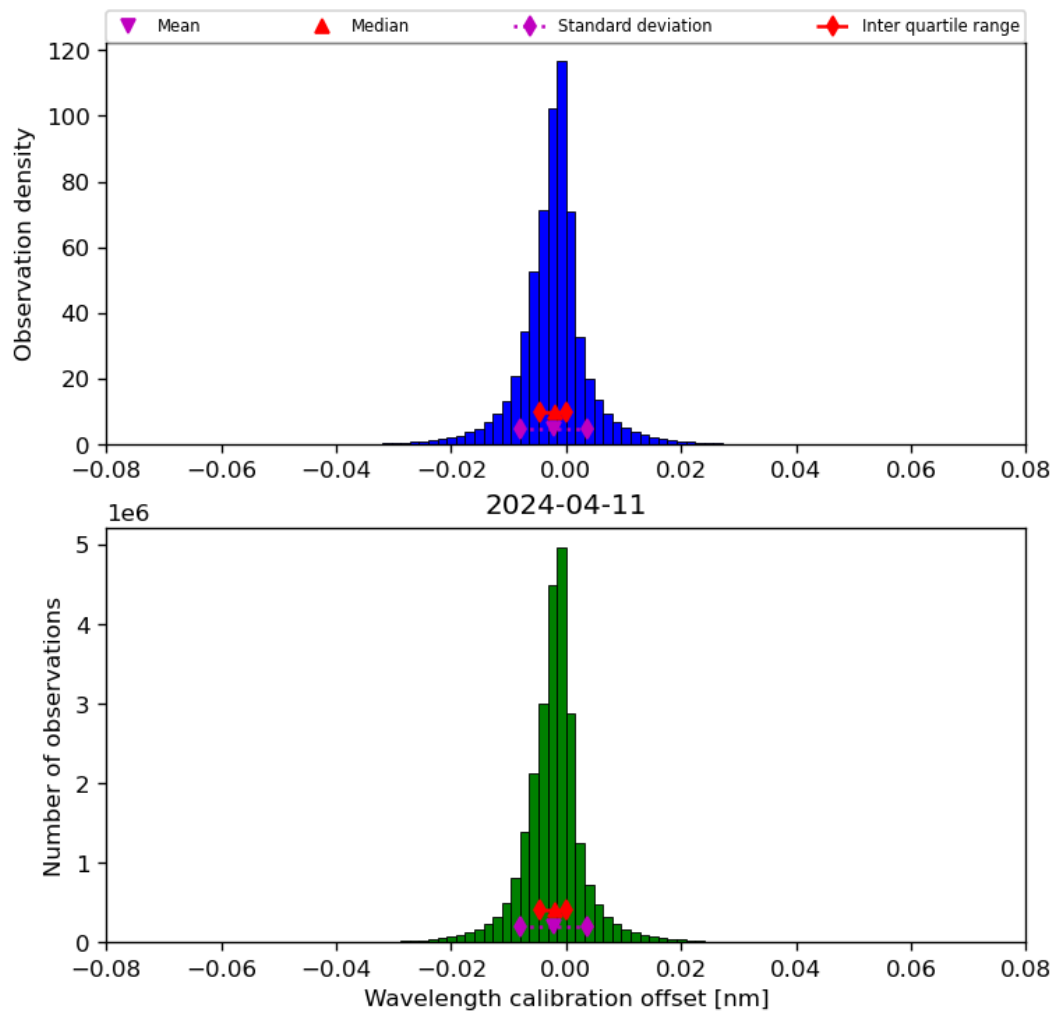
Figure 35: Histogram of “Wavelength calibration offset” for 2024-04-10 to 2024-04-12
