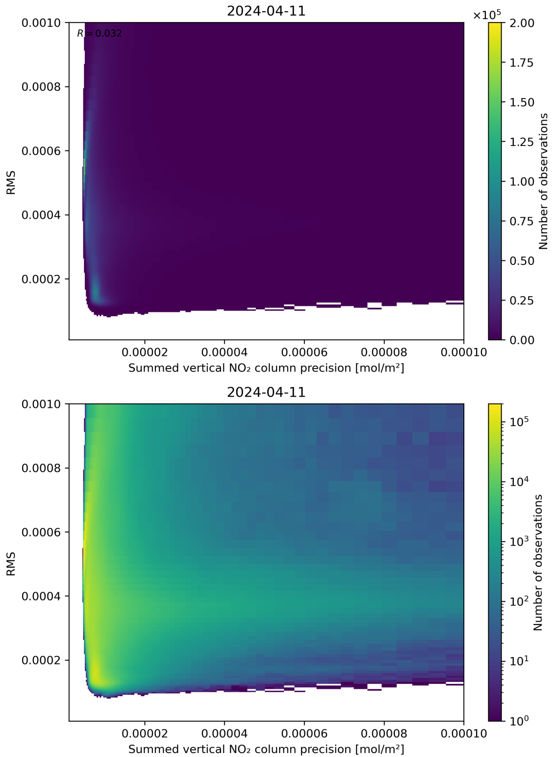
Figure 108: Scatter density plot of “Summed vertical NO 2 column precision” against “RMS” for 2024-04-10 to 2024-04-12.
