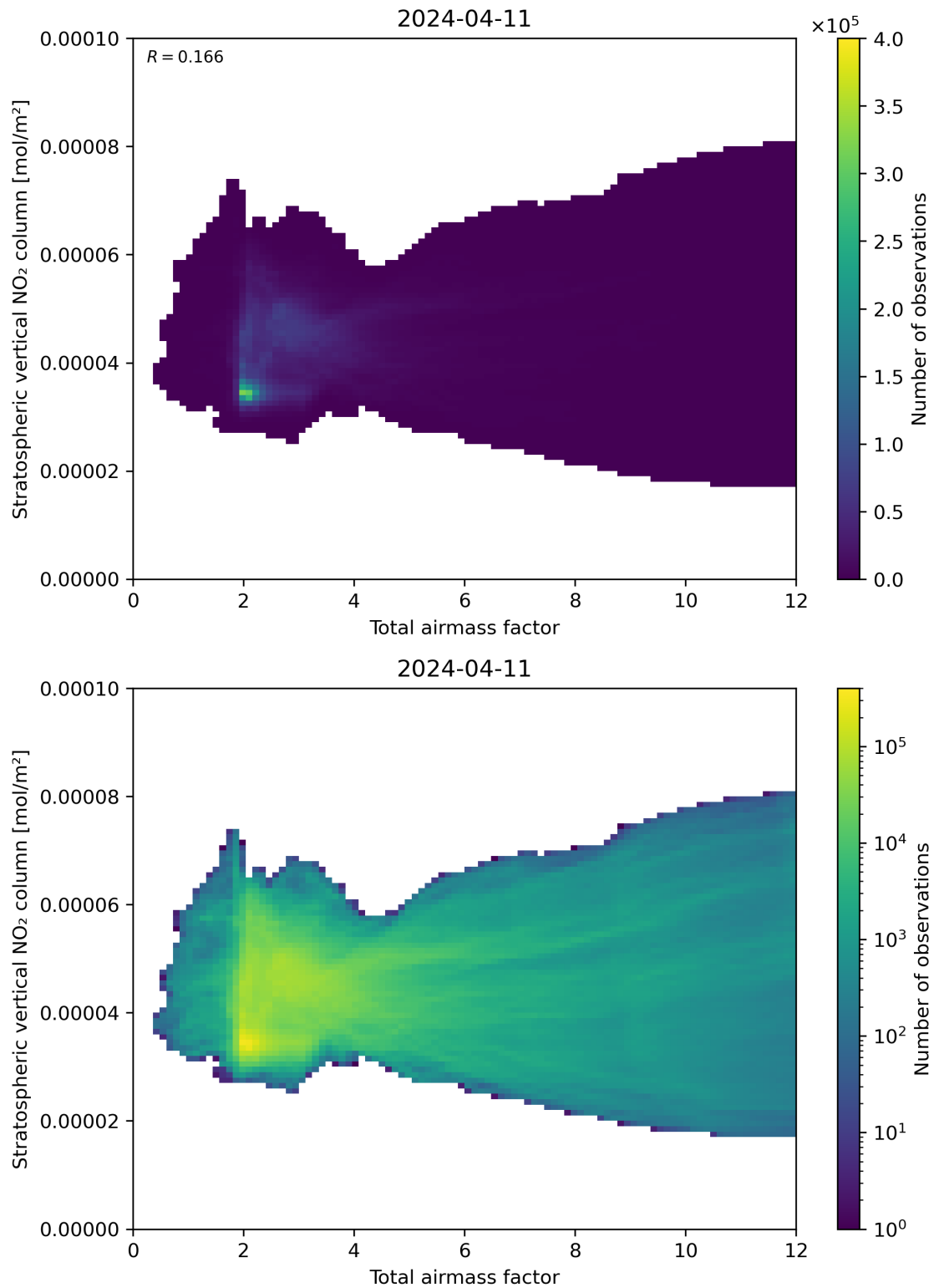
Figure 64: Scatter density plot of “Total airmass factor” against “Stratospheric vertical NO 2 column” for 2024-04-10 to 2024-04-12.
