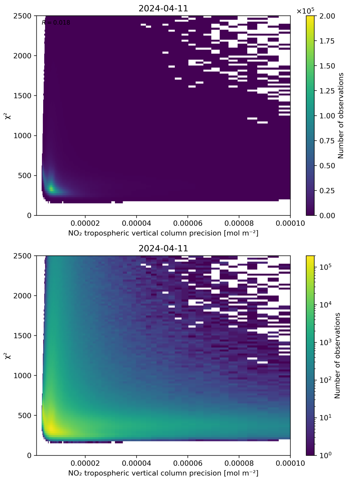
Figure 134: Scatter density plot of “NO 2 tropospheric vertical column precision” against “ \chi^2 ” for 2024-04-10 to 2024-04-12.
