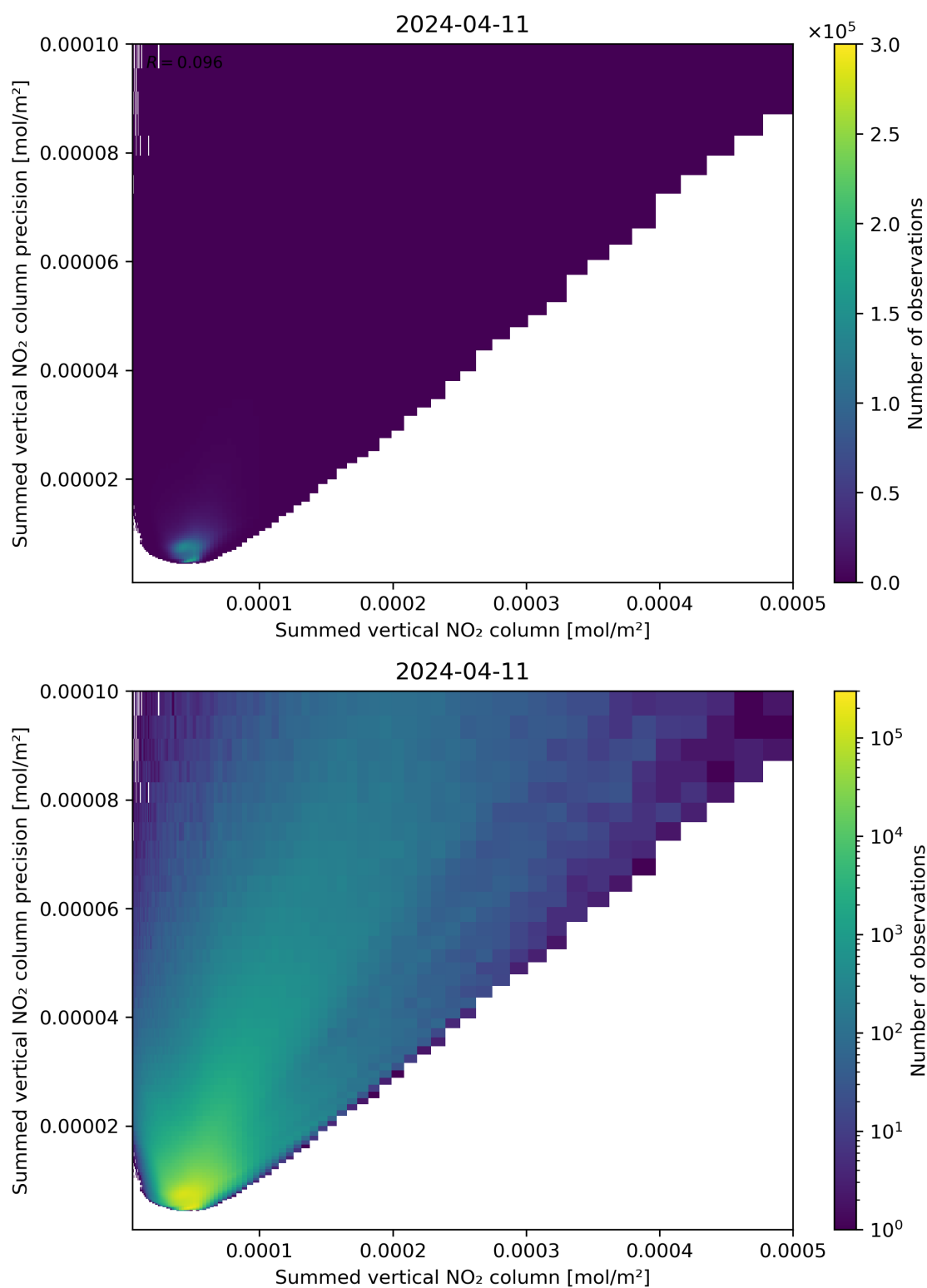
Figure 105: Scatter density plot of “Summed vertical NO 2 column” against “Summed vertical NO 2 column precision” for 2024-04-10 to 2024-04-12.
