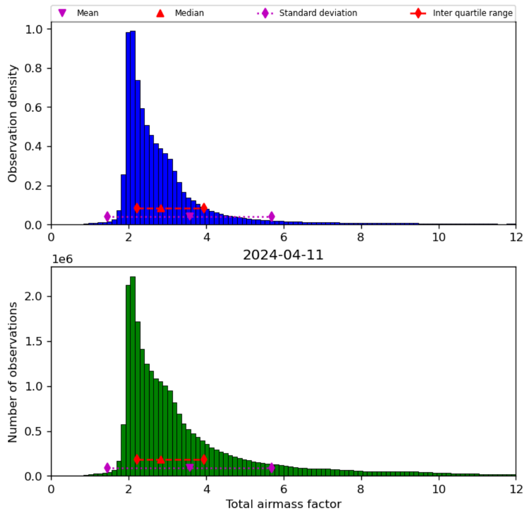
Figure 32: Histogram of “Total airmass factor” for 2024-04-10 to 2024-04-12
