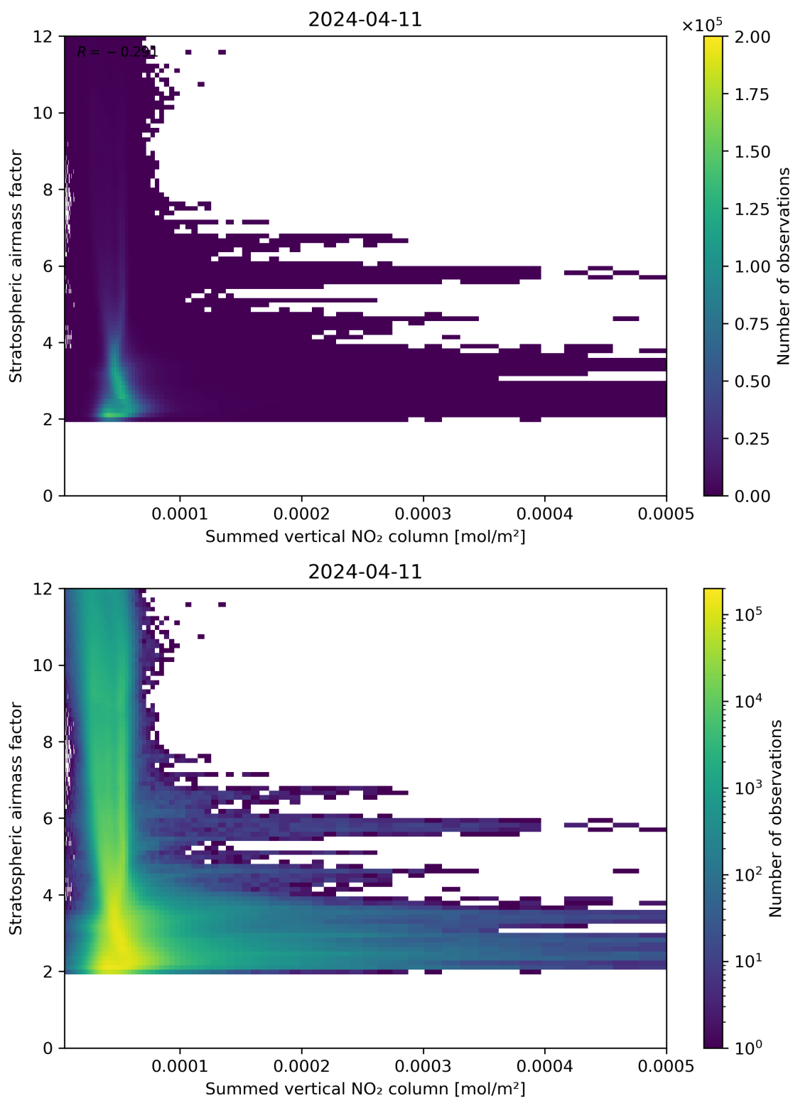
Figure 103: Scatter density plot of “Summed vertical NO 2 column” against “Stratospheric airmass factor” for 2024-04-10 to 2024-04-12.
