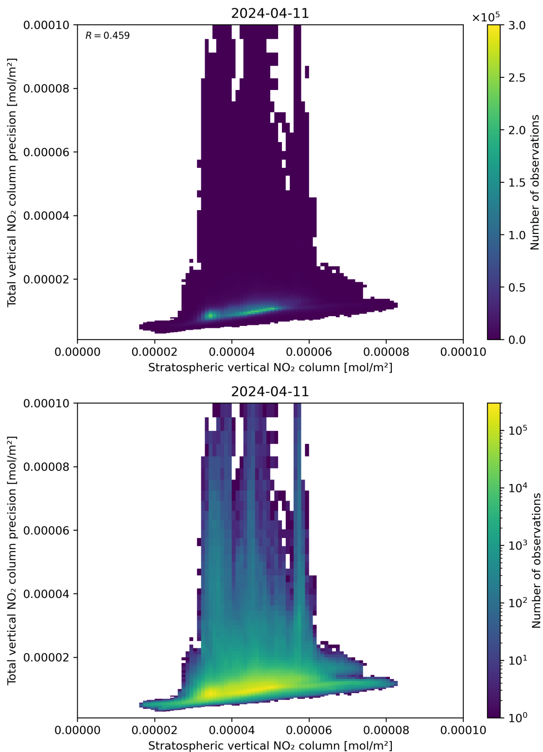
Figure 101: Scatter density plot of “Stratospheric vertical NO 2 column” against “Total vertical NO 2 column precision” for 2024-04-10 to 2024-04-12.
