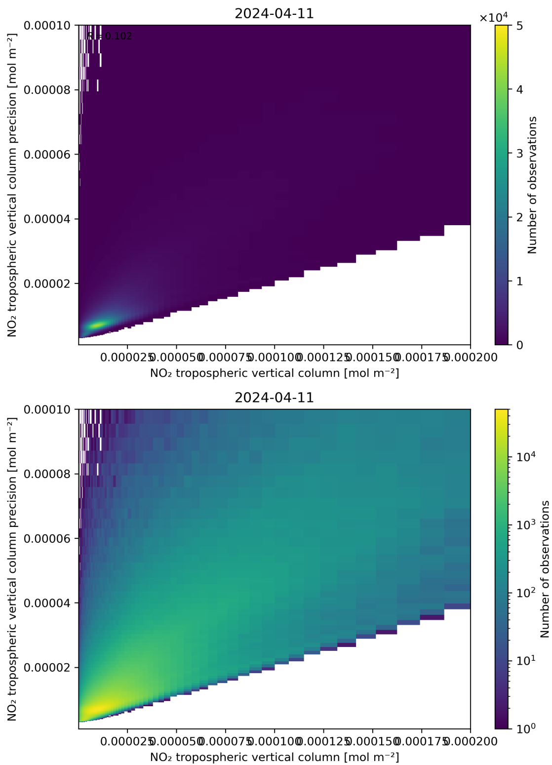
Figure 130: Scatter density plot of “NO 2 tropospheric vertical column” against “NO 2 tropospheric vertical column precision” for 2024-04-10 to 2024-04-12.
