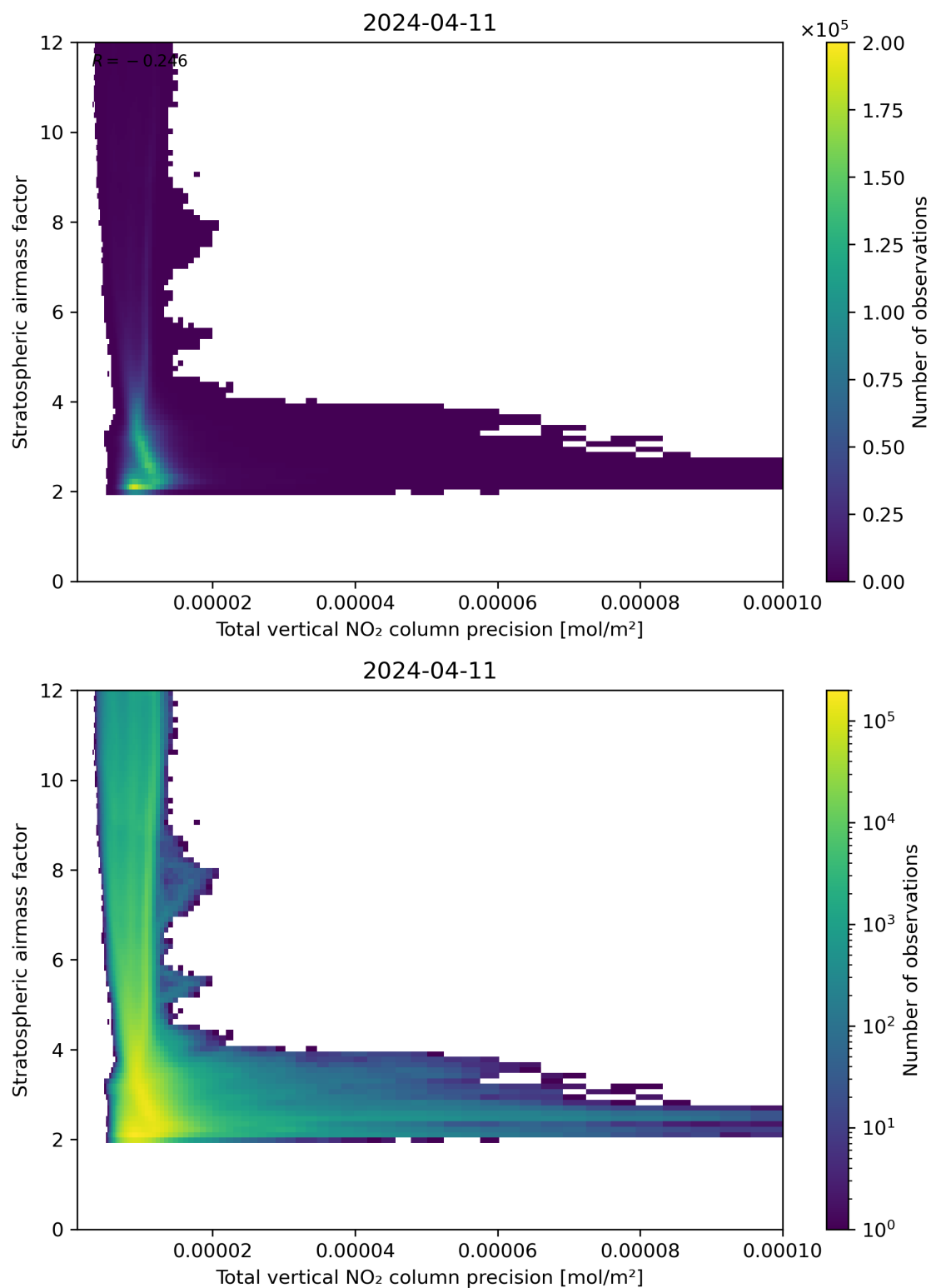
Figure 115: Scatter density plot of “Total vertical NO 2 column precision” against “Stratospheric air mass factor” for 2024-04-10 to 2024-04-12.
