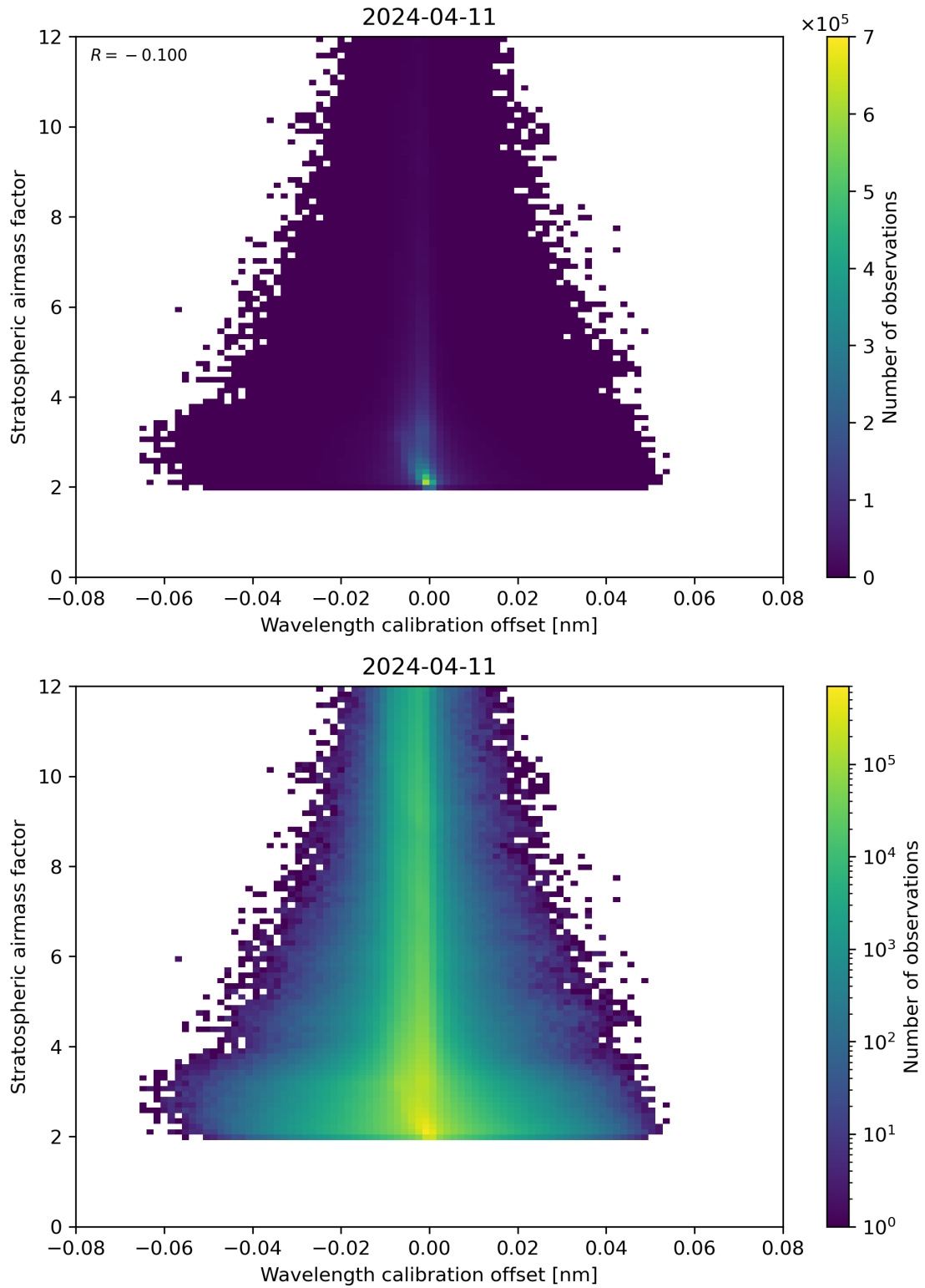
Figure 174: Scatter density plot of “Wavelength calibration offset” against “Stratospheric airmass factor” for 2024-04-10 to 2024-04-12.
