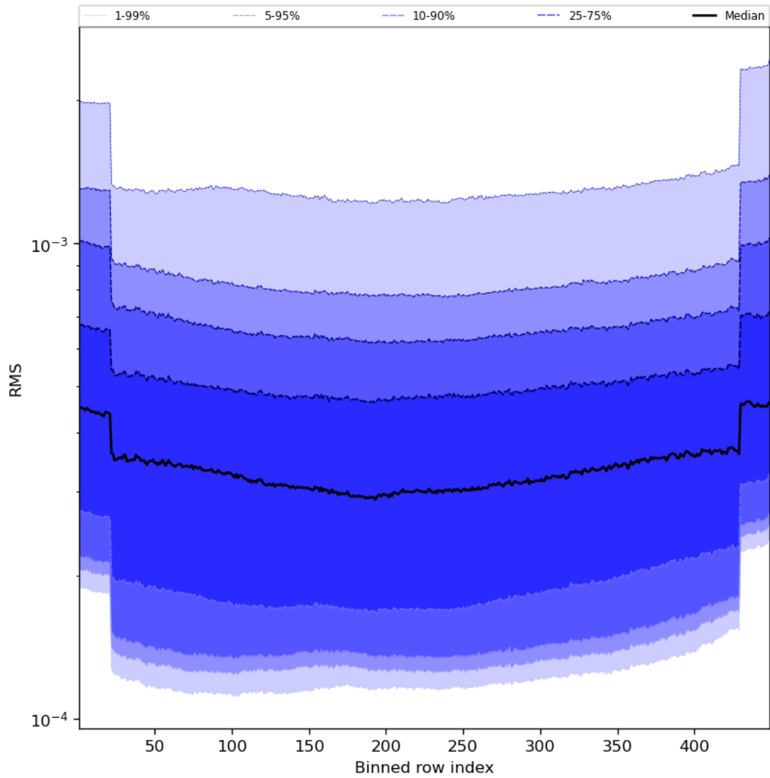
Figure 60: Along track statistics of “RMS” for 2024-04-10 to 2024-04-12
