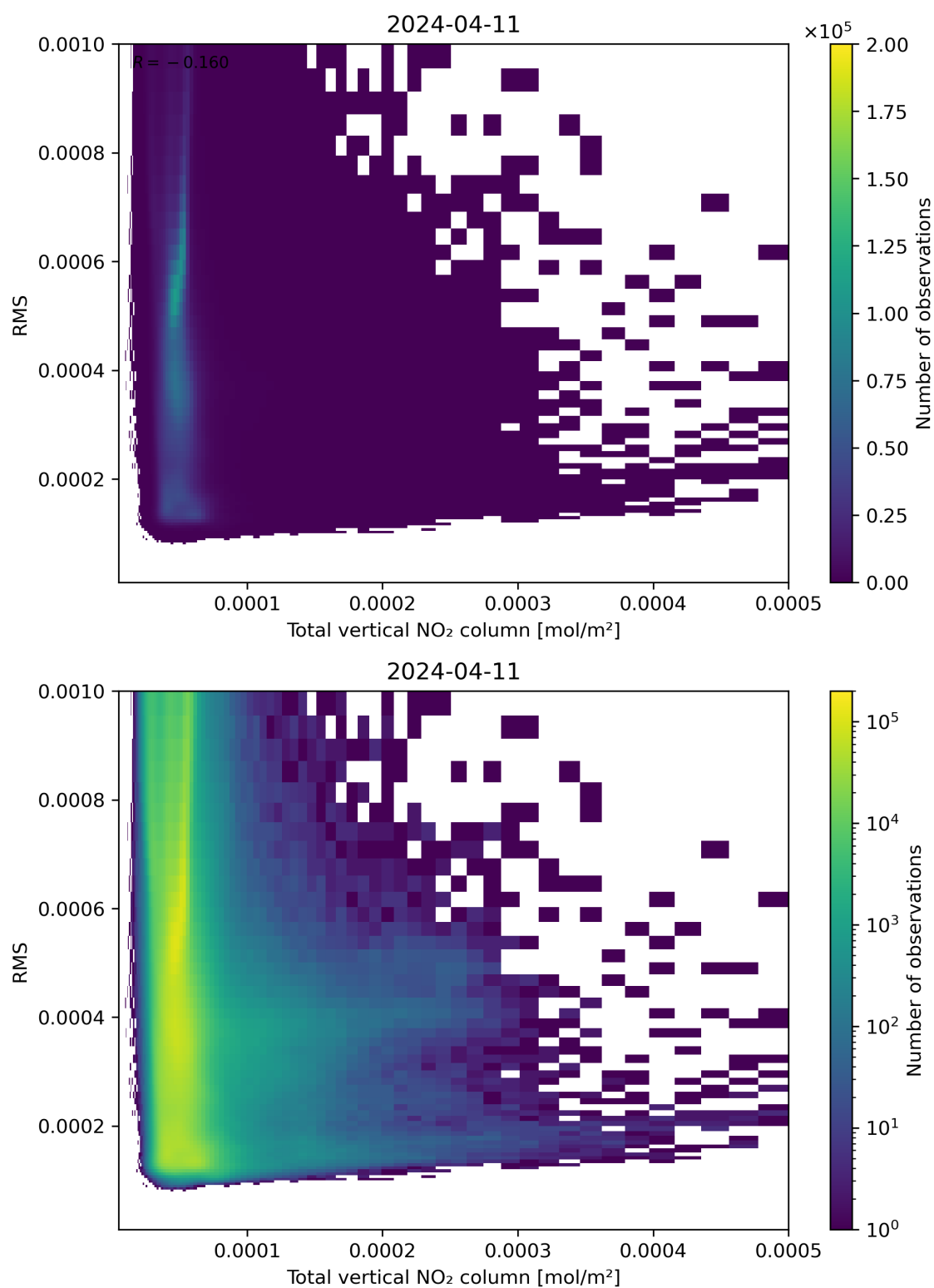
Figure 120: Scatter density plot of “Total vertical NO 2 column” against “RMS” for 2024-04-10 to 2024-04-12.
