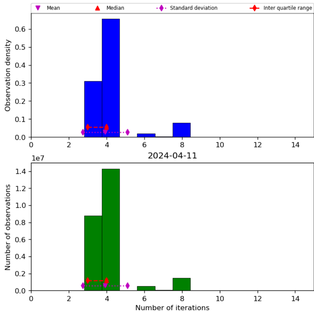
Figure 34: Histogram of “Number of iterations” for 2024-04-10 to 2024-04-12
