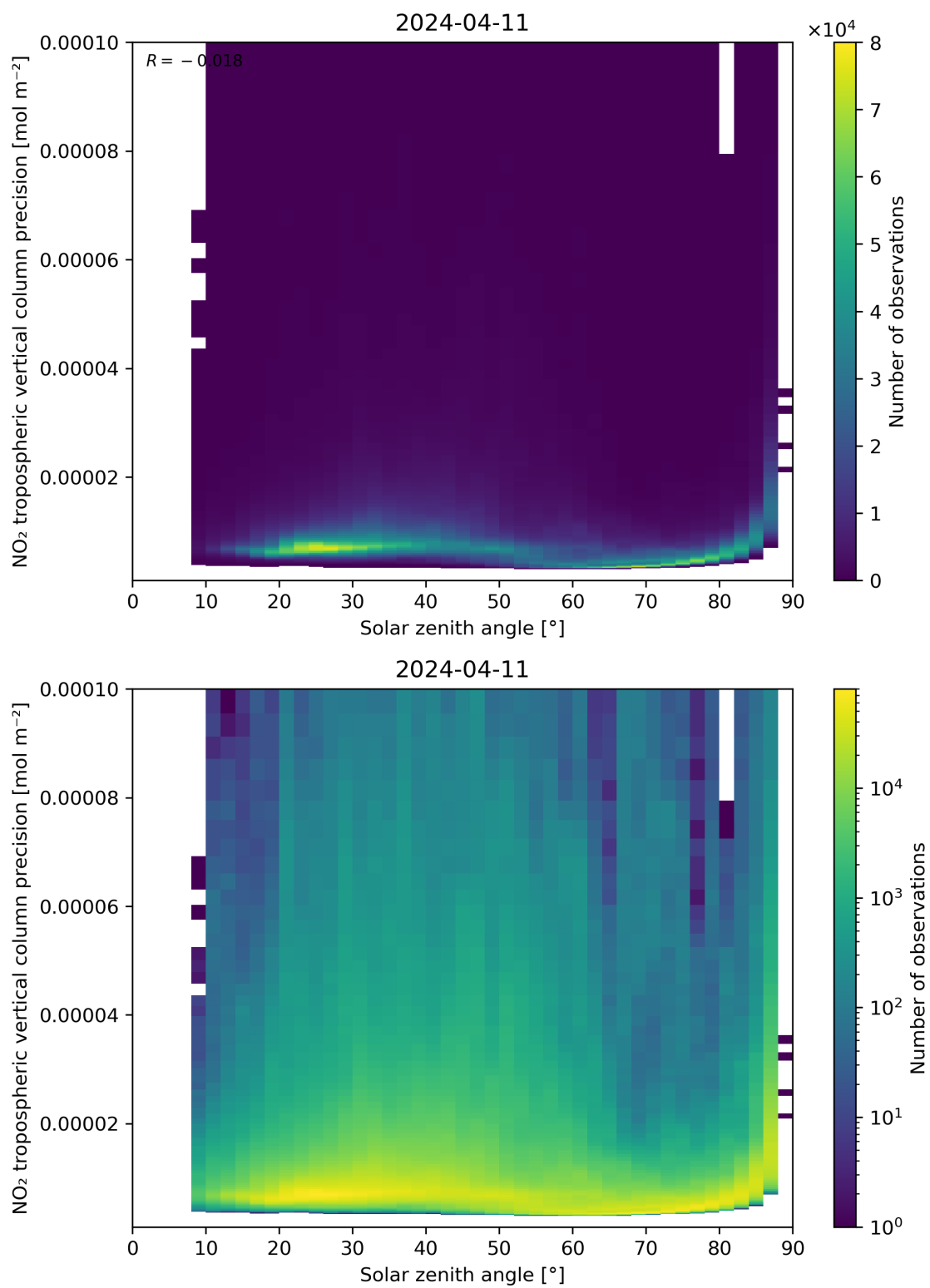
Figure 156: Scatter density plot of “Solar zenith angle” against “NO 2 tropospheric vertical column precision” for 2024-04-10 to 2024-04-12.
