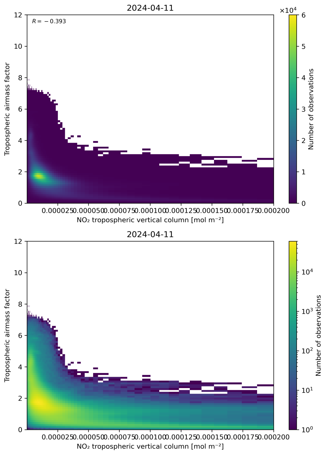
Figure 123: Scatter density plot of “NO 2 tropospheric vertical column” against “Tropospheric air mass factor” for 2024-04-10 to 2024-04-12.
