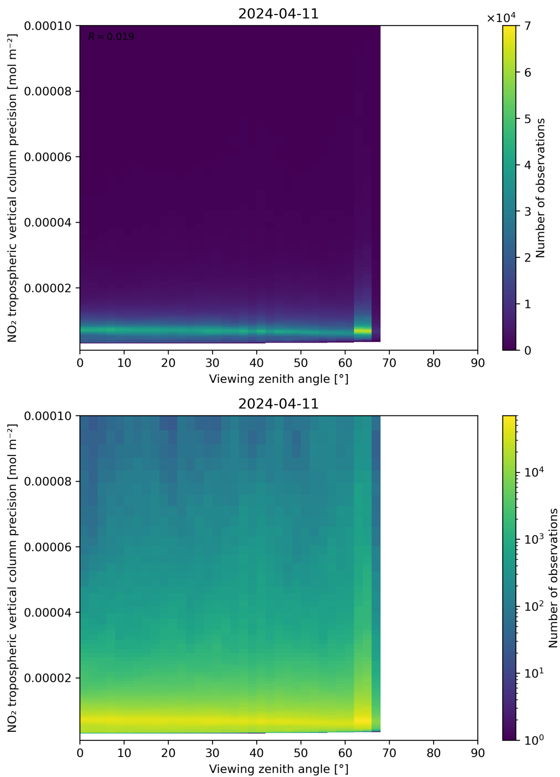
Figure 170: Scatter density plot of “Viewing zenith angle” against “NO 2 tropospheric vertical column precision” for 2024-04-10 to 2024-04-12.
