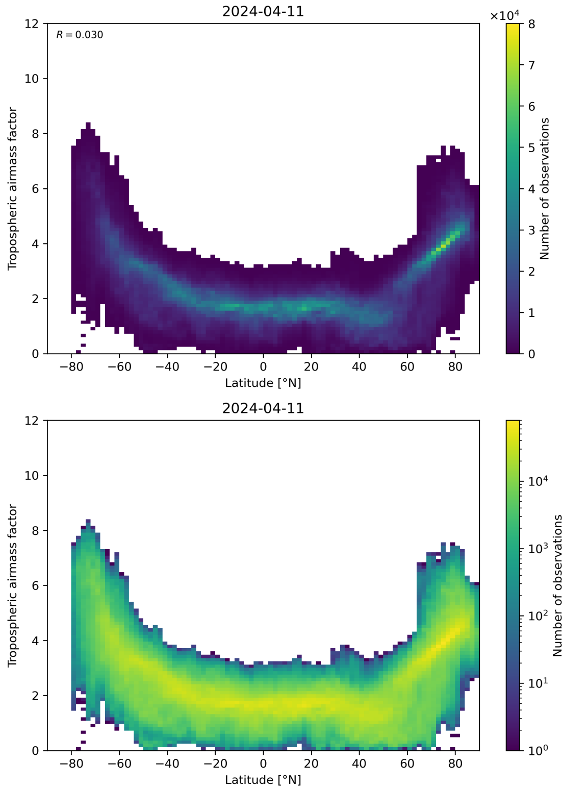
Figure 85: Scatter density plot of “Latitude” against “Tropospheric airmass factor” for 2024-04-10 to 2024-04-12.
