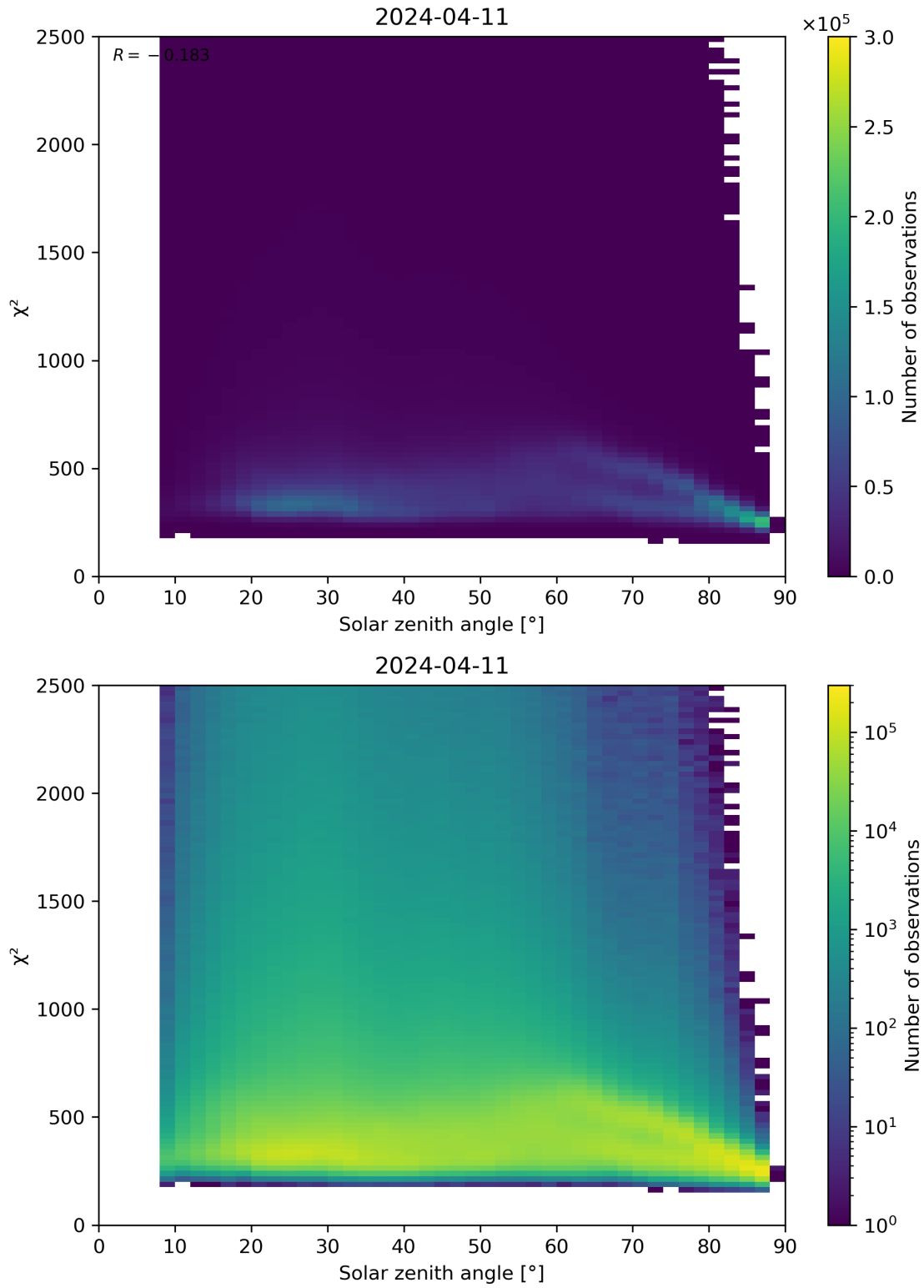
Figure 148: Scatter density plot of “Solar zenith angle” against “ \chi^2 ” for 2024-04-10 to 2024-04-12.
