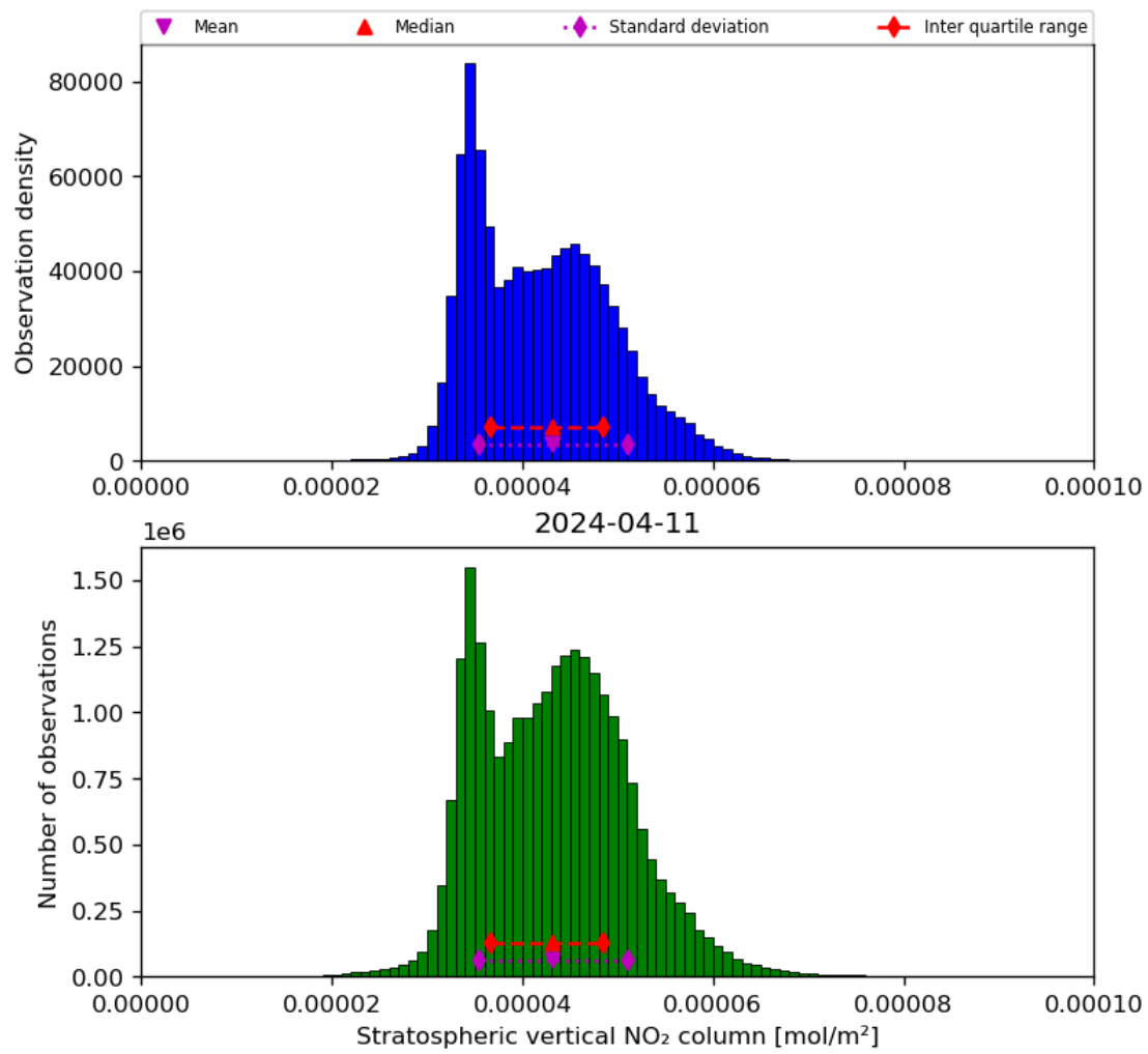
Figure 36: Histogram of “Stratospheric vertical NO 2 column” for 2024-04-10 to 2024-04-12
