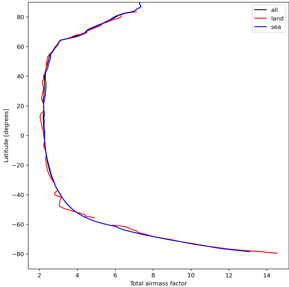
Figure 15: Zonal average of “Total airmass factor” for 2024-04-10 to 2024-04-12.
