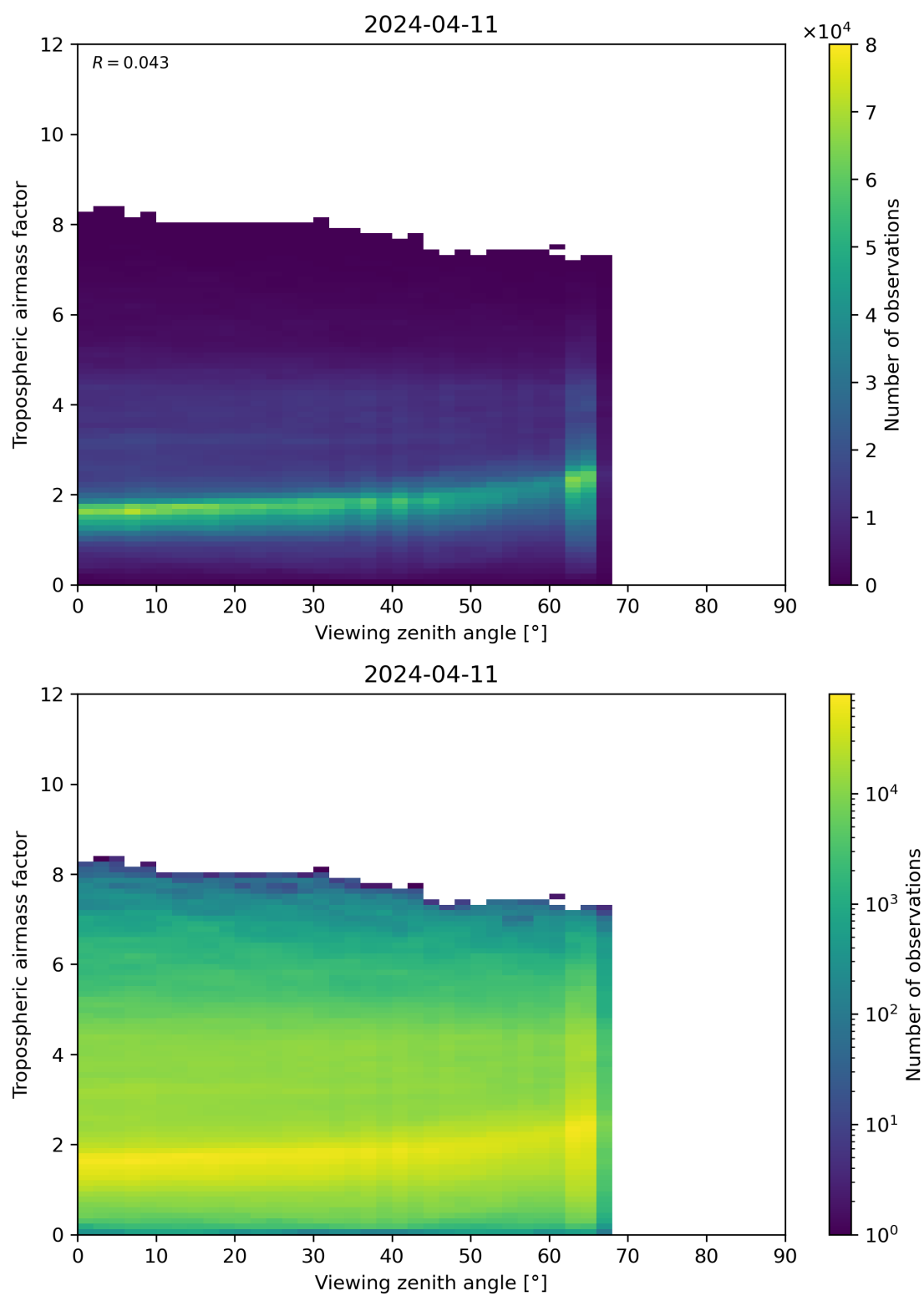
Figure 161: Scatter density plot of “Viewing zenith angle” against “Tropospheric airmass factor” for 2024-04-10 to 2024-04-12.
