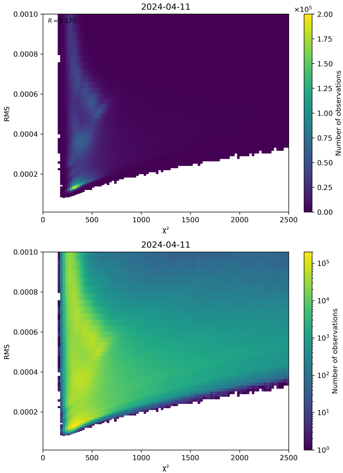
Figure 82: Scatter density plot of “ \chi^2 ” against “RMS” for 2024-04-10 to 2024-04-12.
