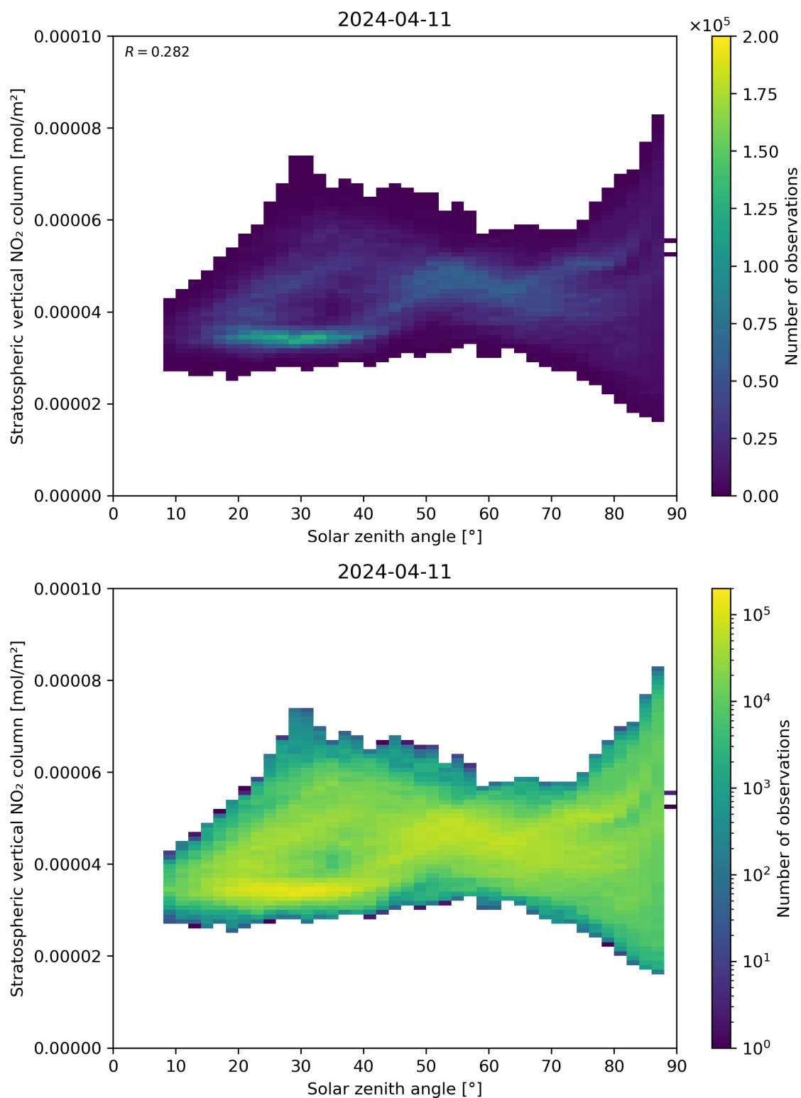
Figure 150: Scatter density plot of “Solar zenith angle” against “Stratospheric vertical NO 2 column” for 2024-04-10 to 2024-04-12.
