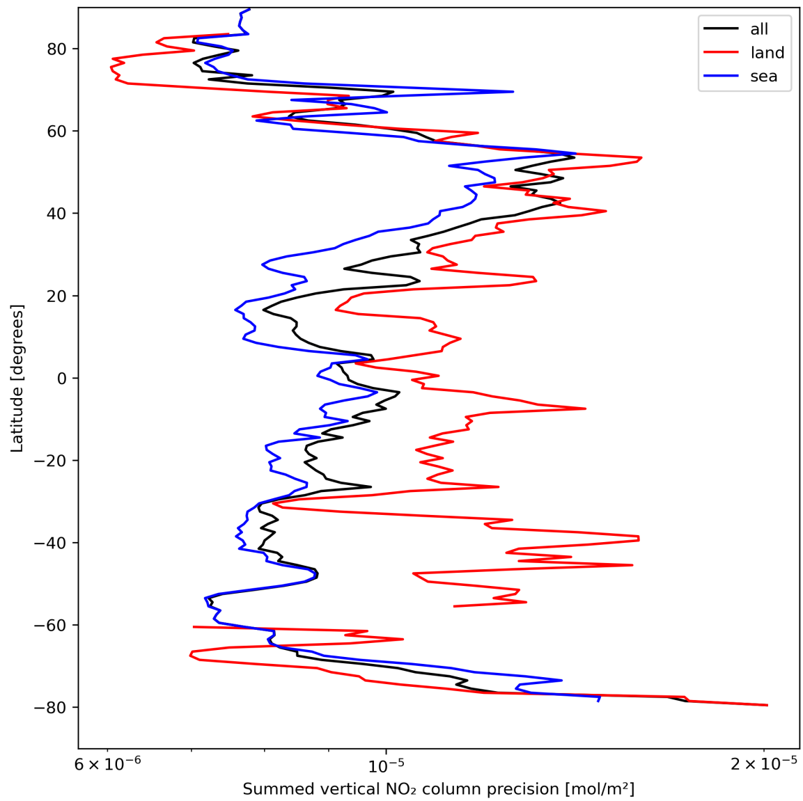
Figure 24: Zonal average of “Summed vertical NO 2 column precision” for 2024-04-10 to 2024-04-12.
