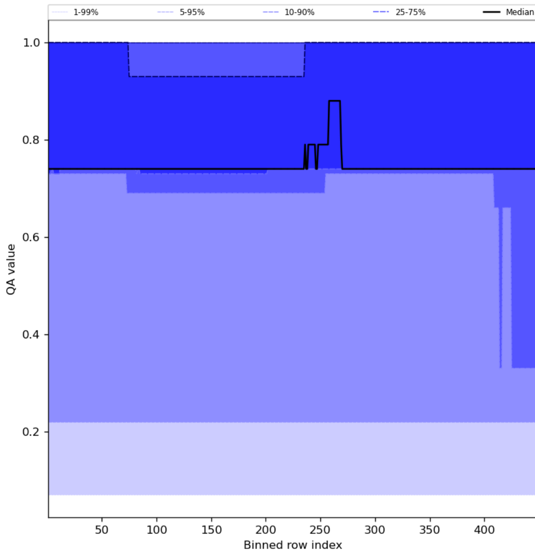
Figure 45: Along track statistics of “QA value” for 2024-04-10 to 2024-04-12
