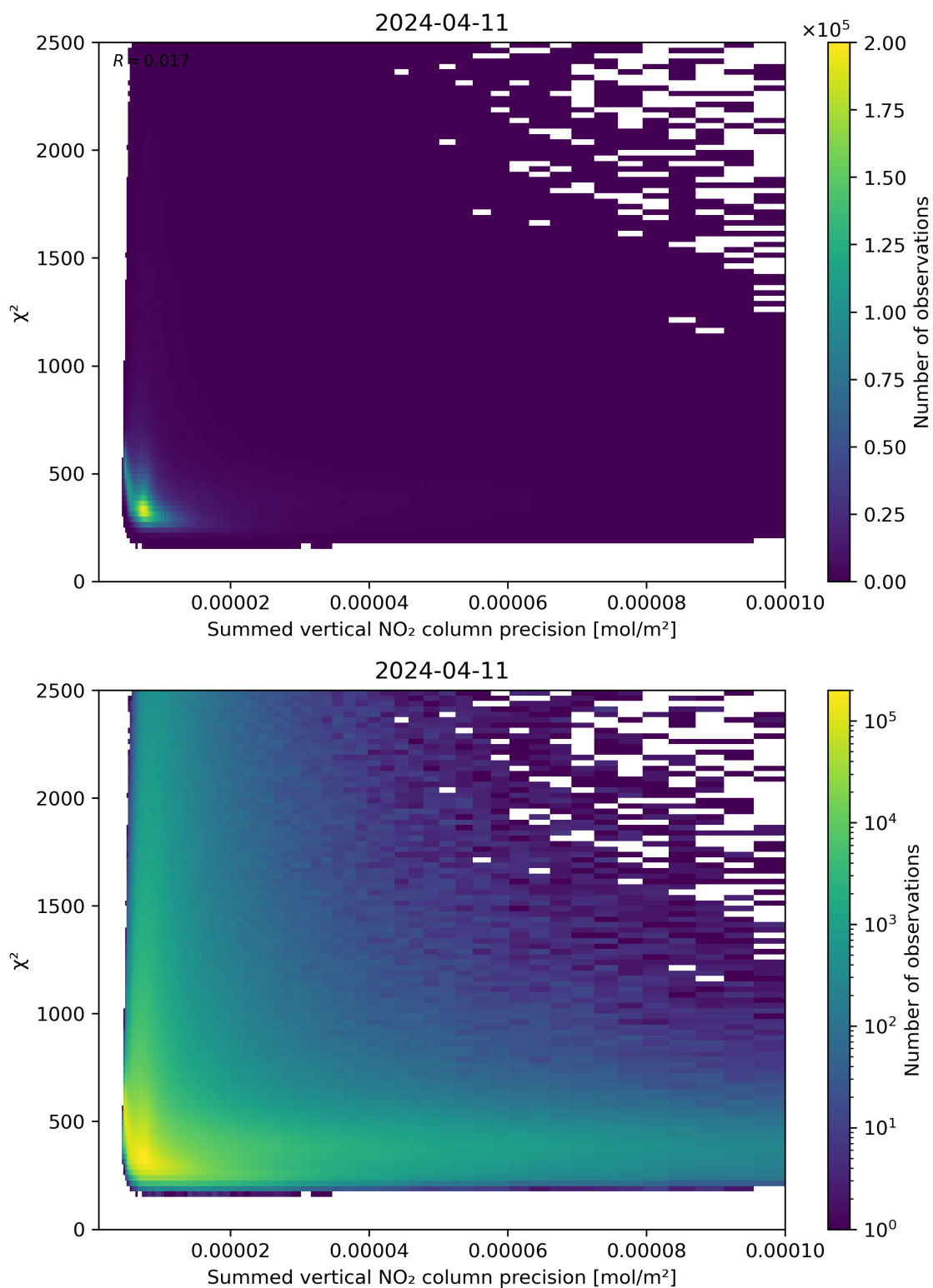
Figure 107: Scatter density plot of “Summed vertical NO 2 column precision” against “ \chi^2 ” for 2024-04-10 to 2024-04-12.
