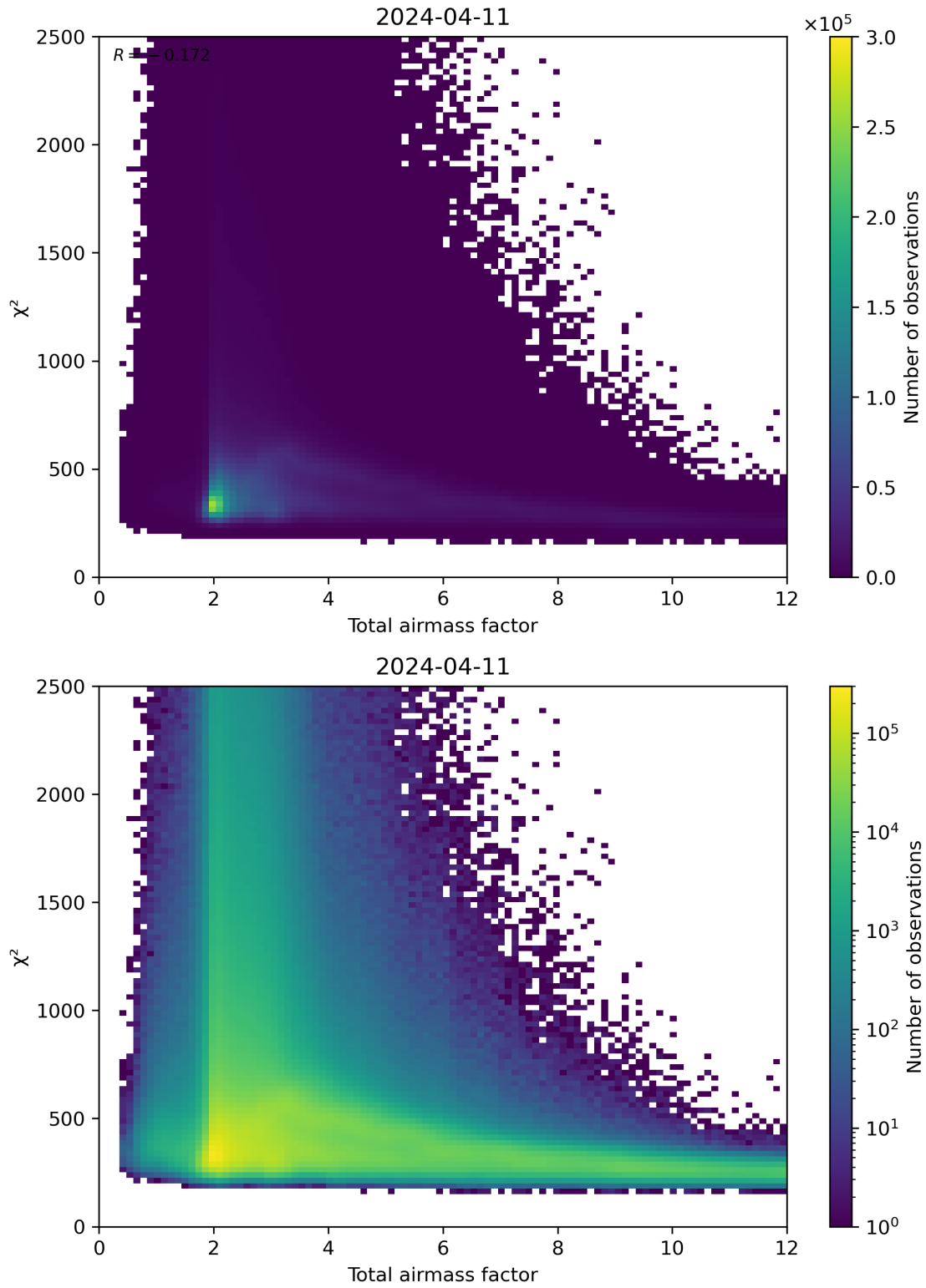
Figure 63: Scatter density plot of “Total airmass factor” against “ \chi^2 ” for 2024-04-10 to 2024-04-12.
