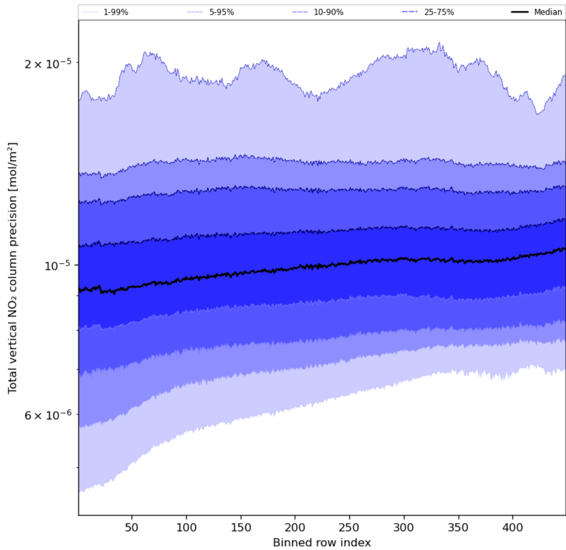
Figure 56: Along track statistics of “Total vertical NO 2 column precision” for 2024-04-10 to 2024-04-12
