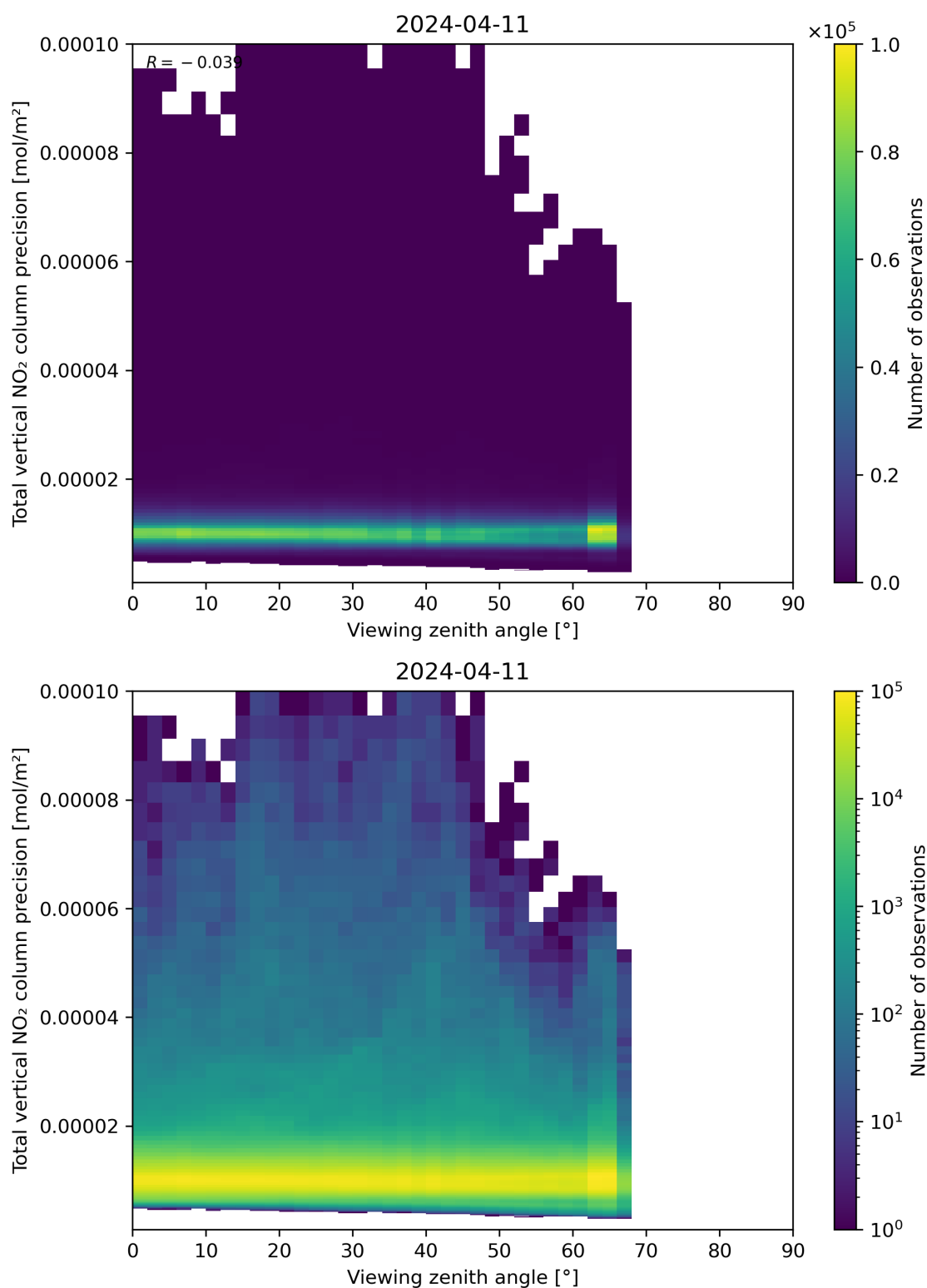
Figure 168: Scatter density plot of “Viewing zenith angle” against “Total vertical NO 2 column precision” for 2024-04-10 to 2024-04-12.
