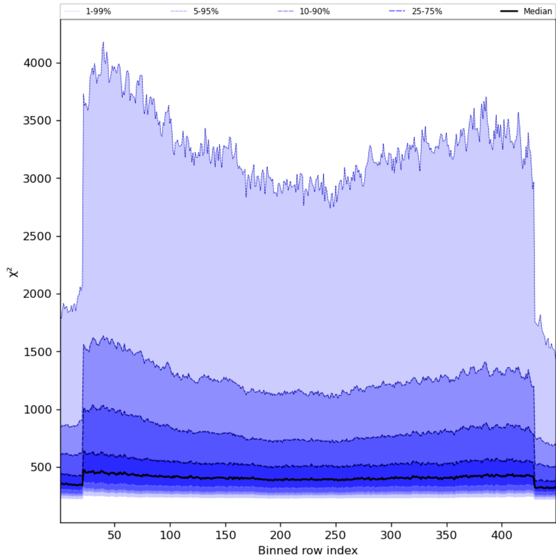
Figure 59: Along track statistics of “ \chi^2 ” for 2024-04-10 to 2024-04-12
