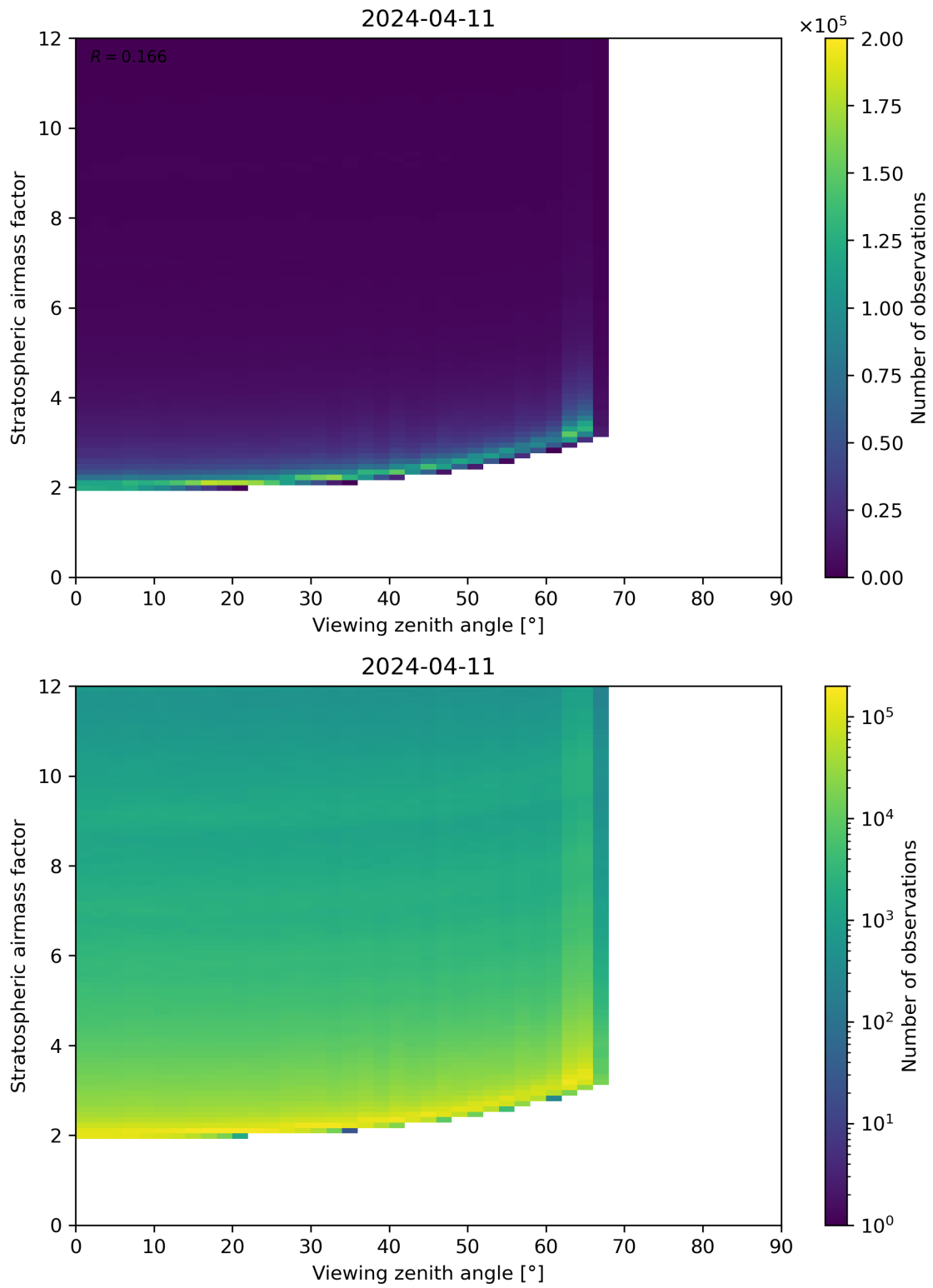
Figure 159: Scatter density plot of “Viewing zenith angle” against “Stratospheric airmass factor” for 2024-04-10 to 2024-04-12.
