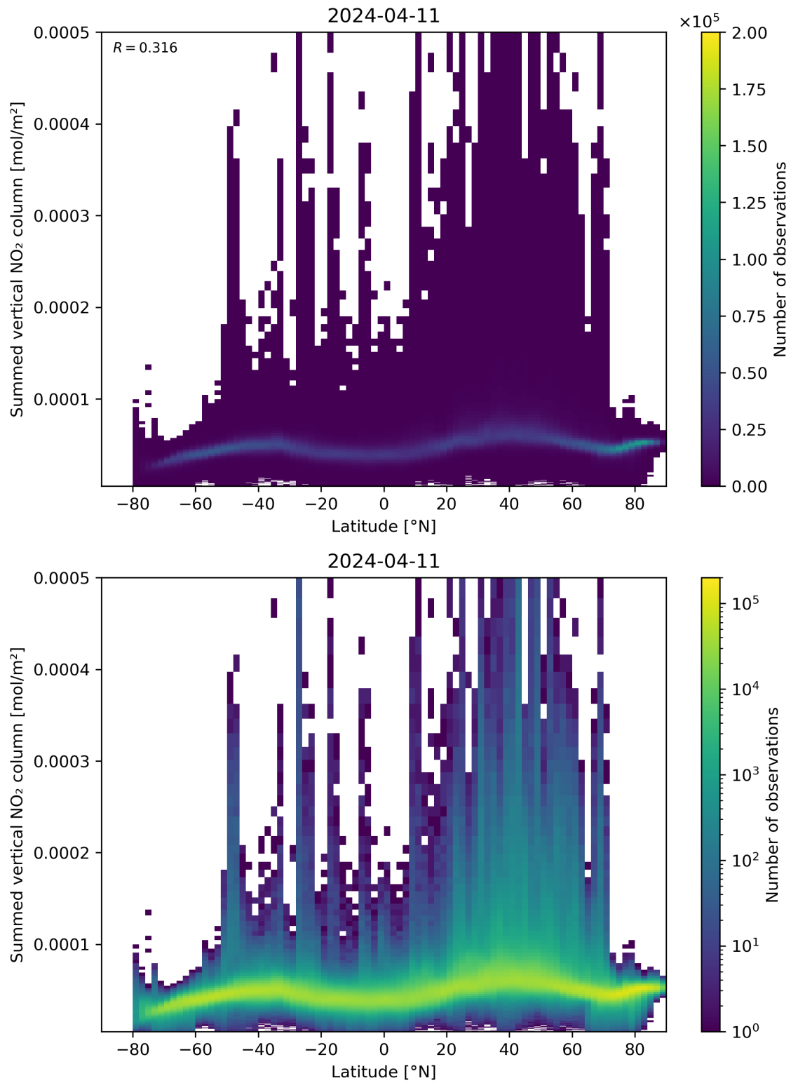
Figure 88: Scatter density plot of “Latitude” against “Summed vertical NO 2 column” for 2024-04-10 to 2024-04-12.
