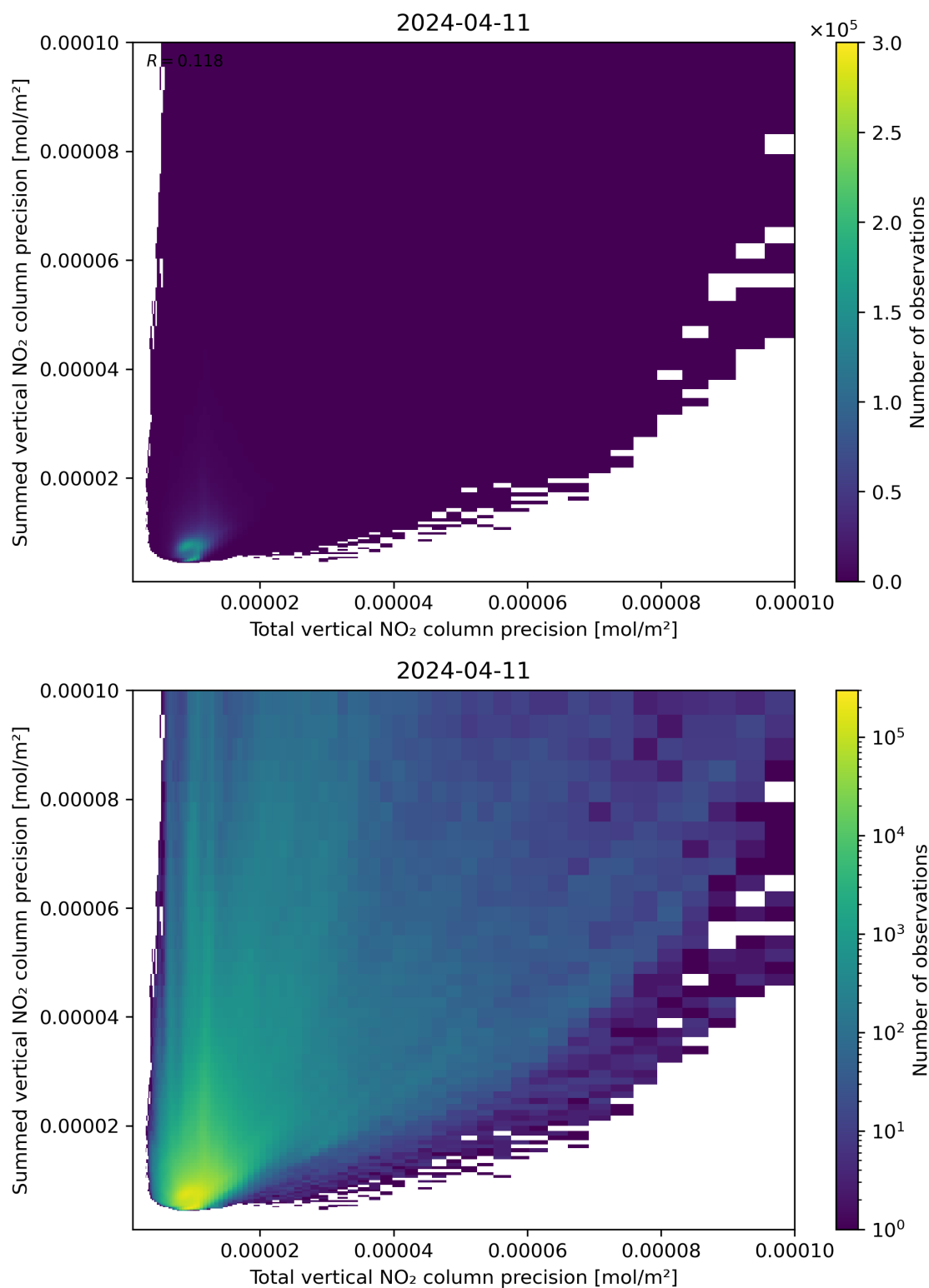
Figure 118: Scatter density plot of “Total vertical NO 2 column precision” against “Summed vertical NO 2 column precision” for 2024-04-10 to 2024-04-12.
