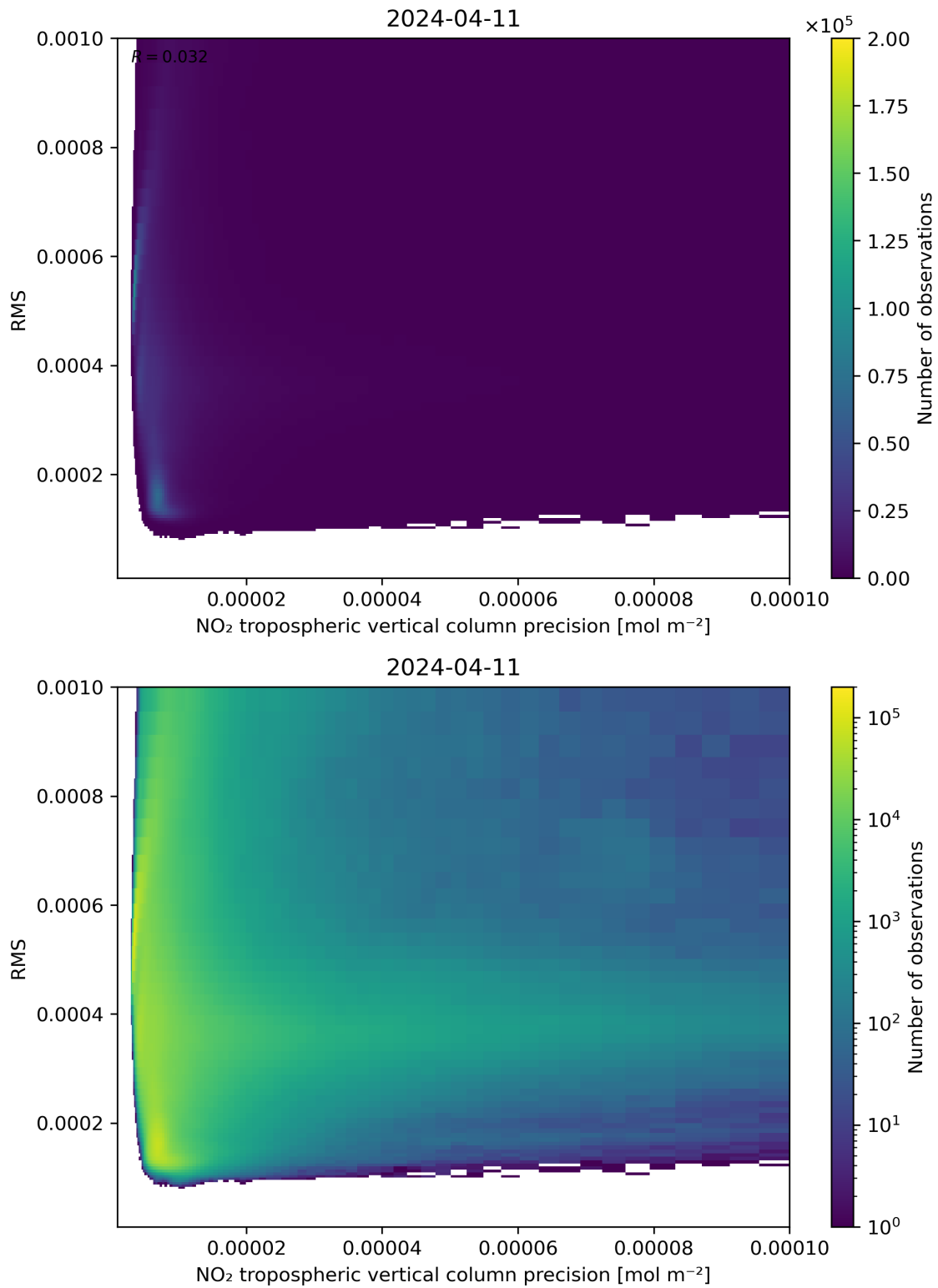
Figure 140: Scatter density plot of “NO 2 tropospheric vertical column precision” against “RMS” for 2024-04-10 to 2024-04-12.
