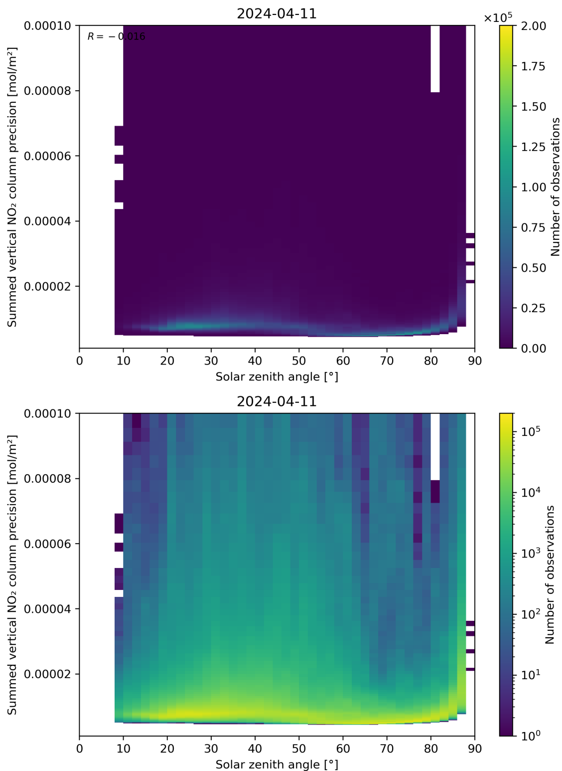
Figure 152: Scatter density plot of “Solar zenith angle” against “Summed vertical NO 2 column precision” for 2024-04-10 to 2024-04-12.
