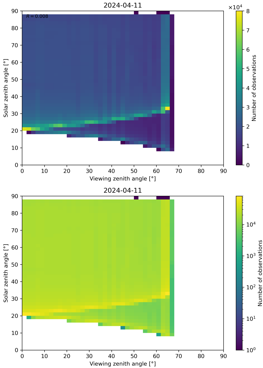
Figure 172: Scatter density plot of “Viewing zenith angle” against “Solar zenith angle” for 2024-04-10 to 2024-04-12.
