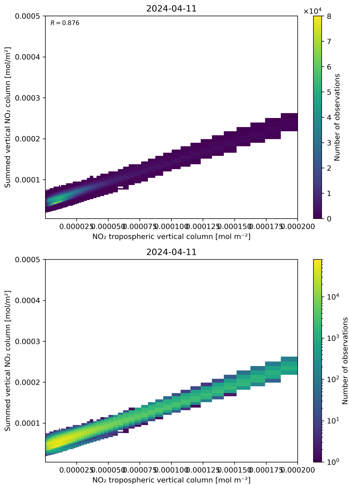
Figure 126: Scatter density plot of “NO 2 tropospheric vertical column” against “Summed vertical NO 2 column” for 2024-04-10 to 2024-04-12.
