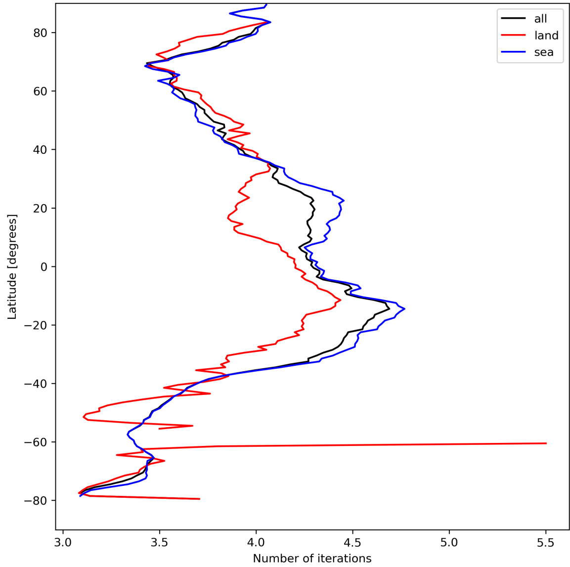
Figure 17: Zonal average of “Number of iterations” for 2024-04-10 to 2024-04-12.
