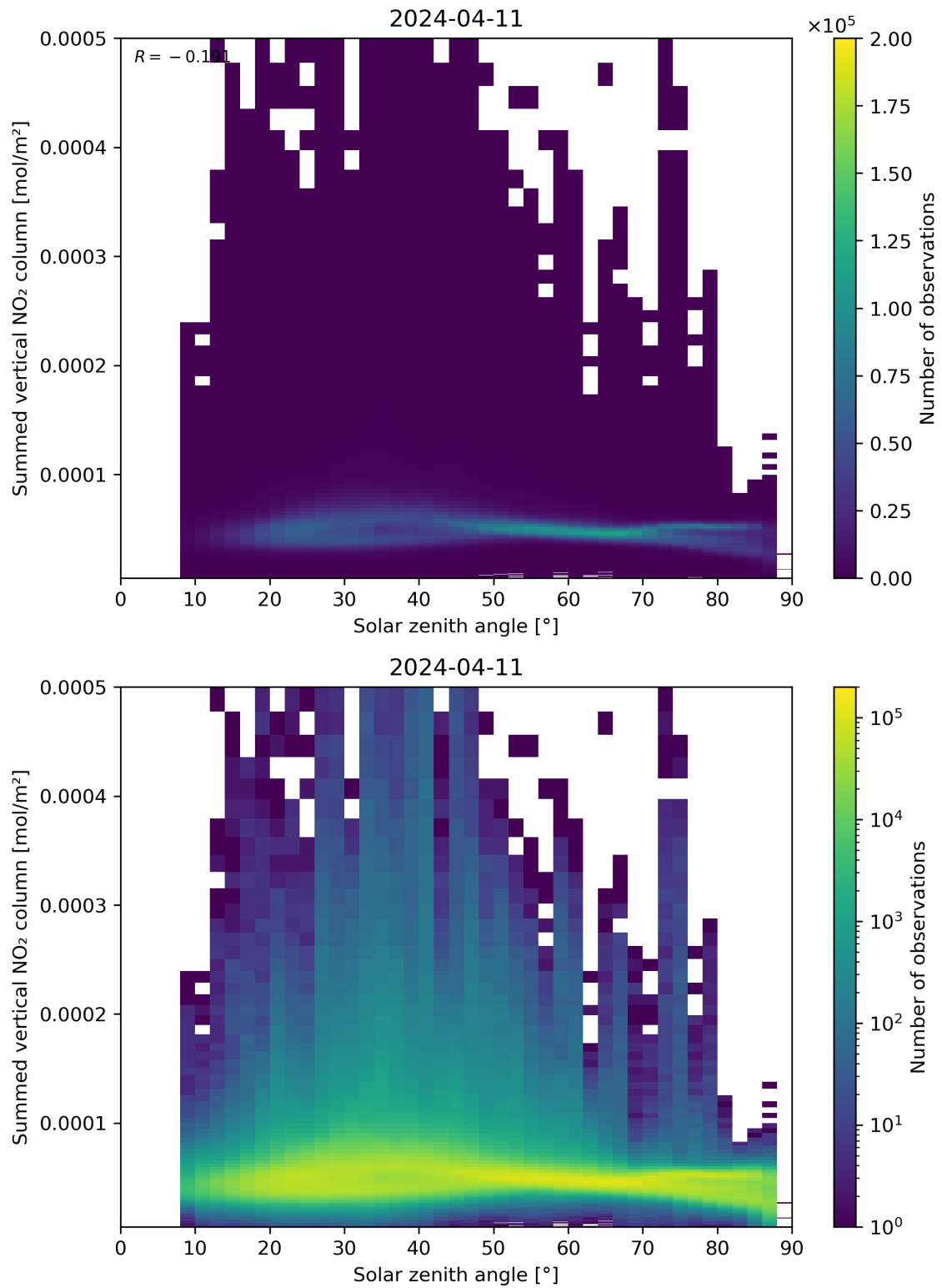
Figure 151: Scatter density plot of “Solar zenith angle” against “Summed vertical NO 2 column” for 2024-04-10 to 2024-04-12.
