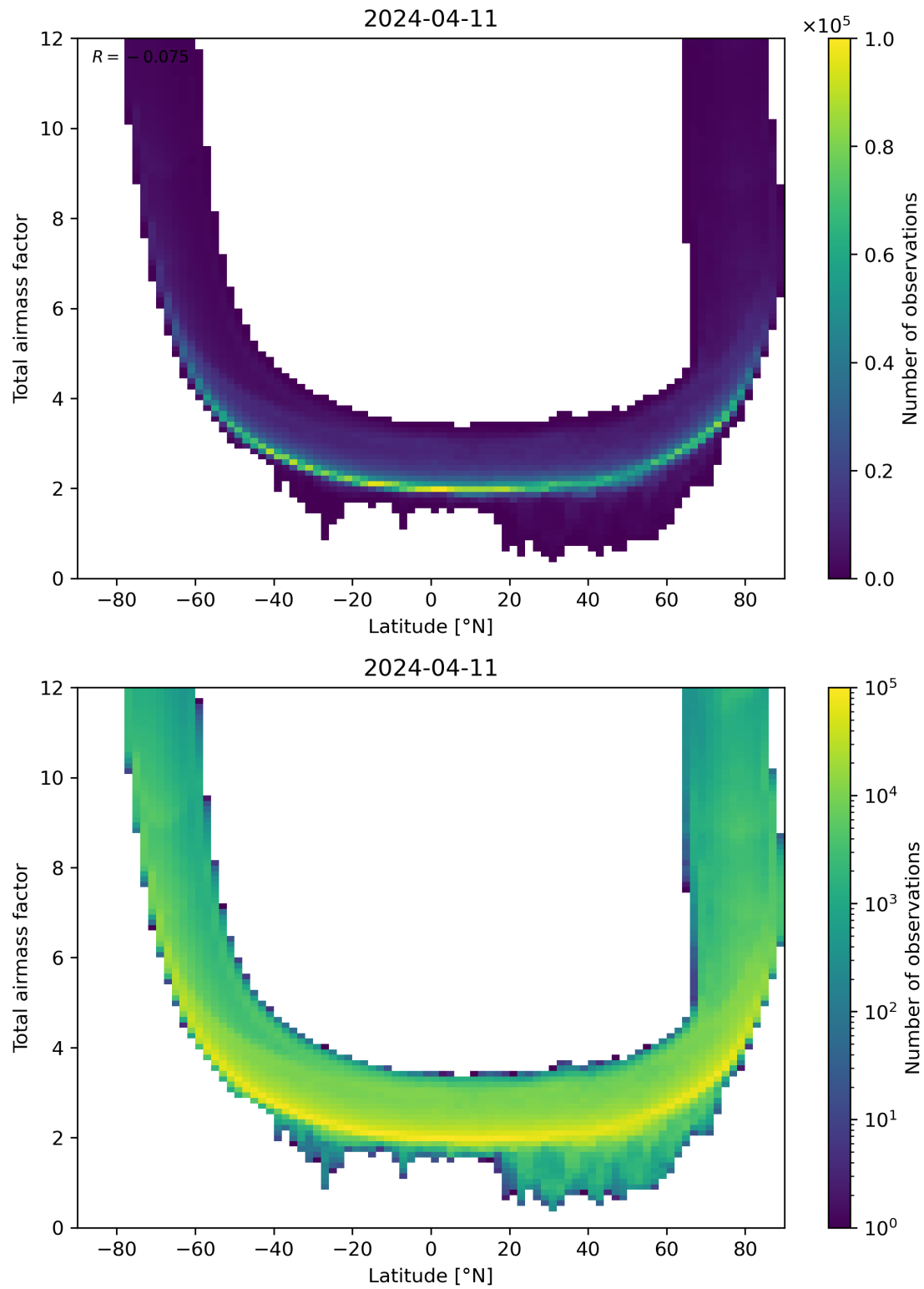
Figure 84: Scatter density plot of “Latitude” against “Total airmass factor” for 2024-04-10 to 2024-04-12.
