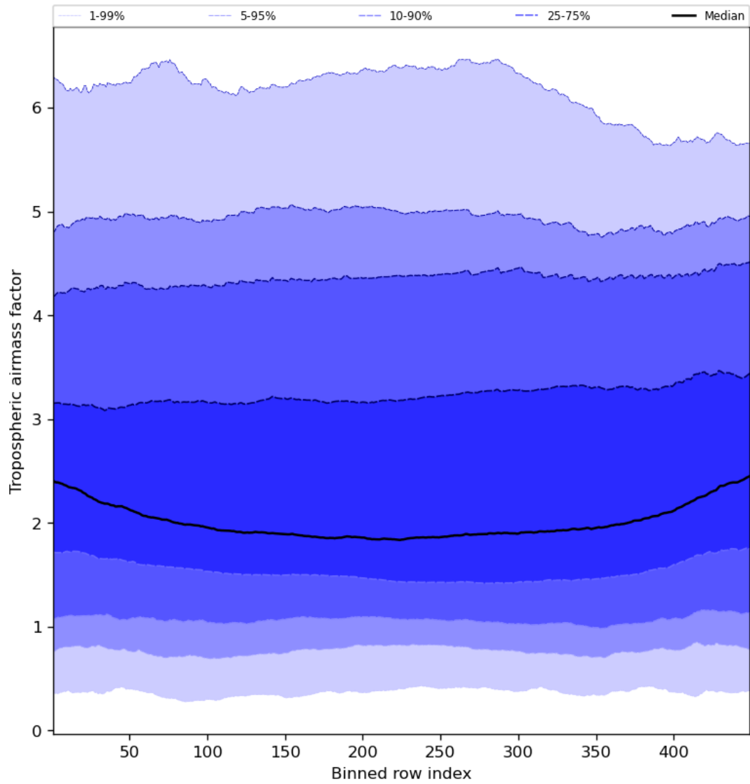
Figure 48: Along track statistics of “Tropospheric airmass factor” for 2024-04-10 to 2024-04-12
