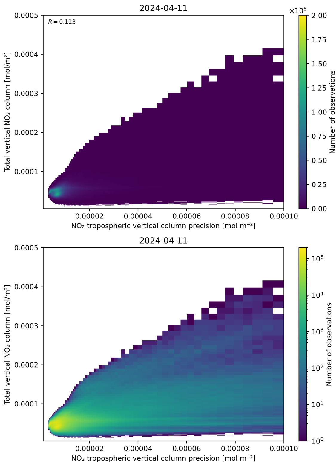
Figure 138: Scatter density plot of “NO 2 tropospheric vertical column precision” against “Total vertical NO 2 column” for 2024-04-10 to 2024-04-12.
