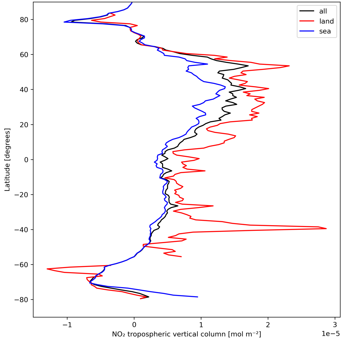
Figure 12: Zonal average of “NO 2 tropospheric vertical column” for 2024-04-11 to 2024-04-13.
