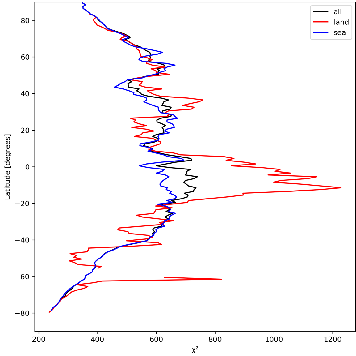
Figure 25: Zonal average of “ \chi^2 ” for 2024-04-11 to 2024-04-13.
