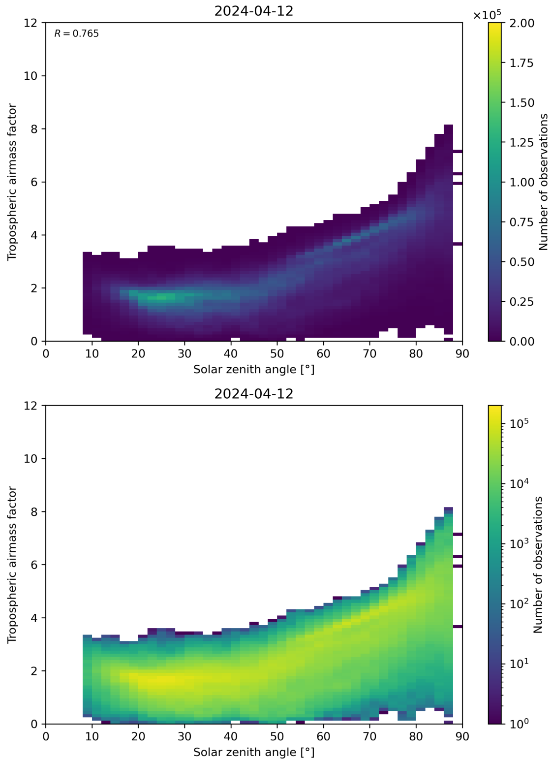
Figure 147: Scatter density plot of “Solar zenith angle” against “Tropospheric airmass factor” for 2024-04-11 to 2024-04-13.
