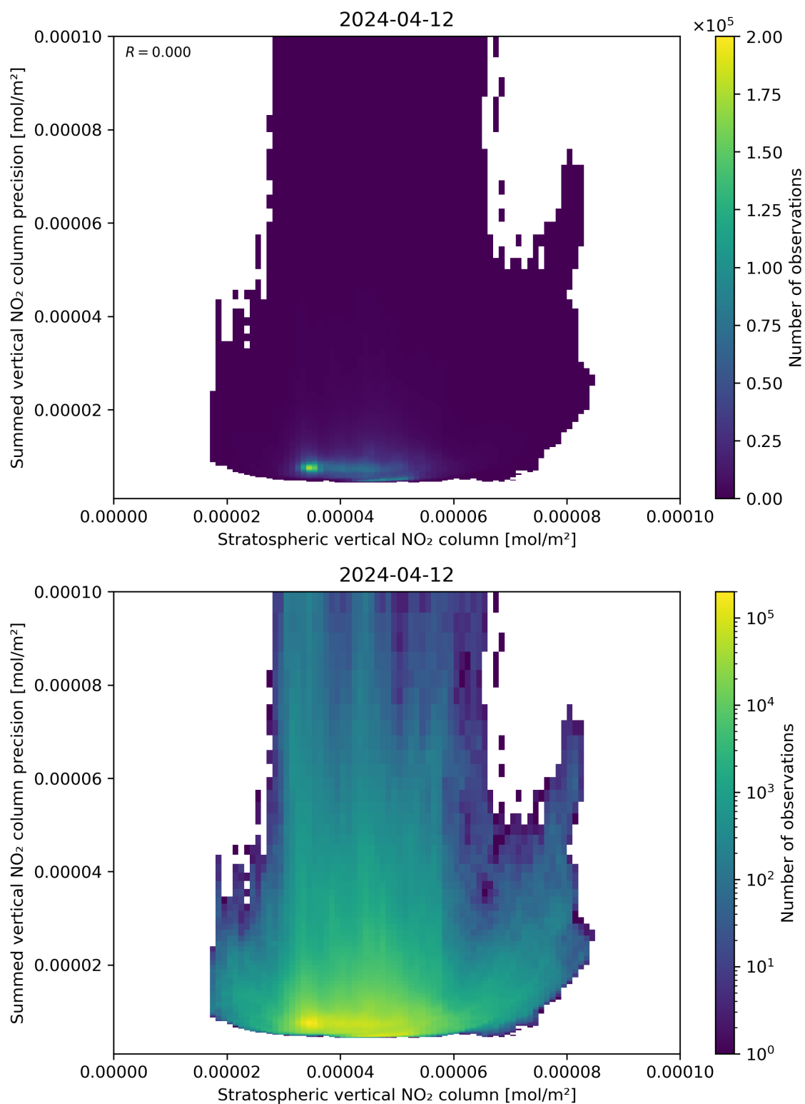
Figure 99: Scatter density plot of “Stratospheric vertical NO 2 column” against “Summed vertical NO 2 column precision” for 2024-04-11 to 2024-04-13.
