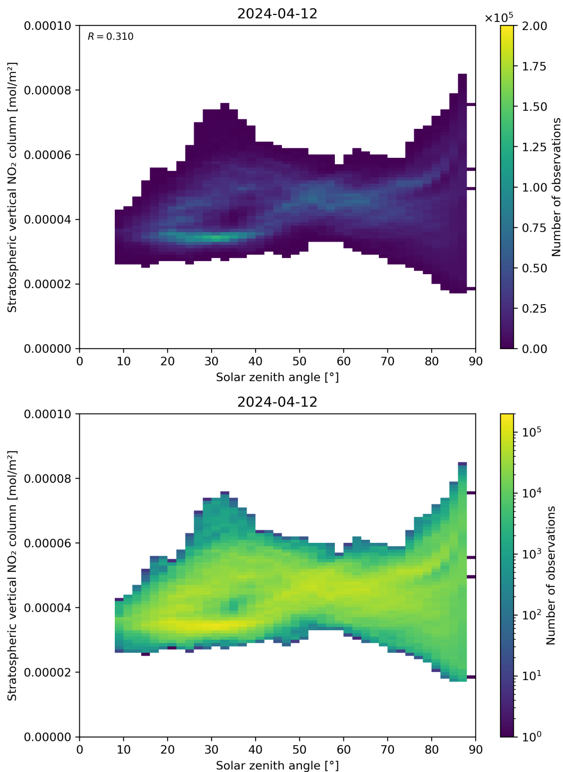
Figure 150: Scatter density plot of “Solar zenith angle” against “Stratospheric vertical NO 2 column” for 2024-04-11 to 2024-04-13.
