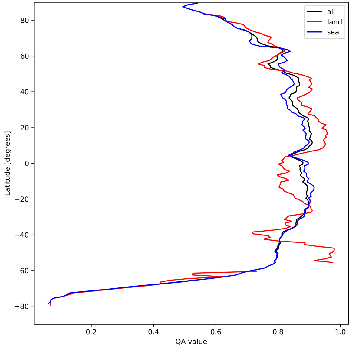
Figure 11: Zonal average of “QA value” for 2024-04-11 to 2024-04-13.
