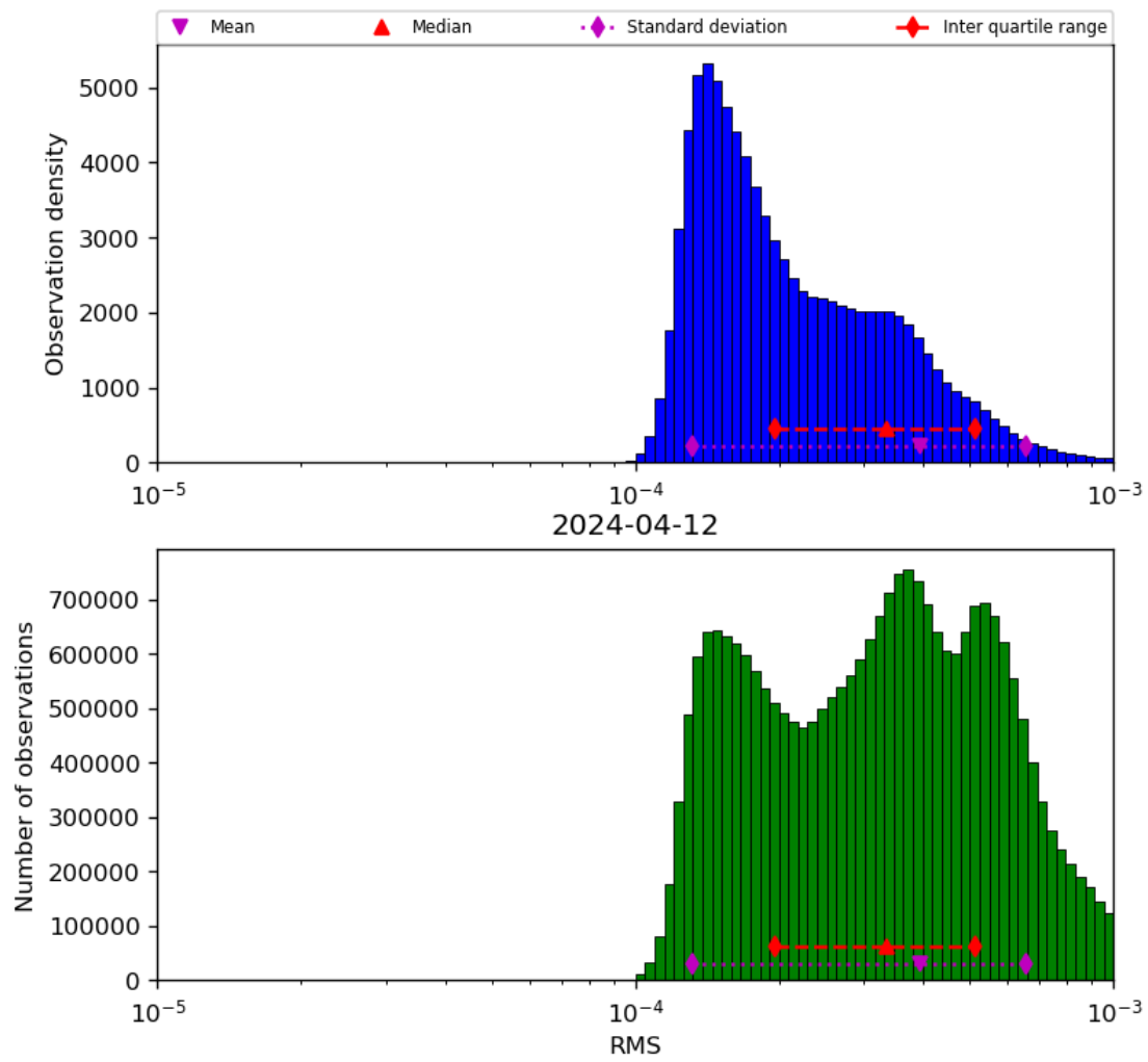
Figure 43: Histogram of “RMS” for 2024-04-11 to 2024-04-13
