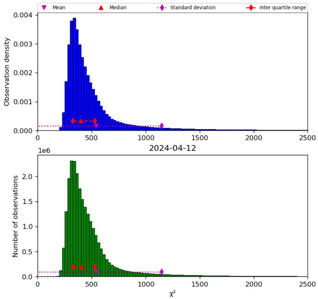
Figure 42: Histogram of “ \chi^2 ” for 2024-04-11 to 2024-04-13
