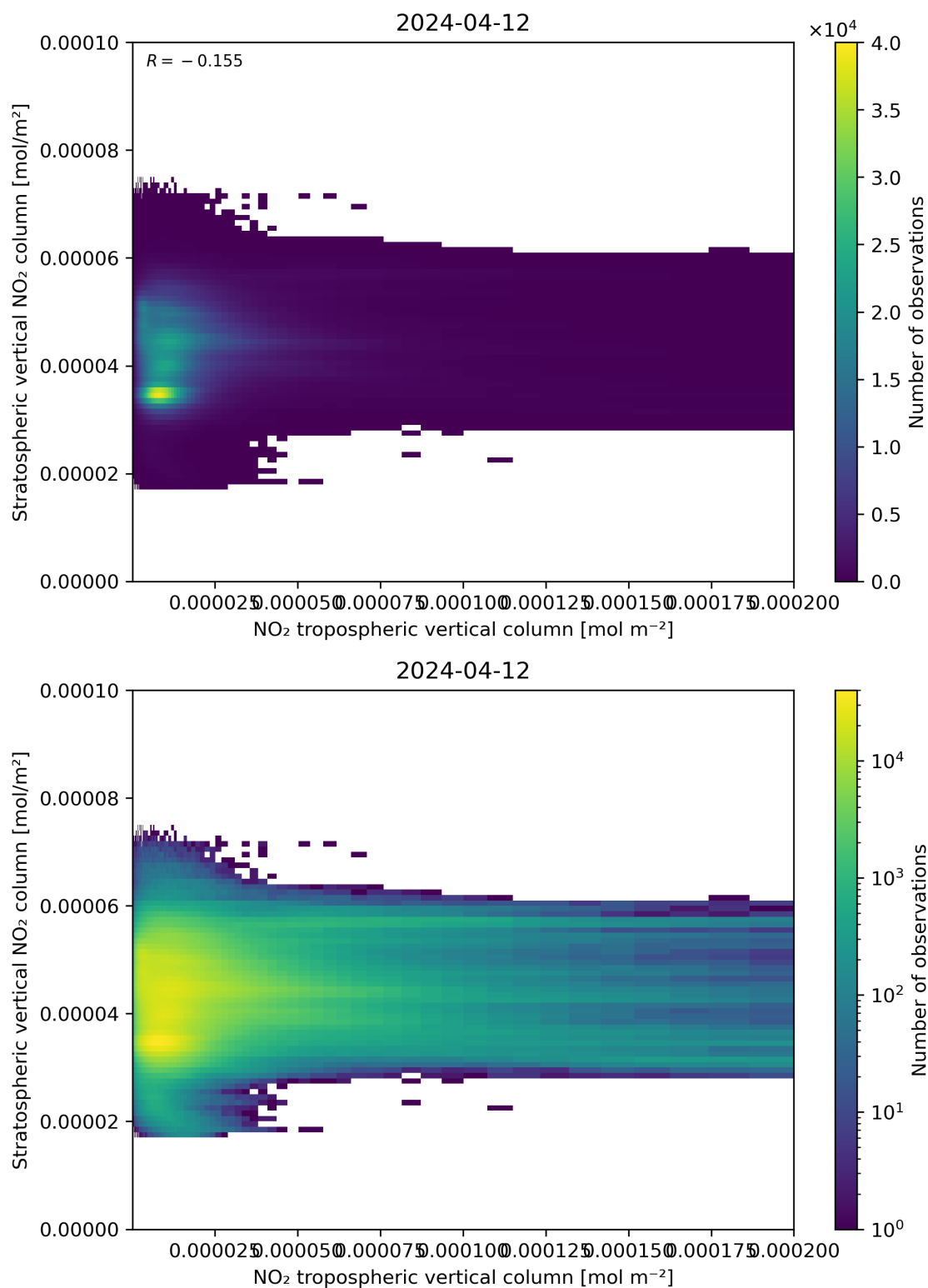
Figure 125: Scatter density plot of “NO 2 tropospheric vertical column” against “Stratospheric vertical NO 2 column” for 2024-04-11 to 2024-04-13.
