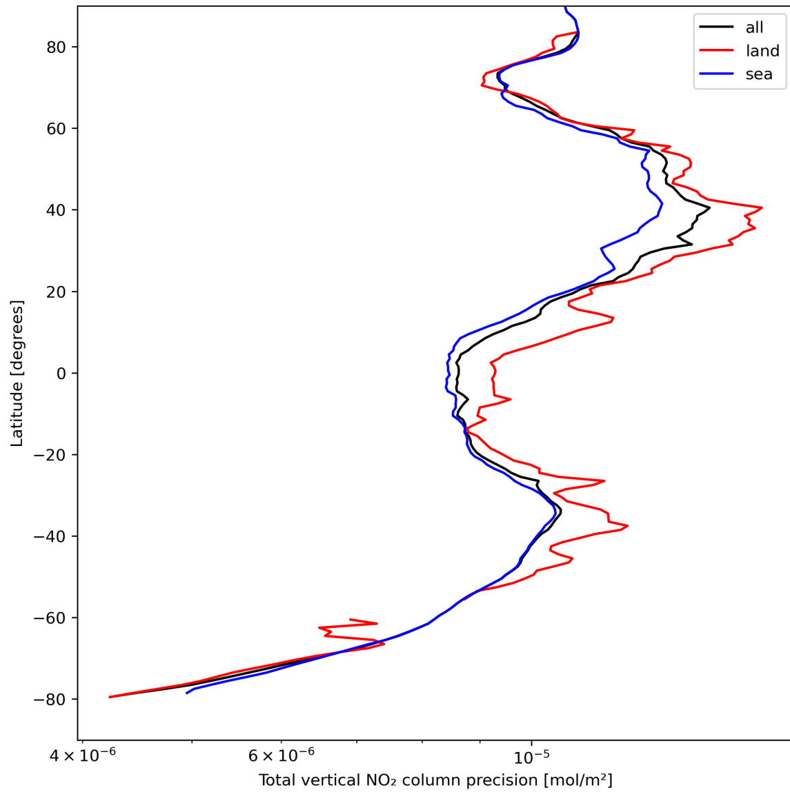
Figure 22: Zonal average of “Total vertical NO 2 column precision” for 2024-04-11 to 2024-04-13.
