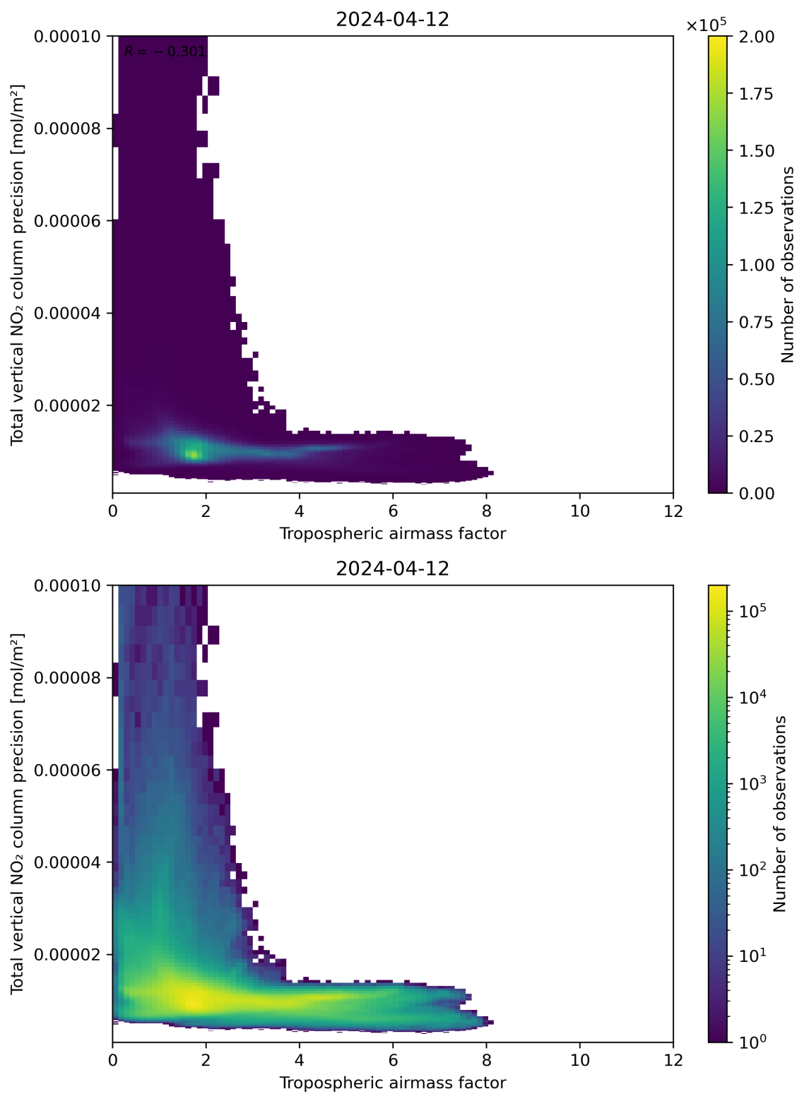
Figure 78: Scatter density plot of “Tropospheric air mass factor” against “Total vertical NO 2 column precision” for 2024-04-11 to 2024-04-13.
