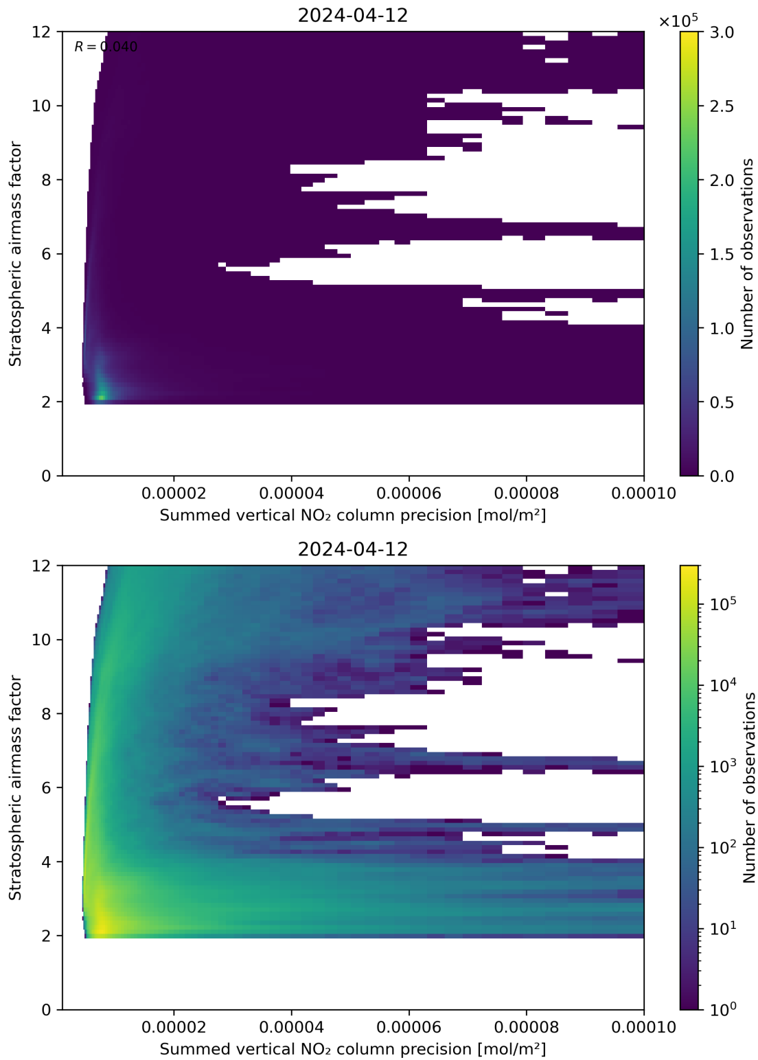
Figure 106: Scatter density plot of “Summed vertical NO 2 column precision” against “Stratospheric airmass factor” for 2024-04-11 to 2024-04-13.
