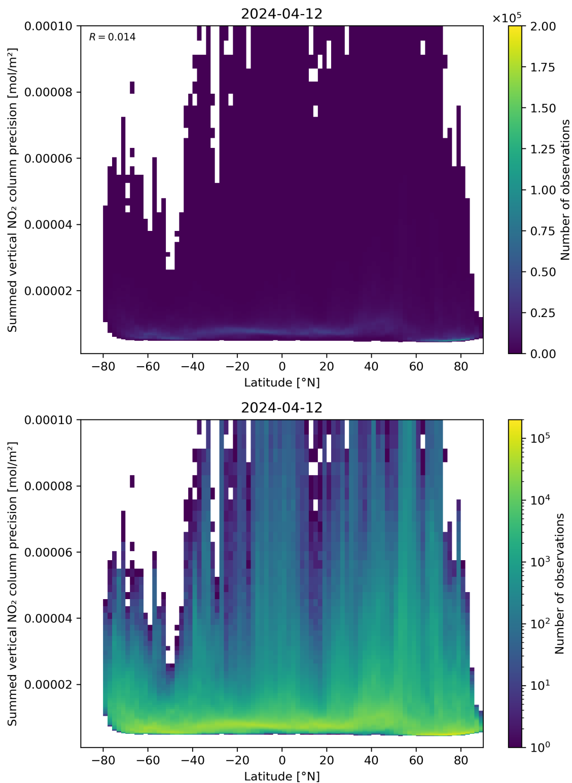
Figure 89: Scatter density plot of “Latitude” against “Summed vertical NO 2 column precision” for 2024-04-11 to 2024-04-13.
