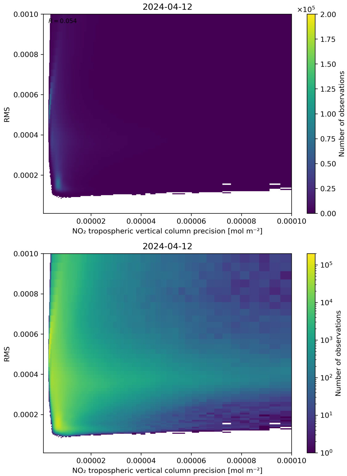
Figure 140: Scatter density plot of “NO 2 tropospheric vertical column precision” against “RMS” for 2024-04-11 to 2024-04-13.
