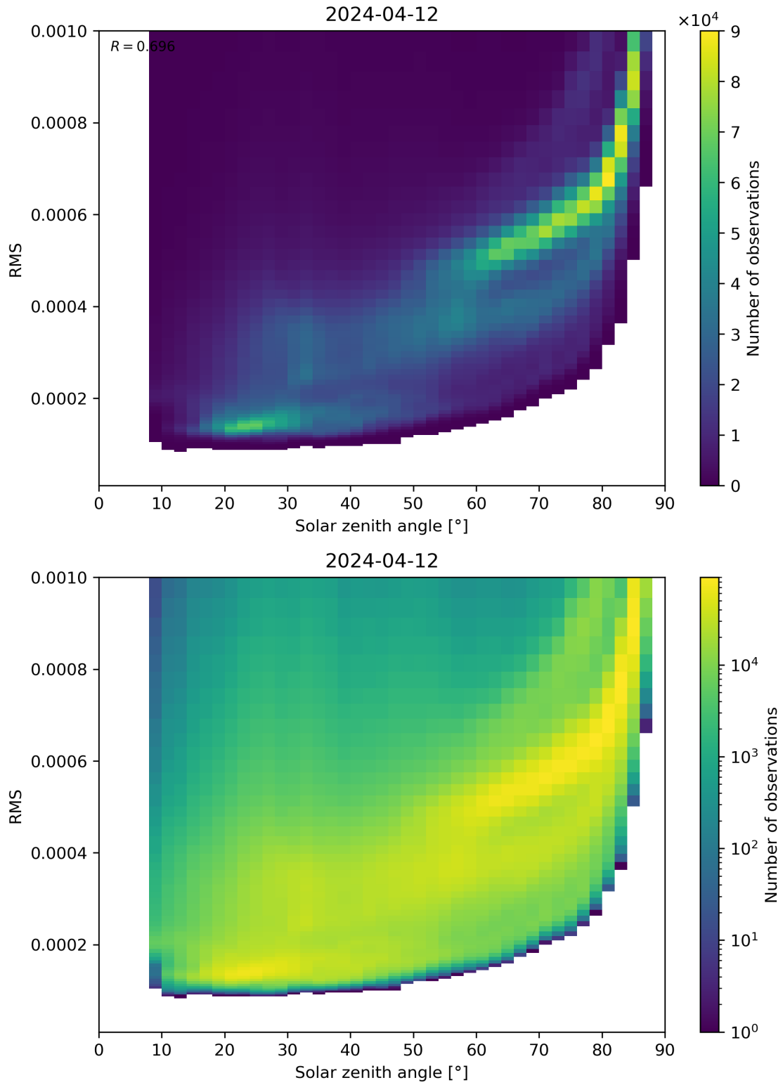
Figure 157: Scatter density plot of “Solar zenith angle” against “RMS” for 2024-04-11 to 2024-04-13.
