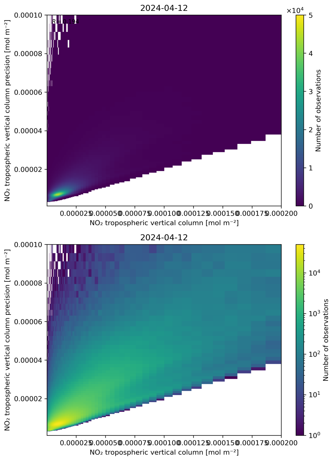
Figure 130: Scatter density plot of “NO 2 tropospheric vertical column” against “NO 2 tropospheric vertical column precision” for 2024-04-11 to 2024-04-13.
