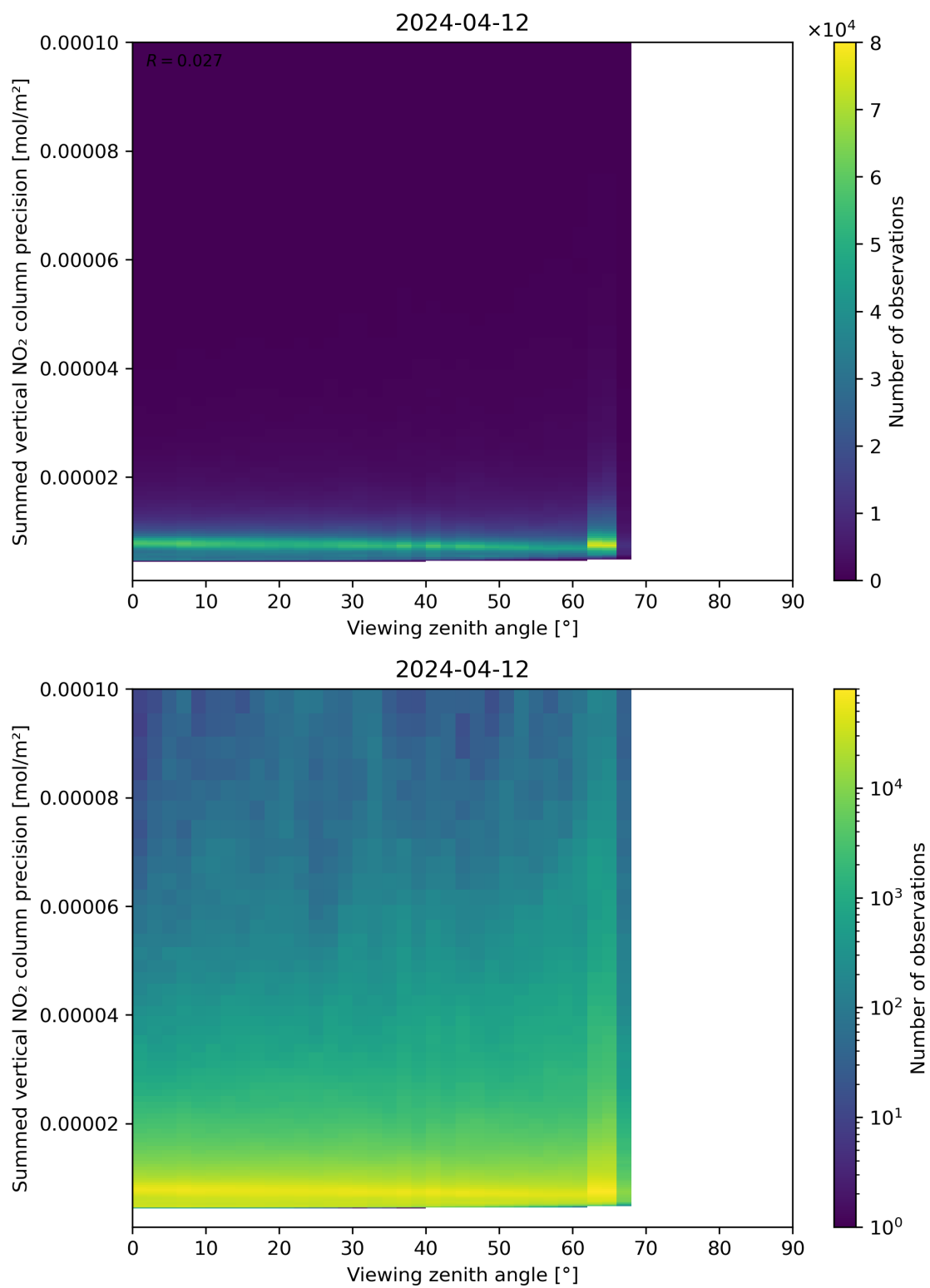
Figure 166: Scatter density plot of “Viewing zenith angle” against “Summed vertical NO 2 column precision” for 2024-04-11 to 2024-04-13.
