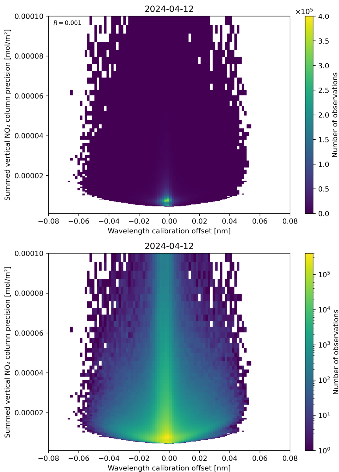
Figure 178: Scatter density plot of “Wavelength calibration offset” against “Summed vertical NO 2 column precision” for 2024-04-11 to 2024-04-13.
