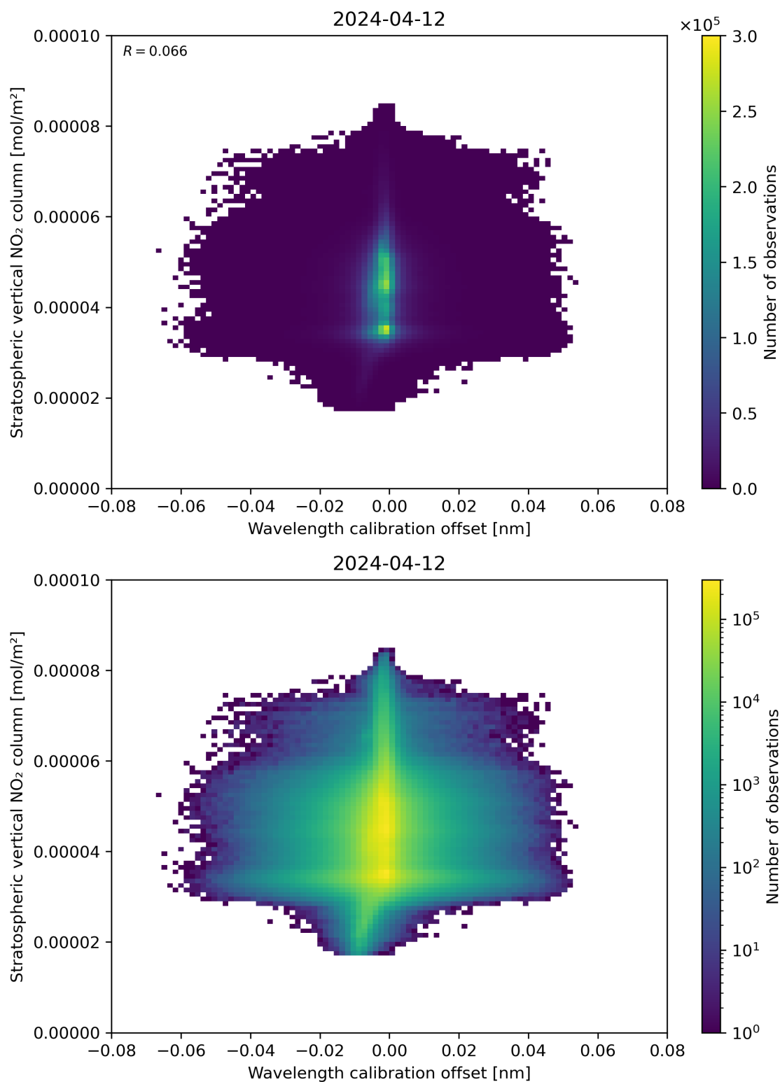
Figure 176: Scatter density plot of “Wavelength calibration offset” against “Stratospheric vertical NO 2 column” for 2024-04-11 to 2024-04-13.
