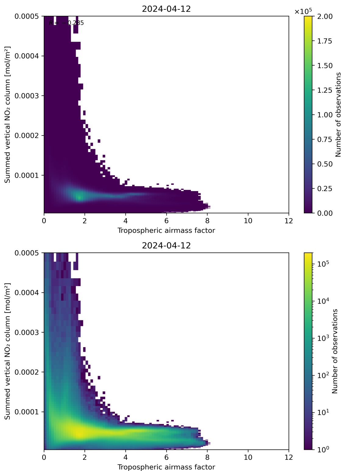
Figure 75: Scatter density plot of “Tropospheric air mass factor” against “Summed vertical NO 2 column” for 2024-04-11 to 2024-04-13.
