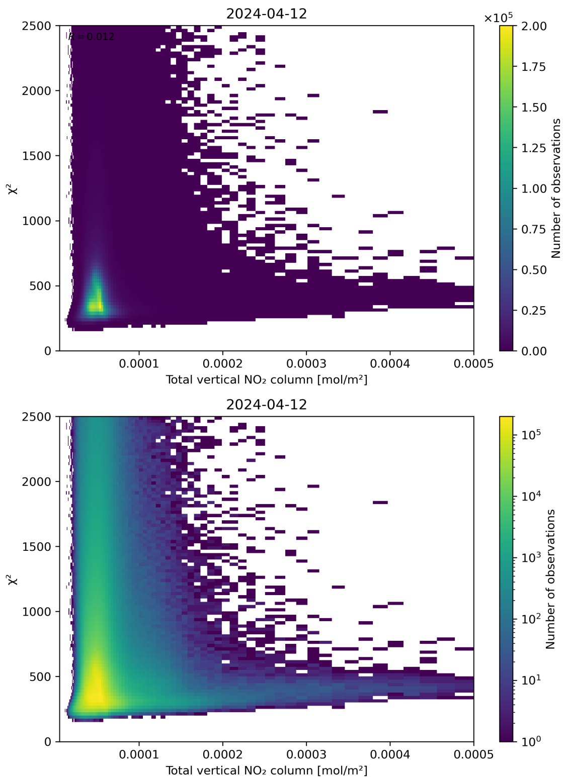
Figure 111: Scatter density plot of “Total vertical NO 2 column” against “ \chi^2 ” for 2024-04-11 to 2024-04-13.
