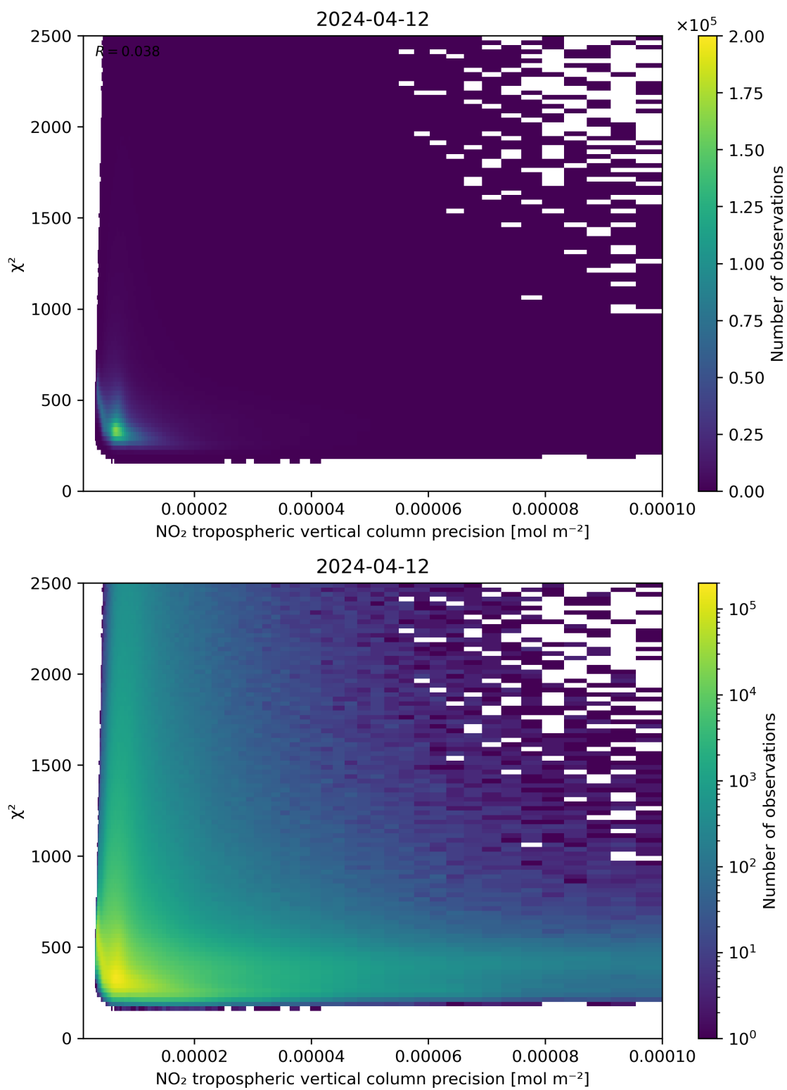
Figure 134: Scatter density plot of “NO 2 tropospheric vertical column precision” against “ \chi^2 ” for 2024-04-11 to 2024-04-13.
