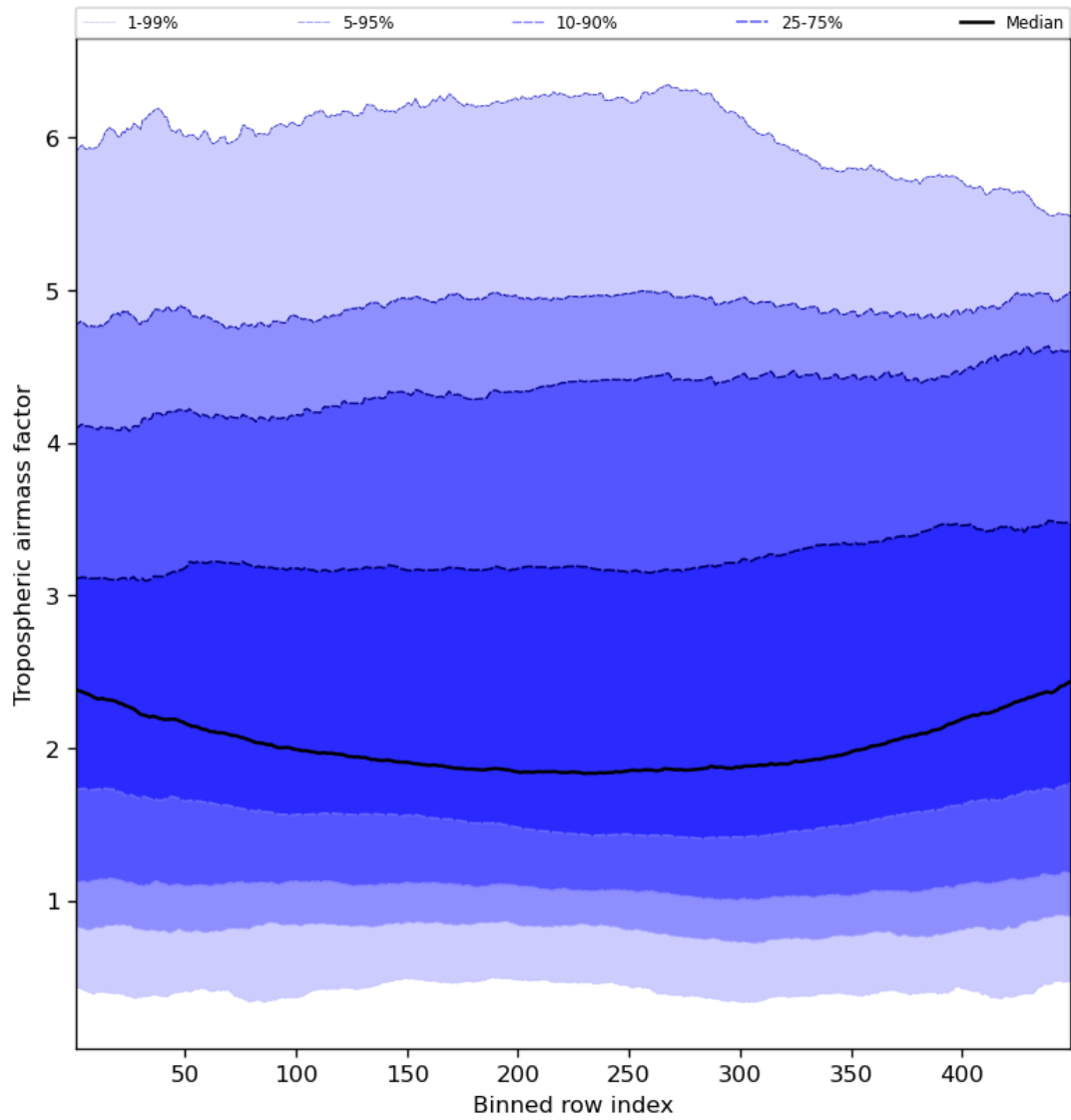
Figure 48: Along track statistics of “Tropospheric air mass factor” for 2024-04-11 to 2024-04-13
