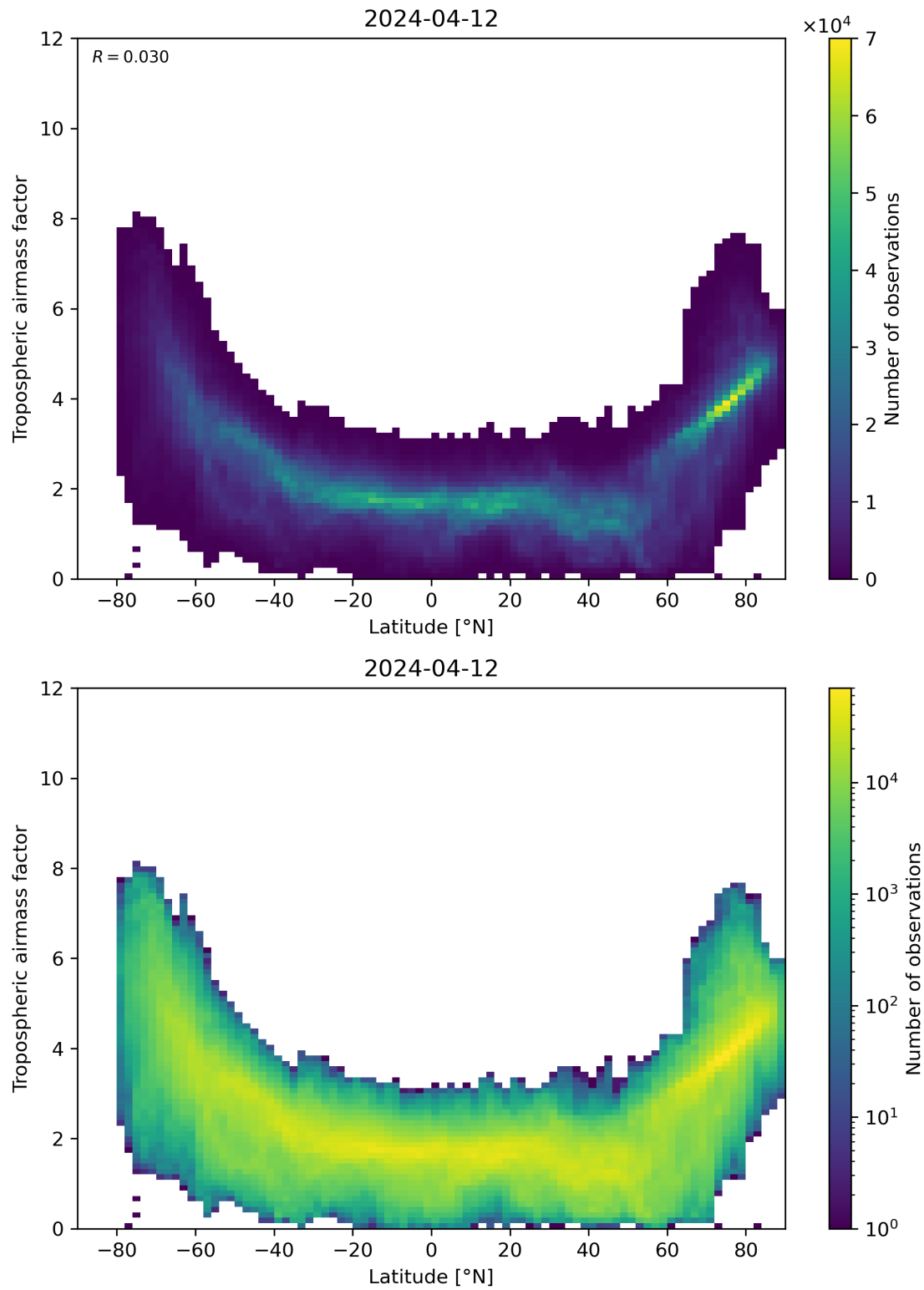
Figure 85: Scatter density plot of “Latitude” against “Tropospheric air mass factor” for 2024-04-11 to 2024-04-13.
