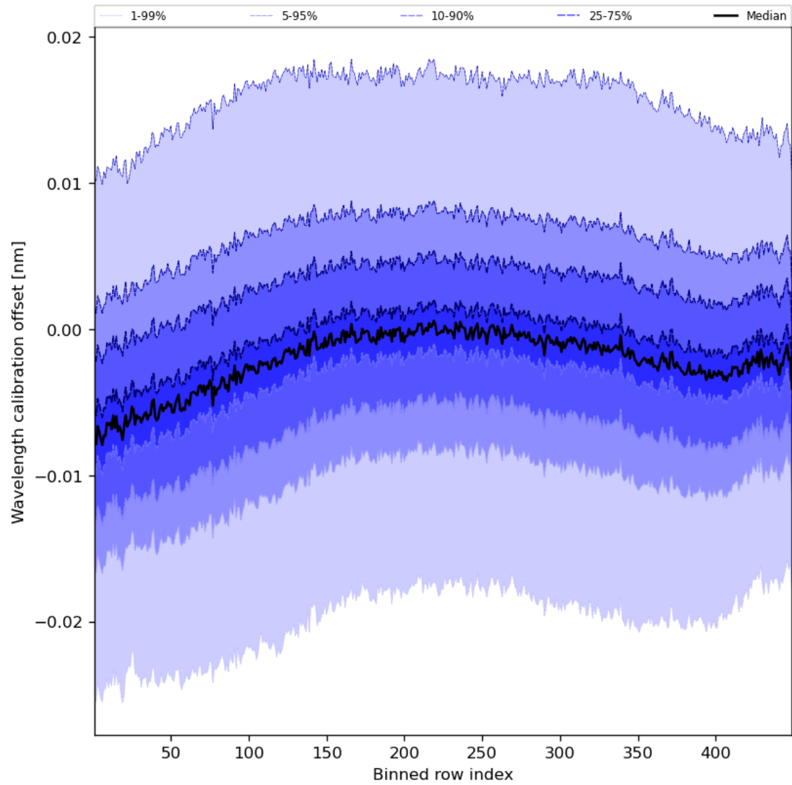
Figure 52: Along track statistics of “Wavelength calibration offset” for 2024-04-11 to 2024-04-13
