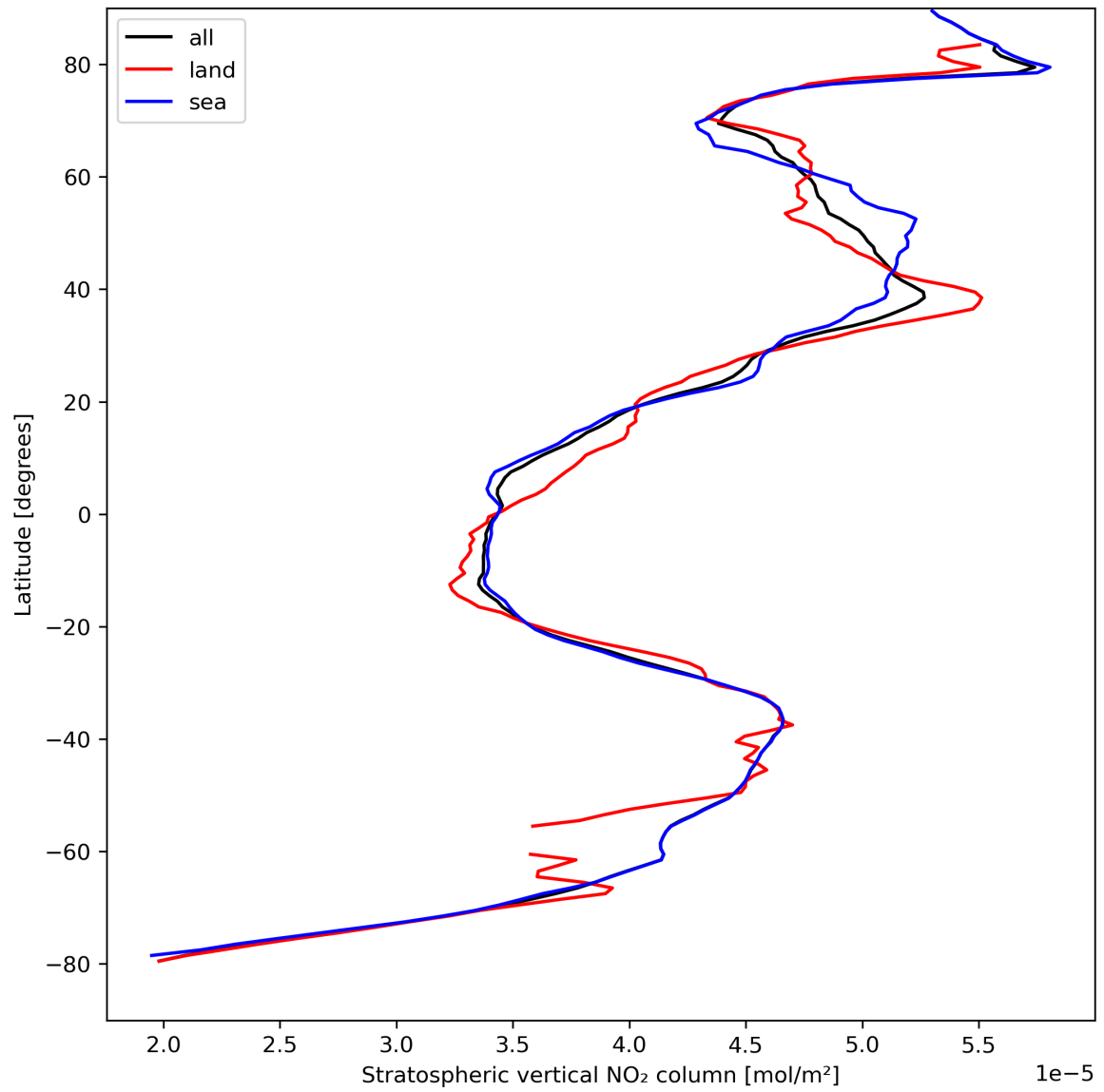
Figure 19: Zonal average of “Stratospheric vertical NO 2 column” for 2024-04-11 to 2024-04-13.
