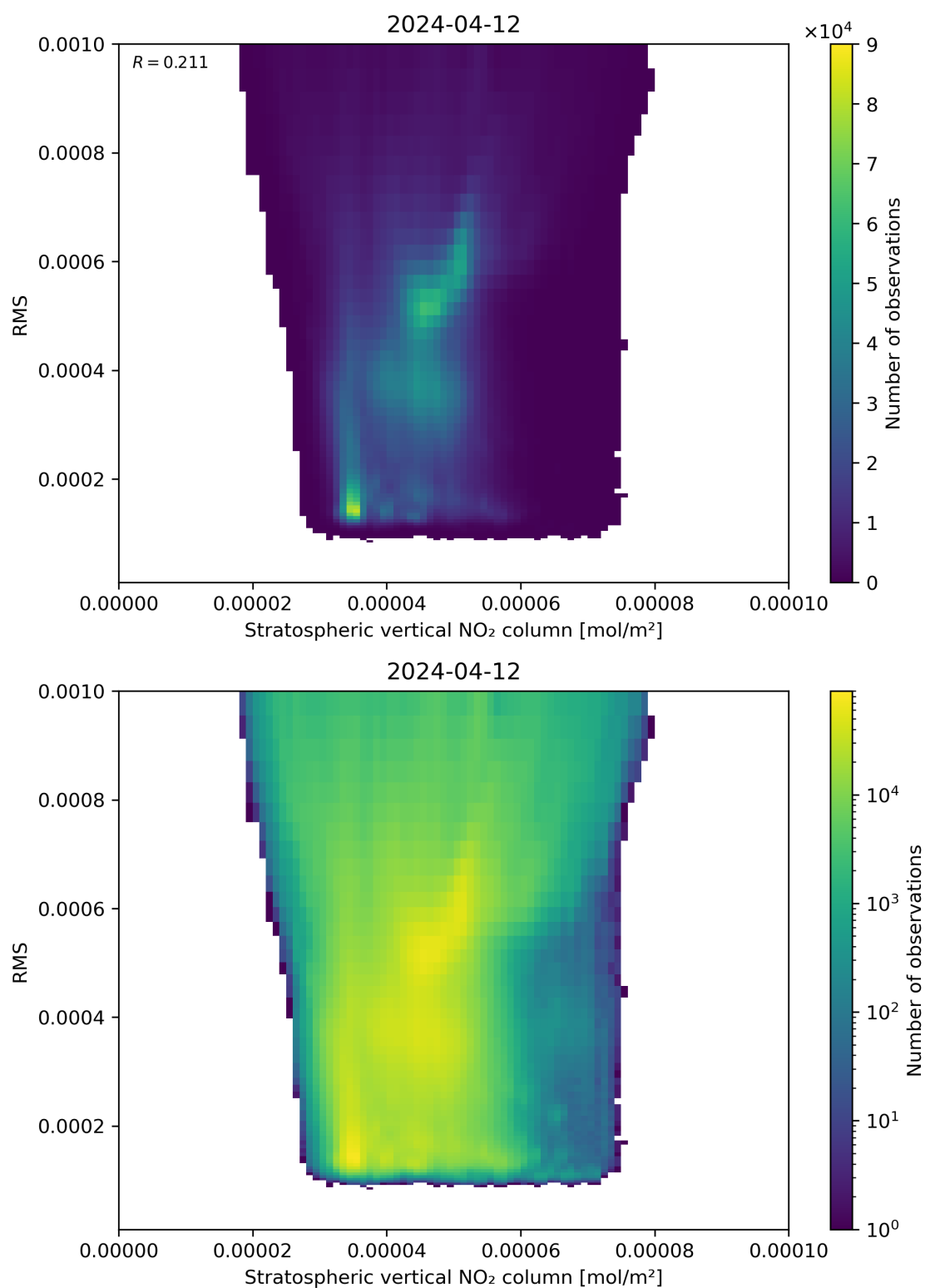
Figure 102: Scatter density plot of “Stratospheric vertical NO 2 column” against “RMS” for 2024-04-11 to 2024-04-13.
