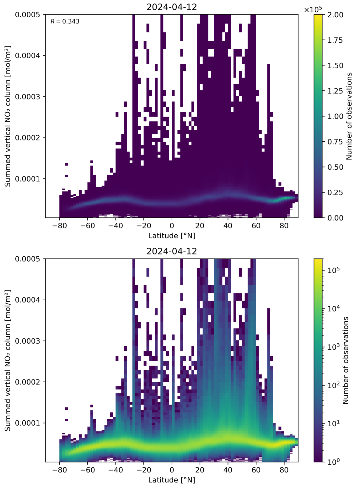
Figure 88: Scatter density plot of “Latitude” against “Summed vertical NO 2 column” for 2024-04-11 to 2024-04-13.
