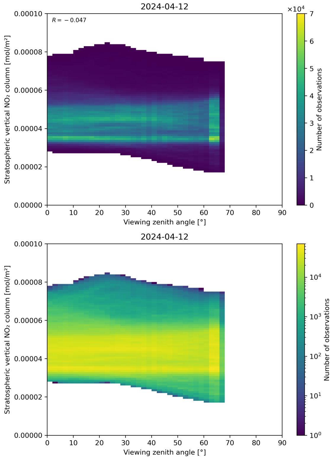
Figure 164: Scatter density plot of “Viewing zenith angle” against “Stratospheric vertical NO 2 column” for 2024-04-11 to 2024-04-13.
