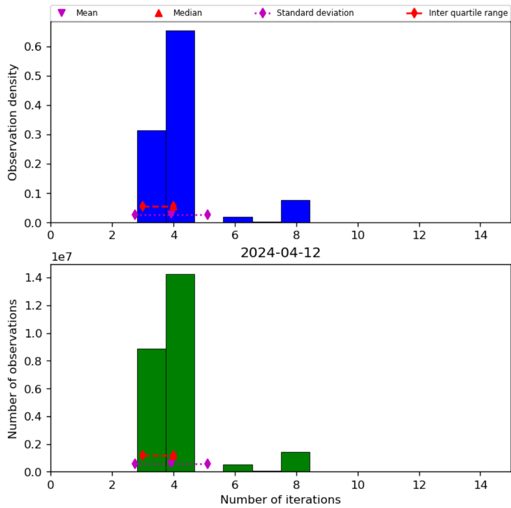
Figure 34: Histogram of “Number of iterations” for 2024-04-11 to 2024-04-13
