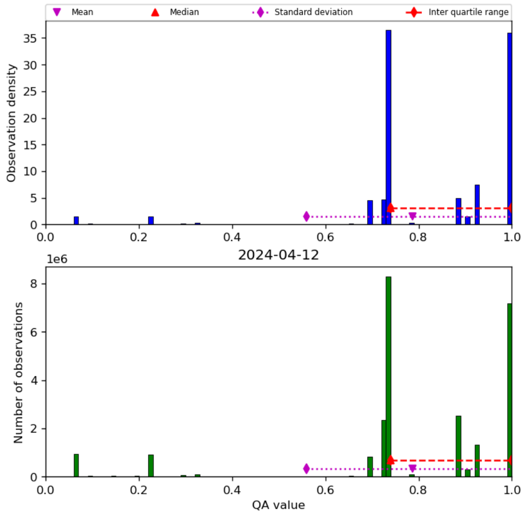
Figure 28: Histogram of “QA value” for 2024-04-11 to 2024-04-13
