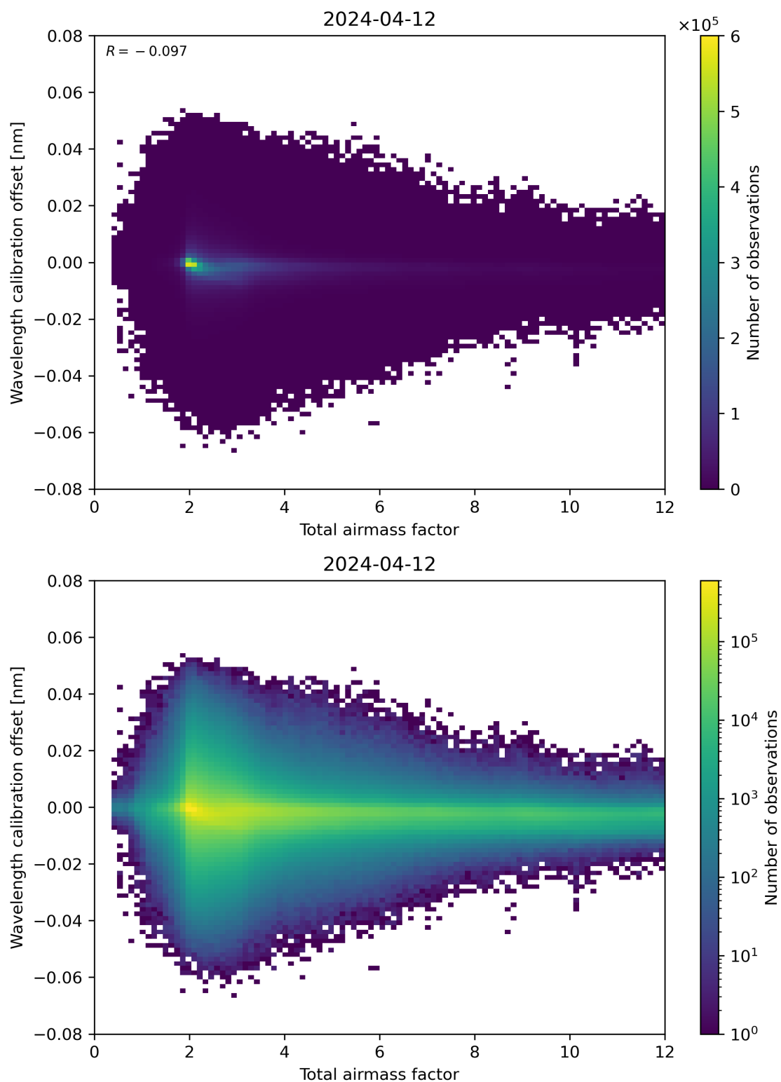
Figure 70: Scatter density plot of “Total airmass factor” against “Wavelength calibration offset” for 2024-04-11 to 2024-04-13.
