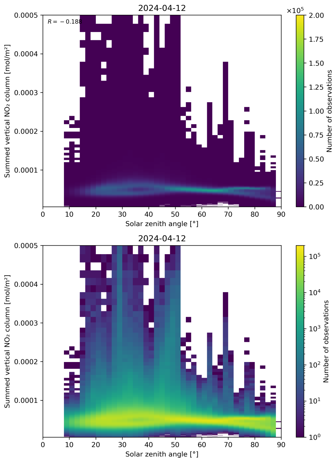
Figure 151: Scatter density plot of “Solar zenith angle” against “Summed vertical NO 2 column” for 2024-04-11 to 2024-04-13.
