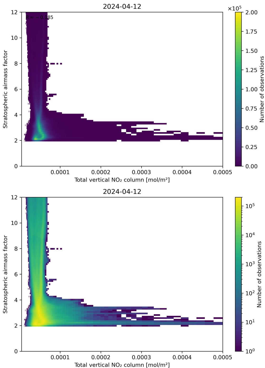
Figure 110: Scatter density plot of “Total vertical NO 2 column” against “Stratospheric airmass factor” for 2024-04-11 to 2024-04-13.
