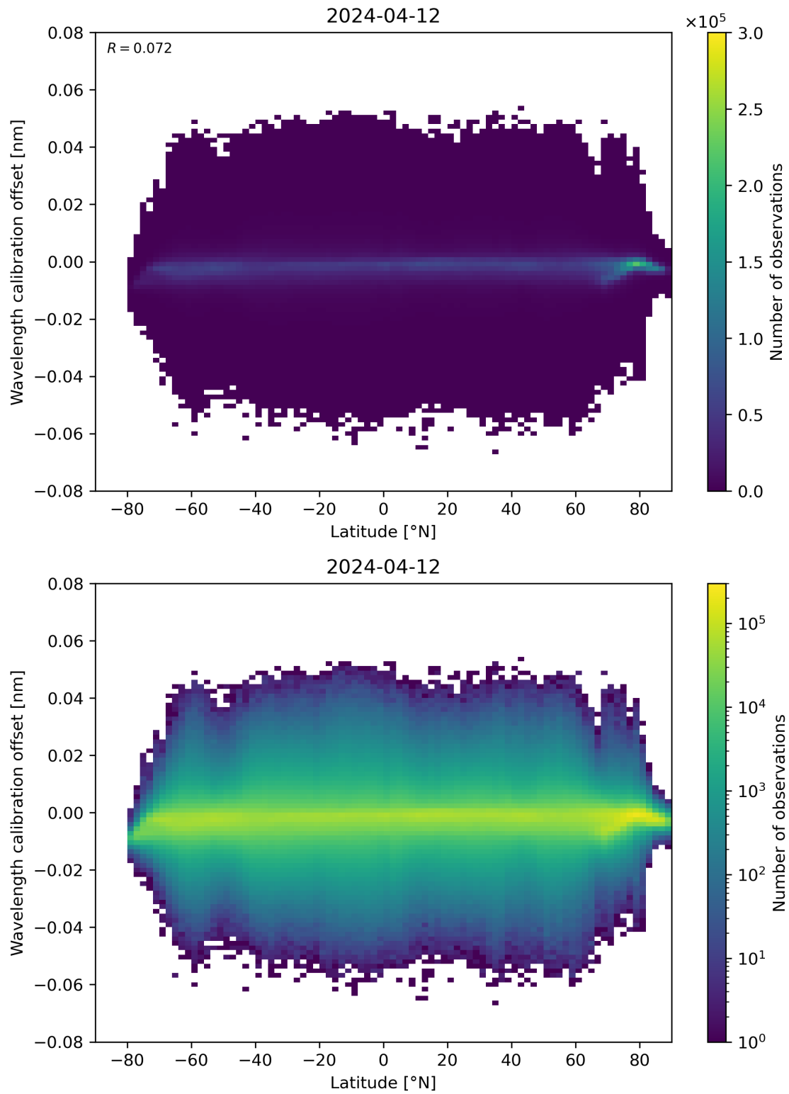
Figure 95: Scatter density plot of “Latitude” against “Wavelength calibration offset” for 2024-04-11 to 2024-04-13.
