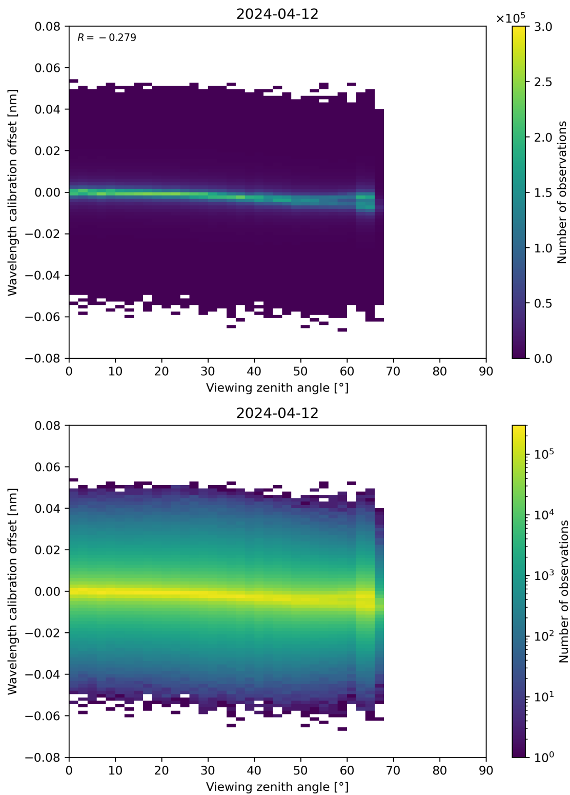
Figure 173: Scatter density plot of “Viewing zenith angle” against “Wavelength calibration offset” for 2024-04-11 to 2024-04-13.
