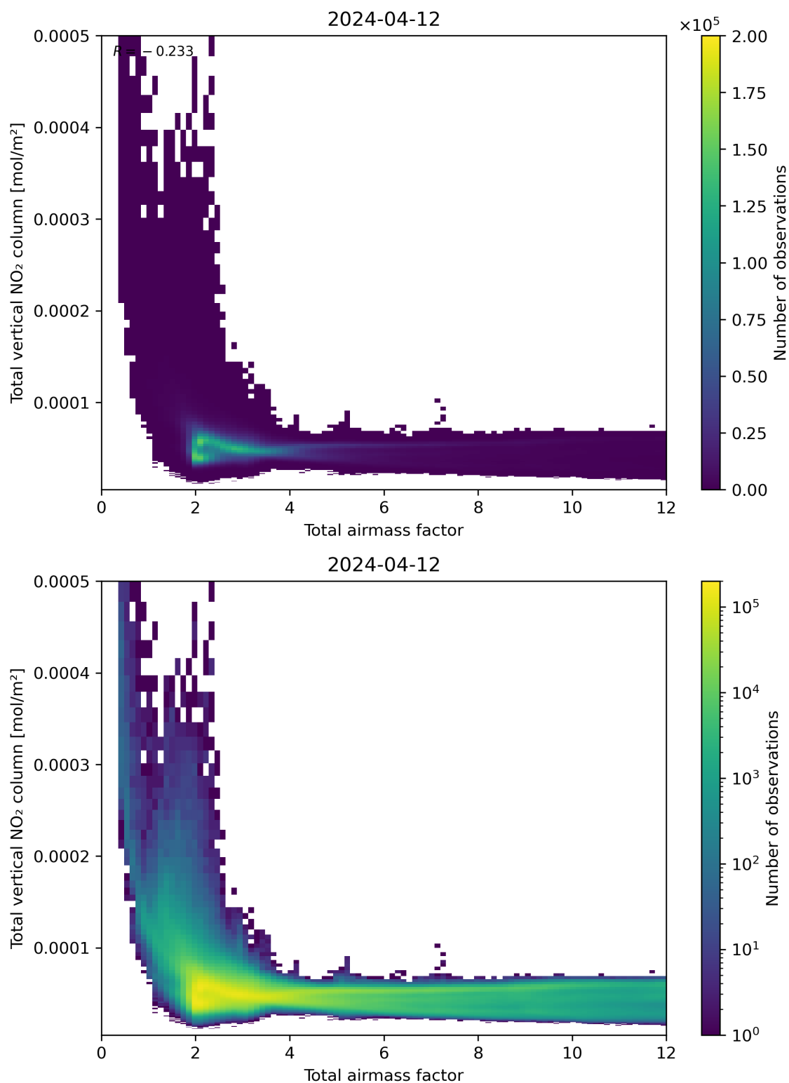
Figure 67: Scatter density plot of “Total airmass factor” against “Total vertical NO 2 column” for 2024-04-11 to 2024-04-13.
