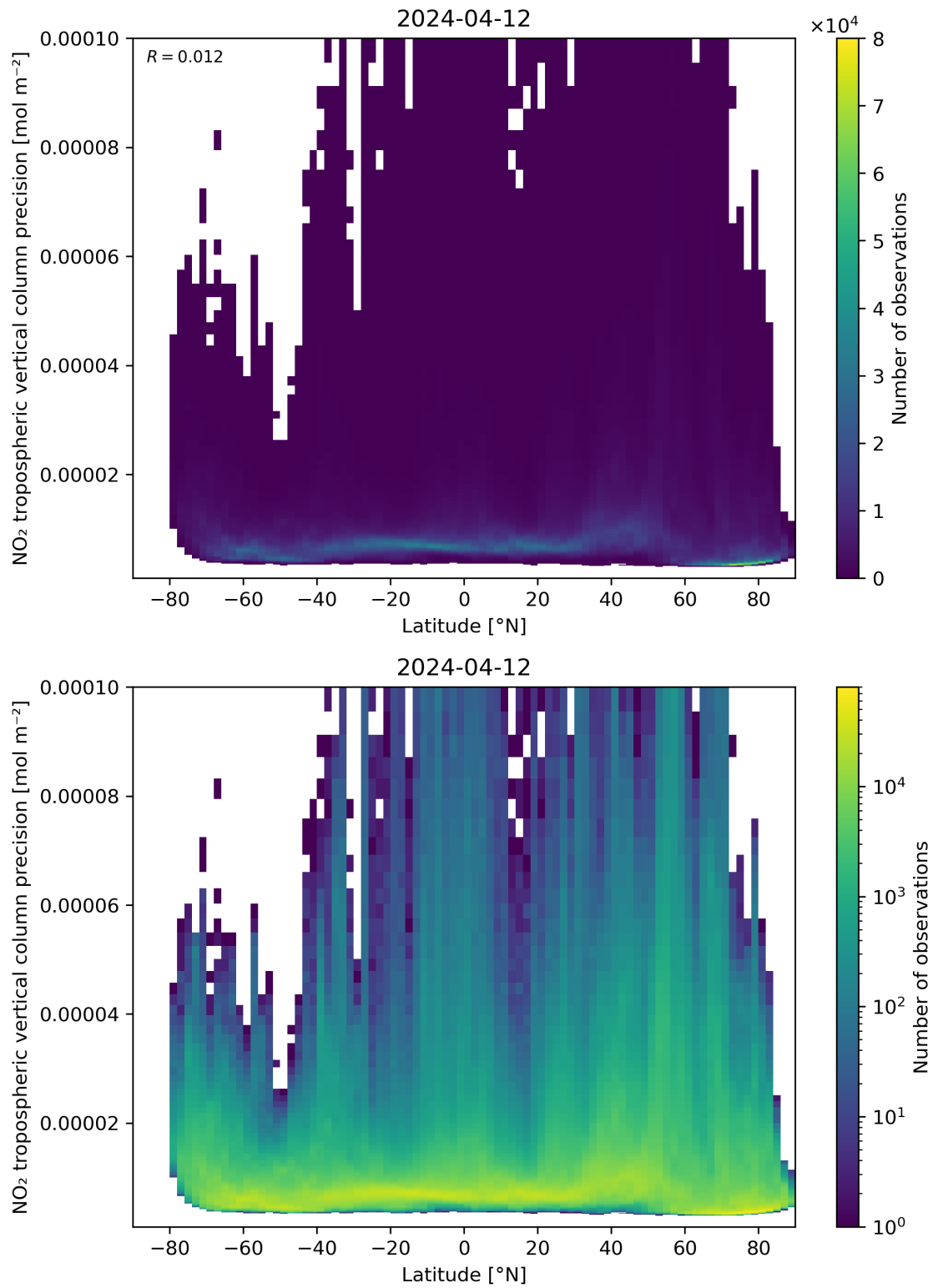
Figure 93: Scatter density plot of “Latitude” against “NO 2 tropospheric vertical column precision” for 2024-04-11 to 2024-04-13.
