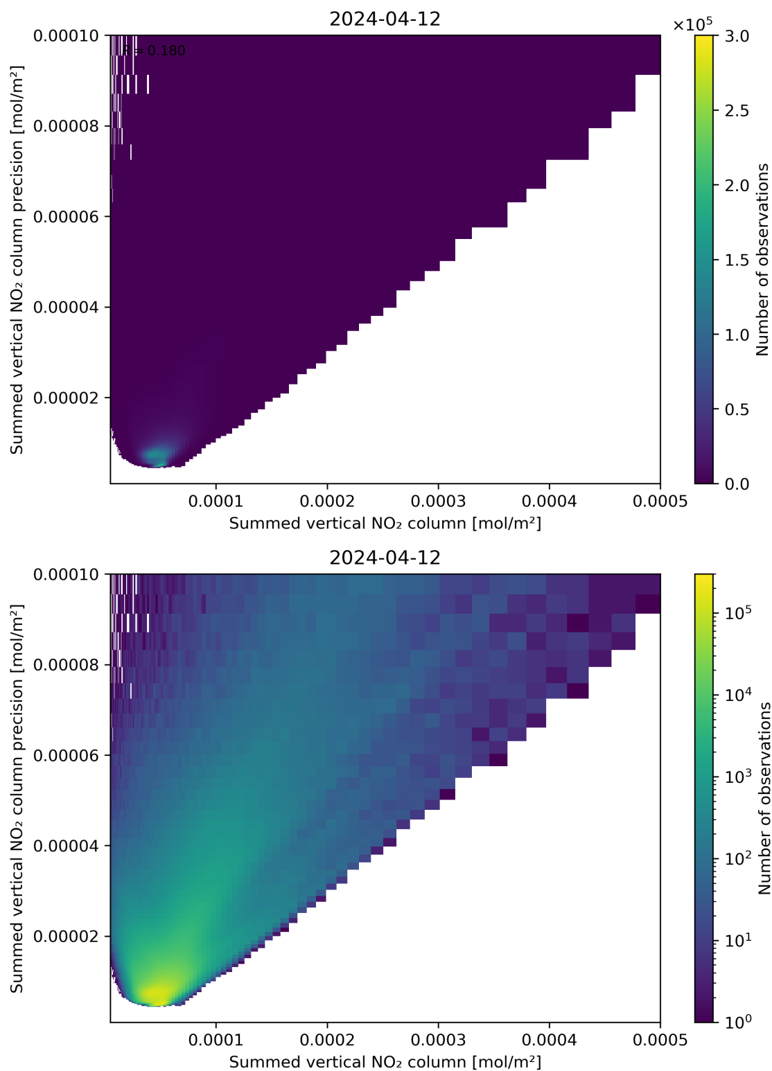
Figure 105: Scatter density plot of “Summed vertical NO 2 column” against “Summed vertical NO 2 column precision” for 2024-04-11 to 2024-04-13.
