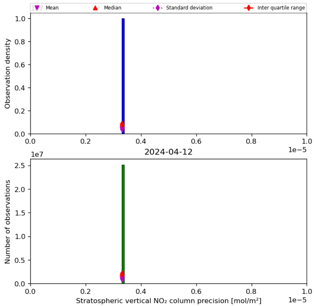
Figure 37: Histogram of “Stratospheric vertical NO 2 column precision” for 2024-04-11 to 2024-04-13
