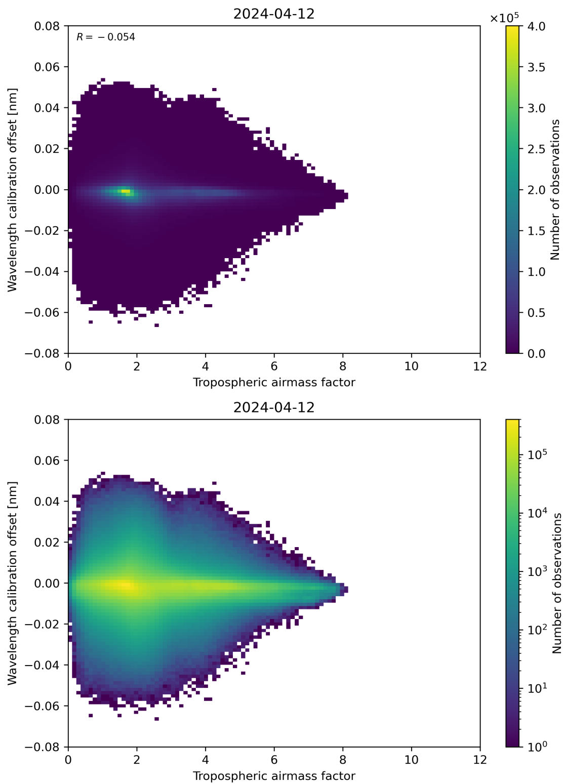
Figure 80: Scatter density plot of “Tropospheric airmass factor” against “Wavelength calibration offset” for 2024-04-11 to 2024-04-13.
