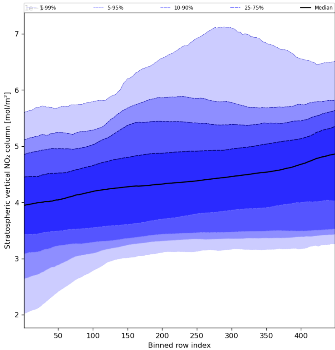
Figure 53: Along track statistics of “Stratospheric vertical NO 2 column” for 2024-04-11 to 2024-04-13
