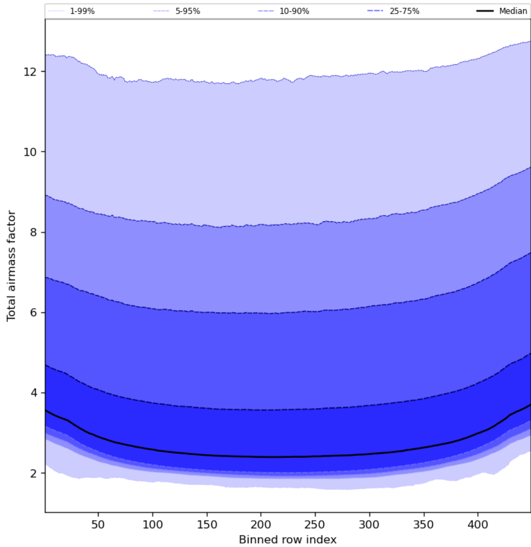
Figure 49: Along track statistics of “Total airmass factor” for 2024-04-11 to 2024-04-13
