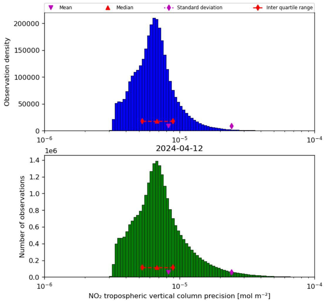
Figure 30: Histogram of “NO 2 tropospheric vertical column precision” for 2024-04-11 to 2024-04-13
