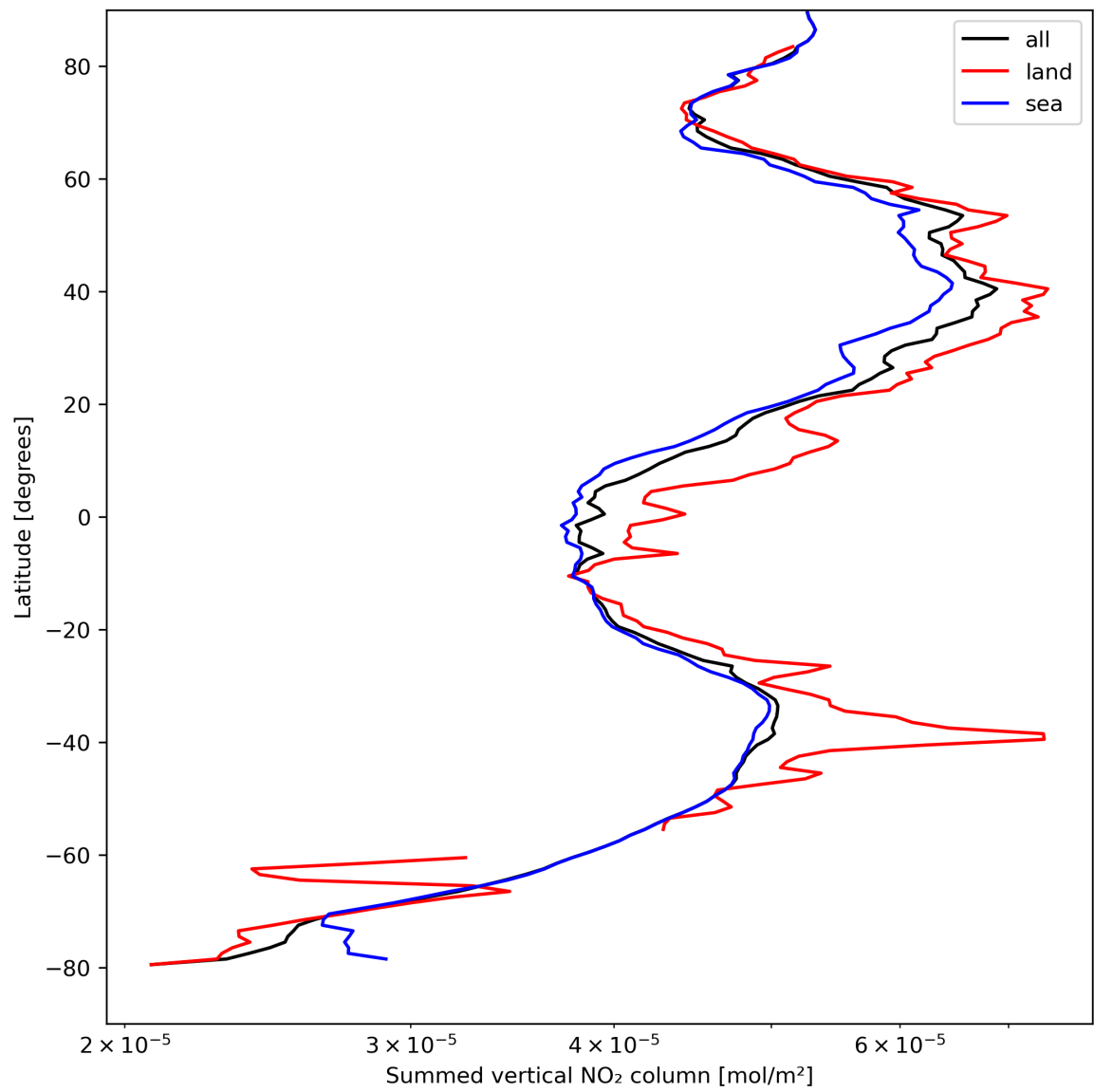
Figure 23: Zonal average of “Summed vertical NO 2 column” for 2024-04-11 to 2024-04-13.
