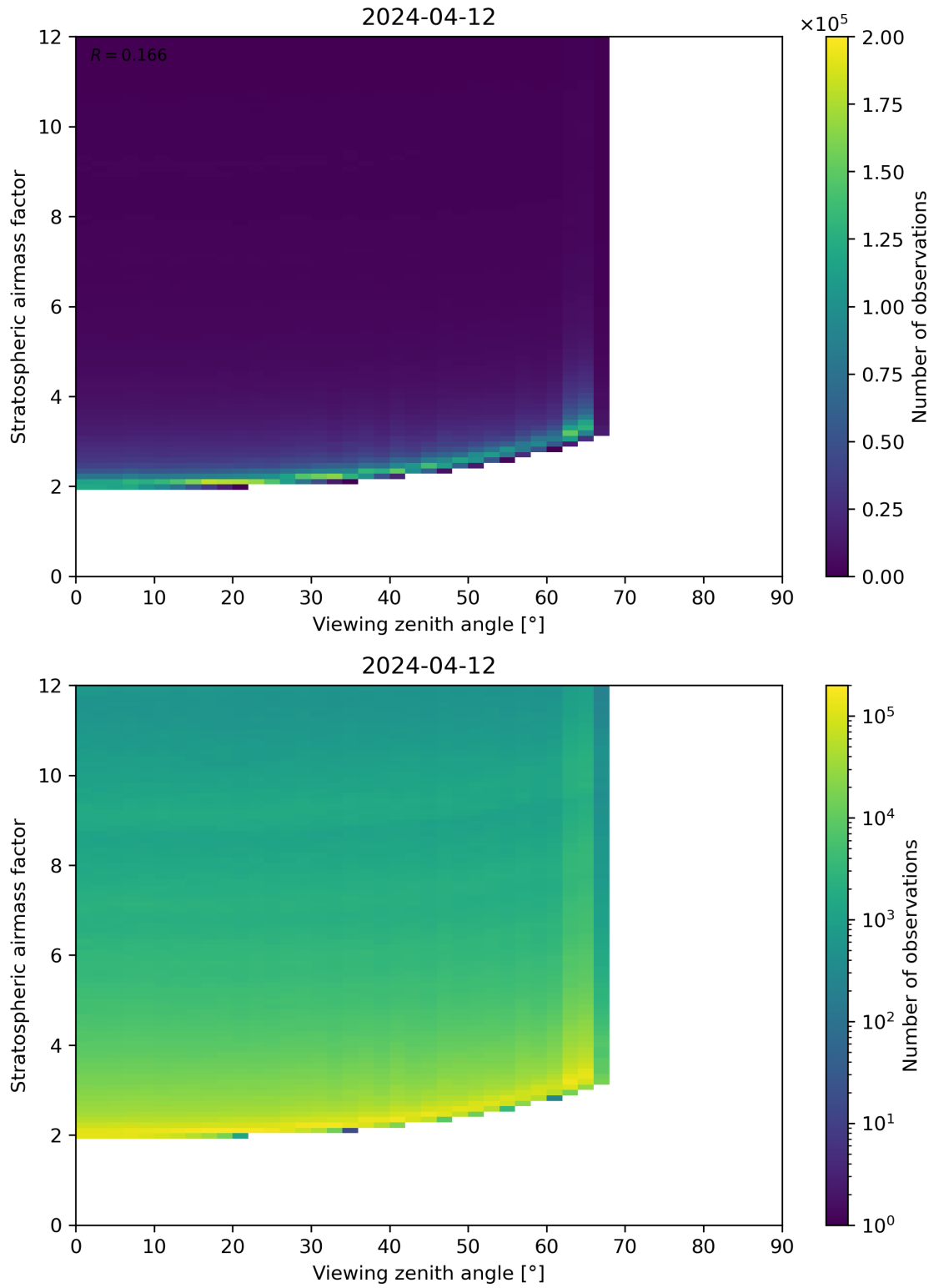
Figure 159: Scatter density plot of “Viewing zenith angle” against “Stratospheric airmass factor” for 2024-04-11 to 2024-04-13.
