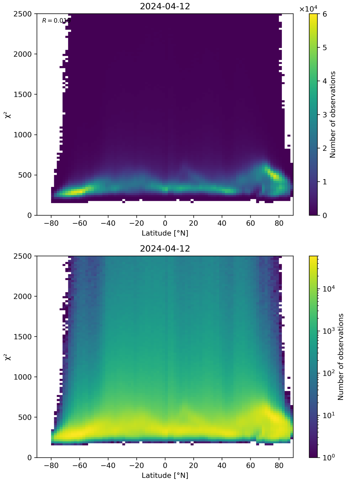
Figure 86: Scatter density plot of “Latitude” against “ \chi^2 ” for 2024-04-11 to 2024-04-13.
