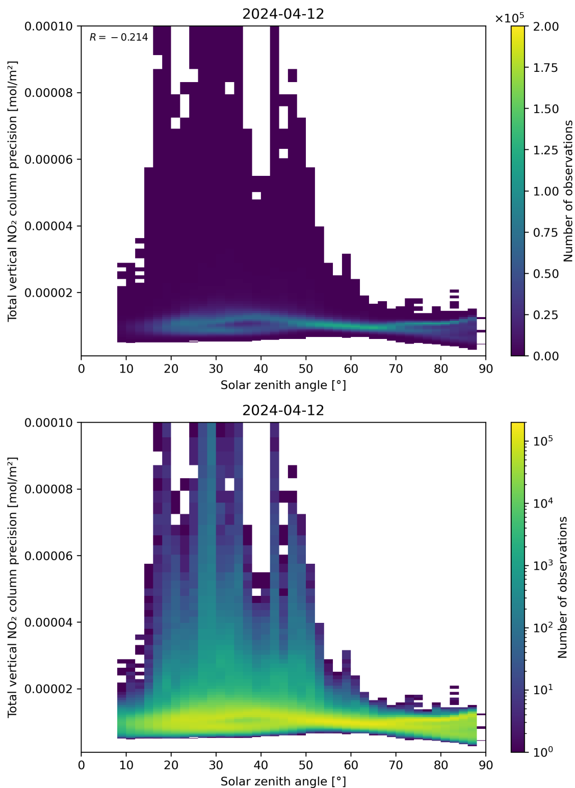
Figure 154: Scatter density plot of “Solar zenith angle” against “Total vertical NO 2 column precision” for 2024-04-11 to 2024-04-13.
