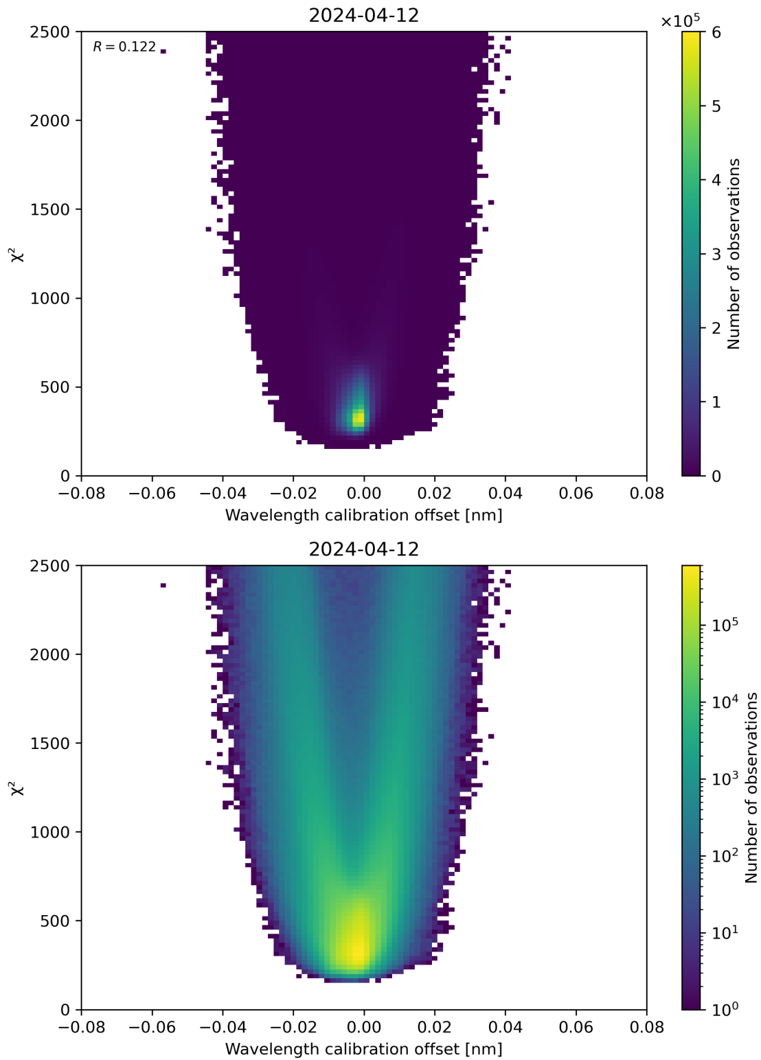
Figure 175: Scatter density plot of “Wavelength calibration offset” against “ \chi^2 ” for 2024-04-11 to 2024-04-13.
