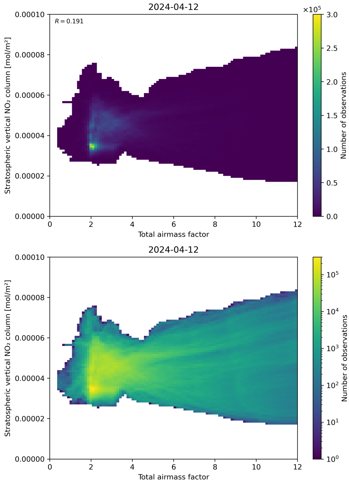
Figure 64: Scatter density plot of “Total airmass factor” against “Stratospheric vertical NO 2 column” for 2024-04-11 to 2024-04-13.
