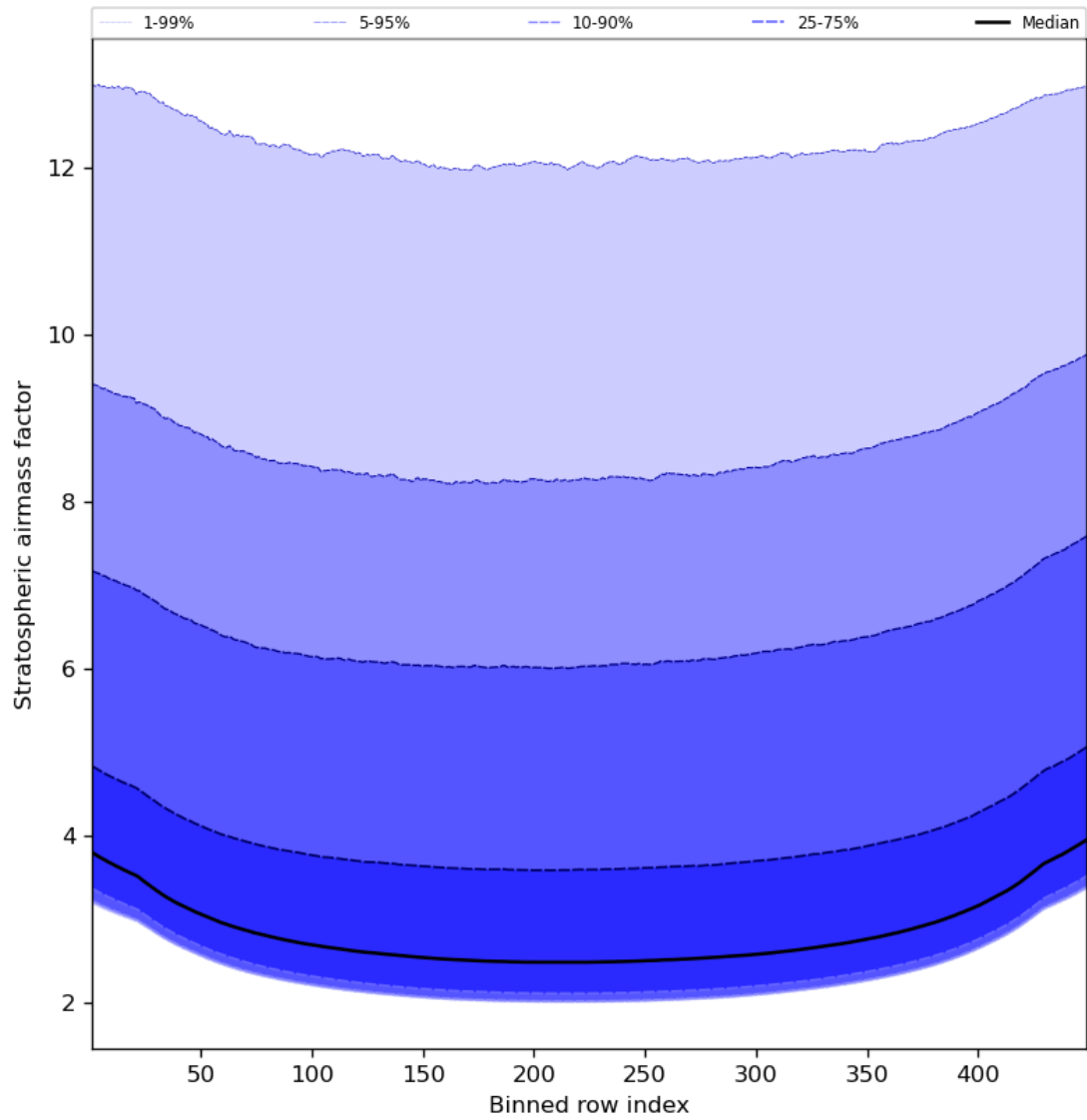
Figure 61: Along track statistics of “Stratospheric airmass factor” for 2024-04-11 to 2024-04-13
