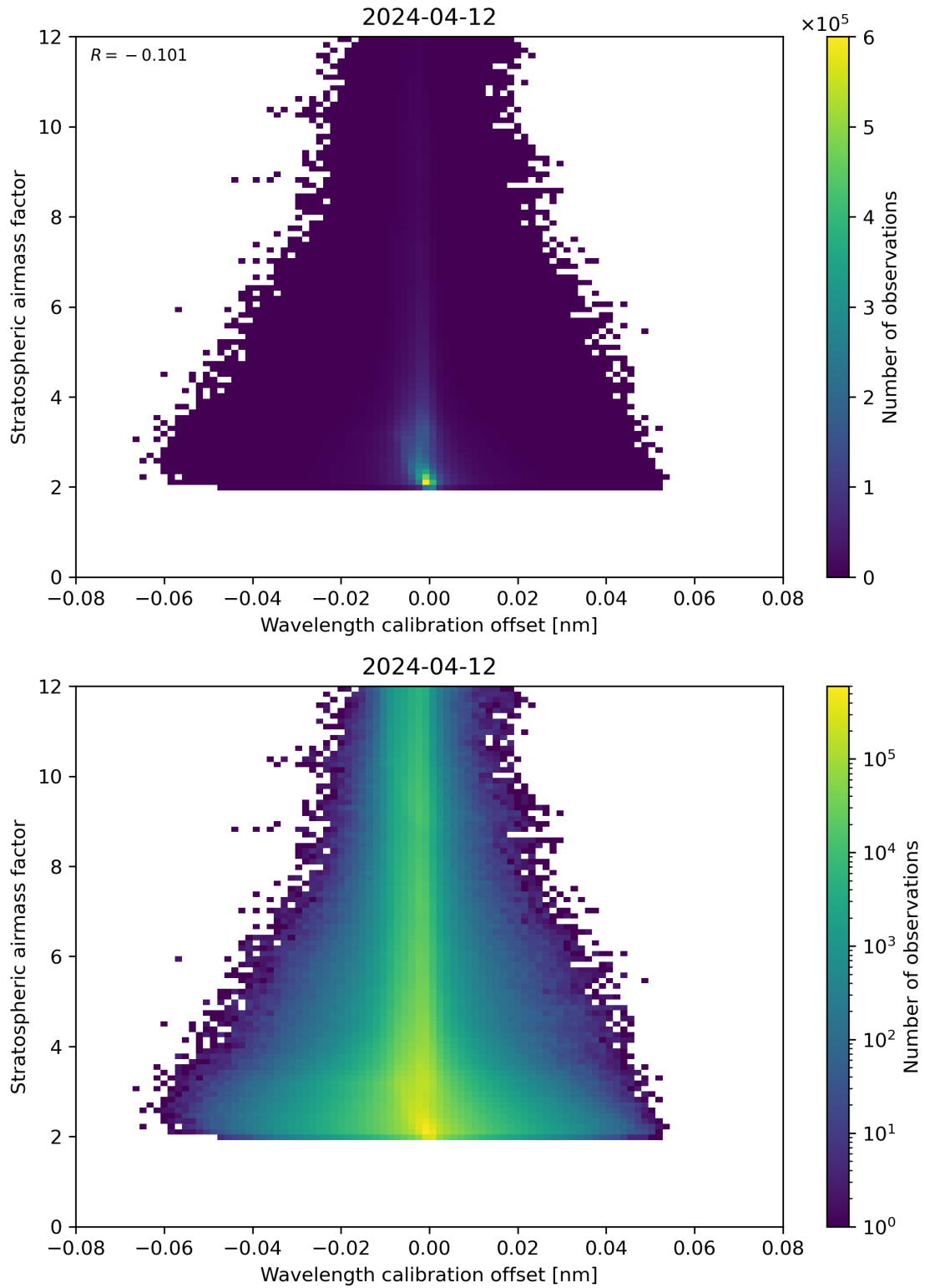
Figure 174: Scatter density plot of “Wavelength calibration offset” against “Stratospheric air mass factor” for 2024-04-11 to 2024-04-13.
