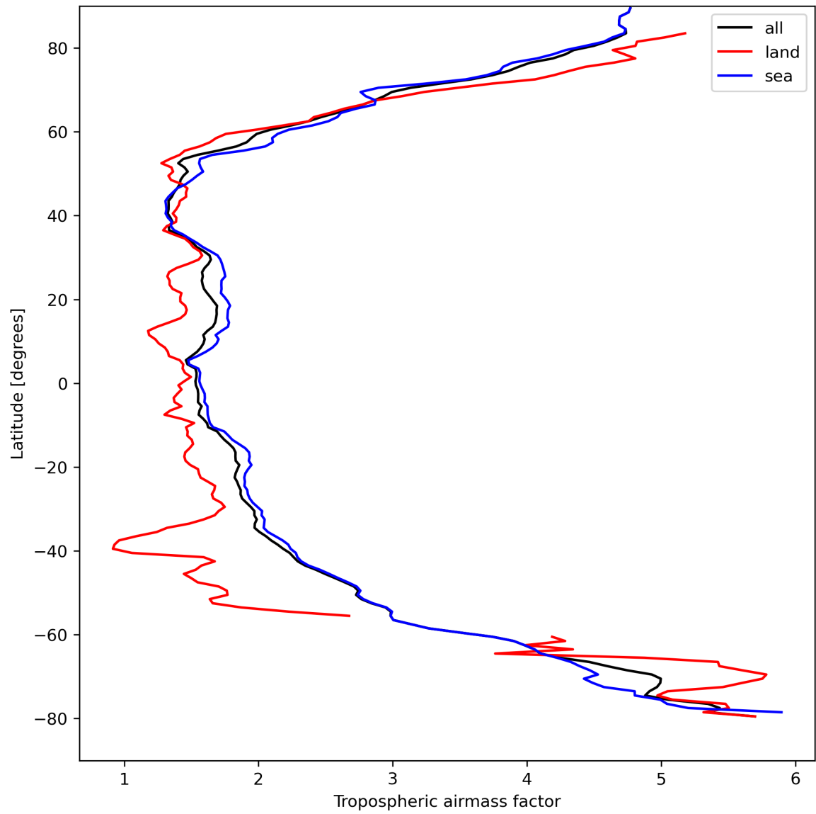
Figure 14: Zonal average of “Tropospheric airmass factor” for 2024-04-11 to 2024-04-13.
