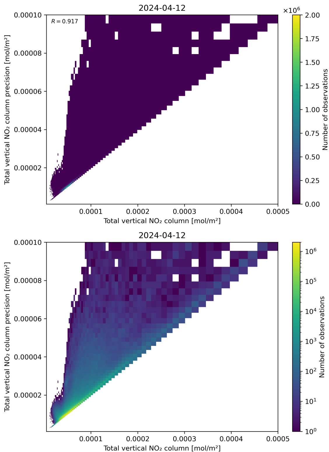
Figure 114: Scatter density plot of “Total vertical NO 2 column” against “Total vertical NO 2 column precision” for 2024-04-11 to 2024-04-13.
