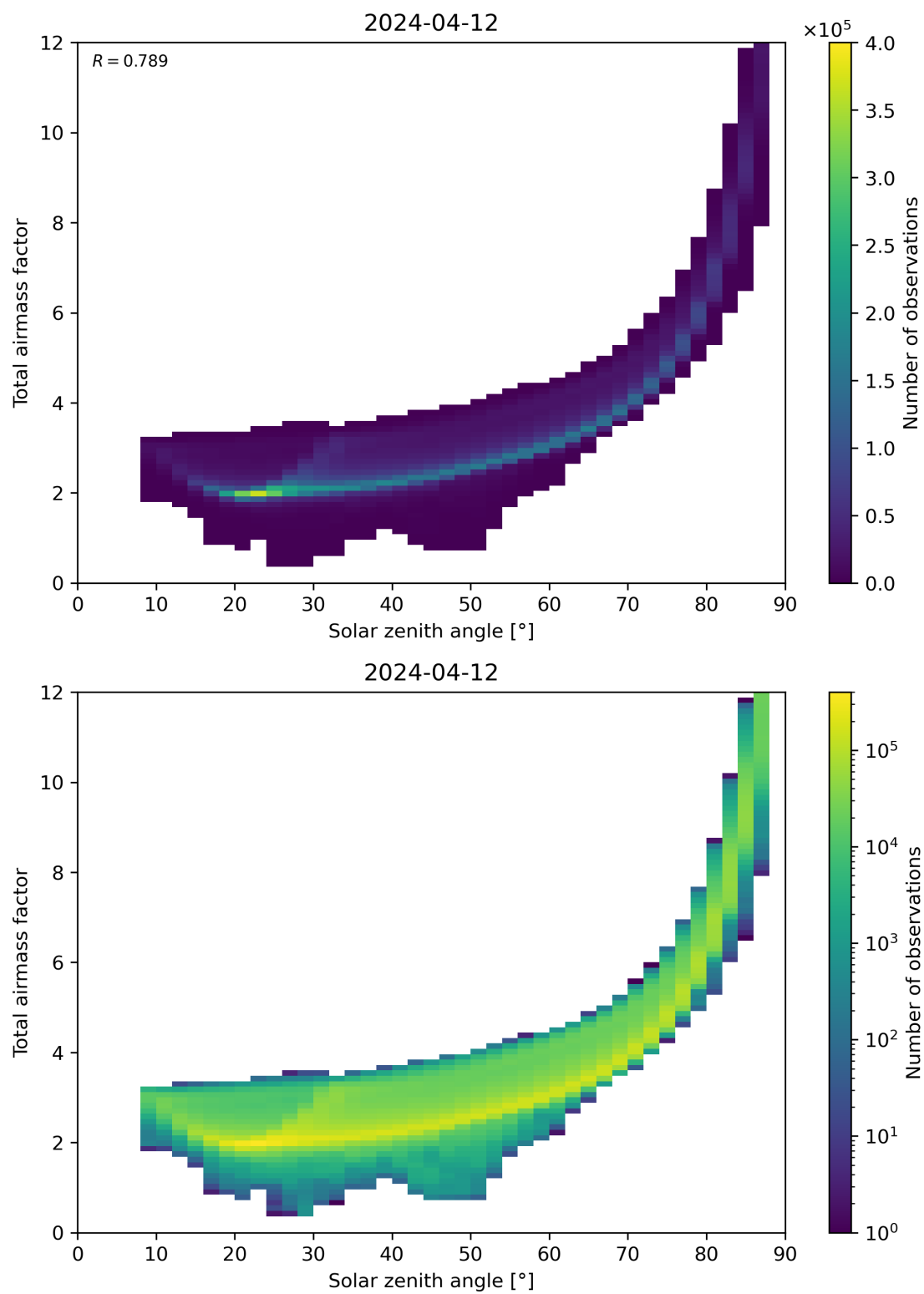
Figure 146: Scatter density plot of “Solar zenith angle” against “Total air mass factor” for 2024-04-11 to 2024-04-13.
