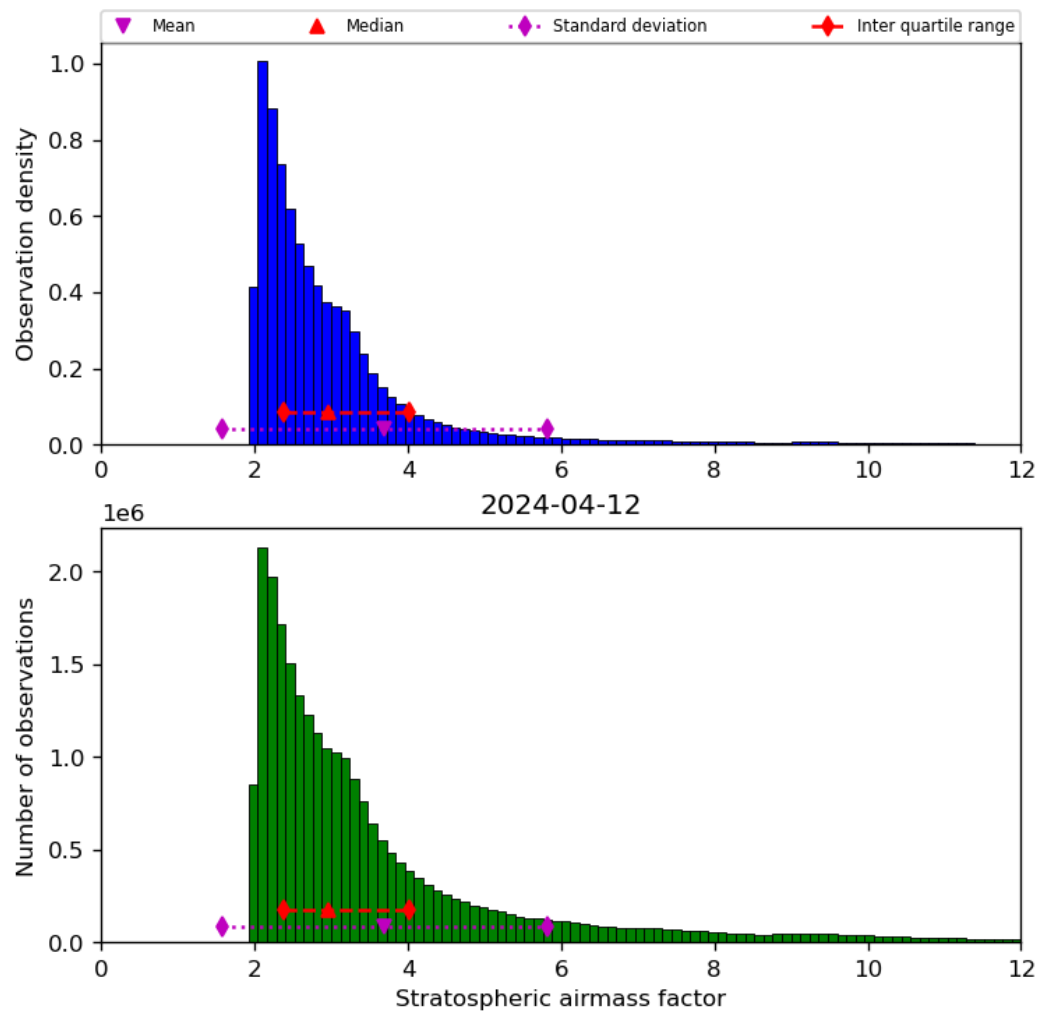
Figure 44: Histogram of “Stratospheric airmass factor” for 2024-04-11 to 2024-04-13
