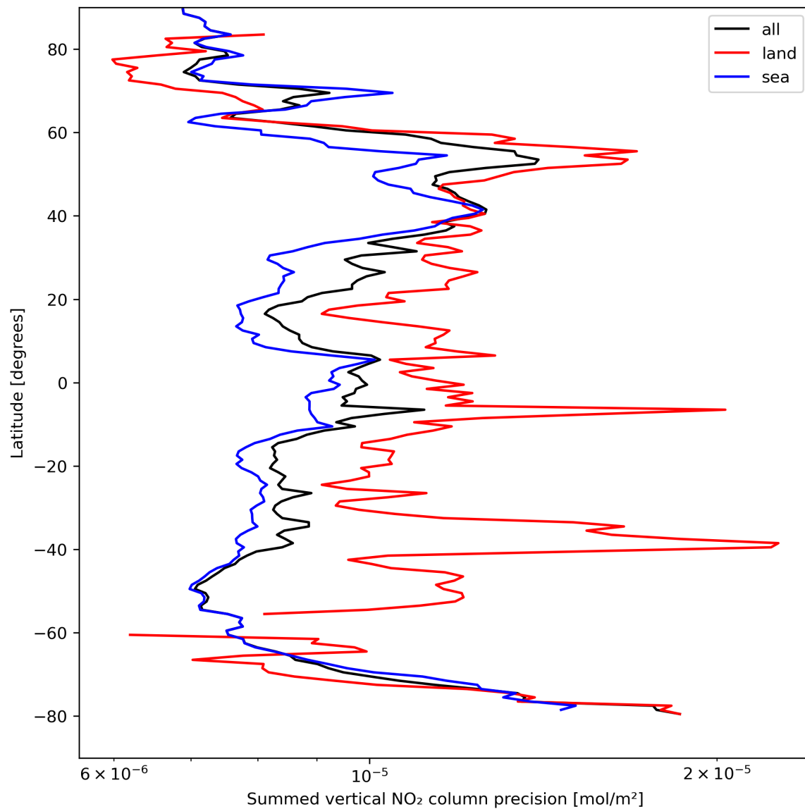
Figure 24: Zonal average of “Summed vertical NO 2 column precision” for 2024-04-11 to 2024-04-13.
