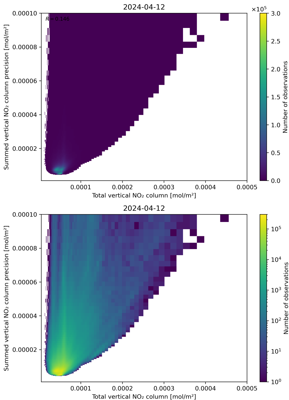
Figure 113: Scatter density plot of “Total vertical NO 2 column” against “Summed vertical NO 2 column precision” for 2024-04-11 to 2024-04-13.
