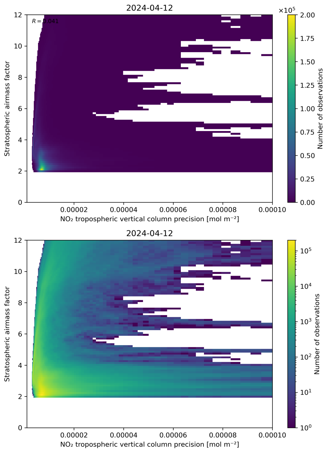
Figure 131: Scatter density plot of “NO 2 tropospheric vertical column precision” against “Stratospheric airmass factor” for 2024-04-11 to 2024-04-13.
