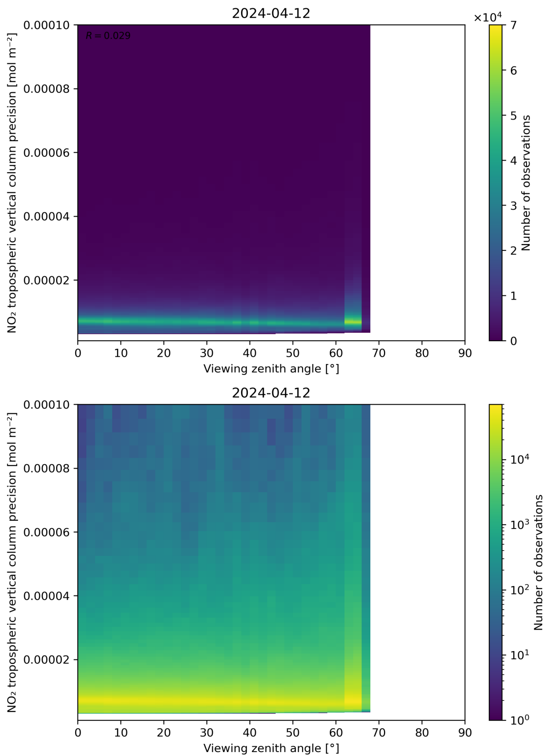
Figure 170: Scatter density plot of “Viewing zenith angle” against “NO 2 tropospheric vertical column precision” for 2024-04-11 to 2024-04-13.
