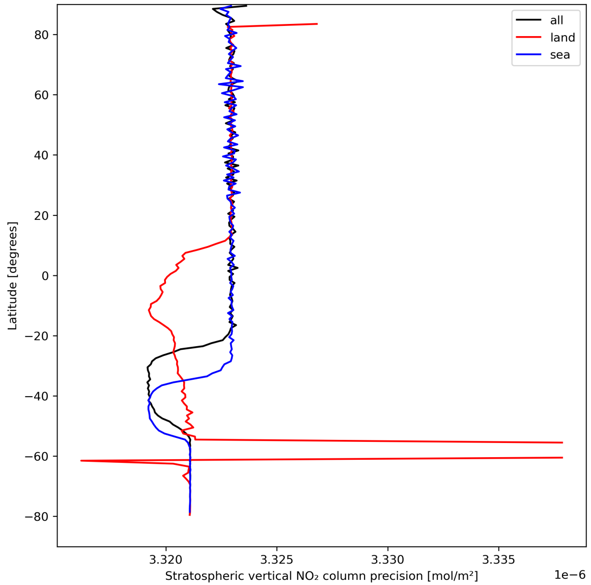
Figure 20: Zonal average of “Stratospheric vertical NO 2 column precision” for 2024-04-11 to 2024-04-13.
