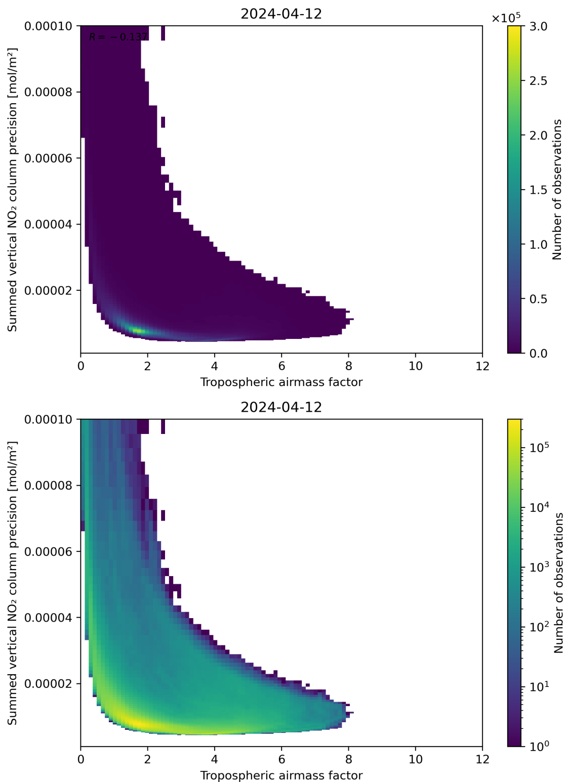
Figure 76: Scatter density plot of “Tropospheric air mass factor” against “Summed vertical NO 2 column precision” for 2024-04-11 to 2024-04-13.
