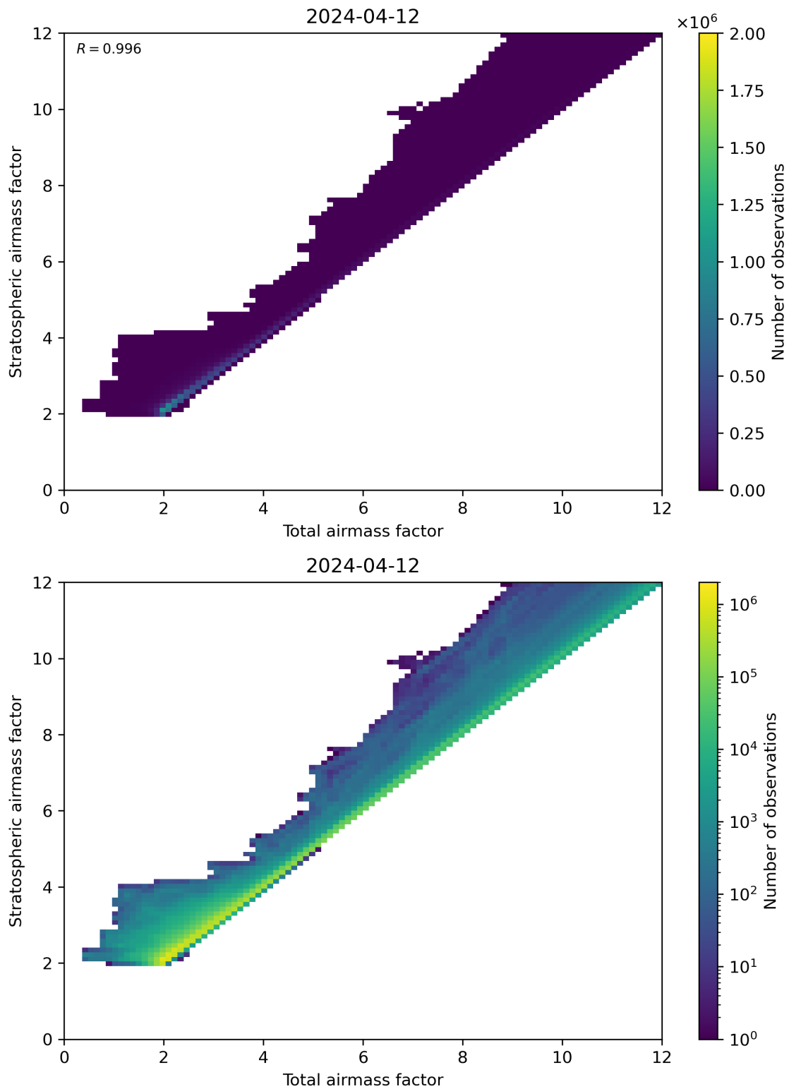
Figure 62: Scatter density plot of “Total airmass factor” against “Stratospheric airmass factor” for 2024-04-11 to 2024-04-13.
