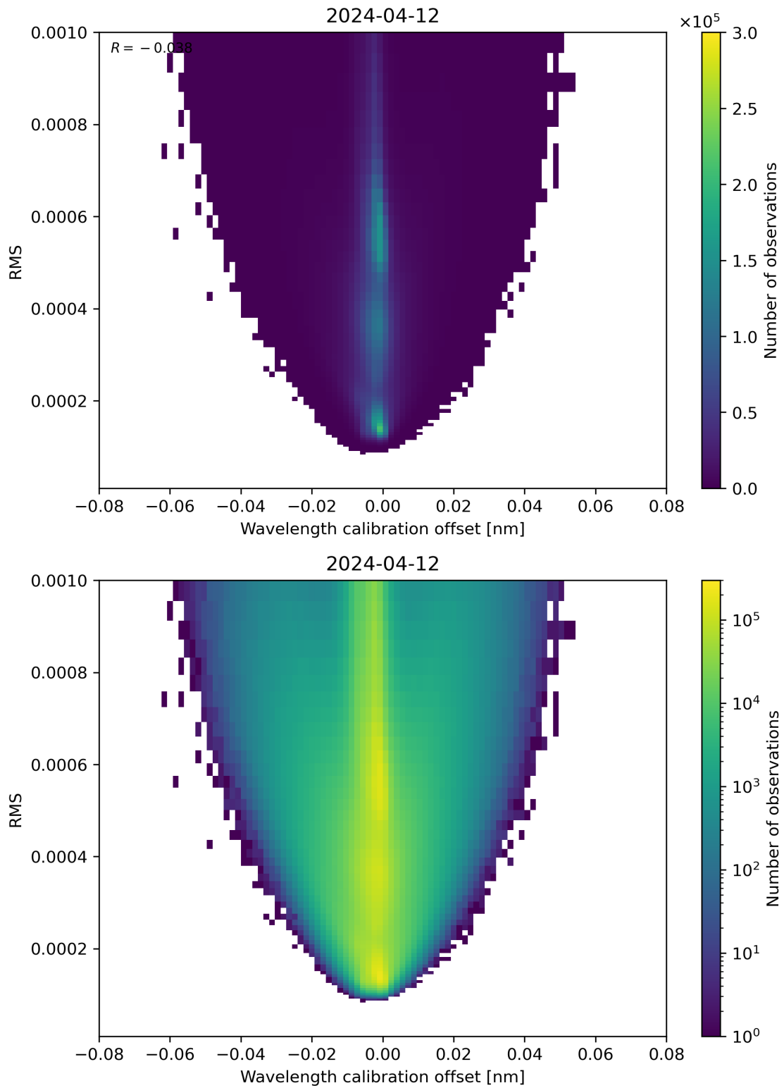
Figure 181: Scatter density plot of “Wavelength calibration offset” against “RMS” for 2024-04-11 to 2024-04-13.
