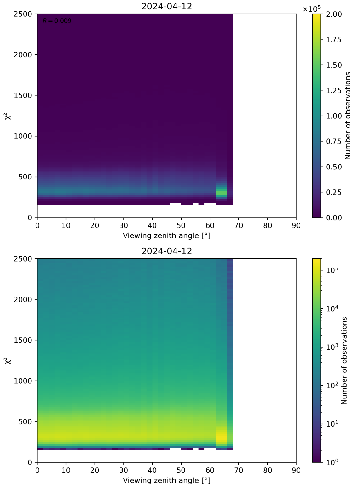
Figure 162: Scatter density plot of “Viewing zenith angle” against “ \chi^2 ” for 2024-04-11 to 2024-04-13.
