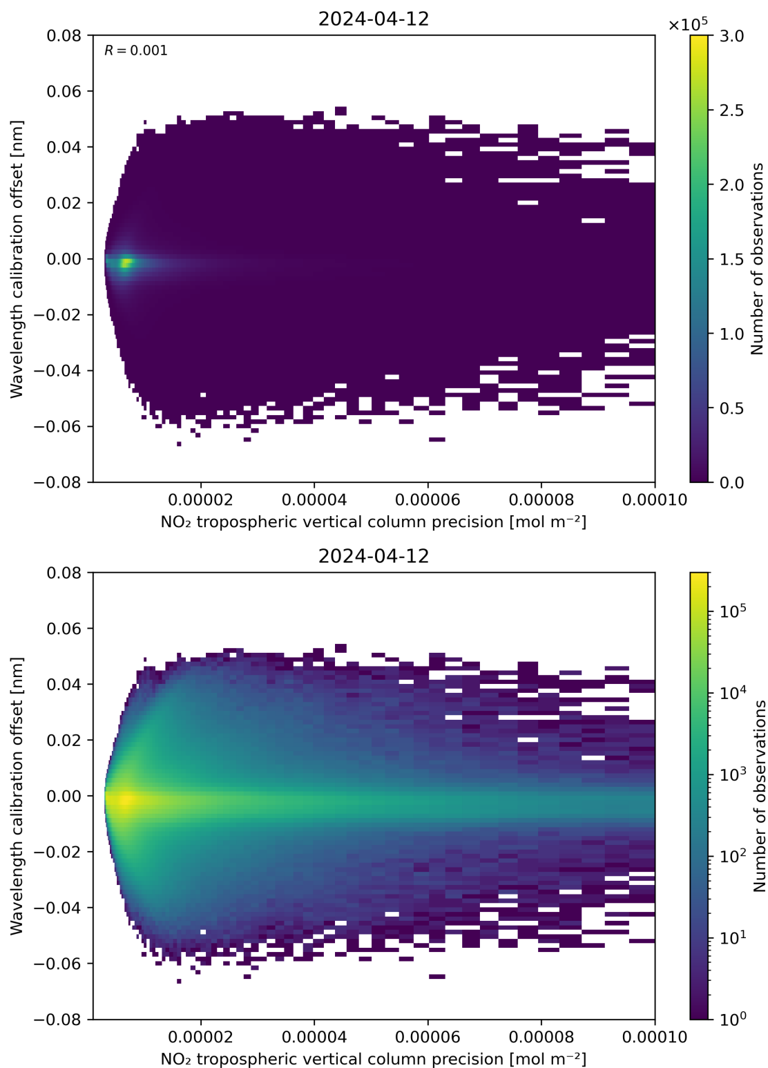
Figure 141: Scatter density plot of “NO 2 tropospheric vertical column precision” against “Wavelength calibration offset” for 2024-04-11 to 2024-04-13.
