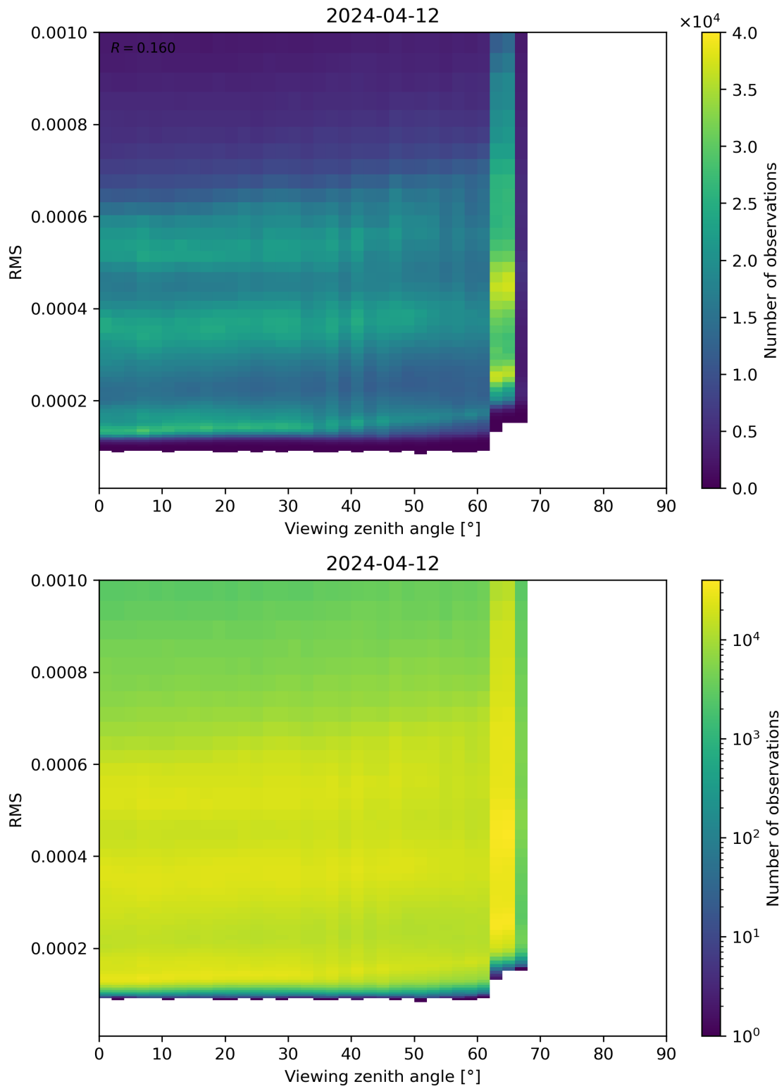
Figure 171: Scatter density plot of “Viewing zenith angle” against “RMS” for 2024-04-11 to 2024-04-13.
