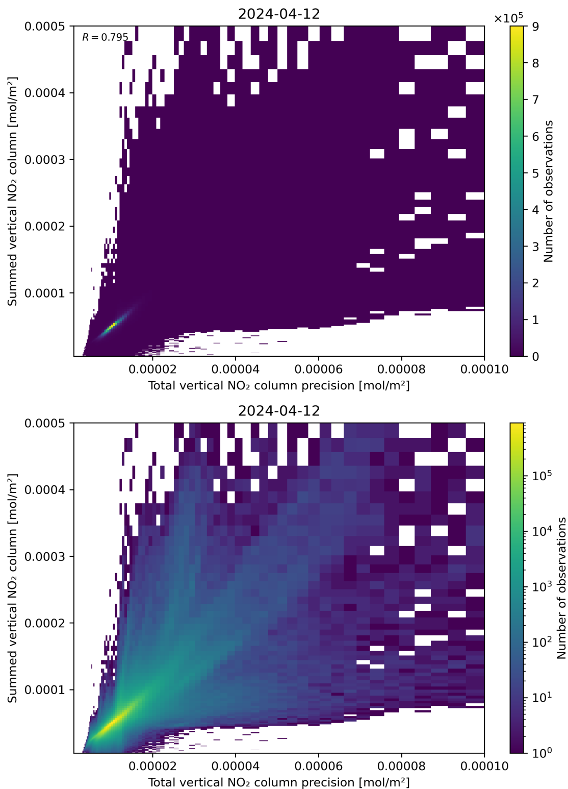
Figure 117: Scatter density plot of “Total vertical NO 2 column precision” against “Summed vertical NO 2 column” for 2024-04-11 to 2024-04-13.
