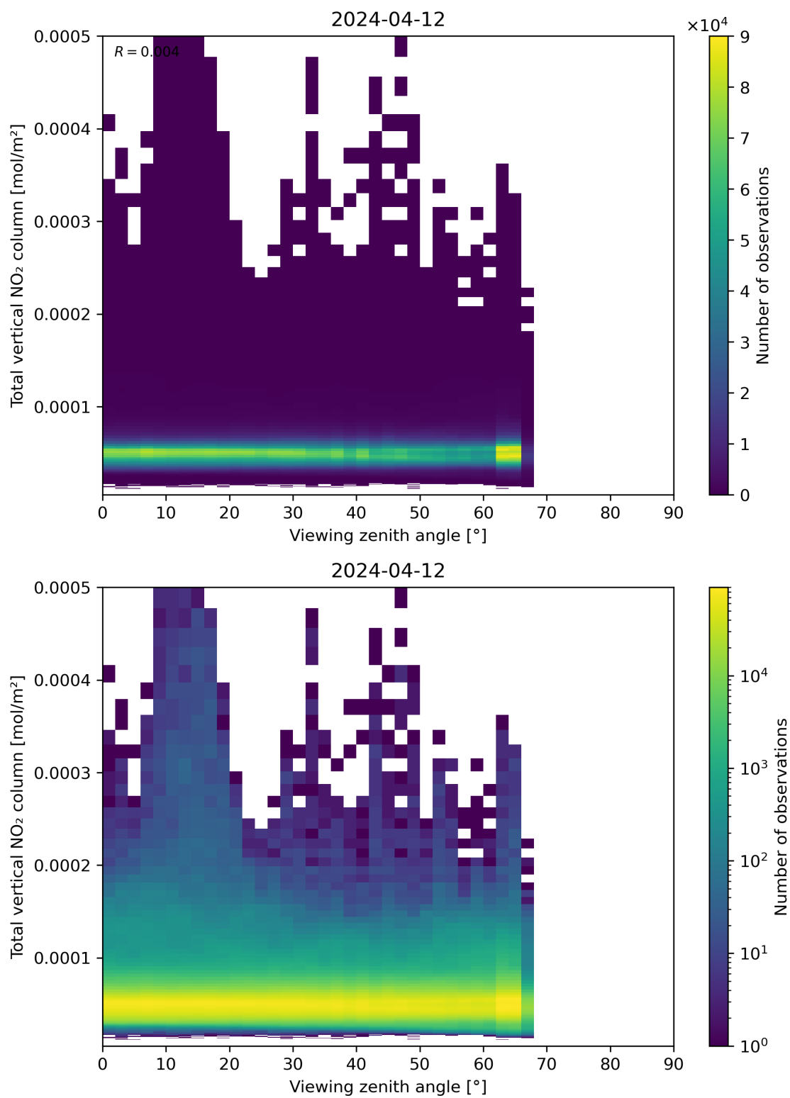
Figure 167: Scatter density plot of “Viewing zenith angle” against “Total vertical NO 2 column” for 2024-04-11 to 2024-04-13.
