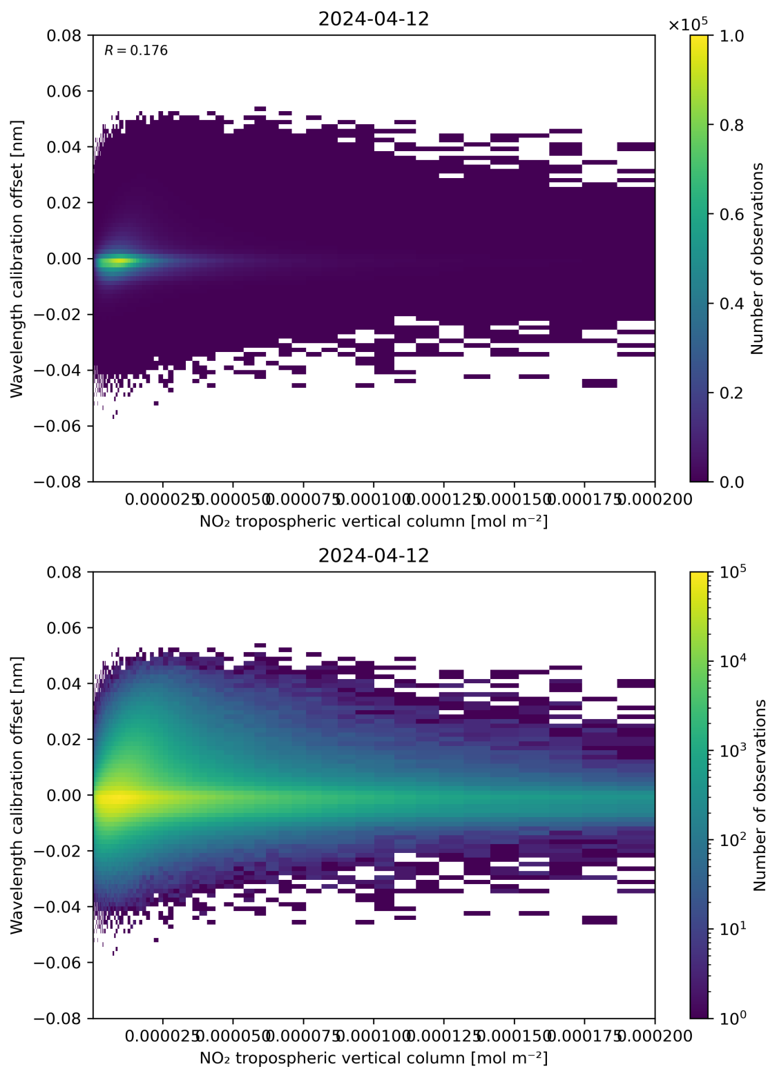
Figure 143: Scatter density plot of “NO 2 tropospheric vertical column” against “Wavelength calibration offset” for 2024-04-11 to 2024-04-13.
