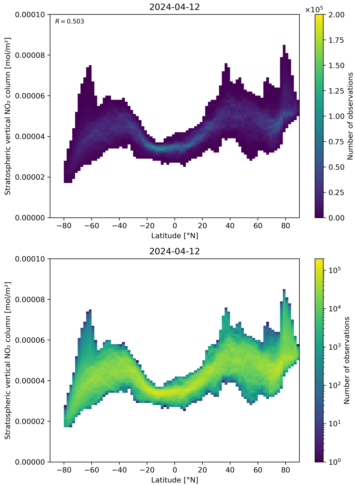
Figure 87: Scatter density plot of “Latitude” against “Stratospheric vertical NO 2 column” for 2024-04-11 to 2024-04-13.
