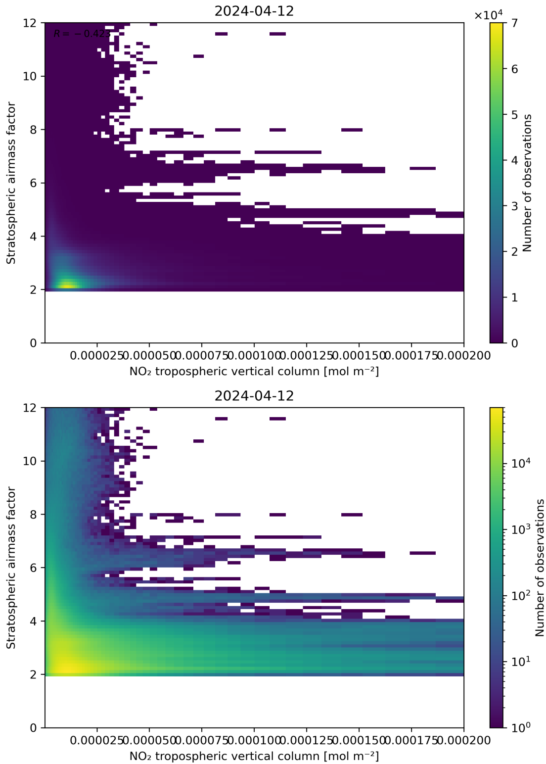
Figure 121: Scatter density plot of “NO 2 tropospheric vertical column” against “Stratospheric air mass factor” for 2024-04-11 to 2024-04-13.
