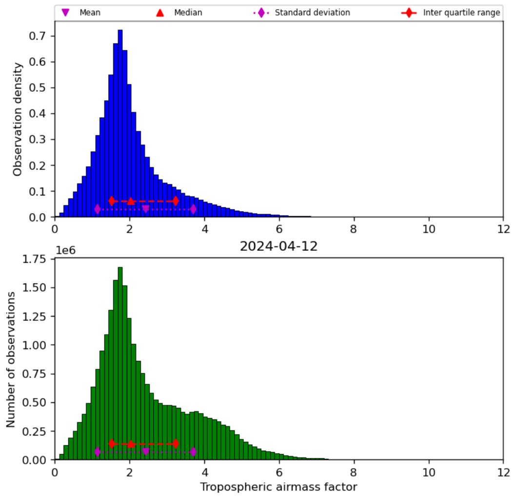
Figure 31: Histogram of “Tropospheric airmass factor” for 2024-04-11 to 2024-04-13
