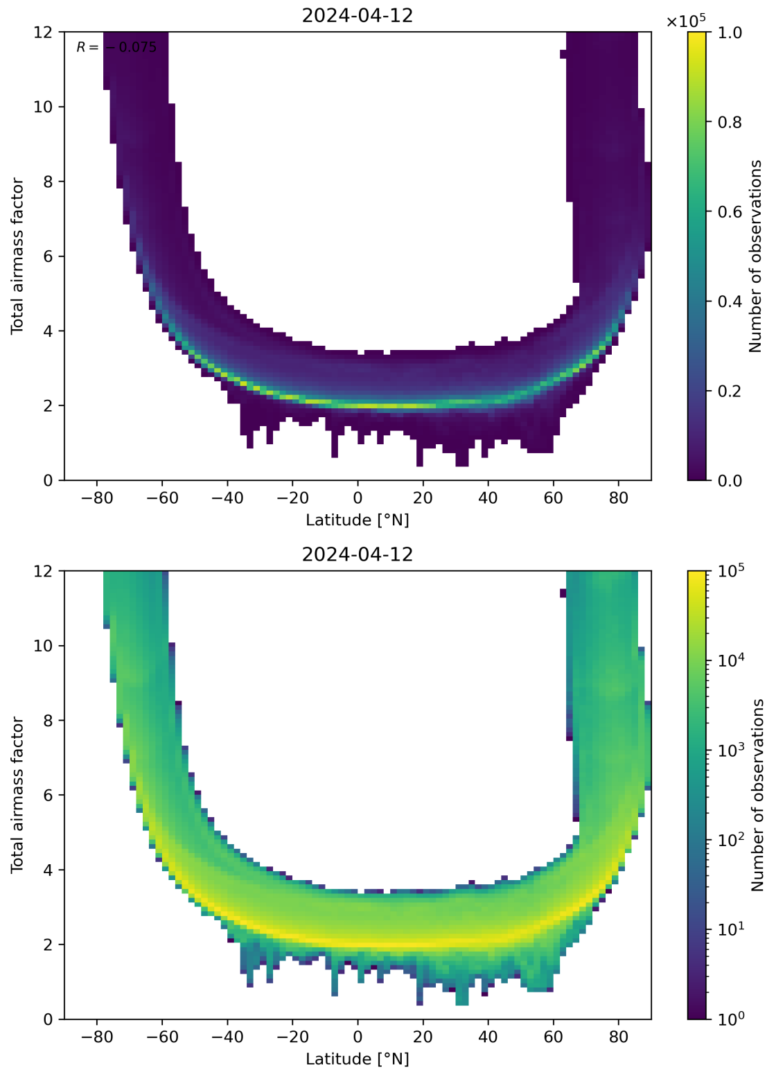
Figure 84: Scatter density plot of “Latitude” against “Total airmass factor” for 2024-04-11 to 2024-04-13.
