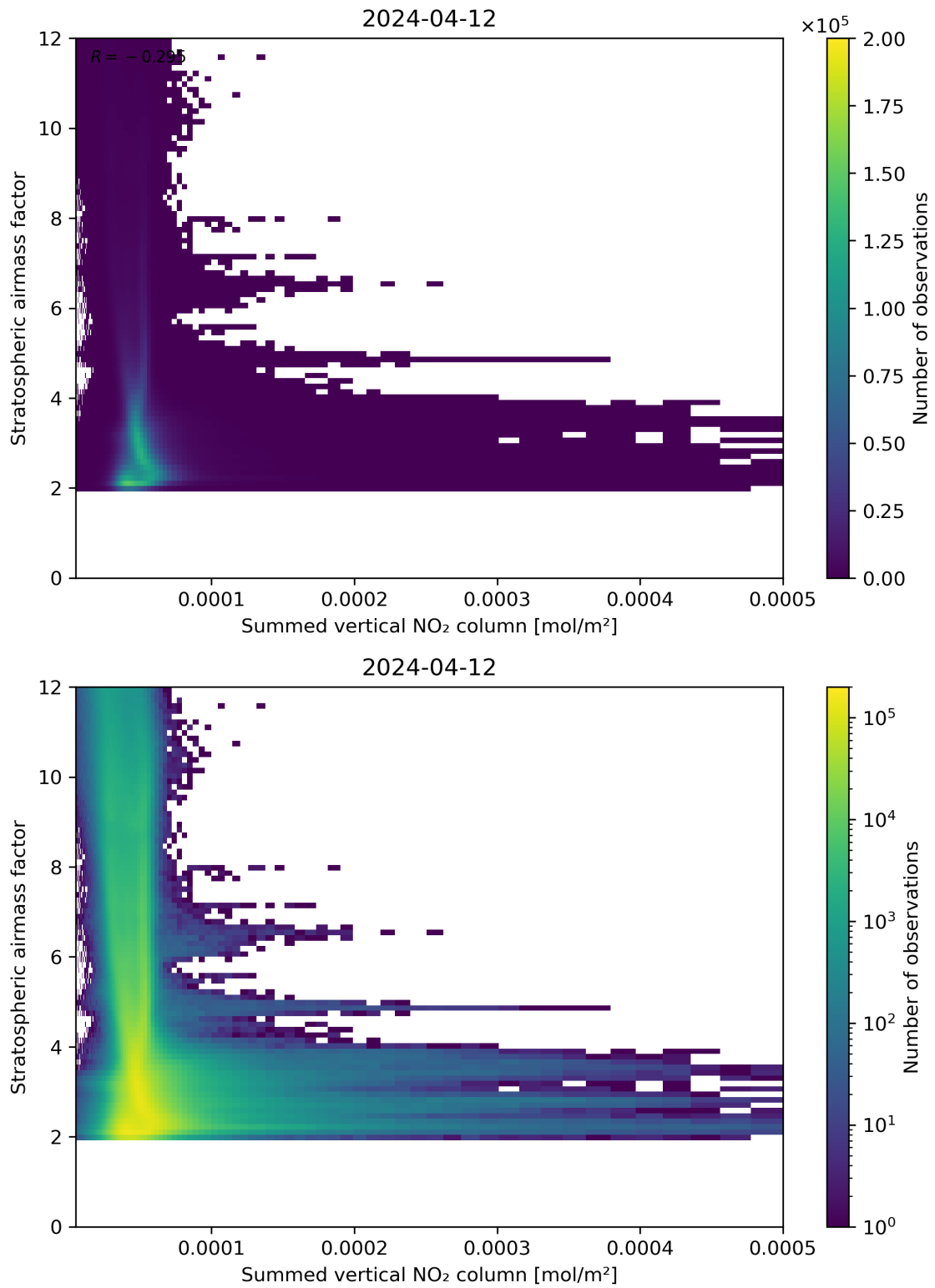
Figure 103: Scatter density plot of “Summed vertical NO 2 column” against “Stratospheric airmass factor” for 2024-04-11 to 2024-04-13.
