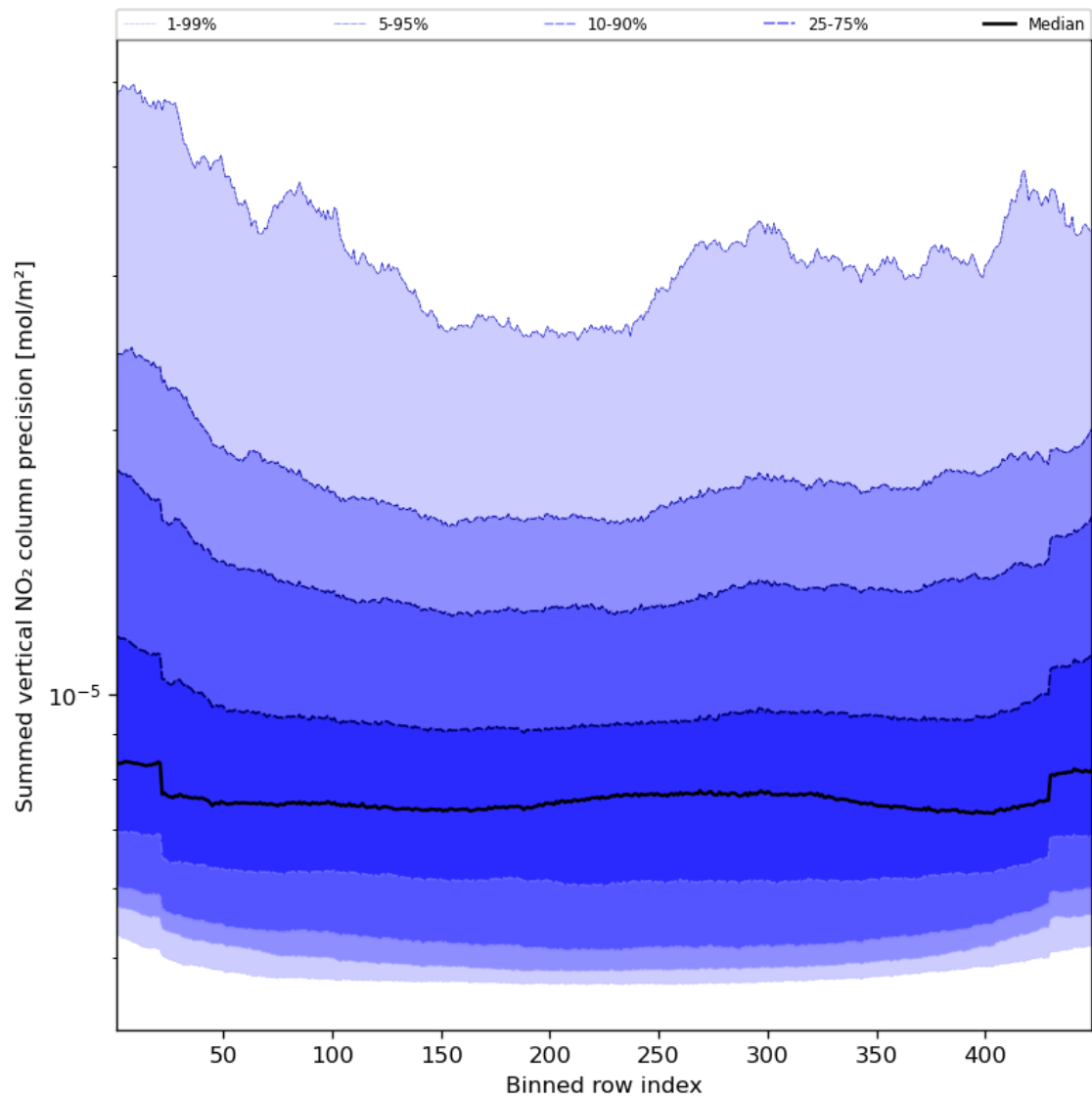
Figure 58: Along track statistics of “Summed vertical NO 2 column precision” for 2024-04-11 to 2024-04-13
