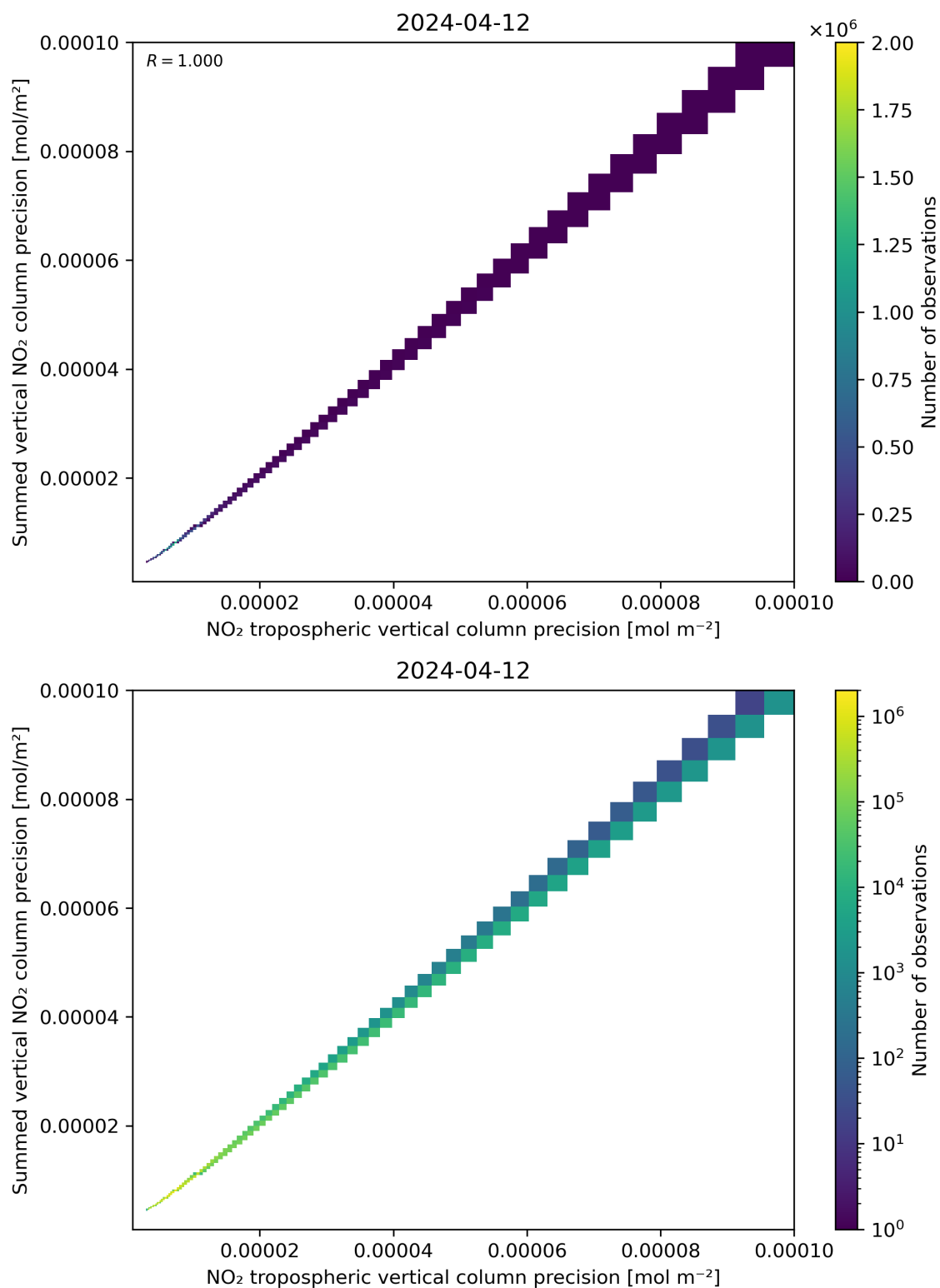
Figure 137: Scatter density plot of “NO 2 tropospheric vertical column precision” against “Summed vertical NO 2 column precision” for 2024-04-11 to 2024-04-13.
