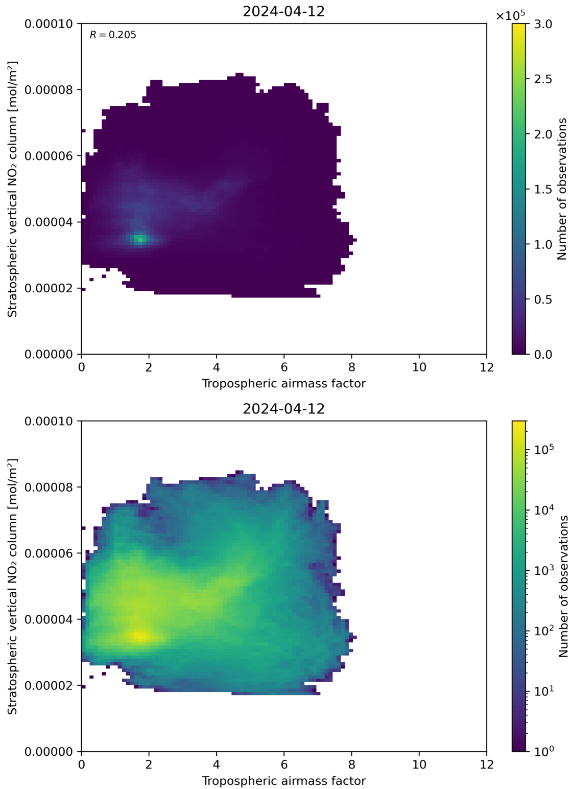
Figure 74: Scatter density plot of “Tropospheric air mass factor” against “Stratospheric vertical NO 2 column” for 2024-04-11 to 2024-04-13.
