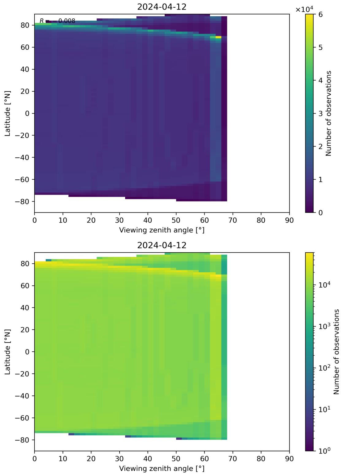
Figure 163: Scatter density plot of “Viewing zenith angle” against “Latitude” for 2024-04-11 to 2024-04-13.
