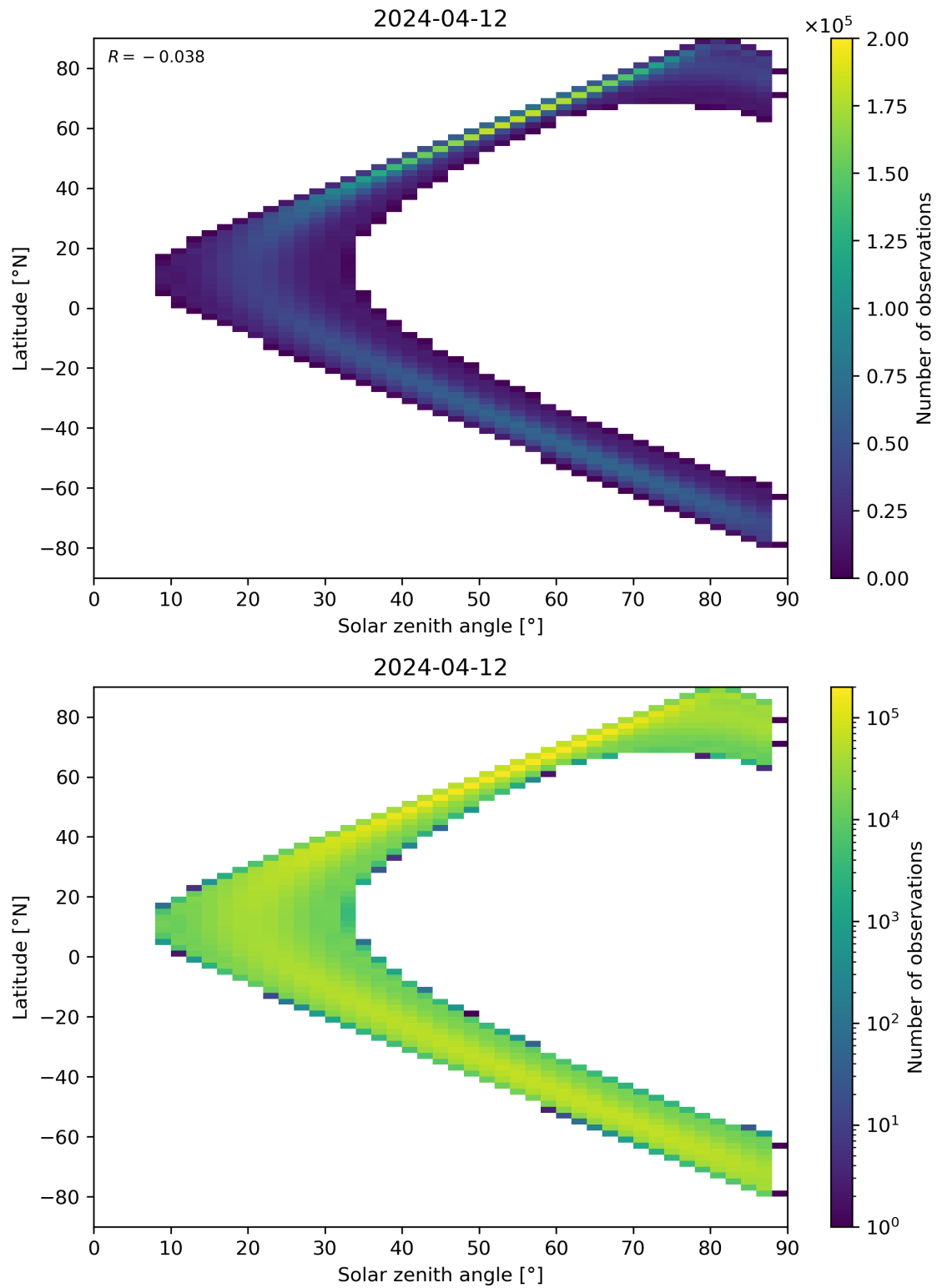
Figure 149: Scatter density plot of “Solar zenith angle” against “Latitude” for 2024-04-11 to 2024-04-13.
