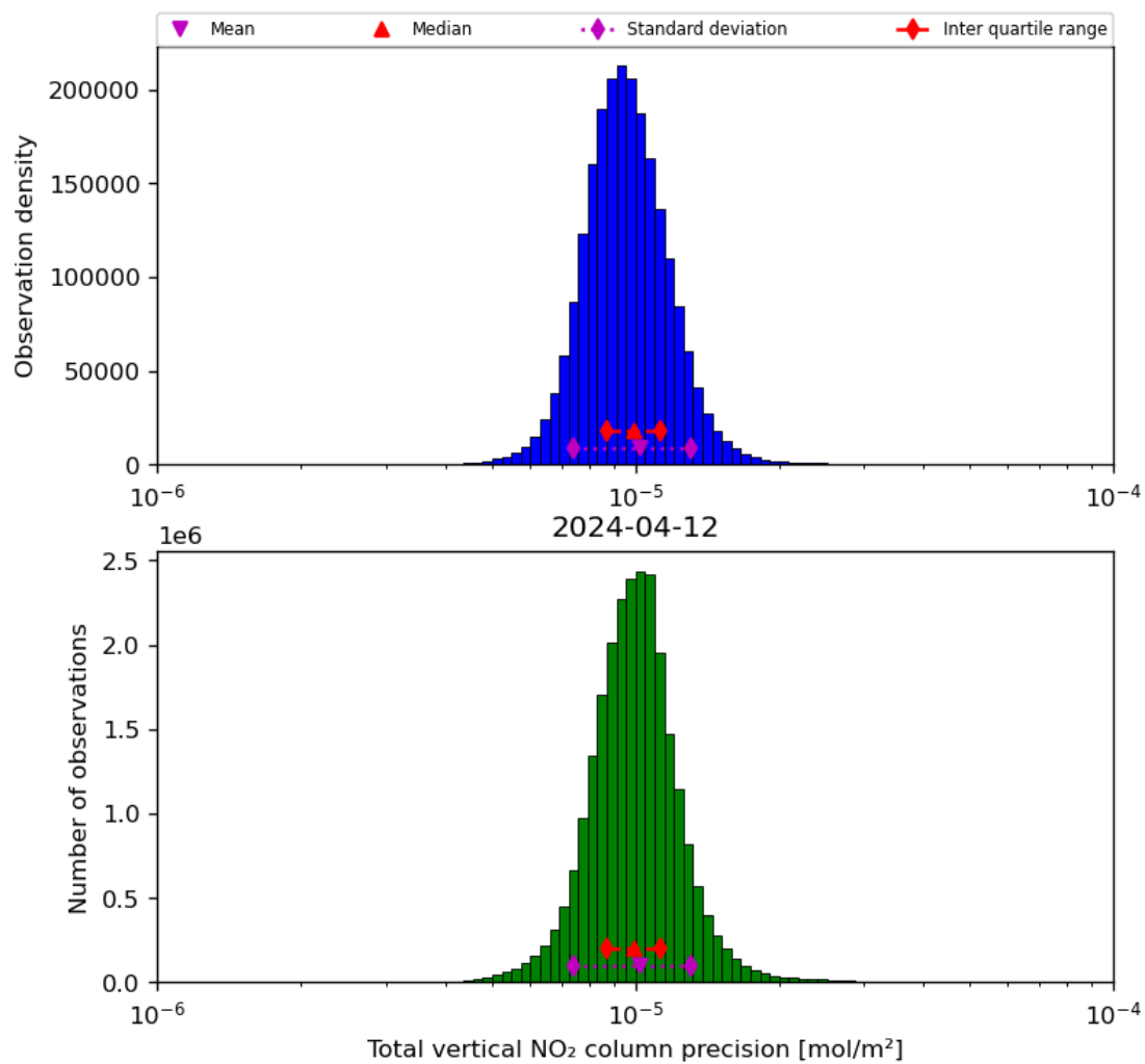
Figure 39: Histogram of "Total vertical NO 2 column precision" for 2024-04-11 to 2024-04-13
