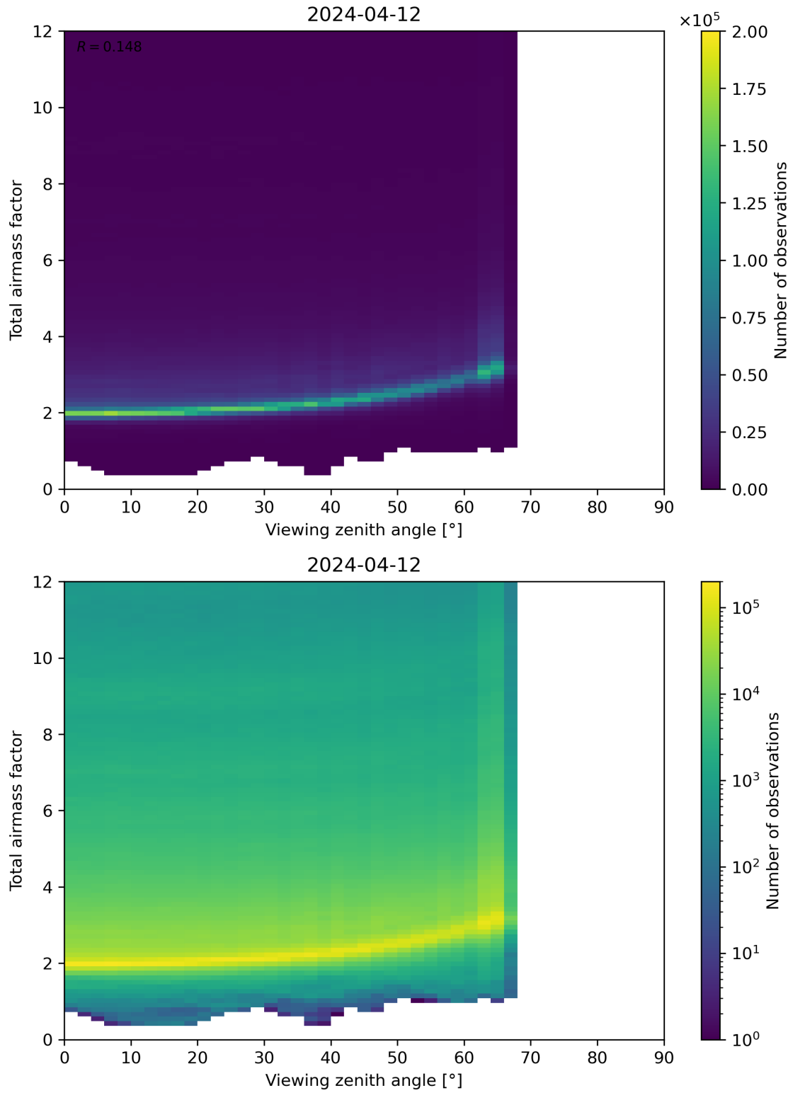
Figure 160: Scatter density plot of “Viewing zenith angle” against “Total airmass factor” for 2024-04-11 to 2024-04-13.
