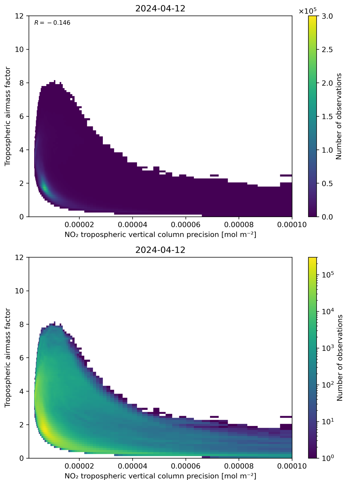
Figure 133: Scatter density plot of “NO 2 tropospheric vertical column precision” against “Tropospheric airmass factor” for 2024-04-11 to 2024-04-13.
