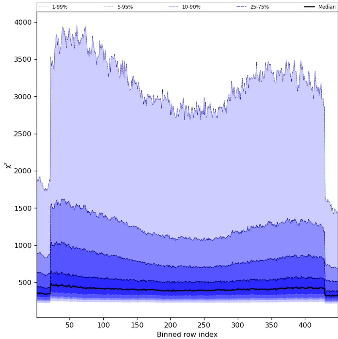
Figure 59: Along track statistics of “ \chi^2 ” for 2024-04-11 to 2024-04-13
