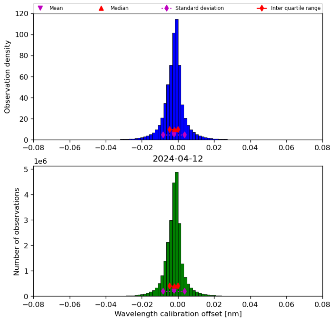
Figure 35: Histogram of “Wavelength calibration offset” for 2024-04-11 to 2024-04-13
