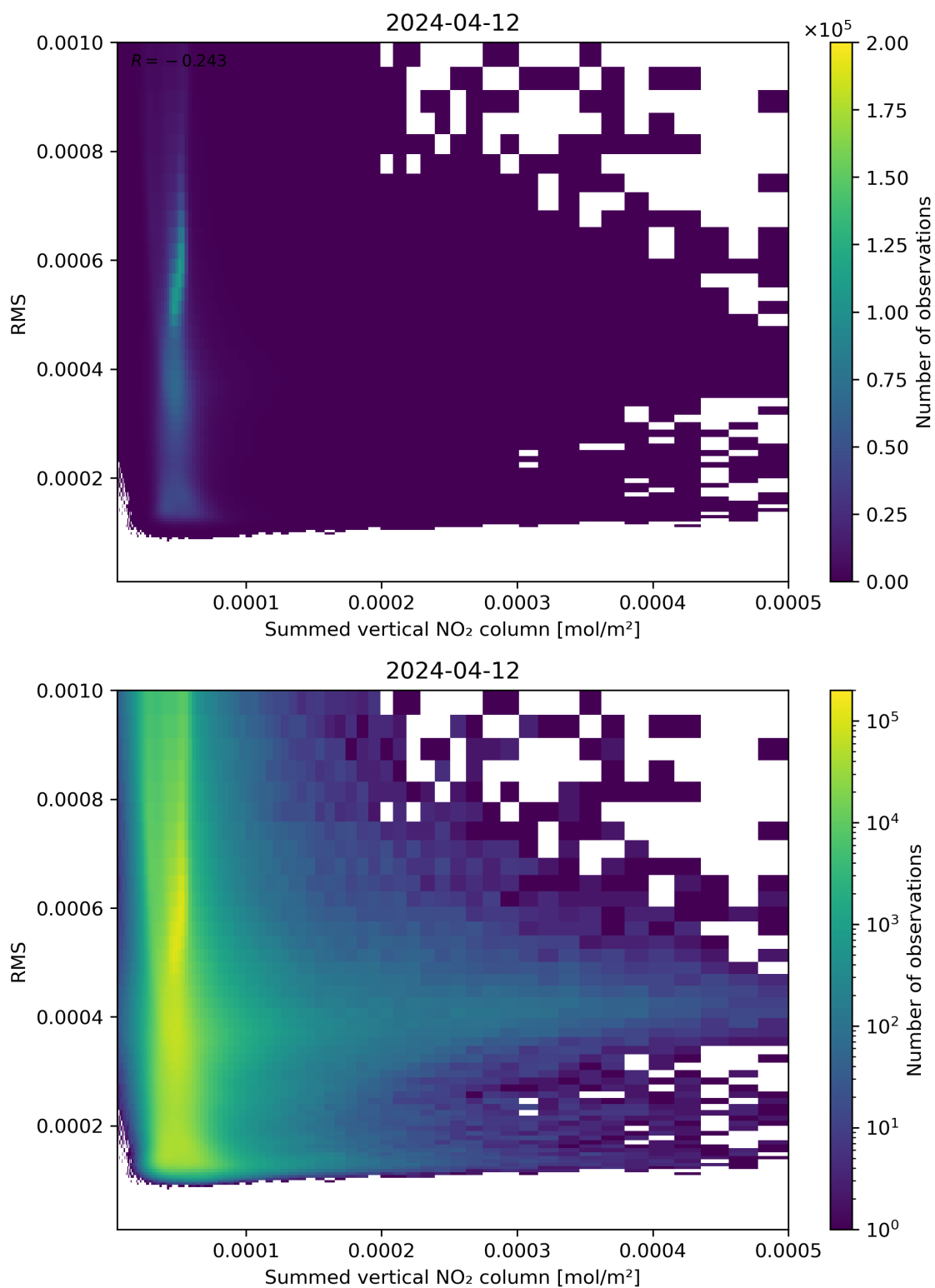
Figure 109: Scatter density plot of “Summed vertical NO 2 column” against “RMS” for 2024-04-11 to 2024-04-13.
