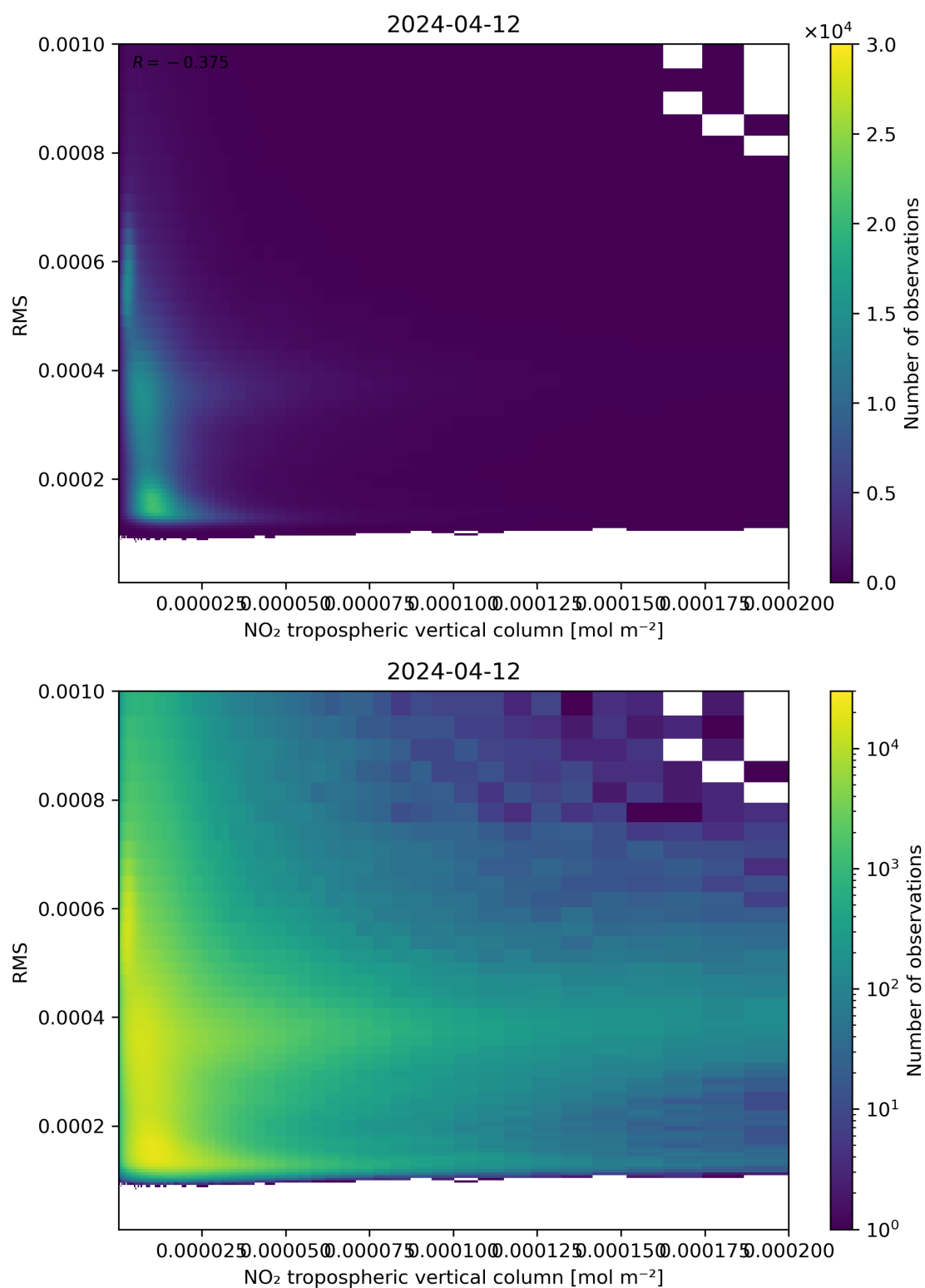
Figure 142: Scatter density plot of “NO 2 tropospheric vertical column” against “RMS” for 2024-04-11 to 2024-04-13.
