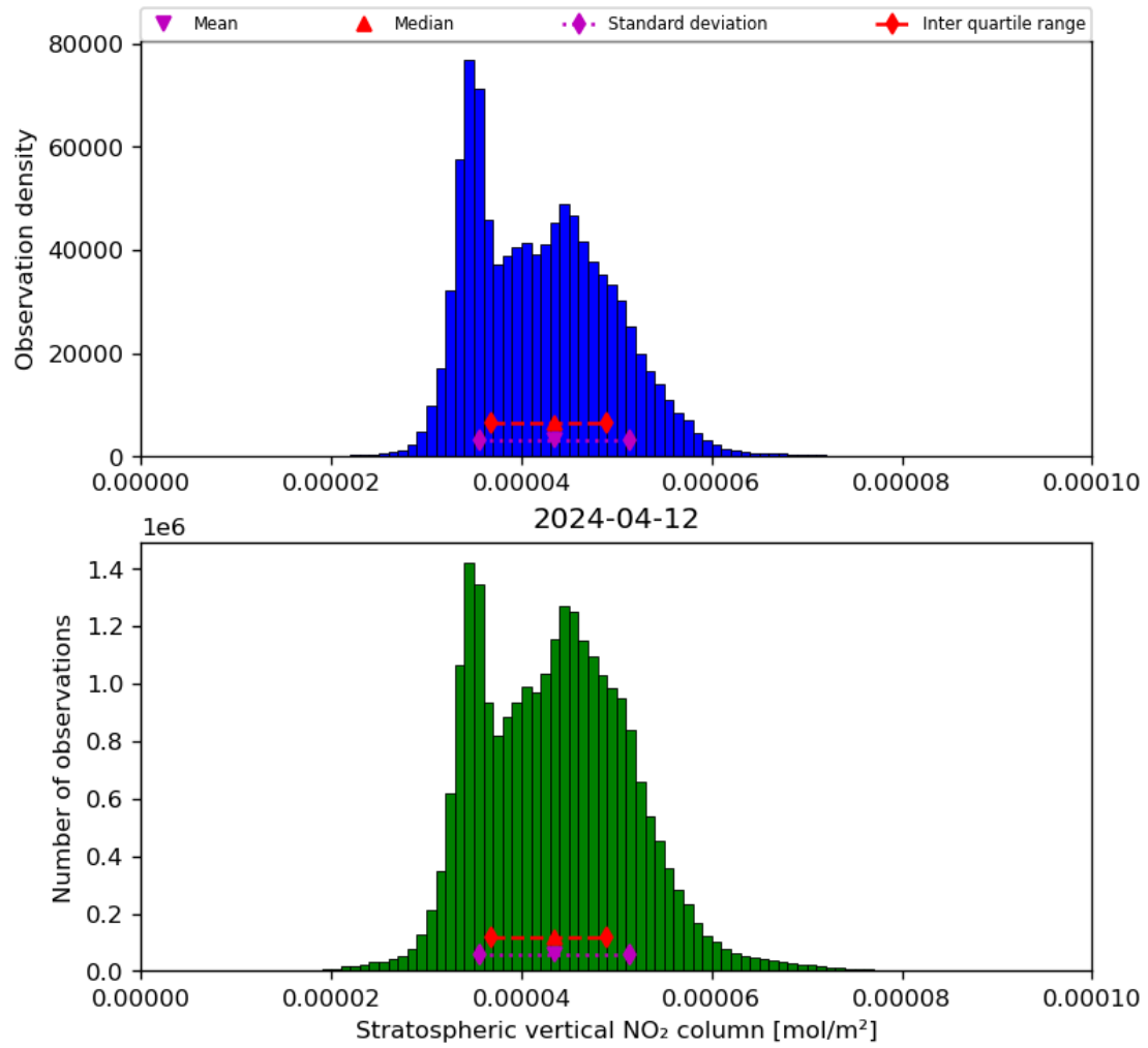
Figure 36: Histogram of “Stratospheric vertical NO 2 column” for 2024-04-11 to 2024-04-13
