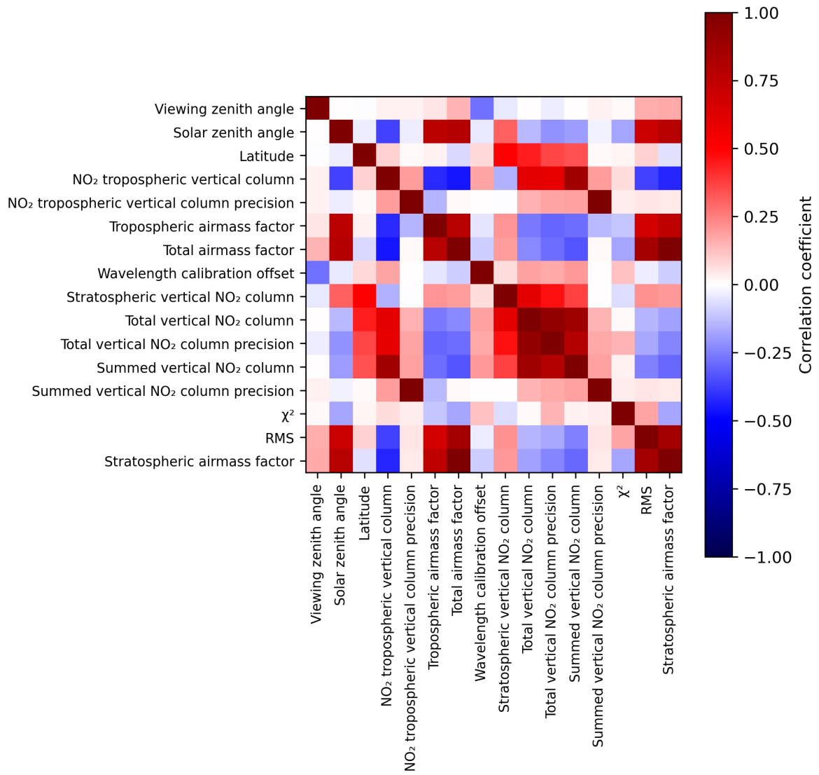
Figure 2: Map of correlation matrix for 2024-04-11 to 2024-04-13.
