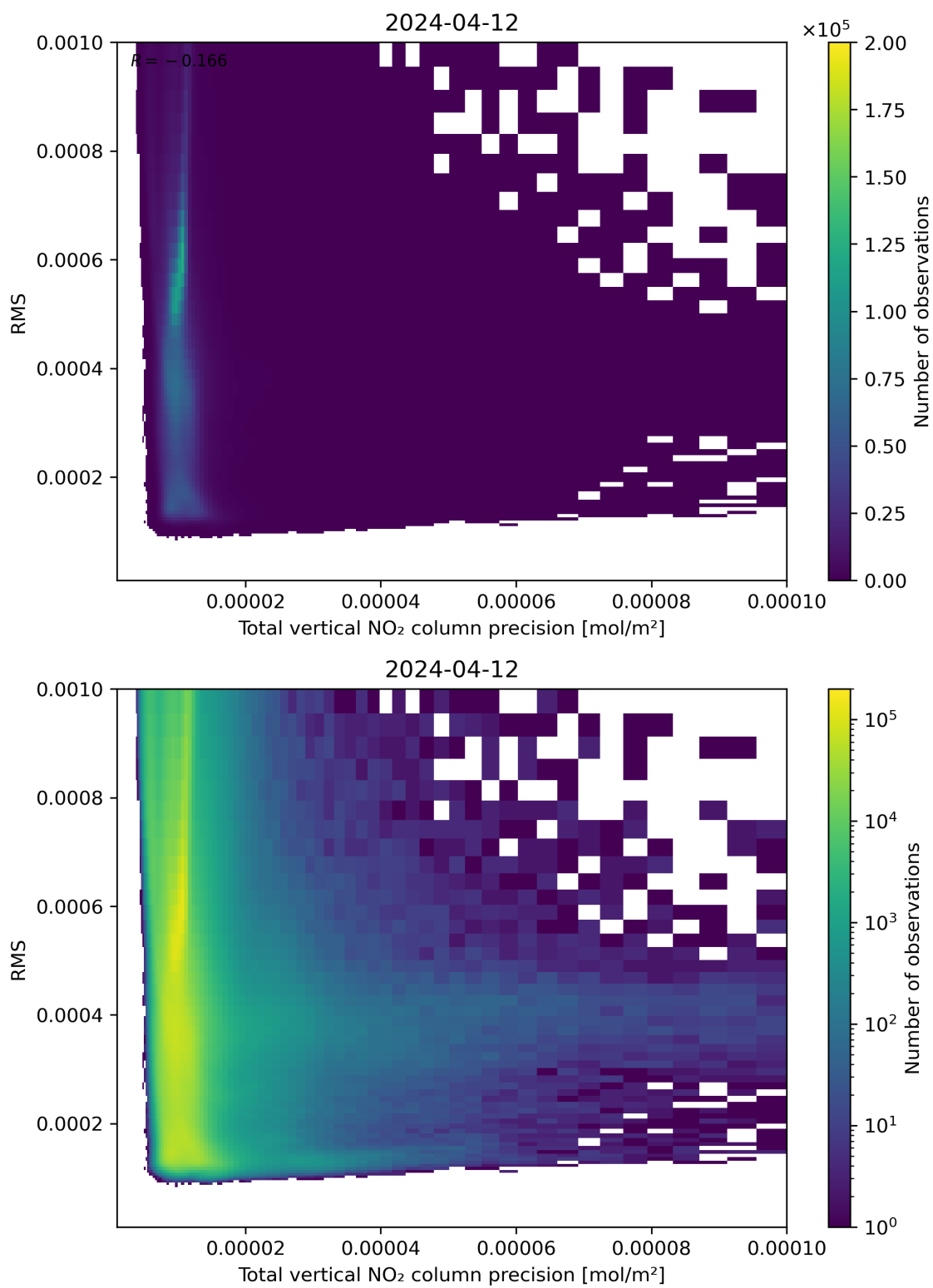
Figure 119: Scatter density plot of “Total vertical NO 2 column precision” against “RMS” for 2024-04-11 to 2024-04-13.
