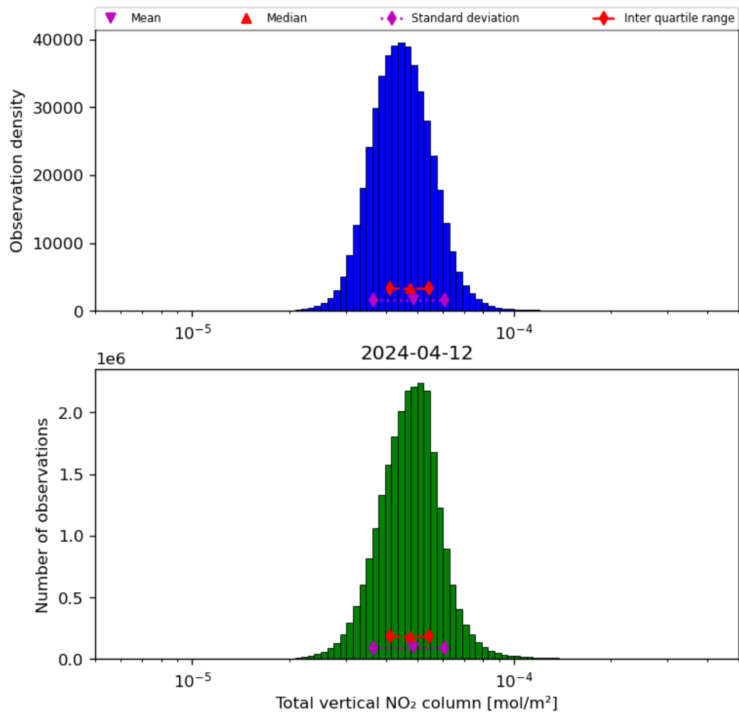
Figure 38: Histogram of "Total vertical NO 2 column" for 2024-04-11 to 2024-04-13
