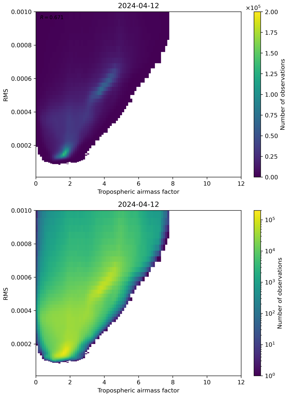
Figure 79: Scatter density plot of “Tropospheric airmass factor” against “RMS” for 2024-04-11 to 2024-04-13.
