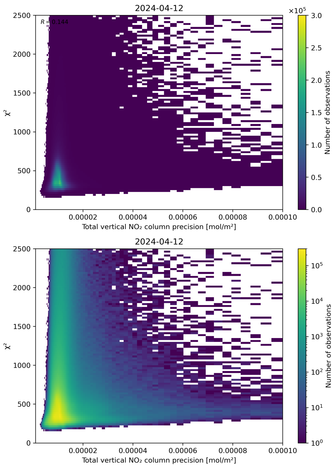
Figure 116: Scatter density plot of “Total vertical NO 2 column precision” against “ \chi^2 ” for 2024-04-11 to 2024-04-13.
