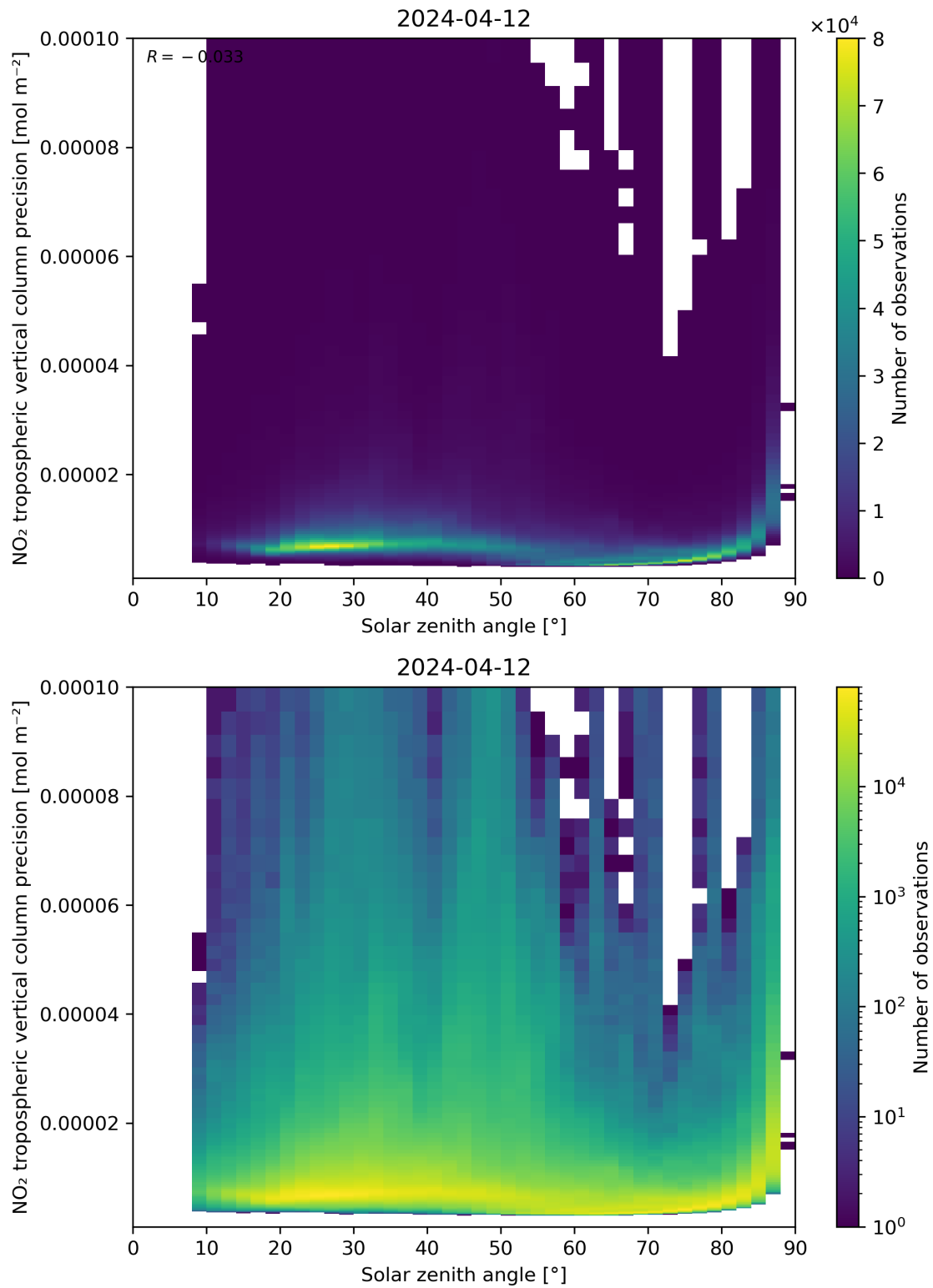
Figure 156: Scatter density plot of “Solar zenith angle” against “NO 2 tropospheric vertical column precision” for 2024-04-11 to 2024-04-13.
