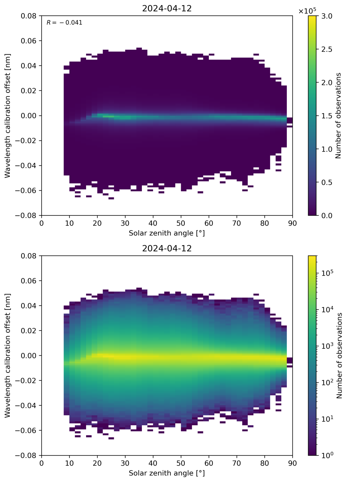
Figure 158: Scatter density plot of “Solar zenith angle” against “Wavelength calibration offset” for 2024-04-11 to 2024-04-13.
