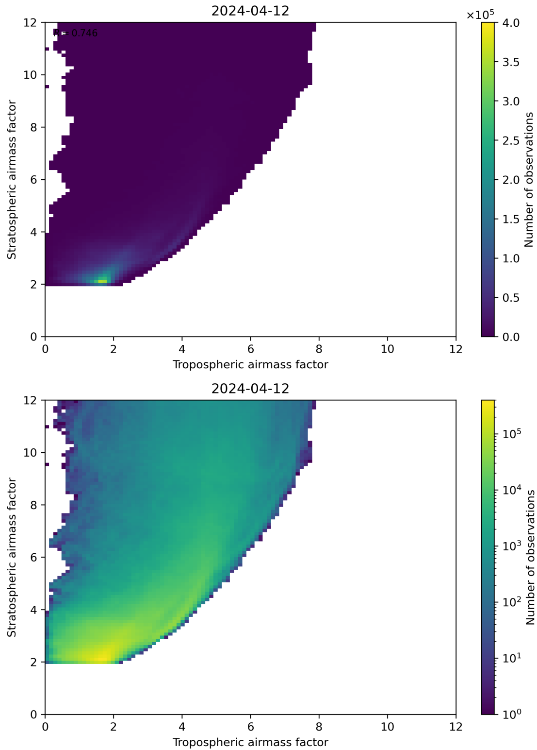
Figure 71: Scatter density plot of “Tropospheric airmass factor” against “Stratospheric airmass factor” for 2024-04-11 to 2024-04-13.
