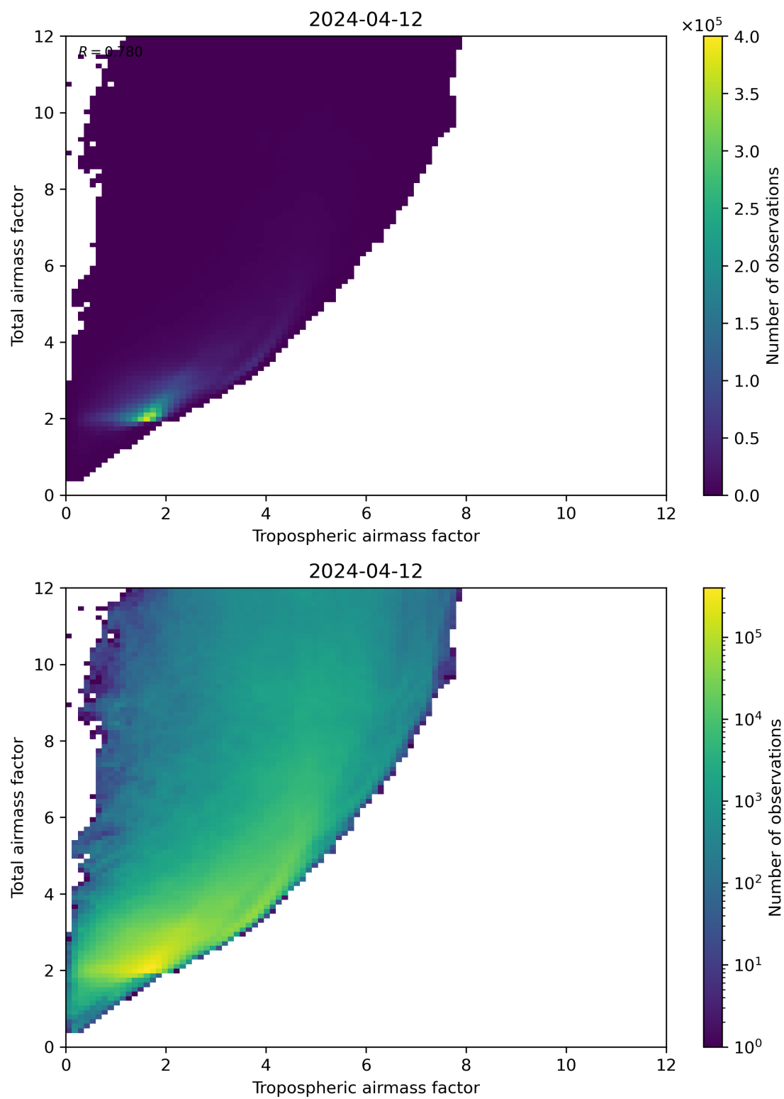
Figure 72: Scatter density plot of “Tropospheric airmass factor” against “Total airmass factor” for 2024-04-11 to 2024-04-13.
