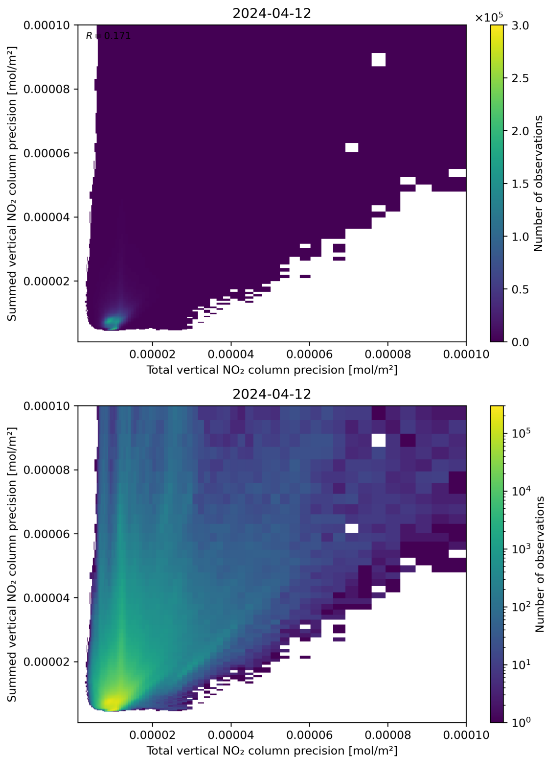
Figure 118: Scatter density plot of “Total vertical NO 2 column precision” against “Summed vertical NO 2 column precision” for 2024-04-11 to 2024-04-13.
