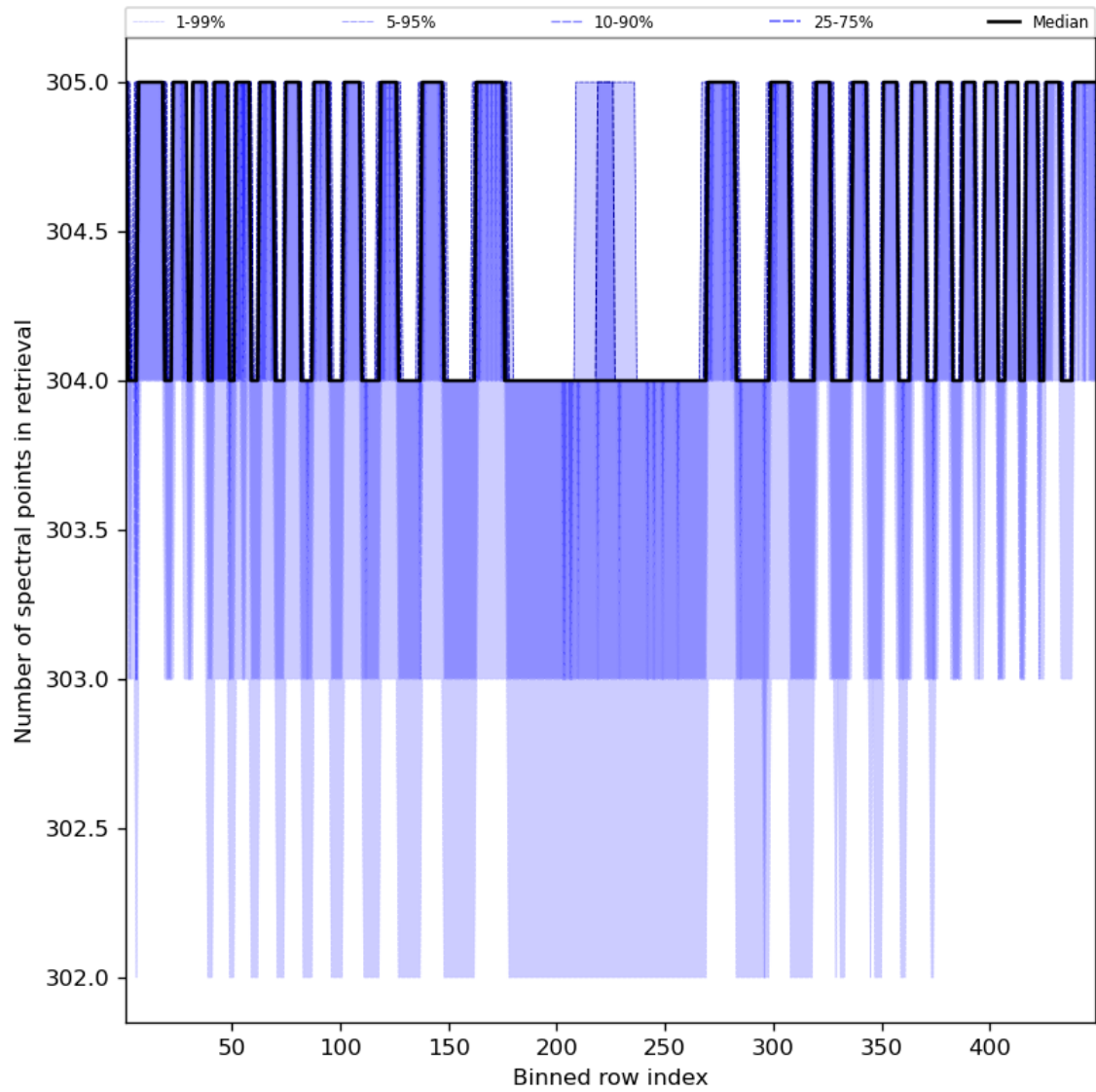
Figure 50: Along track statistics of “Number of spectral points in retrieval” for 2024-04-11 to 2024-04-13
