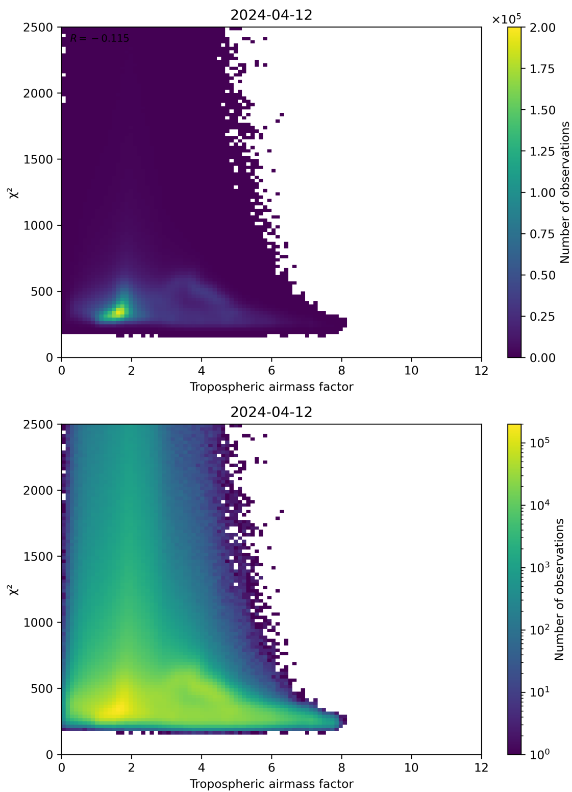
Figure 73: Scatter density plot of “Tropospheric airmass factor” against “ \chi^2 ” for 2024-04-11 to 2024-04-13.
