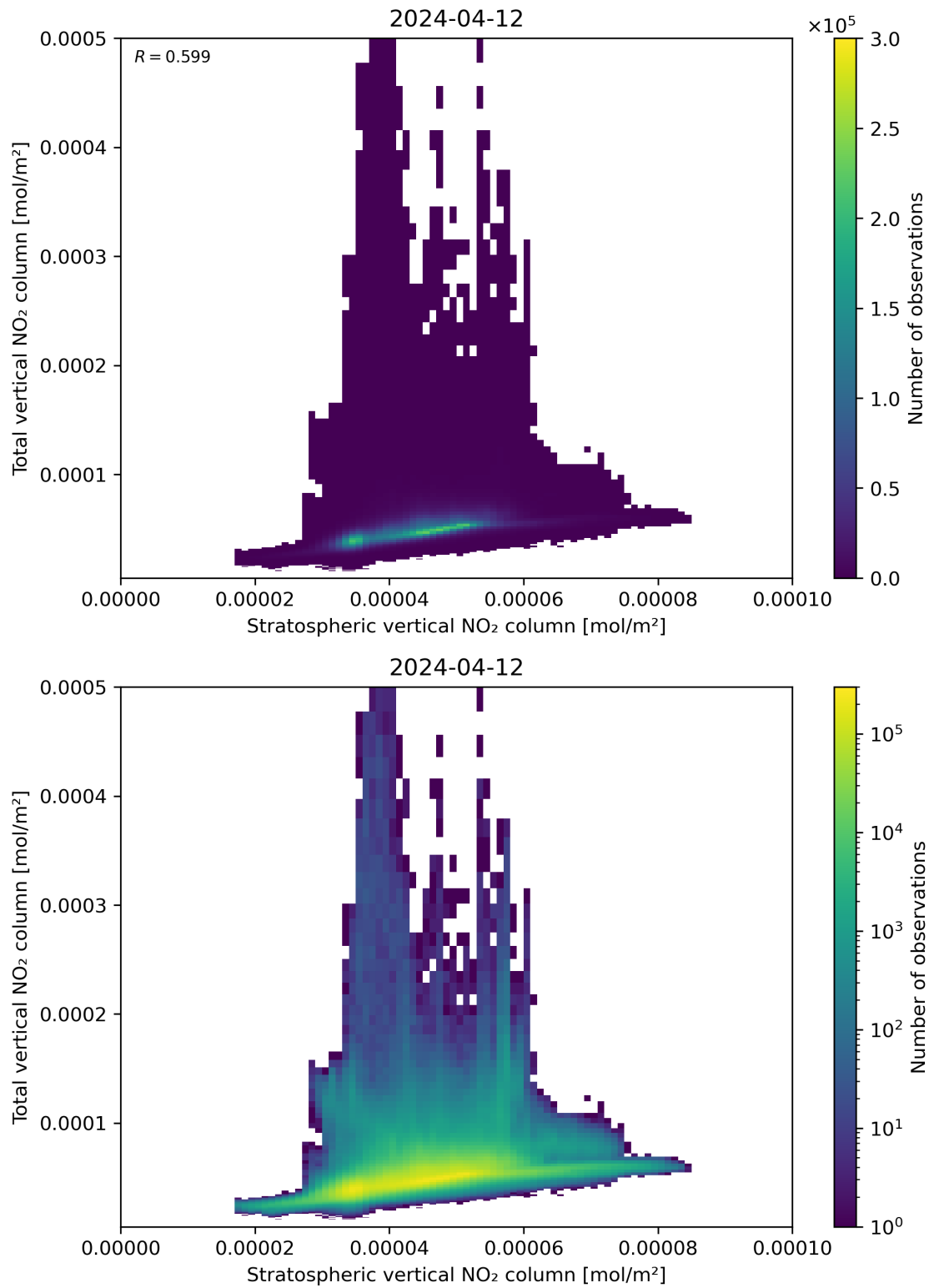
Figure 100: Scatter density plot of “Stratospheric vertical NO 2 column” against “Total vertical NO 2 column” for 2024-04-11 to 2024-04-13.
