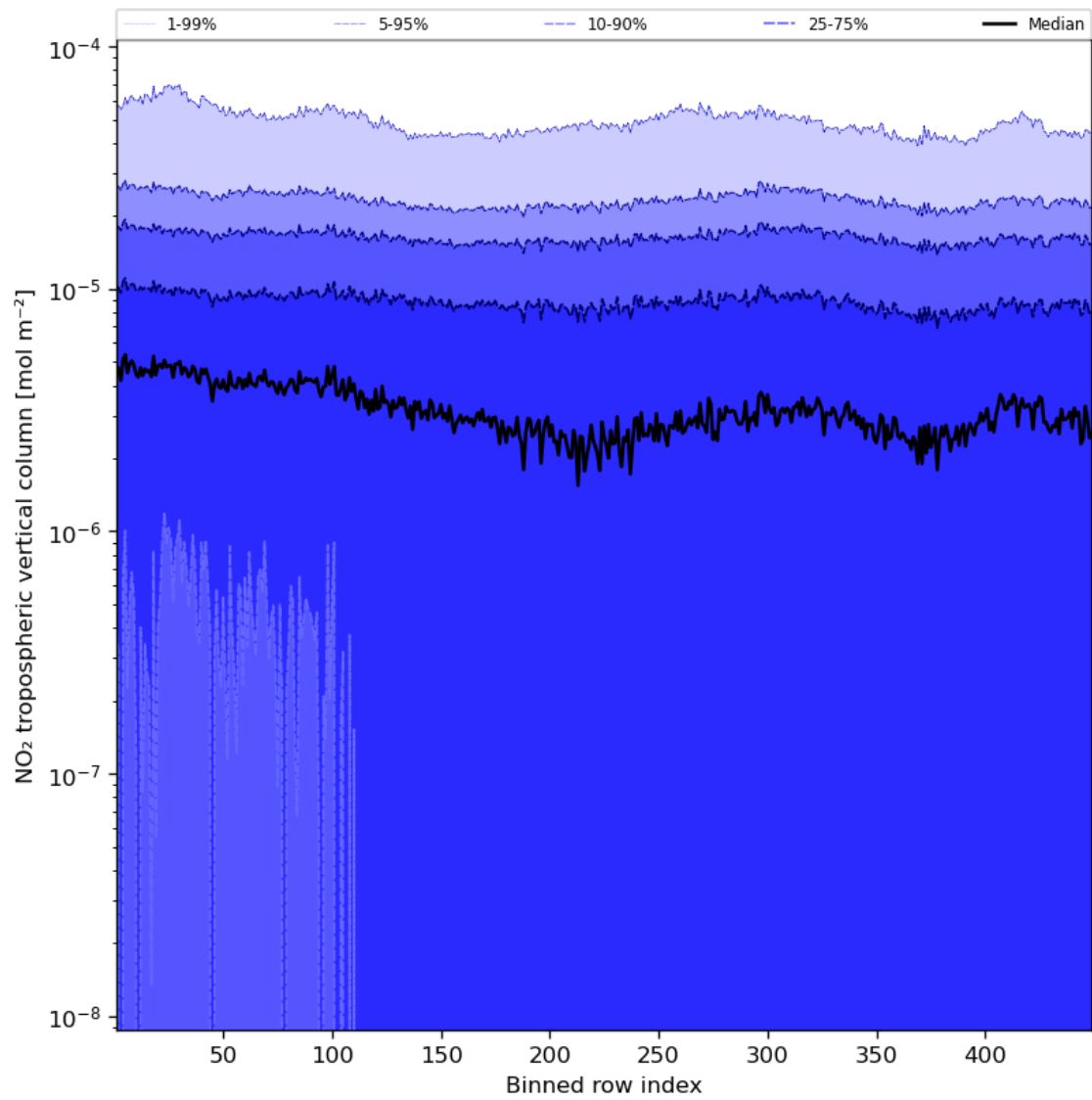
Figure 46: Along track statistics of “NO 2 tropospheric vertical column” for 2024-04-11 to 2024-04-13
