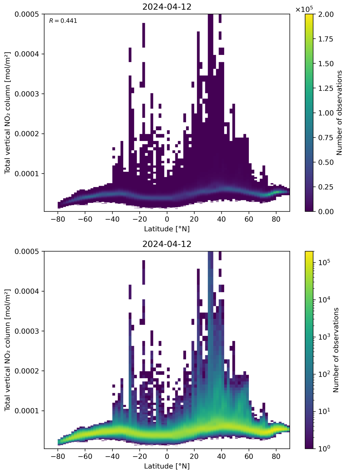
Figure 90: Scatter density plot of “Latitude” against “Total vertical NO 2 column” for 2024-04-11 to 2024-04-13.
