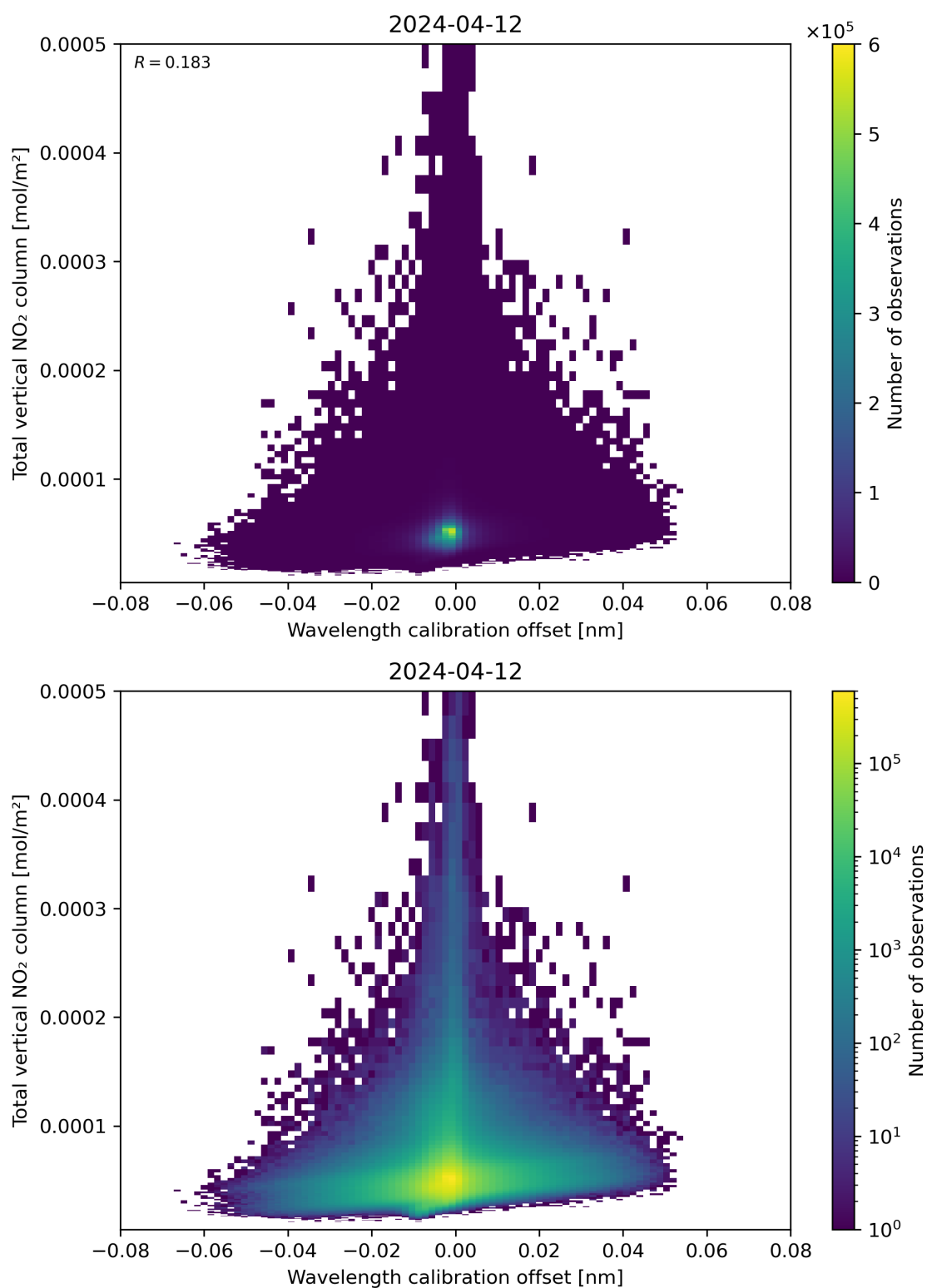
Figure 179: Scatter density plot of “Wavelength calibration offset” against “Total vertical NO 2 column” for 2024-04-11 to 2024-04-13.
