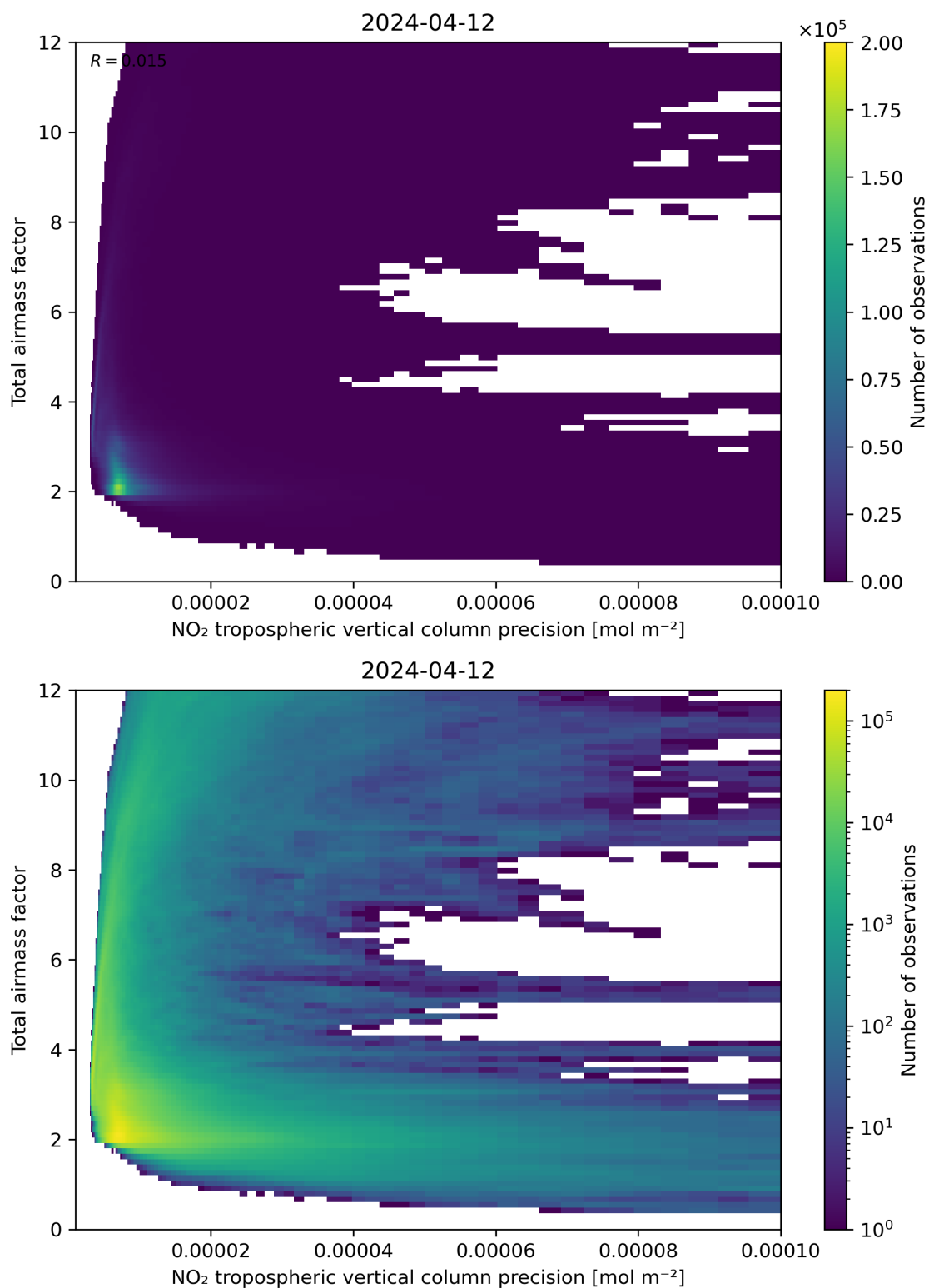
Figure 132: Scatter density plot of “NO 2 tropospheric vertical column precision” against “Total air mass factor” for 2024-04-11 to 2024-04-13.
