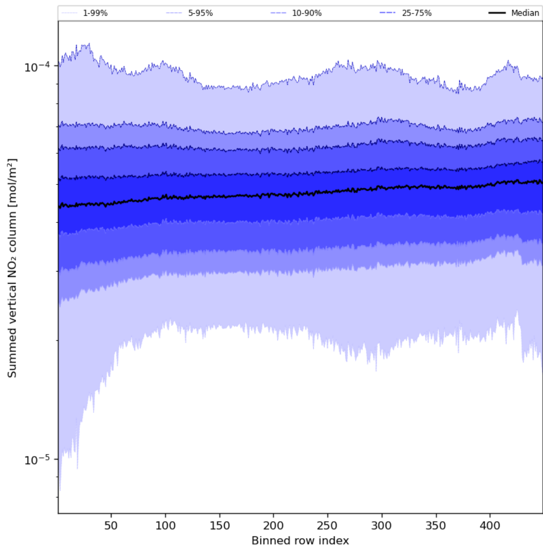
Figure 57: Along track statistics of “Summed vertical NO 2 column” for 2024-04-11 to 2024-04-13
