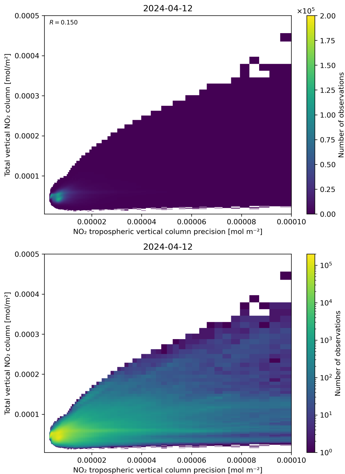
Figure 138: Scatter density plot of “NO 2 tropospheric vertical column precision” against “Total vertical NO 2 column” for 2024-04-11 to 2024-04-13.
