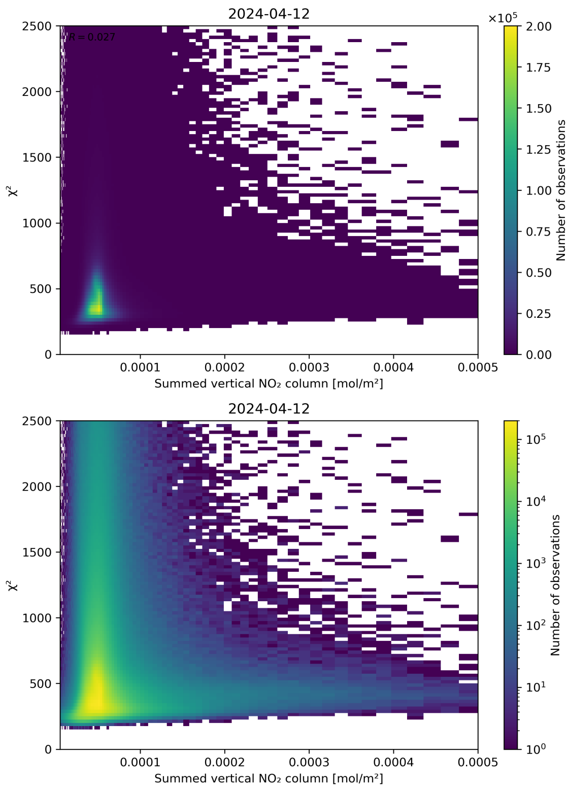
Figure 104: Scatter density plot of “Summed vertical NO 2 column” against “ \chi^2 ” for 2024-04-11 to 2024-04-13.
