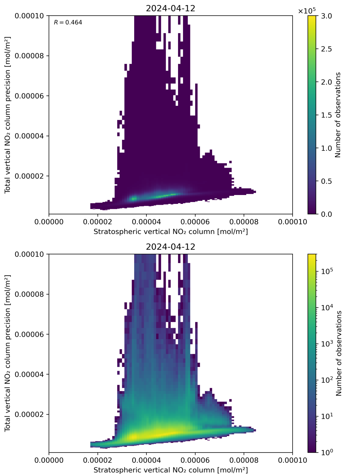
Figure 101: Scatter density plot of “Stratospheric vertical NO 2 column” against “Total vertical NO 2 column precision” for 2024-04-11 to 2024-04-13.
