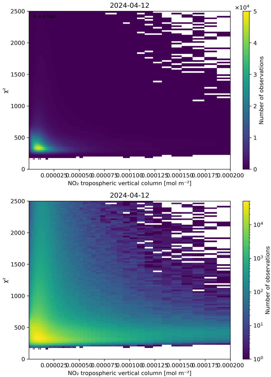
Figure 124: Scatter density plot of “NO 2 tropospheric vertical column” against “ \chi^2 ” for 2024-04-11 to 2024-04-13.
