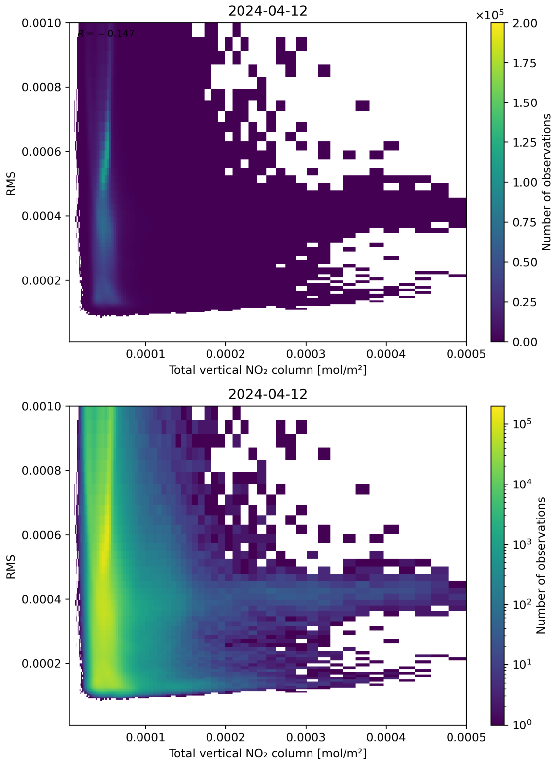
Figure 120: Scatter density plot of “Total vertical NO 2 column” against “RMS” for 2024-04-11 to 2024-04-13.
