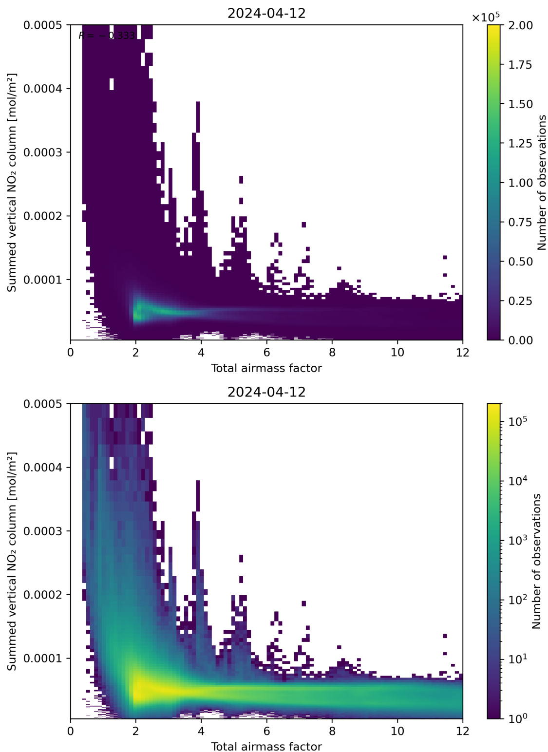
Figure 65: Scatter density plot of “Total airmass factor” against “Summed vertical NO 2 column” for 2024-04-11 to 2024-04-13.
