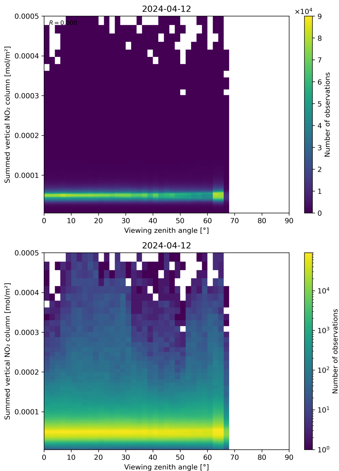
Figure 165: Scatter density plot of “Viewing zenith angle” against “Summed vertical NO 2 column” for 2024-04-11 to 2024-04-13.
