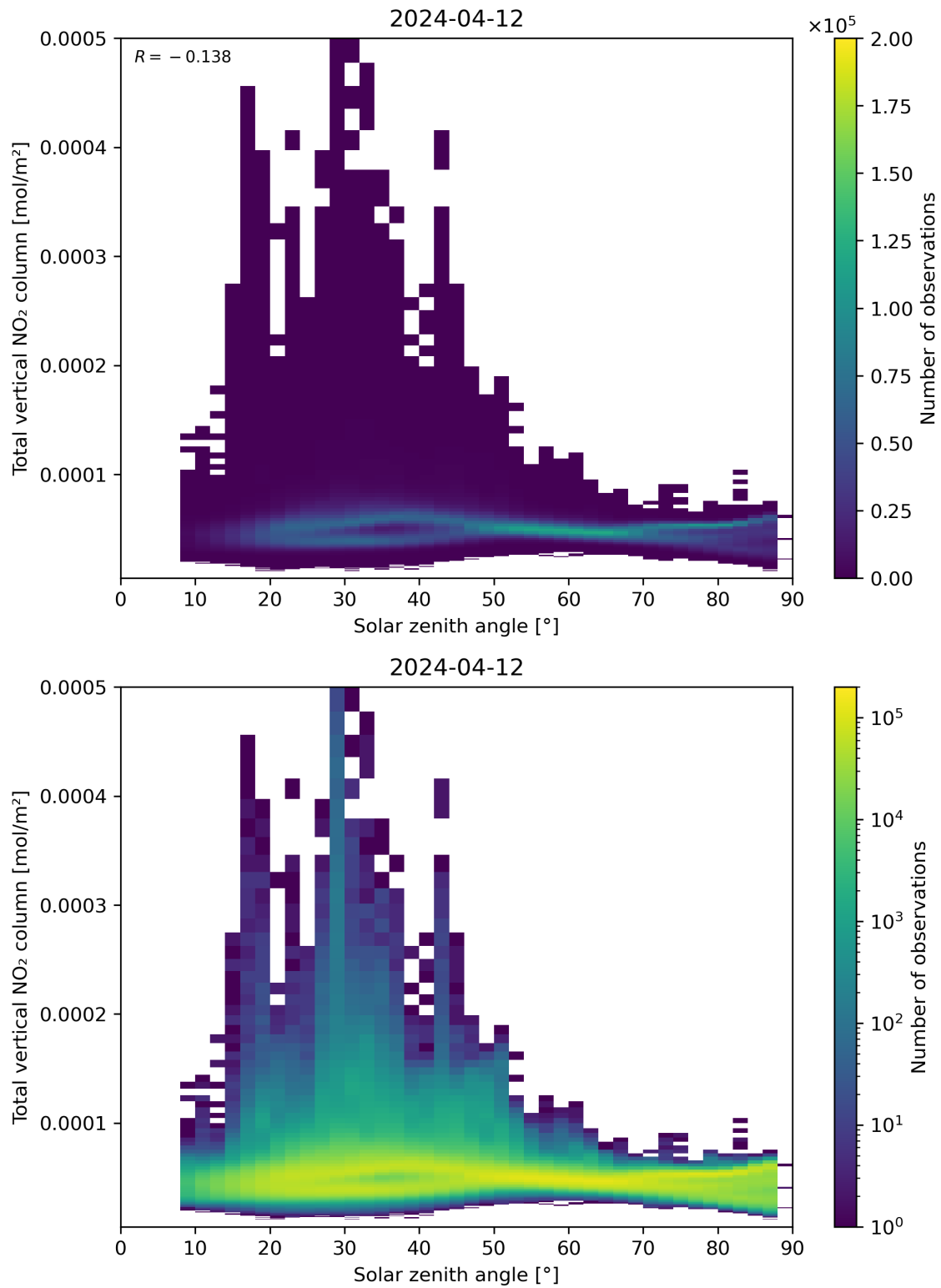
Figure 153: Scatter density plot of “Solar zenith angle” against “Total vertical NO 2 column” for 2024-04-11 to 2024-04-13.
