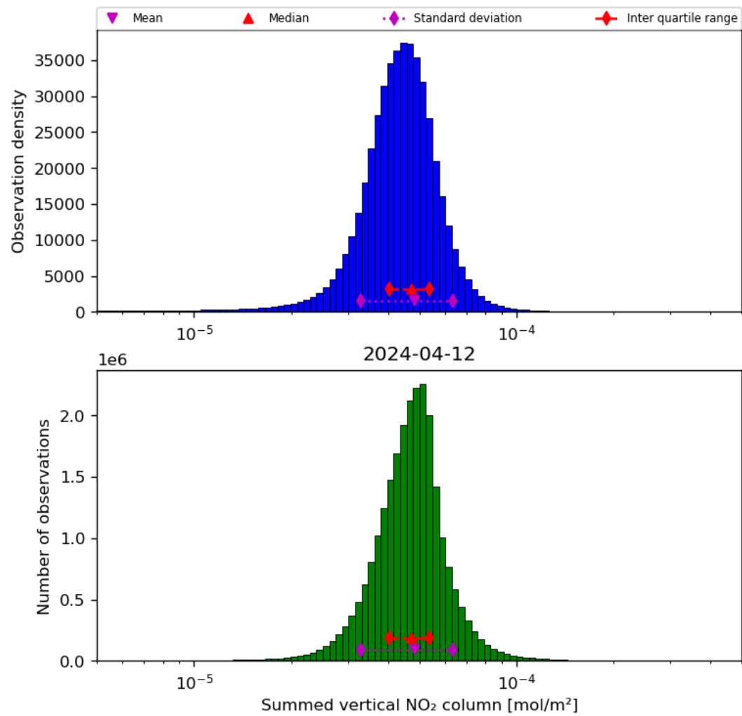
Figure 40: Histogram of “Summed vertical NO 2 column” for 2024-04-11 to 2024-04-13
