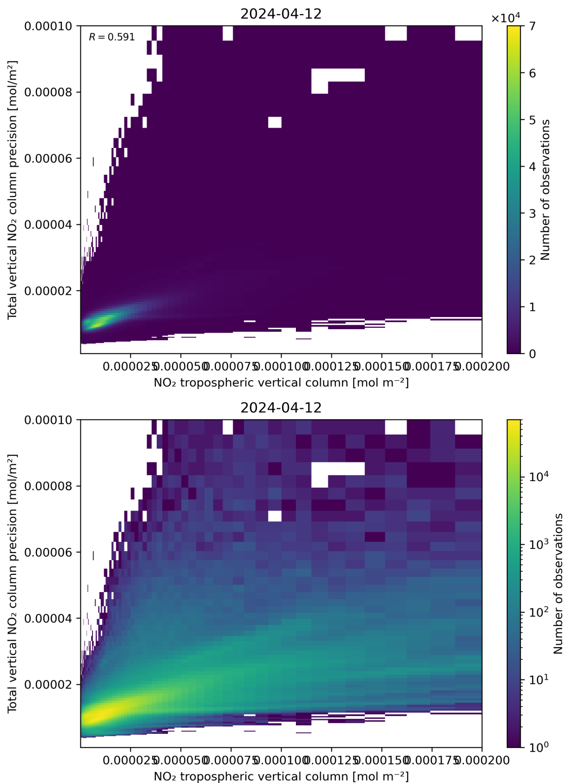
Figure 129: Scatter density plot of “NO 2 tropospheric vertical column” against “Total vertical NO 2 column precision” for 2024-04-11 to 2024-04-13.
