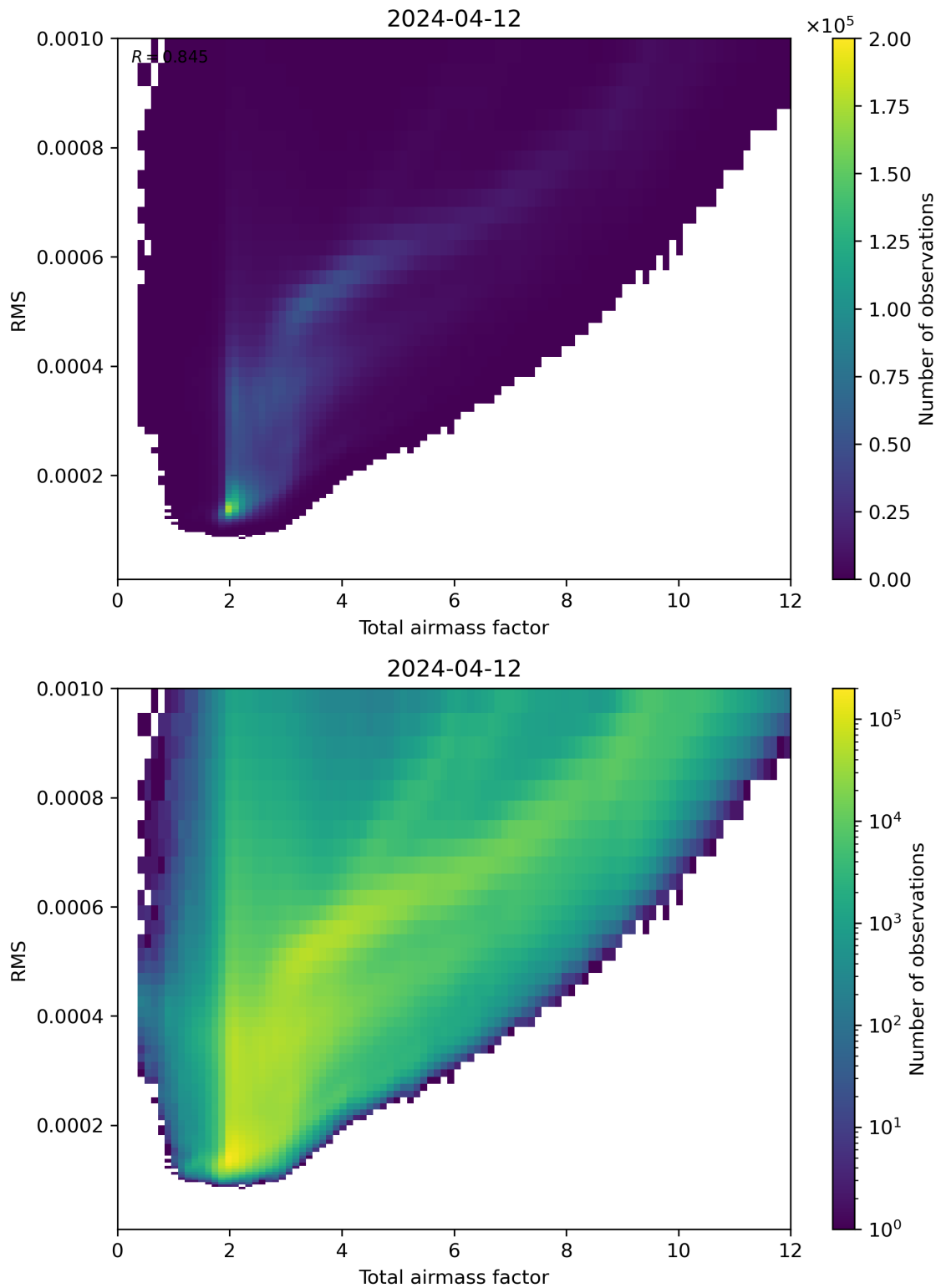
Figure 69: Scatter density plot of “Total airmass factor” against “RMS” for 2024-04-11 to 2024-04-13.
