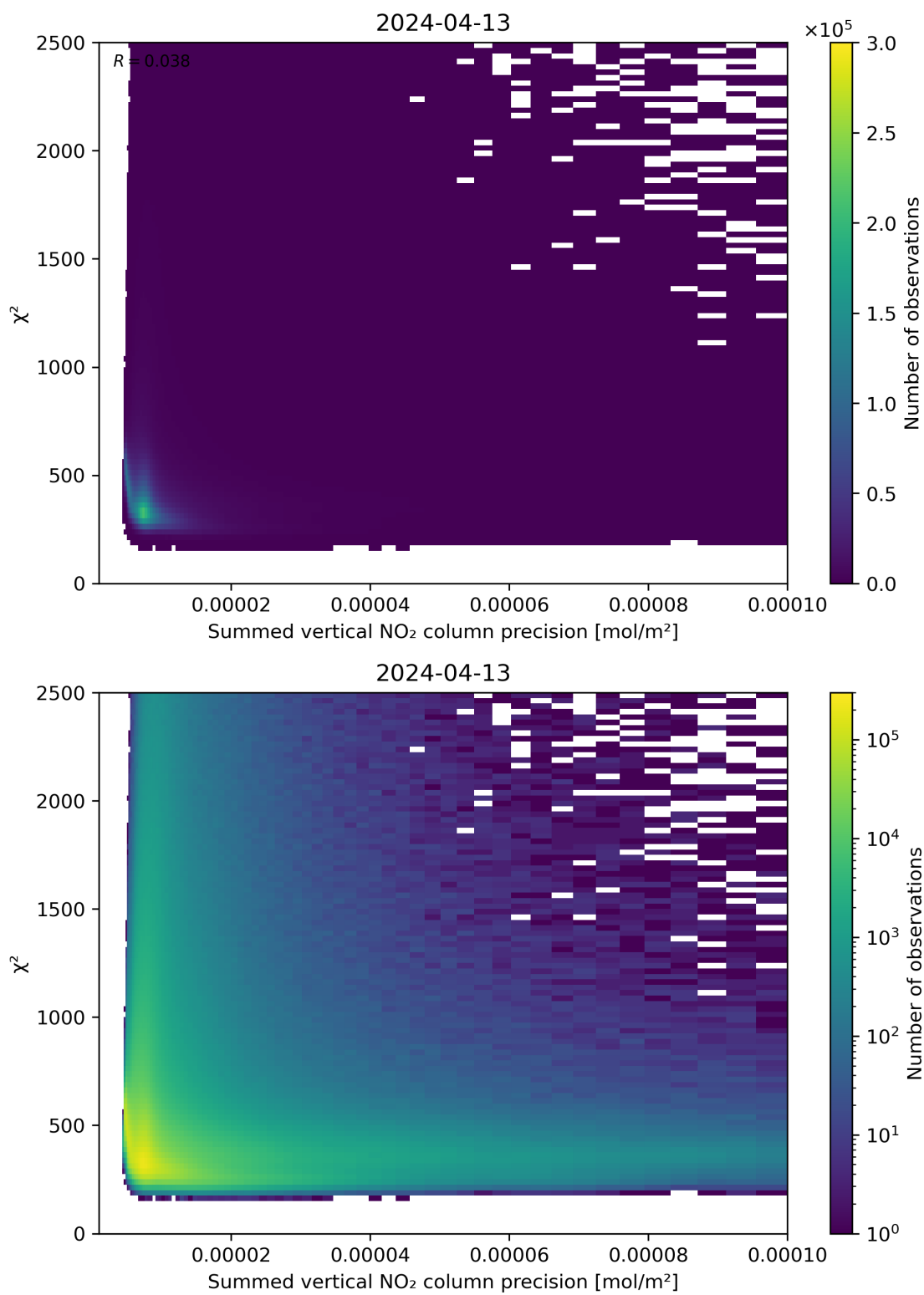
Figure 107: Scatter density plot of “Summed vertical NO 2 column precision” against “ \chi^2 ” for 2024-04-12 to 2024-04-14.
