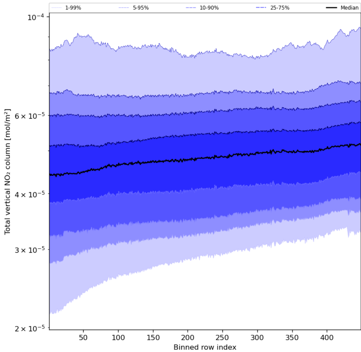
Figure 55: Along track statistics of “Total vertical NO 2 column” for 2024-04-12 to 2024-04-14
