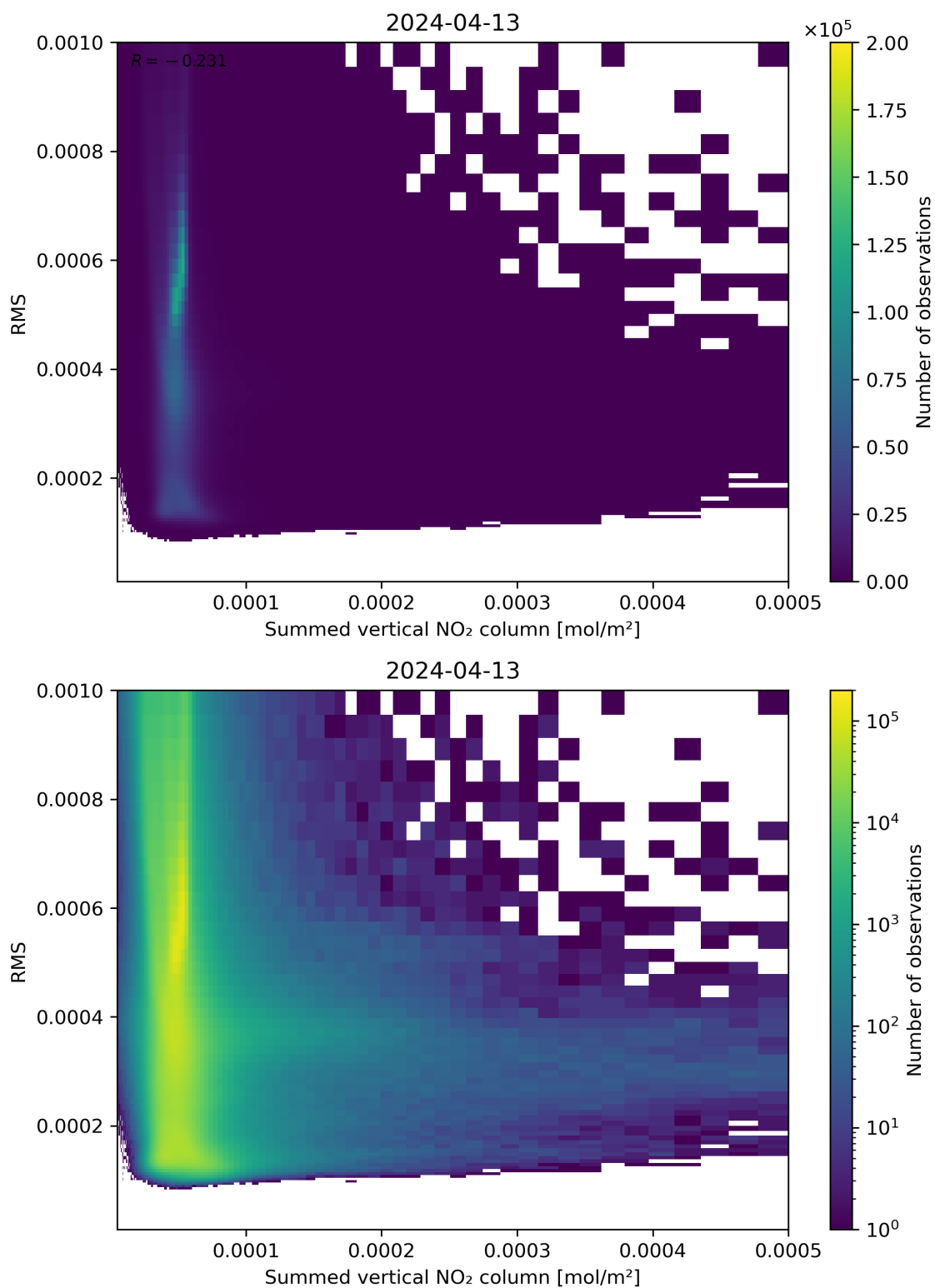
Figure 109: Scatter density plot of “Summed vertical NO 2 column” against “RMS” for 2024-04-12 to 2024-04-14.
