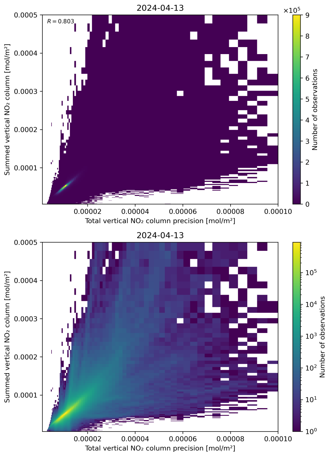
Figure 117: Scatter density plot of “Total vertical NO 2 column precision” against “Summed vertical NO 2 column” for 2024-04-12 to 2024-04-14.
