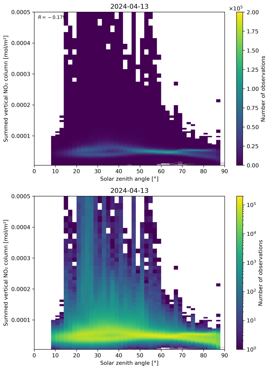
Figure 151: Scatter density plot of “Solar zenith angle” against “Summed vertical NO 2 column” for 2024-04-12 to 2024-04-14.
