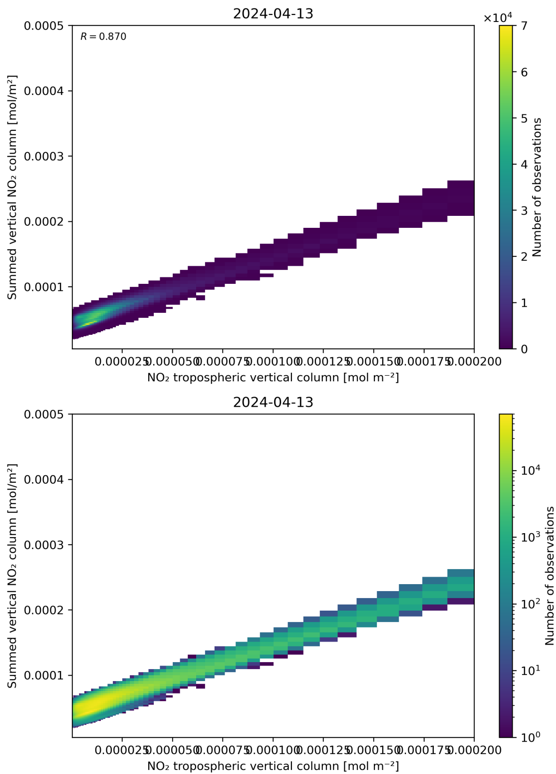
Figure 126: Scatter density plot of “NO 2 tropospheric vertical column” against “Summed vertical NO 2 column” for 2024-04-12 to 2024-04-14.
