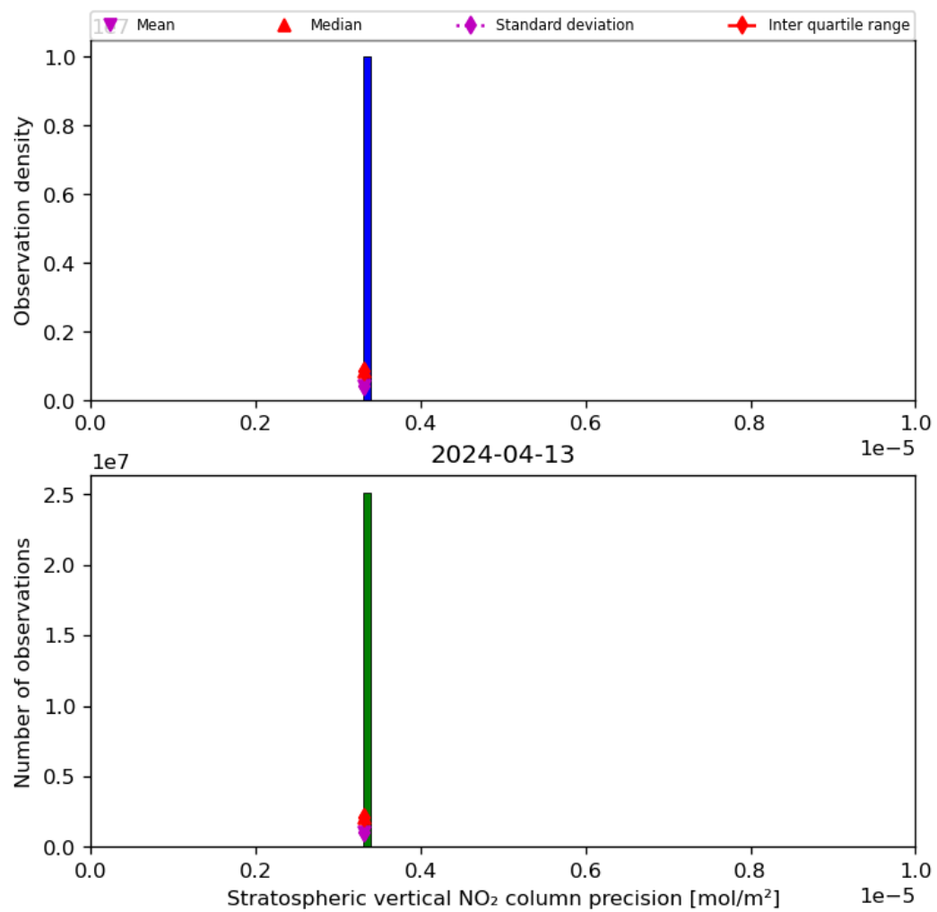
Figure 37: Histogram of “Stratospheric vertical NO 2 column precision” for 2024-04-12 to 2024-04-14
