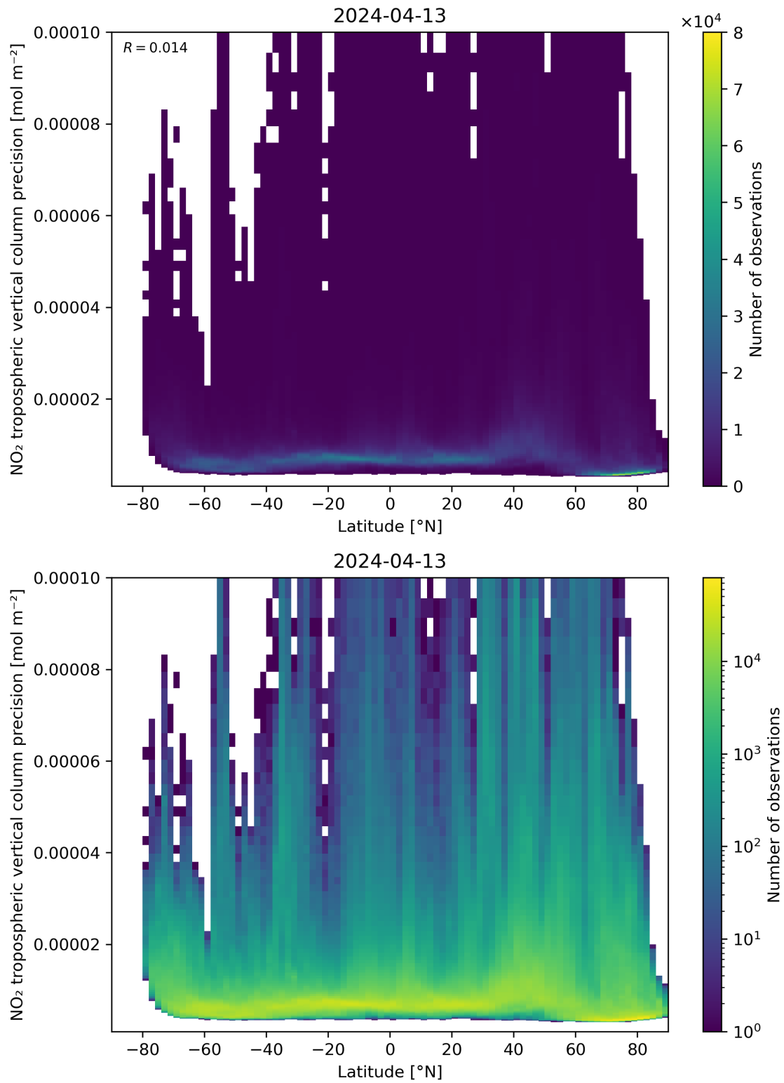
Figure 93: Scatter density plot of “Latitude” against “NO 2 tropospheric vertical column precision” for 2024-04-12 to 2024-04-14.
