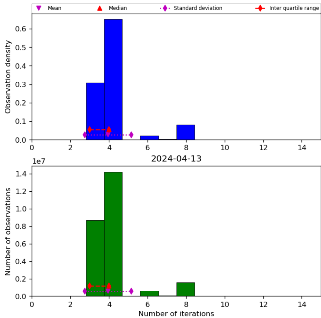
Figure 34: Histogram of “Number of iterations” for 2024-04-12 to 2024-04-14
