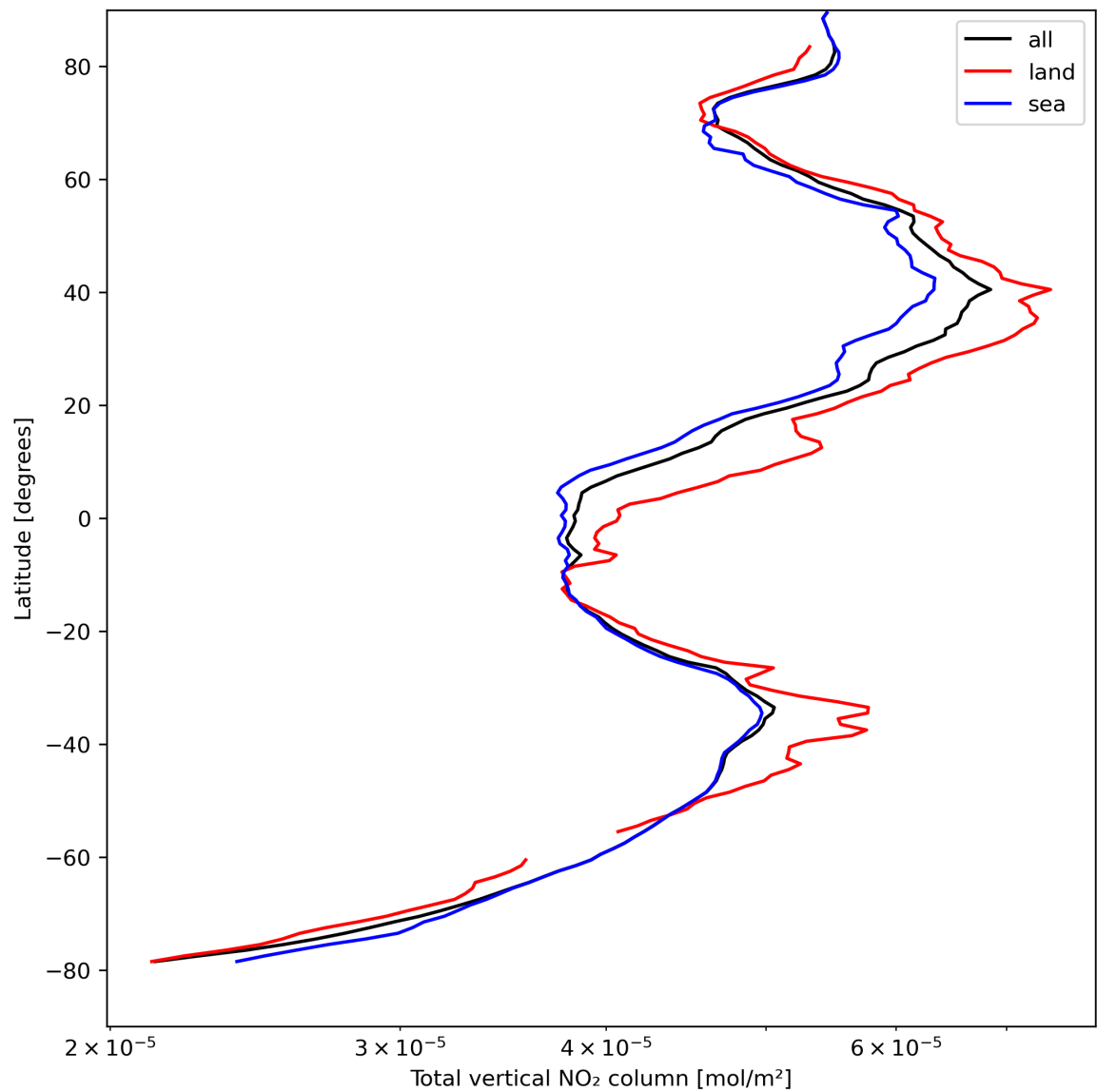
Figure 21: Zonal average of “Total vertical NO 2 column” for 2024-04-12 to 2024-04-14.
