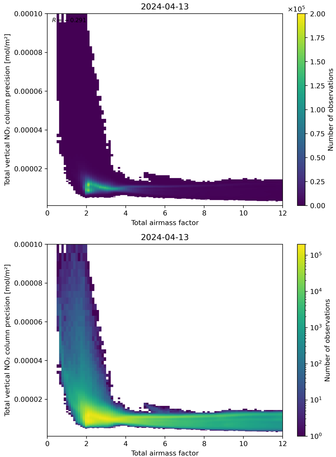
Figure 68: Scatter density plot of “Total airmass factor” against “Total vertical NO 2 column precision” for 2024-04-12 to 2024-04-14.
