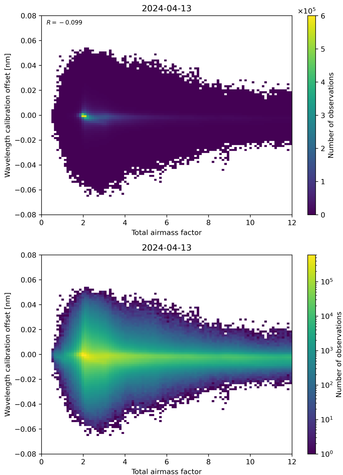
Figure 70: Scatter density plot of “Total airmass factor” against “Wavelength calibration offset” for 2024-04-12 to 2024-04-14.
