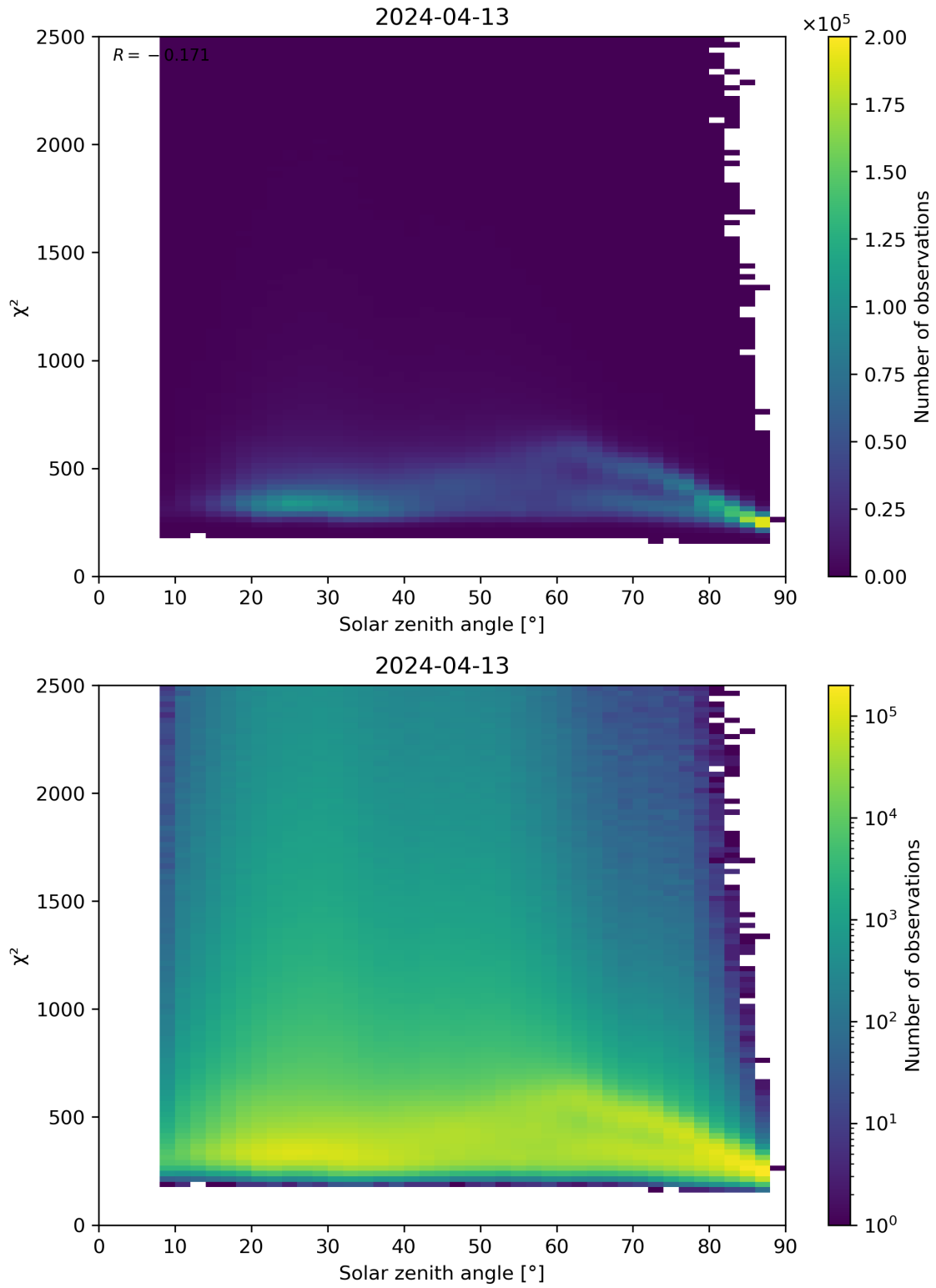
Figure 148: Scatter density plot of “Solar zenith angle” against “ \chi^2 ” for 2024-04-12 to 2024-04-14.
