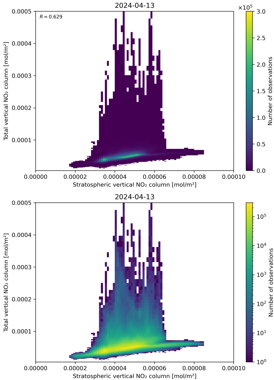
Figure 100: Scatter density plot of “Stratospheric vertical NO 2 column” against “Total vertical NO 2 column” for 2024-04-12 to 2024-04-14.
