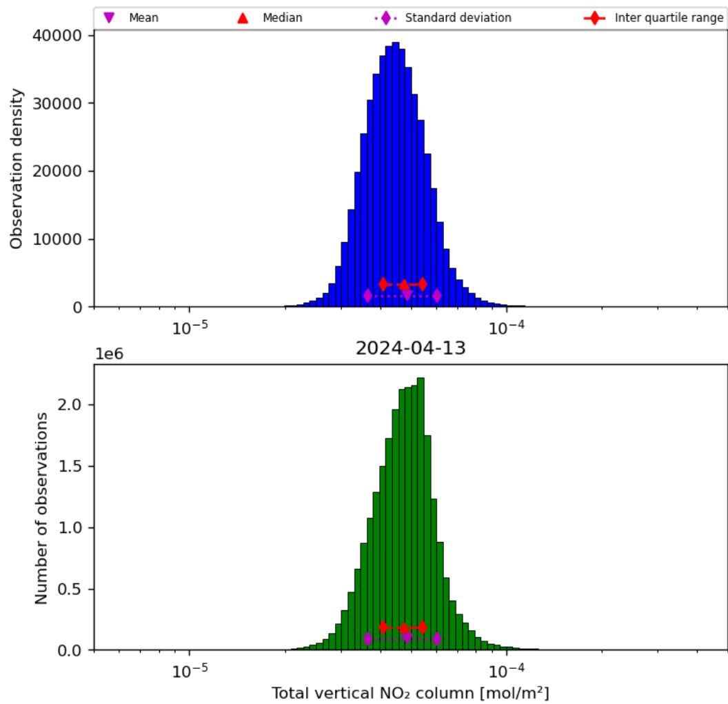
Figure 38: Histogram of "Total vertical NO 2 column" for 2024-04-12 to 2024-04-14
