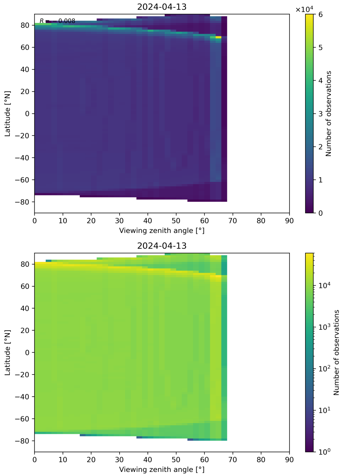
Figure 163: Scatter density plot of “Viewing zenith angle” against “Latitude” for 2024-04-12 to 2024-04-14.
