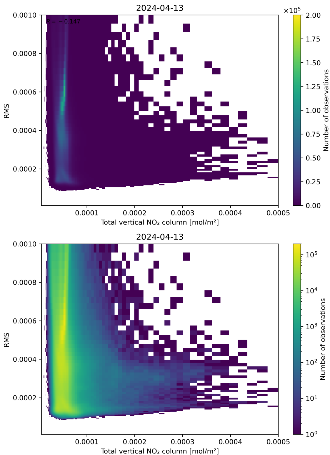
Figure 120: Scatter density plot of “Total vertical NO 2 column” against “RMS” for 2024-04-12 to 2024-04-14.
