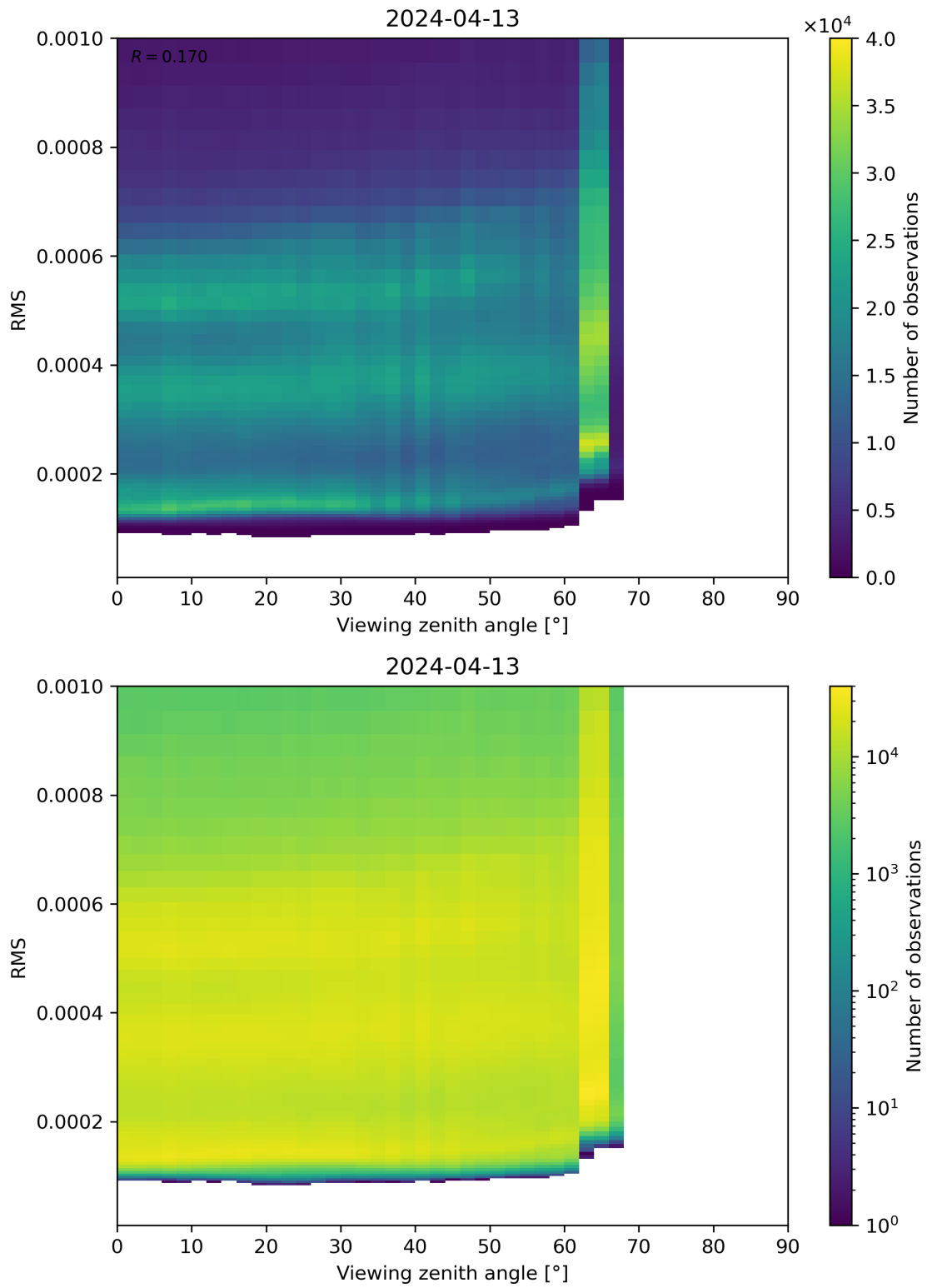
Figure 171: Scatter density plot of “Viewing zenith angle” against “RMS” for 2024-04-12 to 2024-04-14.
