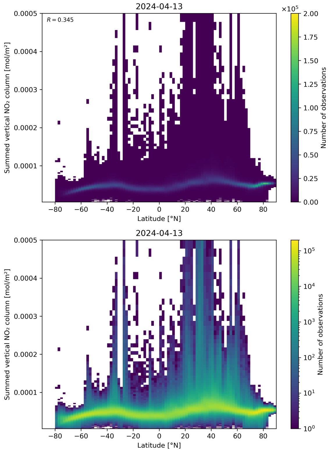
Figure 88: Scatter density plot of “Latitude” against “Summed vertical NO 2 column” for 2024-04-12 to 2024-04-14.
