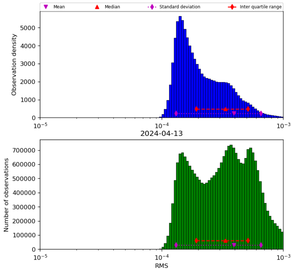
Figure 43: Histogram of “RMS” for 2024-04-12 to 2024-04-14
