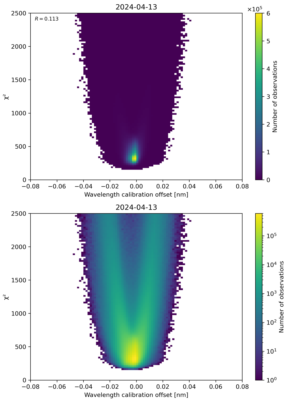
Figure 175: Scatter density plot of “Wavelength calibration offset” against “ \chi^2 ” for 2024-04-12 to 2024-04-14.
