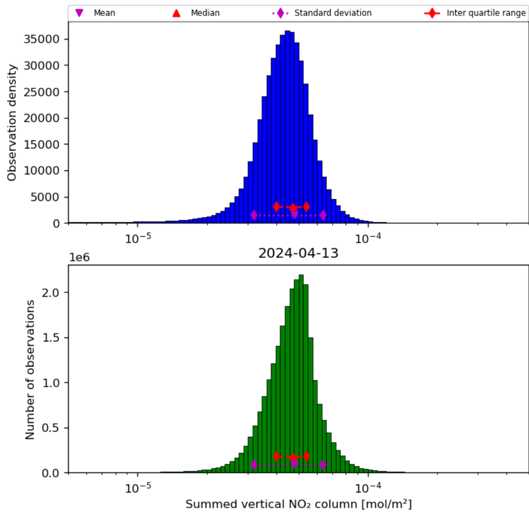
Figure 40: Histogram of "Summed vertical NO 2 column" for 2024-04-12 to 2024-04-14
