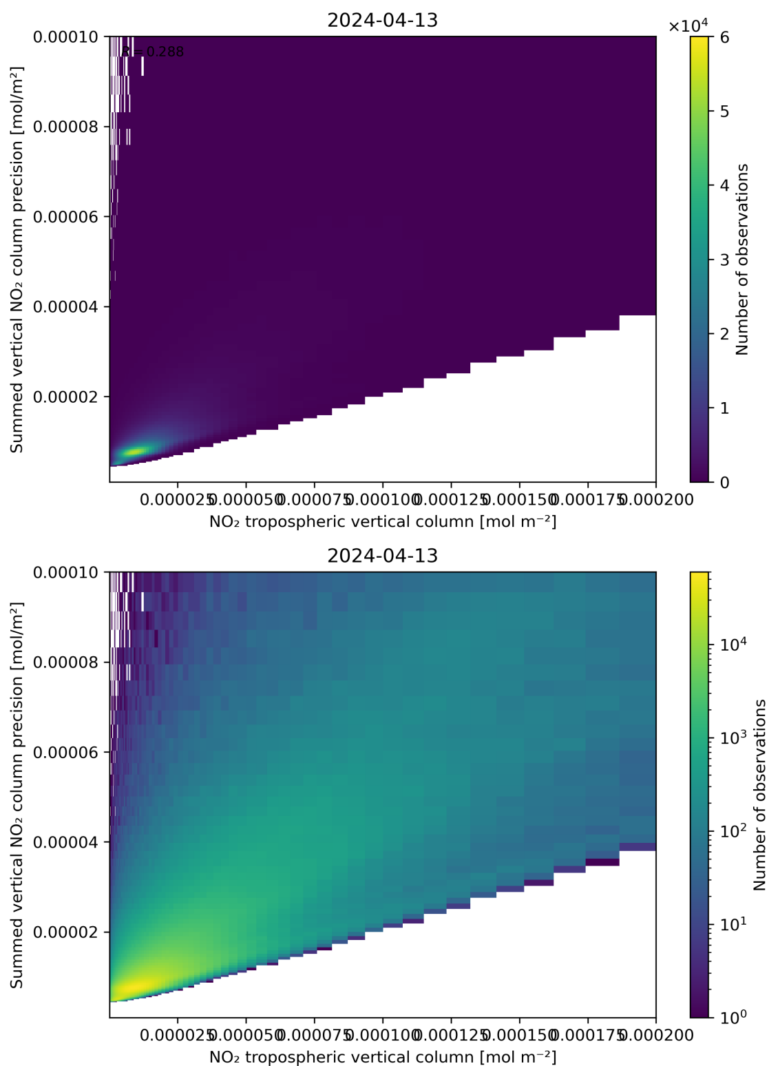
Figure 127: Scatter density plot of “NO 2 tropospheric vertical column” against “Summed vertical NO 2 column precision” for 2024-04-12 to 2024-04-14.
