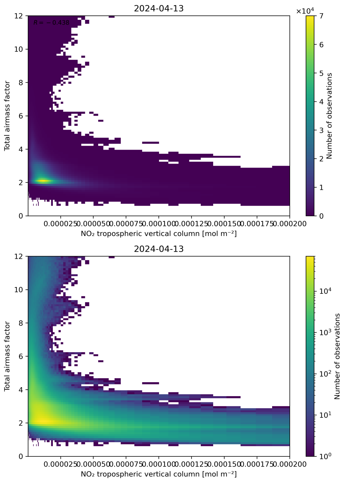
Figure 122: Scatter density plot of “NO 2 tropospheric vertical column” against “Total air mass factor” for 2024-04-12 to 2024-04-14.
