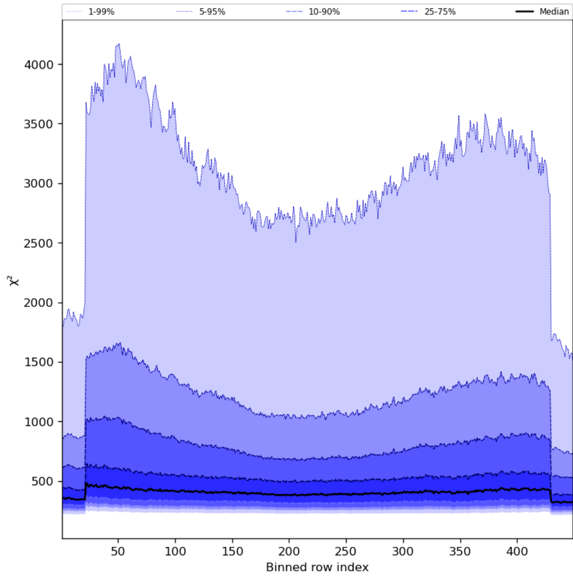
Figure 59: Along track statistics of “ \chi^2 ” for 2024-04-12 to 2024-04-14
