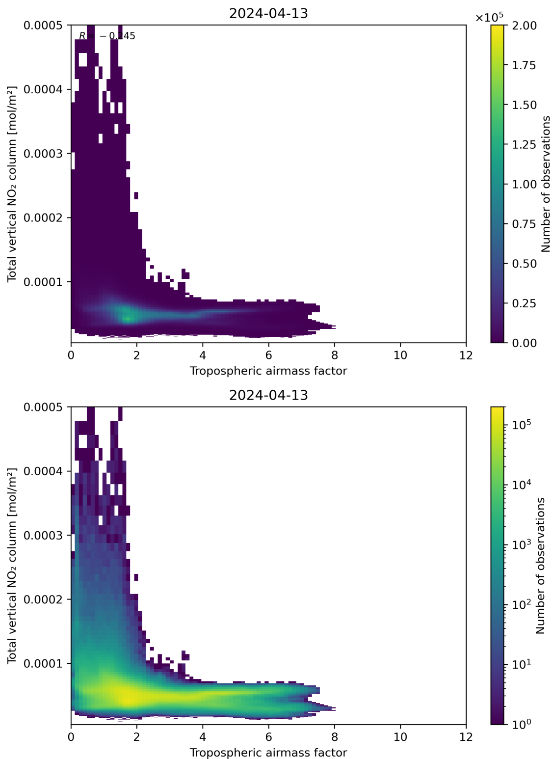
Figure 77: Scatter density plot of “Tropospheric airmass factor” against “Total vertical NO 2 column” for 2024-04-12 to 2024-04-14.
