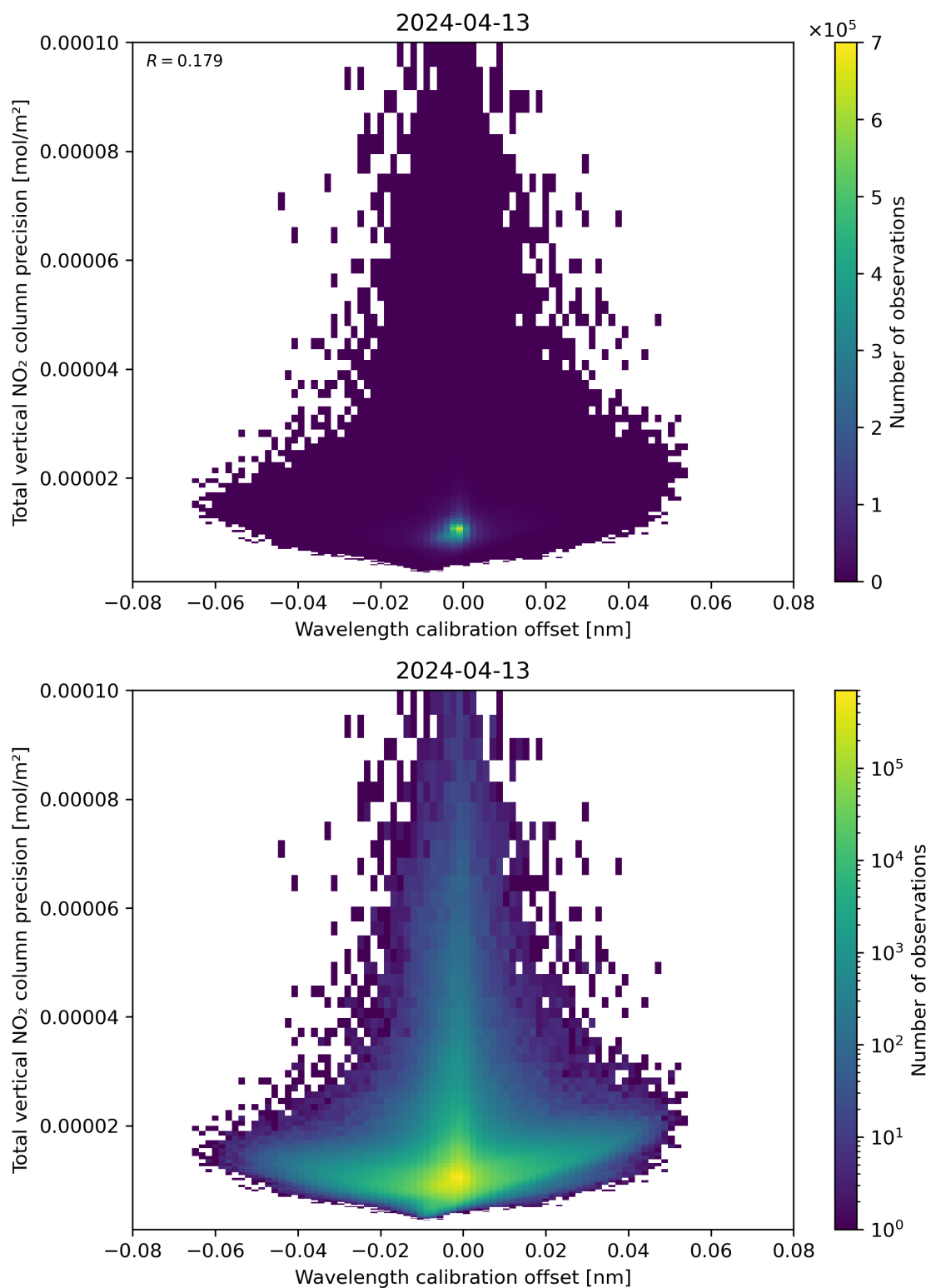
Figure 180: Scatter density plot of “Wavelength calibration offset” against “Total vertical NO 2 column precision” for 2024-04-12 to 2024-04-14.
