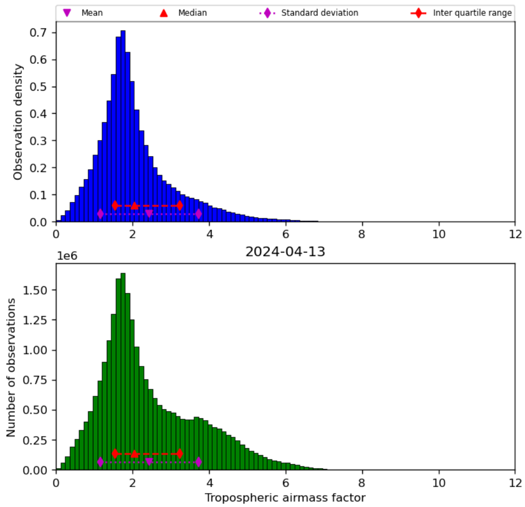
Figure 31: Histogram of “Tropospheric air mass factor” for 2024-04-12 to 2024-04-14
