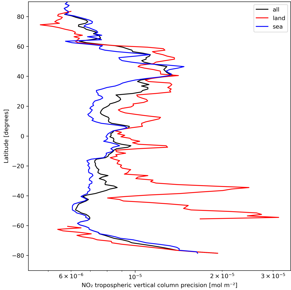
Figure 13: Zonal average of “NO 2 tropospheric vertical column precision” for 2024-04-12 to 2024-04-14.
