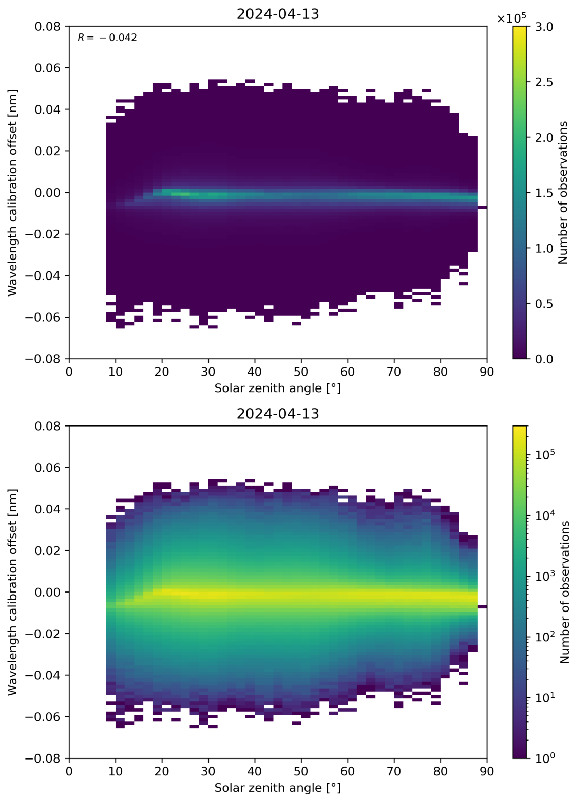
Figure 158: Scatter density plot of “Solar zenith angle” against “Wavelength calibration offset” for 2024-04-12 to 2024-04-14.
