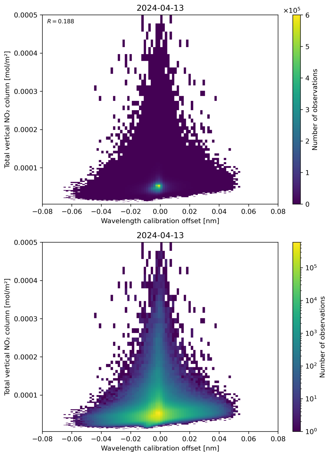
Figure 179: Scatter density plot of “Wavelength calibration offset” against “Total vertical NO 2 column” for 2024-04-12 to 2024-04-14.
