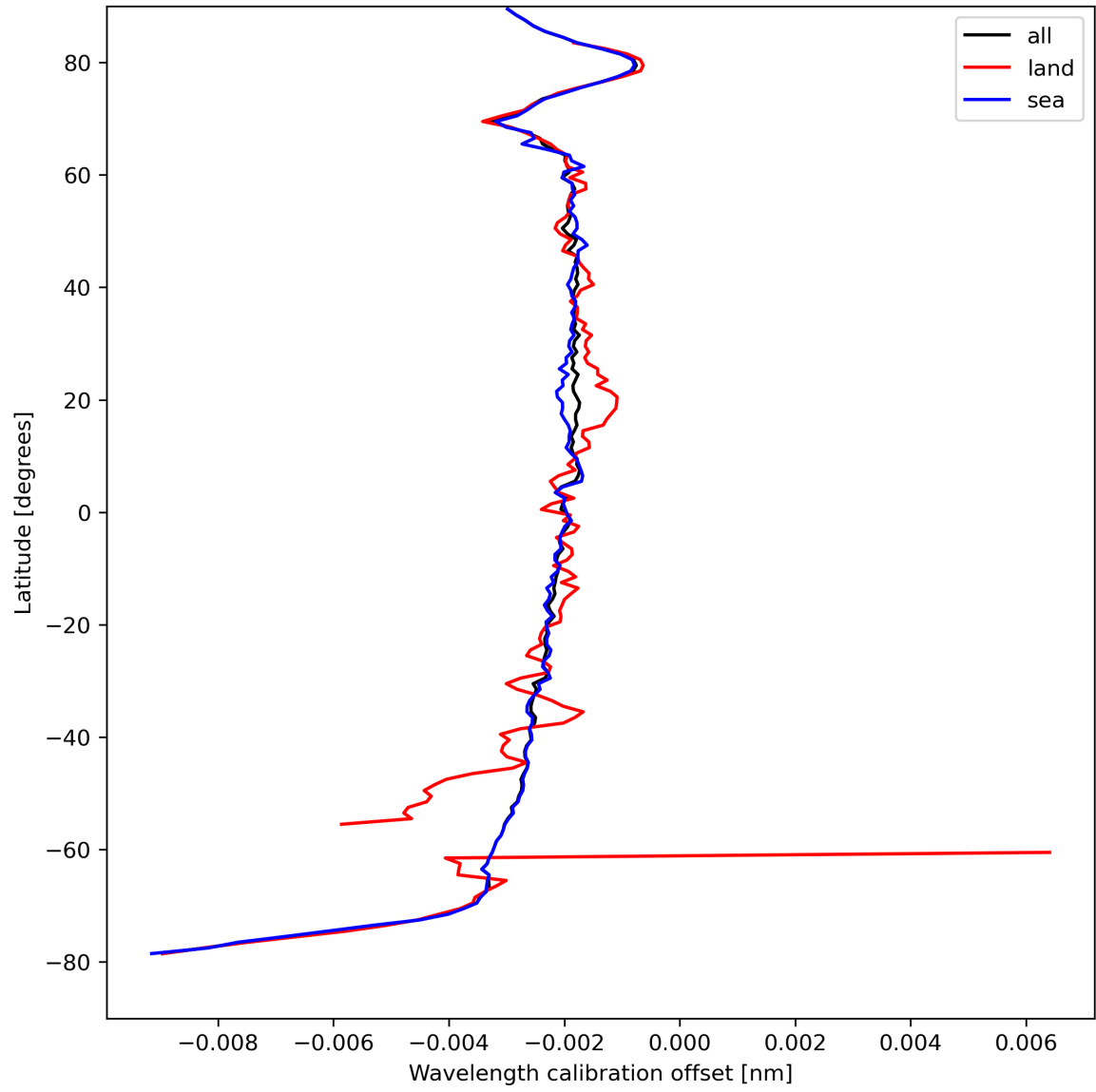
Figure 18: Zonal average of “Wavelength calibration offset” for 2024-04-12 to 2024-04-14.
