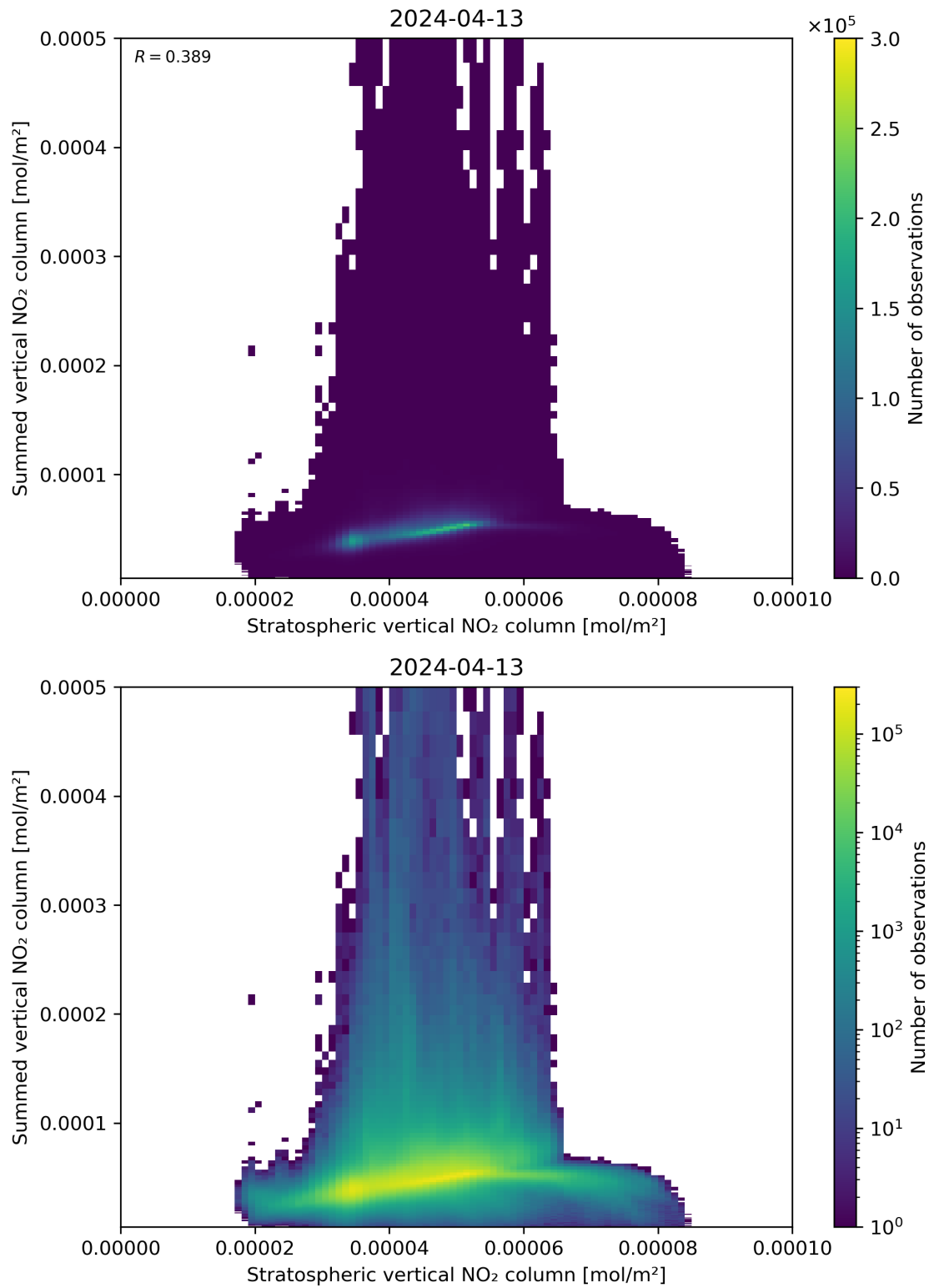
Figure 98: Scatter density plot of “Stratospheric vertical NO 2 column” against “Summed vertical NO 2 column” for 2024-04-12 to 2024-04-14.
