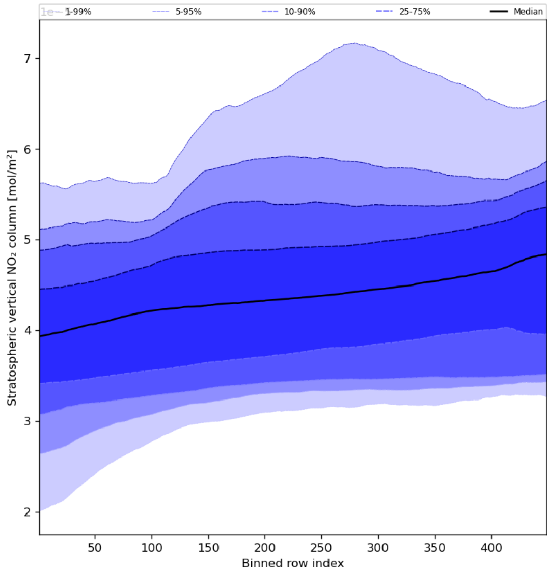
Figure 53: Along track statistics of “Stratospheric vertical NO 2 column” for 2024-04-12 to 2024-04-14
