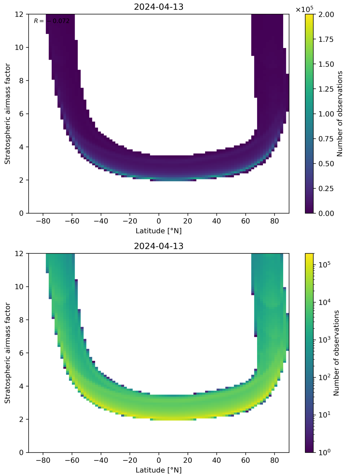
Figure 83: Scatter density plot of “Latitude” against “Stratospheric air mass factor” for 2024-04-12 to 2024-04-14.
