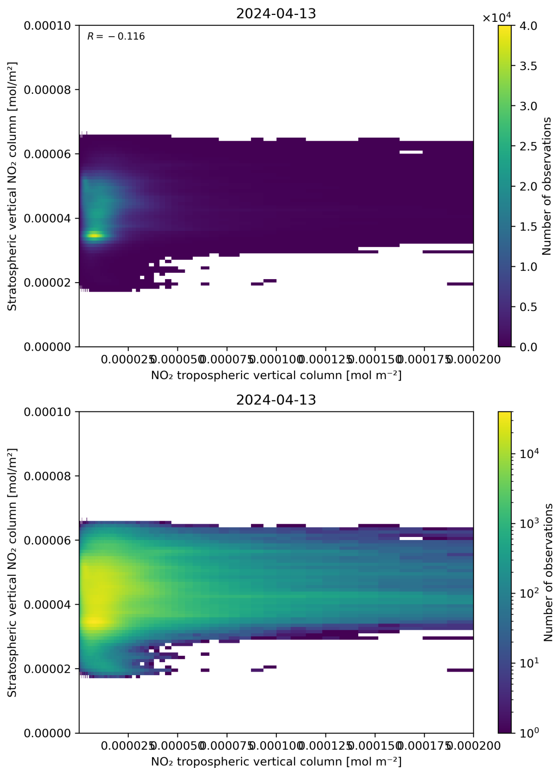
Figure 125: Scatter density plot of “NO 2 tropospheric vertical column” against “Stratospheric vertical NO 2 column” for 2024-04-12 to 2024-04-14.
