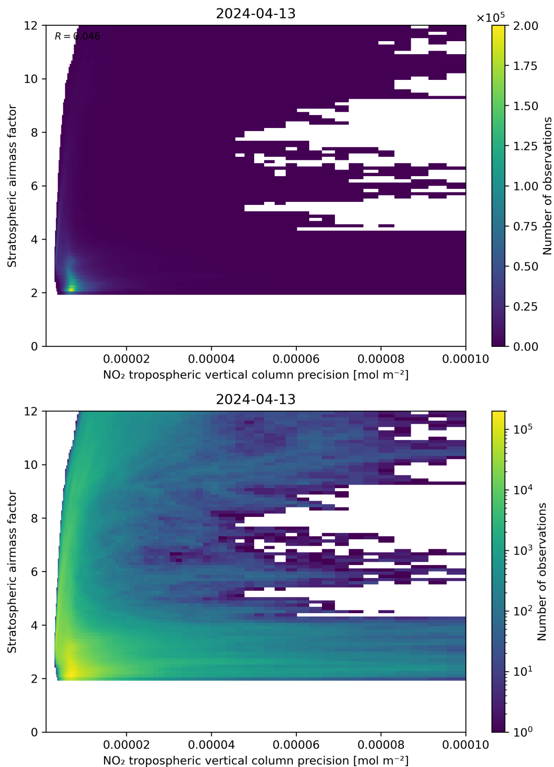
Figure 131: Scatter density plot of “NO 2 tropospheric vertical column precision” against “Stratospheric airmass factor” for 2024-04-12 to 2024-04-14.
