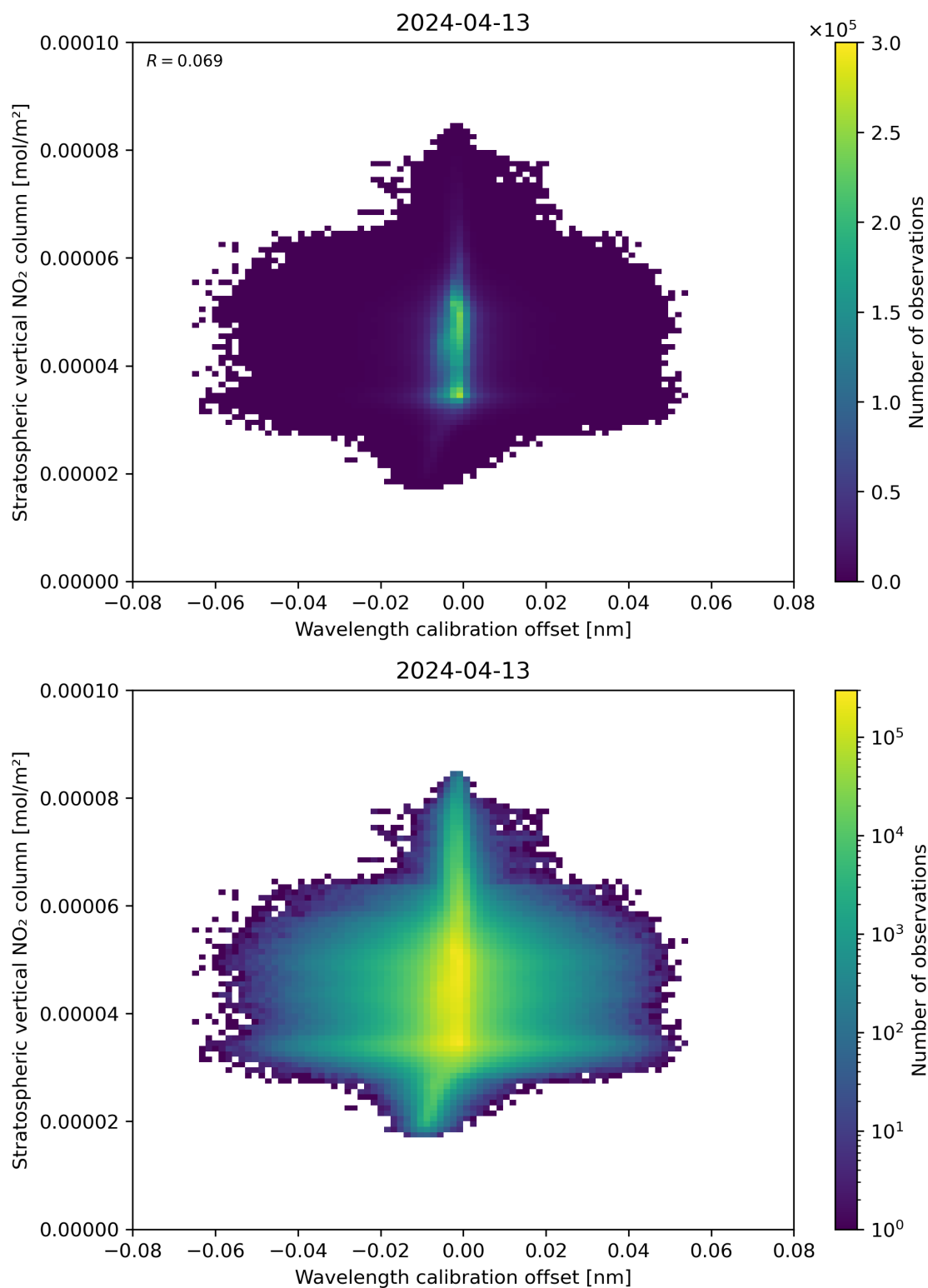
Figure 176: Scatter density plot of “Wavelength calibration offset” against “Stratospheric vertical NO 2 column” for 2024-04-12 to 2024-04-14.
