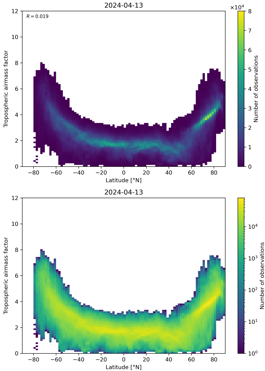
Figure 85: Scatter density plot of “Latitude” against “Tropospheric air mass factor” for 2024-04-12 to 2024-04-14.
