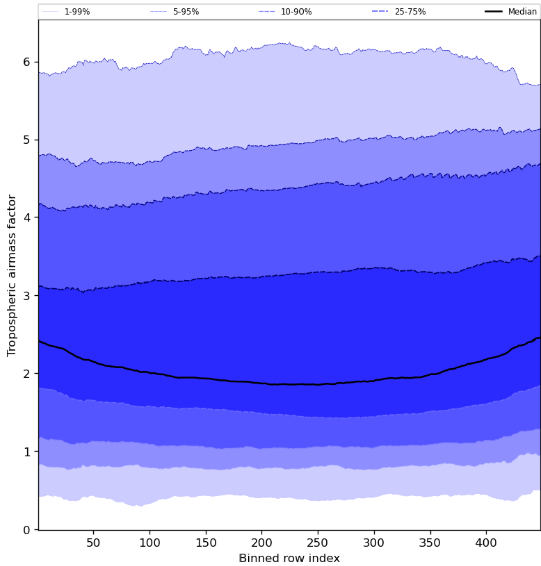
Figure 48: Along track statistics of “Tropospheric airmass factor” for 2024-04-12 to 2024-04-14
