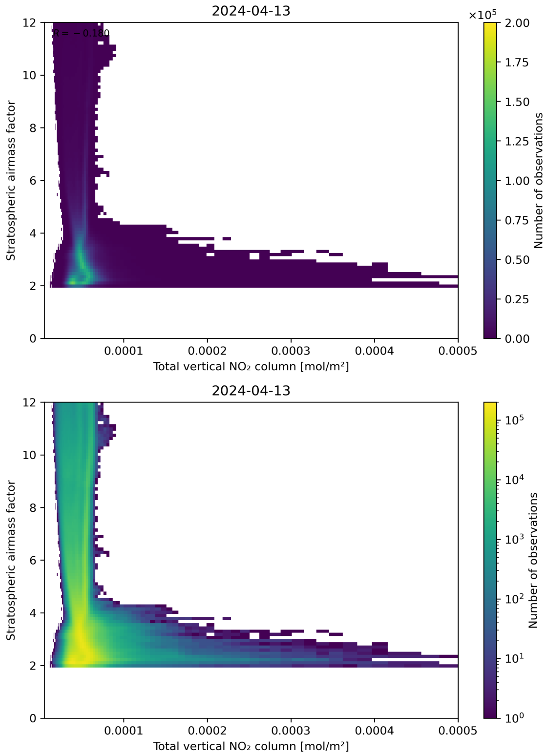
Figure 110: Scatter density plot of “Total vertical NO 2 column” against “Stratospheric airmass factor” for 2024-04-12 to 2024-04-14.
