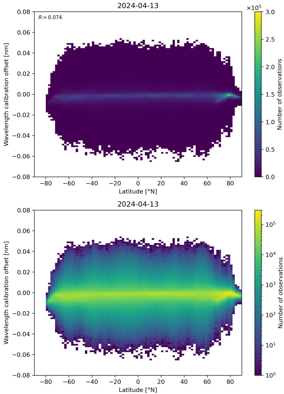
Figure 95: Scatter density plot of “Latitude” against “Wavelength calibration offset” for 2024-04-12 to 2024-04-14.
