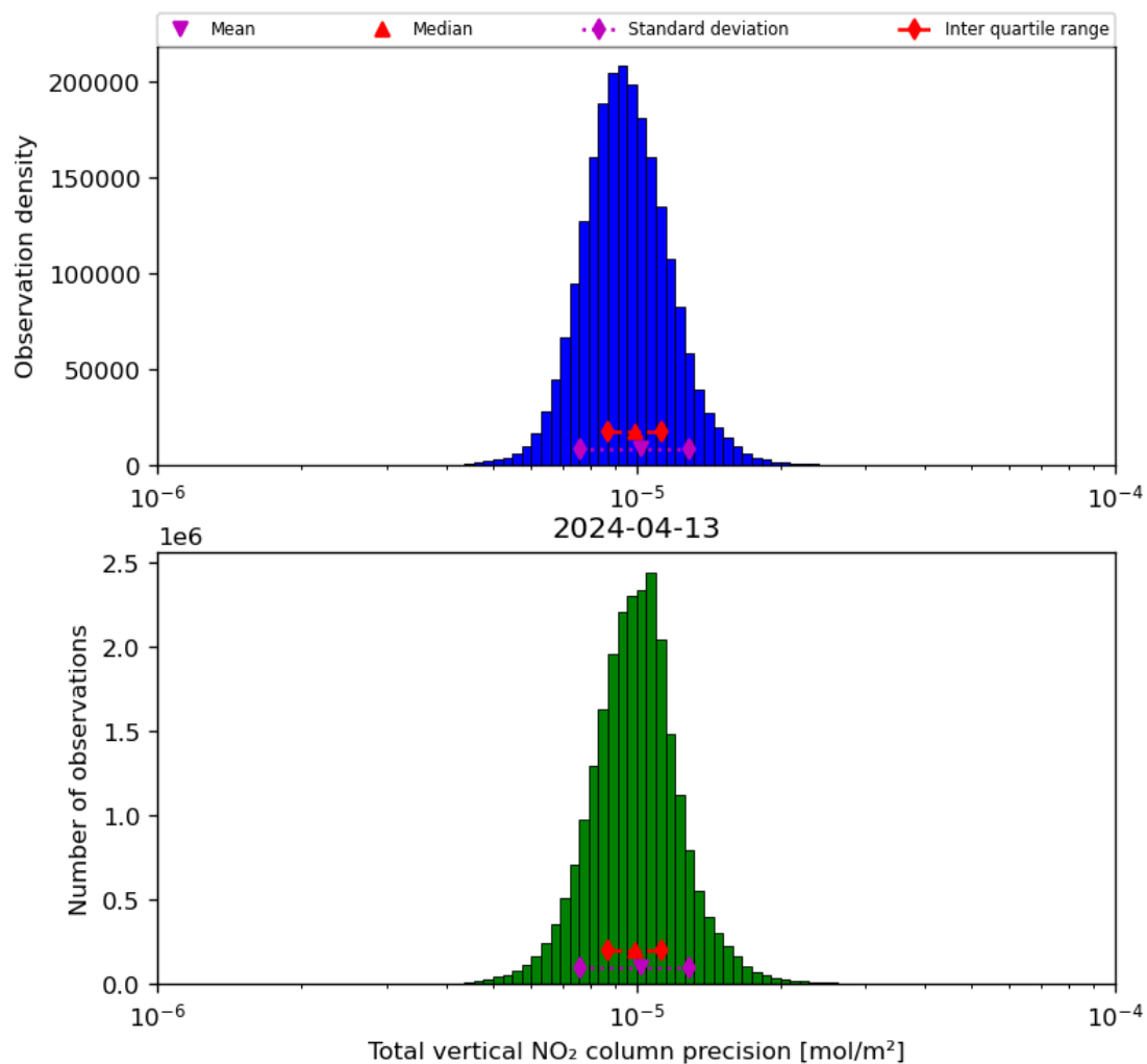
Figure 39: Histogram of “Total vertical NO 2 column precision” for 2024-04-12 to 2024-04-14
