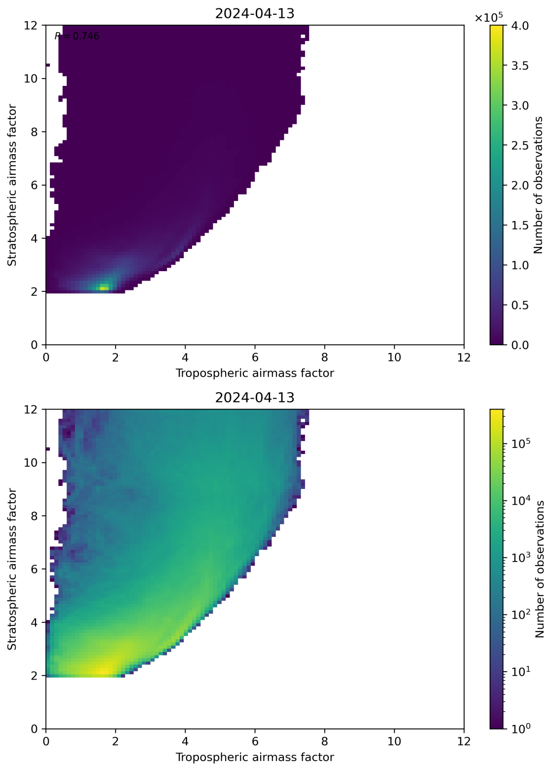
Figure 71: Scatter density plot of “Tropospheric airmass factor” against “Stratospheric airmass factor” for 2024-04-12 to 2024-04-14.
