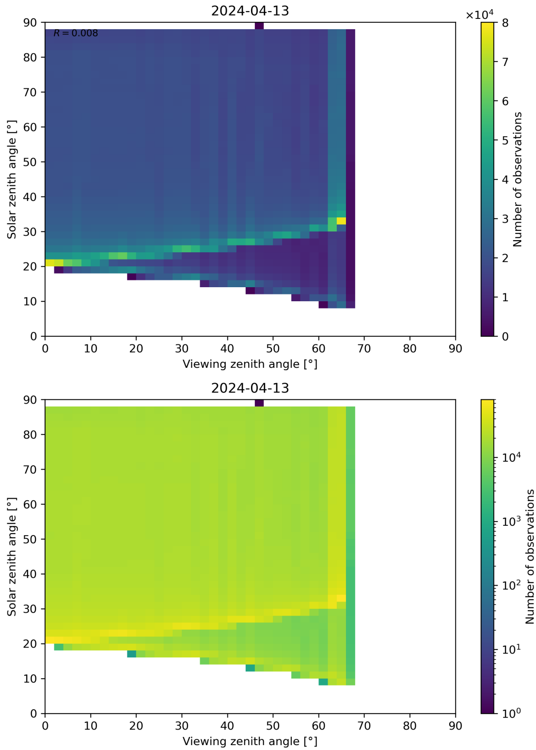
Figure 172: Scatter density plot of “Viewing zenith angle” against “Solar zenith angle” for 2024-04-12 to 2024-04-14.
