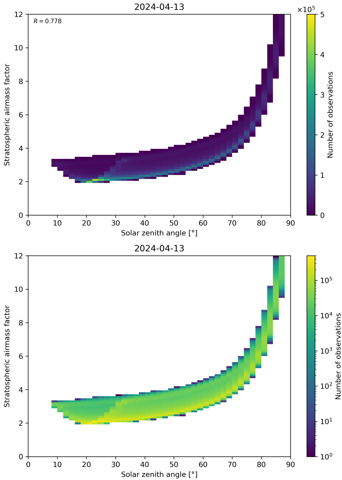
Figure 145: Scatter density plot of “Solar zenith angle” against “Stratospheric airmass factor” for 2024-04-12 to 2024-04-14.
