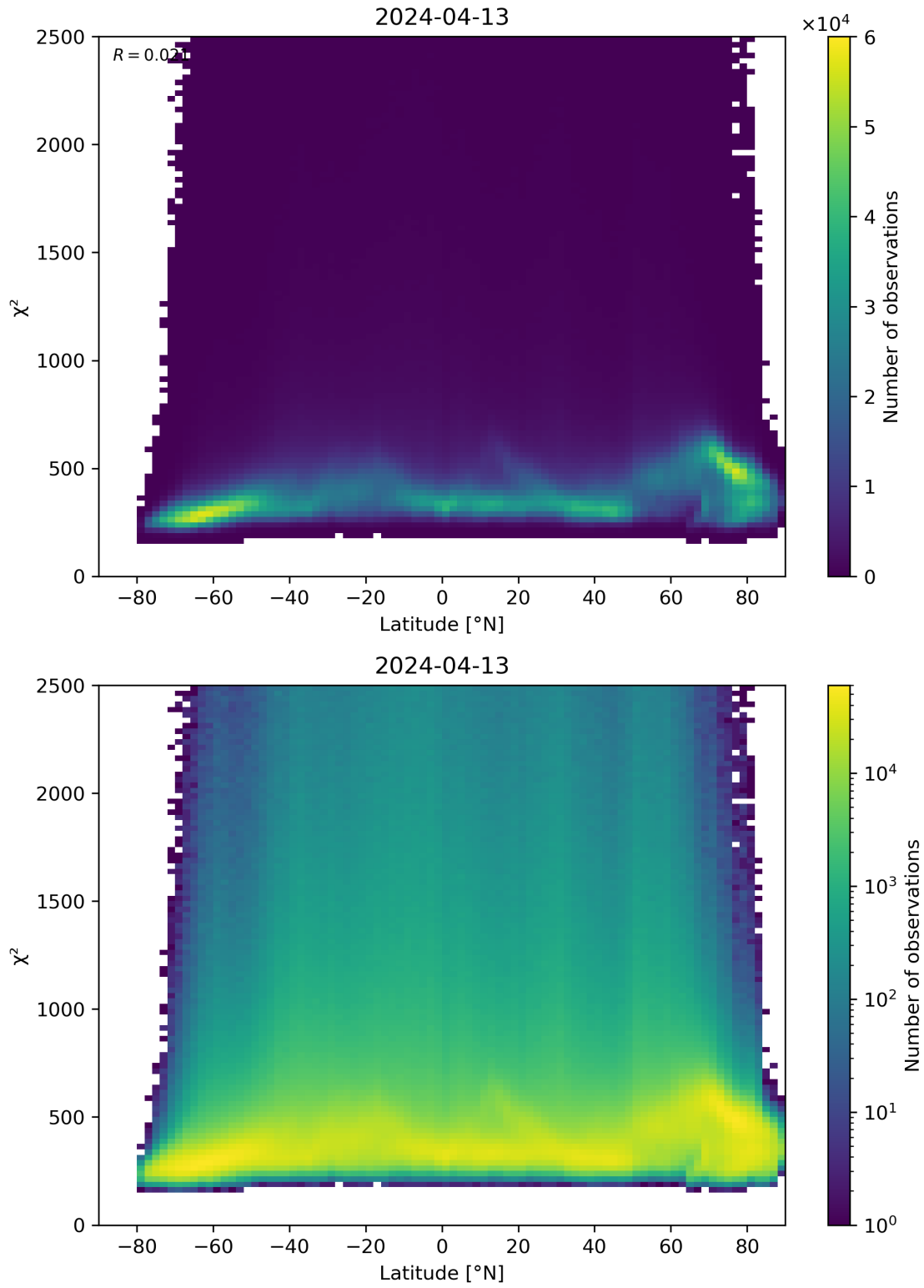
Figure 86: Scatter density plot of “Latitude” against “ \chi^2 ” for 2024-04-12 to 2024-04-14.
