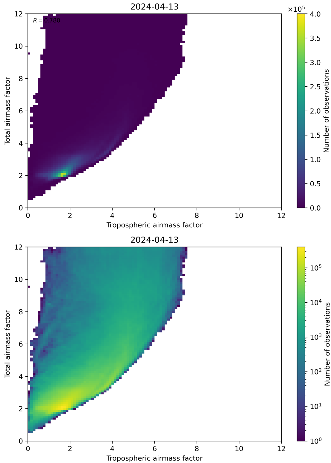
Figure 72: Scatter density plot of “Tropospheric airmass factor” against “Total airmass factor” for 2024-04-12 to 2024-04-14.
