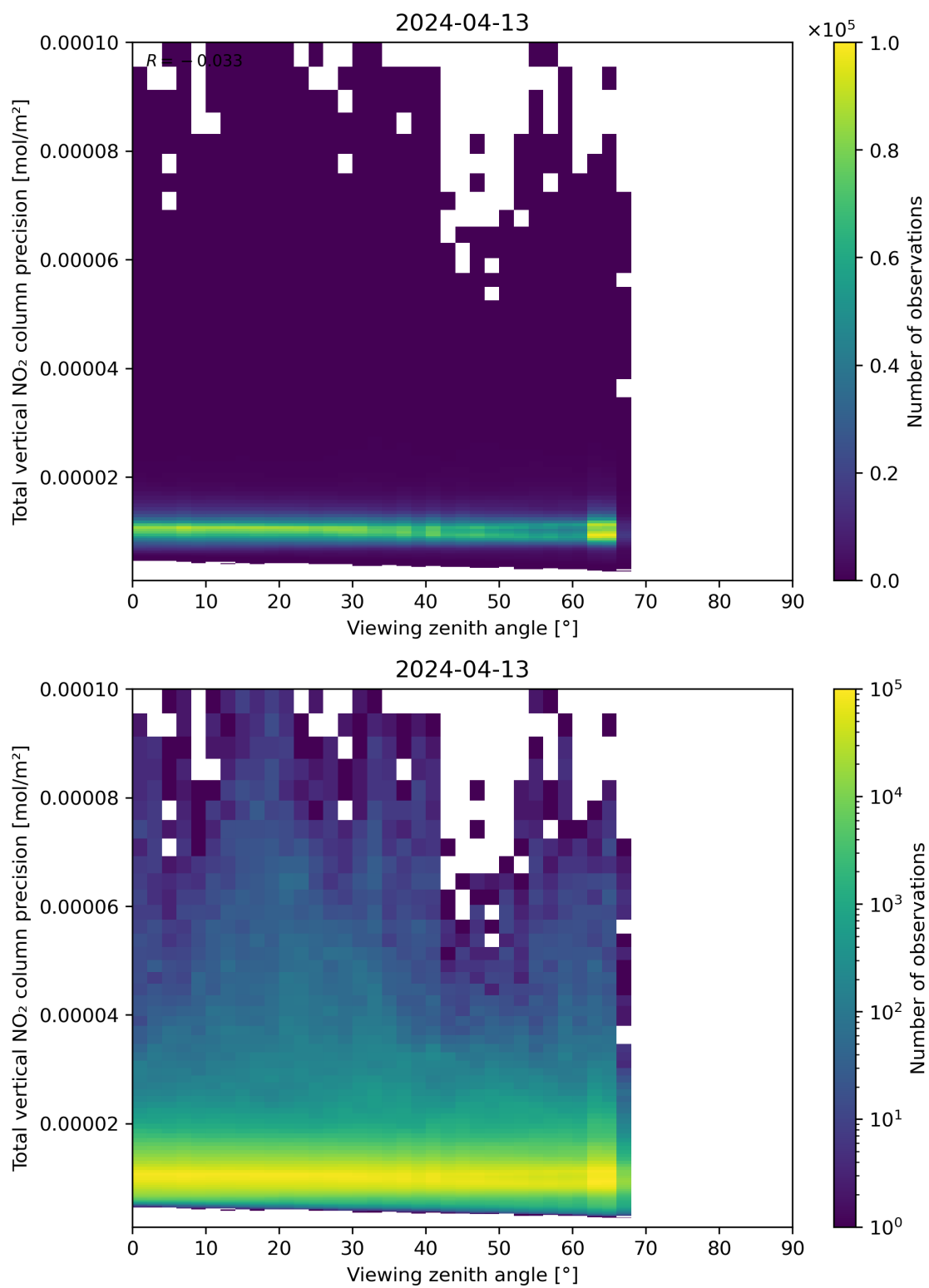
Figure 168: Scatter density plot of “Viewing zenith angle” against “Total vertical NO 2 column precision” for 2024-04-12 to 2024-04-14.
