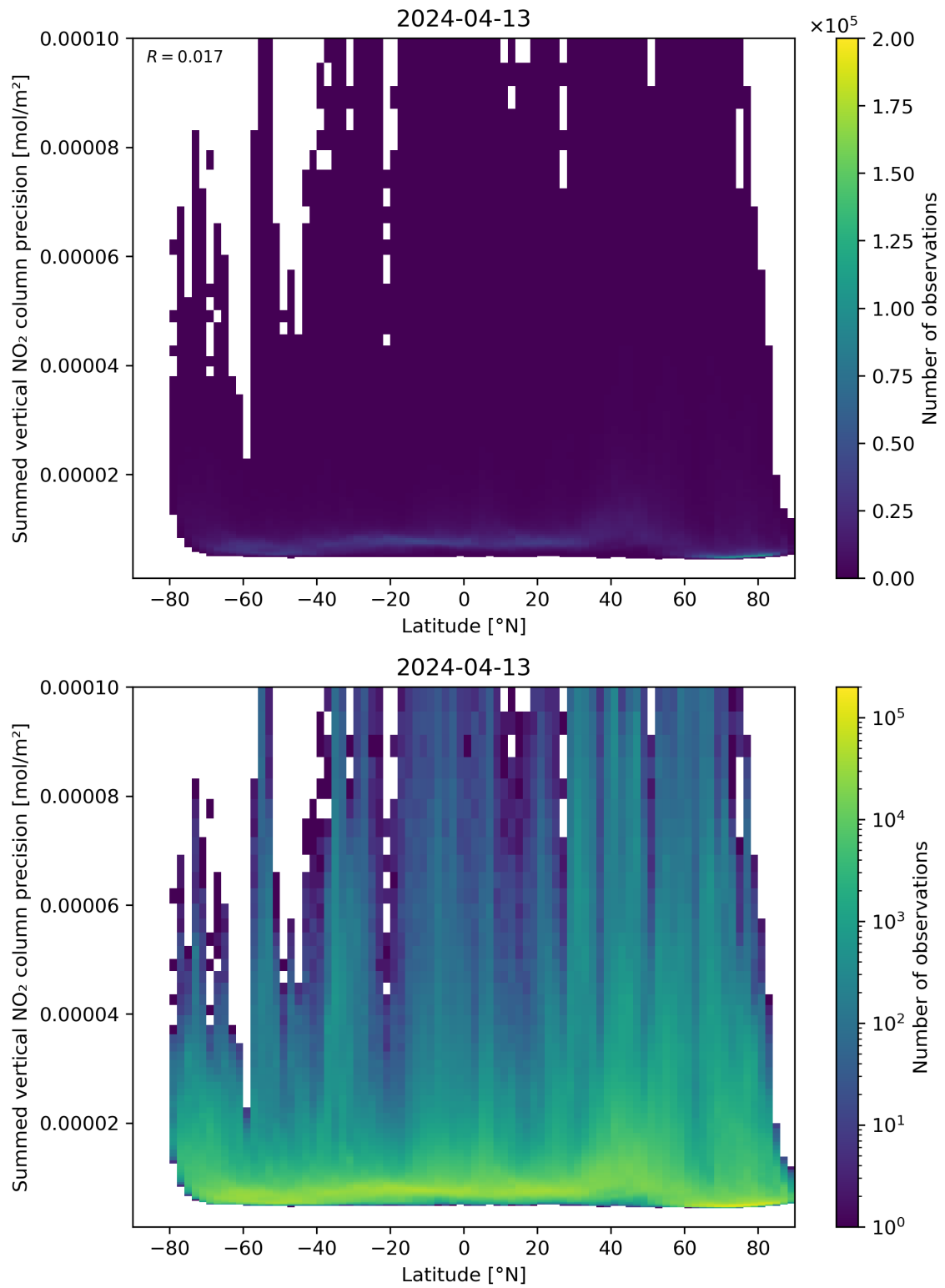
Figure 89: Scatter density plot of “Latitude” against “Summed vertical NO 2 column precision” for 2024-04-12 to 2024-04-14.
