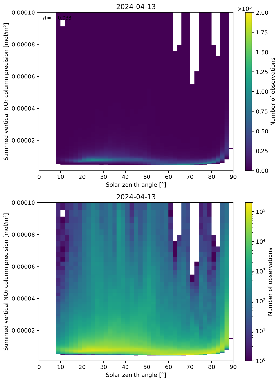
Figure 152: Scatter density plot of “Solar zenith angle” against “Summed vertical NO 2 column precision” for 2024-04-12 to 2024-04-14.
