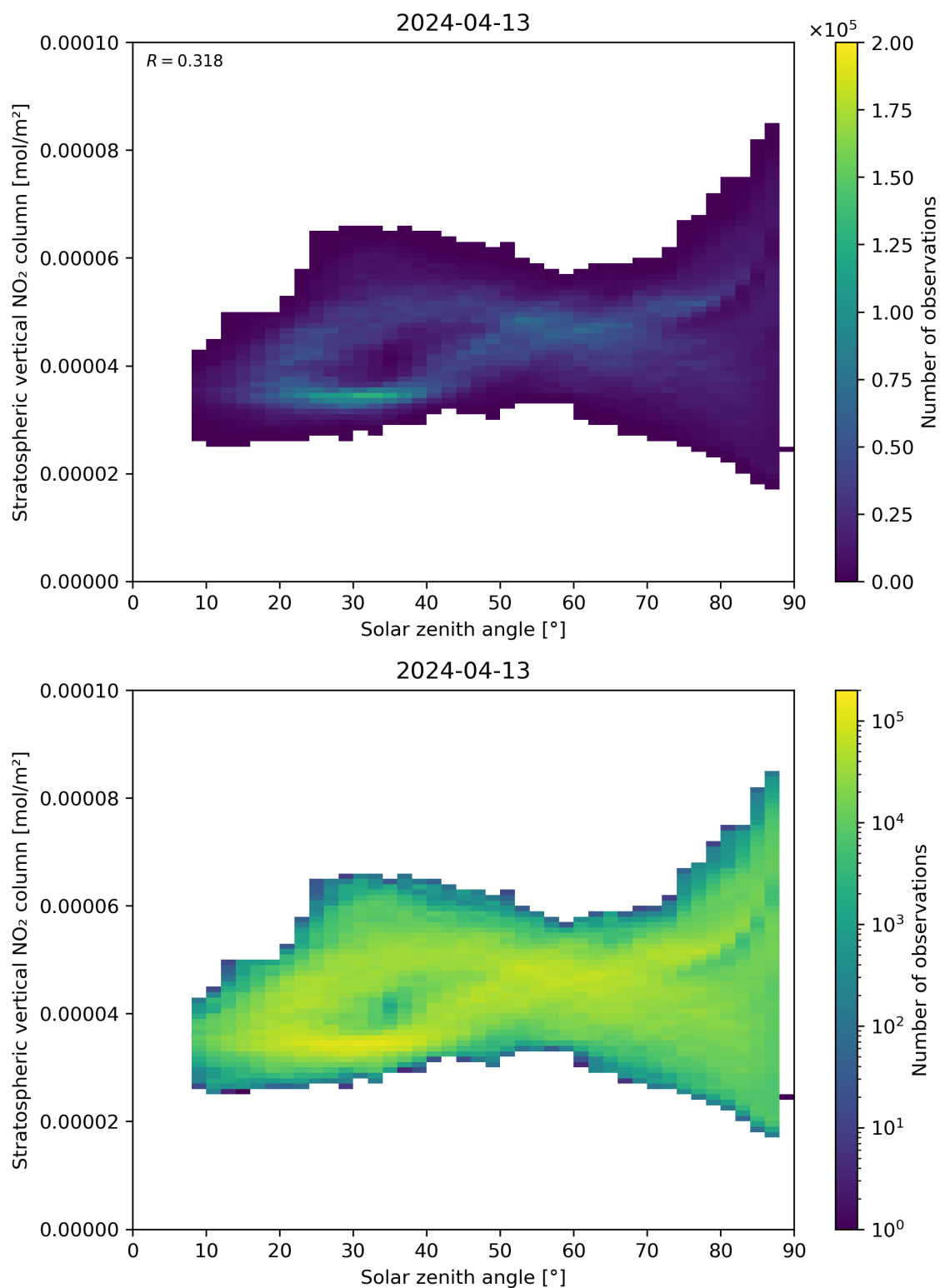
Figure 150: Scatter density plot of “Solar zenith angle” against “Stratospheric vertical NO 2 column” for 2024-04-12 to 2024-04-14.
