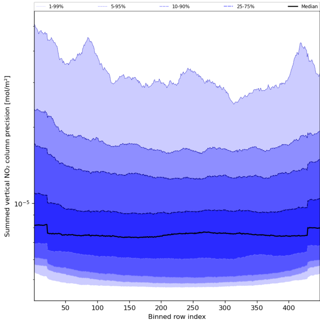
Figure 58: Along track statistics of “Summed vertical NO 2 column precision” for 2024-04-12 to 2024-04-14
