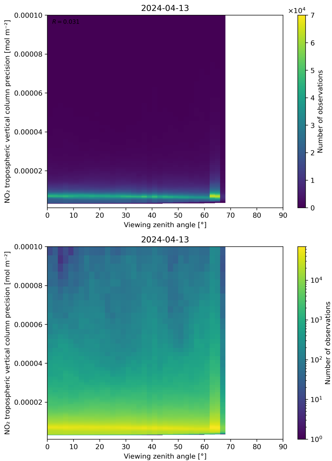
Figure 170: Scatter density plot of “Viewing zenith angle” against “NO 2 tropospheric vertical column precision” for 2024-04-12 to 2024-04-14.
