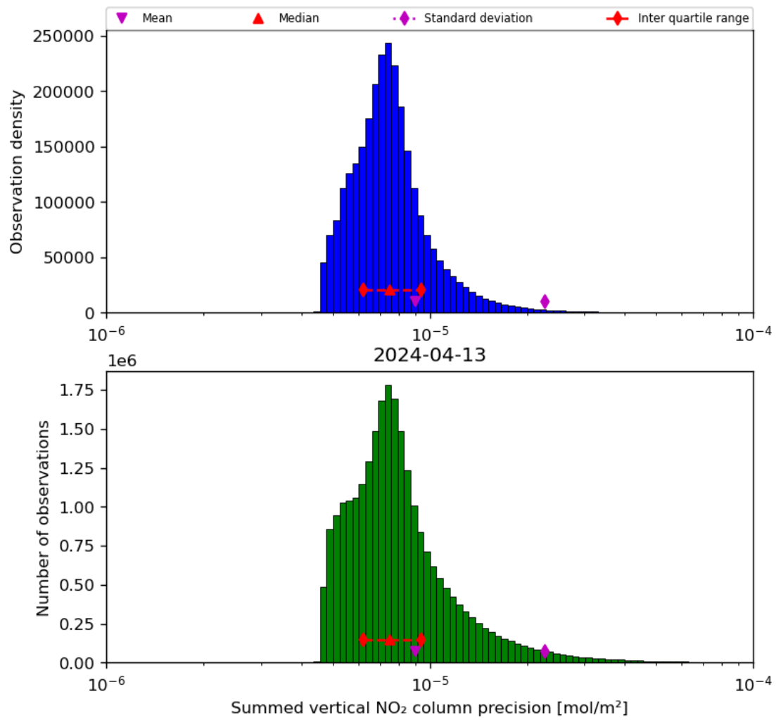
Figure 41: Histogram of “Summed vertical NO 2 column precision” for 2024-04-12 to 2024-04-14
