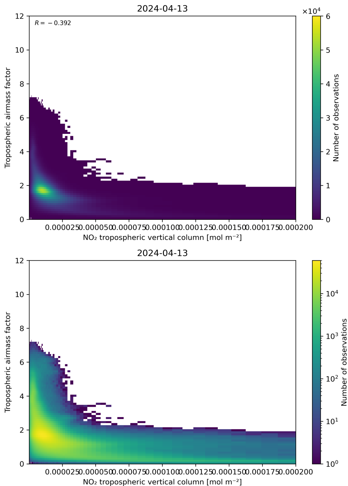
Figure 123: Scatter density plot of “NO 2 tropospheric vertical column” against “Tropospheric air mass factor” for 2024-04-12 to 2024-04-14.
