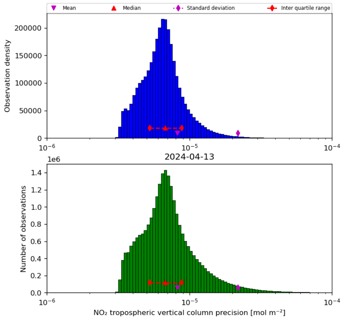
Figure 30: Histogram of “NO 2 tropospheric vertical column precision” for 2024-04-12 to 2024-04-14
