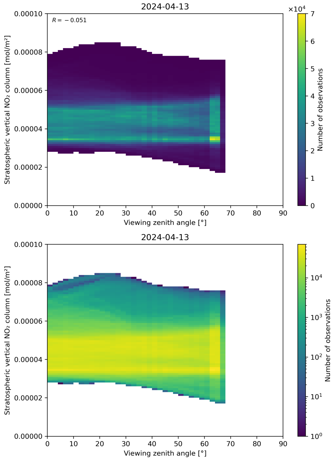
Figure 164: Scatter density plot of “Viewing zenith angle” against “Stratospheric vertical NO 2 column” for 2024-04-12 to 2024-04-14.
