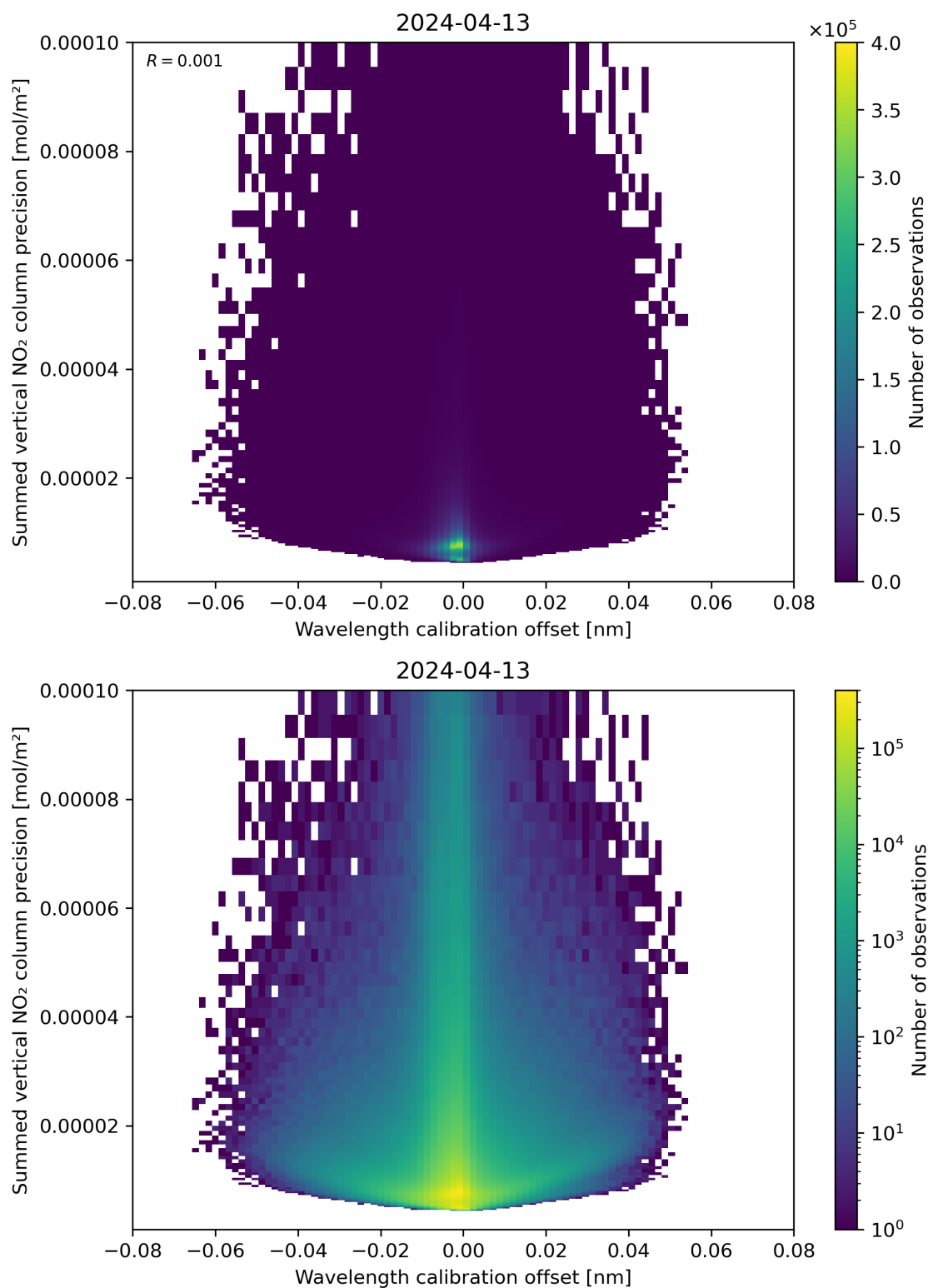
Figure 178: Scatter density plot of “Wavelength calibration offset” against “Summed vertical NO 2 column precision” for 2024-04-12 to 2024-04-14.
