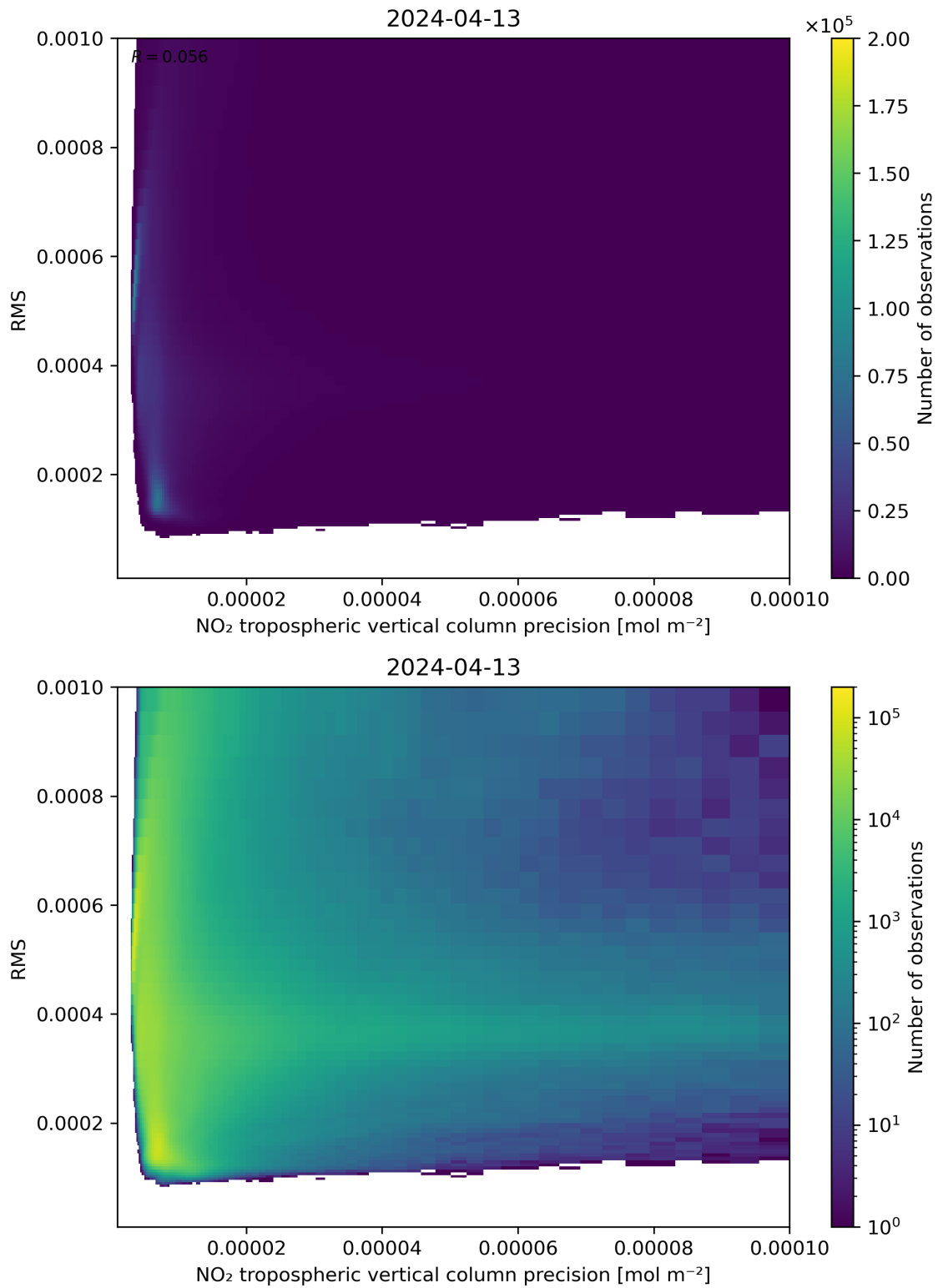
Figure 140: Scatter density plot of “NO 2 tropospheric vertical column precision” against “RMS” for 2024-04-12 to 2024-04-14.
