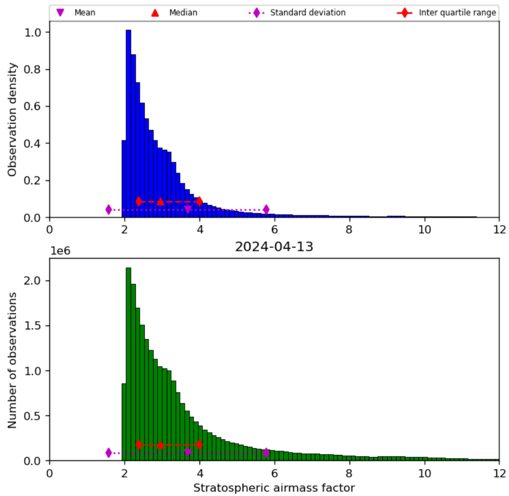
Figure 44: Histogram of “Stratospheric airmass factor” for 2024-04-12 to 2024-04-14
