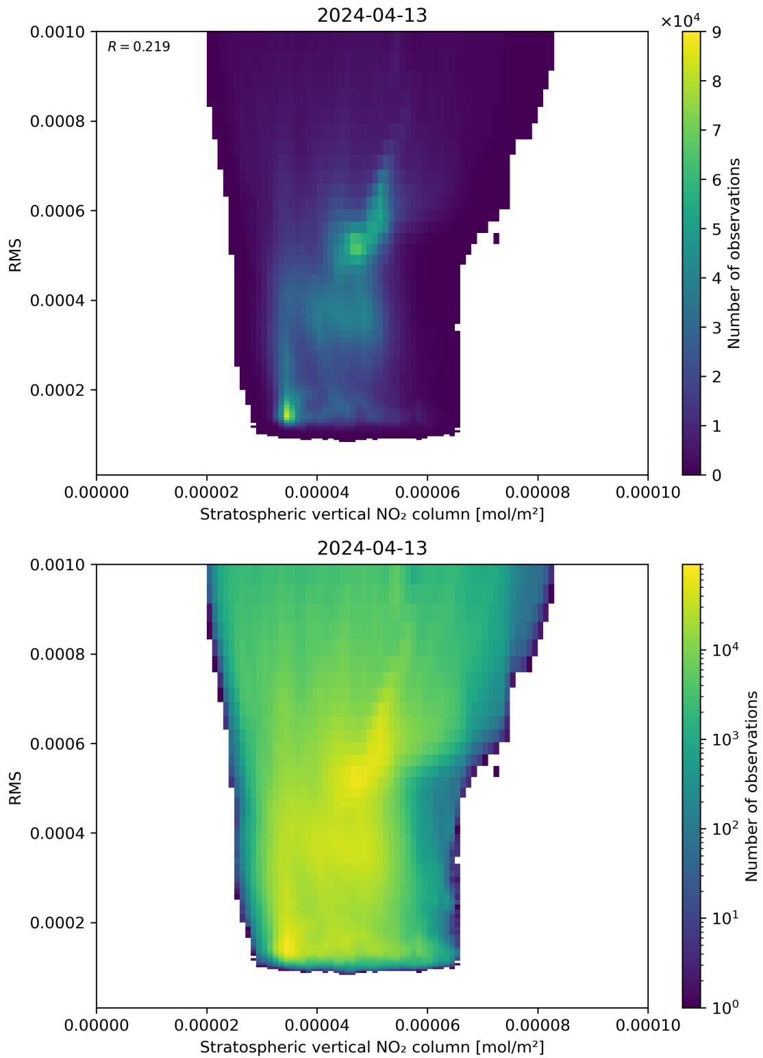
Figure 102: Scatter density plot of “Stratospheric vertical NO 2 column” against “RMS” for 2024-04-12 to 2024-04-14.
