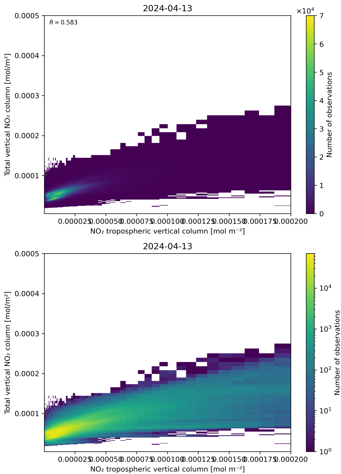
Figure 128: Scatter density plot of “NO 2 tropospheric vertical column” against “Total vertical NO 2 column” for 2024-04-12 to 2024-04-14.
