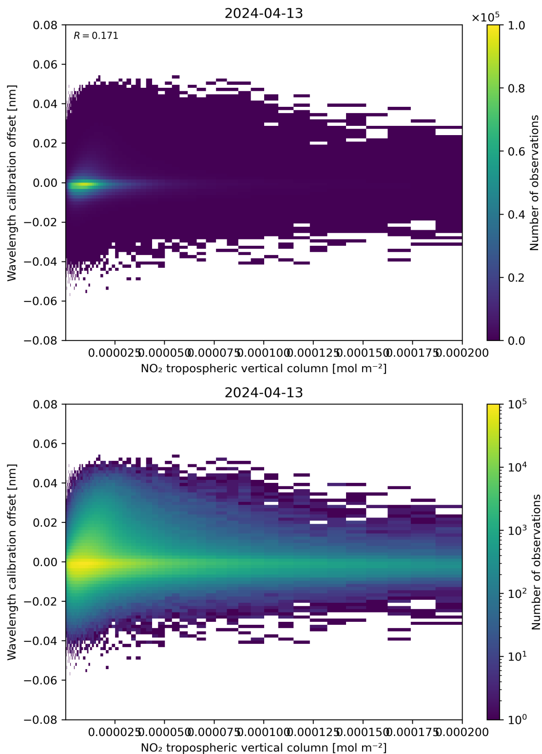
Figure 143: Scatter density plot of “NO 2 tropospheric vertical column” against “Wavelength calibration offset” for 2024-04-12 to 2024-04-14.
