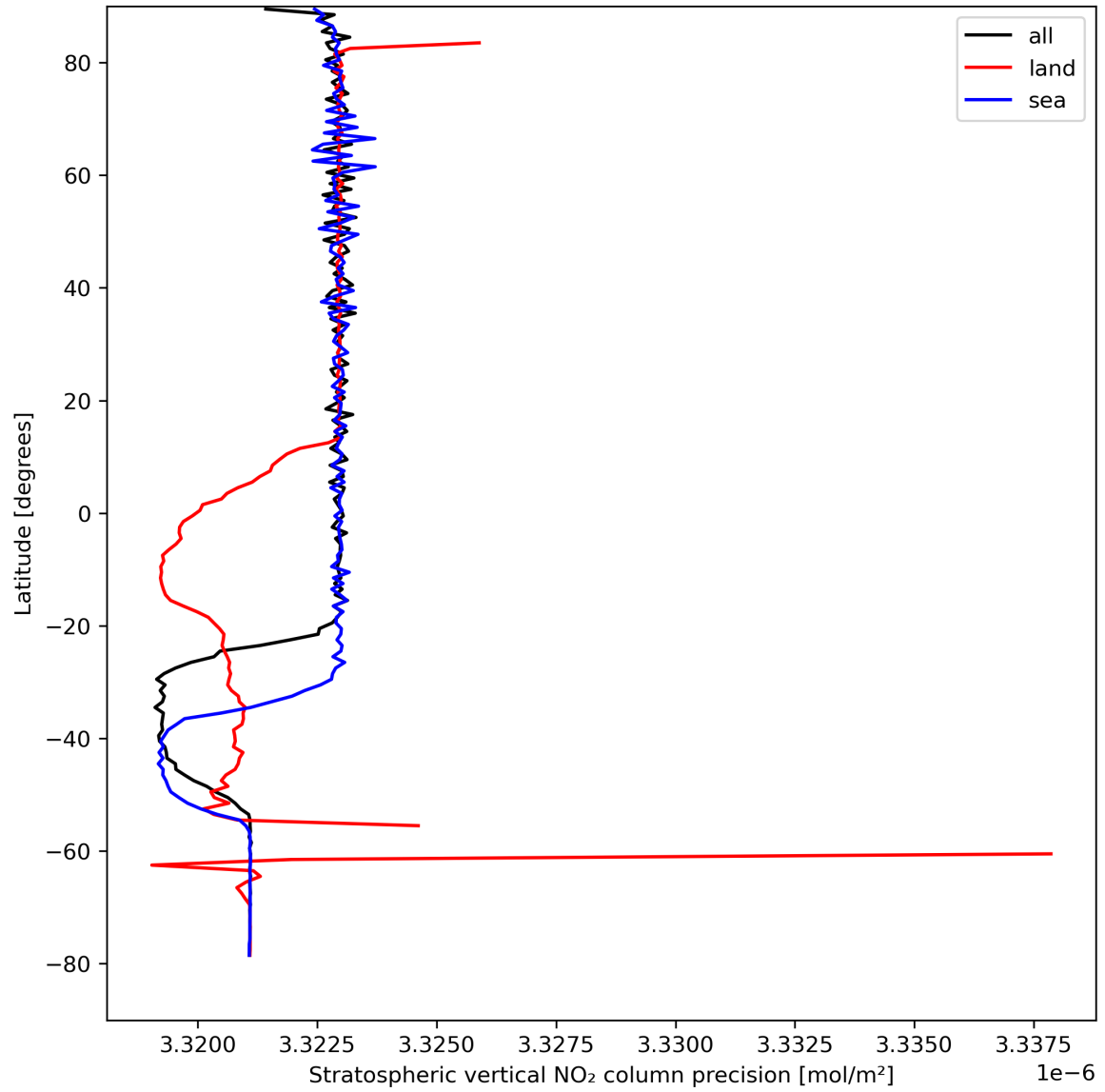
Figure 20: Zonal average of “Stratospheric vertical NO 2 column precision” for 2024-04-12 to 2024-04-14.
