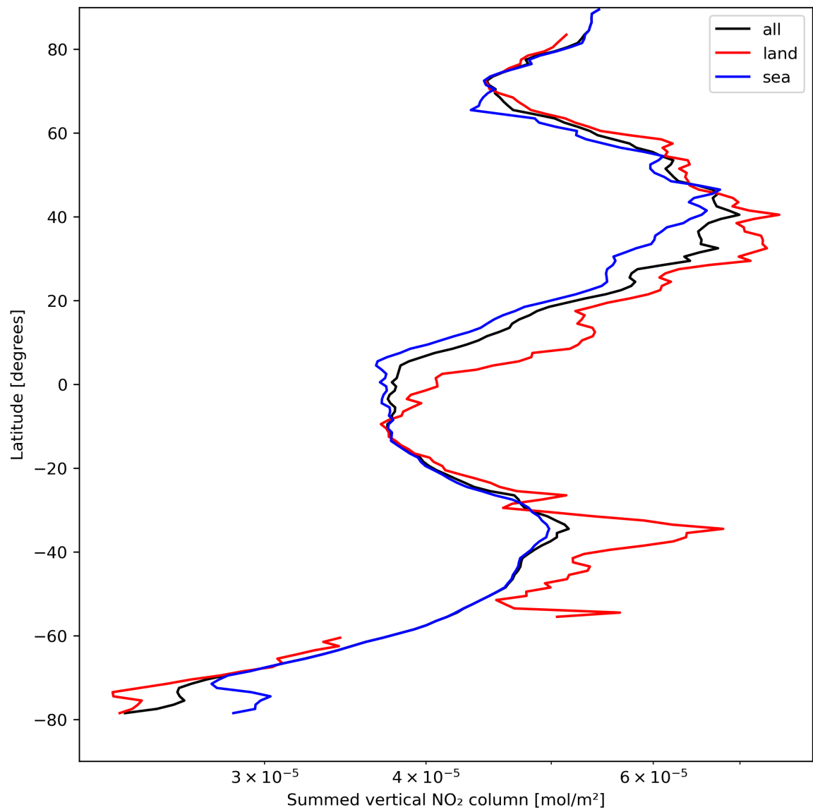
Figure 23: Zonal average of “Summed vertical NO 2 column” for 2024-04-12 to 2024-04-14.
