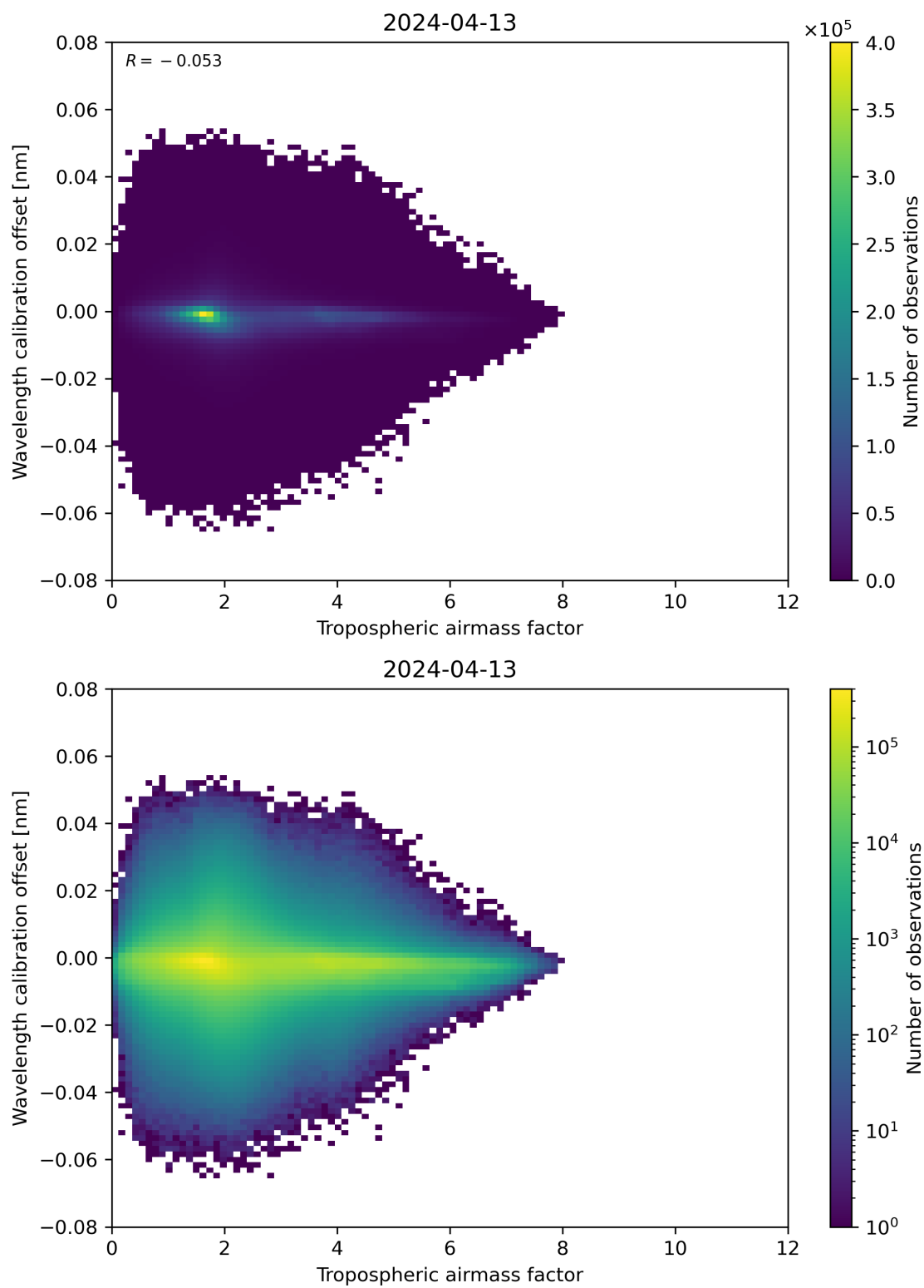
Figure 80: Scatter density plot of “Tropospheric airmass factor” against “Wavelength calibration offset” for 2024-04-12 to 2024-04-14.
