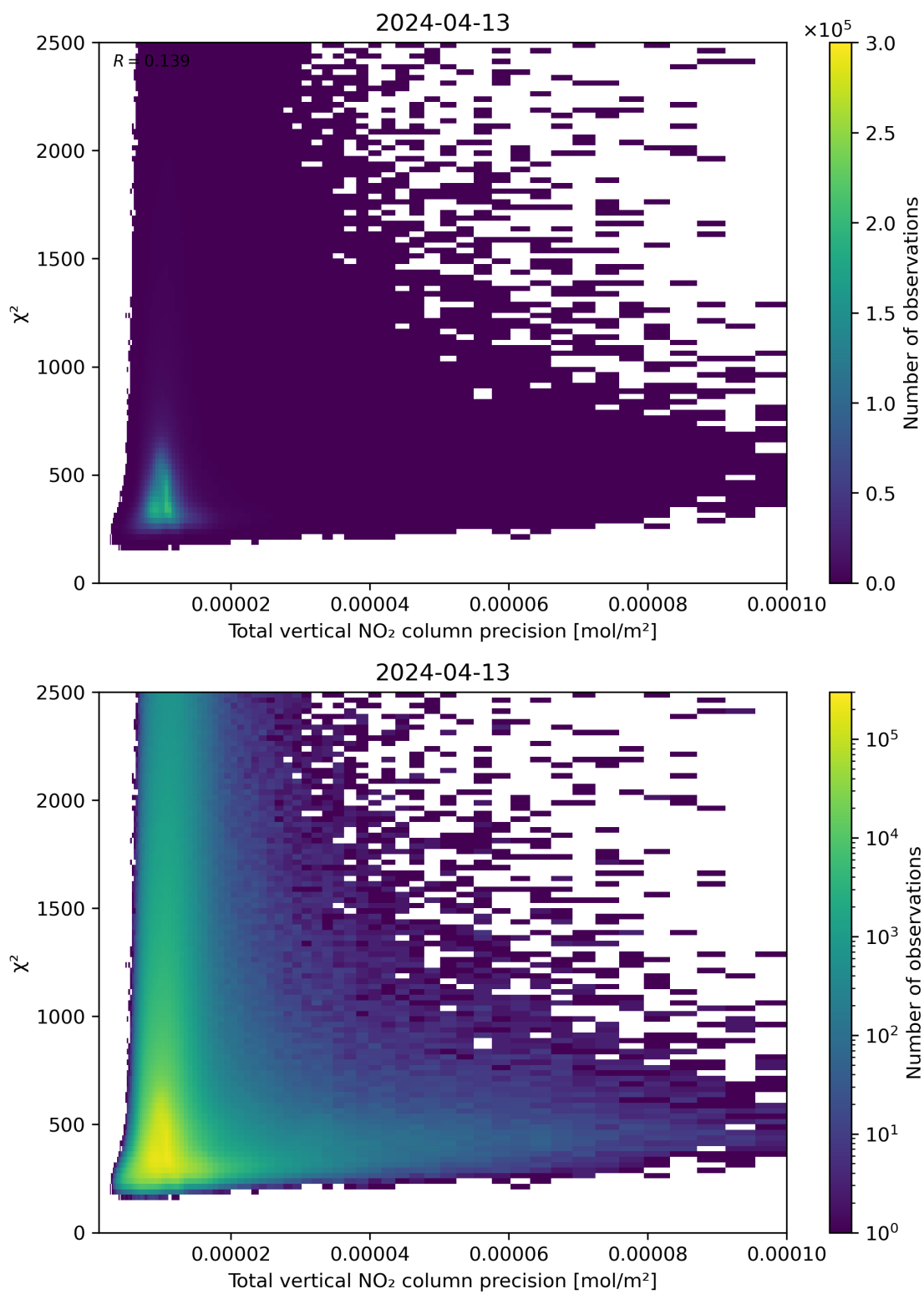
Figure 116: Scatter density plot of “Total vertical NO 2 column precision” against “ \chi^2 ” for 2024-04-12 to 2024-04-14.
