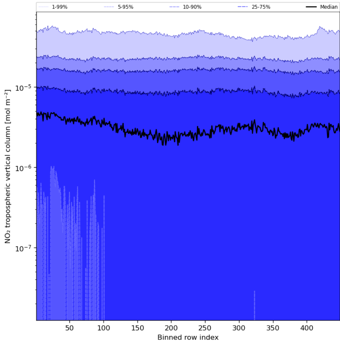
Figure 46: Along track statistics of “NO 2 tropospheric vertical column” for 2024-04-12 to 2024-04-14
