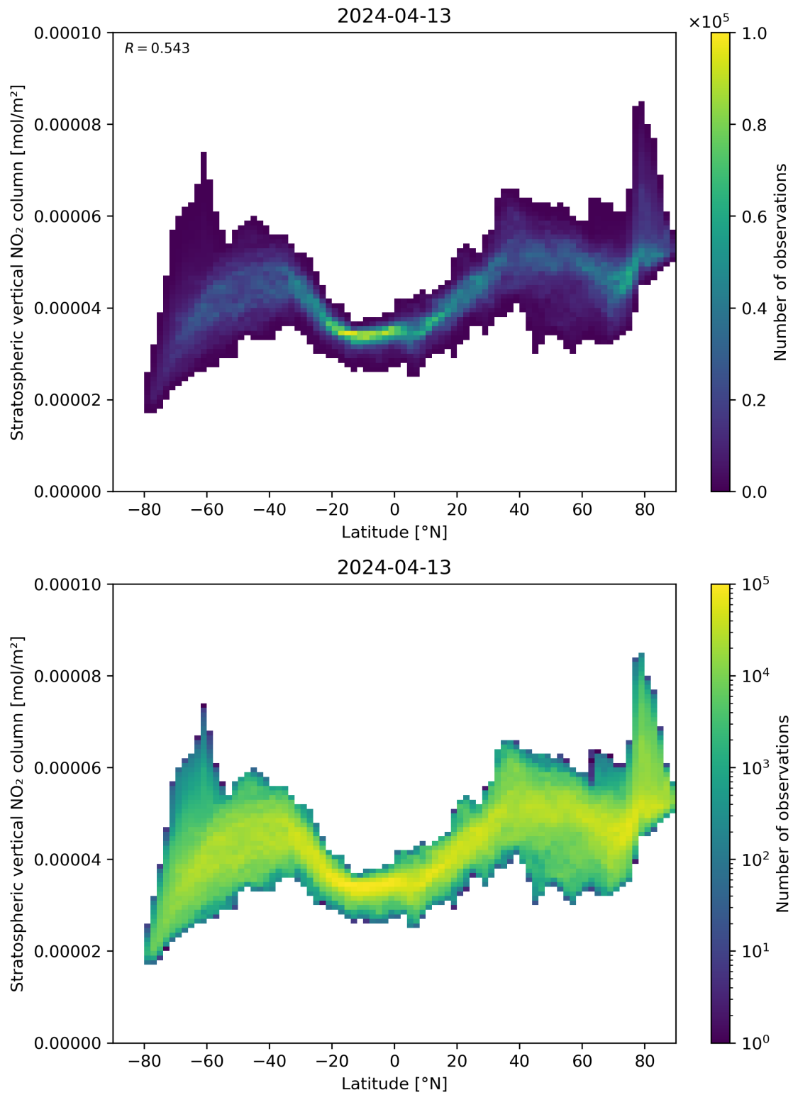
Figure 87: Scatter density plot of “Latitude” against “Stratospheric vertical NO 2 column” for 2024-04-12 to 2024-04-14.
