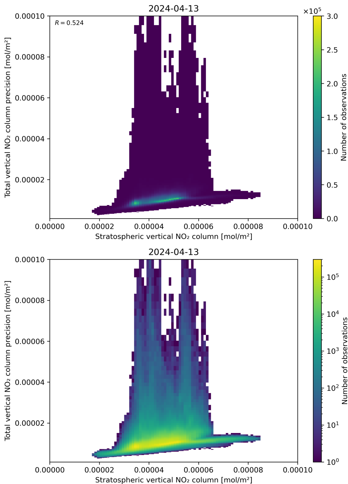
Figure 101: Scatter density plot of “Stratospheric vertical NO 2 column” against “Total vertical NO 2 column precision” for 2024-04-12 to 2024-04-14.
