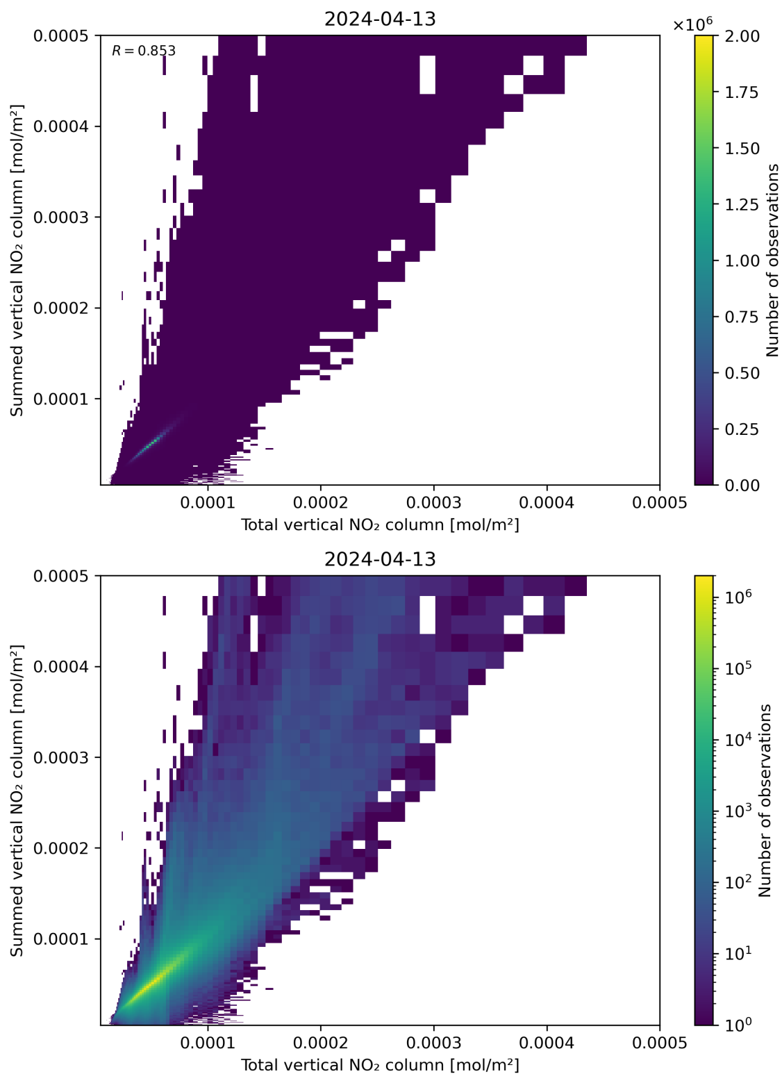
Figure 112: Scatter density plot of “Total vertical NO 2 column” against “Summed vertical NO 2 column” for 2024-04-12 to 2024-04-14.
