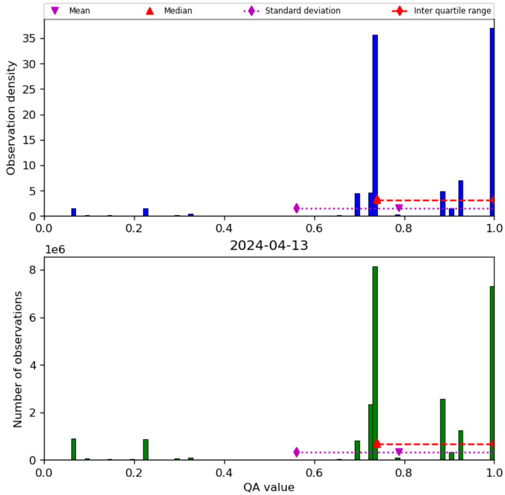
Figure 28: Histogram of “QA value” for 2024-04-12 to 2024-04-14
