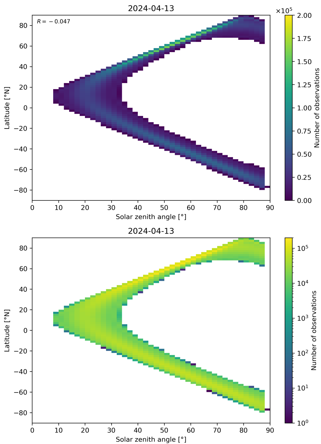
Figure 149: Scatter density plot of “Solar zenith angle” against “Latitude” for 2024-04-12 to 2024-04-14.
