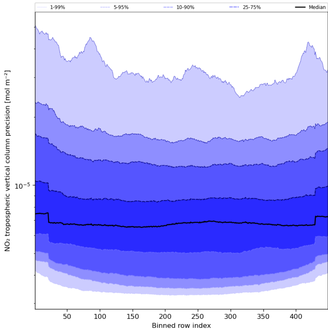
Figure 47: Along track statistics of “NO 2 tropospheric vertical column precision” for 2024-04-12 to 2024-04-14
