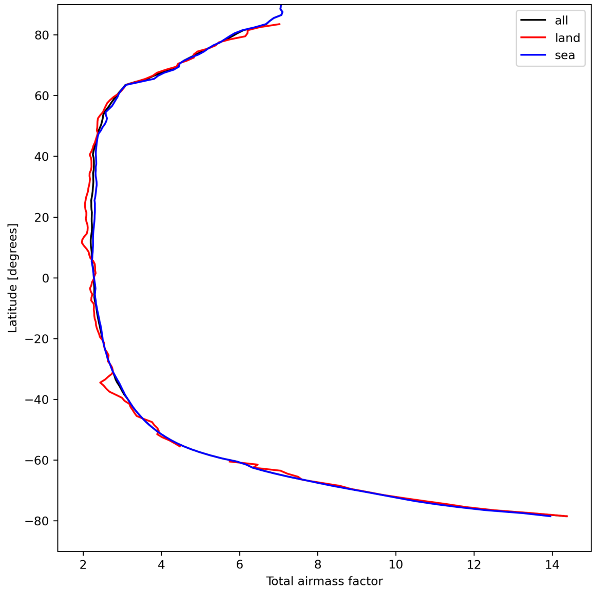
Figure 15: Zonal average of “Total airmass factor” for 2024-04-12 to 2024-04-14.
