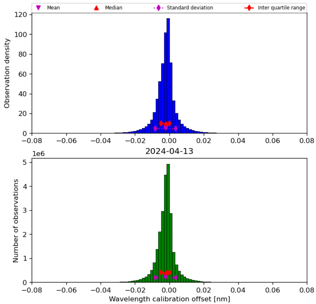
Figure 35: Histogram of “Wavelength calibration offset” for 2024-04-12 to 2024-04-14
