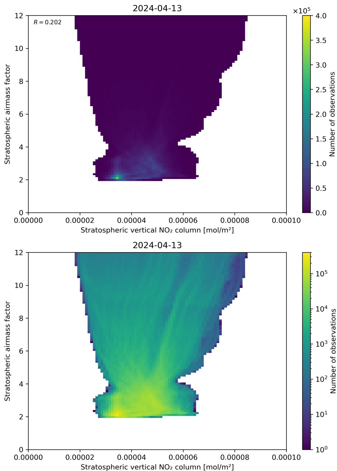
Figure 96: Scatter density plot of “Stratospheric vertical NO 2 column” against “Stratospheric airmass factor” for 2024-04-12 to 2024-04-14.
