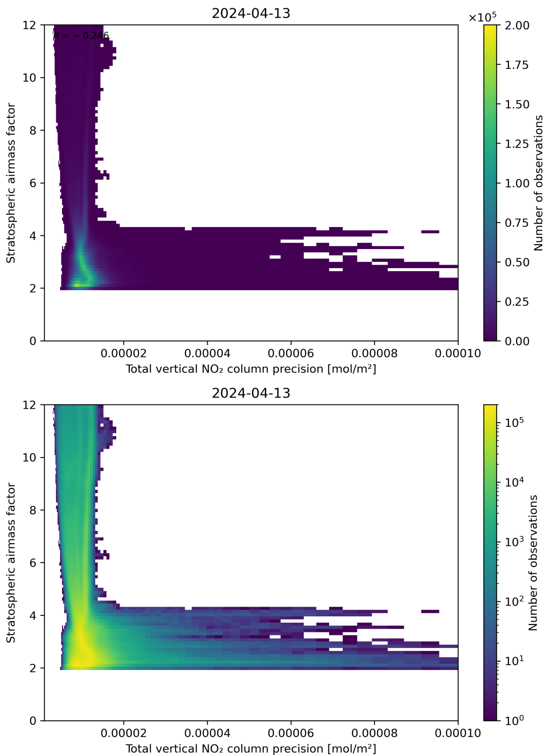
Figure 115: Scatter density plot of “Total vertical NO 2 column precision” against “Stratospheric air mass factor” for 2024-04-12 to 2024-04-14.
