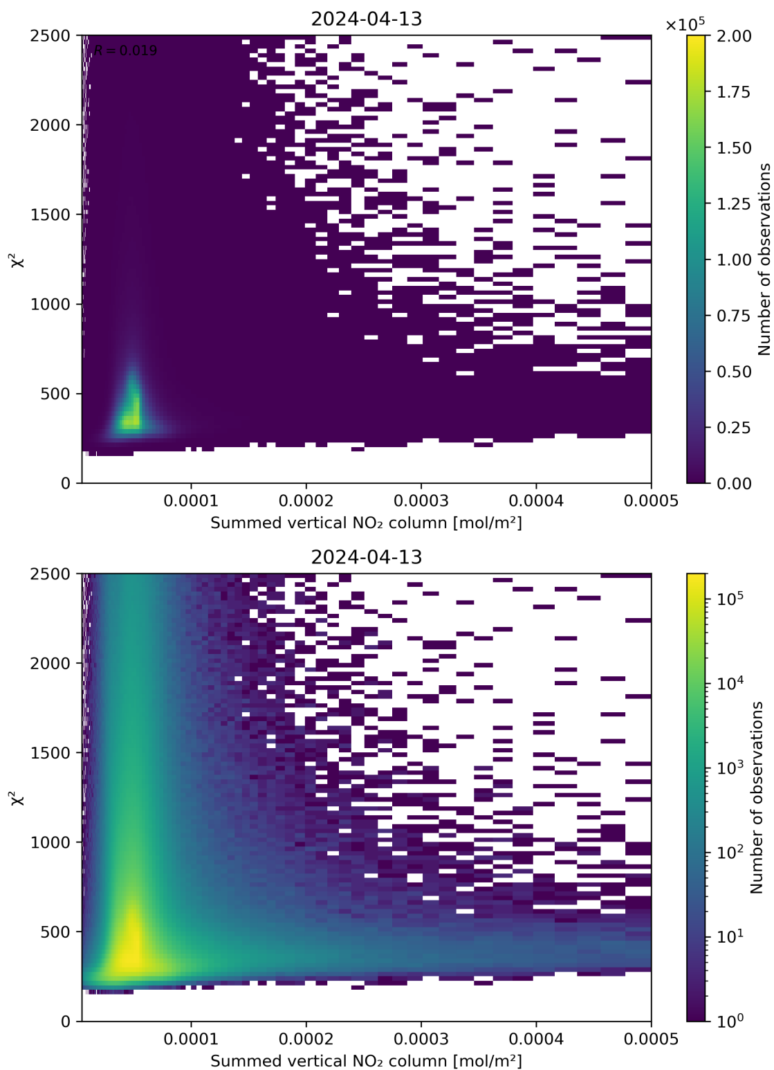
Figure 104: Scatter density plot of “Summed vertical NO 2 column” against “ \chi^2 ” for 2024-04-12 to 2024-04-14.
