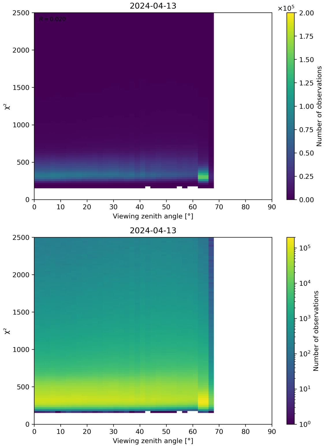
Figure 162: Scatter density plot of “Viewing zenith angle” against “ \chi^2 ” for 2024-04-12 to 2024-04-14.
