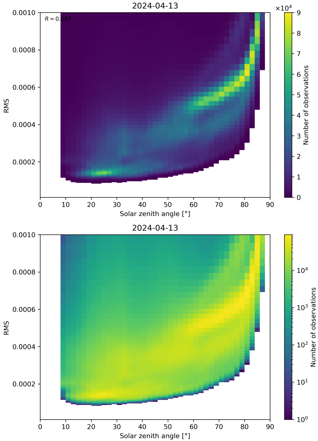
Figure 157: Scatter density plot of “Solar zenith angle” against “RMS” for 2024-04-12 to 2024-04-14.
