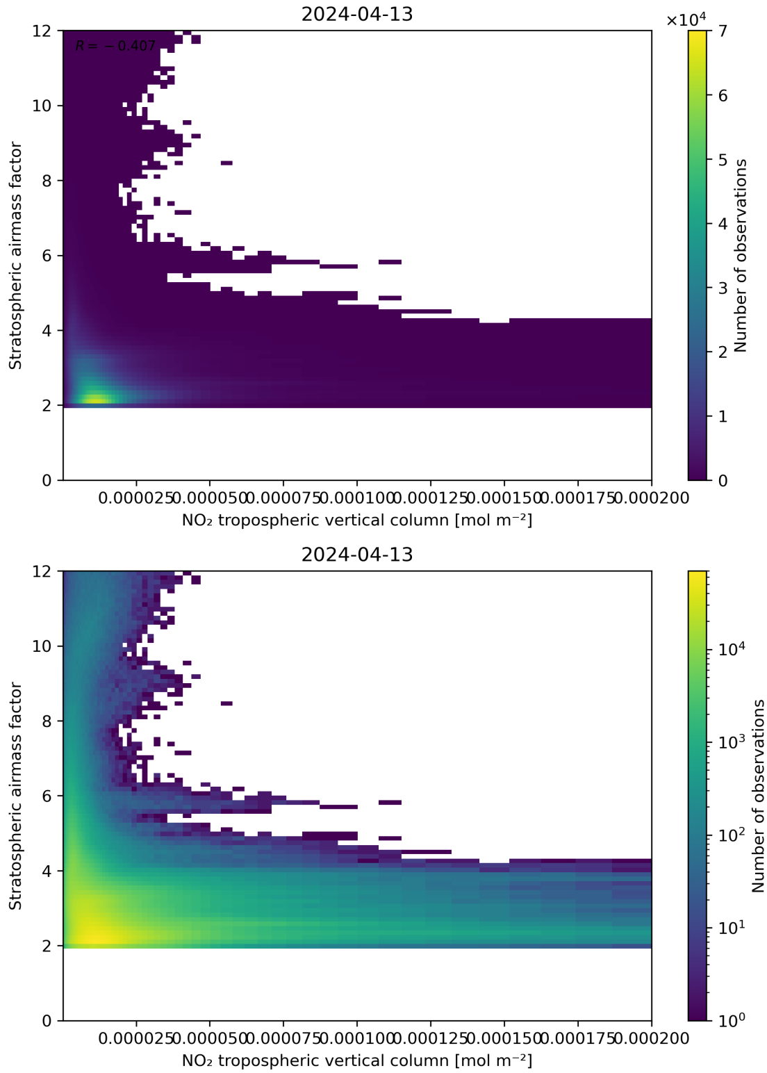
Figure 121: Scatter density plot of “NO 2 tropospheric vertical column” against “Stratospheric air mass factor” for 2024-04-12 to 2024-04-14.
