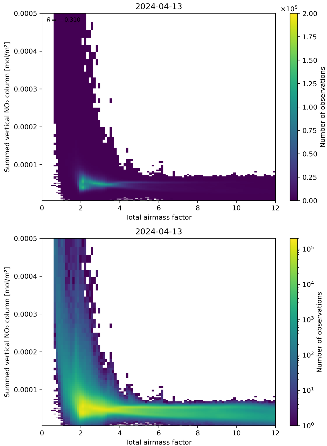
Figure 65: Scatter density plot of “Total airmass factor” against “Summed vertical NO 2 column” for 2024-04-12 to 2024-04-14.
