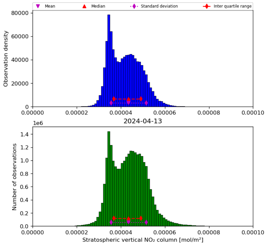
Figure 36: Histogram of “Stratospheric vertical NO 2 column” for 2024-04-12 to 2024-04-14
