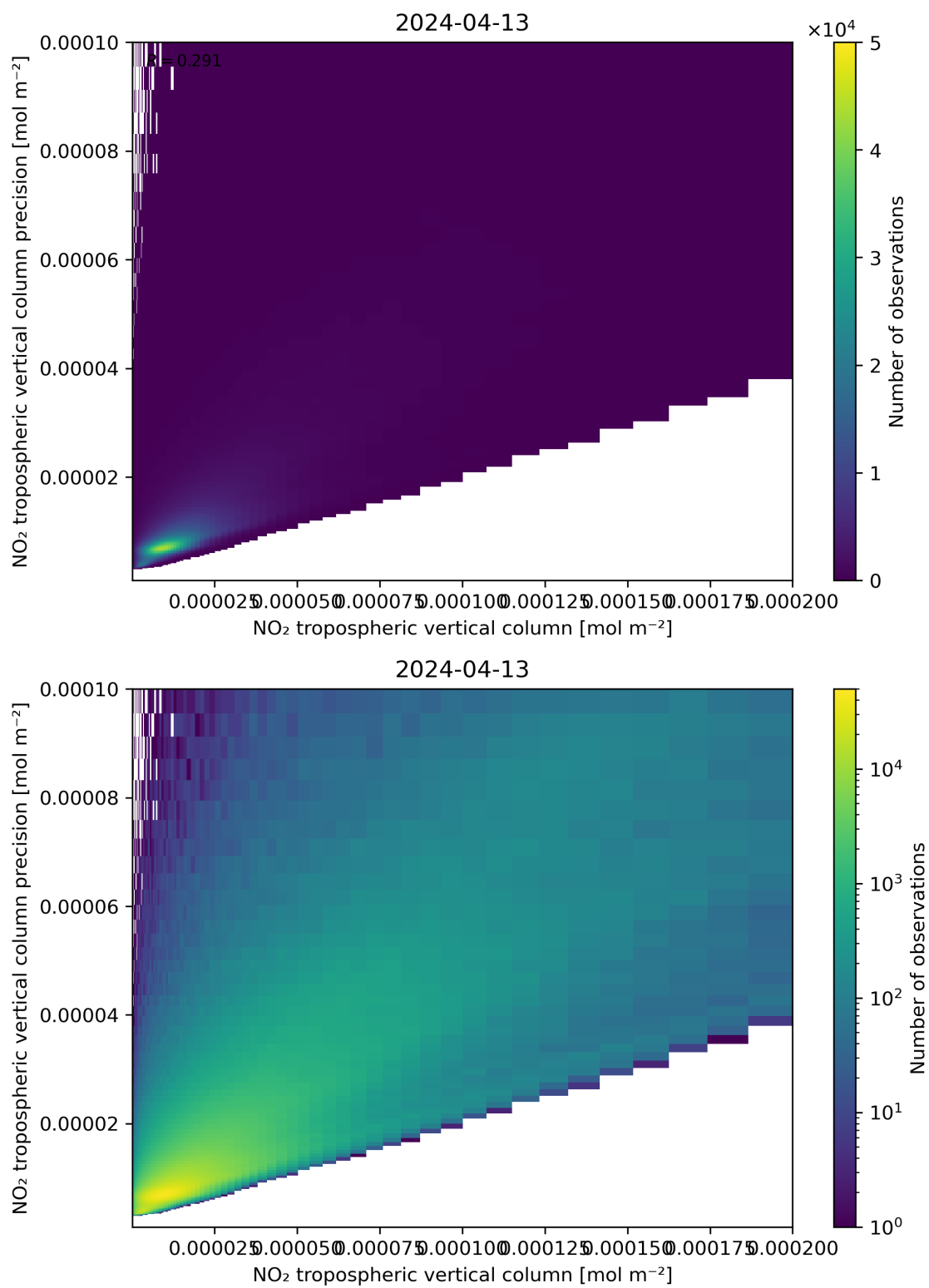
Figure 130: Scatter density plot of “NO 2 tropospheric vertical column” against “NO 2 tropospheric vertical column precision” for 2024-04-12 to 2024-04-14.
