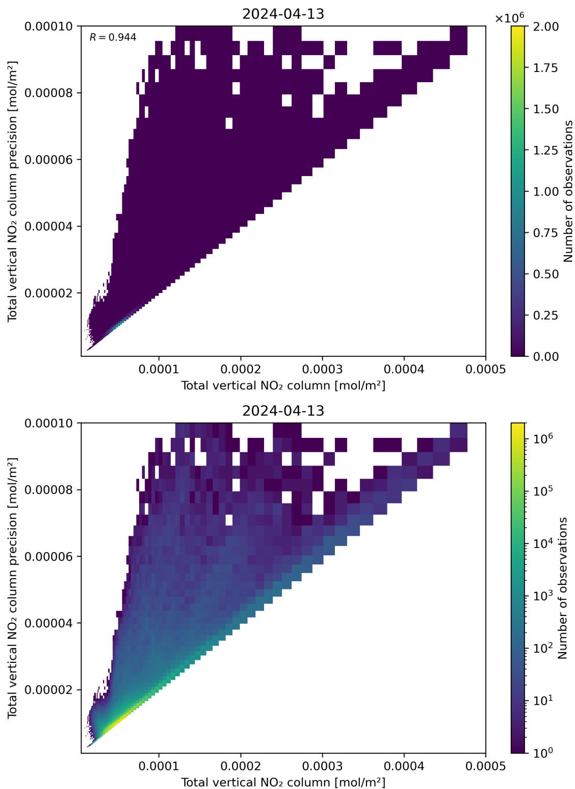
Figure 114: Scatter density plot of “Total vertical NO 2 column” against “Total vertical NO 2 column precision” for 2024-04-12 to 2024-04-14.
