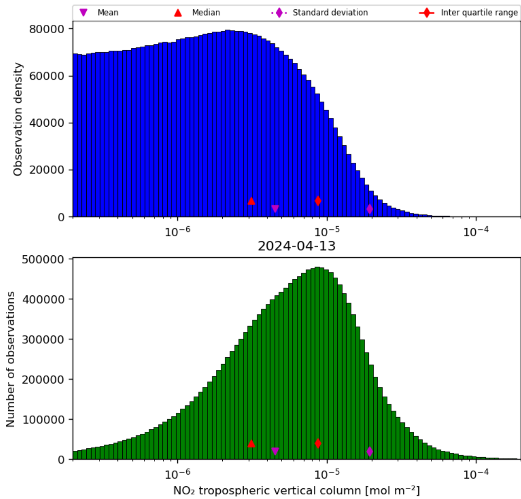
Figure 29: Histogram of “NO 2 tropospheric vertical column” for 2024-04-12 to 2024-04-14
