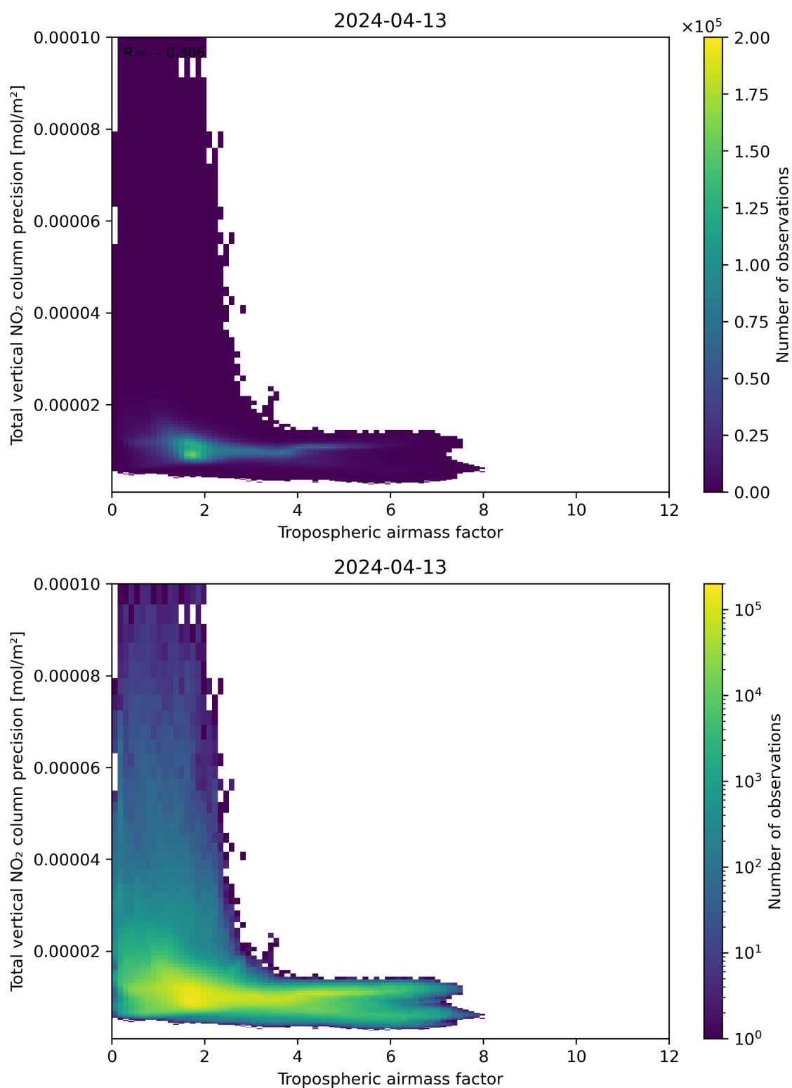
Figure 78: Scatter density plot of “Tropospheric air mass factor” against “Total vertical NO 2 column precision” for 2024-04-12 to 2024-04-14.
