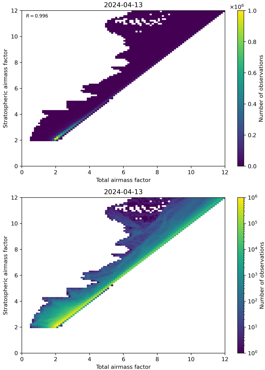
Figure 62: Scatter density plot of “Total airmass factor” against “Stratospheric airmass factor” for 2024-04-12 to 2024-04-14.
