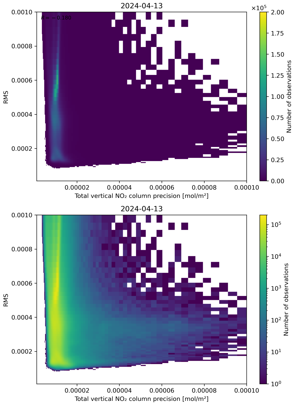
Figure 119: Scatter density plot of “Total vertical NO 2 column precision” against “RMS” for 2024-04-12 to 2024-04-14.
