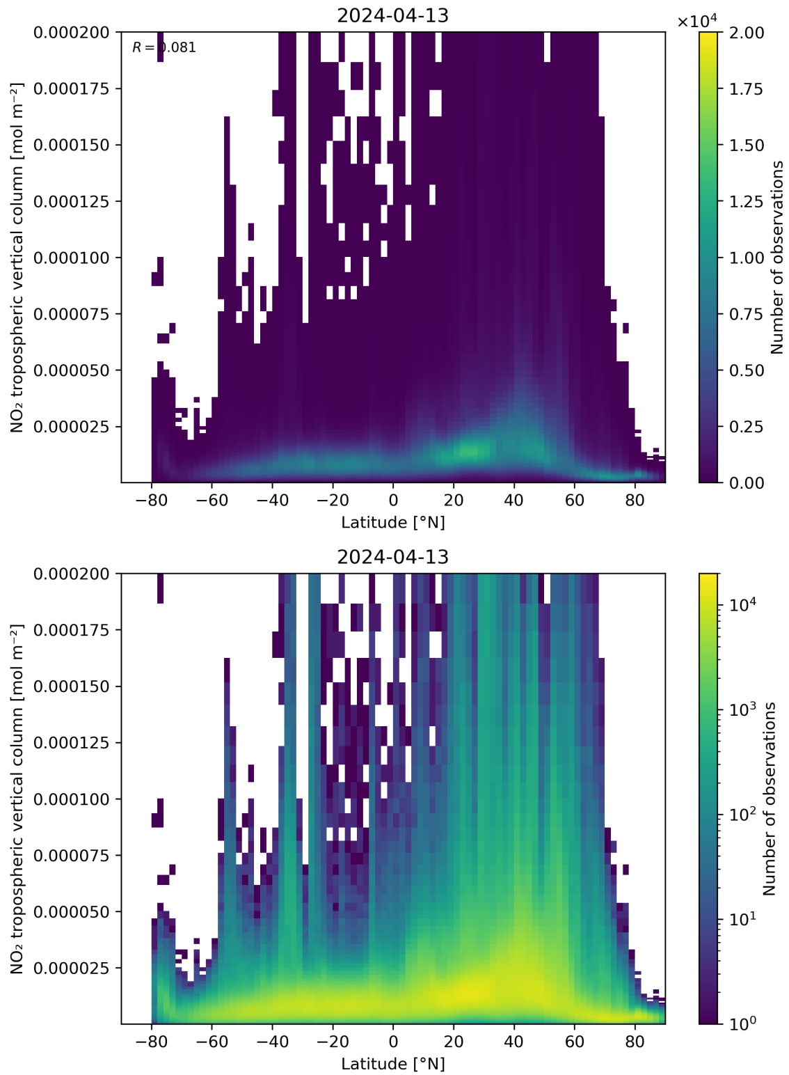
Figure 92: Scatter density plot of “Latitude” against “NO 2 tropospheric vertical column” for 2024-04-12 to 2024-04-14.
