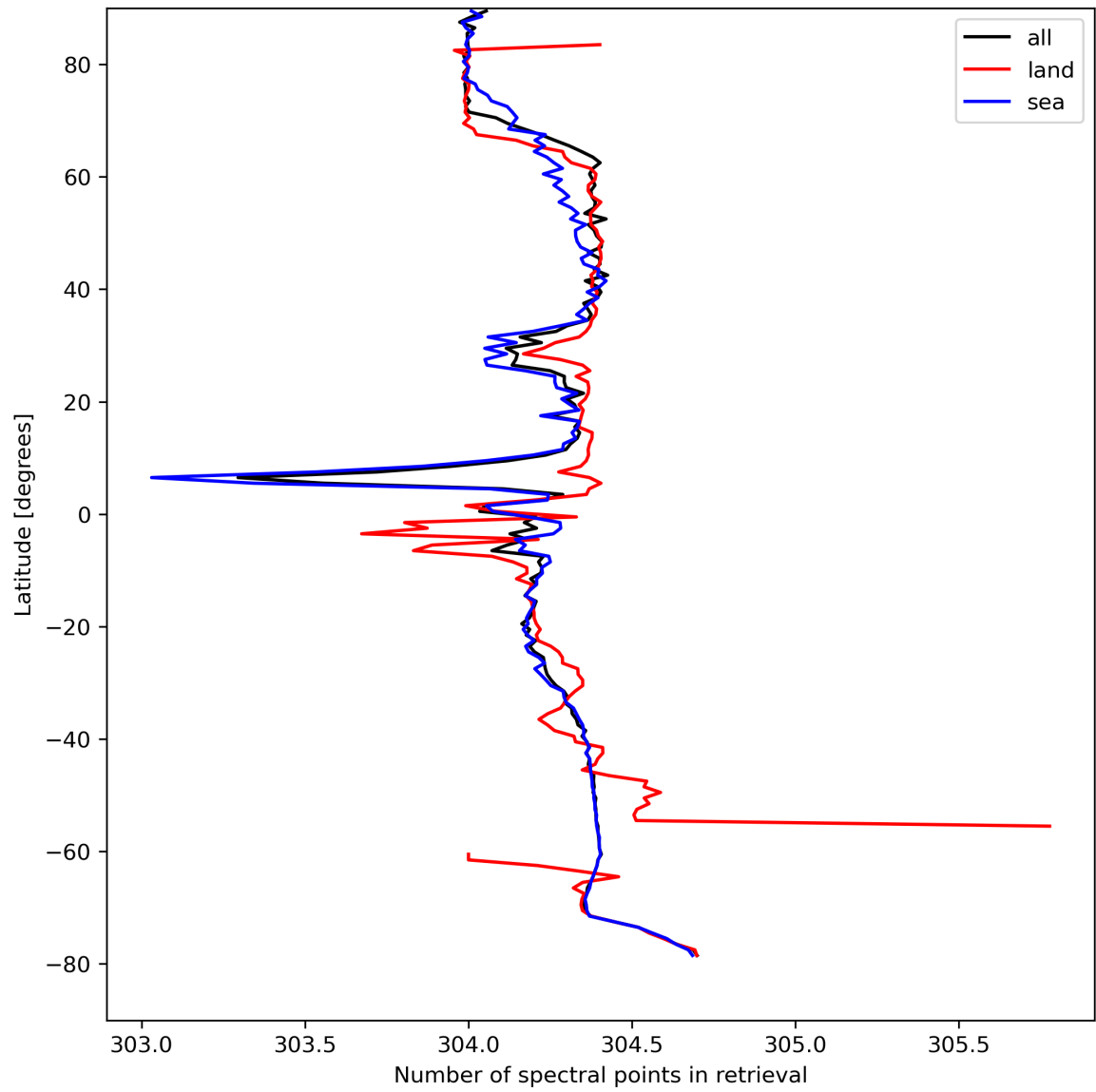
Figure 16: Zonal average of “Number of spectral points in retrieval” for 2024-04-12 to 2024-04-14.
