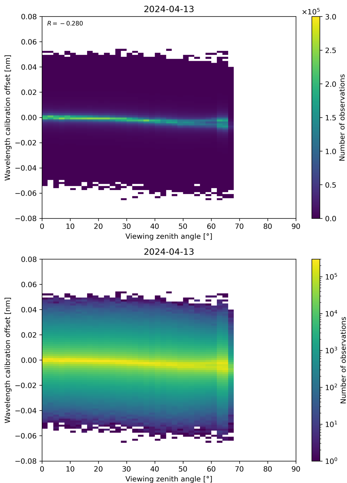
Figure 173: Scatter density plot of “Viewing zenith angle” against “Wavelength calibration offset” for 2024-04-12 to 2024-04-14.
