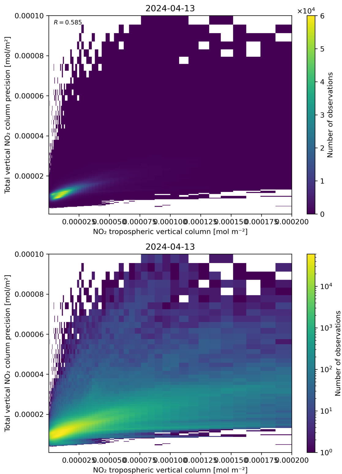
Figure 129: Scatter density plot of “NO 2 tropospheric vertical column” against “Total vertical NO 2 column precision” for 2024-04-12 to 2024-04-14.
