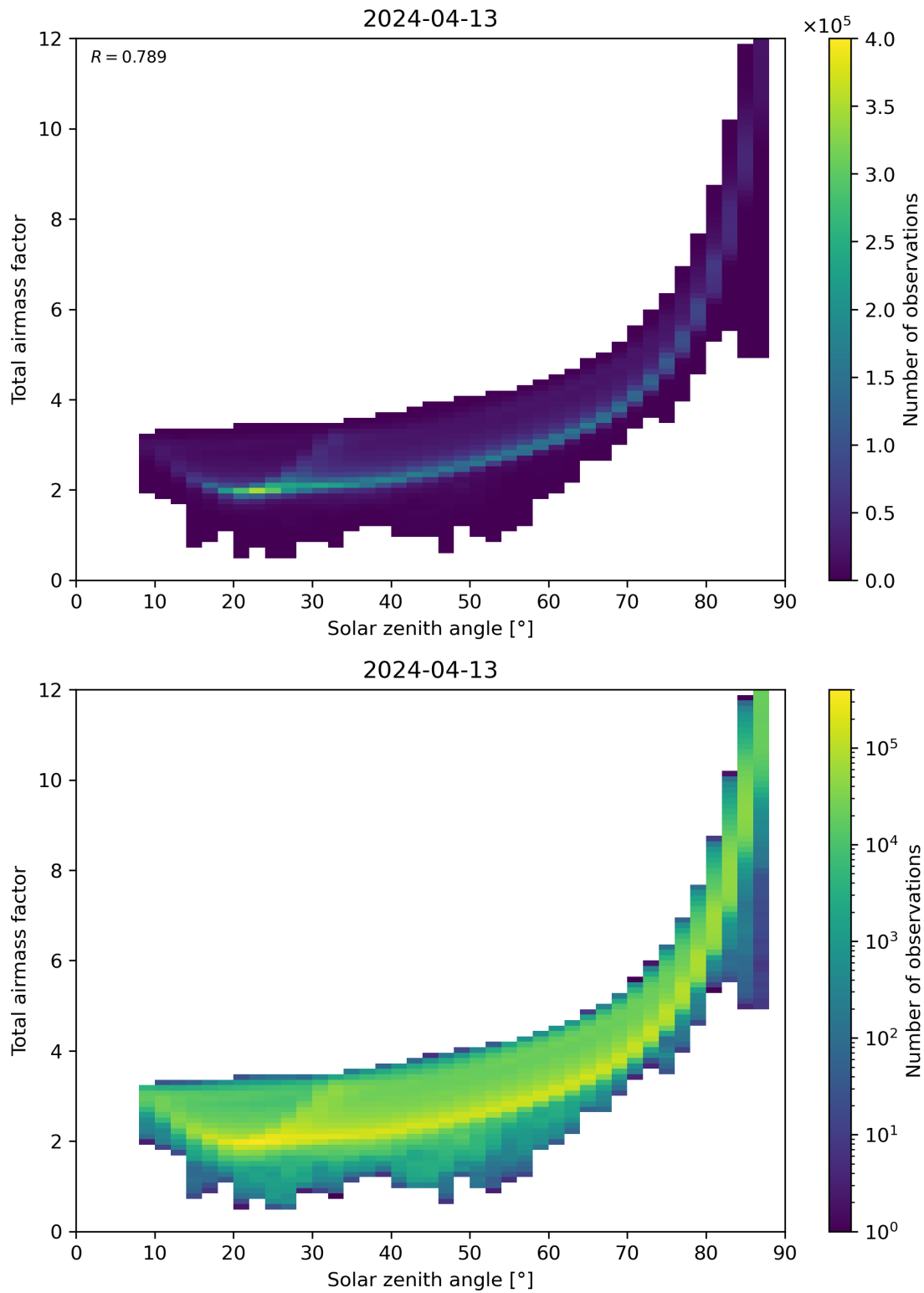
Figure 146: Scatter density plot of “Solar zenith angle” against “Total air mass factor” for 2024-04-12 to 2024-04-14.
