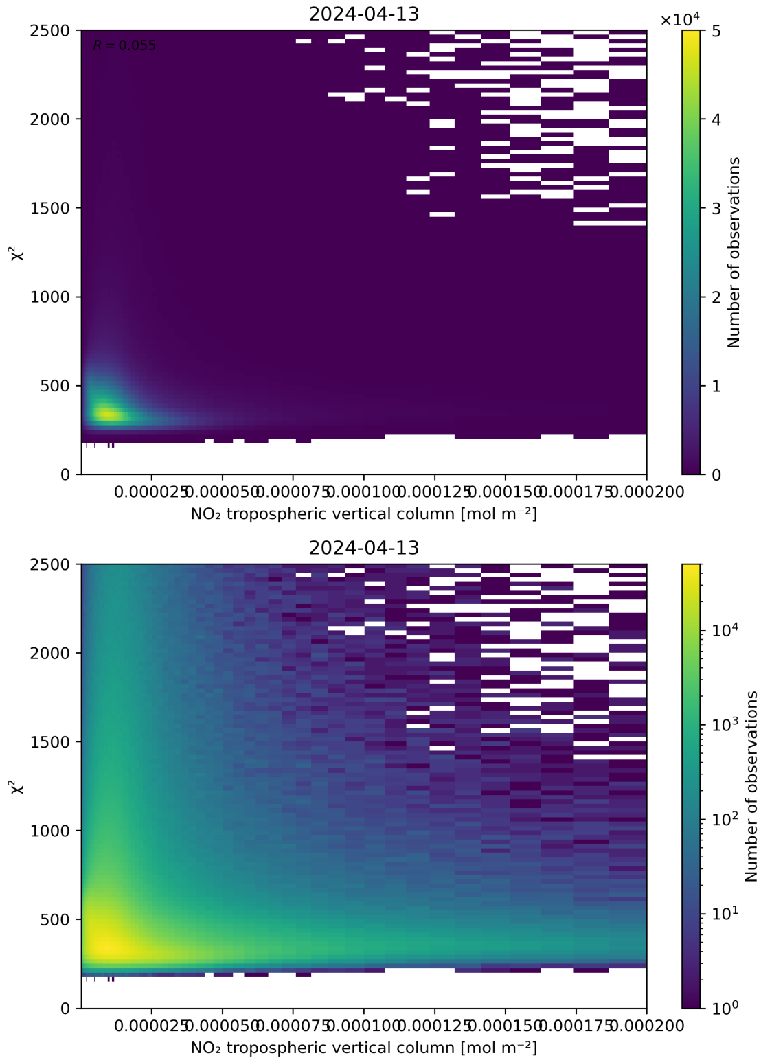
Figure 124: Scatter density plot of “NO 2 tropospheric vertical column” against “ \chi^2 ” for 2024-04-12 to 2024-04-14.
