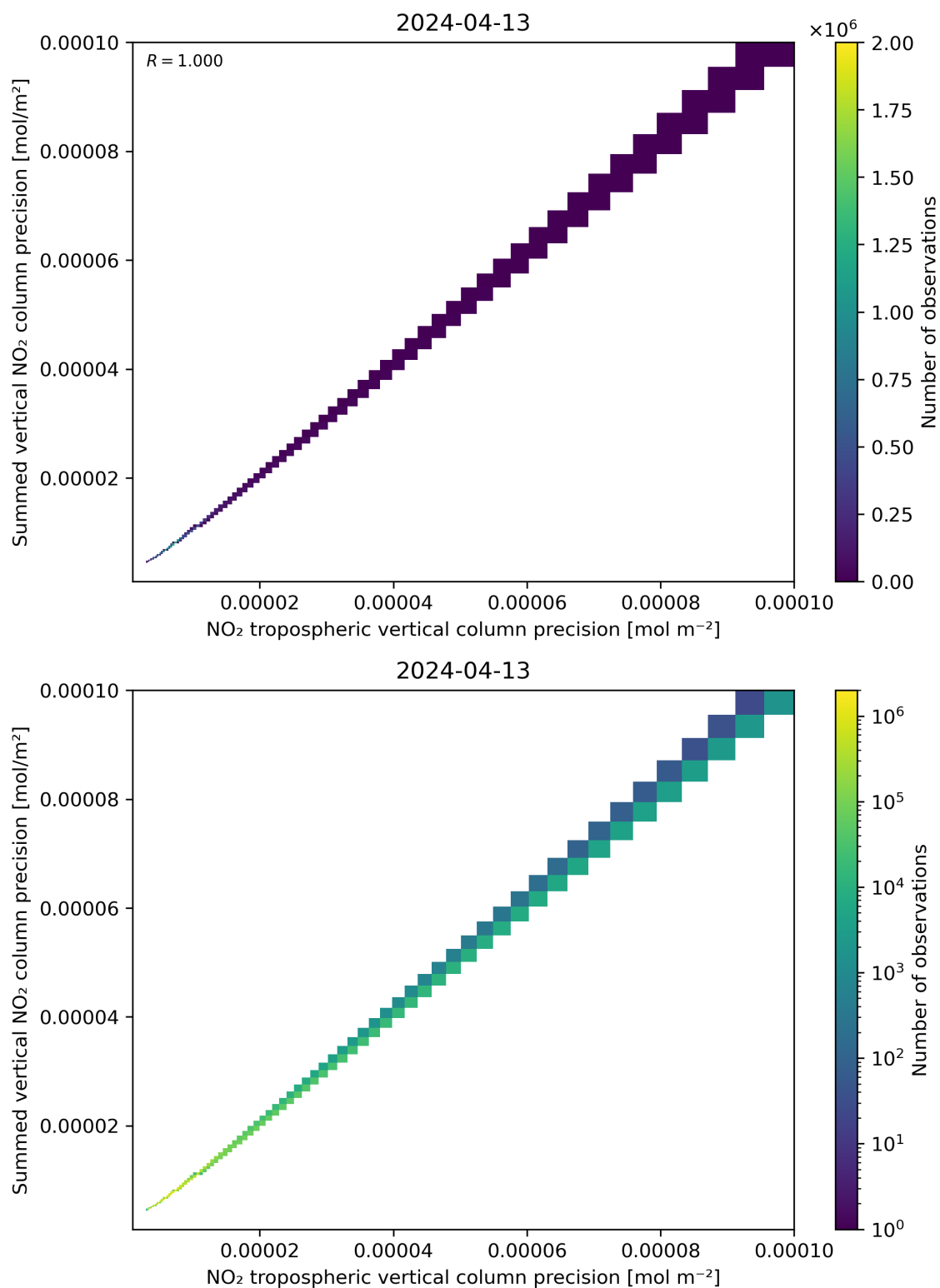
Figure 137: Scatter density plot of “NO 2 tropospheric vertical column precision” against “Summed vertical NO 2 column precision” for 2024-04-12 to 2024-04-14.
