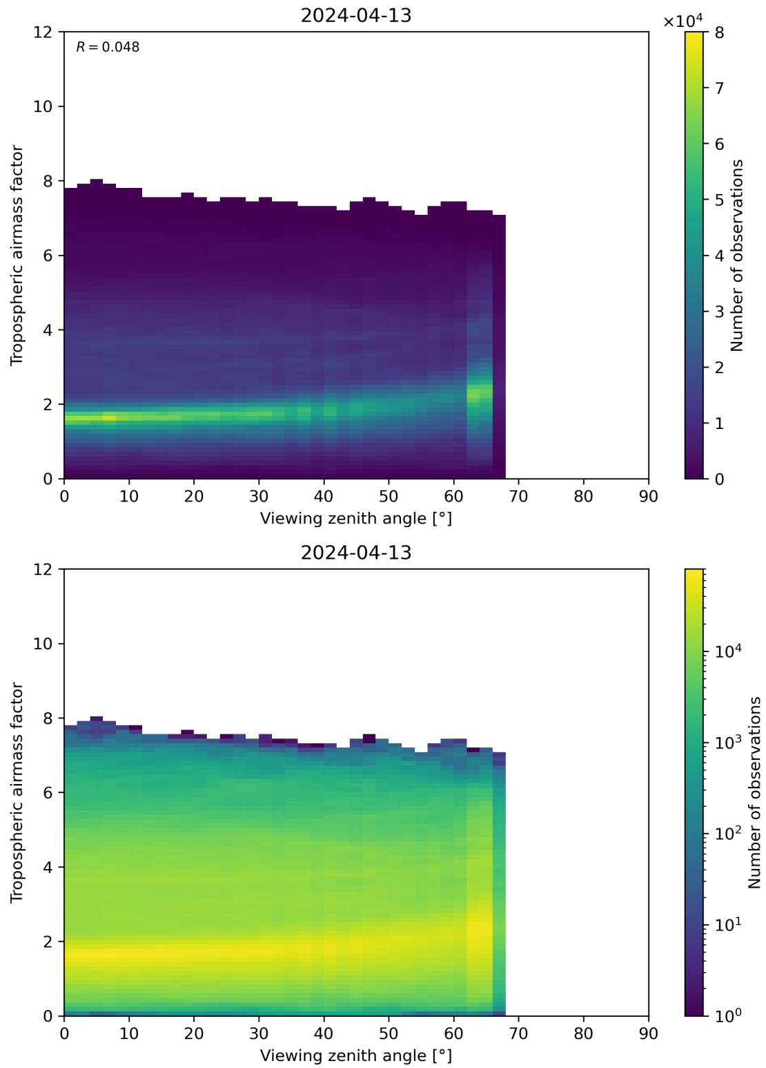
Figure 161: Scatter density plot of “Viewing zenith angle” against “Tropospheric airmass factor” for 2024-04-12 to 2024-04-14.
