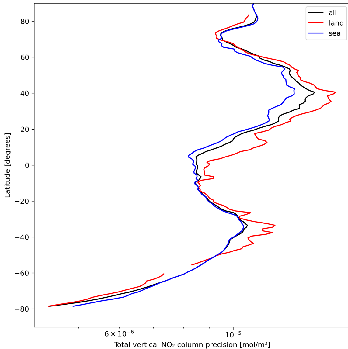
Figure 22: Zonal average of “Total vertical NO 2 column precision” for 2024-04-12 to 2024-04-14.
