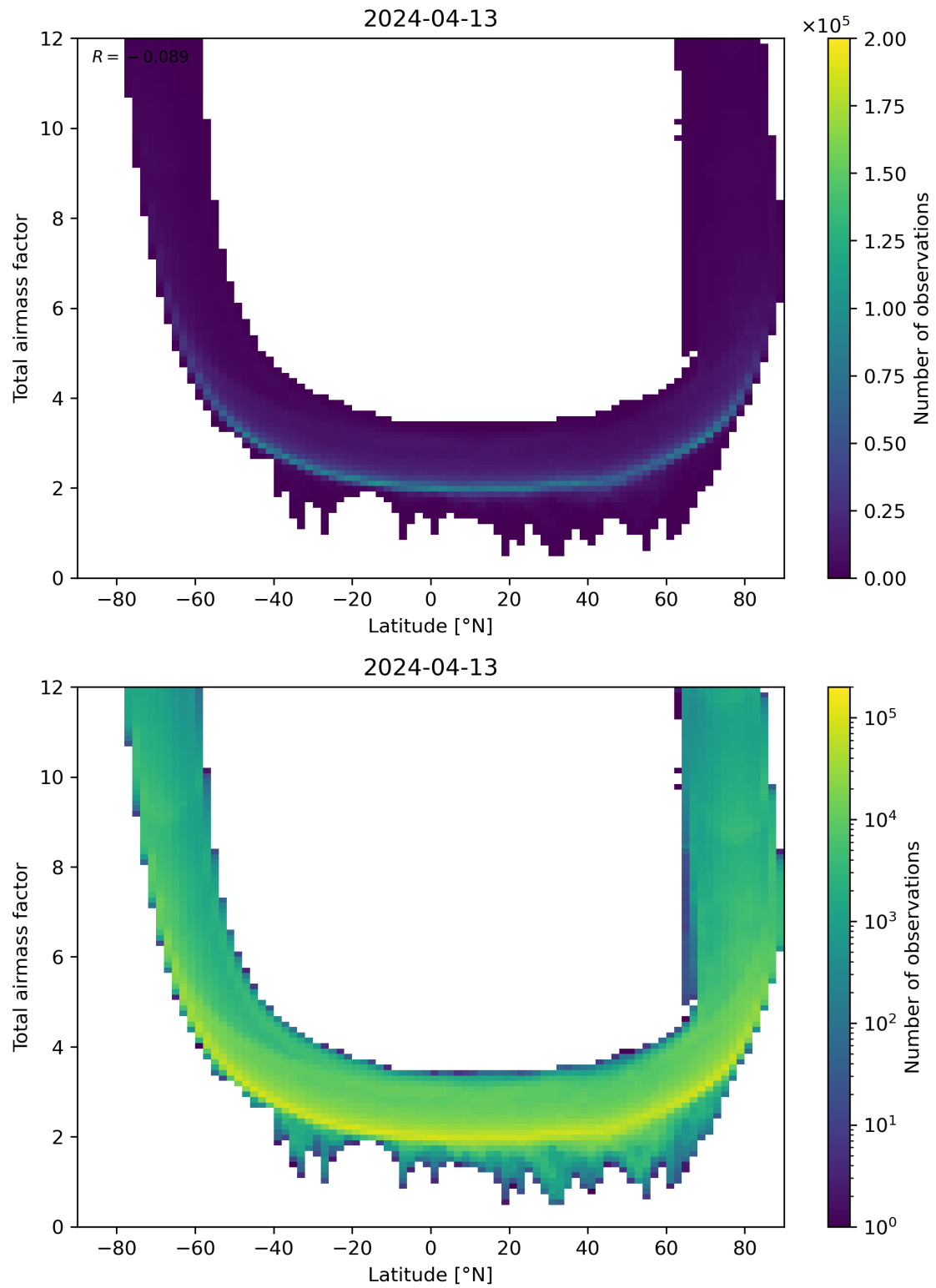
Figure 84: Scatter density plot of “Latitude” against “Total airmass factor” for 2024-04-12 to 2024-04-14.
