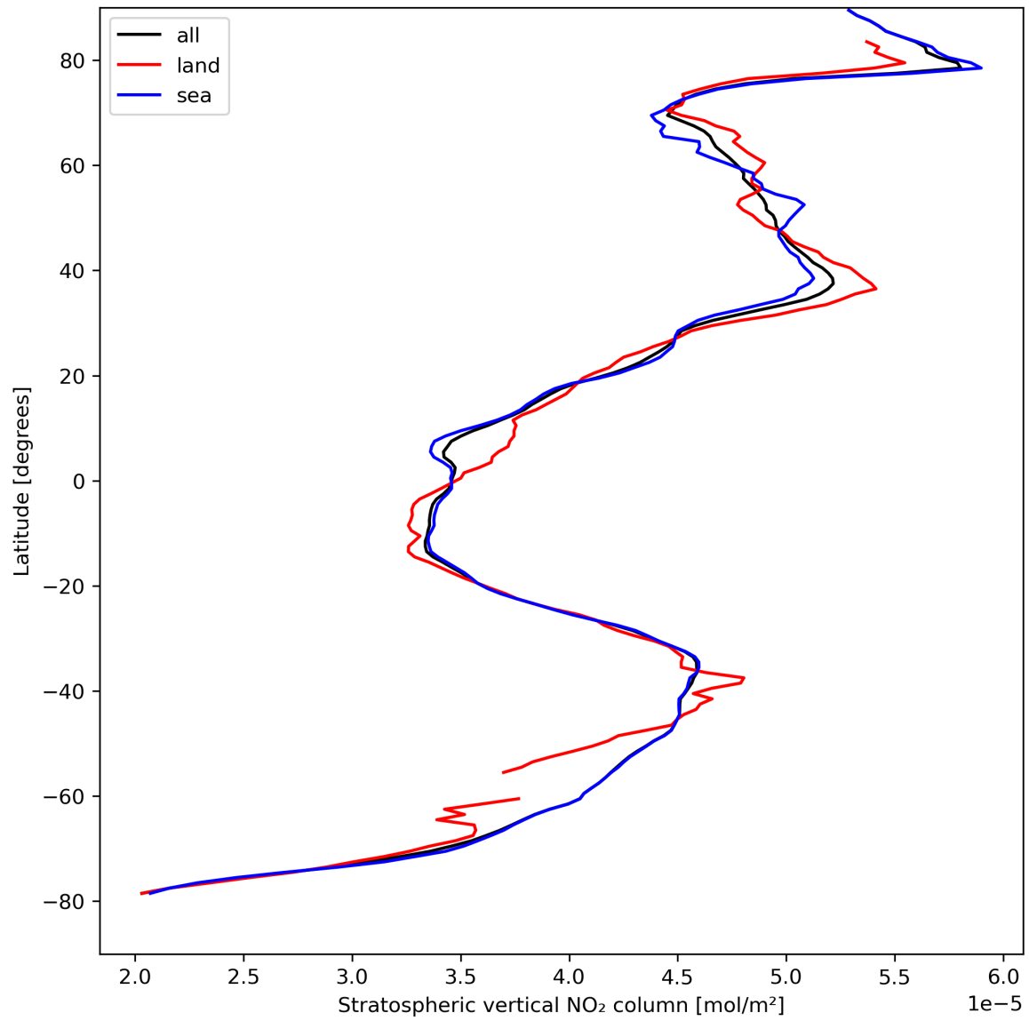
Figure 19: Zonal average of “Stratospheric vertical NO 2 column” for 2024-04-12 to 2024-04-14.
