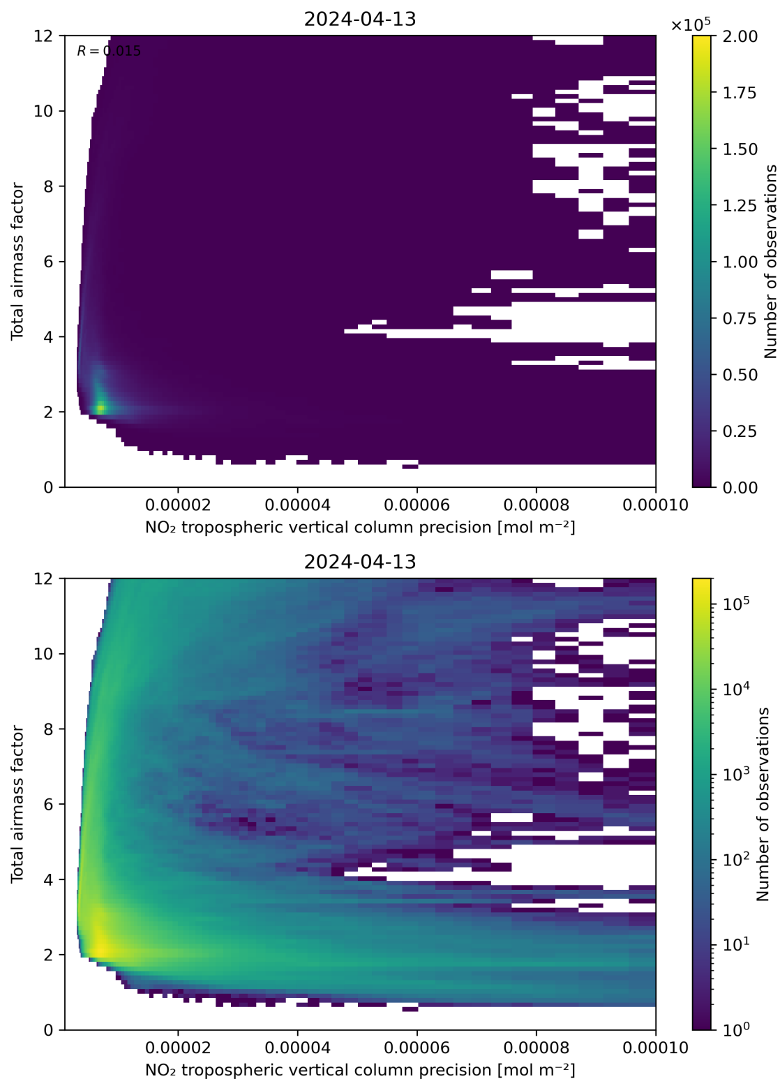
Figure 132: Scatter density plot of “NO 2 tropospheric vertical column precision” against “Total air mass factor” for 2024-04-12 to 2024-04-14.
