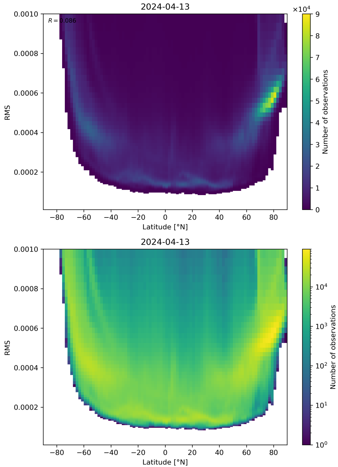
Figure 94: Scatter density plot of “Latitude” against “RMS” for 2024-04-12 to 2024-04-14.
