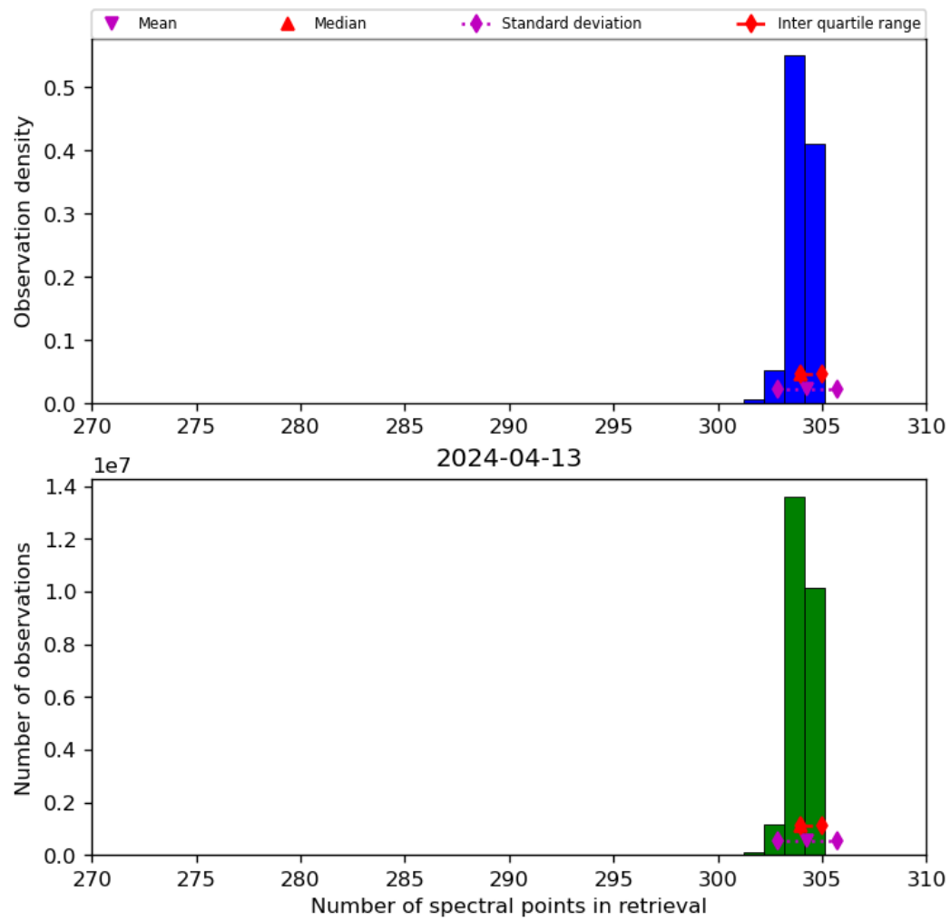
Figure 33: Histogram of “Number of spectral points in retrieval” for 2024-04-12 to 2024-04-14
