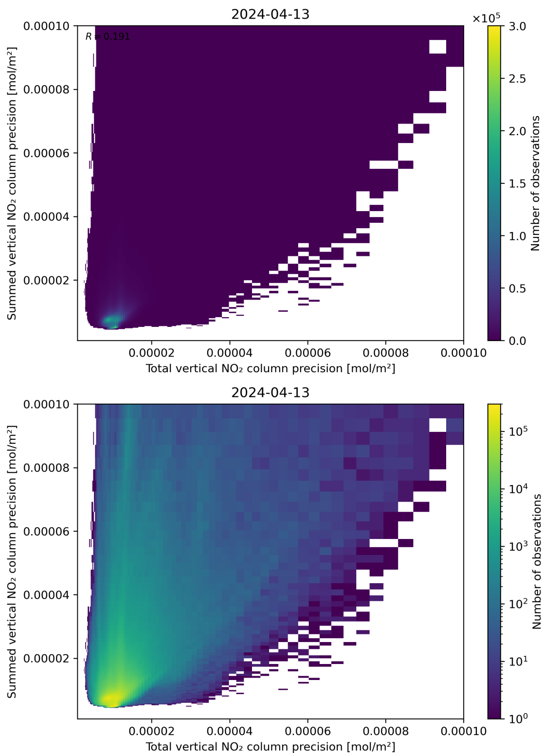
Figure 118: Scatter density plot of “Total vertical NO 2 column precision” against “Summed vertical NO 2 column precision” for 2024-04-12 to 2024-04-14.
