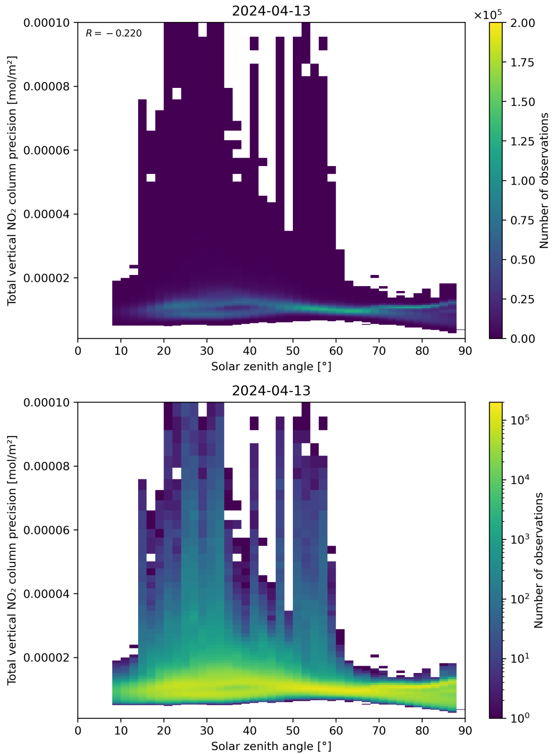
Figure 154: Scatter density plot of “Solar zenith angle” against “Total vertical NO 2 column precision” for 2024-04-12 to 2024-04-14.
