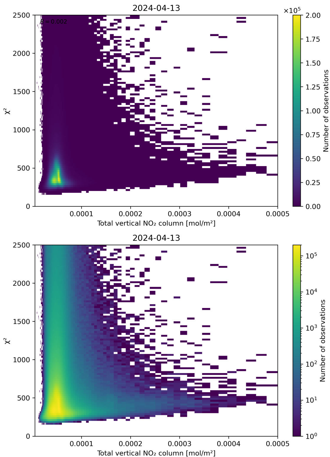
Figure 111: Scatter density plot of “Total vertical NO 2 column” against “ \chi^2 ” for 2024-04-12 to 2024-04-14.
