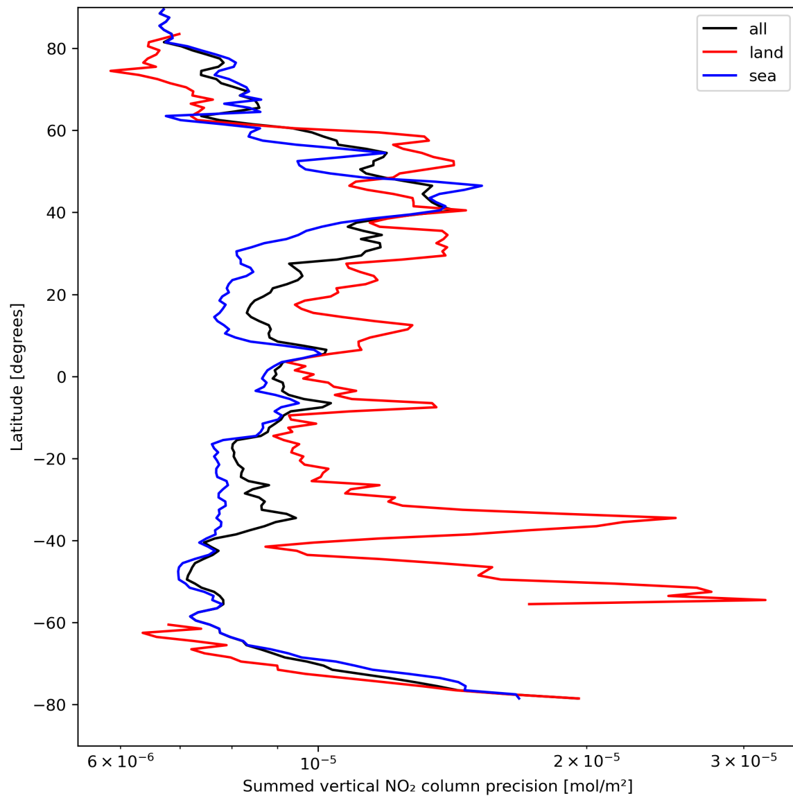
Figure 24: Zonal average of “Summed vertical NO 2 column precision” for 2024-04-12 to 2024-04-14.
