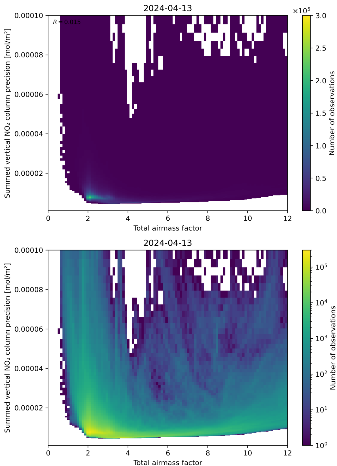
Figure 66: Scatter density plot of “Total airmass factor” against “Summed vertical NO 2 column precision” for 2024-04-12 to 2024-04-14.
