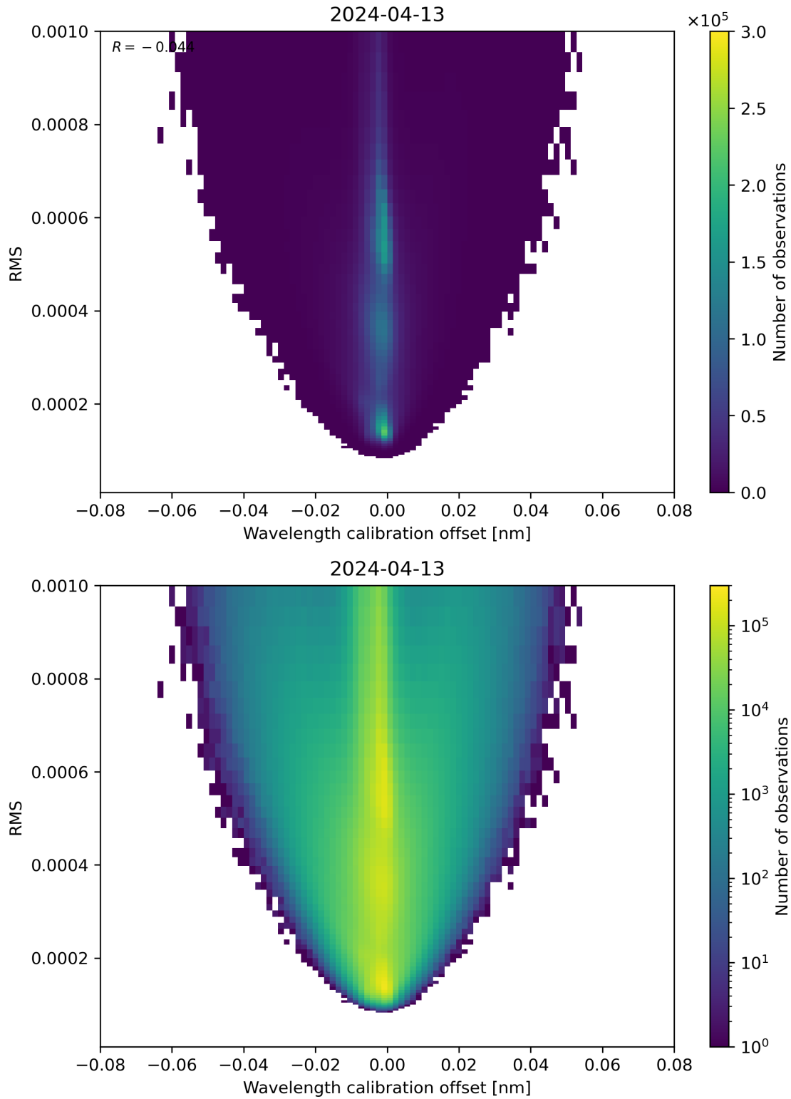
Figure 181: Scatter density plot of “Wavelength calibration offset” against “RMS” for 2024-04-12 to 2024-04-14.
