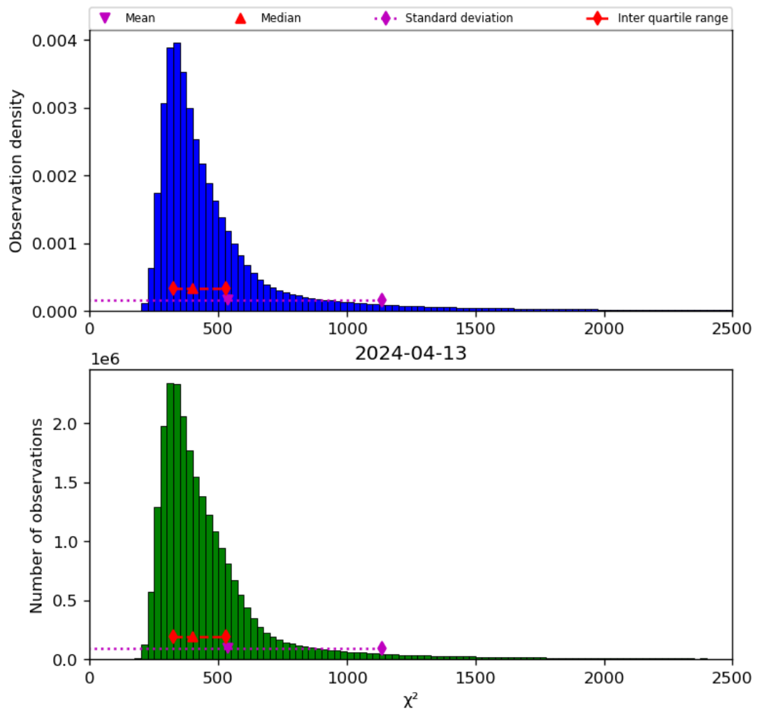
Figure 42: Histogram of “ \chi^2 ” for 2024-04-12 to 2024-04-14
