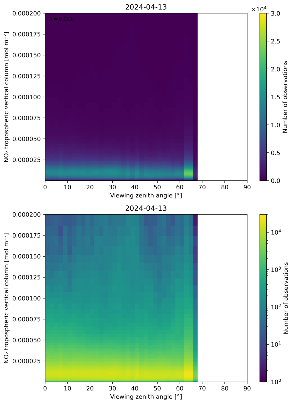
Figure 169: Scatter density plot of “Viewing zenith angle” against “NO 2 tropospheric vertical column” for 2024-04-12 to 2024-04-14.
