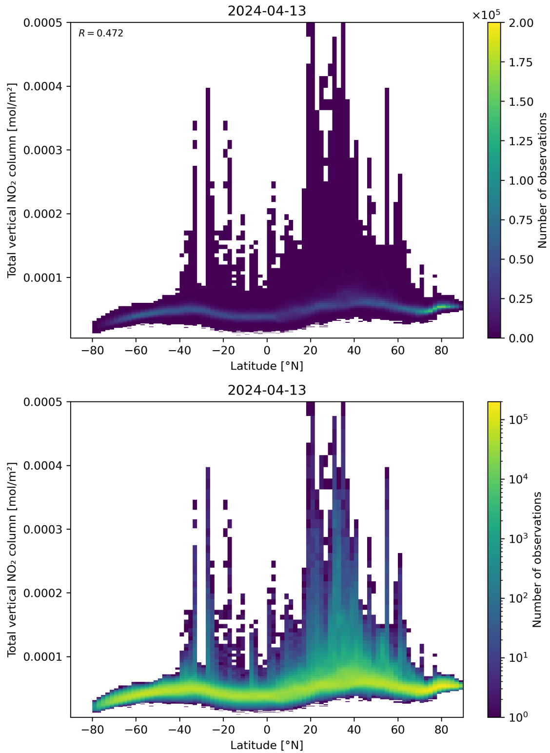
Figure 90: Scatter density plot of “Latitude” against “Total vertical NO 2 column” for 2024-04-12 to 2024-04-14.
