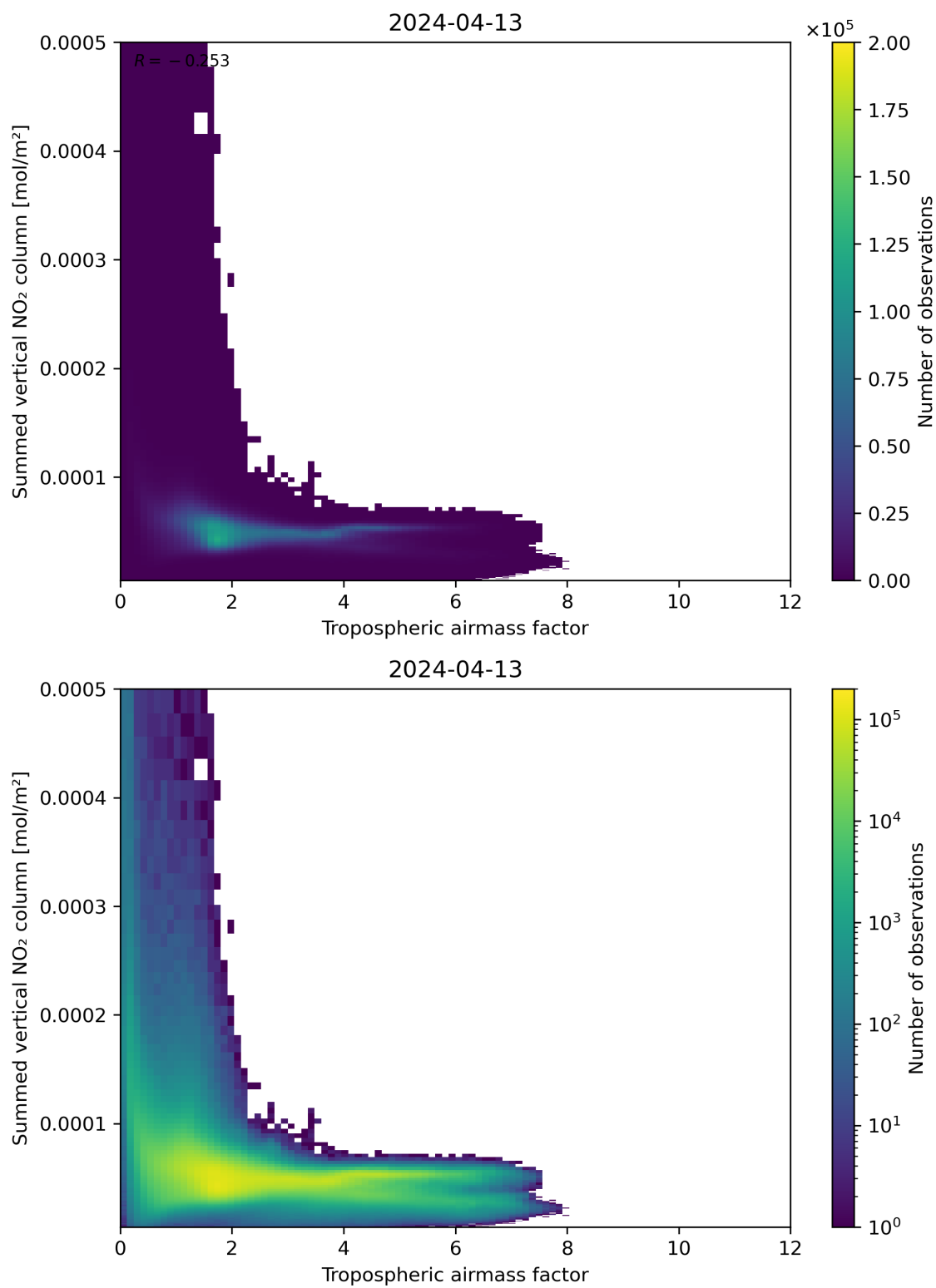
Figure 75: Scatter density plot of “Tropospheric airmass factor” against “Summed vertical NO 2 column” for 2024-04-12 to 2024-04-14.
