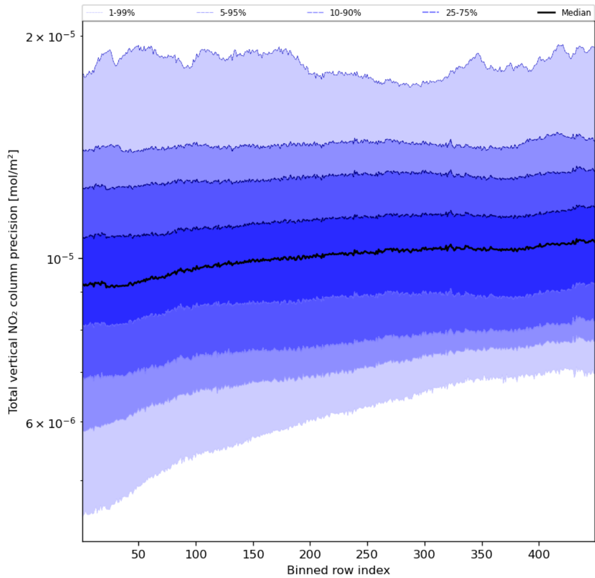
Figure 56: Along track statistics of “Total vertical NO 2 column precision” for 2024-04-12 to 2024-04-14
