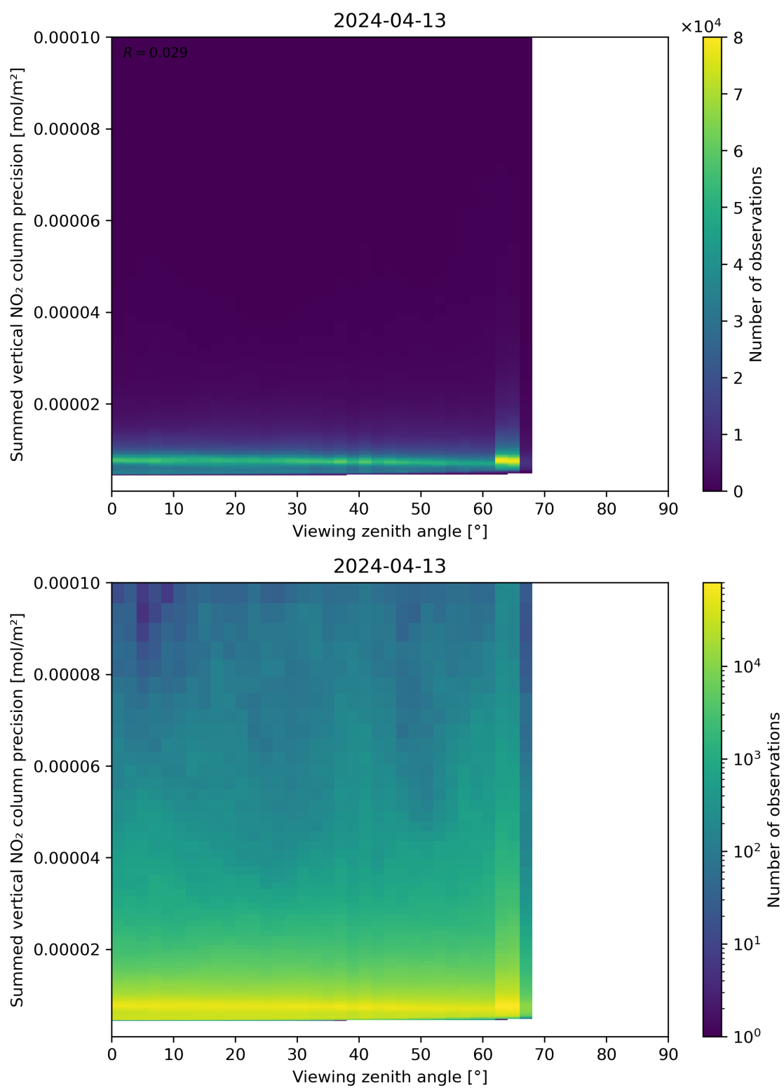
Figure 166: Scatter density plot of “Viewing zenith angle” against “Summed vertical NO 2 column precision” for 2024-04-12 to 2024-04-14.
