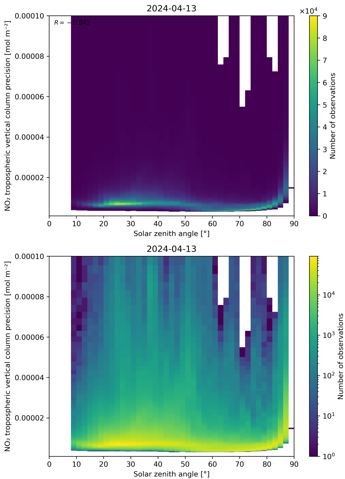
Figure 156: Scatter density plot of “Solar zenith angle” against “NO 2 tropospheric vertical column precision” for 2024-04-12 to 2024-04-14.
