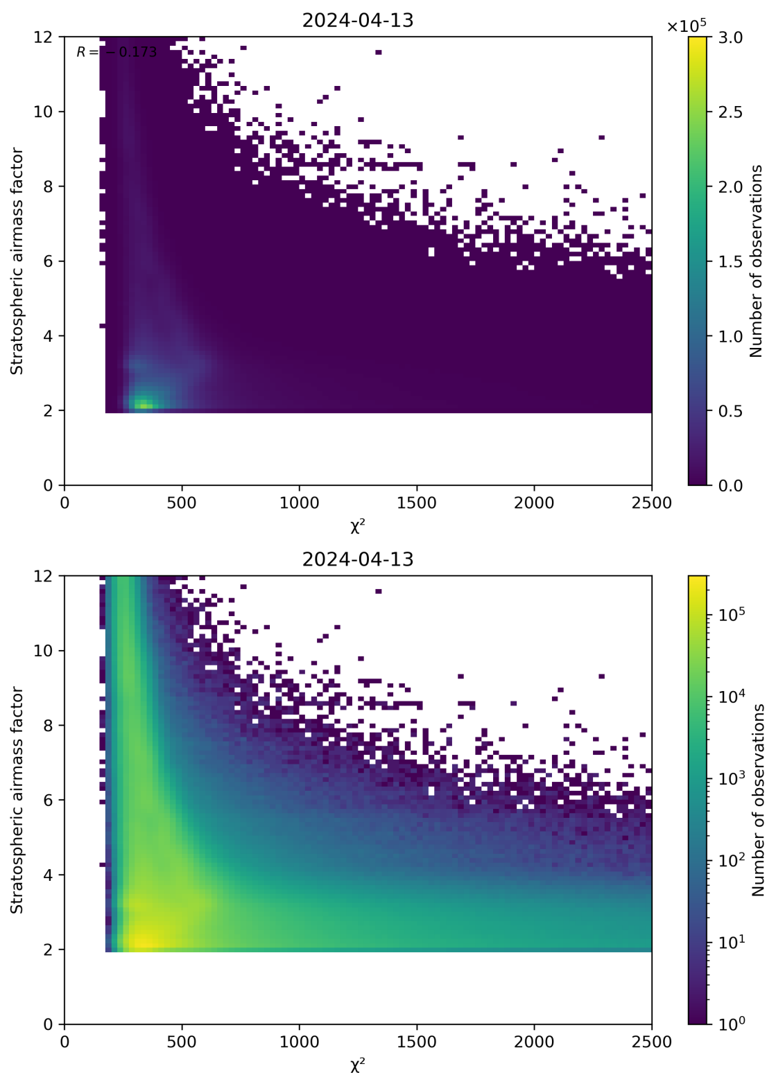
Figure 81: Scatter density plot of “ \chi^2 ” against “Stratospheric air mass factor” for 2024-04-12 to 2024-04-14.
