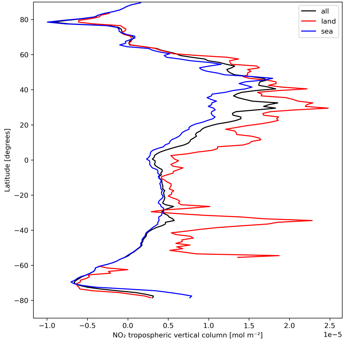
Figure 12: Zonal average of “NO 2 tropospheric vertical column” for 2024-04-12 to 2024-04-14.
