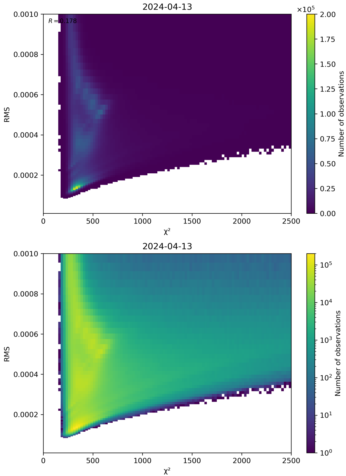
Figure 82: Scatter density plot of “ \chi^2 ” against “RMS” for 2024-04-12 to 2024-04-14.
