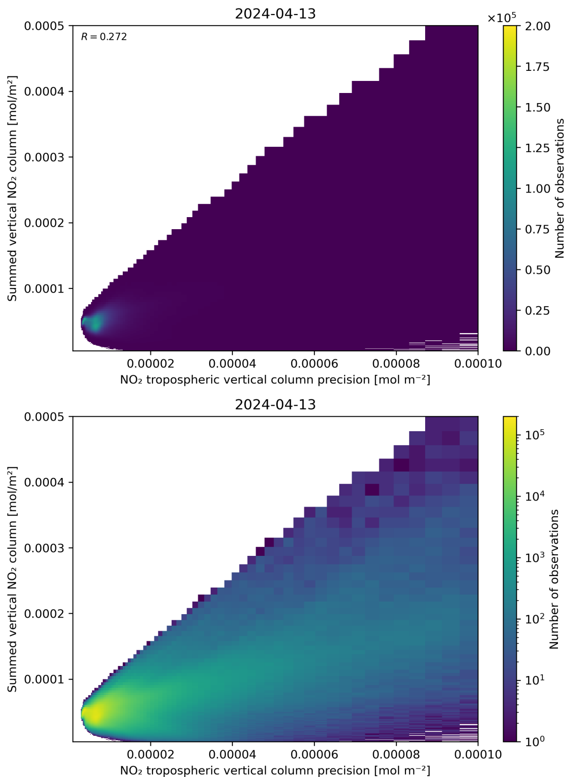
Figure 136: Scatter density plot of “NO 2 tropospheric vertical column precision” against “Summed vertical NO 2 column” for 2024-04-12 to 2024-04-14.
