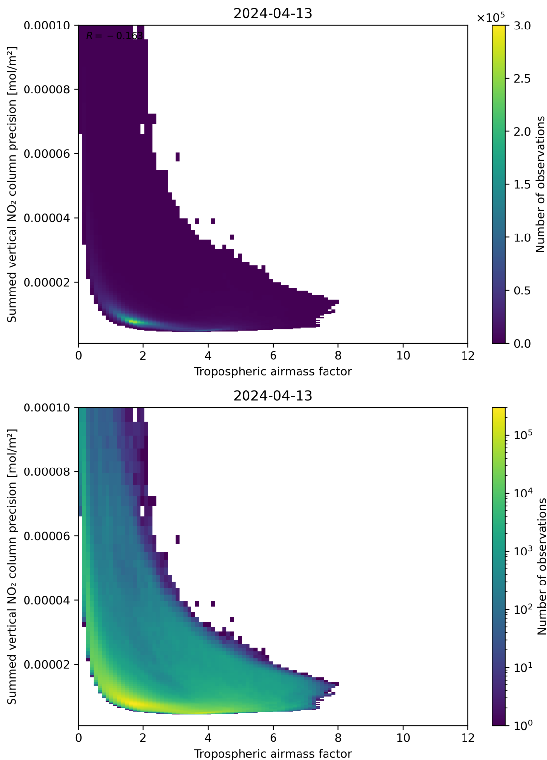
Figure 76: Scatter density plot of “Tropospheric air mass factor” against “Summed vertical NO 2 column precision” for 2024-04-12 to 2024-04-14.
