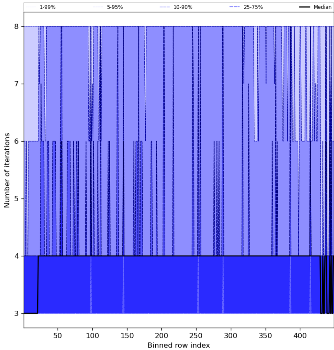
Figure 51: Along track statistics of “Number of iterations” for 2024-04-12 to 2024-04-14
