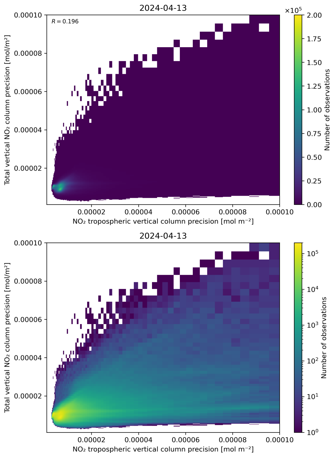
Figure 139: Scatter density plot of “NO 2 tropospheric vertical column precision” against “Total vertical NO 2 column precision” for 2024-04-12 to 2024-04-14.
