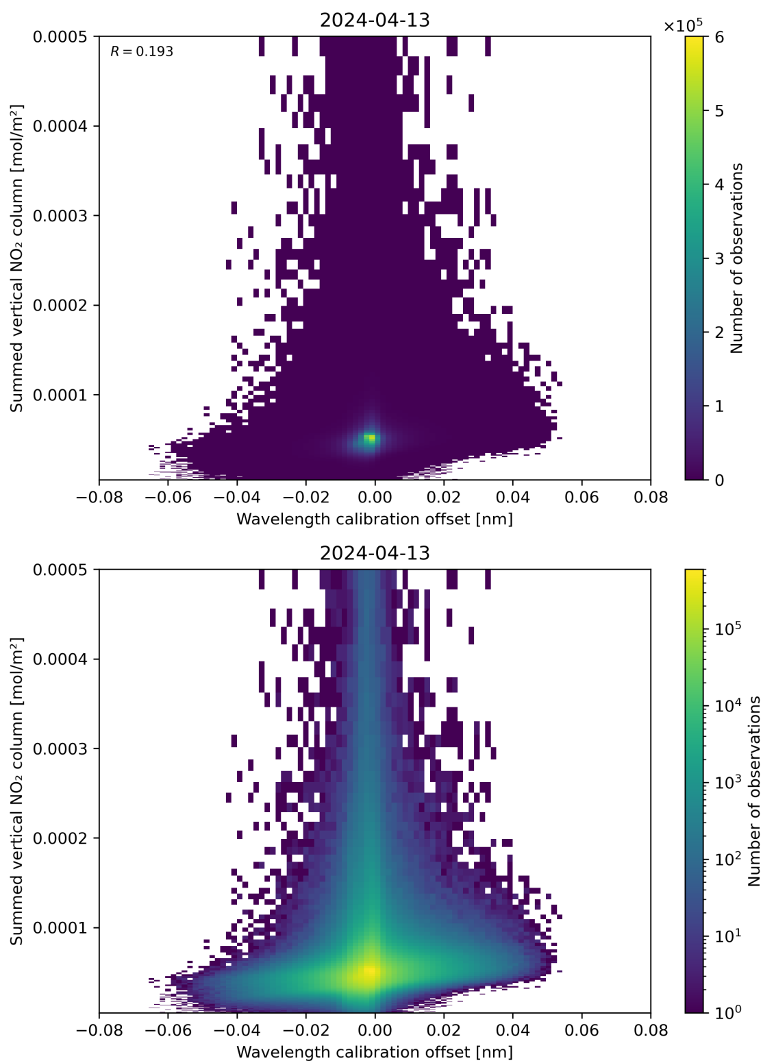
Figure 177: Scatter density plot of “Wavelength calibration offset” against “Summed vertical NO 2 column” for 2024-04-12 to 2024-04-14.
