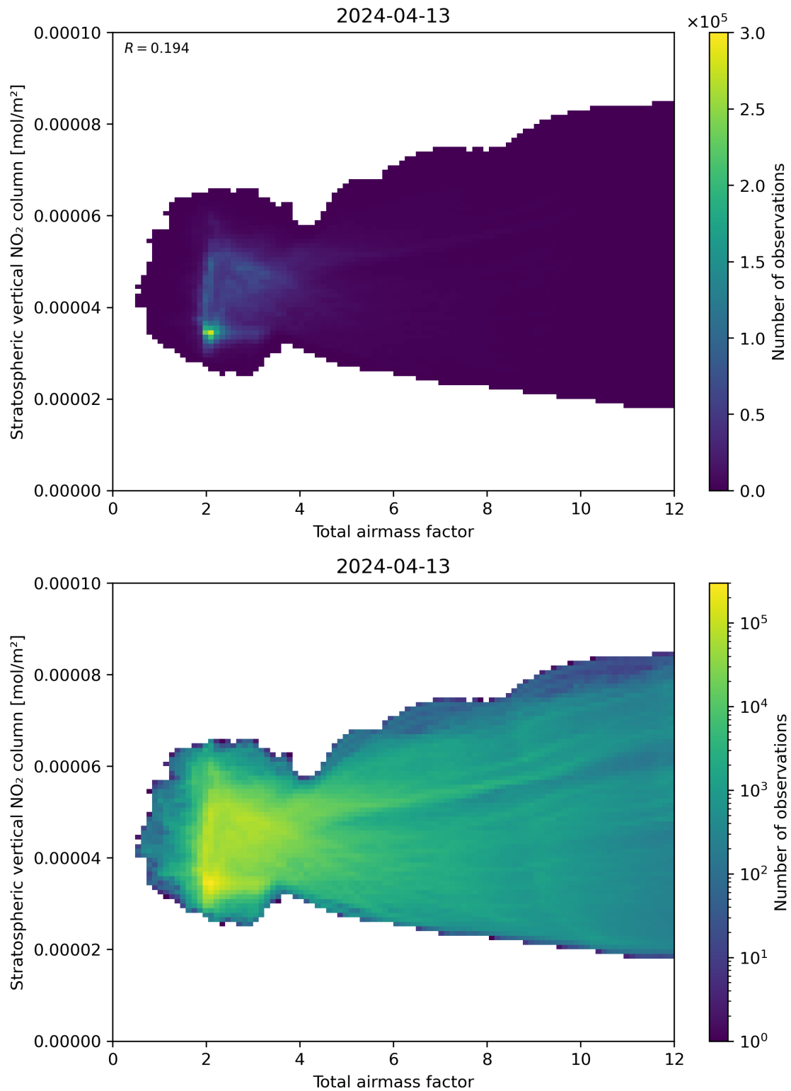
Figure 64: Scatter density plot of “Total airmass factor” against “Stratospheric vertical \text{NO}_2 column” for 2024-04-12 to 2024-04-14.
