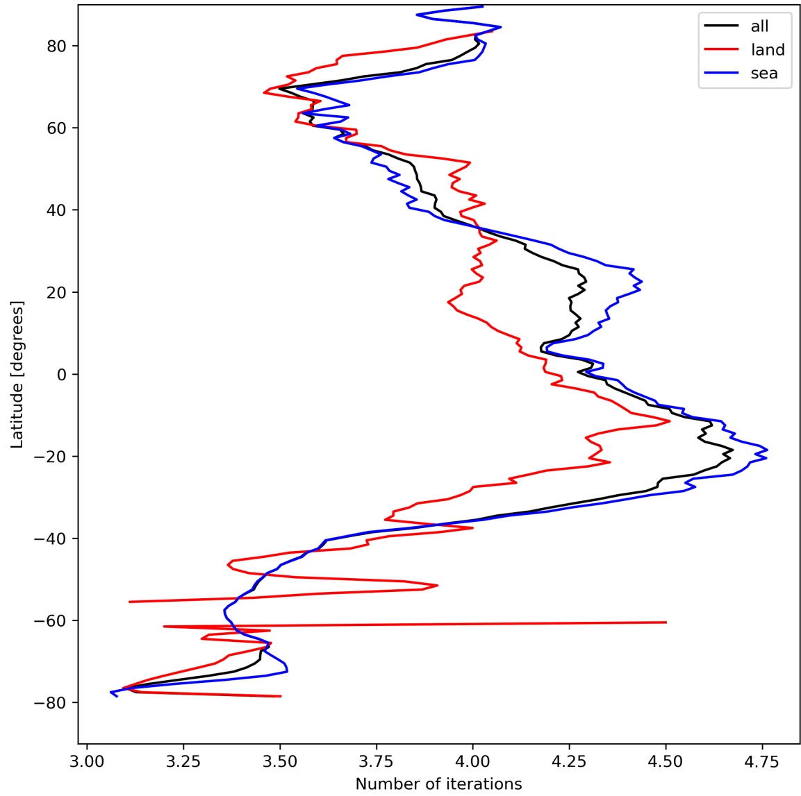
Figure 17: Zonal average of “Number of iterations” for 2024-04-12 to 2024-04-14.
