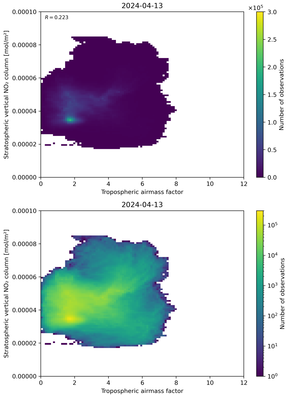
Figure 74: Scatter density plot of “Tropospheric air mass factor” against “Stratospheric vertical NO 2 column” for 2024-04-12 to 2024-04-14.
