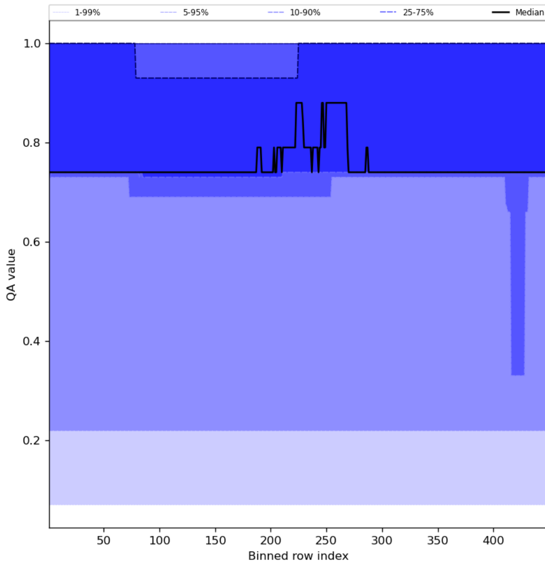
Figure 45: Along track statistics of “QA value” for 2024-04-12 to 2024-04-14
