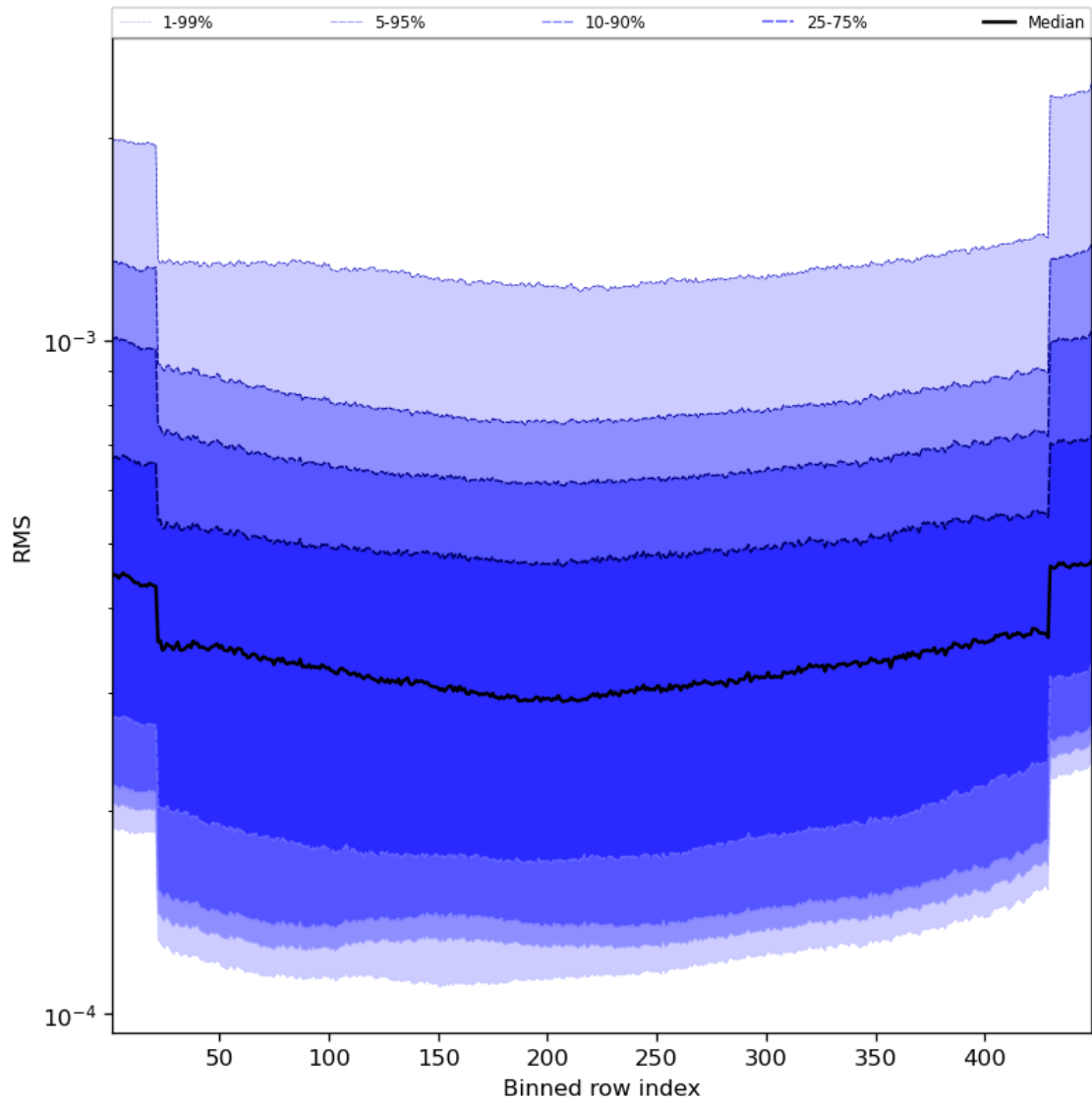
Figure 60: Along track statistics of “RMS” for 2024-04-12 to 2024-04-14
