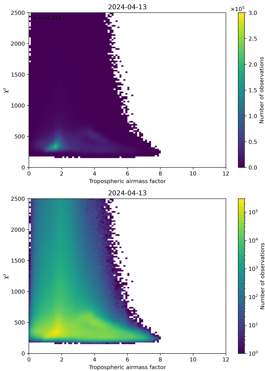
Figure 73: Scatter density plot of “Tropospheric airmass factor” against “ \chi^2 ” for 2024-04-12 to 2024-04-14.
