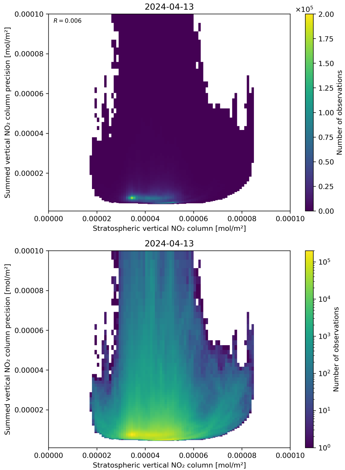
Figure 99: Scatter density plot of “Stratospheric vertical NO 2 column” against “Summed vertical NO 2 column precision” for 2024-04-12 to 2024-04-14.
