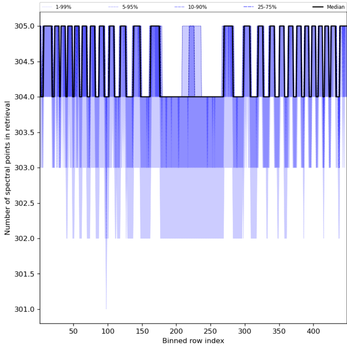
Figure 50: Along track statistics of “Number of spectral points in retrieval” for 2024-04-12 to 2024-04-14
