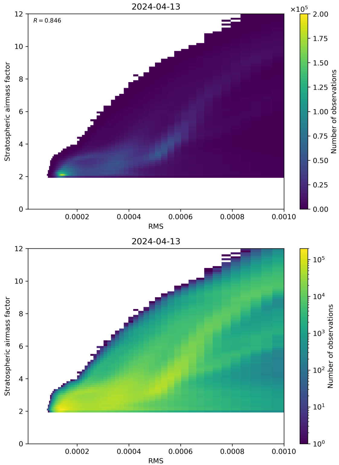
Figure 144: Scatter density plot of “RMS” against “Stratospheric airmass factor” for 2024-04-12 to 2024-04-14.
