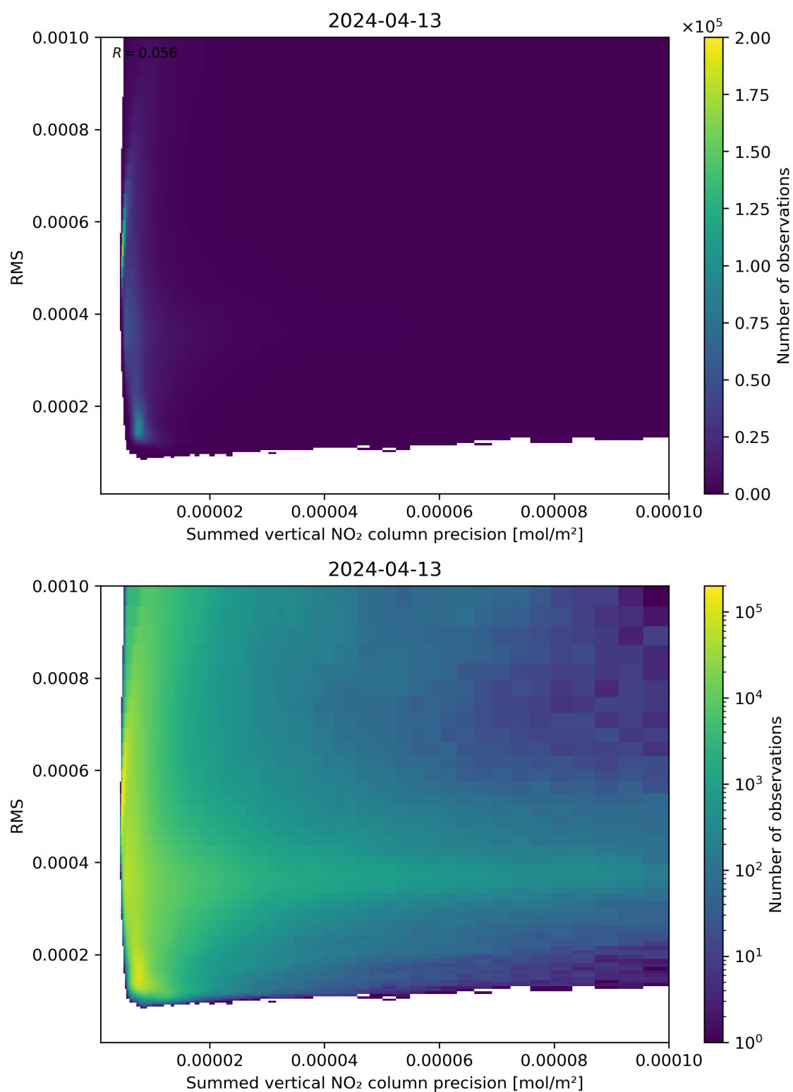
Figure 108: Scatter density plot of “Summed vertical NO 2 column precision” against “RMS” for 2024-04-12 to 2024-04-14.
