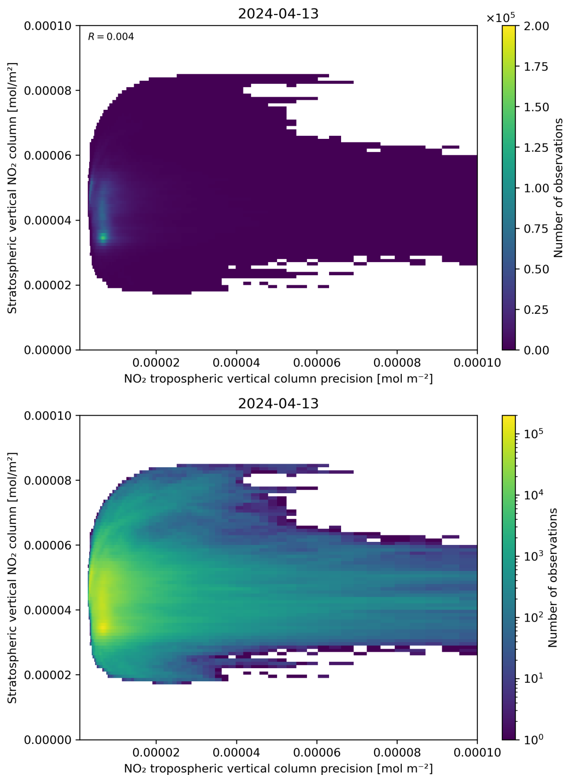
Figure 135: Scatter density plot of “NO 2 tropospheric vertical column precision” against “Stratospheric vertical NO 2 column” for 2024-04-12 to 2024-04-14.
