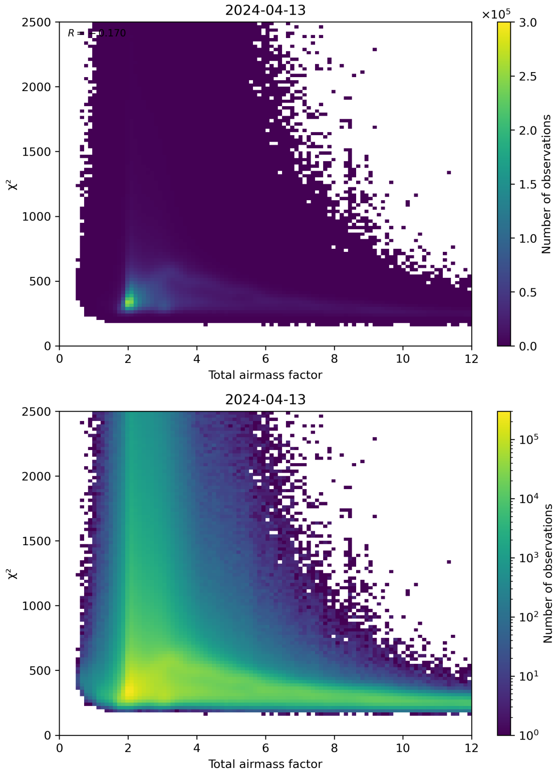
Figure 63: Scatter density plot of “Total airmass factor” against “ \chi^2 ” for 2024-04-12 to 2024-04-14.
