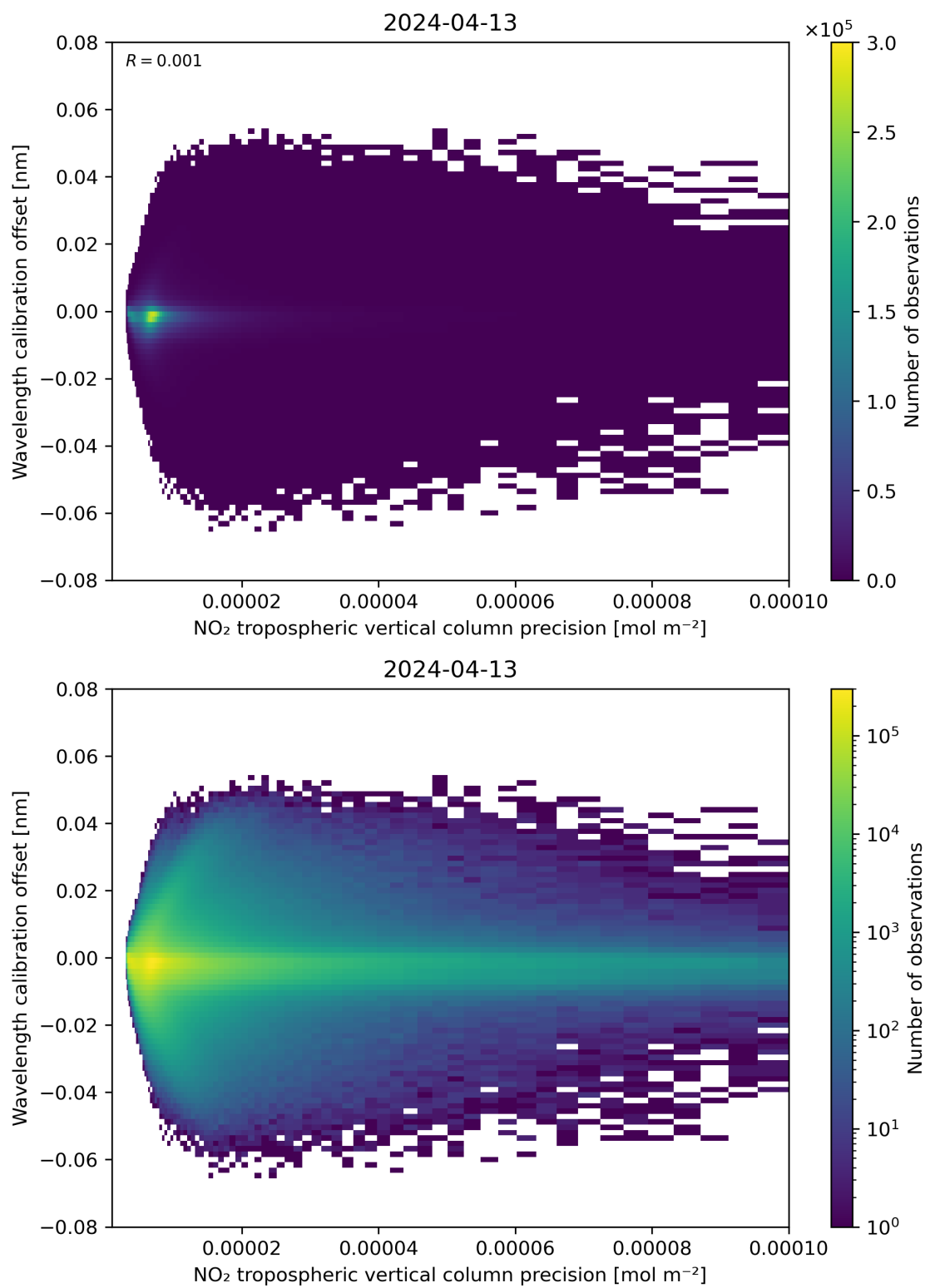
Figure 141: Scatter density plot of “NO 2 tropospheric vertical column precision” against “Wavelength calibration offset” for 2024-04-12 to 2024-04-14.
