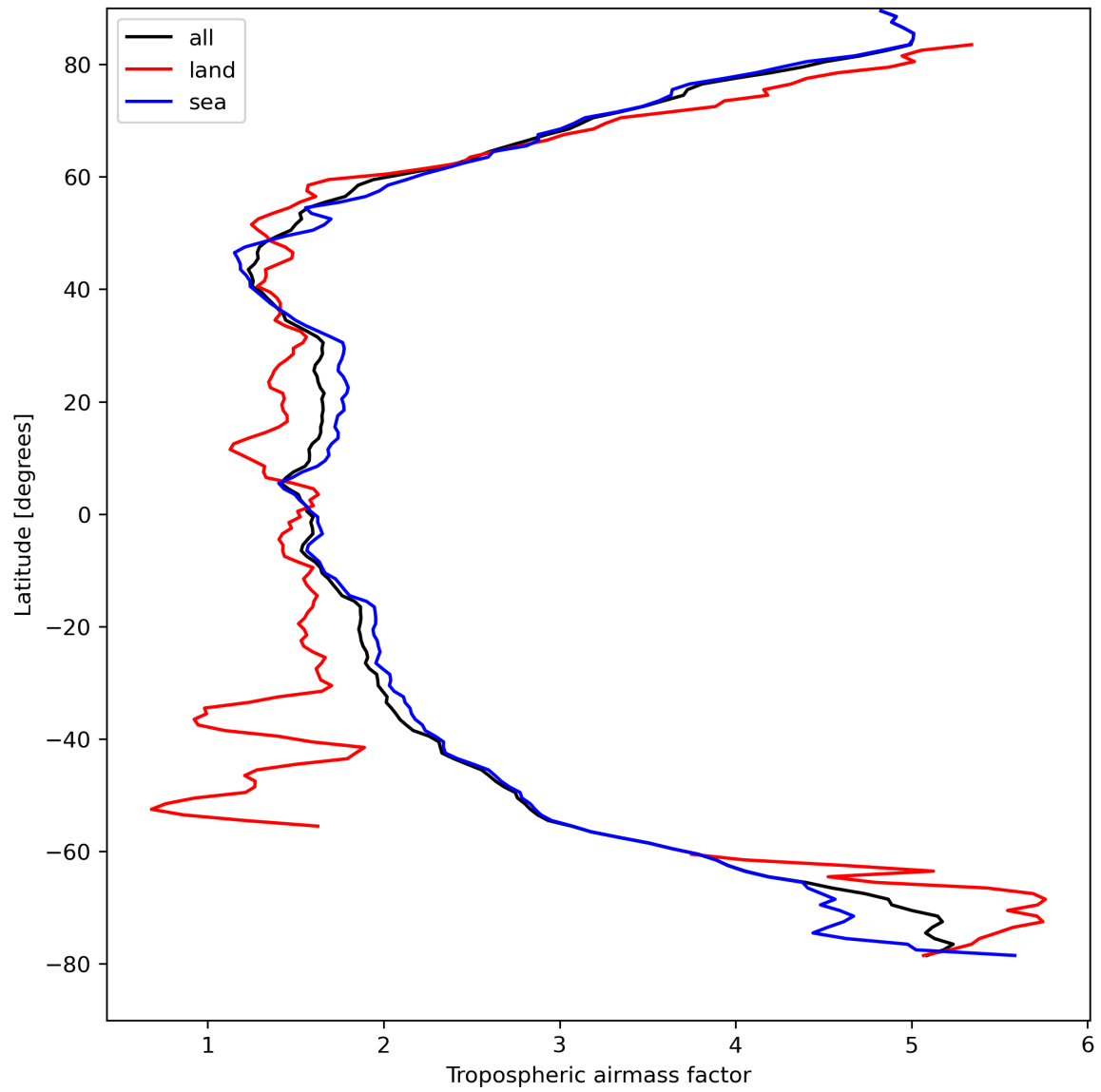
Figure 14: Zonal average of “Tropospheric air mass factor” for 2024-04-12 to 2024-04-14.
