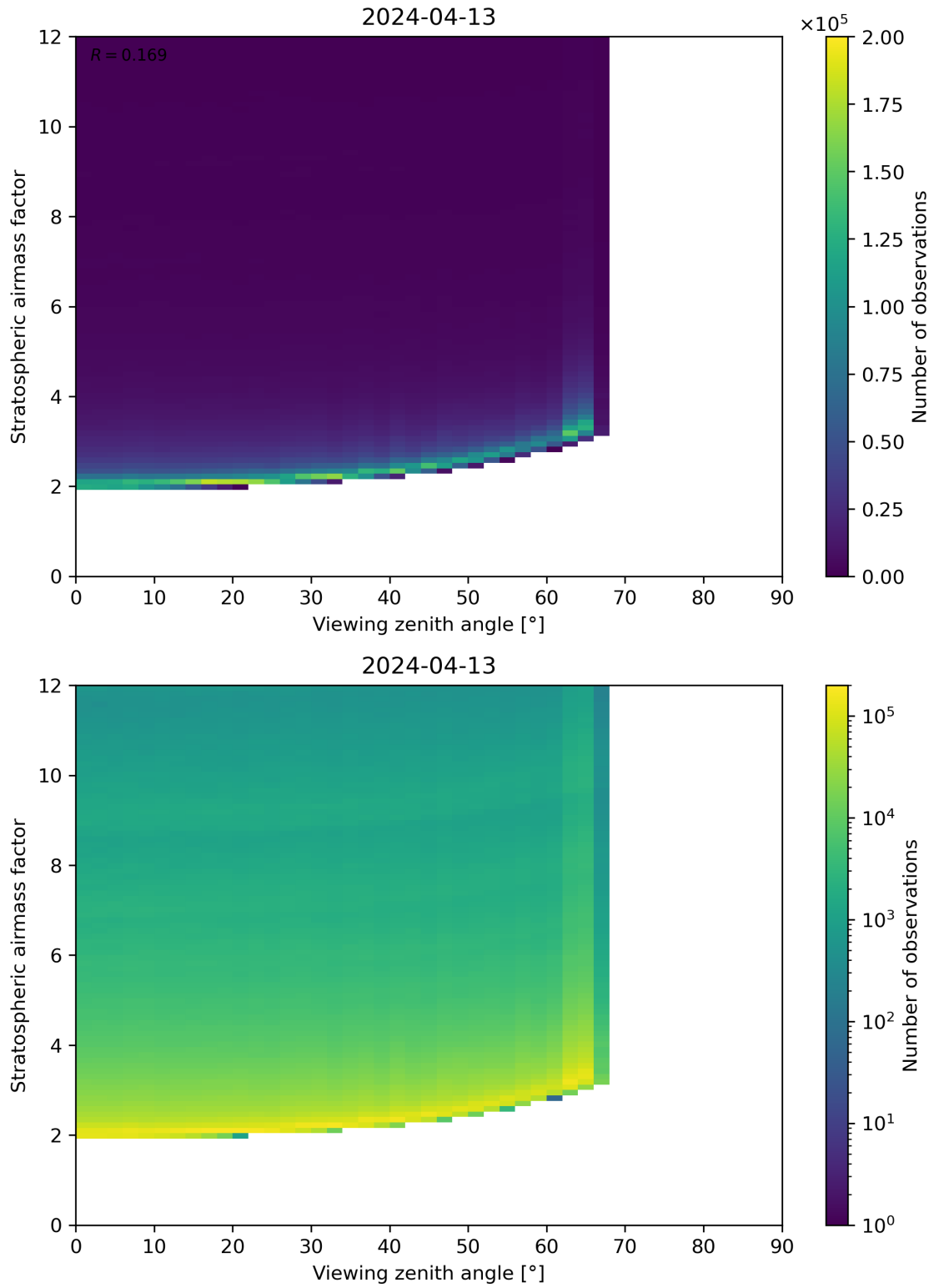
Figure 159: Scatter density plot of “Viewing zenith angle” against “Stratospheric airmass factor” for 2024-04-12 to 2024-04-14.
