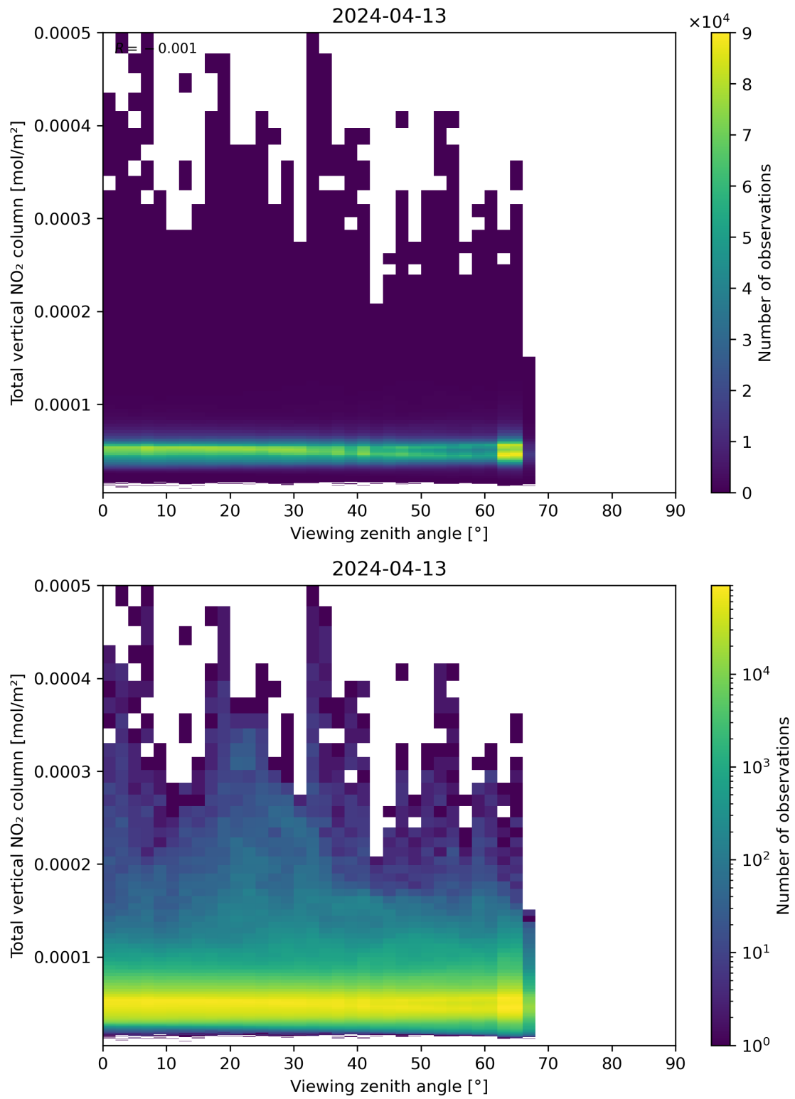
Figure 167: Scatter density plot of “Viewing zenith angle” against “Total vertical NO 2 column” for 2024-04-12 to 2024-04-14.
