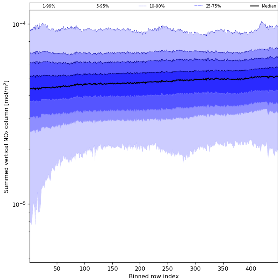
Figure 57: Along track statistics of “Summed vertical NO 2 column” for 2024-04-12 to 2024-04-14
