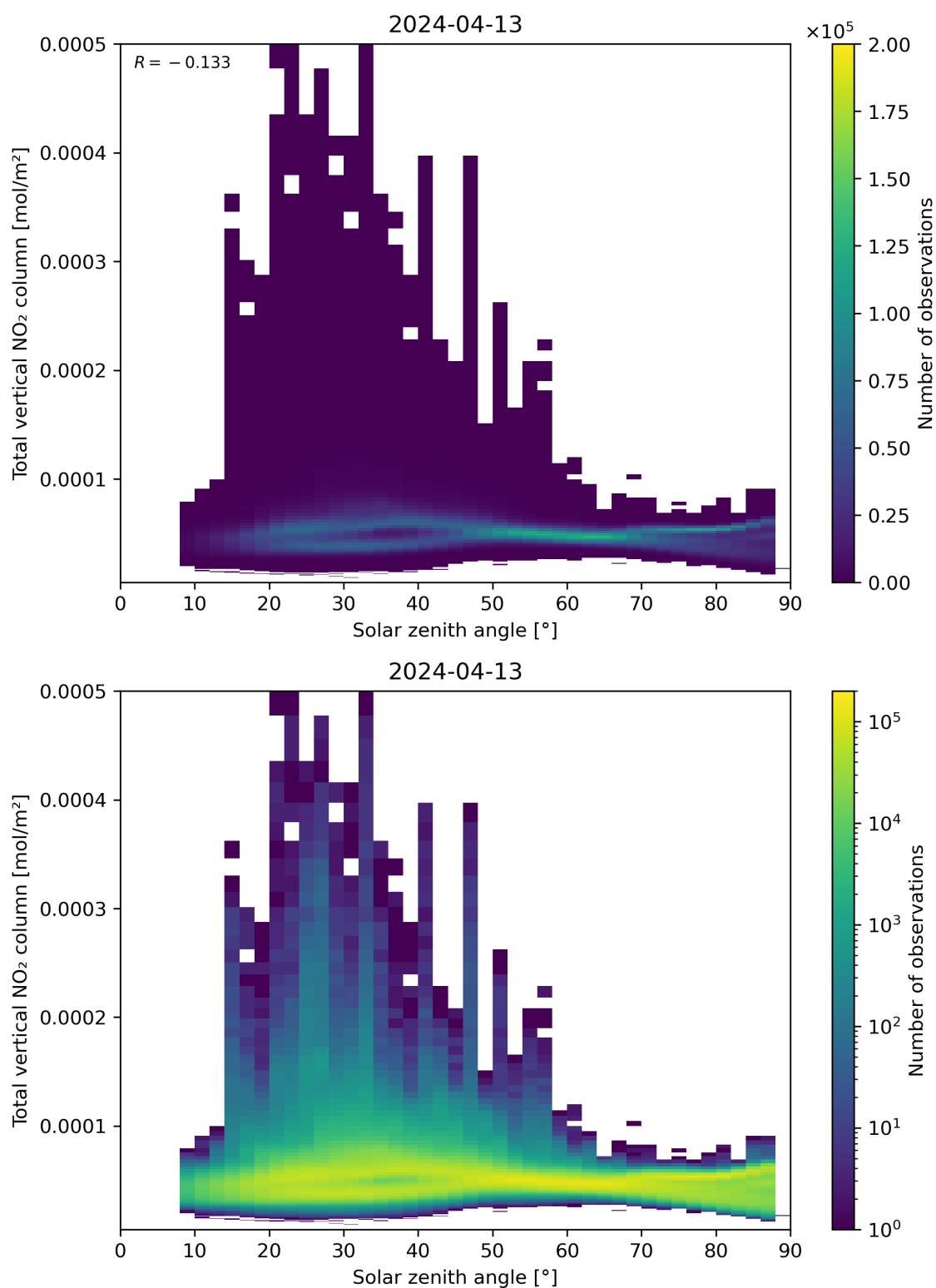
Figure 153: Scatter density plot of “Solar zenith angle” against “Total vertical NO 2 column” for 2024-04-12 to 2024-04-14.
