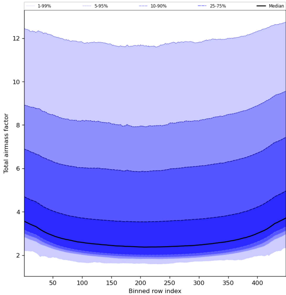
Figure 49: Along track statistics of “Total airmass factor” for 2024-04-12 to 2024-04-14
