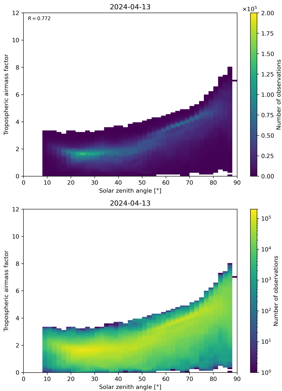
Figure 147: Scatter density plot of “Solar zenith angle” against “Tropospheric airmass factor” for 2024-04-12 to 2024-04-14.
