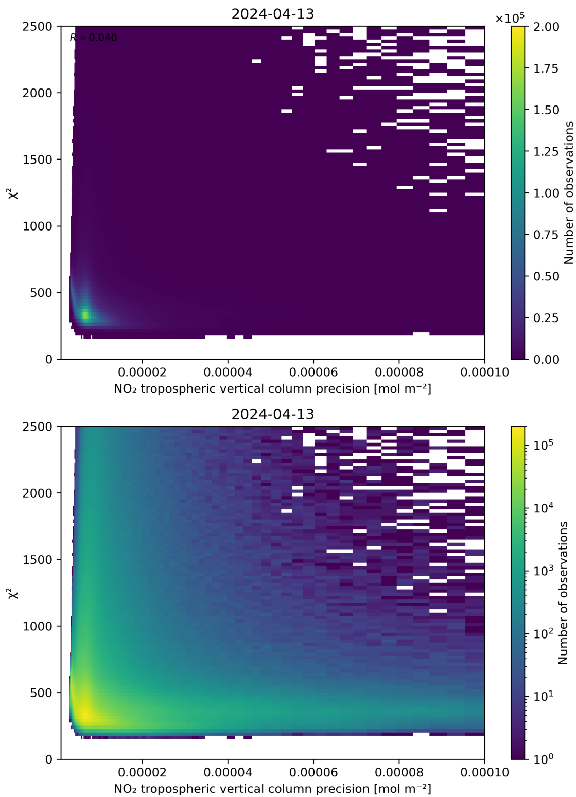
Figure 134: Scatter density plot of “NO 2 tropospheric vertical column precision” against “ \chi^2 ” for 2024-04-12 to 2024-04-14.
