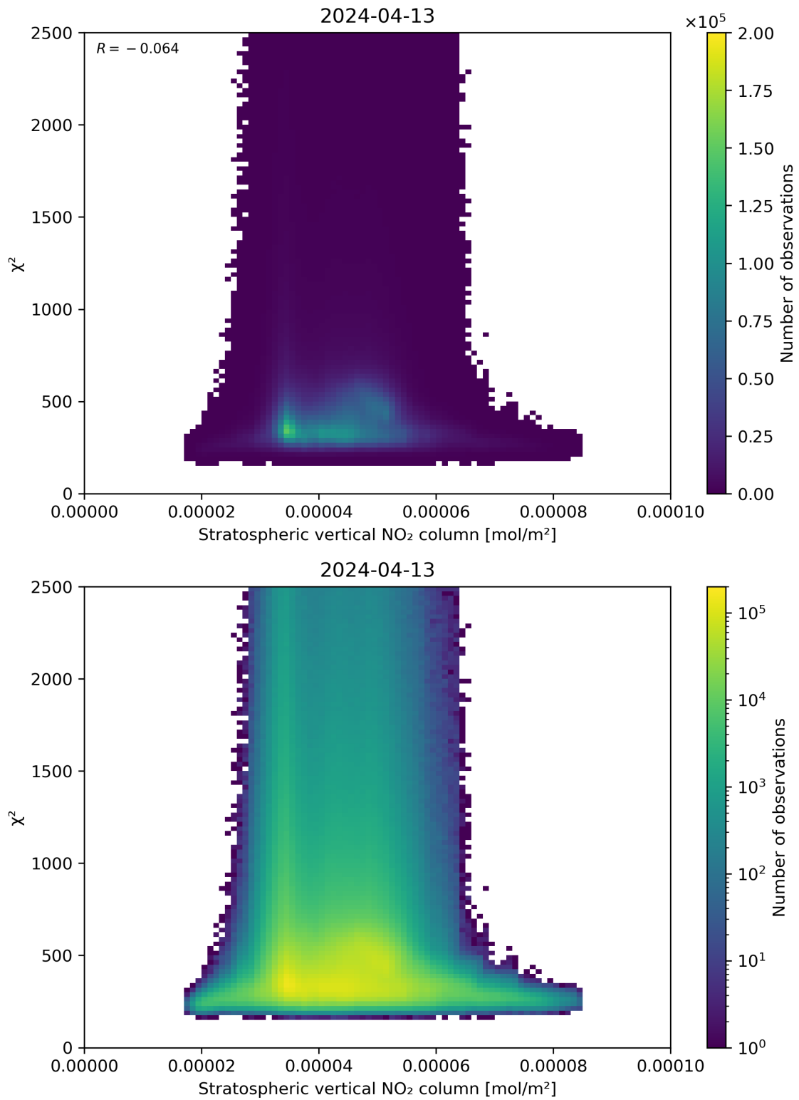
Figure 97: Scatter density plot of “Stratospheric vertical NO 2 column” against “ \chi^2 ” for 2024-04-12 to 2024-04-14.
