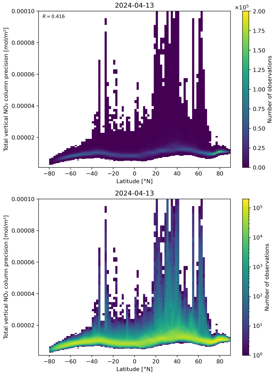
Figure 91: Scatter density plot of “Latitude” against “Total vertical NO 2 column precision” for 2024-04-12 to 2024-04-14.
