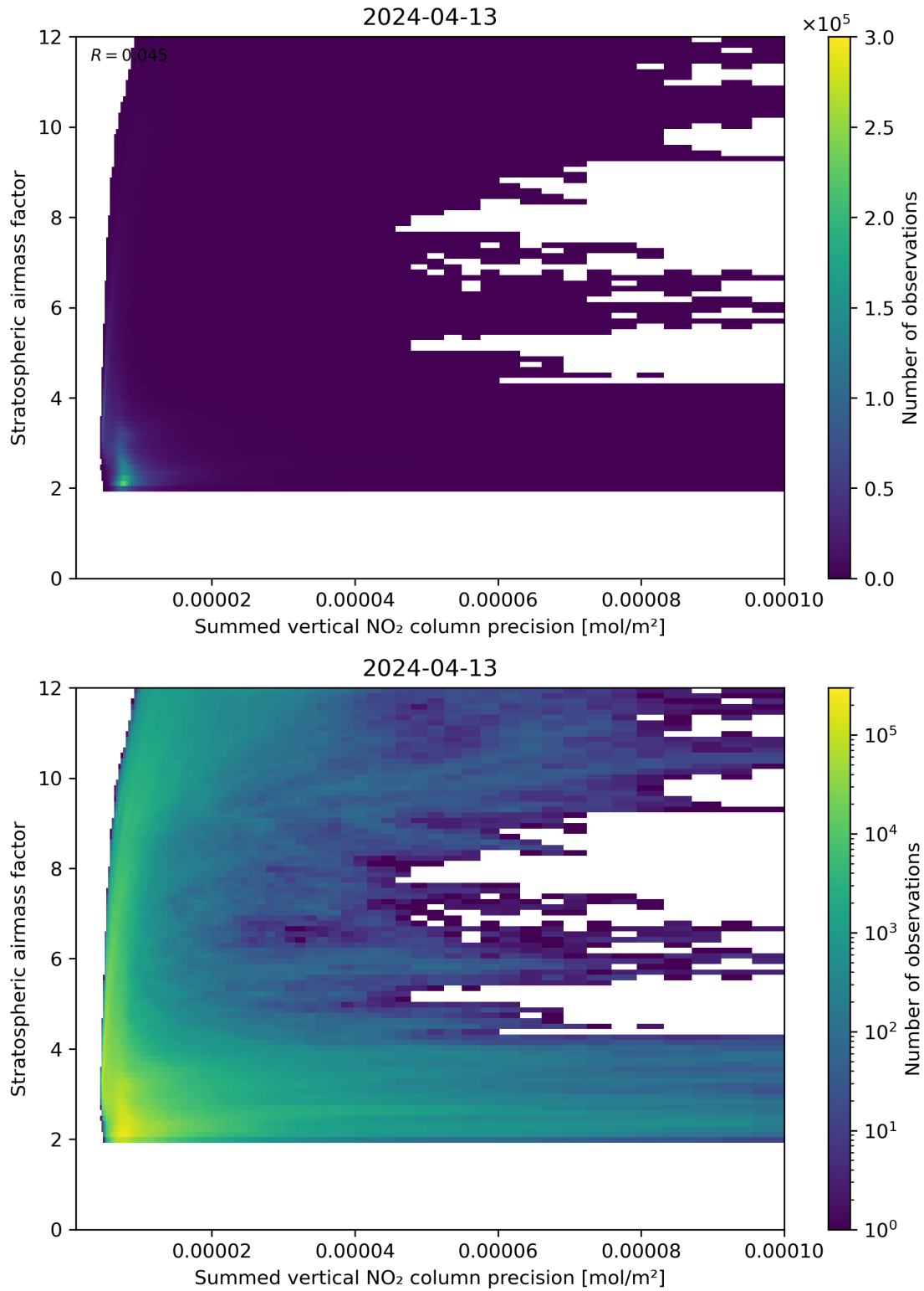
Figure 106: Scatter density plot of “Summed vertical NO 2 column precision” against “Stratospheric airmass factor” for 2024-04-12 to 2024-04-14.
