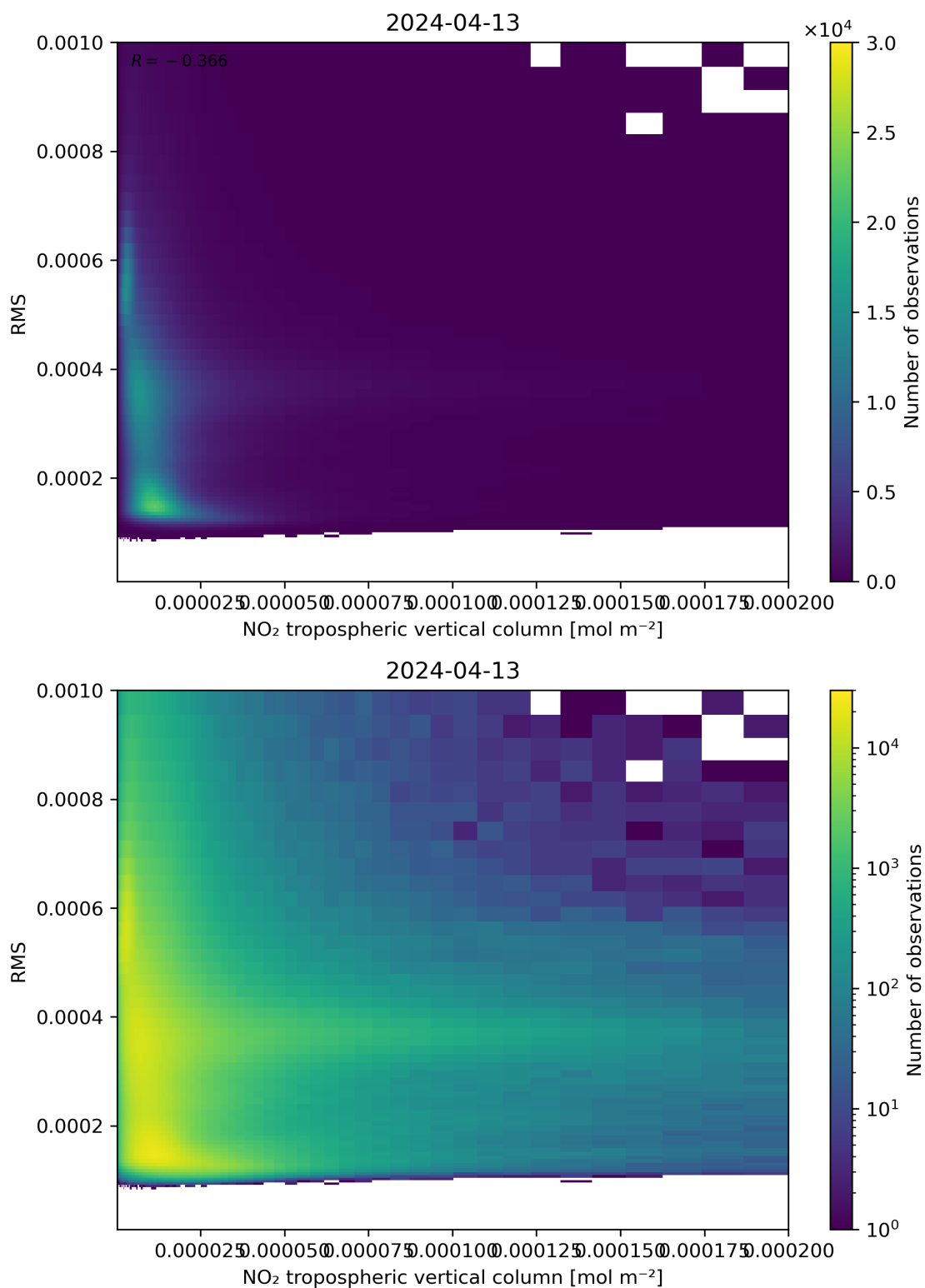
Figure 142: Scatter density plot of “NO 2 tropospheric vertical column” against “RMS” for 2024-04-12 to 2024-04-14.
