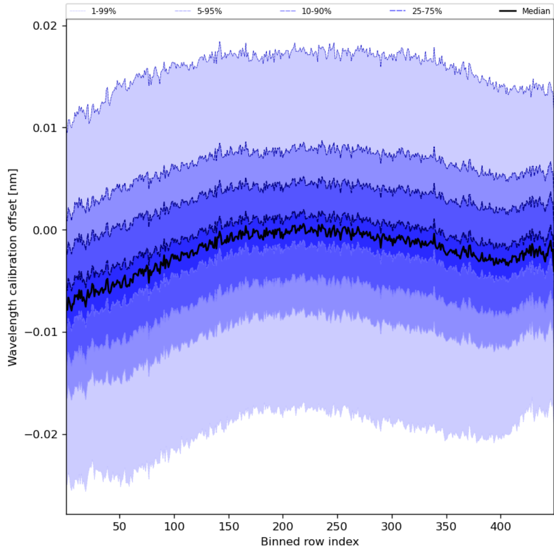
Figure 52: Along track statistics of “Wavelength calibration offset” for 2024-04-12 to 2024-04-14
