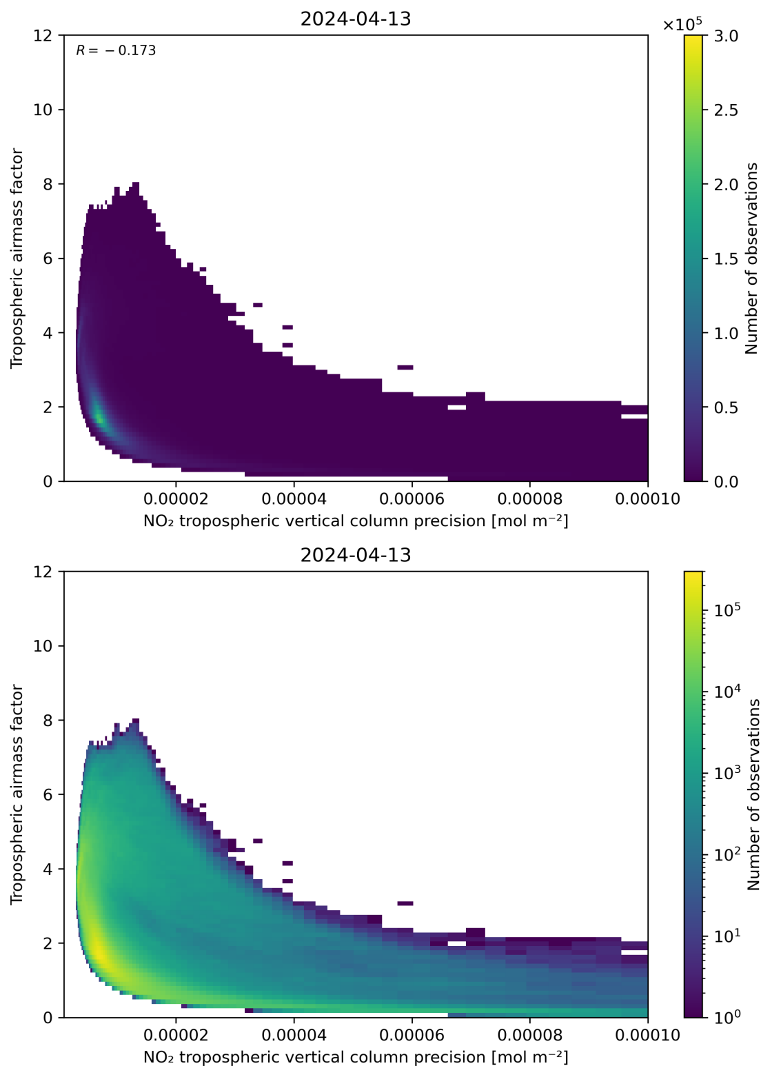
Figure 133: Scatter density plot of “NO 2 tropospheric vertical column precision” against “Tropospheric airmass factor” for 2024-04-12 to 2024-04-14.
