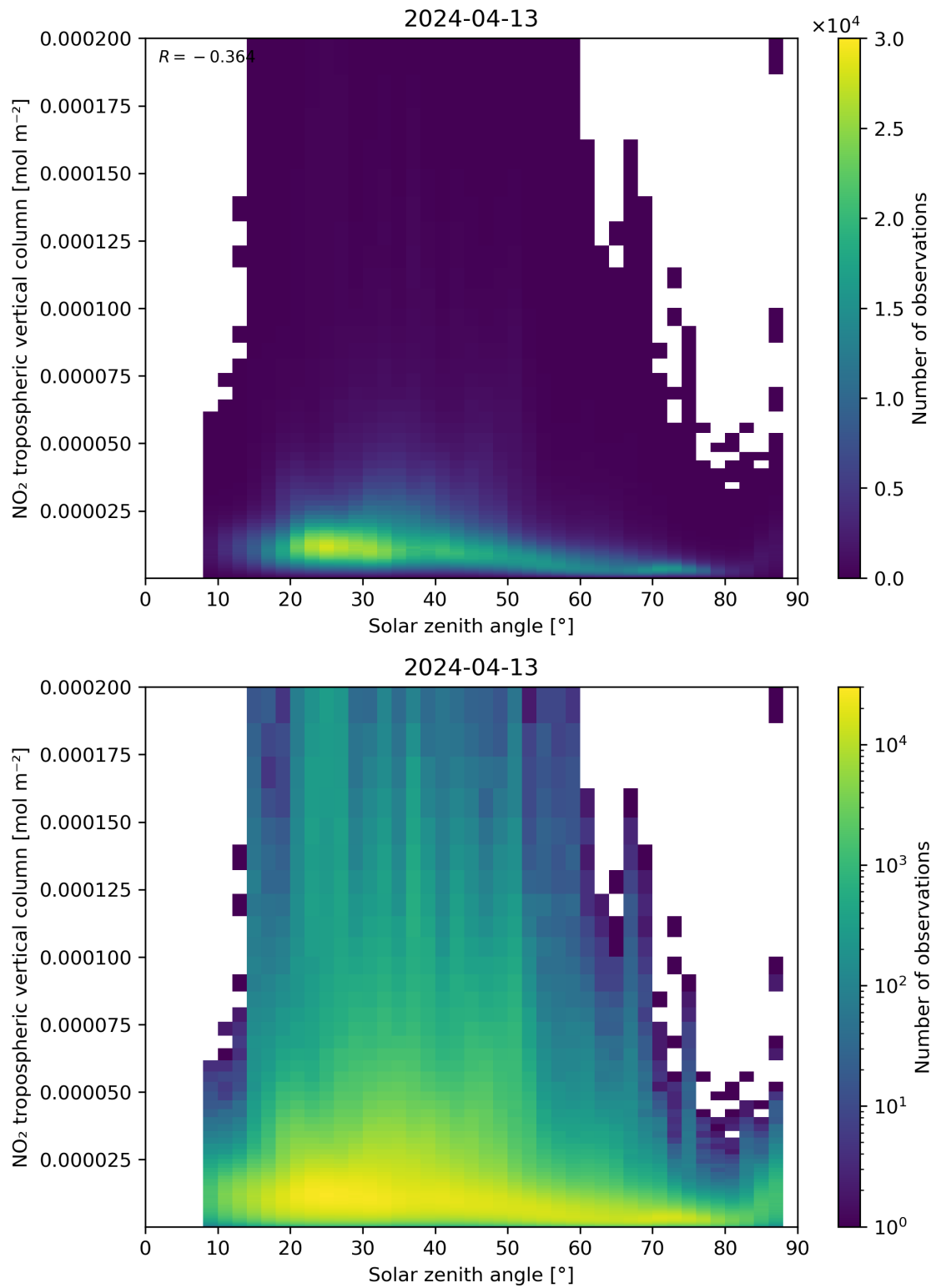
Figure 155: Scatter density plot of “Solar zenith angle” against “NO 2 tropospheric vertical column” for 2024-04-12 to 2024-04-14.
