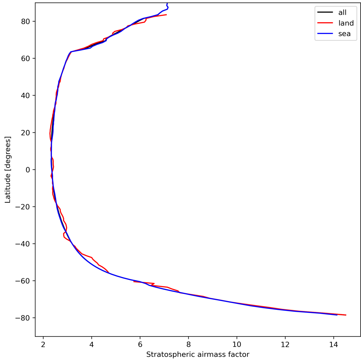
Figure 27: Zonal average of “Stratospheric airmass factor” for 2024-04-12 to 2024-04-14.
