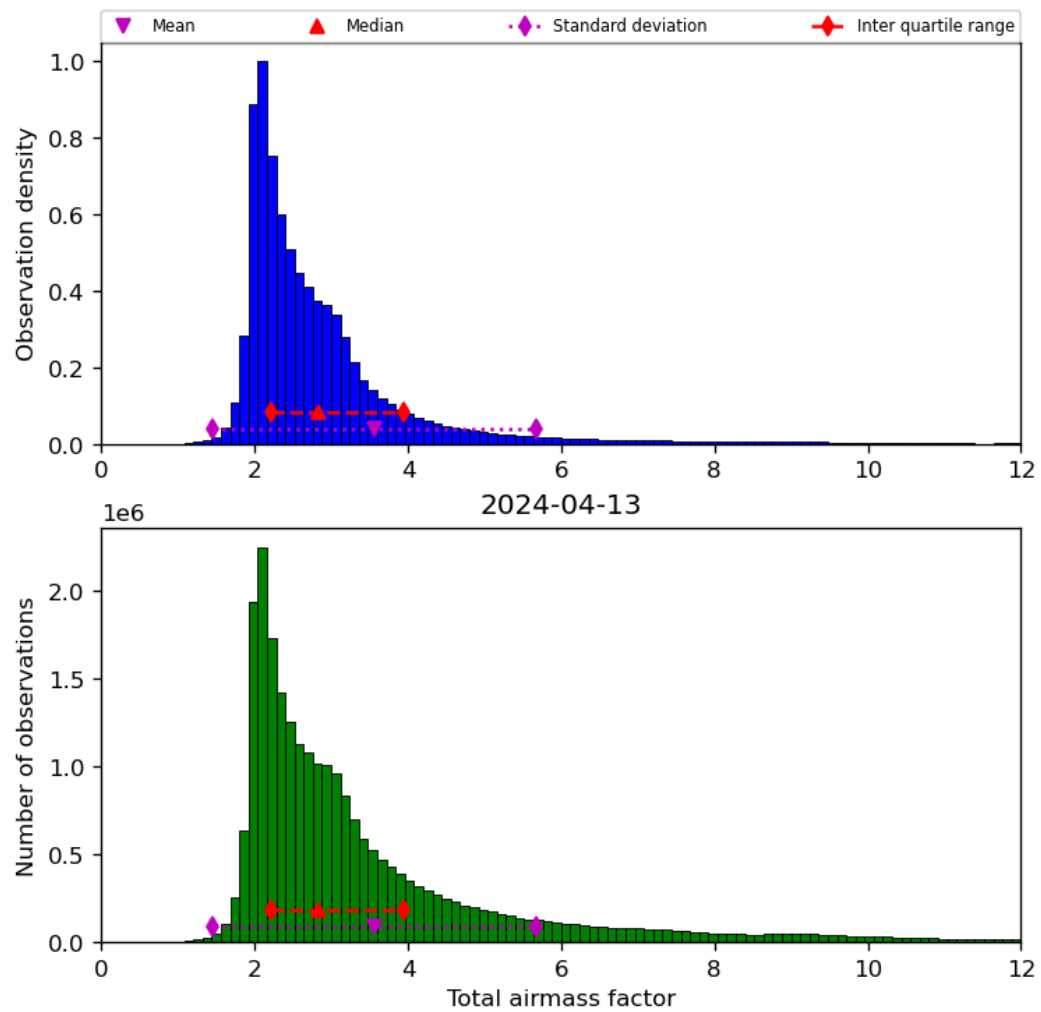
Figure 32: Histogram of “Total airmass factor” for 2024-04-12 to 2024-04-14
