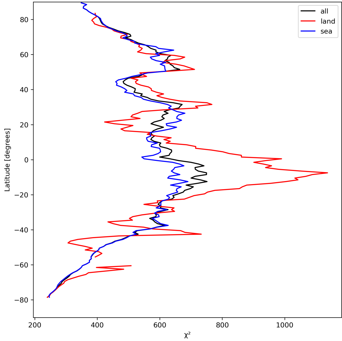
Figure 25: Zonal average of “ \chi^2 ” for 2024-04-12 to 2024-04-14.
