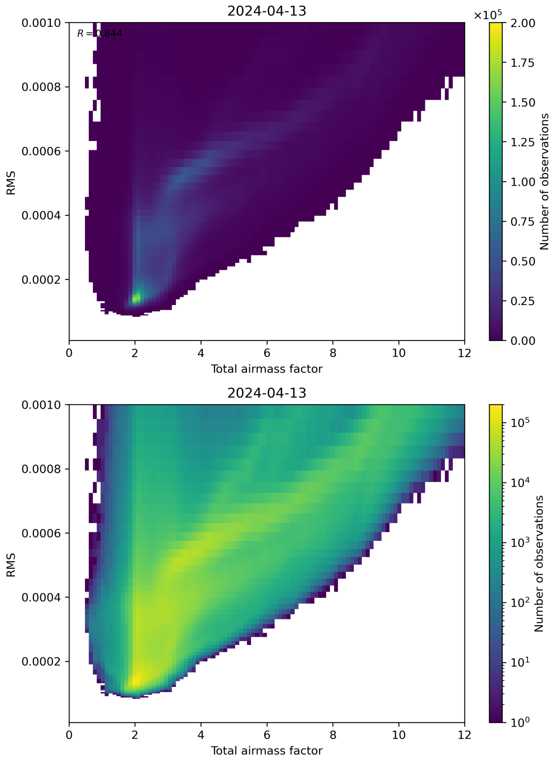
Figure 69: Scatter density plot of “Total airmass factor” against “RMS” for 2024-04-12 to 2024-04-14.
