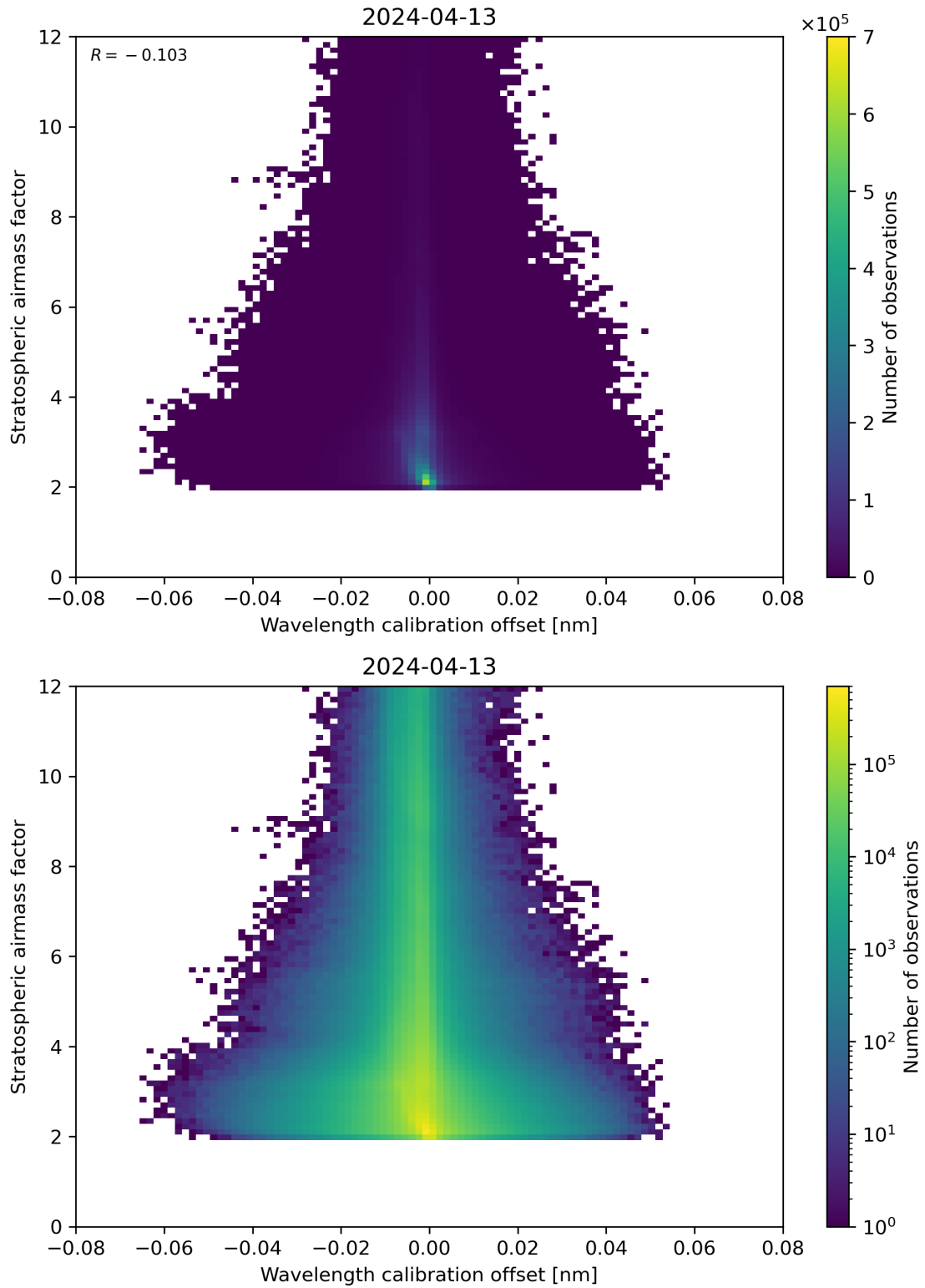
Figure 174: Scatter density plot of “Wavelength calibration offset” against “Stratospheric air mass factor” for 2024-04-12 to 2024-04-14.
