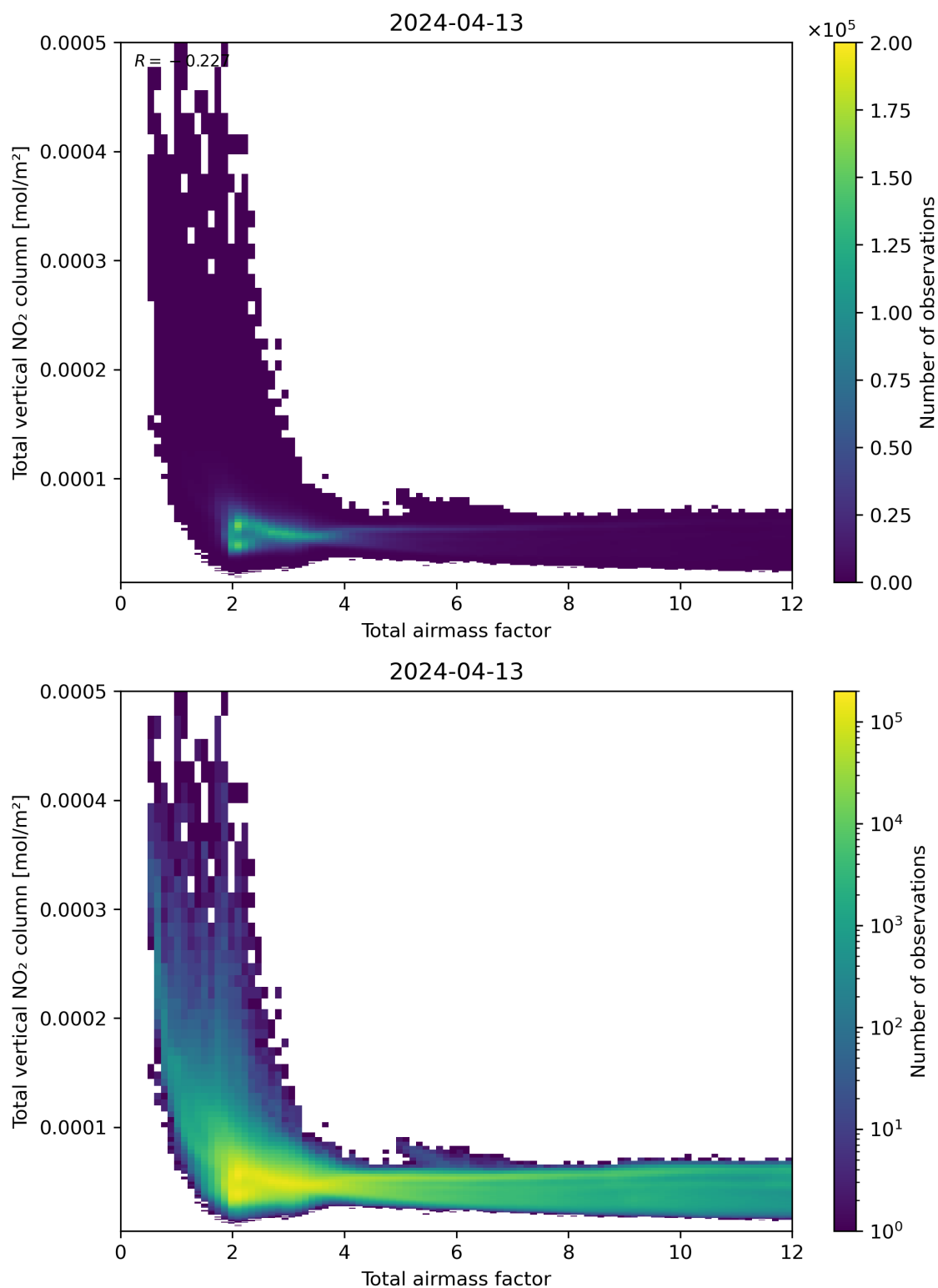
Figure 67: Scatter density plot of “Total airmass factor” against “Total vertical NO 2 column” for 2024-04-12 to 2024-04-14.
