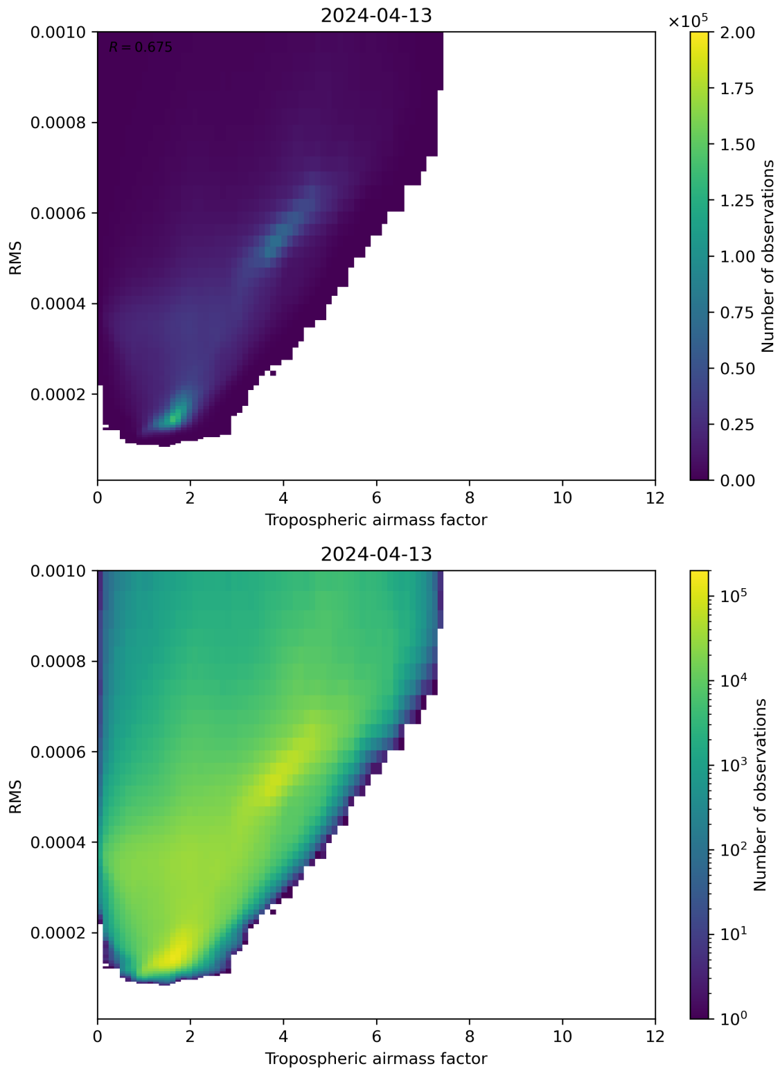
Figure 79: Scatter density plot of “Tropospheric airmass factor” against “RMS” for 2024-04-12 to 2024-04-14.
