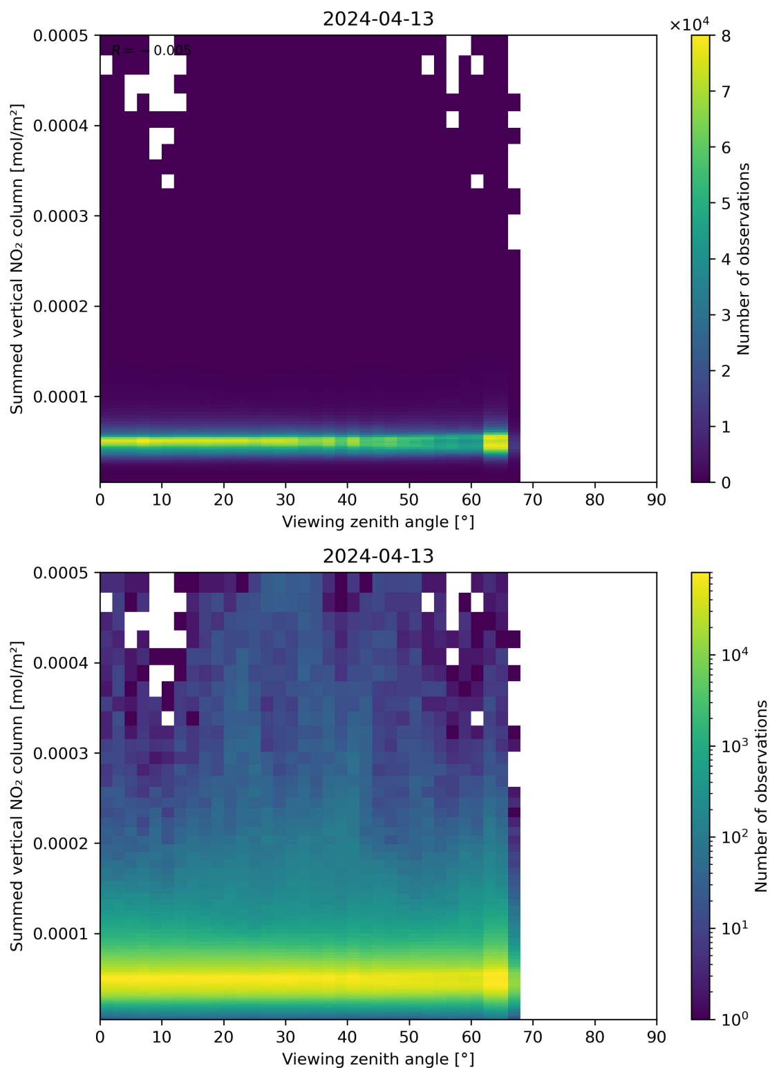
Figure 165: Scatter density plot of “Viewing zenith angle” against “Summed vertical NO 2 column” for 2024-04-12 to 2024-04-14.
