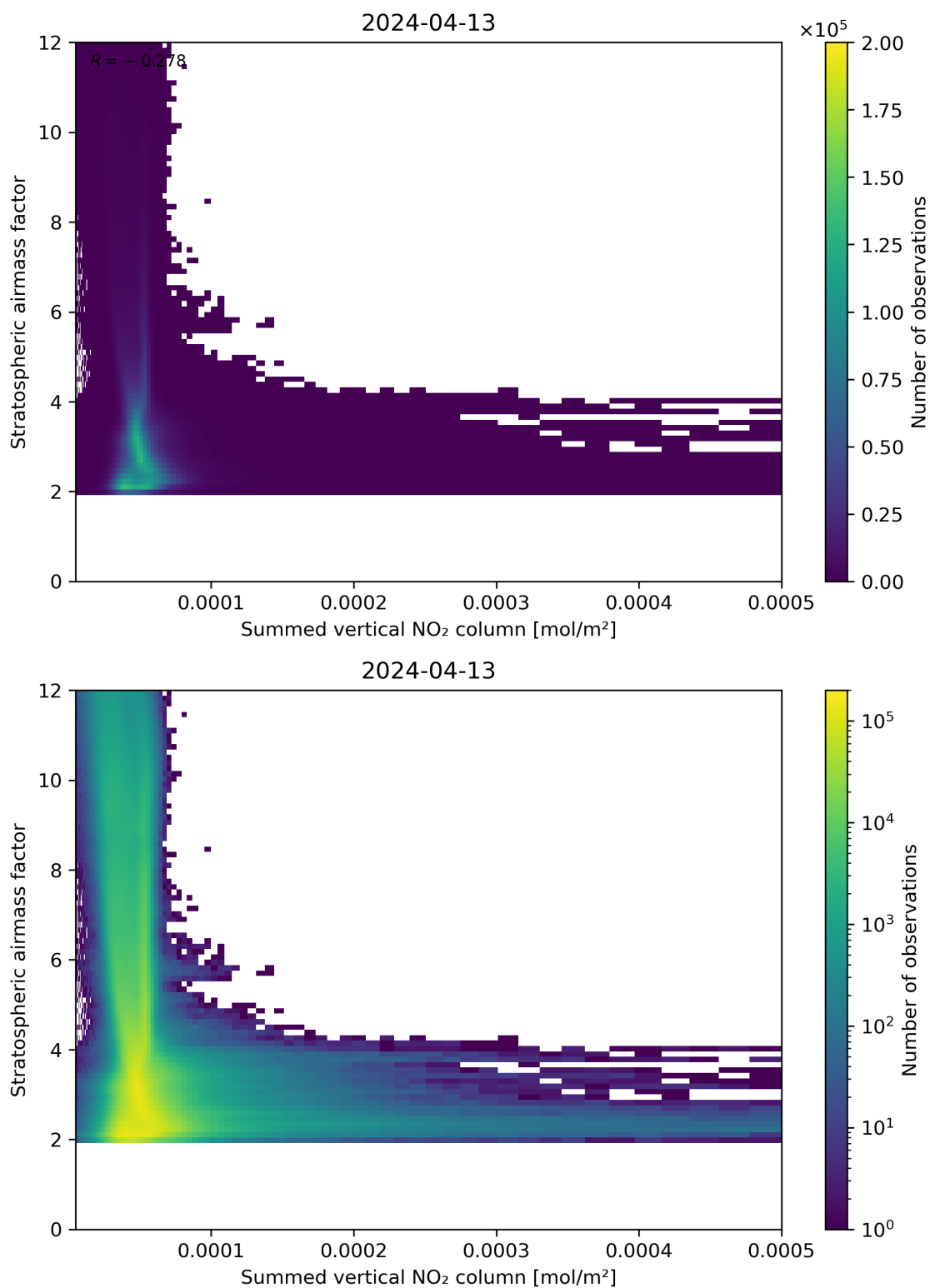
Figure 103: Scatter density plot of “Summed vertical NO 2 column” against “Stratospheric airmass factor” for 2024-04-12 to 2024-04-14.
