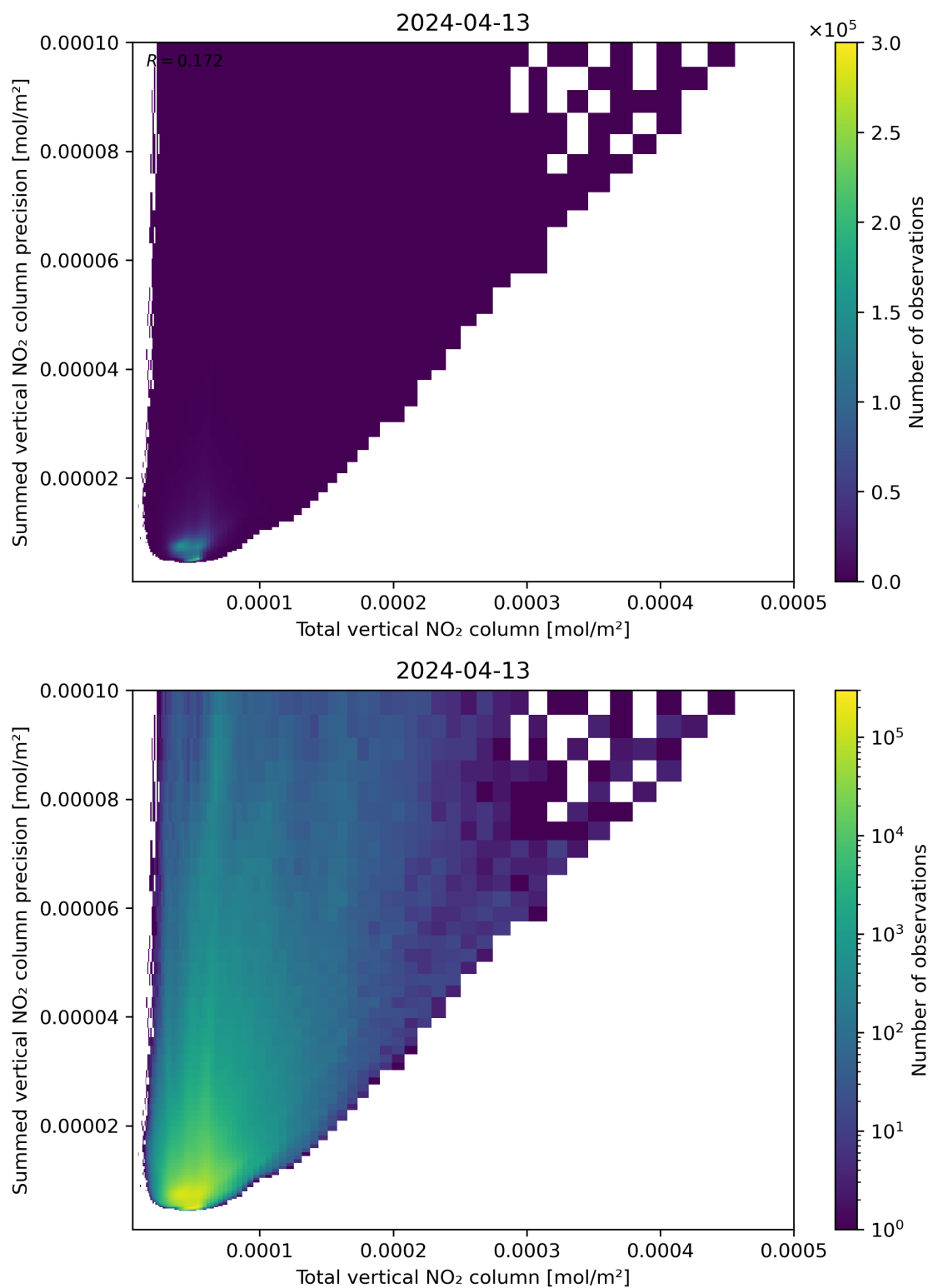
Figure 113: Scatter density plot of “Total vertical NO 2 column” against “Summed vertical NO 2 column precision” for 2024-04-12 to 2024-04-14.
