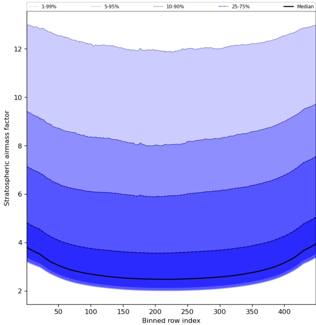
Figure 61: Along track statistics of “Stratospheric airmass factor” for 2024-04-12 to 2024-04-14
