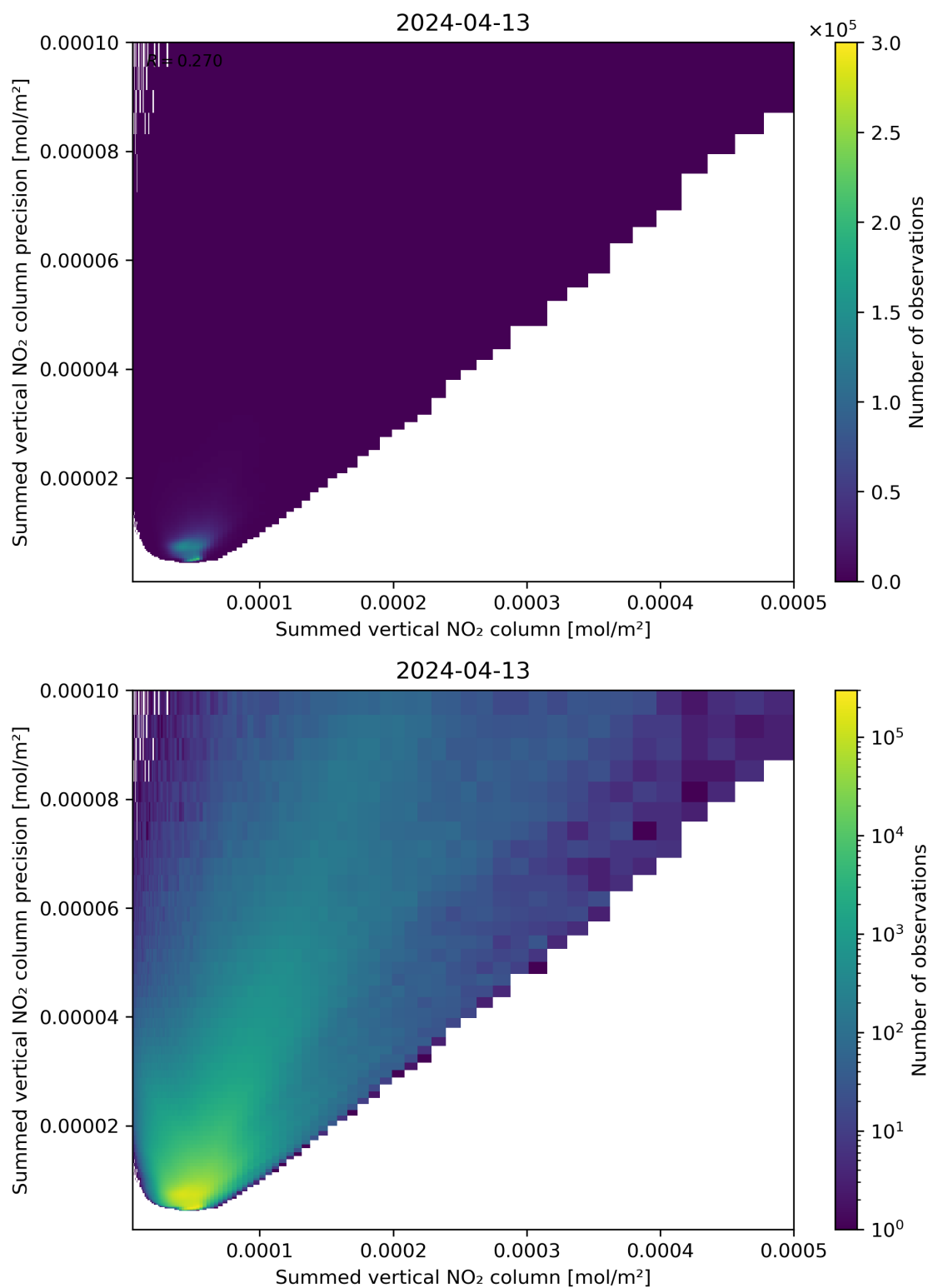
Figure 105: Scatter density plot of “Summed vertical NO 2 column” against “Summed vertical NO 2 column precision” for 2024-04-12 to 2024-04-14.
