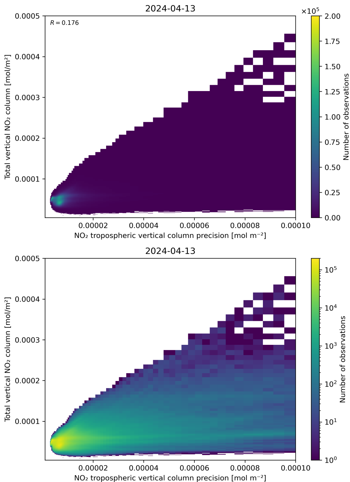
Figure 138: Scatter density plot of “NO 2 tropospheric vertical column precision” against “Total vertical NO 2 column” for 2024-04-12 to 2024-04-14.
