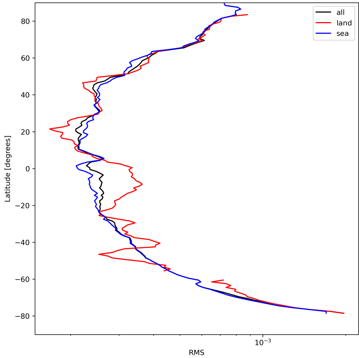
Figure 26: Zonal average of “RMS” for 2024-04-12 to 2024-04-14.
