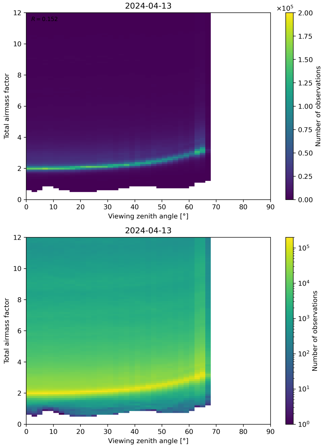
Figure 160: Scatter density plot of “Viewing zenith angle” against “Total airmass factor” for 2024-04-12 to 2024-04-14.
