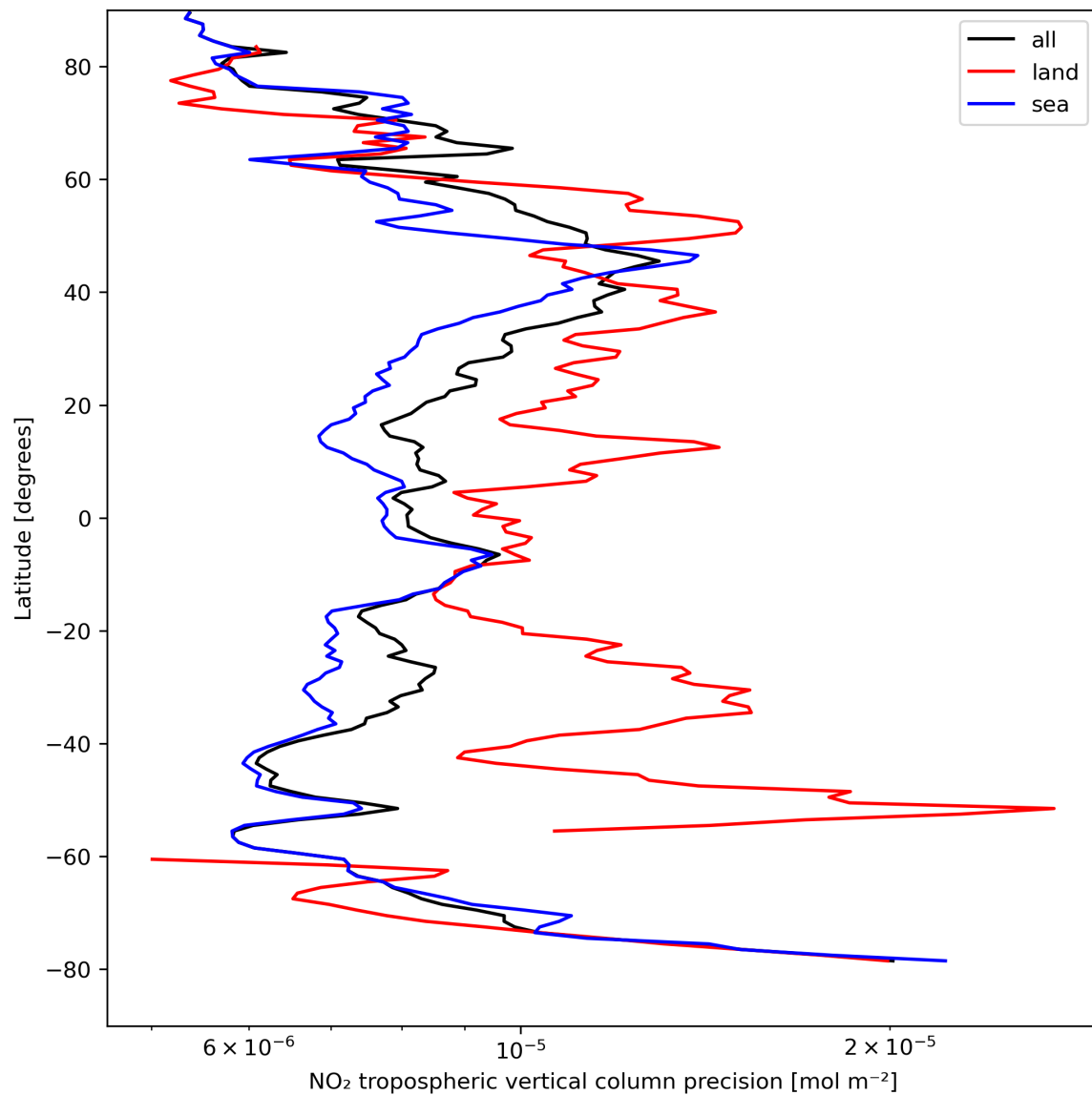
Figure 13: Zonal average of “NO 2 tropospheric vertical column precision” for 2024-04-13 to 2024-04-15.
