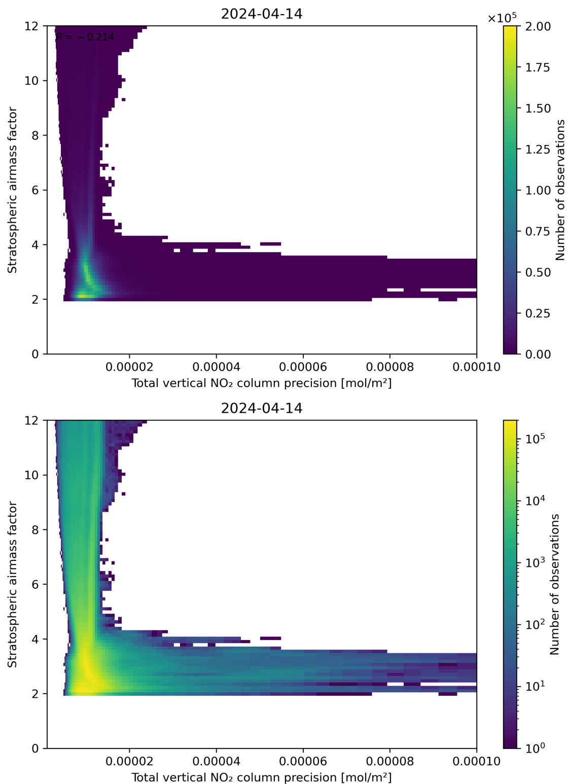
Figure 115: Scatter density plot of “Total vertical NO 2 column precision” against “Stratospheric airmass factor” for 2024-04-13 to 2024-04-15.
