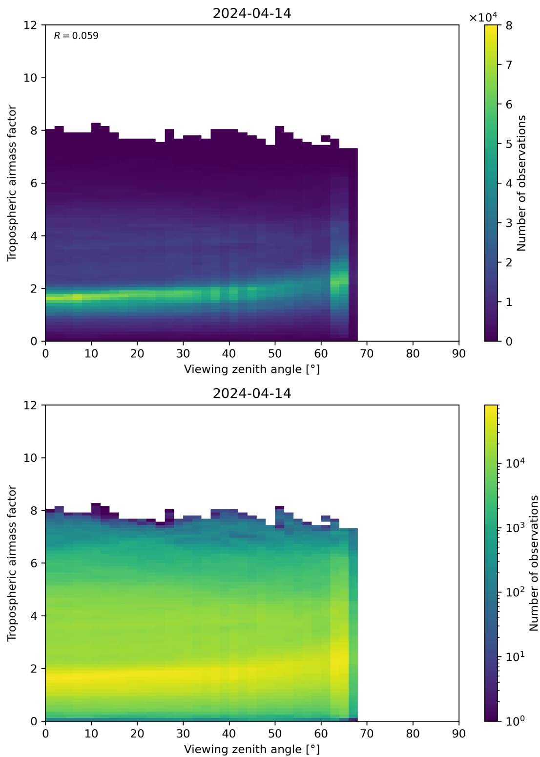
Figure 161: Scatter density plot of “Viewing zenith angle” against “Tropospheric airmass factor” for 2024-04-13 to 2024-04-15.
