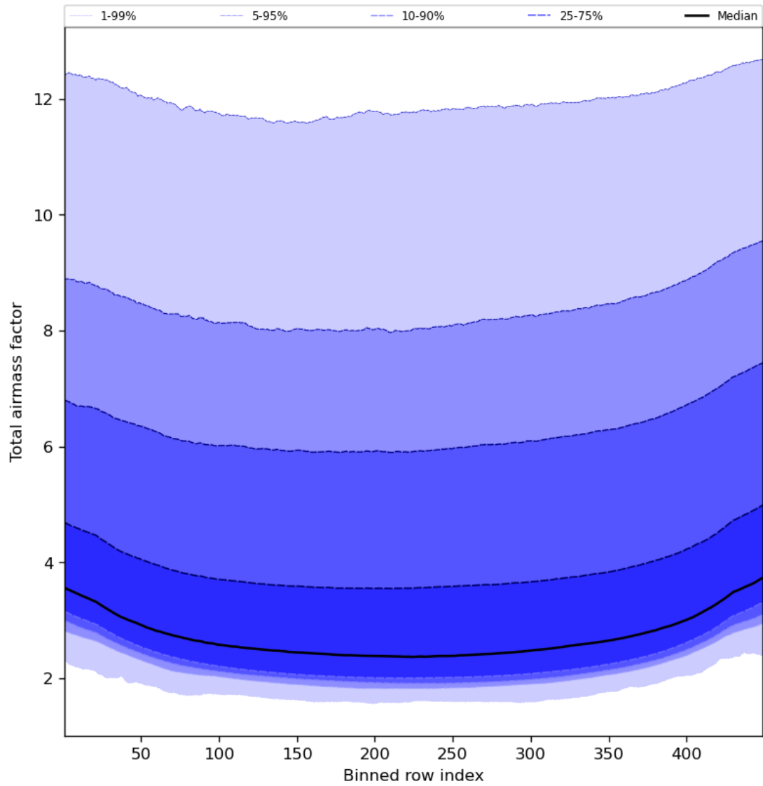
Figure 49: Along track statistics of “Total airmass factor” for 2024-04-13 to 2024-04-15
