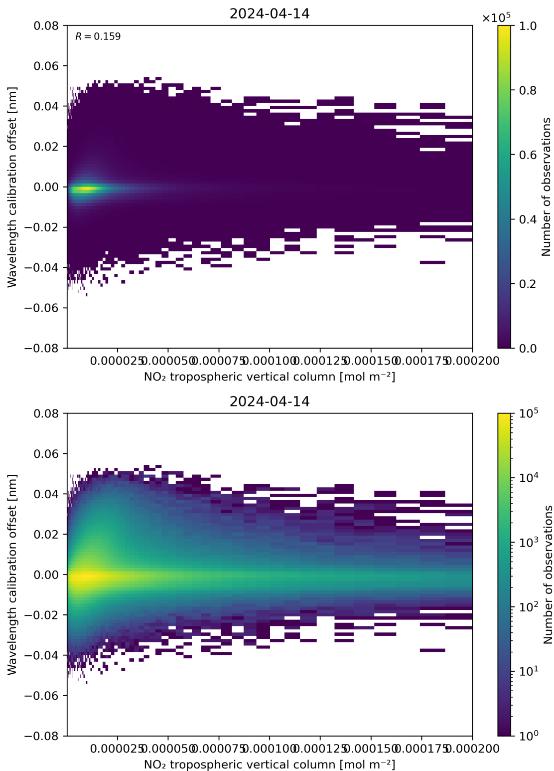
Figure 143: Scatter density plot of “NO 2 tropospheric vertical column” against “Wavelength calibration offset” for 2024-04-13 to 2024-04-15.
