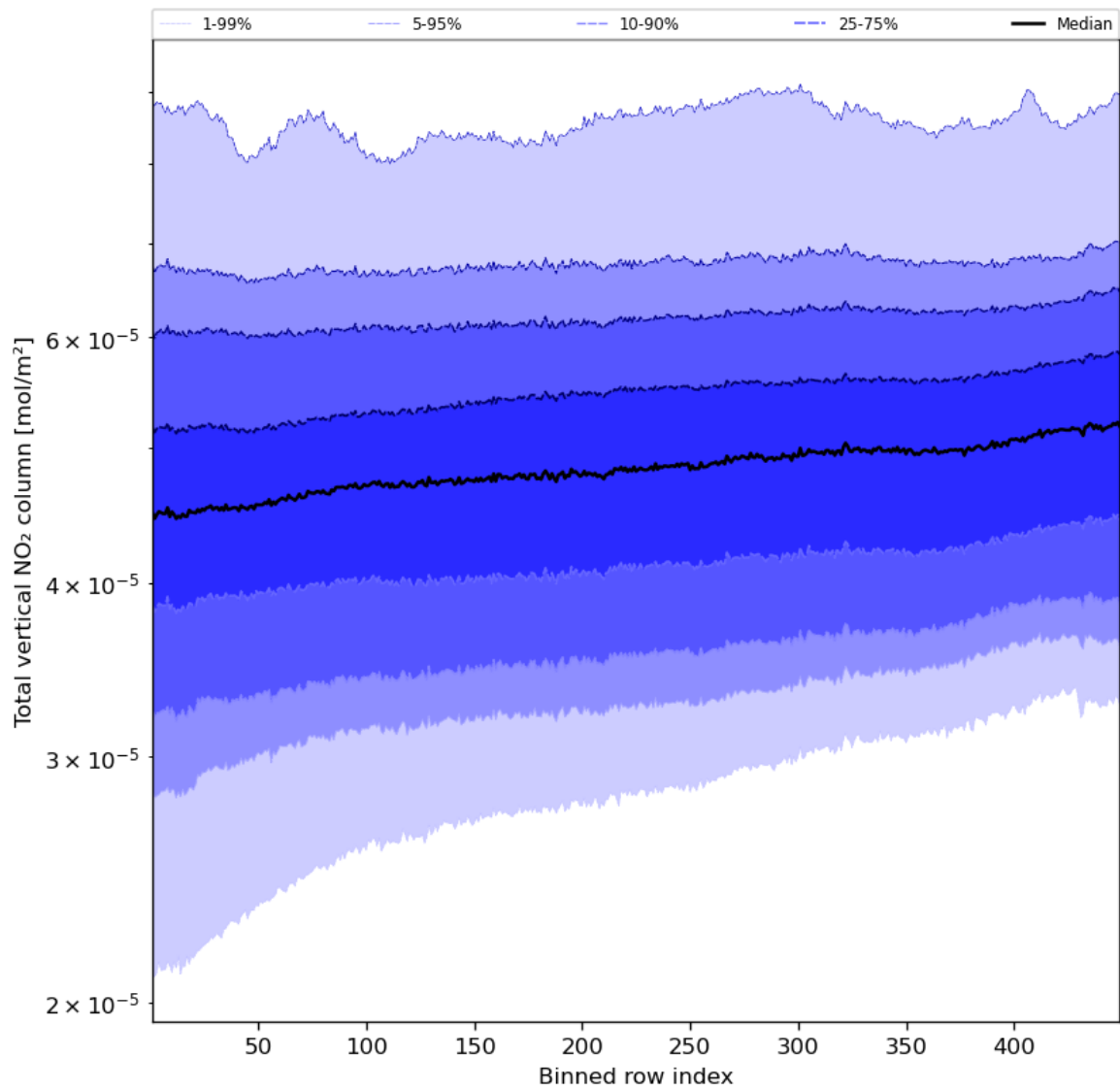
Figure 55: Along track statistics of “Total vertical NO 2 column” for 2024-04-13 to 2024-04-15
