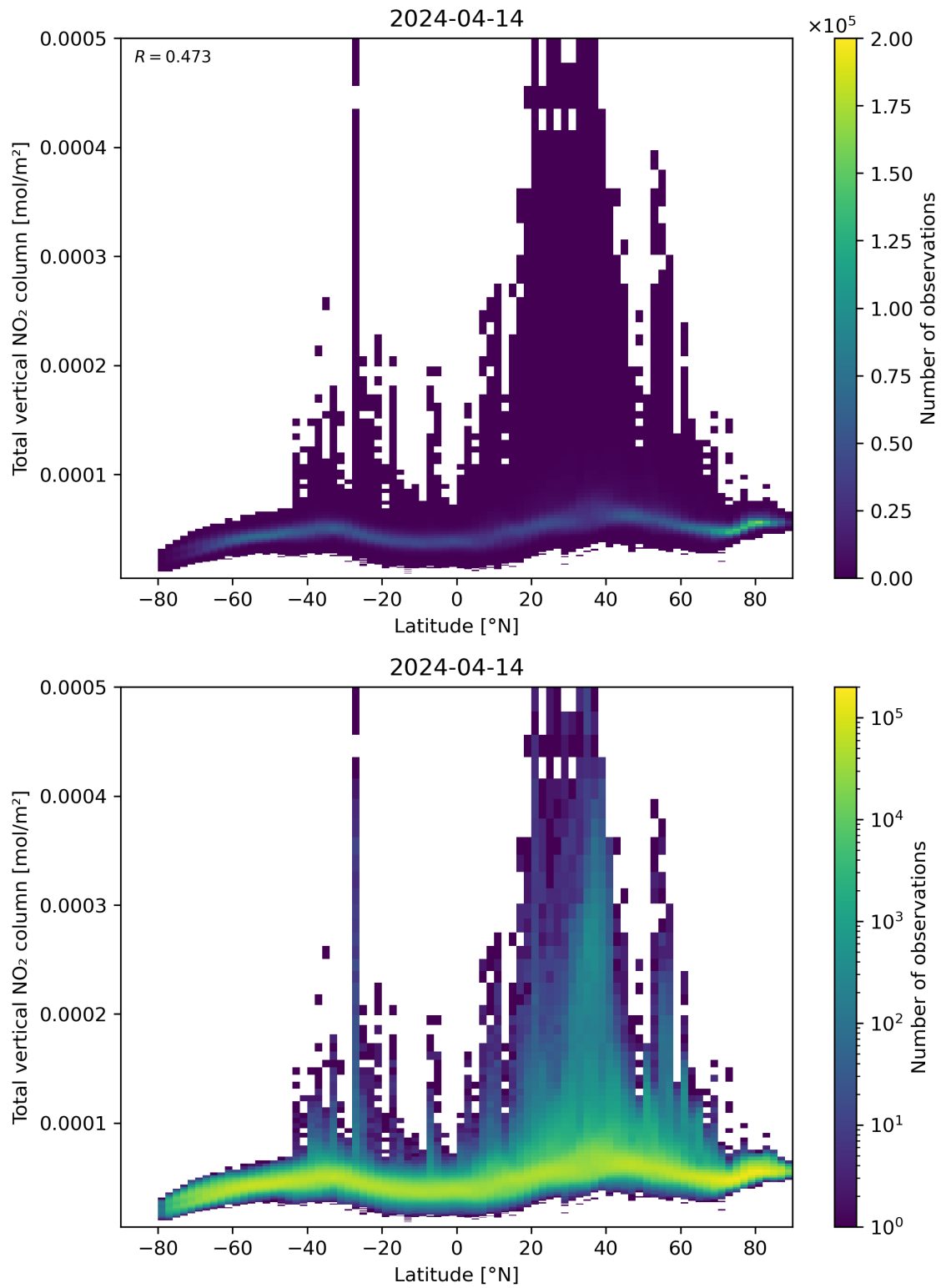
Figure 90: Scatter density plot of “Latitude” against “Total vertical NO 2 column” for 2024-04-13 to 2024-04-15.
