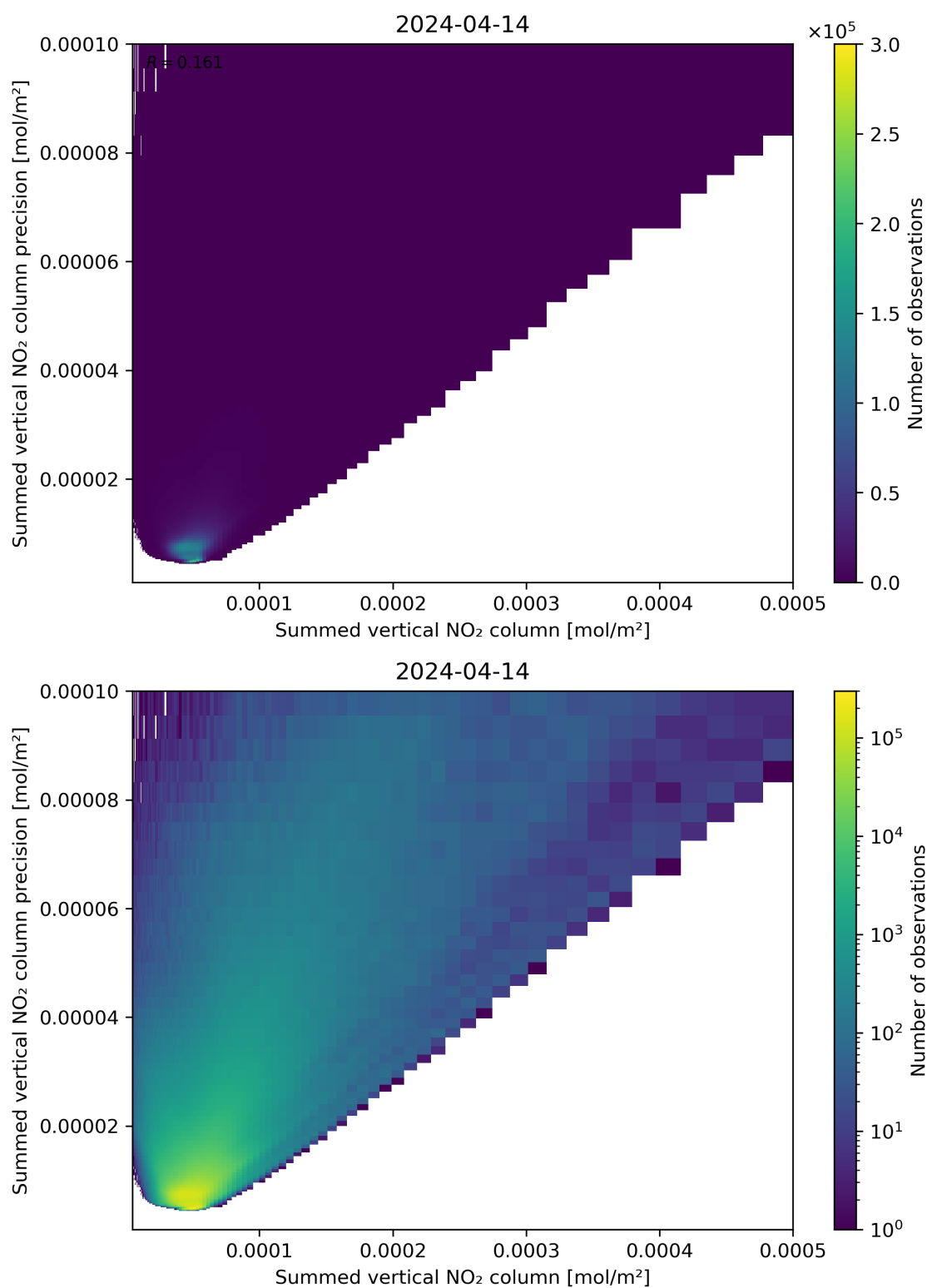
Figure 105: Scatter density plot of “Summed vertical NO 2 column” against “Summed vertical NO 2 column precision” for 2024-04-13 to 2024-04-15.
