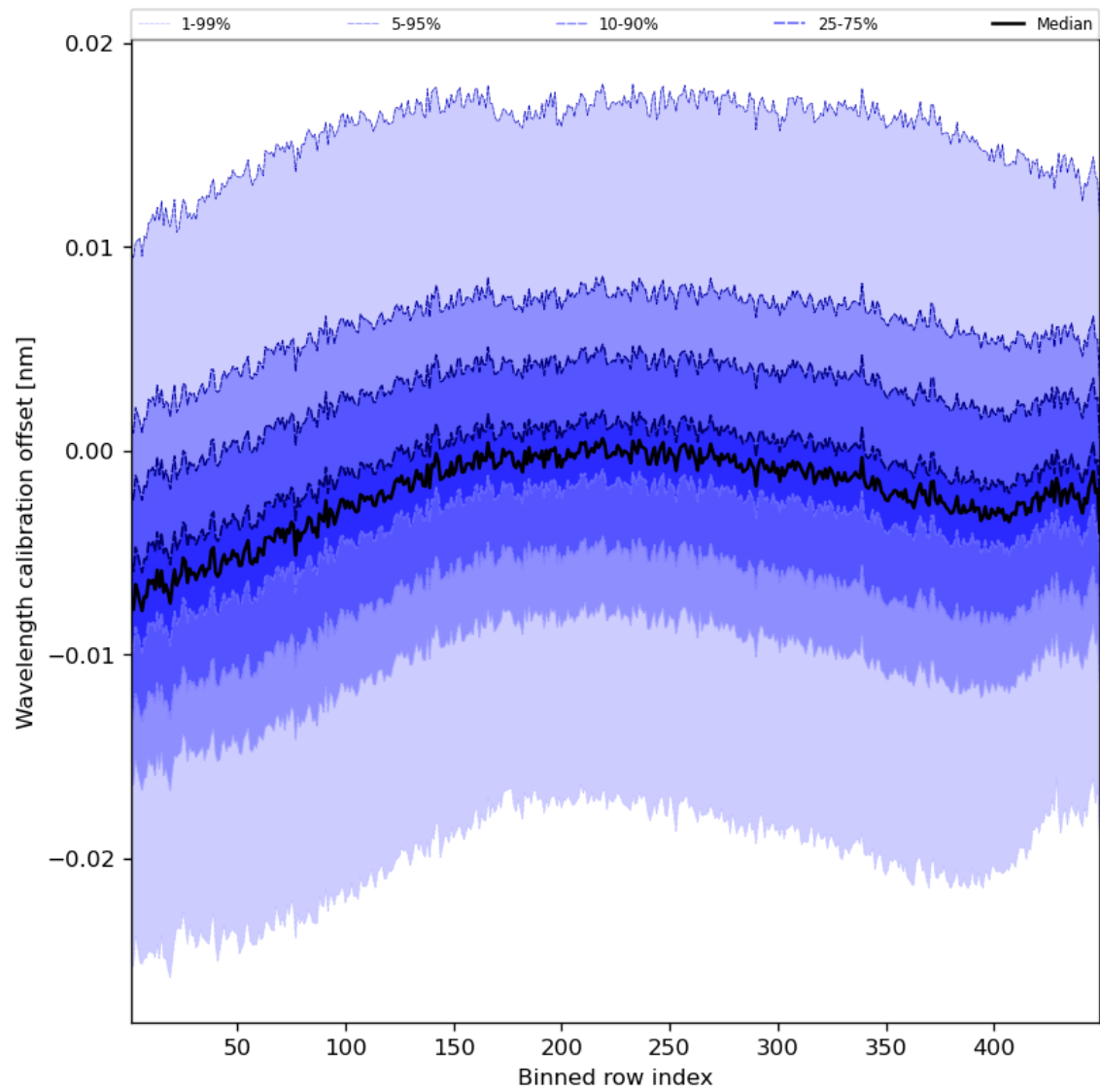
Figure 52: Along track statistics of “Wavelength calibration offset” for 2024-04-13 to 2024-04-15
