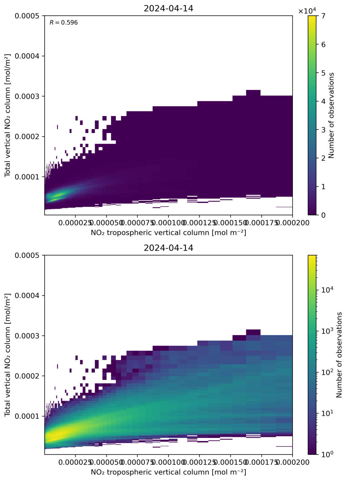
Figure 128: Scatter density plot of “NO 2 tropospheric vertical column” against “Total vertical NO 2 column” for 2024-04-13 to 2024-04-15.
