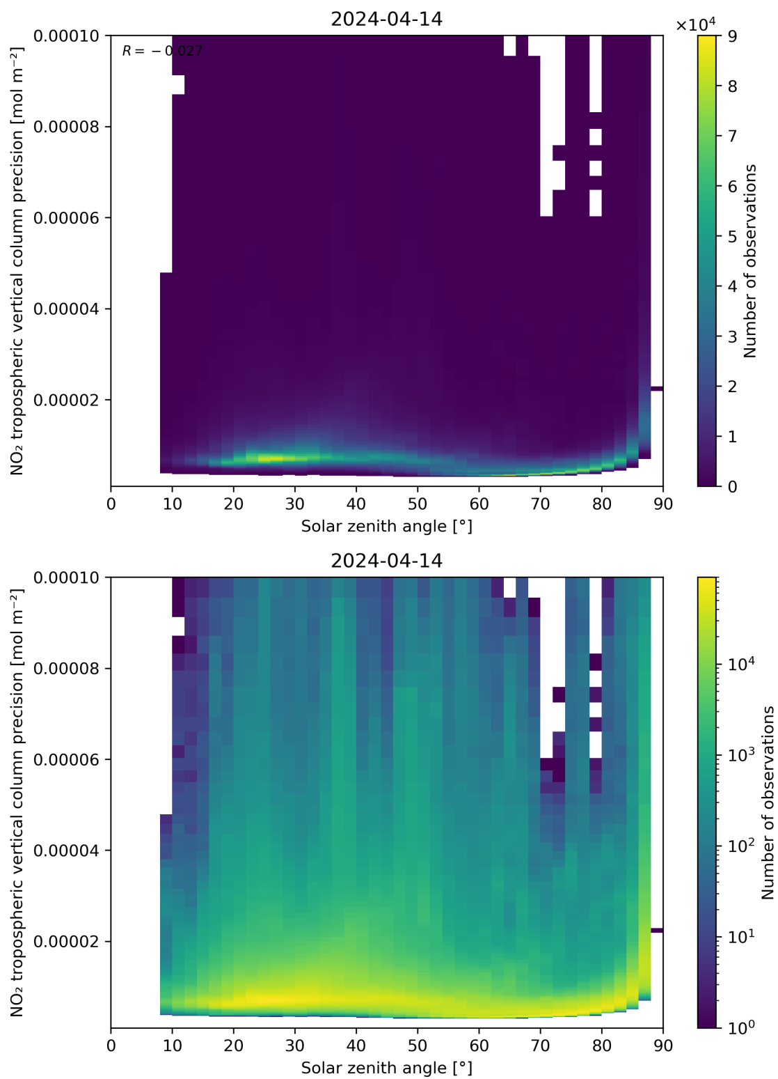
Figure 156: Scatter density plot of “Solar zenith angle” against “NO 2 tropospheric vertical column precision” for 2024-04-13 to 2024-04-15.
