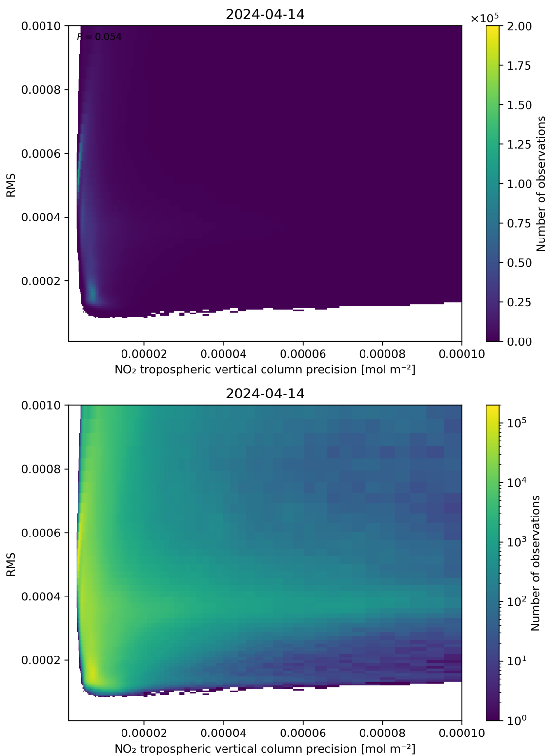
Figure 140: Scatter density plot of “NO 2 tropospheric vertical column precision” against “RMS” for 2024-04-13 to 2024-04-15.
