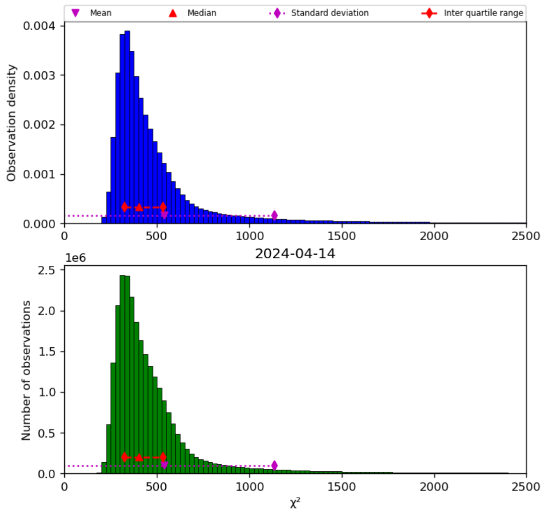
Figure 42: Histogram of “ \chi^2 ” for 2024-04-13 to 2024-04-15
