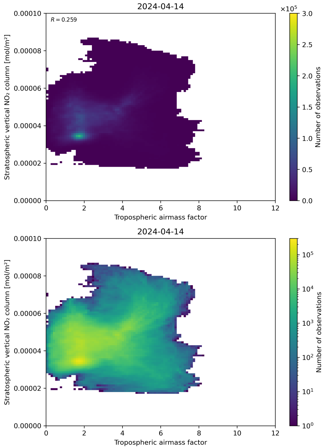
Figure 74: Scatter density plot of “Tropospheric air mass factor” against “Stratospheric vertical \text{NO}_2 column” for 2024-04-13 to 2024-04-15.
