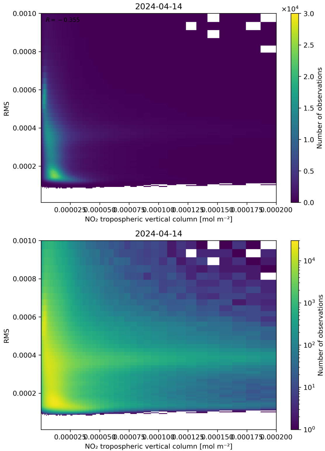
Figure 142: Scatter density plot of “NO 2 tropospheric vertical column” against “RMS” for 2024-04-13 to 2024-04-15.
