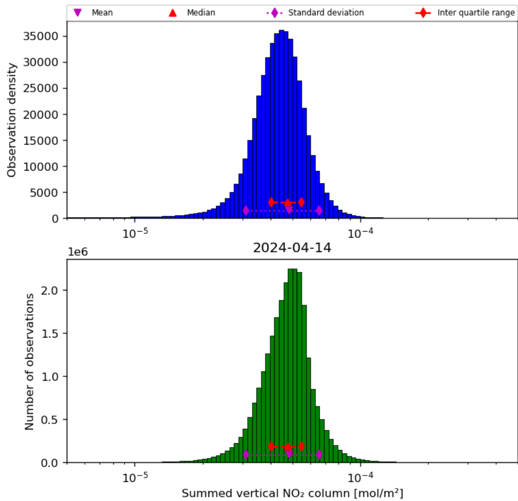
Figure 40: Histogram of “Summed vertical NO 2 column” for 2024-04-13 to 2024-04-15
