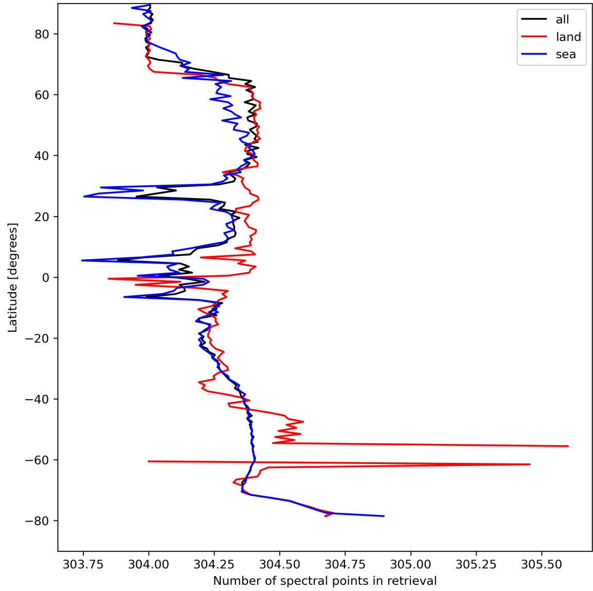
Figure 16: Zonal average of “Number of spectral points in retrieval” for 2024-04-13 to 2024-04-15.
