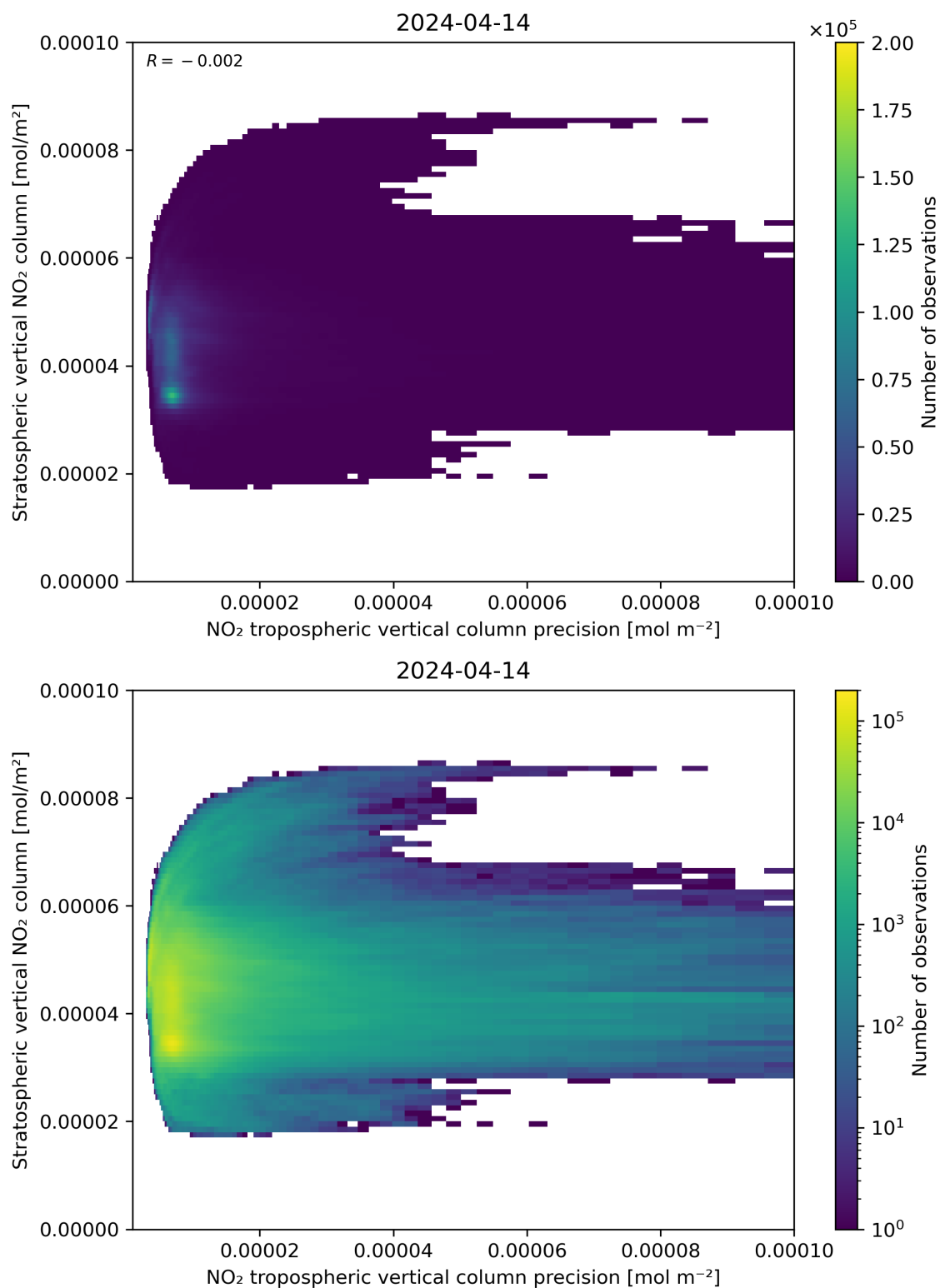
Figure 135: Scatter density plot of “NO 2 tropospheric vertical column precision” against “Stratospheric vertical NO 2 column” for 2024-04-13 to 2024-04-15.
