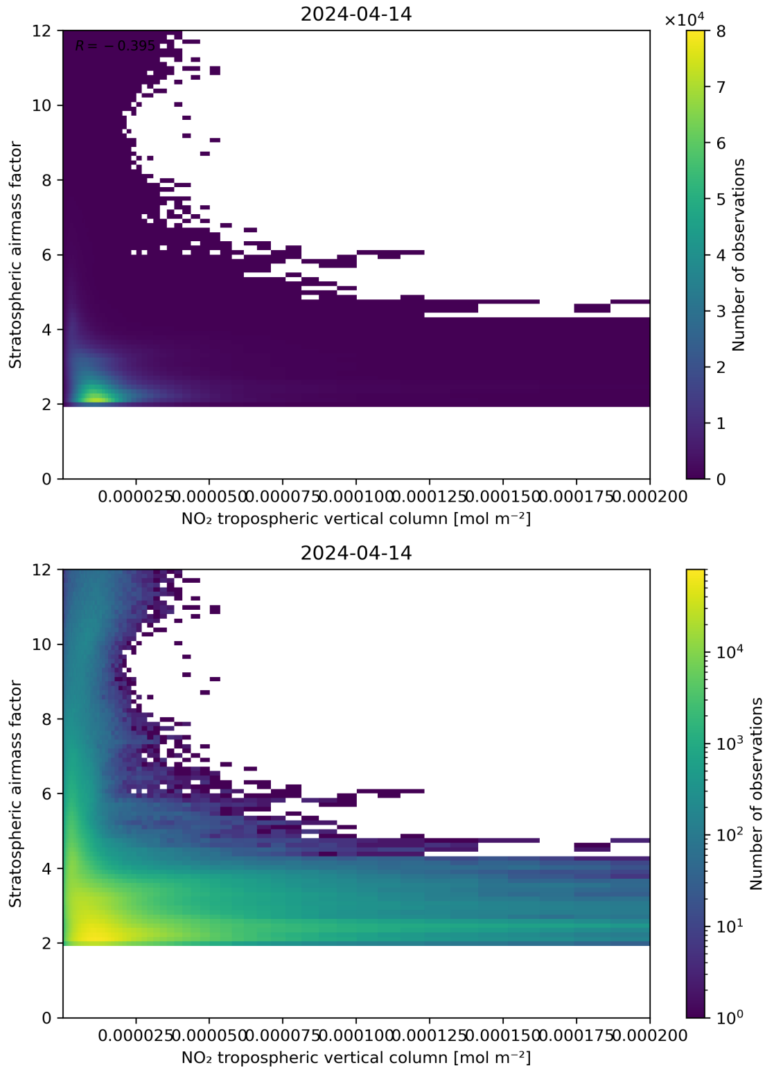
Figure 121: Scatter density plot of “NO 2 tropospheric vertical column” against “Stratospheric air mass factor” for 2024-04-13 to 2024-04-15.
