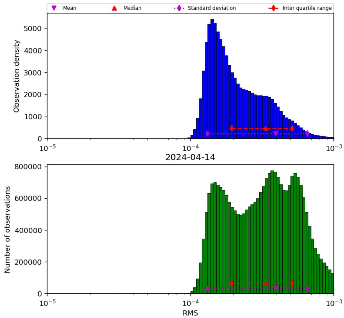
Figure 43: Histogram of “RMS” for 2024-04-13 to 2024-04-15
