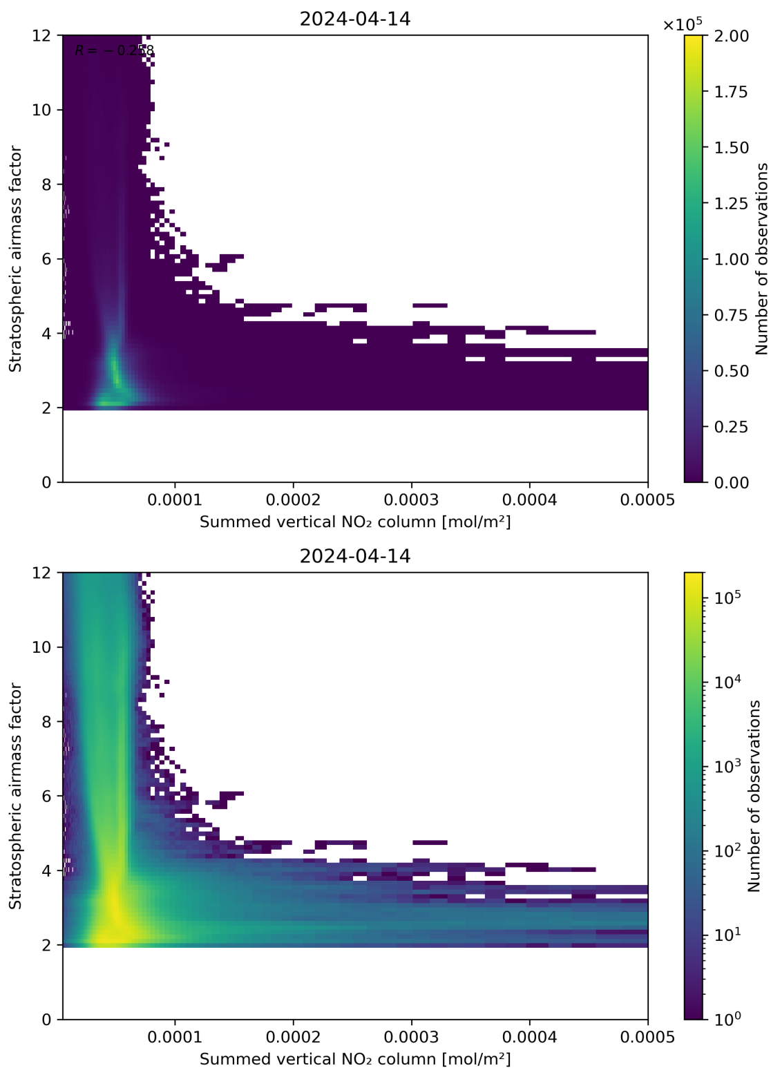
Figure 103: Scatter density plot of “Summed vertical NO 2 column” against “Stratospheric air mass factor” for 2024-04-13 to 2024-04-15.
