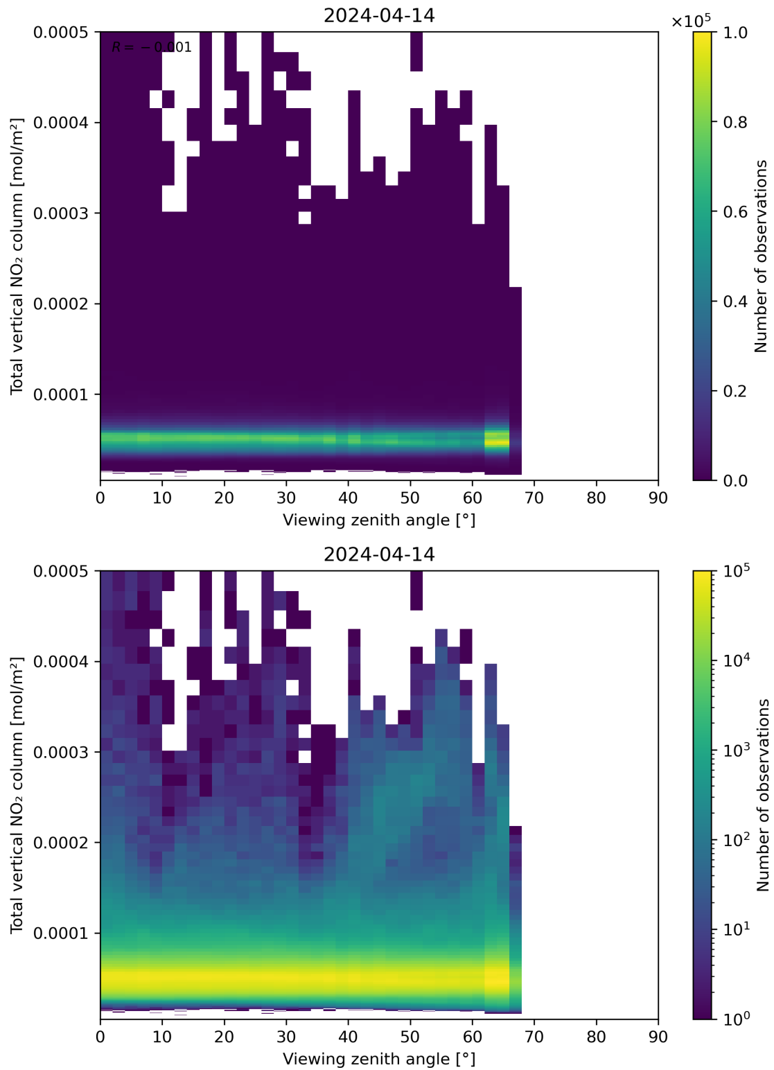
Figure 167: Scatter density plot of “Viewing zenith angle” against “Total vertical NO 2 column” for 2024-04-13 to 2024-04-15.
