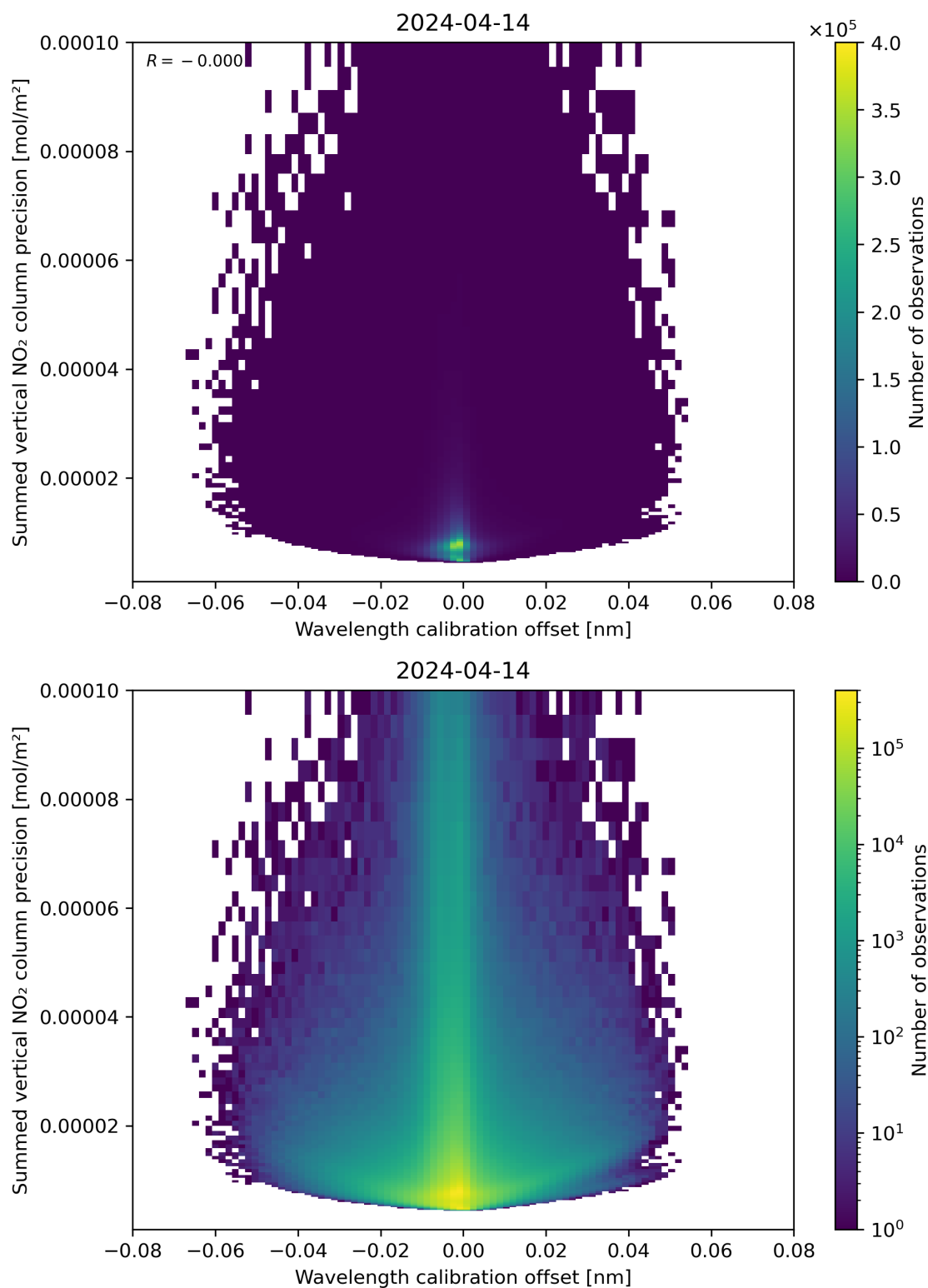
Figure 178: Scatter density plot of “Wavelength calibration offset” against “Summed vertical NO 2 column precision” for 2024-04-13 to 2024-04-15.
