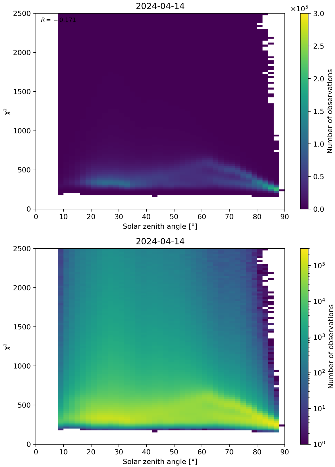
Figure 148: Scatter density plot of “Solar zenith angle” against “ \chi^2 ” for 2024-04-13 to 2024-04-15.
