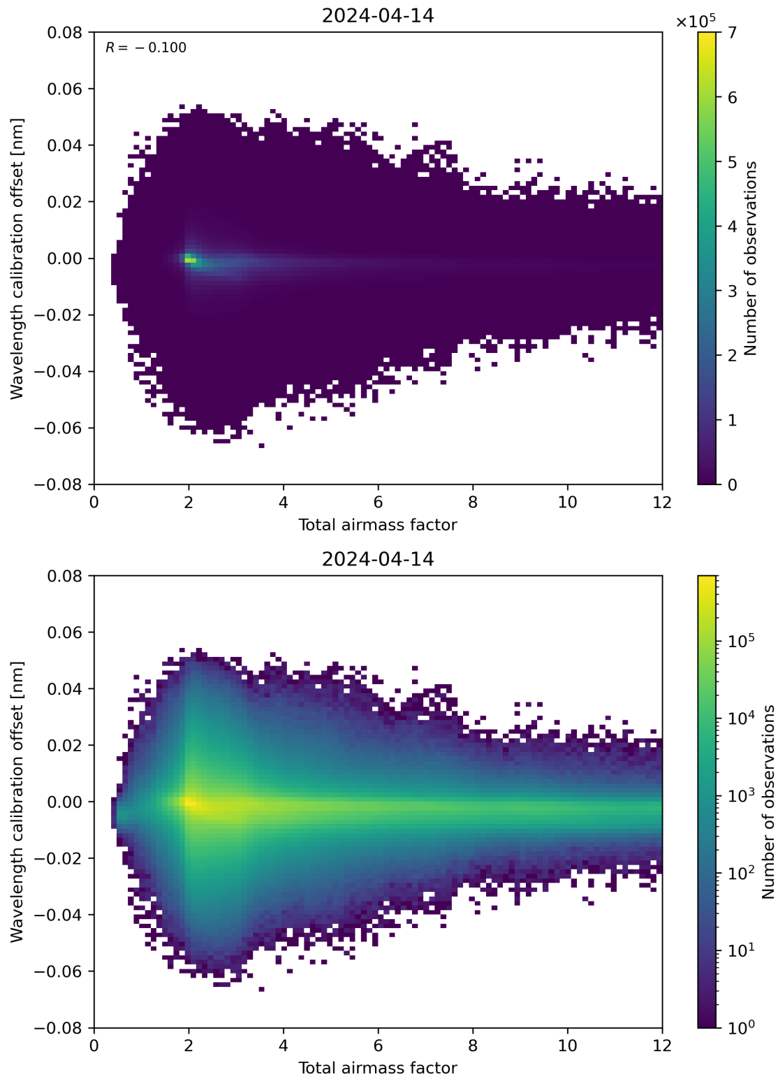
Figure 70: Scatter density plot of “Total airmass factor” against “Wavelength calibration offset” for 2024-04-13 to 2024-04-15.
