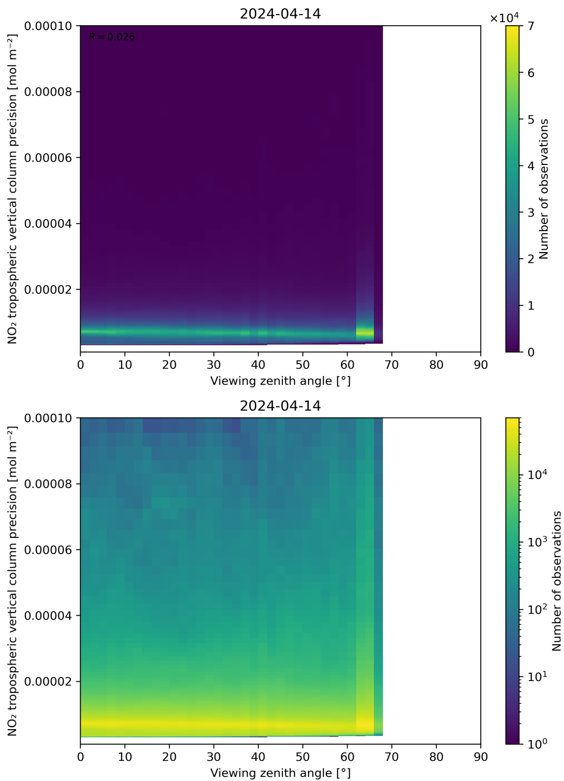
Figure 170: Scatter density plot of “Viewing zenith angle” against “NO 2 tropospheric vertical column precision” for 2024-04-13 to 2024-04-15.
