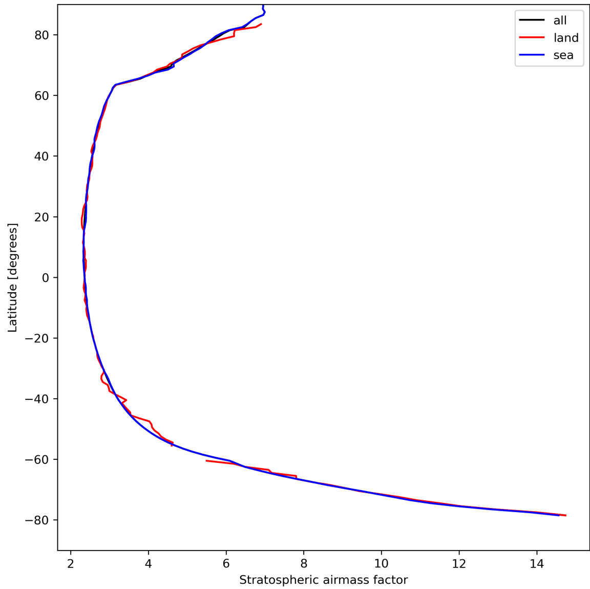
Figure 27: Zonal average of “Stratospheric air mass factor” for 2024-04-13 to 2024-04-15.
