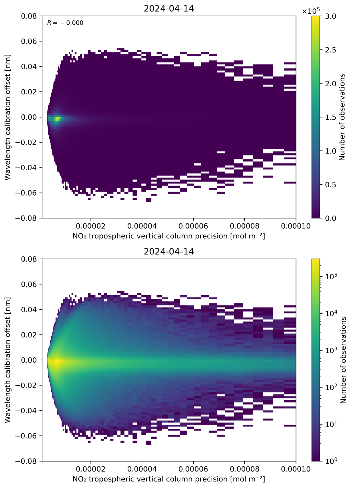
Figure 141: Scatter density plot of “NO 2 tropospheric vertical column precision” against “Wavelength calibration offset” for 2024-04-13 to 2024-04-15.
