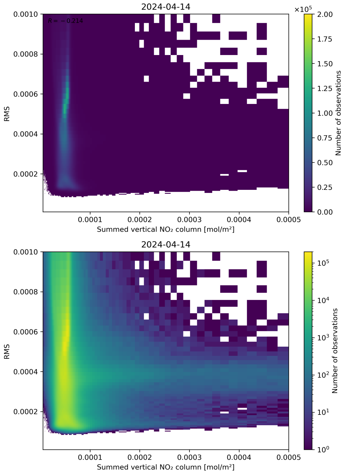
Figure 109: Scatter density plot of “Summed vertical NO 2 column” against “RMS” for 2024-04-13 to 2024-04-15.
