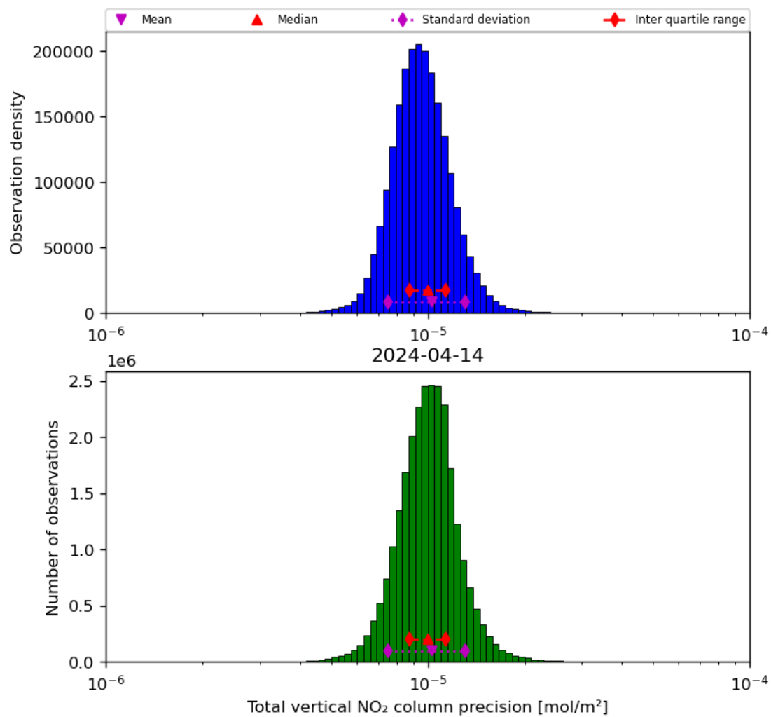
Figure 39: Histogram of "Total vertical NO 2 column precision" for 2024-04-13 to 2024-04-15
