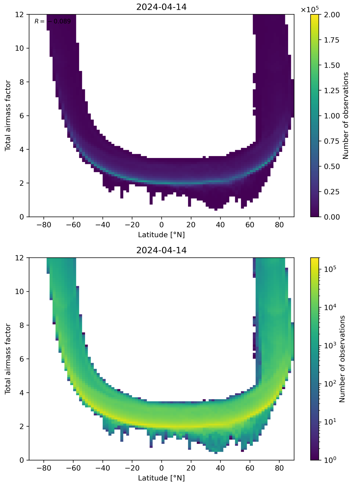
Figure 84: Scatter density plot of “Latitude” against “Total airmass factor” for 2024-04-13 to 2024-04-15.
