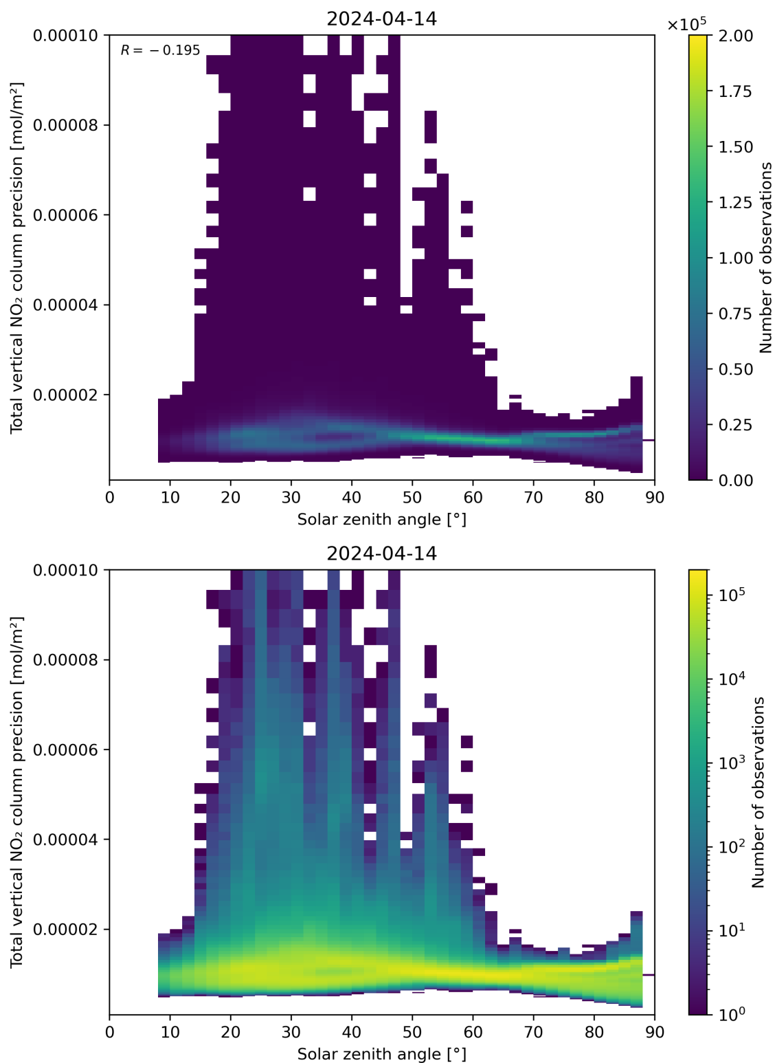
Figure 154: Scatter density plot of “Solar zenith angle” against “Total vertical NO 2 column precision” for 2024-04-13 to 2024-04-15.
