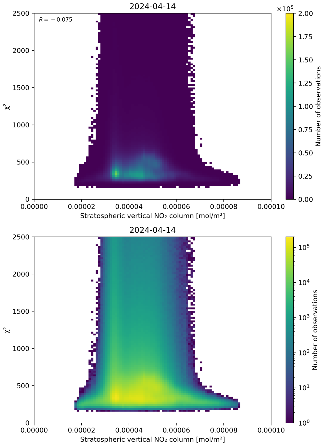
Figure 97: Scatter density plot of “Stratospheric vertical NO 2 column” against “ \chi^2 ” for 2024-04-13 to 2024-04-15.
