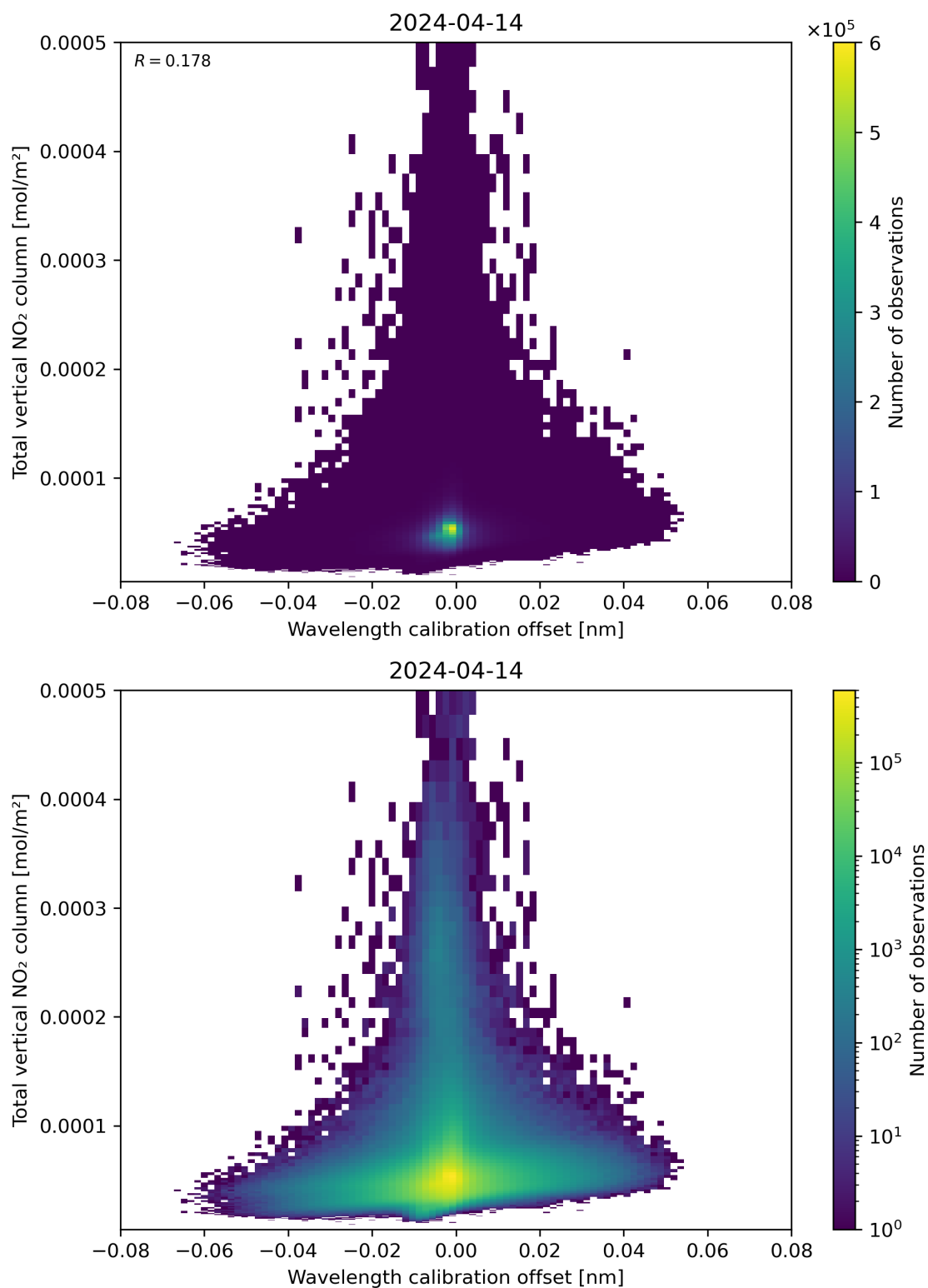
Figure 179: Scatter density plot of “Wavelength calibration offset” against “Total vertical NO 2 column” for 2024-04-13 to 2024-04-15.
