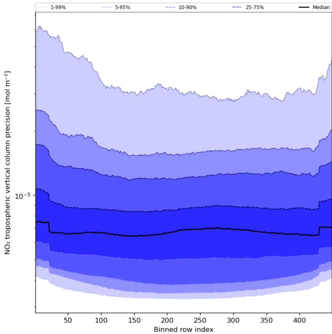
Figure 47: Along track statistics of “NO 2 tropospheric vertical column precision” for 2024-04-13 to 2024-04-15
