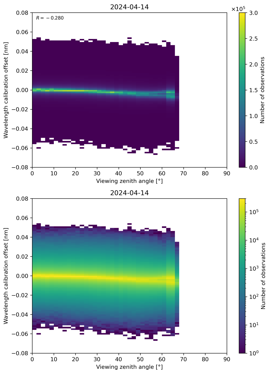
Figure 173: Scatter density plot of “Viewing zenith angle” against “Wavelength calibration offset” for 2024-04-13 to 2024-04-15.
