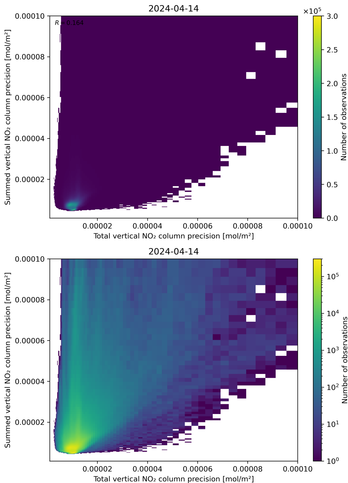
Figure 118: Scatter density plot of “Total vertical NO 2 column precision” against “Summed vertical NO 2 column precision” for 2024-04-13 to 2024-04-15.
