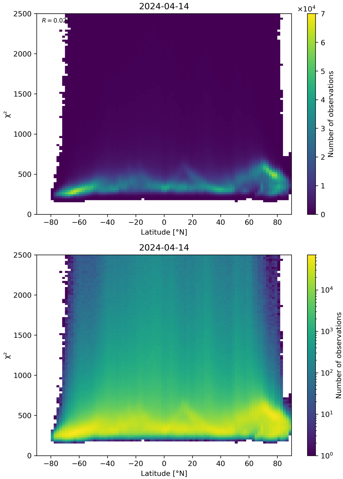
Figure 86: Scatter density plot of “Latitude” against “ \chi^2 ” for 2024-04-13 to 2024-04-15.
