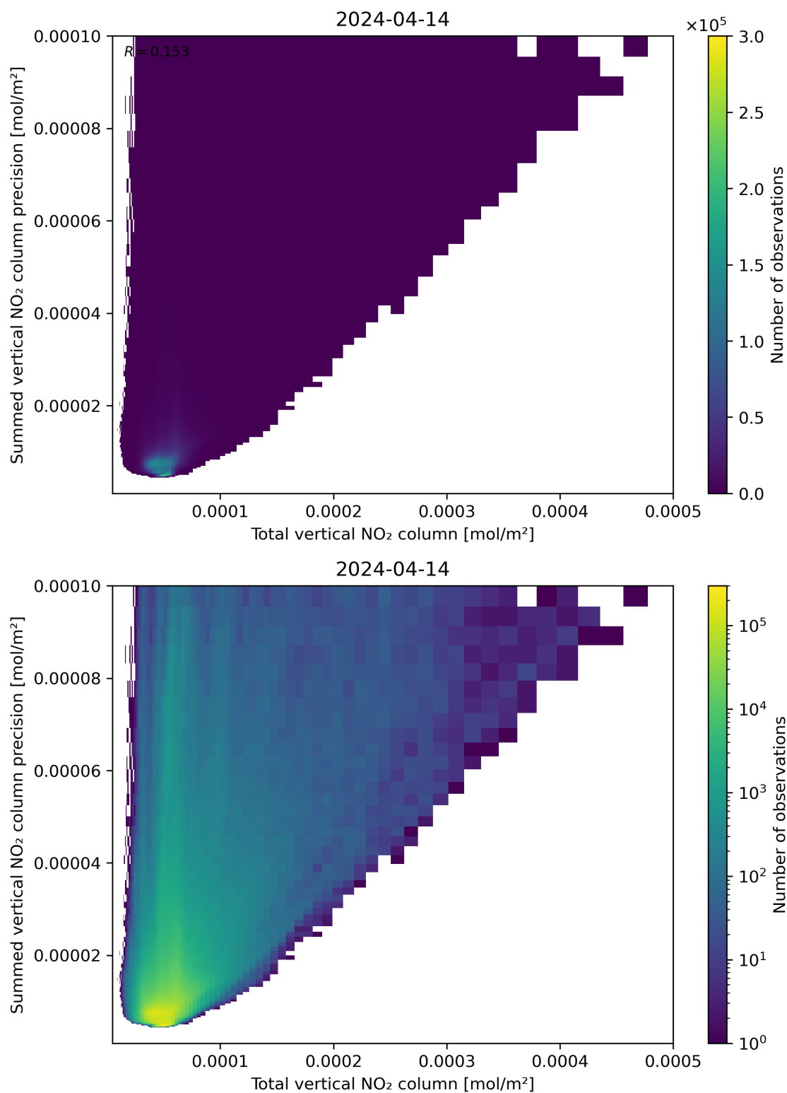
Figure 113: Scatter density plot of “Total vertical NO 2 column” against “Summed vertical NO 2 column precision” for 2024-04-13 to 2024-04-15.
