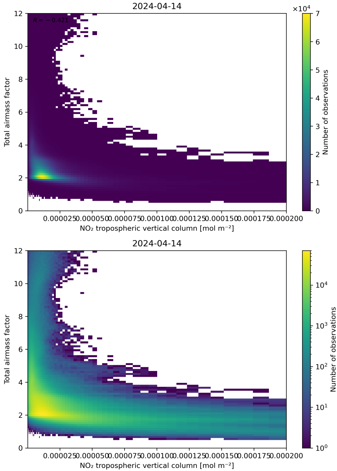
Figure 122: Scatter density plot of “NO 2 tropospheric vertical column” against “Total air mass factor” for 2024-04-13 to 2024-04-15.
