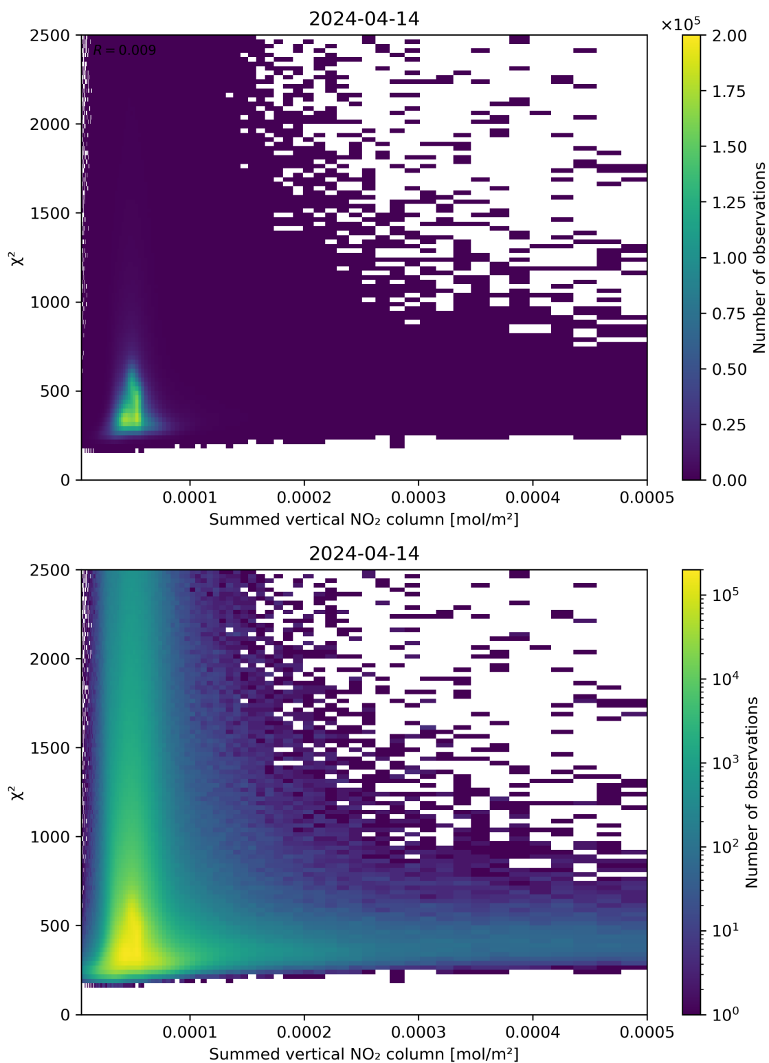
Figure 104: Scatter density plot of “Summed vertical NO 2 column” against “ \chi^2 ” for 2024-04-13 to 2024-04-15.
