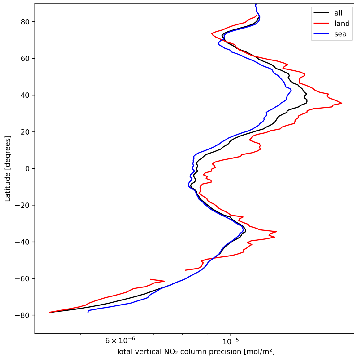
Figure 22: Zonal average of “Total vertical NO 2 column precision” for 2024-04-13 to 2024-04-15.
