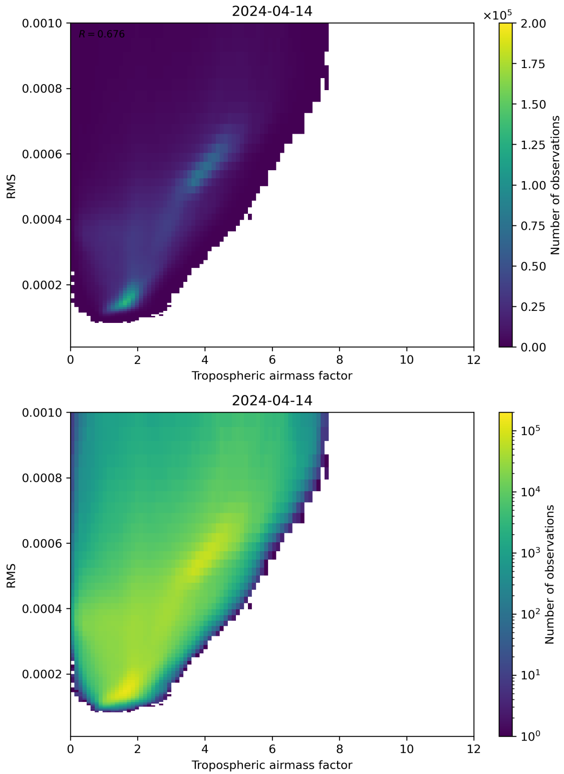
Figure 79: Scatter density plot of “Tropospheric airmass factor” against “RMS” for 2024-04-13 to 2024-04-15.
