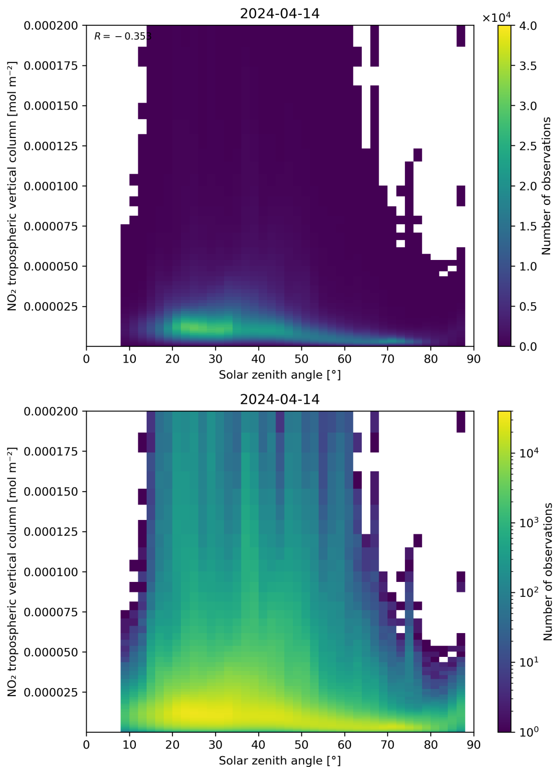
Figure 155: Scatter density plot of “Solar zenith angle” against “NO 2 tropospheric vertical column” for 2024-04-13 to 2024-04-15.
