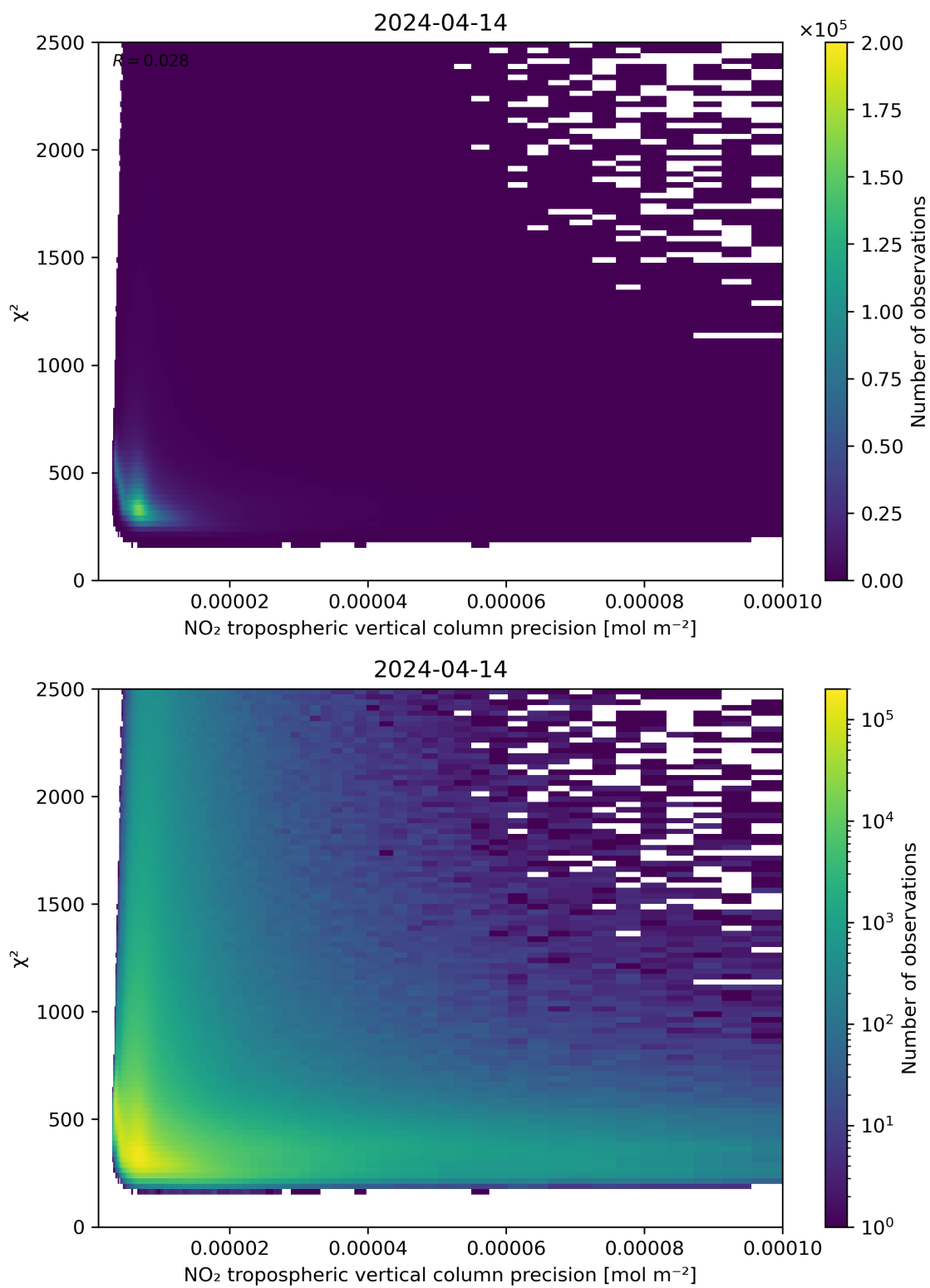
Figure 134: Scatter density plot of “NO 2 tropospheric vertical column precision” against “ \chi^2 ” for 2024-04-13 to 2024-04-15.
