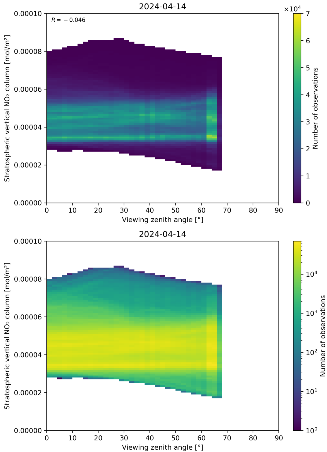
Figure 164: Scatter density plot of “Viewing zenith angle” against “Stratospheric vertical NO 2 column” for 2024-04-13 to 2024-04-15.
