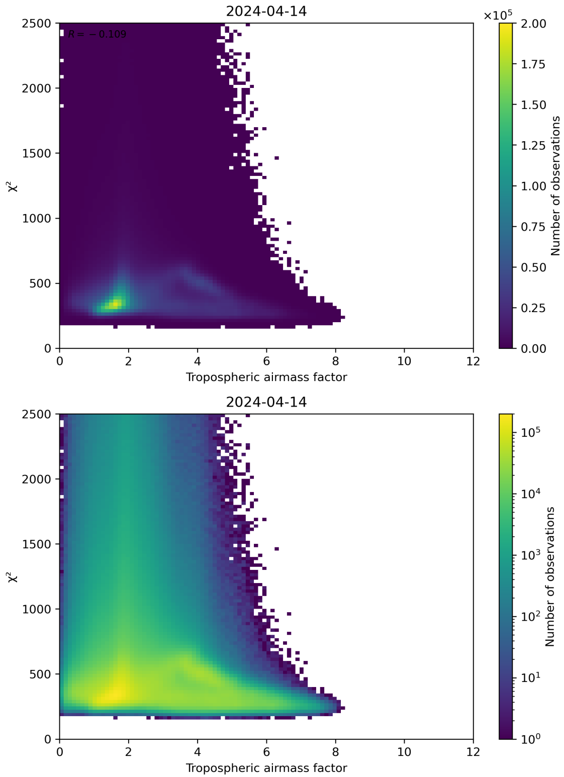
Figure 73: Scatter density plot of “Tropospheric airmass factor” against “ \chi^2 ” for 2024-04-13 to 2024-04-15.
