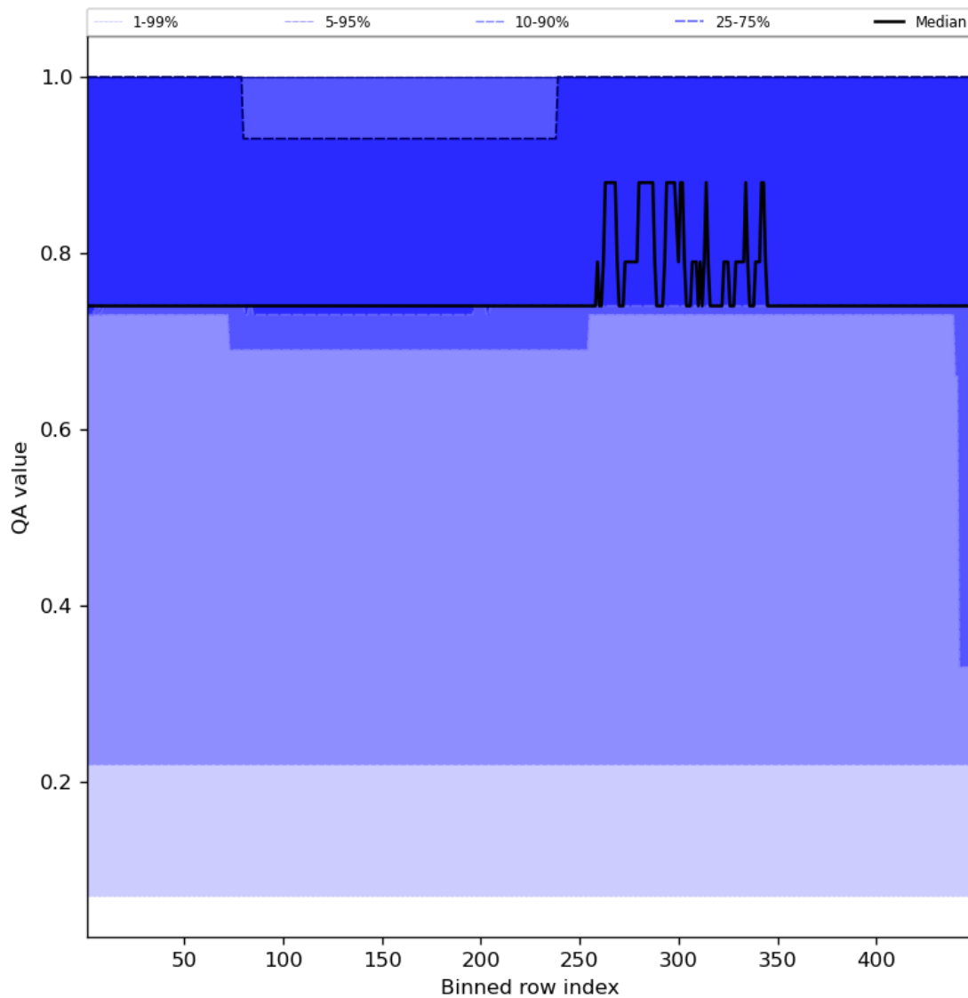
Figure 45: Along track statistics of “QA value” for 2024-04-13 to 2024-04-15
