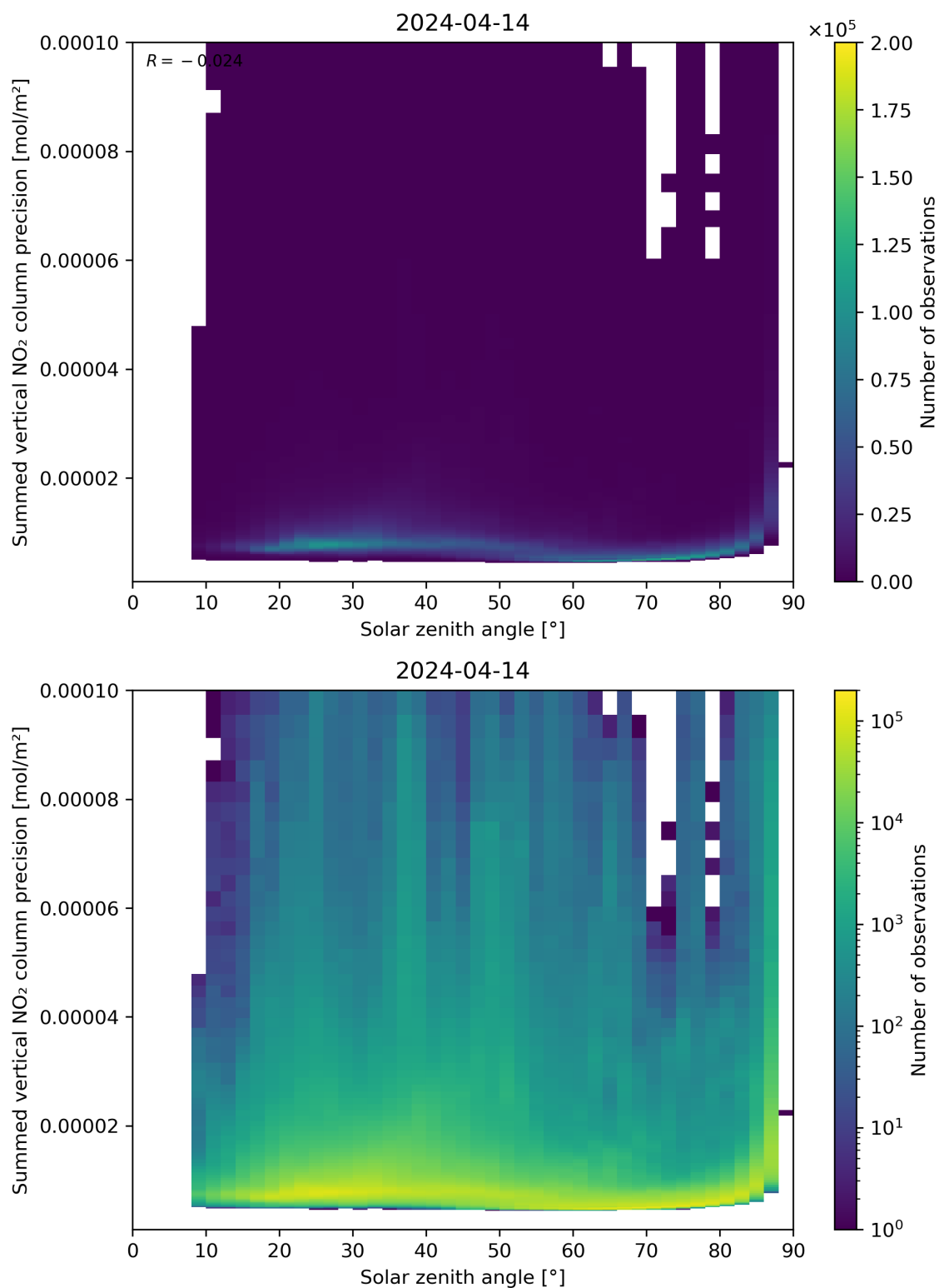
Figure 152: Scatter density plot of “Solar zenith angle” against “Summed vertical NO 2 column precision” for 2024-04-13 to 2024-04-15.
