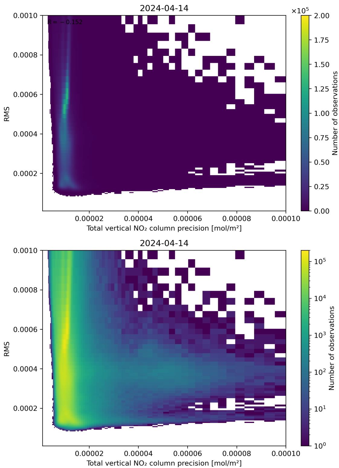
Figure 119: Scatter density plot of “Total vertical NO 2 column precision” against “RMS” for 2024-04-13 to 2024-04-15.
