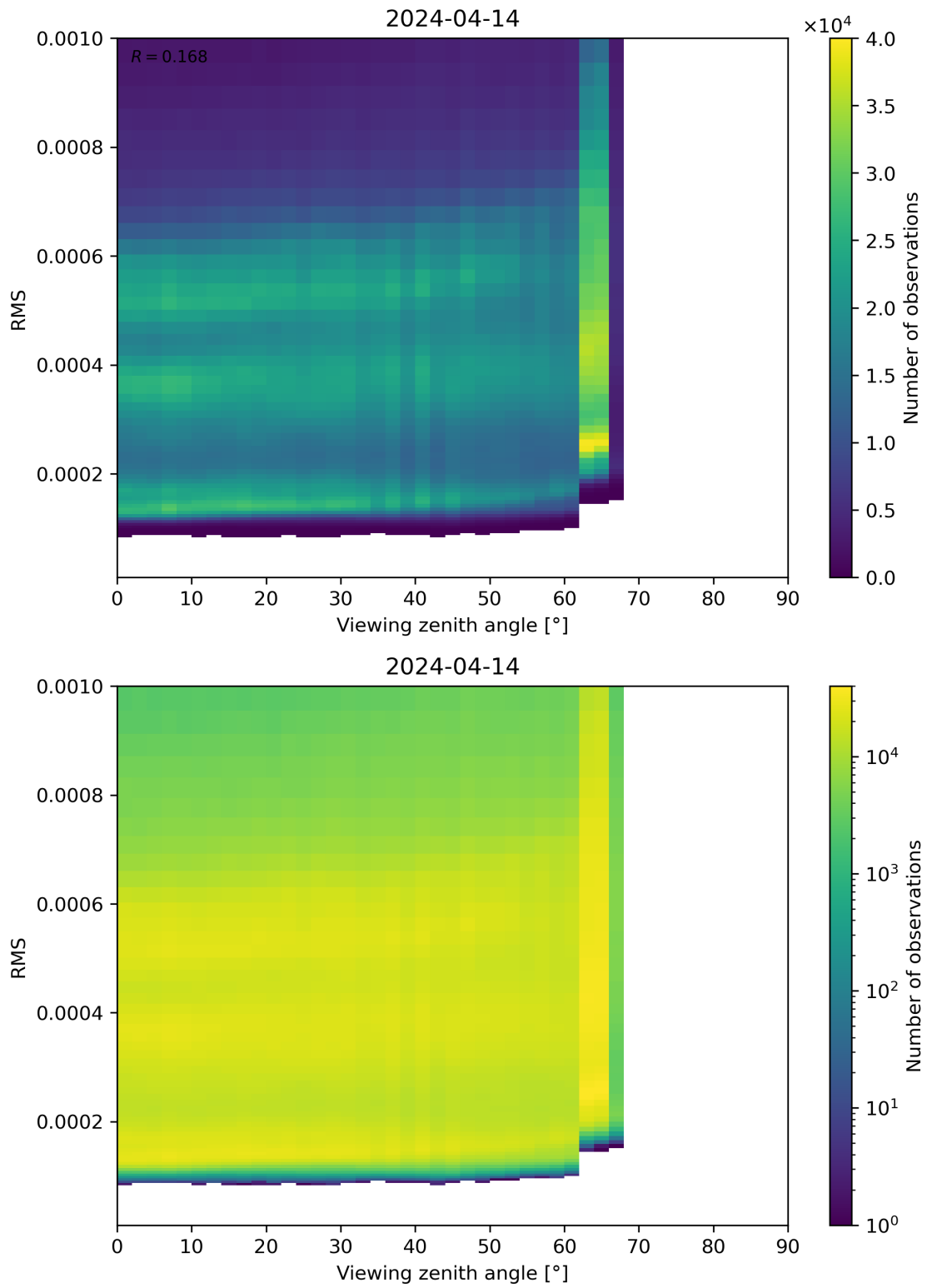
Figure 171: Scatter density plot of “Viewing zenith angle” against “RMS” for 2024-04-13 to 2024-04-15.
