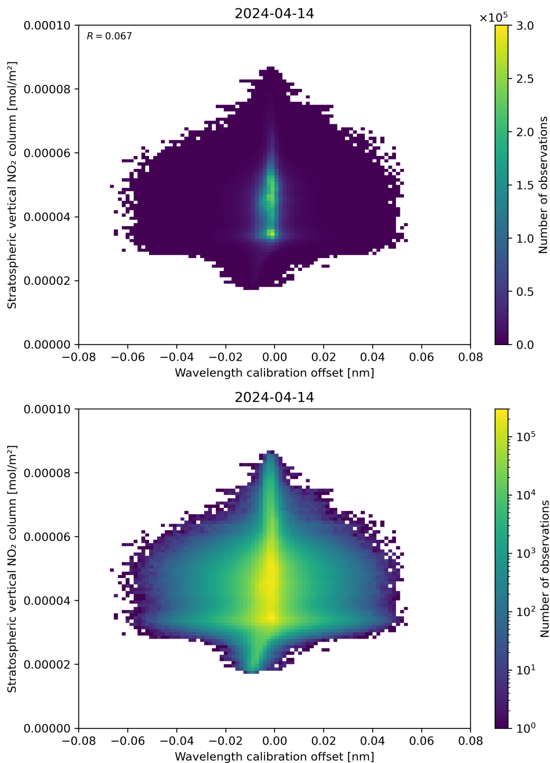
Figure 176: Scatter density plot of “Wavelength calibration offset” against “Stratospheric vertical NO 2 column” for 2024-04-13 to 2024-04-15.
