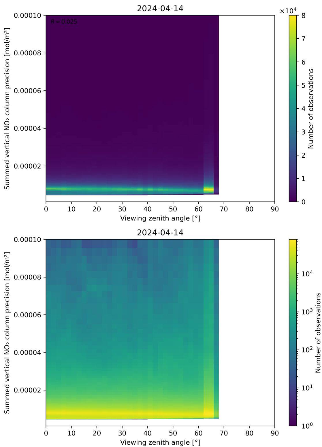
Figure 166: Scatter density plot of “Viewing zenith angle” against “Summed vertical NO 2 column precision” for 2024-04-13 to 2024-04-15.
