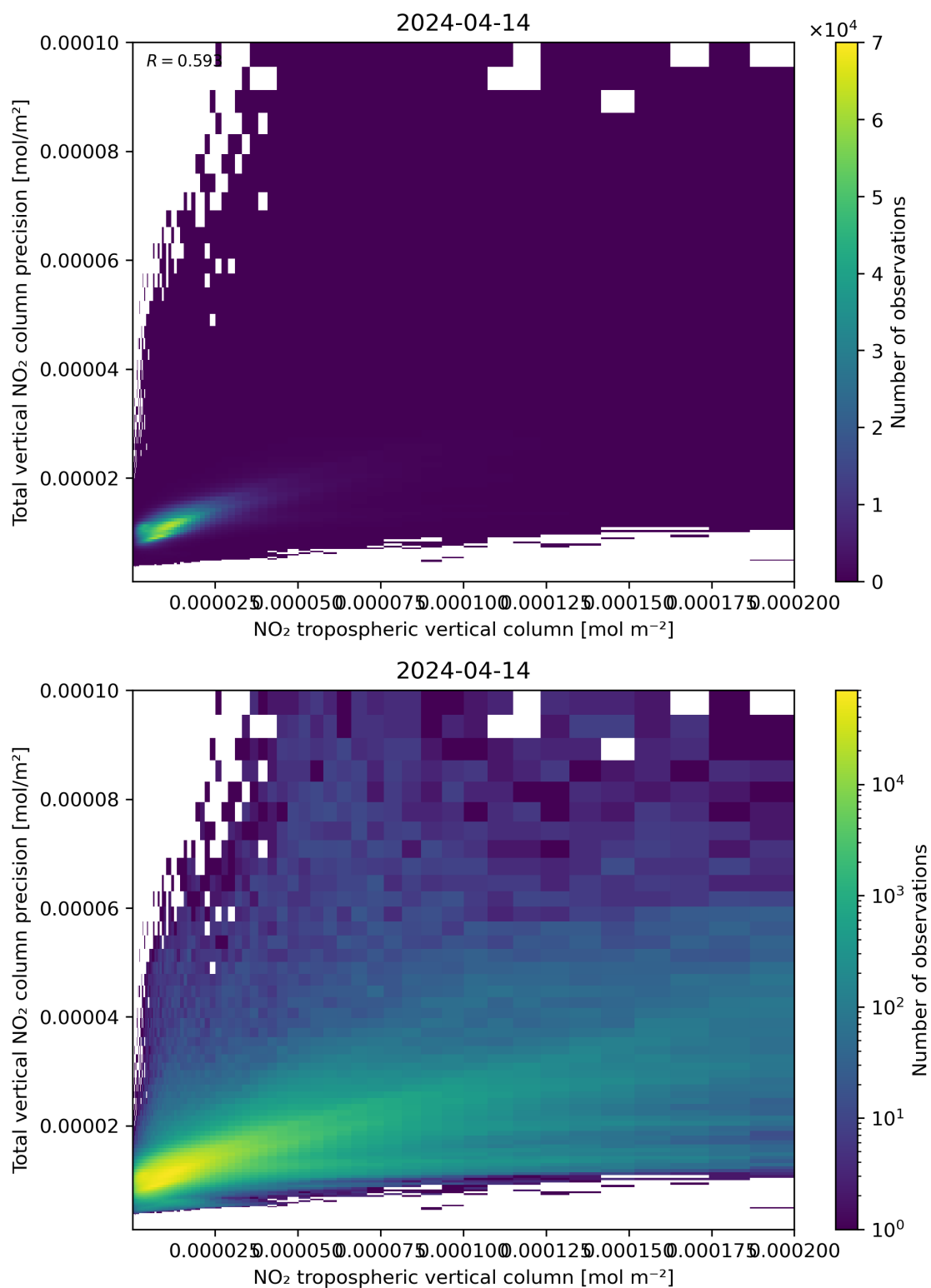
Figure 129: Scatter density plot of “NO 2 tropospheric vertical column” against “Total vertical NO 2 column precision” for 2024-04-13 to 2024-04-15.
