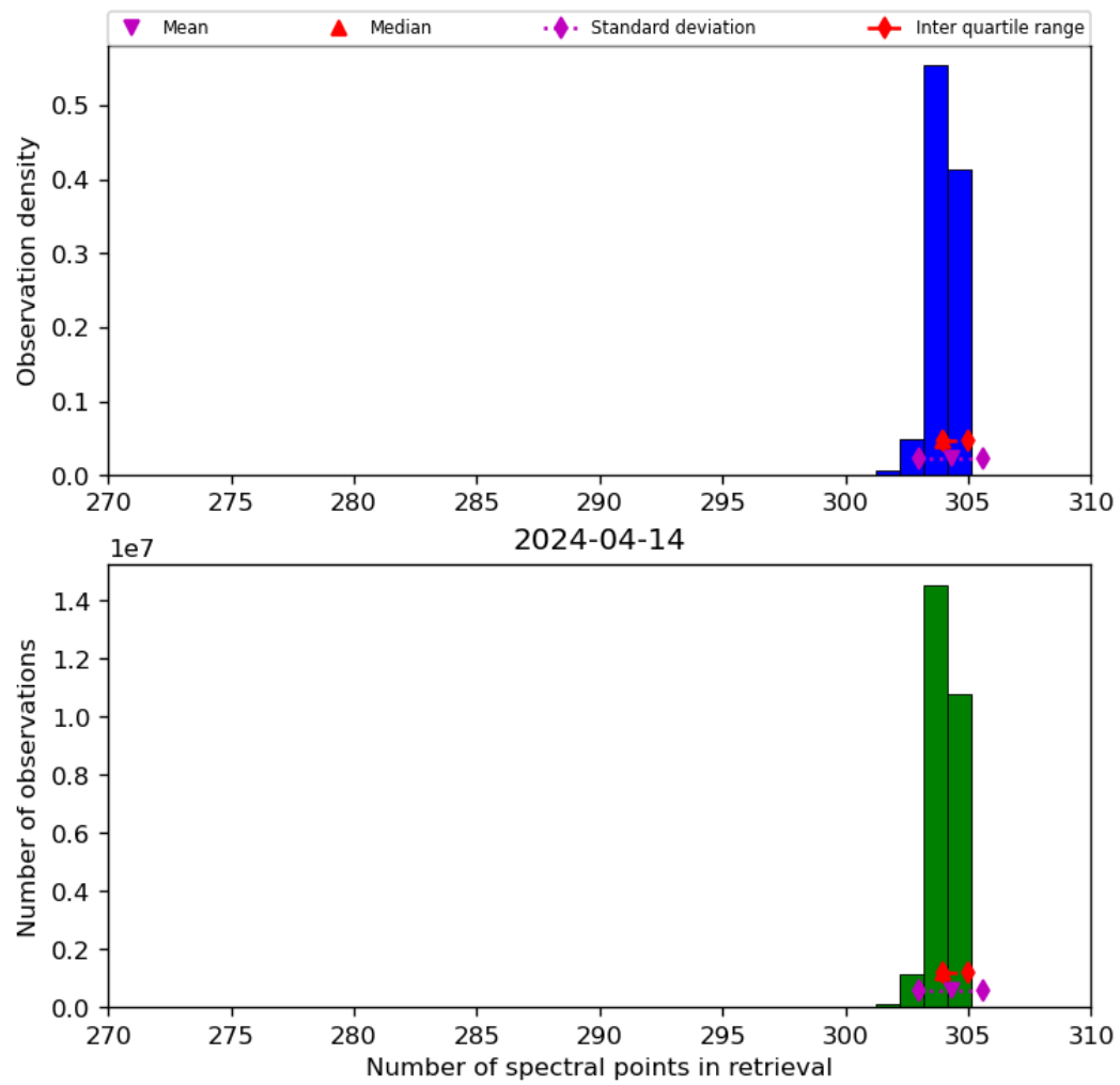
Figure 33: Histogram of “Number of spectral points in retrieval” for 2024-04-13 to 2024-04-15
