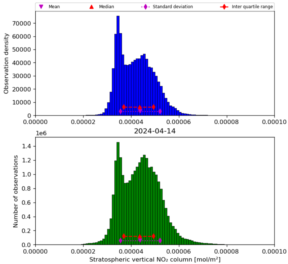
Figure 36: Histogram of “Stratospheric vertical NO 2 column” for 2024-04-13 to 2024-04-15
