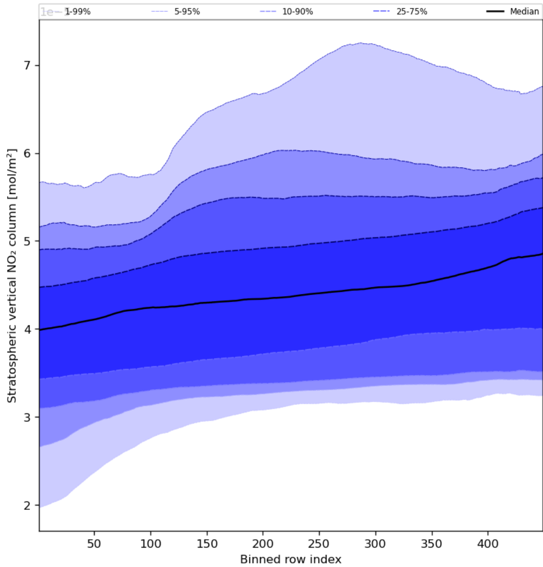
Figure 53: Along track statistics of “Stratospheric vertical NO 2 column” for 2024-04-13 to 2024-04-15
