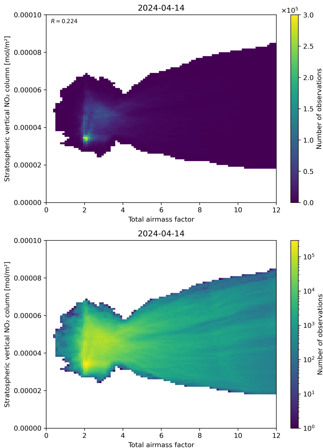
Figure 64: Scatter density plot of “Total airmass factor” against “Stratospheric vertical \text{NO}_2 column” for 2024-04-13 to 2024-04-15.
