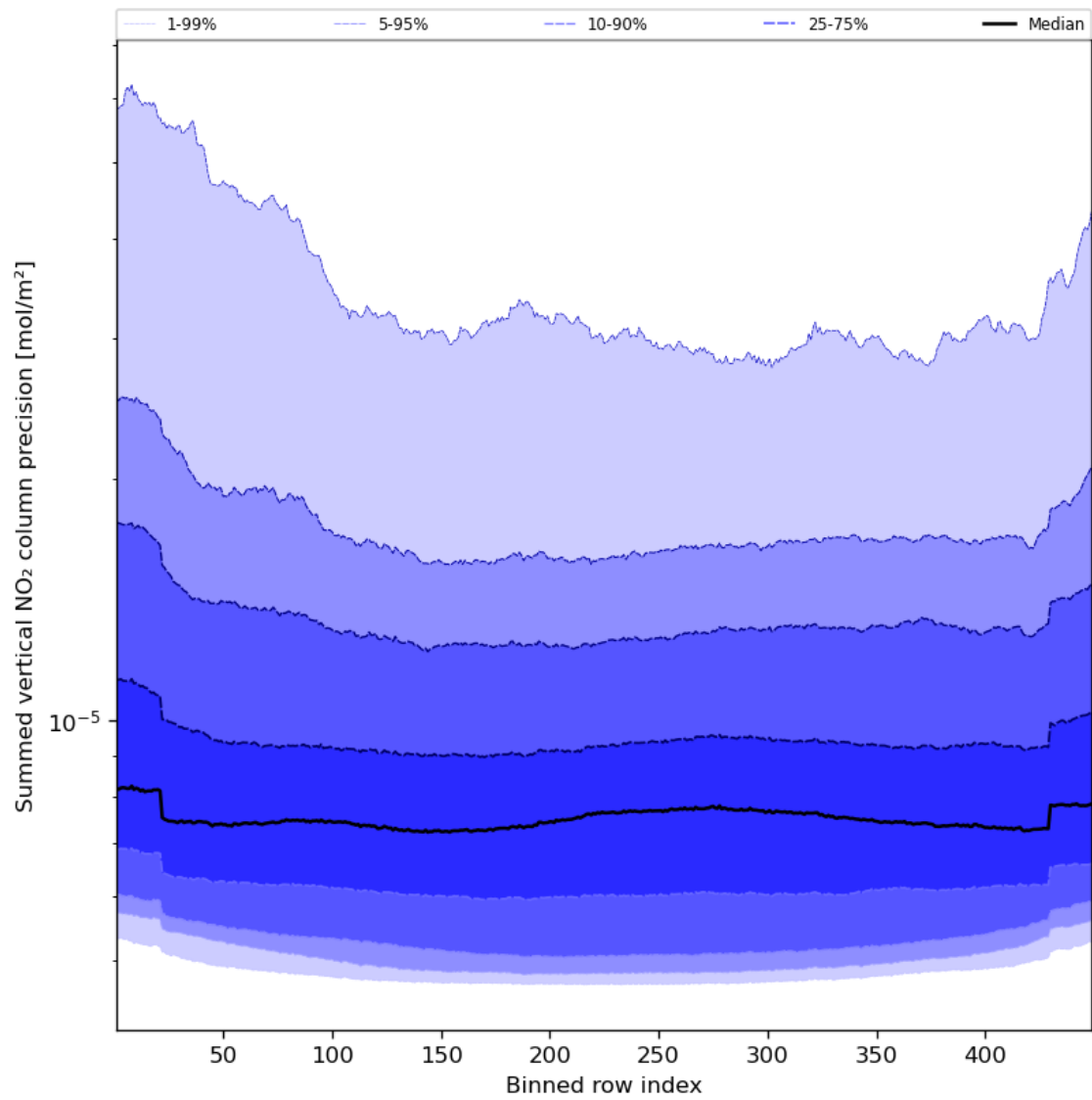
Figure 58: Along track statistics of “Summed vertical NO 2 column precision” for 2024-04-13 to 2024-04-15
