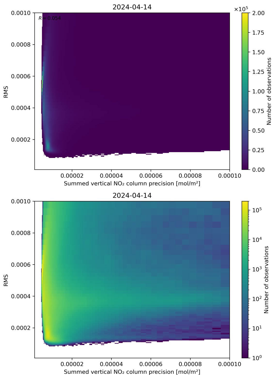
Figure 108: Scatter density plot of “Summed vertical NO 2 column precision” against “RMS” for 2024-04-13 to 2024-04-15.
