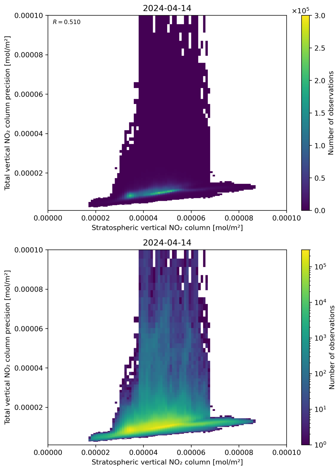
Figure 101: Scatter density plot of “Stratospheric vertical NO 2 column” against “Total vertical NO 2 column precision” for 2024-04-13 to 2024-04-15.
