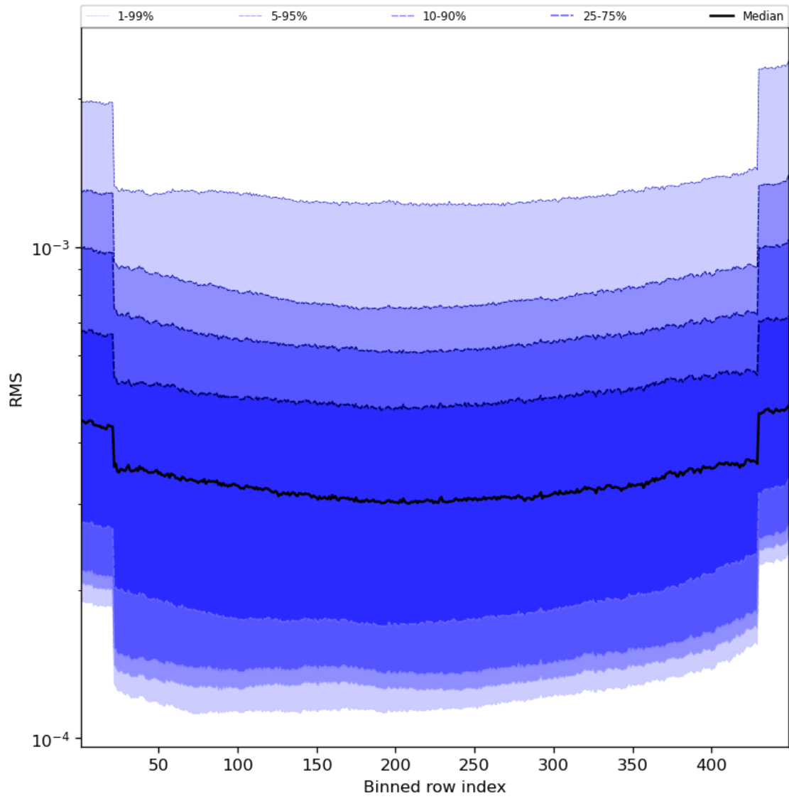
Figure 60: Along track statistics of “RMS” for 2024-04-13 to 2024-04-15
