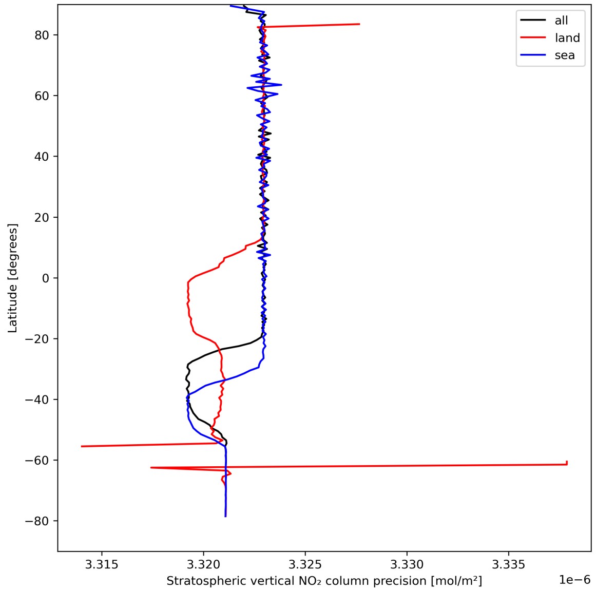
Figure 20: Zonal average of “Stratospheric vertical NO 2 column precision” for 2024-04-13 to 2024-04-15.
