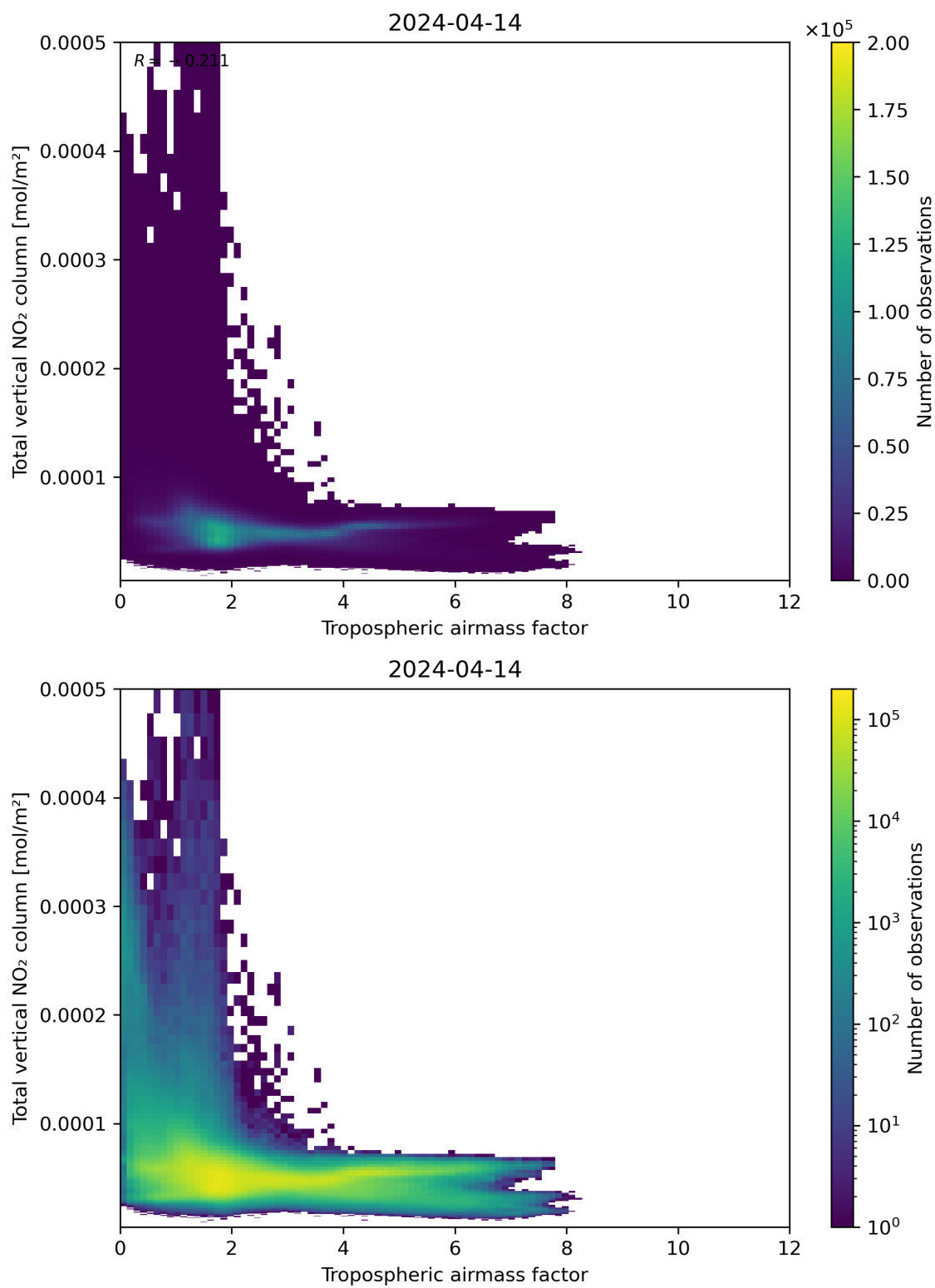
Figure 77: Scatter density plot of “Tropospheric airmass factor” against “Total vertical NO 2 column” for 2024-04-13 to 2024-04-15.
