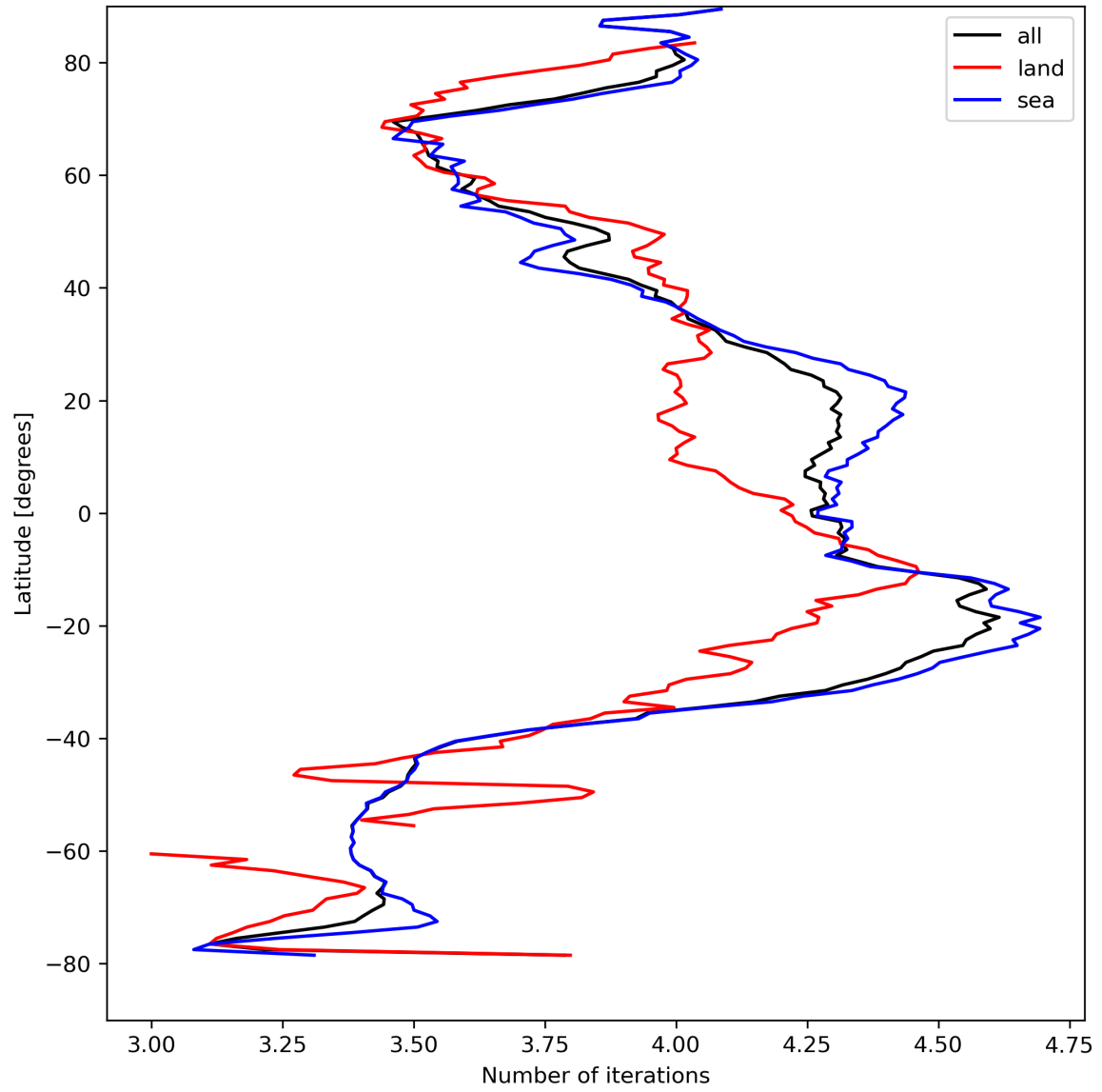
Figure 17: Zonal average of “Number of iterations” for 2024-04-13 to 2024-04-15.
