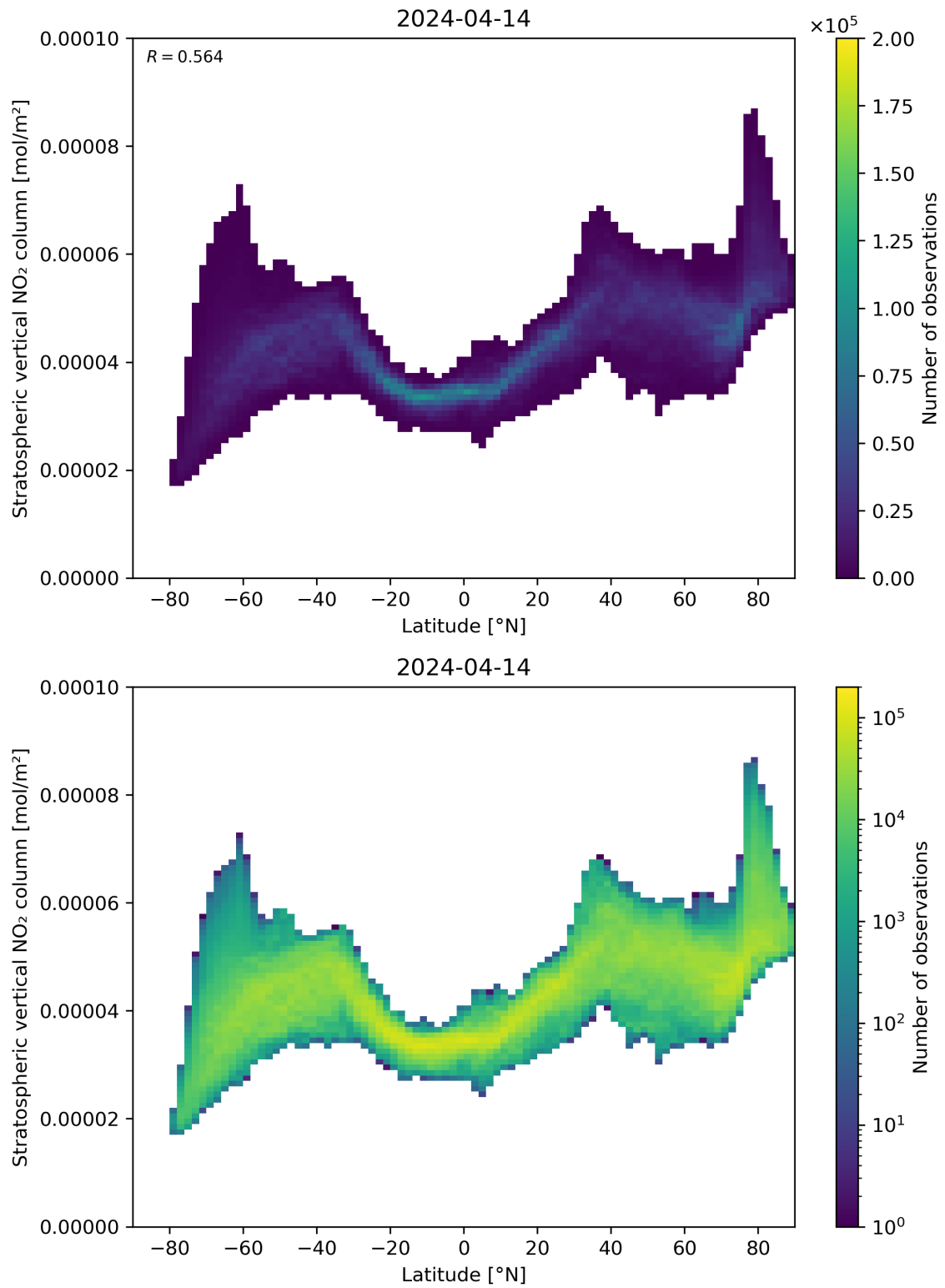
Figure 87: Scatter density plot of “Latitude” against “Stratospheric vertical \text{NO}_2 column” for 2024-04-13 to 2024-04-15.
