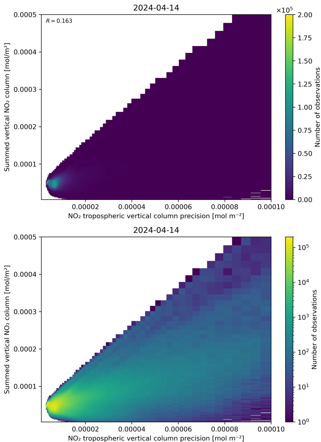
Figure 136: Scatter density plot of “NO 2 tropospheric vertical column precision” against “Summed vertical NO 2 column” for 2024-04-13 to 2024-04-15.
