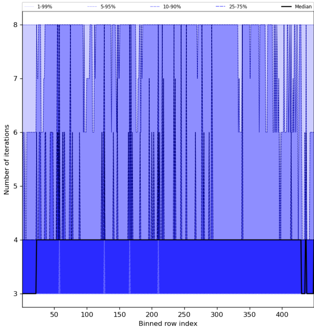
Figure 51: Along track statistics of “Number of iterations” for 2024-04-13 to 2024-04-15
