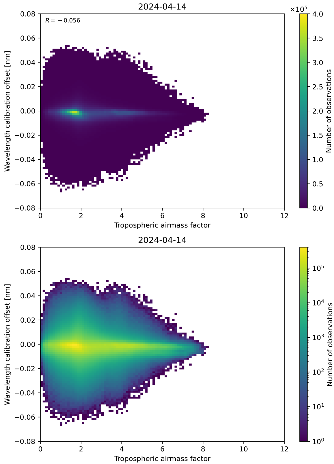
Figure 80: Scatter density plot of “Tropospheric airmass factor” against “Wavelength calibration offset” for 2024-04-13 to 2024-04-15.
