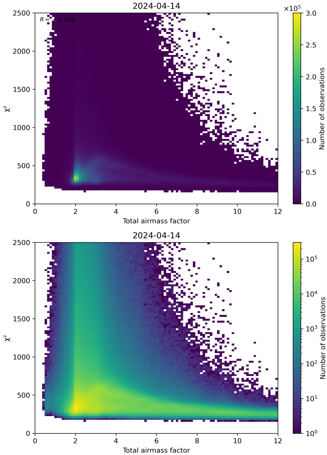
Figure 63: Scatter density plot of “Total airmass factor” against “ \chi^2 ” for 2024-04-13 to 2024-04-15.
