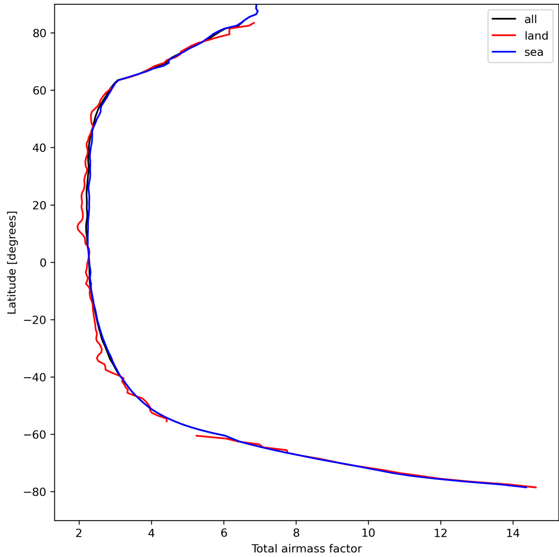
Figure 15: Zonal average of “Total airmass factor” for 2024-04-13 to 2024-04-15.
