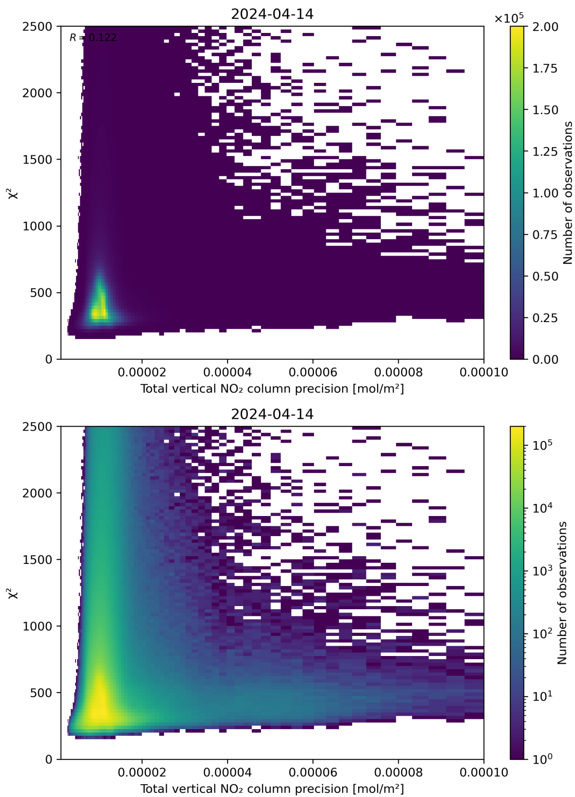
Figure 116: Scatter density plot of “Total vertical NO 2 column precision” against “ \chi^2 ” for 2024-04-13 to 2024-04-15.
