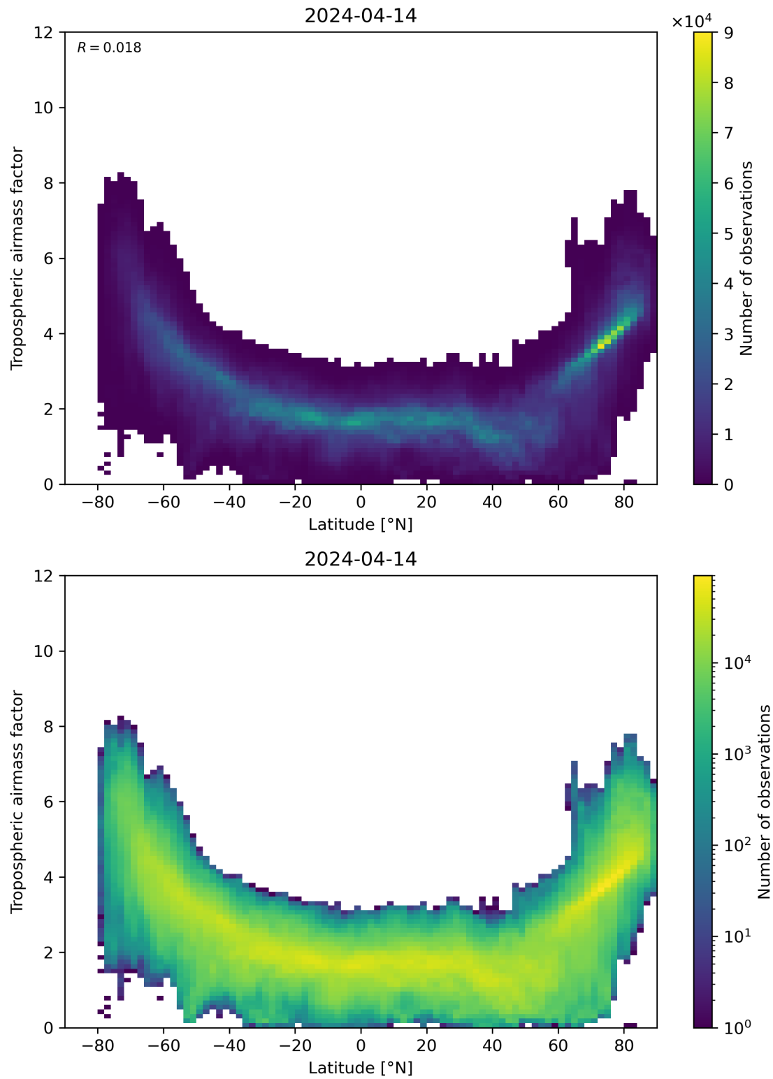
Figure 85: Scatter density plot of “Latitude” against “Tropospheric air mass factor” for 2024-04-13 to 2024-04-15.
