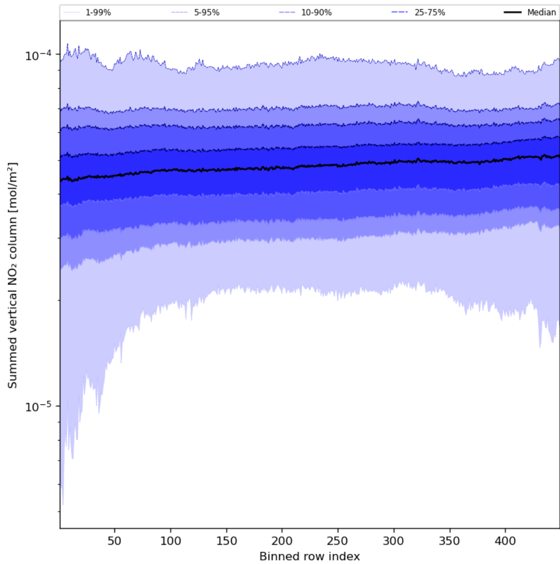
Figure 57: Along track statistics of “Summed vertical NO 2 column” for 2024-04-13 to 2024-04-15
