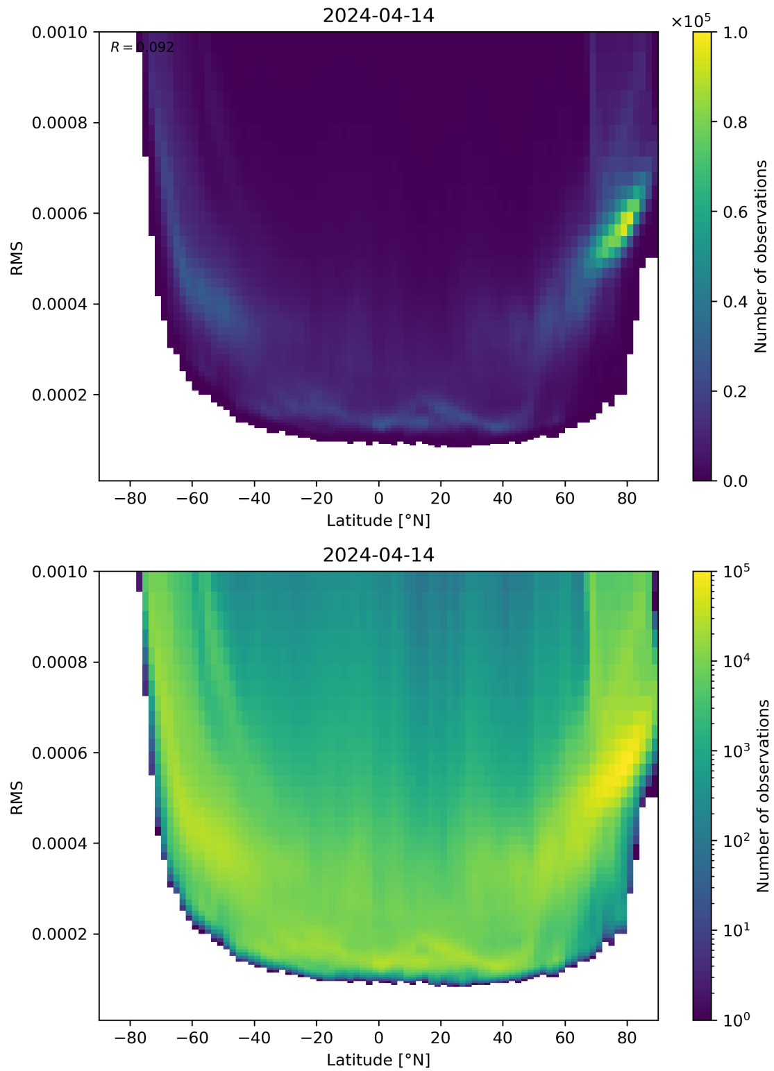
Figure 94: Scatter density plot of “Latitude” against “RMS” for 2024-04-13 to 2024-04-15.
