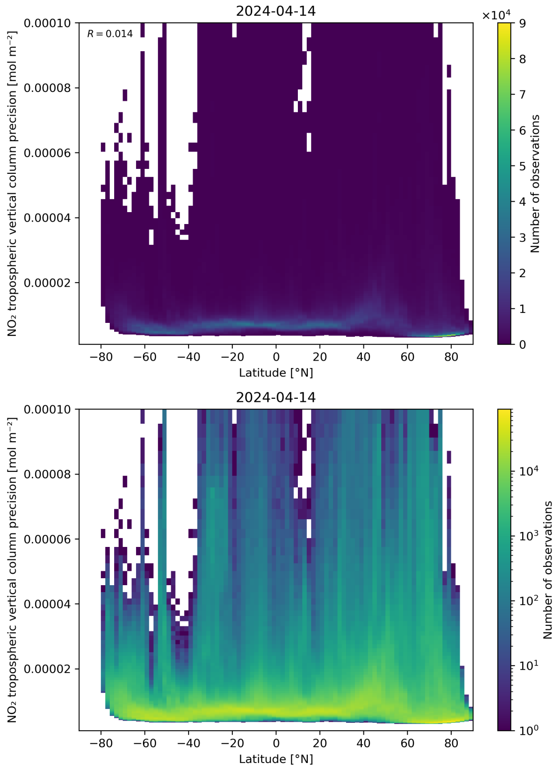
Figure 93: Scatter density plot of “Latitude” against “NO 2 tropospheric vertical column precision” for 2024-04-13 to 2024-04-15.
