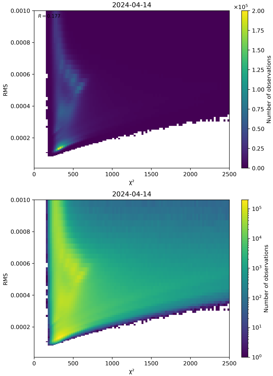
Figure 82: Scatter density plot of “ \chi^2 ” against “RMS” for 2024-04-13 to 2024-04-15.
