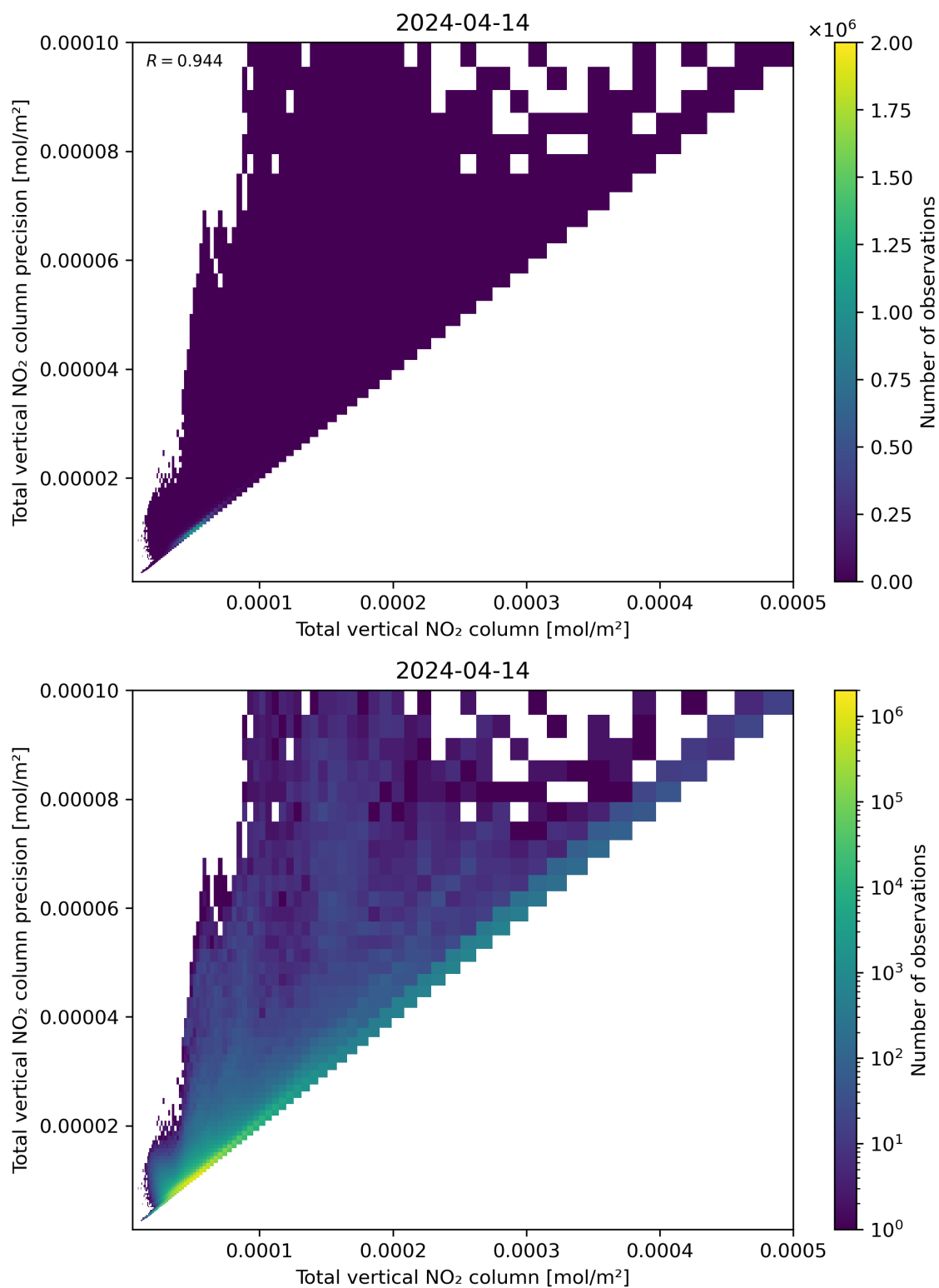
Figure 114: Scatter density plot of “Total vertical NO 2 column” against “Total vertical NO 2 column precision” for 2024-04-13 to 2024-04-15.
