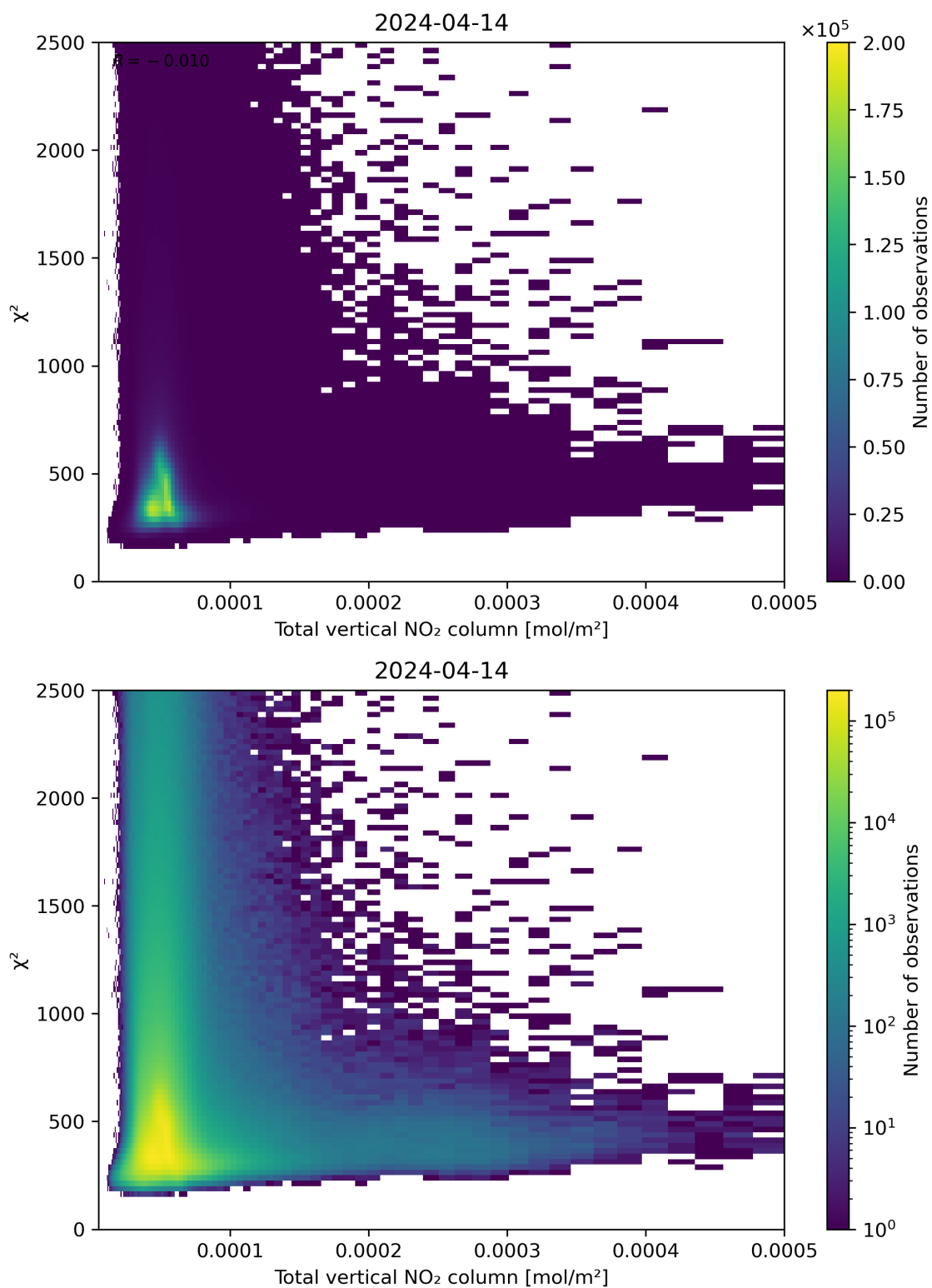
Figure 111: Scatter density plot of “Total vertical NO 2 column” against “ \chi^2 ” for 2024-04-13 to 2024-04-15.
