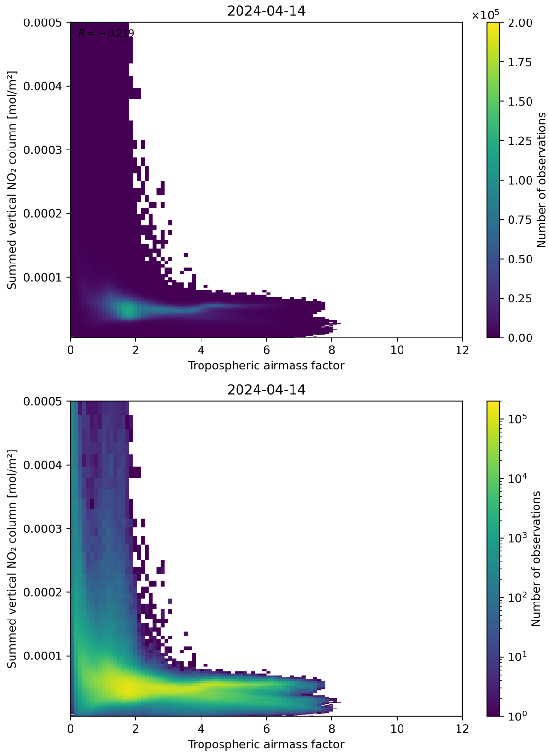
Figure 75: Scatter density plot of “Tropospheric air mass factor” against “Summed vertical NO 2 column” for 2024-04-13 to 2024-04-15.
