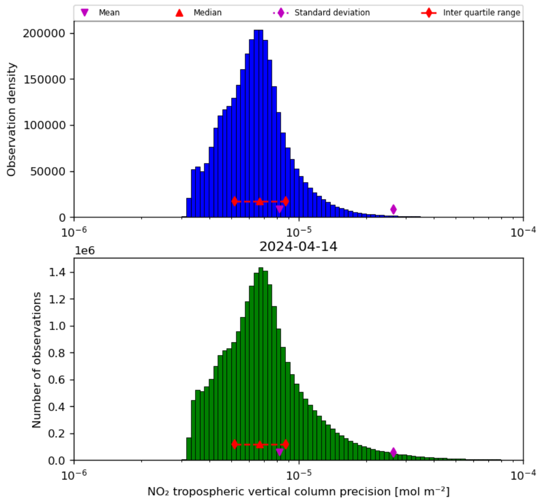
Figure 30: Histogram of “NO 2 tropospheric vertical column precision” for 2024-04-13 to 2024-04-15
