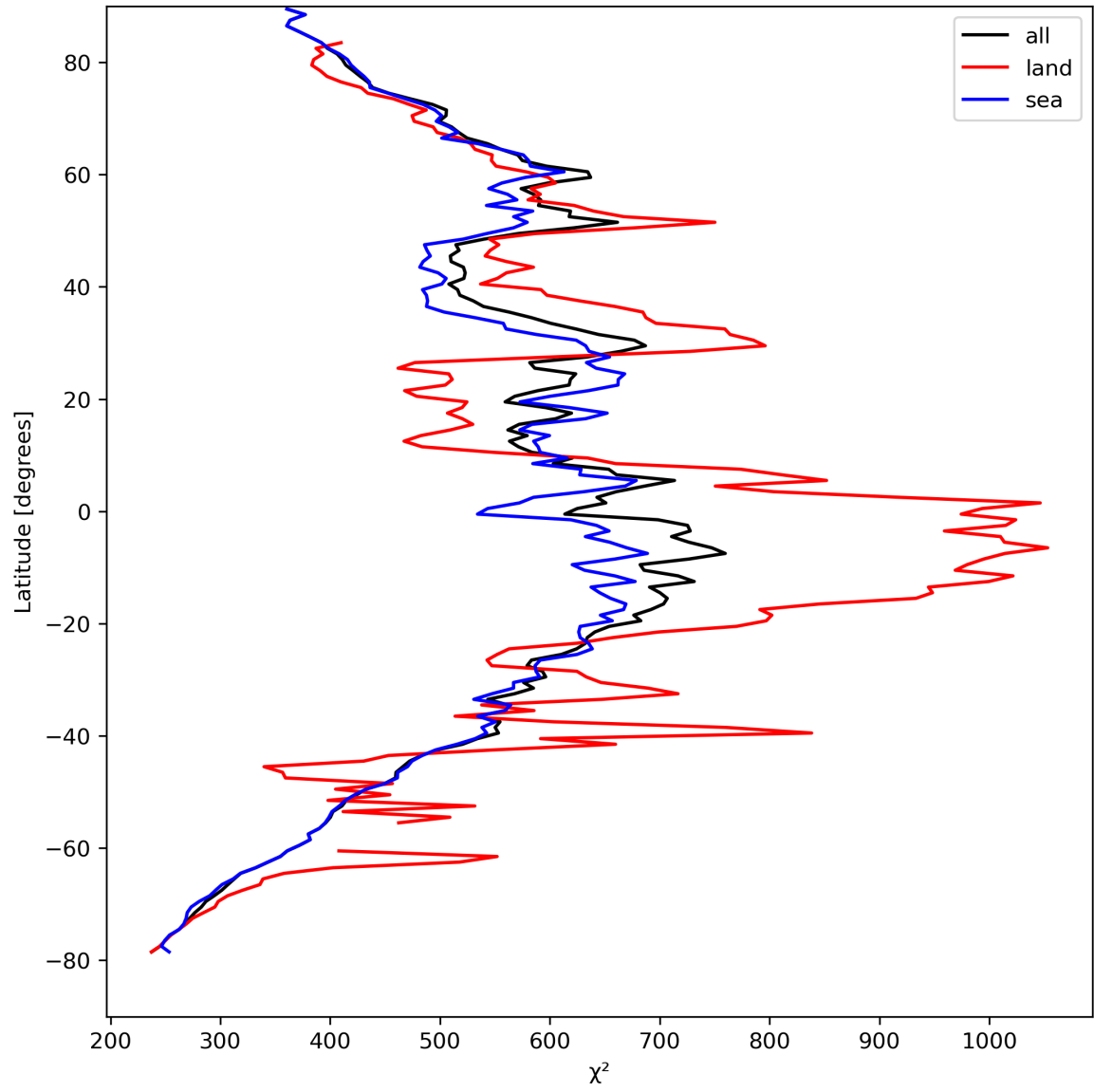
Figure 25: Zonal average of “ \chi^2 ” for 2024-04-13 to 2024-04-15.
