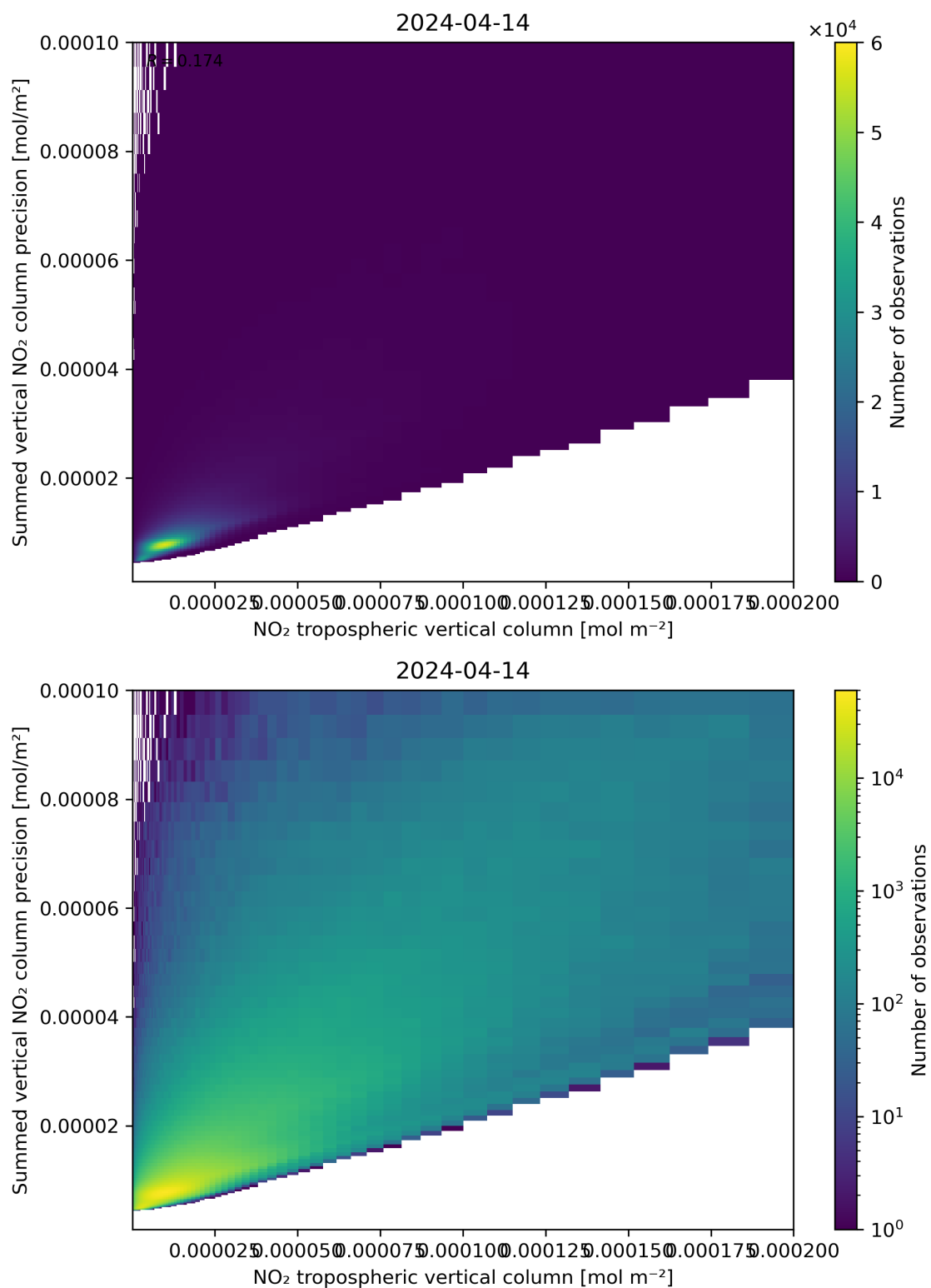
Figure 127: Scatter density plot of “NO 2 tropospheric vertical column” against “Summed vertical NO 2 column precision” for 2024-04-13 to 2024-04-15.
