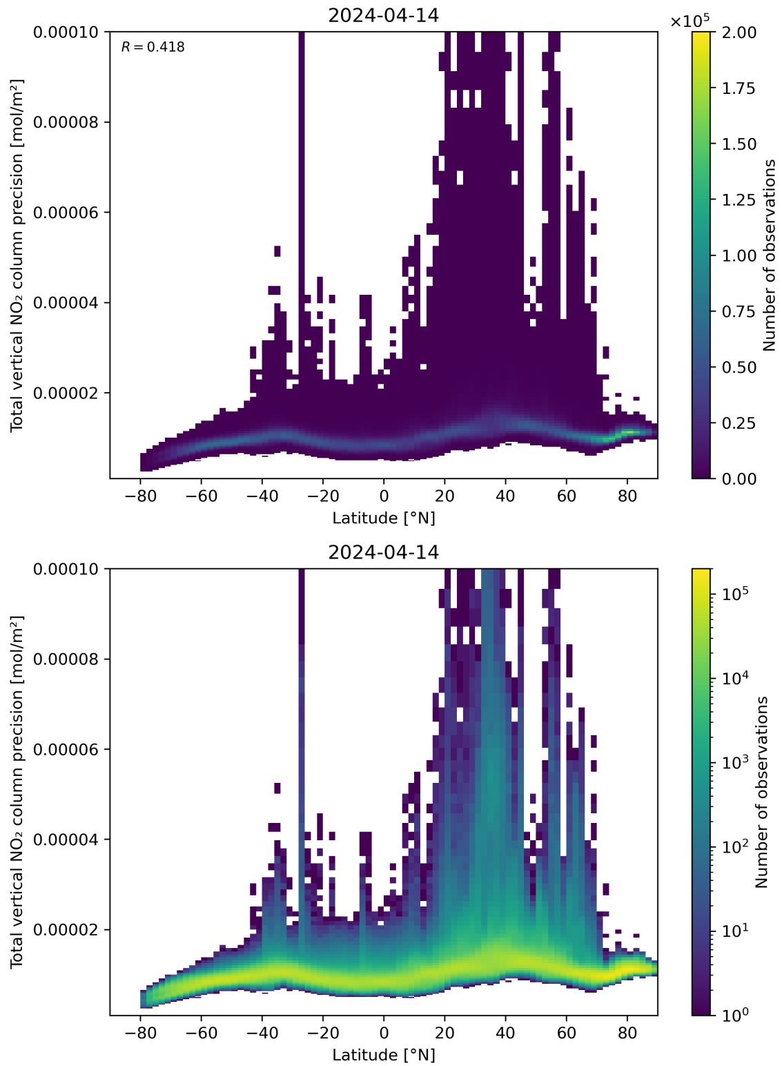
Figure 91: Scatter density plot of “Latitude” against “Total vertical NO 2 column precision” for 2024-04-13 to 2024-04-15.
