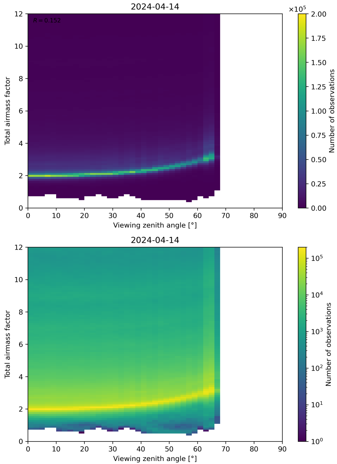
Figure 160: Scatter density plot of “Viewing zenith angle” against “Total airmass factor” for 2024-04-13 to 2024-04-15.
