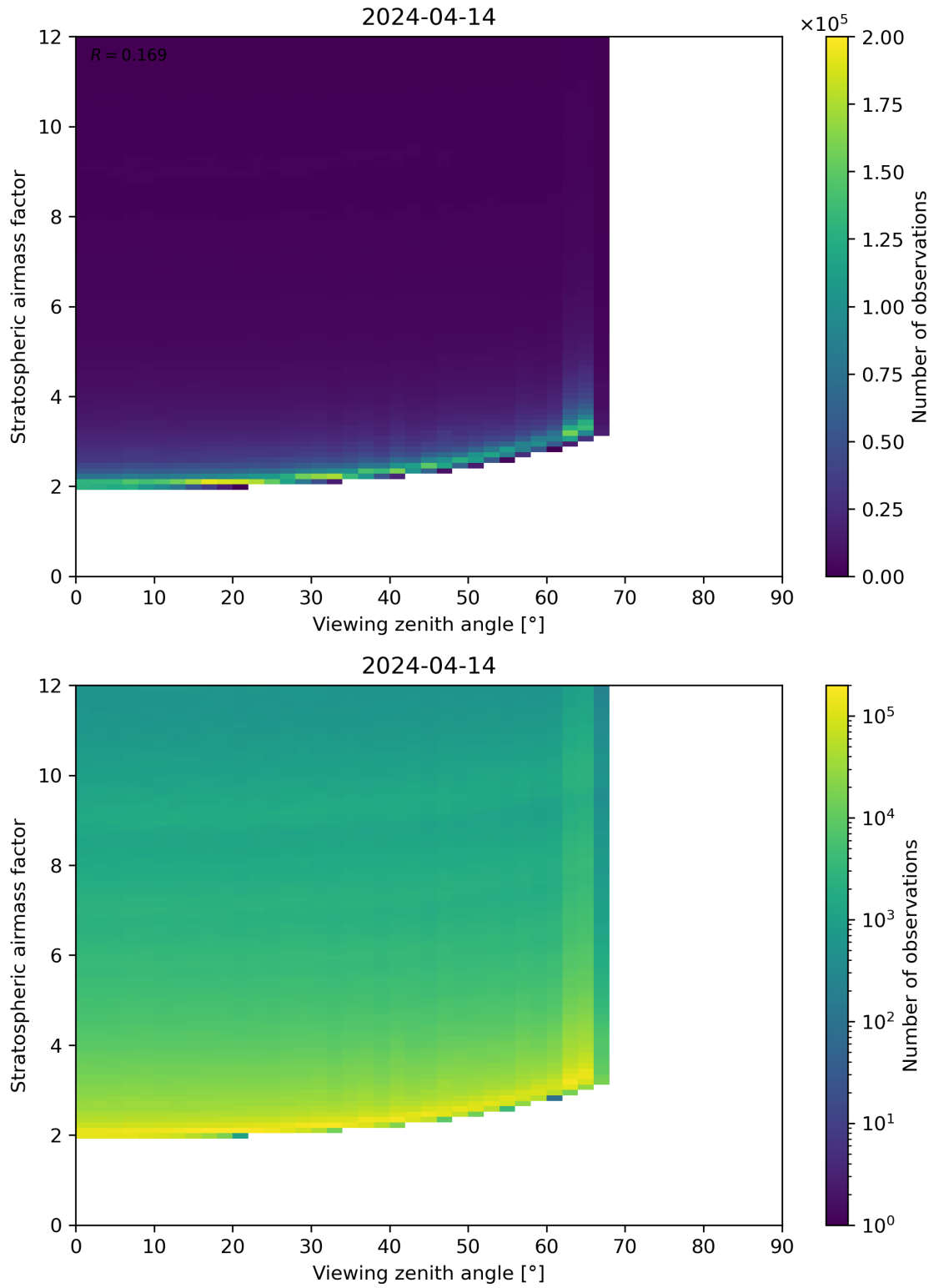
Figure 159: Scatter density plot of “Viewing zenith angle” against “Stratospheric airmass factor” for 2024-04-13 to 2024-04-15.
