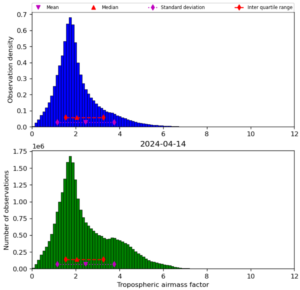
Figure 31: Histogram of “Tropospheric airmass factor” for 2024-04-13 to 2024-04-15
