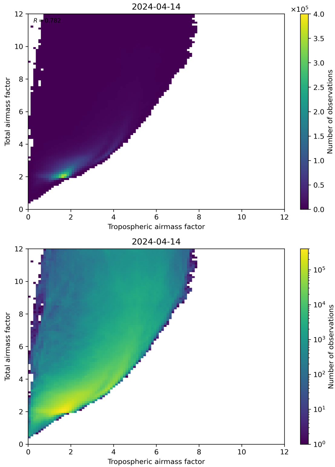
Figure 72: Scatter density plot of “Tropospheric airmass factor” against “Total airmass factor” for 2024-04-13 to 2024-04-15.
