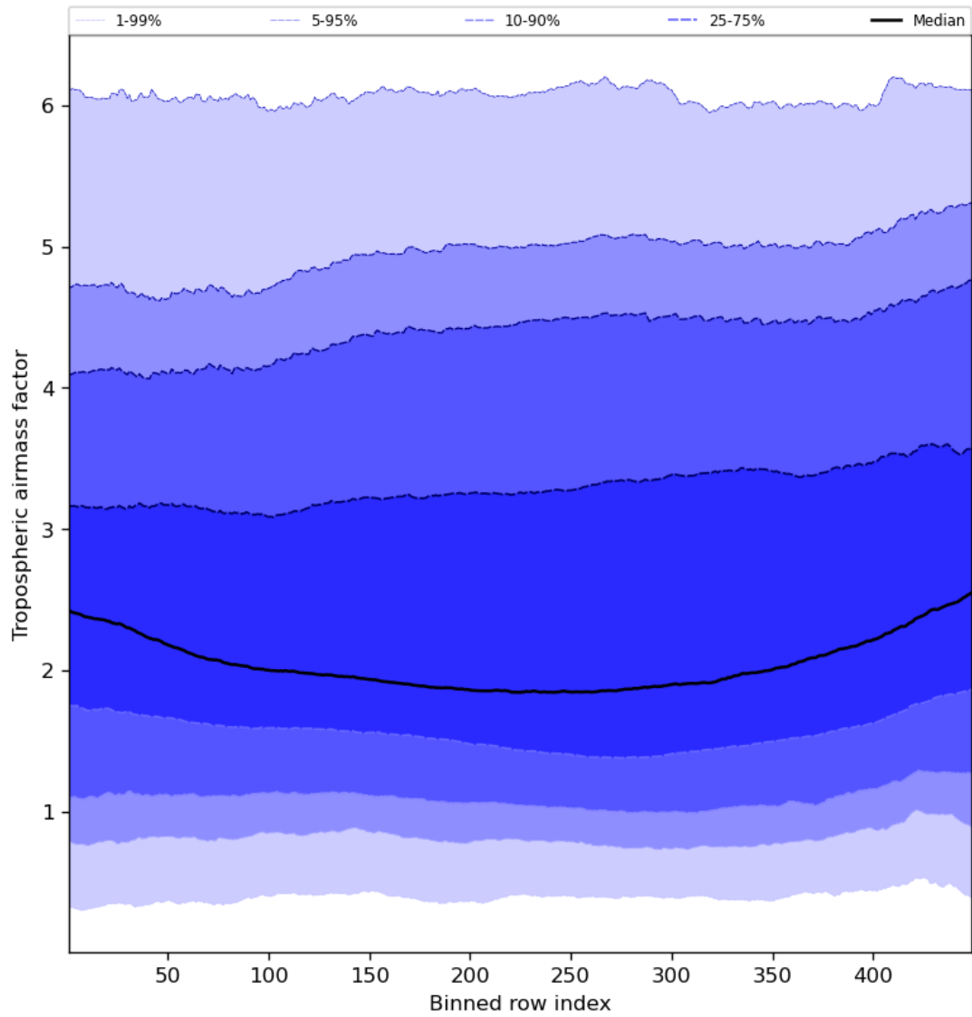
Figure 48: Along track statistics of “Tropospheric airmass factor” for 2024-04-13 to 2024-04-15
