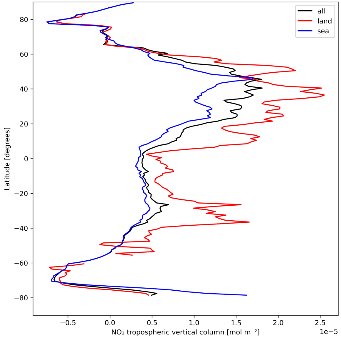
Figure 12: Zonal average of “NO 2 tropospheric vertical column” for 2024-04-13 to 2024-04-15.
