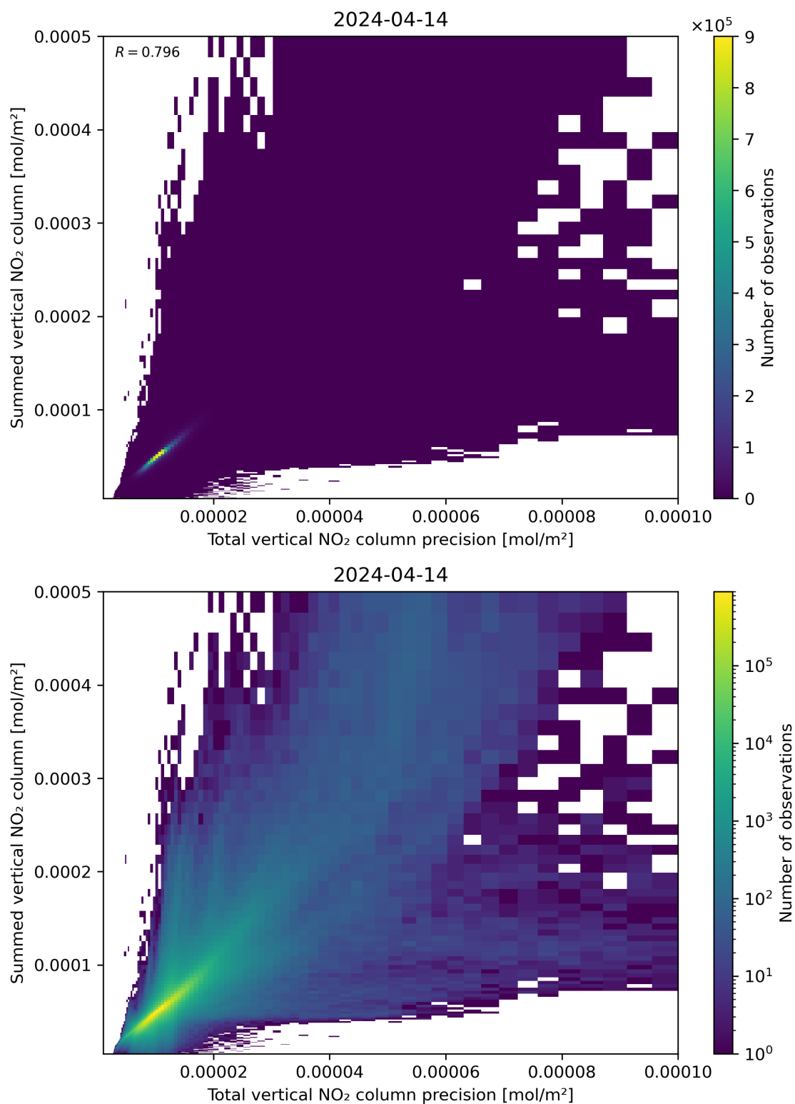
Figure 117: Scatter density plot of “Total vertical NO 2 column precision” against “Summed vertical NO 2 column” for 2024-04-13 to 2024-04-15.
