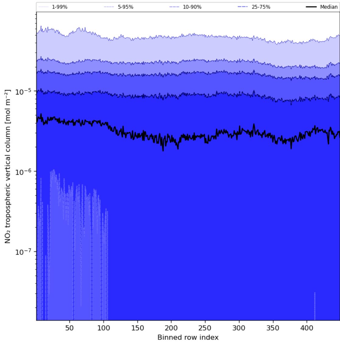
Figure 46: Along track statistics of “NO 2 tropospheric vertical column” for 2024-04-13 to 2024-04-15
