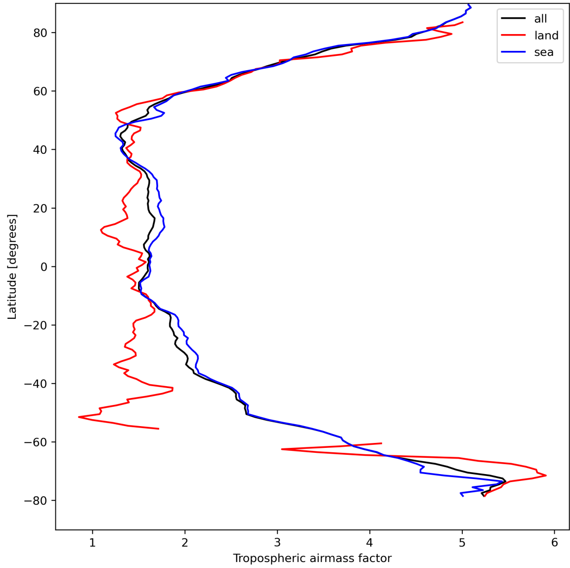
Figure 14: Zonal average of “Tropospheric airmass factor” for 2024-04-13 to 2024-04-15.
