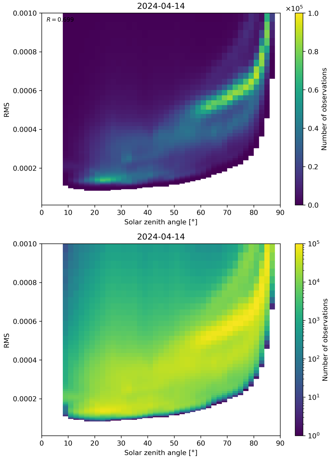
Figure 157: Scatter density plot of “Solar zenith angle” against “RMS” for 2024-04-13 to 2024-04-15.
