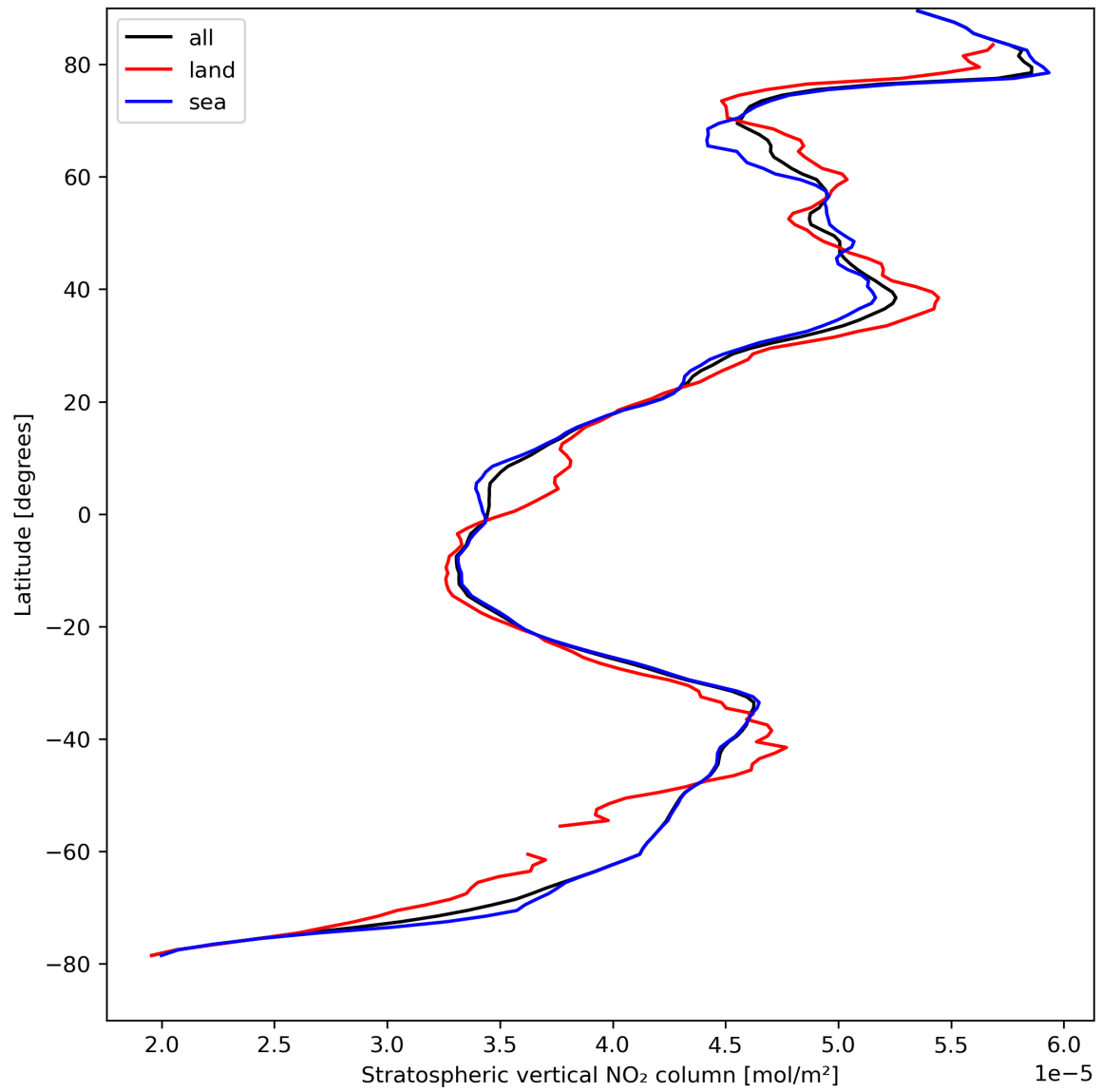
Figure 19: Zonal average of “Stratospheric vertical NO 2 column” for 2024-04-13 to 2024-04-15.
