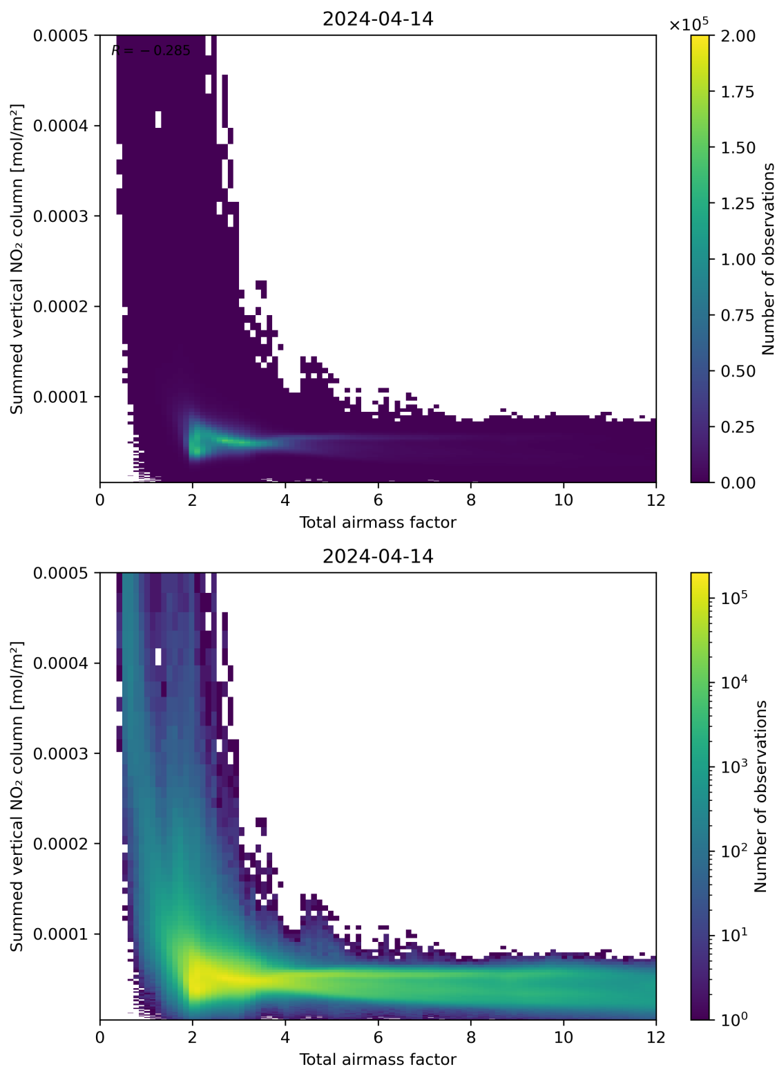
Figure 65: Scatter density plot of “Total airmass factor” against “Summed vertical NO 2 column” for 2024-04-13 to 2024-04-15.
