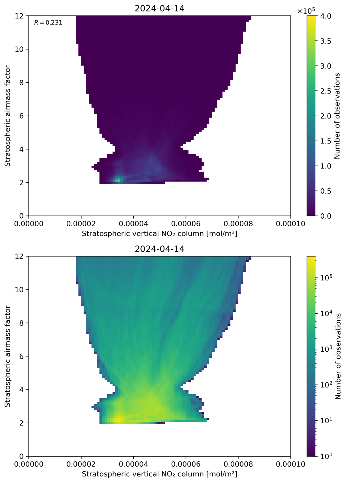
Figure 96: Scatter density plot of “Stratospheric vertical NO 2 column” against “Stratospheric airmass factor” for 2024-04-13 to 2024-04-15.
