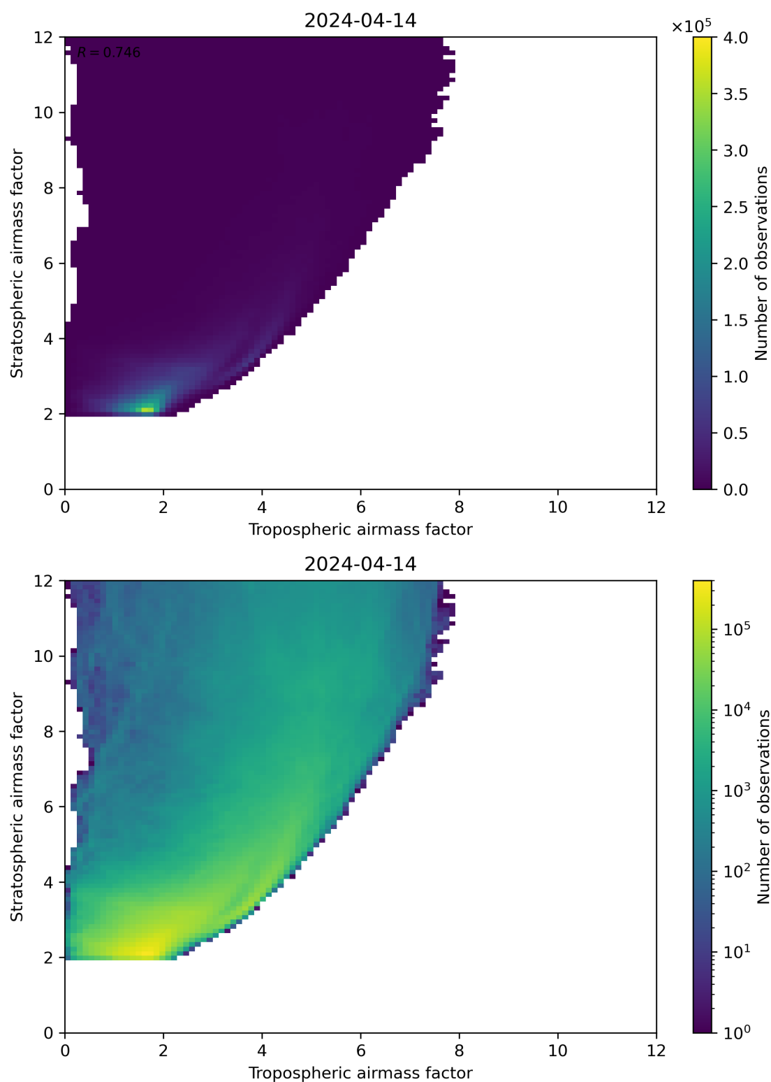
Figure 71: Scatter density plot of “Tropospheric airmass factor” against “Stratospheric airmass factor” for 2024-04-13 to 2024-04-15.
