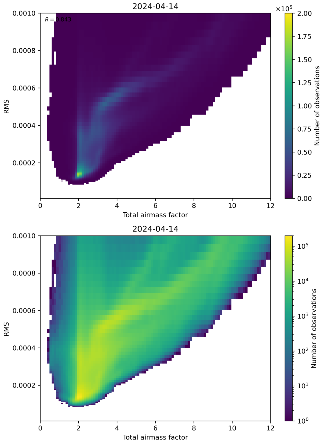
Figure 69: Scatter density plot of “Total airmass factor” against “RMS” for 2024-04-13 to 2024-04-15.
