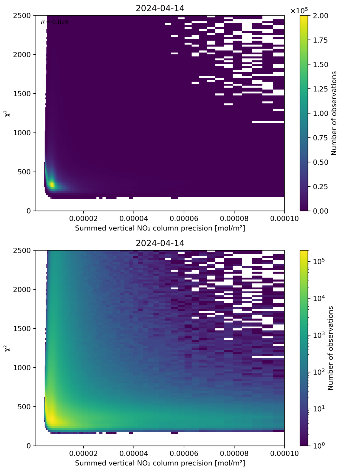
Figure 107: Scatter density plot of “Summed vertical NO 2 column precision” against “ \chi^2 ” for 2024-04-13 to 2024-04-15.
