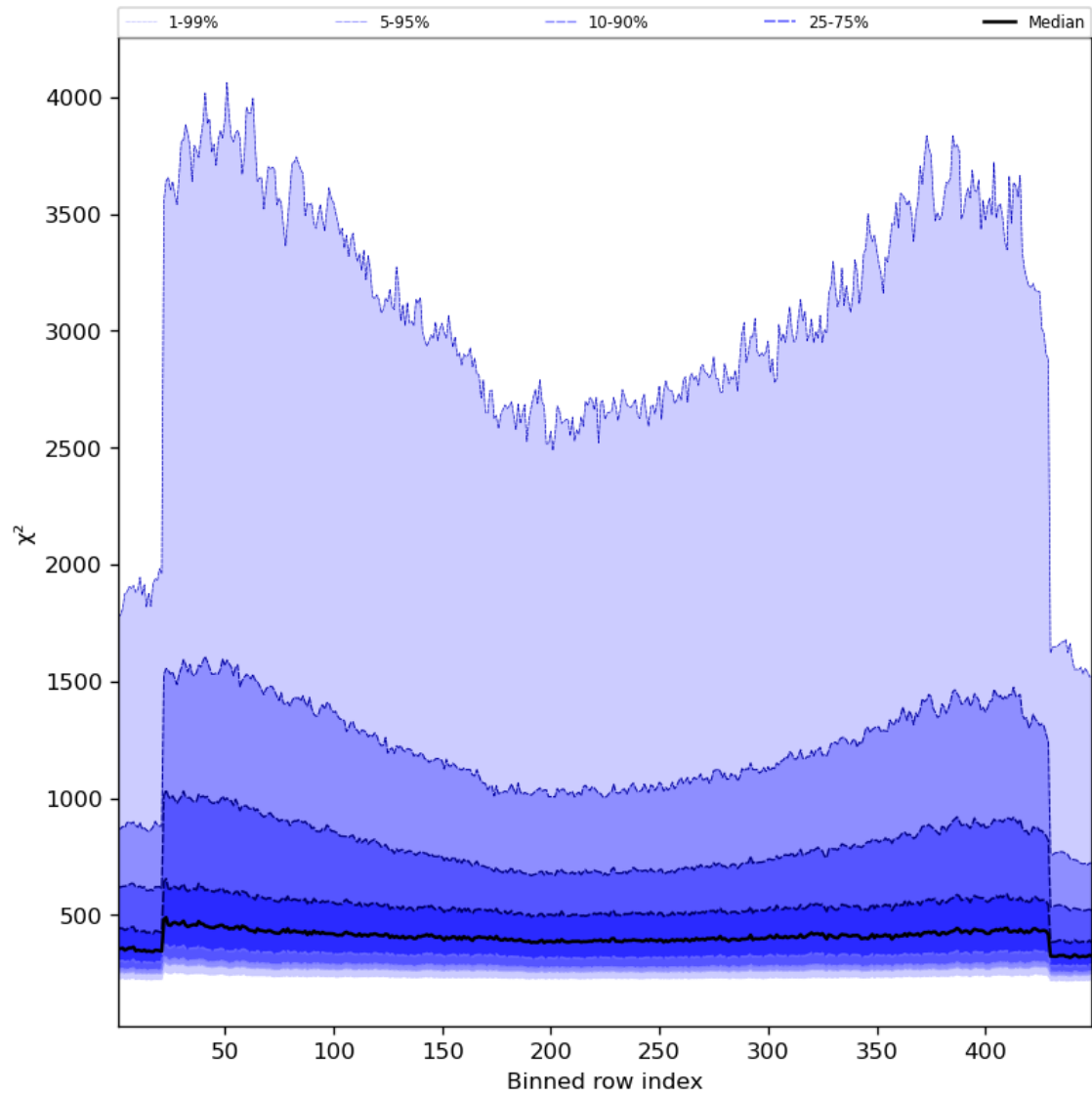
Figure 59: Along track statistics of “ \chi^2 ” for 2024-04-13 to 2024-04-15
