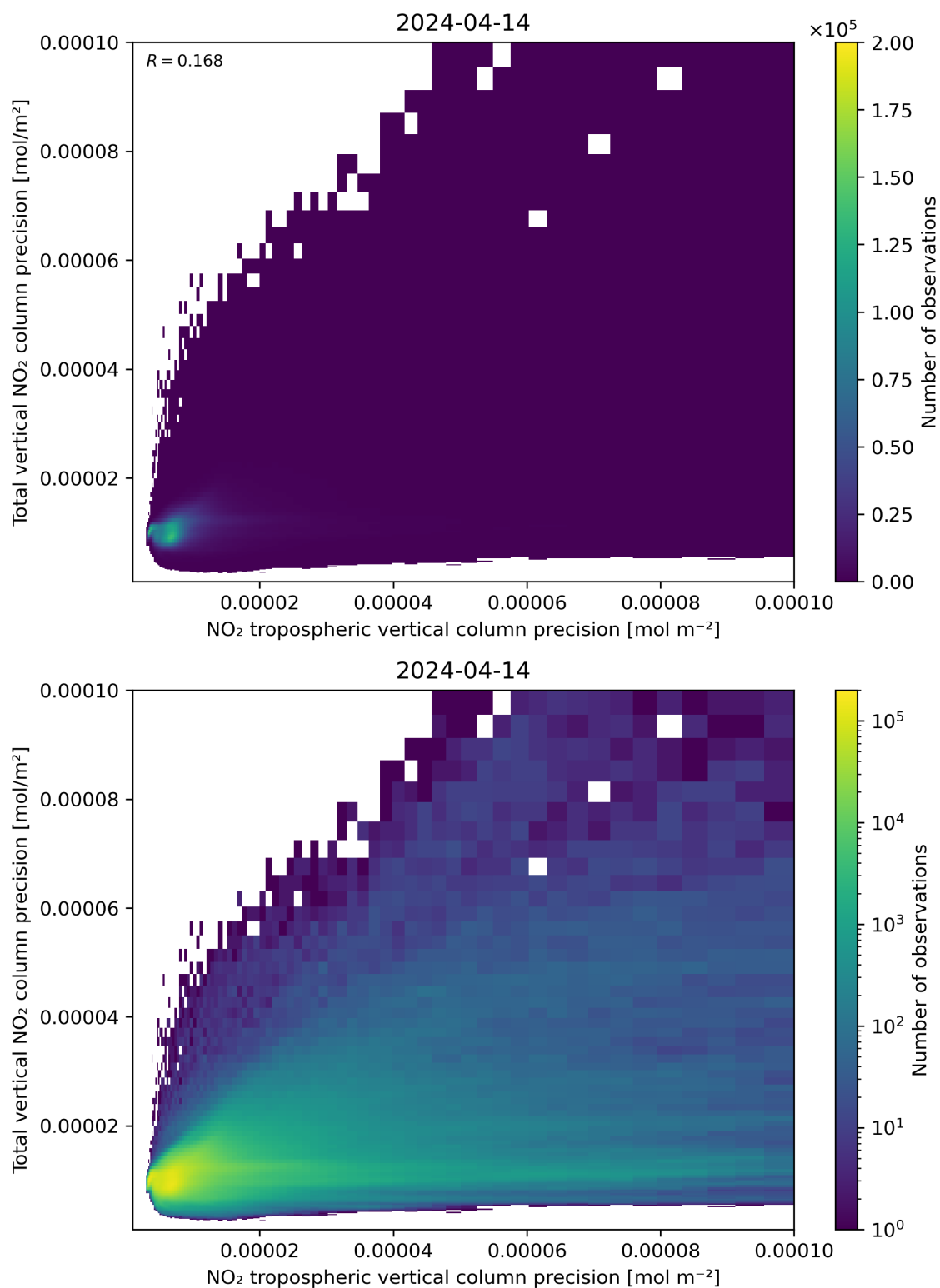
Figure 139: Scatter density plot of “NO 2 tropospheric vertical column precision” against “Total vertical NO 2 column precision” for 2024-04-13 to 2024-04-15.
