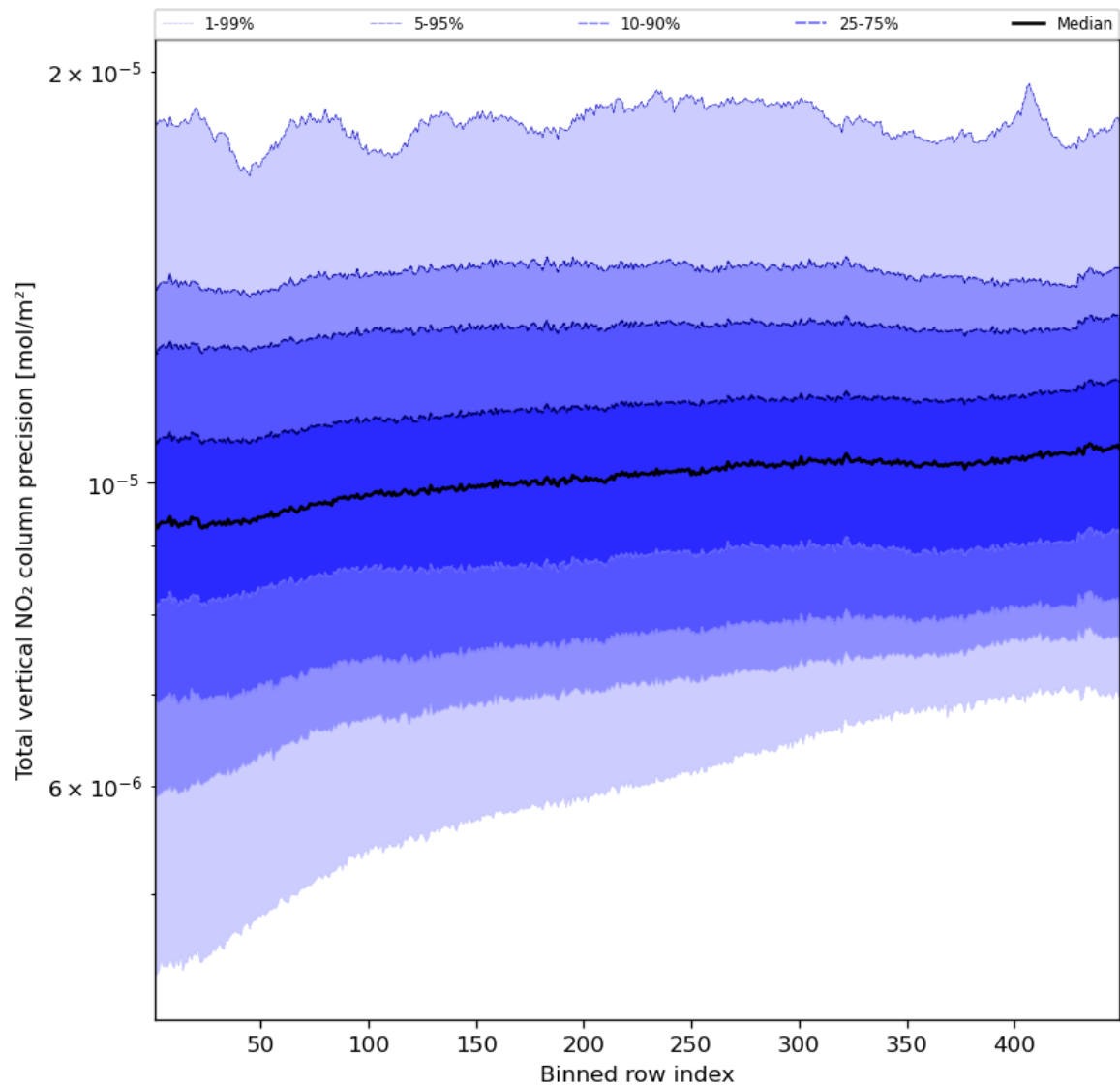
Figure 56: Along track statistics of “Total vertical NO 2 column precision” for 2024-04-13 to 2024-04-15
