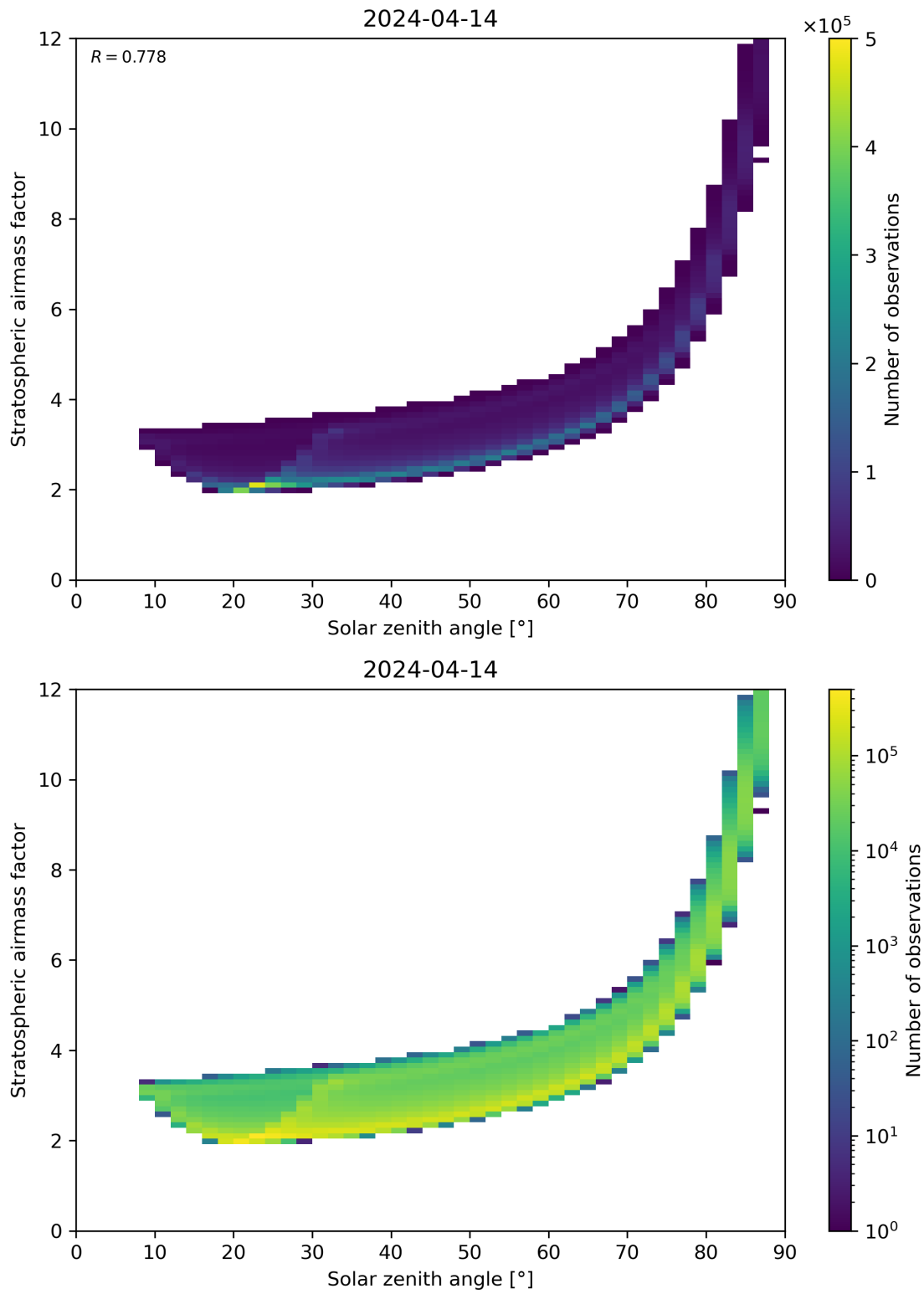
Figure 145: Scatter density plot of “Solar zenith angle” against “Stratospheric airmass factor” for 2024-04-13 to 2024-04-15.
