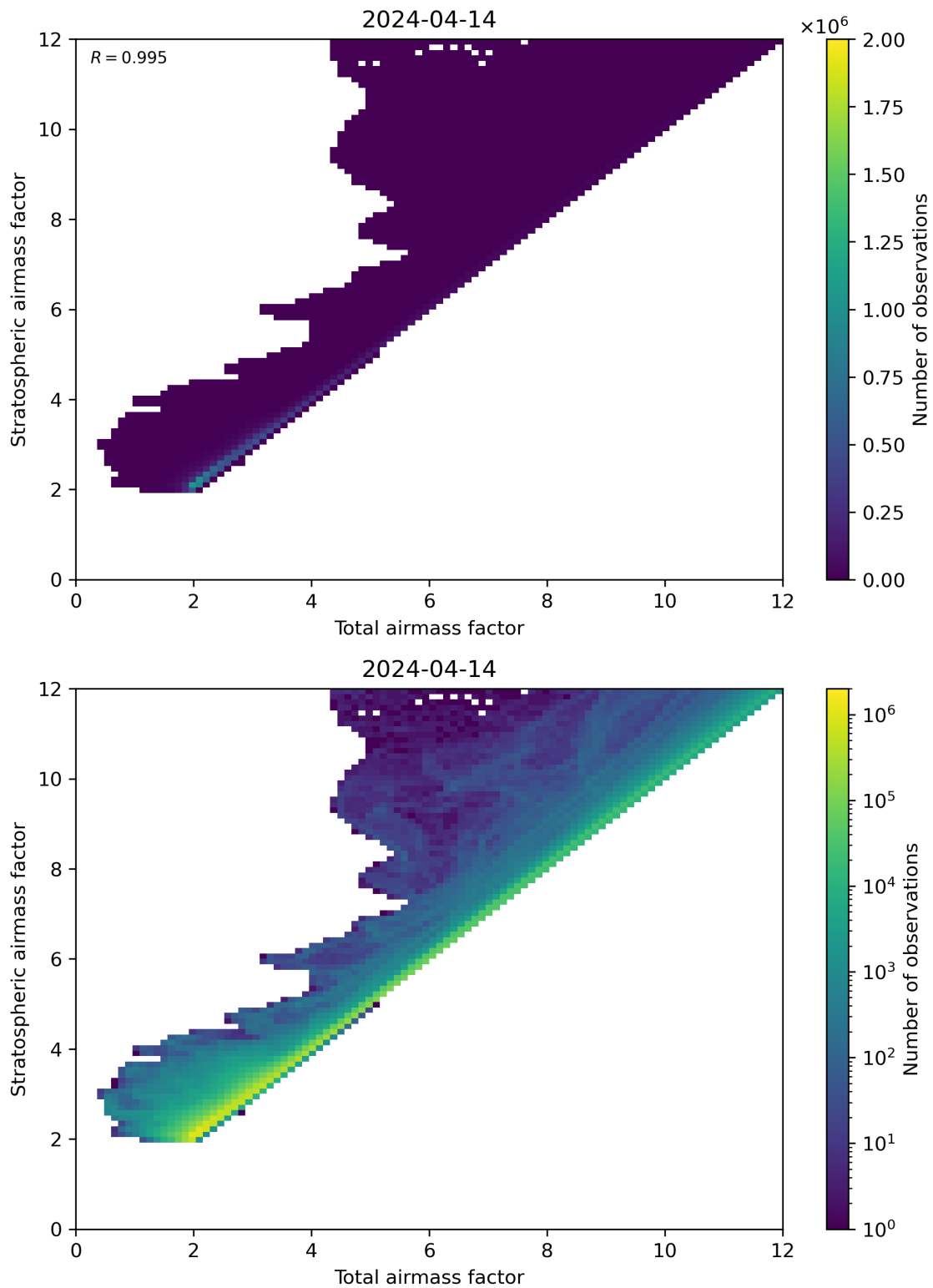
Figure 62: Scatter density plot of “Total airmass factor” against “Stratospheric airmass factor” for 2024-04-13 to 2024-04-15.
