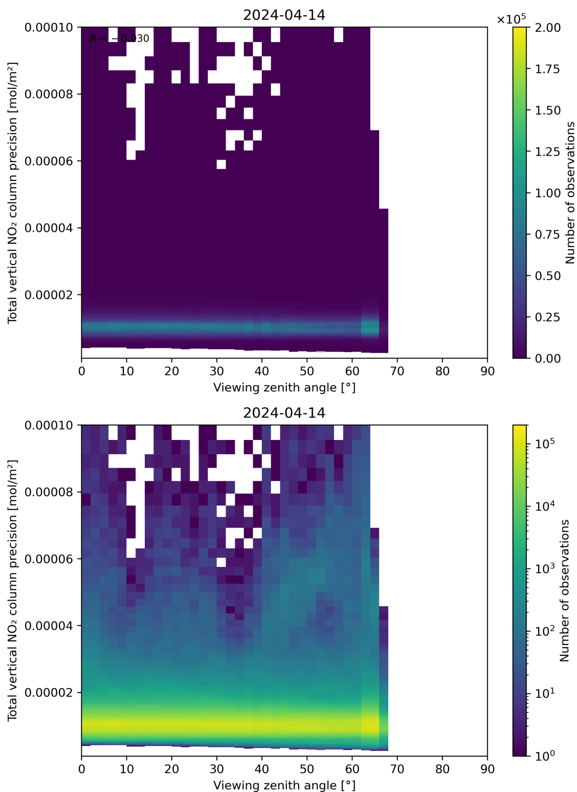
Figure 168: Scatter density plot of “Viewing zenith angle” against “Total vertical NO 2 column precision” for 2024-04-13 to 2024-04-15.
