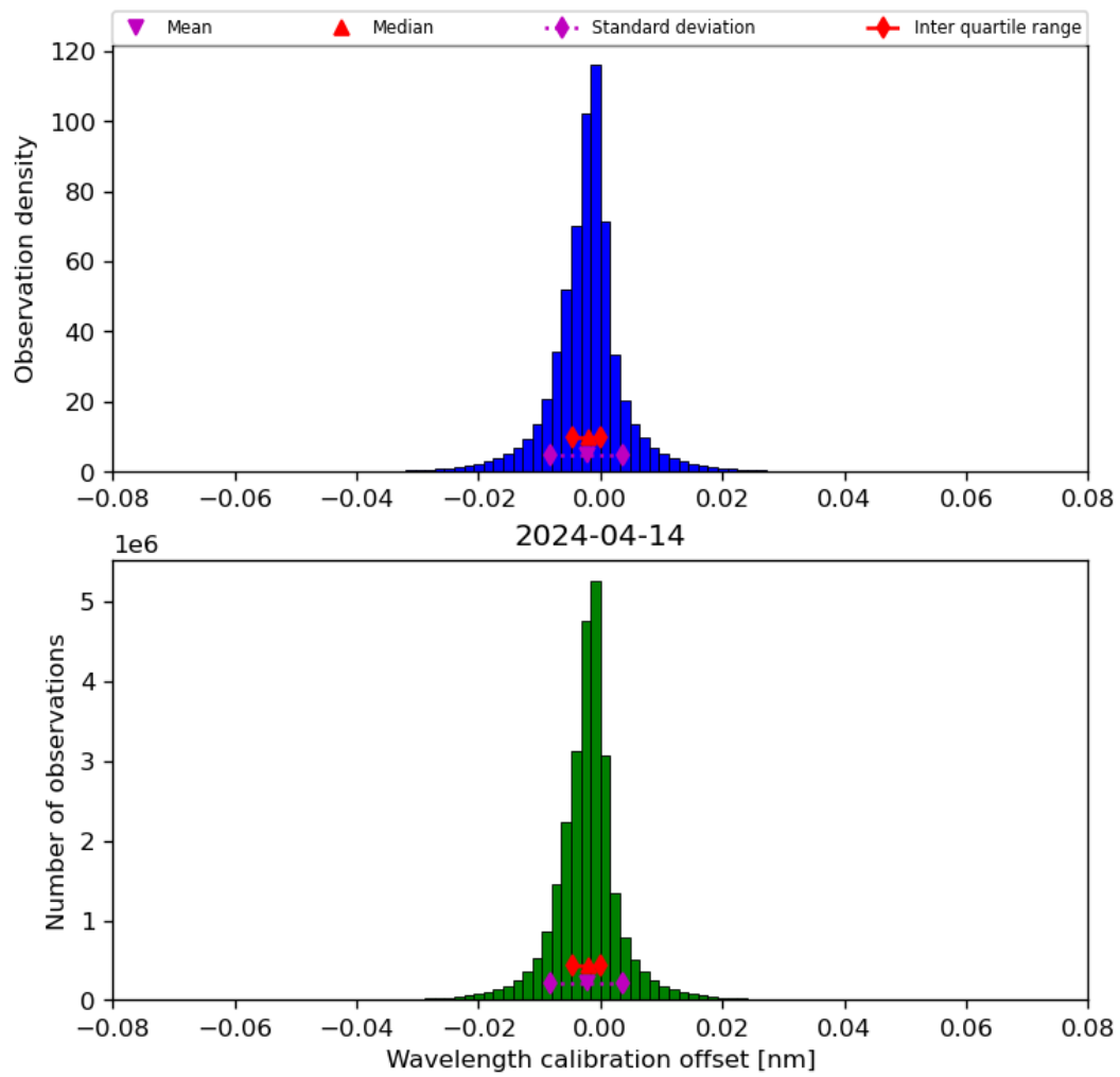
Figure 35: Histogram of “Wavelength calibration offset” for 2024-04-13 to 2024-04-15
