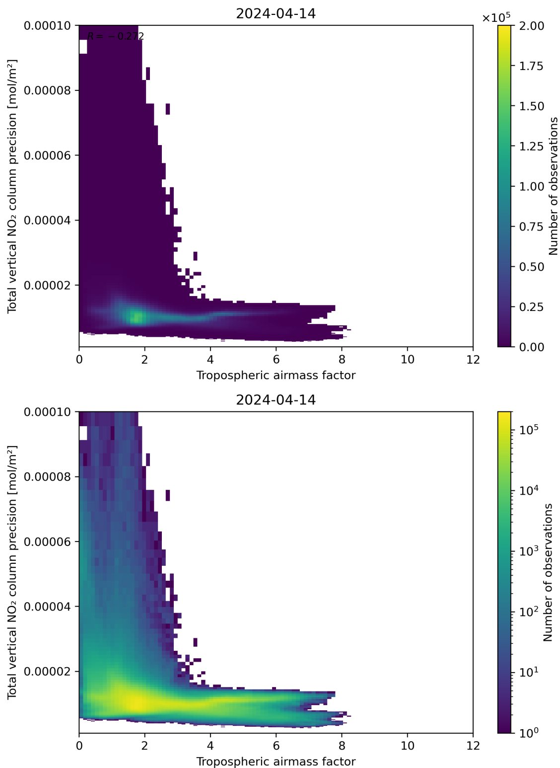
Figure 78: Scatter density plot of “Tropospheric air mass factor” against “Total vertical NO 2 column precision” for 2024-04-13 to 2024-04-15.
