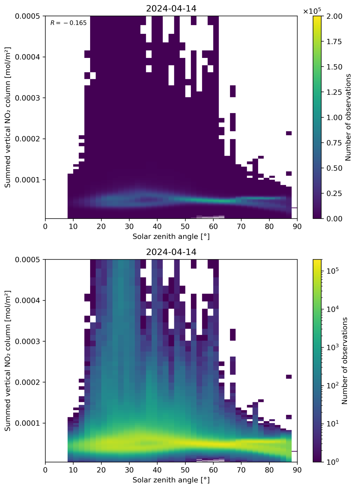
Figure 151: Scatter density plot of “Solar zenith angle” against “Summed vertical NO 2 column” for 2024-04-13 to 2024-04-15.
