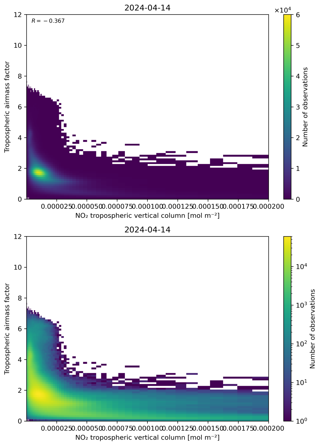
Figure 123: Scatter density plot of “NO 2 tropospheric vertical column” against “Tropospheric air mass factor” for 2024-04-13 to 2024-04-15.
