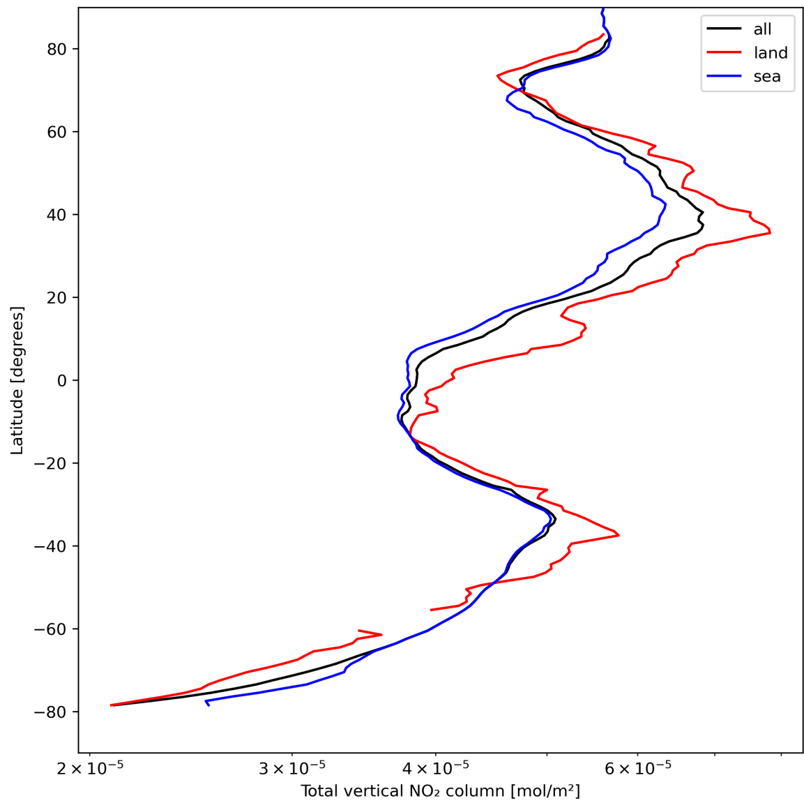
Figure 21: Zonal average of “Total vertical NO 2 column” for 2024-04-13 to 2024-04-15.
