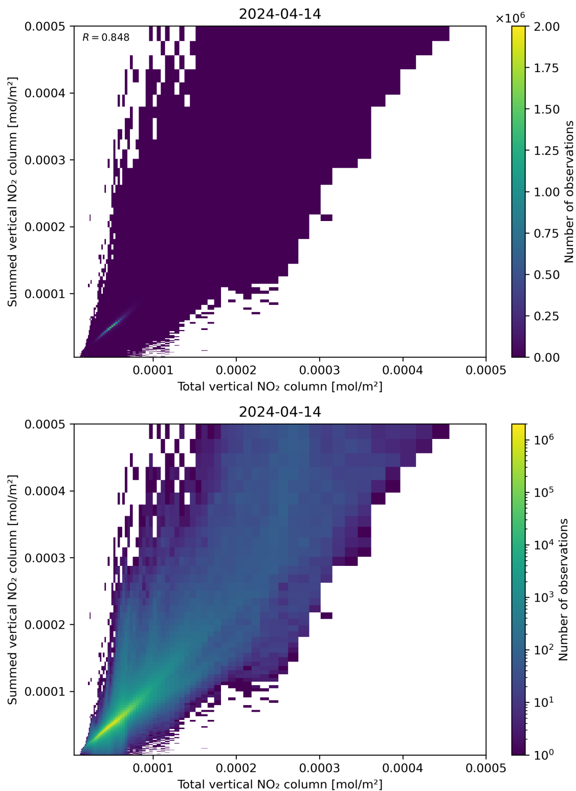
Figure 112: Scatter density plot of “Total vertical NO 2 column” against “Summed vertical NO 2 column” for 2024-04-13 to 2024-04-15.
