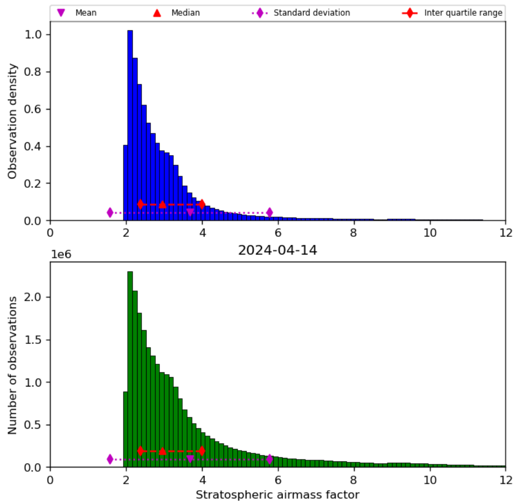
Figure 44: Histogram of “Stratospheric airmass factor” for 2024-04-13 to 2024-04-15
