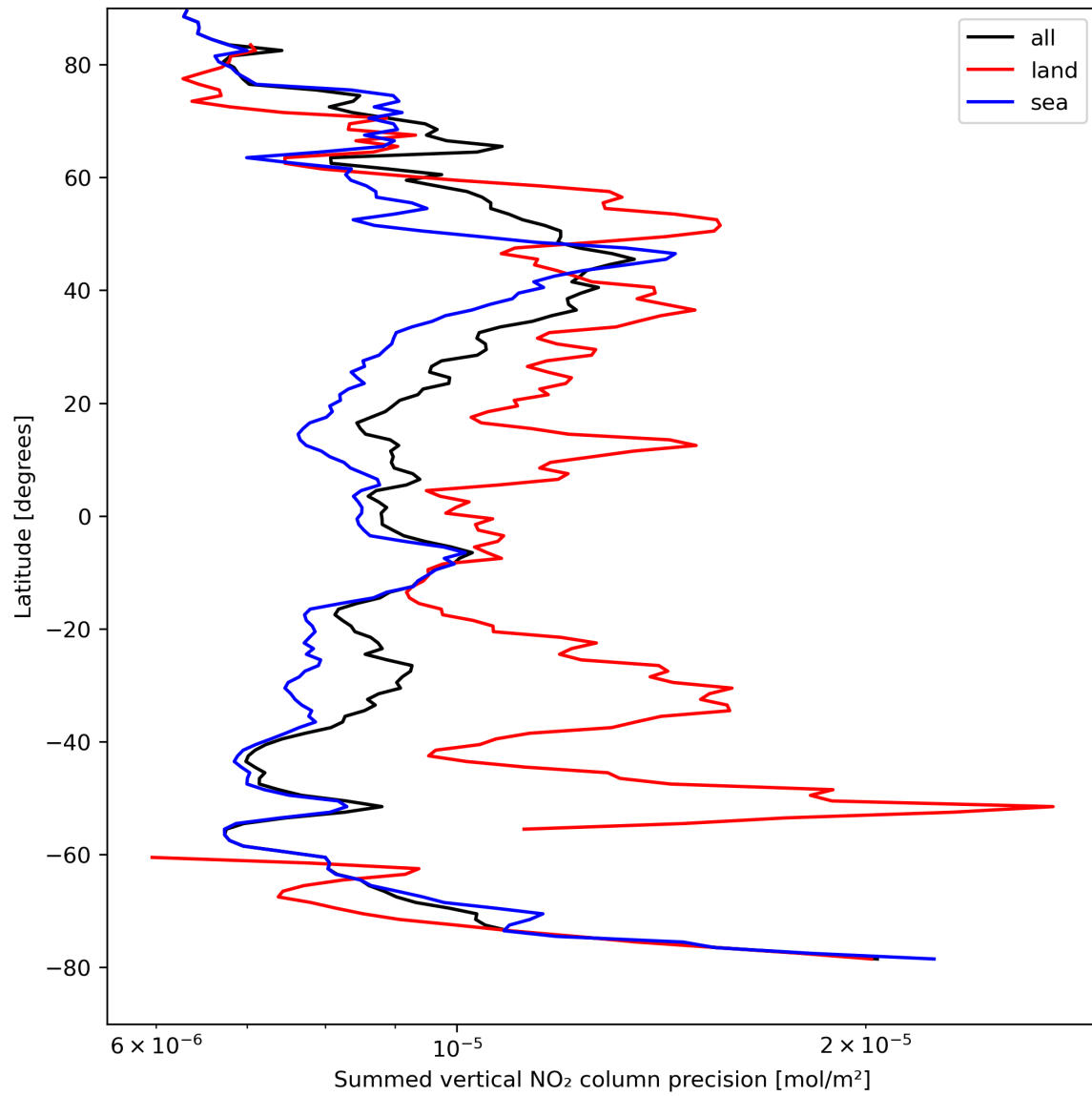
Figure 24: Zonal average of “Summed vertical NO 2 column precision” for 2024-04-13 to 2024-04-15.
