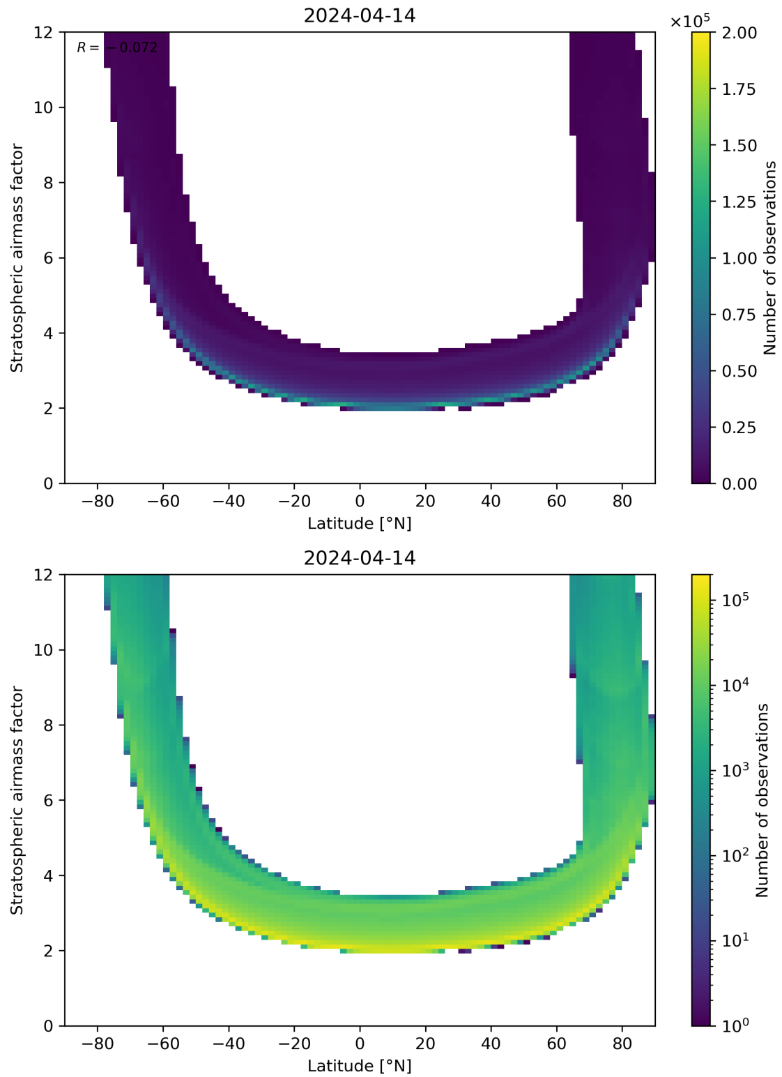
Figure 83: Scatter density plot of “Latitude” against “Stratospheric air mass factor” for 2024-04-13 to 2024-04-15.
