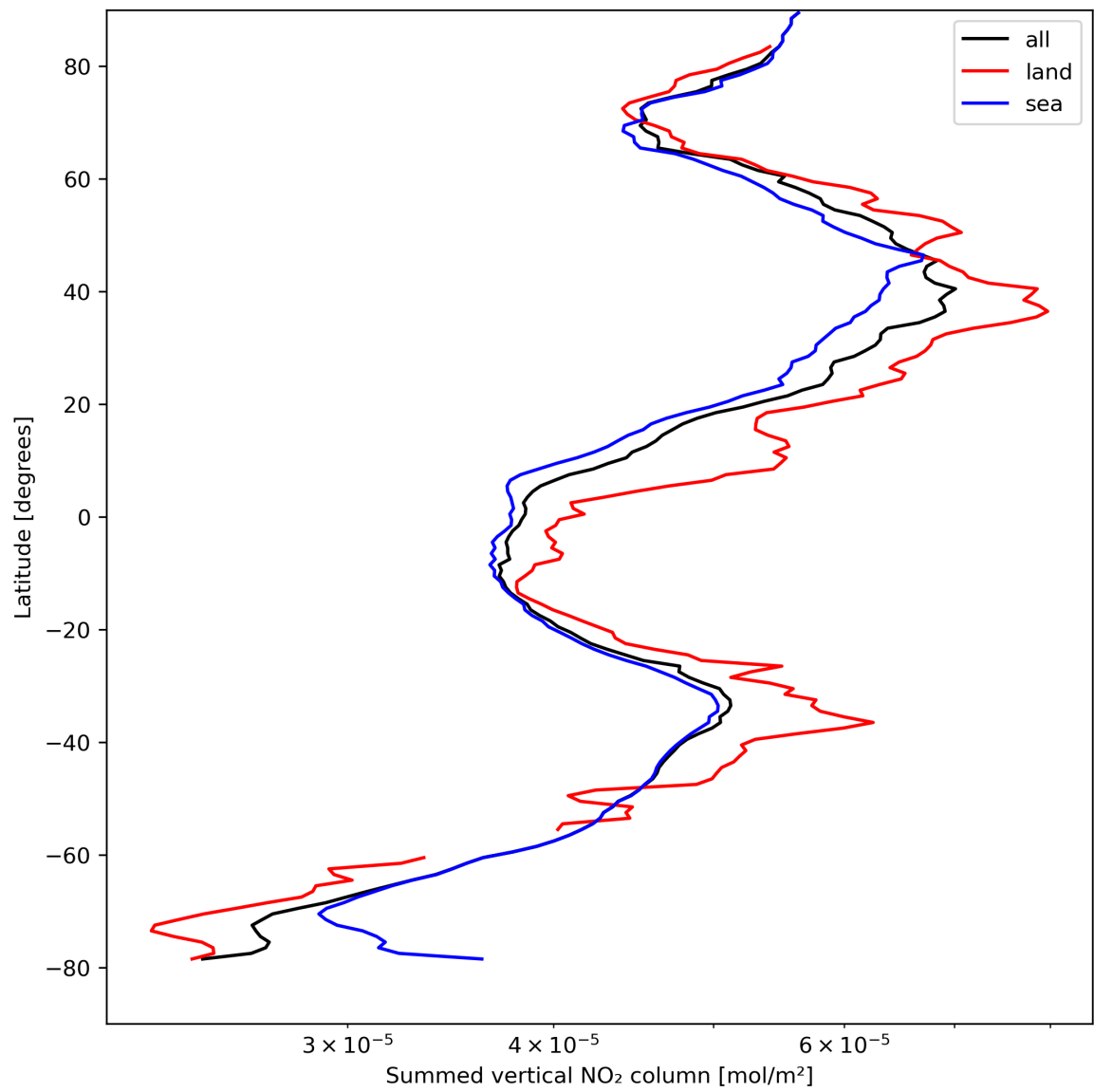
Figure 23: Zonal average of “Summed vertical NO 2 column” for 2024-04-13 to 2024-04-15.
