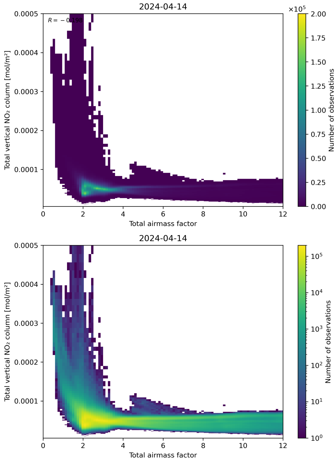
Figure 67: Scatter density plot of “Total airmass factor” against “Total vertical NO 2 column” for 2024-04-13 to 2024-04-15.
