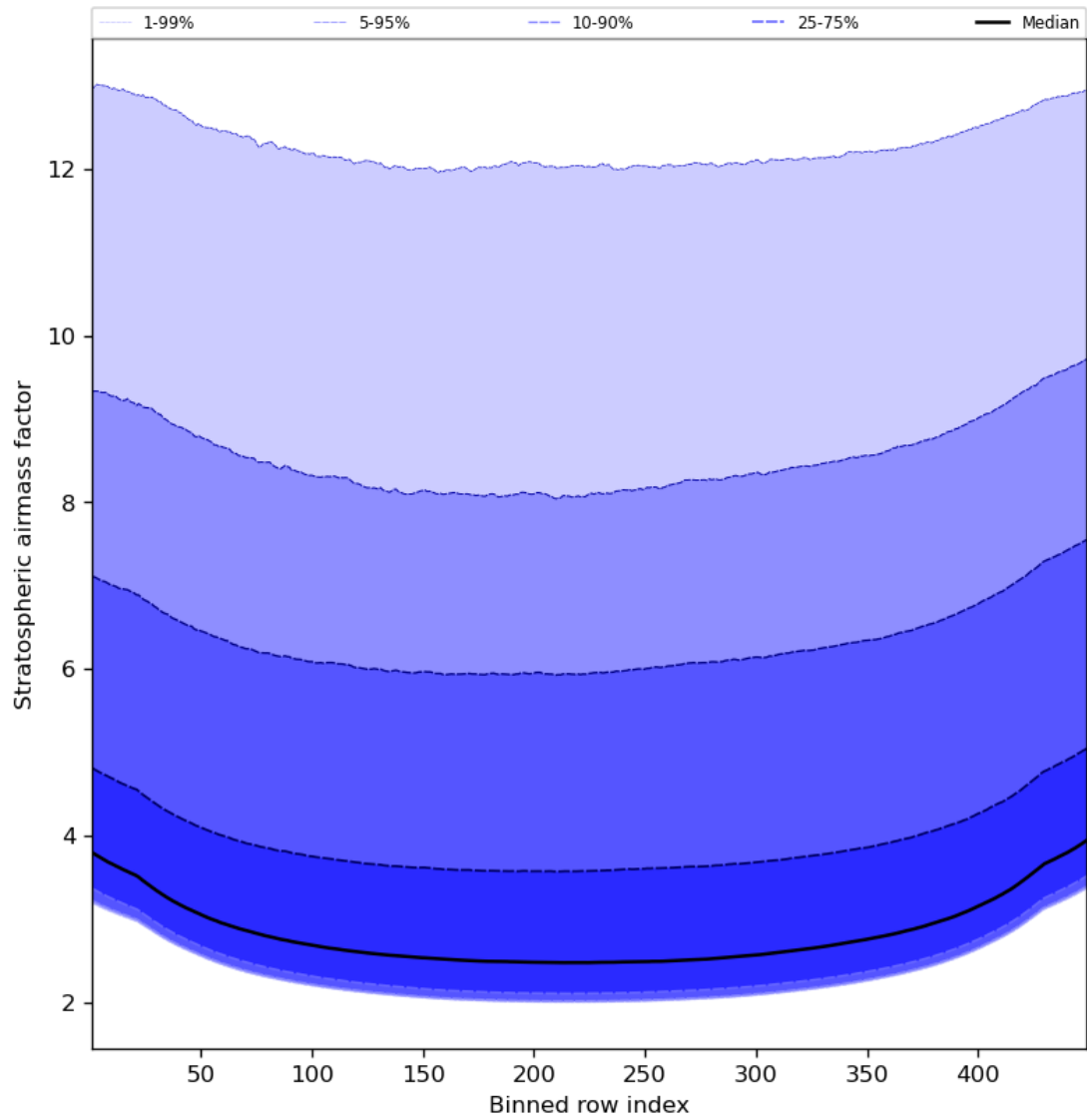
Figure 61: Along track statistics of “Stratospheric airmass factor” for 2024-04-13 to 2024-04-15
