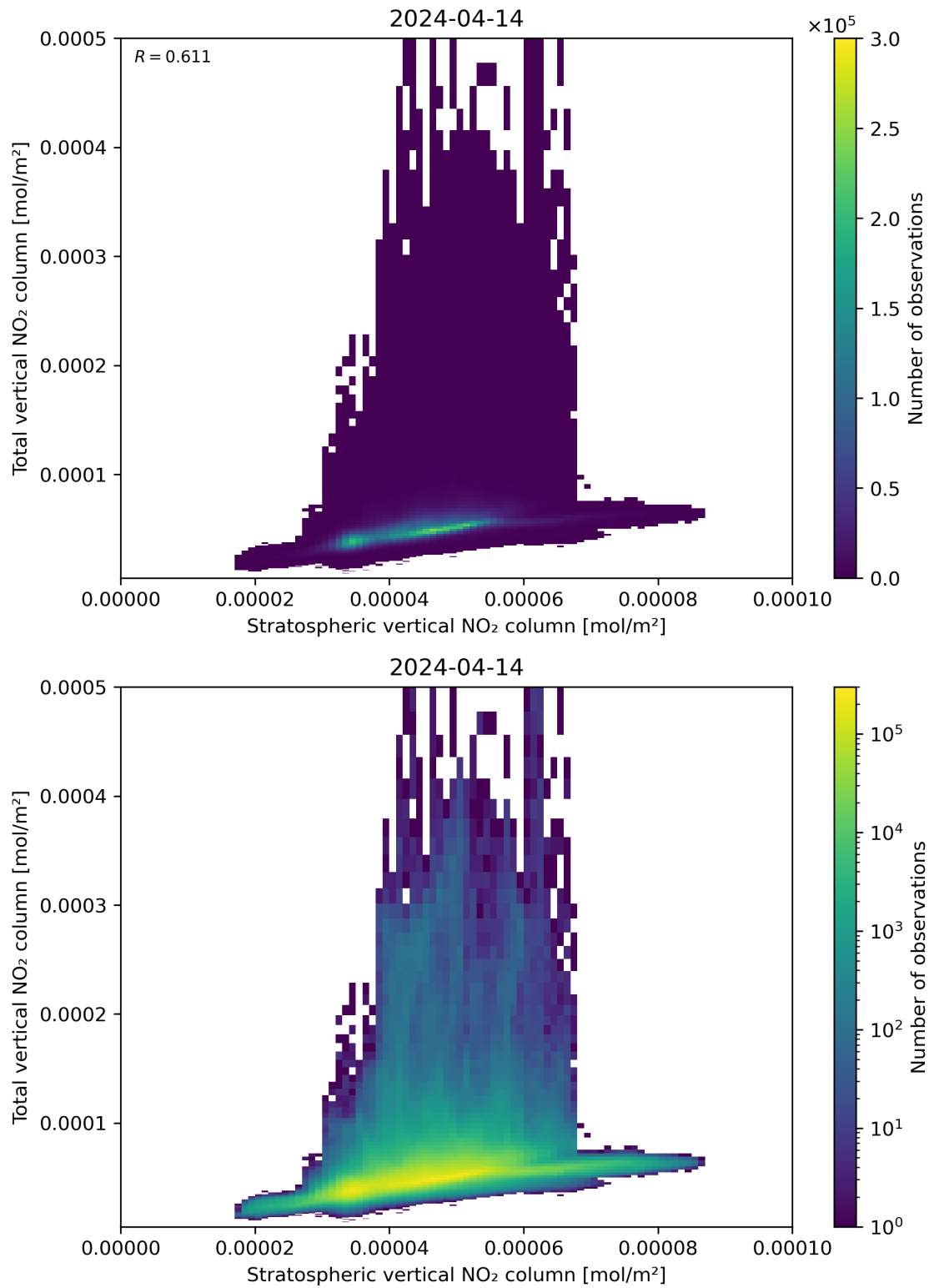
Figure 100: Scatter density plot of “Stratospheric vertical NO 2 column” against “Total vertical NO 2 column” for 2024-04-13 to 2024-04-15.
