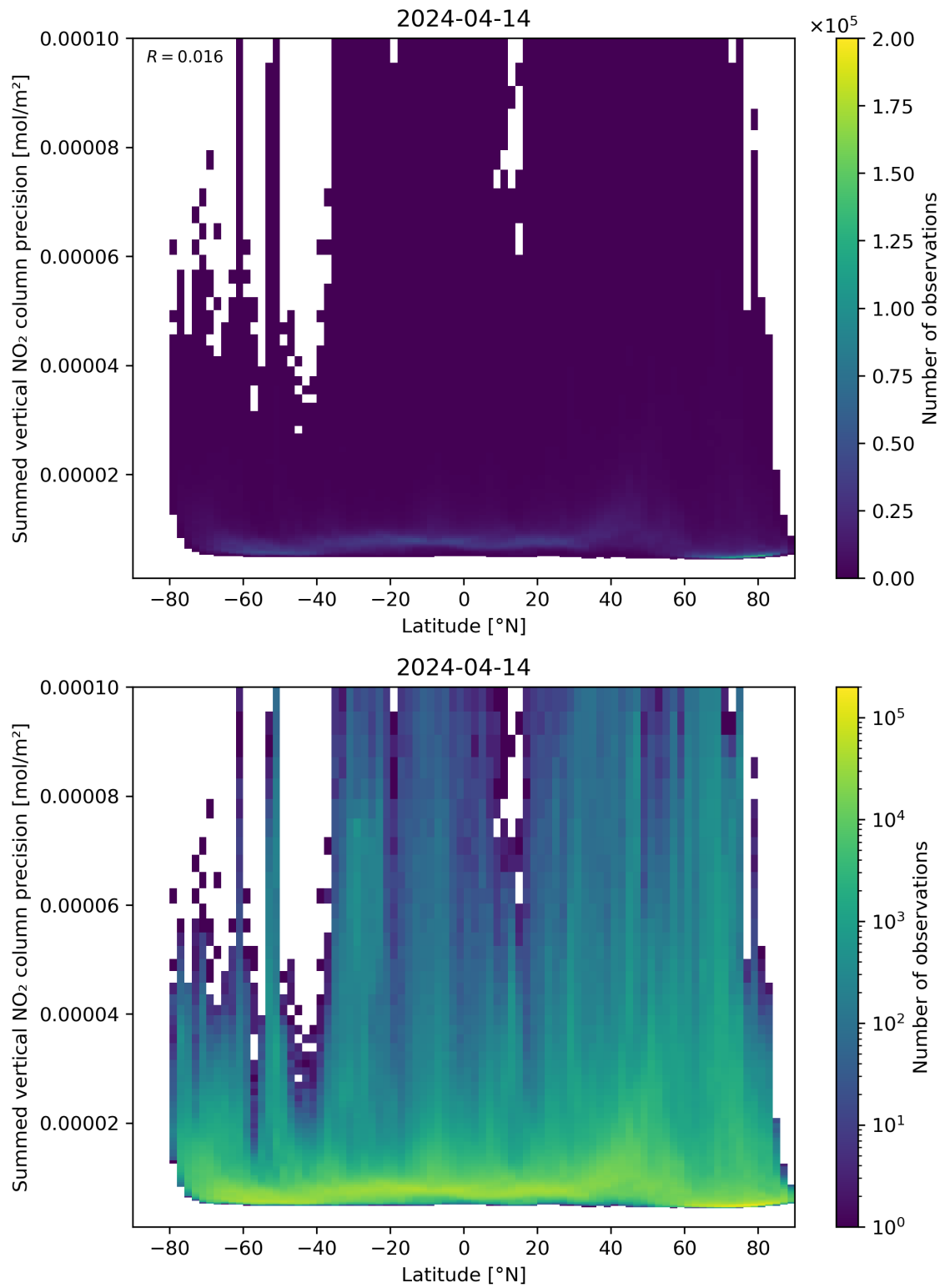
Figure 89: Scatter density plot of “Latitude” against “Summed vertical NO 2 column precision” for 2024-04-13 to 2024-04-15.
