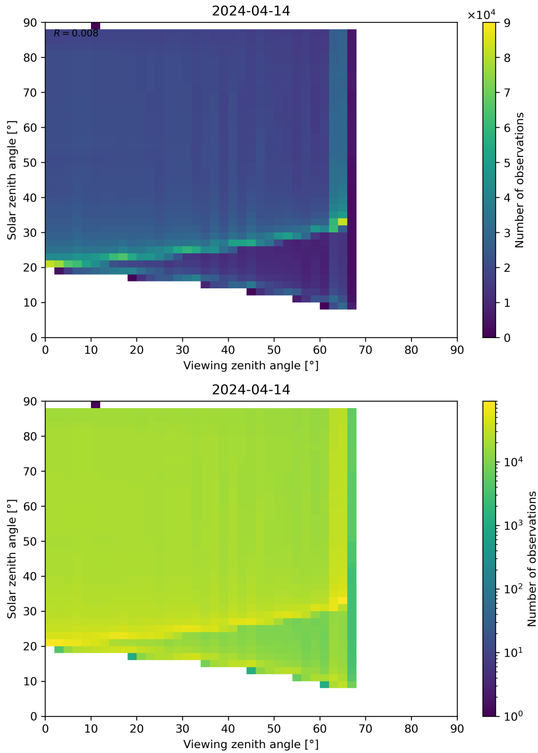
Figure 172: Scatter density plot of “Viewing zenith angle” against “Solar zenith angle” for 2024-04-13 to 2024-04-15.
