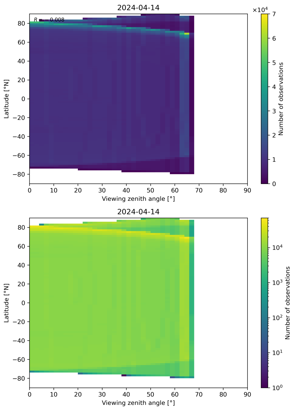
Figure 163: Scatter density plot of “Viewing zenith angle” against “Latitude” for 2024-04-13 to 2024-04-15.
