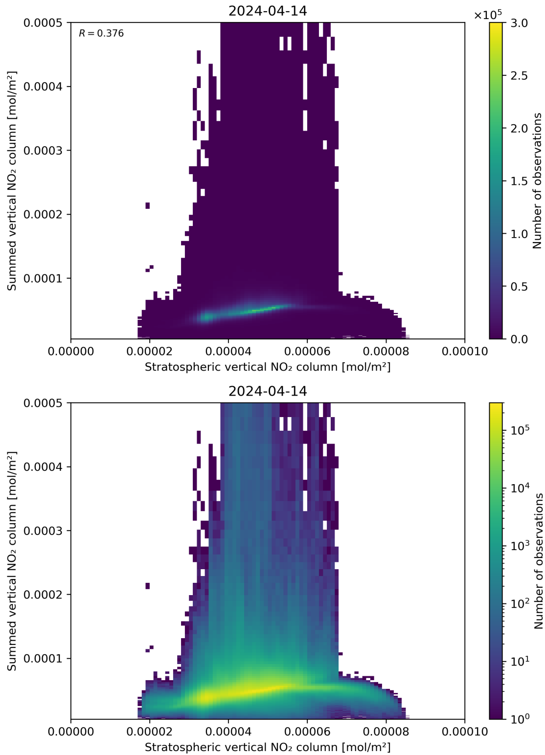
Figure 98: Scatter density plot of “Stratospheric vertical NO 2 column” against “Summed vertical NO 2 column” for 2024-04-13 to 2024-04-15.
