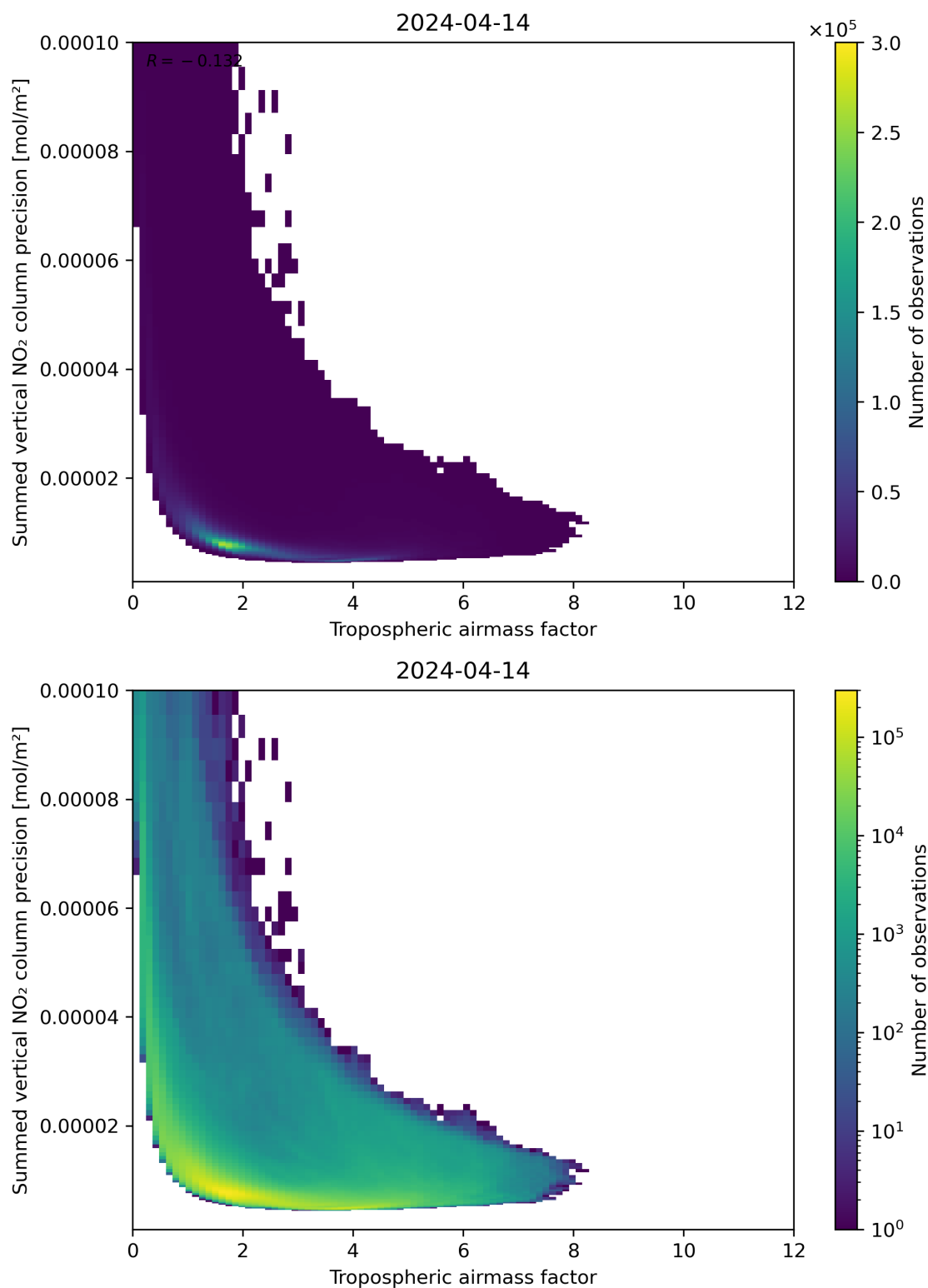
Figure 76: Scatter density plot of “Tropospheric air mass factor” against “Summed vertical NO 2 column precision” for 2024-04-13 to 2024-04-15.
