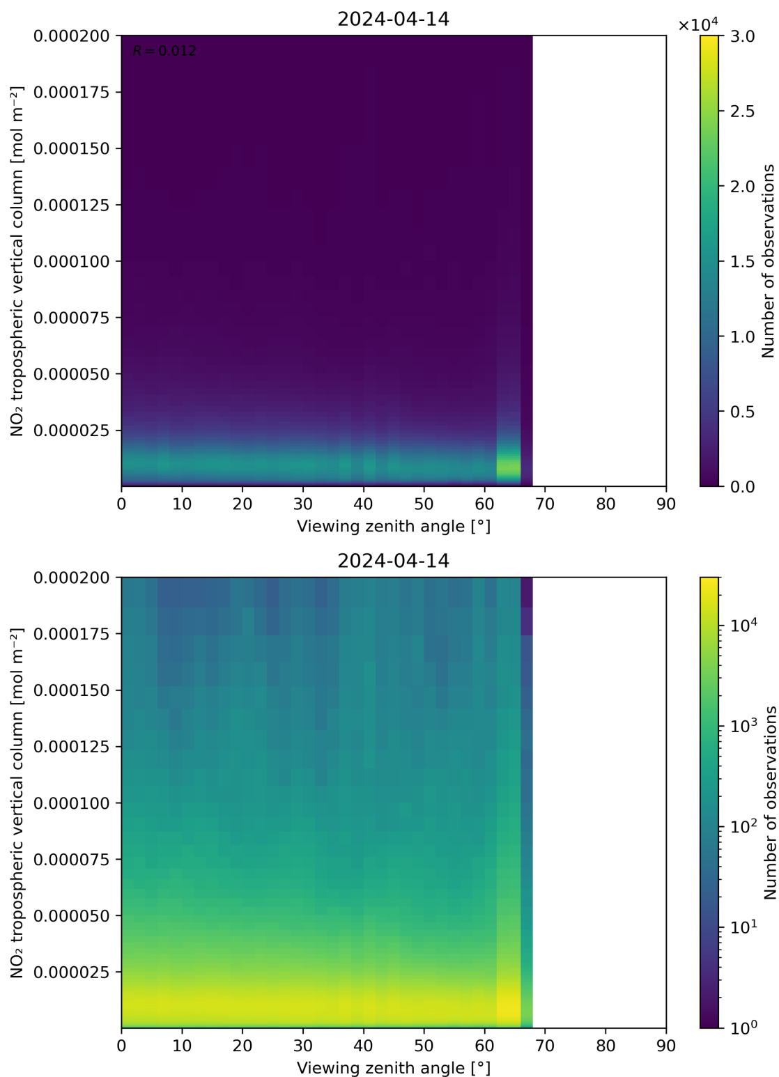
Figure 169: Scatter density plot of “Viewing zenith angle” against “NO 2 tropospheric vertical column” for 2024-04-13 to 2024-04-15.
