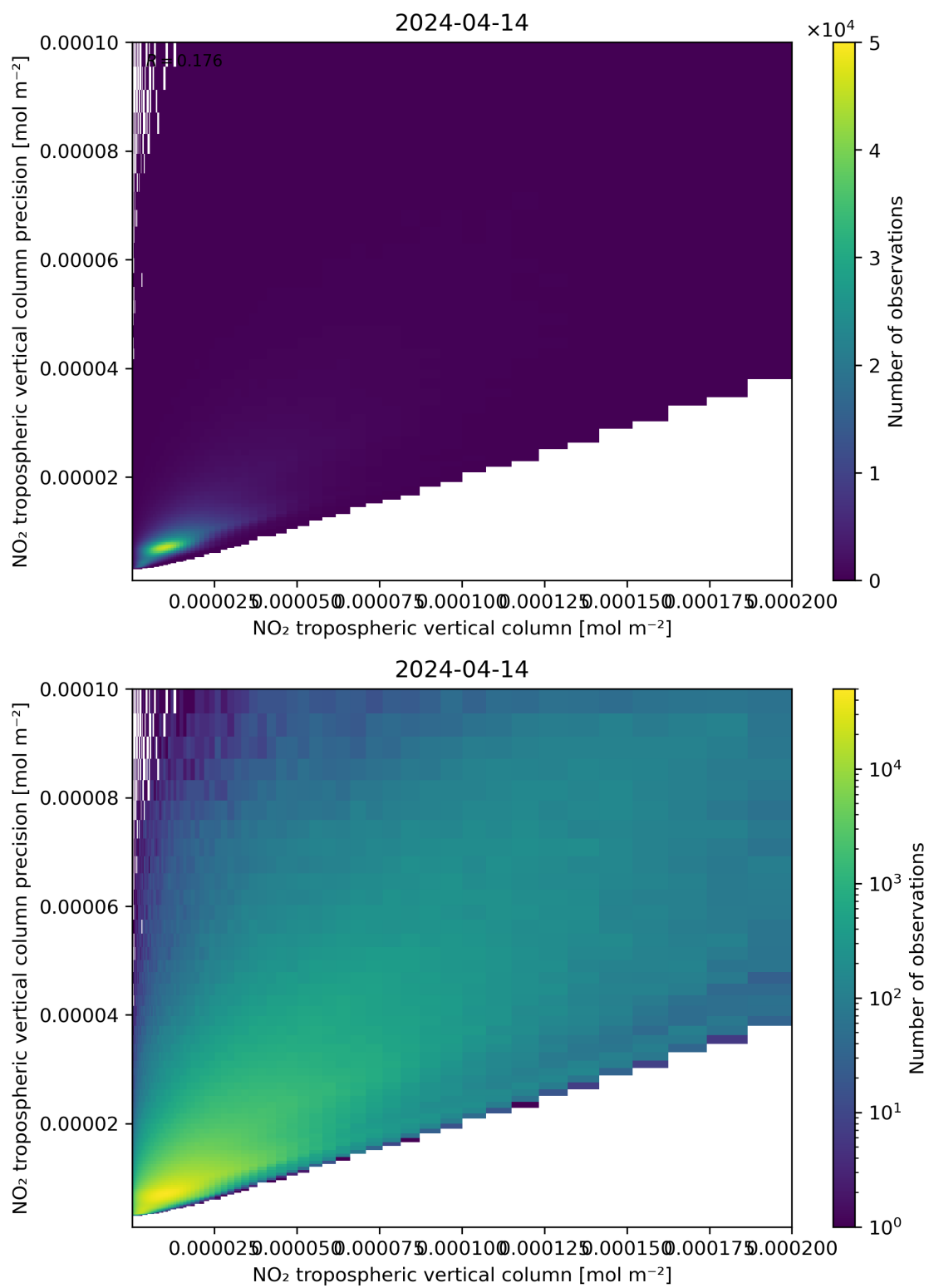
Figure 130: Scatter density plot of “NO 2 tropospheric vertical column” against “NO 2 tropospheric vertical column precision” for 2024-04-13 to 2024-04-15.
