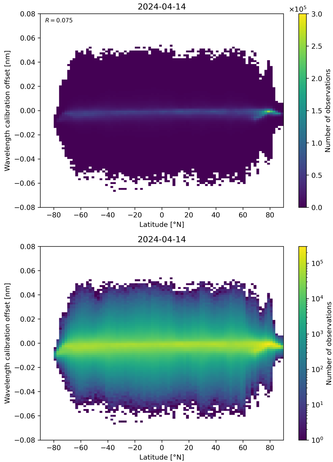
Figure 95: Scatter density plot of “Latitude” against “Wavelength calibration offset” for 2024-04-13 to 2024-04-15.
