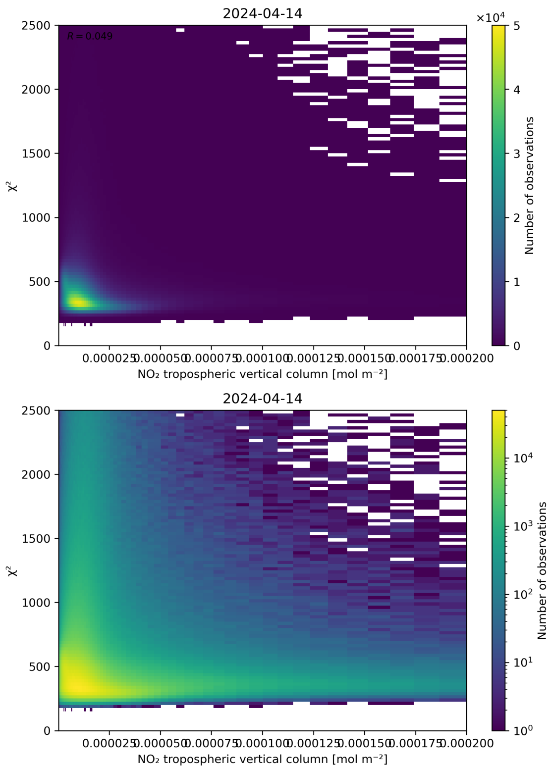
Figure 124: Scatter density plot of “NO 2 tropospheric vertical column” against “ \chi^2 ” for 2024-04-13 to 2024-04-15.
