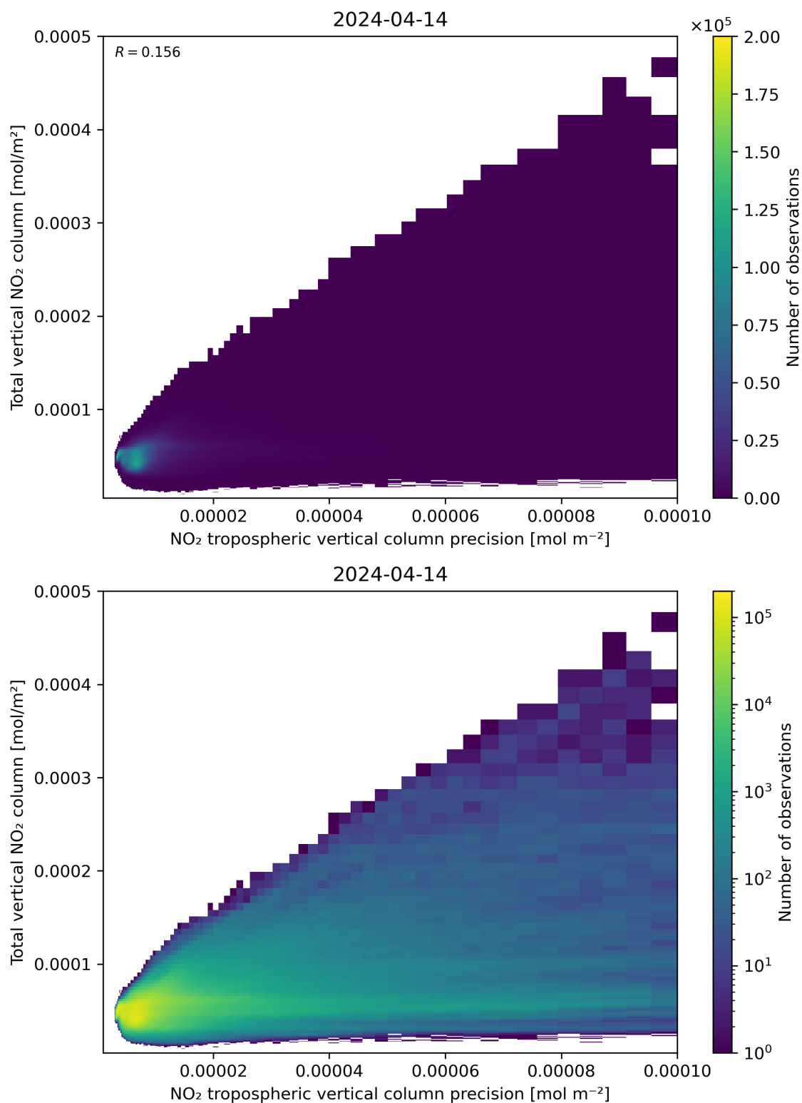
Figure 138: Scatter density plot of “NO 2 tropospheric vertical column precision” against “Total vertical NO 2 column” for 2024-04-13 to 2024-04-15.
