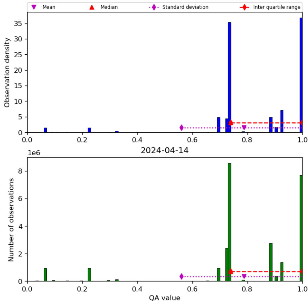
Figure 28: Histogram of “QA value” for 2024-04-13 to 2024-04-15
