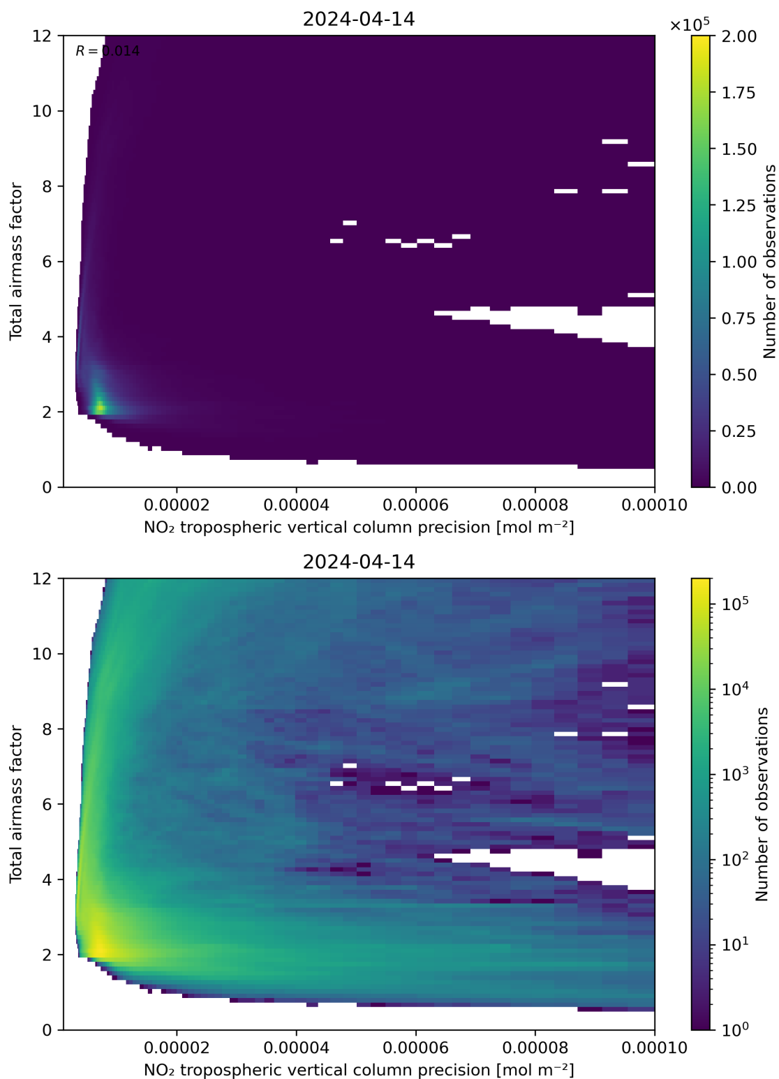
Figure 132: Scatter density plot of “NO 2 tropospheric vertical column precision” against “Total air mass factor” for 2024-04-13 to 2024-04-15.
