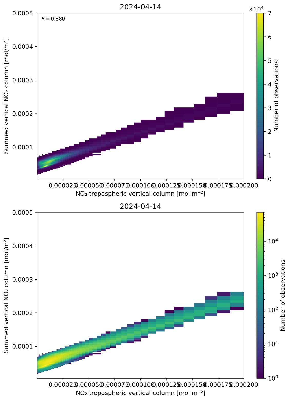
Figure 126: Scatter density plot of “NO 2 tropospheric vertical column” against “Summed vertical NO 2 column” for 2024-04-13 to 2024-04-15.
