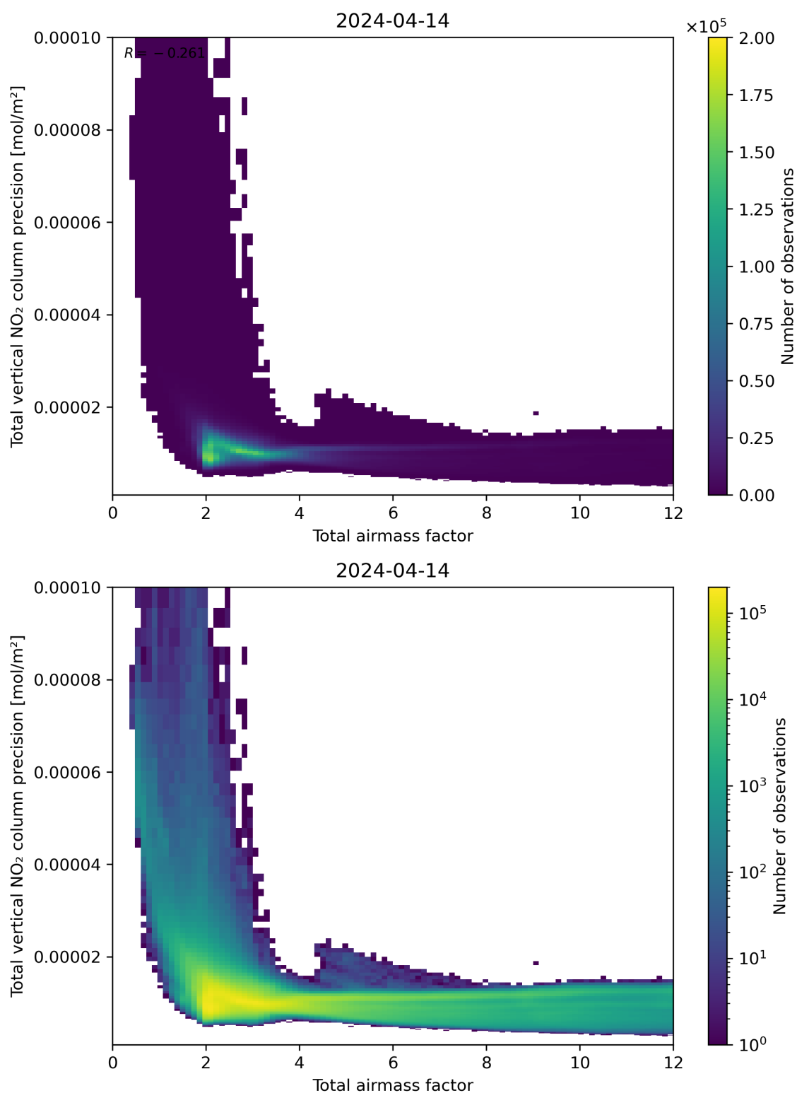
Figure 68: Scatter density plot of “Total airmass factor” against “Total vertical NO 2 column precision” for 2024-04-13 to 2024-04-15.
