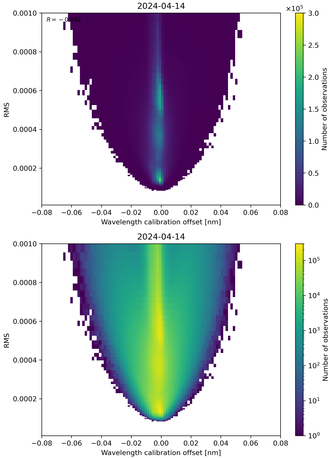
Figure 181: Scatter density plot of “Wavelength calibration offset” against “RMS” for 2024-04-13 to 2024-04-15.
