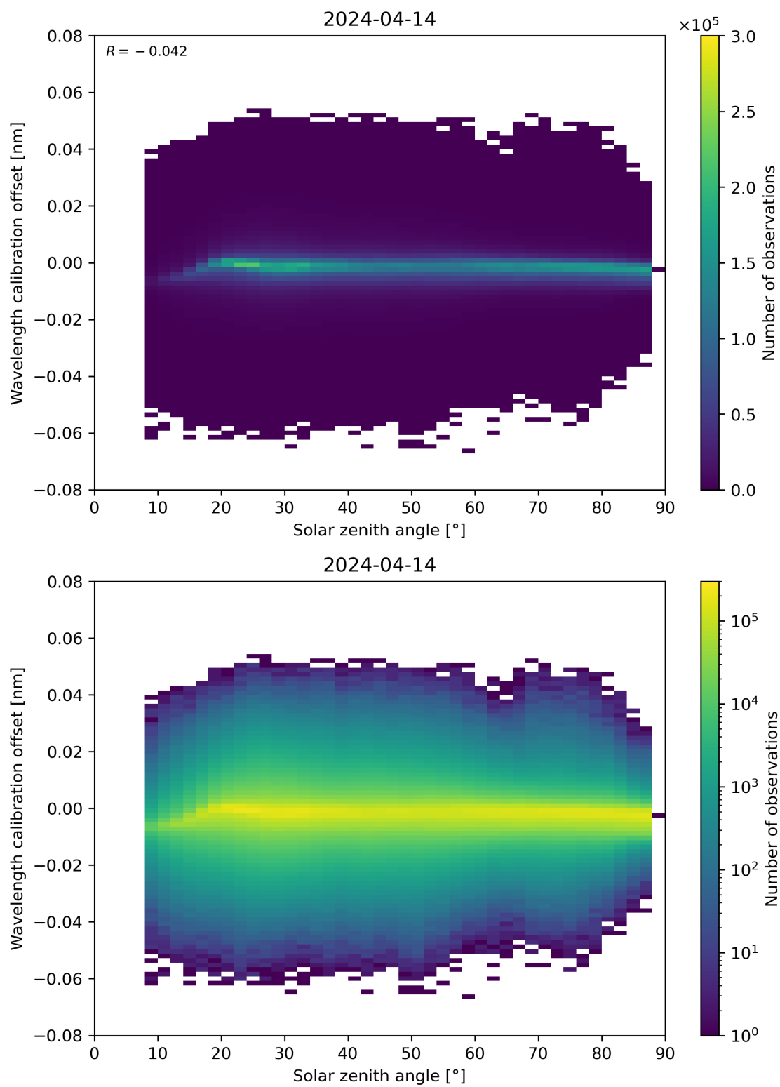
Figure 158: Scatter density plot of “Solar zenith angle” against “Wavelength calibration offset” for 2024-04-13 to 2024-04-15.
