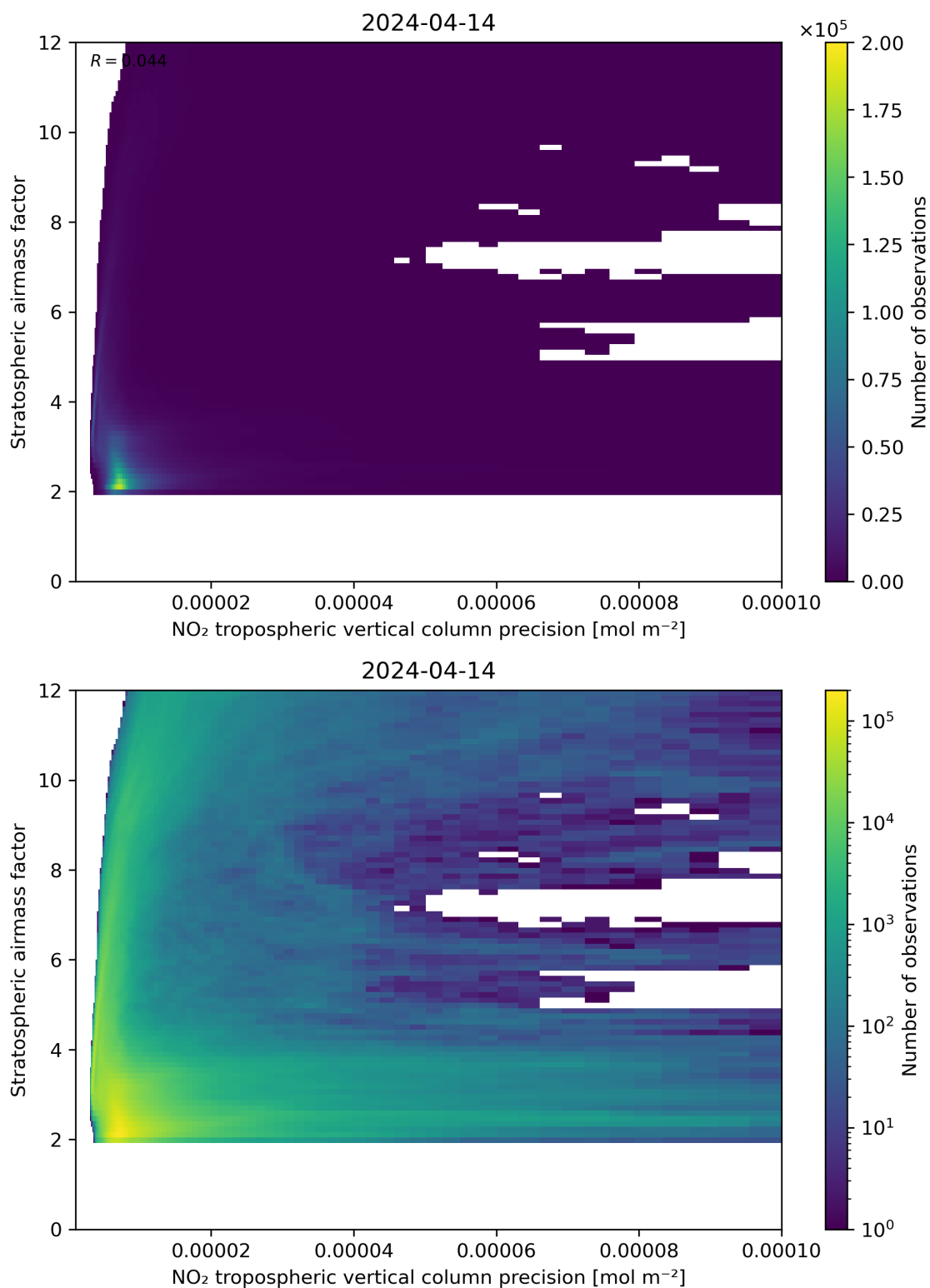
Figure 131: Scatter density plot of “NO 2 tropospheric vertical column precision” against “Stratospheric airmass factor” for 2024-04-13 to 2024-04-15.
