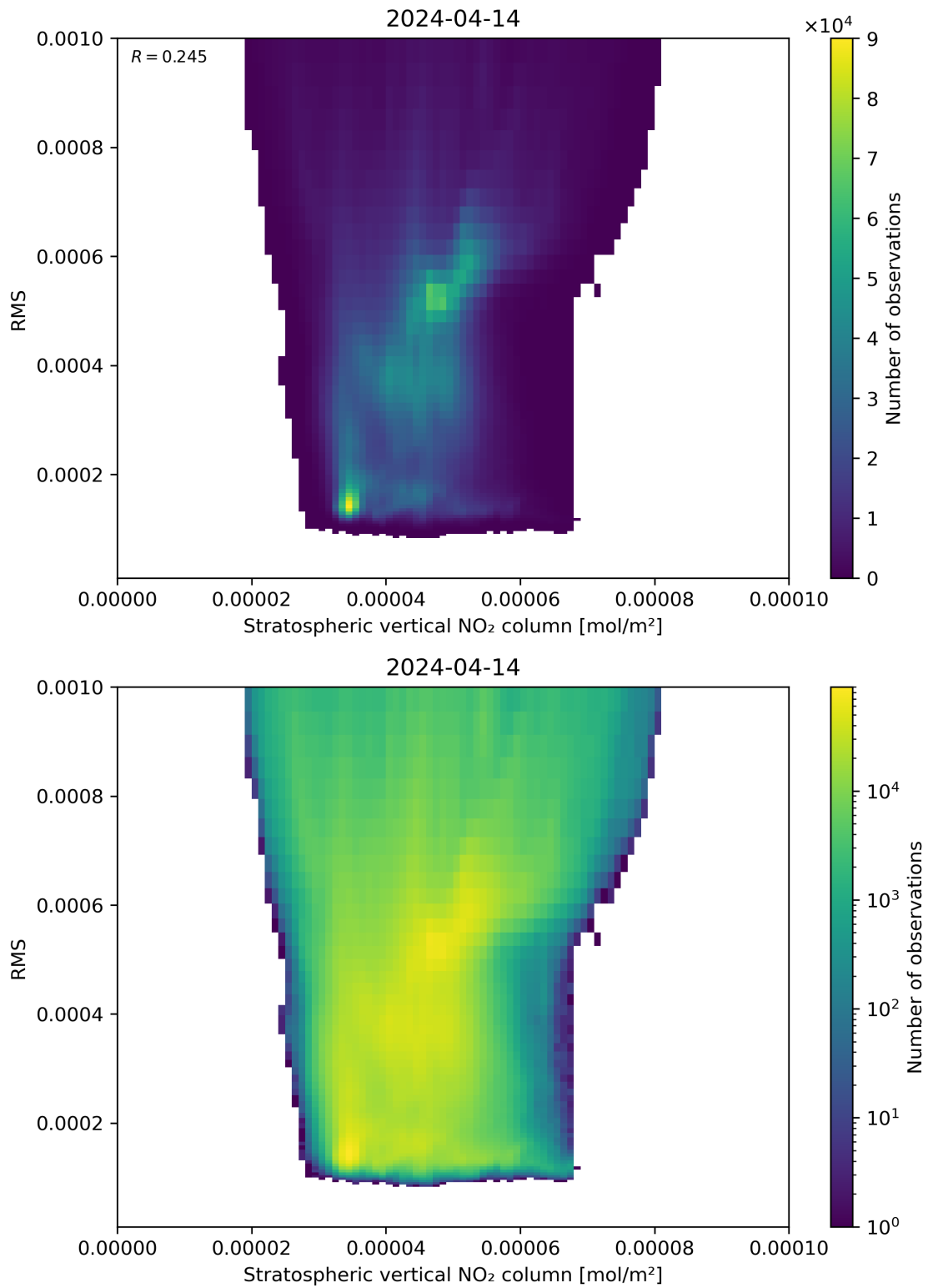
Figure 102: Scatter density plot of “Stratospheric vertical NO 2 column” against “RMS” for 2024-04-13 to 2024-04-15.
