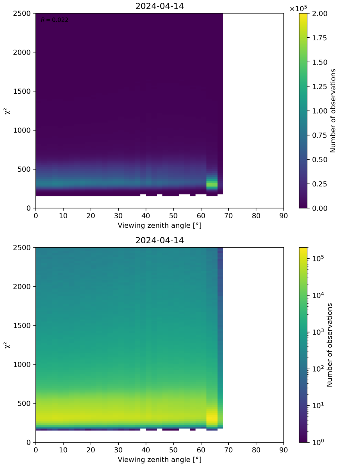
Figure 162: Scatter density plot of “Viewing zenith angle” against “ \chi^2 ” for 2024-04-13 to 2024-04-15.
