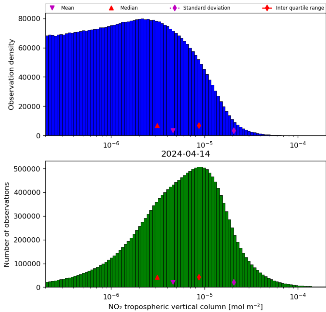
Figure 29: Histogram of “NO 2 tropospheric vertical column” for 2024-04-13 to 2024-04-15
