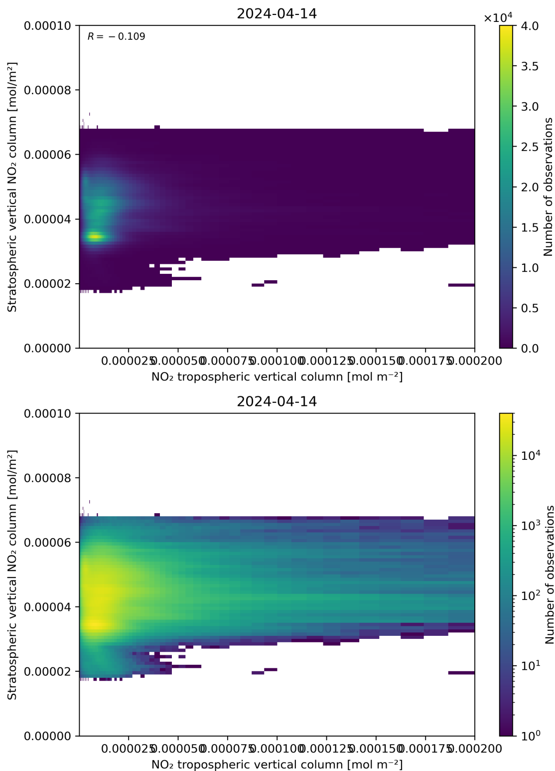
Figure 125: Scatter density plot of “NO 2 tropospheric vertical column” against “Stratospheric vertical NO 2 column” for 2024-04-13 to 2024-04-15.
