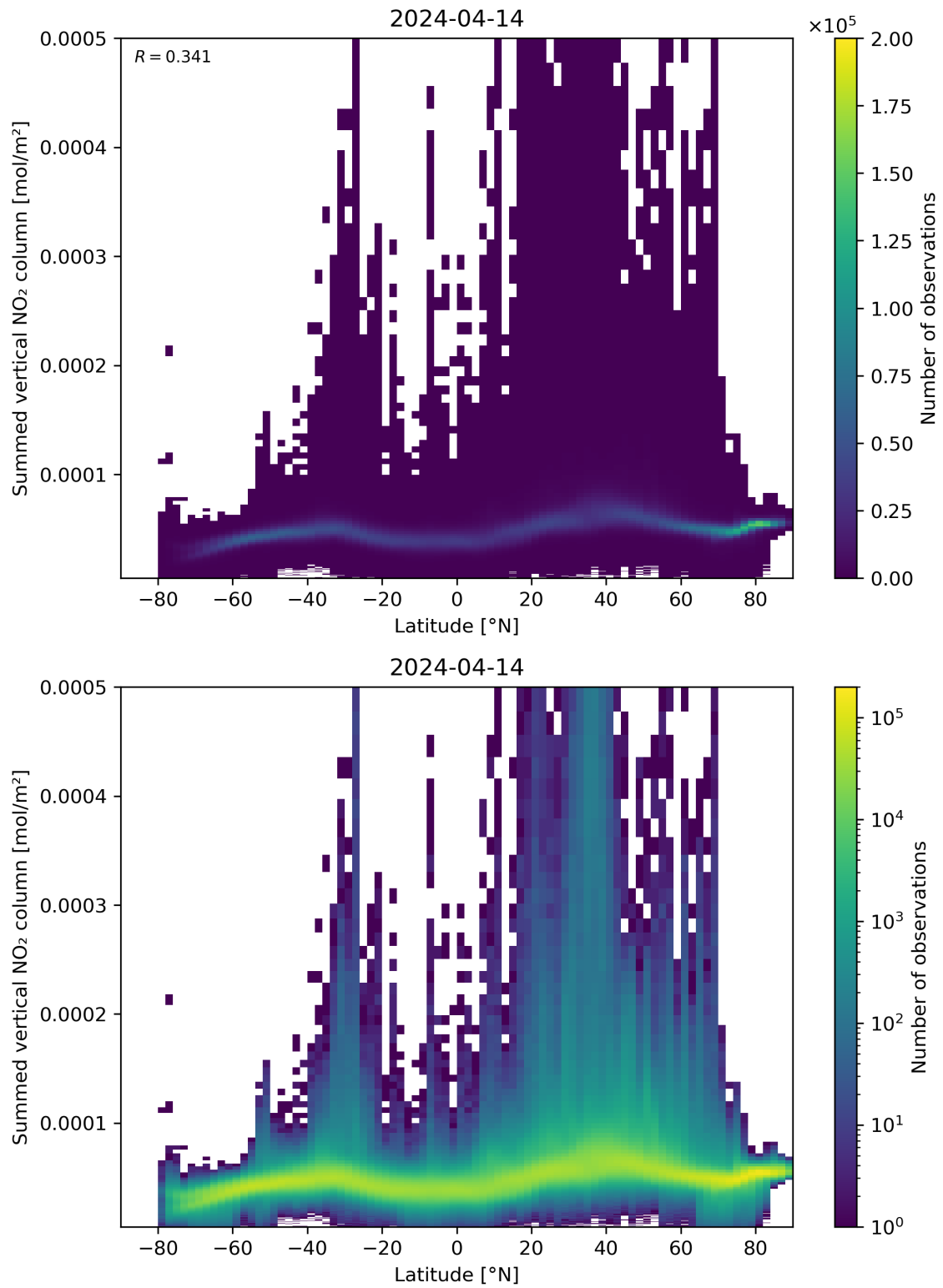
Figure 88: Scatter density plot of “Latitude” against “Summed vertical NO 2 column” for 2024-04-13 to 2024-04-15.
