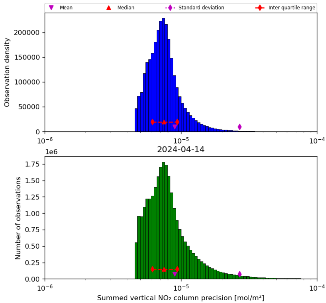
Figure 41: Histogram of “Summed vertical NO 2 column precision” for 2024-04-13 to 2024-04-15
