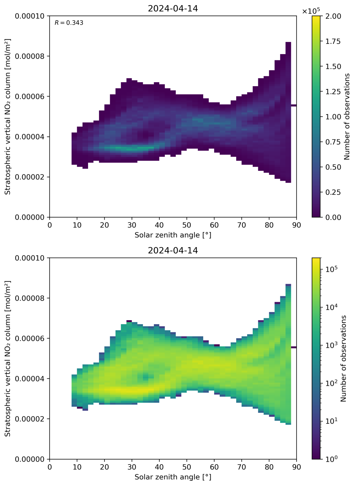
Figure 150: Scatter density plot of “Solar zenith angle” against “Stratospheric vertical NO 2 column” for 2024-04-13 to 2024-04-15.
