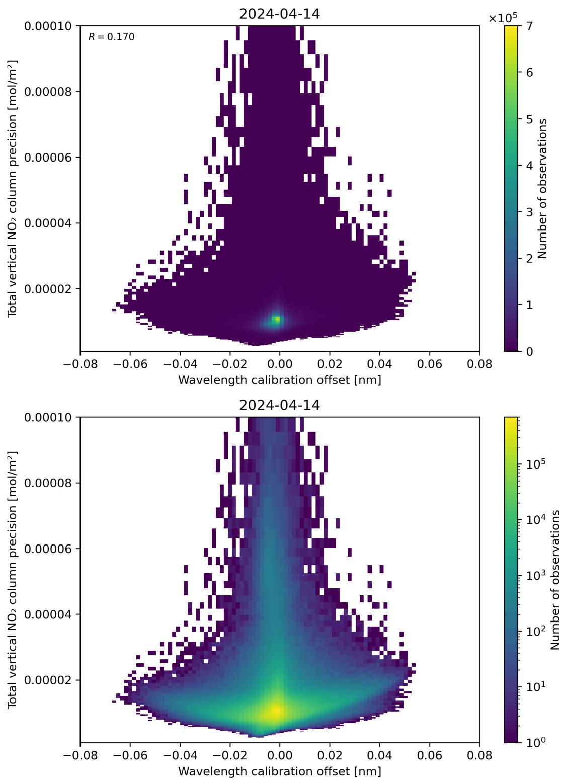
Figure 180: Scatter density plot of “Wavelength calibration offset” against “Total vertical NO 2 column precision” for 2024-04-13 to 2024-04-15.
