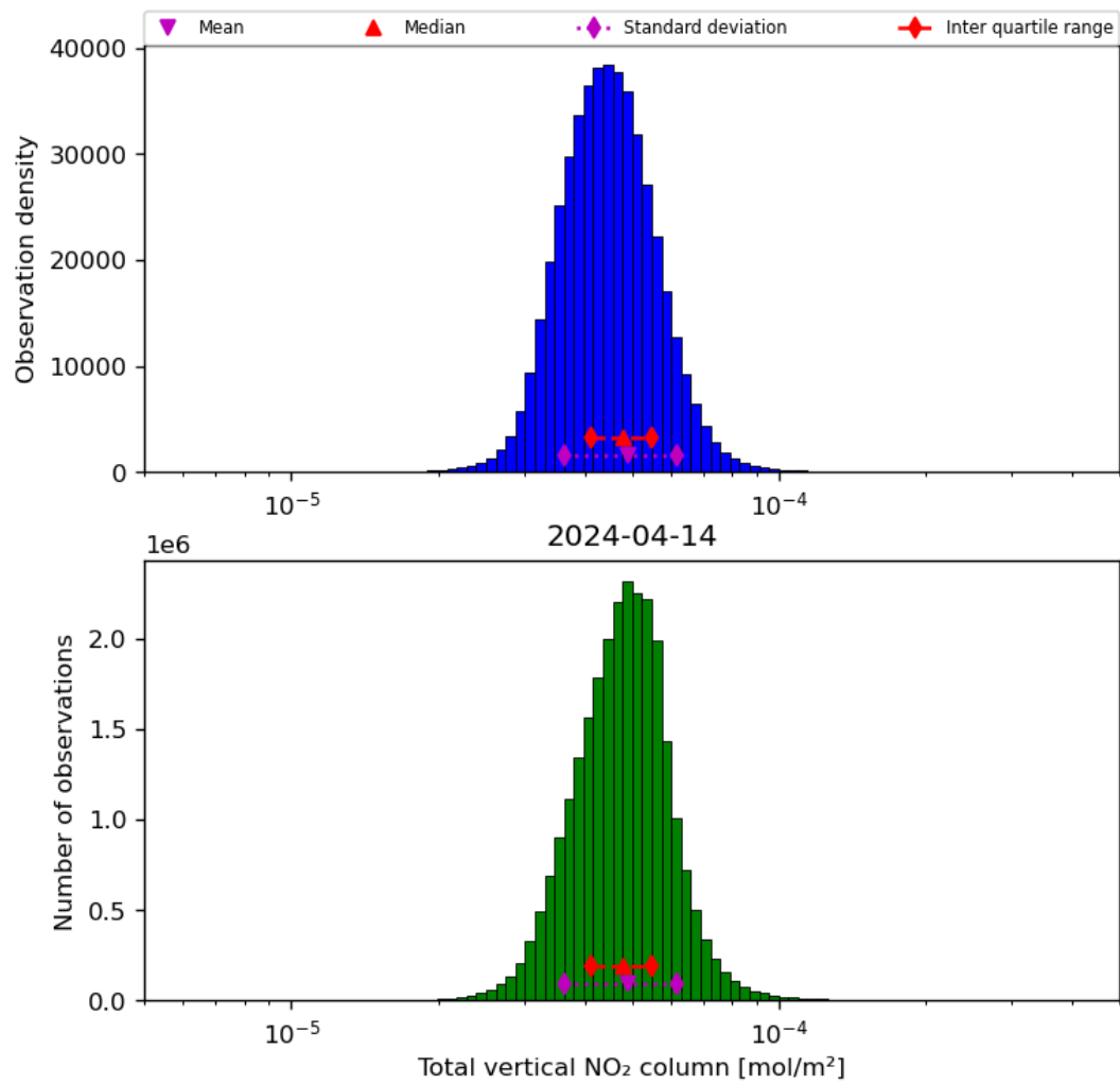
Figure 38: Histogram of “Total vertical NO 2 column” for 2024-04-13 to 2024-04-15
