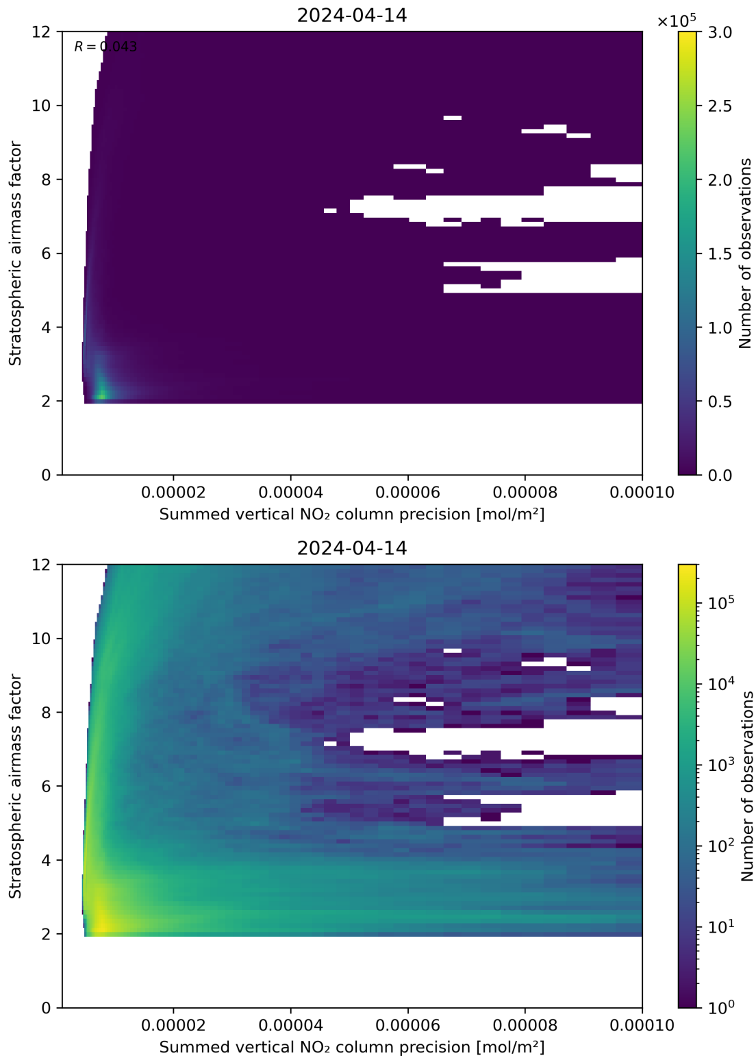
Figure 106: Scatter density plot of “Summed vertical NO 2 column precision” against “Stratospheric airmass factor” for 2024-04-13 to 2024-04-15.
