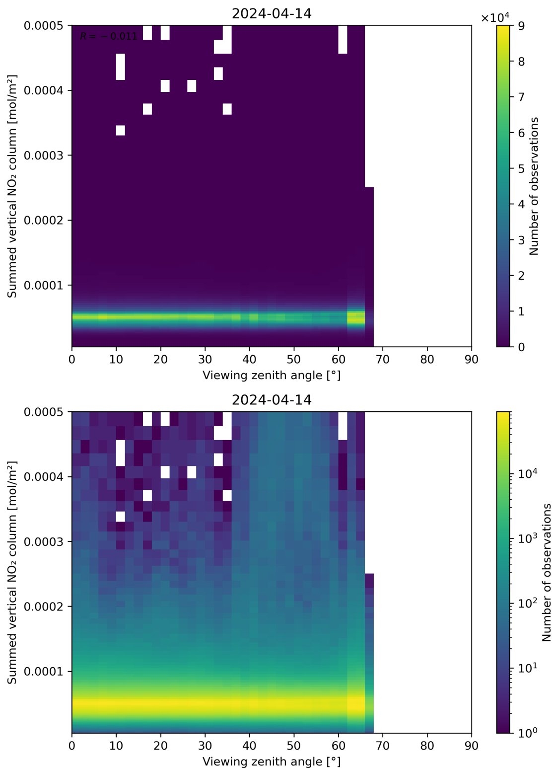
Figure 165: Scatter density plot of “Viewing zenith angle” against “Summed vertical NO 2 column” for 2024-04-13 to 2024-04-15.
