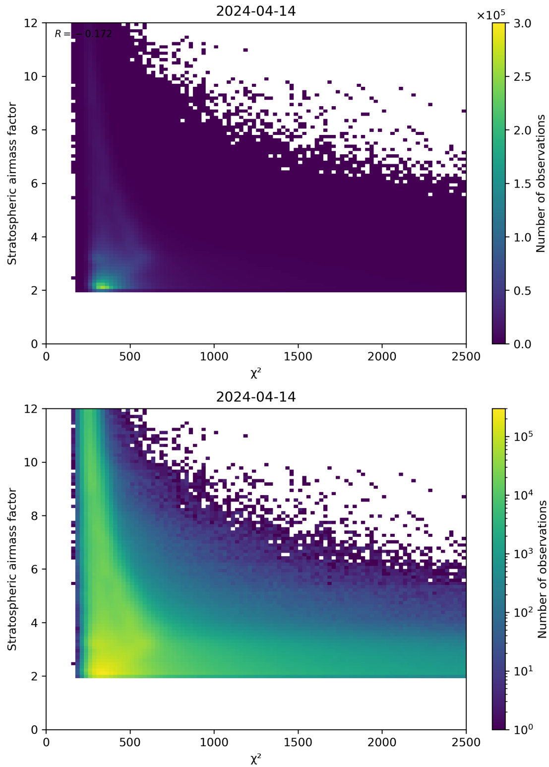
Figure 81: Scatter density plot of “ \chi^2 ” against “Stratospheric airmass factor” for 2024-04-13 to 2024-04-15.
