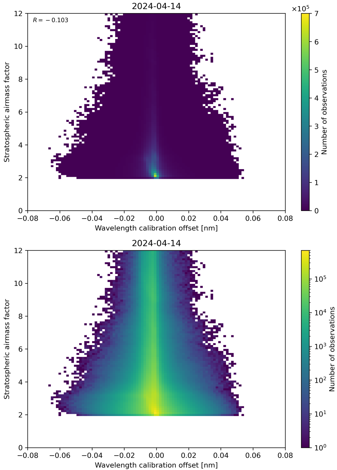
Figure 174: Scatter density plot of “Wavelength calibration offset” against “Stratospheric airmass factor” for 2024-04-13 to 2024-04-15.
