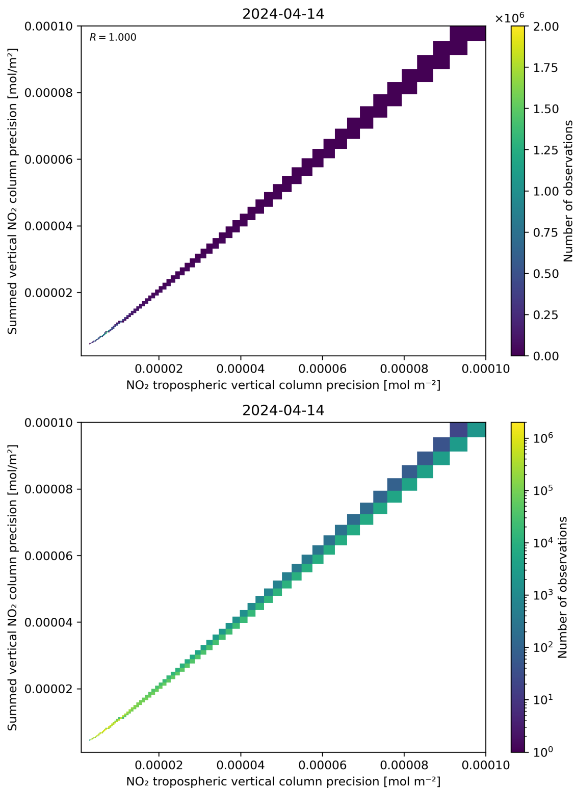
Figure 137: Scatter density plot of “NO 2 tropospheric vertical column precision” against “Summed vertical NO 2 column precision” for 2024-04-13 to 2024-04-15.
