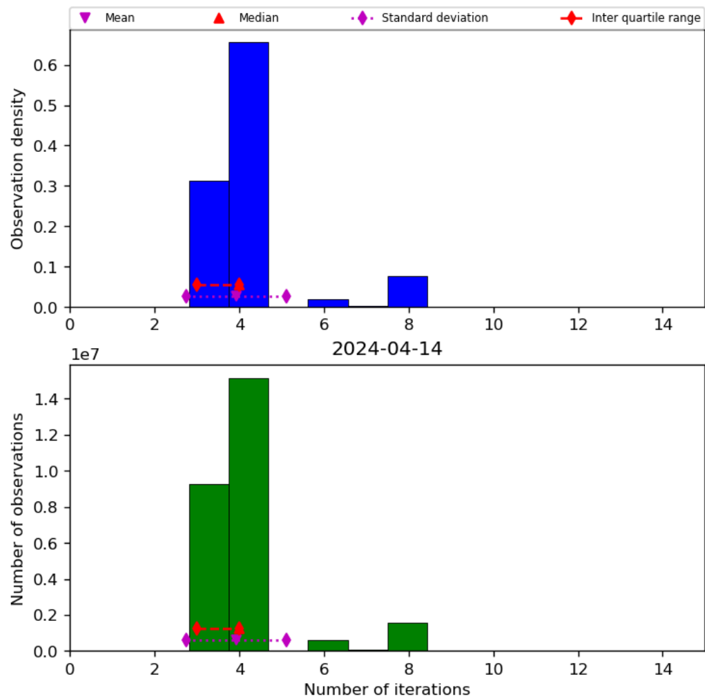
Figure 34: Histogram of “Number of iterations” for 2024-04-13 to 2024-04-15
