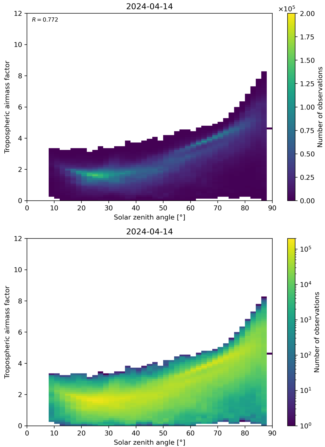
Figure 147: Scatter density plot of “Solar zenith angle” against “Tropospheric airmass factor” for 2024-04-13 to 2024-04-15.
