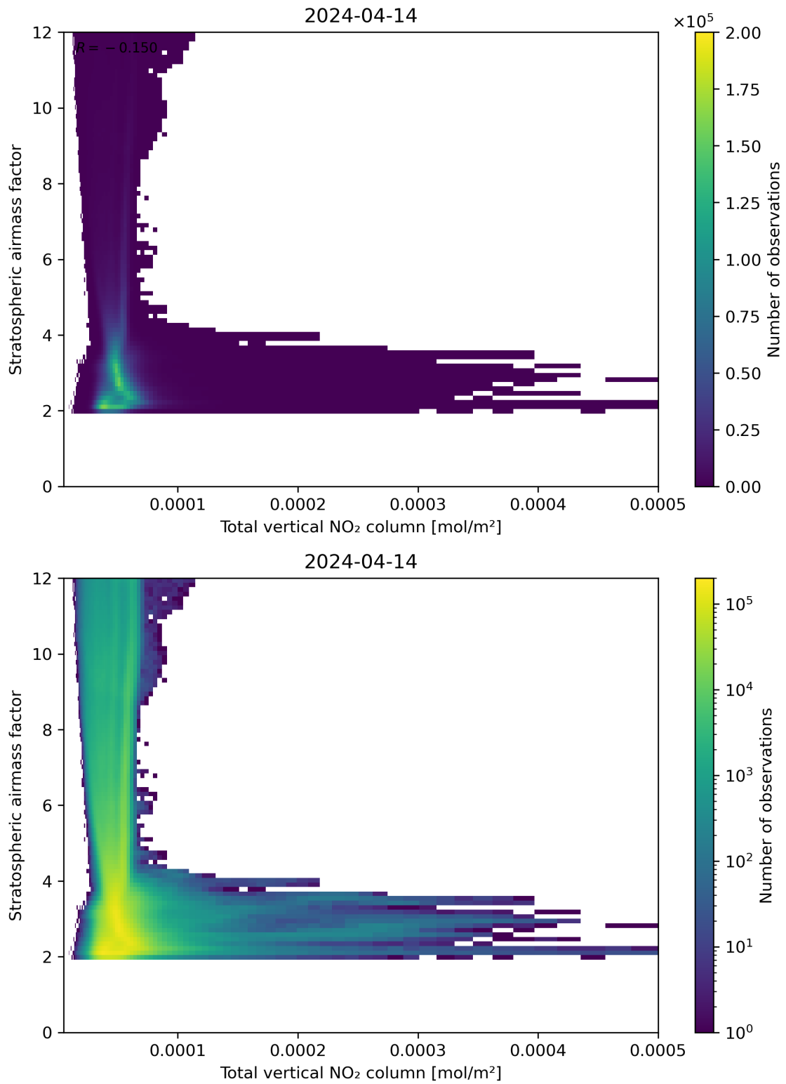
Figure 110: Scatter density plot of “Total vertical NO 2 column” against “Stratospheric airmass factor” for 2024-04-13 to 2024-04-15.
