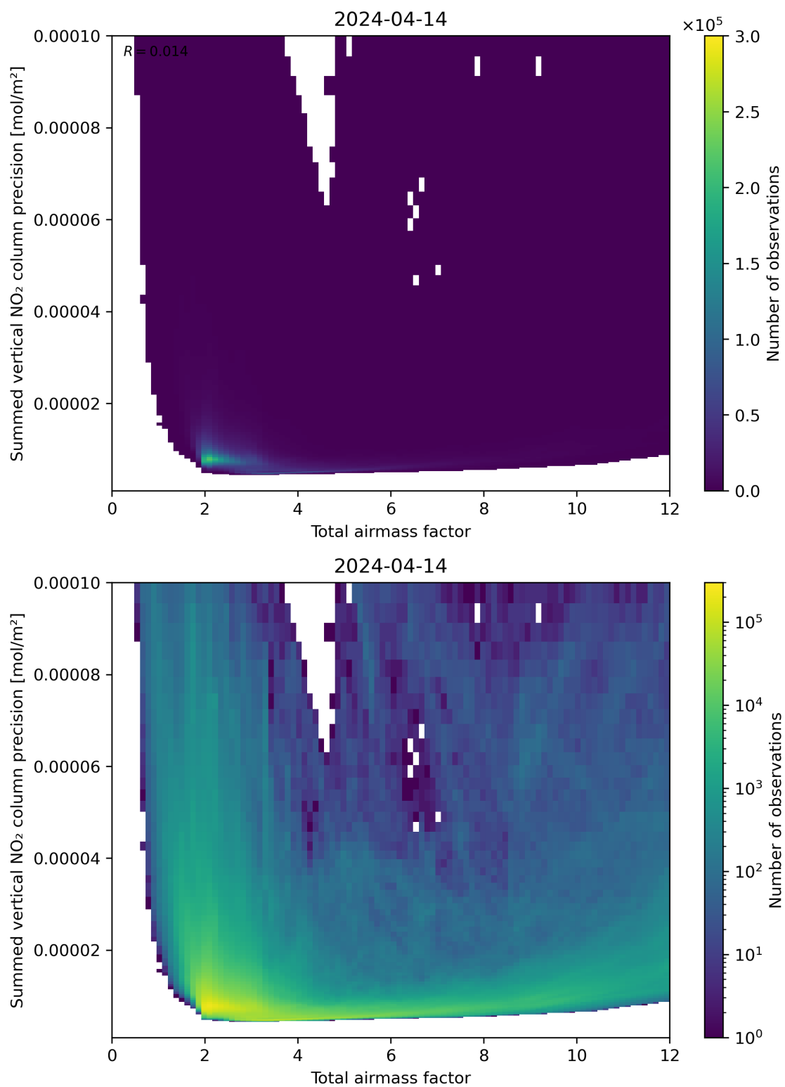
Figure 66: Scatter density plot of “Total airmass factor” against “Summed vertical NO 2 column precision” for 2024-04-13 to 2024-04-15.
