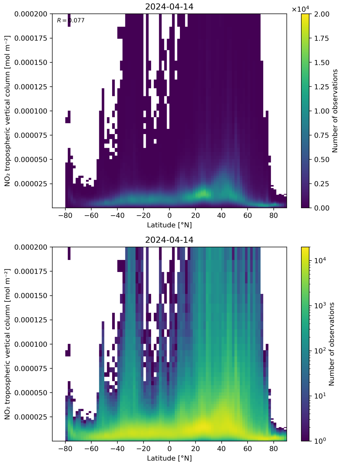
Figure 92: Scatter density plot of “Latitude” against “NO 2 tropospheric vertical column” for 2024-04-13 to 2024-04-15.
