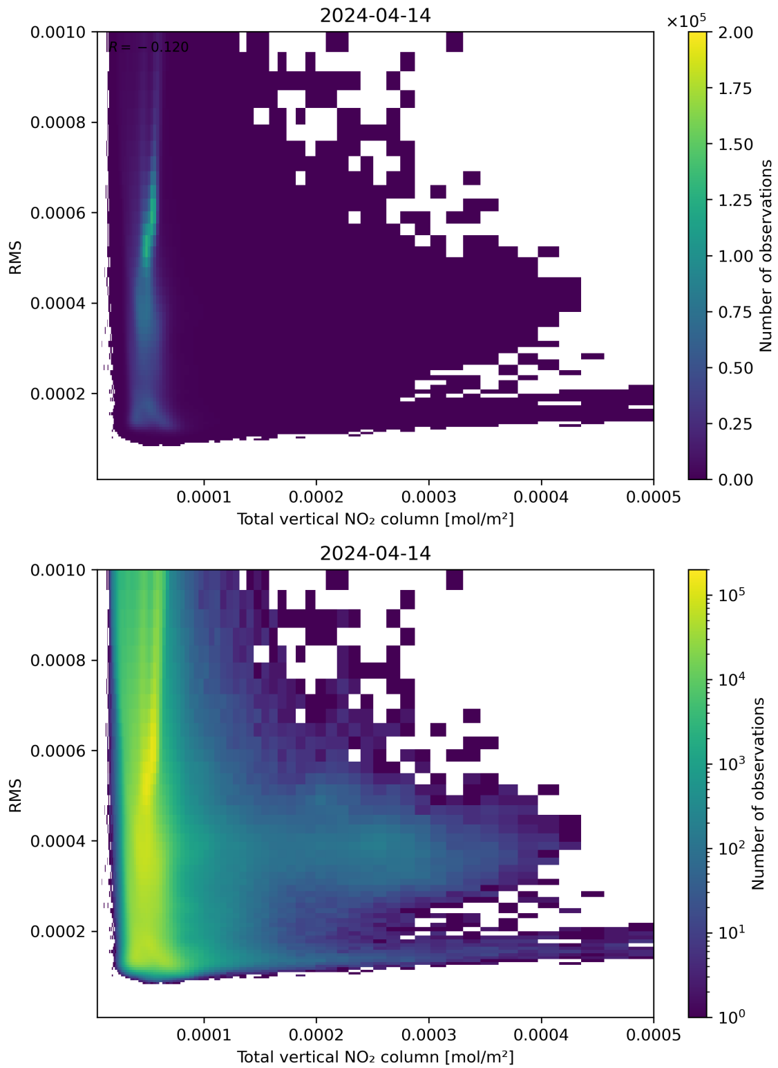
Figure 120: Scatter density plot of “Total vertical NO 2 column” against “RMS” for 2024-04-13 to 2024-04-15.
