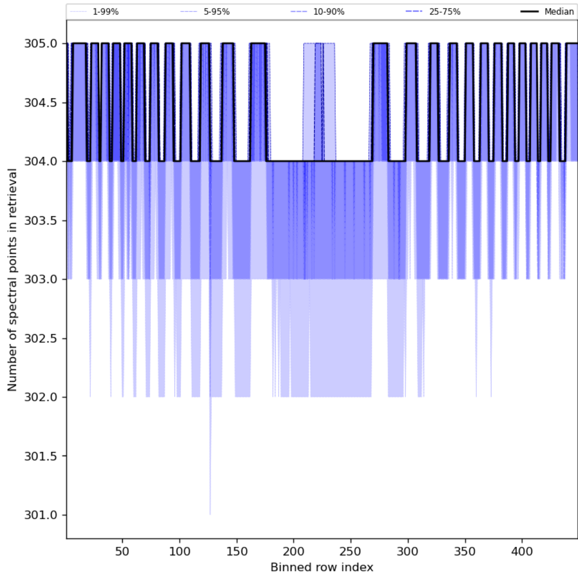
Figure 50: Along track statistics of “Number of spectral points in retrieval” for 2024-04-13 to 2024-04-15
