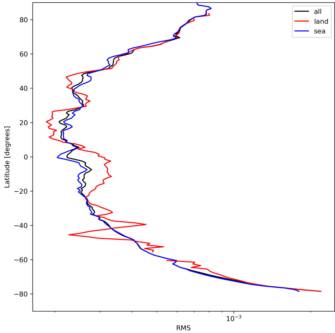
Figure 26: Zonal average of “RMS” for 2024-04-13 to 2024-04-15.
