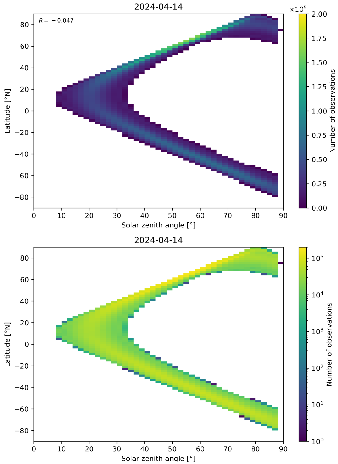
Figure 149: Scatter density plot of “Solar zenith angle” against “Latitude” for 2024-04-13 to 2024-04-15.
