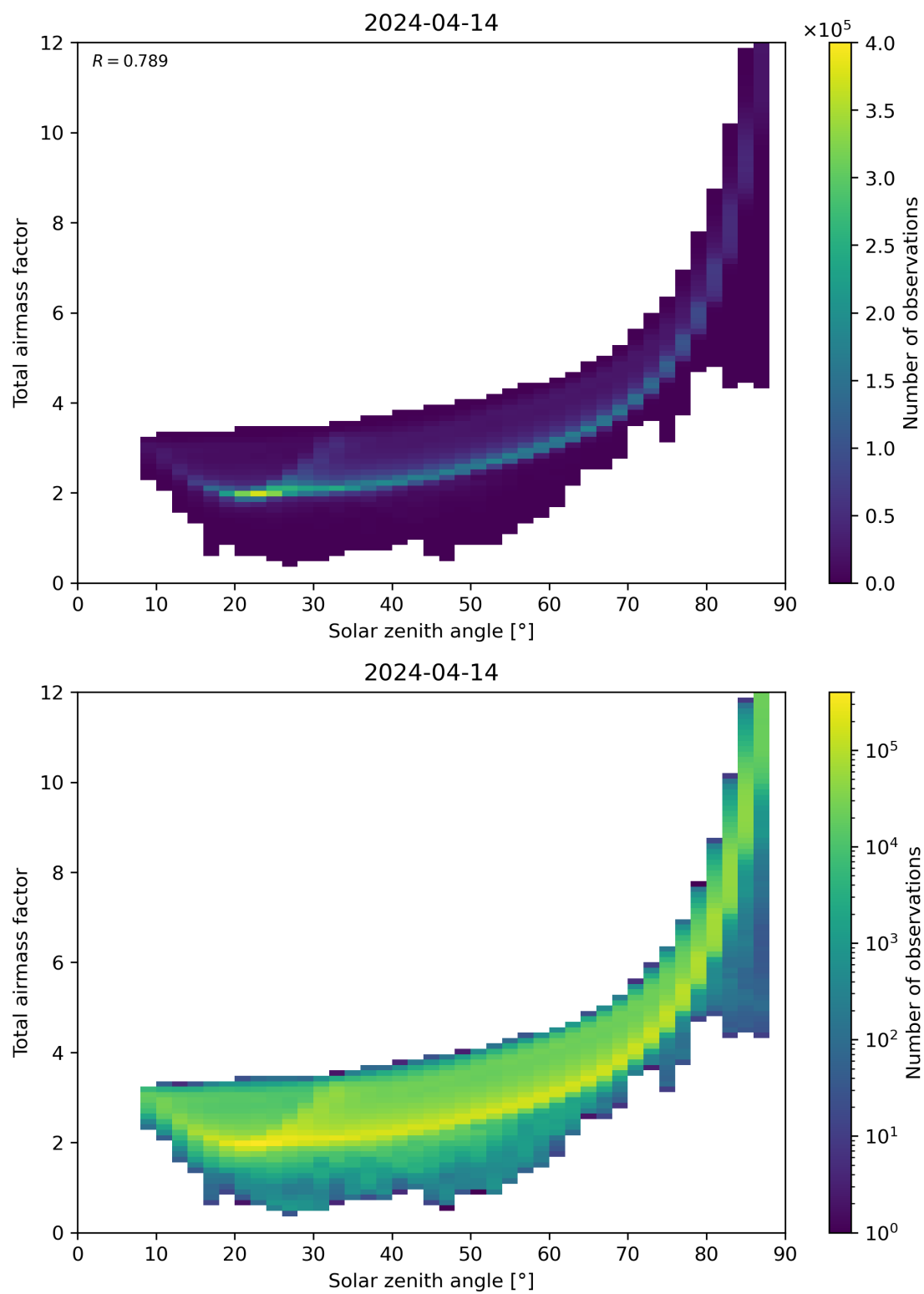
Figure 146: Scatter density plot of “Solar zenith angle” against “Total air mass factor” for 2024-04-13 to 2024-04-15.
