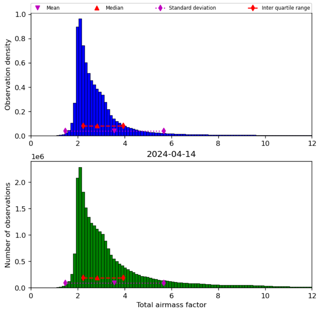
Figure 32: Histogram of “Total airmass factor” for 2024-04-13 to 2024-04-15
