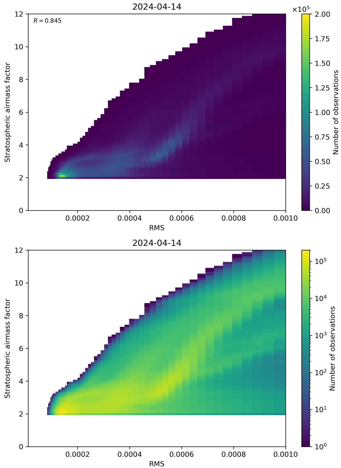
Figure 144: Scatter density plot of “RMS” against “Stratospheric airmass factor” for 2024-04-13 to 2024-04-15.
