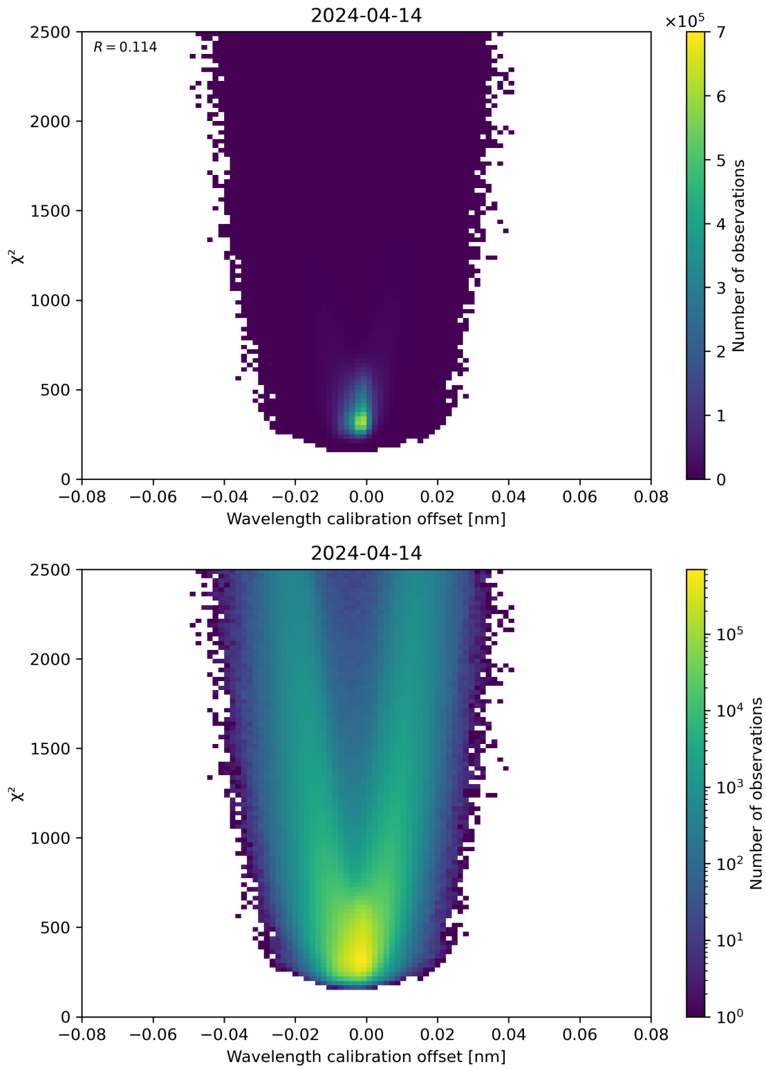
Figure 175: Scatter density plot of “Wavelength calibration offset” against “ \chi^2 ” for 2024-04-13 to 2024-04-15.
