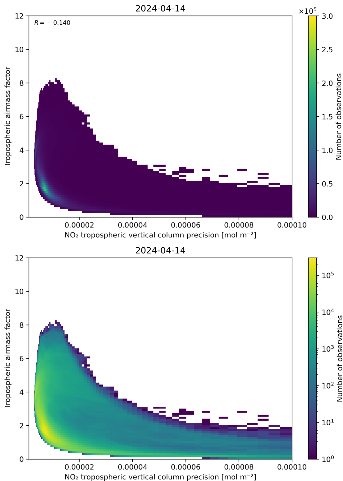
Figure 133: Scatter density plot of “NO 2 tropospheric vertical column precision” against “Tropospheric airmass factor” for 2024-04-13 to 2024-04-15.
