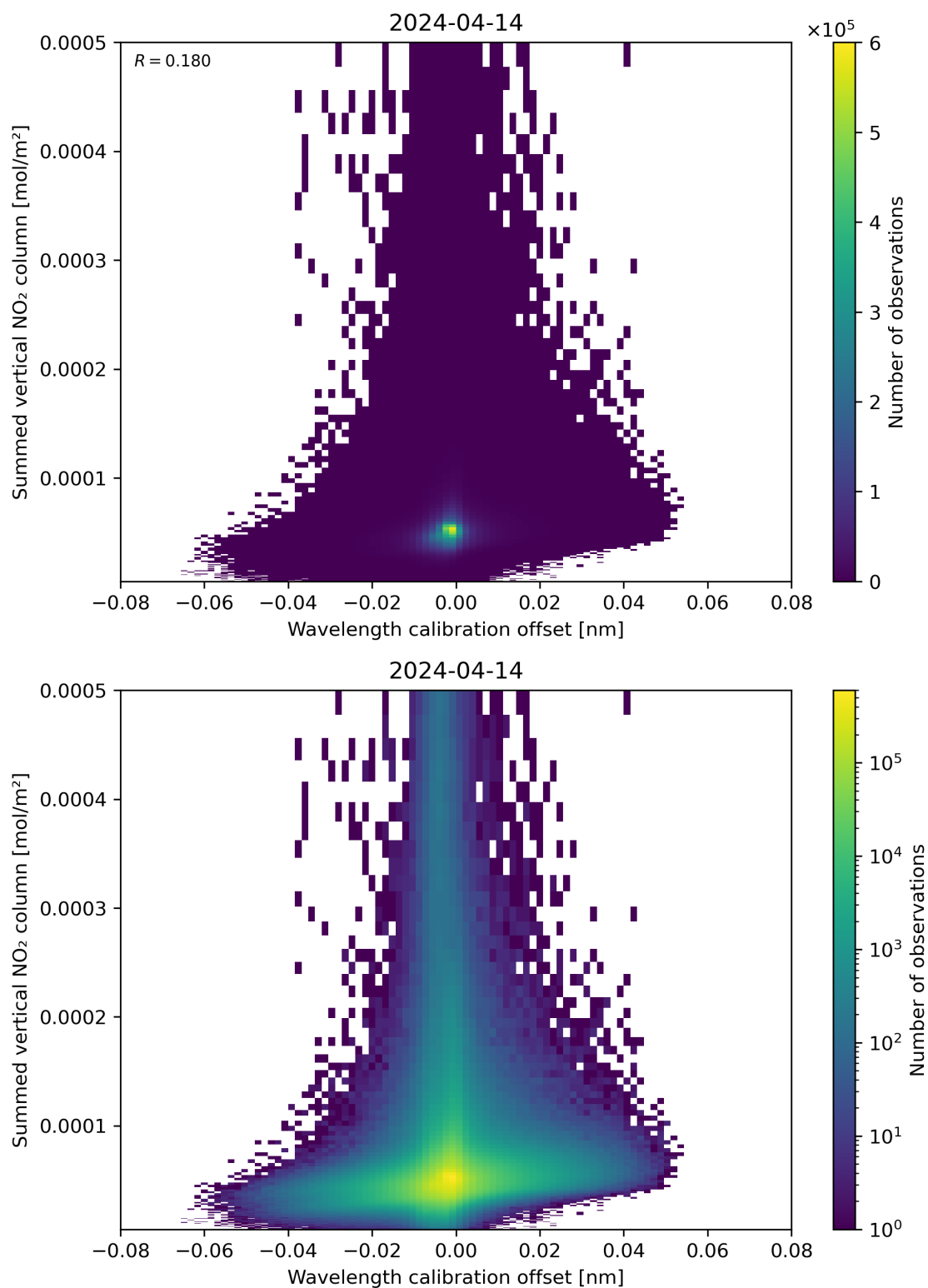
Figure 177: Scatter density plot of “Wavelength calibration offset” against “Summed vertical NO 2 column” for 2024-04-13 to 2024-04-15.
