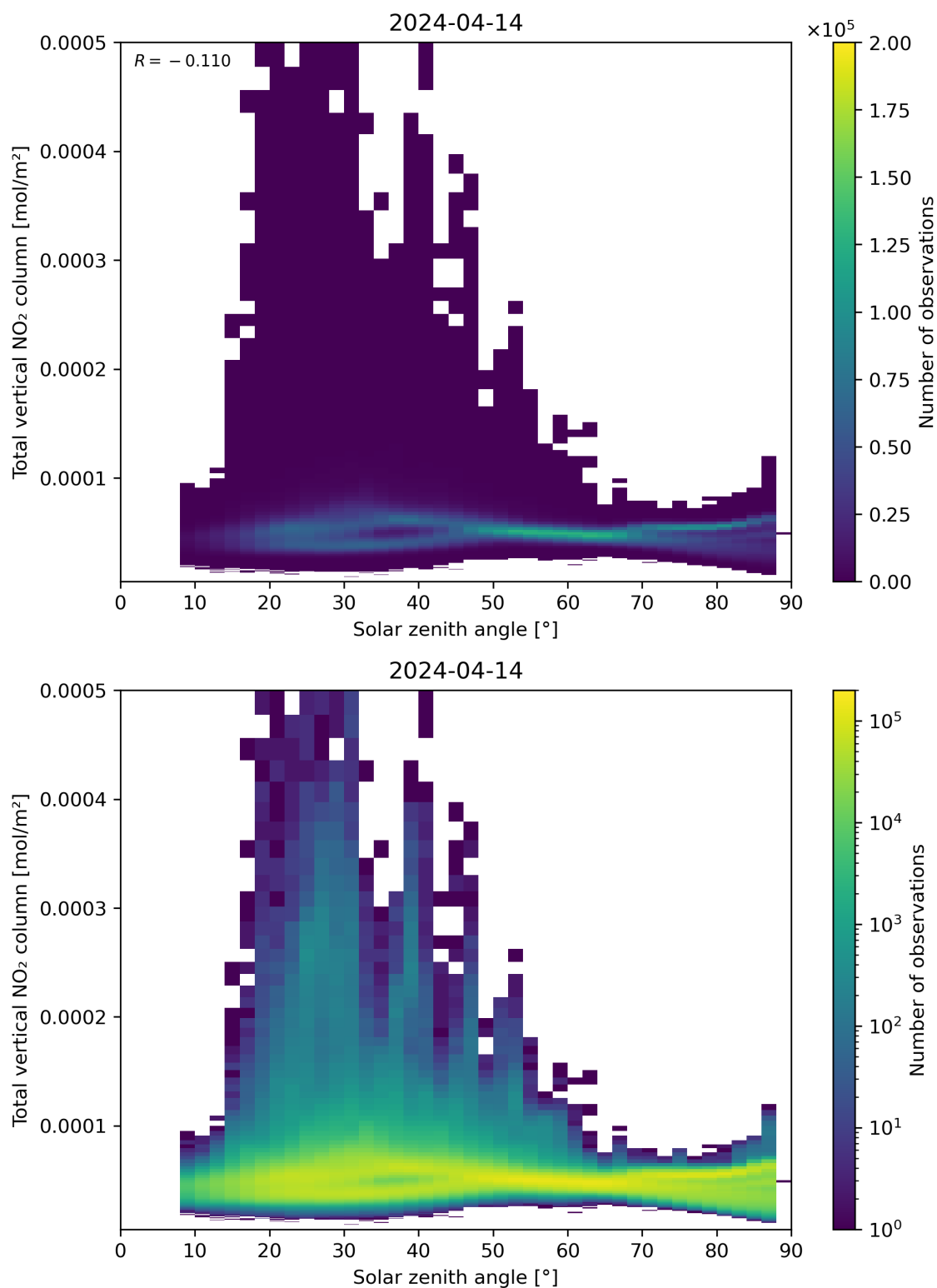
Figure 153: Scatter density plot of “Solar zenith angle” against “Total vertical NO 2 column” for 2024-04-13 to 2024-04-15.
