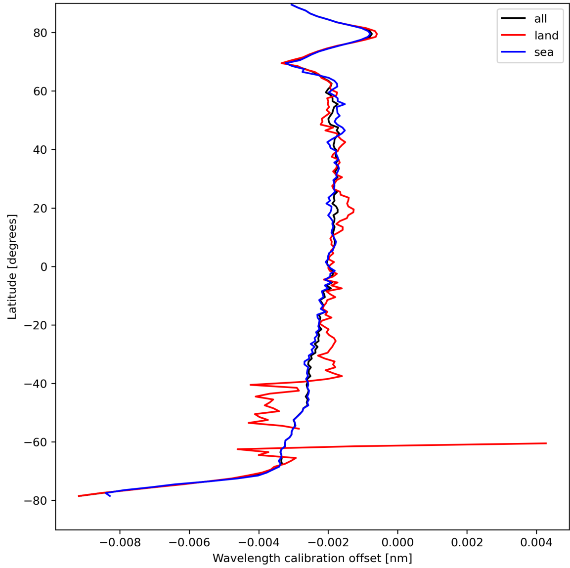
Figure 18: Zonal average of “Wavelength calibration offset” for 2024-04-13 to 2024-04-15.
