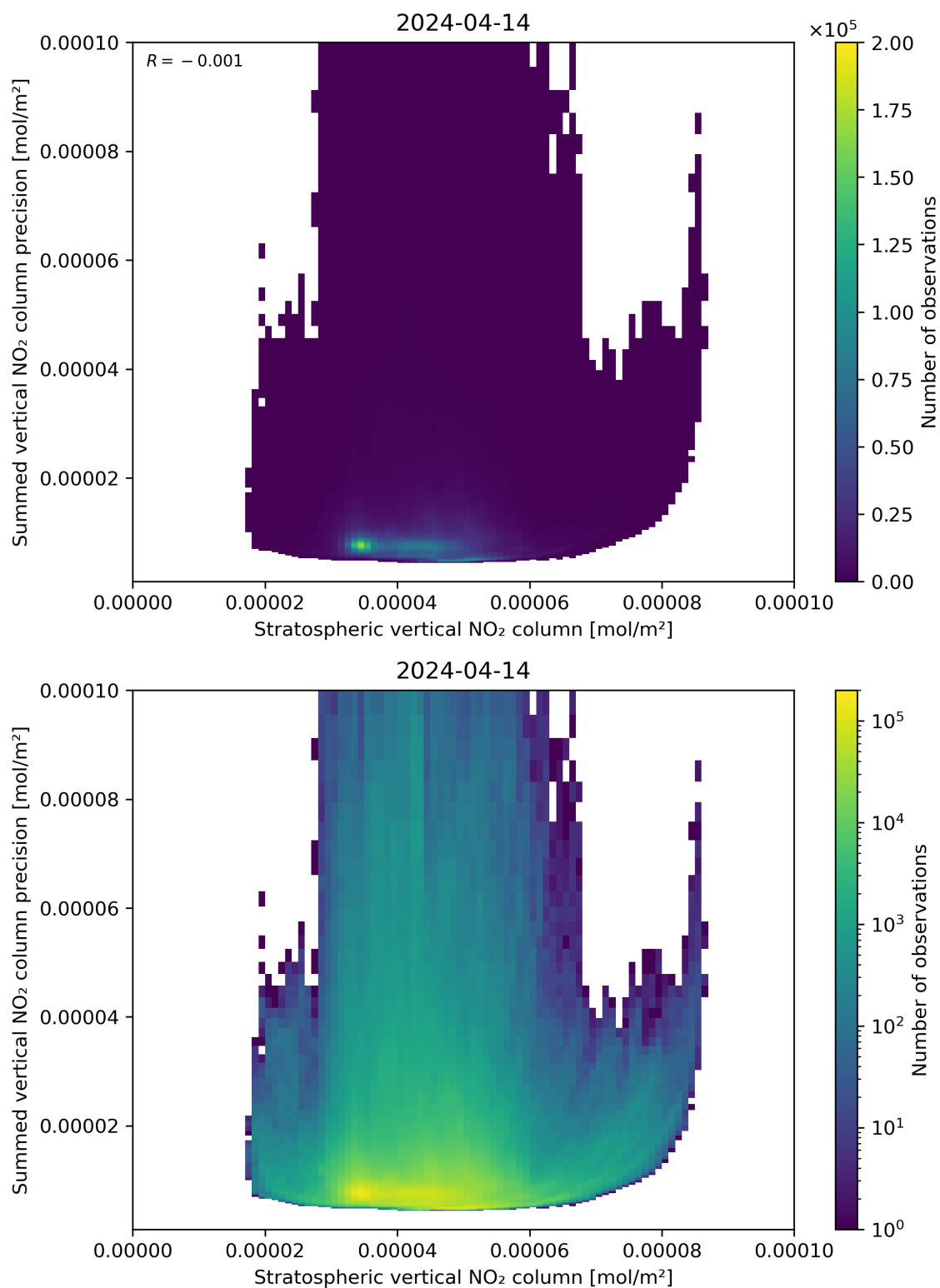
Figure 99: Scatter density plot of “Stratospheric vertical NO 2 column” against “Summed vertical NO 2 column precision” for 2024-04-13 to 2024-04-15.
