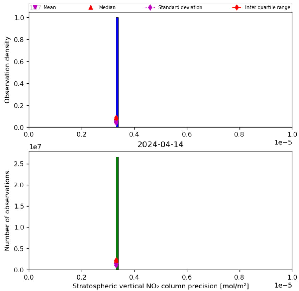
Figure 37: Histogram of “Stratospheric vertical NO 2 column precision” for 2024-04-13 to 2024-04-15
