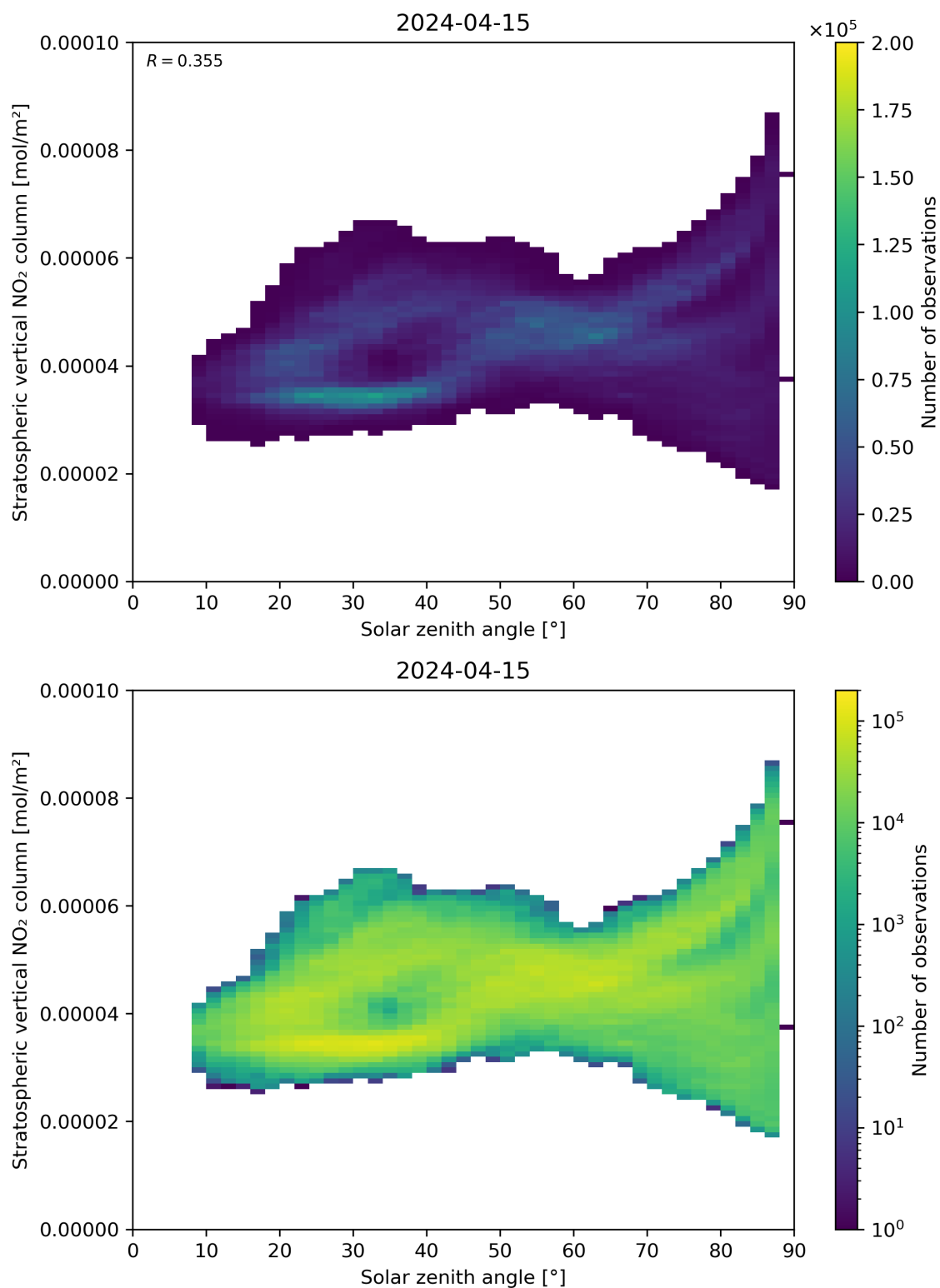
Figure 150: Scatter density plot of “Solar zenith angle” against “Stratospheric vertical NO 2 column” for 2024-04-15 to 2024-04-16.
