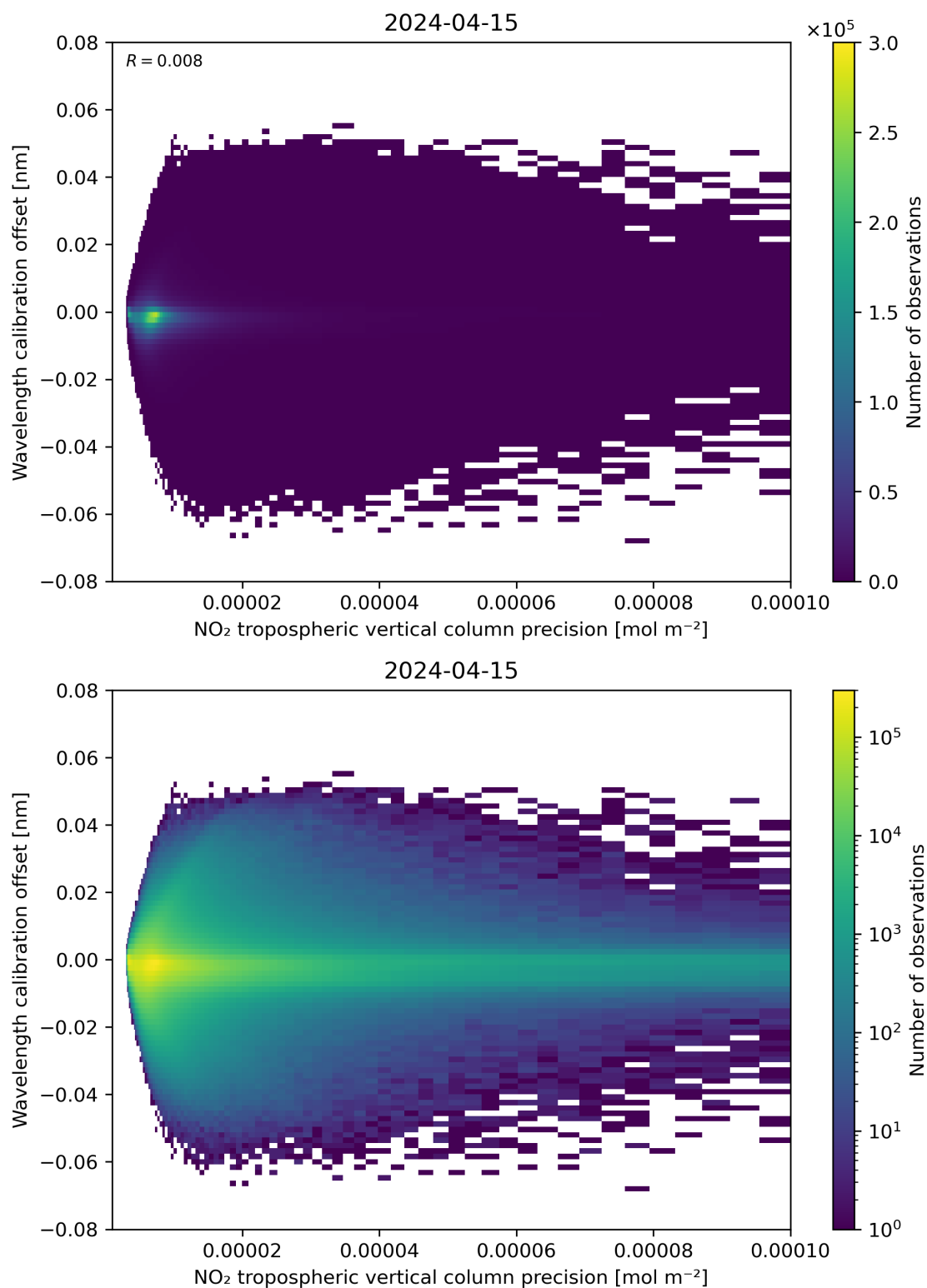
Figure 141: Scatter density plot of “NO 2 tropospheric vertical column precision” against “Wavelength calibration offset” for 2024-04-15 to 2024-04-16.
