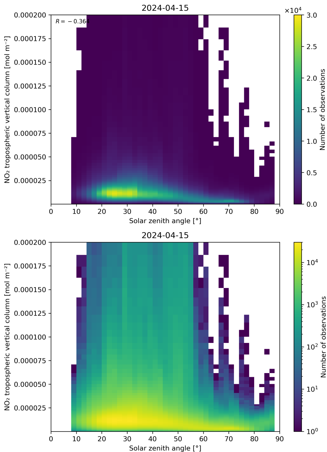
Figure 155: Scatter density plot of “Solar zenith angle” against “NO 2 tropospheric vertical column” for 2024-04-15 to 2024-04-16.
