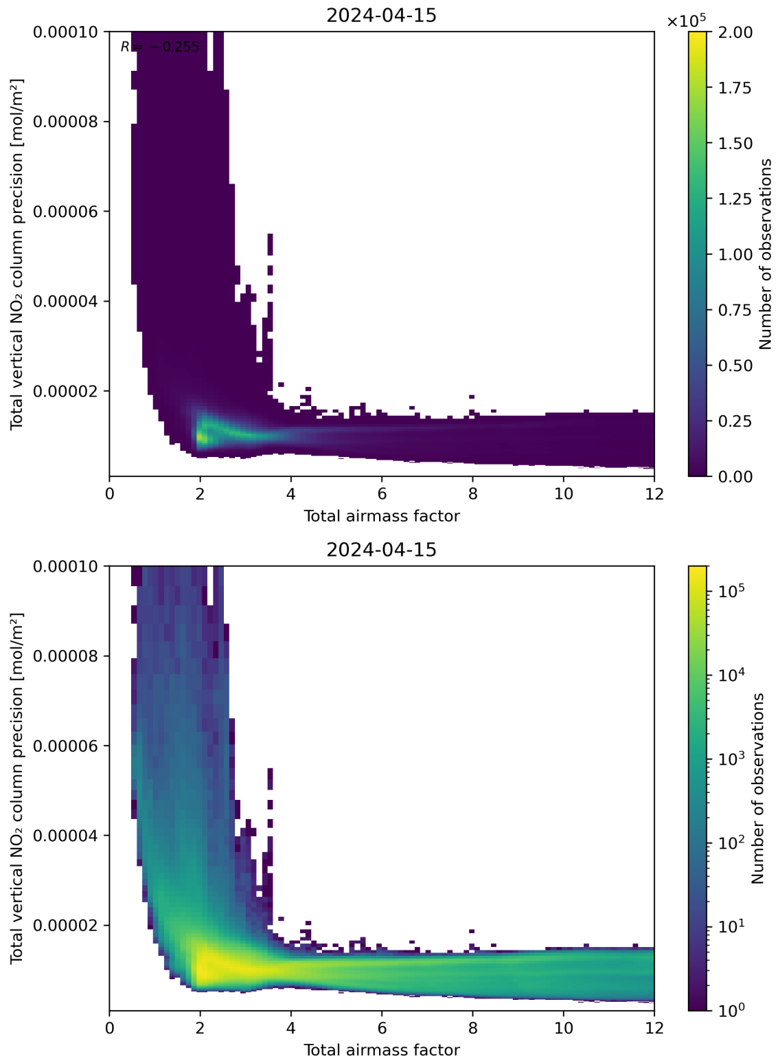
Figure 68: Scatter density plot of “Total airmass factor” against “Total vertical NO 2 column precision” for 2024-04-15 to 2024-04-16.
