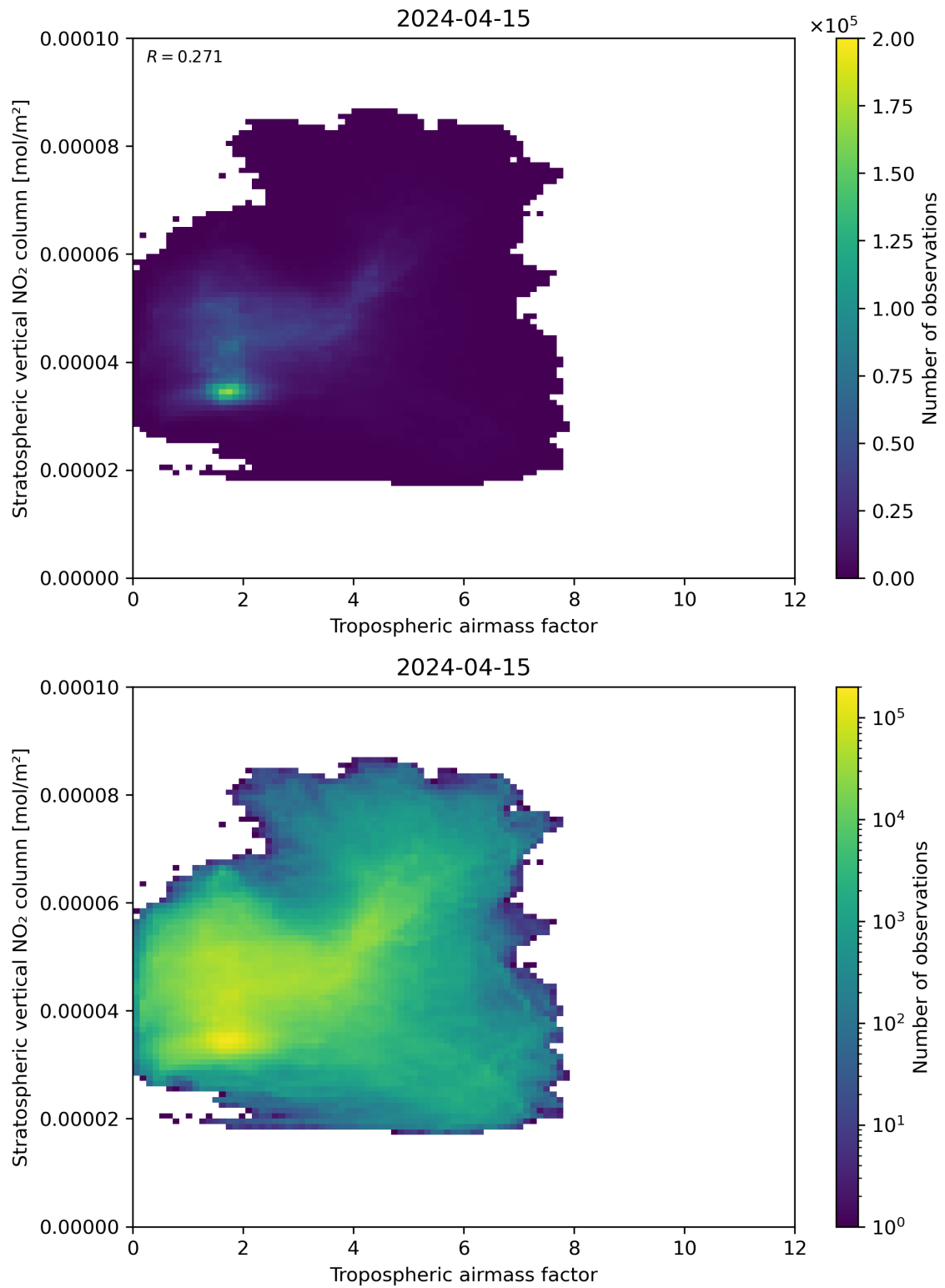
Figure 74: Scatter density plot of “Tropospheric air mass factor” against “Stratospheric vertical NO 2 column” for 2024-04-15 to 2024-04-16.
