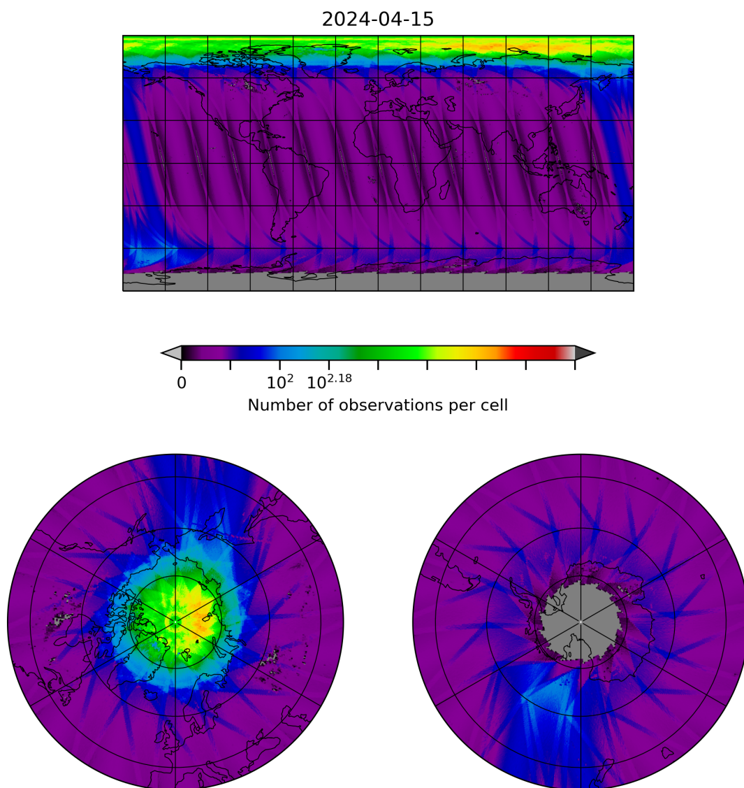
Figure 10: Map of the number of observations for 2024-04-15 to 2024-04-16
