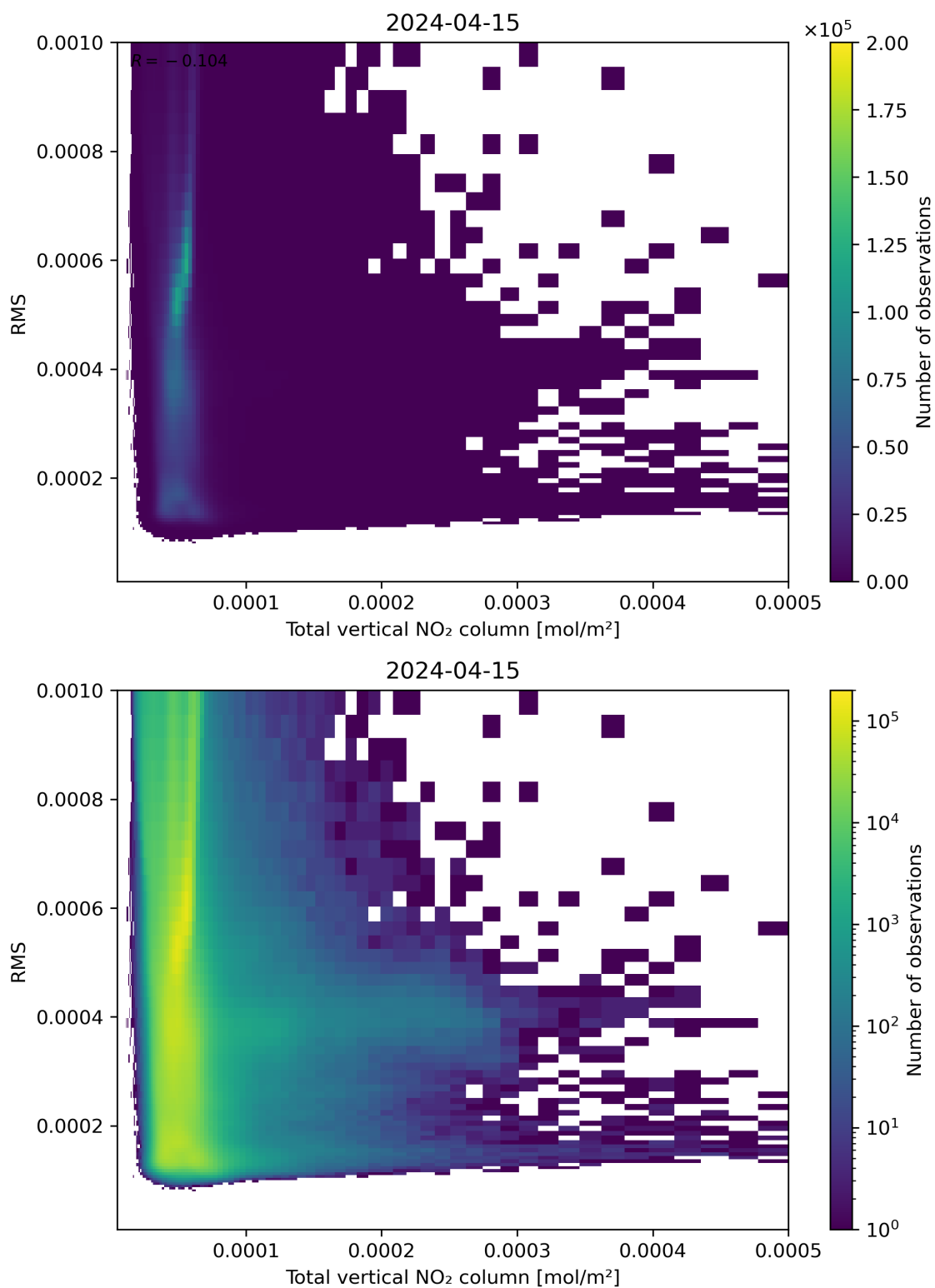
Figure 120: Scatter density plot of “Total vertical NO 2 column” against “RMS” for 2024-04-15 to 2024-04-16.
