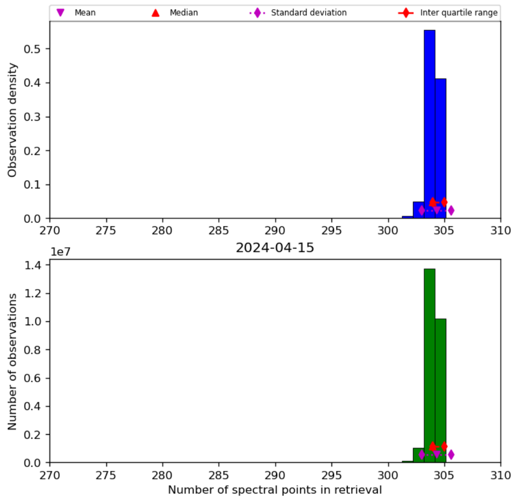
Figure 33: Histogram of “Number of spectral points in retrieval” for 2024-04-15 to 2024-04-16
