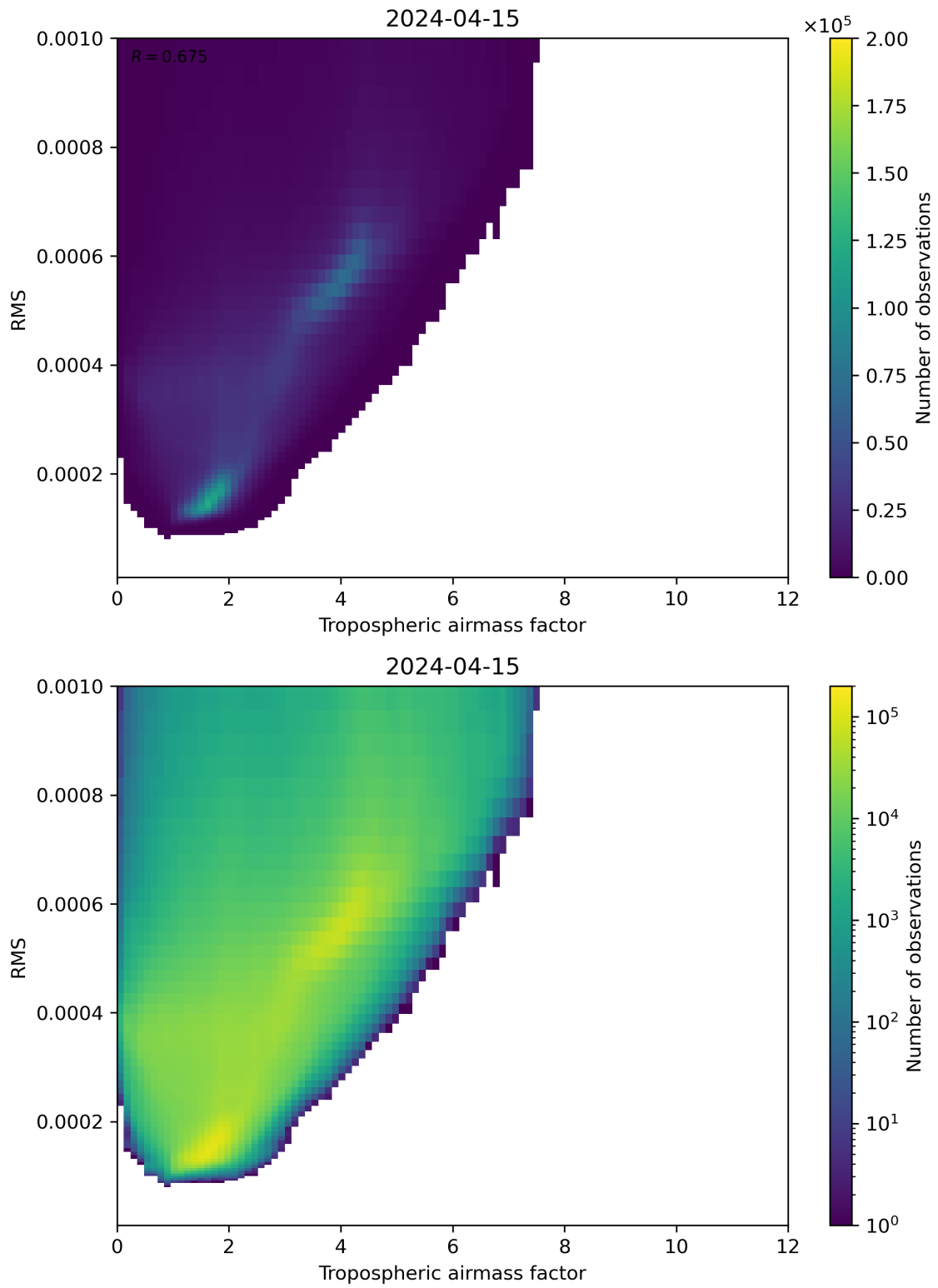
Figure 79: Scatter density plot of “Tropospheric airmass factor” against “RMS” for 2024-04-15 to 2024-04-16.
