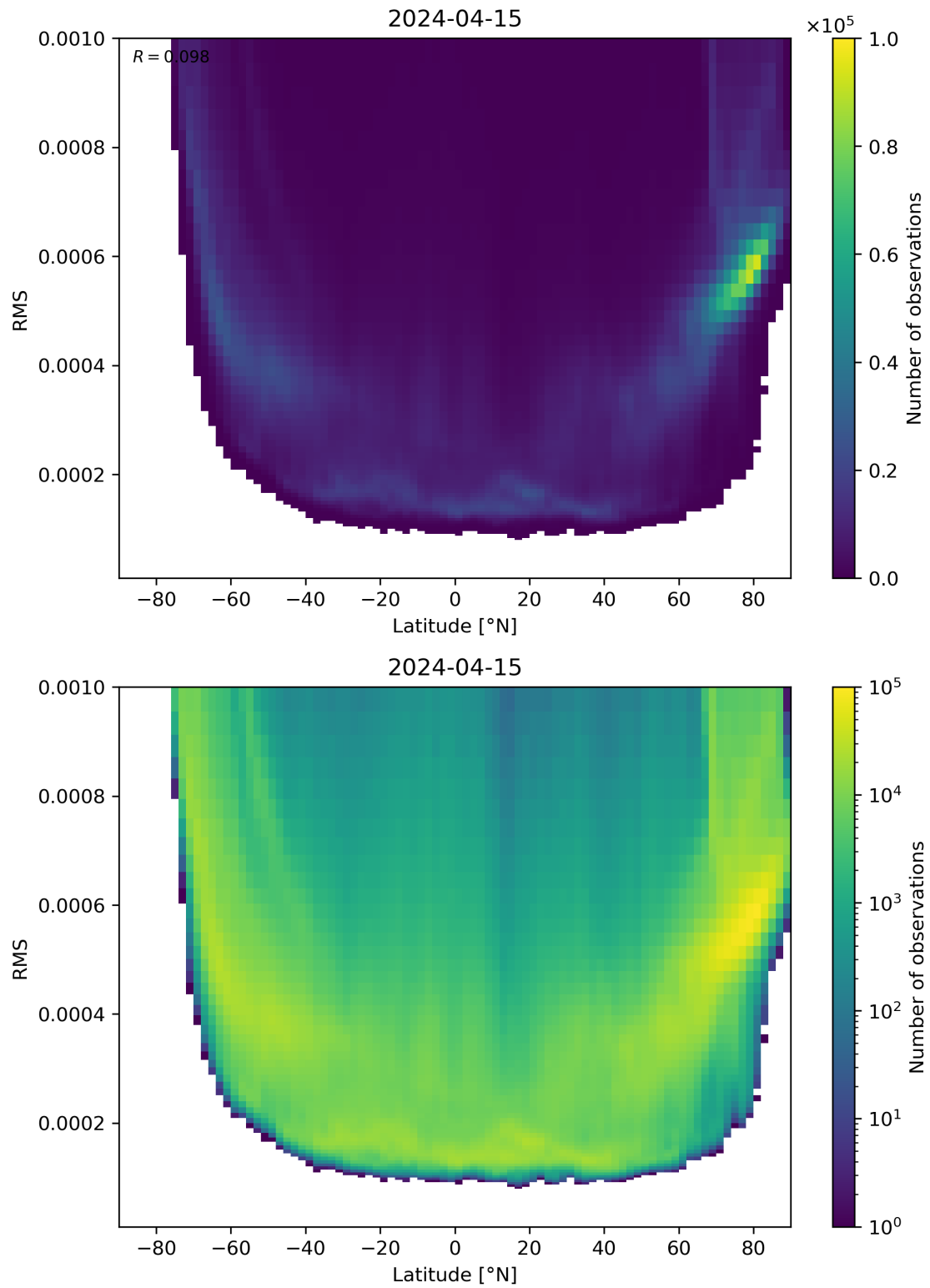
Figure 94: Scatter density plot of “Latitude” against “RMS” for 2024-04-15 to 2024-04-16.
