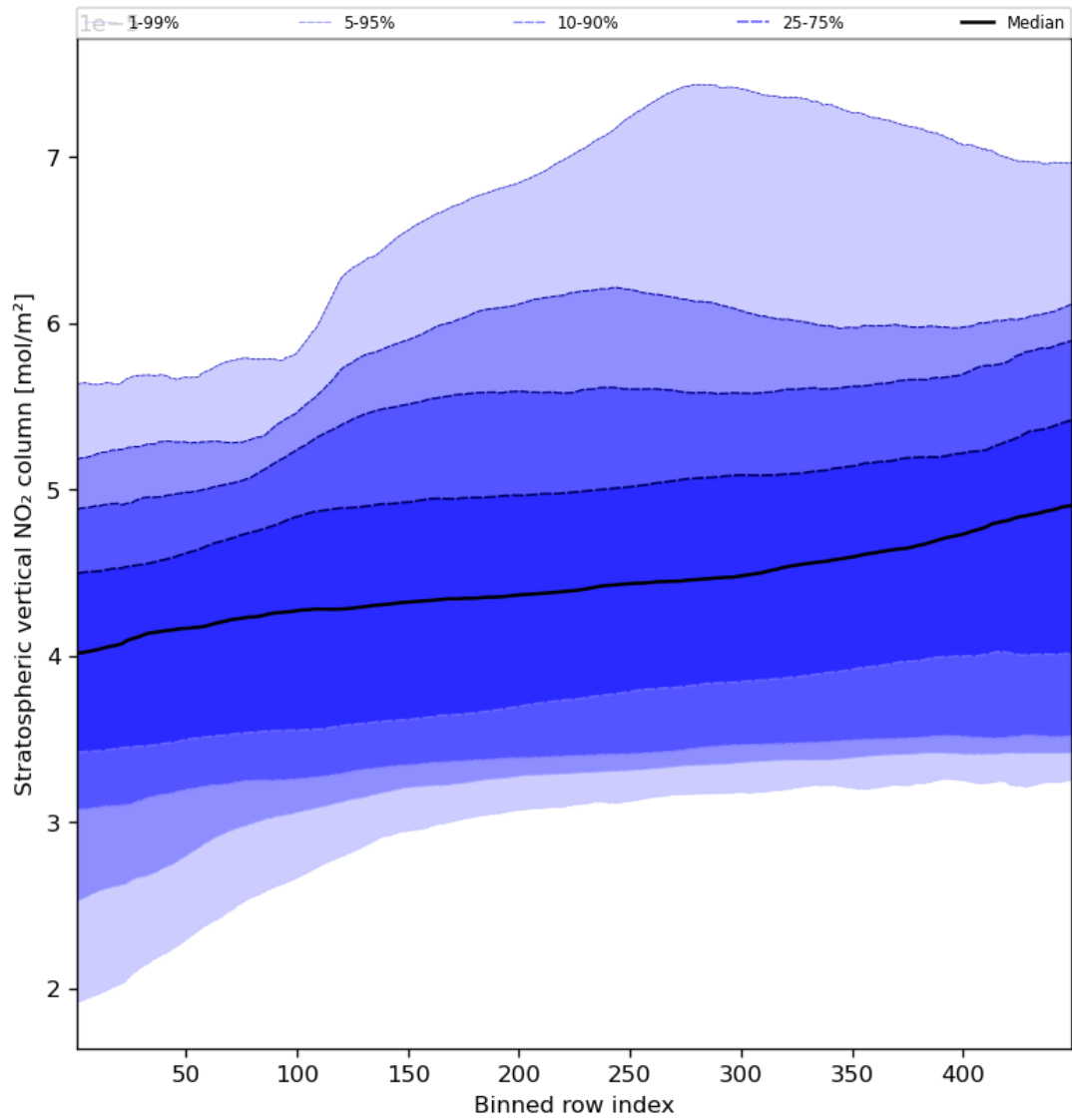
Figure 53: Along track statistics of “Stratospheric vertical NO 2 column” for 2024-04-15 to 2024-04-16
