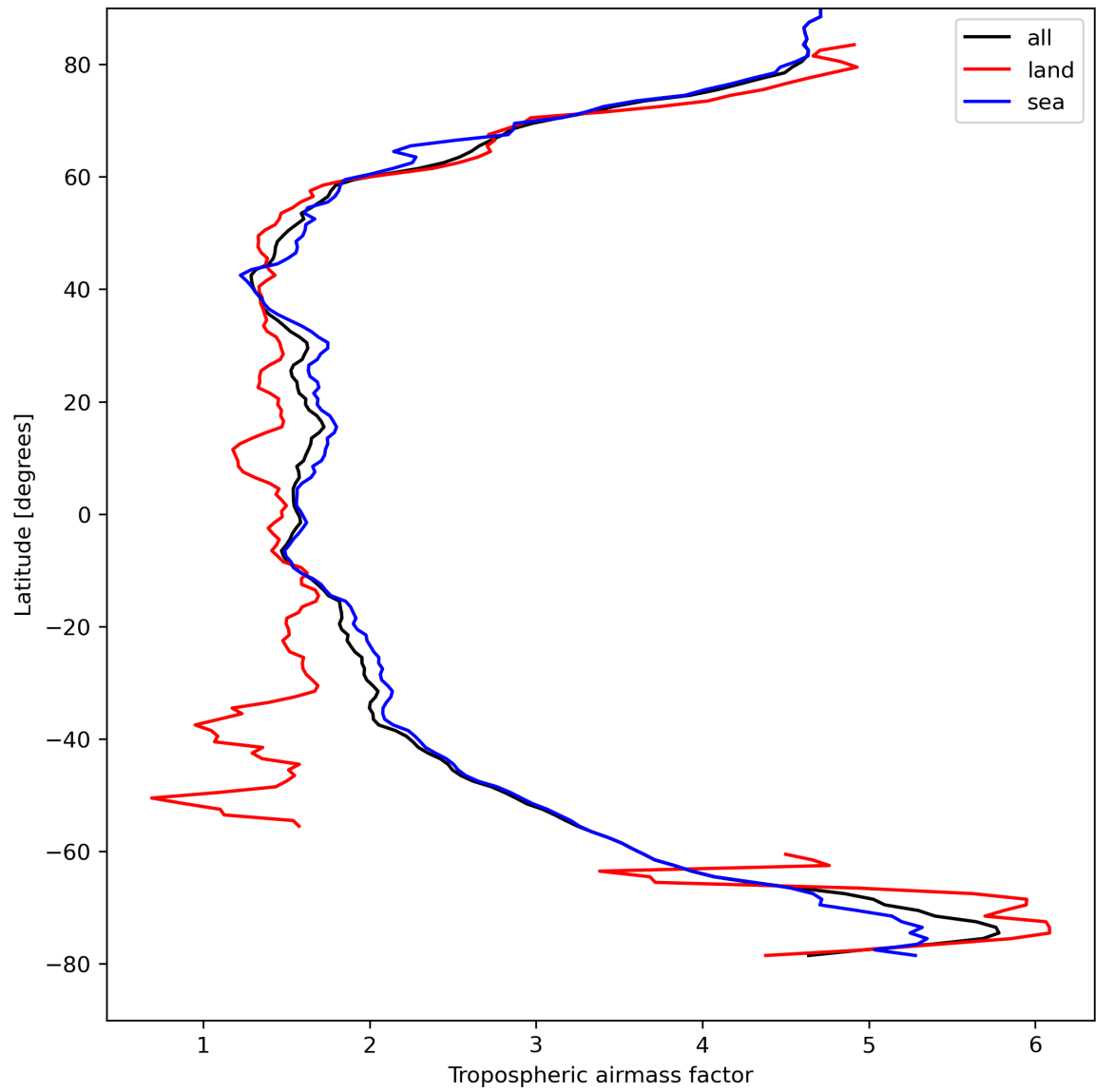
Figure 14: Zonal average of “Tropospheric airmass factor” for 2024-04-15 to 2024-04-16.
