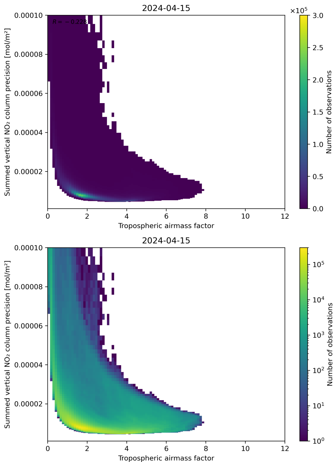
Figure 76: Scatter density plot of “Tropospheric air mass factor” against “Summed vertical NO 2 column precision” for 2024-04-15 to 2024-04-16.
