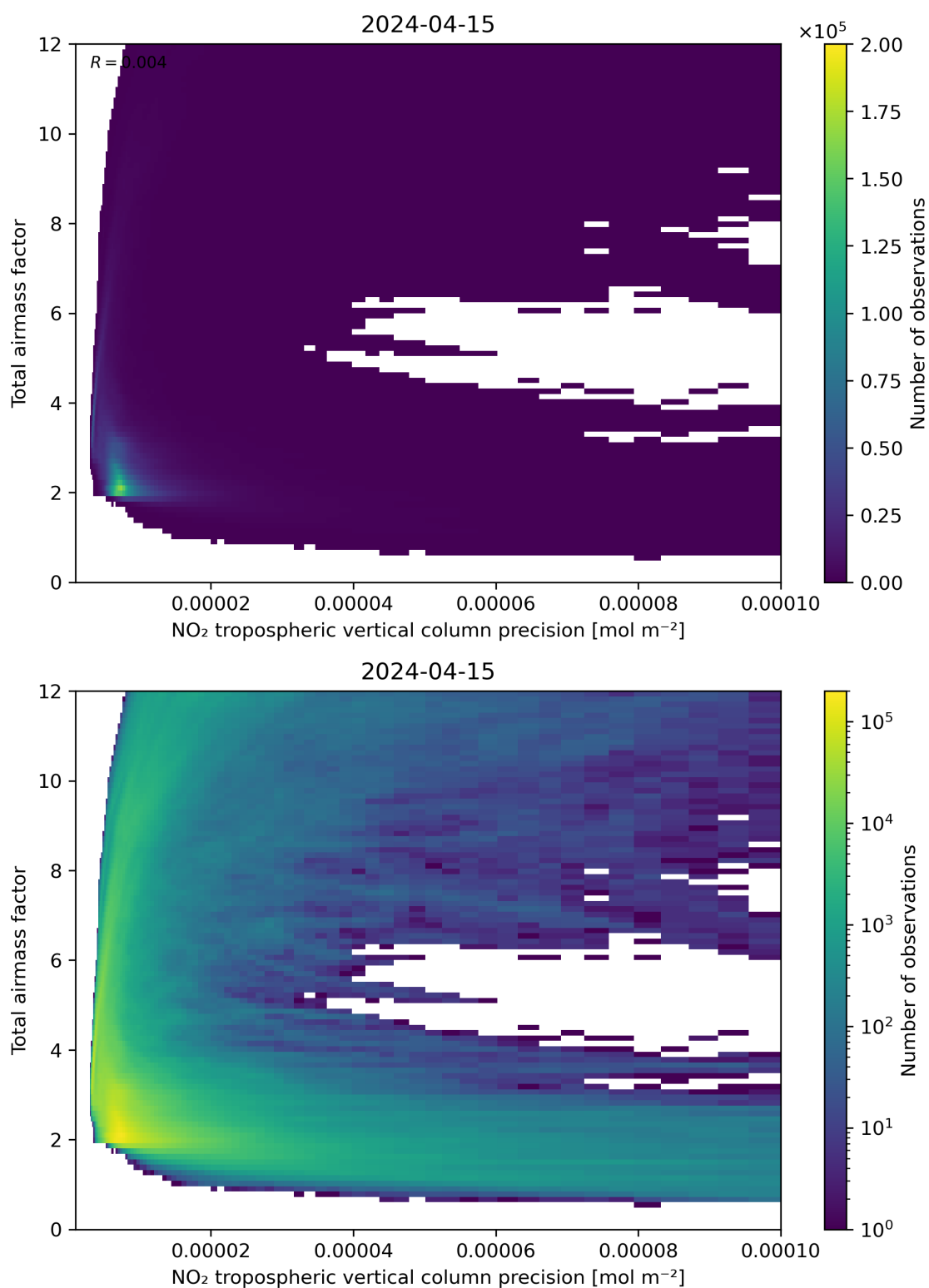
Figure 132: Scatter density plot of “NO 2 tropospheric vertical column precision” against “Total air mass factor” for 2024-04-15 to 2024-04-16.
