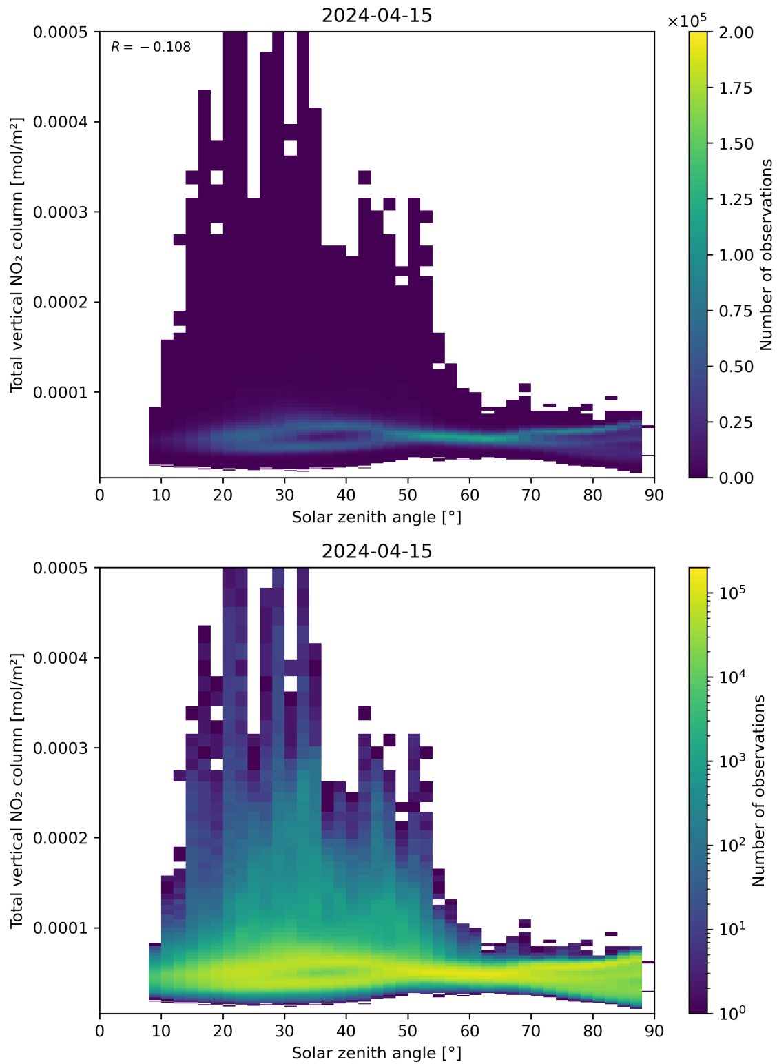
Figure 153: Scatter density plot of “Solar zenith angle” against “Total vertical NO 2 column” for 2024-04-15 to 2024-04-16.
