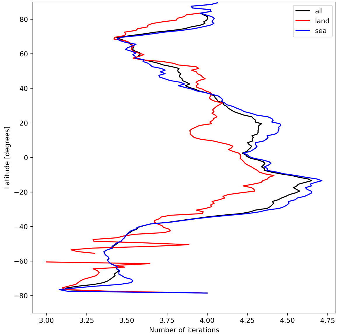
Figure 17: Zonal average of “Number of iterations” for 2024-04-15 to 2024-04-16.
