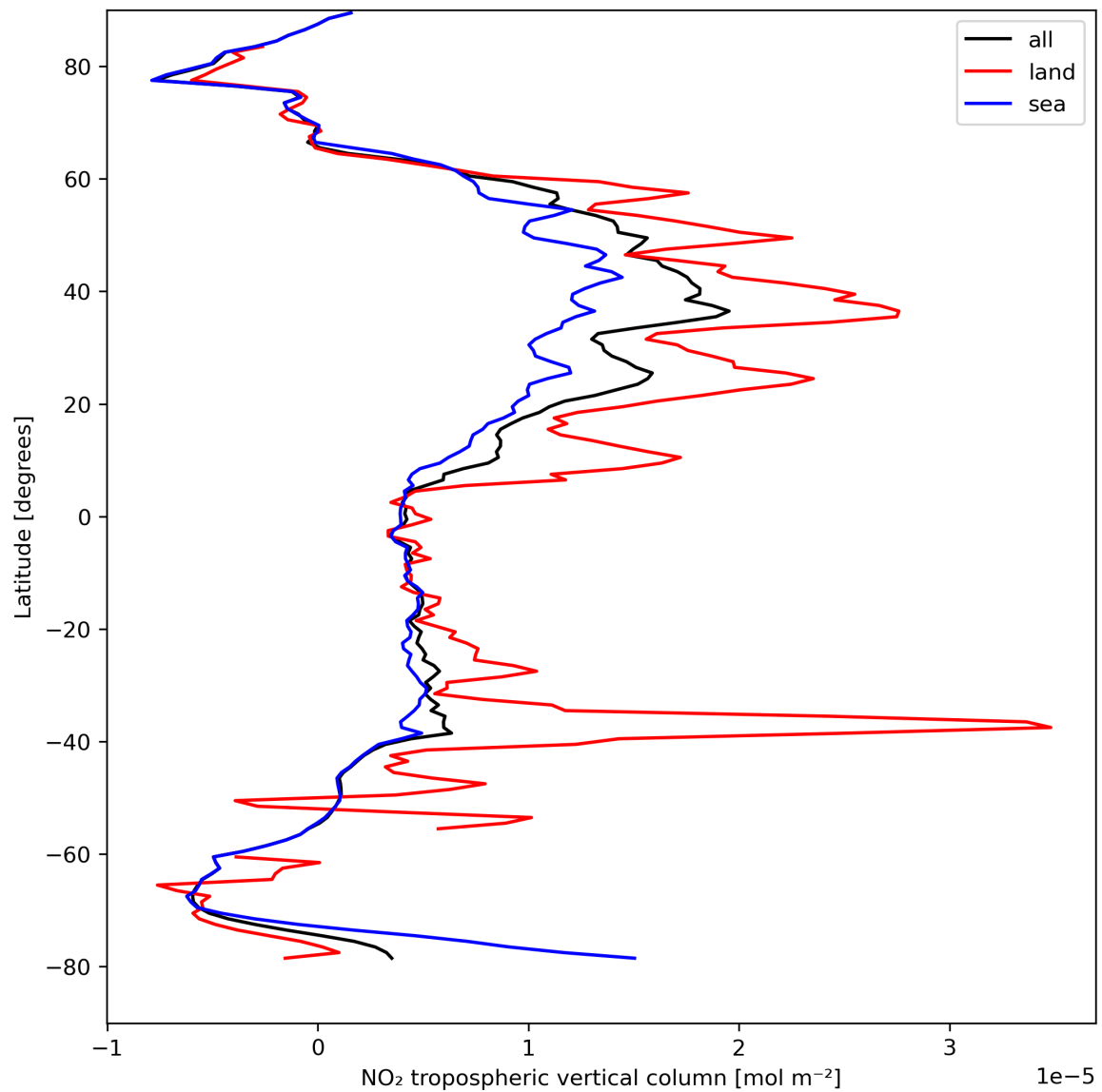
Figure 12: Zonal average of “NO 2 tropospheric vertical column” for 2024-04-15 to 2024-04-16.
