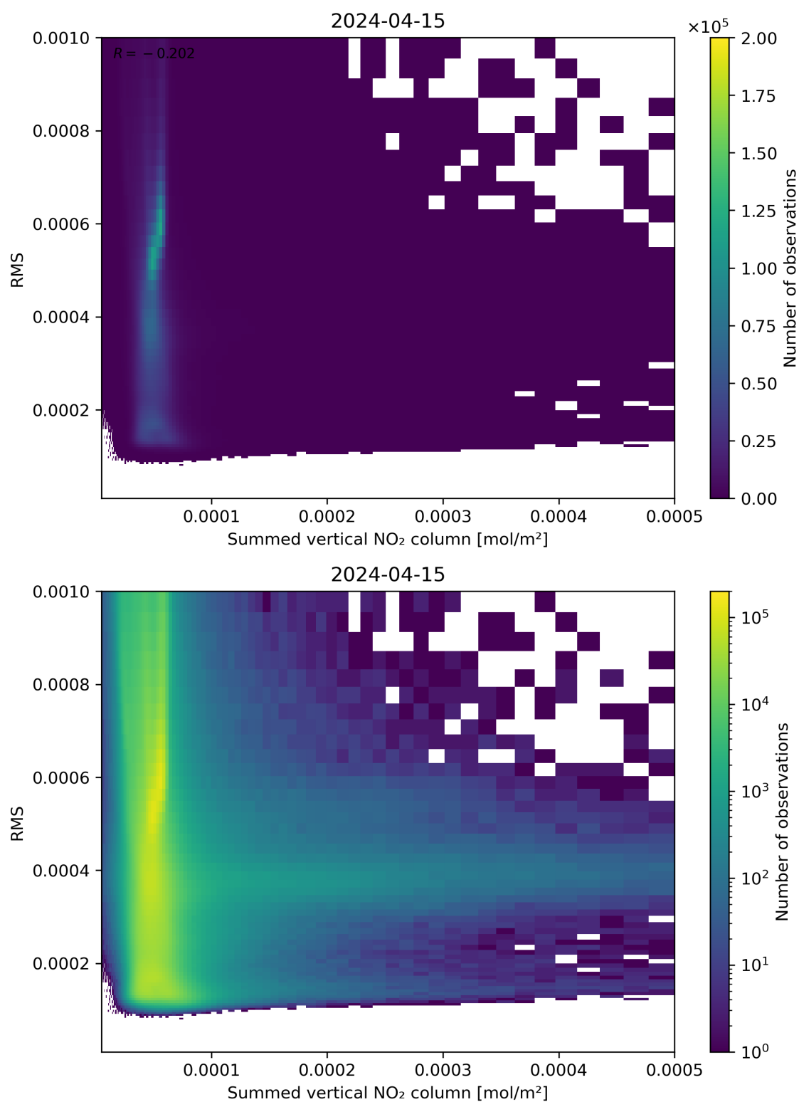
Figure 109: Scatter density plot of “Summed vertical NO 2 column” against “RMS” for 2024-04-15 to 2024-04-16.
