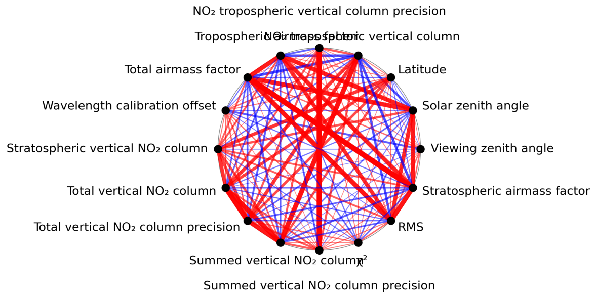
Figure 1: Map of correlation graph for 2024-04-15 to 2024-04-16.
