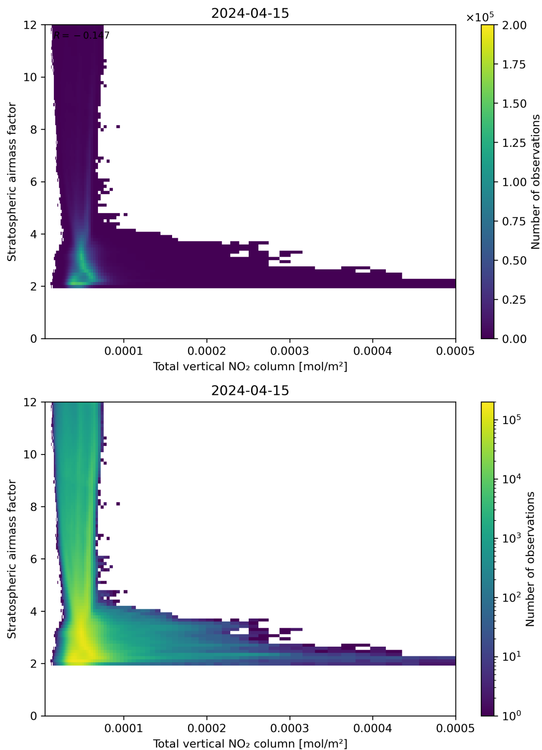
Figure 110: Scatter density plot of “Total vertical NO 2 column” against “Stratospheric airmass factor” for 2024-04-15 to 2024-04-16.
