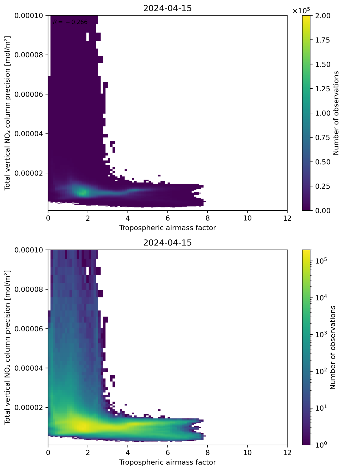
Figure 78: Scatter density plot of “Tropospheric air mass factor” against “Total vertical NO 2 column precision” for 2024-04-15 to 2024-04-16.
