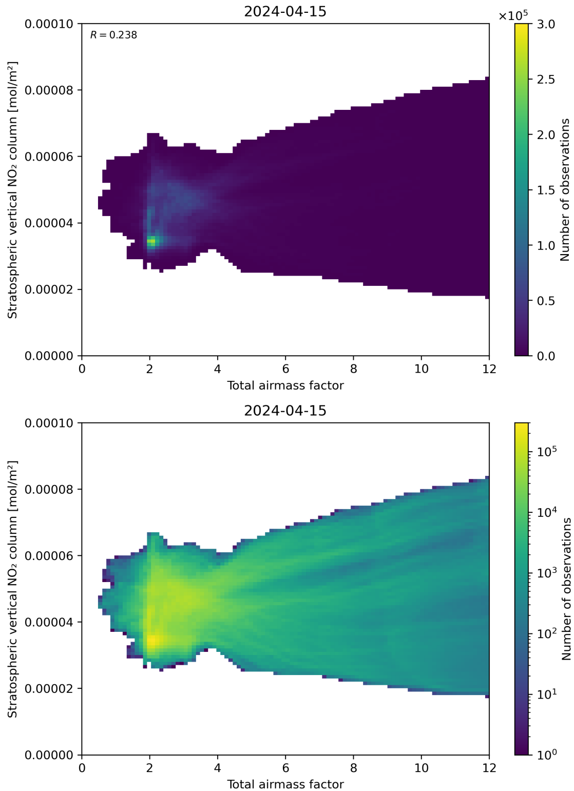
Figure 64: Scatter density plot of “Total airmass factor” against “Stratospheric vertical NO 2 column” for 2024-04-15 to 2024-04-16.
