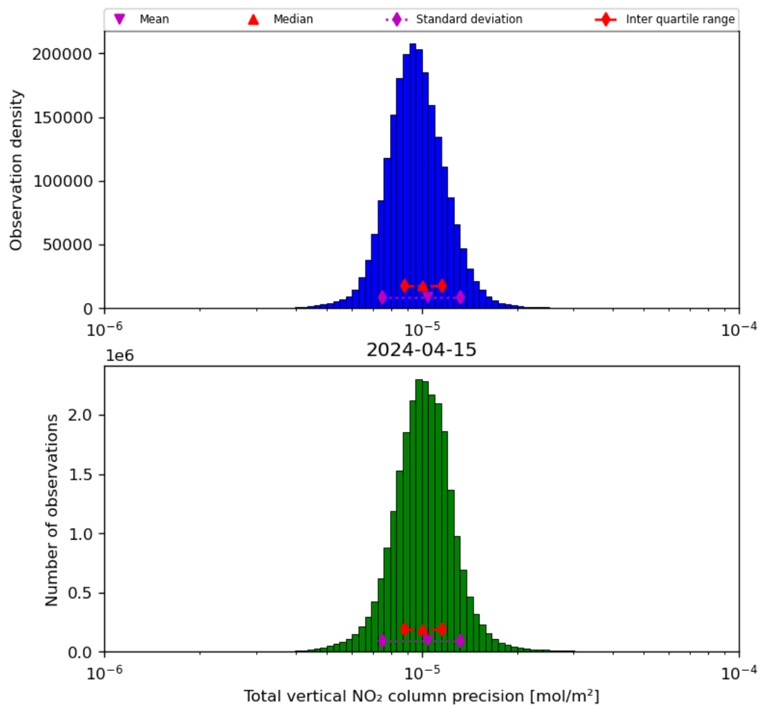
Figure 39: Histogram of “Total vertical NO 2 column precision” for 2024-04-15 to 2024-04-16
