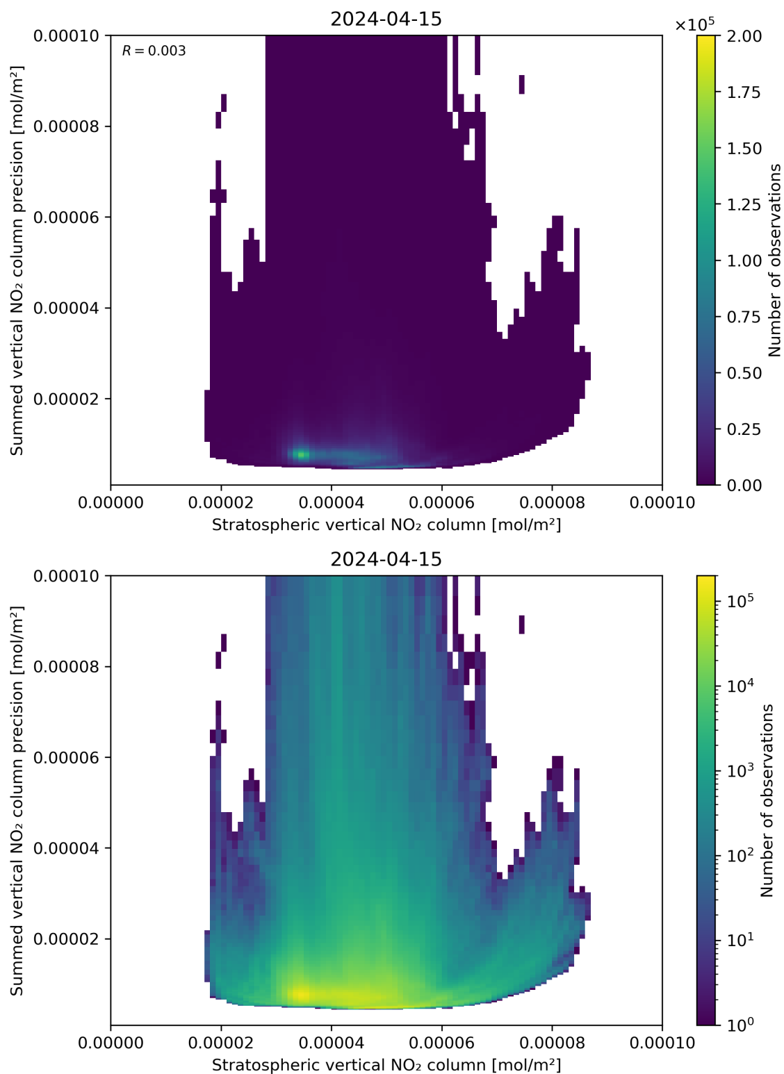
Figure 99: Scatter density plot of “Stratospheric vertical NO 2 column” against “Summed vertical NO 2 column precision” for 2024-04-15 to 2024-04-16.
