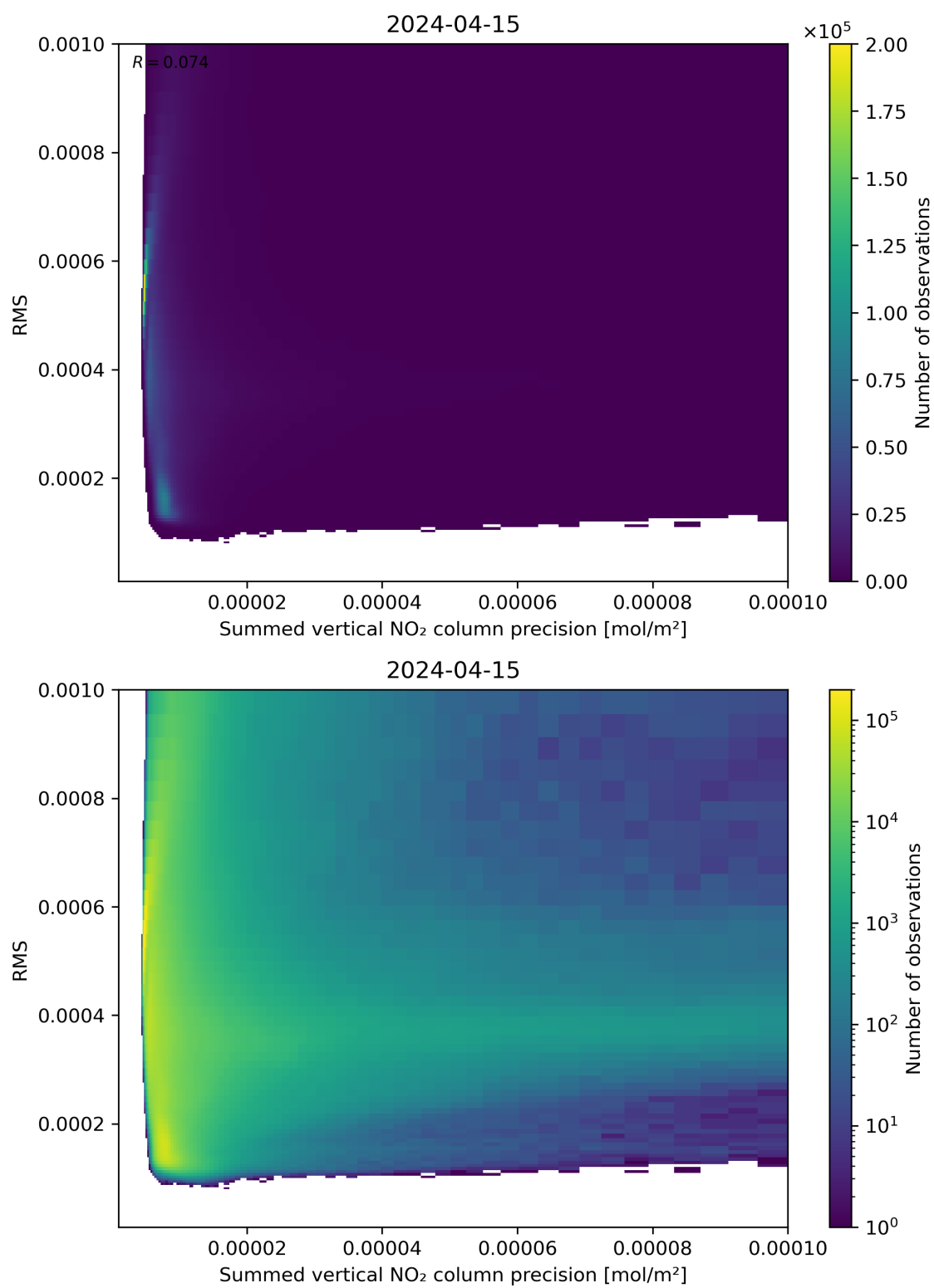
Figure 108: Scatter density plot of “Summed vertical NO 2 column precision” against “RMS” for 2024-04-15 to 2024-04-16.
