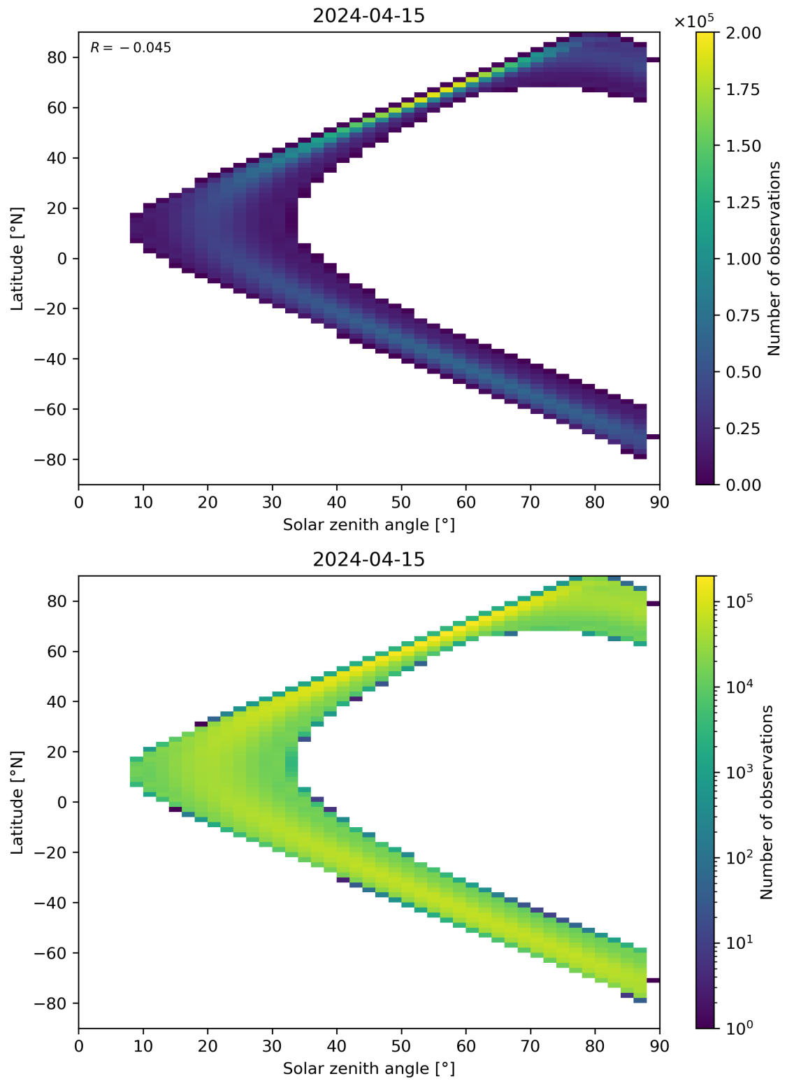
Figure 149: Scatter density plot of “Solar zenith angle” against “Latitude” for 2024-04-15 to 2024-04-16.
