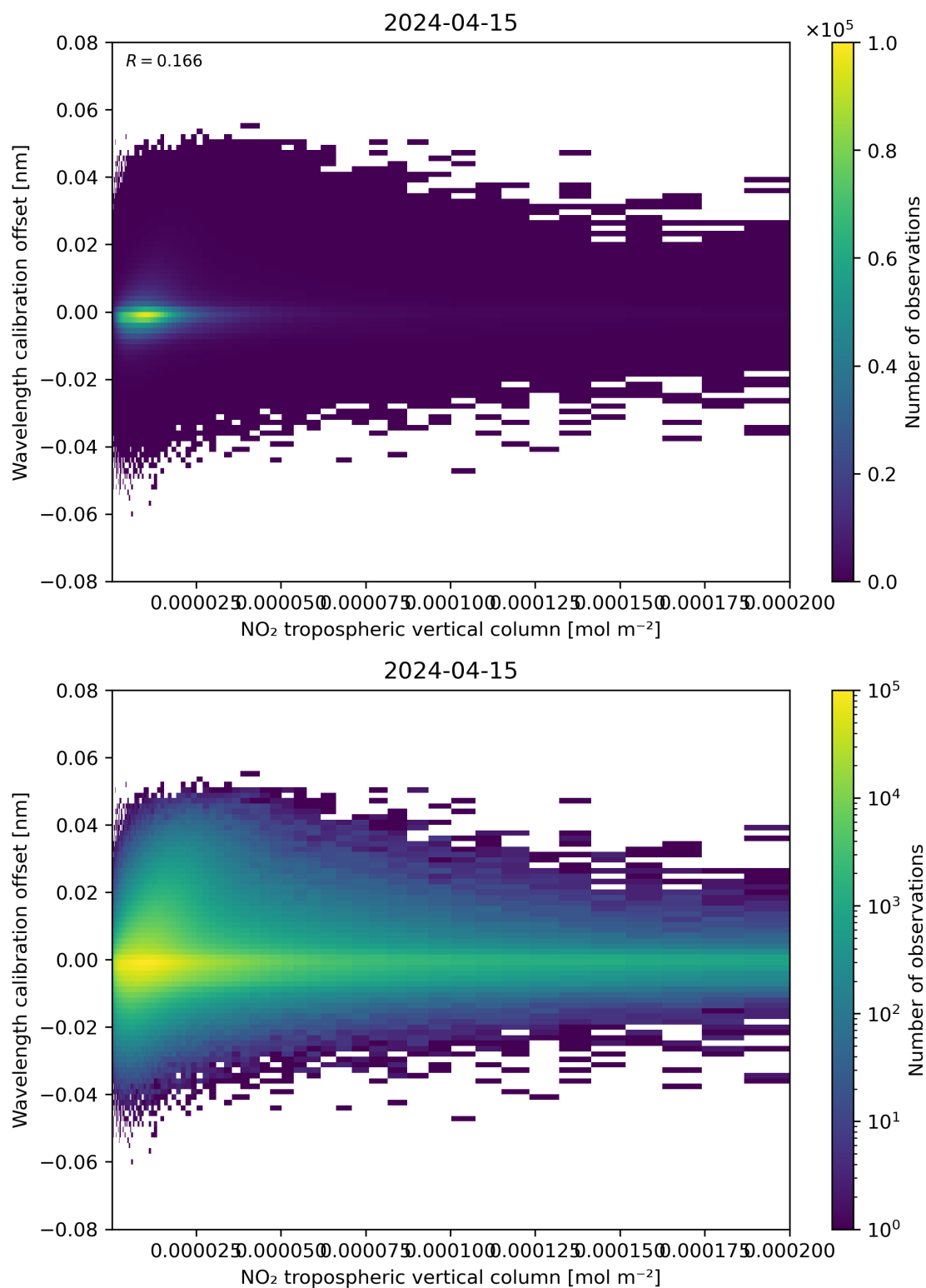
Figure 143: Scatter density plot of “NO 2 tropospheric vertical column” against “Wavelength calibration offset” for 2024-04-15 to 2024-04-16.
