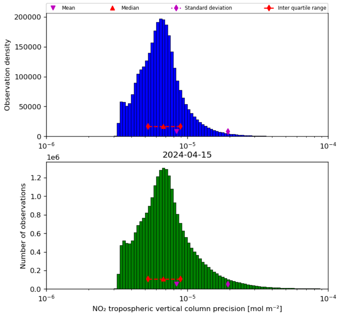
Figure 30: Histogram of “NO 2 tropospheric vertical column precision” for 2024-04-15 to 2024-04-16
