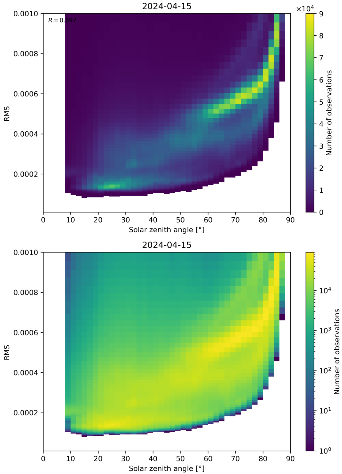
Figure 157: Scatter density plot of “Solar zenith angle” against “RMS” for 2024-04-15 to 2024-04-16.
