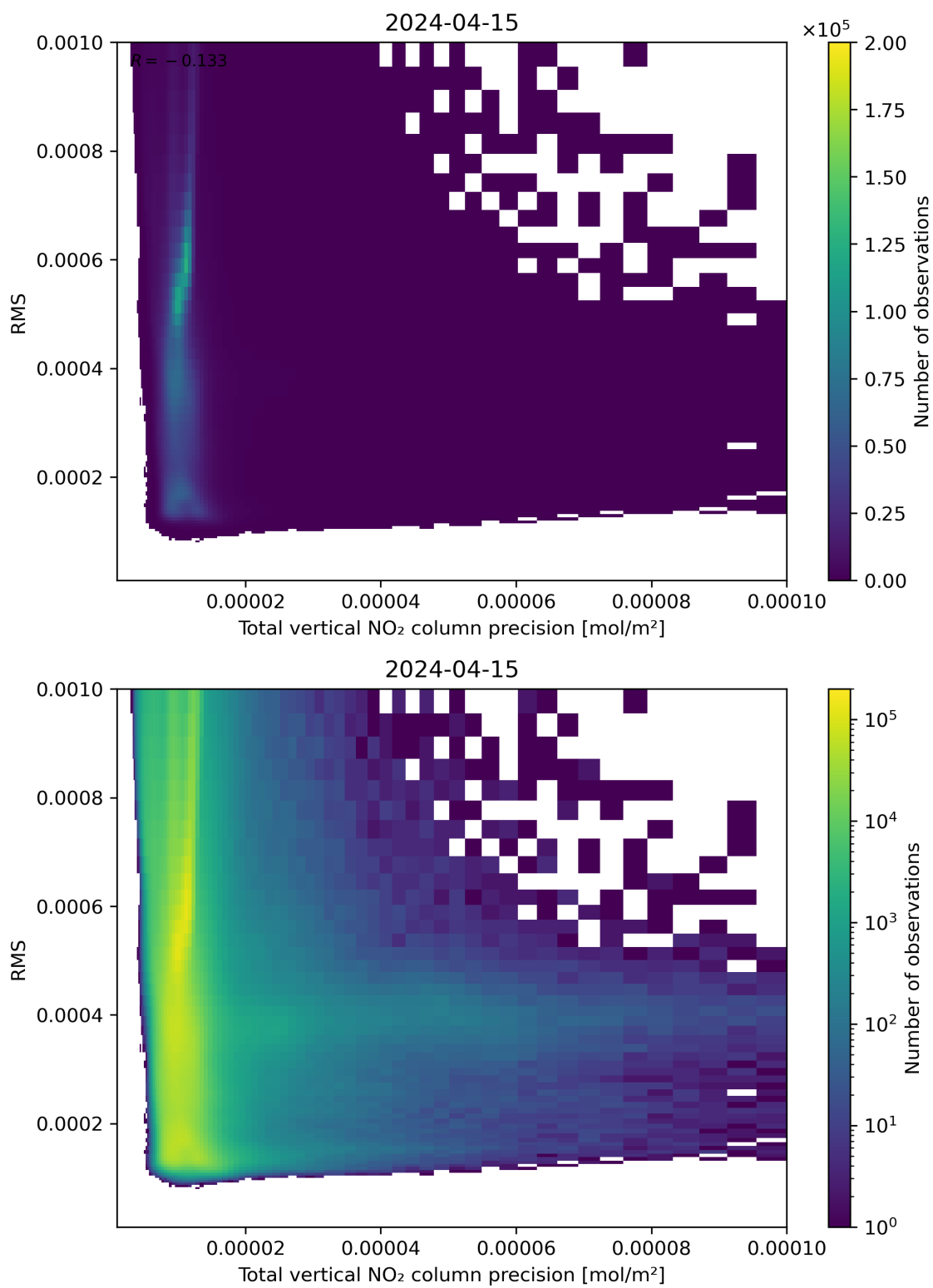
Figure 119: Scatter density plot of “Total vertical NO 2 column precision” against “RMS” for 2024-04-15 to 2024-04-16.
