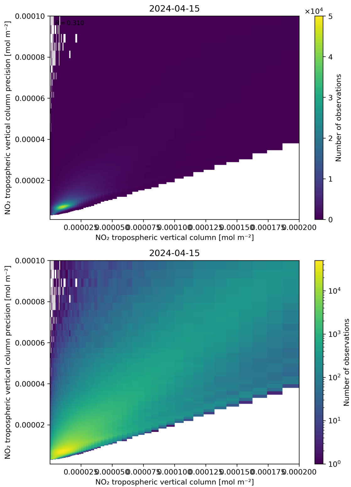
Figure 130: Scatter density plot of “NO 2 tropospheric vertical column” against “NO 2 tropospheric vertical column precision” for 2024-04-15 to 2024-04-16.
