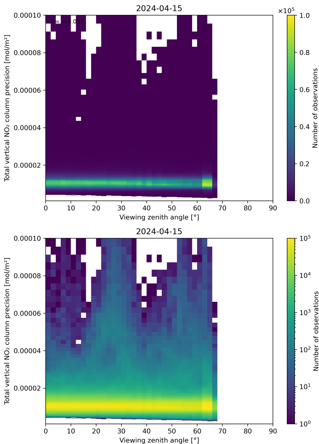
Figure 168: Scatter density plot of “Viewing zenith angle” against “Total vertical NO 2 column precision” for 2024-04-15 to 2024-04-16.
