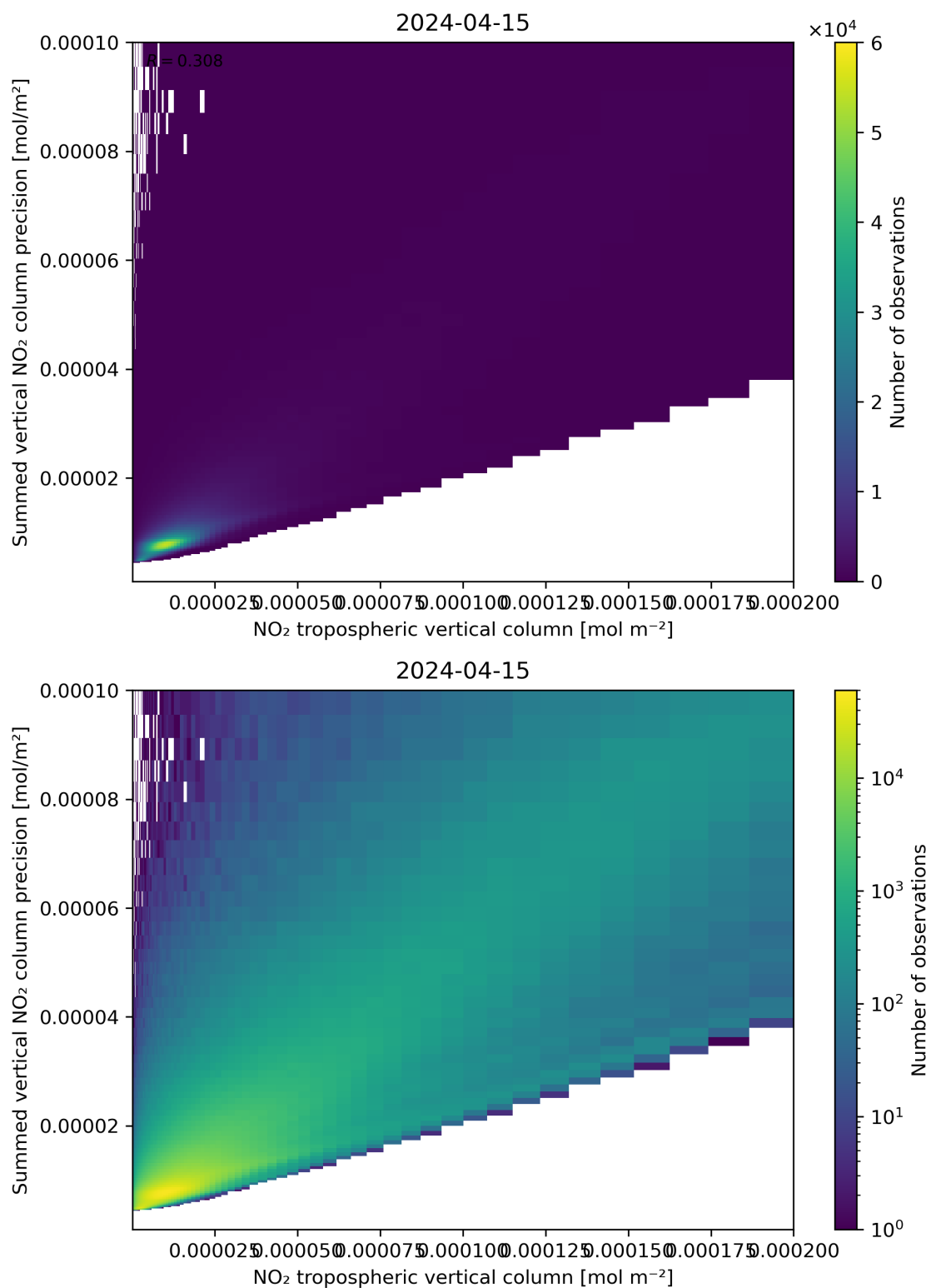
Figure 127: Scatter density plot of “NO 2 tropospheric vertical column” against “Summed vertical NO 2 column precision” for 2024-04-15 to 2024-04-16.
