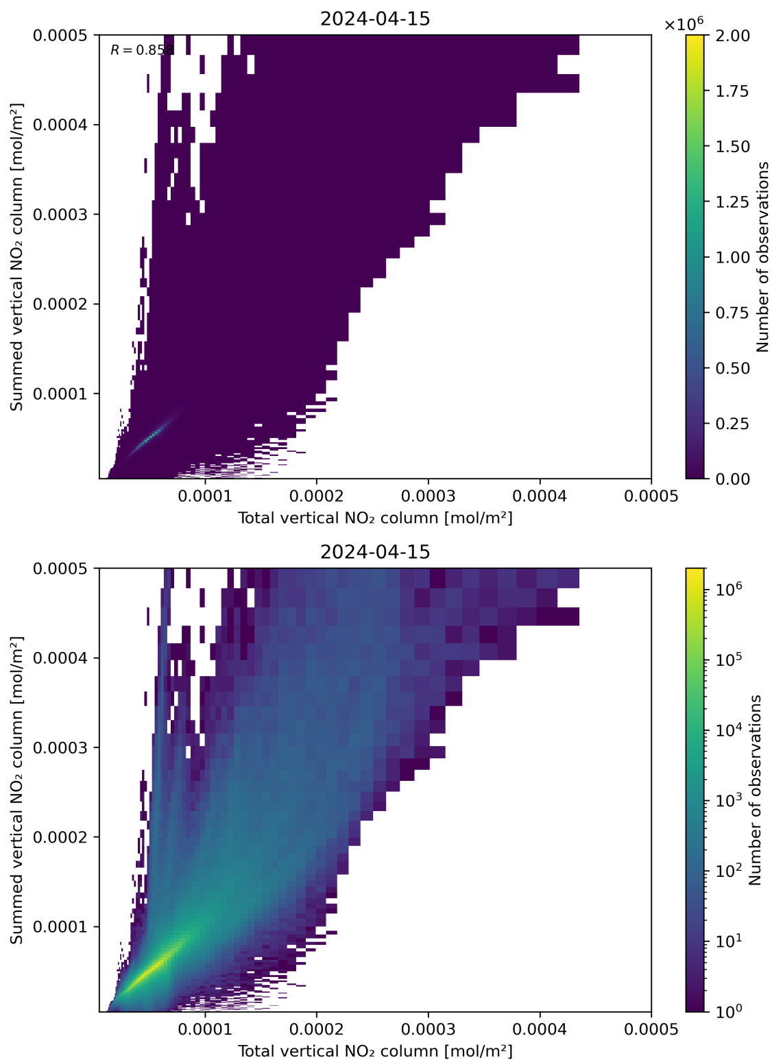
Figure 112: Scatter density plot of “Total vertical NO 2 column” against “Summed vertical NO 2 column” for 2024-04-15 to 2024-04-16.
