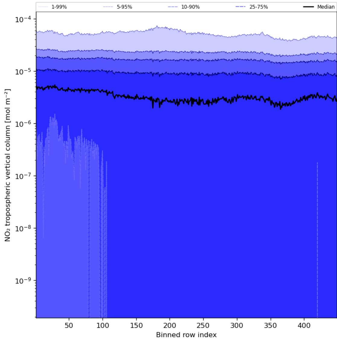
Figure 46: Along track statistics of “NO 2 tropospheric vertical column” for 2024-04-15 to 2024-04-16
