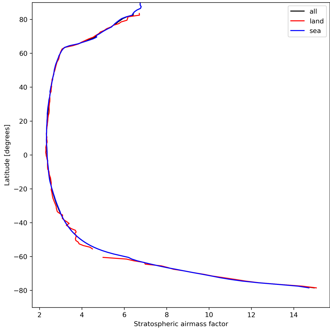
Figure 27: Zonal average of “Stratospheric air mass factor” for 2024-04-15 to 2024-04-16.
