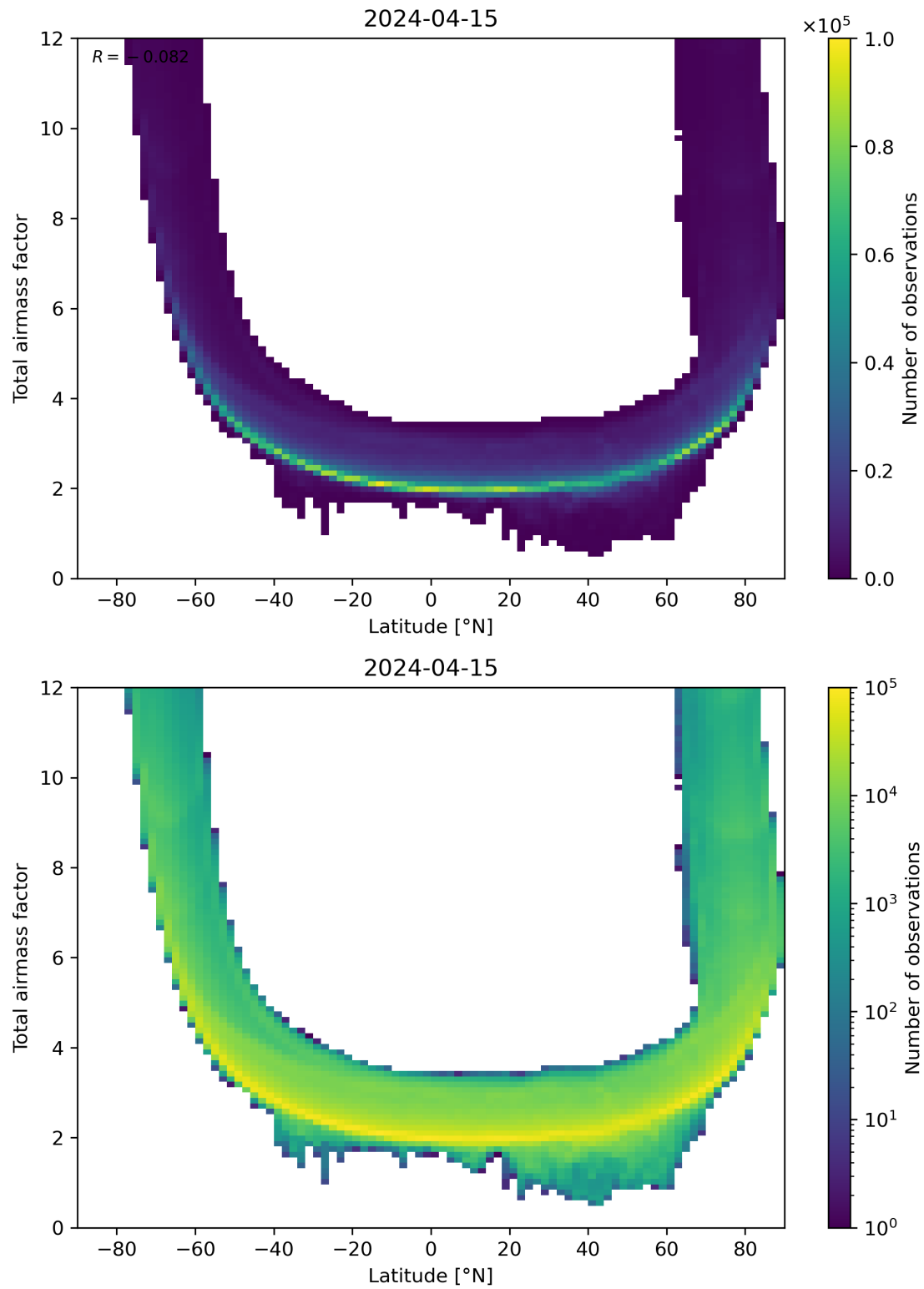
Figure 84: Scatter density plot of “Latitude” against “Total airmass factor” for 2024-04-15 to 2024-04-16.
