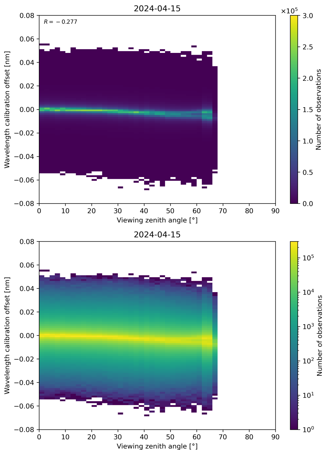
Figure 173: Scatter density plot of “Viewing zenith angle” against “Wavelength calibration offset” for 2024-04-15 to 2024-04-16.
