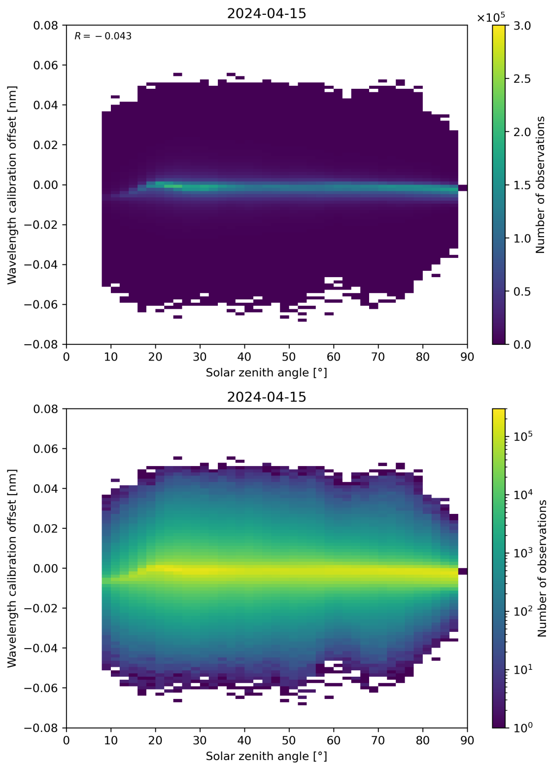
Figure 158: Scatter density plot of “Solar zenith angle” against “Wavelength calibration offset” for 2024-04-15 to 2024-04-16.
