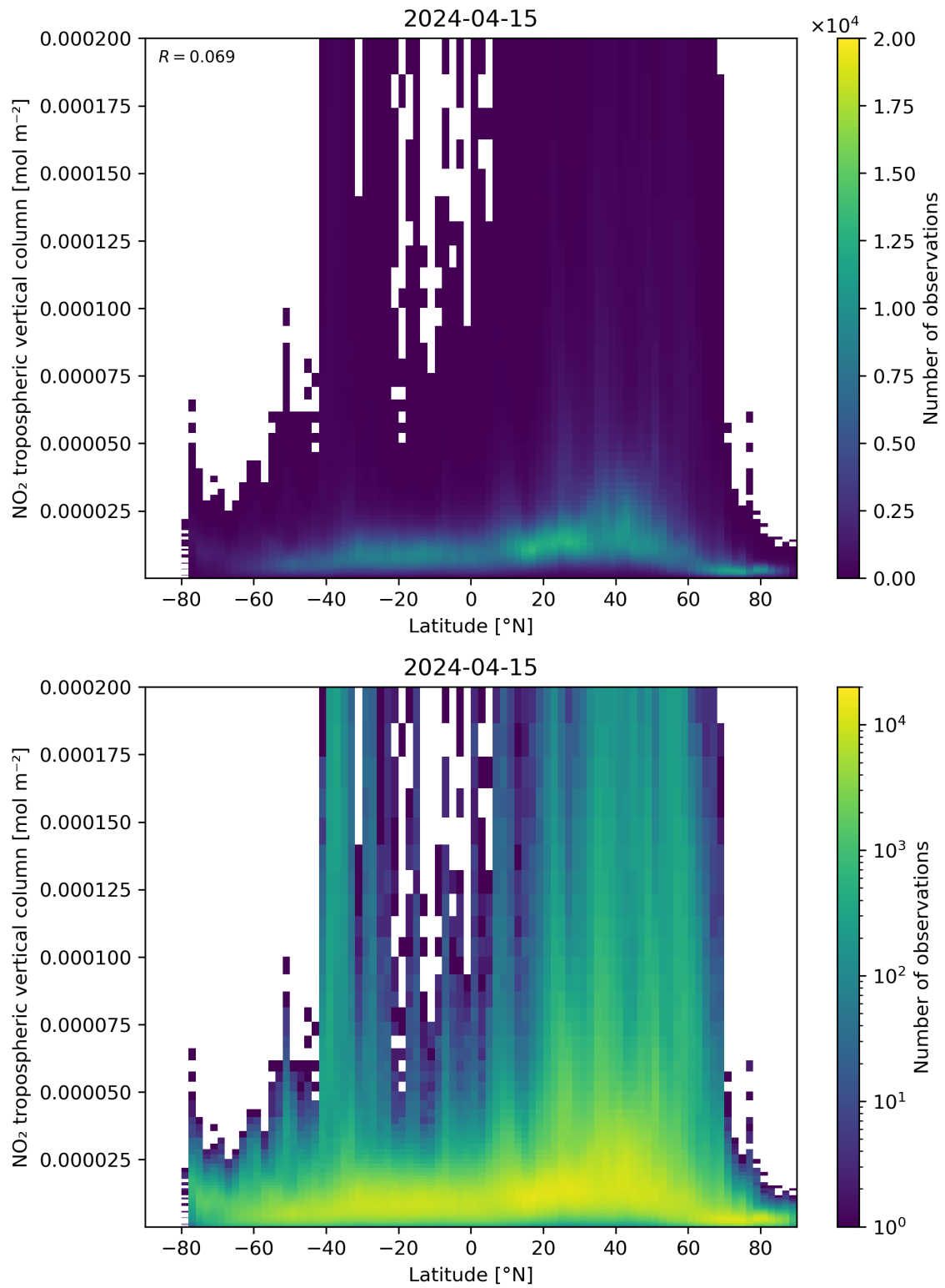
Figure 92: Scatter density plot of “Latitude” against “NO 2 tropospheric vertical column” for 2024-04-15 to 2024-04-16.
