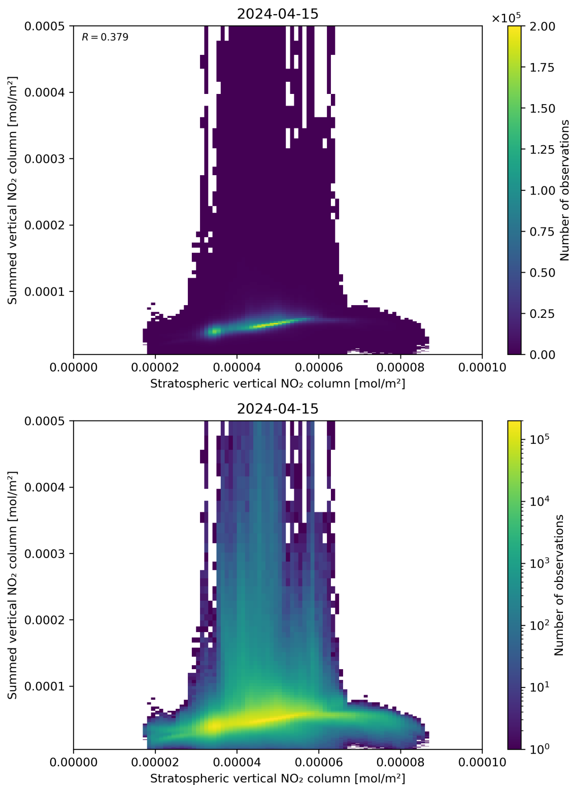
Figure 98: Scatter density plot of “Stratospheric vertical NO 2 column” against “Summed vertical NO 2 column” for 2024-04-15 to 2024-04-16.
