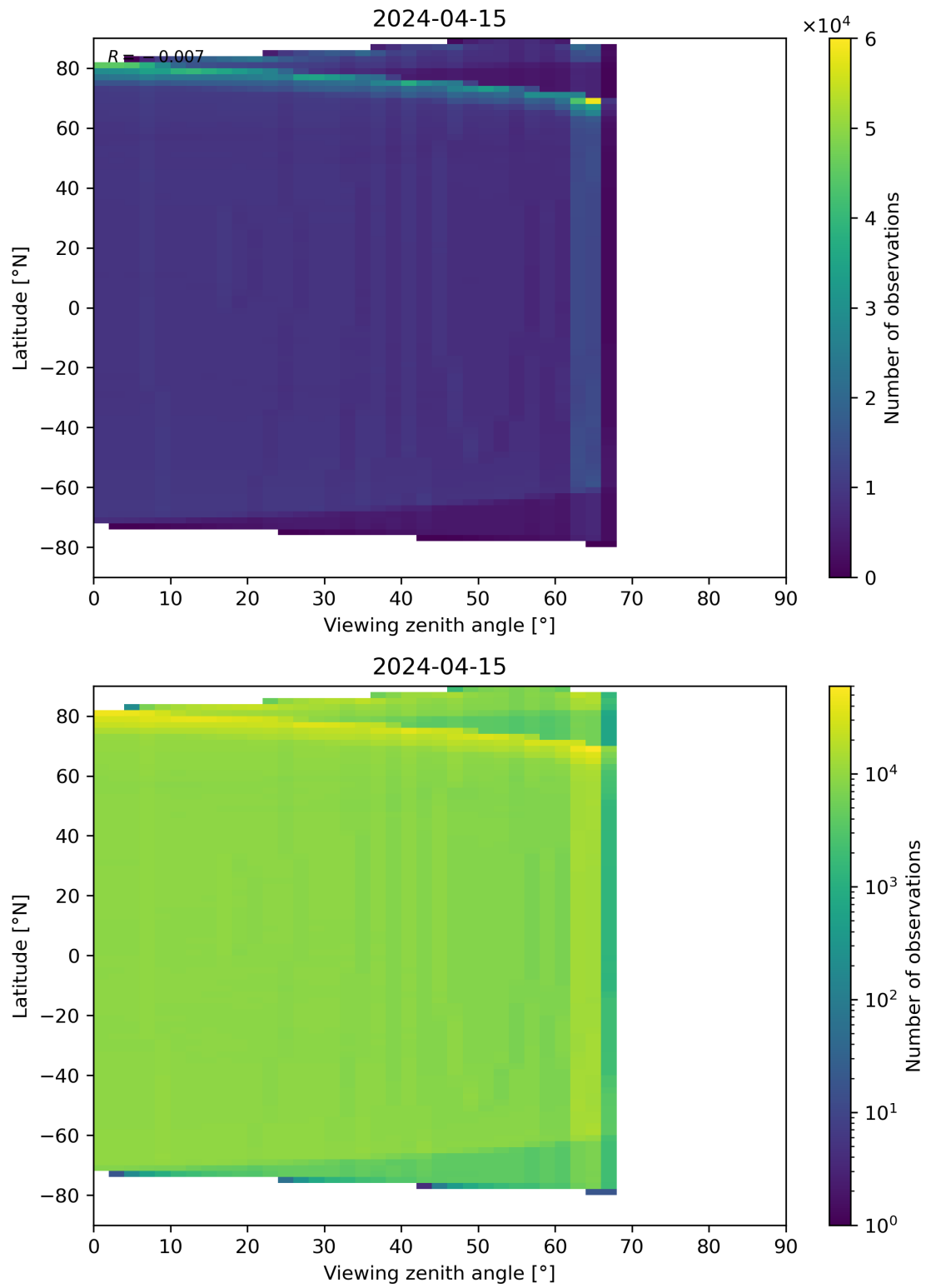
Figure 163: Scatter density plot of “Viewing zenith angle” against “Latitude” for 2024-04-15 to 2024-04-16.
