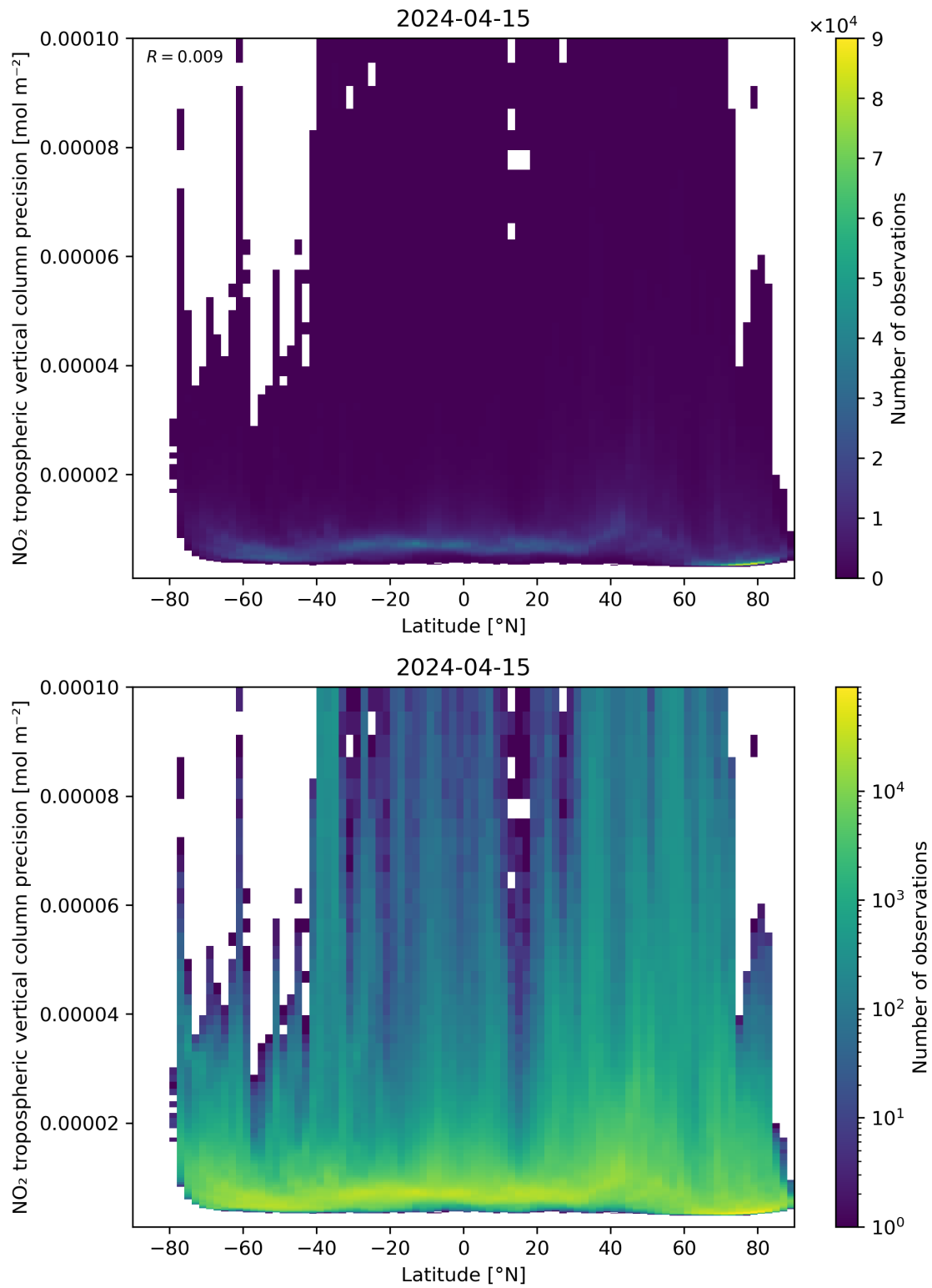
Figure 93: Scatter density plot of “Latitude” against “NO 2 tropospheric vertical column precision” for 2024-04-15 to 2024-04-16.
