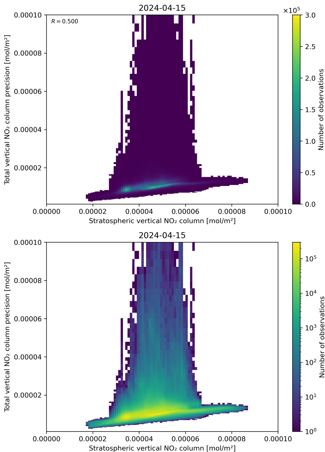
Figure 101: Scatter density plot of “Stratospheric vertical NO 2 column” against “Total vertical NO 2 column precision” for 2024-04-15 to 2024-04-16.
