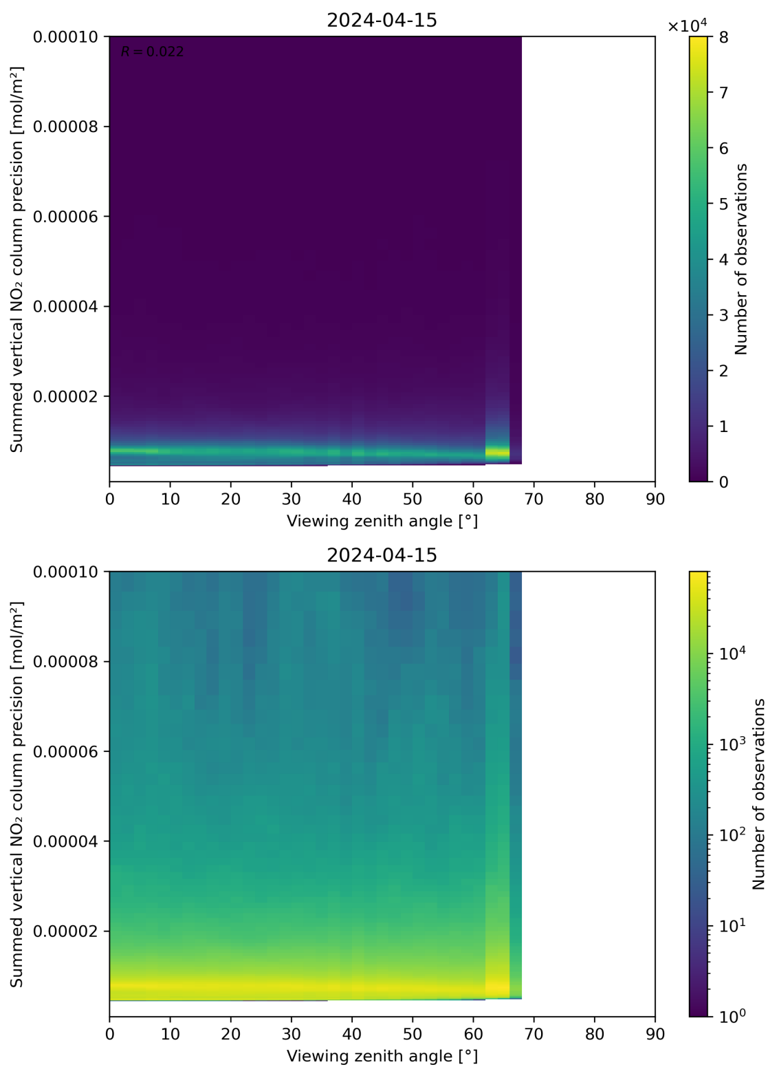
Figure 166: Scatter density plot of “Viewing zenith angle” against “Summed vertical NO 2 column precision” for 2024-04-15 to 2024-04-16.
