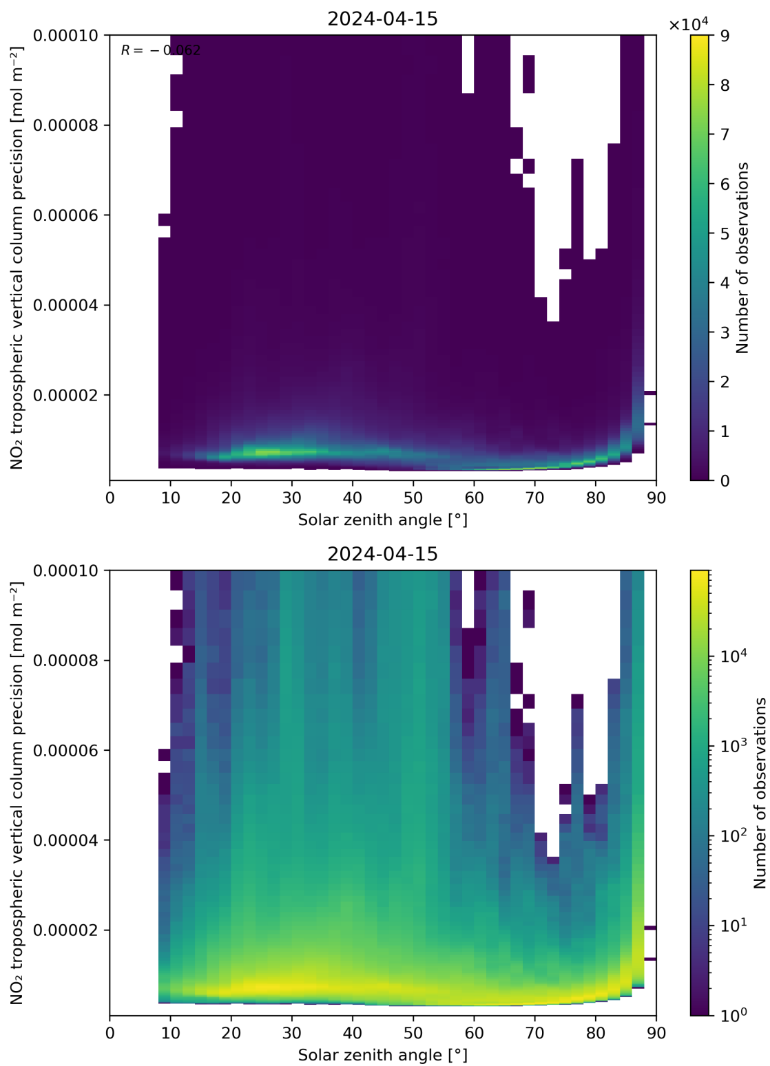
Figure 156: Scatter density plot of “Solar zenith angle” against “NO 2 tropospheric vertical column precision” for 2024-04-15 to 2024-04-16.
