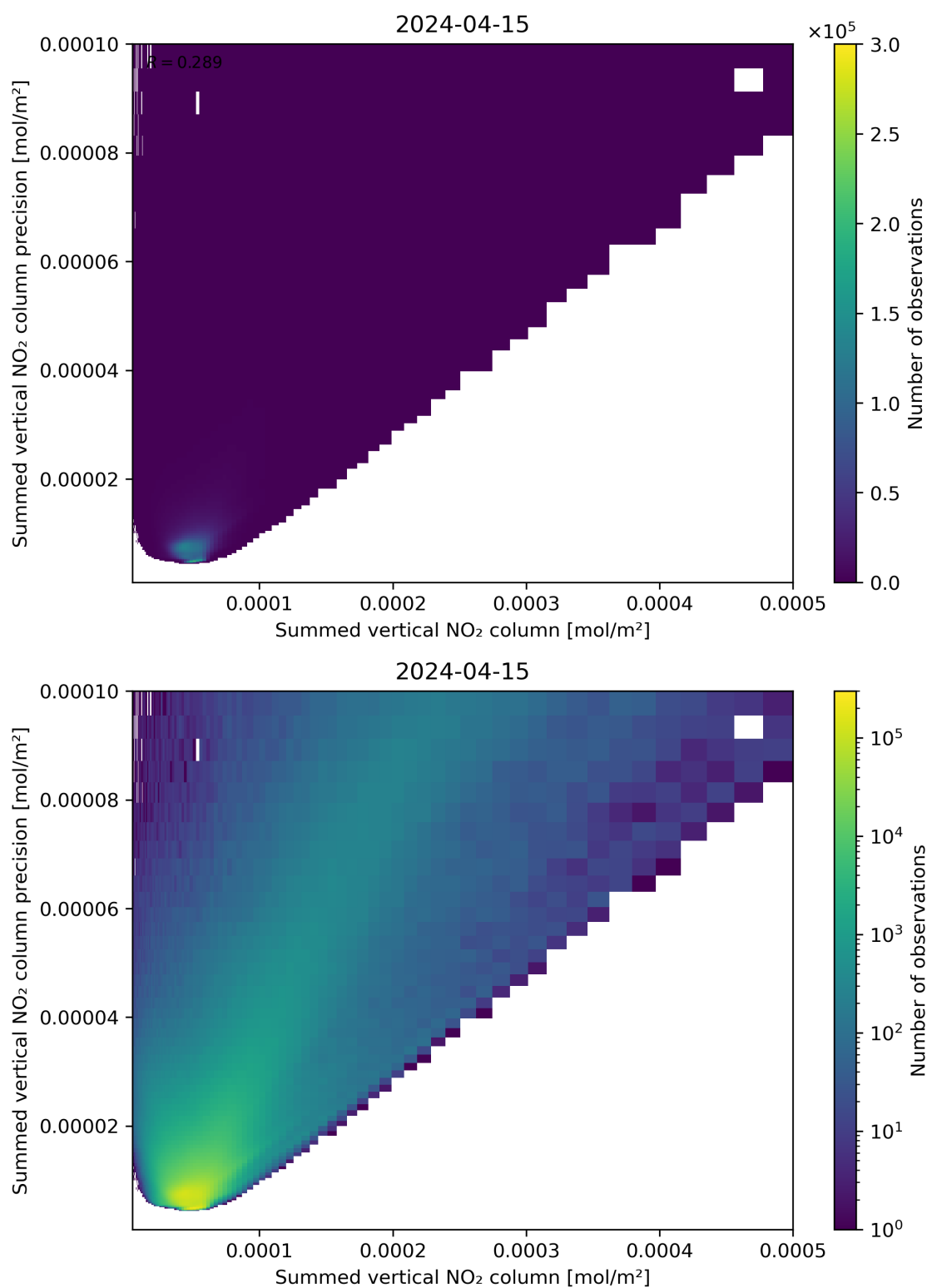
Figure 105: Scatter density plot of “Summed vertical NO 2 column” against “Summed vertical NO 2 column precision” for 2024-04-15 to 2024-04-16.
