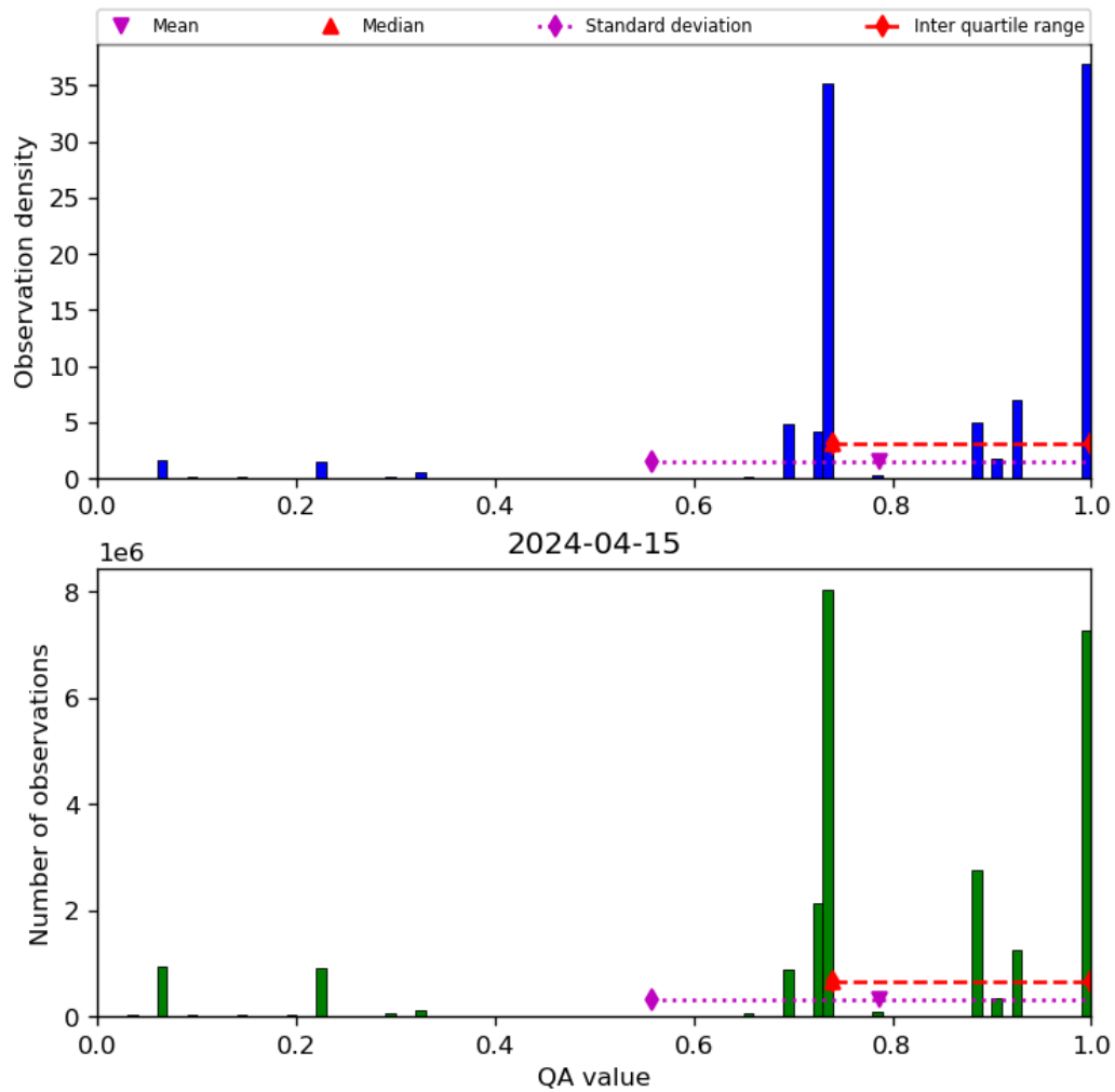
Figure 28: Histogram of “QA value” for 2024-04-15 to 2024-04-16
