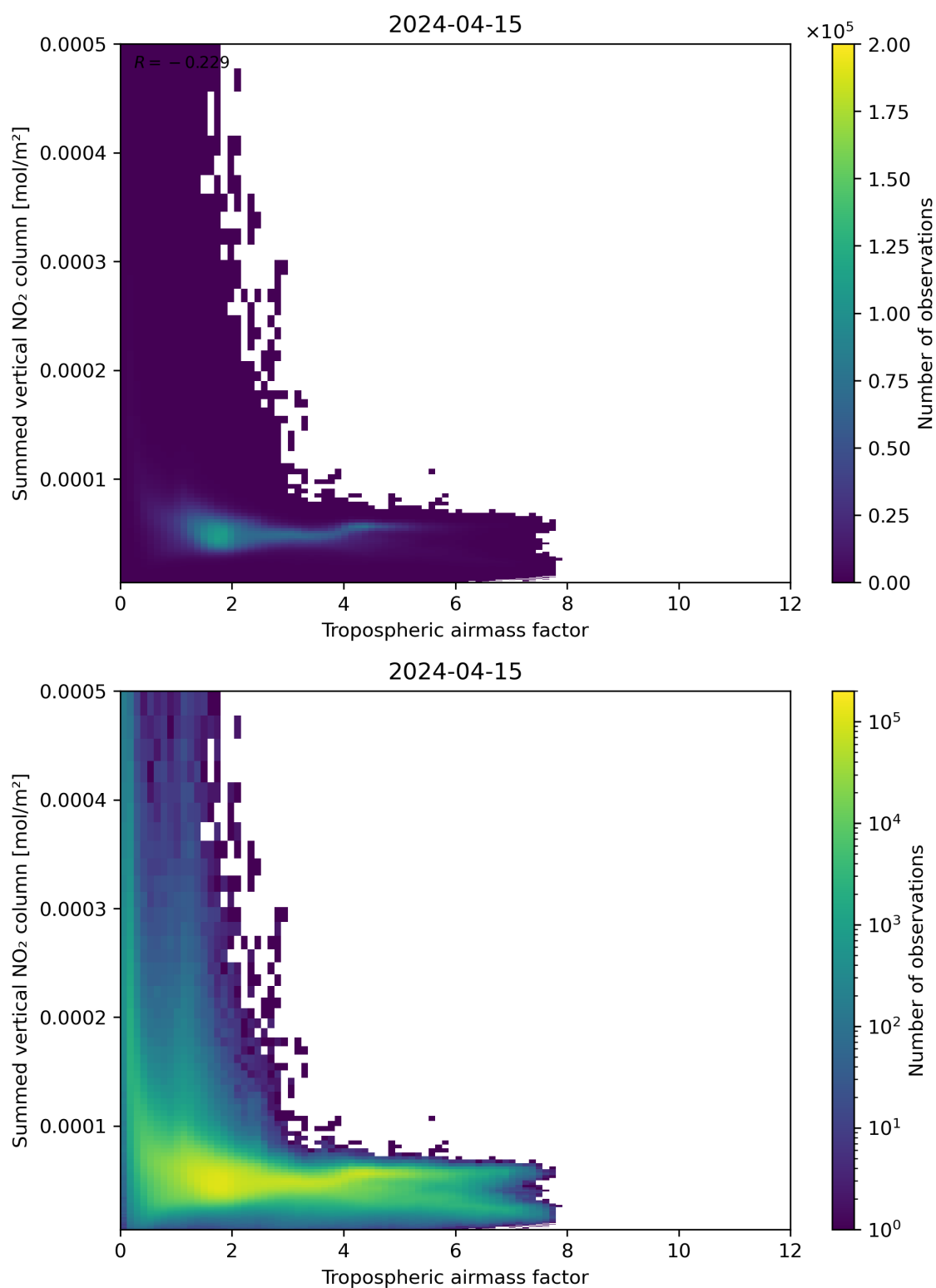
Figure 75: Scatter density plot of “Tropospheric airmass factor” against “Summed vertical NO 2 column” for 2024-04-15 to 2024-04-16.
