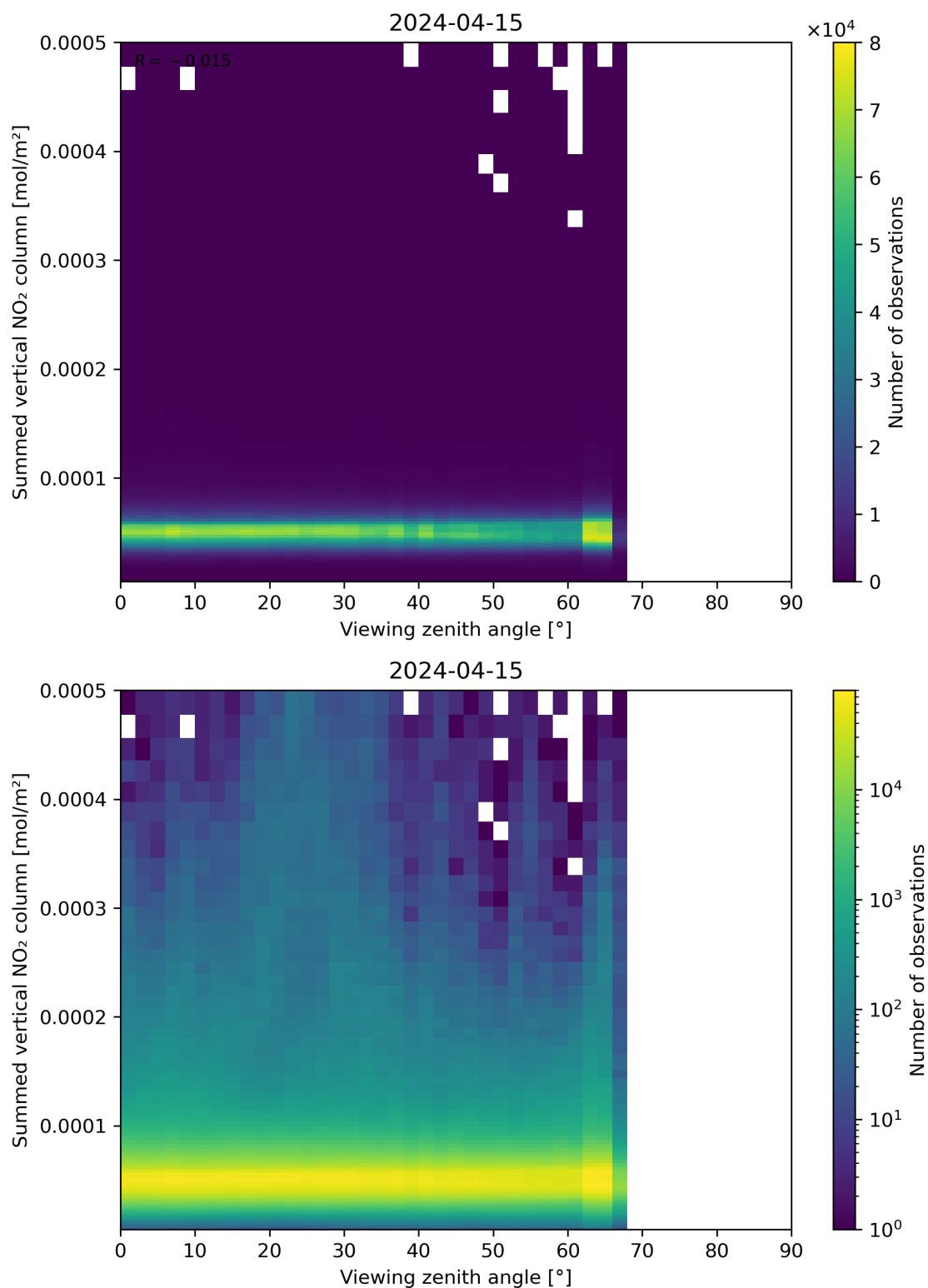
Figure 165: Scatter density plot of “Viewing zenith angle” against “Summed vertical NO 2 column” for 2024-04-15 to 2024-04-16.
