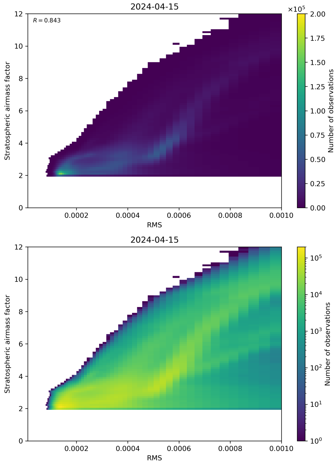
Figure 144: Scatter density plot of “RMS” against “Stratospheric airmass factor” for 2024-04-15 to 2024-04-16.
