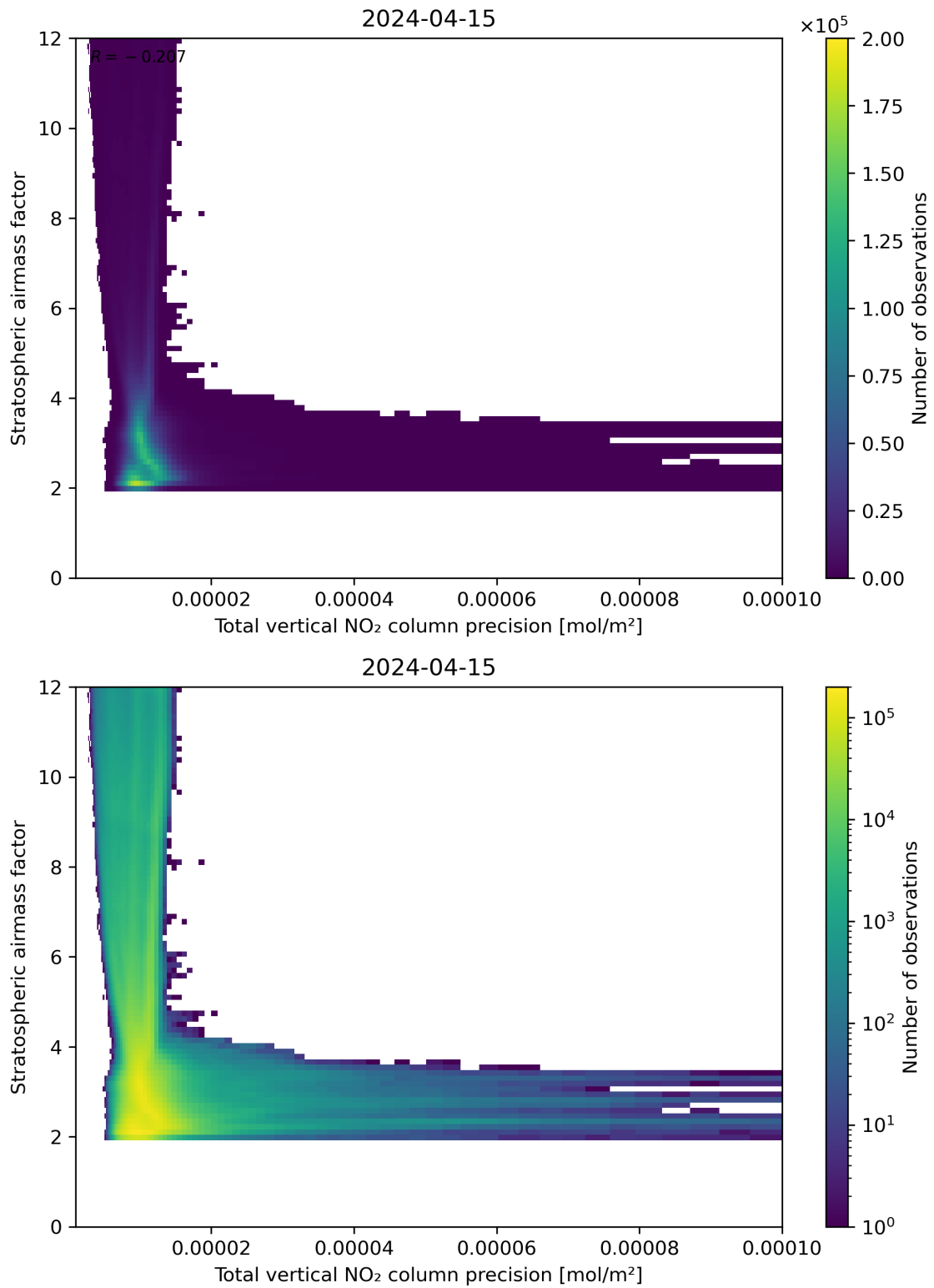
Figure 115: Scatter density plot of “Total vertical NO 2 column precision” against “Stratospheric air mass factor” for 2024-04-15 to 2024-04-16.
