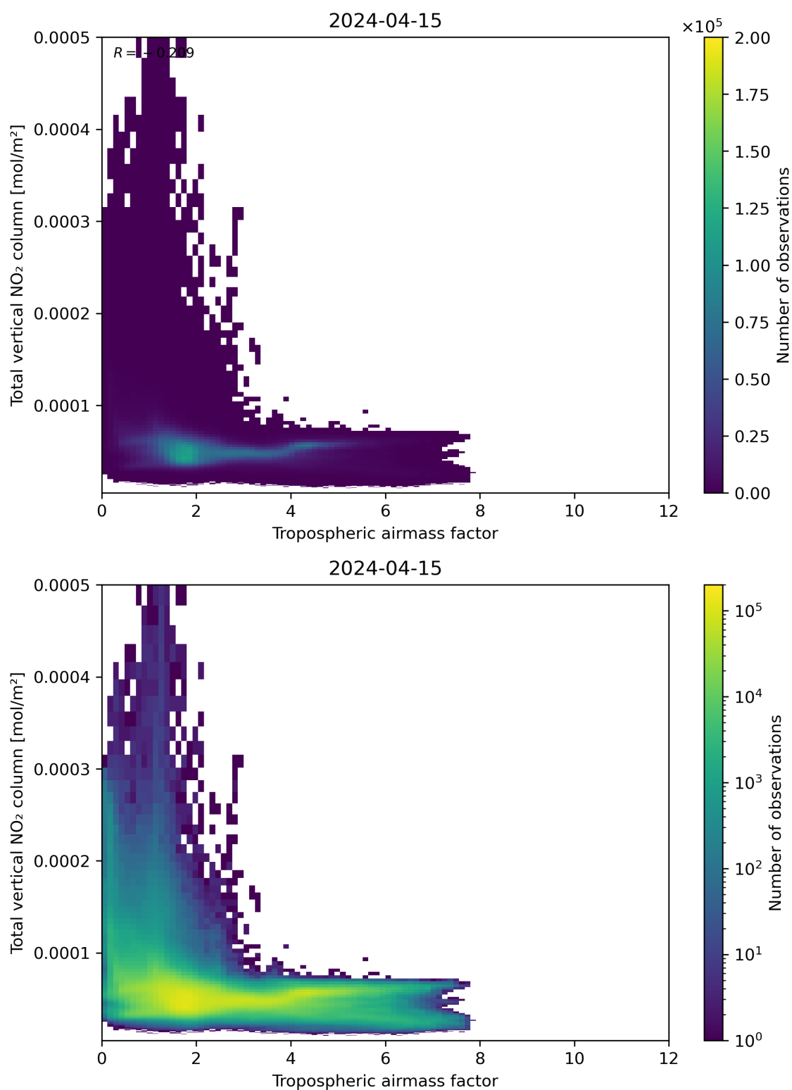
Figure 77: Scatter density plot of “Tropospheric airmass factor” against “Total vertical NO 2 column” for 2024-04-15 to 2024-04-16.
