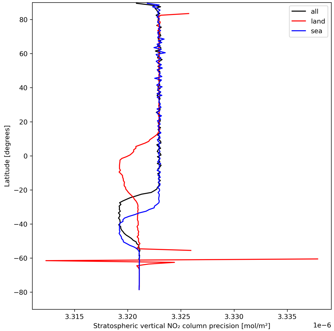
Figure 20: Zonal average of “Stratospheric vertical NO 2 column precision” for 2024-04-15 to 2024-04-16.
