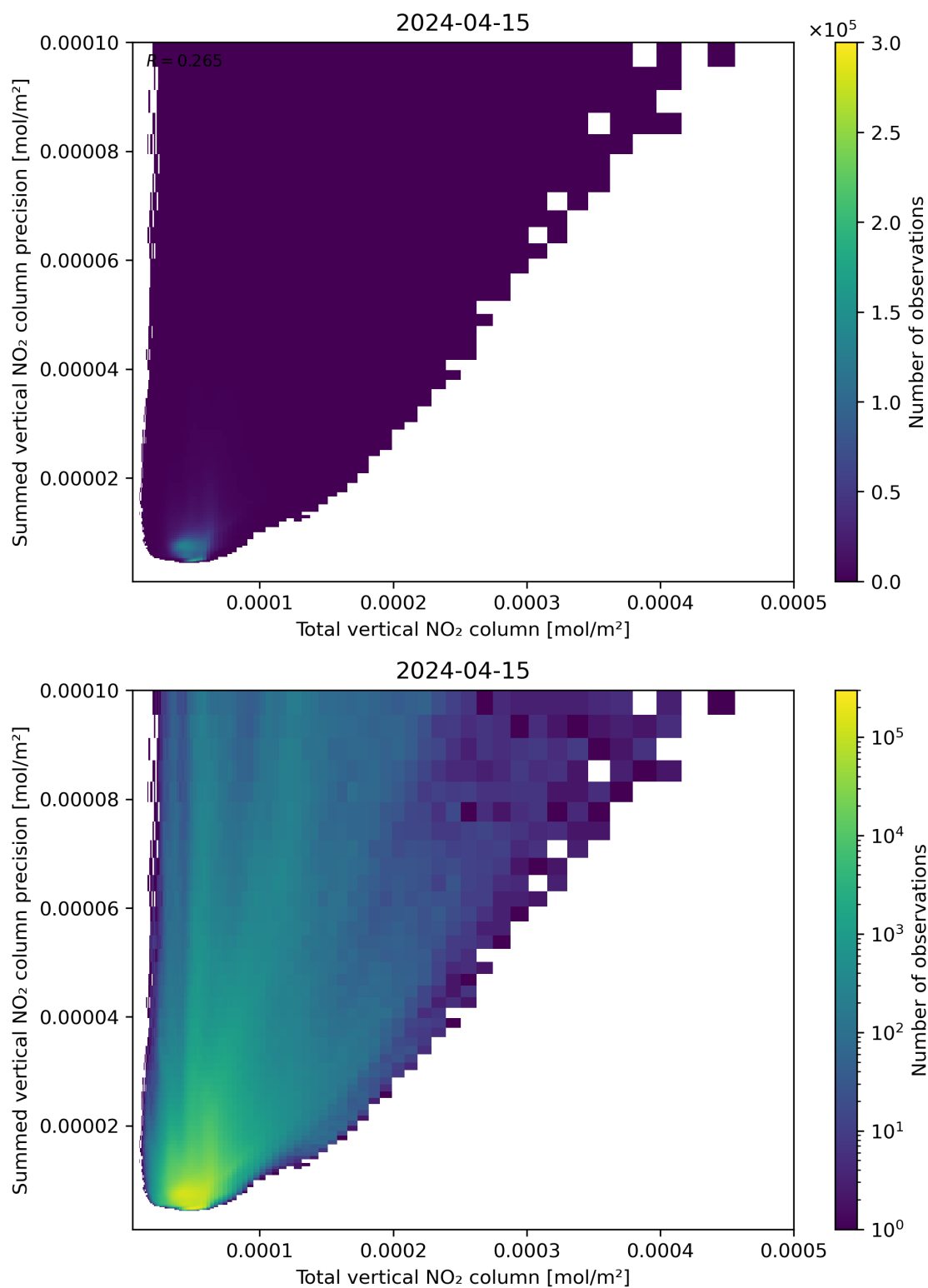
Figure 113: Scatter density plot of “Total vertical NO 2 column” against “Summed vertical NO 2 column precision” for 2024-04-15 to 2024-04-16.
