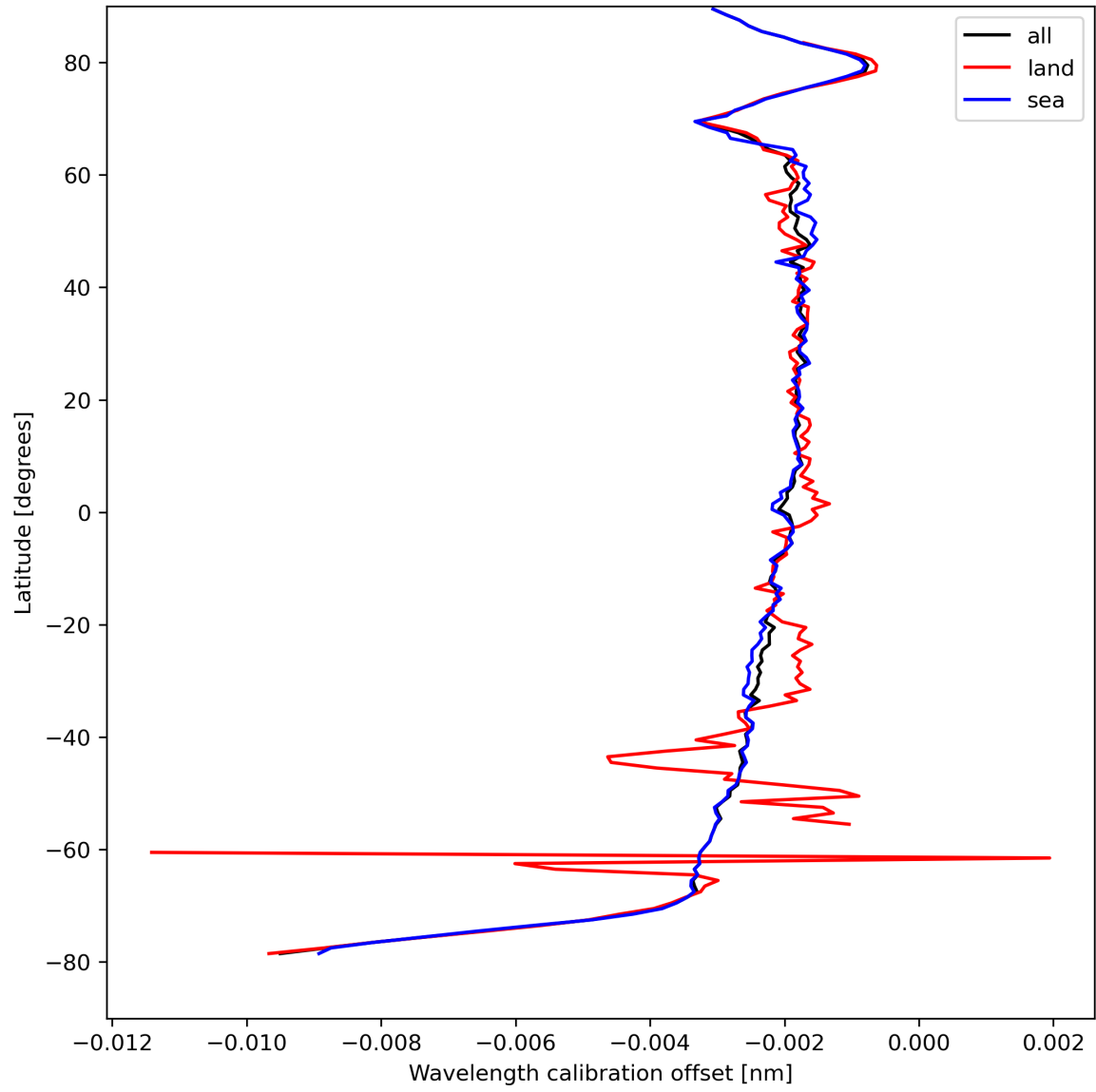
Figure 18: Zonal average of “Wavelength calibration offset” for 2024-04-15 to 2024-04-16.
