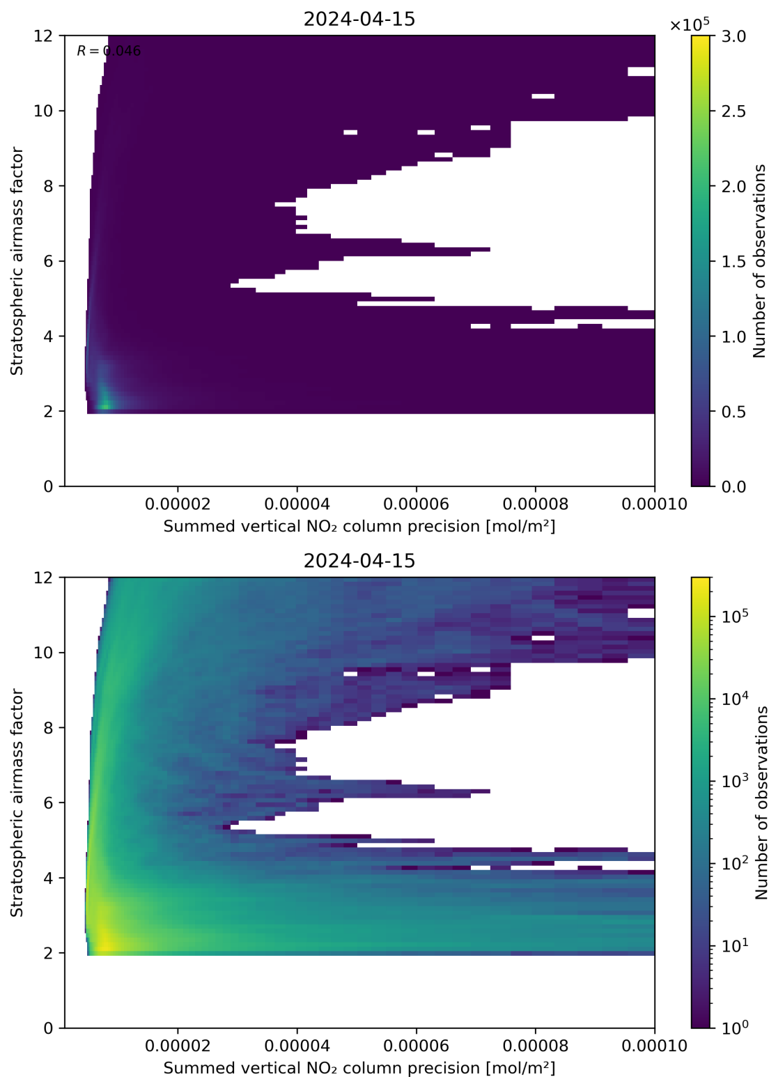
Figure 106: Scatter density plot of “Summed vertical NO 2 column precision” against “Stratospheric airmass factor” for 2024-04-15 to 2024-04-16.
