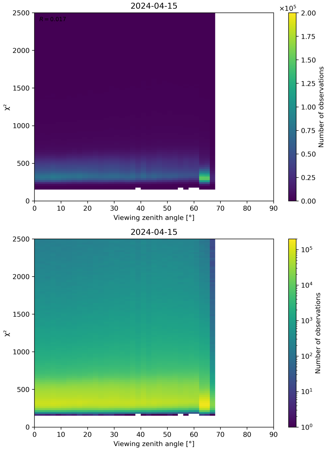
Figure 162: Scatter density plot of “Viewing zenith angle” against “ \chi^2 ” for 2024-04-15 to 2024-04-16.
