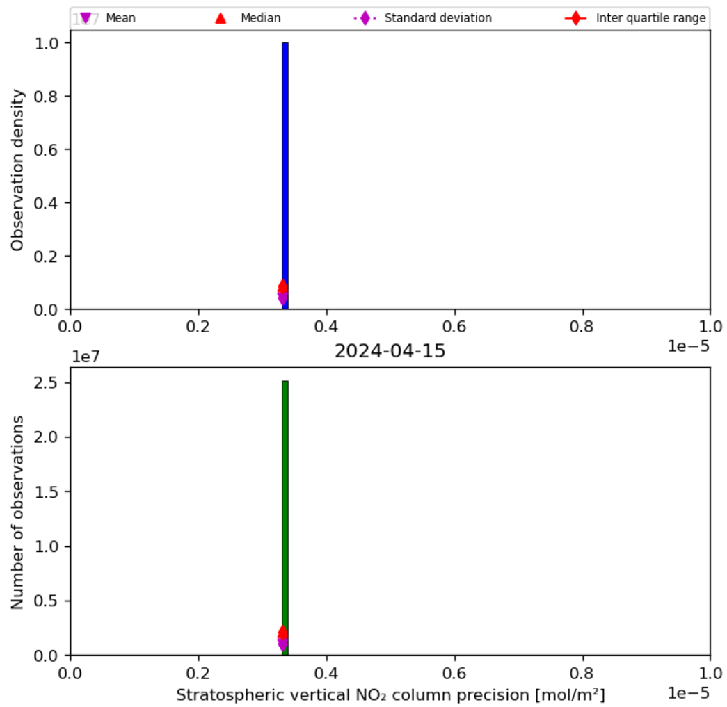
Figure 37: Histogram of “Stratospheric vertical NO 2 column precision” for 2024-04-15 to 2024-04-16
