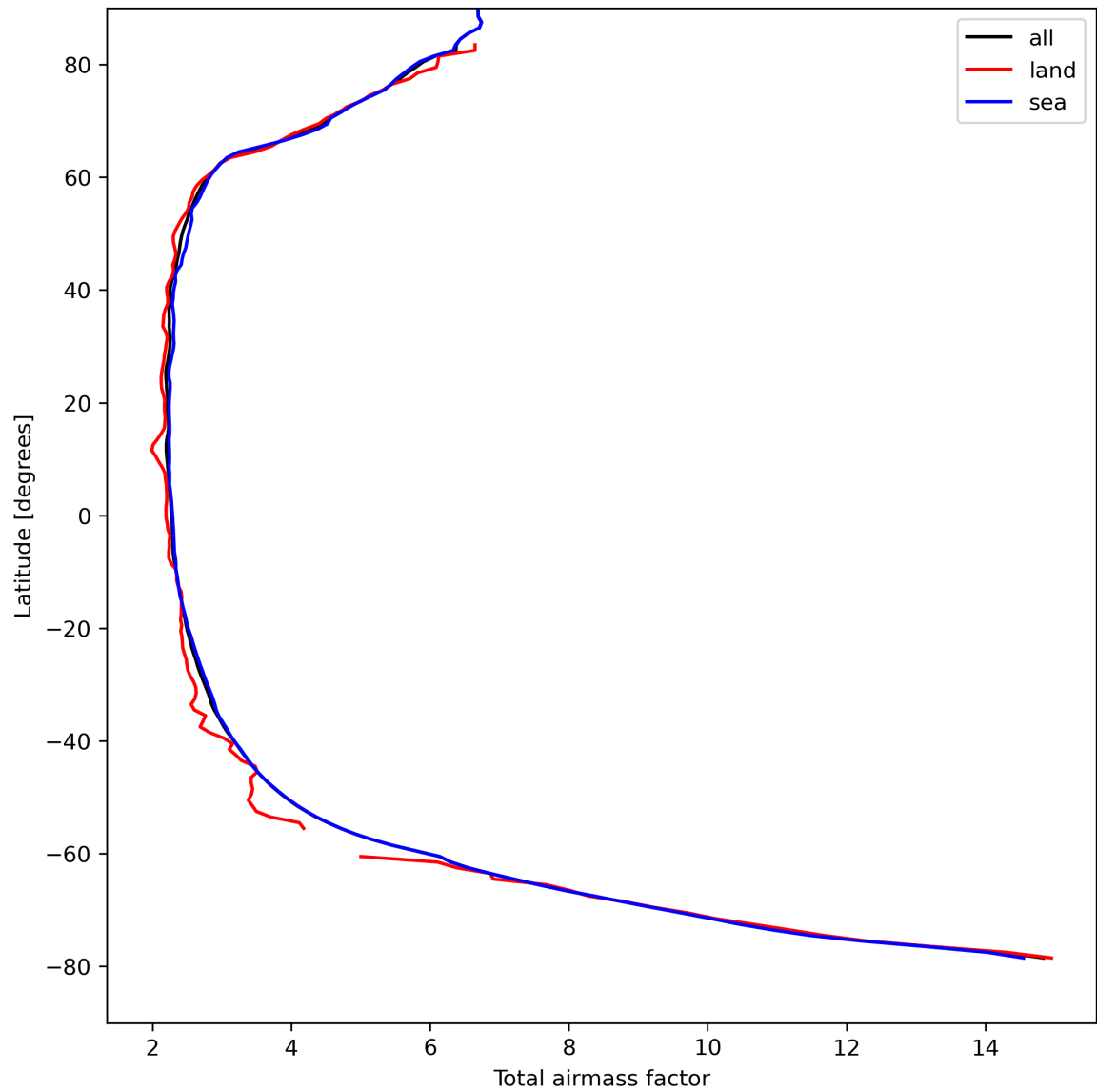
Figure 15: Zonal average of “Total airmass factor” for 2024-04-15 to 2024-04-16.
