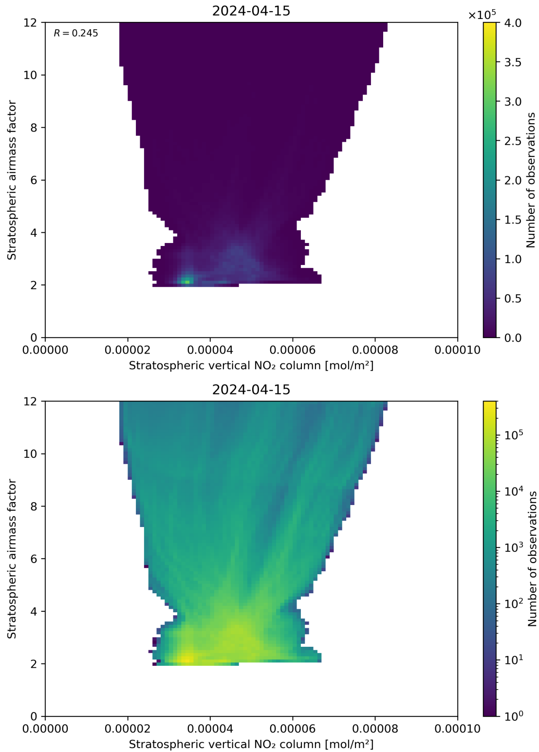
Figure 96: Scatter density plot of “Stratospheric vertical NO 2 column” against “Stratospheric airmass factor” for 2024-04-15 to 2024-04-16.
