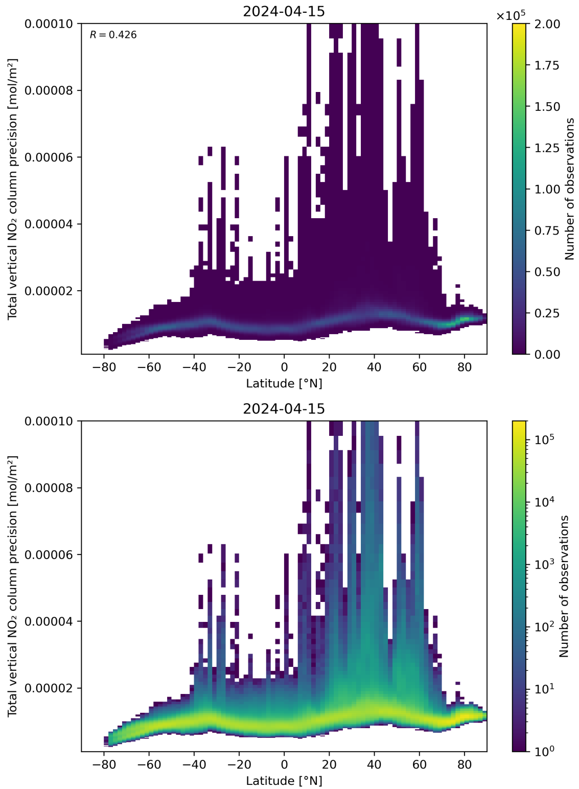
Figure 91: Scatter density plot of “Latitude” against “Total vertical NO 2 column precision” for 2024-04-15 to 2024-04-16.
