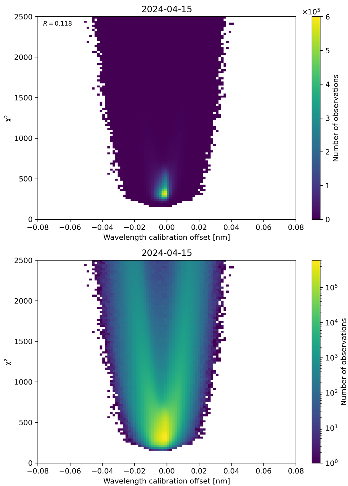
Figure 175: Scatter density plot of “Wavelength calibration offset” against “ \chi^2 ” for 2024-04-15 to 2024-04-16.
