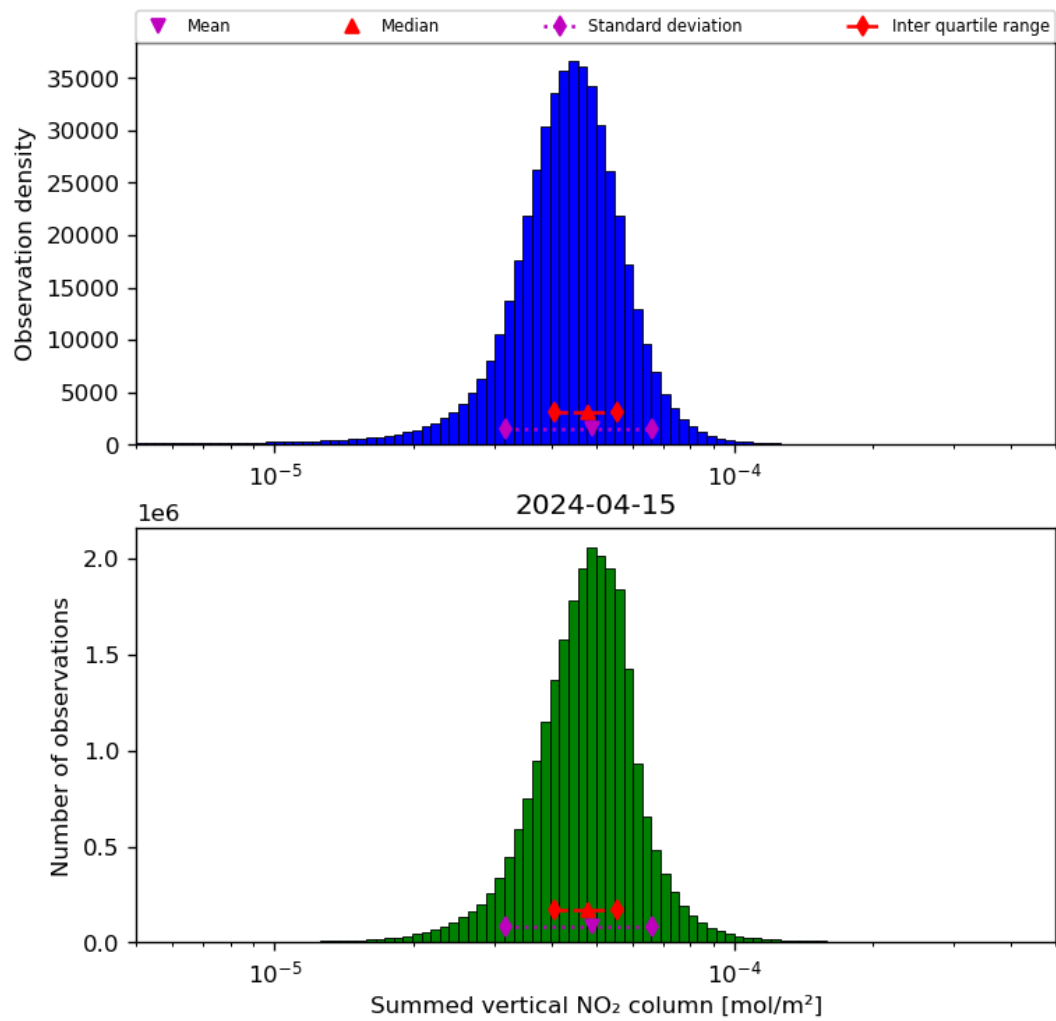
Figure 40: Histogram of “Summed vertical NO 2 column” for 2024-04-15 to 2024-04-16
