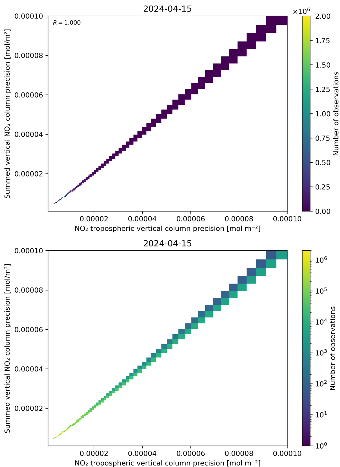
Figure 137: Scatter density plot of “NO 2 tropospheric vertical column precision” against “Summed vertical NO 2 column precision” for 2024-04-15 to 2024-04-16.
