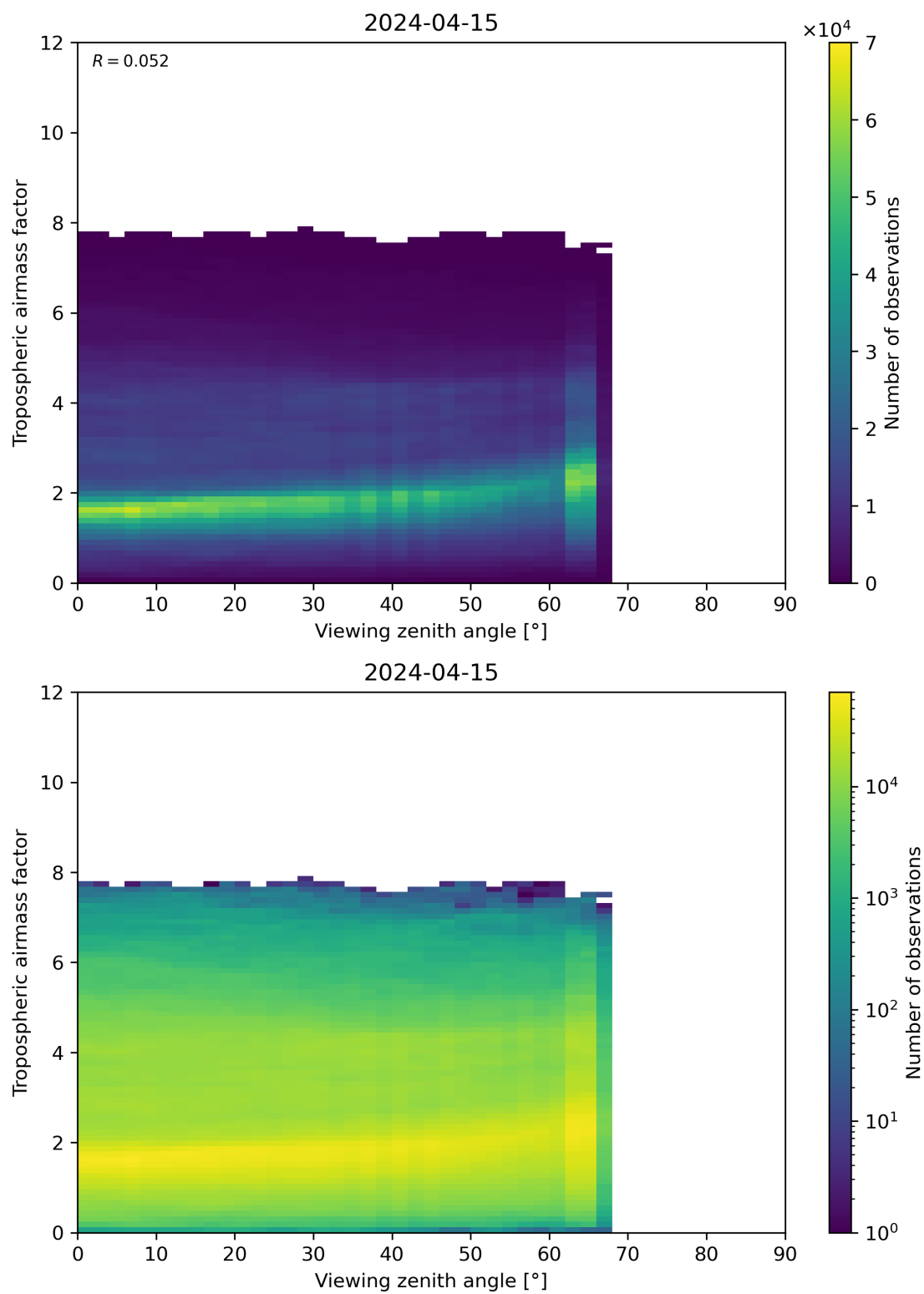
Figure 161: Scatter density plot of “Viewing zenith angle” against “Tropospheric airmass factor” for 2024-04-15 to 2024-04-16.
