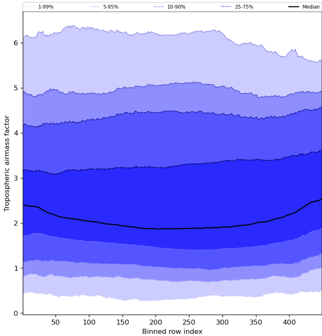
Figure 48: Along track statistics of “Tropospheric airmass factor” for 2024-04-15 to 2024-04-16
