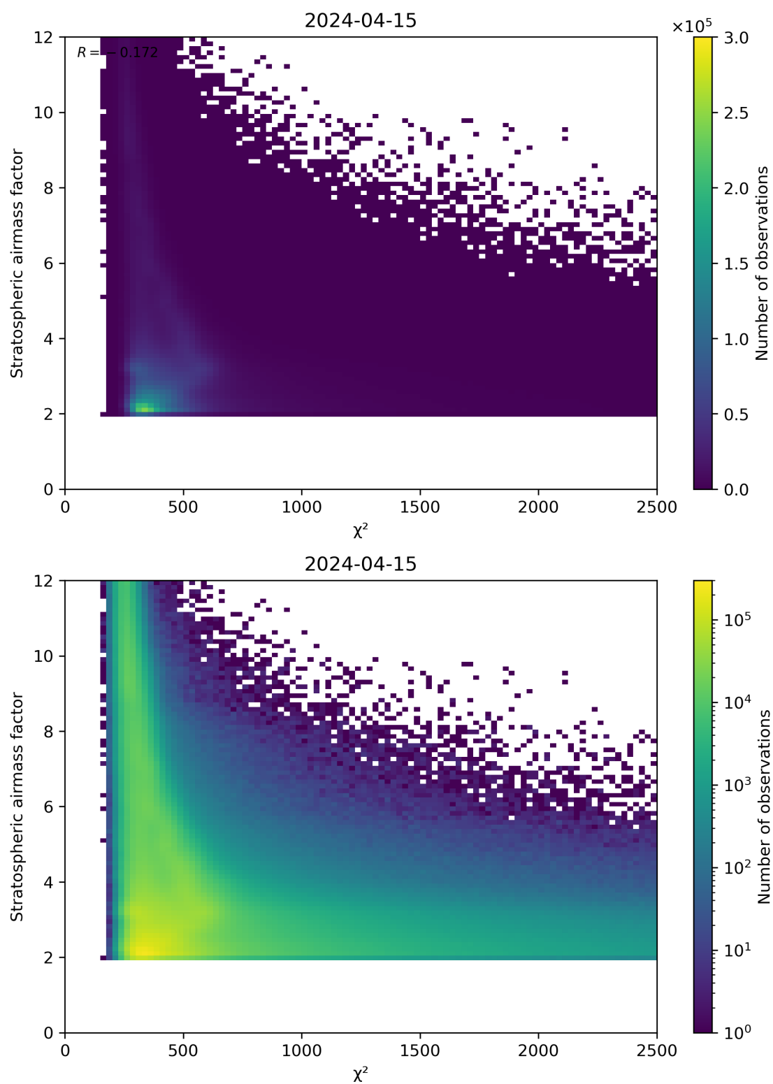
Figure 81: Scatter density plot of “ \chi^2 ” against “Stratospheric airmass factor” for 2024-04-15 to 2024-04-16.
