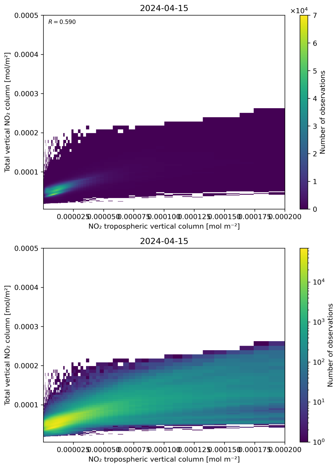
Figure 128: Scatter density plot of “NO 2 tropospheric vertical column” against “Total vertical NO 2 column” for 2024-04-15 to 2024-04-16.
