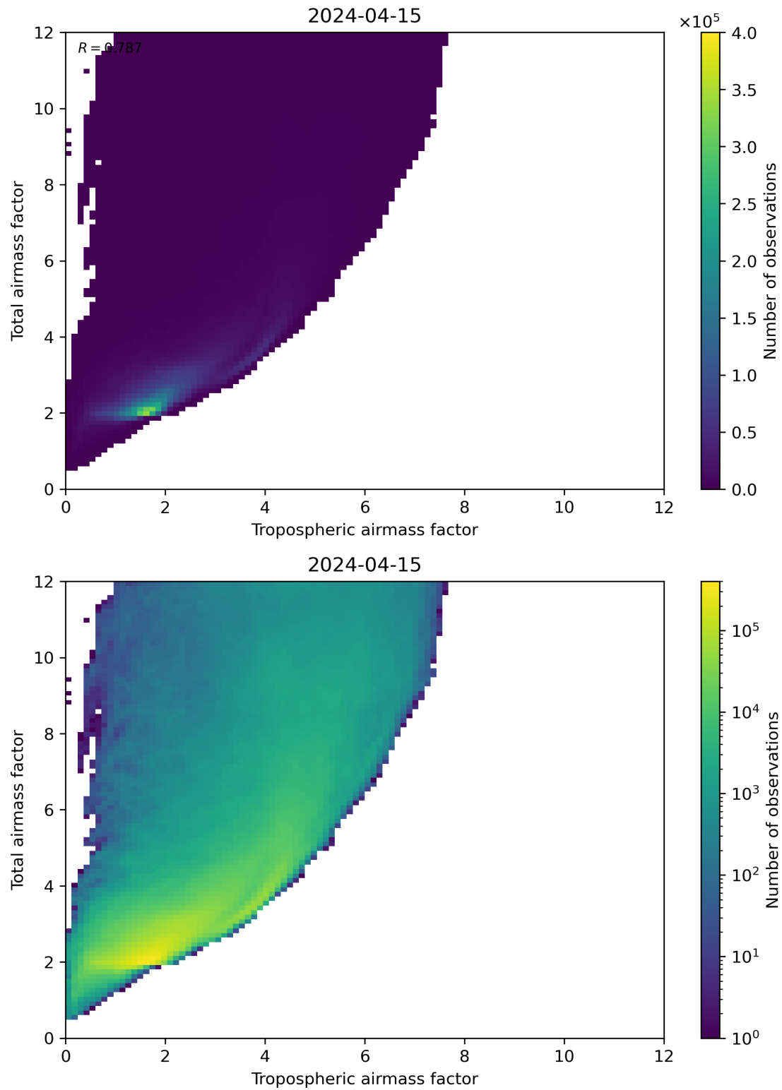
Figure 72: Scatter density plot of “Tropospheric airmass factor” against “Total airmass factor” for 2024-04-15 to 2024-04-16.
