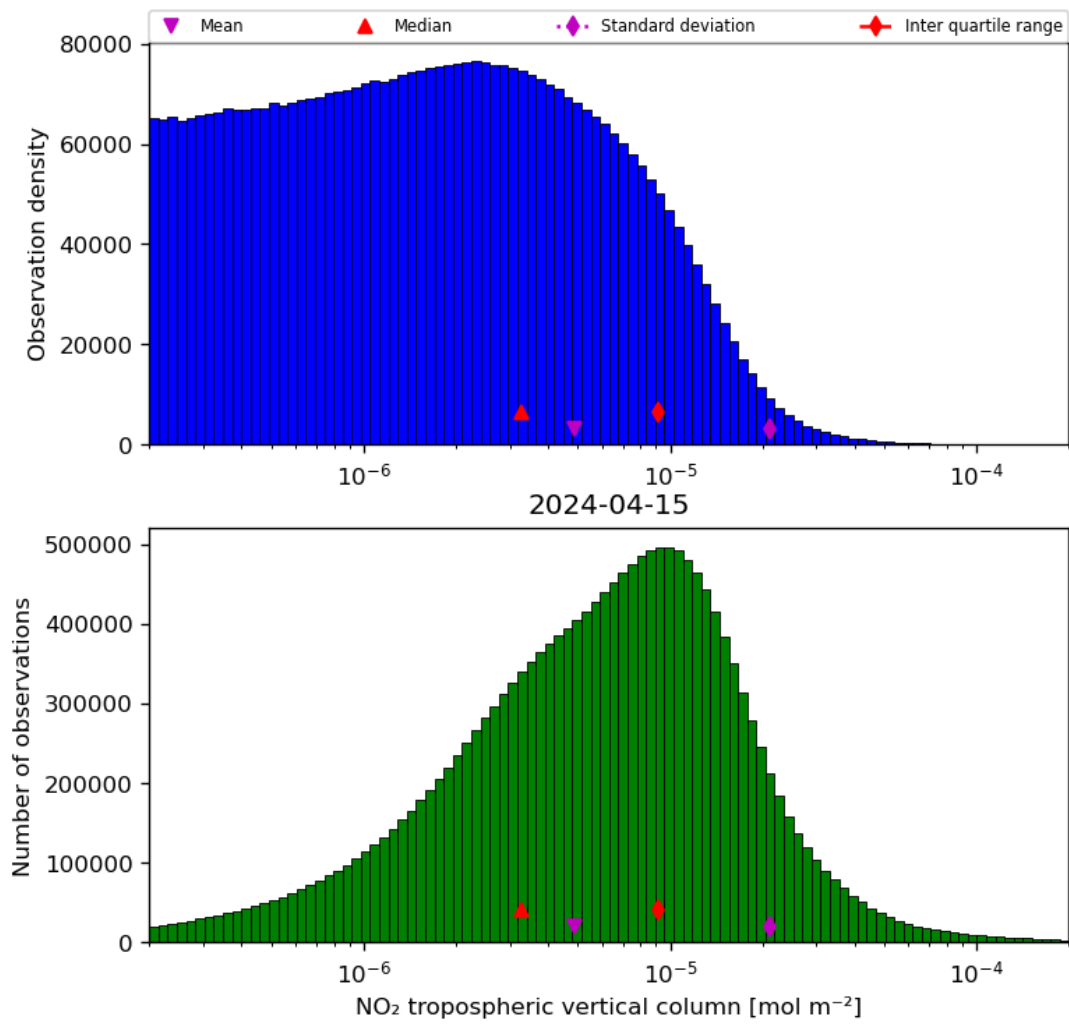
Figure 29: Histogram of “NO 2 tropospheric vertical column” for 2024-04-15 to 2024-04-16
