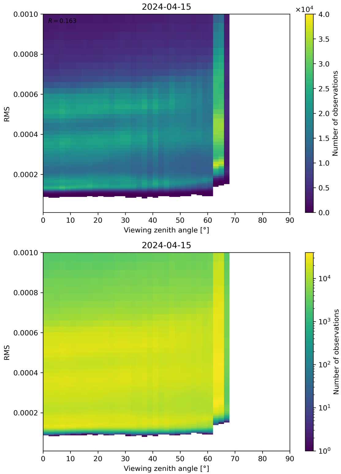
Figure 171: Scatter density plot of “Viewing zenith angle” against “RMS” for 2024-04-15 to 2024-04-16.
