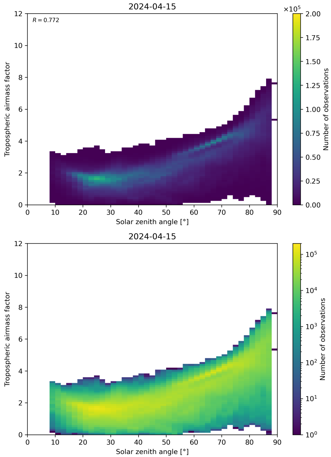
Figure 147: Scatter density plot of “Solar zenith angle” against “Tropospheric airmass factor” for 2024-04-15 to 2024-04-16.
