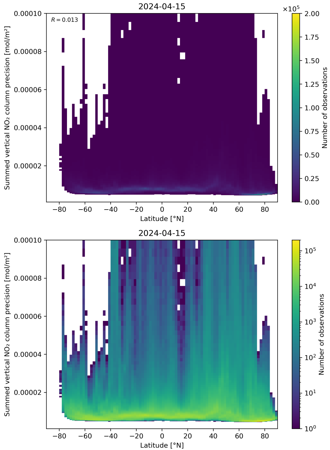
Figure 89: Scatter density plot of “Latitude” against “Summed vertical NO 2 column precision” for 2024-04-15 to 2024-04-16.
