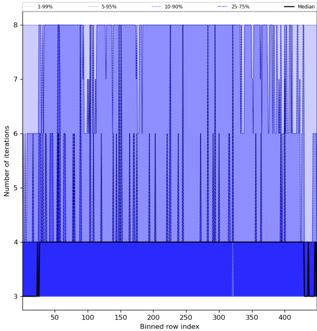
Figure 51: Along track statistics of "Number of iterations" for 2024-04-15 to 2024-04-16
