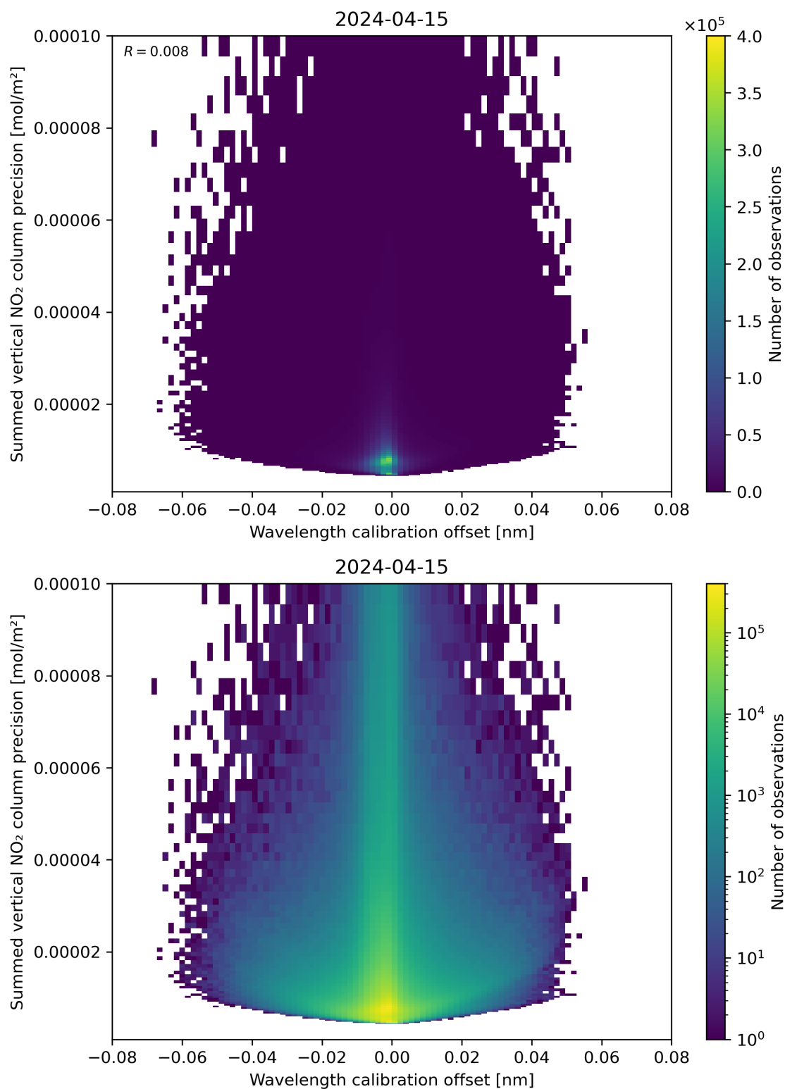
Figure 178: Scatter density plot of “Wavelength calibration offset” against “Summed vertical NO 2 column precision” for 2024-04-15 to 2024-04-16.
