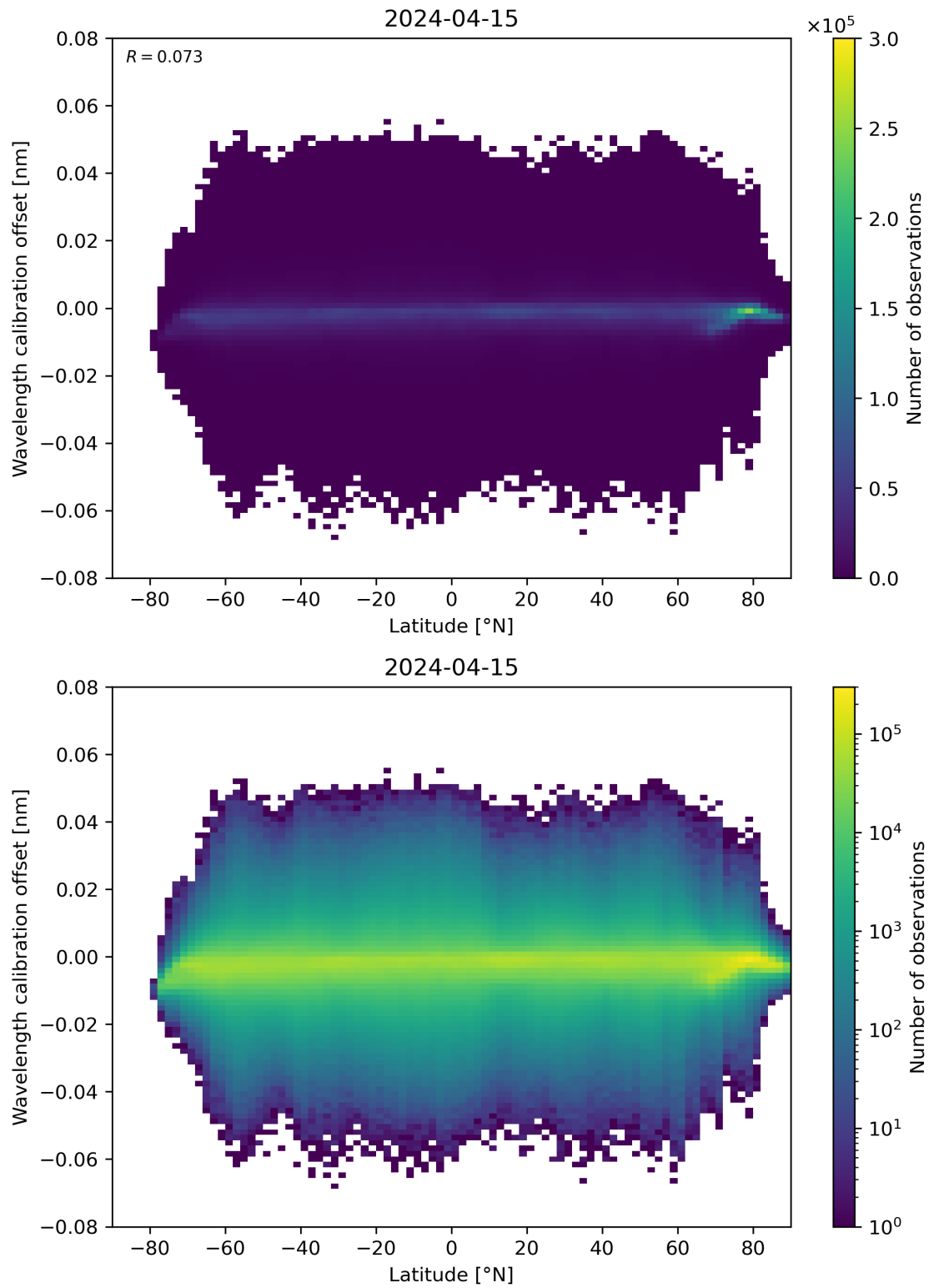
Figure 95: Scatter density plot of “Latitude” against “Wavelength calibration offset” for 2024-04-15 to 2024-04-16.
