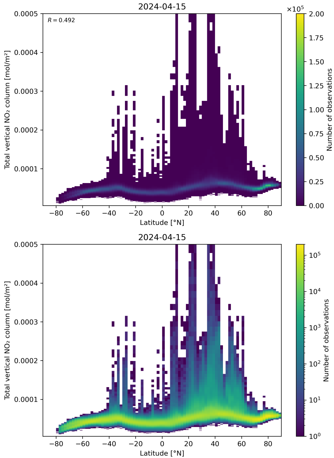
Figure 90: Scatter density plot of “Latitude” against “Total vertical NO 2 column” for 2024-04-15 to 2024-04-16.
