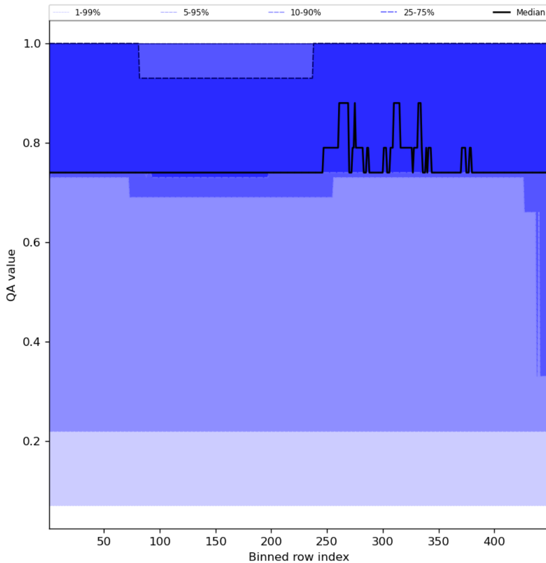
Figure 45: Along track statistics of “QA value” for 2024-04-15 to 2024-04-16
