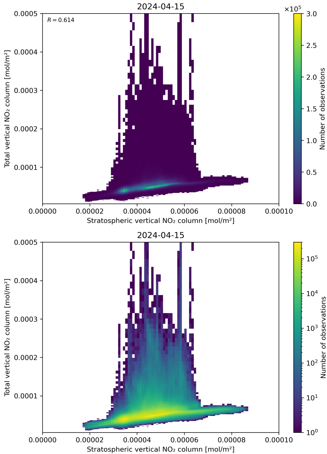
Figure 100: Scatter density plot of “Stratospheric vertical NO 2 column” against “Total vertical NO 2 column” for 2024-04-15 to 2024-04-16.
