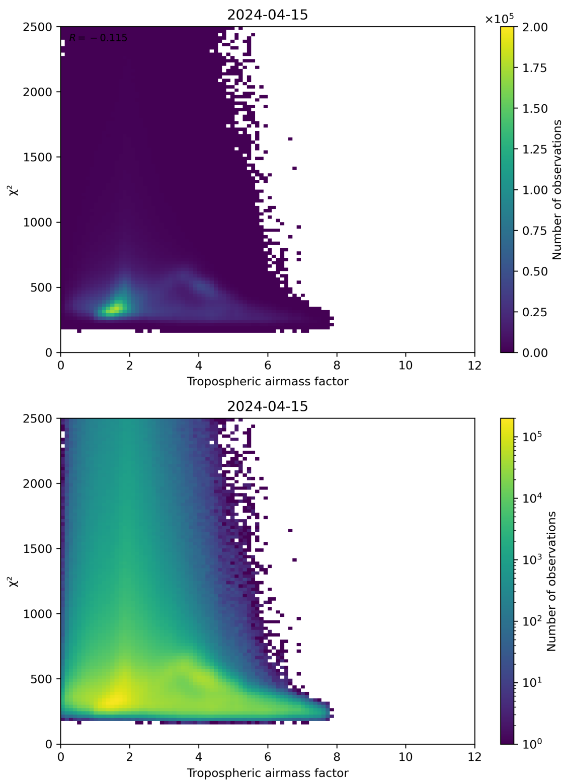
Figure 73: Scatter density plot of “Tropospheric airmass factor” against “ \chi^2 ” for 2024-04-15 to 2024-04-16.
