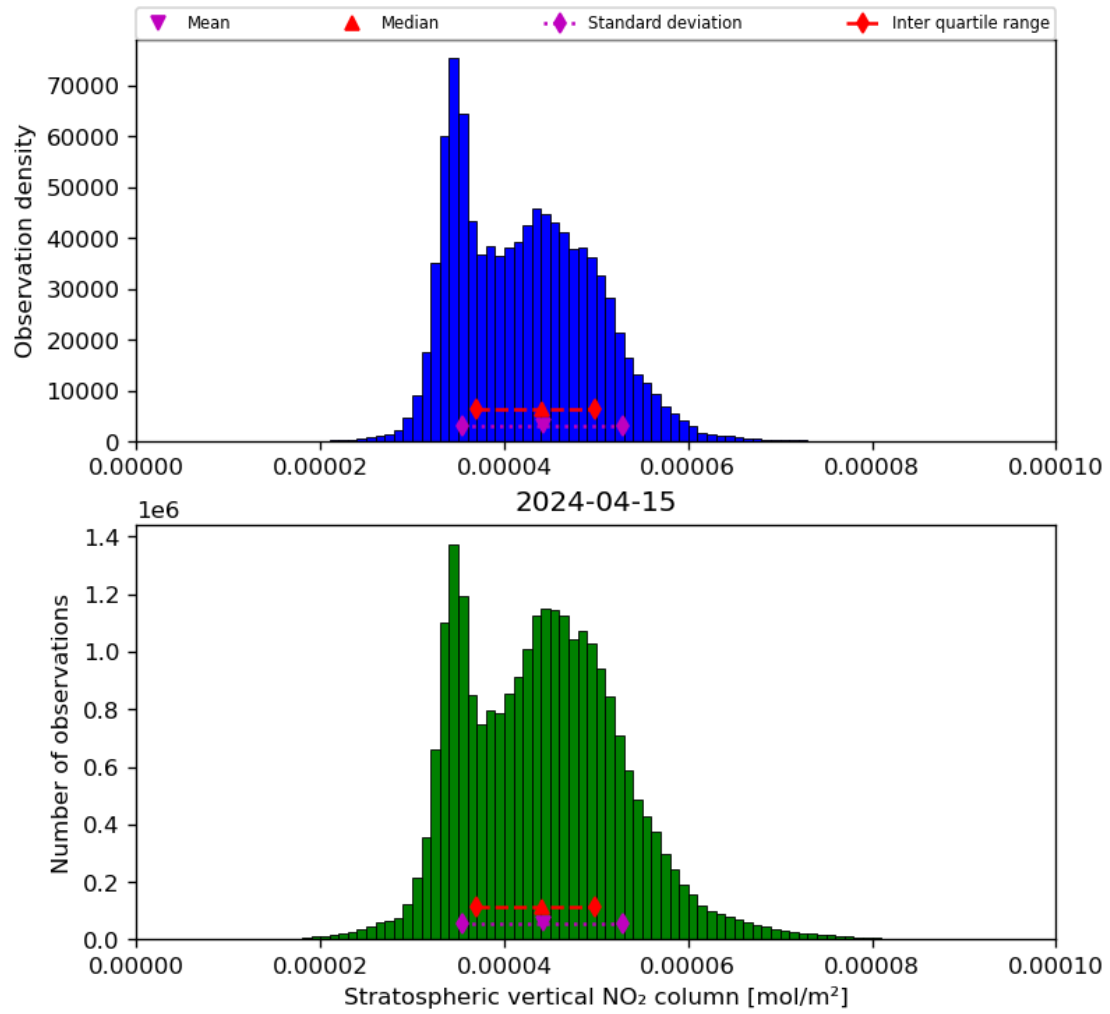
Figure 36: Histogram of “Stratospheric vertical NO 2 column” for 2024-04-15 to 2024-04-16
