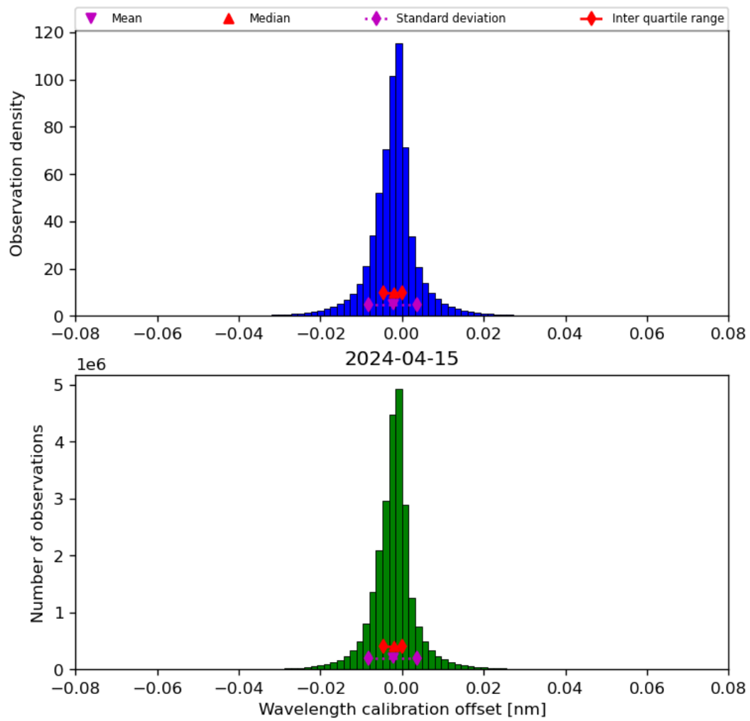
Figure 35: Histogram of “Wavelength calibration offset” for 2024-04-15 to 2024-04-16
