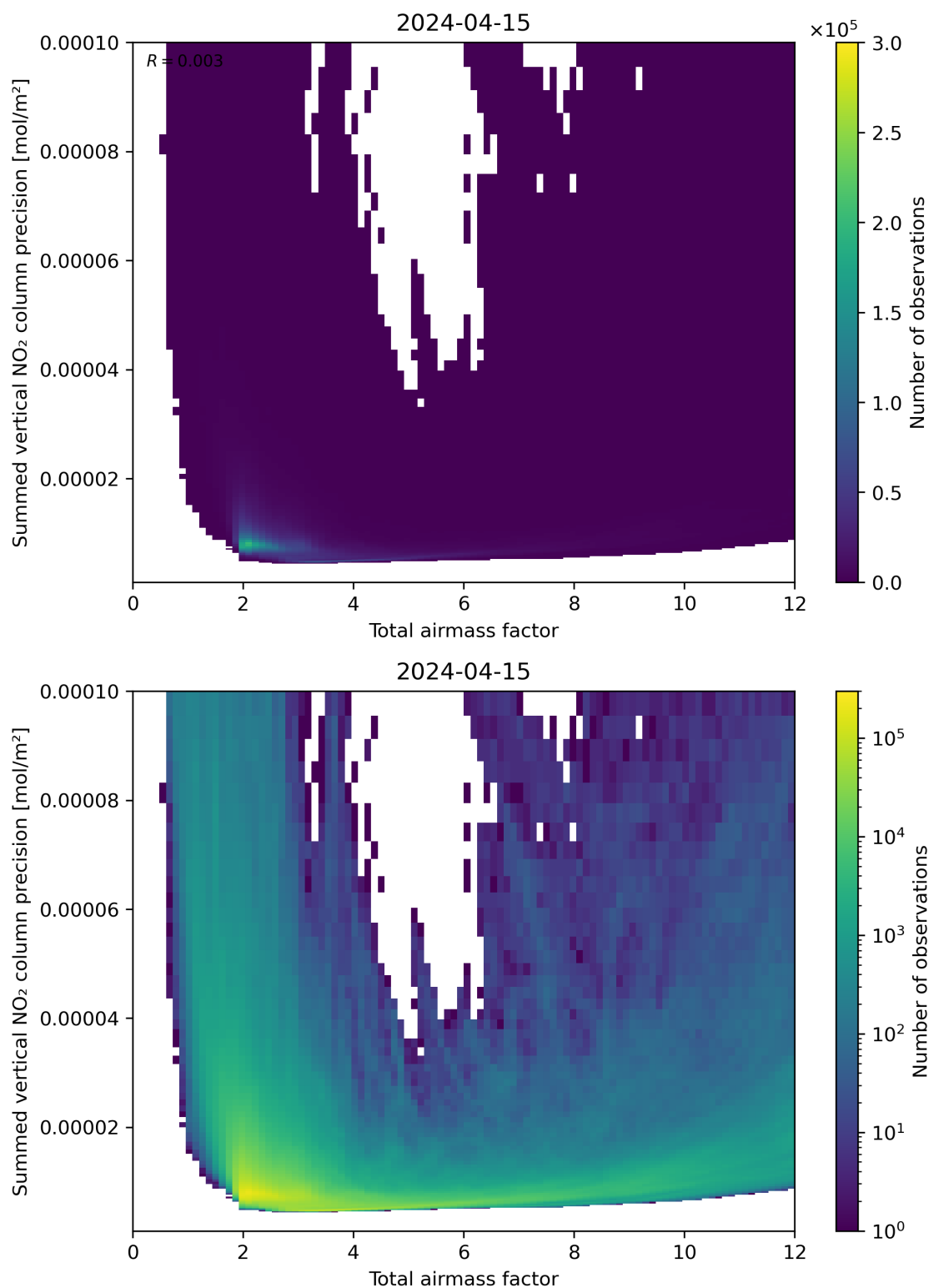
Figure 66: Scatter density plot of “Total airmass factor” against “Summed vertical NO 2 column precision” for 2024-04-15 to 2024-04-16.
