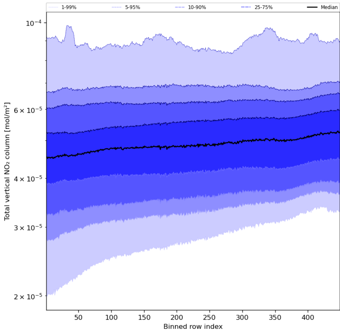
Figure 55: Along track statistics of “Total vertical NO 2 column” for 2024-04-15 to 2024-04-16
