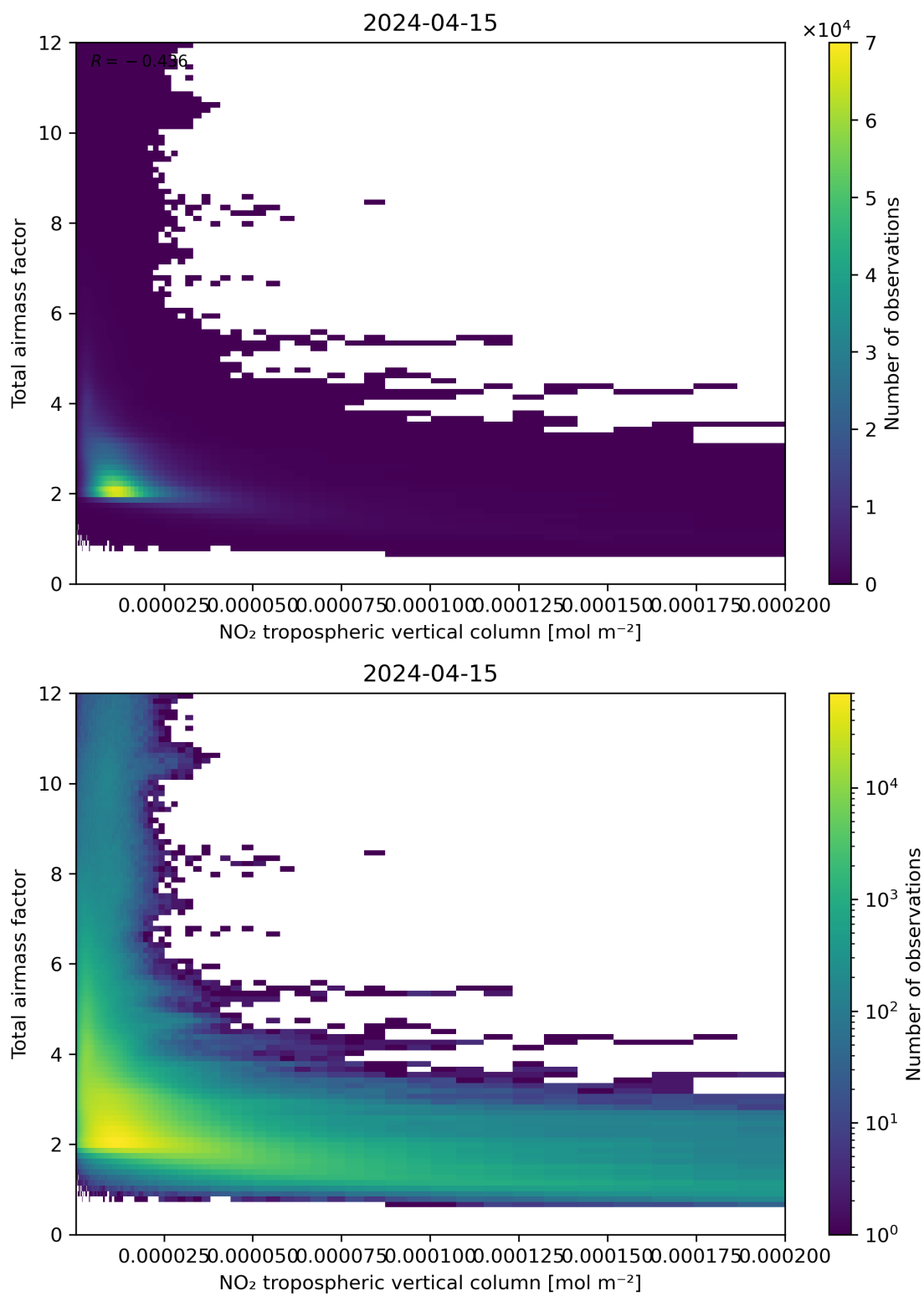
Figure 122: Scatter density plot of “NO 2 tropospheric vertical column” against “Total air mass factor” for 2024-04-15 to 2024-04-16.
