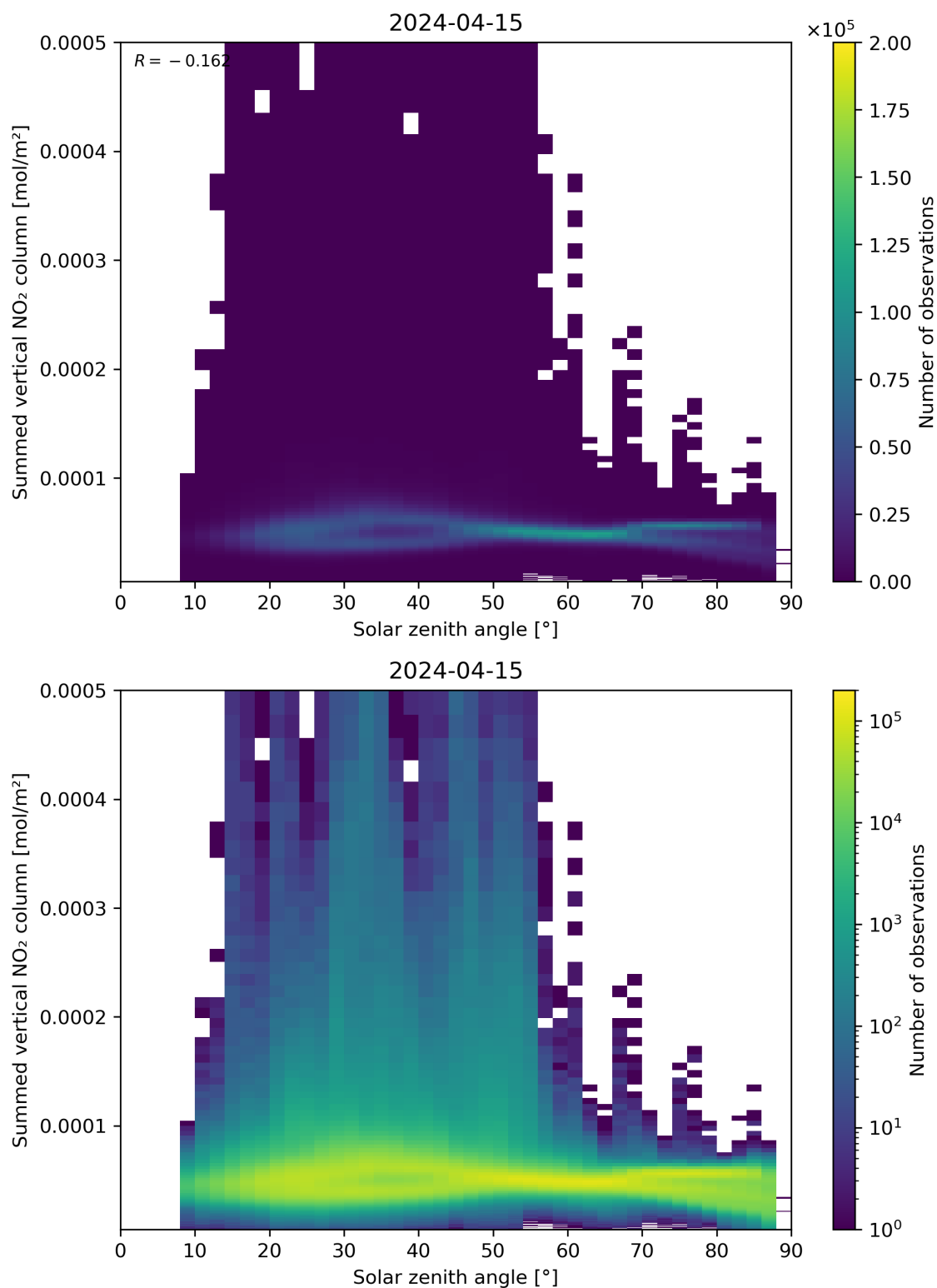
Figure 151: Scatter density plot of “Solar zenith angle” against “Summed vertical NO 2 column” for 2024-04-15 to 2024-04-16.
