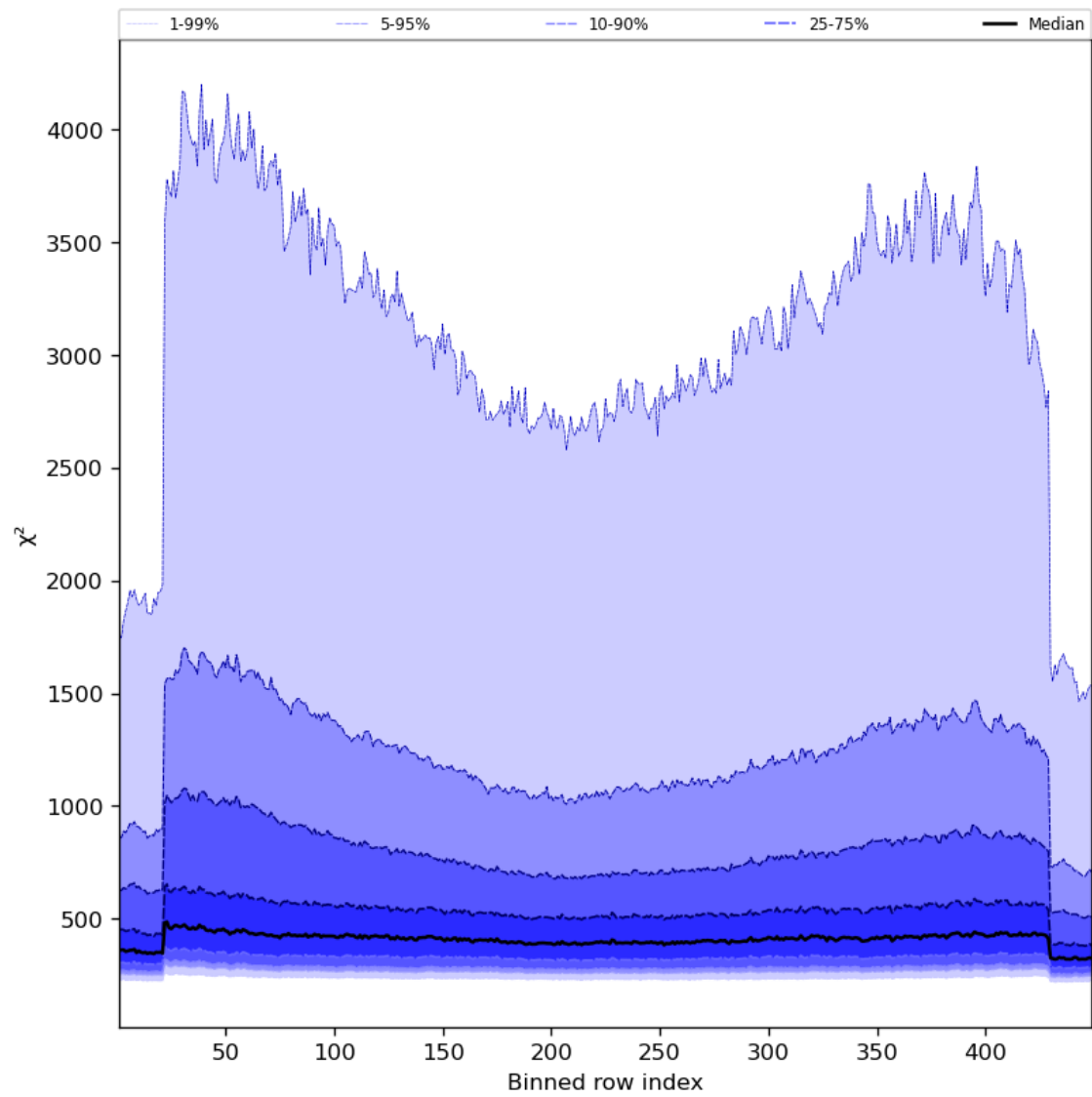
Figure 59: Along track statistics of “ \chi^2 ” for 2024-04-15 to 2024-04-16
