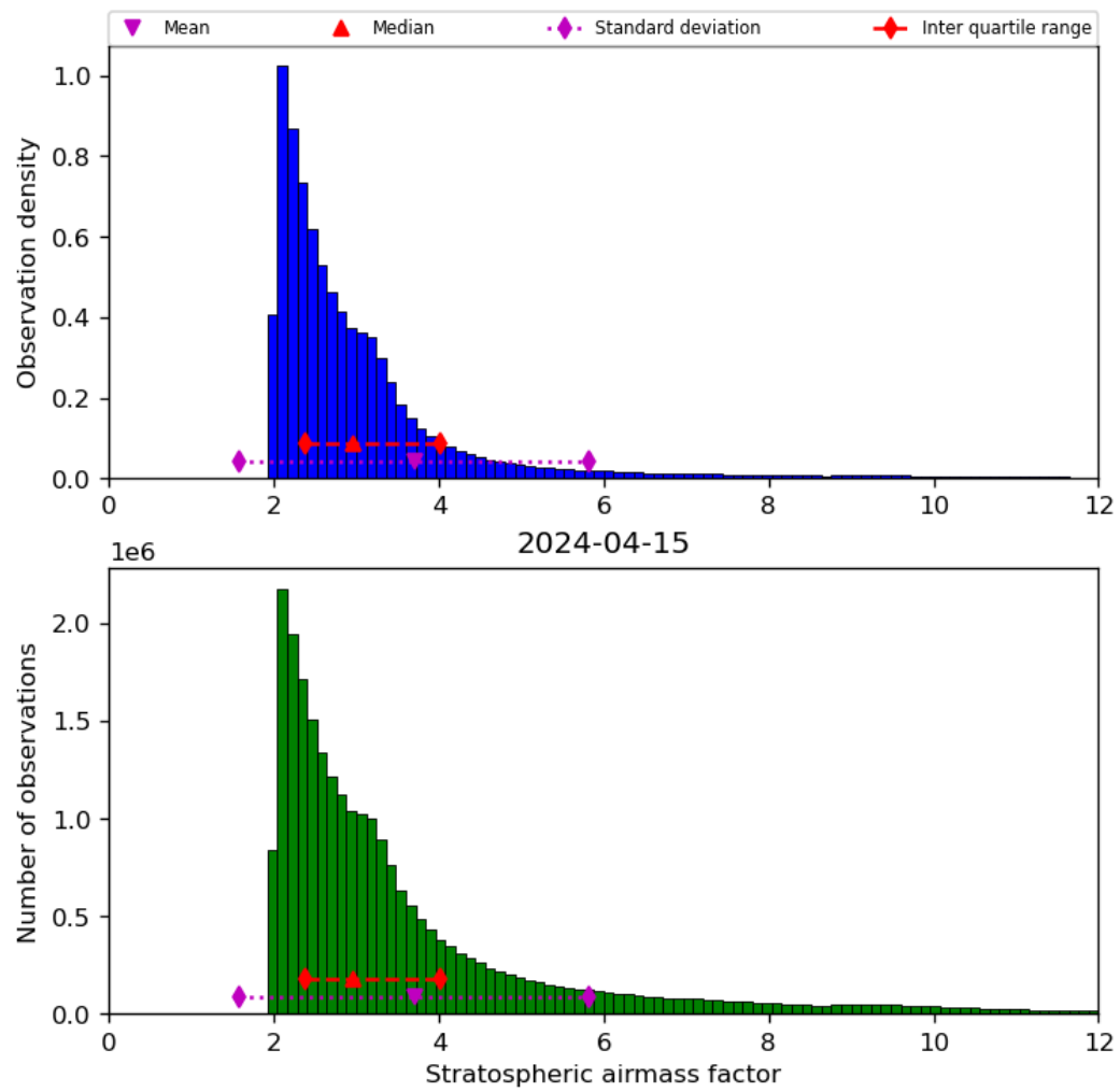
Figure 44: Histogram of “Stratospheric airmass factor” for 2024-04-15 to 2024-04-16
