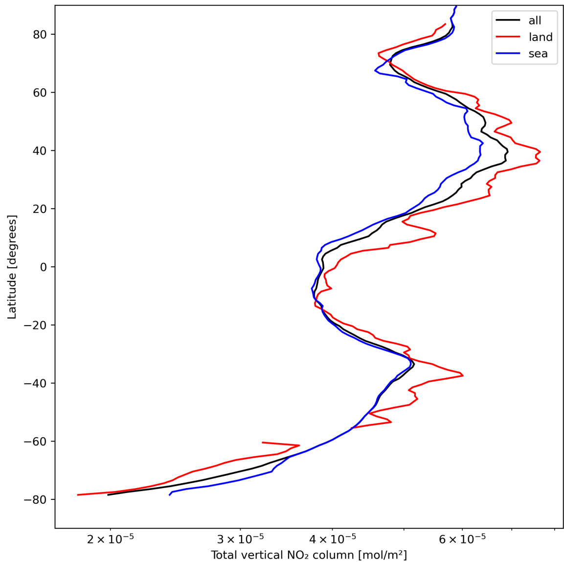
Figure 21: Zonal average of “Total vertical NO 2 column” for 2024-04-15 to 2024-04-16.
