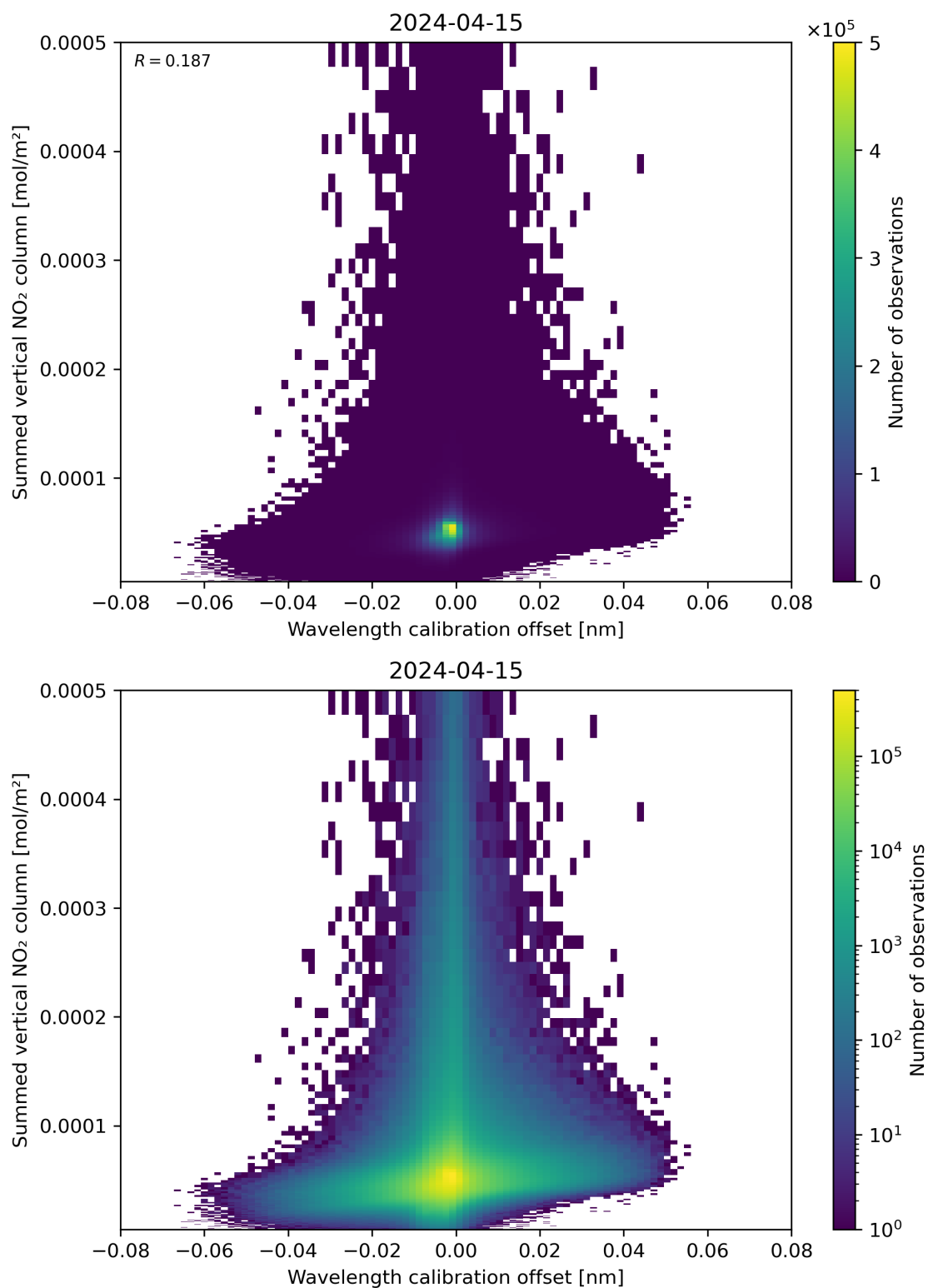
Figure 177: Scatter density plot of “Wavelength calibration offset” against “Summed vertical NO 2 column” for 2024-04-15 to 2024-04-16.
