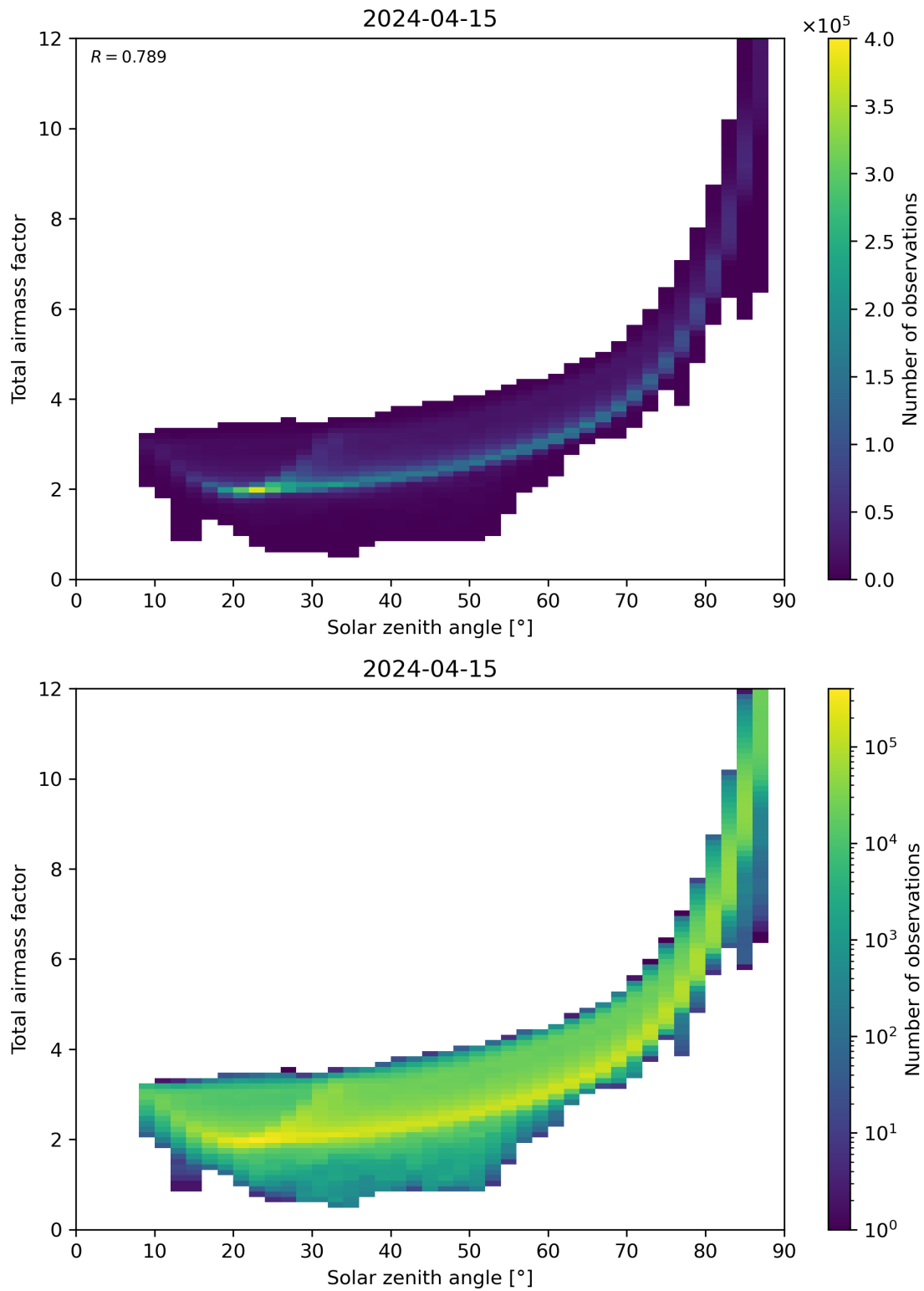
Figure 146: Scatter density plot of “Solar zenith angle” against “Total air mass factor” for 2024-04-15 to 2024-04-16.
