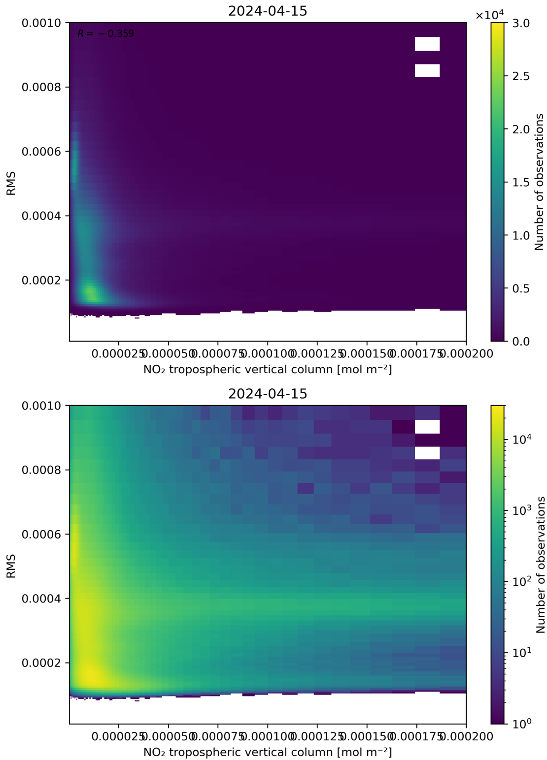
Figure 142: Scatter density plot of “NO 2 tropospheric vertical column” against “RMS” for 2024-04-15 to 2024-04-16.
