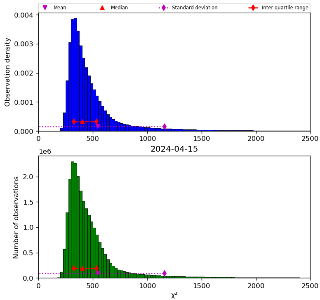
Figure 42: Histogram of “ \chi^2 ” for 2024-04-15 to 2024-04-16
