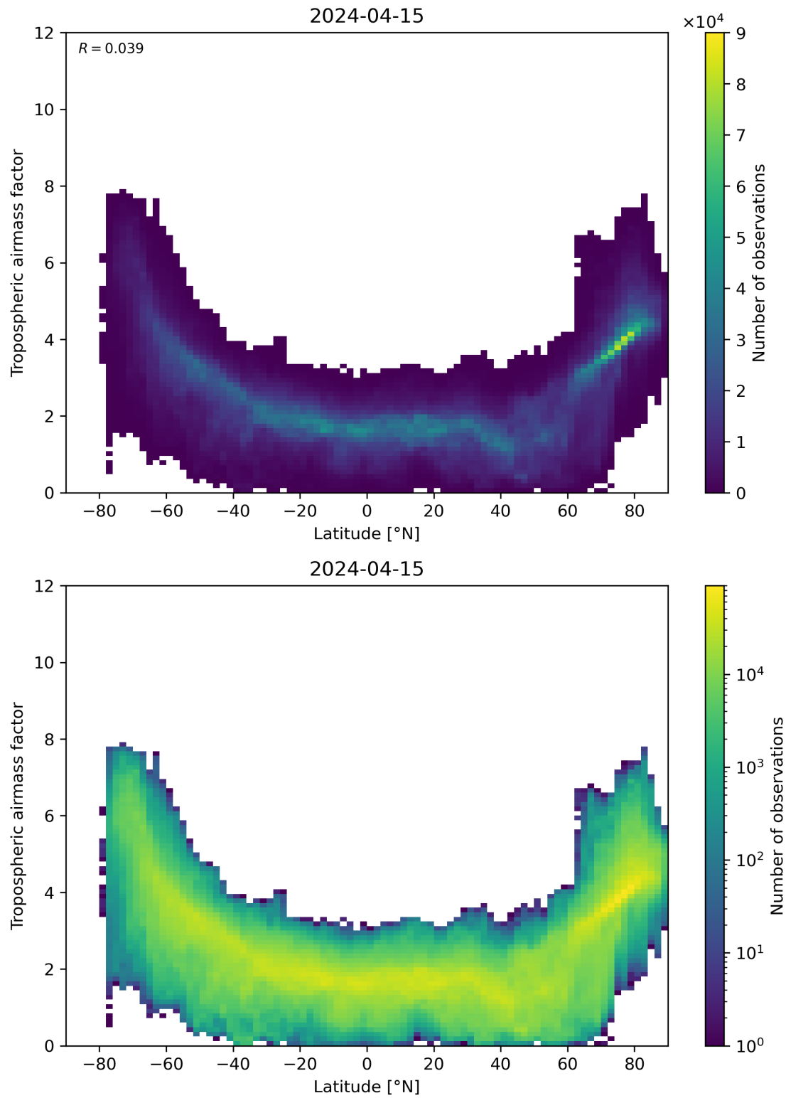
Figure 85: Scatter density plot of “Latitude” against “Tropospheric air mass factor” for 2024-04-15 to 2024-04-16.
