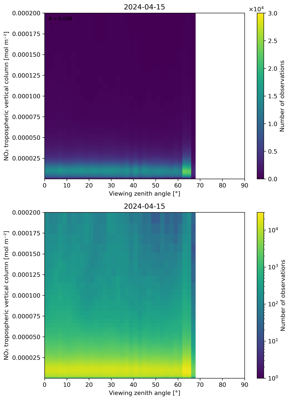
Figure 169: Scatter density plot of “Viewing zenith angle” against “NO 2 tropospheric vertical column” for 2024-04-15 to 2024-04-16.
