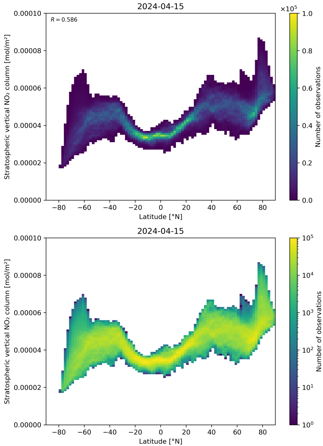
Figure 87: Scatter density plot of “Latitude” against “Stratospheric vertical \text{NO}_2 column” for 2024-04-15 to 2024-04-16.
