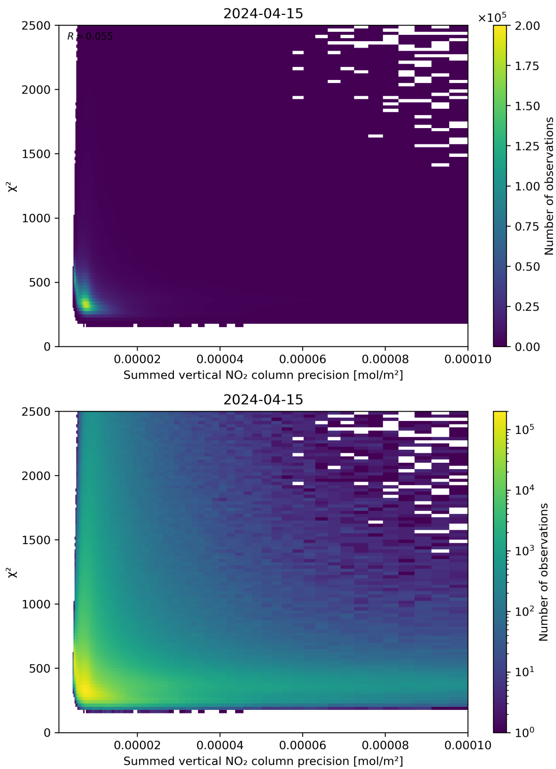
Figure 107: Scatter density plot of “Summed vertical NO 2 column precision” against “ \chi^2 ” for 2024-04-15 to 2024-04-16.
