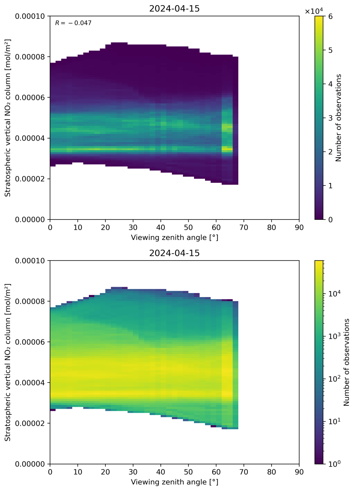
Figure 164: Scatter density plot of “Viewing zenith angle” against “Stratospheric vertical NO 2 column” for 2024-04-15 to 2024-04-16.
