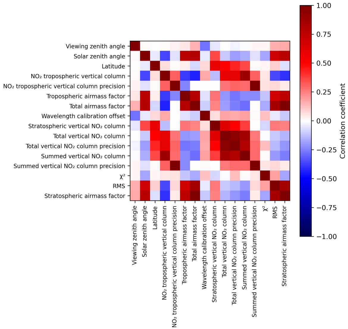
Figure 2: Map of correlation matrix for 2024-04-15 to 2024-04-16.
