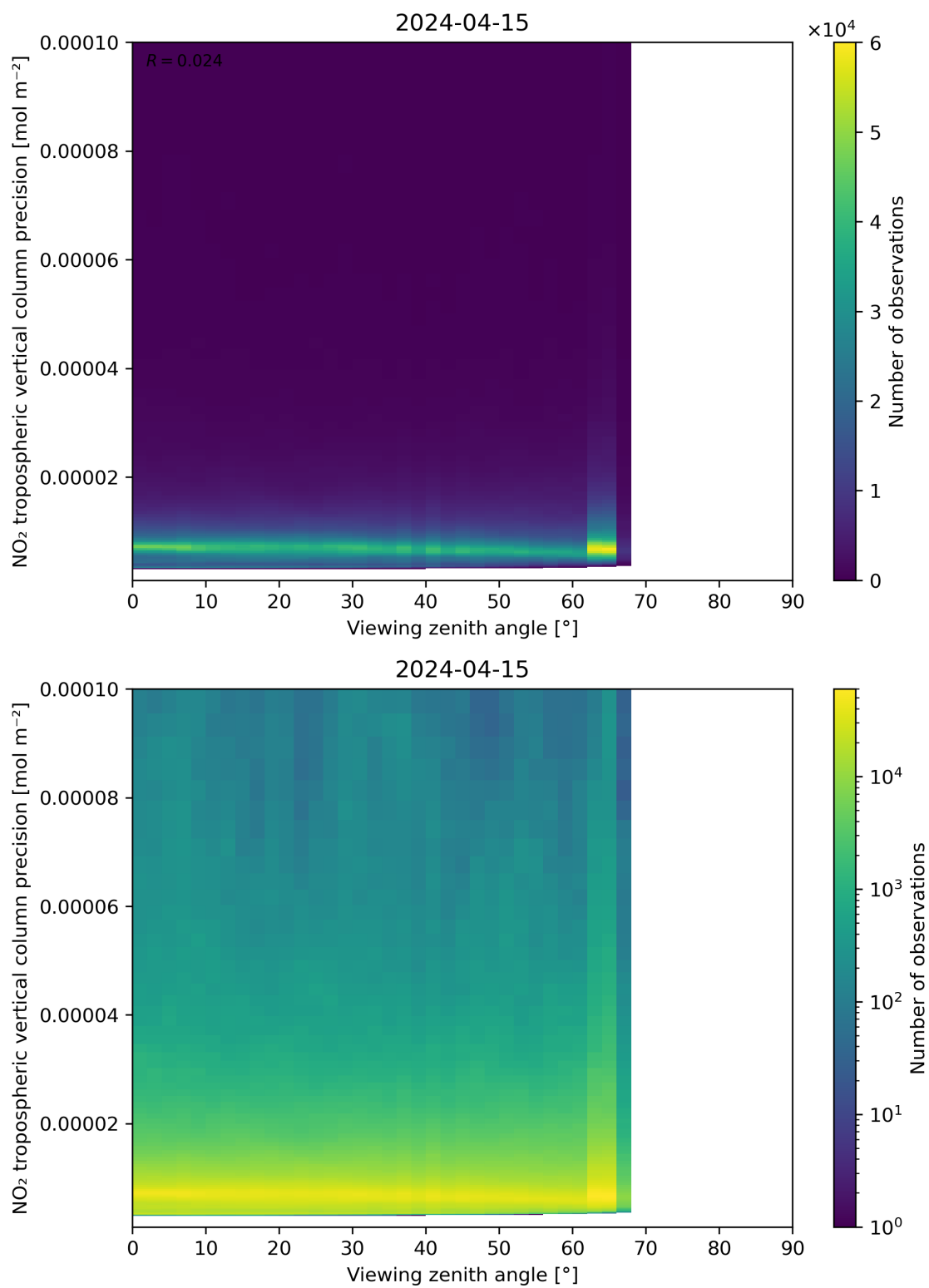
Figure 170: Scatter density plot of “Viewing zenith angle” against “NO 2 tropospheric vertical column precision” for 2024-04-15 to 2024-04-16.
