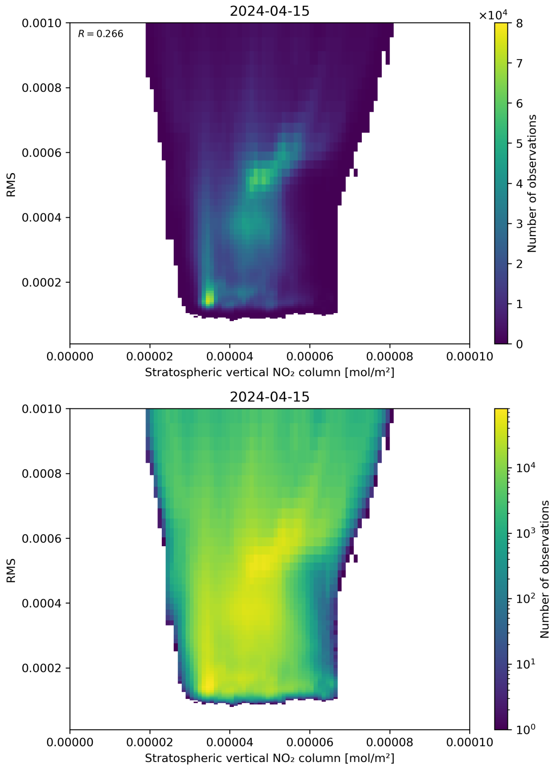
Figure 102: Scatter density plot of “Stratospheric vertical NO 2 column” against “RMS” for 2024-04-15 to 2024-04-16.
