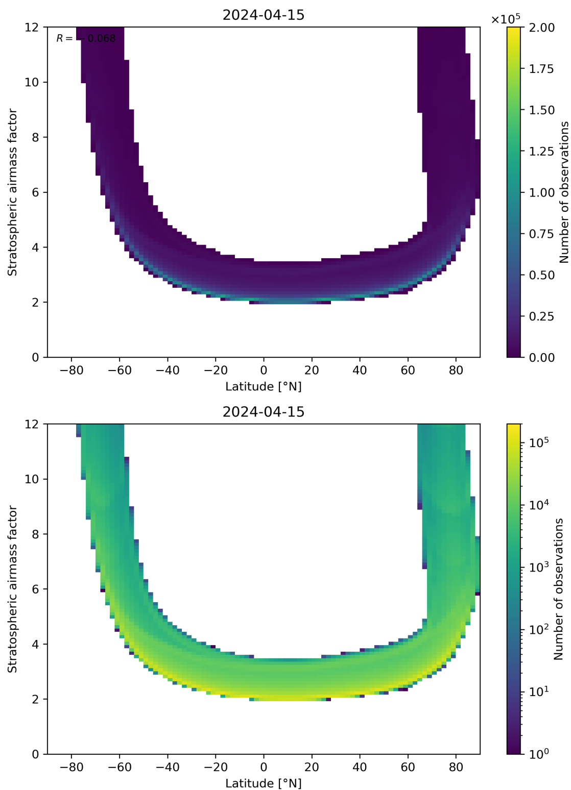
Figure 83: Scatter density plot of “Latitude” against “Stratospheric air mass factor” for 2024-04-15 to 2024-04-16.
