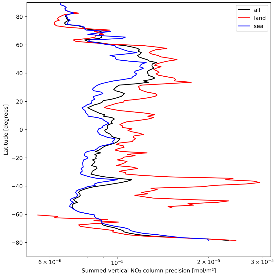
Figure 24: Zonal average of “Summed vertical NO 2 column precision” for 2024-04-15 to 2024-04-16.
