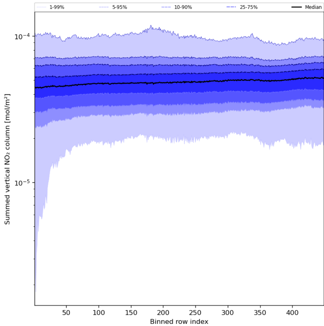
Figure 57: Along track statistics of “Summed vertical NO 2 column” for 2024-04-15 to 2024-04-16
