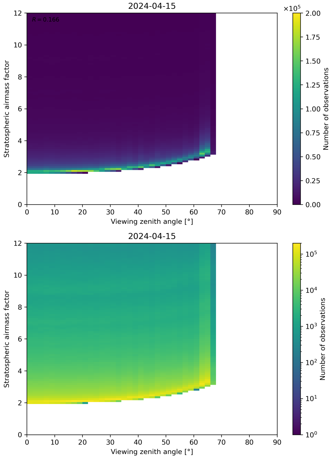
Figure 159: Scatter density plot of “Viewing zenith angle” against “Stratospheric airmass factor” for 2024-04-15 to 2024-04-16.
