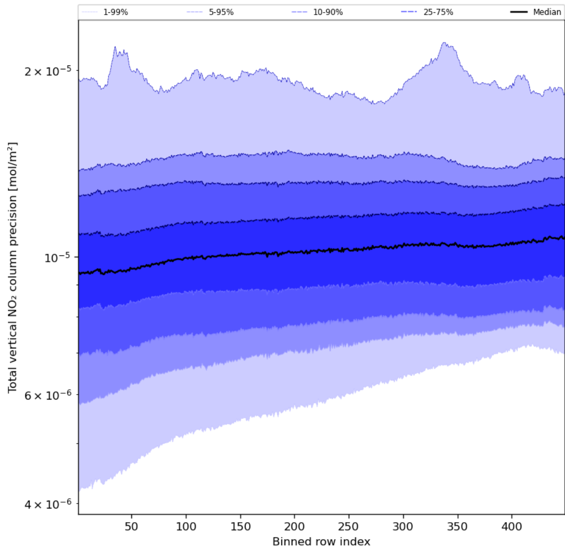
Figure 56: Along track statistics of “Total vertical NO 2 column precision” for 2024-04-15 to 2024-04-16
