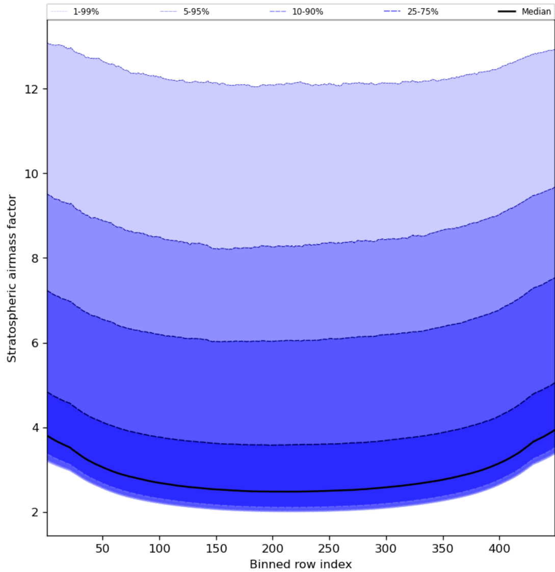
Figure 61: Along track statistics of “Stratospheric airmass factor” for 2024-04-15 to 2024-04-16
