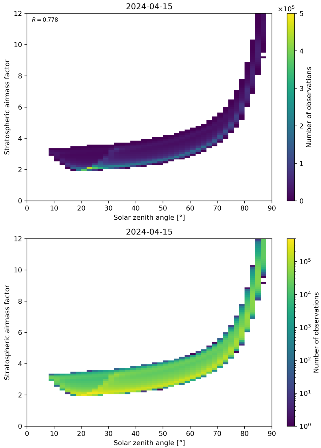
Figure 145: Scatter density plot of “Solar zenith angle” against “Stratospheric airmass factor” for 2024-04-15 to 2024-04-16.
