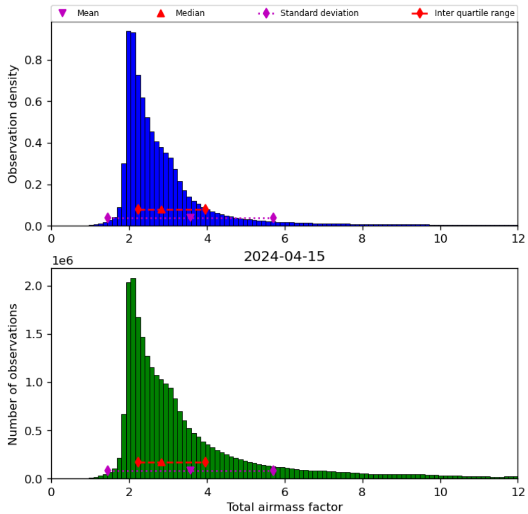
Figure 32: Histogram of “Total airmass factor” for 2024-04-15 to 2024-04-16
