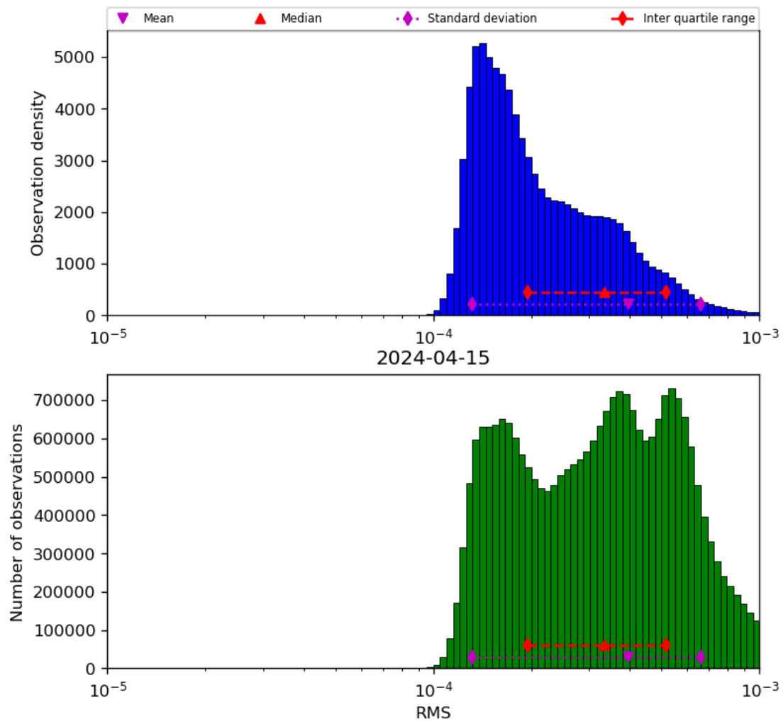
Figure 43: Histogram of “RMS” for 2024-04-15 to 2024-04-16
