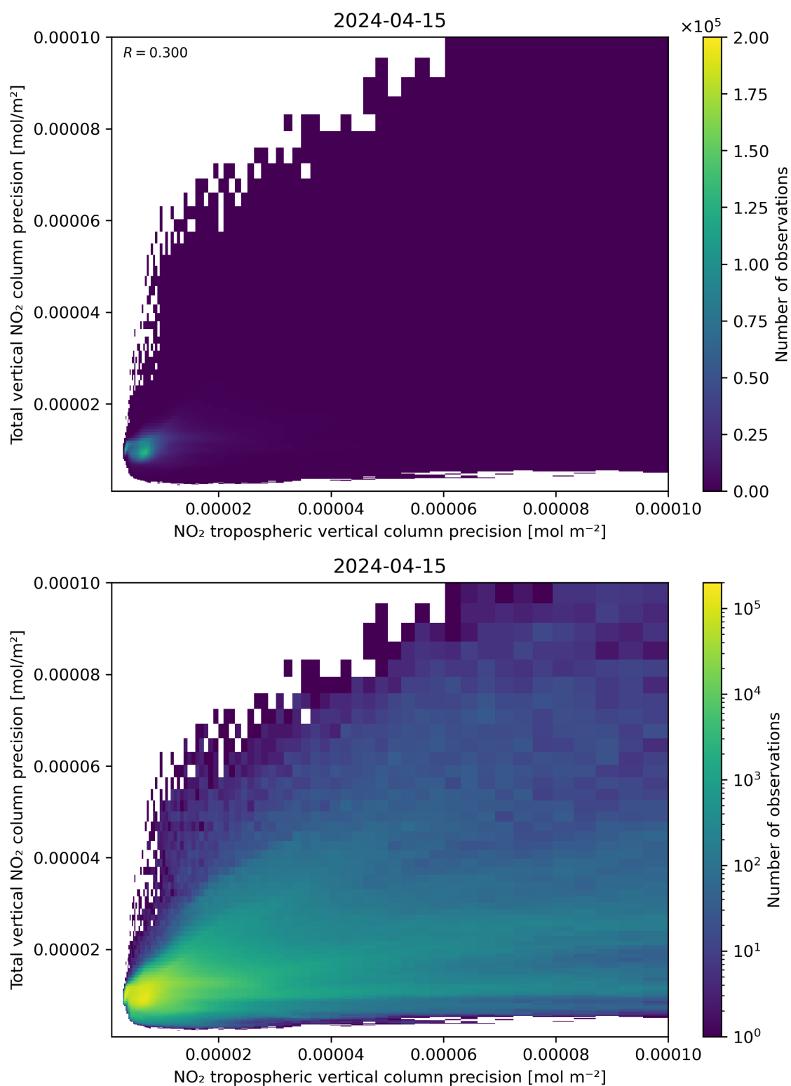
Figure 139: Scatter density plot of “NO 2 tropospheric vertical column precision” against “Total vertical NO 2 column precision” for 2024-04-15 to 2024-04-16.
