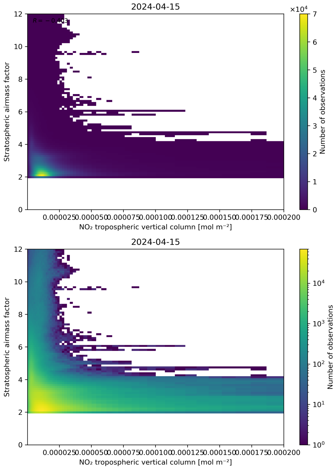
Figure 121: Scatter density plot of “NO 2 tropospheric vertical column” against “Stratospheric airmass factor” for 2024-04-15 to 2024-04-16.
