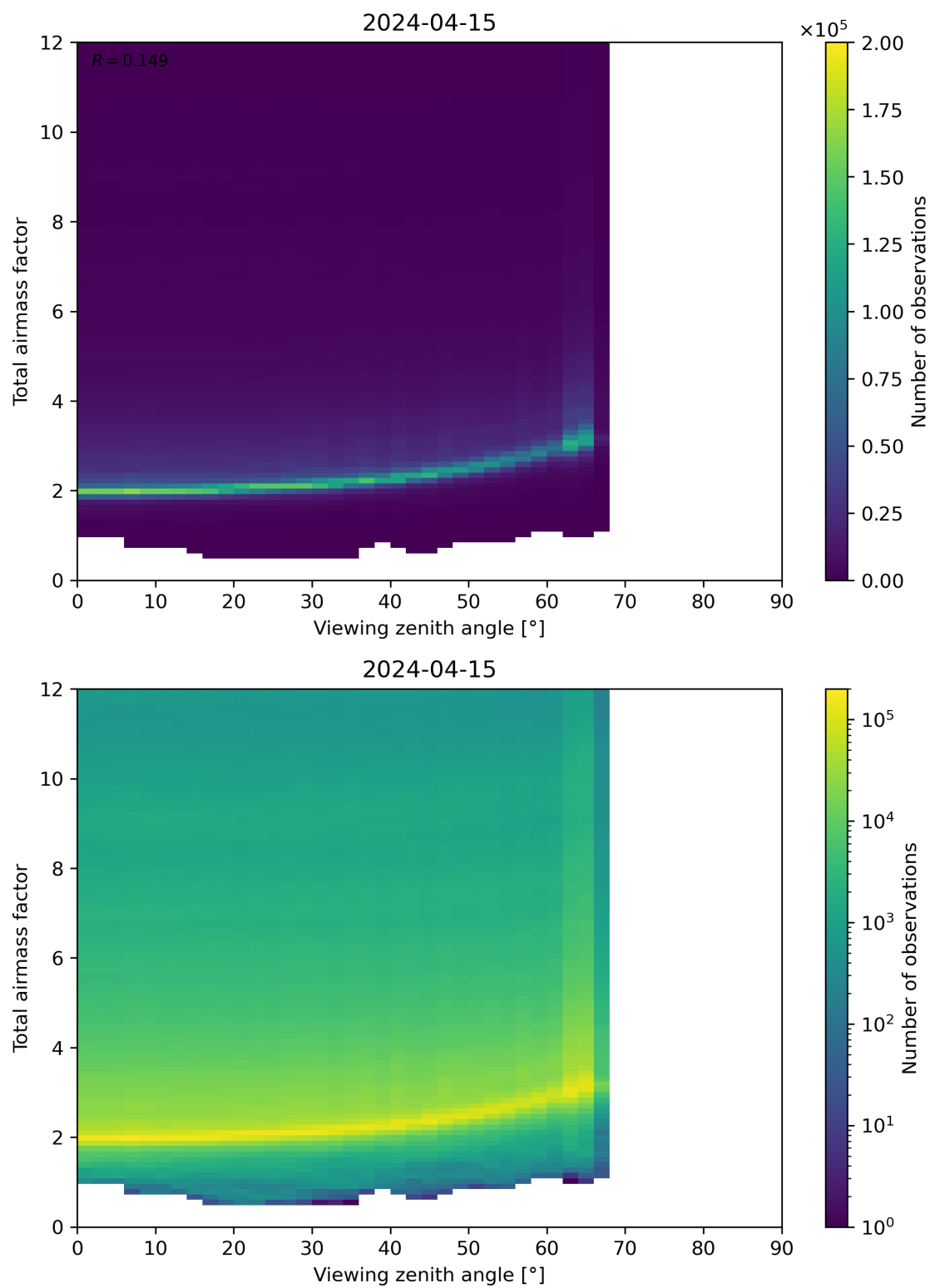
Figure 160: Scatter density plot of “Viewing zenith angle” against “Total airmass factor” for 2024-04-15 to 2024-04-16.
