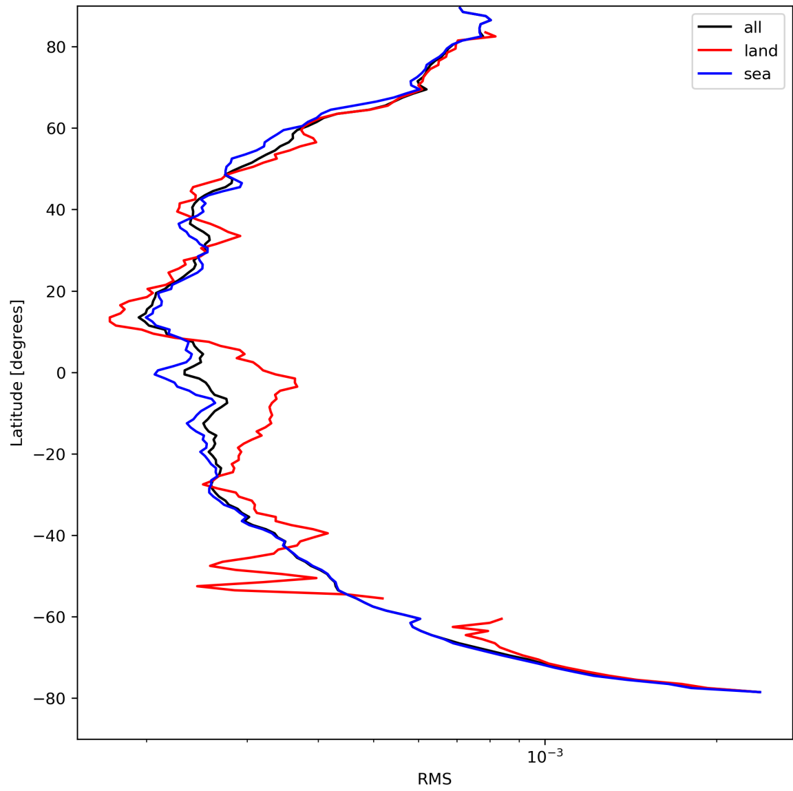
Figure 26: Zonal average of “RMS” for 2024-04-15 to 2024-04-16.
