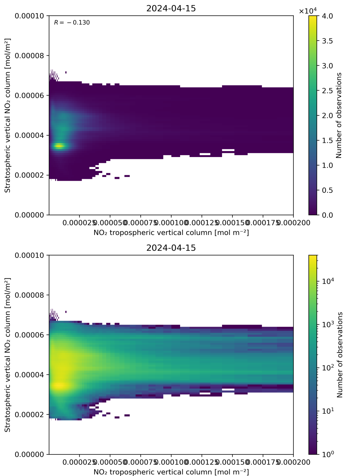
Figure 125: Scatter density plot of “NO 2 tropospheric vertical column” against “Stratospheric vertical NO 2 column” for 2024-04-15 to 2024-04-16.
