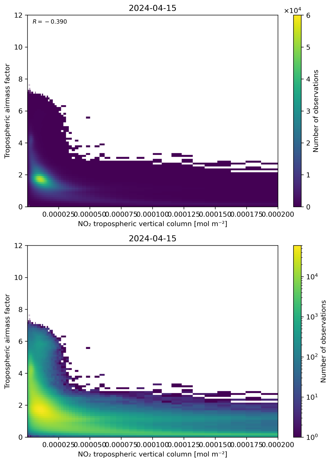
Figure 123: Scatter density plot of “NO 2 tropospheric vertical column” against “Tropospheric airmass factor” for 2024-04-15 to 2024-04-16.
