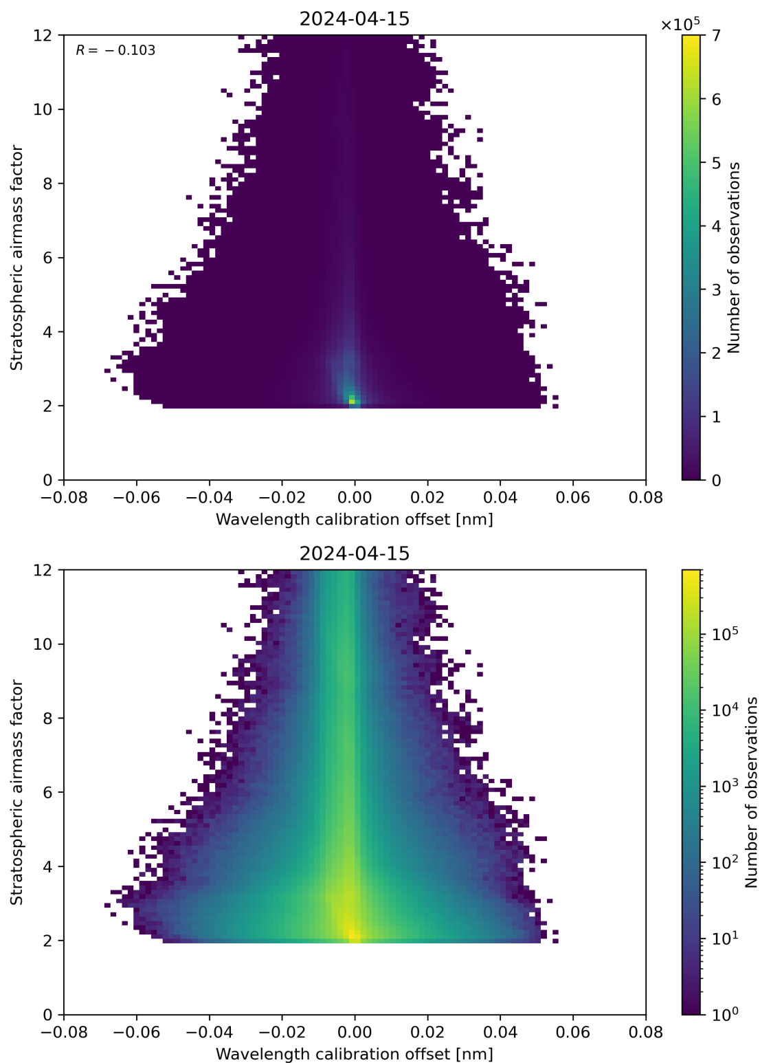
Figure 174: Scatter density plot of “Wavelength calibration offset” against “Stratospheric airmass factor” for 2024-04-15 to 2024-04-16.
