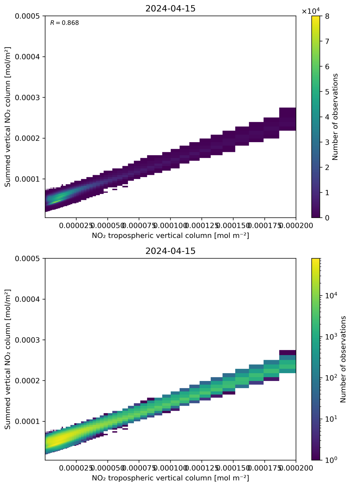
Figure 126: Scatter density plot of “NO 2 tropospheric vertical column” against “Summed vertical NO 2 column” for 2024-04-15 to 2024-04-16.
