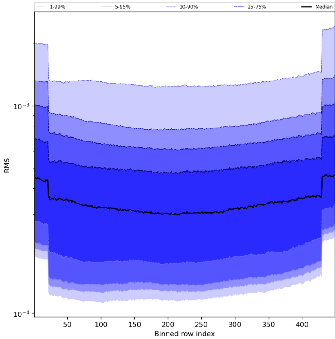
Figure 60: Along track statistics of “RMS” for 2024-04-15 to 2024-04-16
