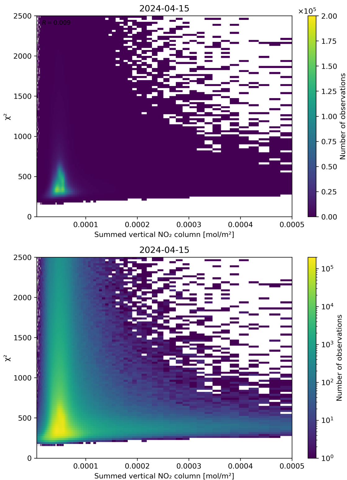
Figure 104: Scatter density plot of “Summed vertical NO 2 column” against “ \chi^2 ” for 2024-04-15 to 2024-04-16.
