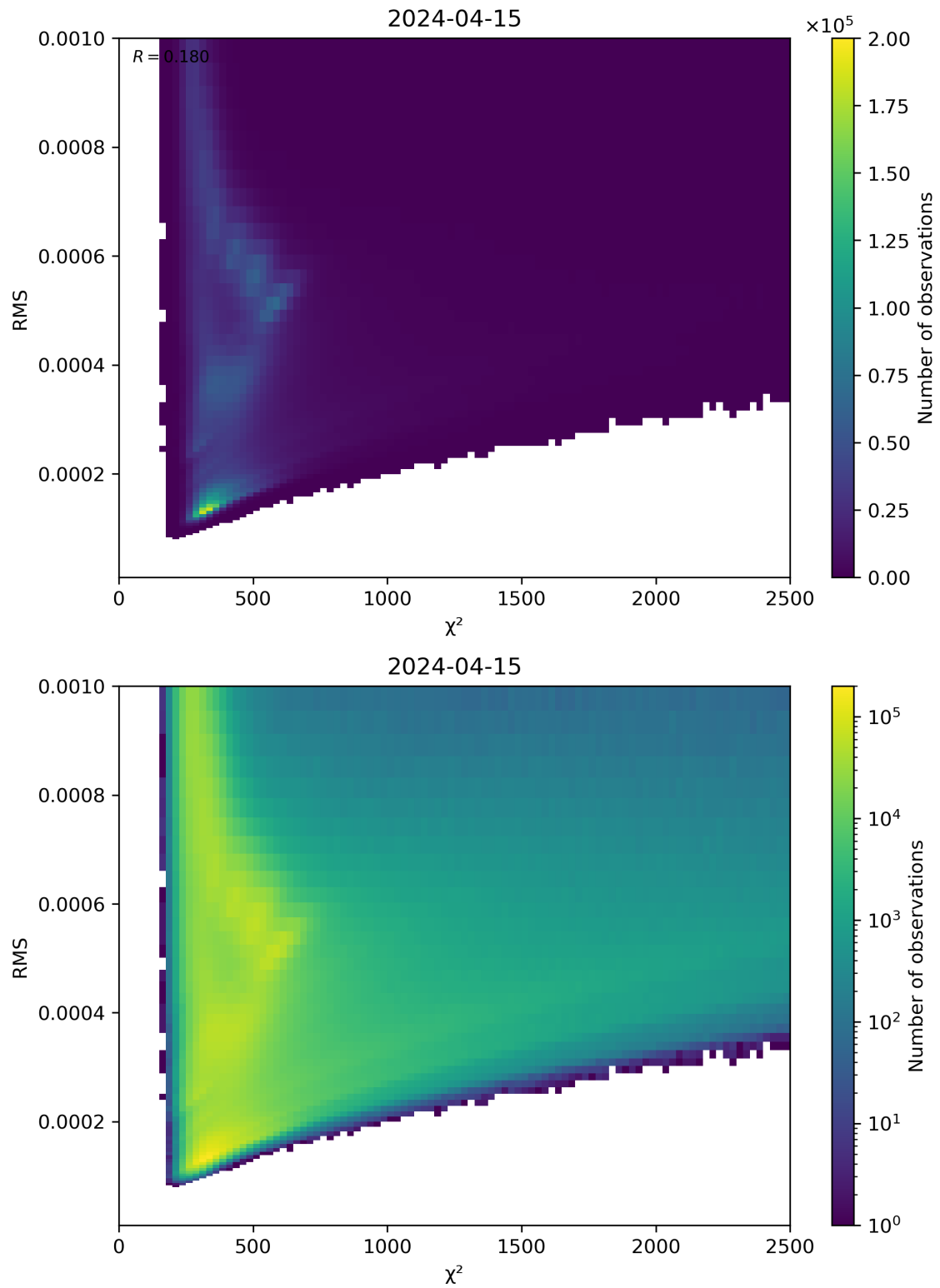
Figure 82: Scatter density plot of “ \chi^2 ” against “RMS” for 2024-04-15 to 2024-04-16.
