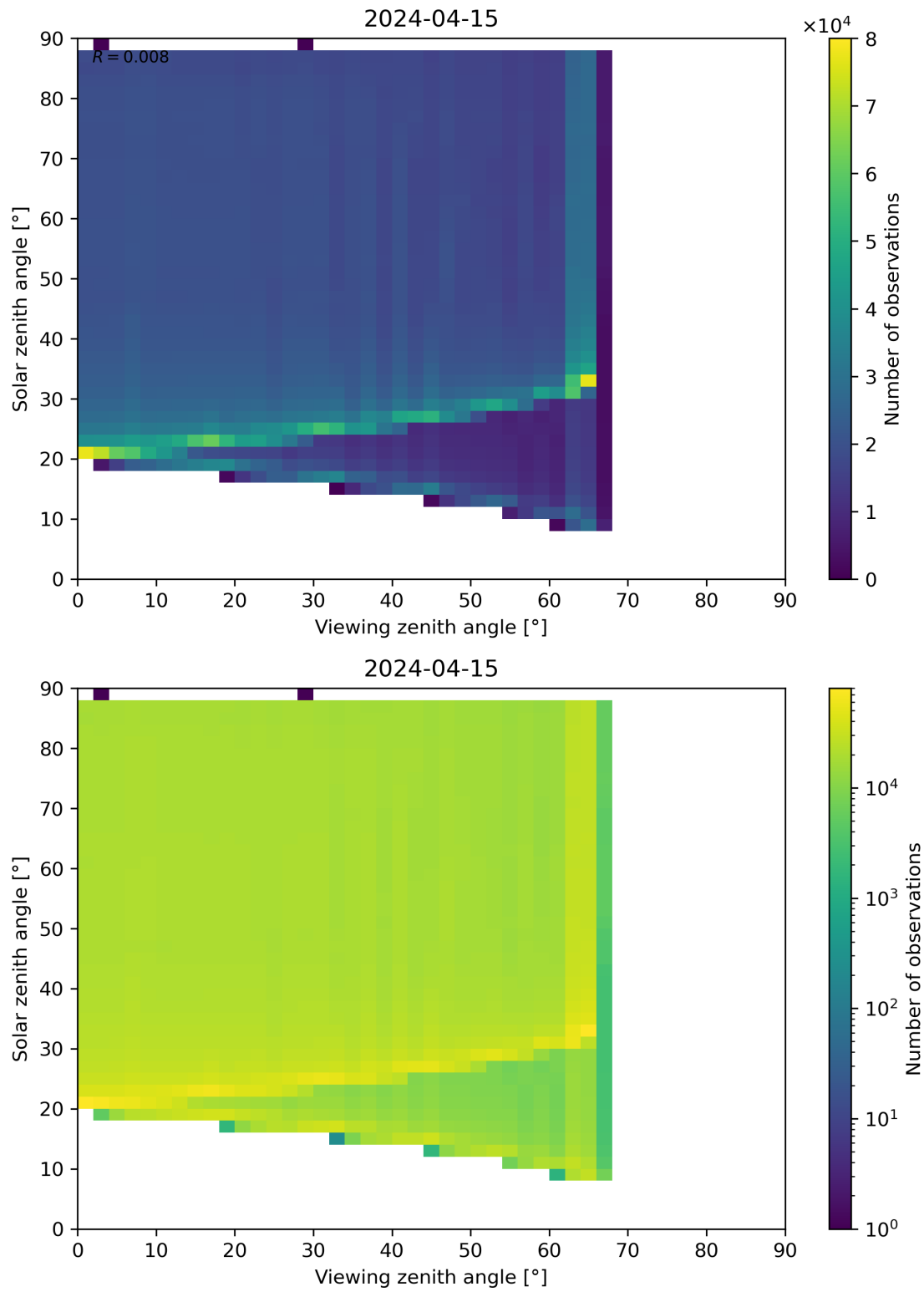
Figure 172: Scatter density plot of “Viewing zenith angle” against “Solar zenith angle” for 2024-04-15 to 2024-04-16.
