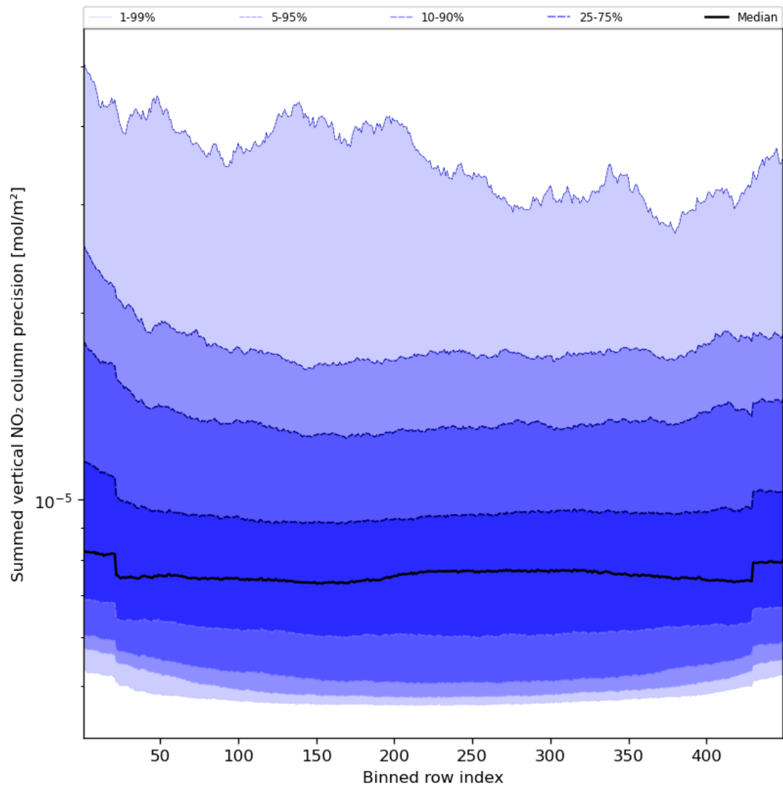
Figure 58: Along track statistics of “Summed vertical NO 2 column precision” for 2024-04-15 to 2024-04-16
