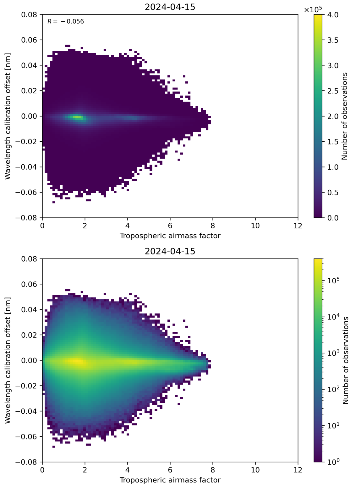
Figure 80: Scatter density plot of “Tropospheric airmass factor” against “Wavelength calibration offset” for 2024-04-15 to 2024-04-16.
