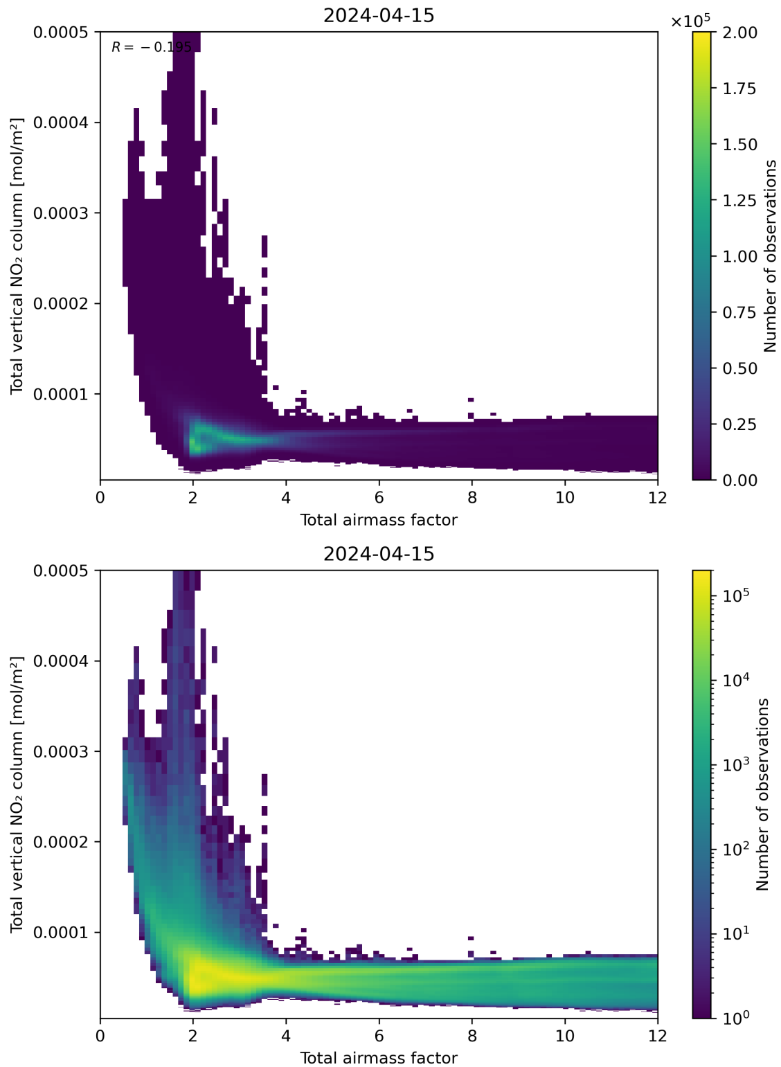
Figure 67: Scatter density plot of “Total airmass factor” against “Total vertical NO 2 column” for 2024-04-15 to 2024-04-16.
