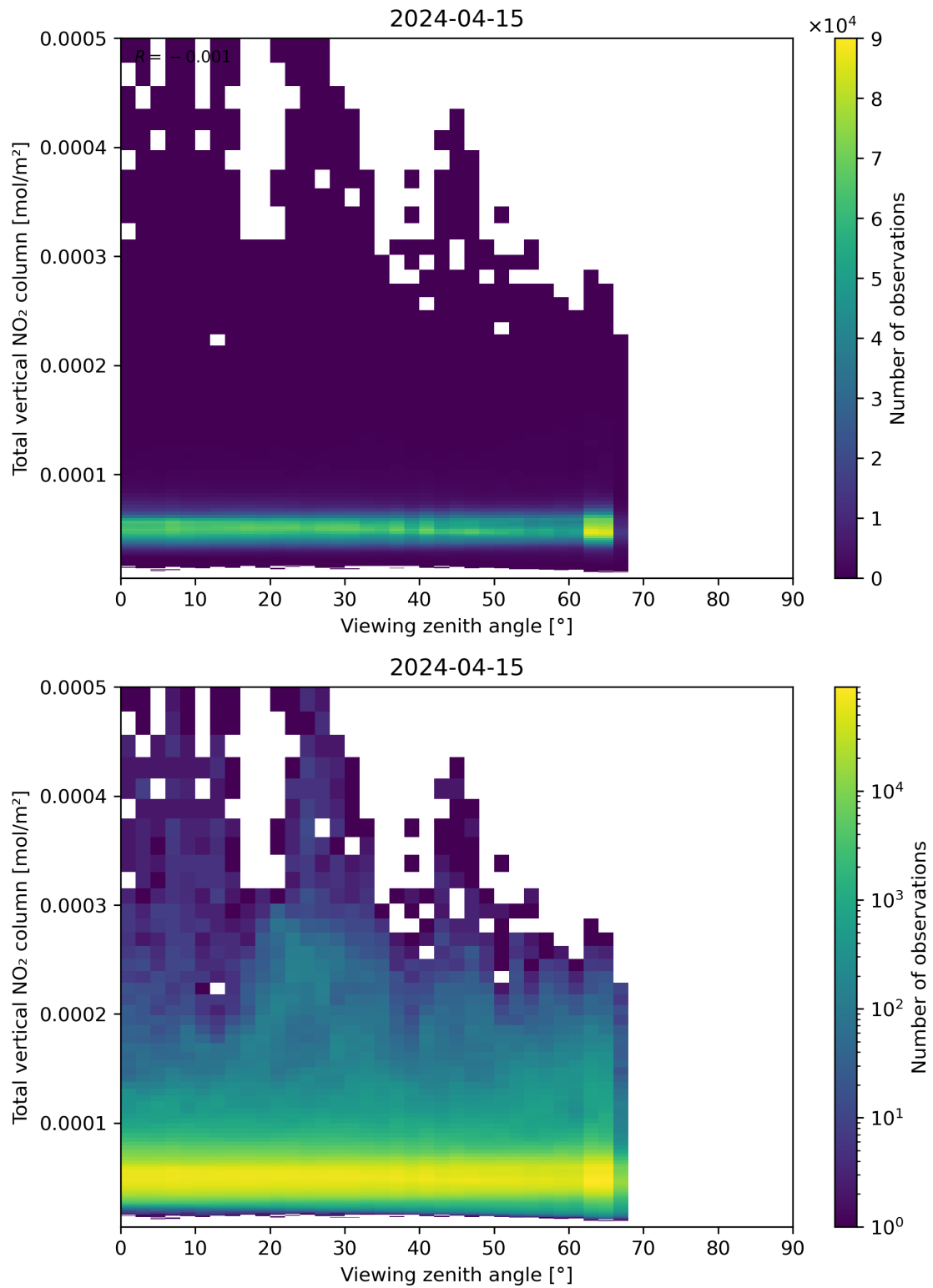
Figure 167: Scatter density plot of “Viewing zenith angle” against “Total vertical NO 2 column” for 2024-04-15 to 2024-04-16.
