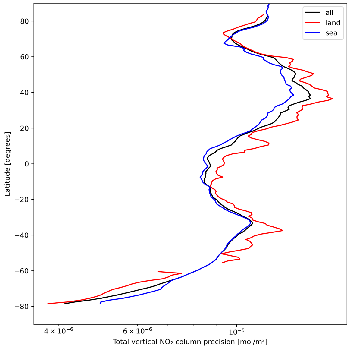
Figure 22: Zonal average of “Total vertical NO 2 column precision” for 2024-04-15 to 2024-04-16.
