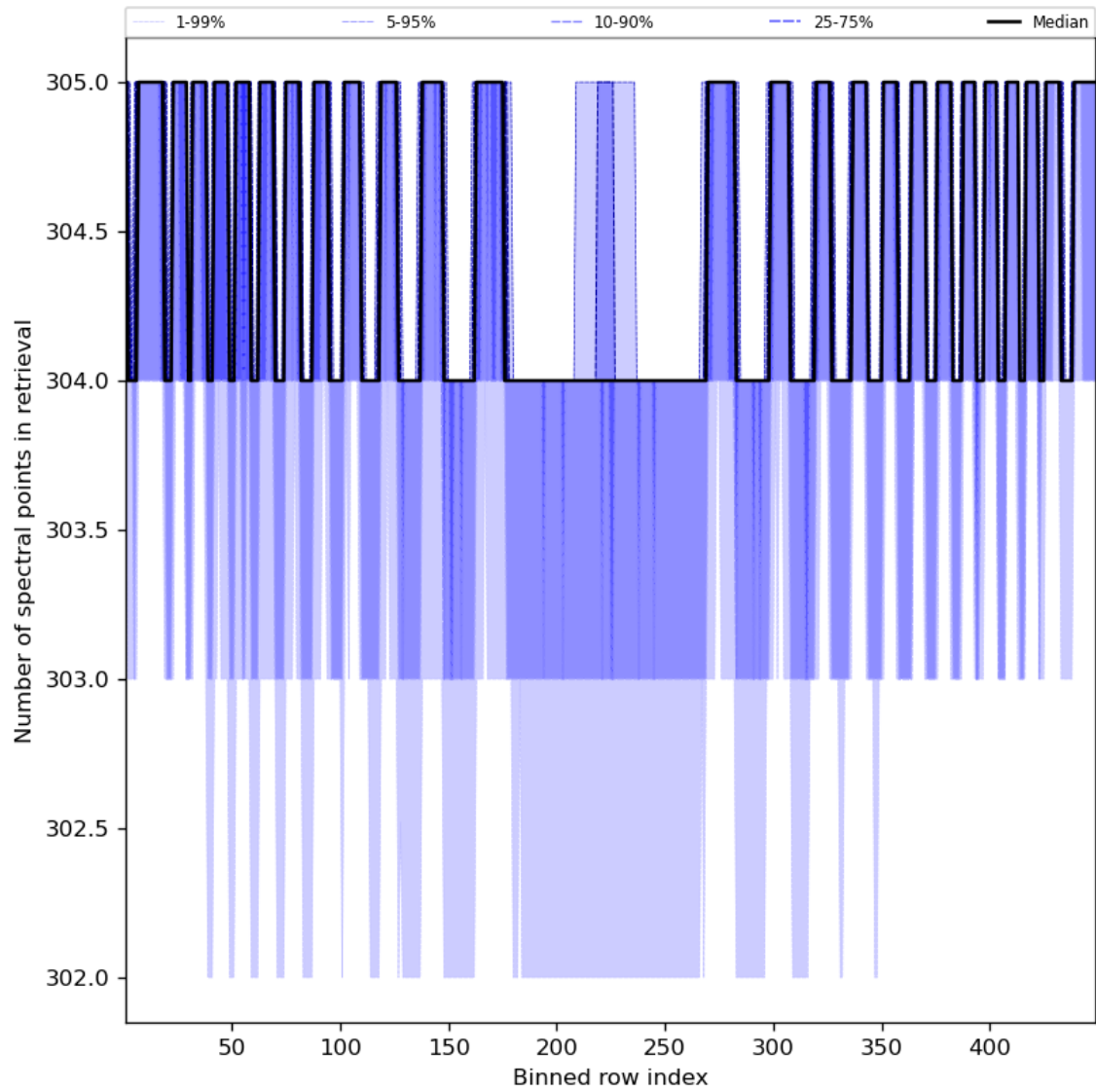
Figure 50: Along track statistics of “Number of spectral points in retrieval” for 2024-04-15 to 2024-04-16
