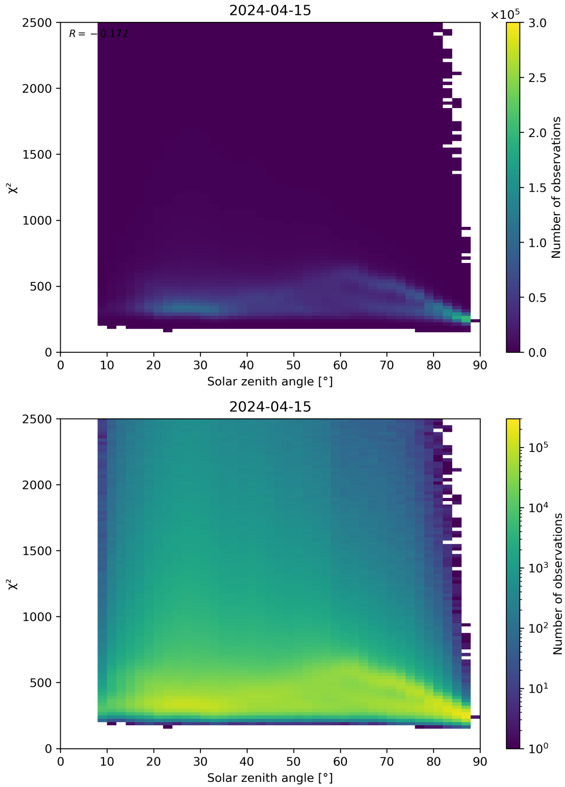
Figure 148: Scatter density plot of “Solar zenith angle” against “ \chi^2 ” for 2024-04-15 to 2024-04-16.
