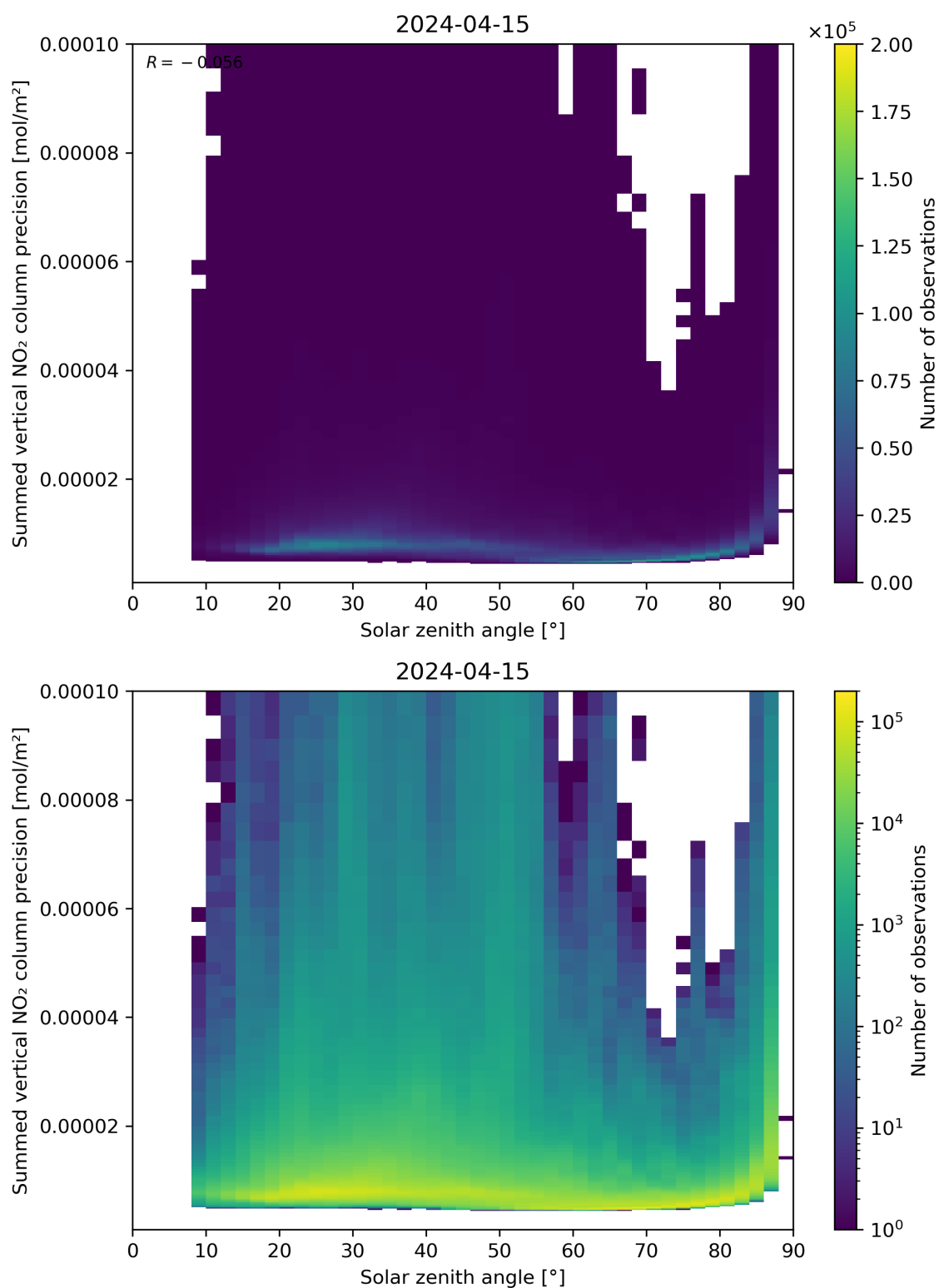
Figure 152: Scatter density plot of “Solar zenith angle” against “Summed vertical NO 2 column precision” for 2024-04-15 to 2024-04-16.
