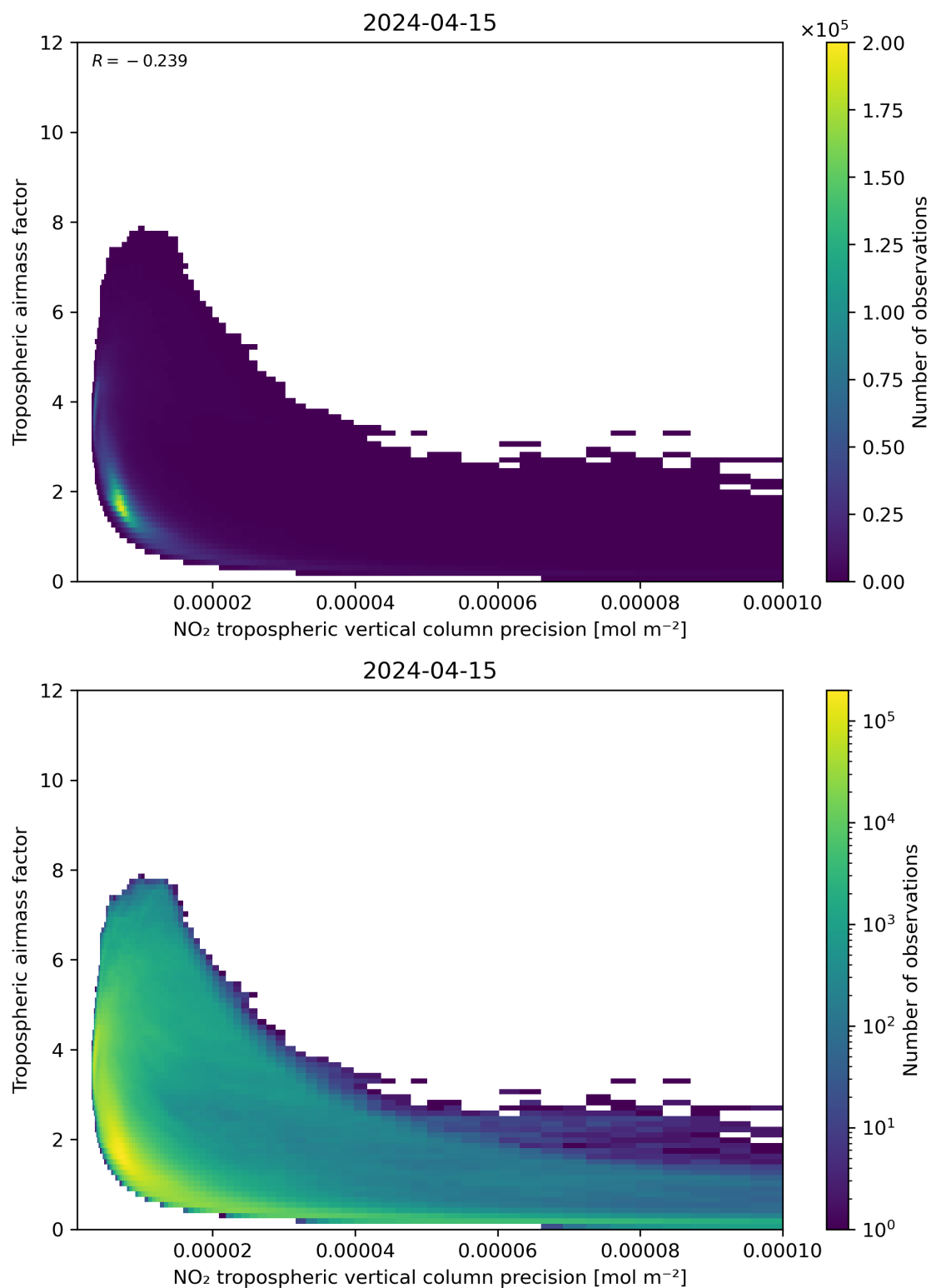
Figure 133: Scatter density plot of “NO 2 tropospheric vertical column precision” against “Tropospheric airmass factor” for 2024-04-15 to 2024-04-16.
