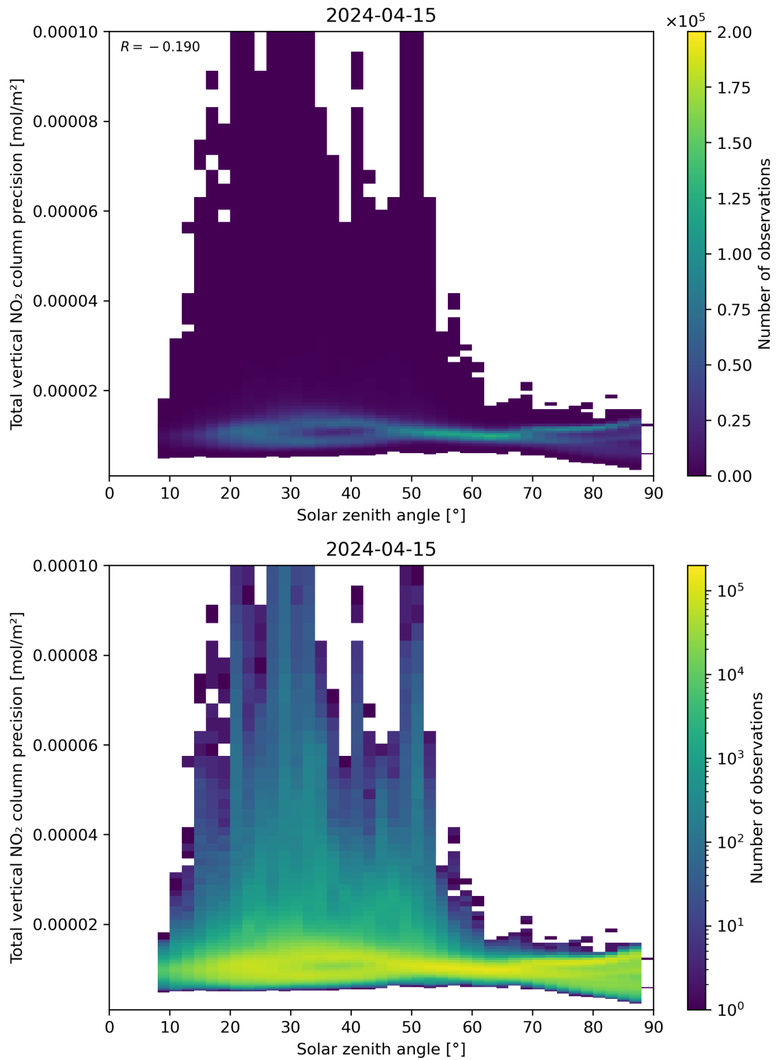
Figure 154: Scatter density plot of “Solar zenith angle” against “Total vertical NO 2 column precision” for 2024-04-15 to 2024-04-16.
