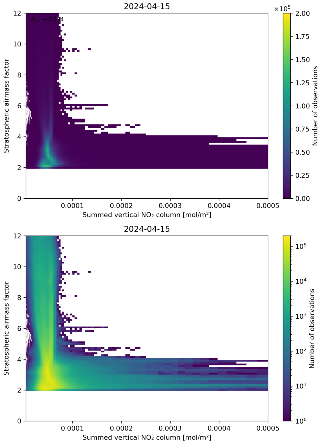
Figure 103: Scatter density plot of “Summed vertical NO 2 column” against “Stratospheric air mass factor” for 2024-04-15 to 2024-04-16.
