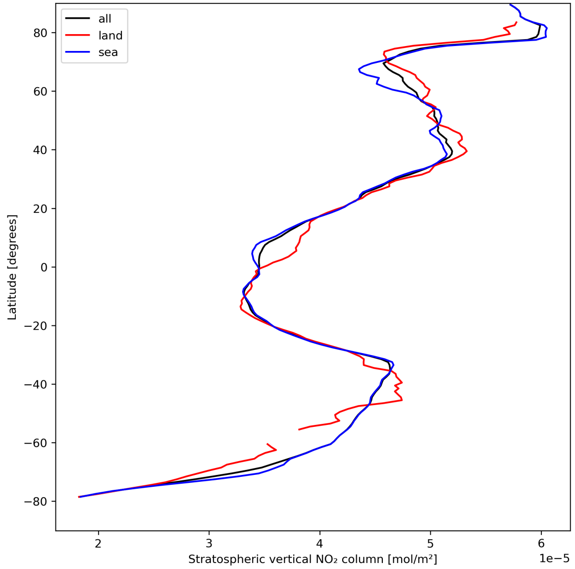
Figure 19: Zonal average of “Stratospheric vertical NO 2 column” for 2024-04-15 to 2024-04-16.
