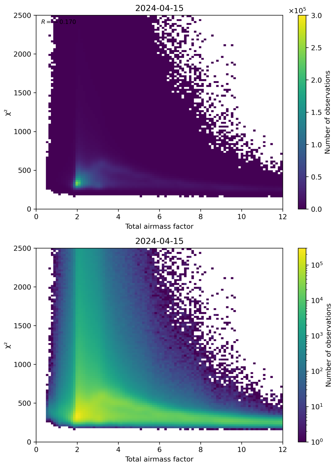
Figure 63: Scatter density plot of “Total airmass factor” against “ \chi^2 ” for 2024-04-15 to 2024-04-16.
