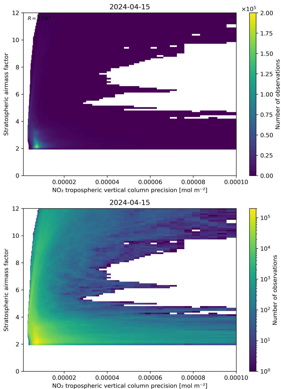
Figure 131: Scatter density plot of “NO 2 tropospheric vertical column precision” against “Stratospheric airmass factor” for 2024-04-15 to 2024-04-16.
