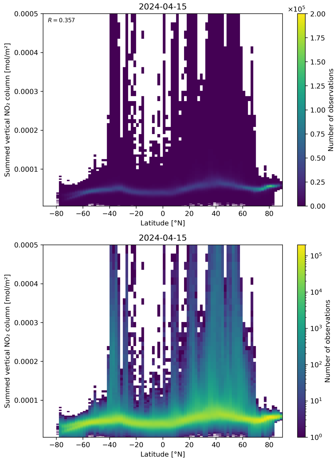
Figure 88: Scatter density plot of “Latitude” against “Summed vertical NO 2 column” for 2024-04-15 to 2024-04-16.
