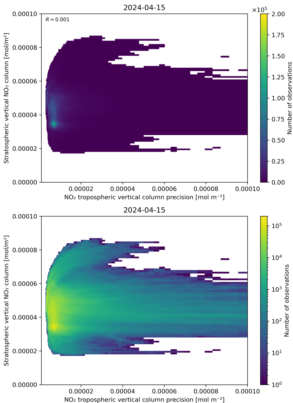
Figure 135: Scatter density plot of “NO 2 tropospheric vertical column precision” against “Stratospheric vertical NO 2 column” for 2024-04-15 to 2024-04-16.
