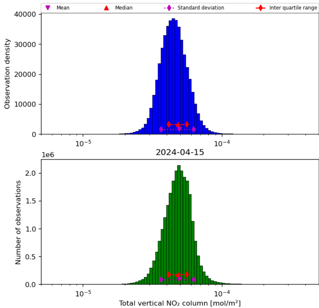
Figure 38: Histogram of "Total vertical NO 2 column" for 2024-04-15 to 2024-04-16
