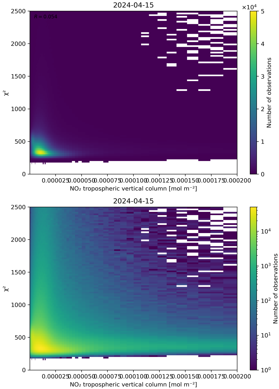
Figure 124: Scatter density plot of “NO 2 tropospheric vertical column” against “ \chi^2 ” for 2024-04-15 to 2024-04-16.
