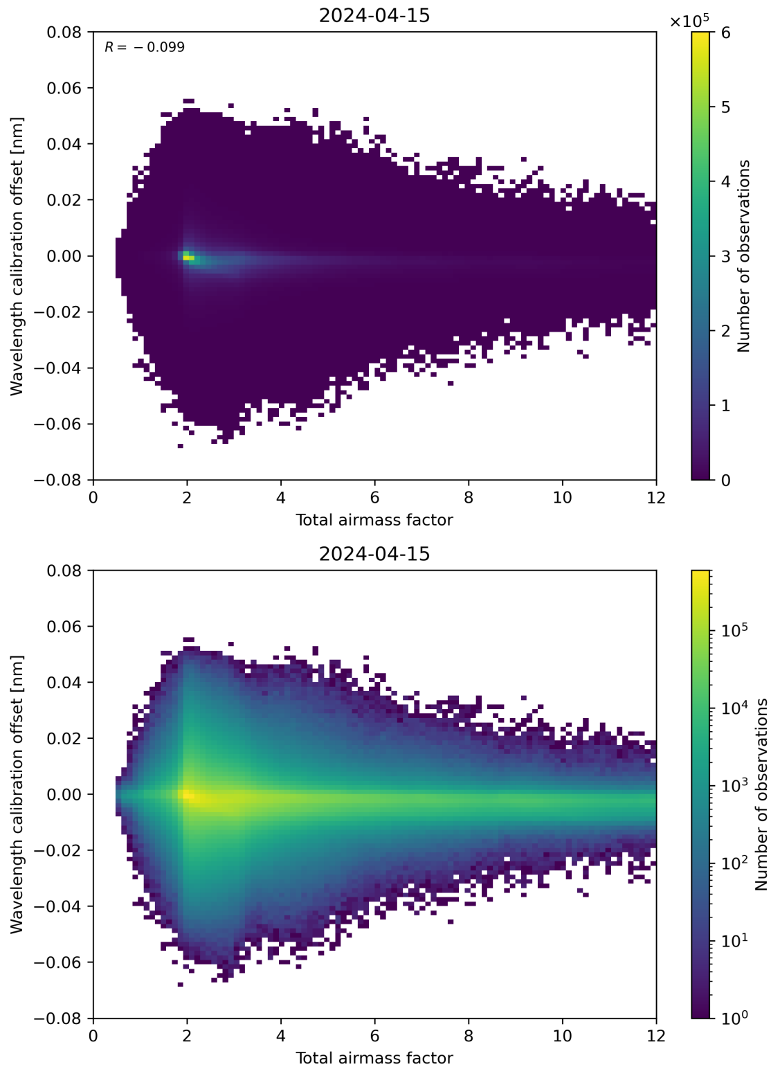
Figure 70: Scatter density plot of “Total airmass factor” against “Wavelength calibration offset” for 2024-04-15 to 2024-04-16.
