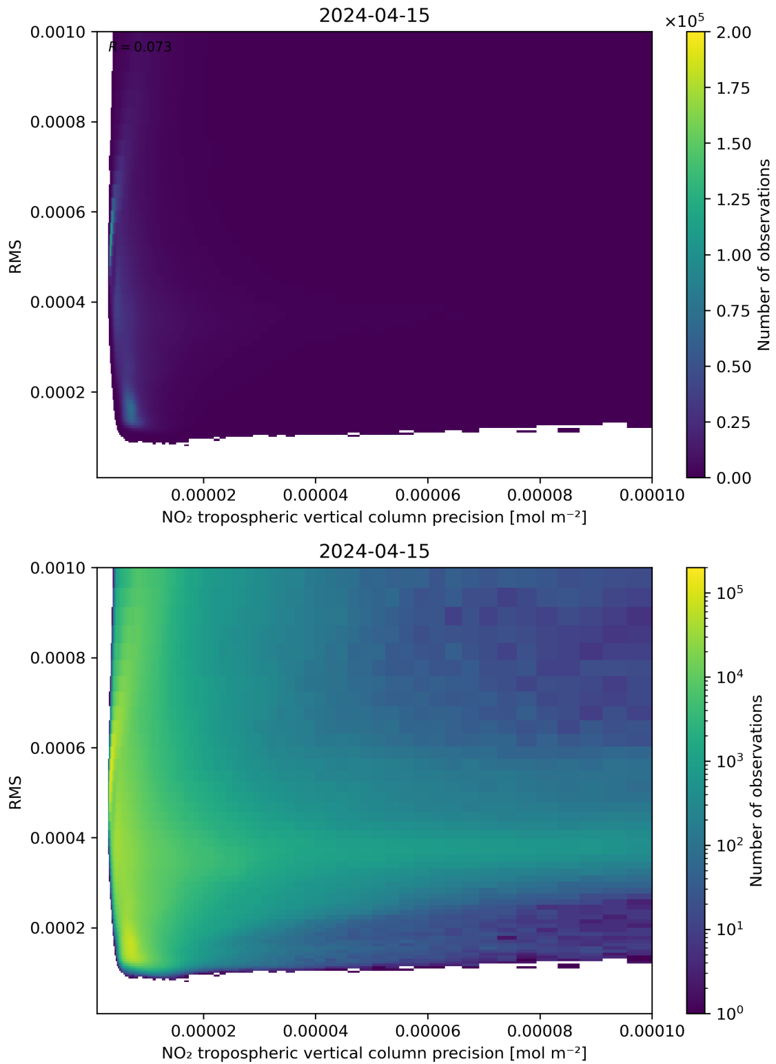
Figure 140: Scatter density plot of “NO 2 tropospheric vertical column precision” against “RMS” for 2024-04-15 to 2024-04-16.
