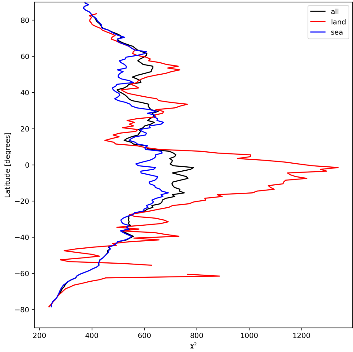
Figure 25: Zonal average of “ \chi^2 ” for 2024-04-15 to 2024-04-16.
