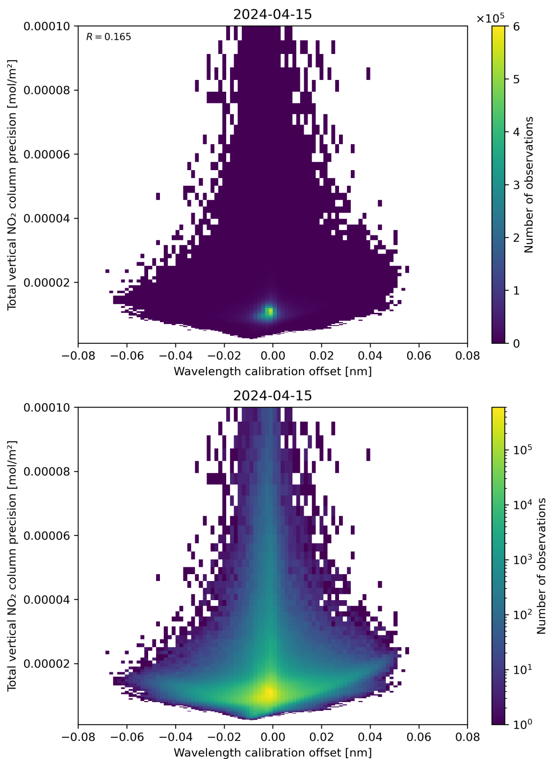
Figure 180: Scatter density plot of “Wavelength calibration offset” against “Total vertical NO 2 column precision” for 2024-04-15 to 2024-04-16.
