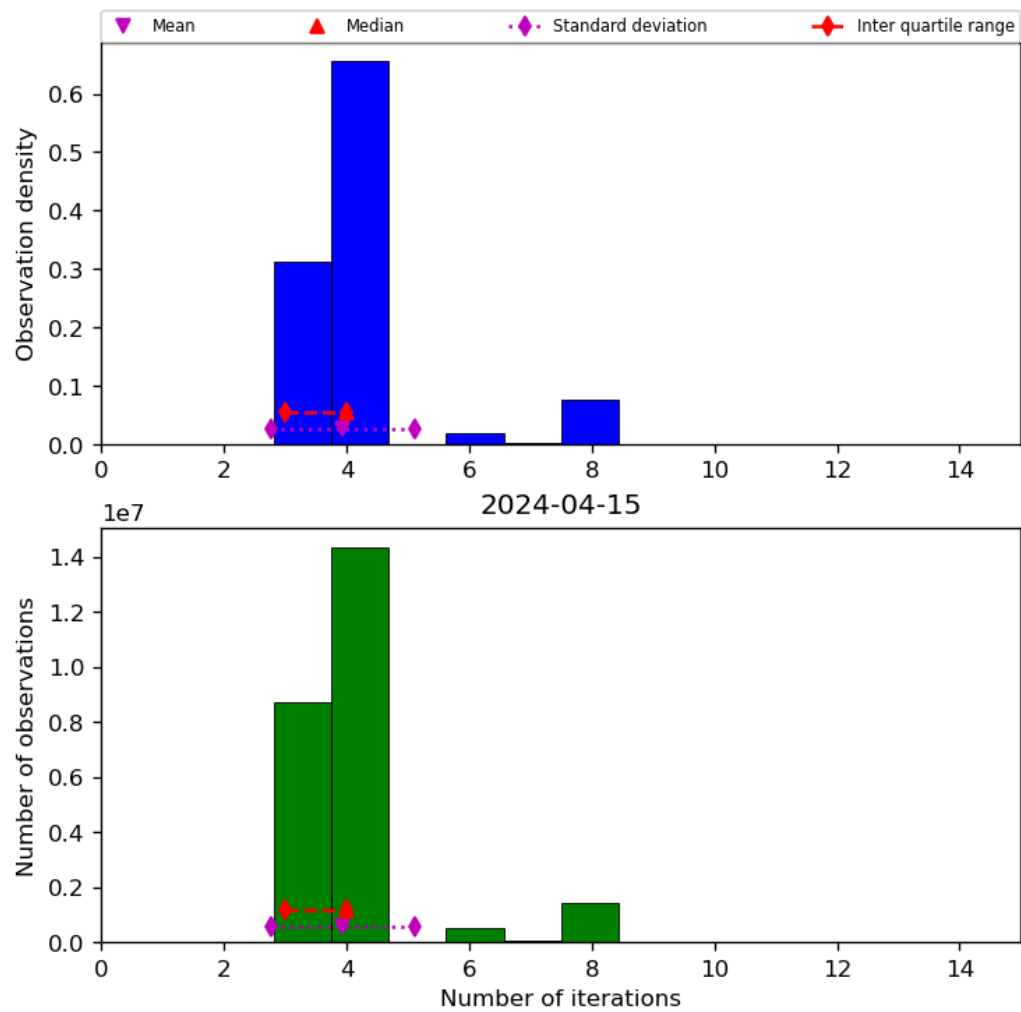
Figure 34: Histogram of “Number of iterations” for 2024-04-15 to 2024-04-16
