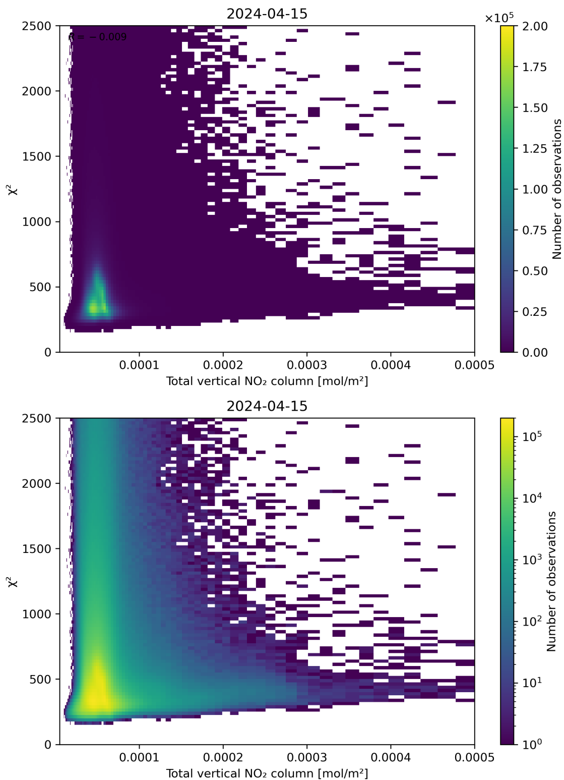
Figure 111: Scatter density plot of “Total vertical NO 2 column” against “ \chi^2 ” for 2024-04-15 to 2024-04-16.
