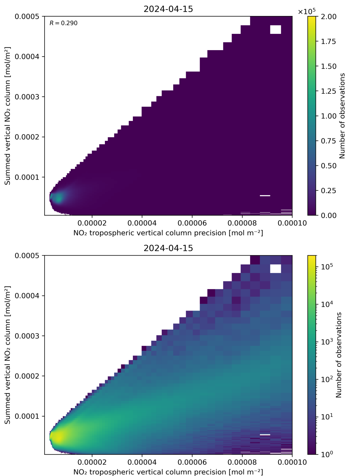
Figure 136: Scatter density plot of “NO 2 tropospheric vertical column precision” against “Summed vertical NO 2 column” for 2024-04-15 to 2024-04-16.
