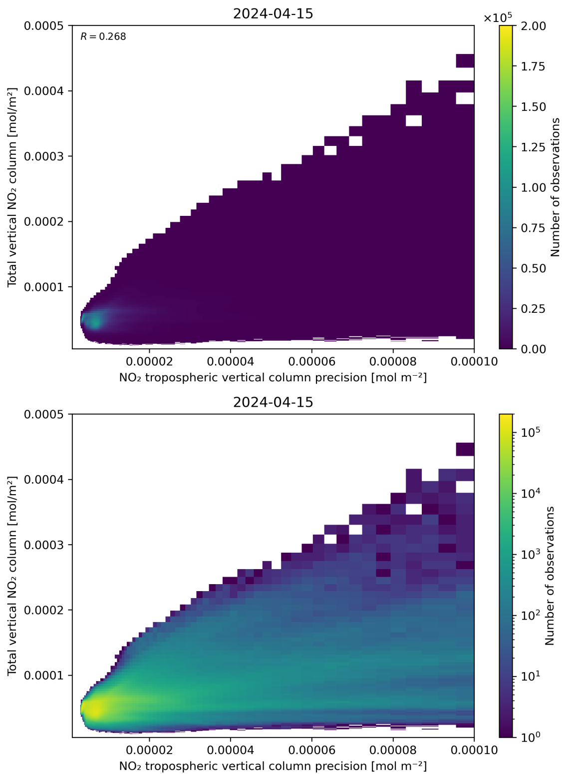
Figure 138: Scatter density plot of “NO 2 tropospheric vertical column precision” against “Total vertical NO 2 column” for 2024-04-15 to 2024-04-16.
