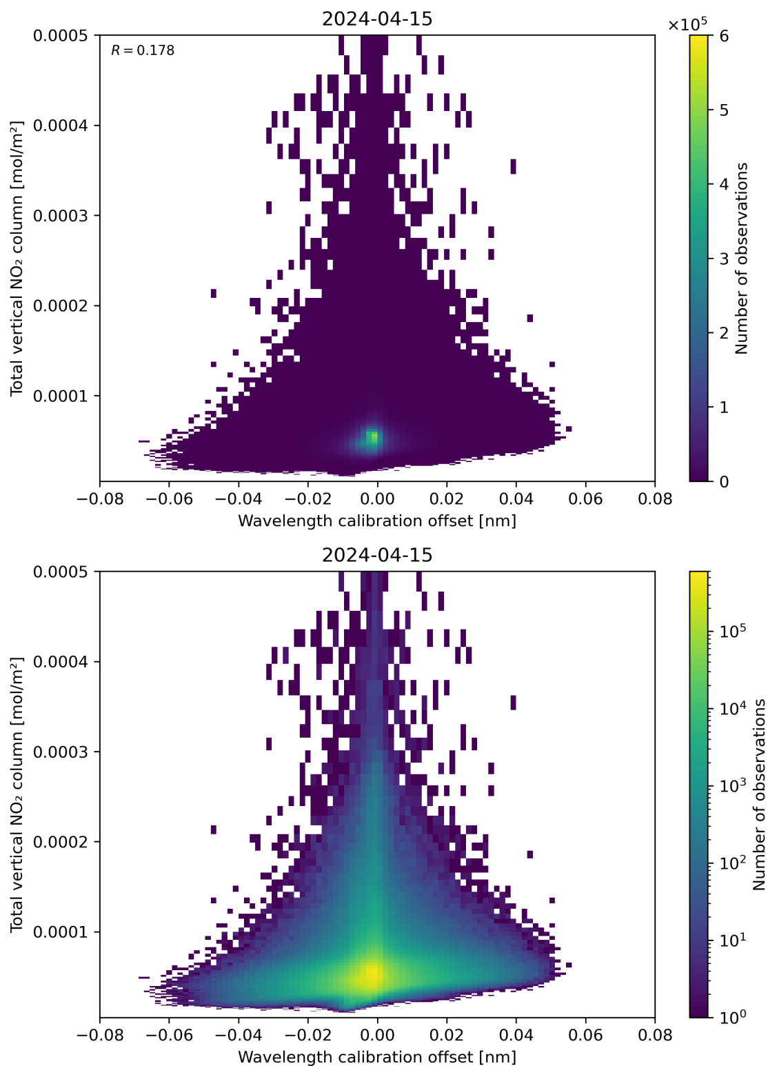
Figure 179: Scatter density plot of “Wavelength calibration offset” against “Total vertical NO 2 column” for 2024-04-15 to 2024-04-16.
