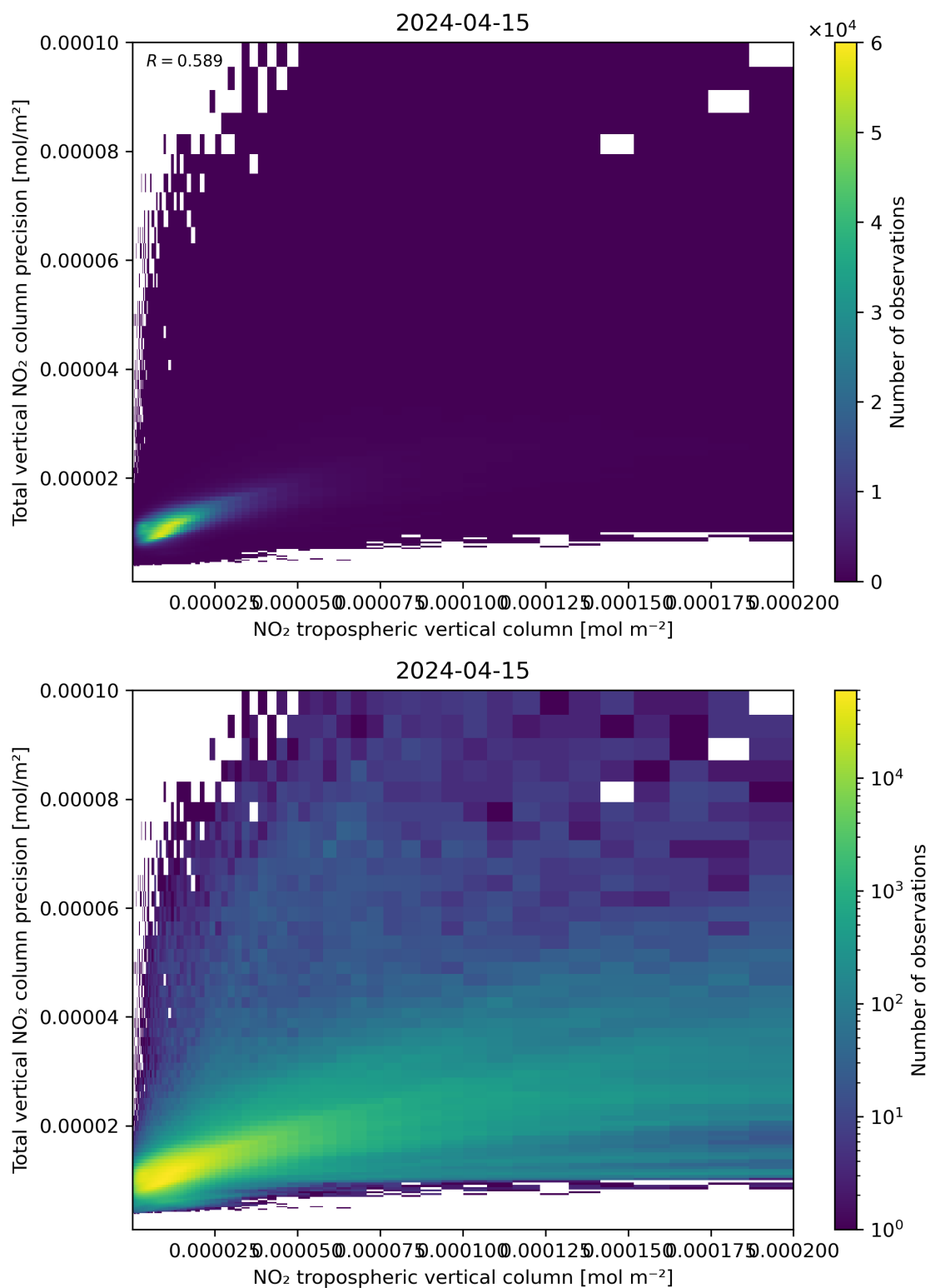
Figure 129: Scatter density plot of “NO 2 tropospheric vertical column” against “Total vertical NO 2 column precision” for 2024-04-15 to 2024-04-16.
