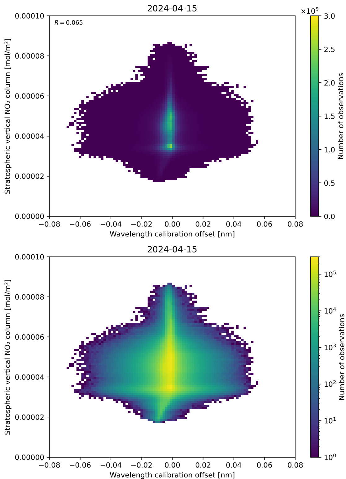
Figure 176: Scatter density plot of “Wavelength calibration offset” against “Stratospheric vertical NO 2 column” for 2024-04-15 to 2024-04-16.
