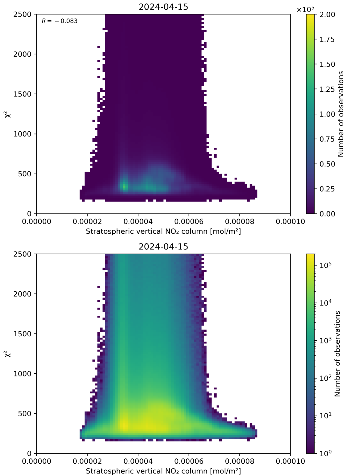
Figure 97: Scatter density plot of “Stratospheric vertical NO 2 column” against “ \chi^2 ” for 2024-04-15 to 2024-04-16.
