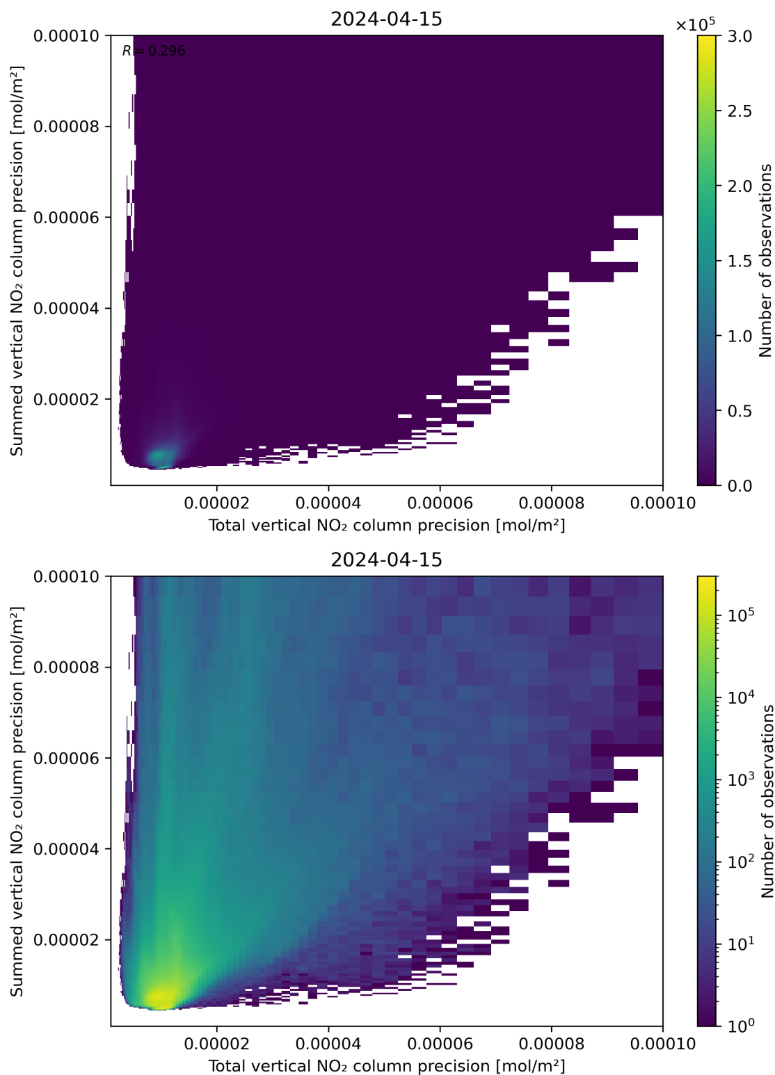
Figure 118: Scatter density plot of “Total vertical NO 2 column precision” against “Summed vertical NO 2 column precision” for 2024-04-15 to 2024-04-16.
