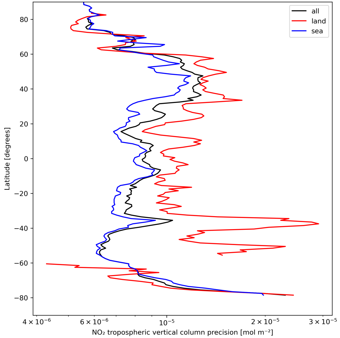
Figure 13: Zonal average of “NO 2 tropospheric vertical column precision” for 2024-04-15 to 2024-04-16.
