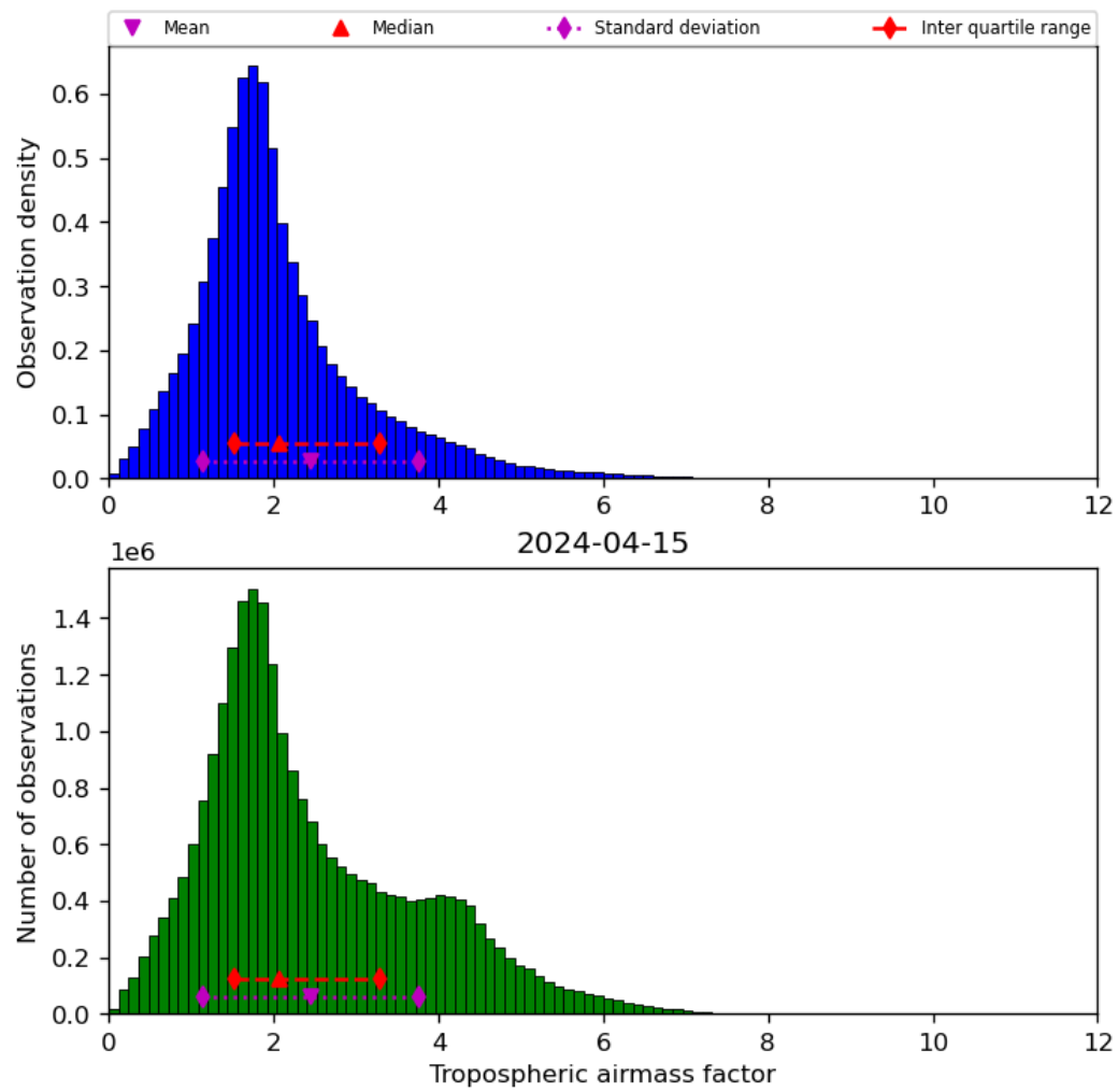
Figure 31: Histogram of “Tropospheric airmass factor” for 2024-04-15 to 2024-04-16
