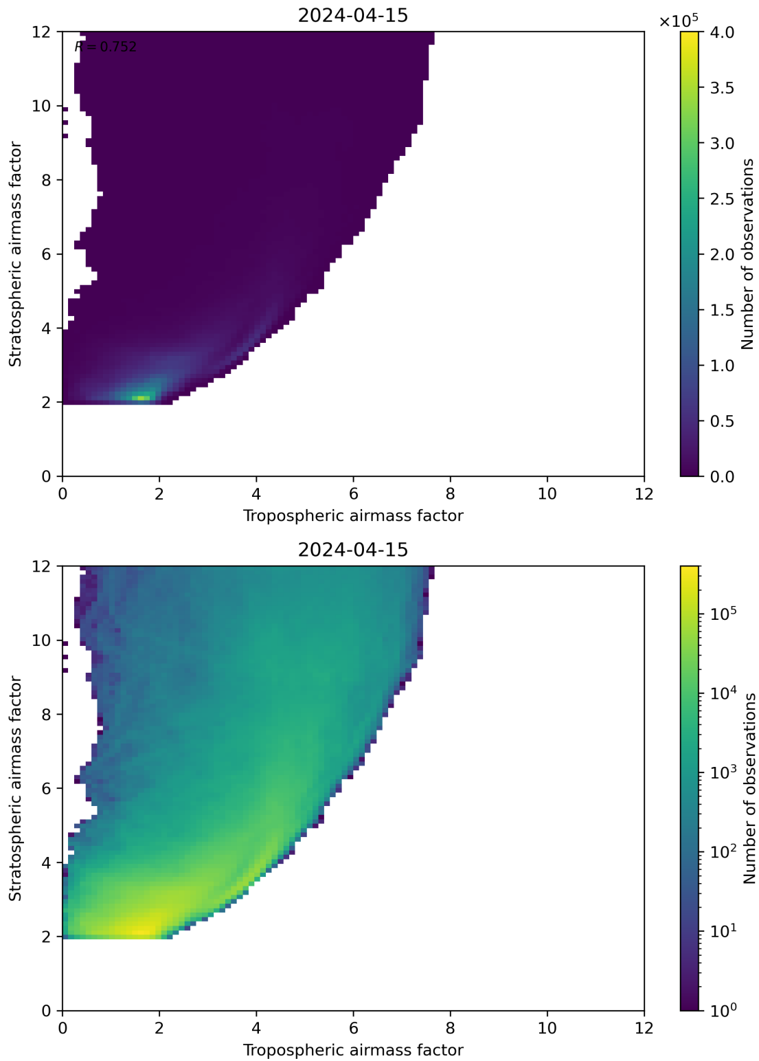
Figure 71: Scatter density plot of “Tropospheric airmass factor” against “Stratospheric airmass factor” for 2024-04-15 to 2024-04-16.
