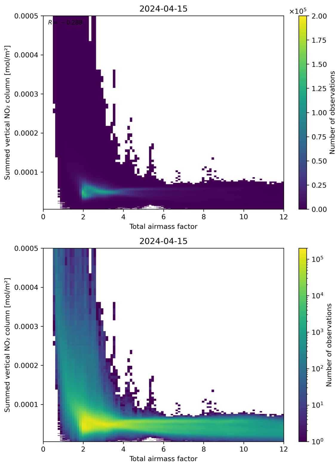
Figure 65: Scatter density plot of “Total airmass factor” against “Summed vertical NO 2 column” for 2024-04-15 to 2024-04-16.
