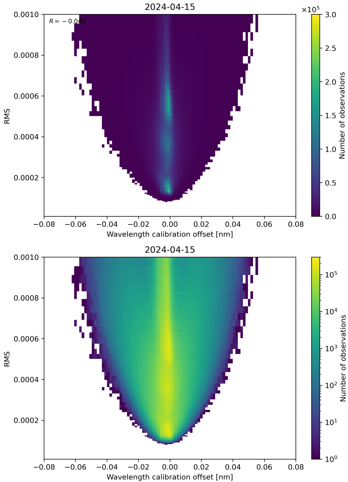
Figure 181: Scatter density plot of “Wavelength calibration offset” against “RMS” for 2024-04-15 to 2024-04-16.
