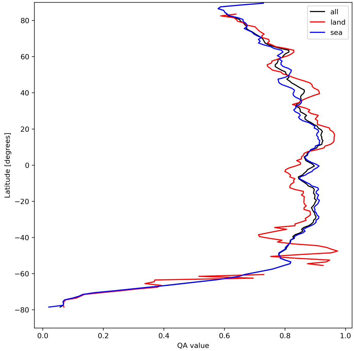
Figure 11: Zonal average of “QA value” for 2024-04-15 to 2024-04-16.
