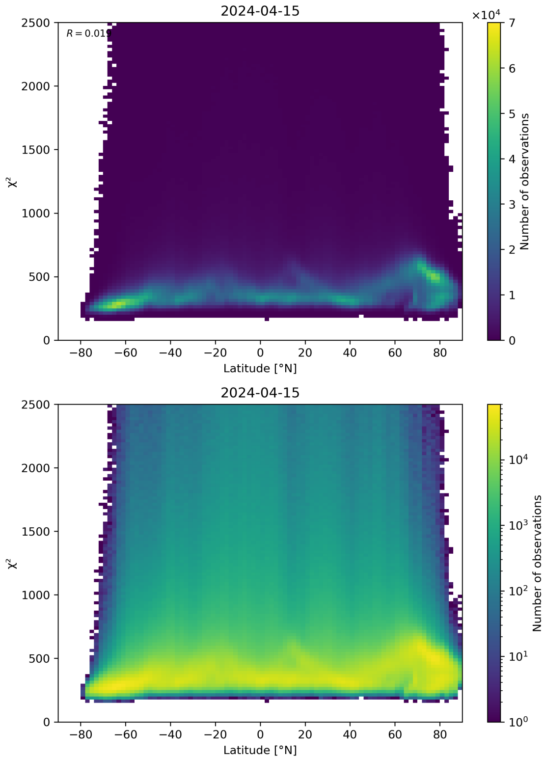
Figure 86: Scatter density plot of “Latitude” against “ \chi^2 ” for 2024-04-15 to 2024-04-16.
