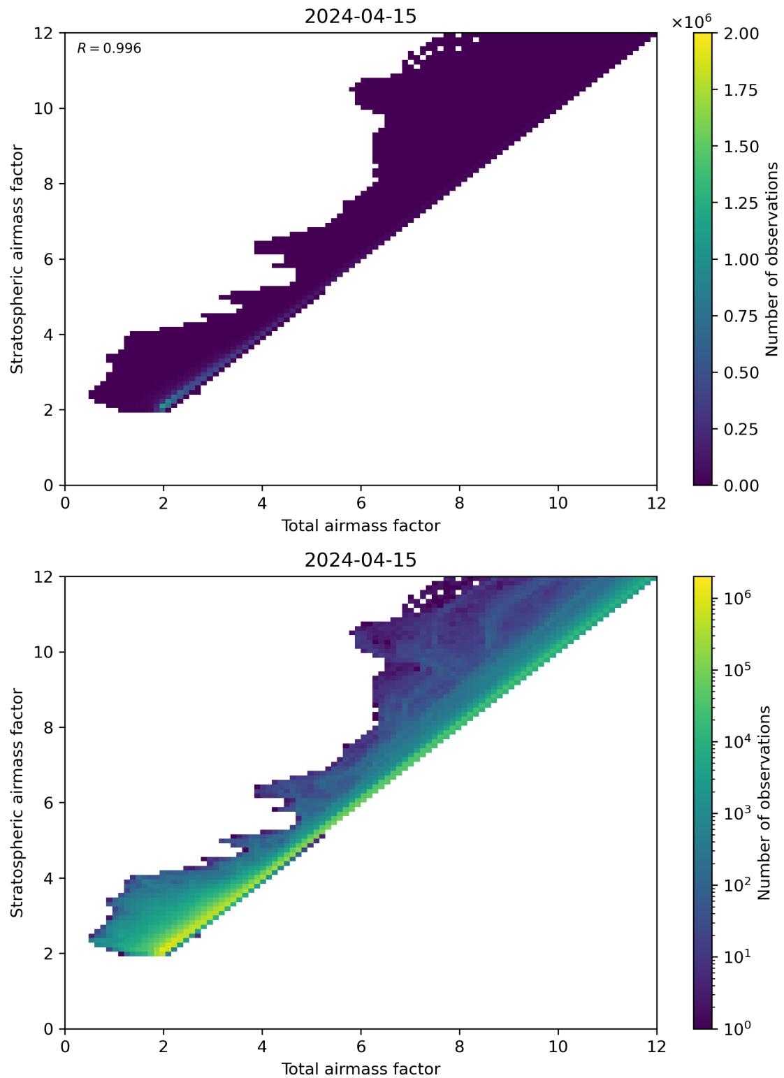
Figure 62: Scatter density plot of “Total airmass factor” against “Stratospheric airmass factor” for 2024-04-15 to 2024-04-16.
