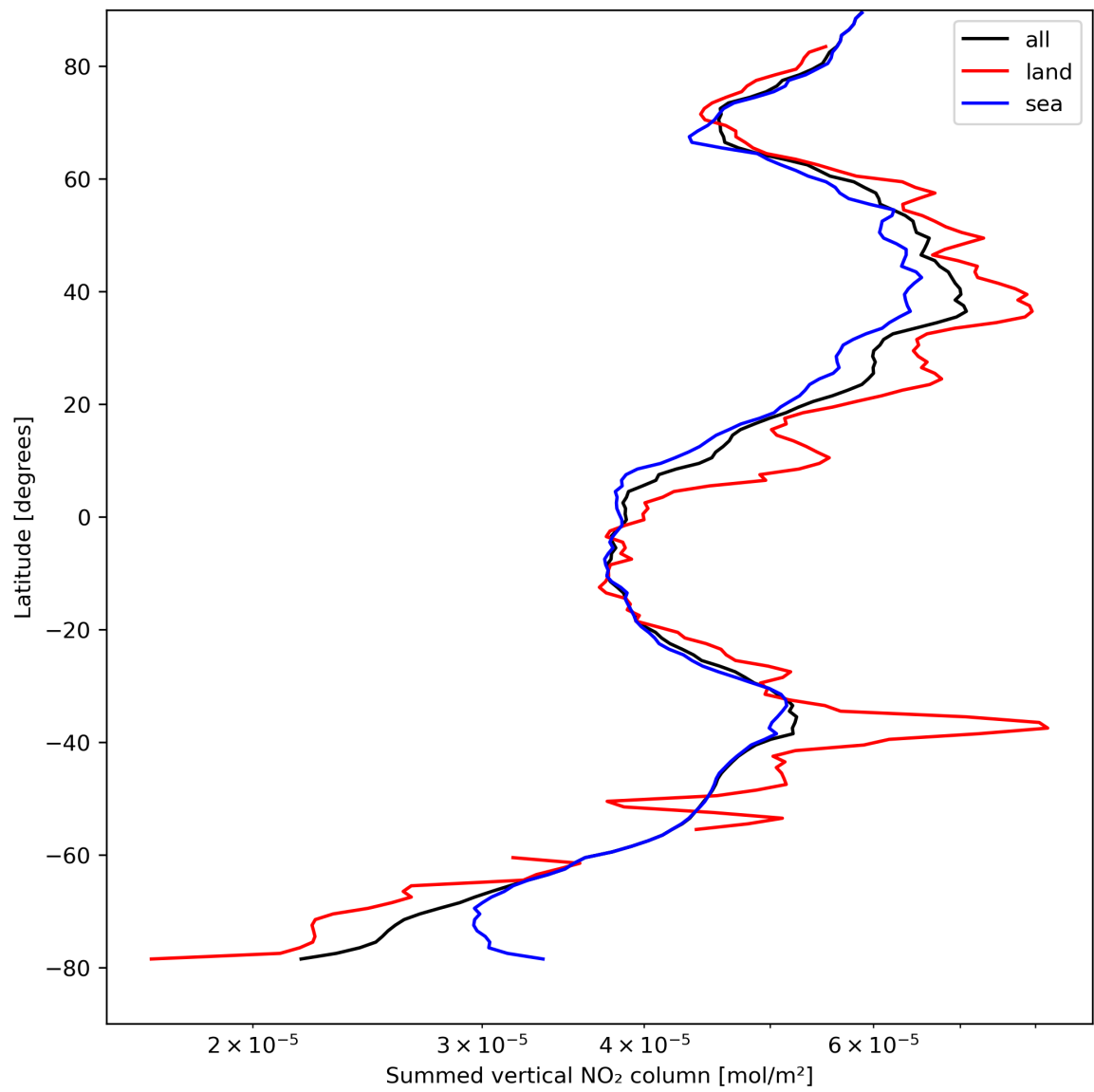
Figure 23: Zonal average of “Summed vertical NO 2 column” for 2024-04-15 to 2024-04-16.
