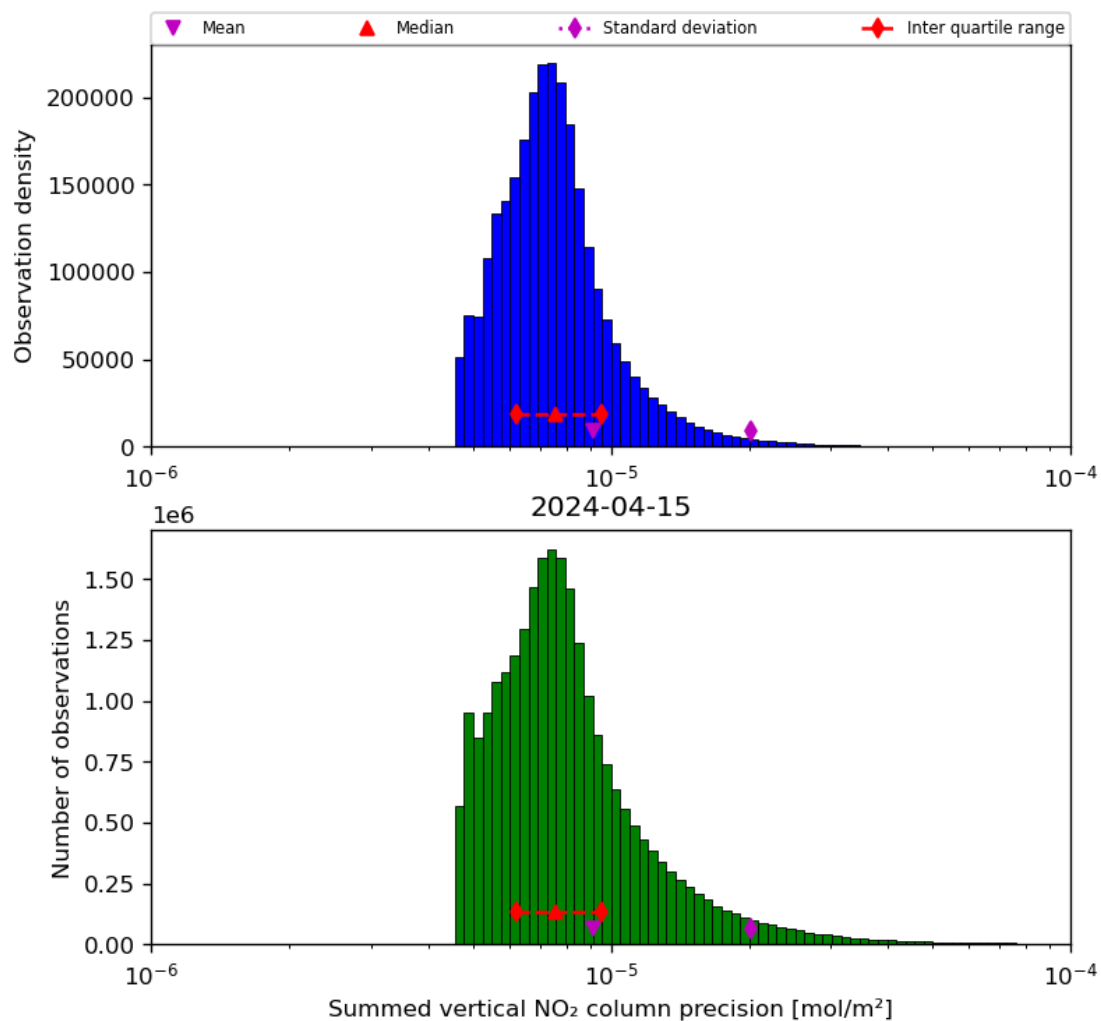
Figure 41: Histogram of “Summed vertical NO 2 column precision” for 2024-04-15 to 2024-04-16
