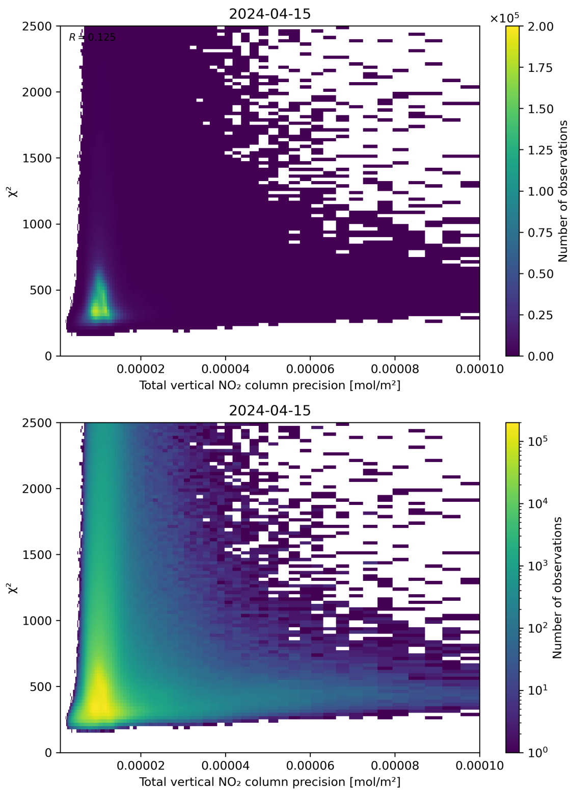
Figure 116: Scatter density plot of “Total vertical NO 2 column precision” against “ \chi^2 ” for 2024-04-15 to 2024-04-16.
