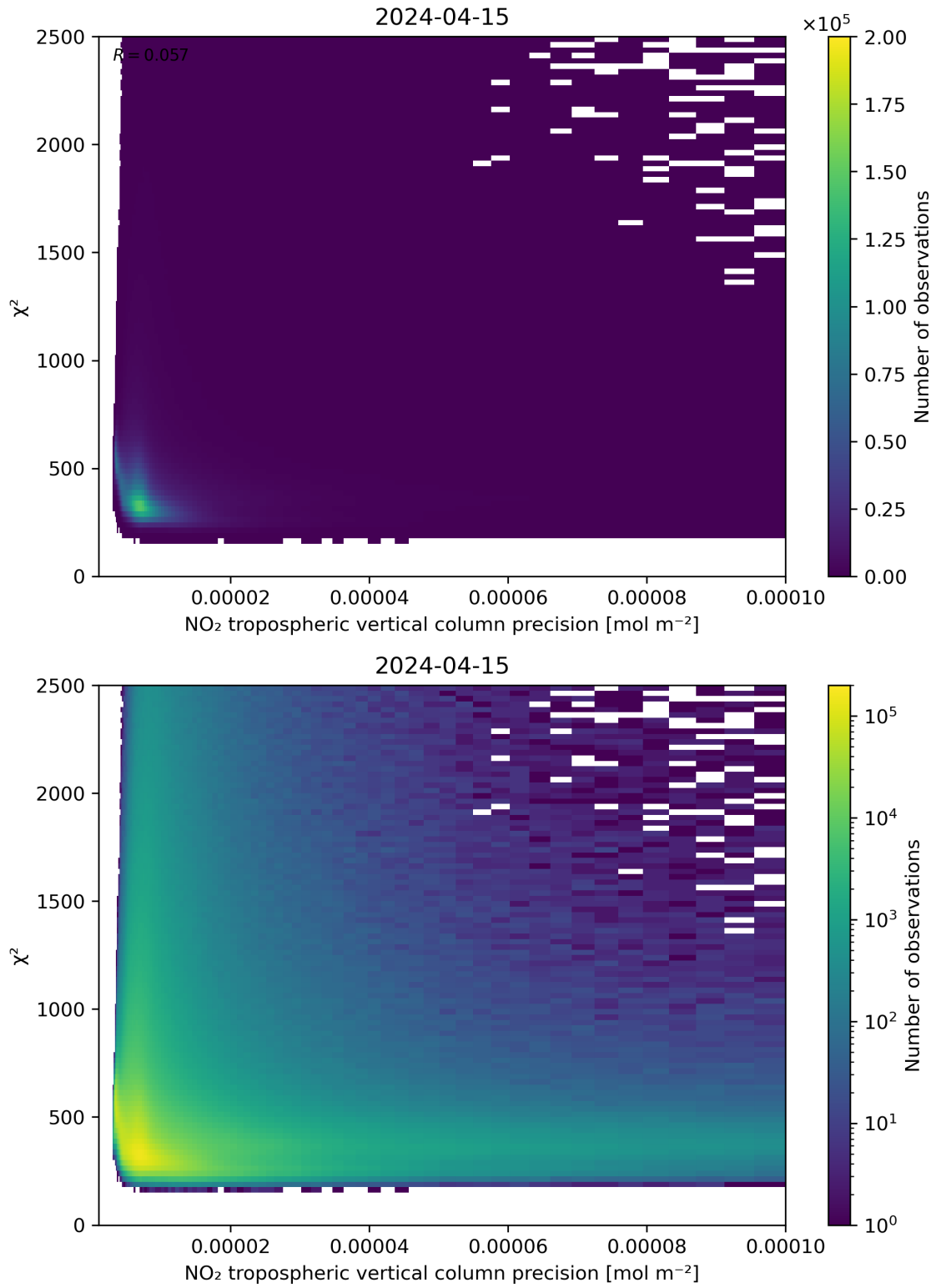
Figure 134: Scatter density plot of “NO 2 tropospheric vertical column precision” against “ \chi^2 ” for 2024-04-15 to 2024-04-16.
