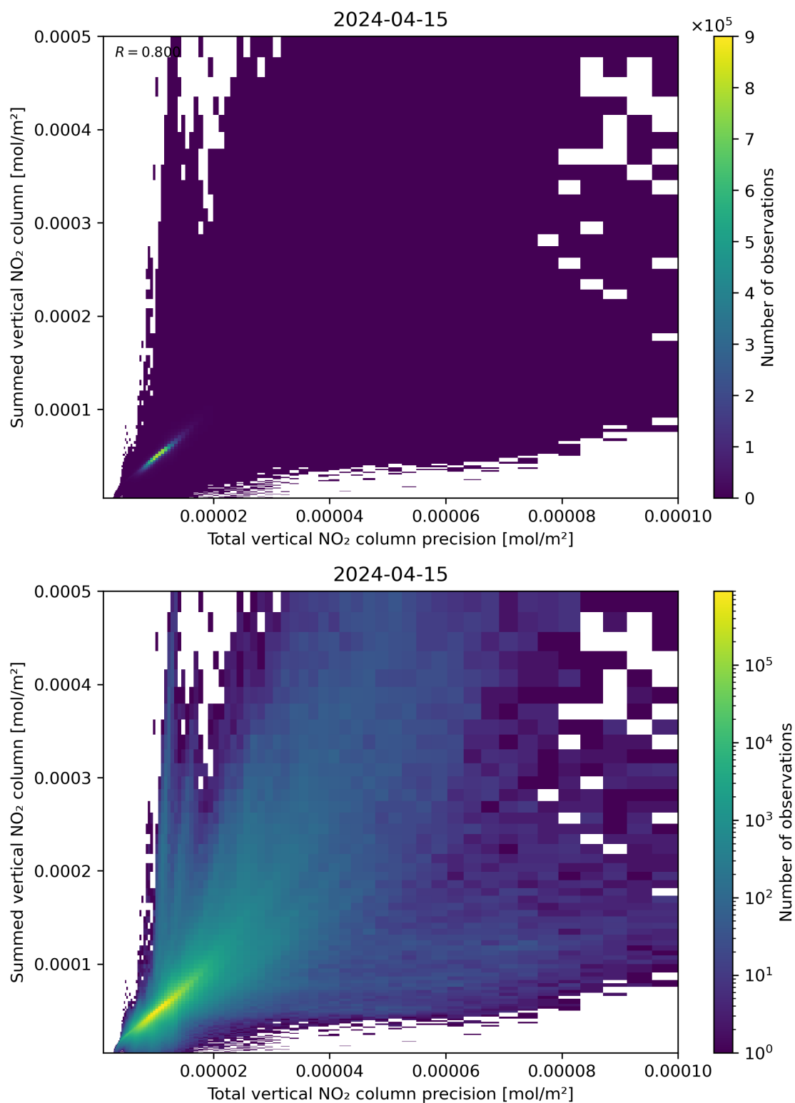
Figure 117: Scatter density plot of “Total vertical NO 2 column precision” against “Summed vertical NO 2 column” for 2024-04-15 to 2024-04-16.
