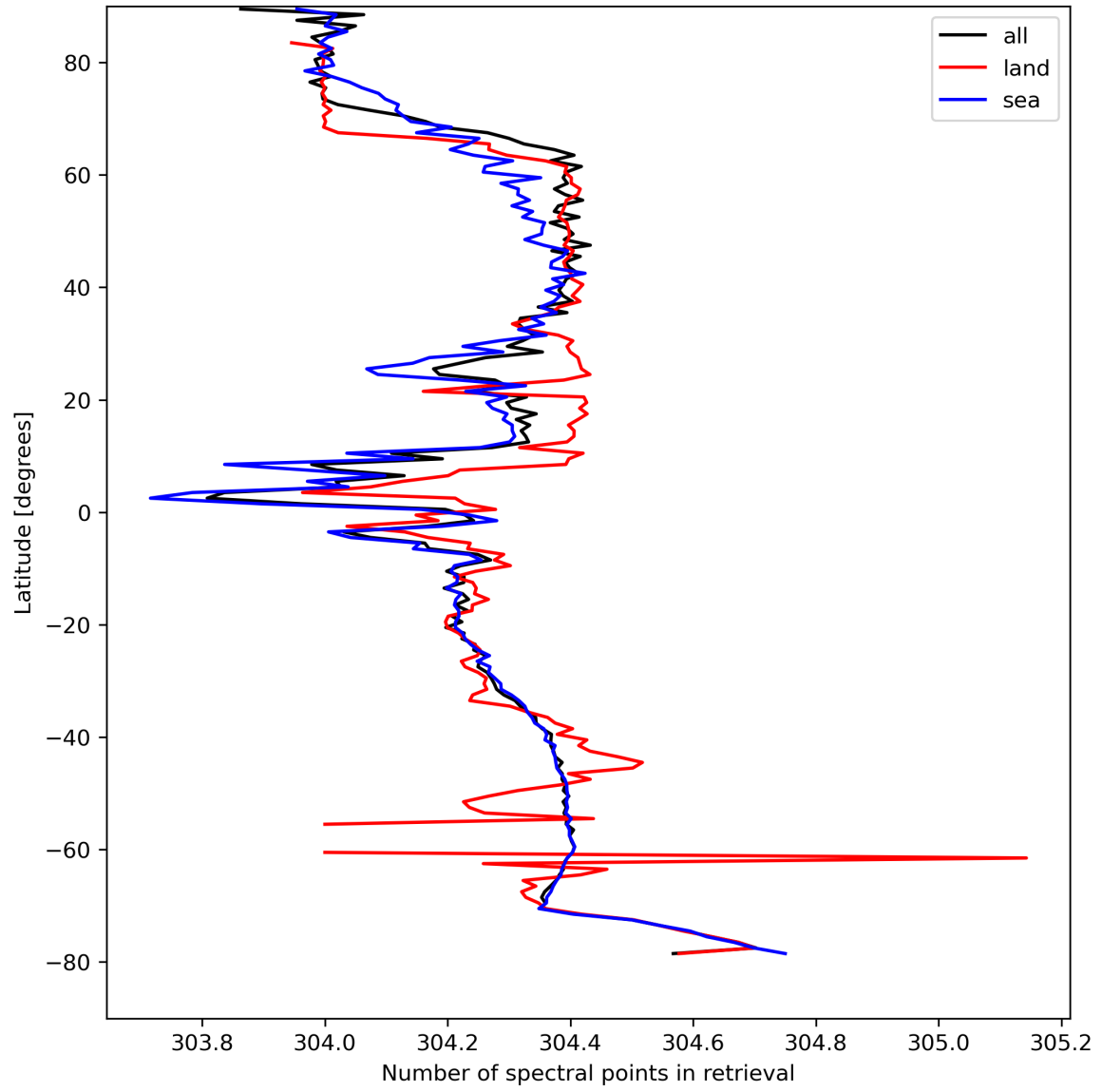
Figure 16: Zonal average of “Number of spectral points in retrieval” for 2024-04-15 to 2024-04-16.
