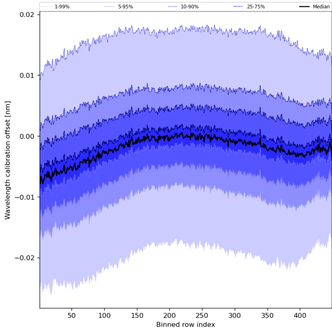
Figure 52: Along track statistics of “Wavelength calibration offset” for 2024-04-15 to 2024-04-16
