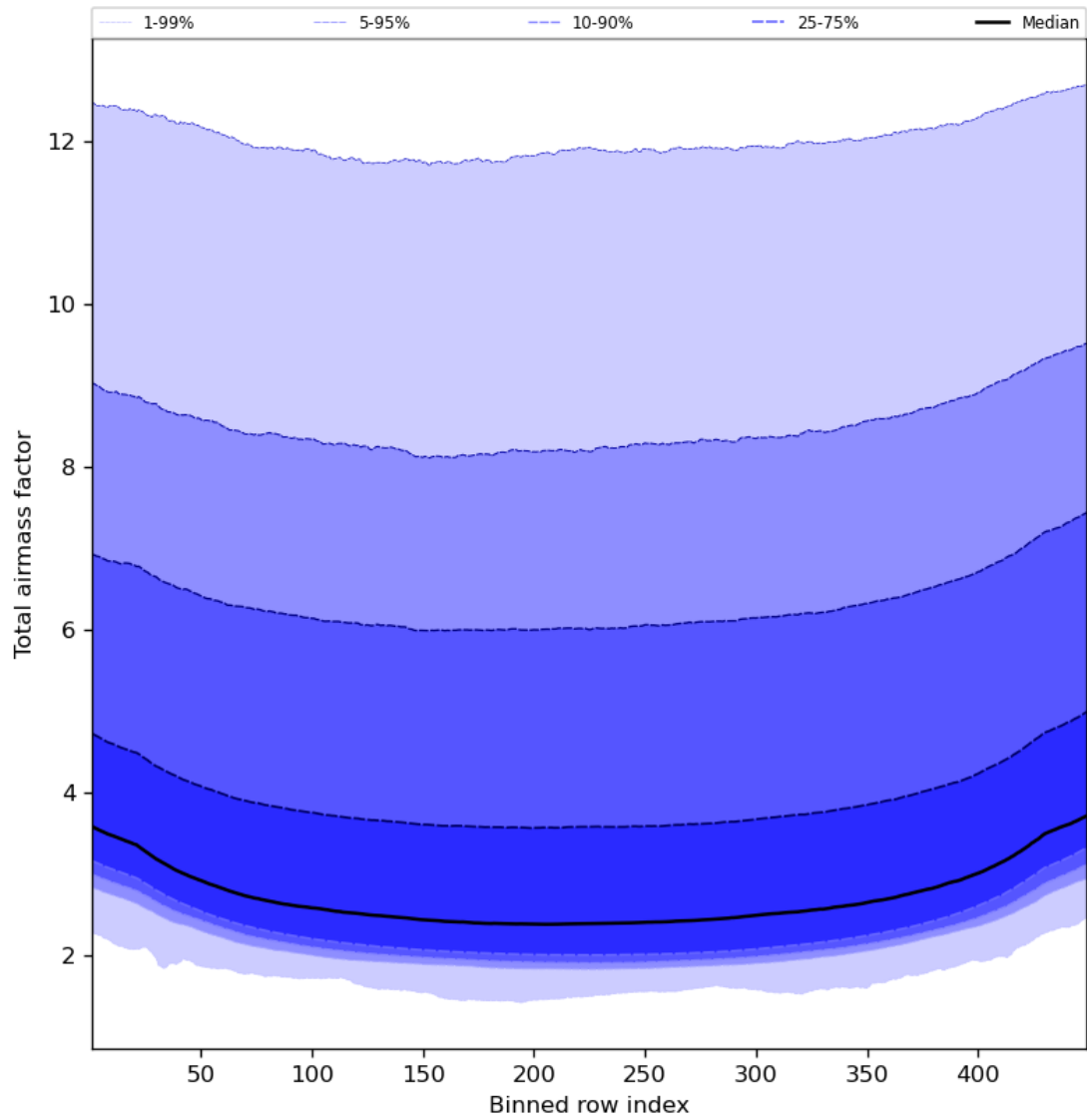
Figure 49: Along track statistics of “Total airmass factor” for 2024-04-15 to 2024-04-16
