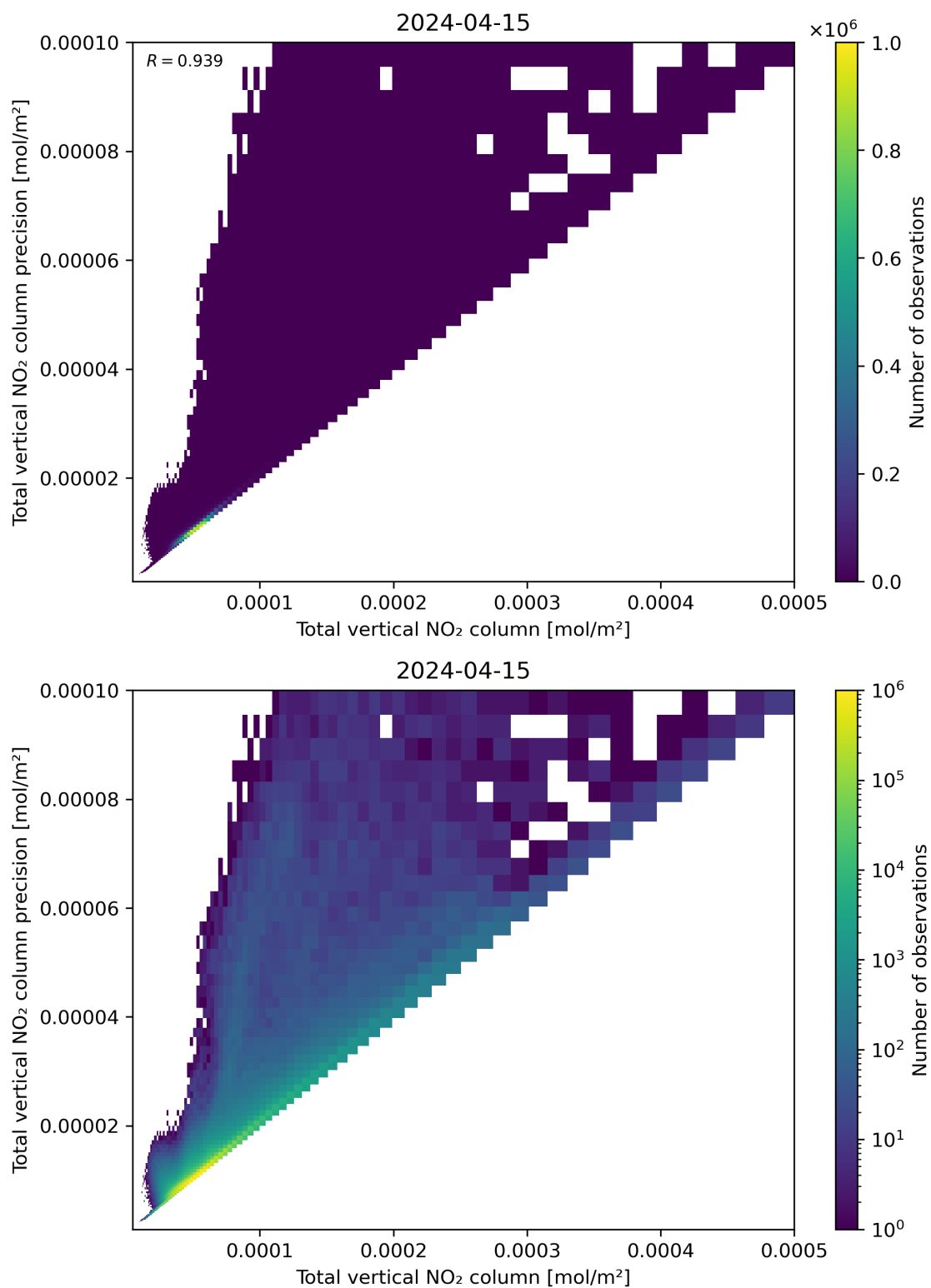
Figure 114: Scatter density plot of “Total vertical NO 2 column” against “Total vertical NO 2 column precision” for 2024-04-15 to 2024-04-16.
