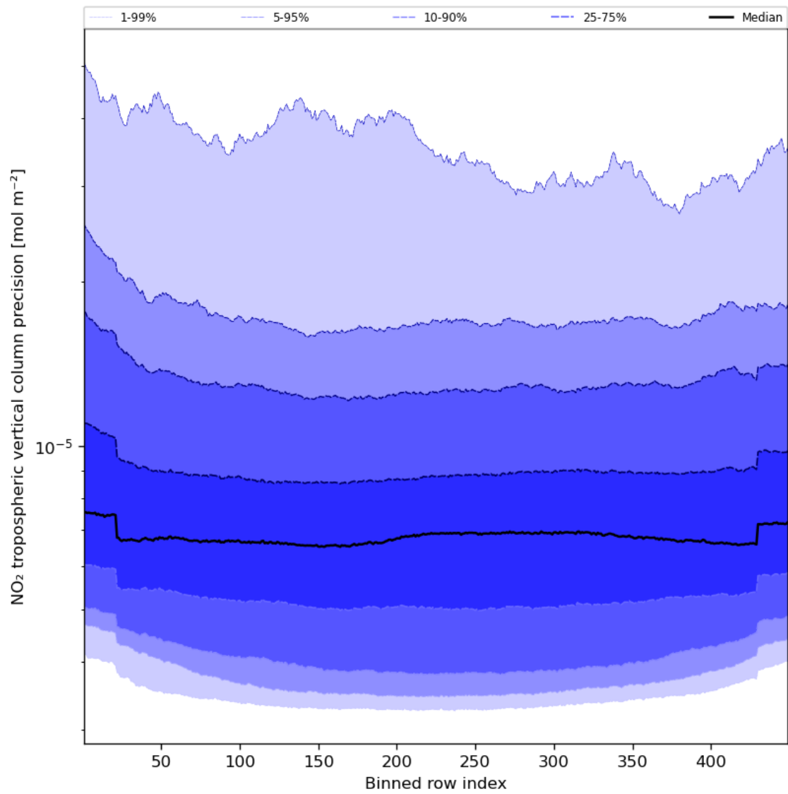
Figure 47: Along track statistics of “NO 2 tropospheric vertical column precision” for 2024-04-15 to 2024-04-16
