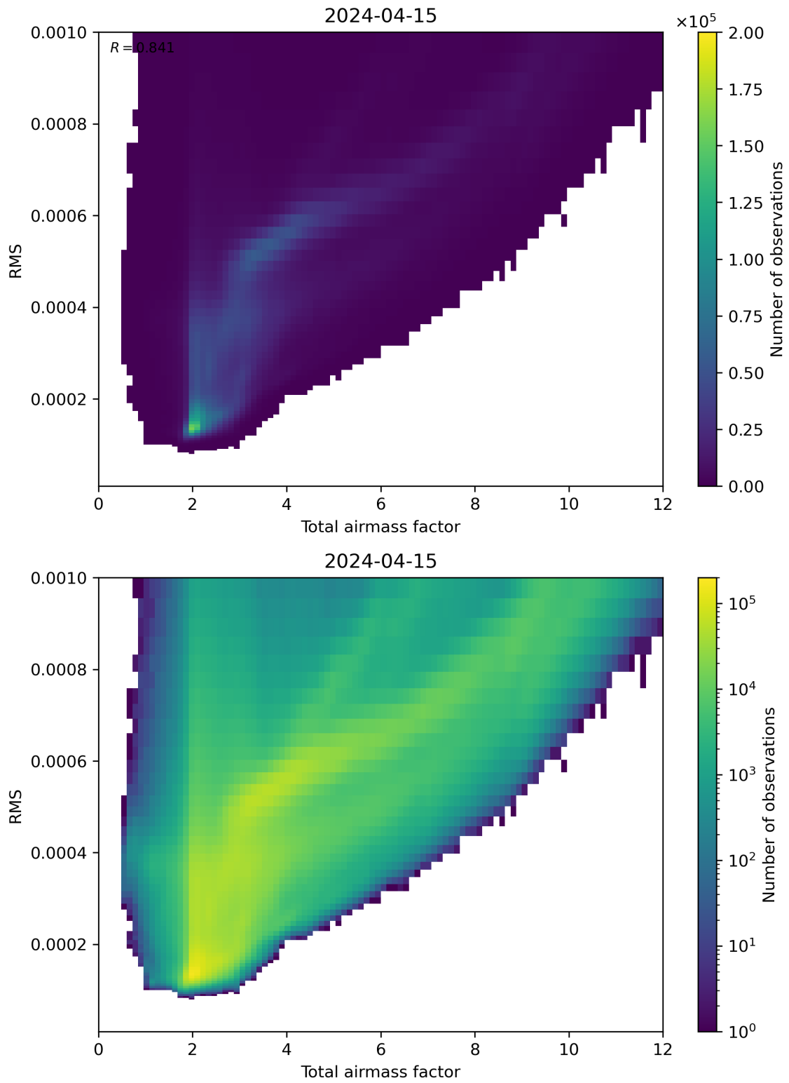
Figure 69: Scatter density plot of “Total airmass factor” against “RMS” for 2024-04-15 to 2024-04-16.
