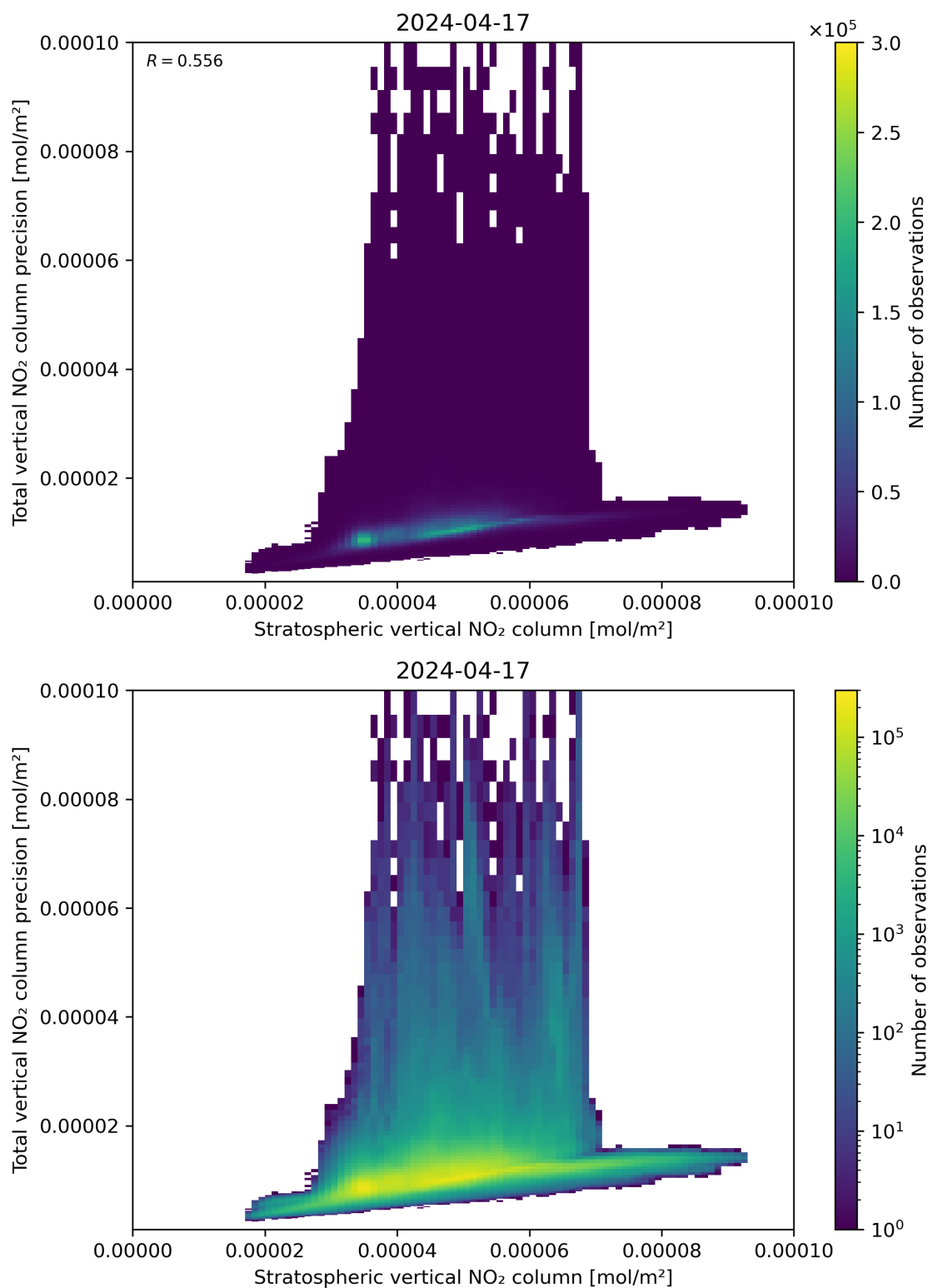
Figure 101: Scatter density plot of “Stratospheric vertical NO 2 column” against “Total vertical NO 2 column precision” for 2024-04-16 to 2024-04-18.
