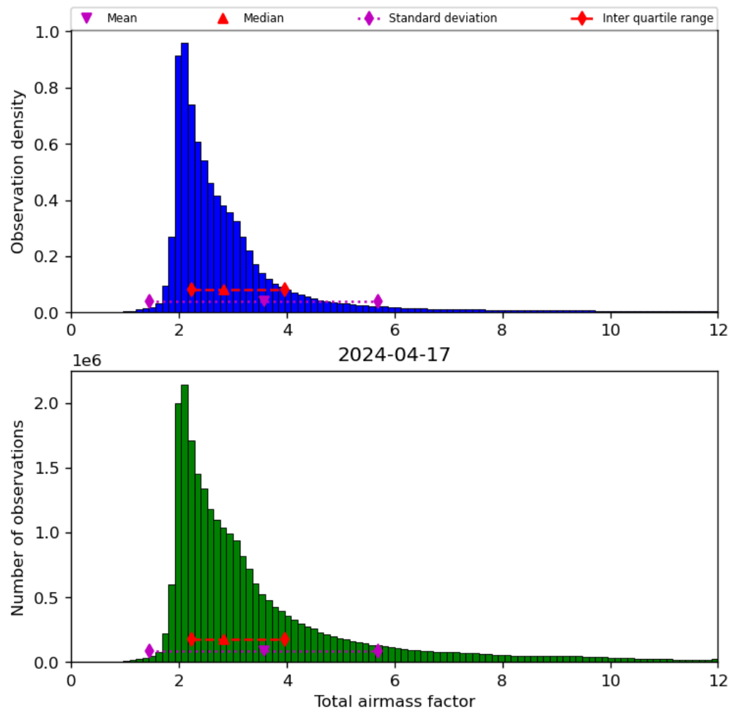
Figure 32: Histogram of “Total airmass factor” for 2024-04-16 to 2024-04-18
