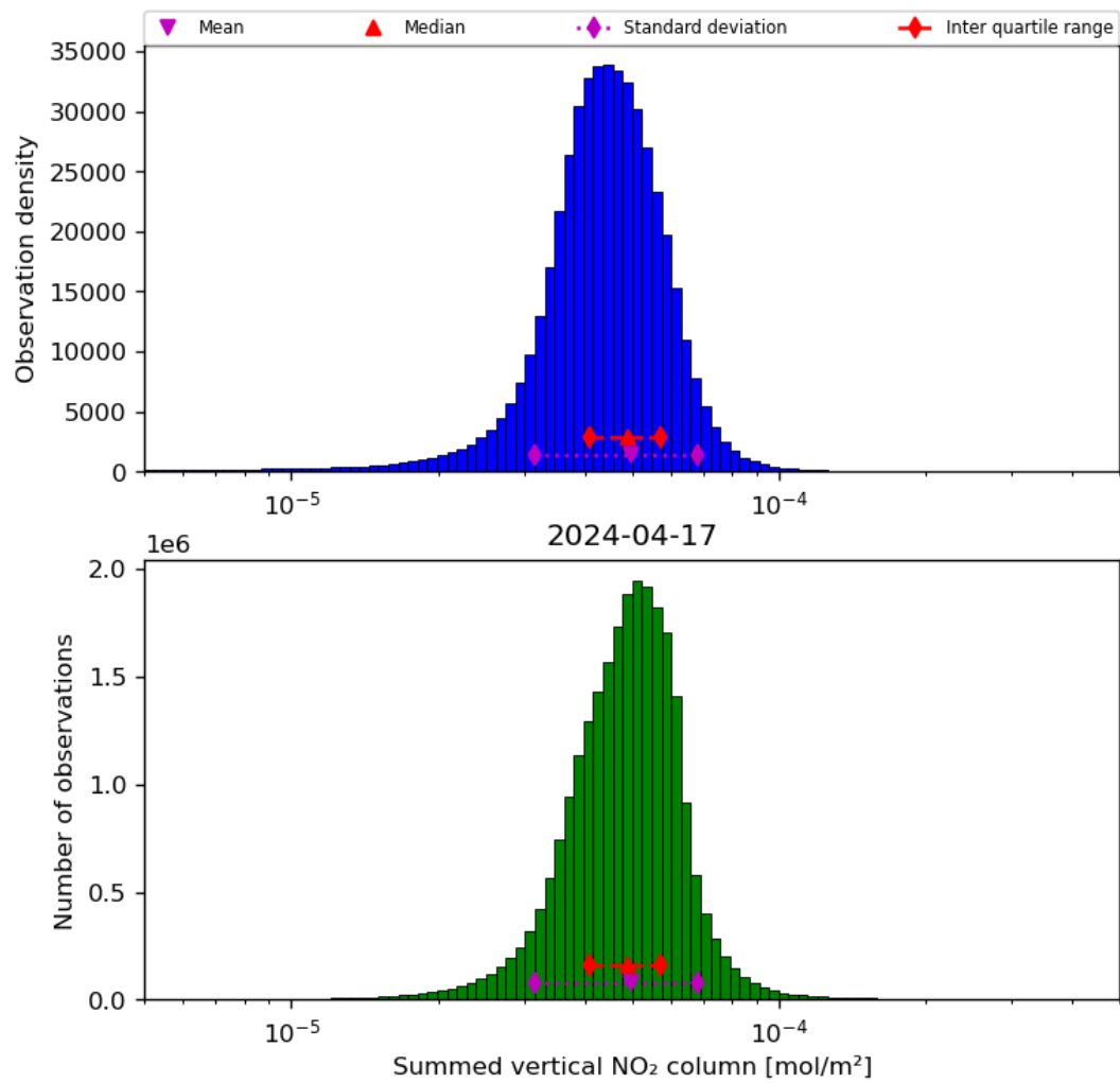
Figure 40: Histogram of “Summed vertical NO 2 column” for 2024-04-16 to 2024-04-18
