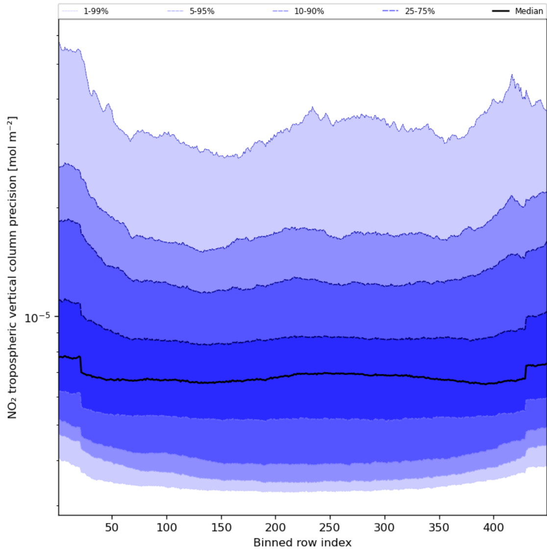
Figure 47: Along track statistics of “NO 2 tropospheric vertical column precision” for 2024-04-16 to 2024-04-18
