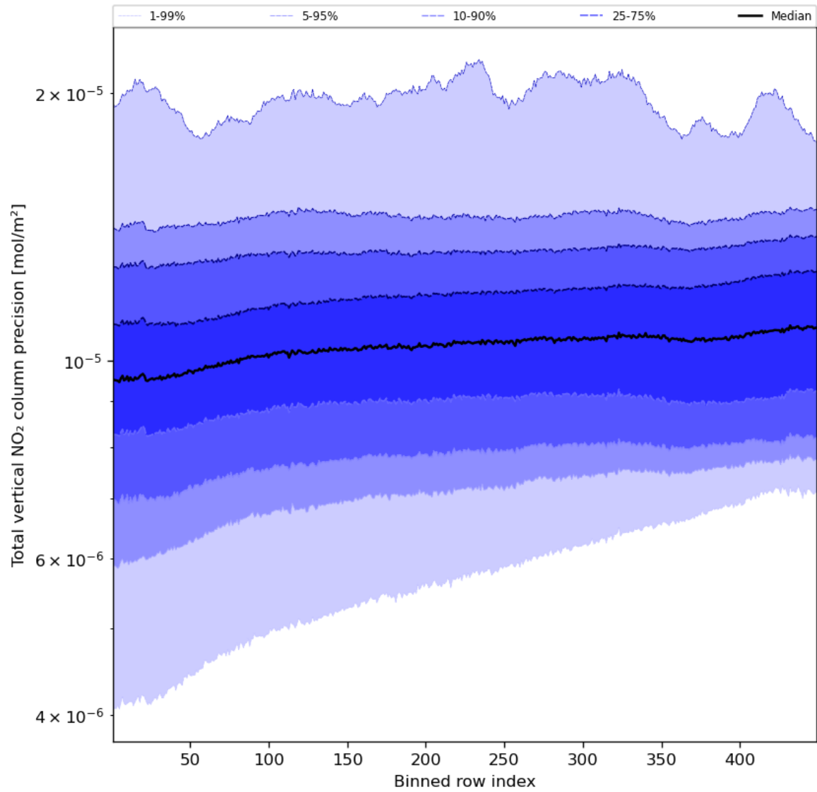
Figure 56: Along track statistics of “Total vertical NO 2 column precision” for 2024-04-16 to 2024-04-18
