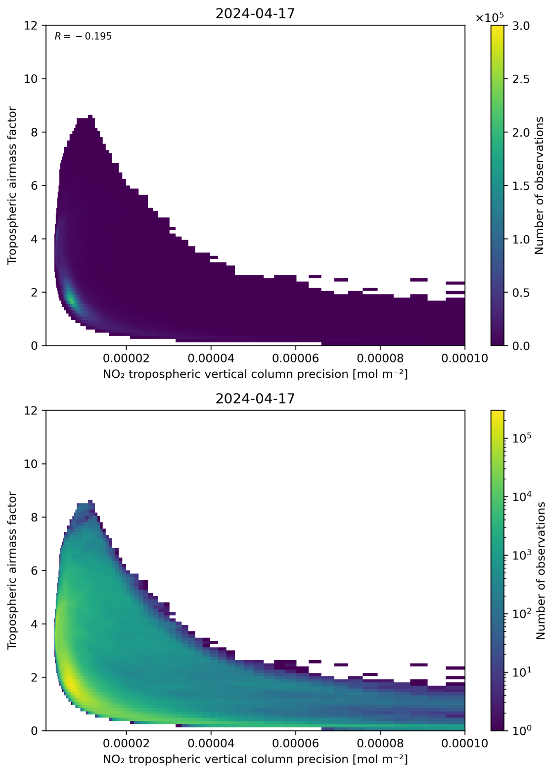
Figure 133: Scatter density plot of “NO 2 tropospheric vertical column precision” against “Tropospheric airmass factor” for 2024-04-16 to 2024-04-18.
