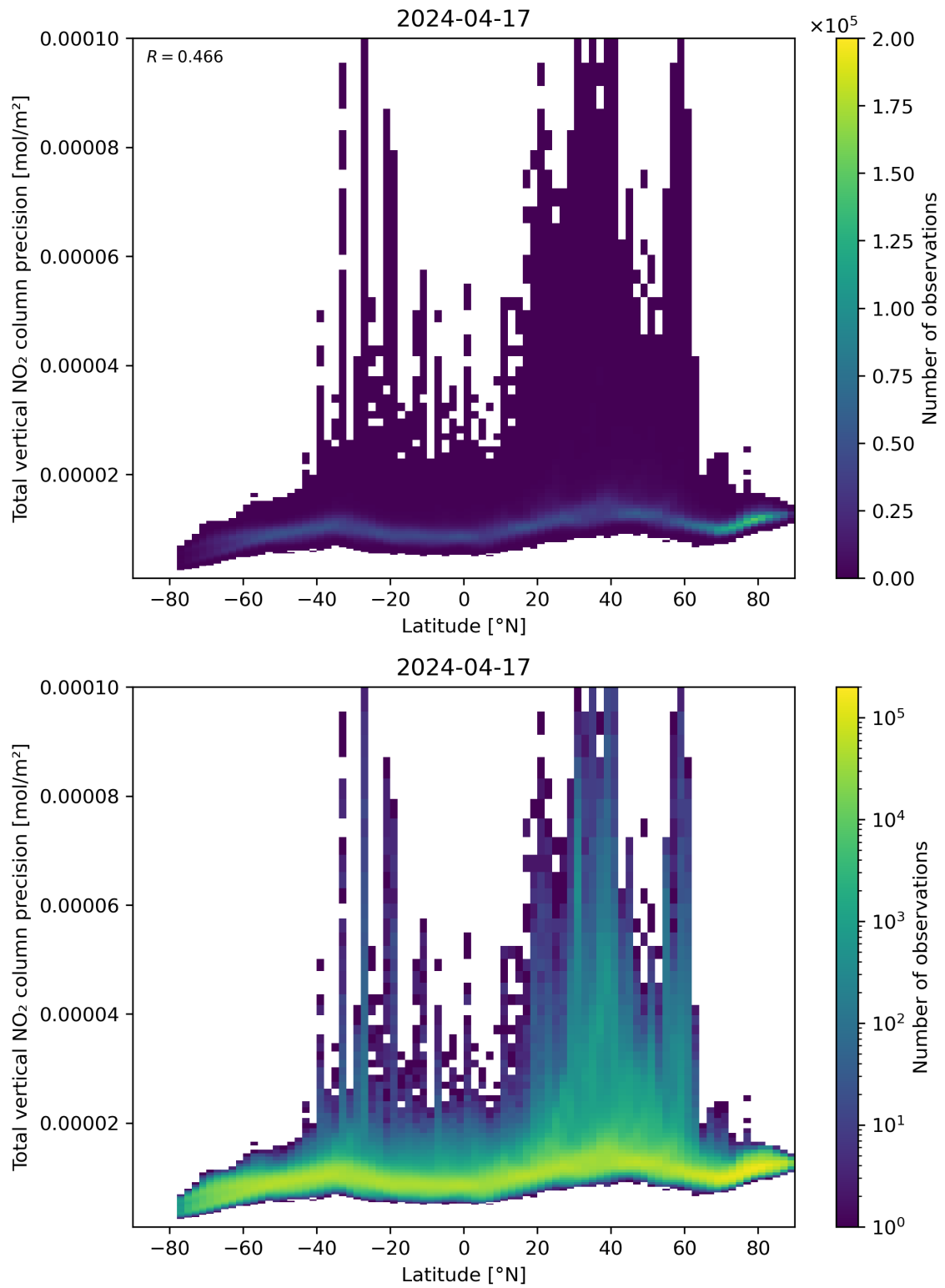
Figure 91: Scatter density plot of “Latitude” against “Total vertical NO 2 column precision” for 2024-04-16 to 2024-04-18.
