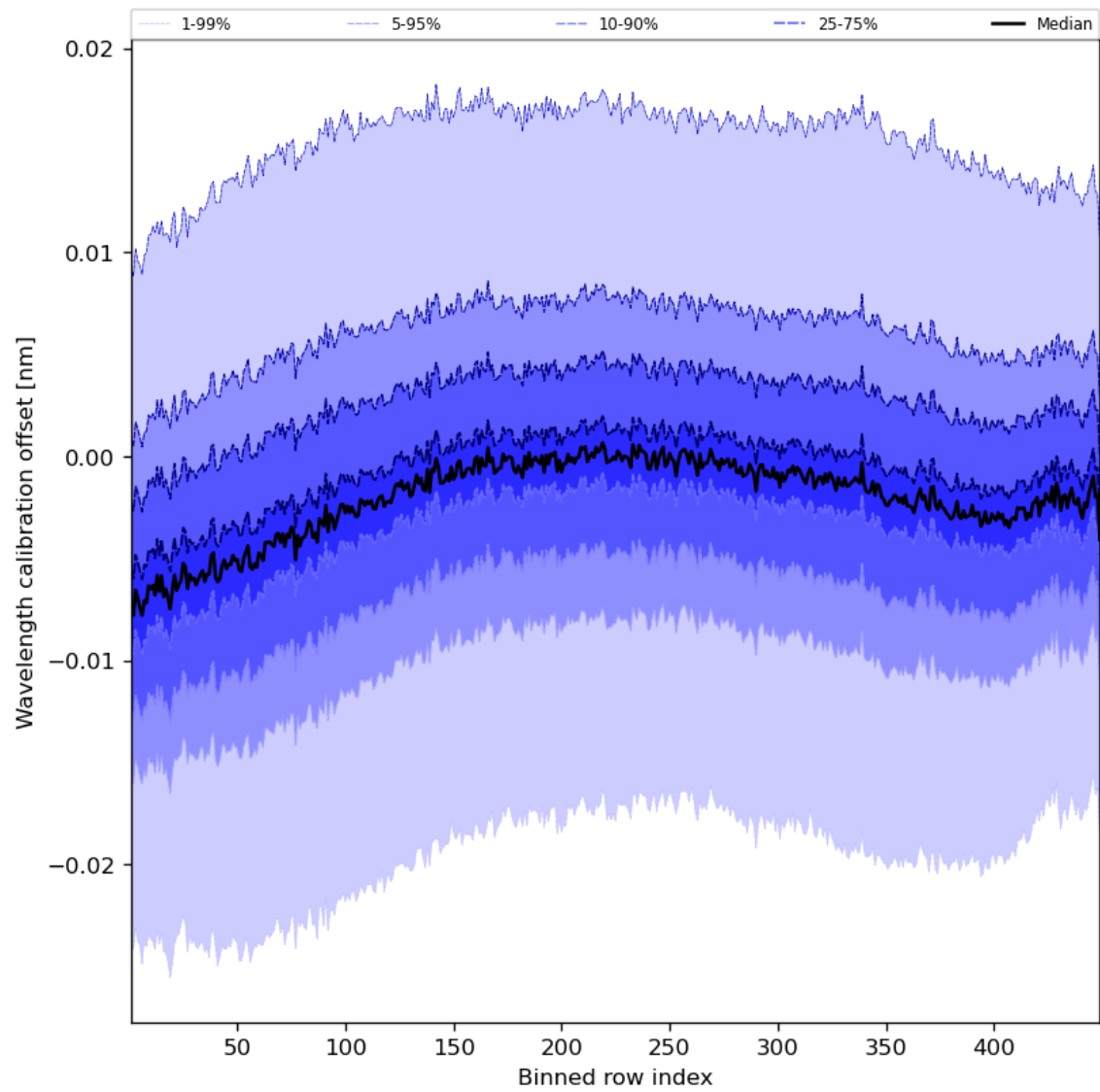
Figure 52: Along track statistics of “Wavelength calibration offset” for 2024-04-16 to 2024-04-18
