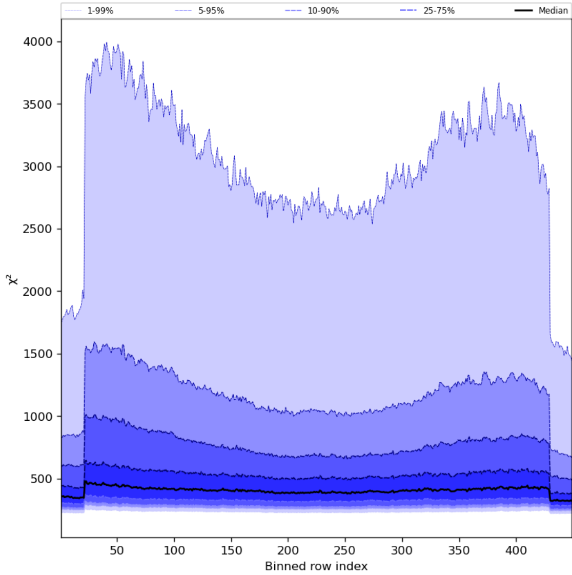
Figure 59: Along track statistics of “ \chi^2 ” for 2024-04-16 to 2024-04-18
