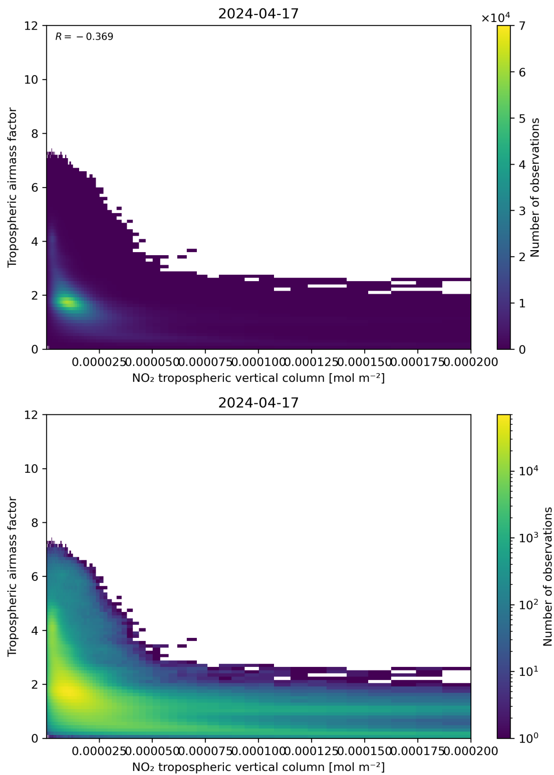
Figure 123: Scatter density plot of “NO 2 tropospheric vertical column” against “Tropospheric air mass factor” for 2024-04-16 to 2024-04-18.
