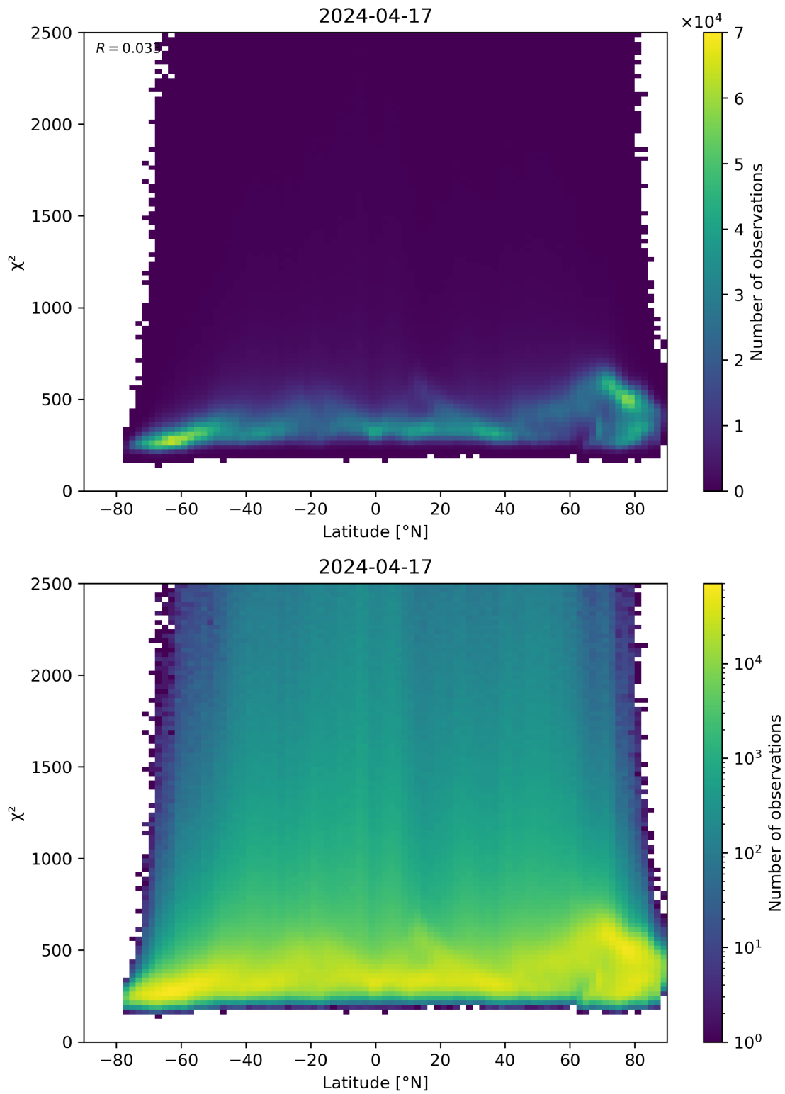
Figure 86: Scatter density plot of “Latitude” against “ \chi^2 ” for 2024-04-16 to 2024-04-18.
