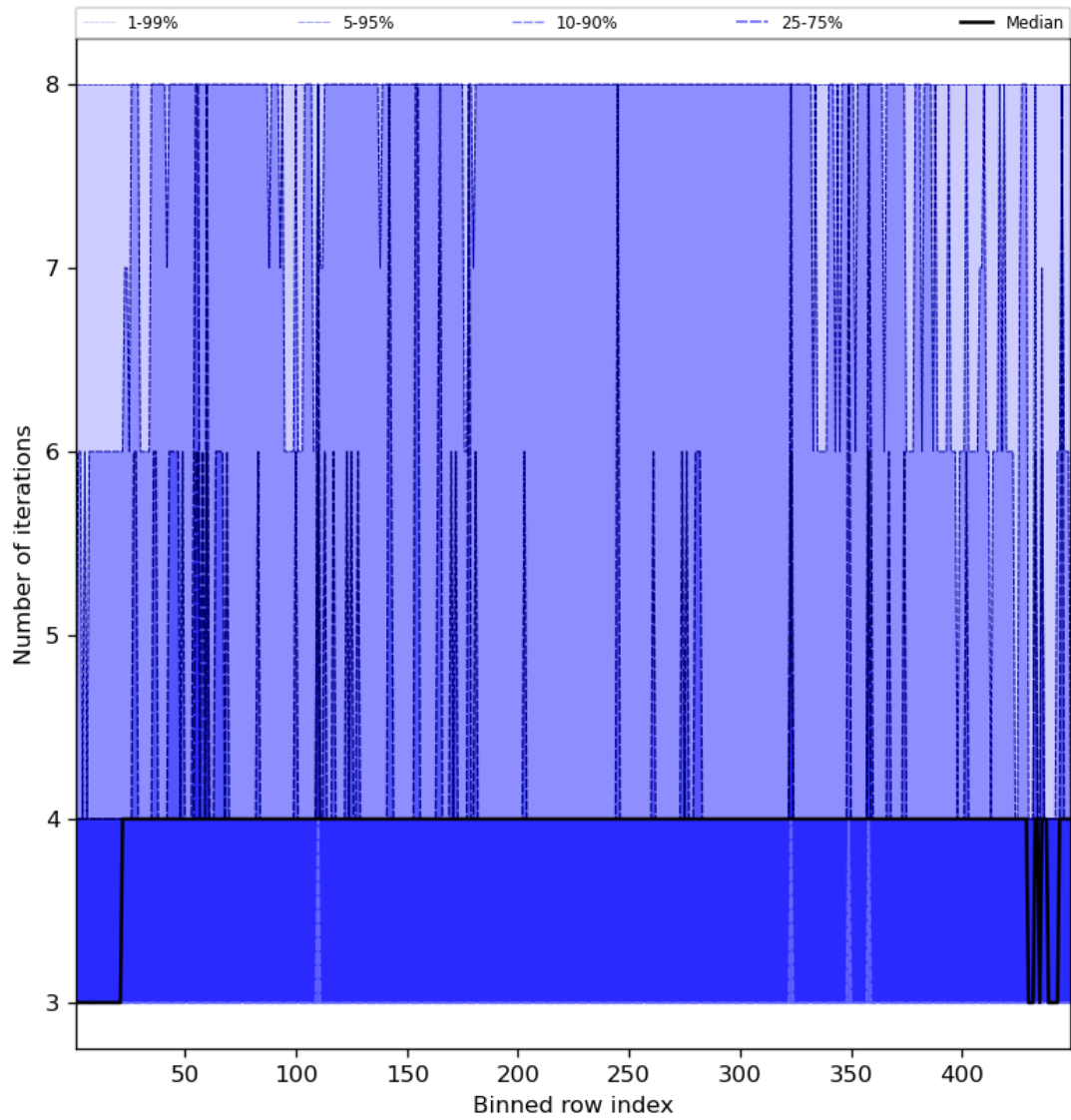
Figure 51: Along track statistics of “Number of iterations” for 2024-04-16 to 2024-04-18
