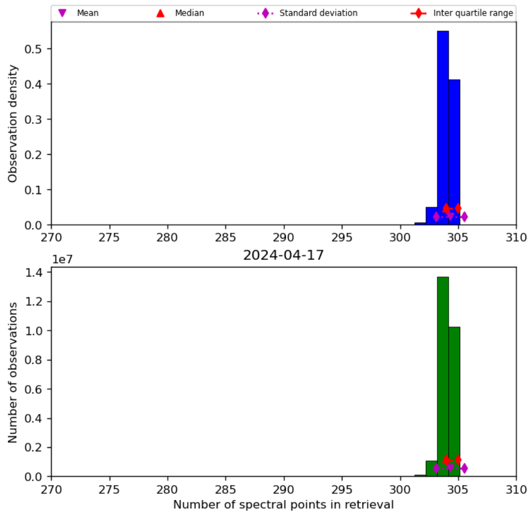
Figure 33: Histogram of “Number of spectral points in retrieval” for 2024-04-16 to 2024-04-18
