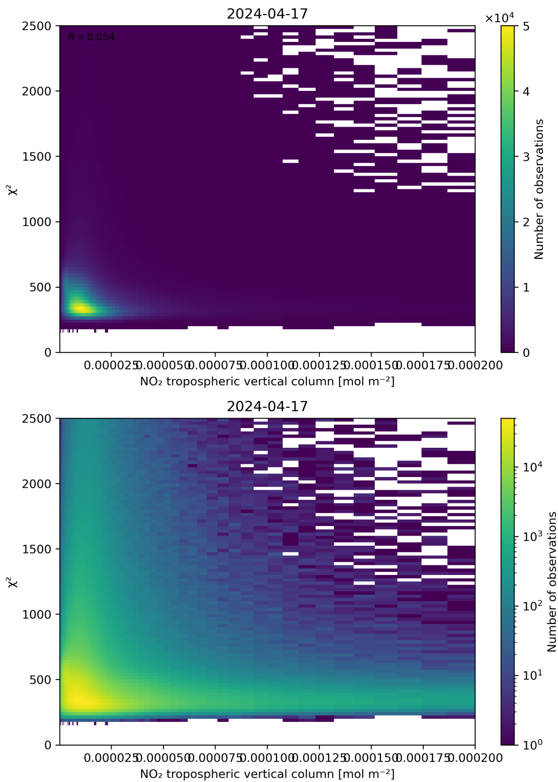
Figure 124: Scatter density plot of “NO 2 tropospheric vertical column” against “ \chi^2 ” for 2024-04-16 to 2024-04-18.
