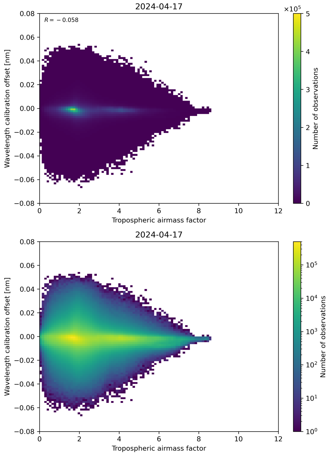
Figure 80: Scatter density plot of “Tropospheric air mass factor” against “Wavelength calibration offset” for 2024-04-16 to 2024-04-18.
