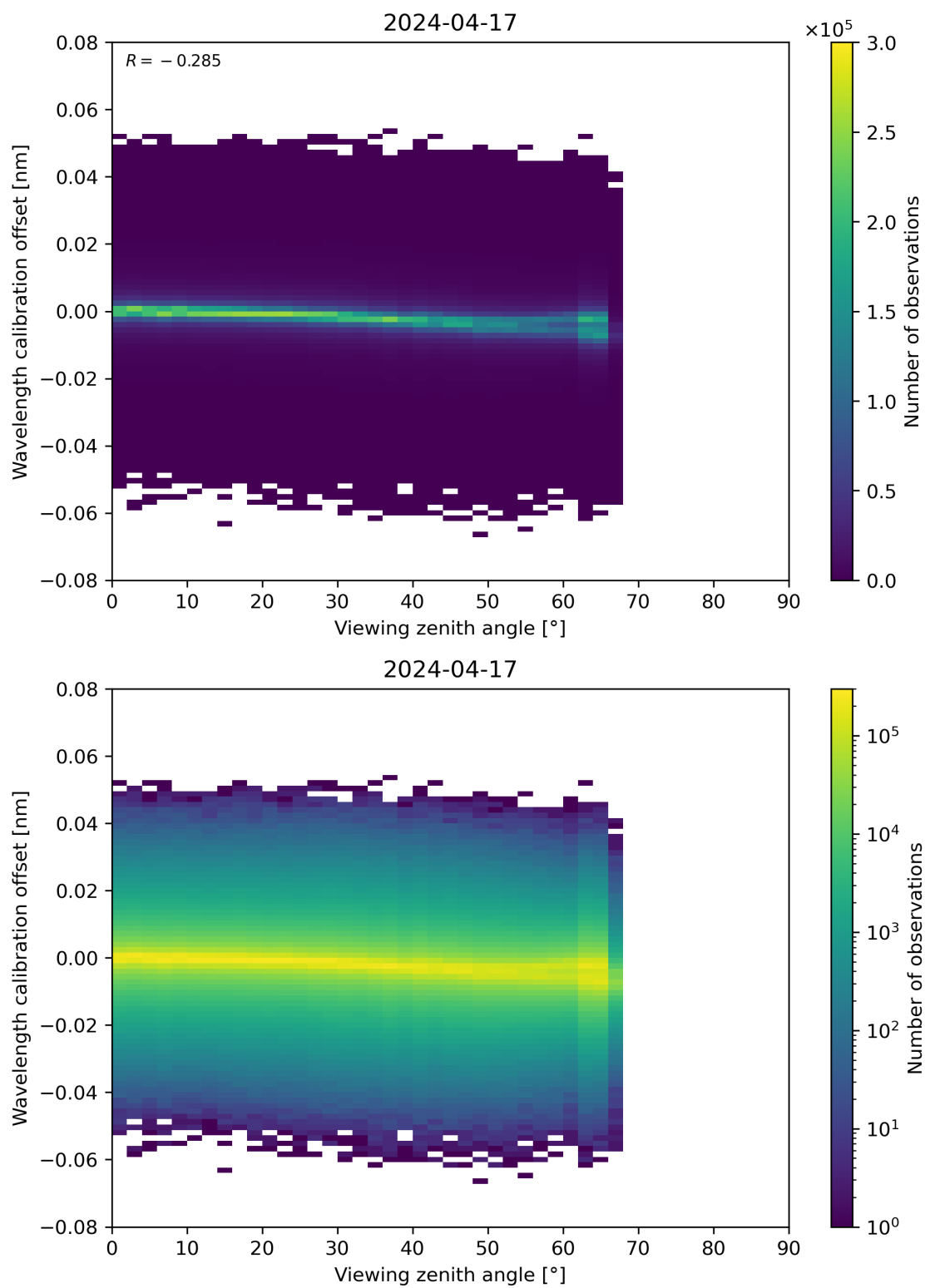
Figure 173: Scatter density plot of “Viewing zenith angle” against “Wavelength calibration offset” for 2024-04-16 to 2024-04-18.
