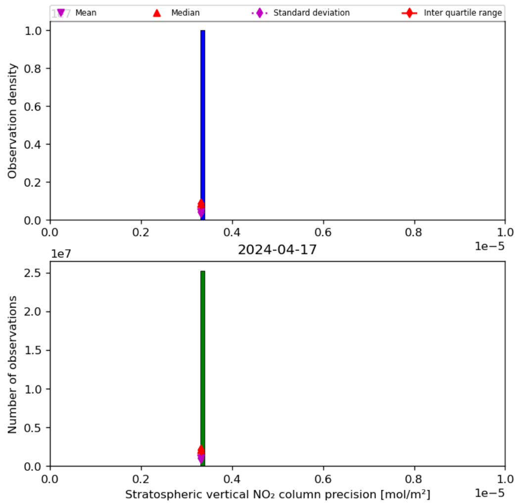
Figure 37: Histogram of “Stratospheric vertical NO 2 column precision” for 2024-04-16 to 2024-04-18
