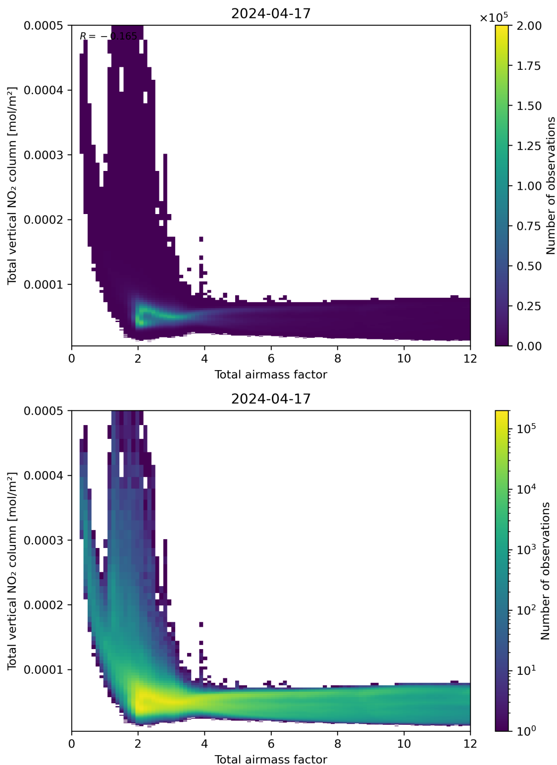
Figure 67: Scatter density plot of “Total airmass factor” against “Total vertical NO 2 column” for 2024-04-16 to 2024-04-18.
