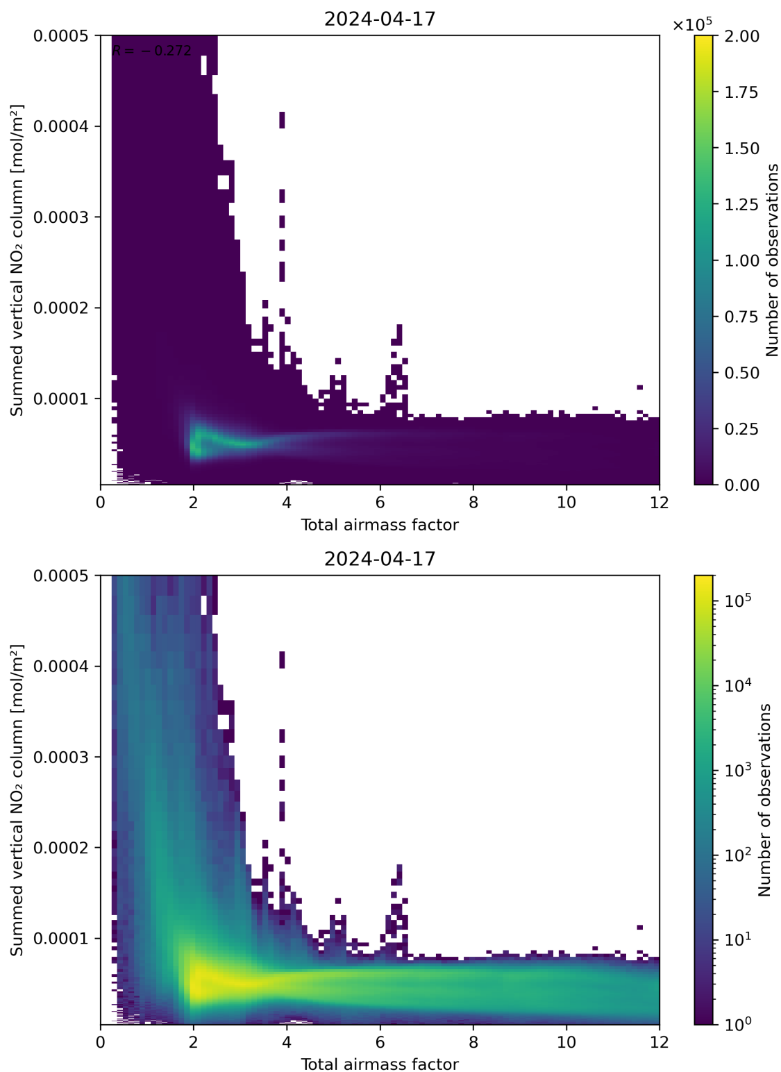
Figure 65: Scatter density plot of “Total airmass factor” against “Summed vertical NO 2 column” for 2024-04-16 to 2024-04-18.
