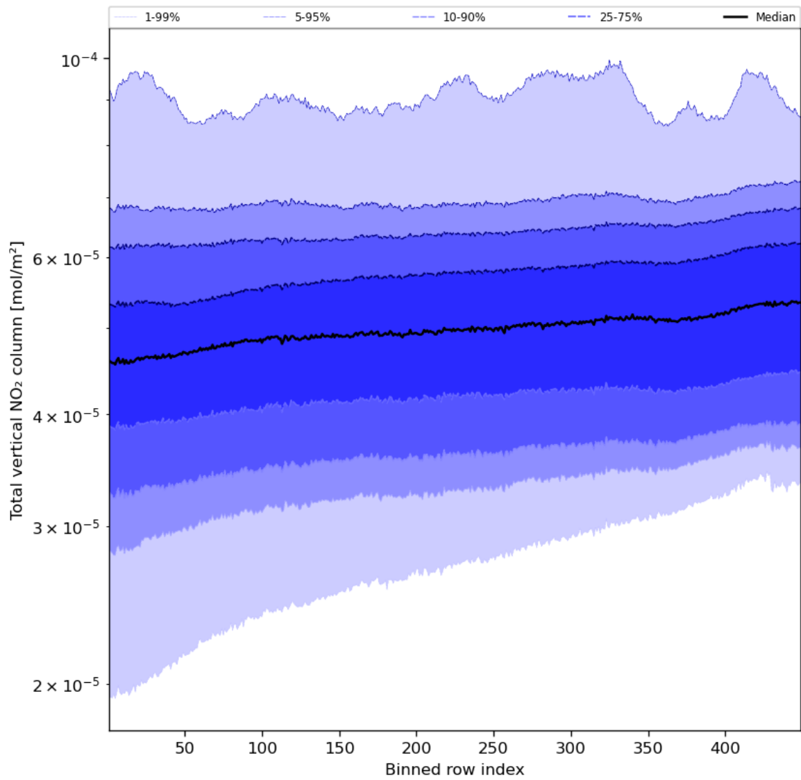
Figure 55: Along track statistics of “Total vertical NO 2 column” for 2024-04-16 to 2024-04-18
