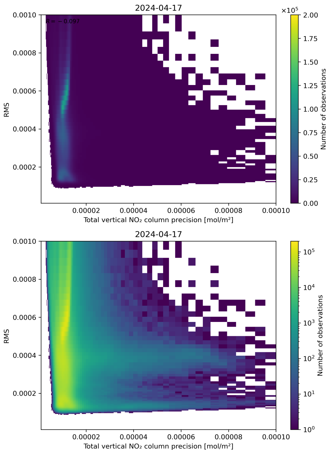
Figure 119: Scatter density plot of “Total vertical NO 2 column precision” against “RMS” for 2024-04-16 to 2024-04-18.
