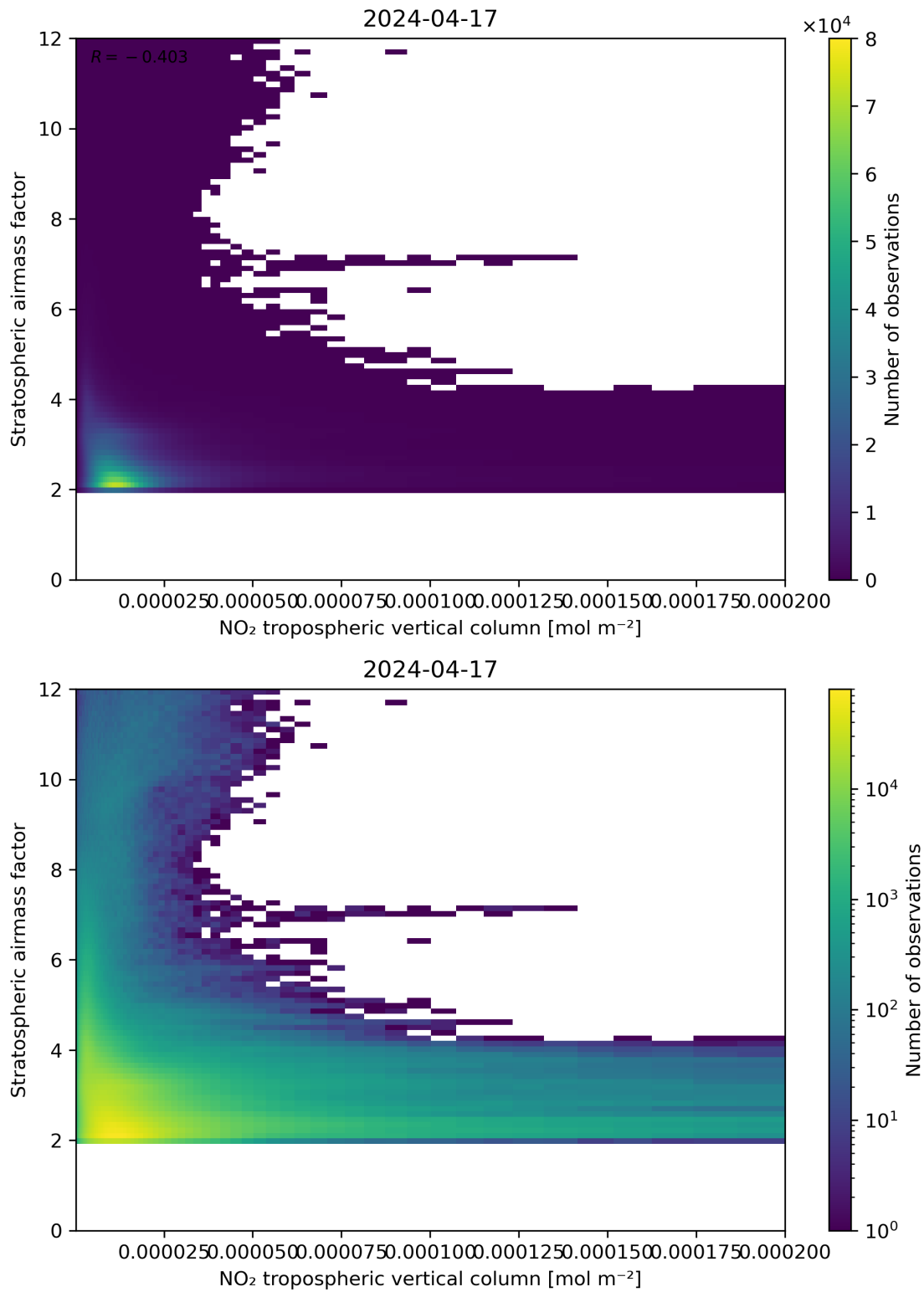
Figure 121: Scatter density plot of “NO 2 tropospheric vertical column” against “Stratospheric air mass factor” for 2024-04-16 to 2024-04-18.
