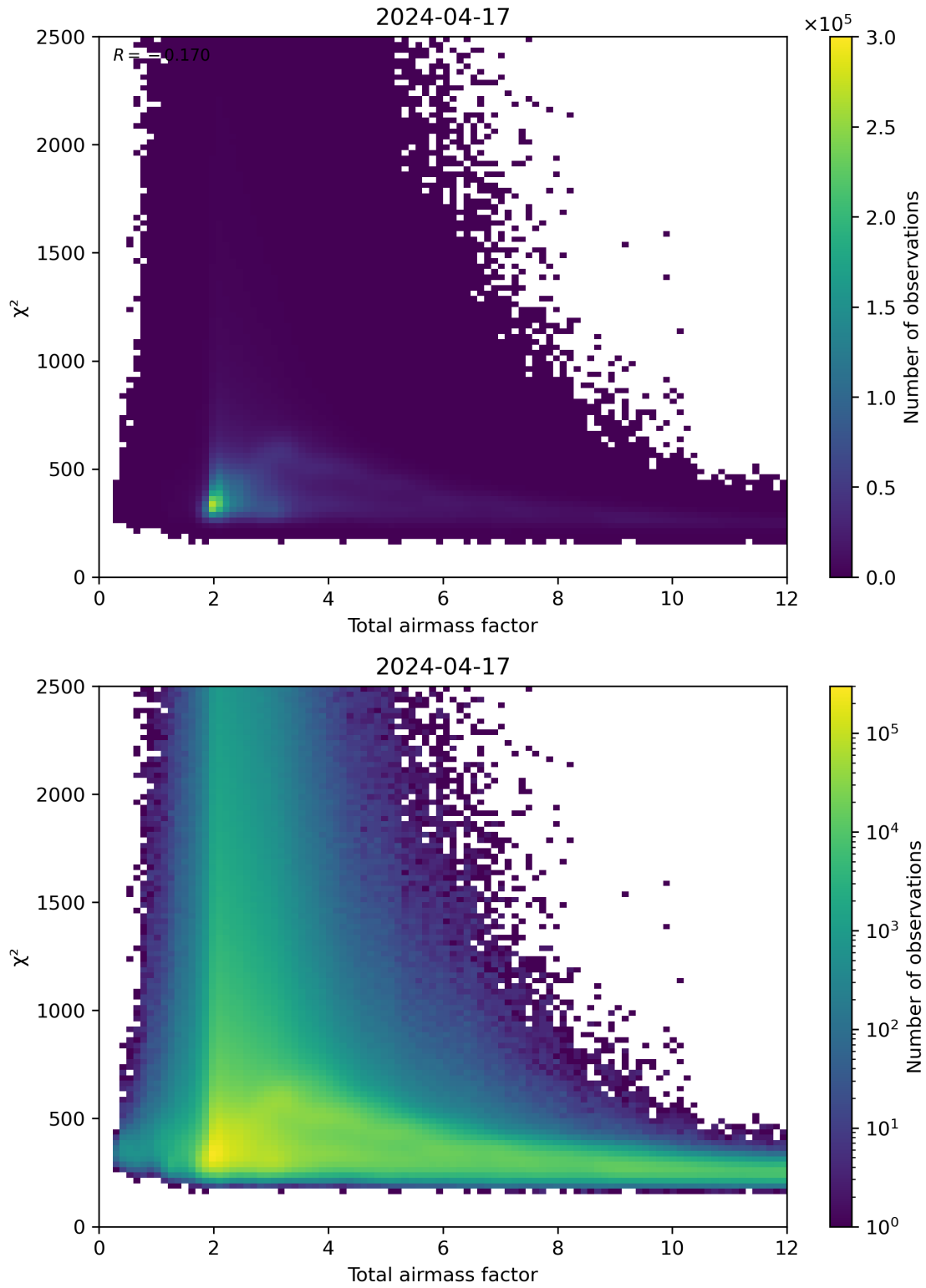
Figure 63: Scatter density plot of “Total airmass factor” against “ \chi^2 ” for 2024-04-16 to 2024-04-18.
