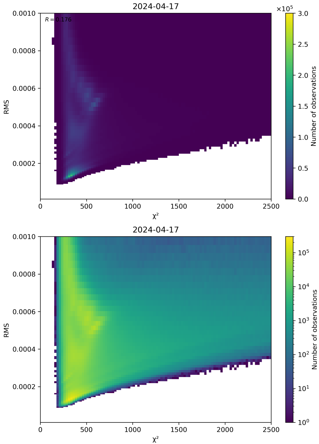
Figure 82: Scatter density plot of “ \chi^2 ” against “RMS” for 2024-04-16 to 2024-04-18.
