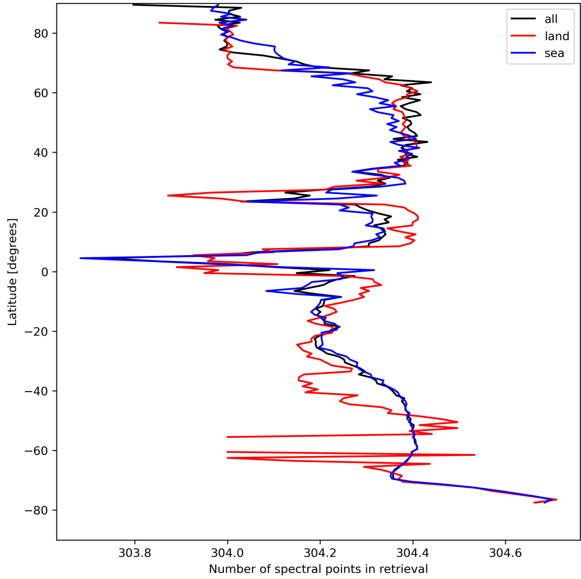
Figure 16: Zonal average of “Number of spectral points in retrieval” for 2024-04-16 to 2024-04-18.
