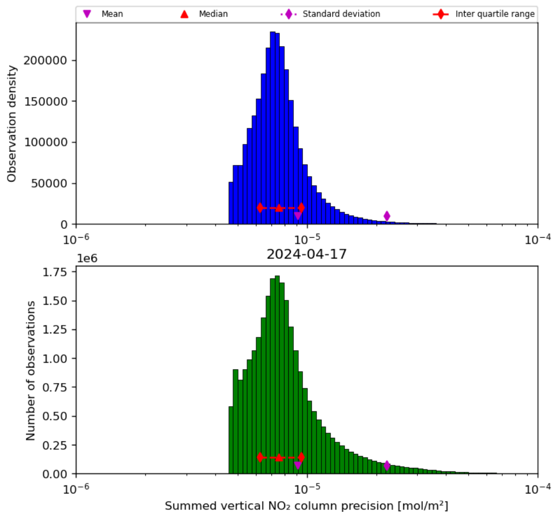
Figure 41: Histogram of "Summed vertical NO 2 column precision" for 2024-04-16 to 2024-04-18
