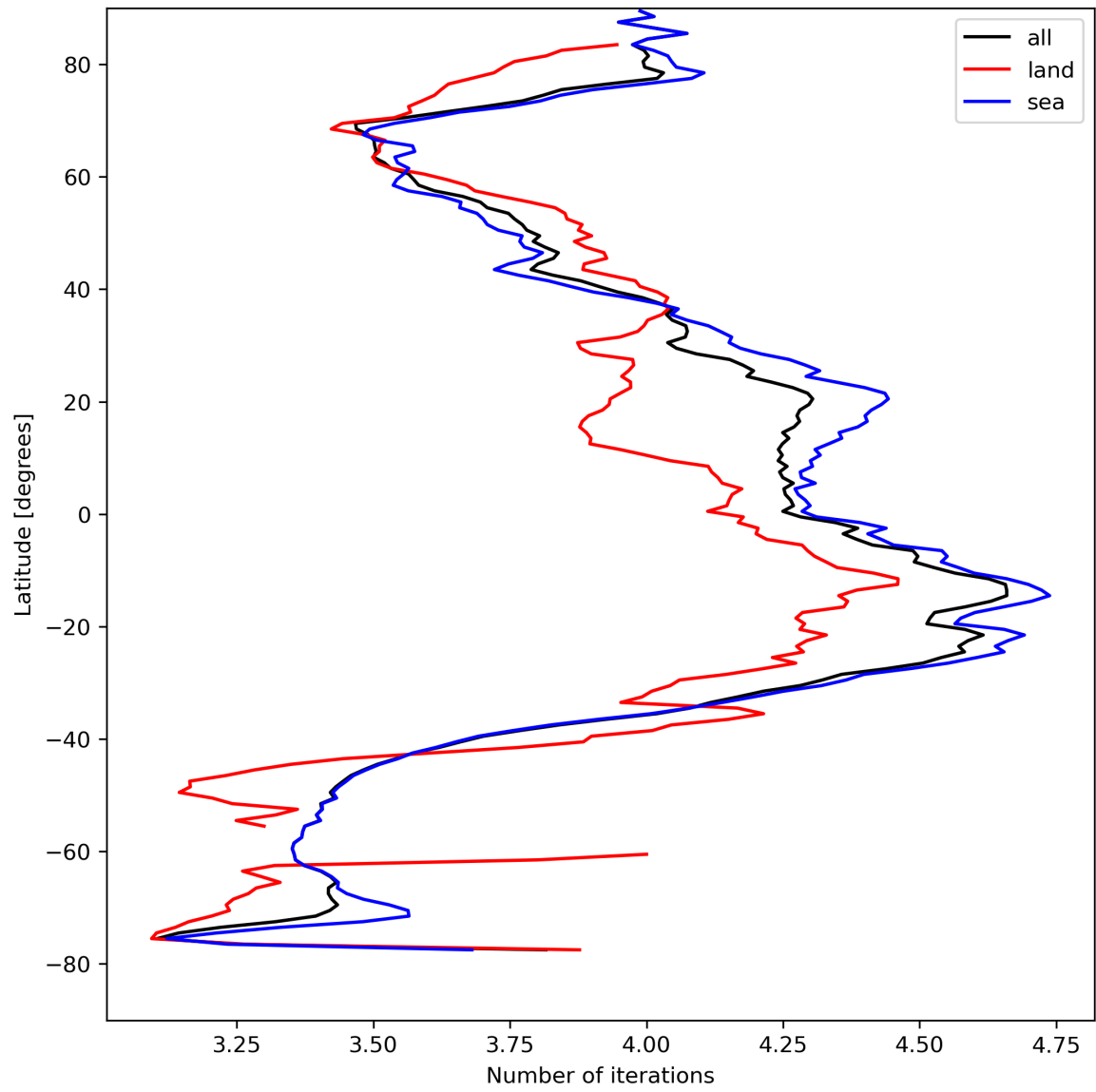
Figure 17: Zonal average of “Number of iterations” for 2024-04-16 to 2024-04-18.
