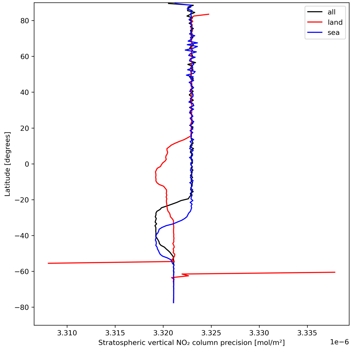
Figure 20: Zonal average of “Stratospheric vertical NO 2 column precision” for 2024-04-16 to 2024-04-18.
