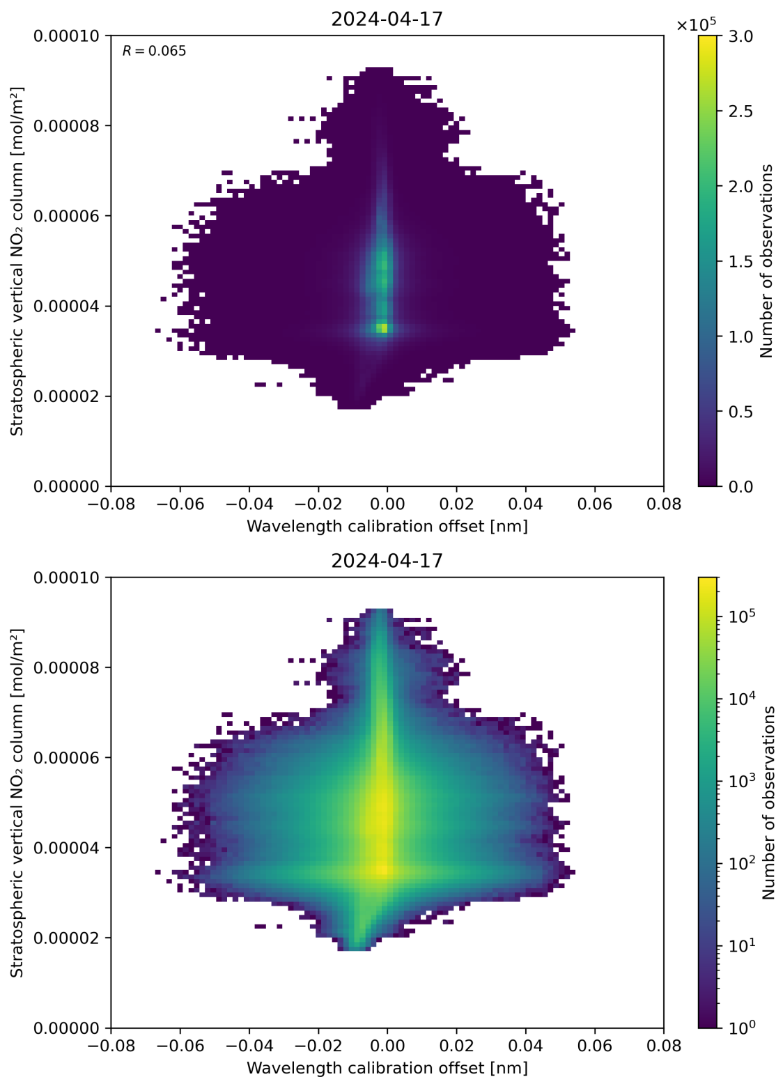
Figure 176: Scatter density plot of “Wavelength calibration offset” against “Stratospheric vertical NO 2 column” for 2024-04-16 to 2024-04-18.
