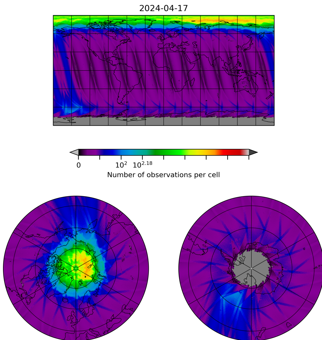
Figure 10: Map of the number of observations for 2024-04-16 to 2024-04-18
