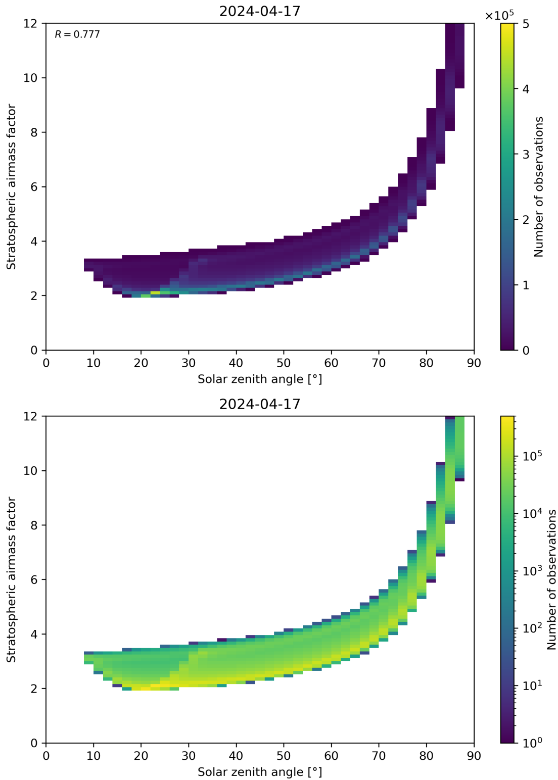
Figure 145: Scatter density plot of “Solar zenith angle” against “Stratospheric airmass factor” for 2024-04-16 to 2024-04-18.
