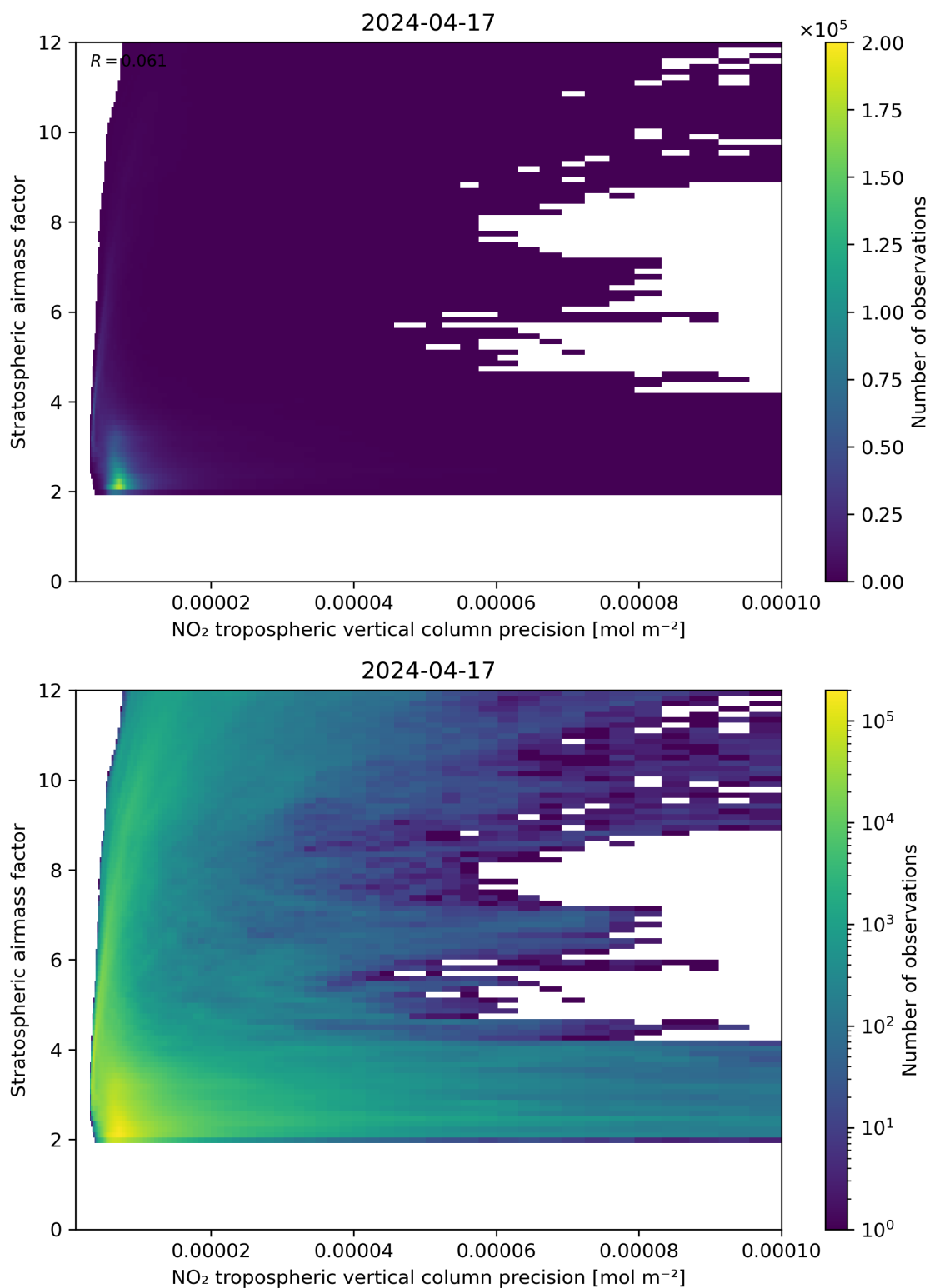
Figure 131: Scatter density plot of “NO 2 tropospheric vertical column precision” against “Stratospheric airmass factor” for 2024-04-16 to 2024-04-18.
