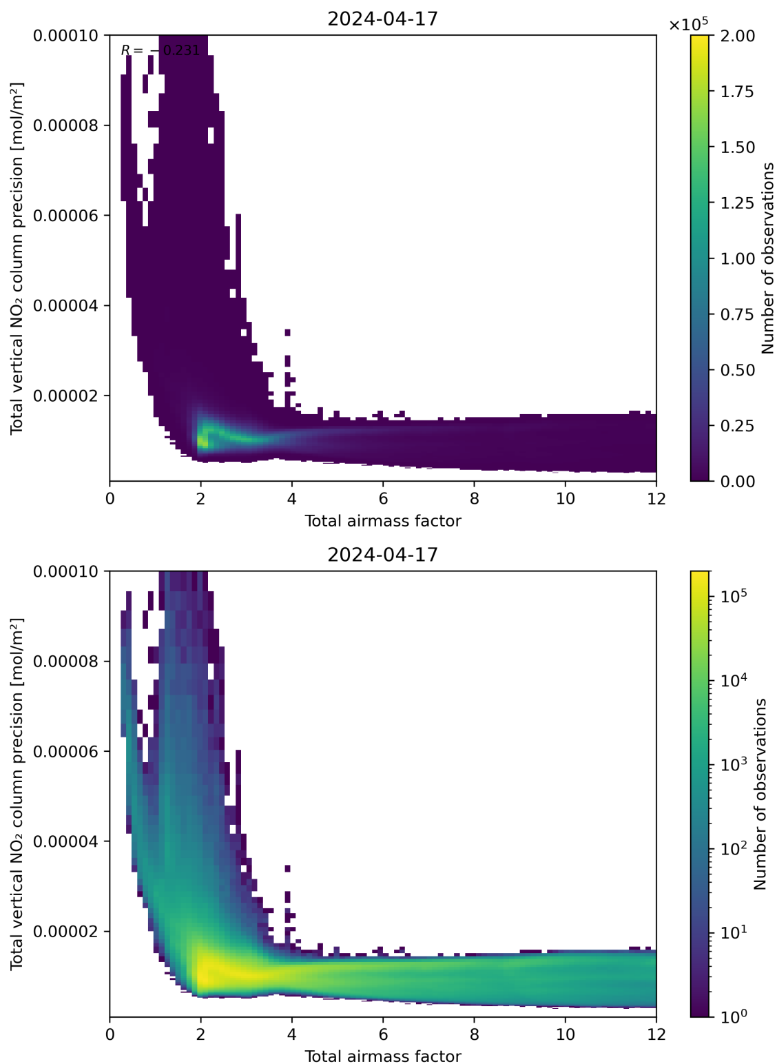
Figure 68: Scatter density plot of “Total airmass factor” against “Total vertical NO 2 column precision” for 2024-04-16 to 2024-04-18.
