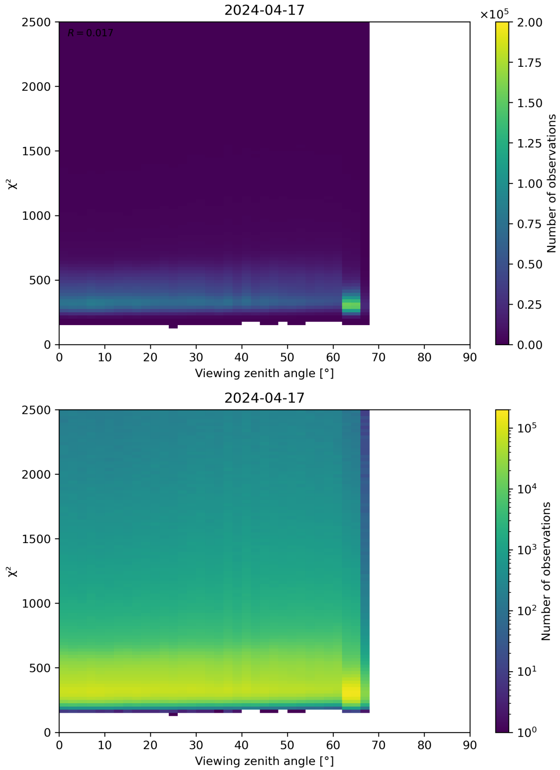
Figure 162: Scatter density plot of “Viewing zenith angle” against “ \chi^2 ” for 2024-04-16 to 2024-04-18.
