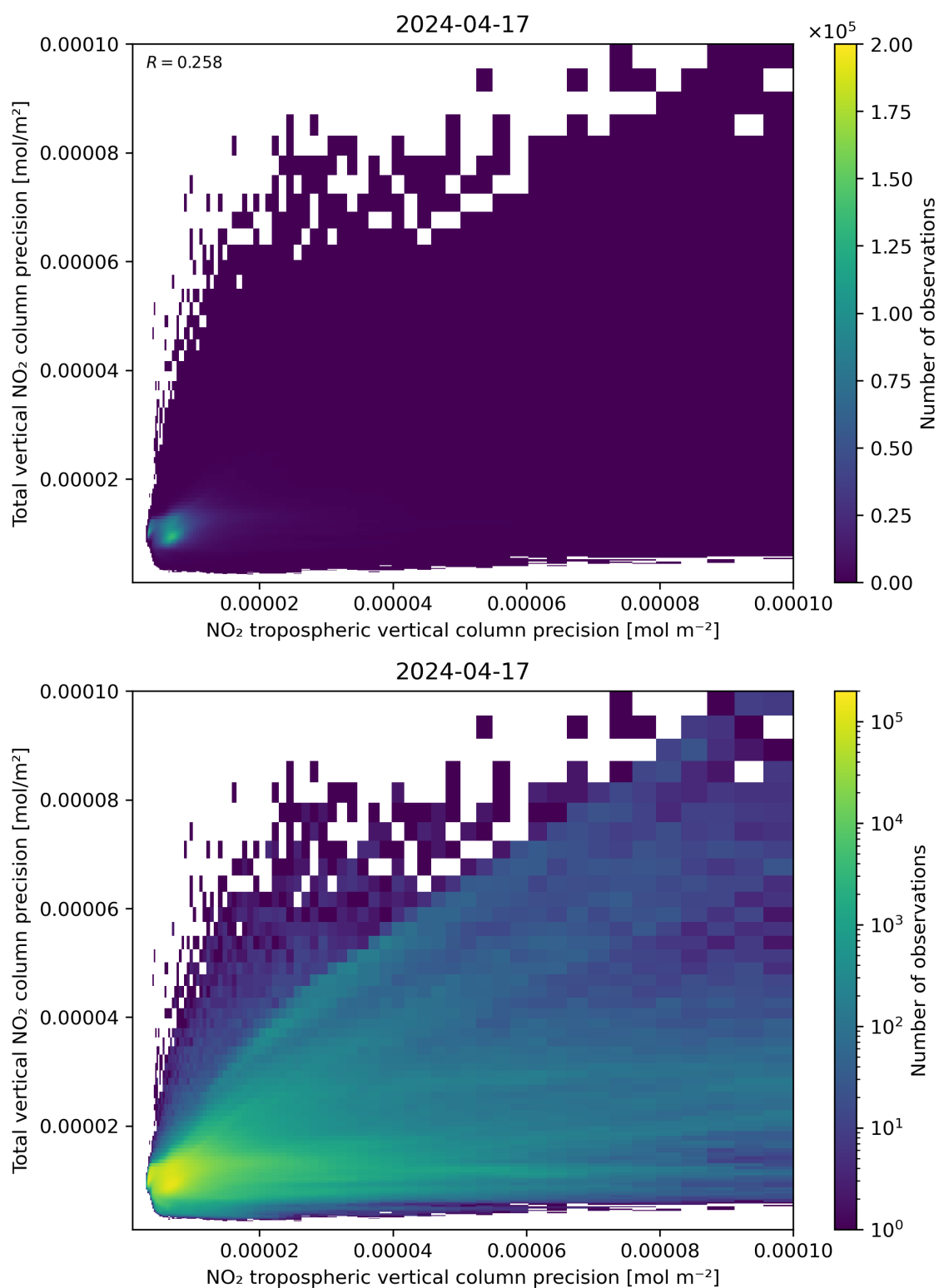
Figure 139: Scatter density plot of “NO 2 tropospheric vertical column precision” against “Total vertical NO 2 column precision” for 2024-04-16 to 2024-04-18.
