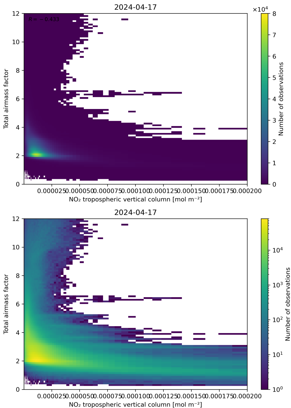
Figure 122: Scatter density plot of “NO 2 tropospheric vertical column” against “Total air mass factor” for 2024-04-16 to 2024-04-18.
