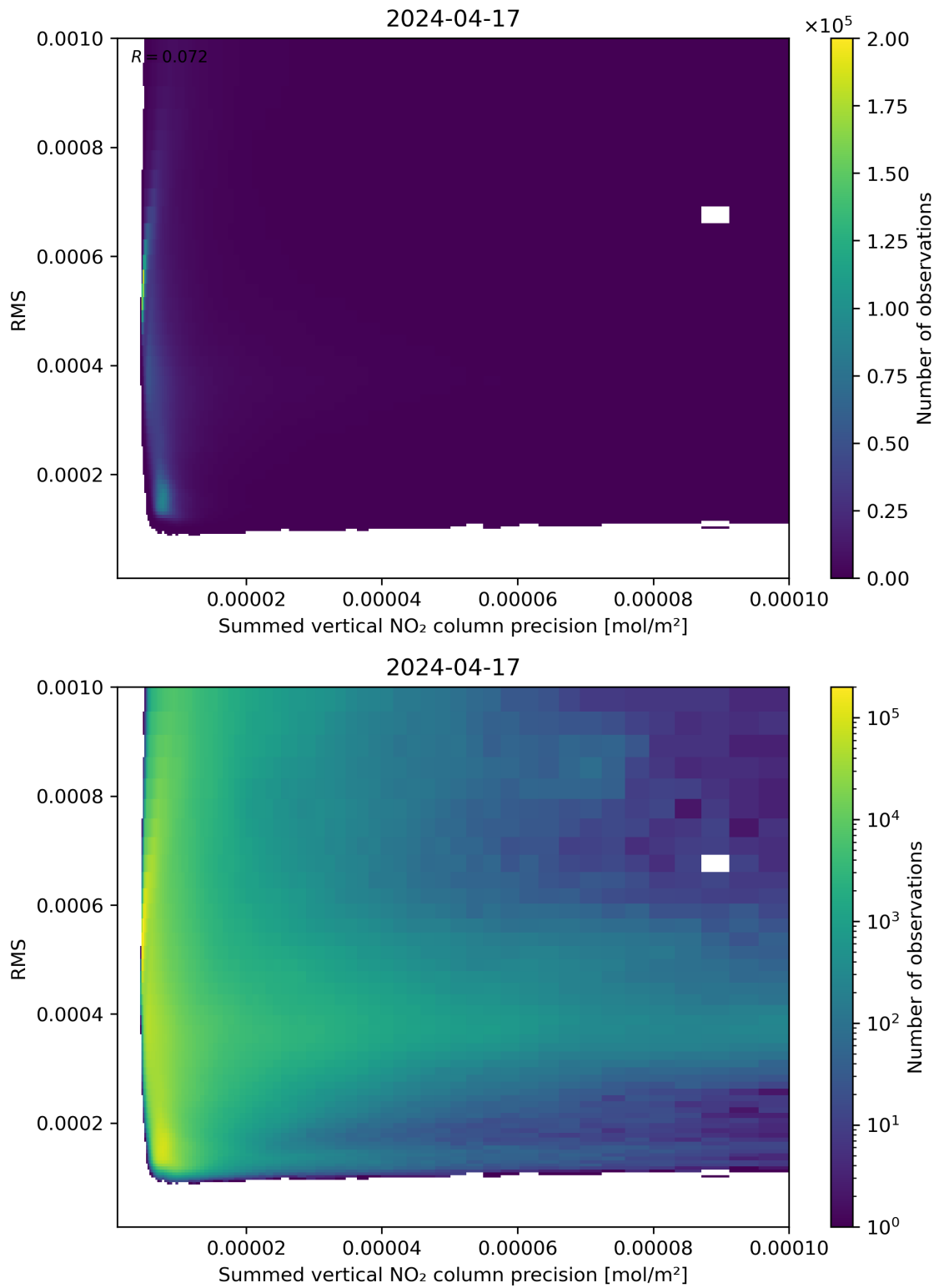
Figure 108: Scatter density plot of “Summed vertical NO 2 column precision” against “RMS” for 2024-04-16 to 2024-04-18.
