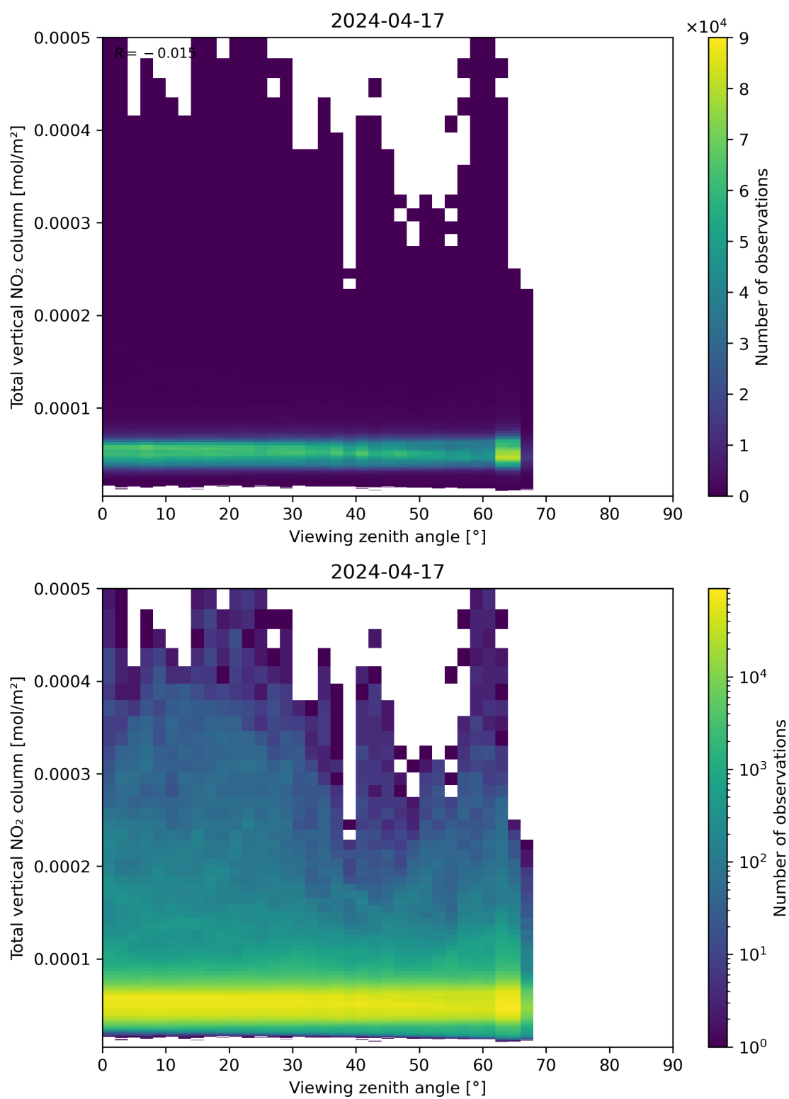
Figure 167: Scatter density plot of “Viewing zenith angle” against “Total vertical NO 2 column” for 2024-04-16 to 2024-04-18.
