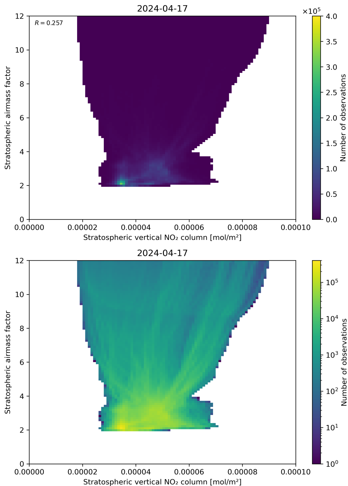
Figure 96: Scatter density plot of “Stratospheric vertical NO 2 column” against “Stratospheric airmass factor” for 2024-04-16 to 2024-04-18.
