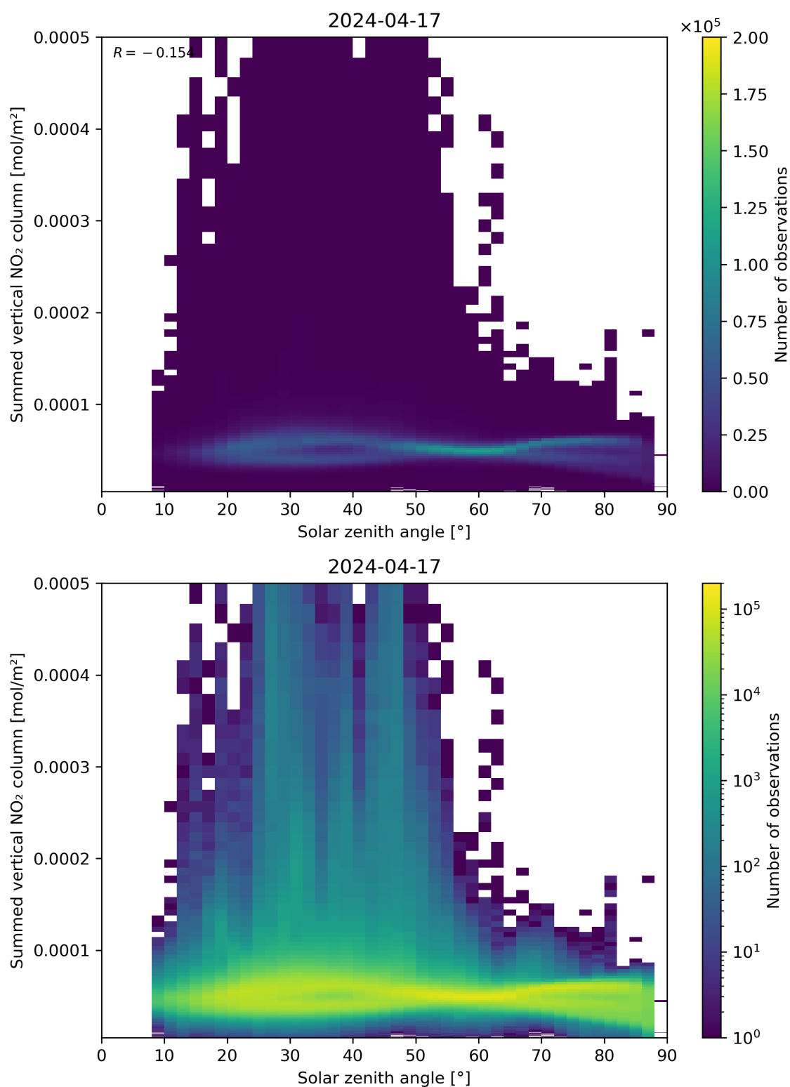
Figure 151: Scatter density plot of “Solar zenith angle” against “Summed vertical NO 2 column” for 2024-04-16 to 2024-04-18.
