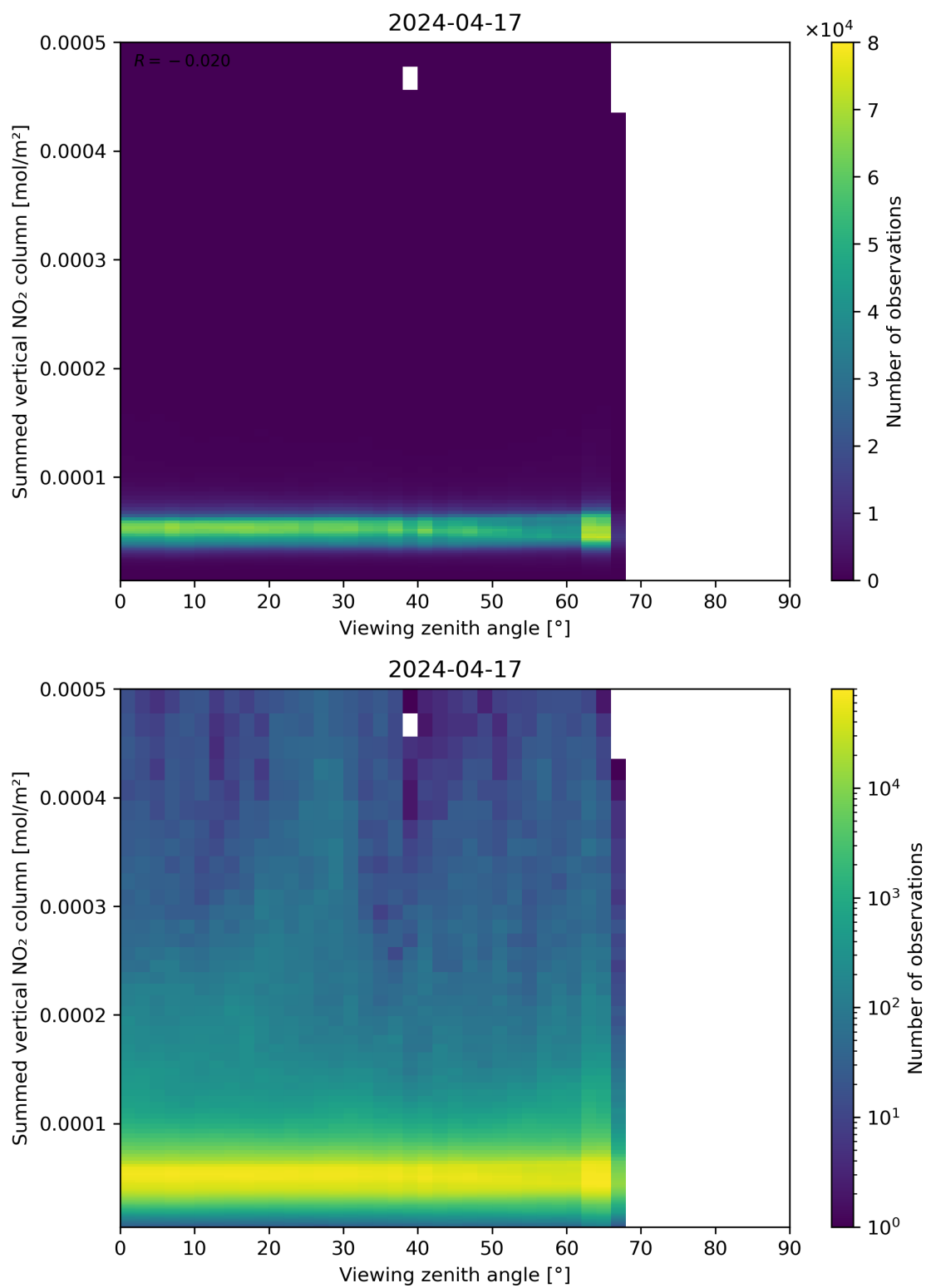
Figure 165: Scatter density plot of “Viewing zenith angle” against “Summed vertical NO 2 column” for 2024-04-16 to 2024-04-18.
