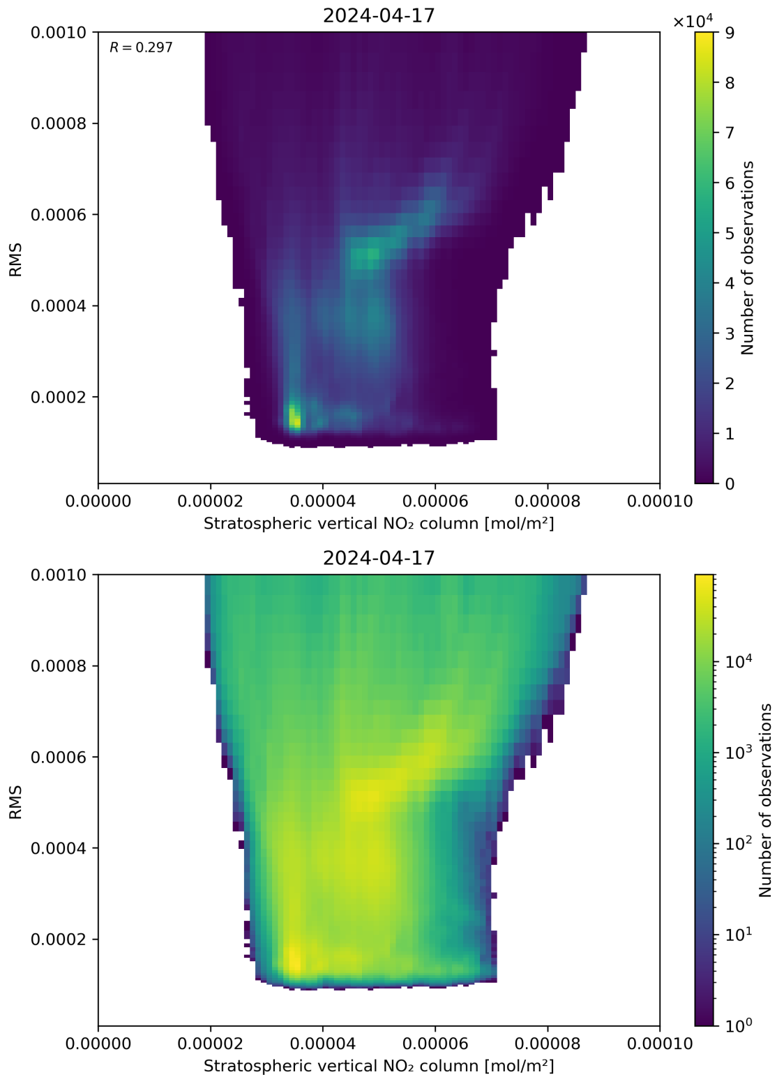
Figure 102: Scatter density plot of “Stratospheric vertical NO 2 column” against “RMS” for 2024-04-16 to 2024-04-18.
