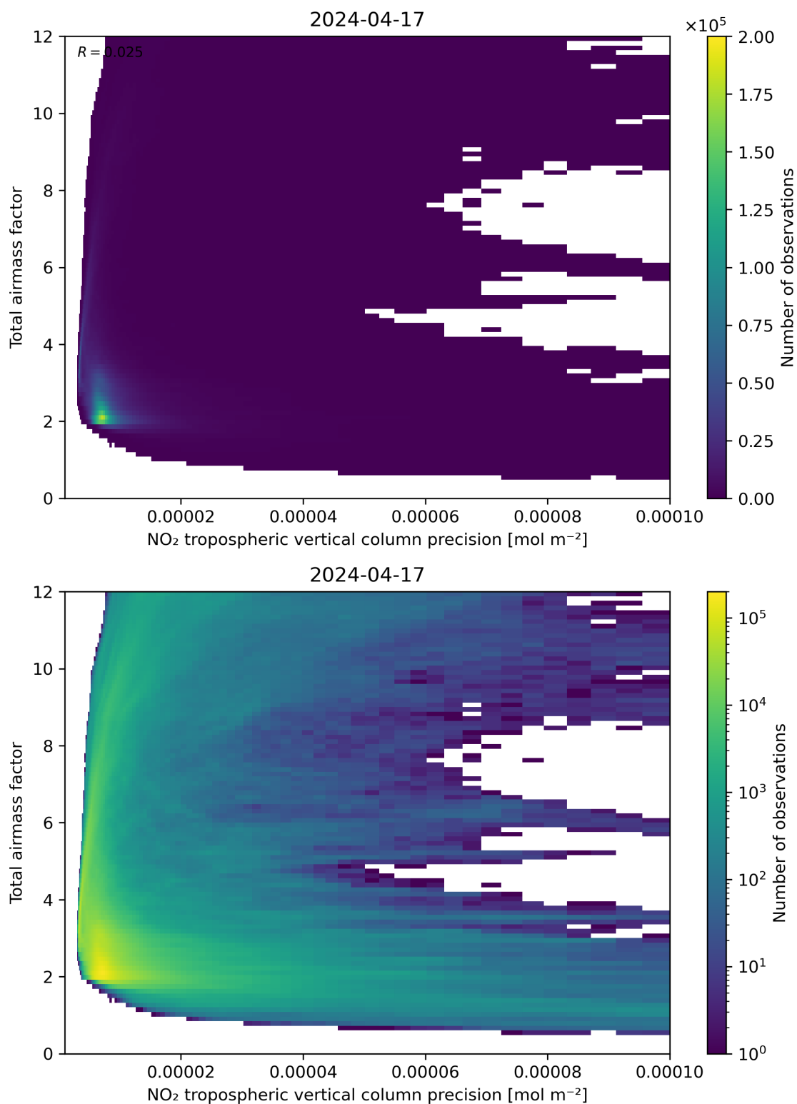
Figure 132: Scatter density plot of “NO 2 tropospheric vertical column precision” against “Total airmass factor” for 2024-04-16 to 2024-04-18.
