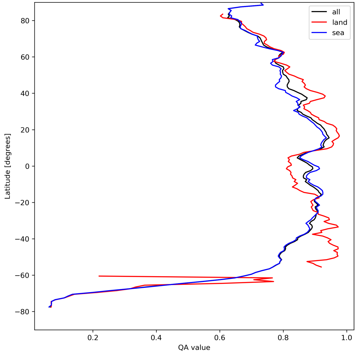
Figure 11: Zonal average of “QA value” for 2024-04-16 to 2024-04-18.
