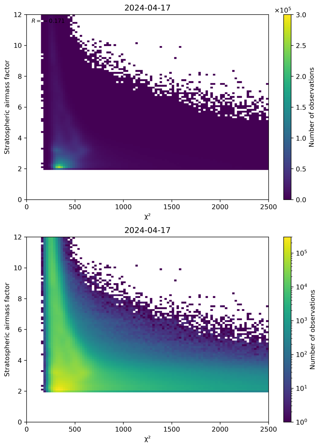
Figure 81: Scatter density plot of “ \chi^2 ” against “Stratospheric airmass factor” for 2024-04-16 to 2024-04-18.
