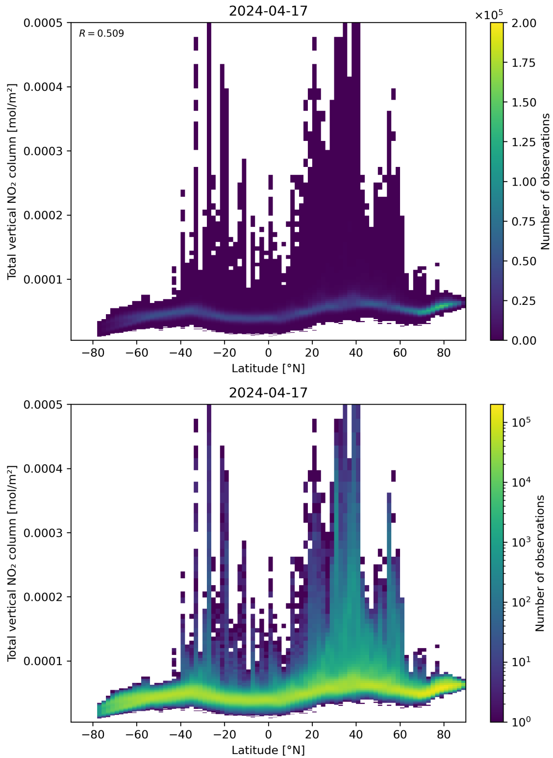
Figure 90: Scatter density plot of “Latitude” against “Total vertical NO 2 column” for 2024-04-16 to 2024-04-18.
