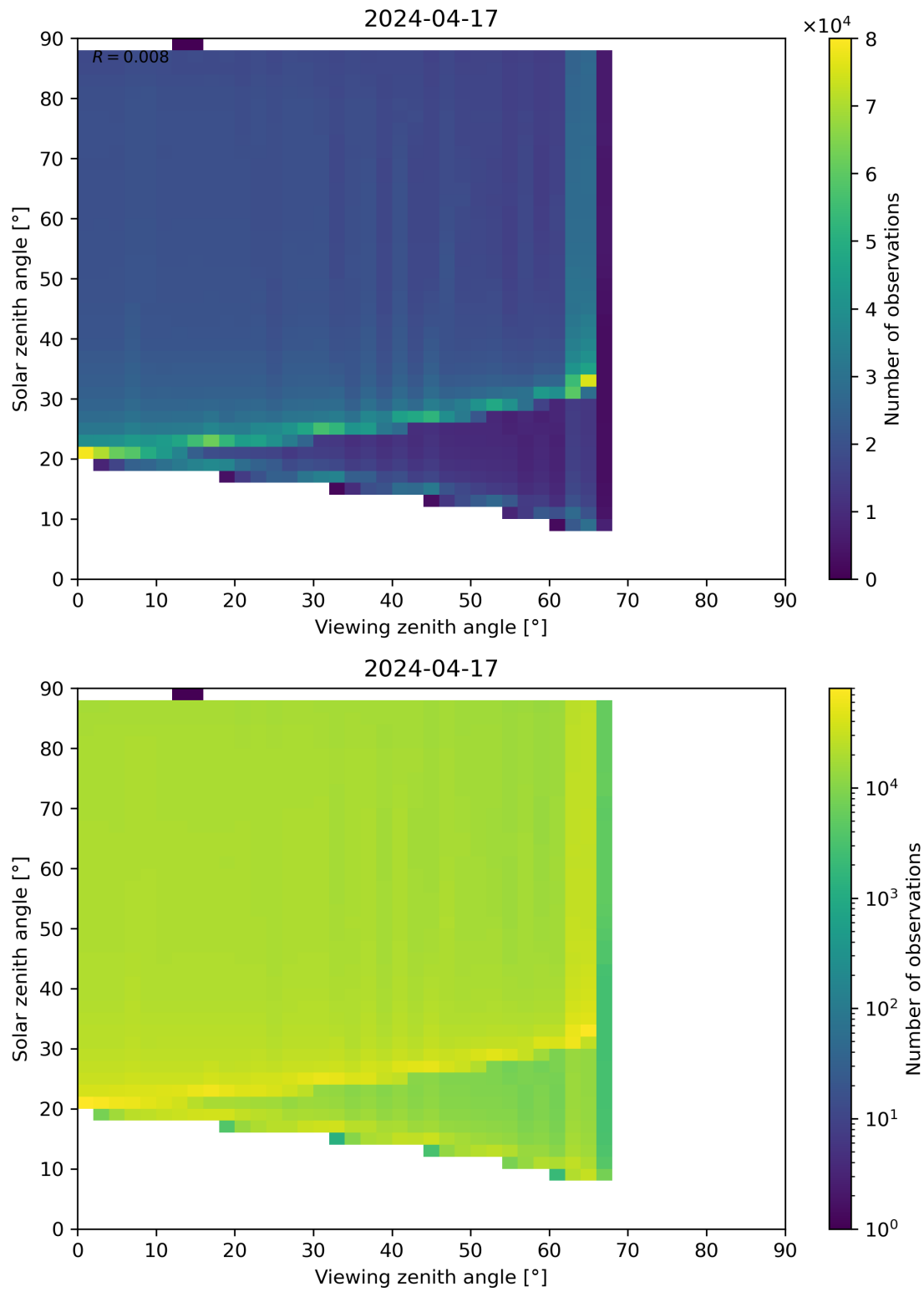
Figure 172: Scatter density plot of “Viewing zenith angle” against “Solar zenith angle” for 2024-04-16 to 2024-04-18.
