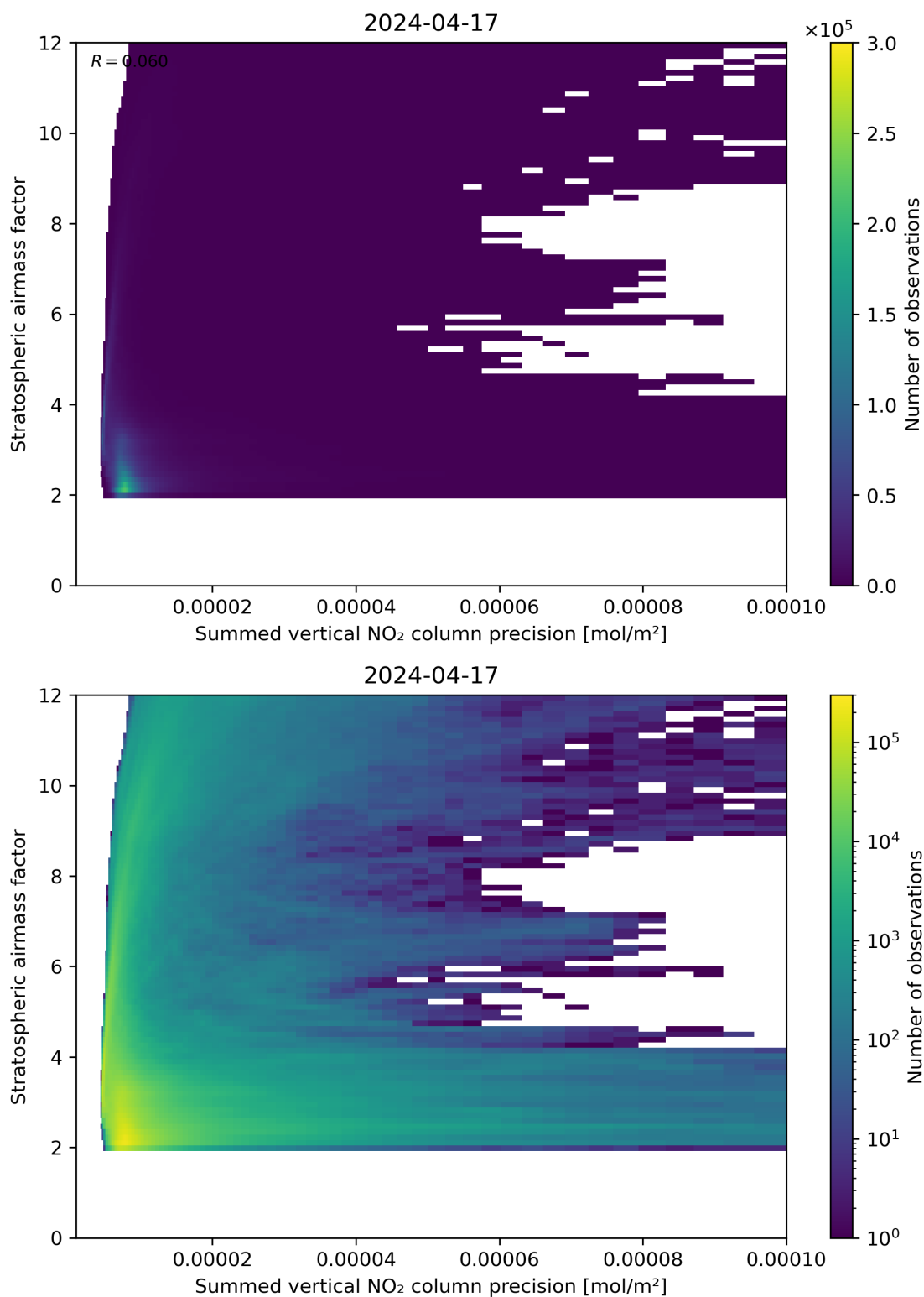
Figure 106: Scatter density plot of “Summed vertical NO 2 column precision” against “Stratospheric airmass factor” for 2024-04-16 to 2024-04-18.
