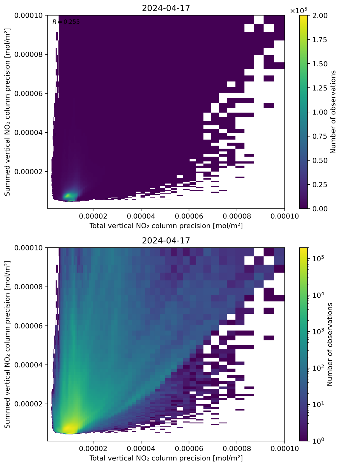
Figure 118: Scatter density plot of “Total vertical NO 2 column precision” against “Summed vertical NO 2 column precision” for 2024-04-16 to 2024-04-18.
