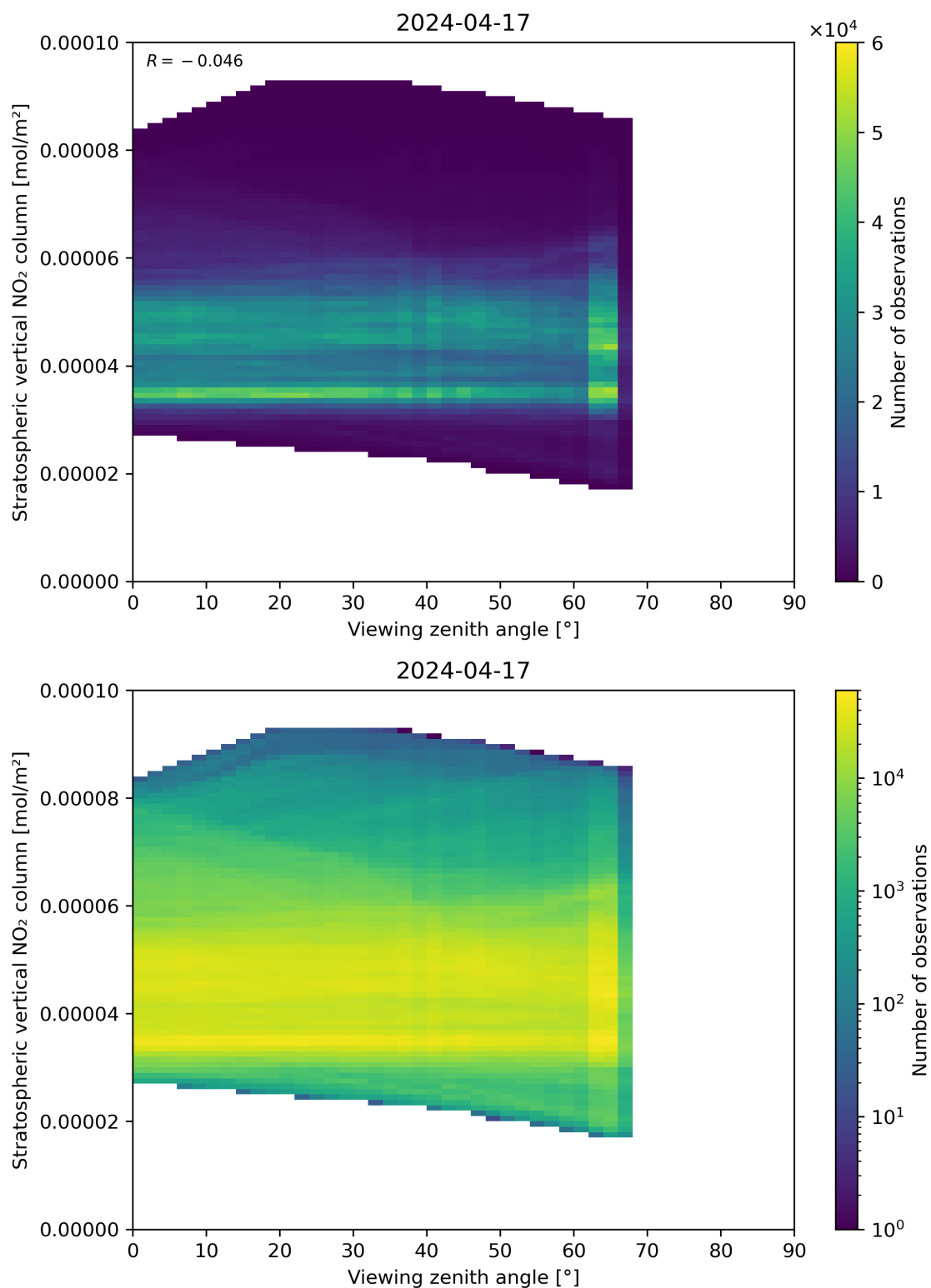
Figure 164: Scatter density plot of “Viewing zenith angle” against “Stratospheric vertical NO 2 column” for 2024-04-16 to 2024-04-18.
