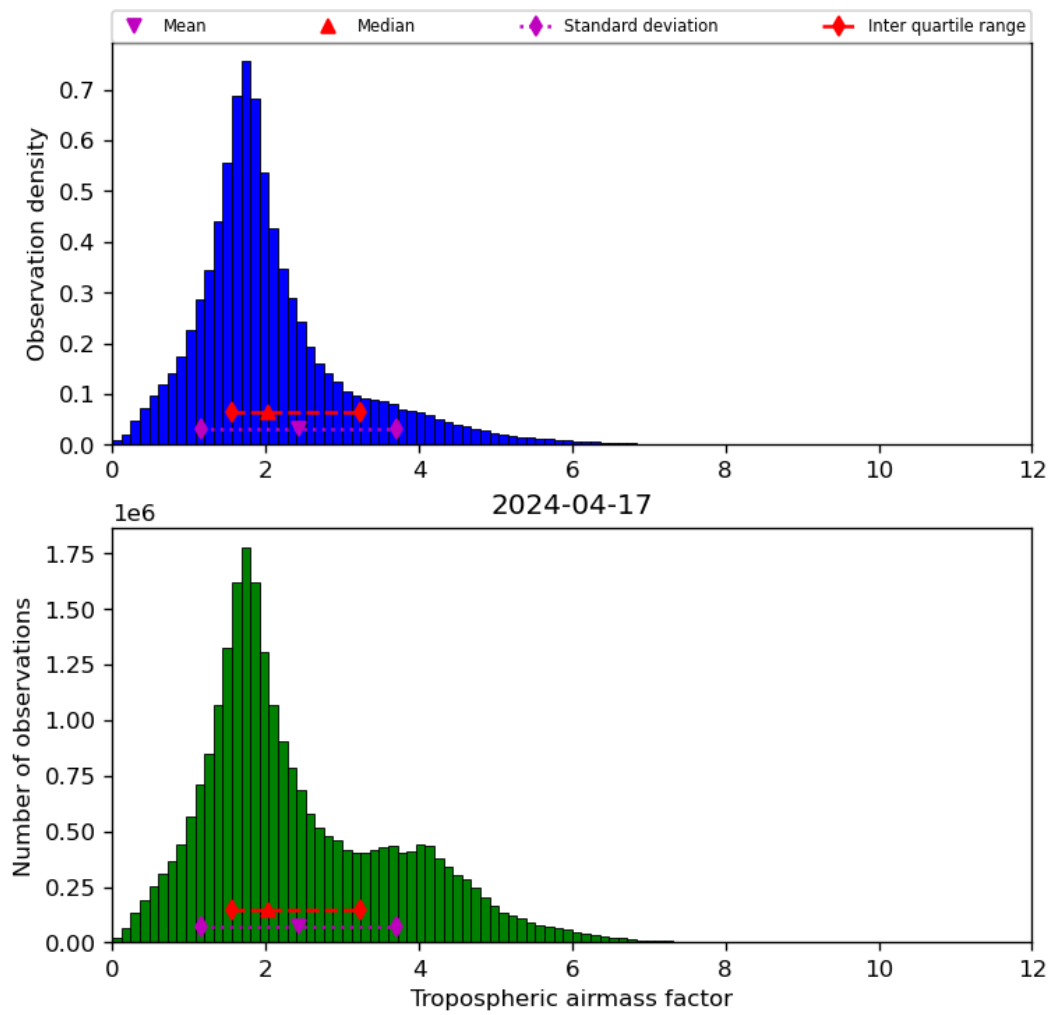
Figure 31: Histogram of “Tropospheric airmass factor” for 2024-04-16 to 2024-04-18
