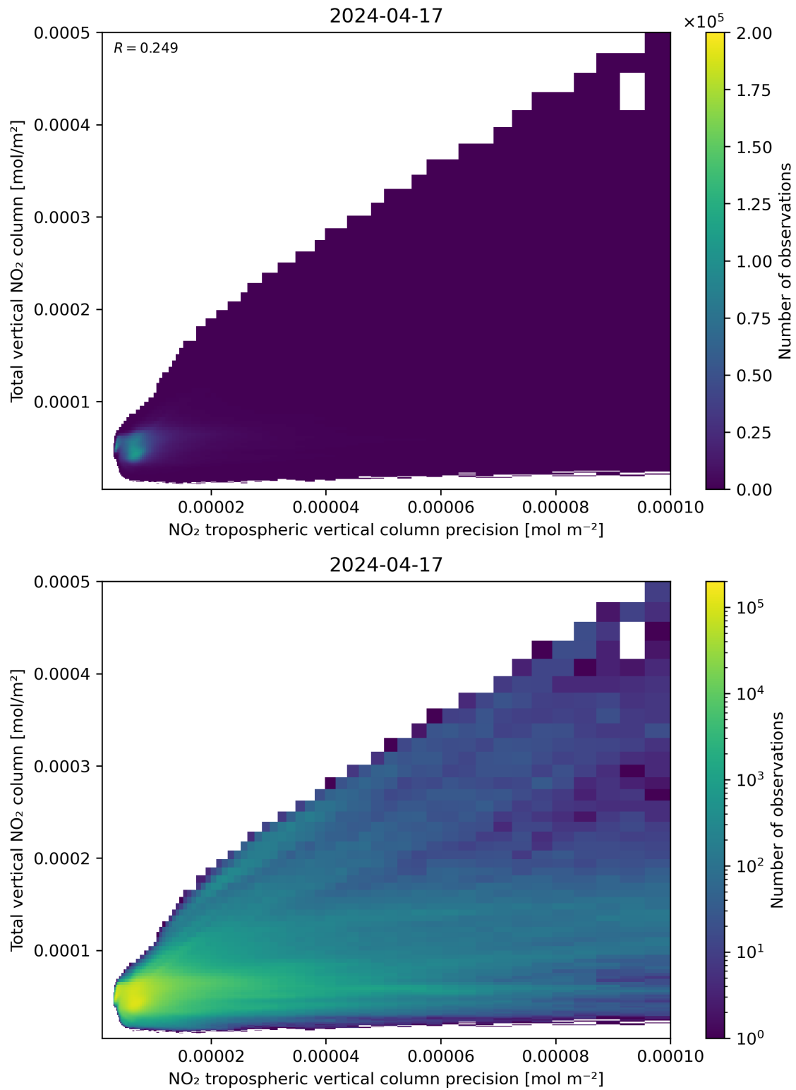
Figure 138: Scatter density plot of “NO 2 tropospheric vertical column precision” against “Total vertical NO 2 column” for 2024-04-16 to 2024-04-18.
