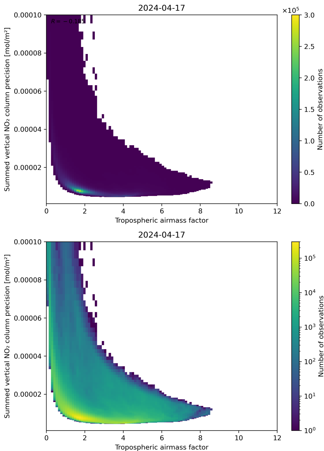
Figure 76: Scatter density plot of “Tropospheric air mass factor” against “Summed vertical NO 2 column precision” for 2024-04-16 to 2024-04-18.
