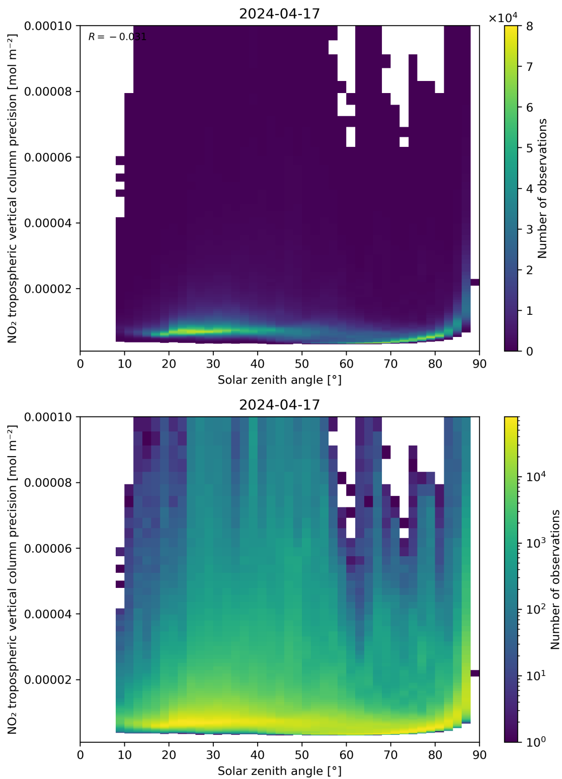
Figure 156: Scatter density plot of “Solar zenith angle” against “NO 2 tropospheric vertical column precision” for 2024-04-16 to 2024-04-18.
