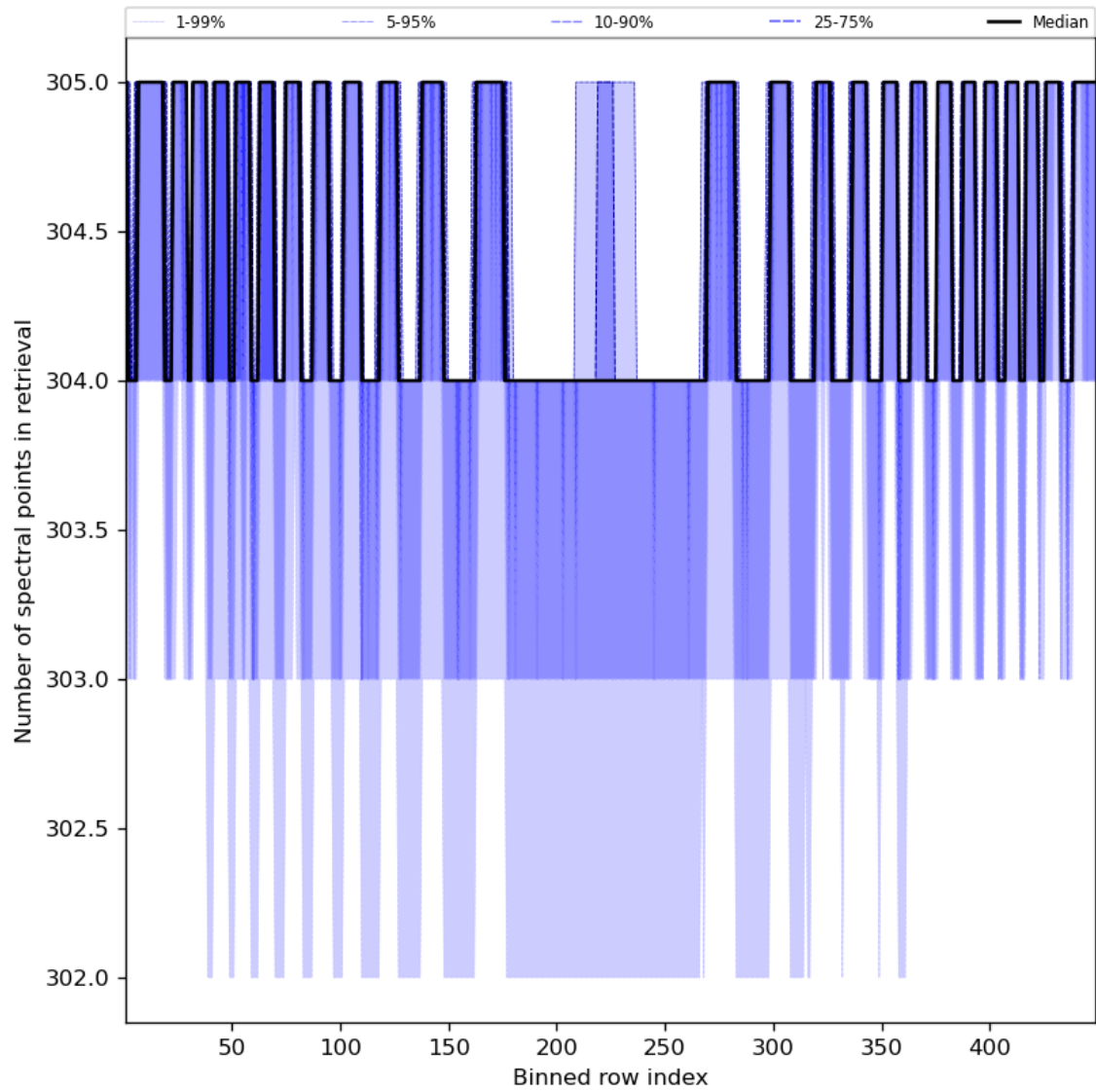
Figure 50: Along track statistics of “Number of spectral points in retrieval” for 2024-04-16 to 2024-04-18
