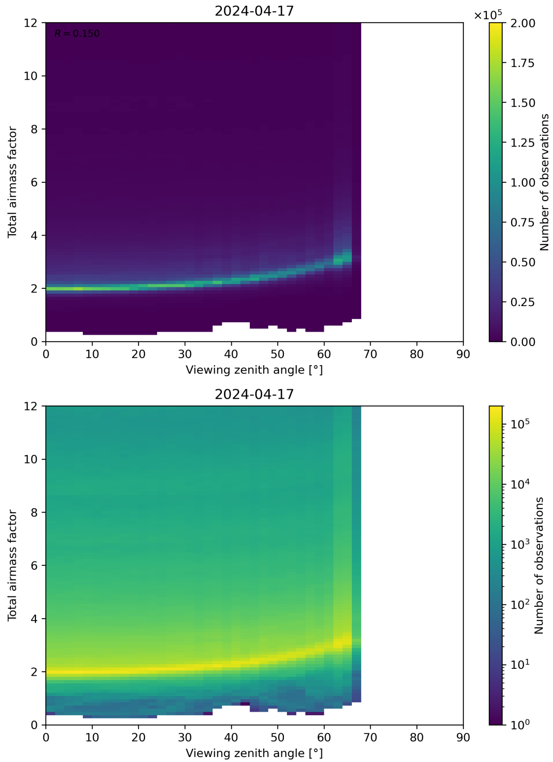
Figure 160: Scatter density plot of “Viewing zenith angle” against “Total airmass factor” for 2024-04-16 to 2024-04-18.
