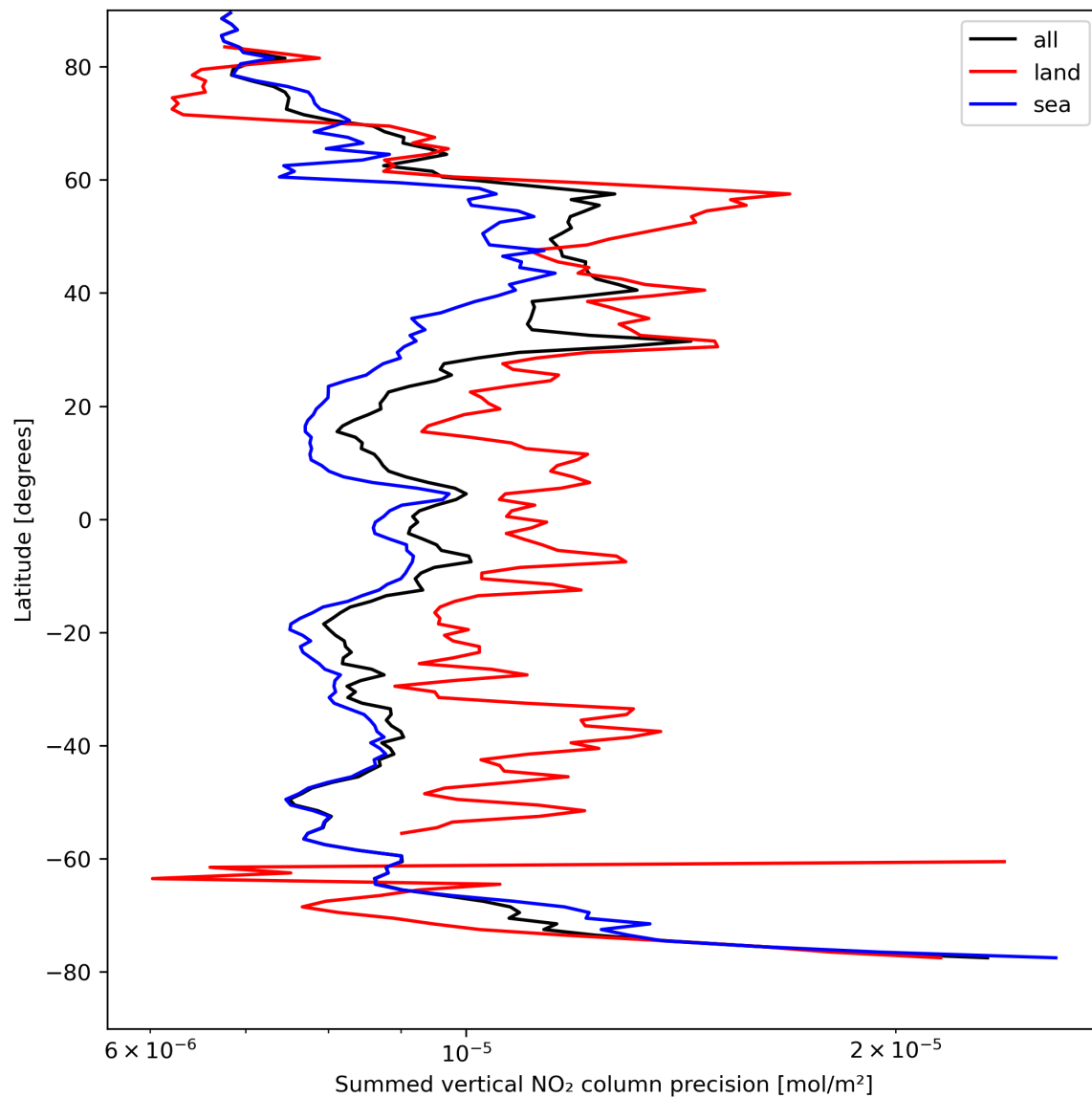
Figure 24: Zonal average of “Summed vertical NO 2 column precision” for 2024-04-16 to 2024-04-18.
