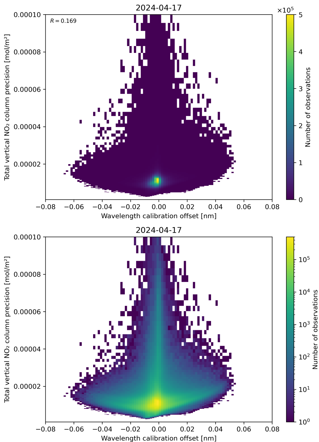
Figure 180: Scatter density plot of “Wavelength calibration offset” against “Total vertical NO 2 column precision” for 2024-04-16 to 2024-04-18.
