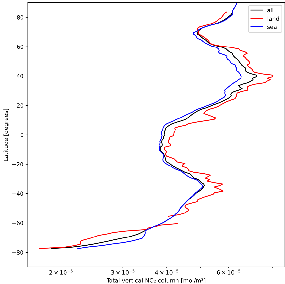
Figure 21: Zonal average of “Total vertical NO 2 column” for 2024-04-16 to 2024-04-18.
