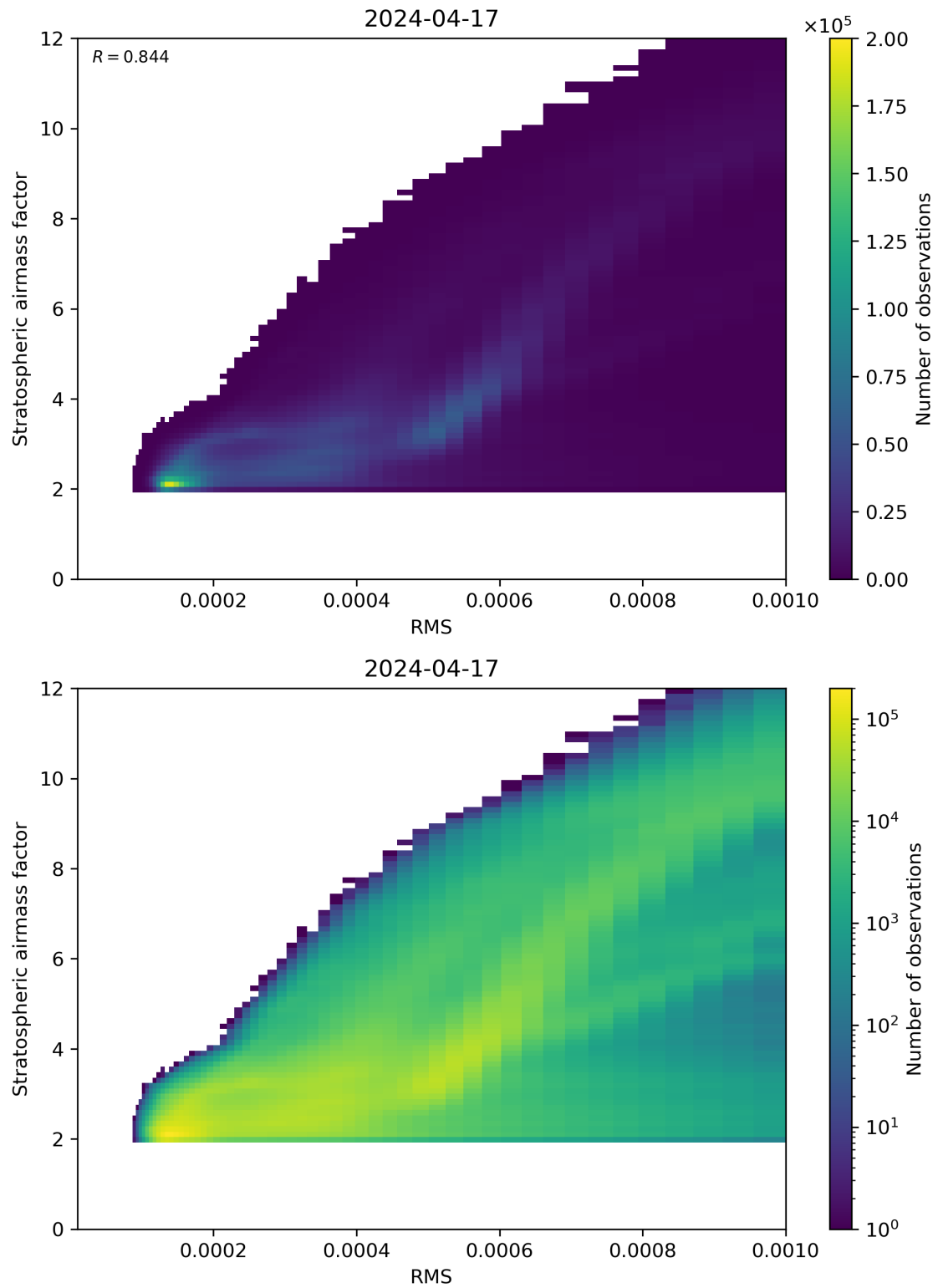
Figure 144: Scatter density plot of “RMS” against “Stratospheric airmass factor” for 2024-04-16 to 2024-04-18.
