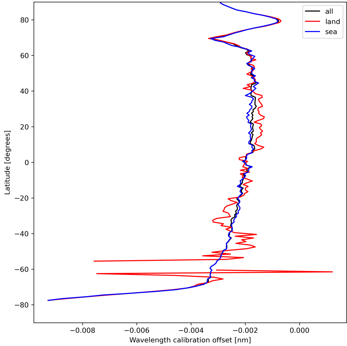
Figure 18: Zonal average of “Wavelength calibration offset” for 2024-04-16 to 2024-04-18.
