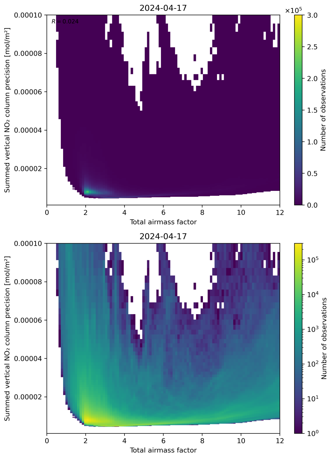
Figure 66: Scatter density plot of “Total airmass factor” against “Summed vertical NO 2 column precision” for 2024-04-16 to 2024-04-18.
