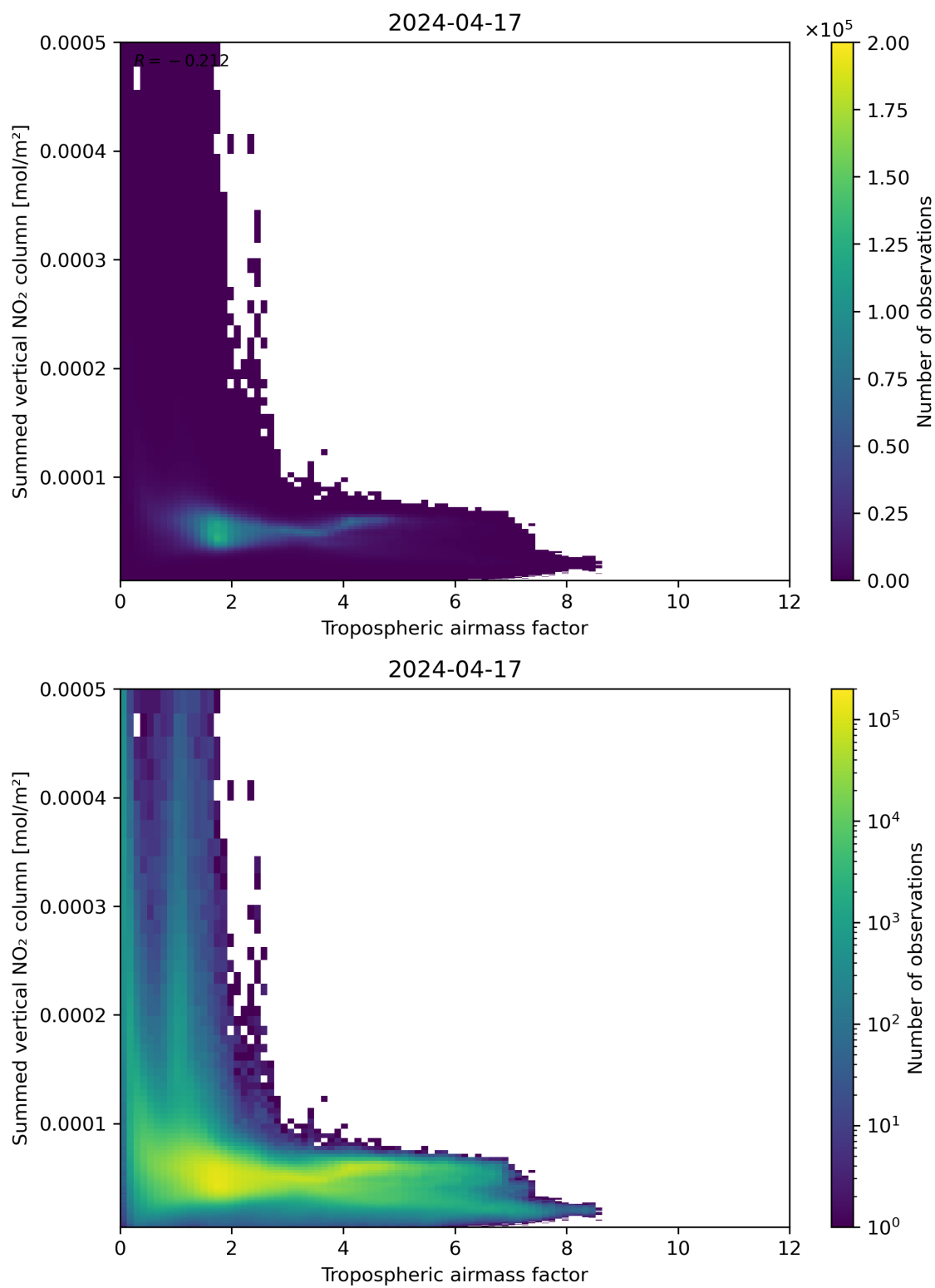
Figure 75: Scatter density plot of “Tropospheric airmass factor” against “Summed vertical NO 2 column” for 2024-04-16 to 2024-04-18.
