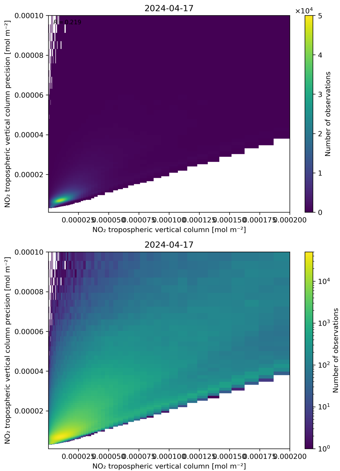
Figure 130: Scatter density plot of “NO 2 tropospheric vertical column” against “NO 2 tropospheric vertical column precision” for 2024-04-16 to 2024-04-18.
