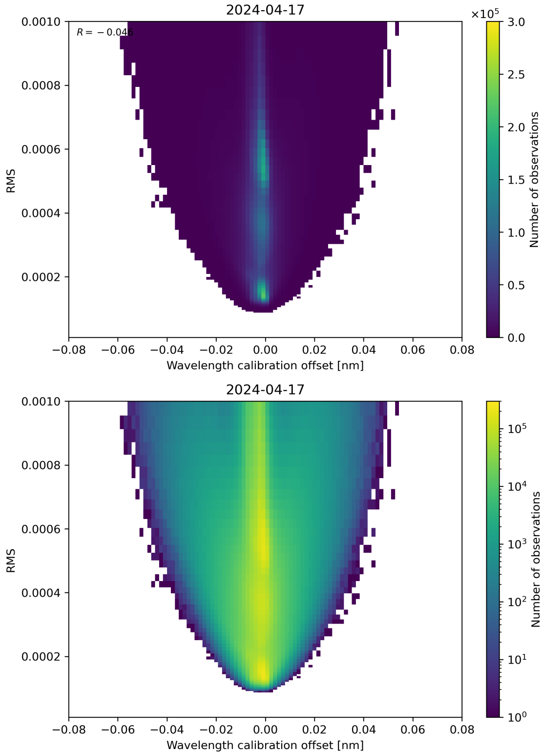
Figure 181: Scatter density plot of “Wavelength calibration offset” against “RMS” for 2024-04-16 to 2024-04-18.
