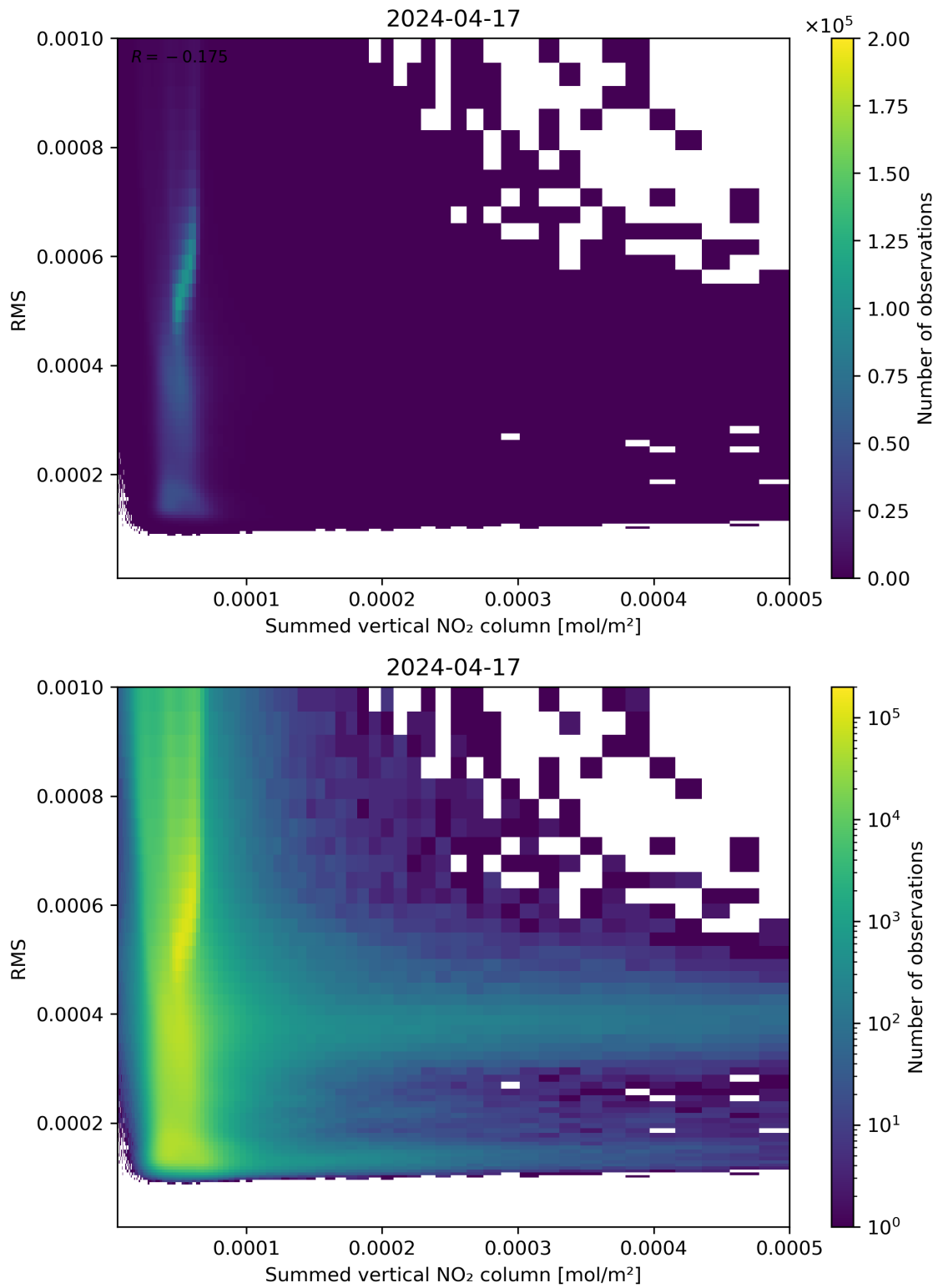
Figure 109: Scatter density plot of “Summed vertical NO 2 column” against “RMS” for 2024-04-16 to 2024-04-18.
