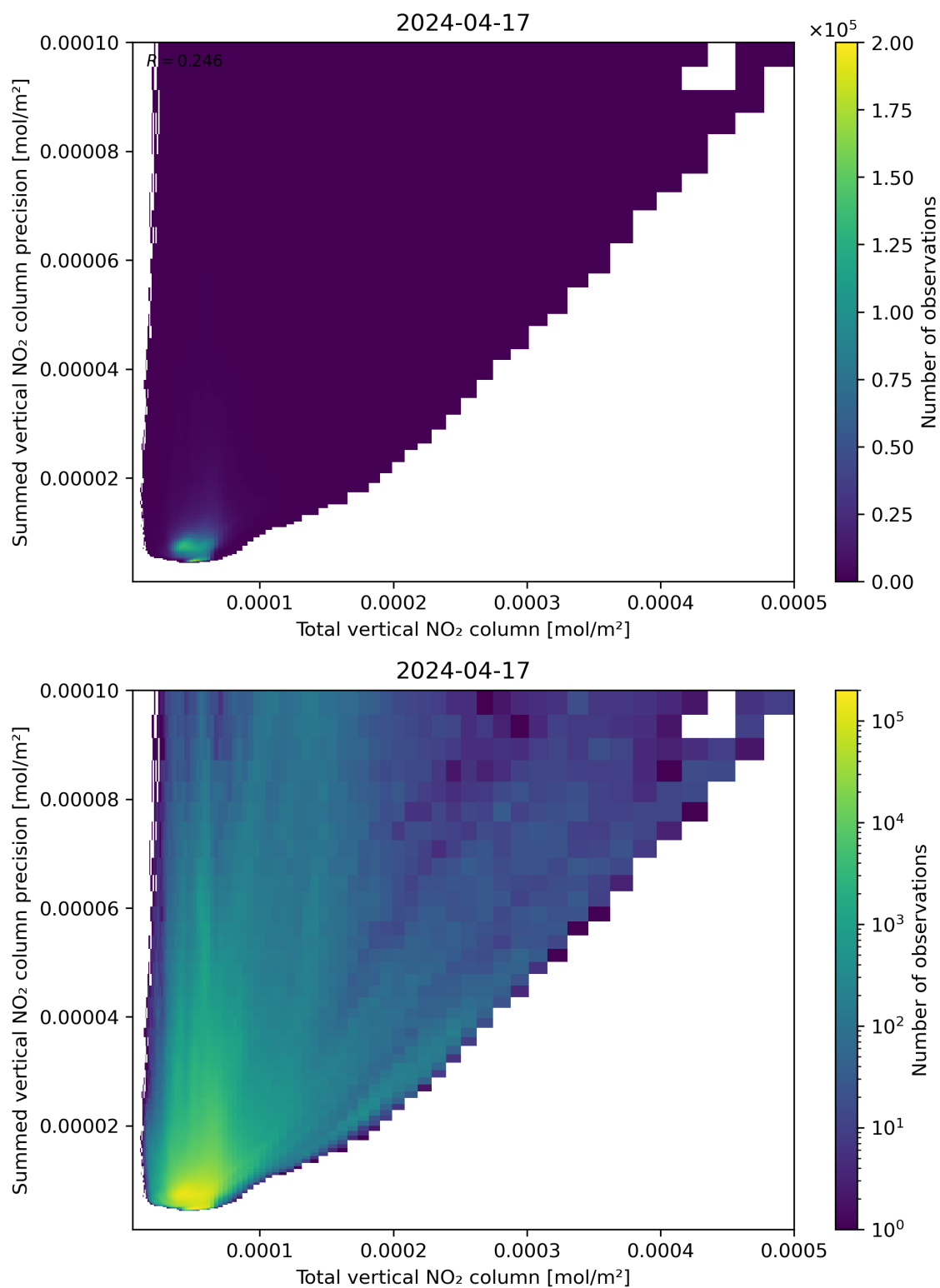
Figure 113: Scatter density plot of “Total vertical NO 2 column” against “Summed vertical NO 2 column precision” for 2024-04-16 to 2024-04-18.
