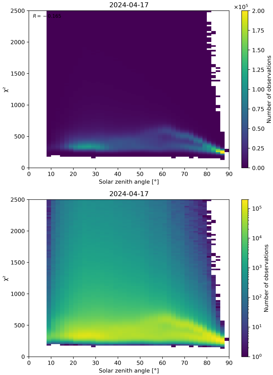
Figure 148: Scatter density plot of “Solar zenith angle” against “ \chi^2 ” for 2024-04-16 to 2024-04-18.
