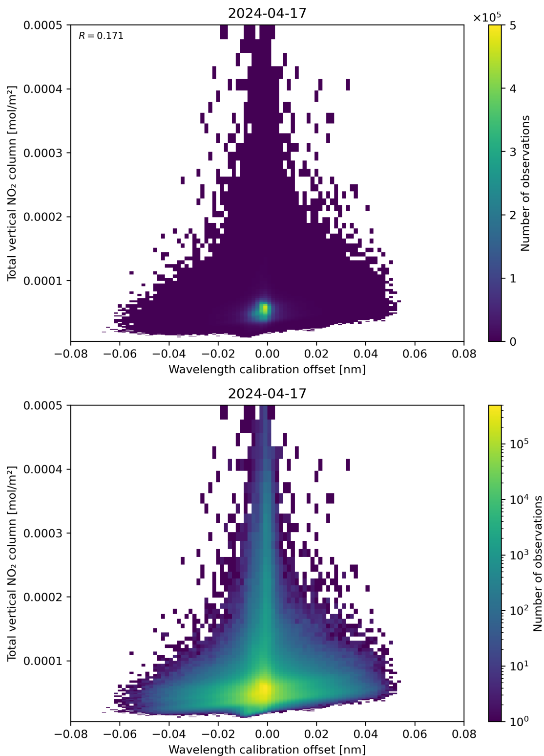
Figure 179: Scatter density plot of “Wavelength calibration offset” against “Total vertical NO 2 column” for 2024-04-16 to 2024-04-18.
