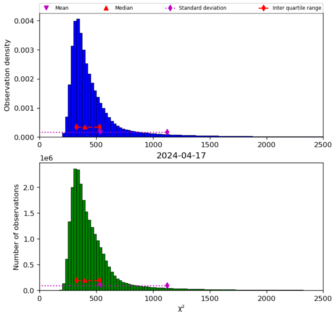
Figure 42: Histogram of “ \chi^2 ” for 2024-04-16 to 2024-04-18
