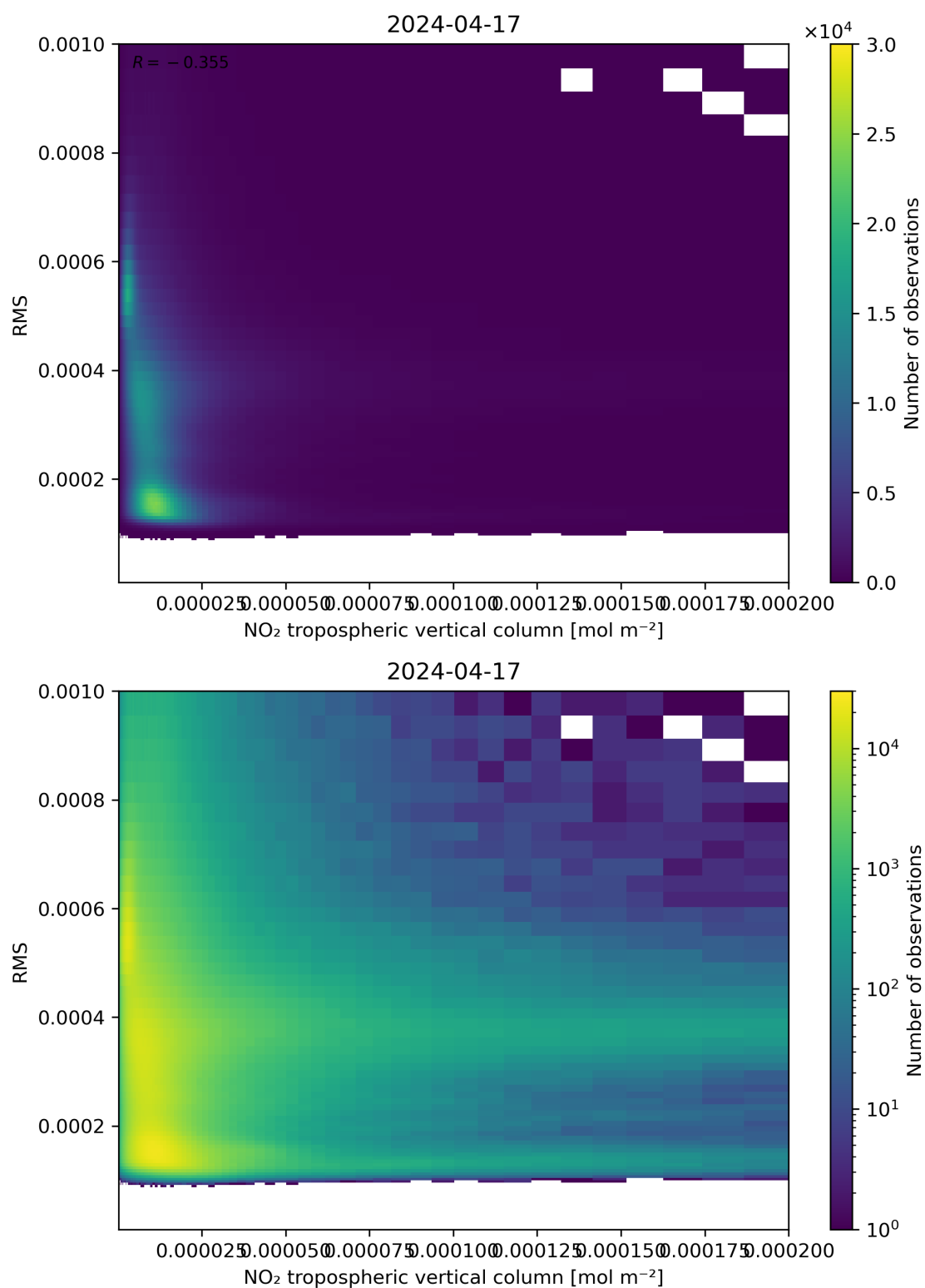
Figure 142: Scatter density plot of “NO 2 tropospheric vertical column” against “RMS” for 2024-04-16 to 2024-04-18.
