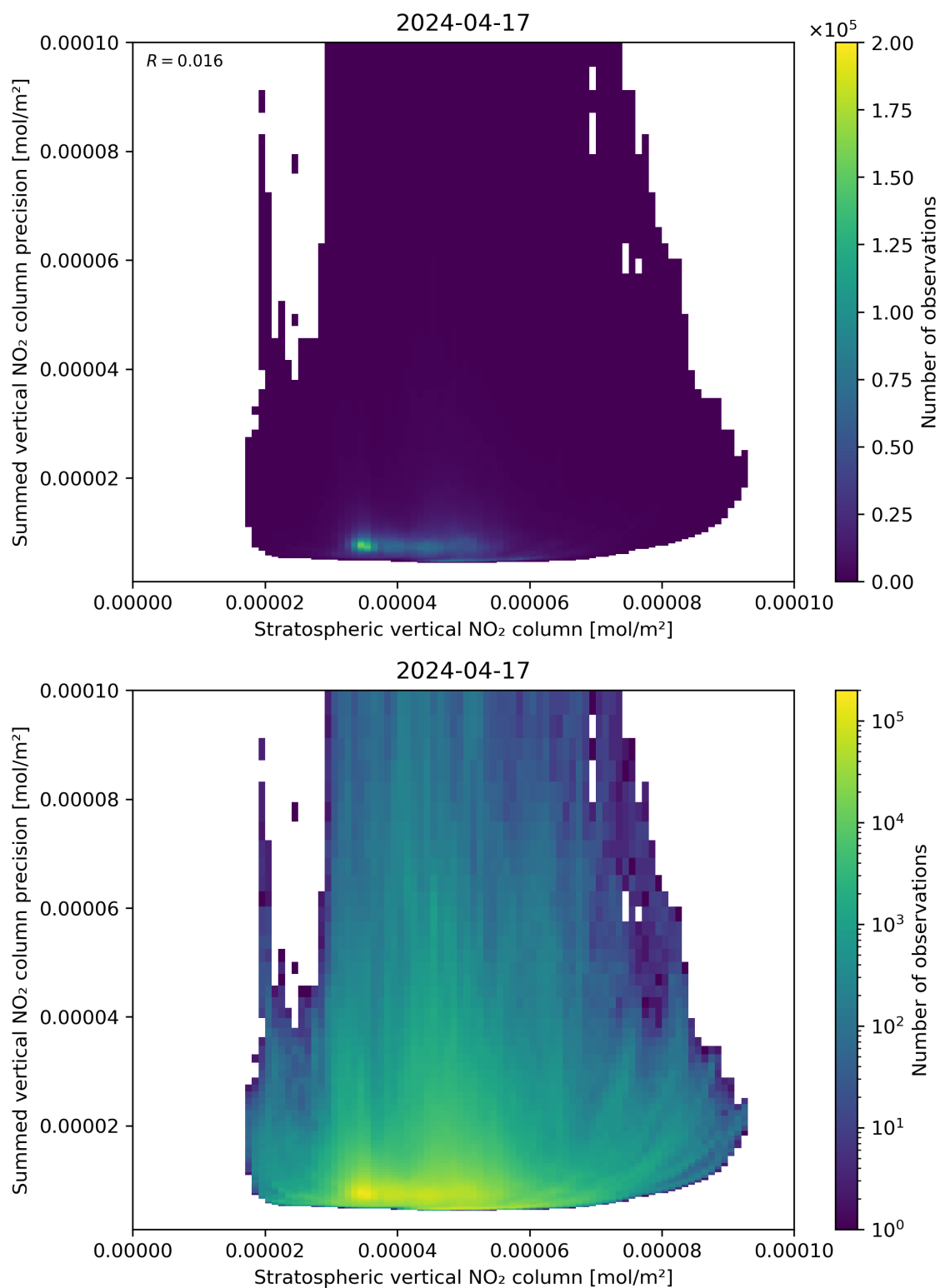
Figure 99: Scatter density plot of “Stratospheric vertical NO 2 column” against “Summed vertical NO 2 column precision” for 2024-04-16 to 2024-04-18.
