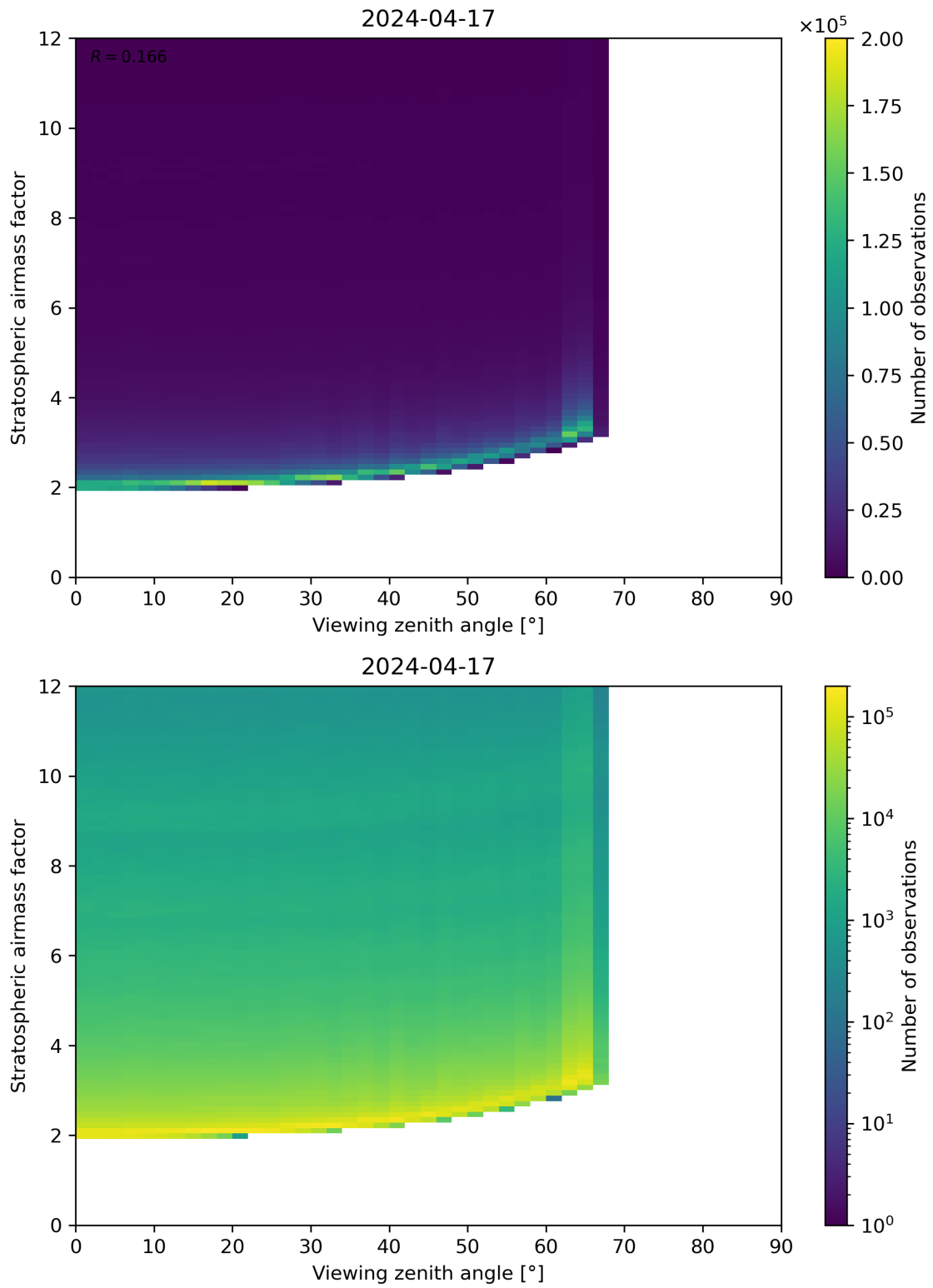
Figure 159: Scatter density plot of “Viewing zenith angle” against “Stratospheric airmass factor” for 2024-04-16 to 2024-04-18.
