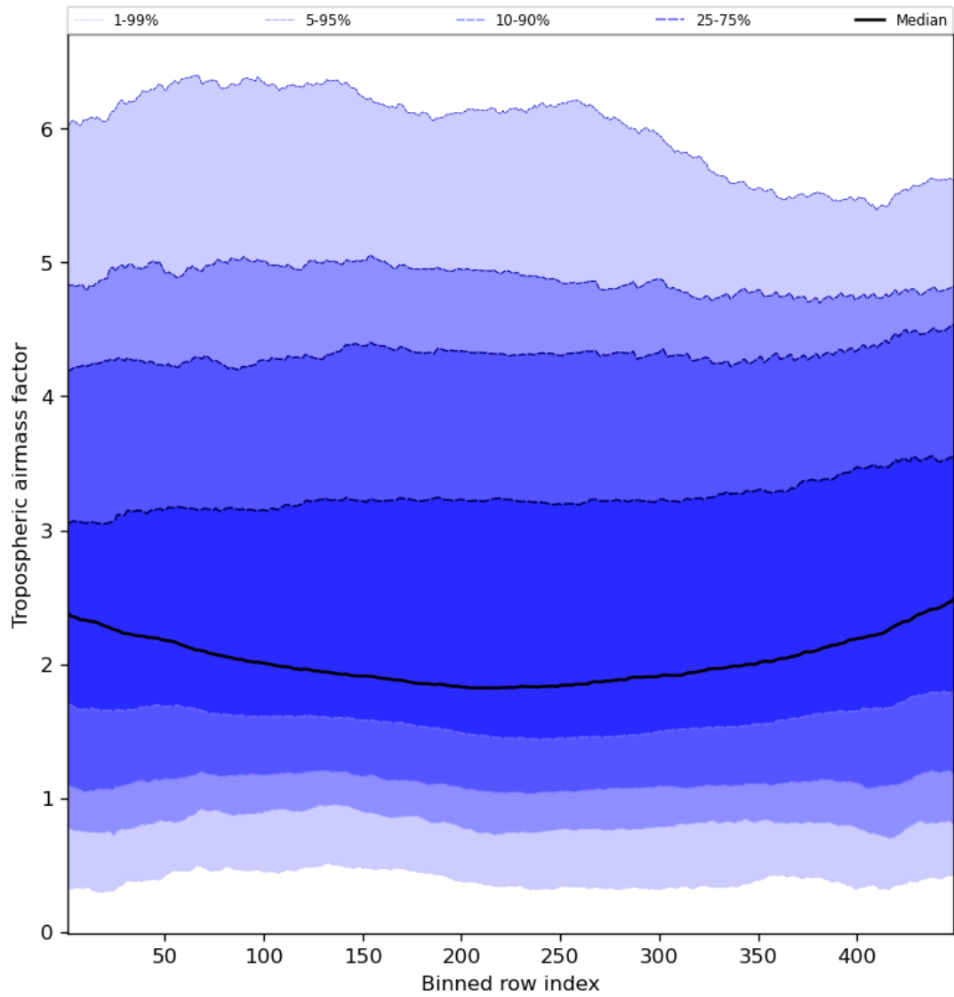
Figure 48: Along track statistics of “Tropospheric airmass factor” for 2024-04-16 to 2024-04-18
