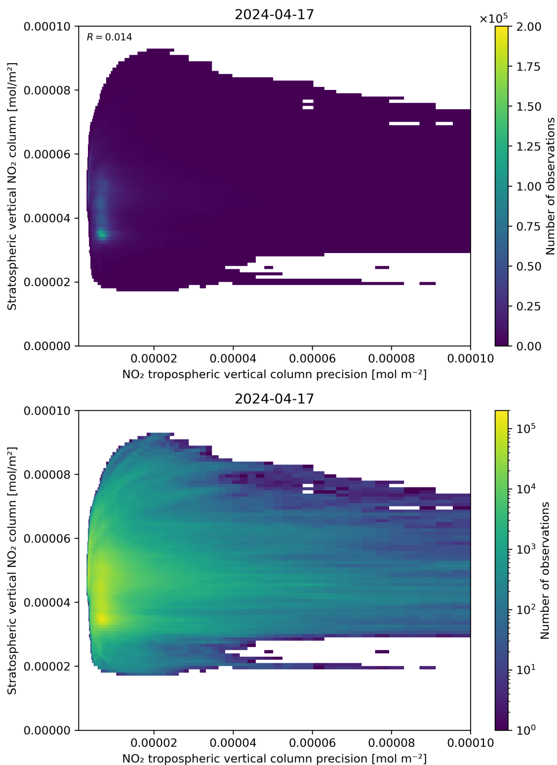
Figure 135: Scatter density plot of “NO 2 tropospheric vertical column precision” against “Stratospheric vertical NO 2 column” for 2024-04-16 to 2024-04-18.
