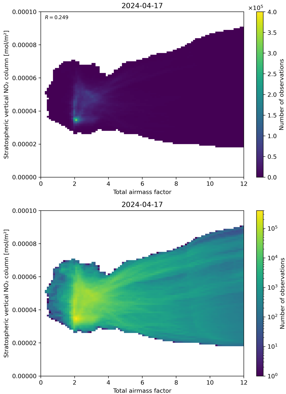
Figure 64: Scatter density plot of “Total airmass factor” against “Stratospheric vertical NO 2 column” for 2024-04-16 to 2024-04-18.
