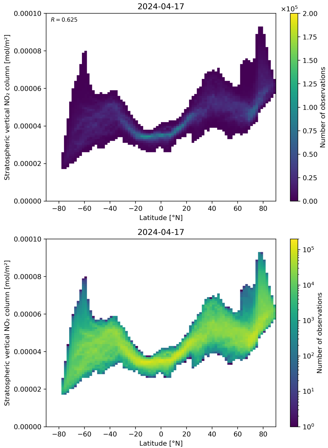
Figure 87: Scatter density plot of “Latitude” against “Stratospheric vertical NO 2 column” for 2024-04-16 to 2024-04-18.
