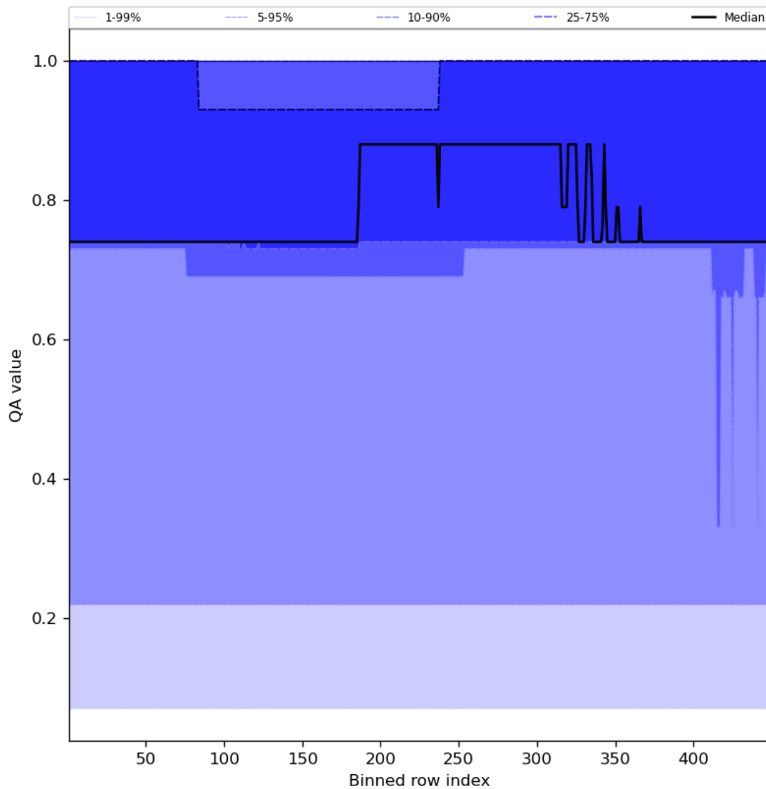
Figure 45: Along track statistics of “QA value” for 2024-04-16 to 2024-04-18
