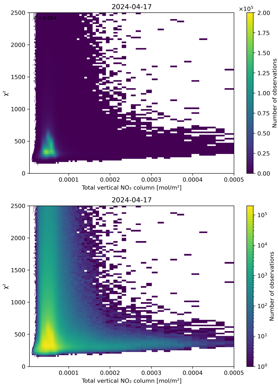
Figure 111: Scatter density plot of “Total vertical NO 2 column” against “ \chi^2 ” for 2024-04-16 to 2024-04-18.
