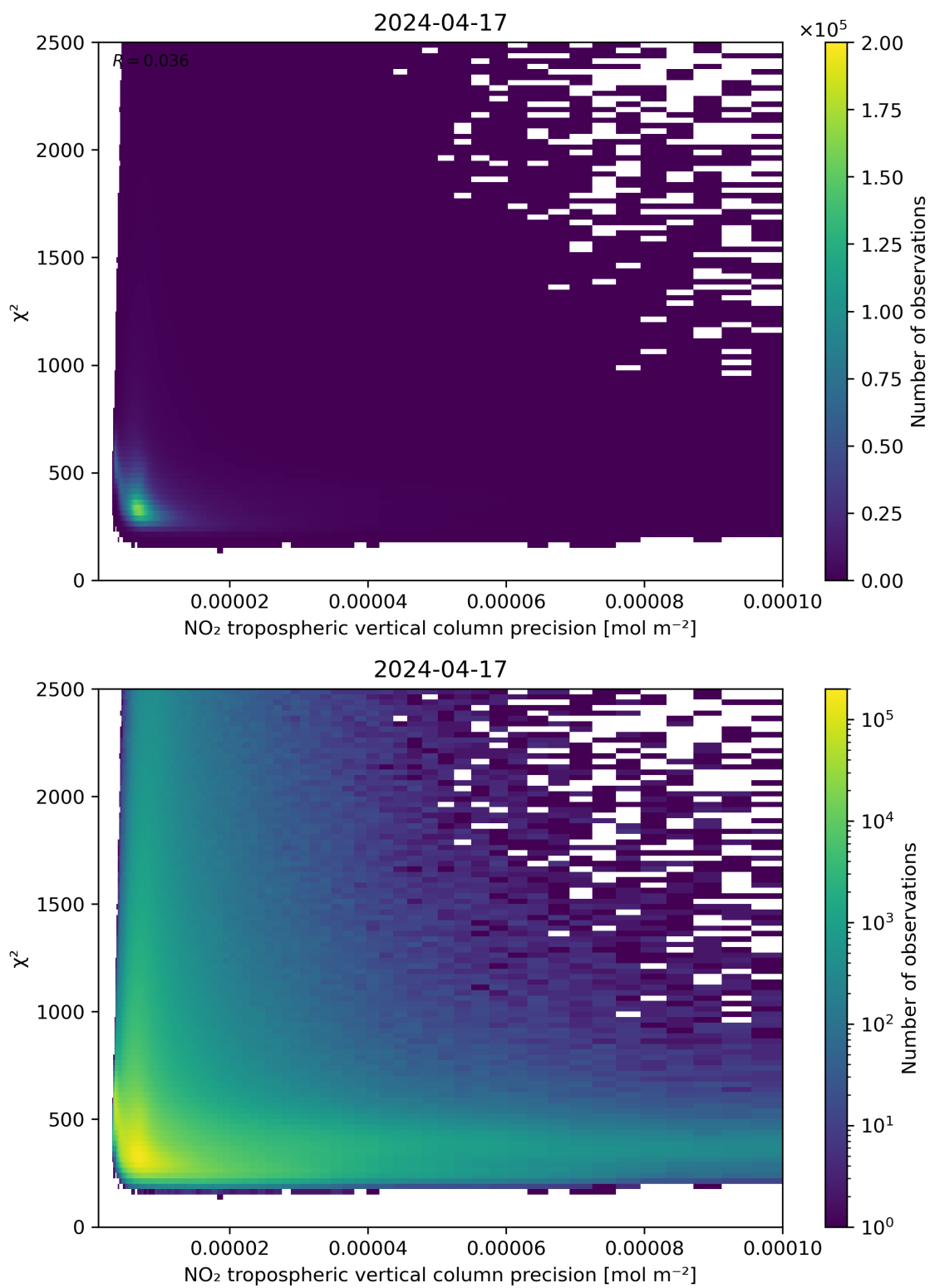
Figure 134: Scatter density plot of “NO 2 tropospheric vertical column precision” against “ \chi^2 ” for 2024-04-16 to 2024-04-18.
