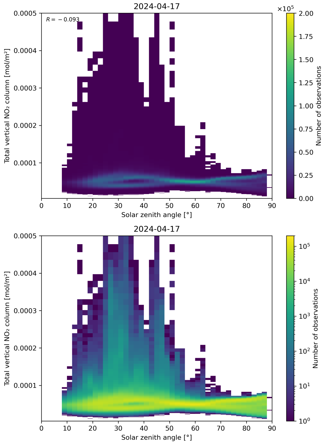
Figure 153: Scatter density plot of “Solar zenith angle” against “Total vertical NO 2 column” for 2024-04-16 to 2024-04-18.
