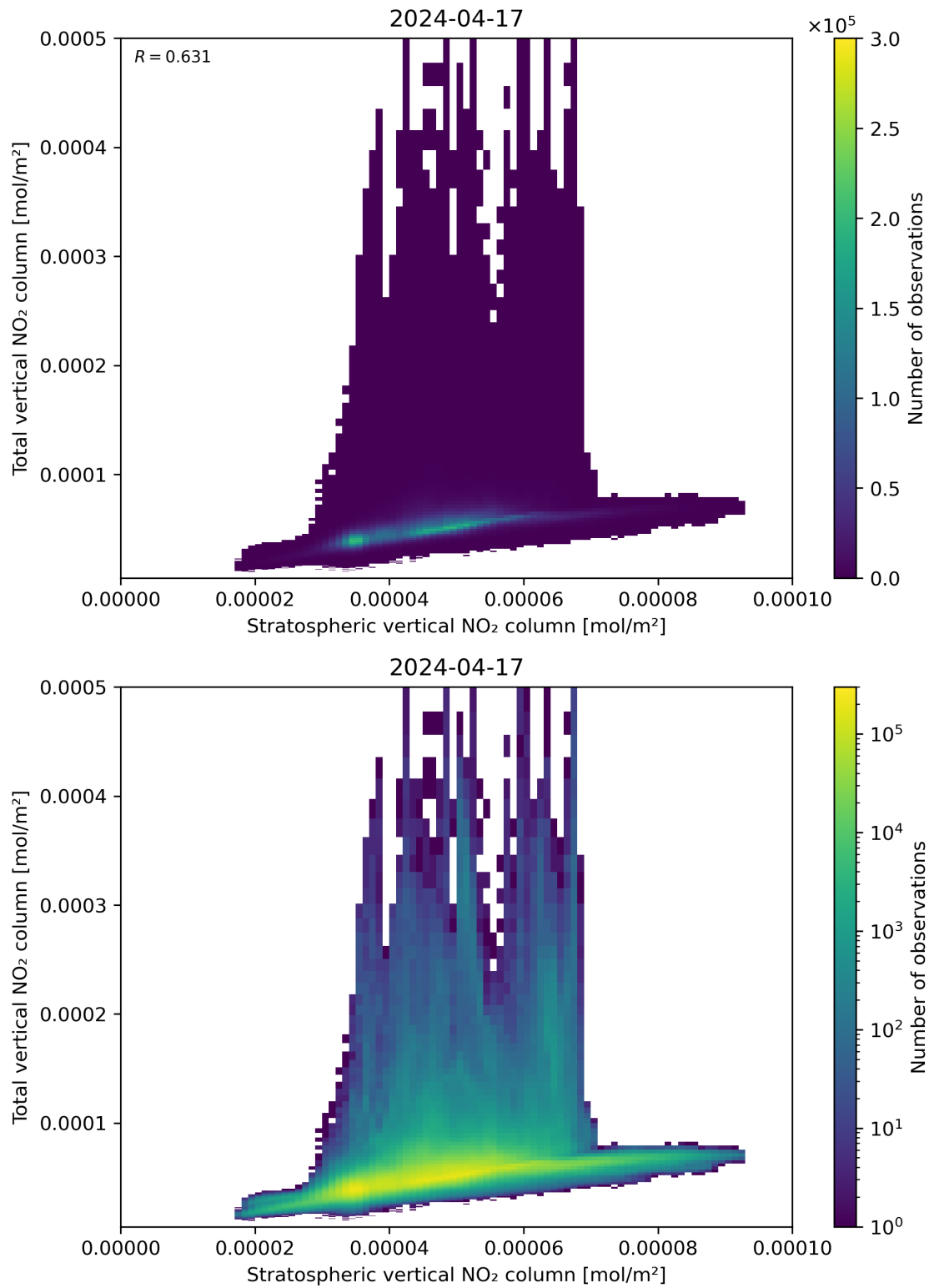
Figure 100: Scatter density plot of “Stratospheric vertical NO 2 column” against “Total vertical NO 2 column” for 2024-04-16 to 2024-04-18.
