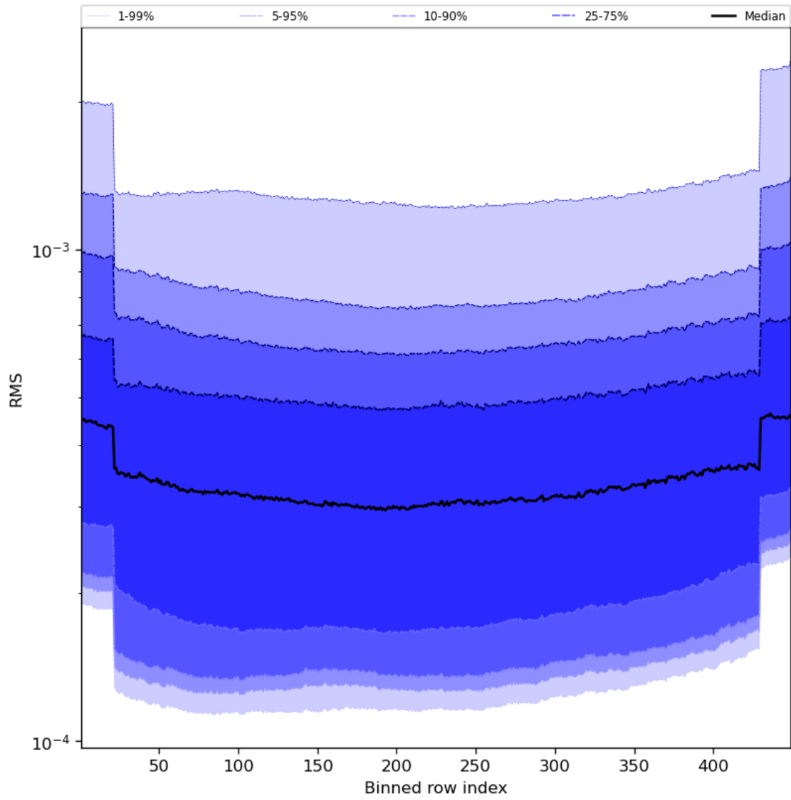
Figure 60: Along track statistics of “RMS” for 2024-04-16 to 2024-04-18
