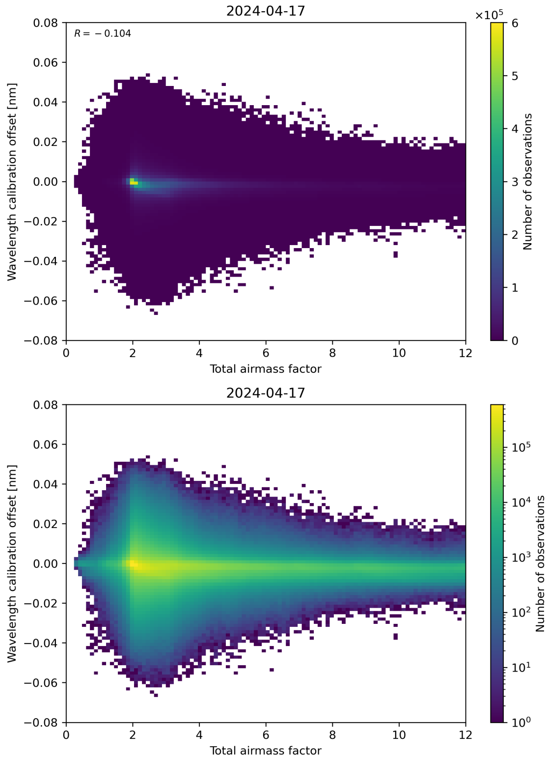
Figure 70: Scatter density plot of “Total airmass factor” against “Wavelength calibration offset” for 2024-04-16 to 2024-04-18.
