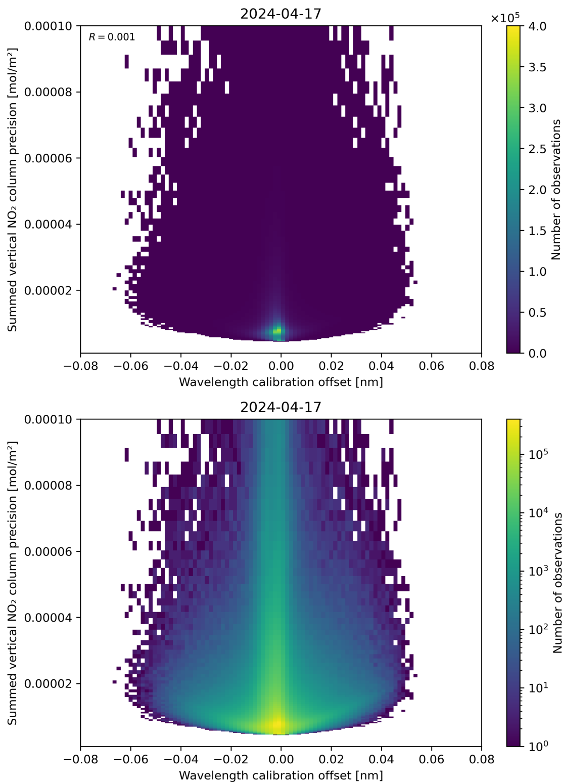
Figure 178: Scatter density plot of “Wavelength calibration offset” against “Summed vertical NO 2 column precision” for 2024-04-16 to 2024-04-18.
