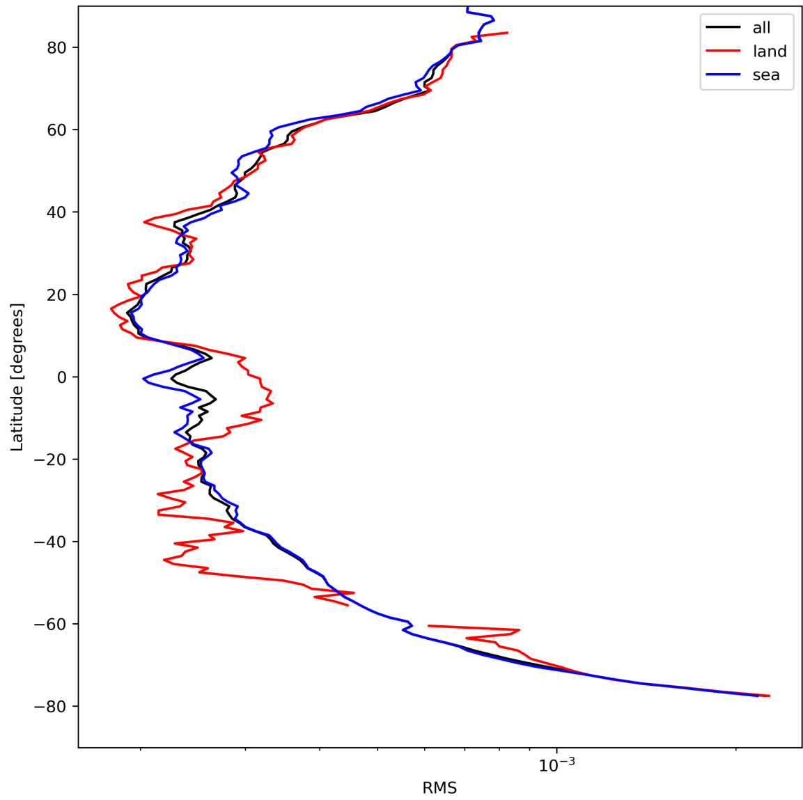
Figure 26: Zonal average of “RMS” for 2024-04-16 to 2024-04-18.
