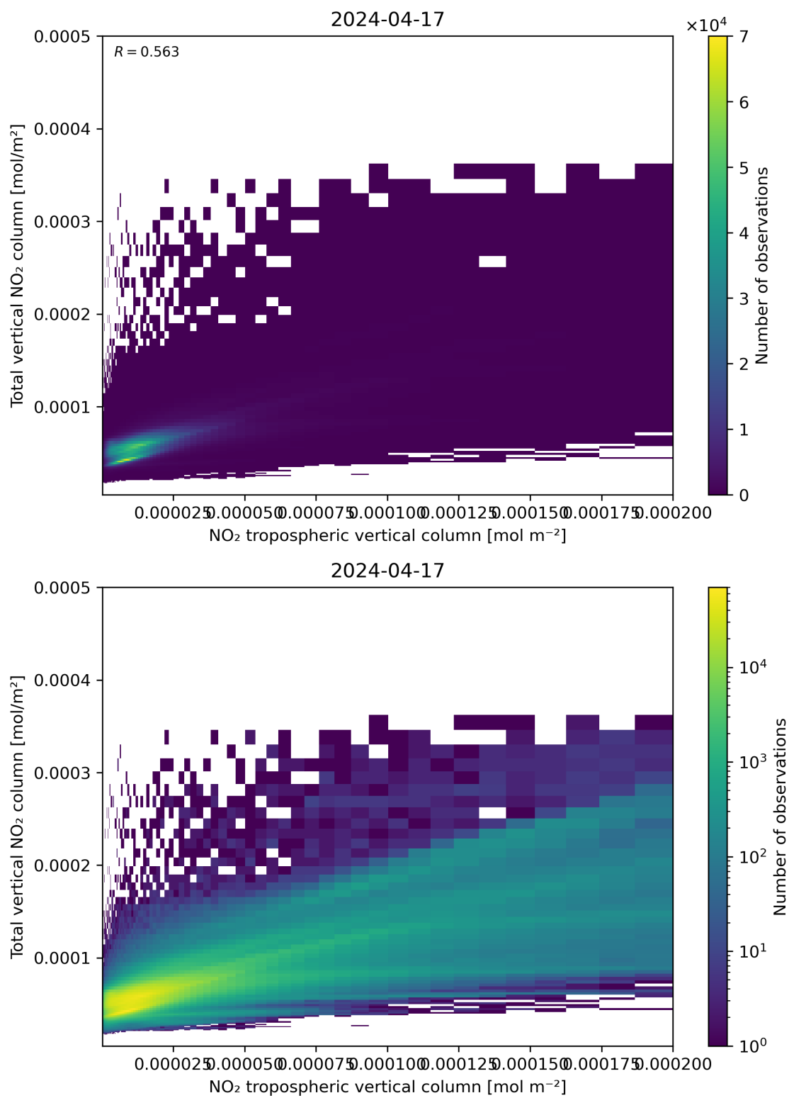
Figure 128: Scatter density plot of “NO 2 tropospheric vertical column” against “Total vertical NO 2 column” for 2024-04-16 to 2024-04-18.
