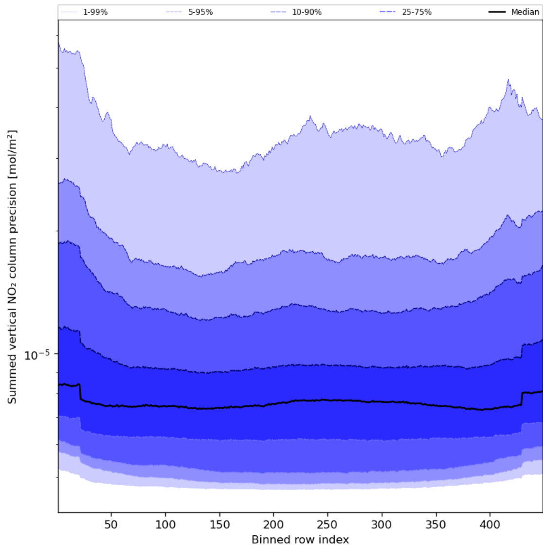
Figure 58: Along track statistics of “Summed vertical NO 2 column precision” for 2024-04-16 to 2024-04-18
