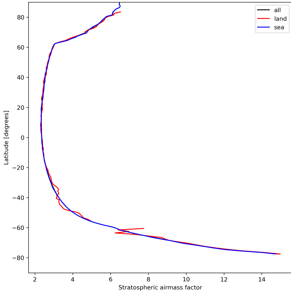
Figure 27: Zonal average of “Stratospheric airmass factor” for 2024-04-16 to 2024-04-18.
