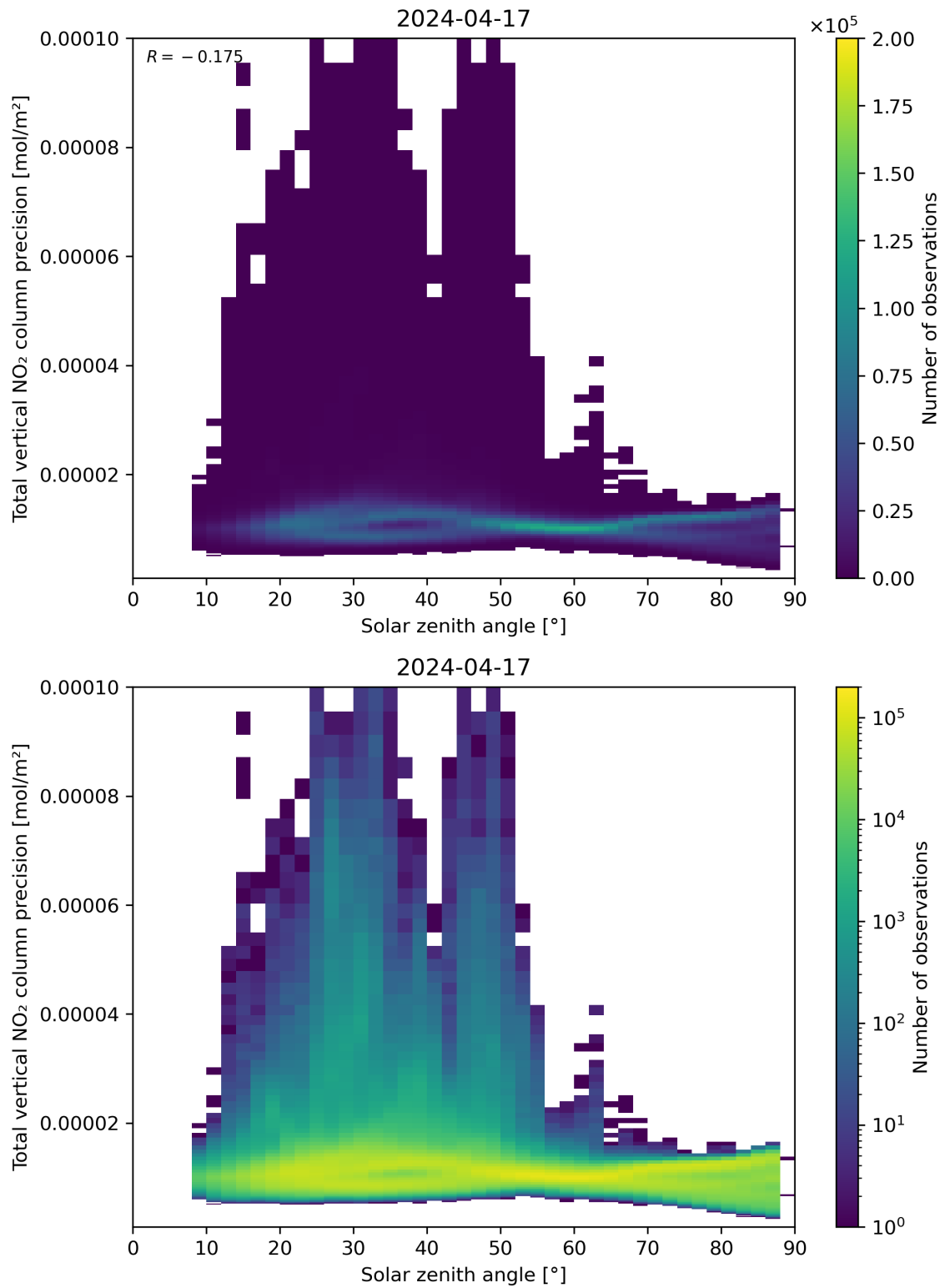
Figure 154: Scatter density plot of “Solar zenith angle” against “Total vertical NO 2 column precision” for 2024-04-16 to 2024-04-18.
