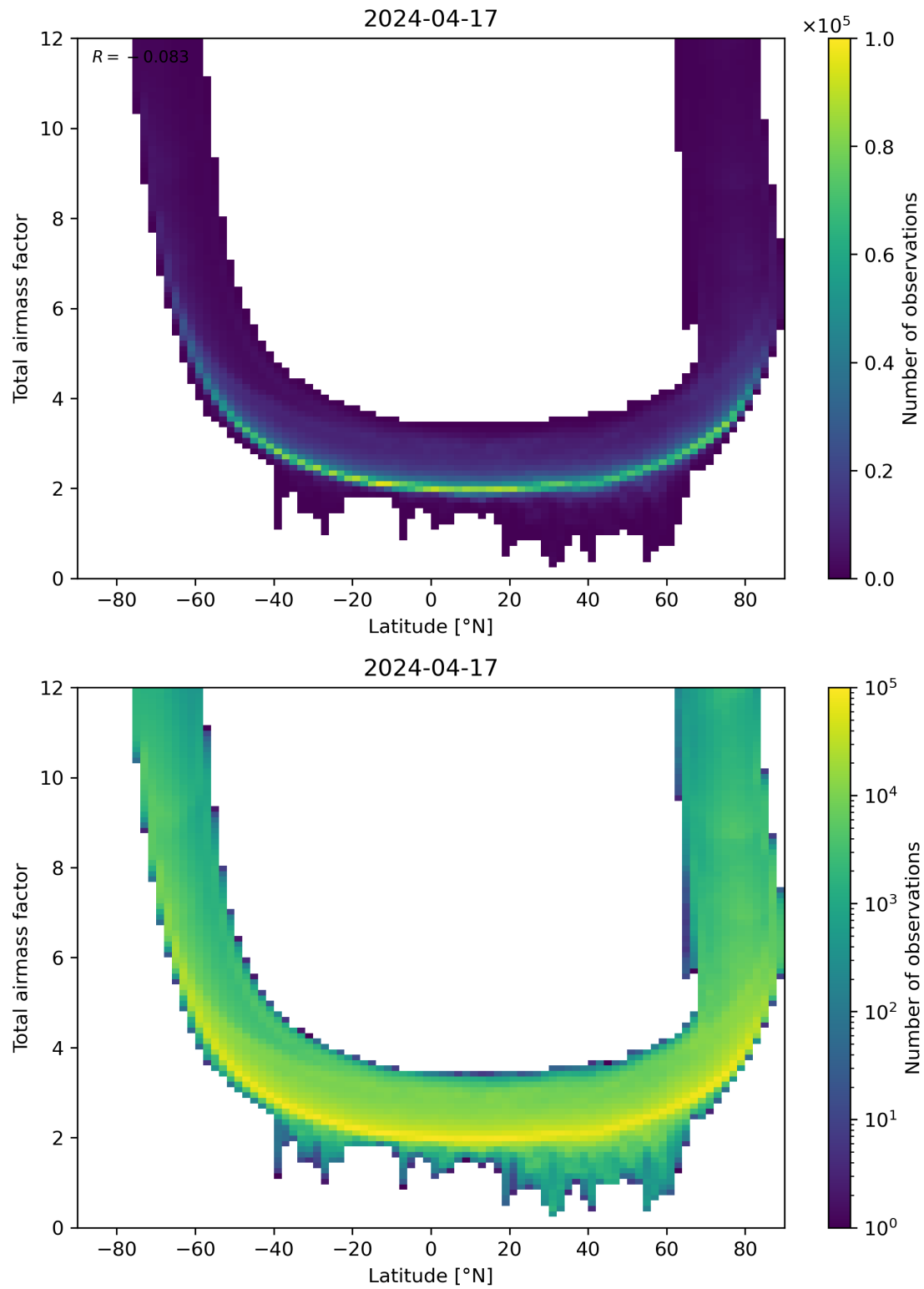
Figure 84: Scatter density plot of “Latitude” against “Total airmass factor” for 2024-04-16 to 2024-04-18.
