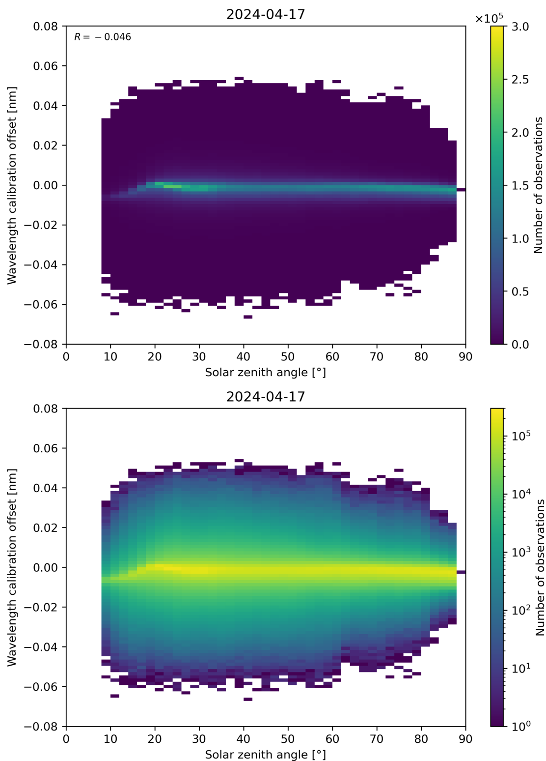
Figure 158: Scatter density plot of “Solar zenith angle” against “Wavelength calibration offset” for 2024-04-16 to 2024-04-18.
