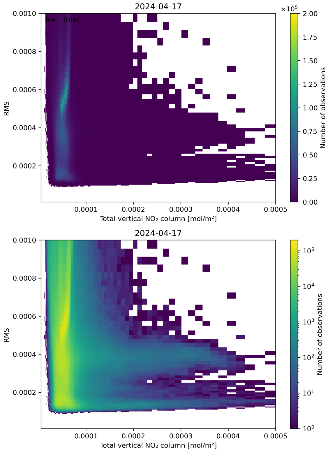
Figure 120: Scatter density plot of “Total vertical NO 2 column” against “RMS” for 2024-04-16 to 2024-04-18.
