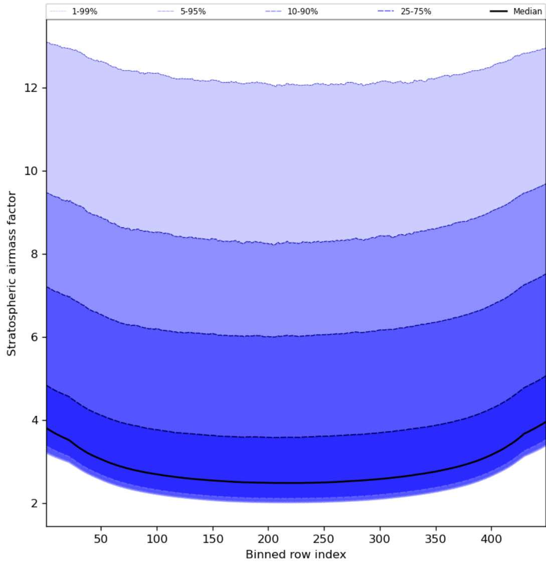
Figure 61: Along track statistics of “Stratospheric airmass factor” for 2024-04-16 to 2024-04-18
