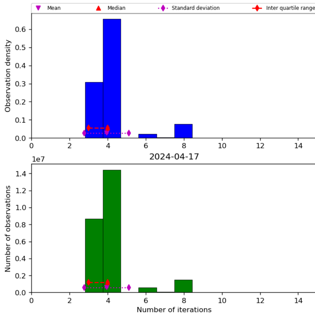
Figure 34: Histogram of “Number of iterations” for 2024-04-16 to 2024-04-18
