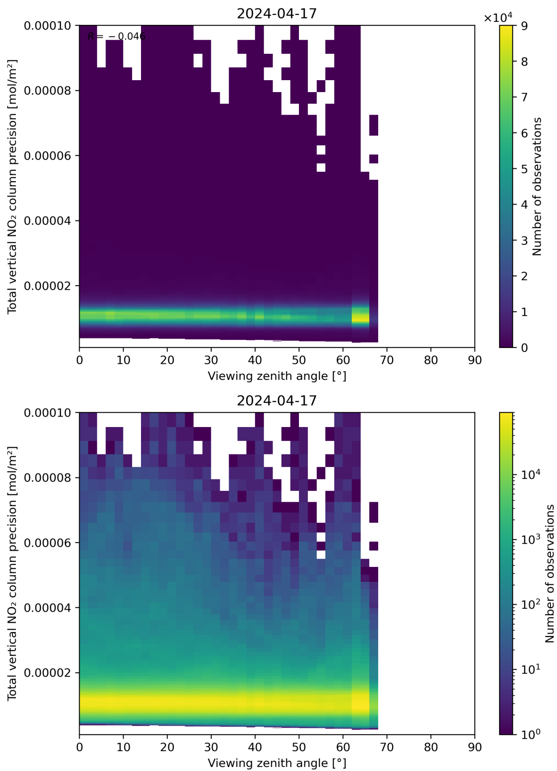
Figure 168: Scatter density plot of “Viewing zenith angle” against “Total vertical NO 2 column precision” for 2024-04-16 to 2024-04-18.
