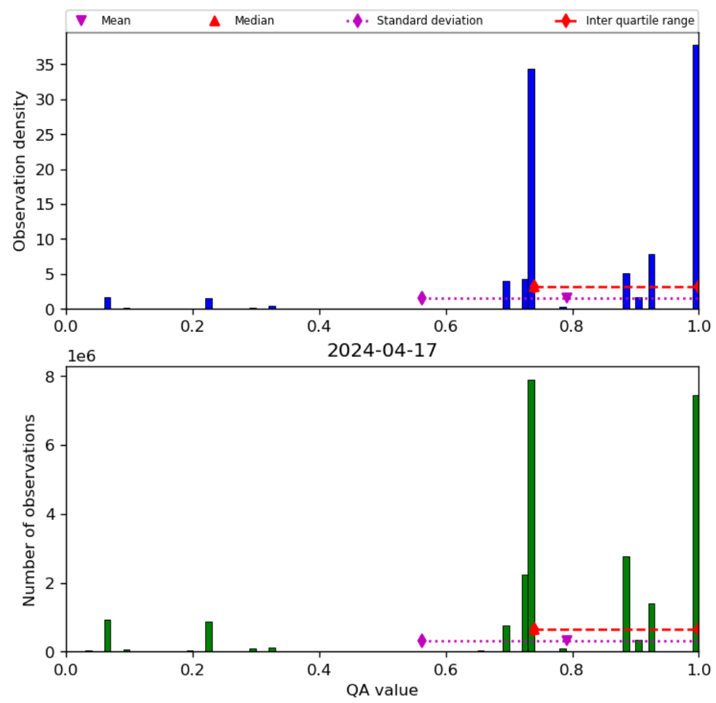
Figure 28: Histogram of “QA value” for 2024-04-16 to 2024-04-18
