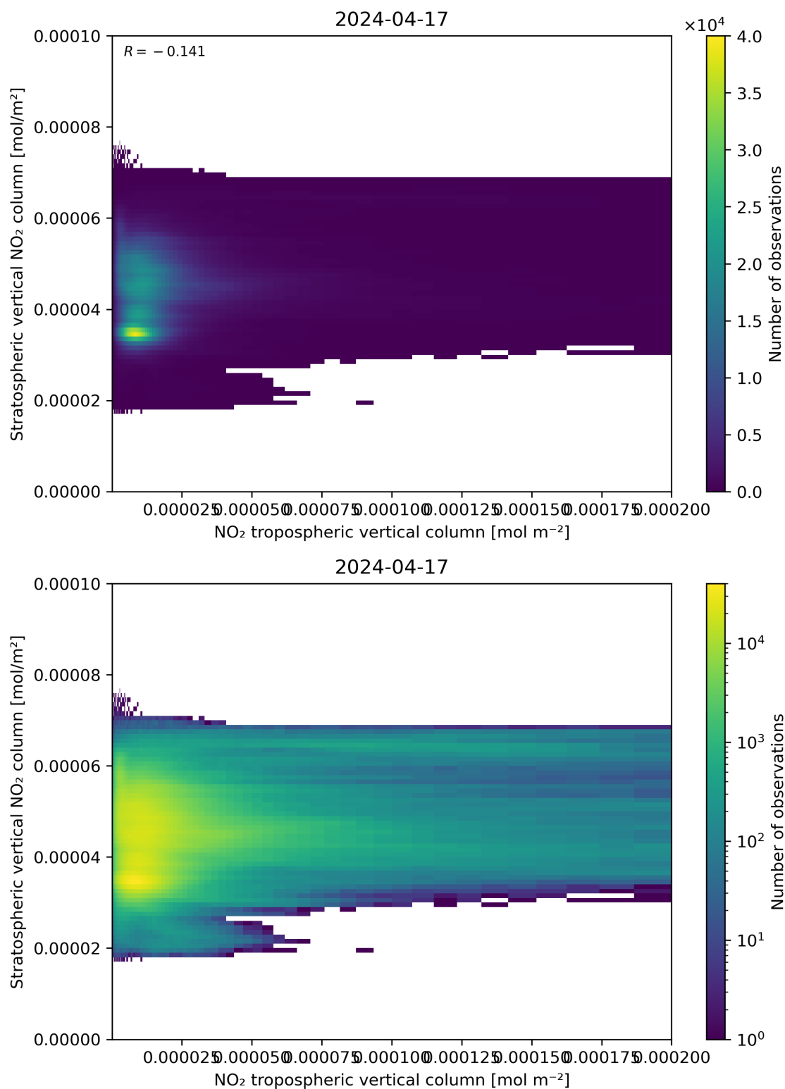
Figure 125: Scatter density plot of “NO 2 tropospheric vertical column” against “Stratospheric vertical NO 2 column” for 2024-04-16 to 2024-04-18.
