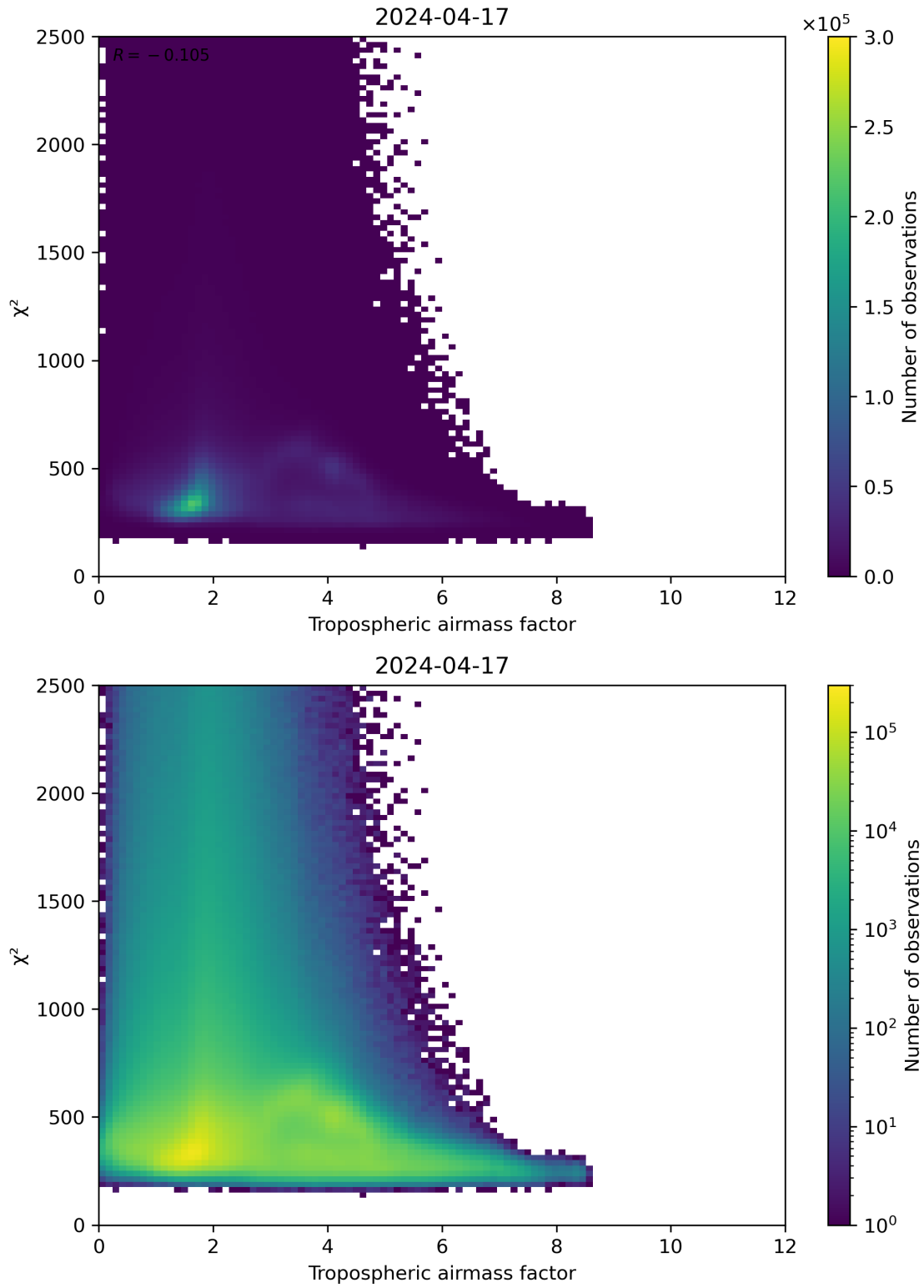
Figure 73: Scatter density plot of “Tropospheric airmass factor” against “ \chi^2 ” for 2024-04-16 to 2024-04-18.
