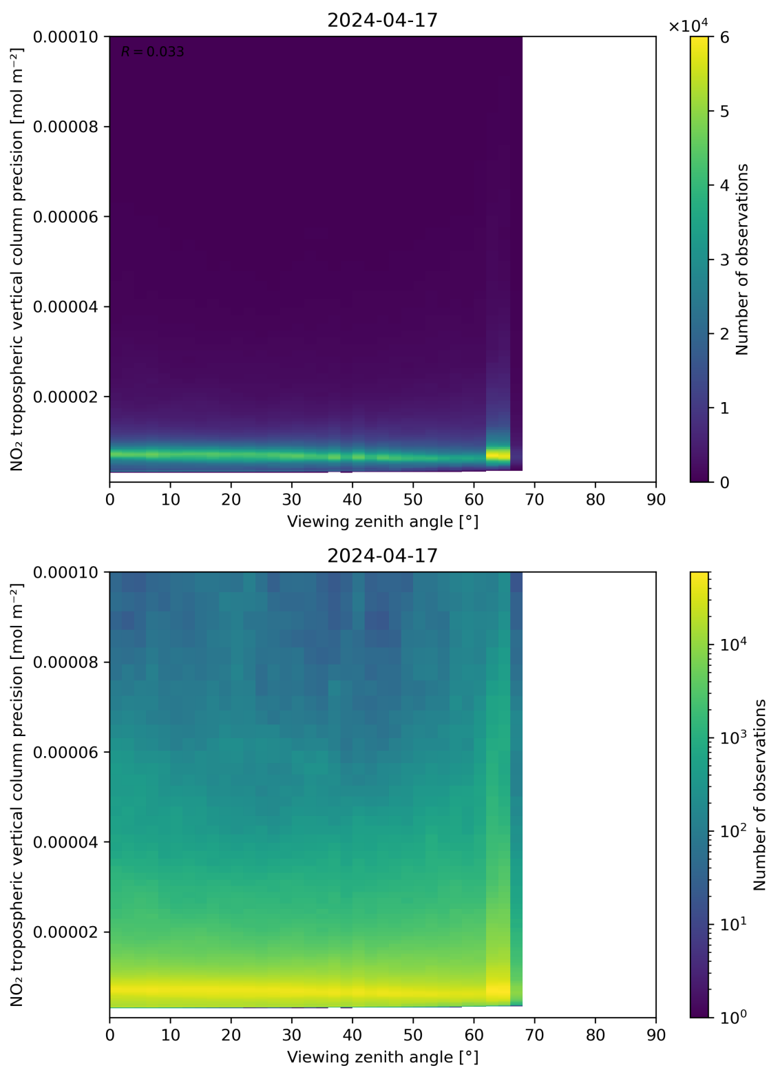
Figure 170: Scatter density plot of “Viewing zenith angle” against “NO 2 tropospheric vertical column precision” for 2024-04-16 to 2024-04-18.
