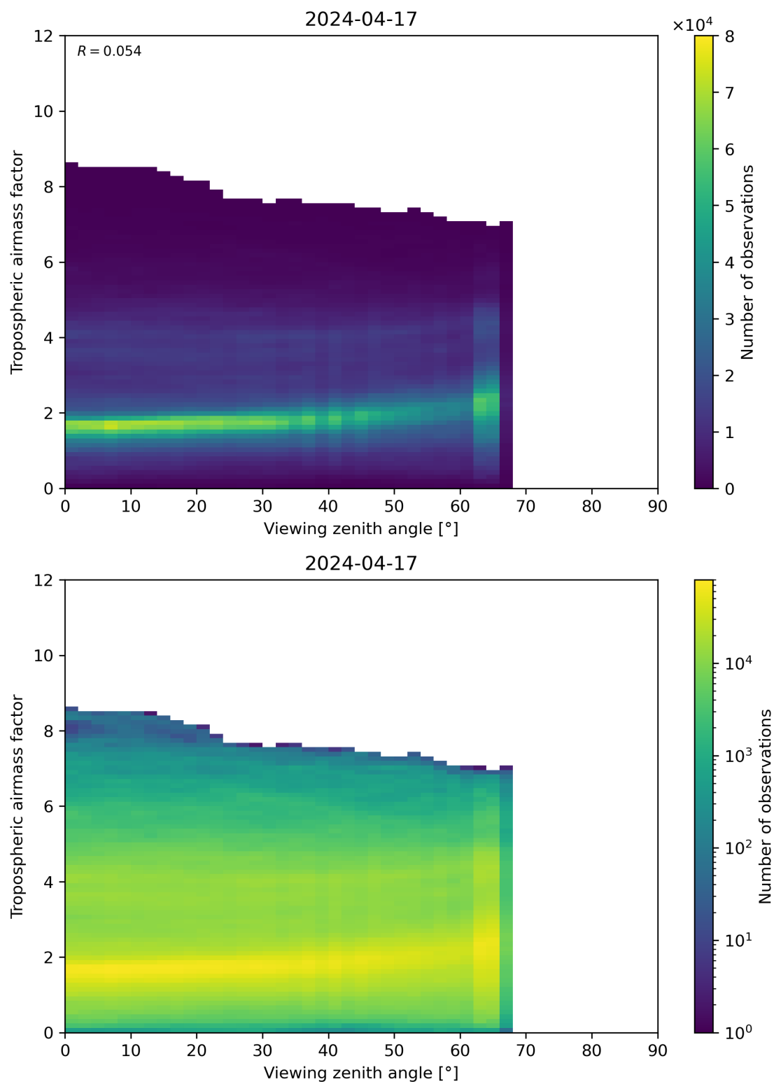
Figure 161: Scatter density plot of “Viewing zenith angle” against “Tropospheric airmass factor” for 2024-04-16 to 2024-04-18.
