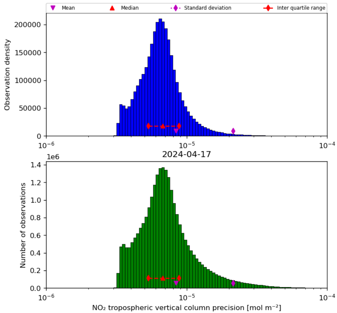
Figure 30: Histogram of “NO 2 tropospheric vertical column precision” for 2024-04-16 to 2024-04-18
