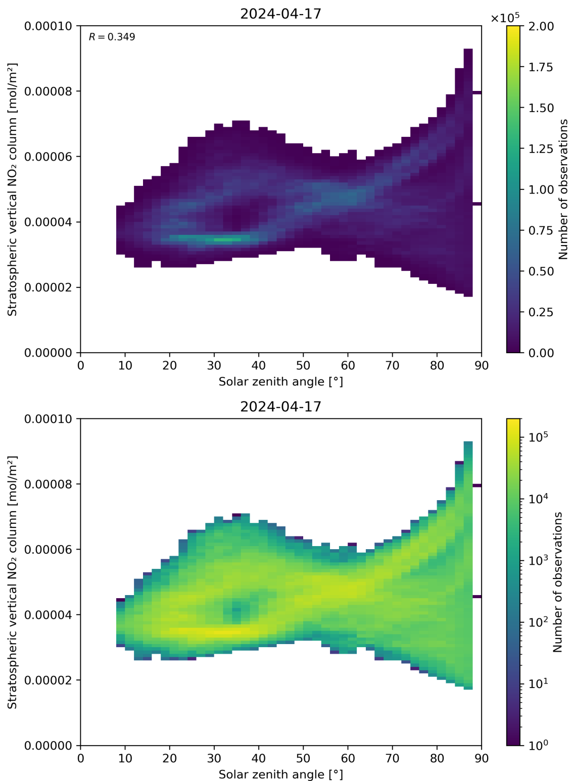
Figure 150: Scatter density plot of “Solar zenith angle” against “Stratospheric vertical NO 2 column” for 2024-04-16 to 2024-04-18.
