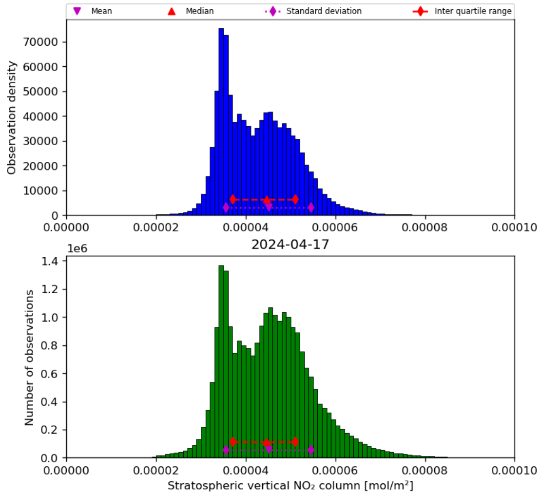
Figure 36: Histogram of “Stratospheric vertical NO 2 column” for 2024-04-16 to 2024-04-18
