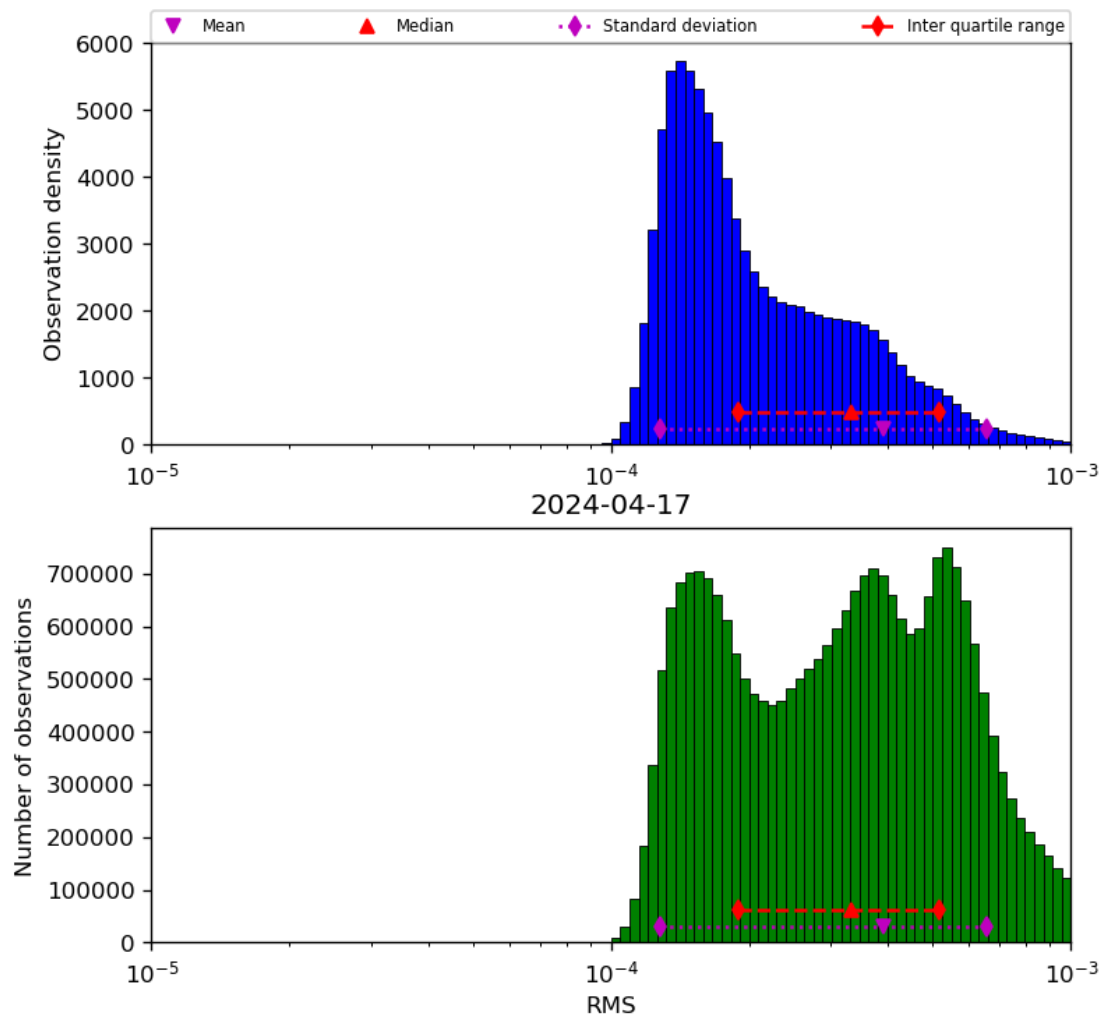
Figure 43: Histogram of “RMS” for 2024-04-16 to 2024-04-18
