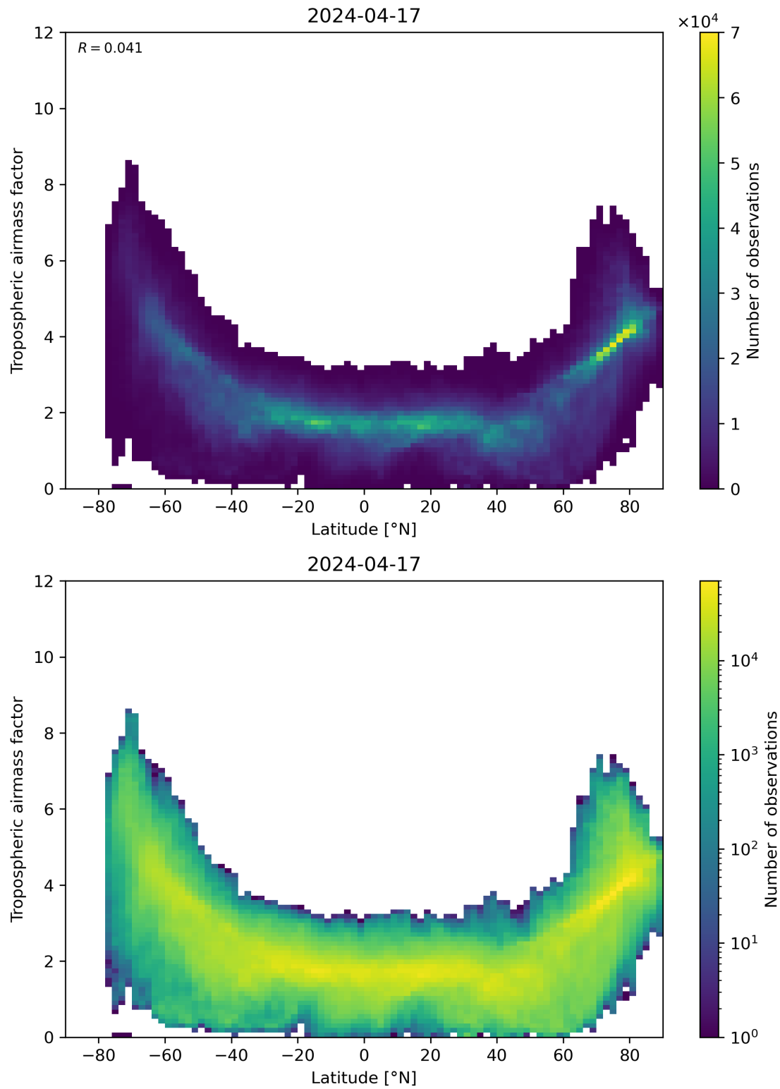
Figure 85: Scatter density plot of “Latitude” against “Tropospheric airmass factor” for 2024-04-16 to 2024-04-18.
