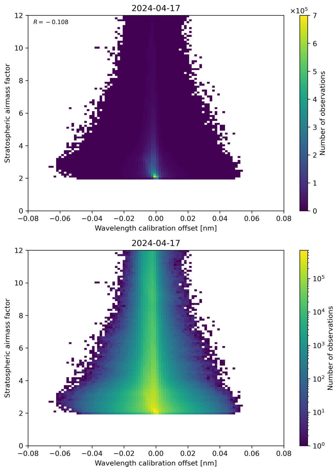
Figure 174: Scatter density plot of “Wavelength calibration offset” against “Stratospheric airmass factor” for 2024-04-16 to 2024-04-18.
