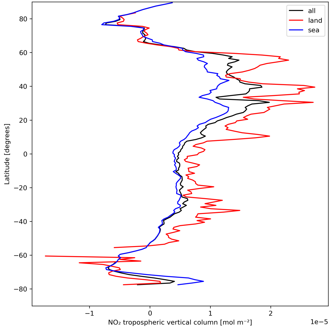
Figure 12: Zonal average of “NO 2 tropospheric vertical column” for 2024-04-16 to 2024-04-18.
