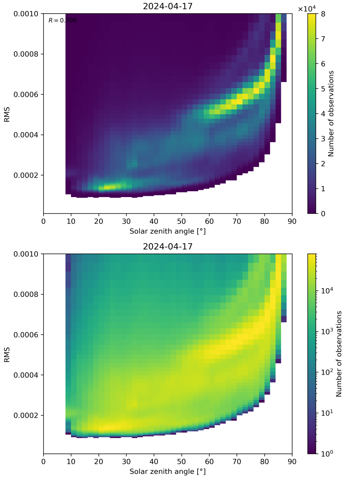
Figure 157: Scatter density plot of “Solar zenith angle” against “RMS” for 2024-04-16 to 2024-04-18.
