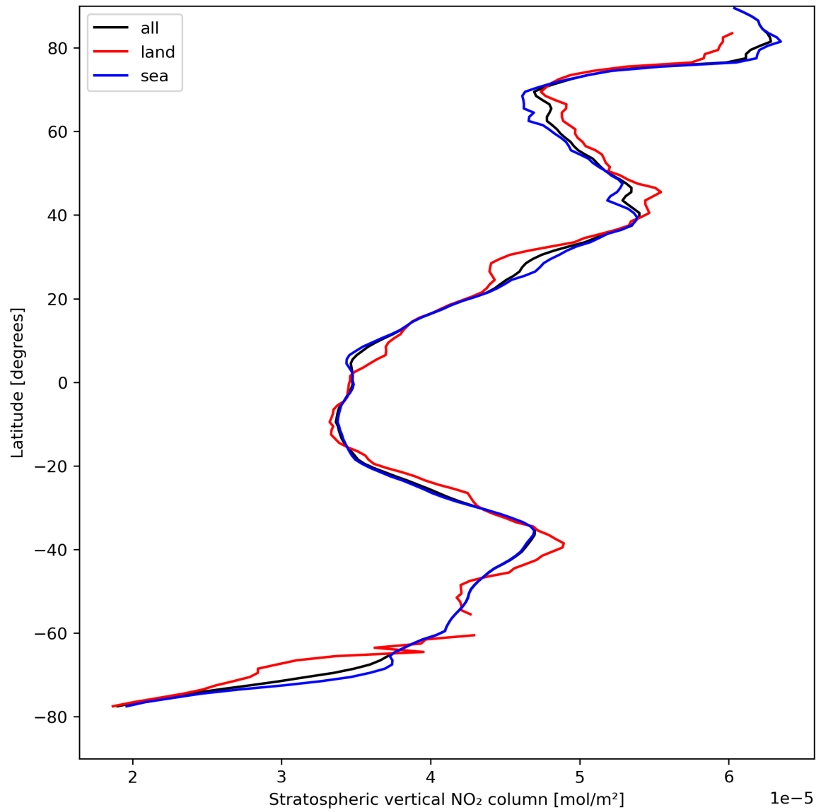
Figure 19: Zonal average of “Stratospheric vertical NO 2 column” for 2024-04-16 to 2024-04-18.
