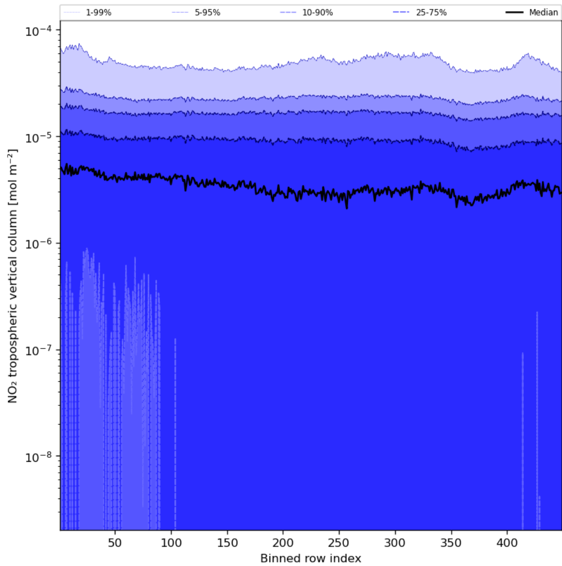
Figure 46: Along track statistics of “NO 2 tropospheric vertical column” for 2024-04-16 to 2024-04-18
