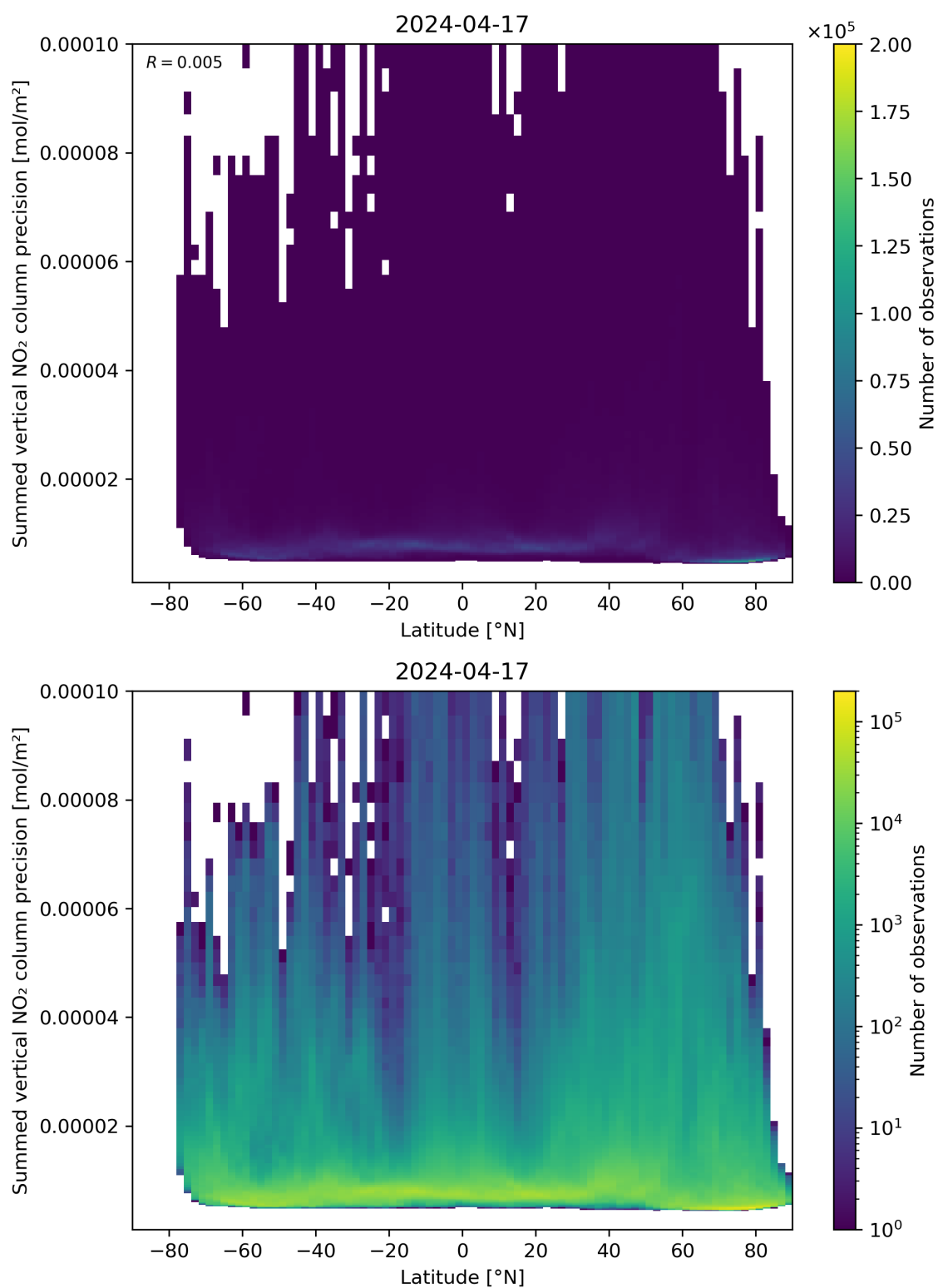
Figure 89: Scatter density plot of “Latitude” against “Summed vertical NO 2 column precision” for 2024-04-16 to 2024-04-18.
