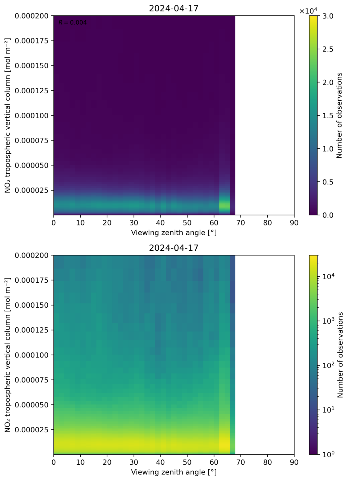
Figure 169: Scatter density plot of “Viewing zenith angle” against “NO 2 tropospheric vertical column” for 2024-04-16 to 2024-04-18.
