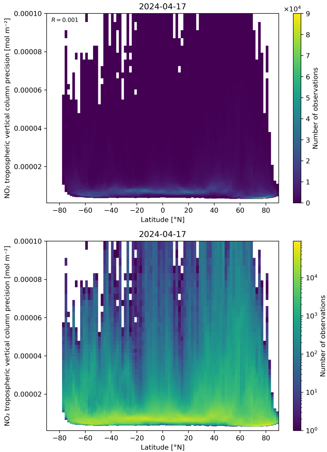
Figure 93: Scatter density plot of “Latitude” against “NO 2 tropospheric vertical column precision” for 2024-04-16 to 2024-04-18.
