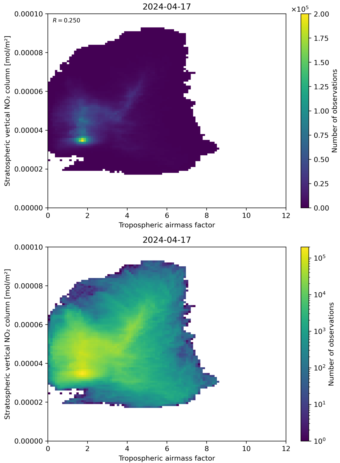
Figure 74: Scatter density plot of “Tropospheric airmass factor” against “Stratospheric vertical NO 2 column” for 2024-04-16 to 2024-04-18.
