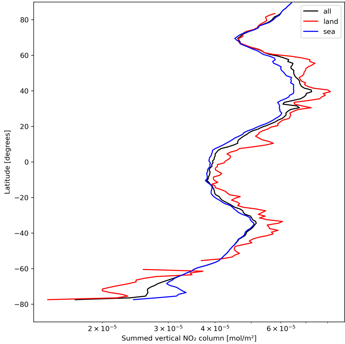
Figure 23: Zonal average of “Summed vertical NO 2 column” for 2024-04-16 to 2024-04-18.
