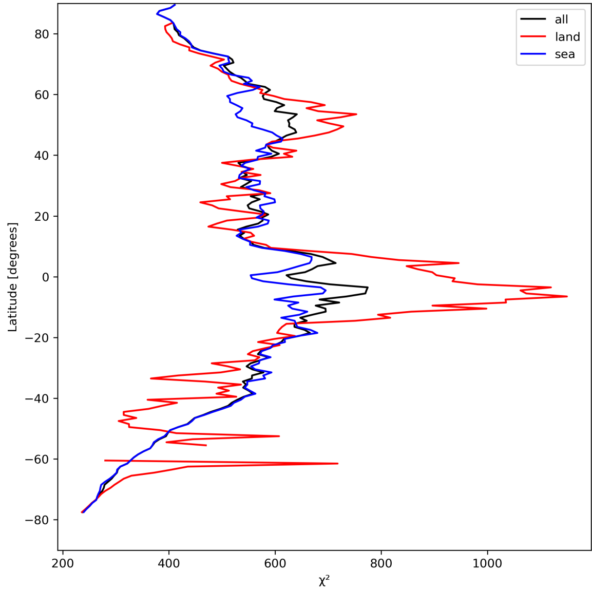
Figure 25: Zonal average of “ \chi^2 ” for 2024-04-16 to 2024-04-18.
