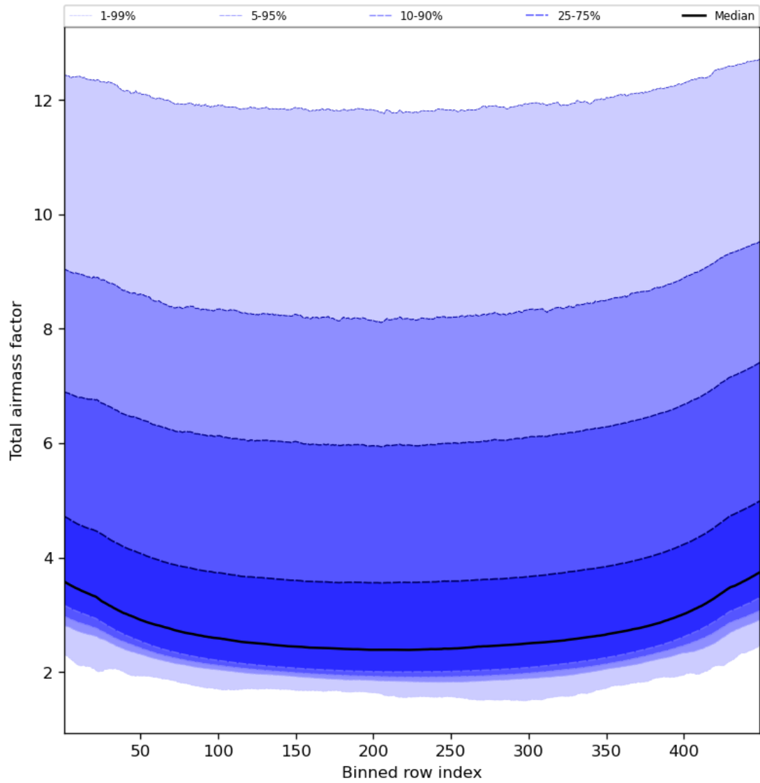
Figure 49: Along track statistics of “Total airmass factor” for 2024-04-16 to 2024-04-18
