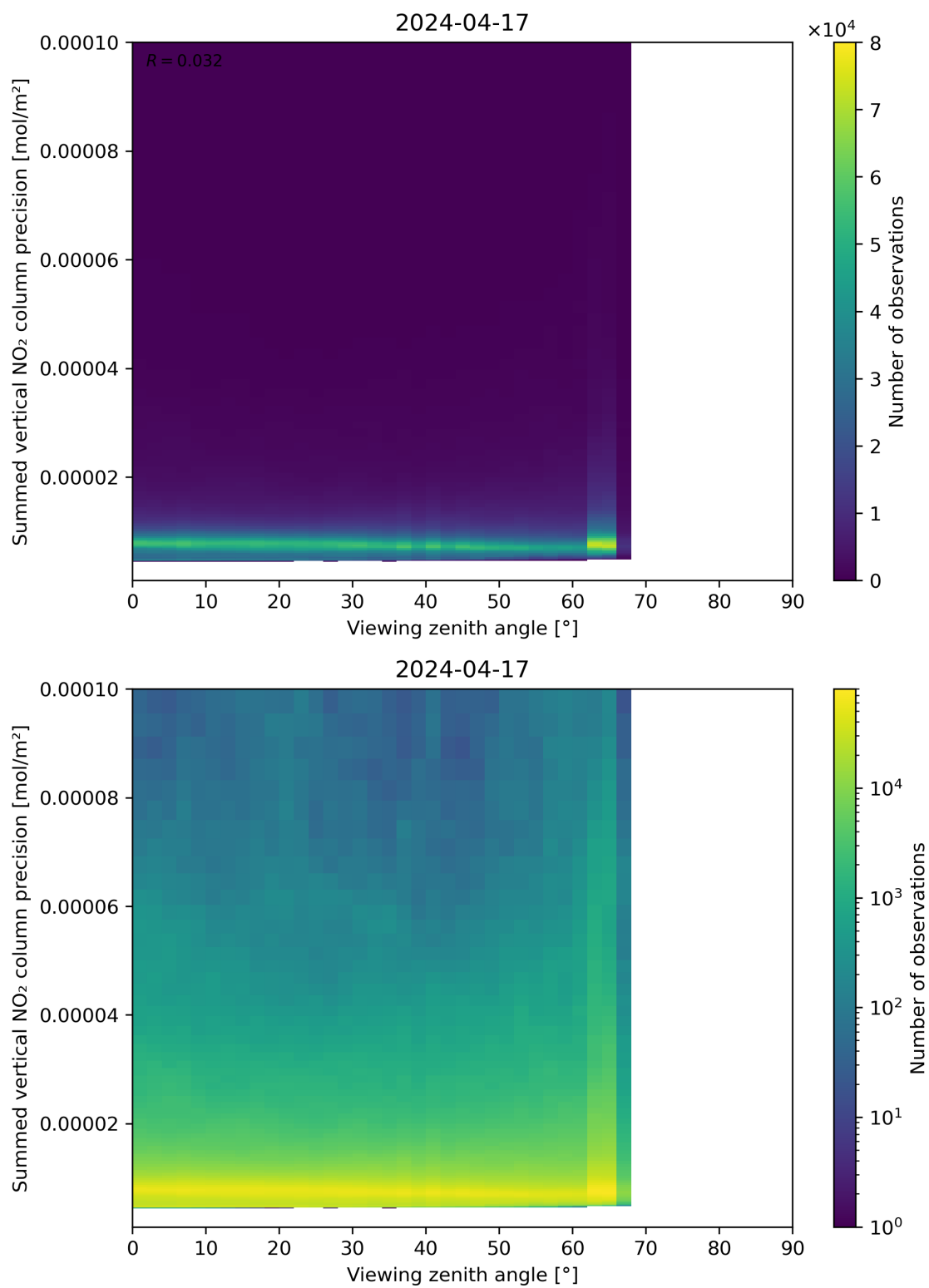
Figure 166: Scatter density plot of “Viewing zenith angle” against “Summed vertical NO 2 column precision” for 2024-04-16 to 2024-04-18.
