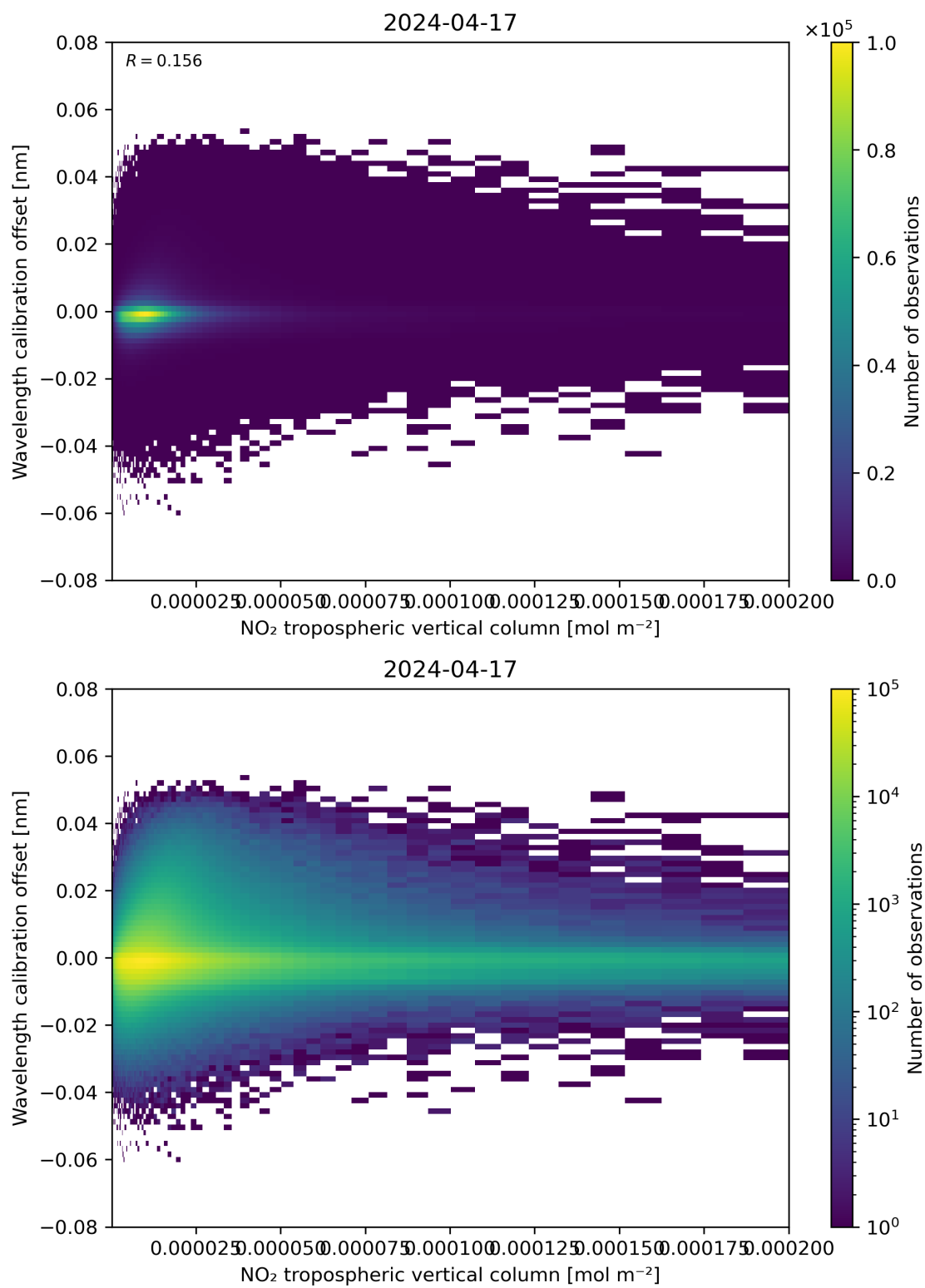
Figure 143: Scatter density plot of “NO 2 tropospheric vertical column” against “Wavelength calibration offset” for 2024-04-16 to 2024-04-18.
