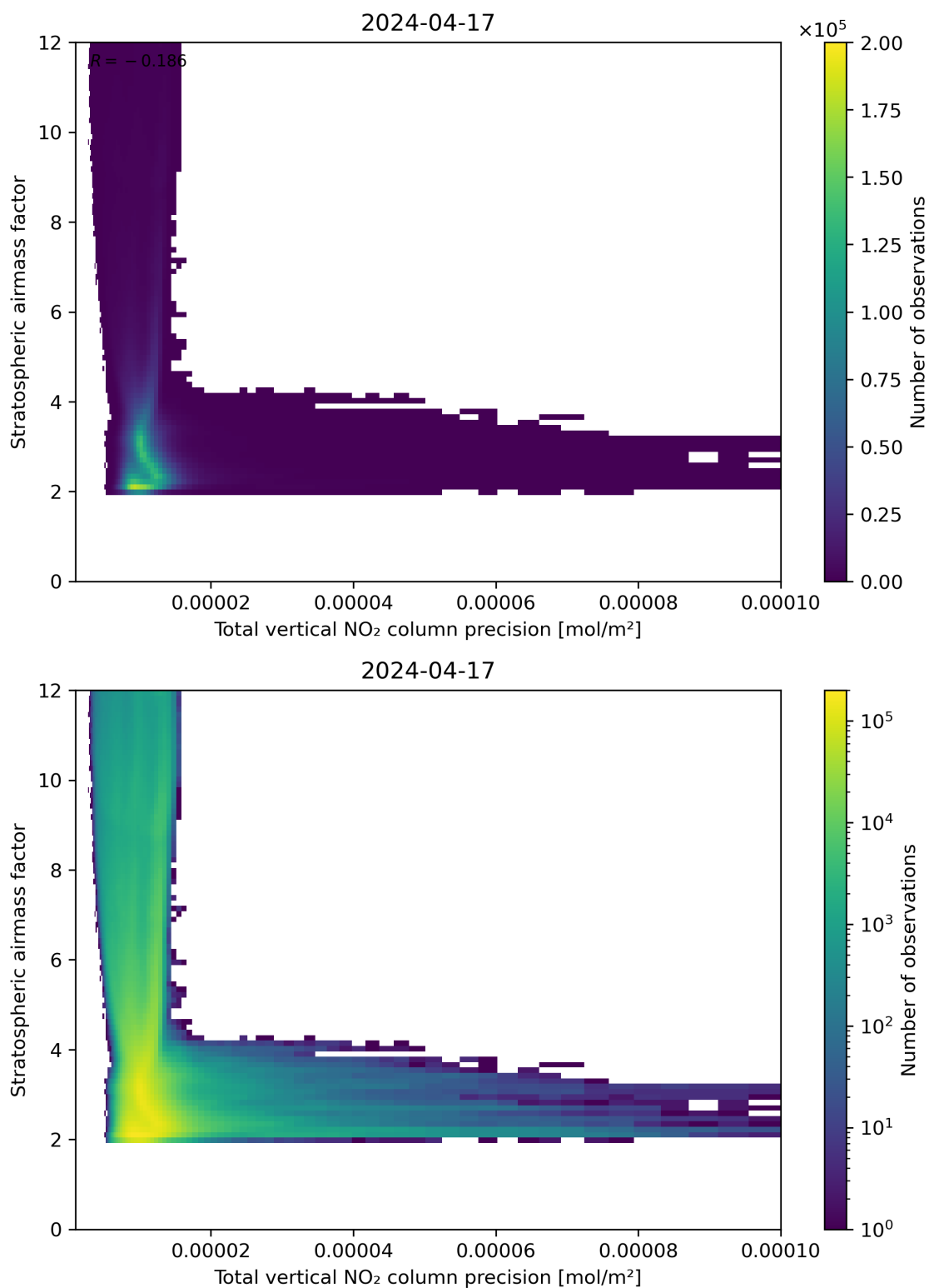
Figure 115: Scatter density plot of “Total vertical NO 2 column precision” against “Stratospheric airmass factor” for 2024-04-16 to 2024-04-18.
