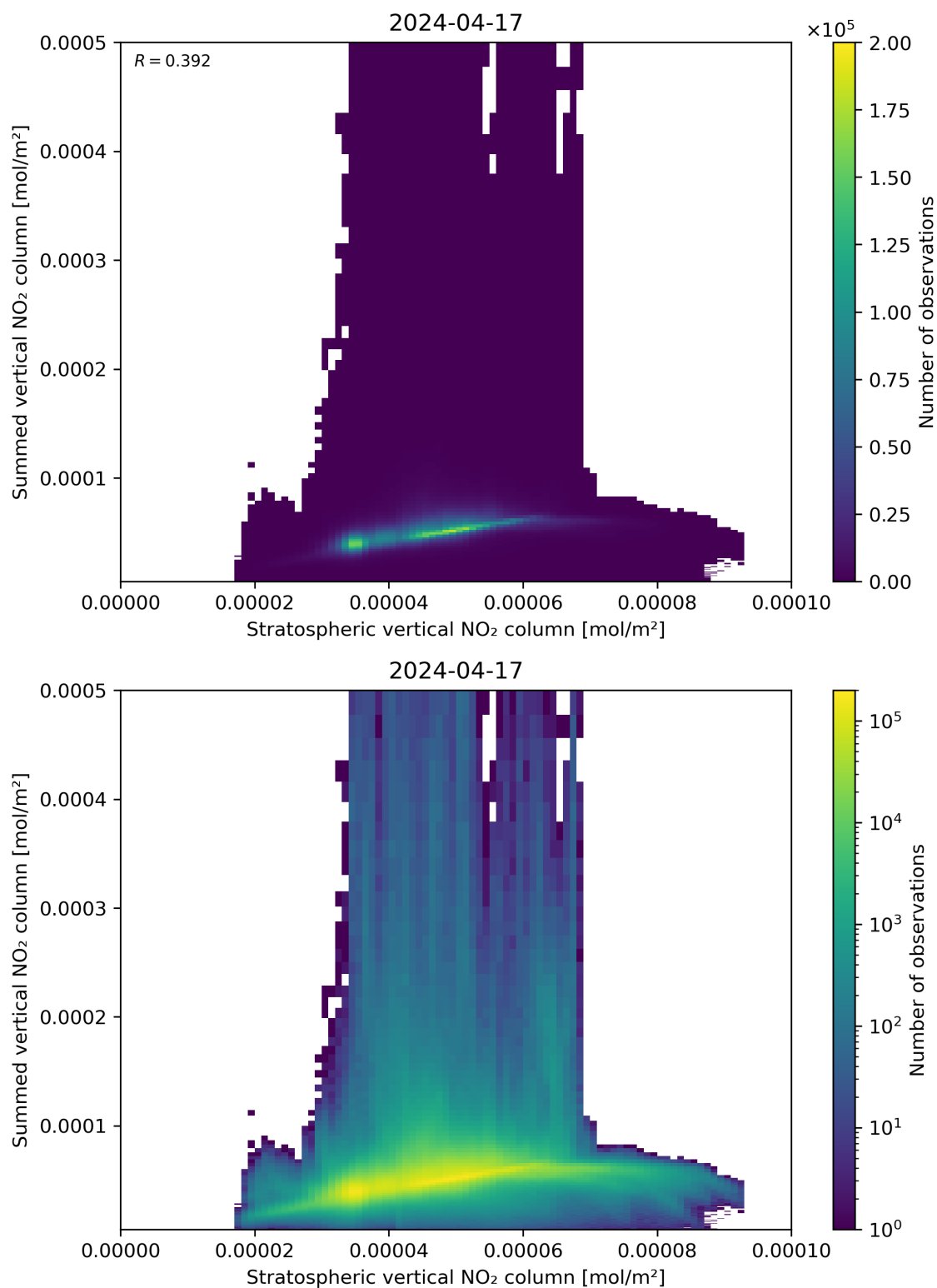
Figure 98: Scatter density plot of “Stratospheric vertical NO 2 column” against “Summed vertical NO 2 column” for 2024-04-16 to 2024-04-18.
