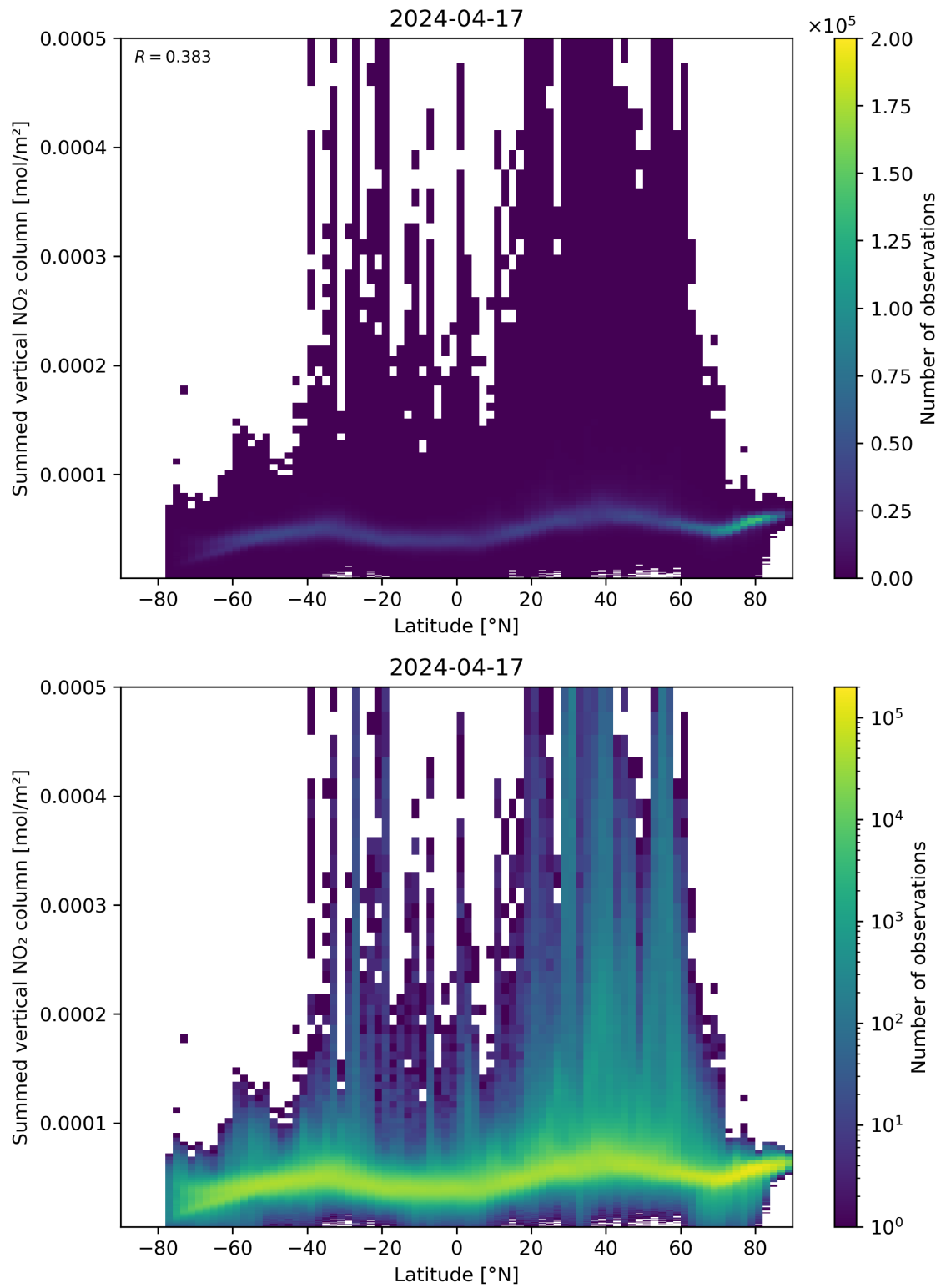
Figure 88: Scatter density plot of “Latitude” against “Summed vertical NO 2 column” for 2024-04-16 to 2024-04-18.
