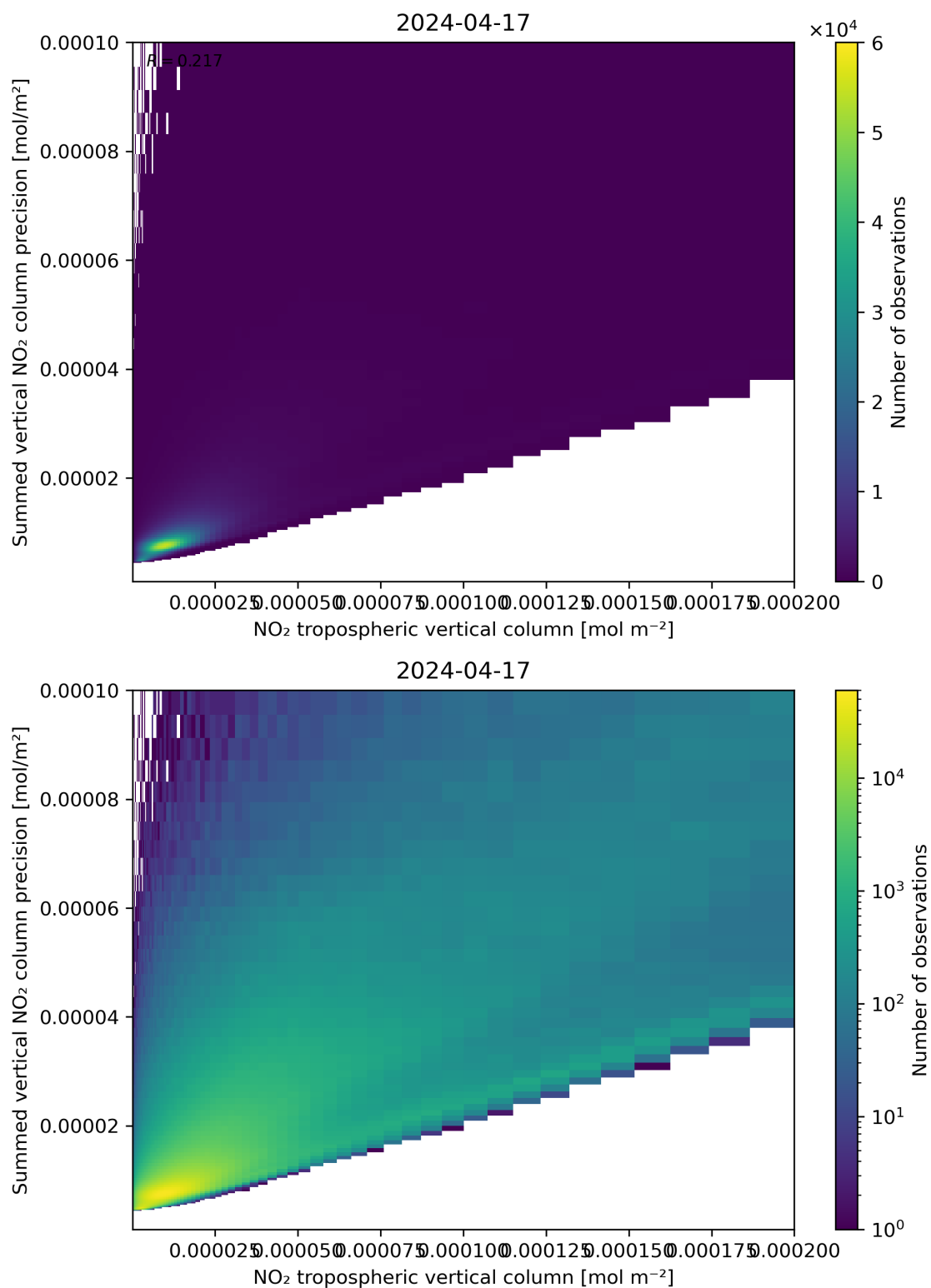
Figure 127: Scatter density plot of “NO 2 tropospheric vertical column” against “Summed vertical NO 2 column precision” for 2024-04-16 to 2024-04-18.
