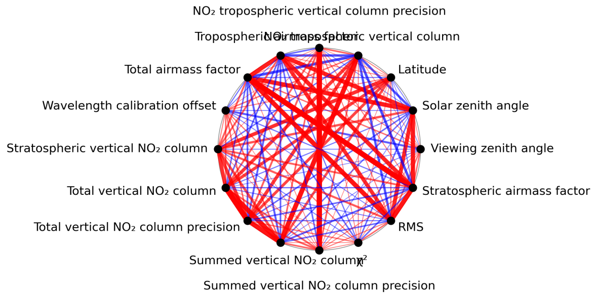
Figure 1: Map of correlation graph for 2024-04-16 to 2024-04-18.
