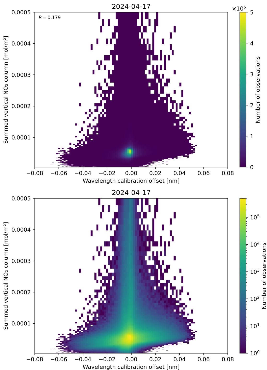
Figure 177: Scatter density plot of “Wavelength calibration offset” against “Summed vertical NO 2 column” for 2024-04-16 to 2024-04-18.
