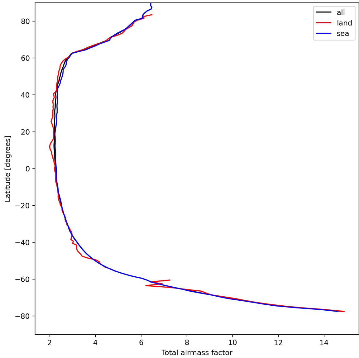
Figure 15: Zonal average of “Total airmass factor” for 2024-04-16 to 2024-04-18.
