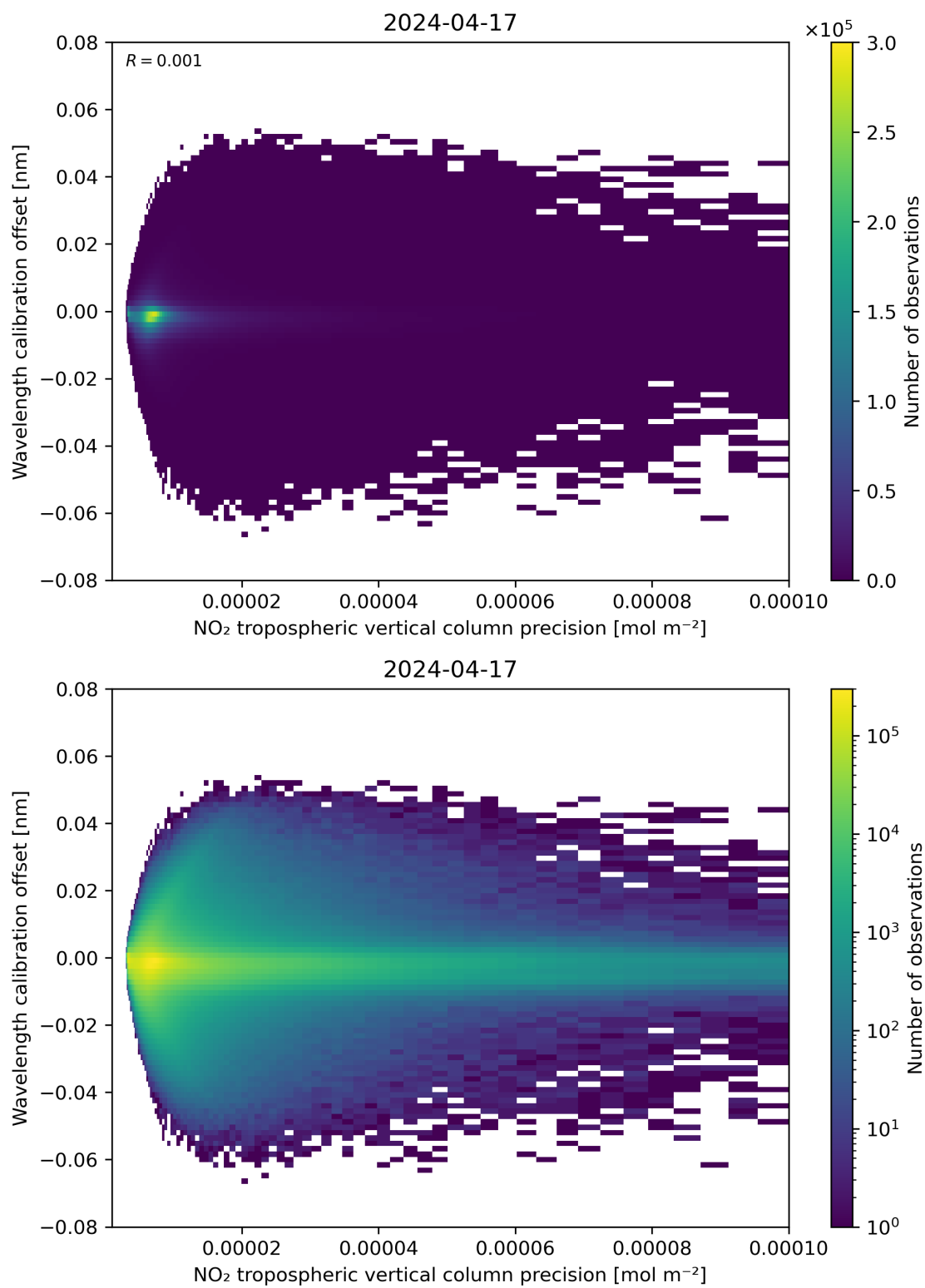
Figure 141: Scatter density plot of “NO 2 tropospheric vertical column precision” against “Wavelength calibration offset” for 2024-04-16 to 2024-04-18.
