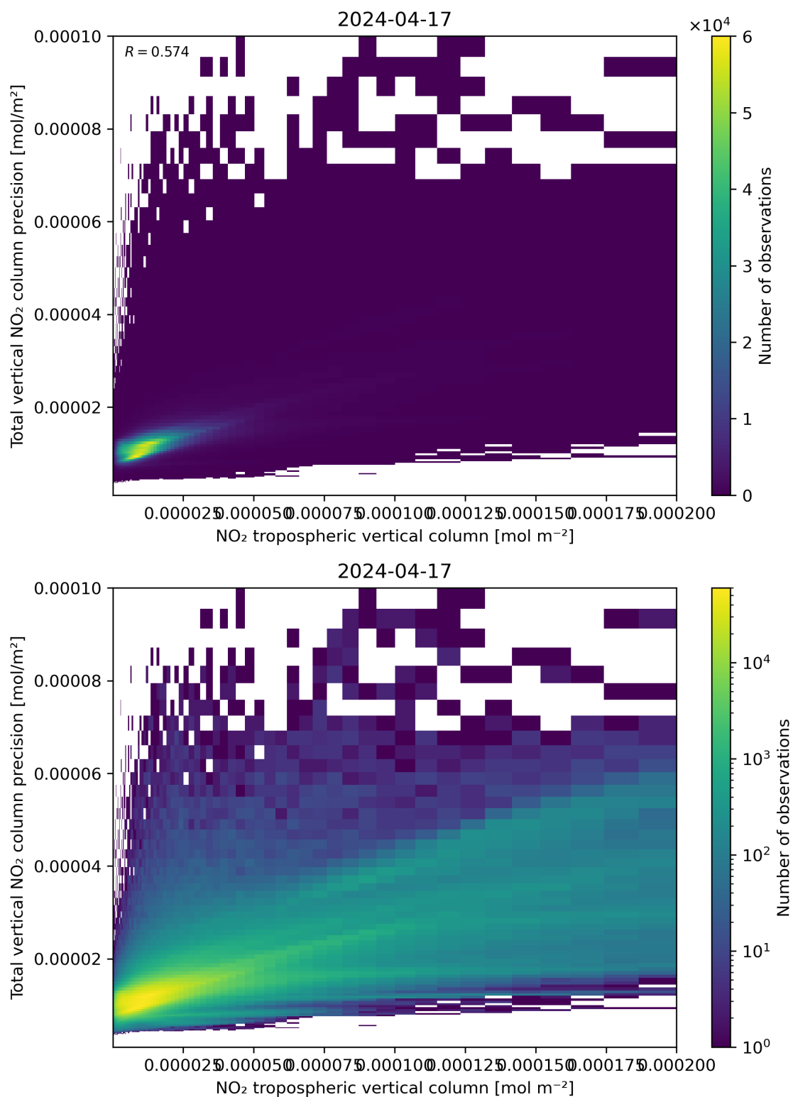
Figure 129: Scatter density plot of “NO 2 tropospheric vertical column” against “Total vertical NO 2 column precision” for 2024-04-16 to 2024-04-18.
