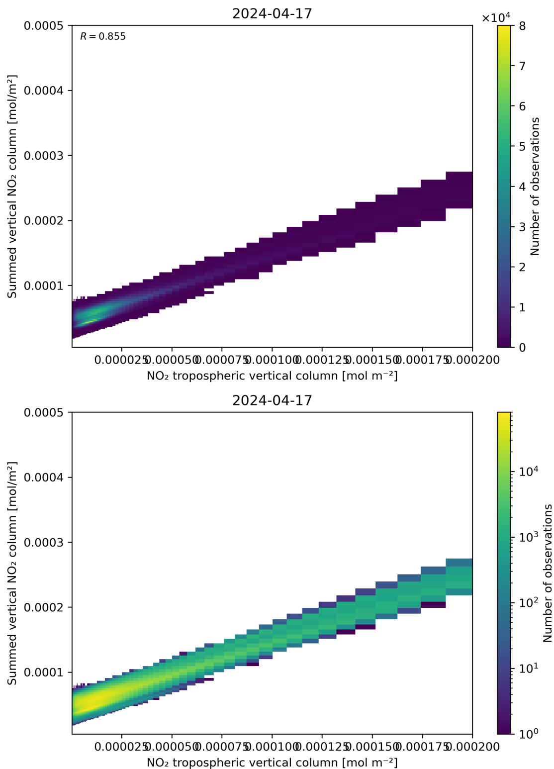
Figure 126: Scatter density plot of “NO 2 tropospheric vertical column” against “Summed vertical NO 2 column” for 2024-04-16 to 2024-04-18.
