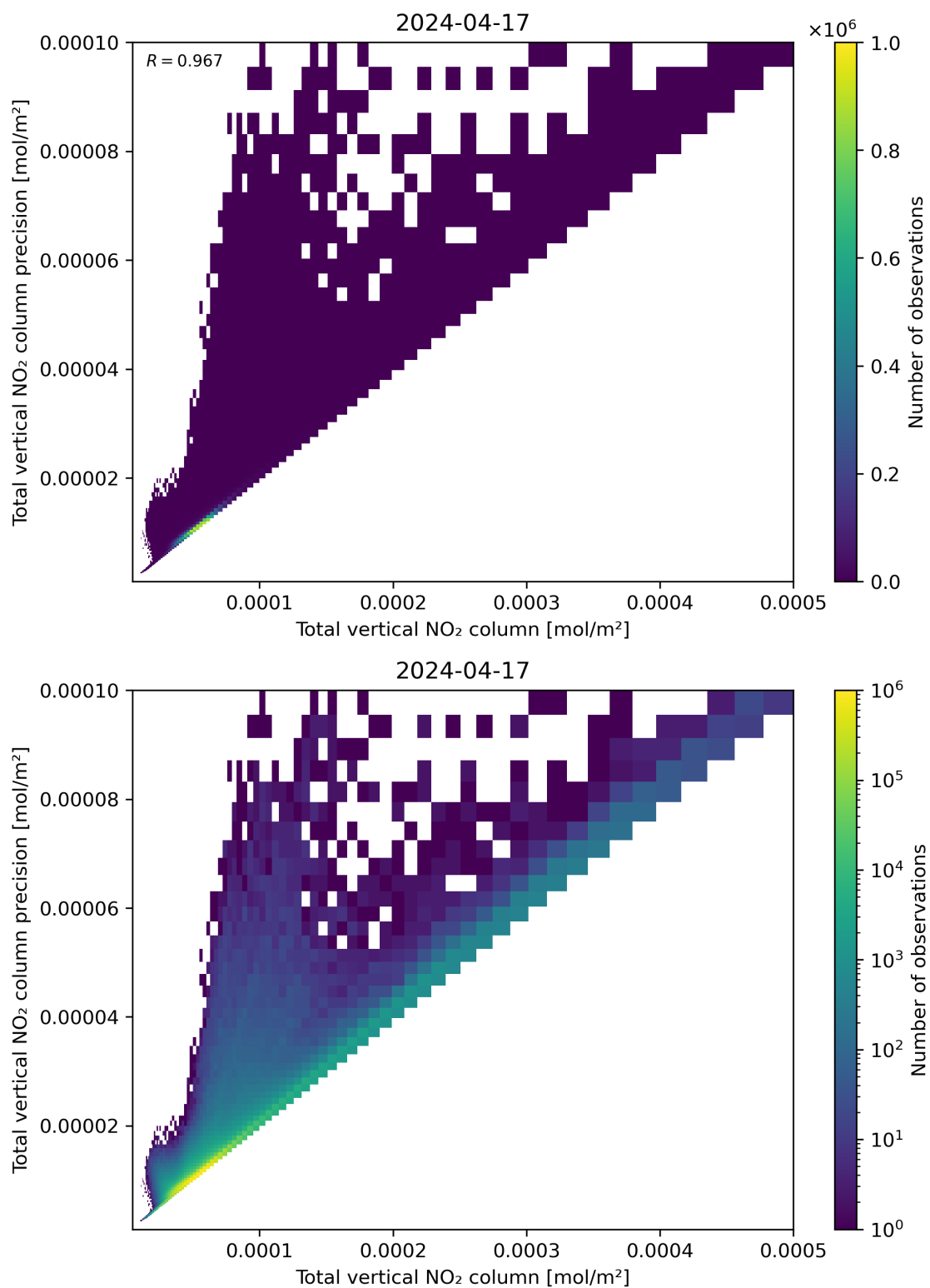
Figure 114: Scatter density plot of “Total vertical NO 2 column” against “Total vertical NO 2 column precision” for 2024-04-16 to 2024-04-18.
