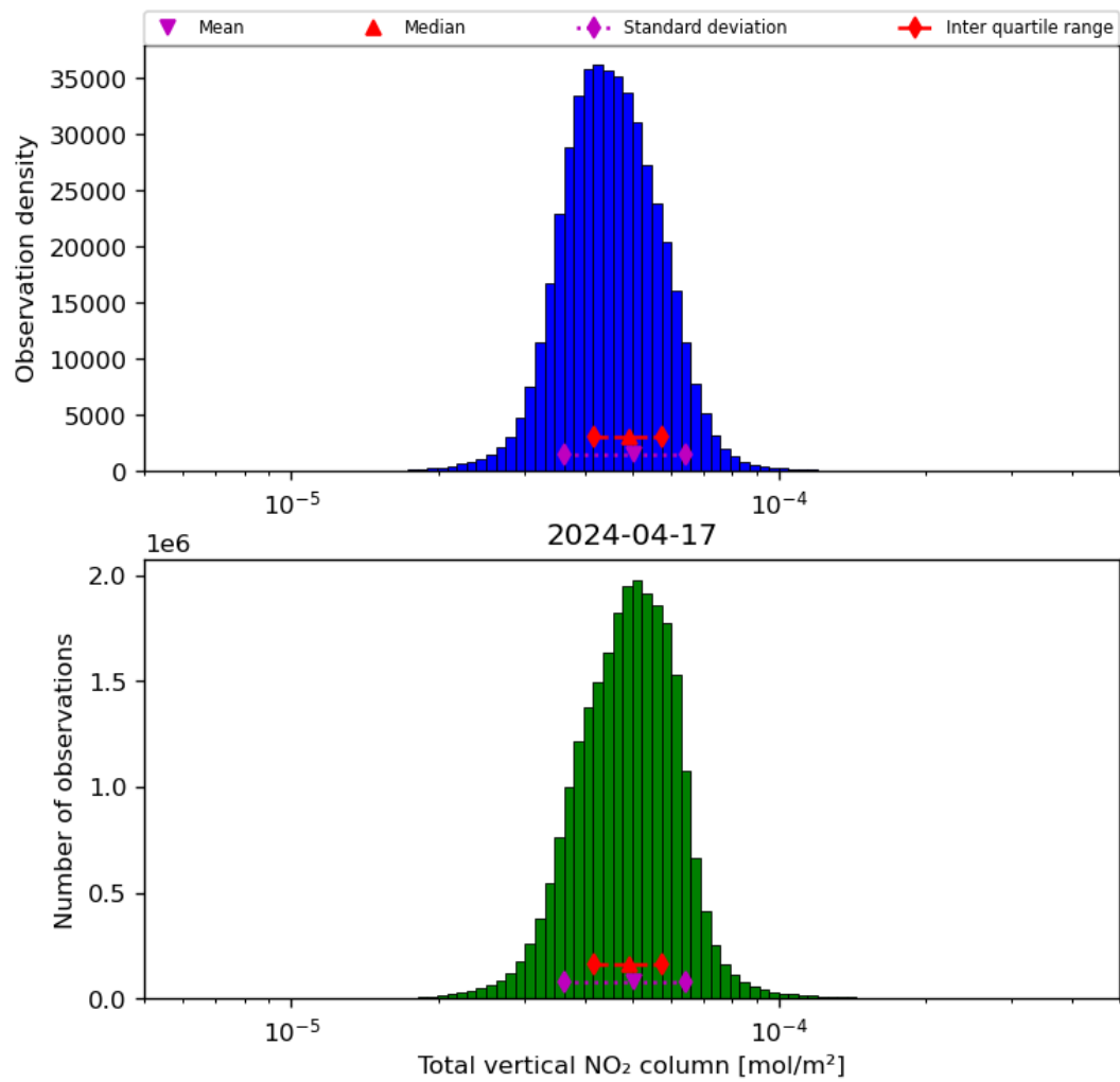
Figure 38: Histogram of “Total vertical NO 2 column” for 2024-04-16 to 2024-04-18
