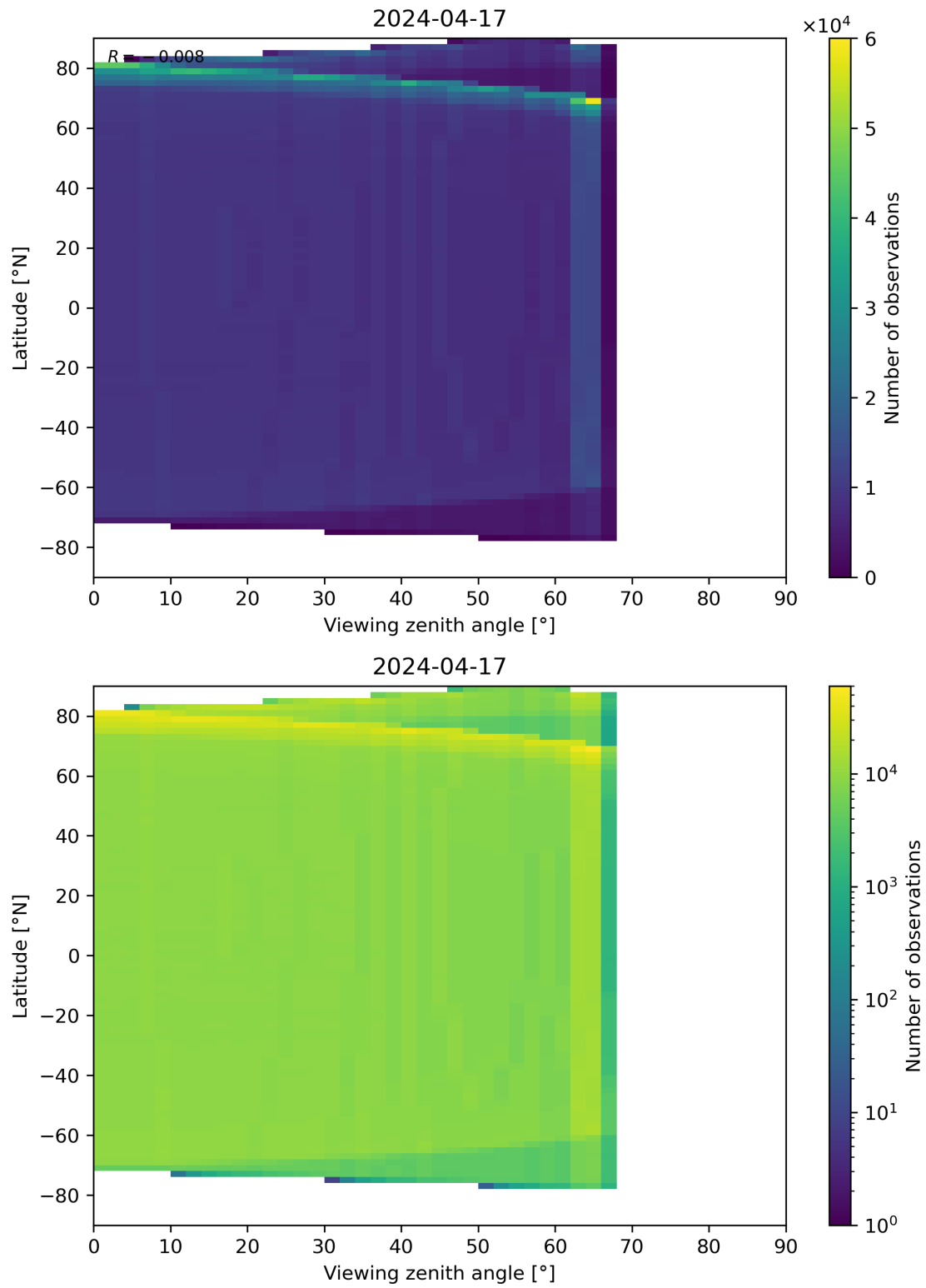
Figure 163: Scatter density plot of “Viewing zenith angle” against “Latitude” for 2024-04-16 to 2024-04-18.
