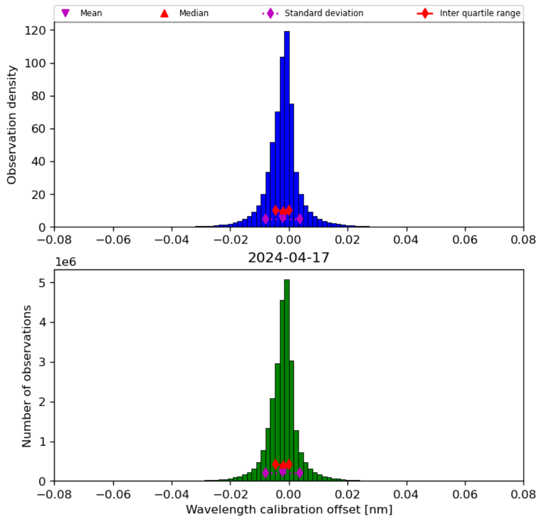
Figure 35: Histogram of “Wavelength calibration offset” for 2024-04-16 to 2024-04-18
