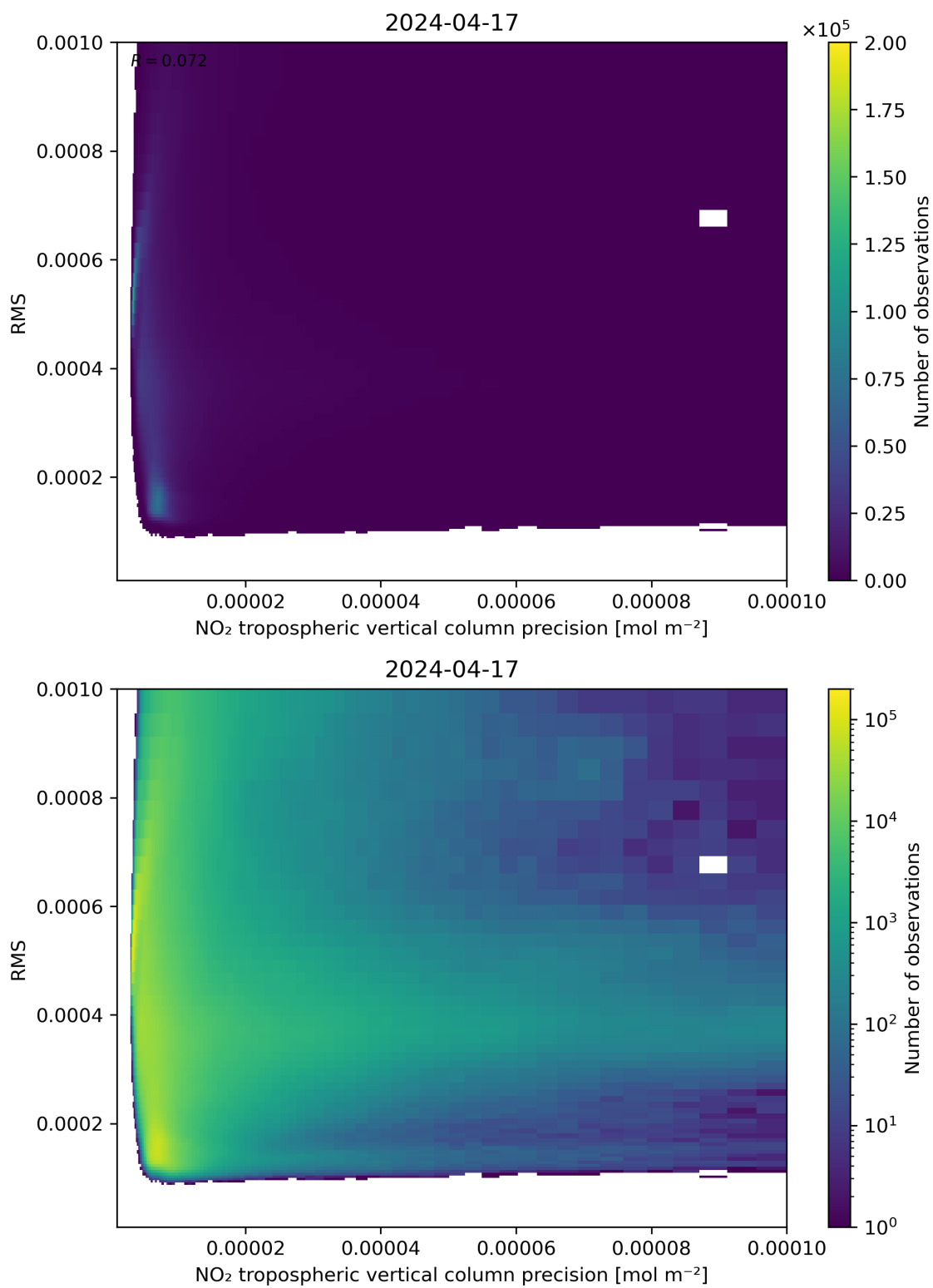
Figure 140: Scatter density plot of “NO 2 tropospheric vertical column precision” against “RMS” for 2024-04-16 to 2024-04-18.
