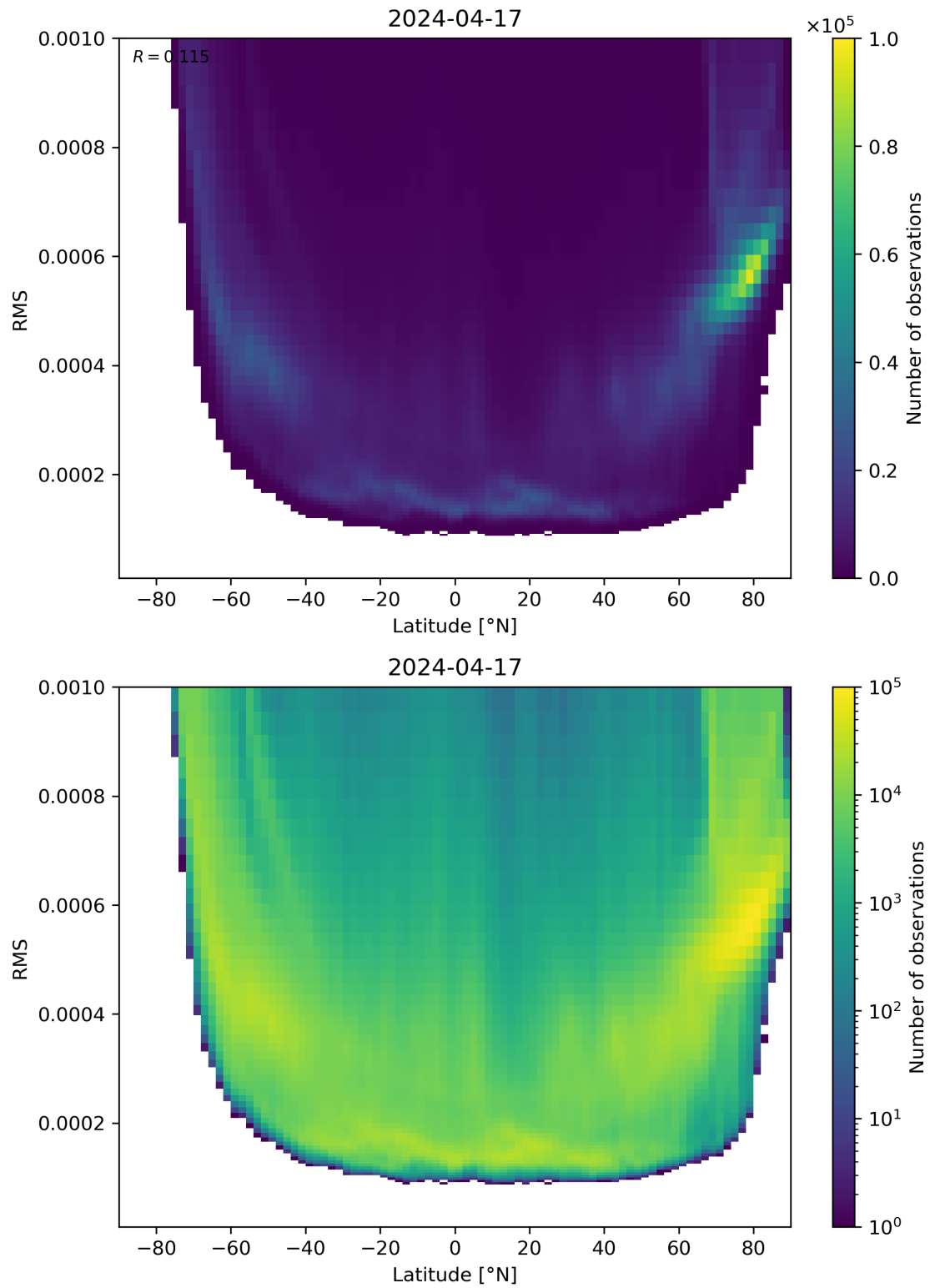
Figure 94: Scatter density plot of “Latitude” against “RMS” for 2024-04-16 to 2024-04-18.
