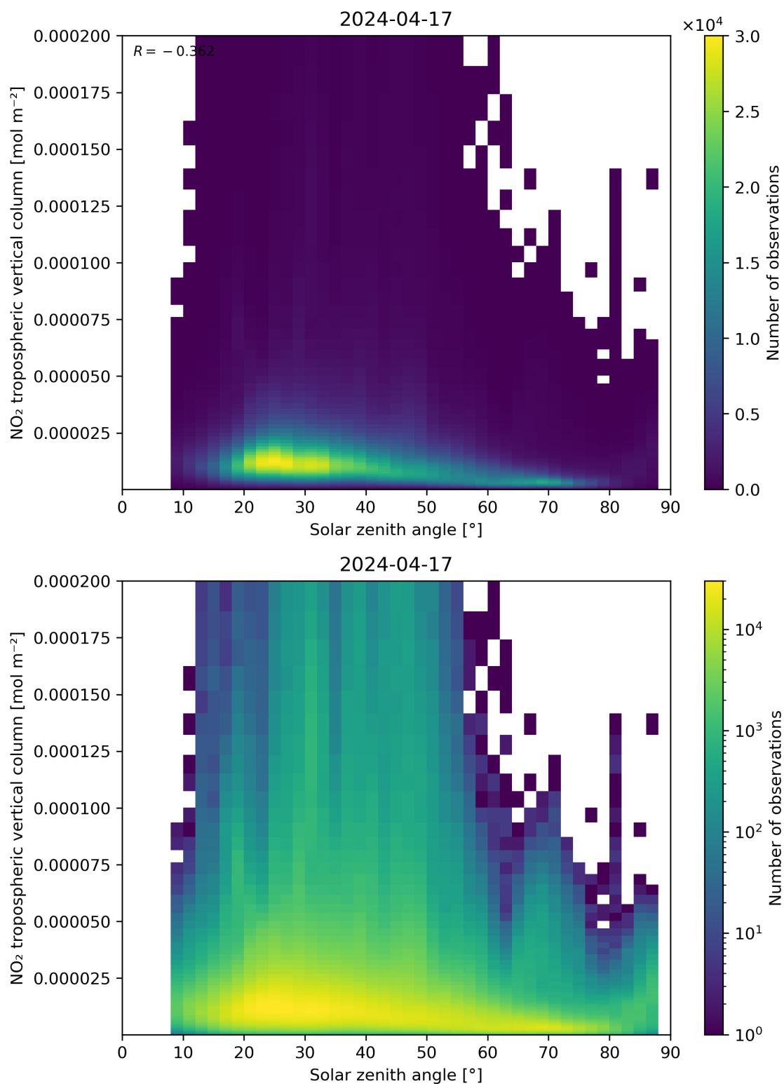
Figure 155: Scatter density plot of “Solar zenith angle” against “NO 2 tropospheric vertical column” for 2024-04-16 to 2024-04-18.
