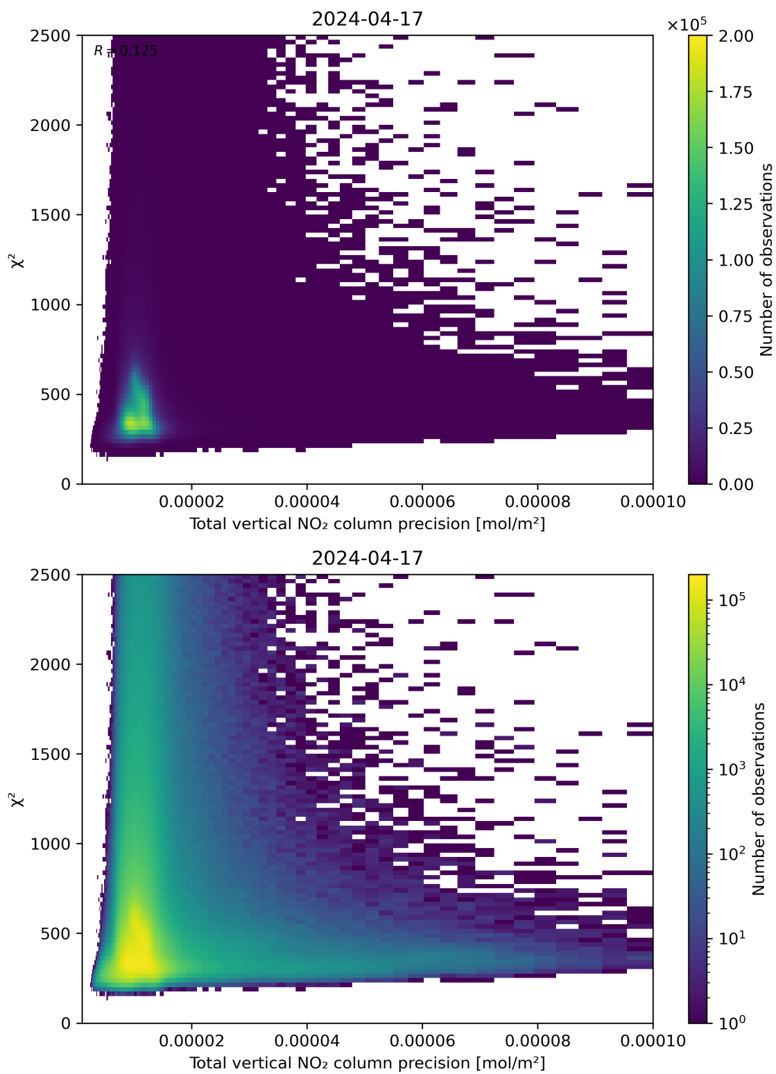
Figure 116: Scatter density plot of “Total vertical NO 2 column precision” against “ \chi^2 ” for 2024-04-16 to 2024-04-18.
