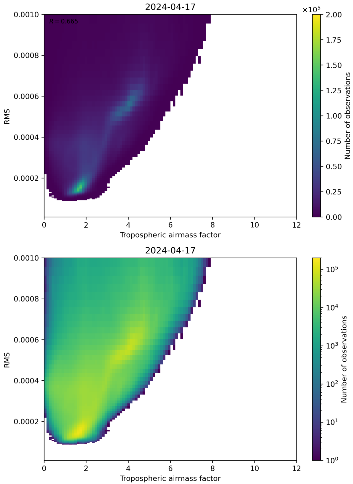
Figure 79: Scatter density plot of “Tropospheric airmass factor” against “RMS” for 2024-04-16 to 2024-04-18.
