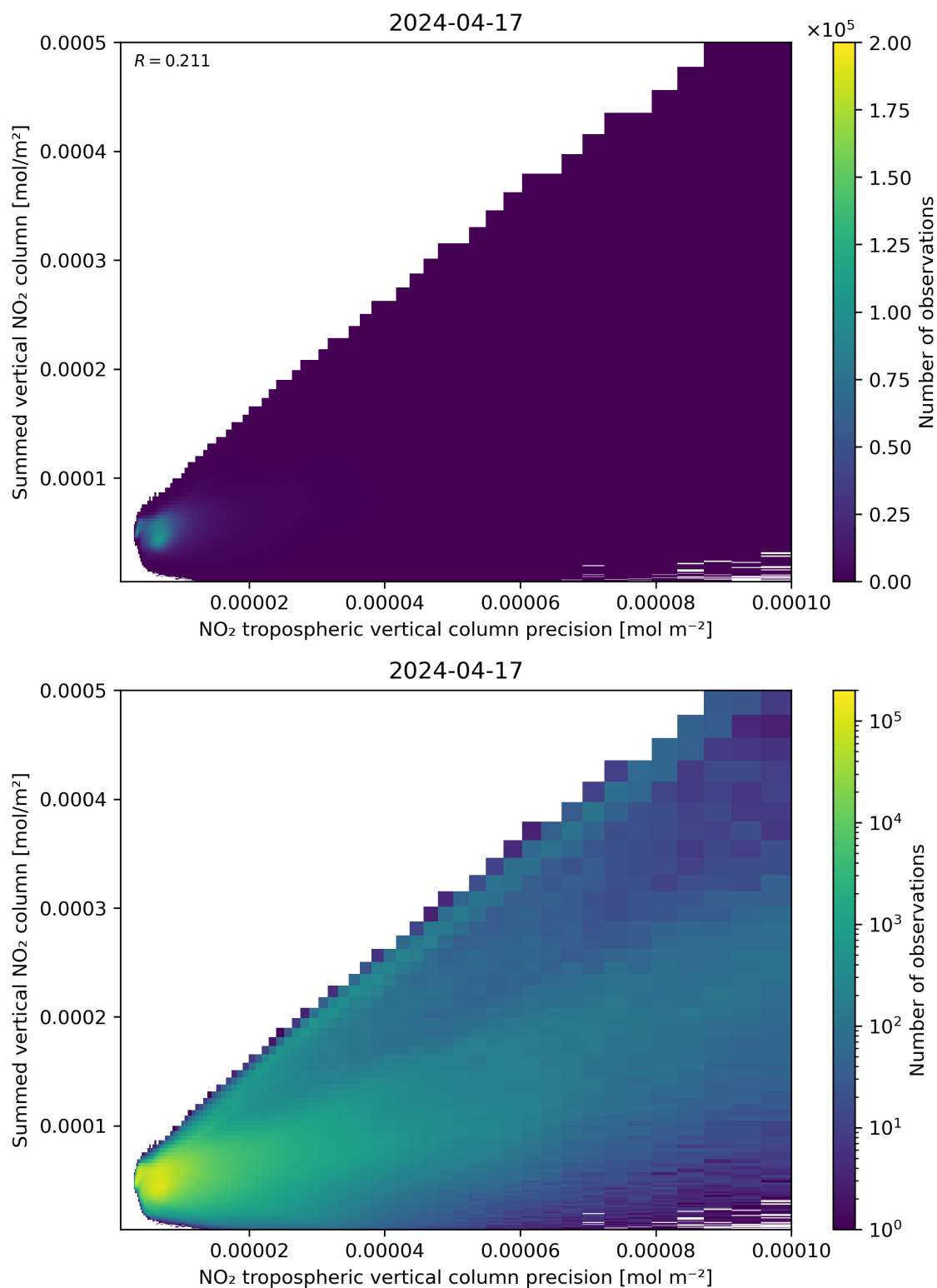
Figure 136: Scatter density plot of “NO 2 tropospheric vertical column precision” against “Summed vertical NO 2 column” for 2024-04-16 to 2024-04-18.
