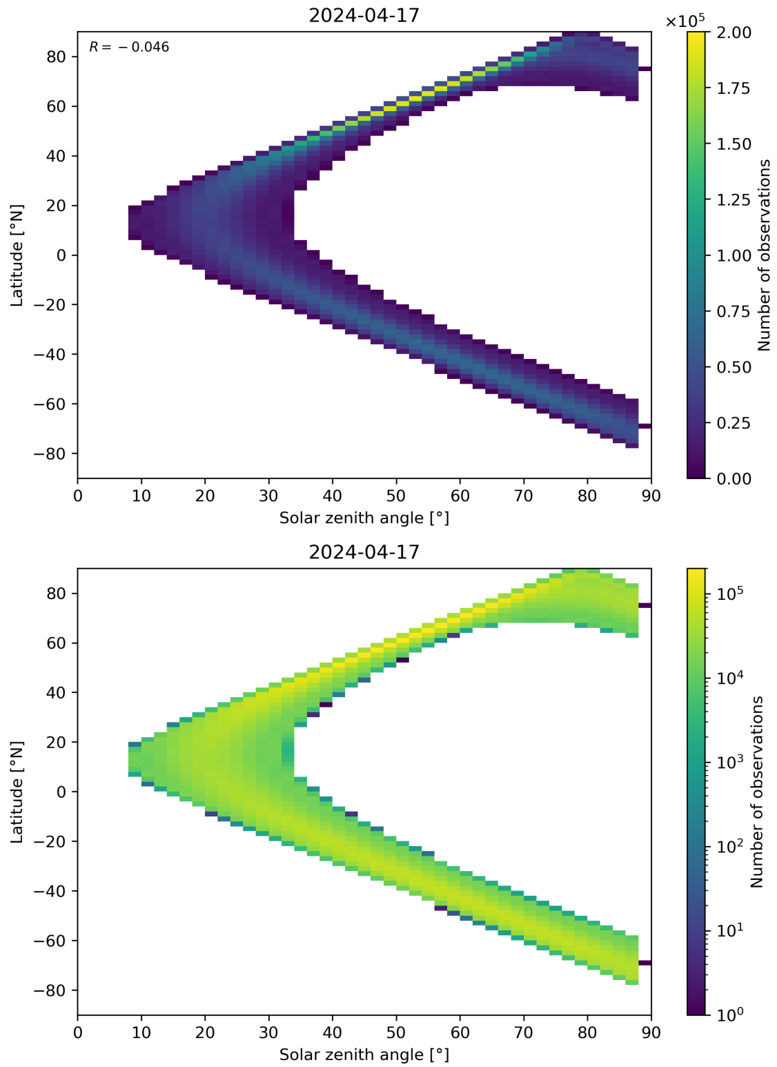
Figure 149: Scatter density plot of “Solar zenith angle” against “Latitude” for 2024-04-16 to 2024-04-18.
