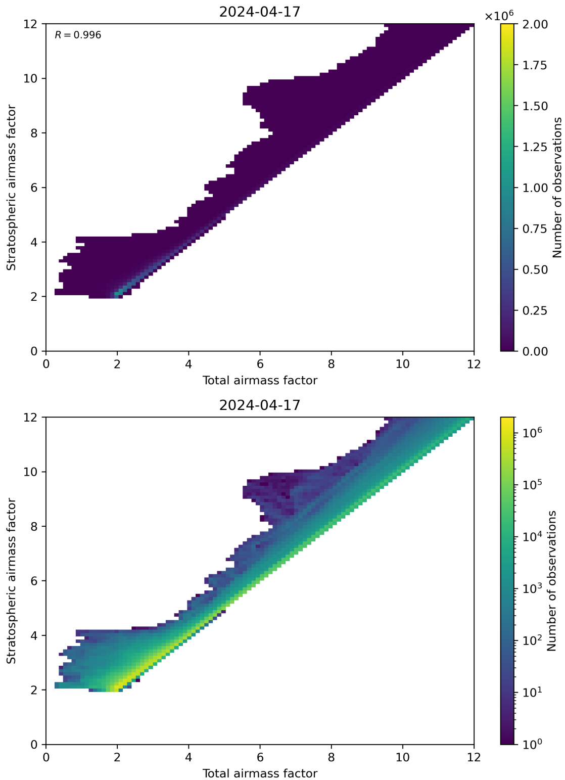
Figure 62: Scatter density plot of “Total airmass factor” against “Stratospheric airmass factor” for 2024-04-16 to 2024-04-18.
