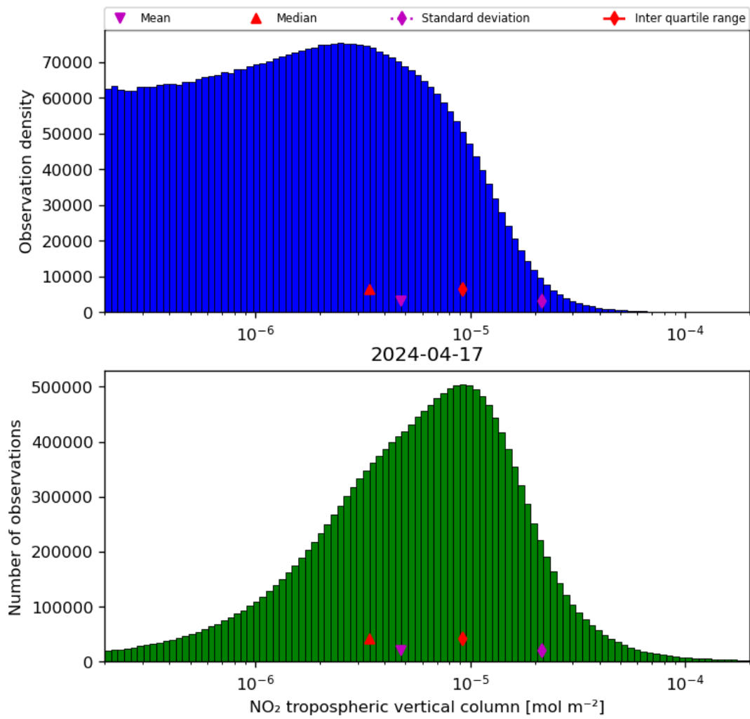
Figure 29: Histogram of “NO 2 tropospheric vertical column” for 2024-04-16 to 2024-04-18
