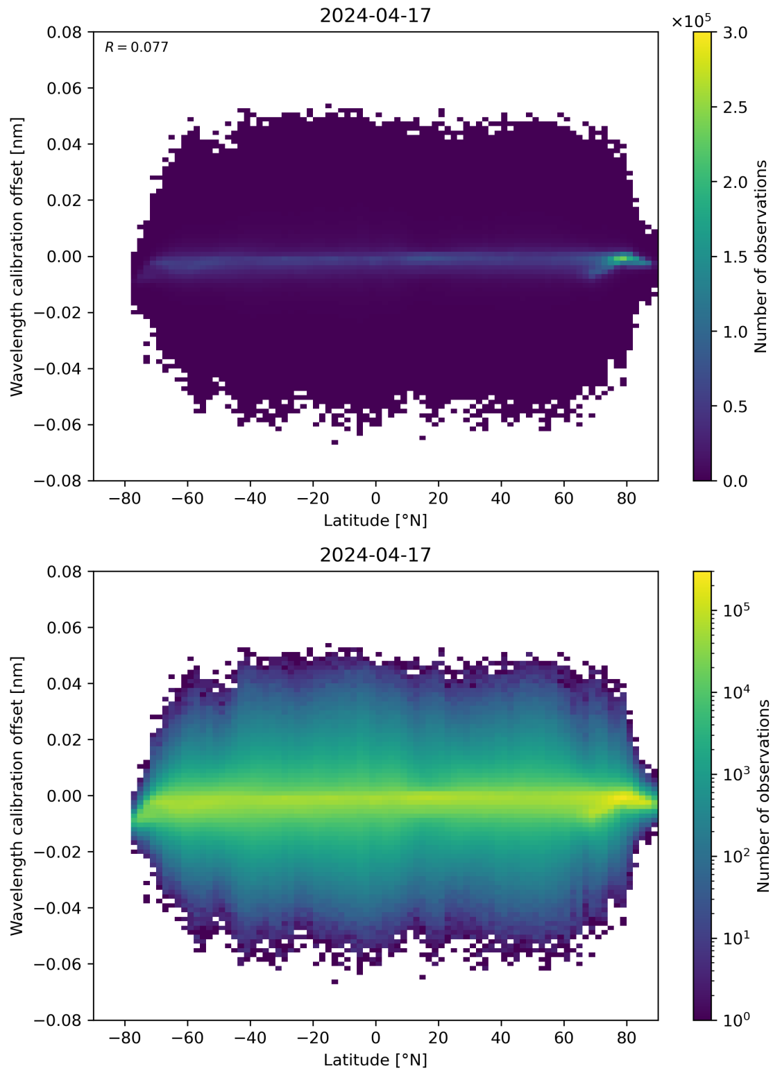
Figure 95: Scatter density plot of “Latitude” against “Wavelength calibration offset” for 2024-04-16 to 2024-04-18.
