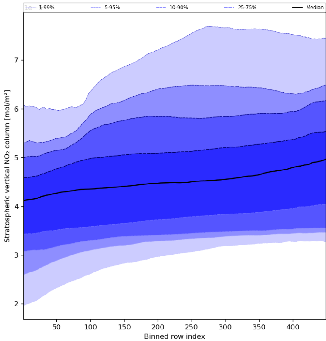
Figure 53: Along track statistics of “Stratospheric vertical NO 2 column” for 2024-04-16 to 2024-04-18
