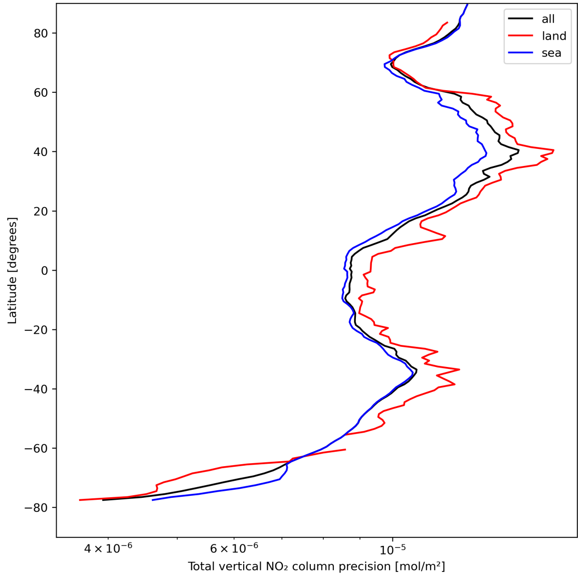
Figure 22: Zonal average of "Total vertical NO 2 column precision" for 2024-04-16 to 2024-04-18.
