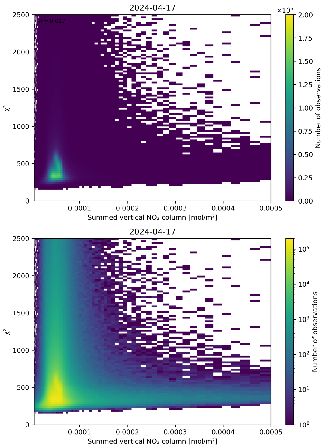
Figure 104: Scatter density plot of “Summed vertical NO 2 column” against “ \chi^2 ” for 2024-04-16 to 2024-04-18.
