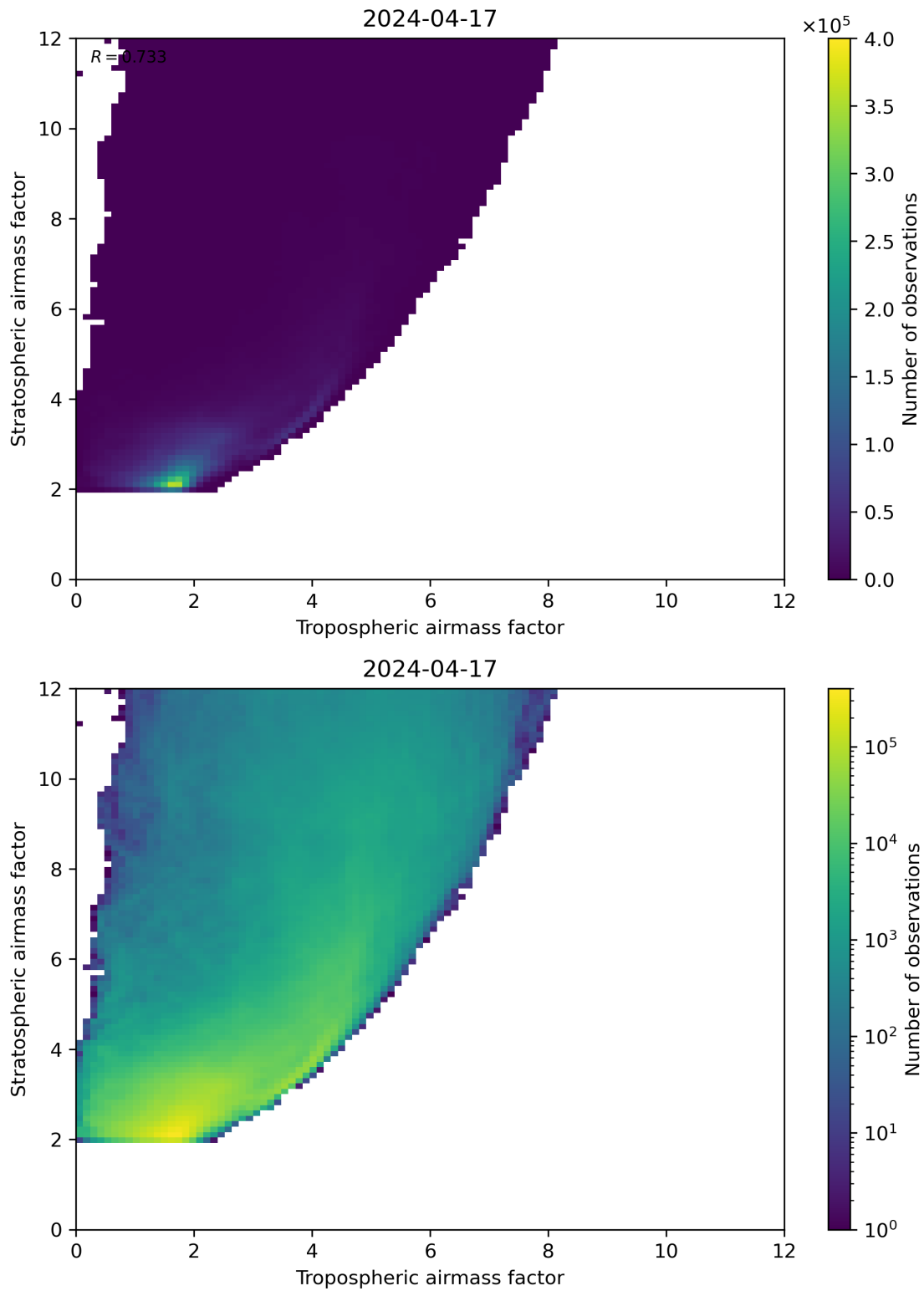
Figure 71: Scatter density plot of “Tropospheric airmass factor” against “Stratospheric airmass factor” for 2024-04-16 to 2024-04-18.
