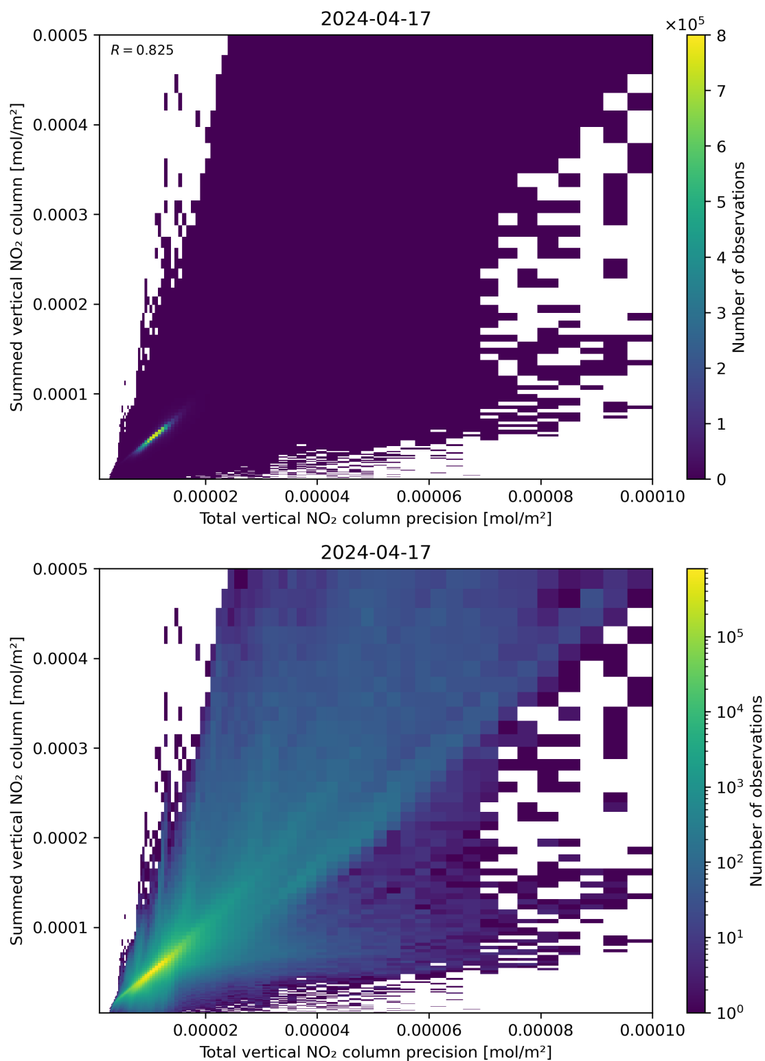
Figure 117: Scatter density plot of “Total vertical NO 2 column precision” against “Summed vertical NO 2 column” for 2024-04-16 to 2024-04-18.
