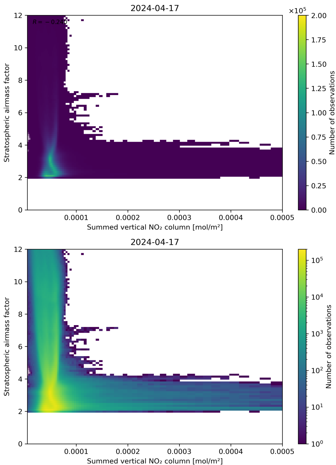
Figure 103: Scatter density plot of “Summed vertical NO 2 column” against “Stratospheric airmass factor” for 2024-04-16 to 2024-04-18.
