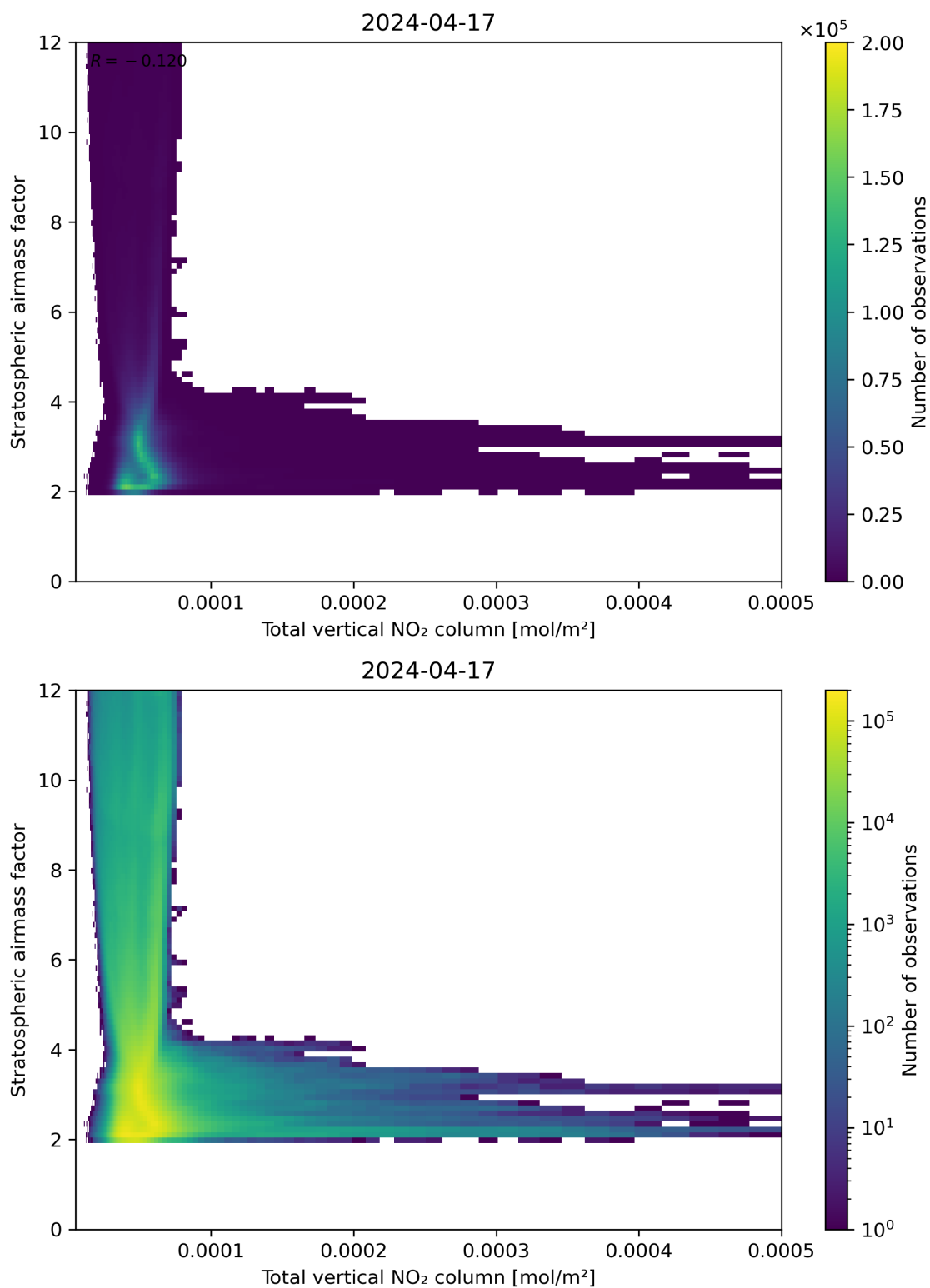
Figure 110: Scatter density plot of “Total vertical NO 2 column” against “Stratospheric airmass factor” for 2024-04-16 to 2024-04-18.
