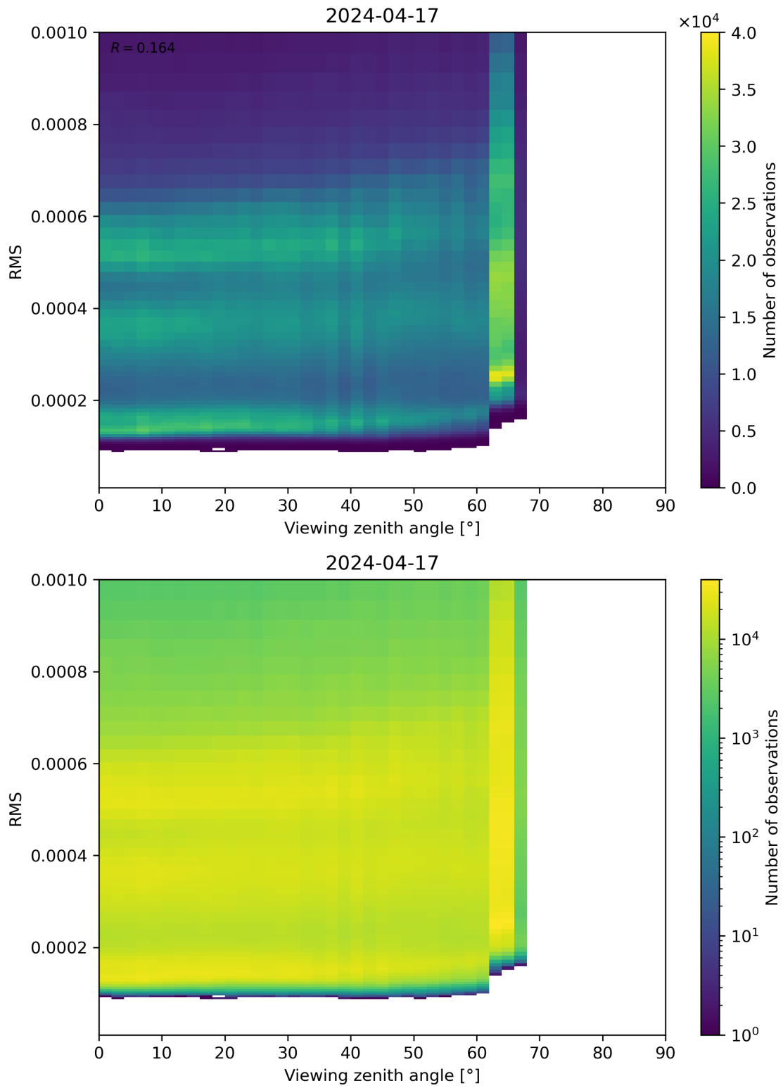
Figure 171: Scatter density plot of “Viewing zenith angle” against “RMS” for 2024-04-16 to 2024-04-18.
