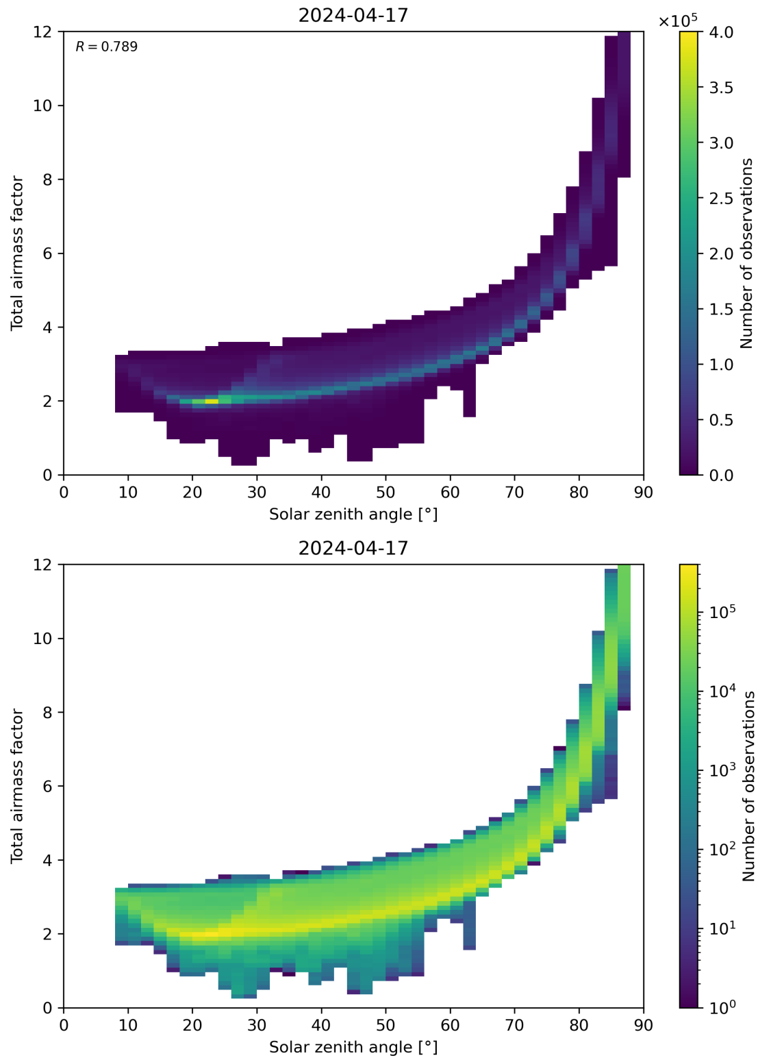
Figure 146: Scatter density plot of “Solar zenith angle” against “Total air mass factor” for 2024-04-16 to 2024-04-18.
