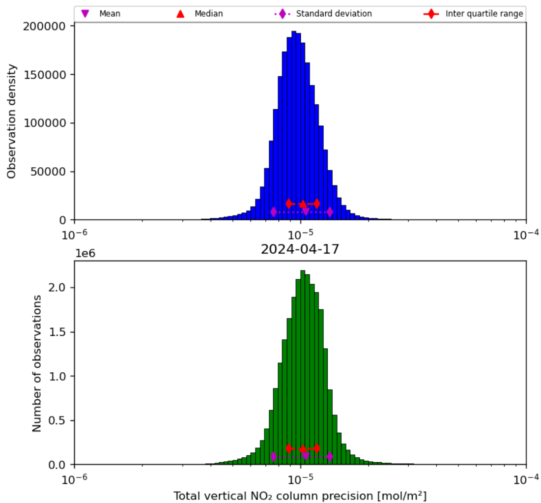
Figure 39: Histogram of "Total vertical NO 2 column precision" for 2024-04-16 to 2024-04-18
