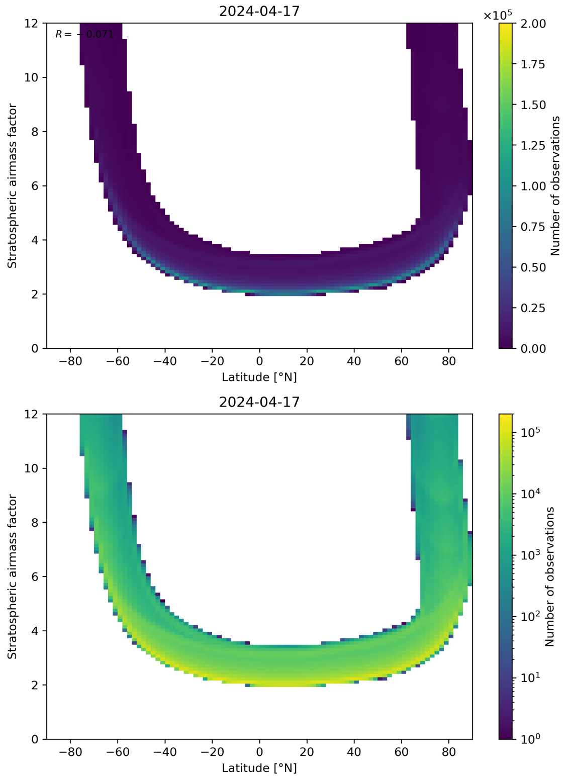
Figure 83: Scatter density plot of “Latitude” against “Stratospheric air mass factor” for 2024-04-16 to 2024-04-18.
