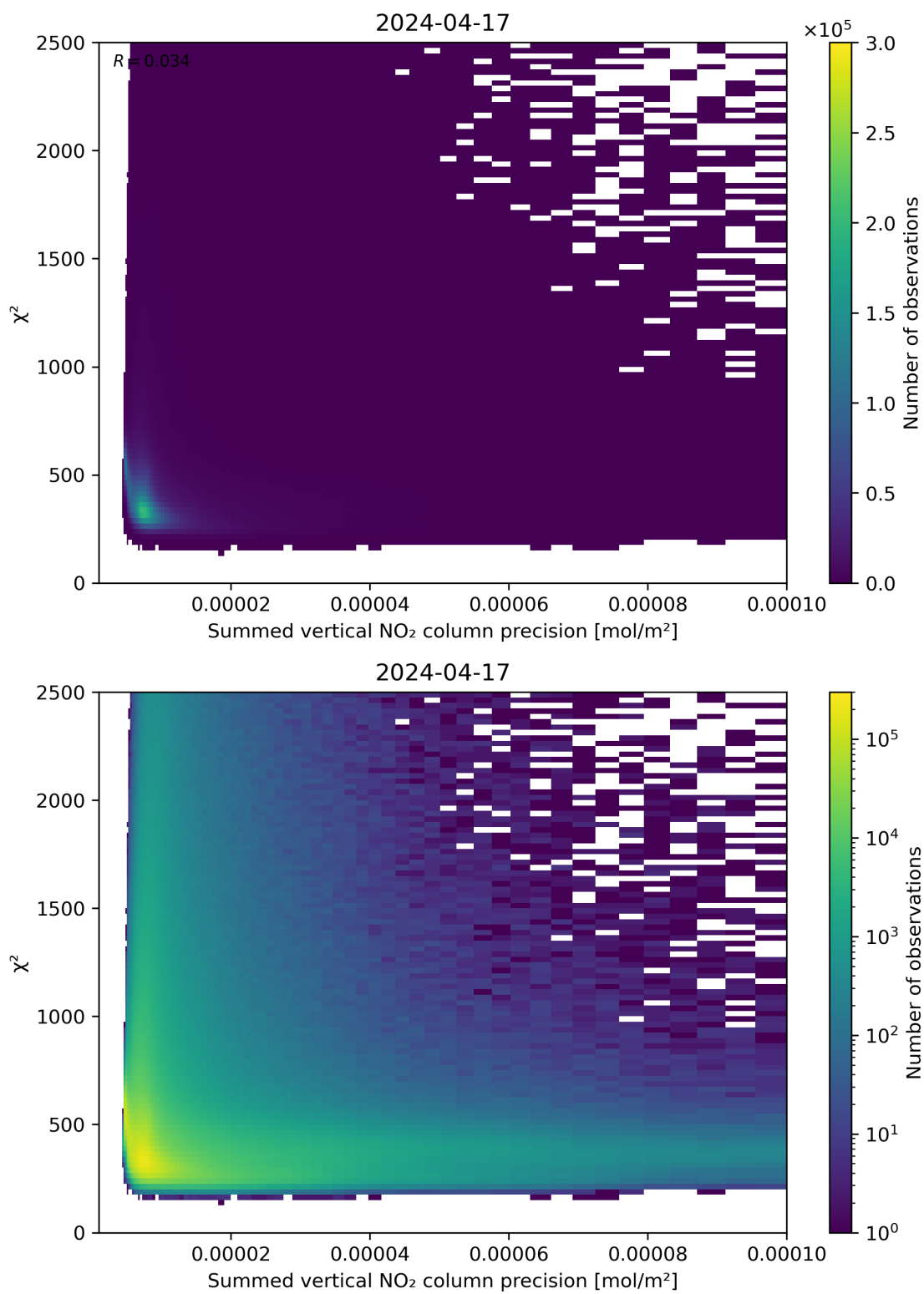
Figure 107: Scatter density plot of “Summed vertical NO 2 column precision” against “ \chi^2 ” for 2024-04-16 to 2024-04-18.
