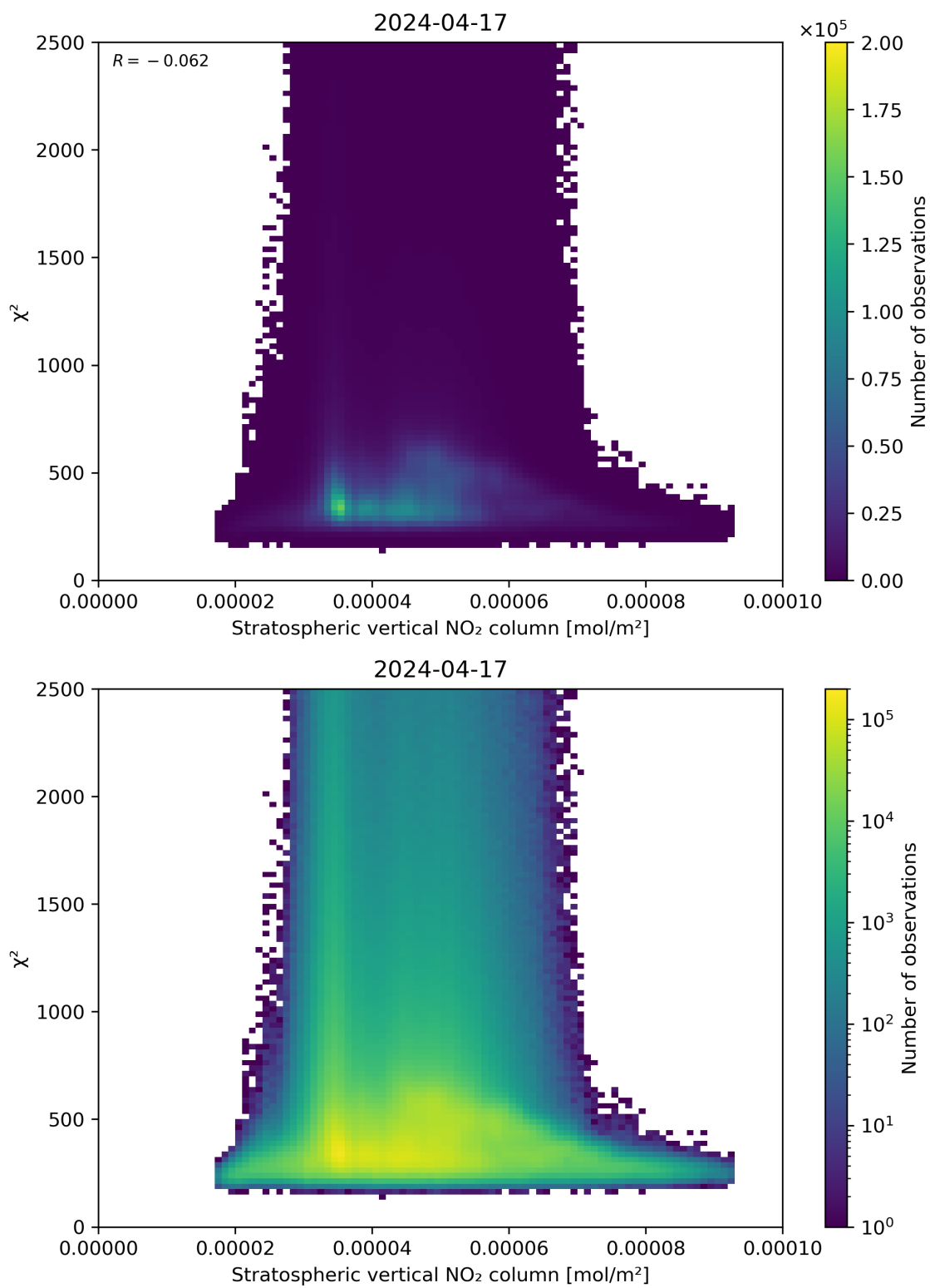
Figure 97: Scatter density plot of “Stratospheric vertical NO 2 column” against “ \chi^2 ” for 2024-04-16 to 2024-04-18.
