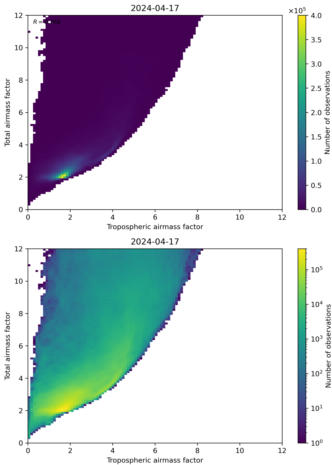
Figure 72: Scatter density plot of “Tropospheric airmass factor” against “Total airmass factor” for 2024-04-16 to 2024-04-18.
