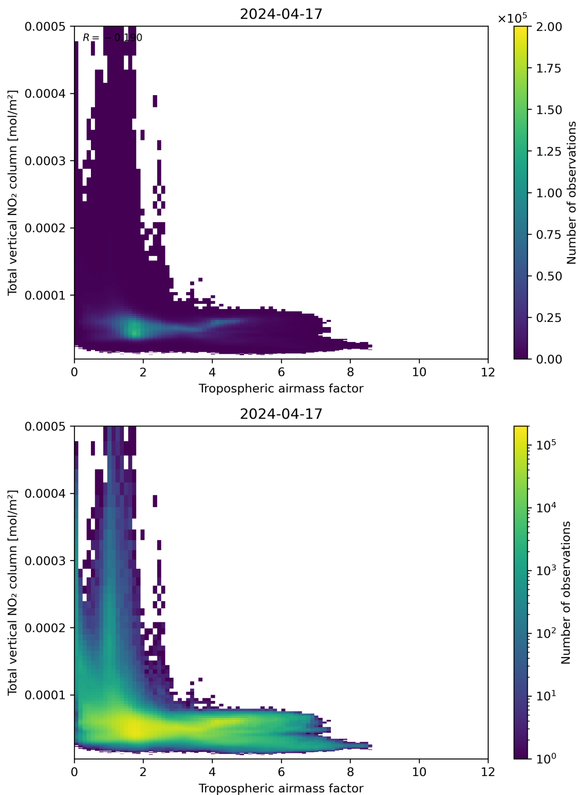
Figure 77: Scatter density plot of “Tropospheric airmass factor” against “Total vertical NO 2 column” for 2024-04-16 to 2024-04-18.
