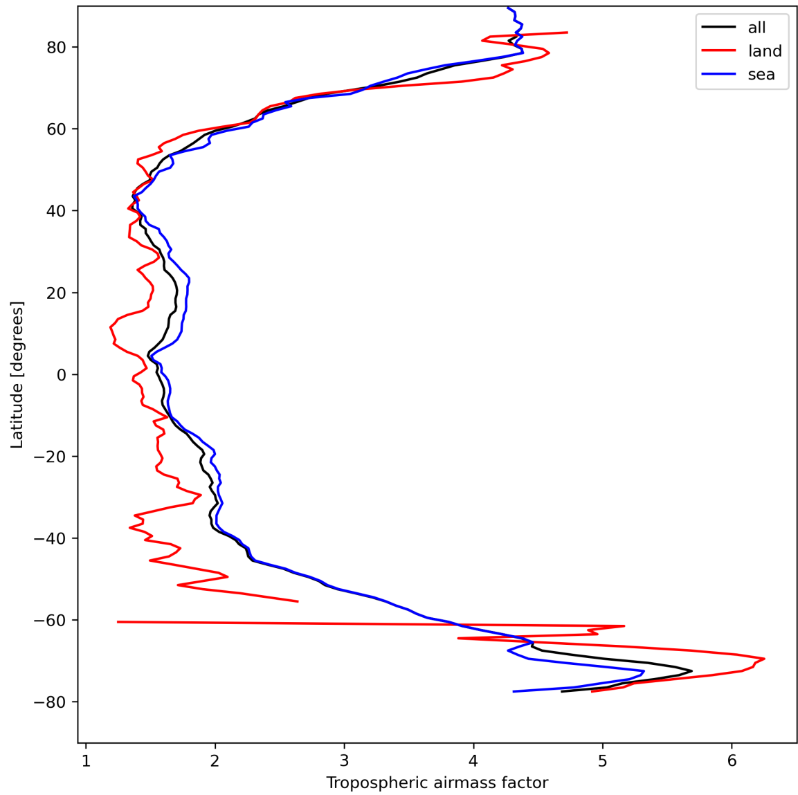
Figure 14: Zonal average of “Tropospheric airmass factor” for 2024-04-16 to 2024-04-18.
