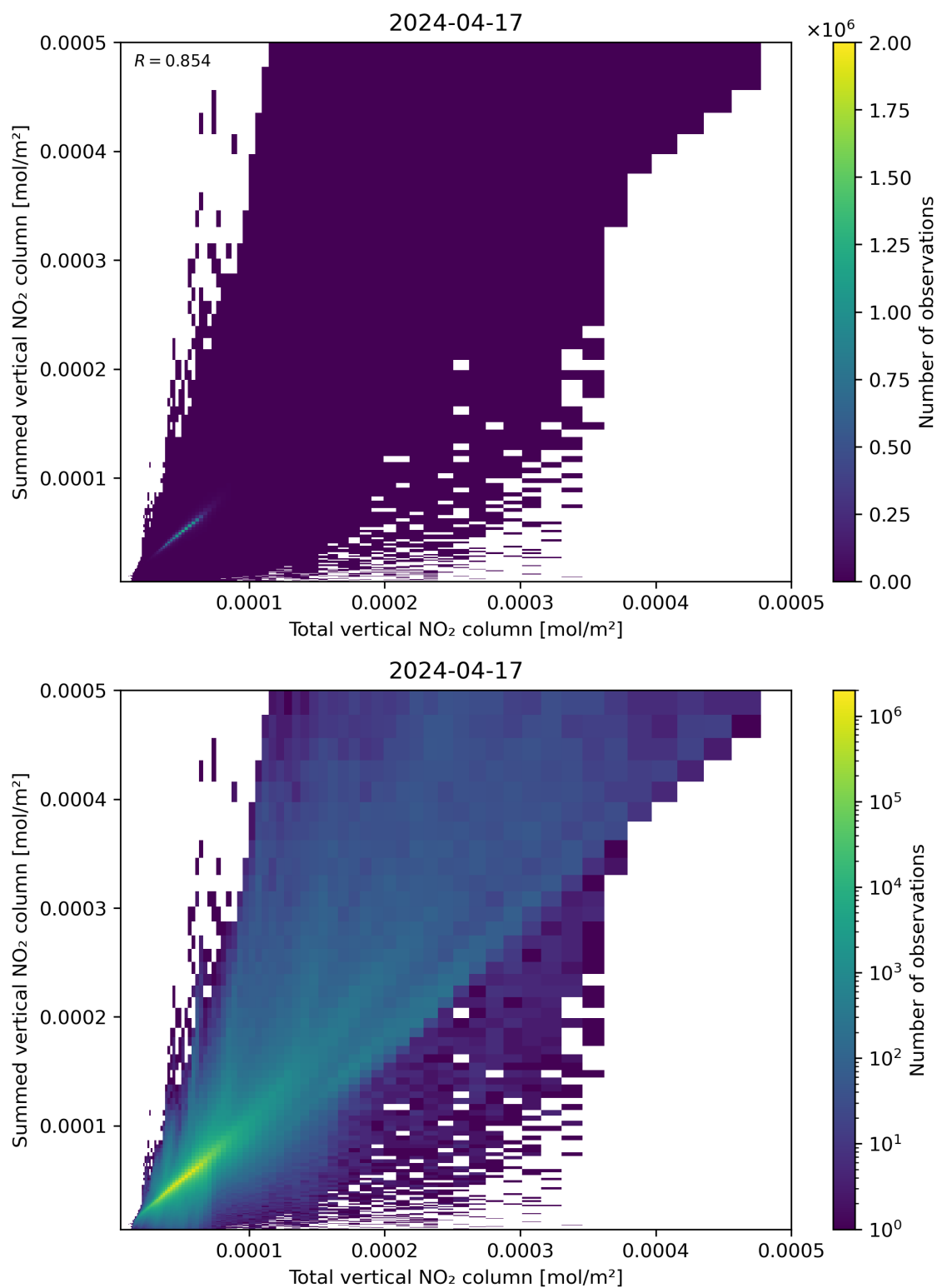
Figure 112: Scatter density plot of “Total vertical NO 2 column” against “Summed vertical NO 2 column” for 2024-04-16 to 2024-04-18.
