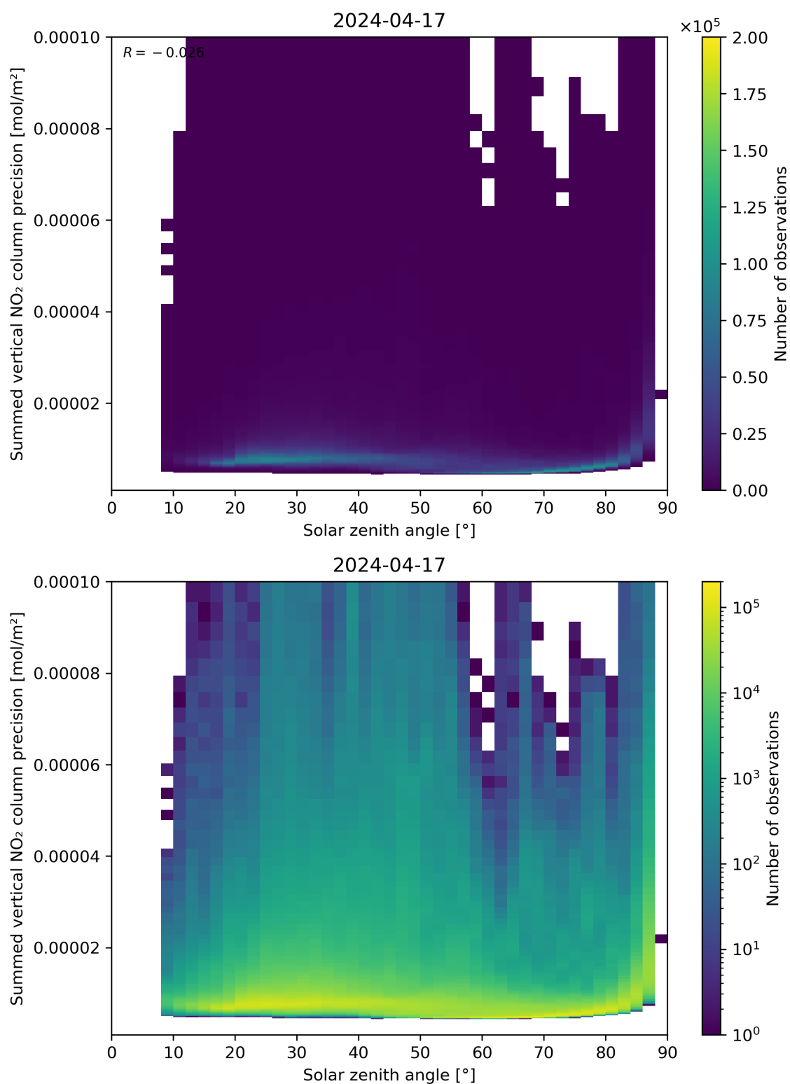
Figure 152: Scatter density plot of “Solar zenith angle” against “Summed vertical NO 2 column precision” for 2024-04-16 to 2024-04-18.
