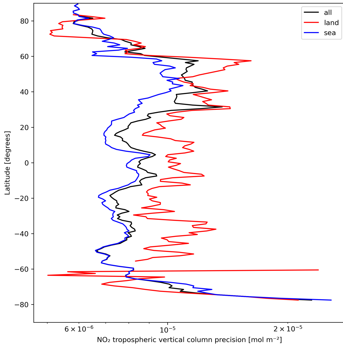
Figure 13: Zonal average of “NO 2 tropospheric vertical column precision” for 2024-04-16 to 2024-04-18.
