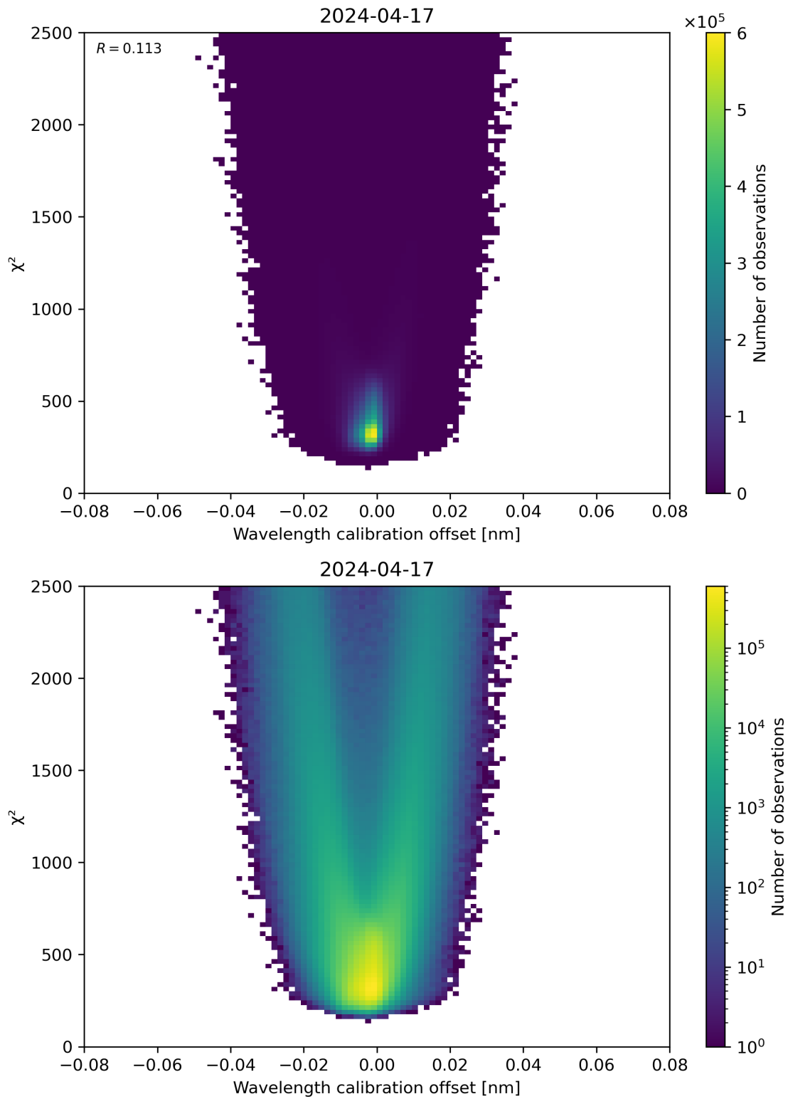
Figure 175: Scatter density plot of “Wavelength calibration offset” against “ \chi^2 ” for 2024-04-16 to 2024-04-18.
