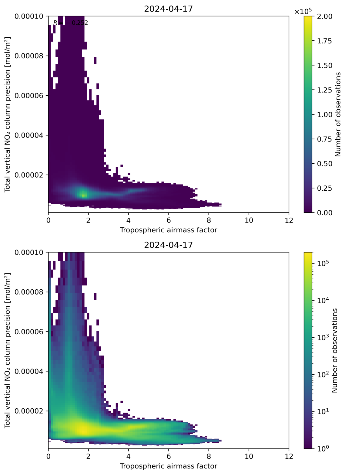
Figure 78: Scatter density plot of “Tropospheric air mass factor” against “Total vertical NO 2 column precision” for 2024-04-16 to 2024-04-18.
