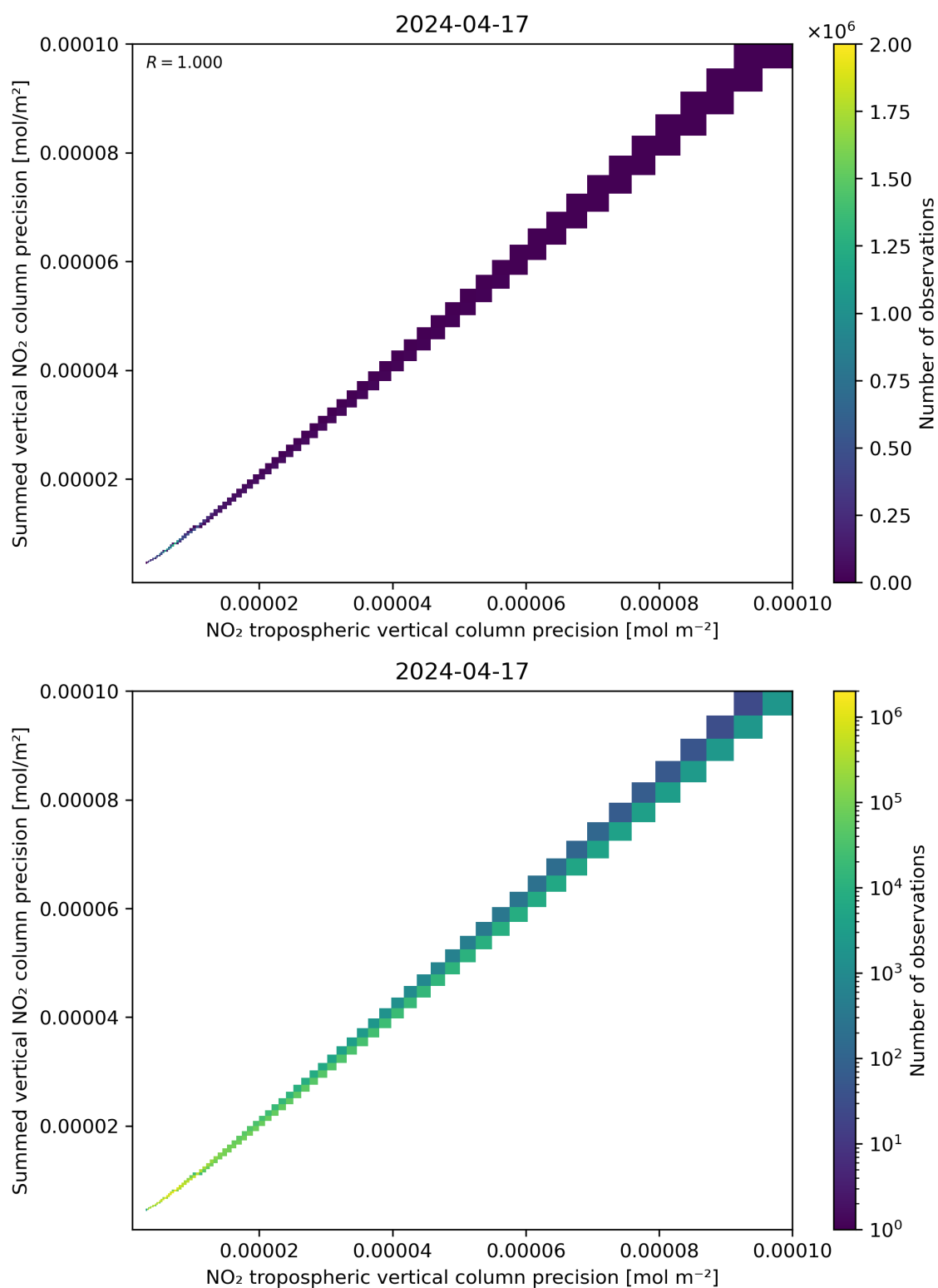
Figure 137: Scatter density plot of “NO 2 tropospheric vertical column precision” against “Summed vertical NO 2 column precision” for 2024-04-16 to 2024-04-18.
