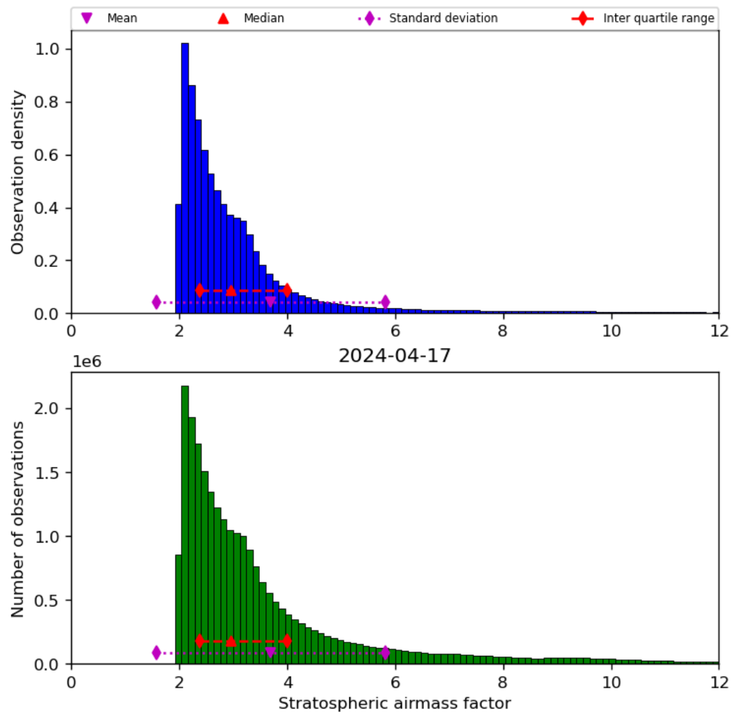
Figure 44: Histogram of “Stratospheric airmass factor” for 2024-04-16 to 2024-04-18
