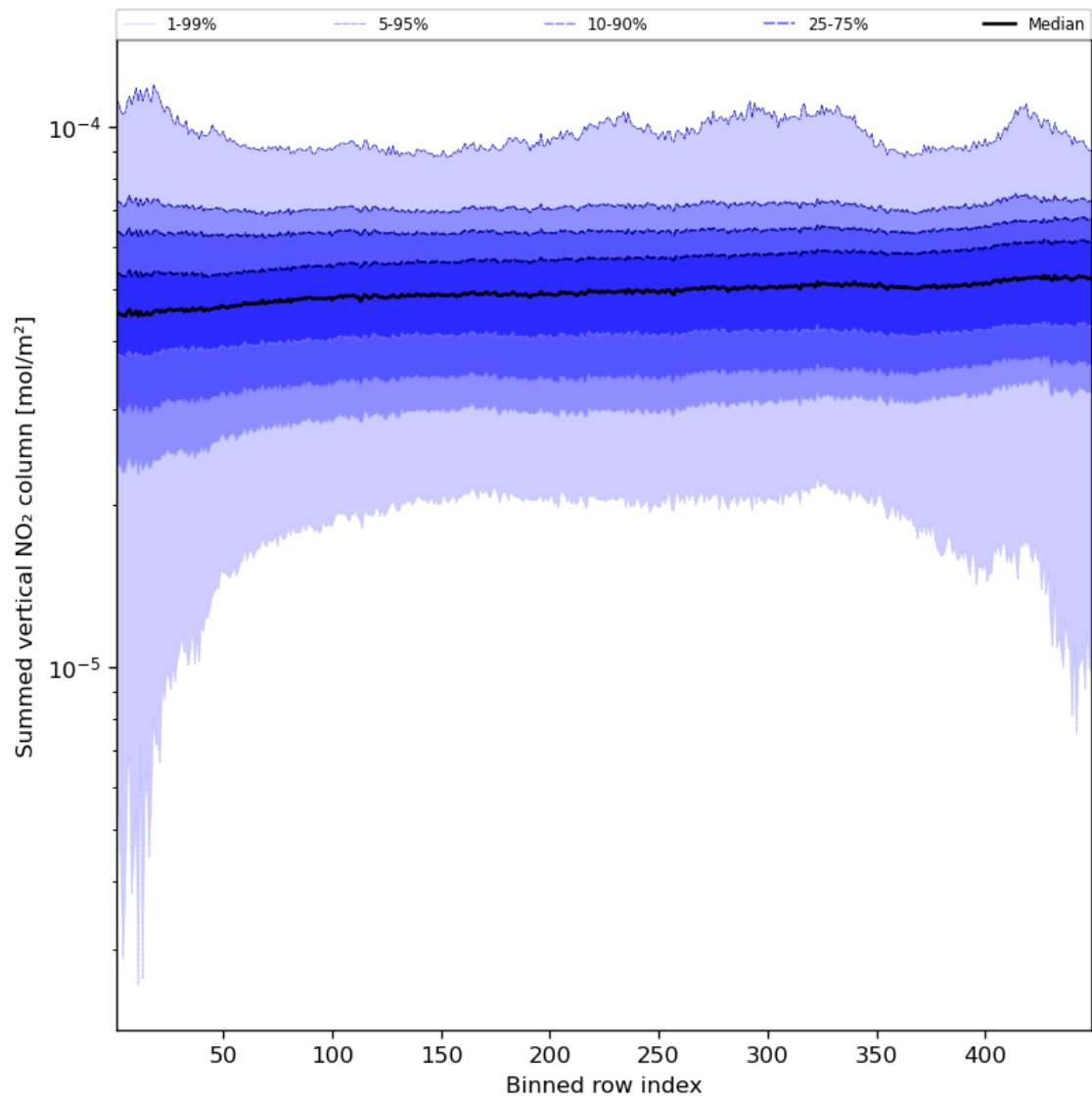
Figure 57: Along track statistics of “Summed vertical NO 2 column” for 2024-04-16 to 2024-04-18
