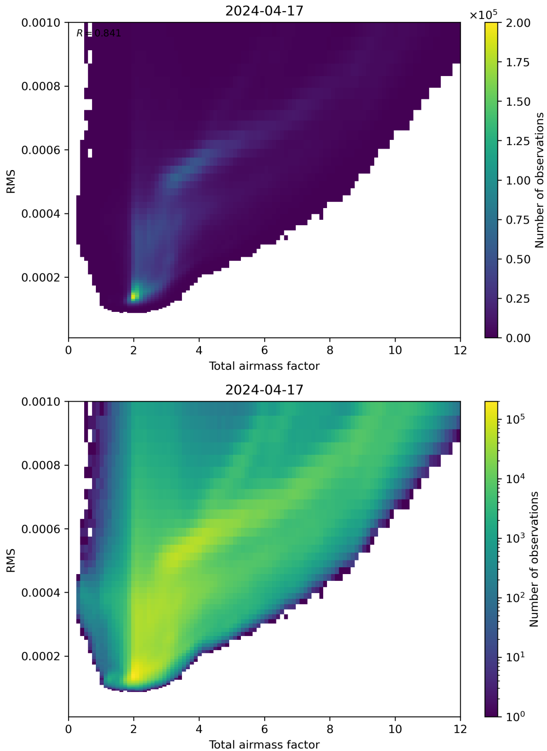
Figure 69: Scatter density plot of “Total airmass factor” against “RMS” for 2024-04-16 to 2024-04-18.
