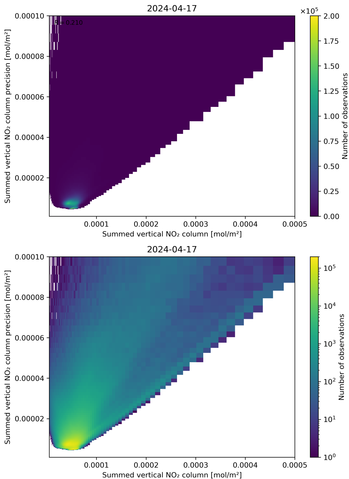
Figure 105: Scatter density plot of “Summed vertical NO 2 column” against “Summed vertical NO 2 column precision” for 2024-04-16 to 2024-04-18.
