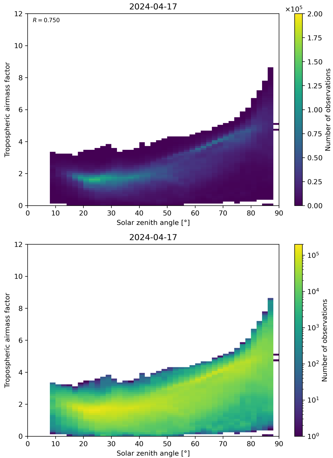
Figure 147: Scatter density plot of “Solar zenith angle” against “Tropospheric airmass factor” for 2024-04-16 to 2024-04-18.
