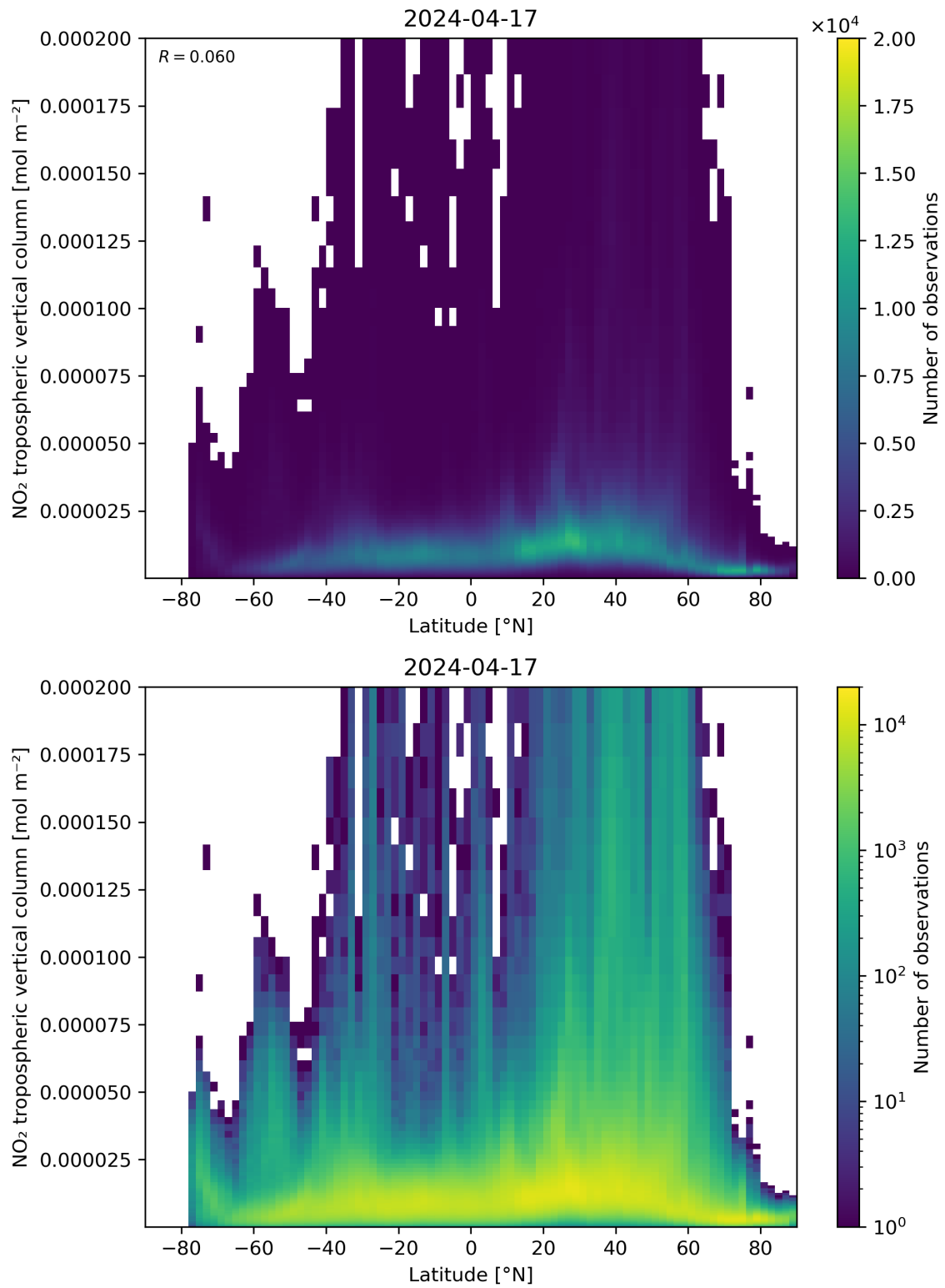
Figure 92: Scatter density plot of “Latitude” against “NO 2 tropospheric vertical column” for 2024-04-16 to 2024-04-18.
