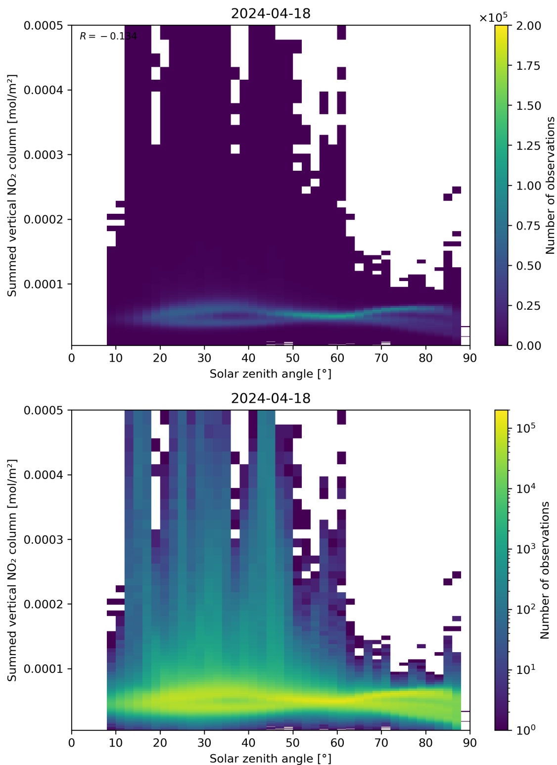
Figure 151: Scatter density plot of “Solar zenith angle” against “Summed vertical NO 2 column” for 2024-04-17 to 2024-04-19.
