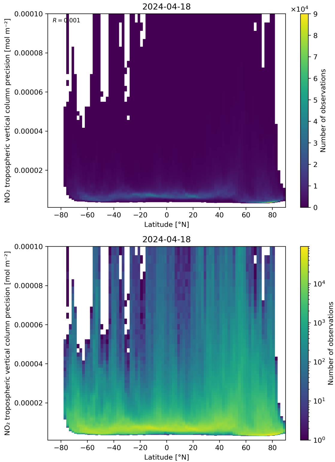
Figure 93: Scatter density plot of “Latitude” against “NO 2 tropospheric vertical column precision” for 2024-04-17 to 2024-04-19.
