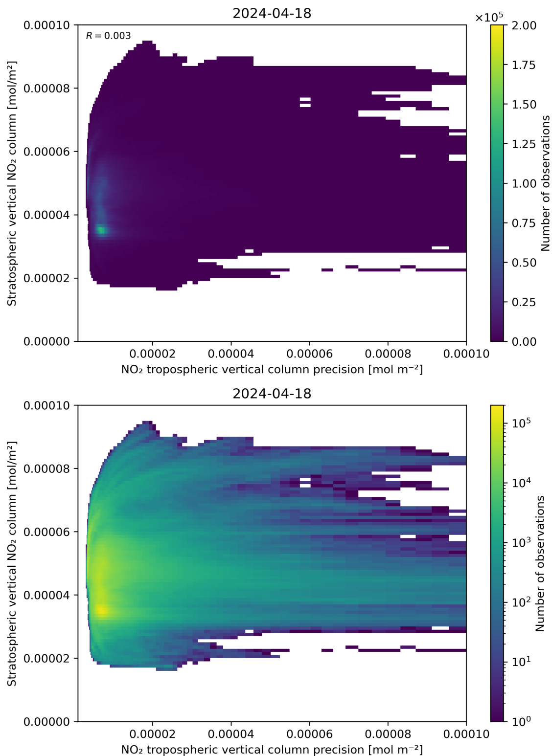
Figure 135: Scatter density plot of “NO 2 tropospheric vertical column precision” against “Stratospheric vertical NO 2 column” for 2024-04-17 to 2024-04-19.
