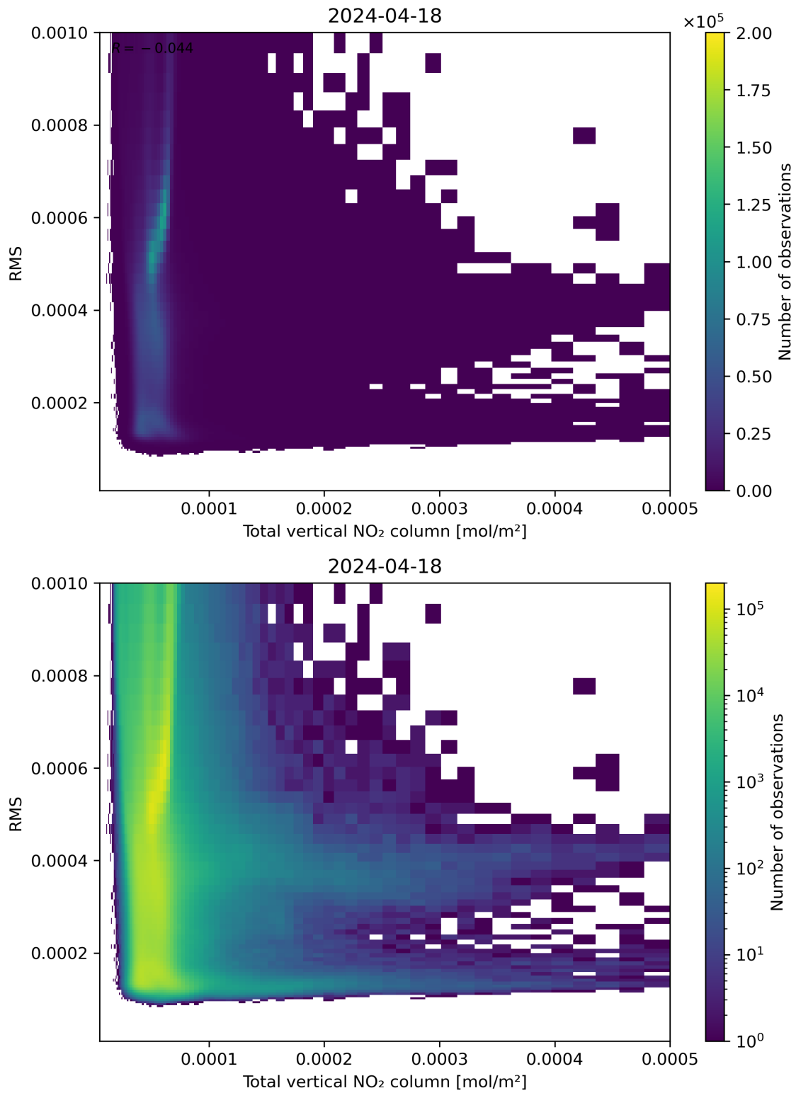
Figure 120: Scatter density plot of “Total vertical NO 2 column” against “RMS” for 2024-04-17 to 2024-04-19.
