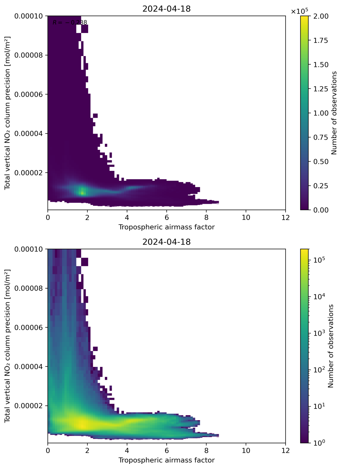
Figure 78: Scatter density plot of “Tropospheric air mass factor” against “Total vertical NO 2 column precision” for 2024-04-17 to 2024-04-19.
