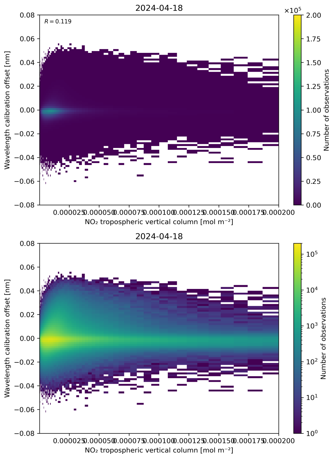
Figure 143: Scatter density plot of “NO 2 tropospheric vertical column” against “Wavelength calibration offset” for 2024-04-17 to 2024-04-19.
