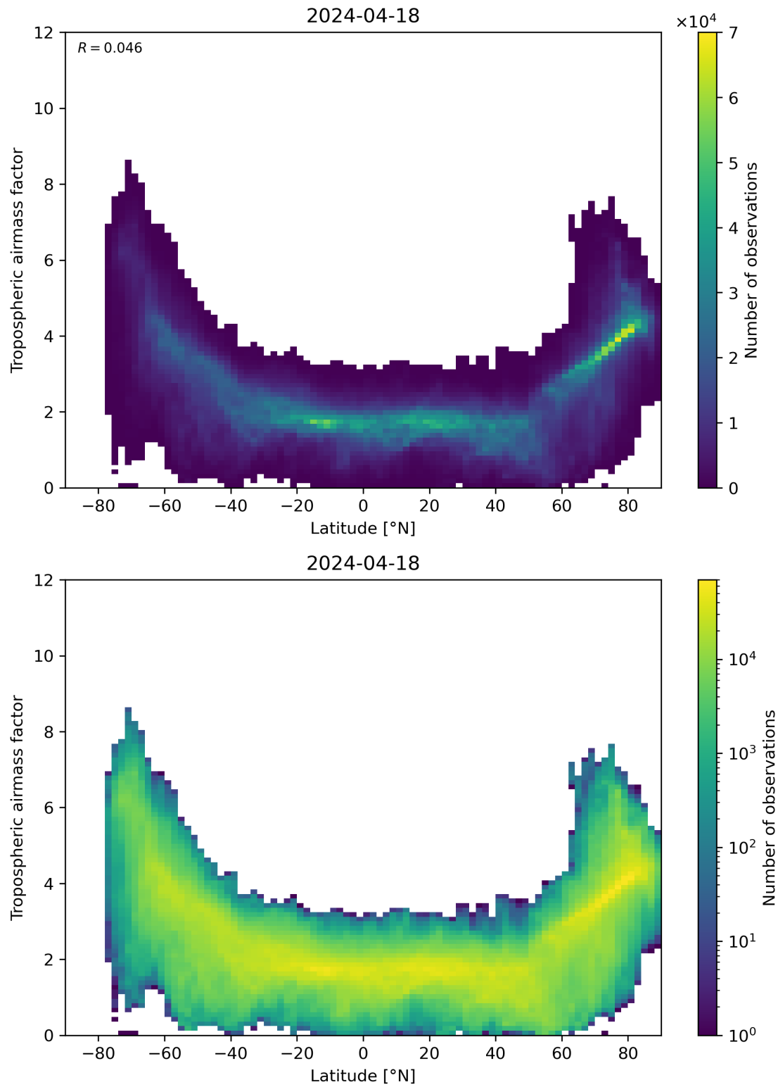
Figure 85: Scatter density plot of “Latitude” against “Tropospheric airmass factor” for 2024-04-17 to 2024-04-19.
