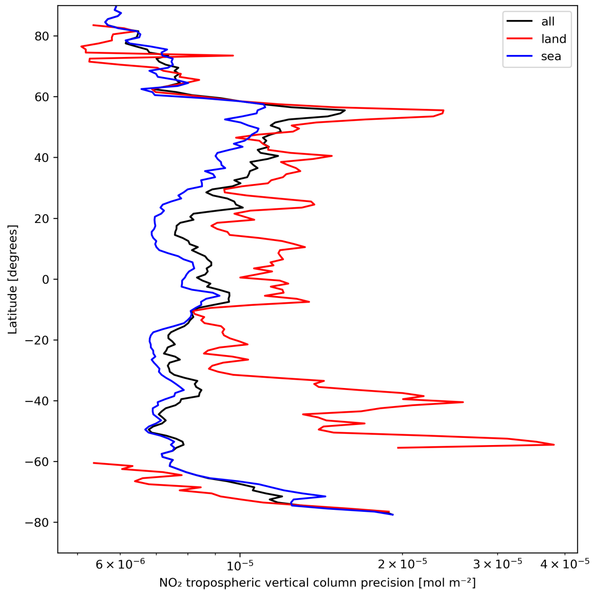
Figure 13: Zonal average of “NO 2 tropospheric vertical column precision” for 2024-04-17 to 2024-04-19.
