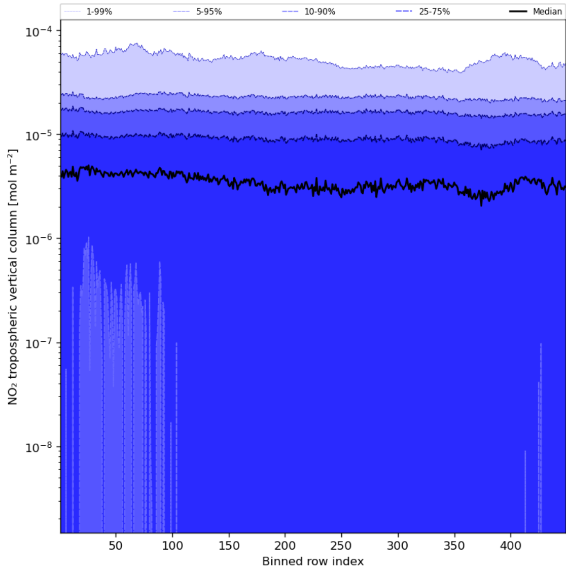
Figure 46: Along track statistics of “NO 2 tropospheric vertical column” for 2024-04-17 to 2024-04-19
