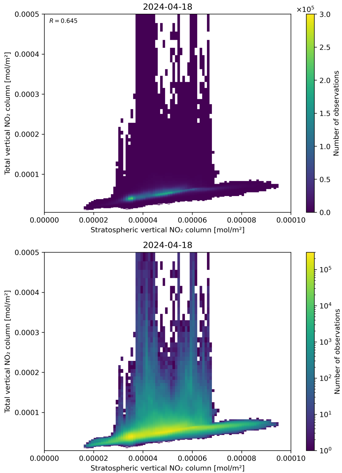
Figure 100: Scatter density plot of “Stratospheric vertical NO 2 column” against “Total vertical NO 2 column” for 2024-04-17 to 2024-04-19.
