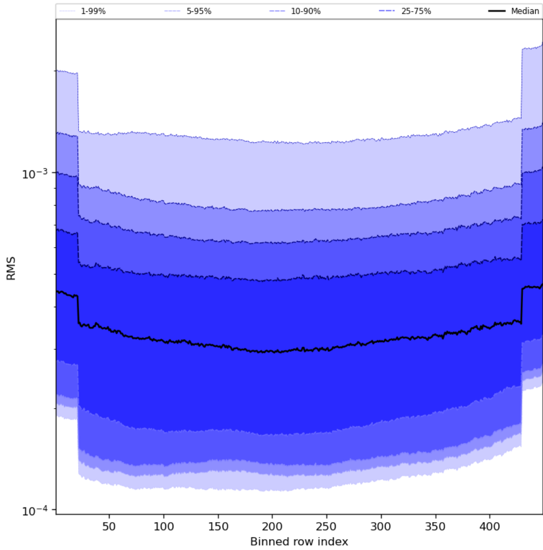
Figure 60: Along track statistics of “RMS” for 2024-04-17 to 2024-04-19
