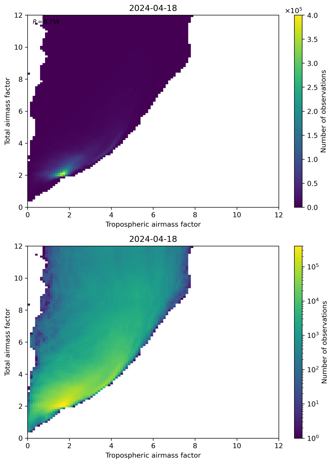
Figure 72: Scatter density plot of “Tropospheric airmass factor” against “Total airmass factor” for 2024-04-17 to 2024-04-19.
