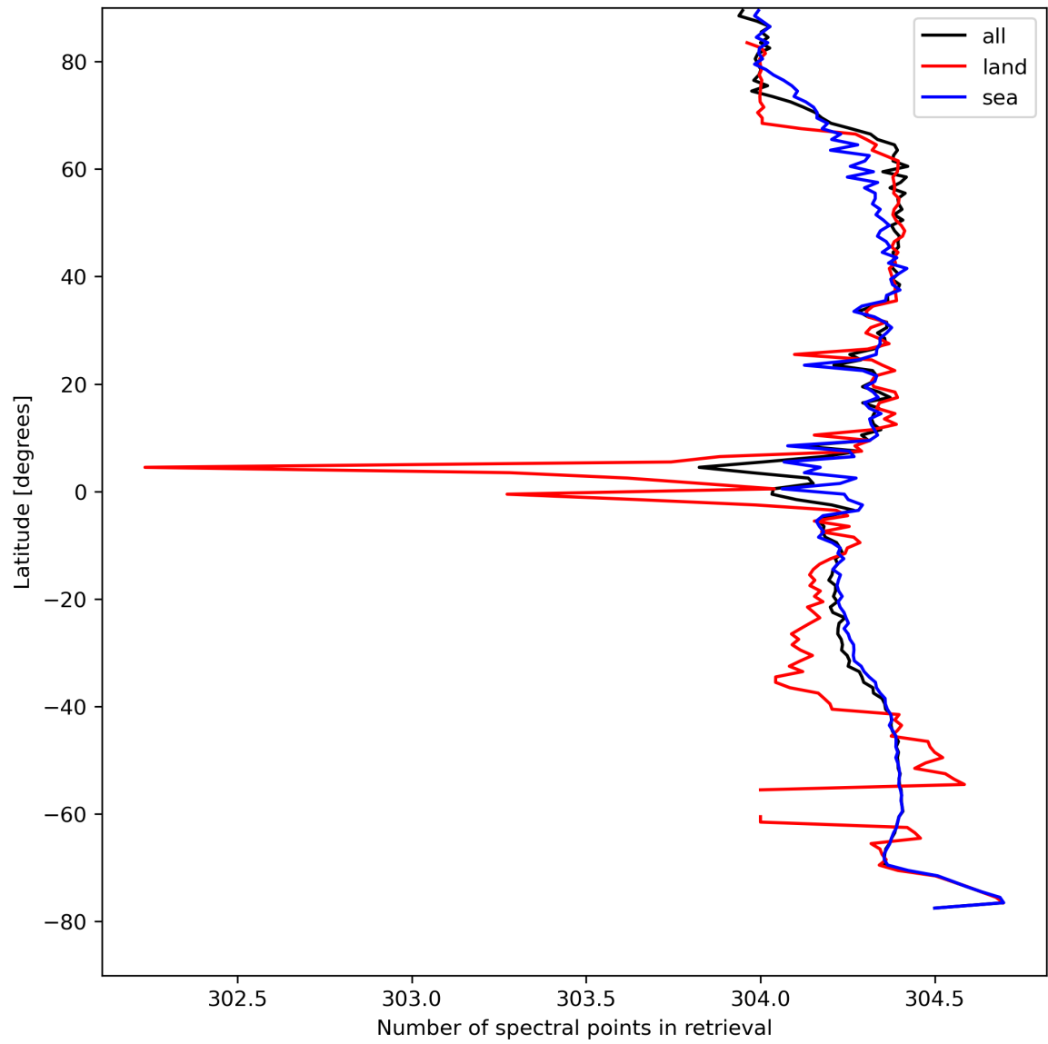
Figure 16: Zonal average of “Number of spectral points in retrieval” for 2024-04-17 to 2024-04-19.
