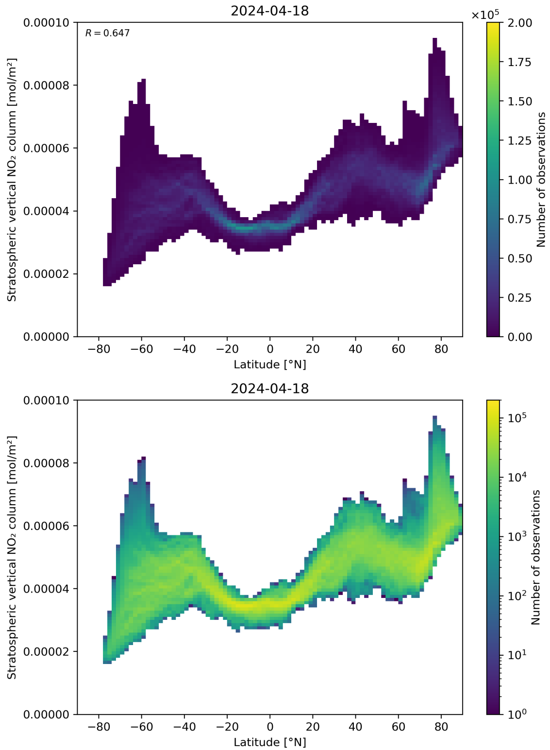
Figure 87: Scatter density plot of “Latitude” against “Stratospheric vertical NO 2 column” for 2024-04-17 to 2024-04-19.
