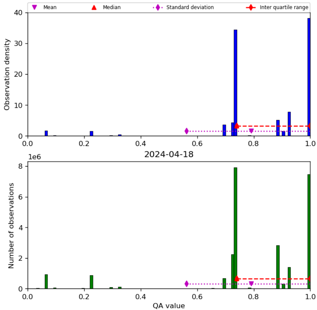
Figure 28: Histogram of “QA value” for 2024-04-17 to 2024-04-19
