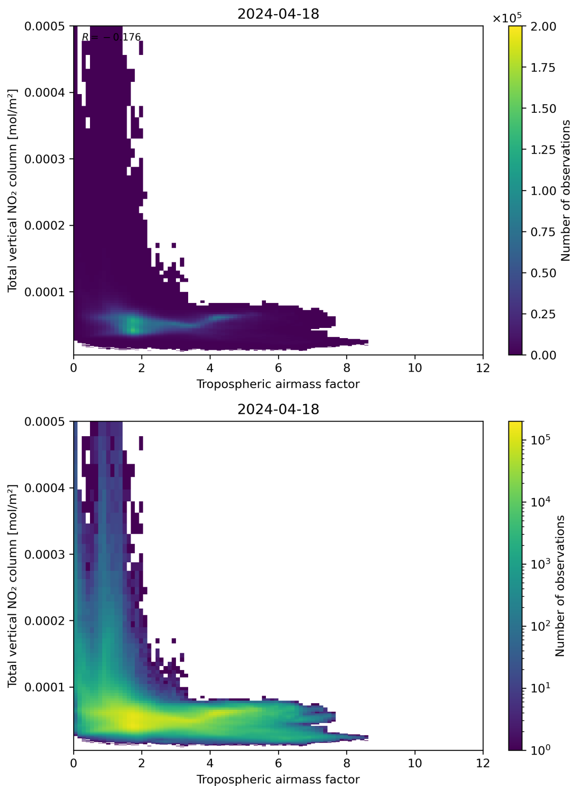
Figure 77: Scatter density plot of “Tropospheric airmass factor” against “Total vertical NO 2 column” for 2024-04-17 to 2024-04-19.
