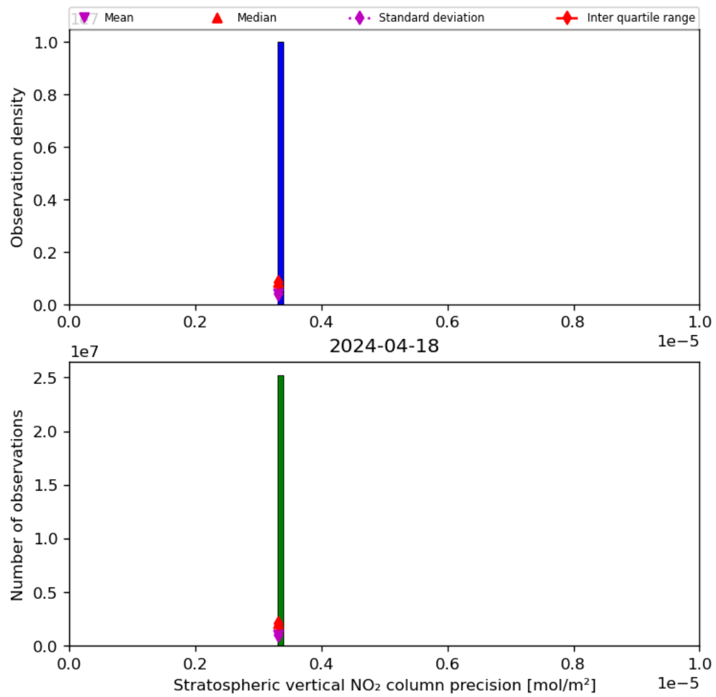
Figure 37: Histogram of “Stratospheric vertical NO 2 column precision” for 2024-04-17 to 2024-04-19
