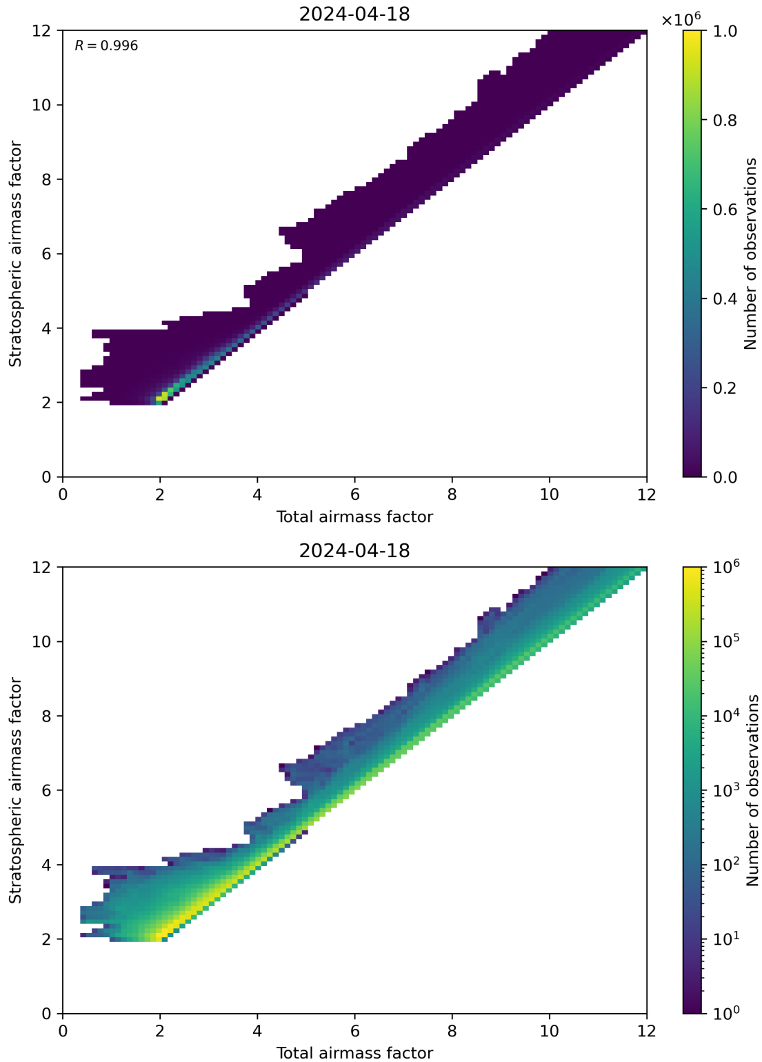
Figure 62: Scatter density plot of “Total airmass factor” against “Stratospheric airmass factor” for 2024-04-17 to 2024-04-19.
