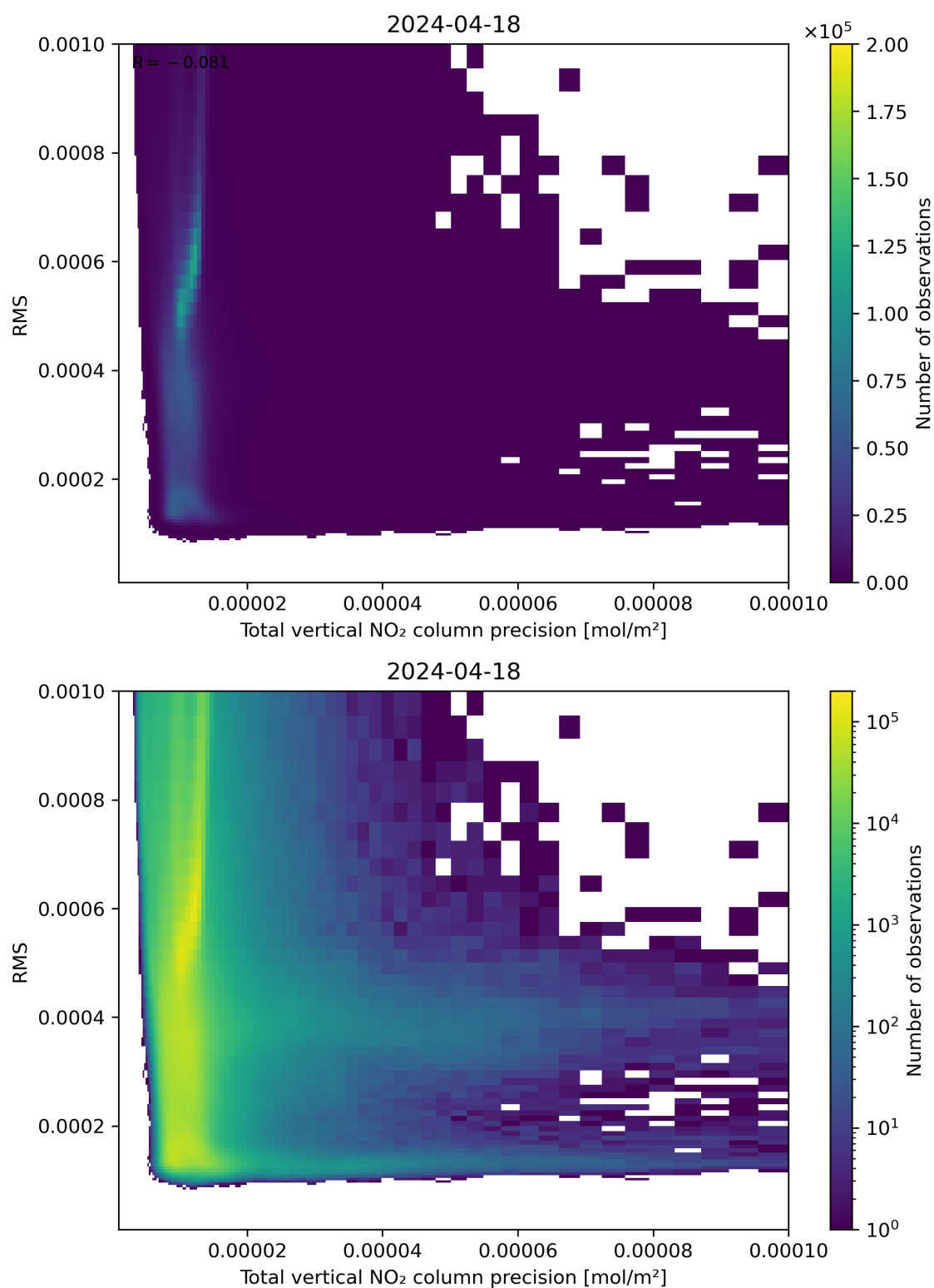
Figure 119: Scatter density plot of “Total vertical NO 2 column precision” against “RMS” for 2024-04-17 to 2024-04-19.
