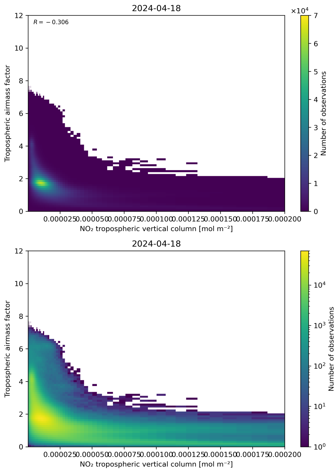
Figure 123: Scatter density plot of “NO 2 tropospheric vertical column” against “Tropospheric air mass factor” for 2024-04-17 to 2024-04-19.
