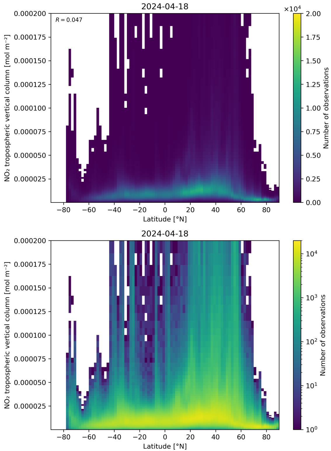
Figure 92: Scatter density plot of “Latitude” against “NO 2 tropospheric vertical column” for 2024-04-17 to 2024-04-19.
