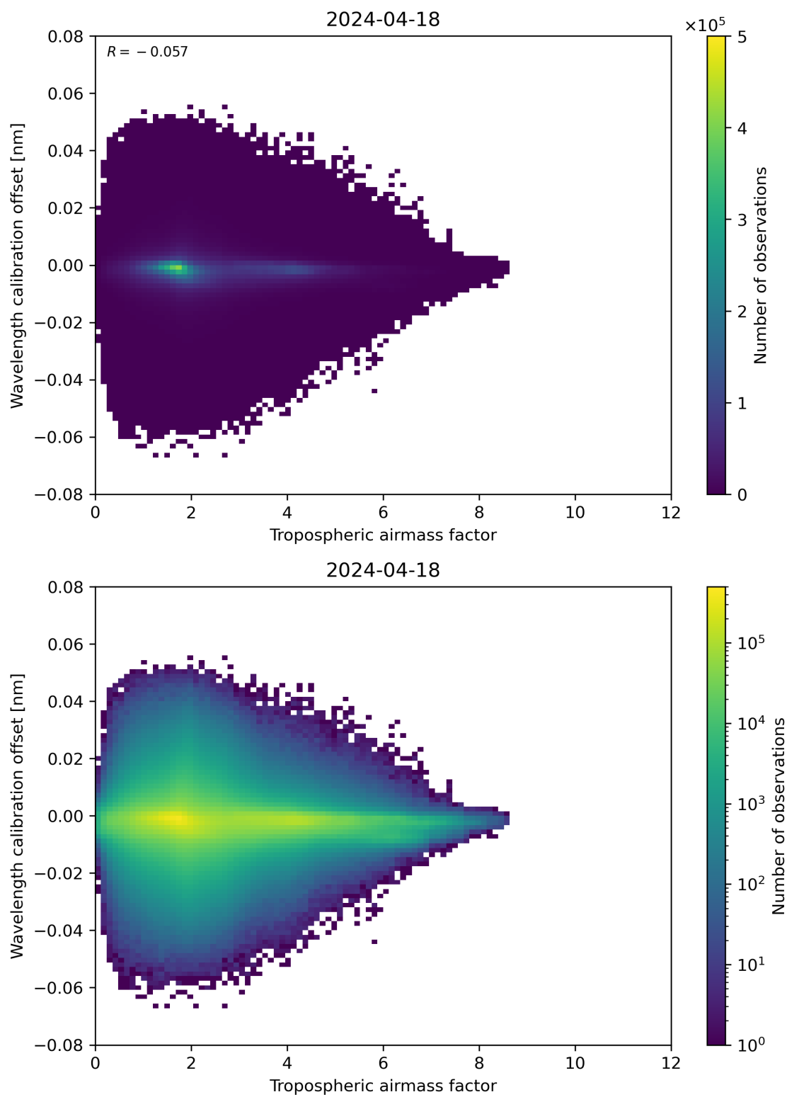
Figure 80: Scatter density plot of “Tropospheric air mass factor” against “Wavelength calibration offset” for 2024-04-17 to 2024-04-19.
