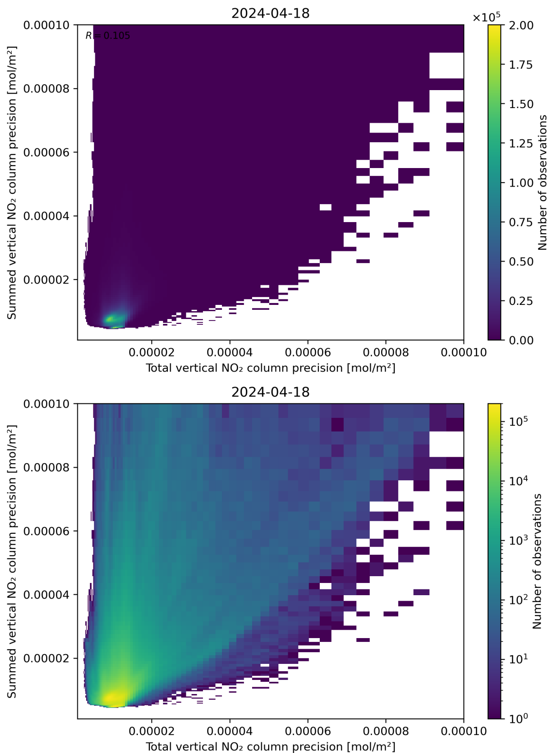
Figure 118: Scatter density plot of “Total vertical NO 2 column precision” against “Summed vertical NO 2 column precision” for 2024-04-17 to 2024-04-19.
