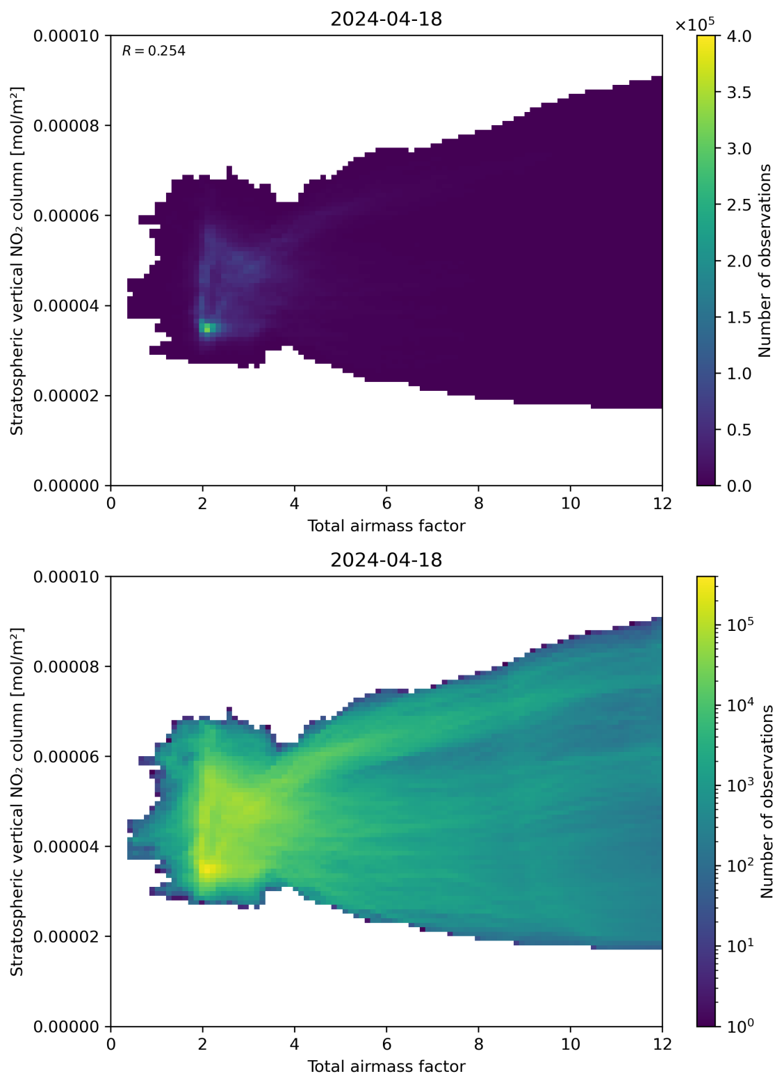
Figure 64: Scatter density plot of “Total airmass factor” against “Stratospheric vertical \text{NO}_2 column” for 2024-04-17 to 2024-04-19.
