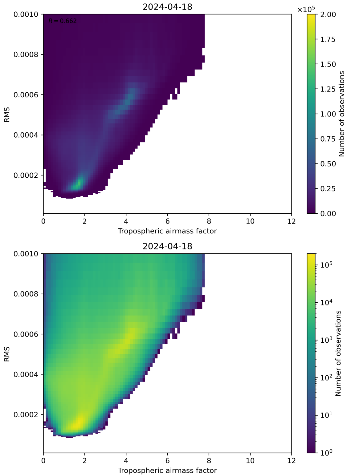
Figure 79: Scatter density plot of “Tropospheric airmass factor” against “RMS” for 2024-04-17 to 2024-04-19.
