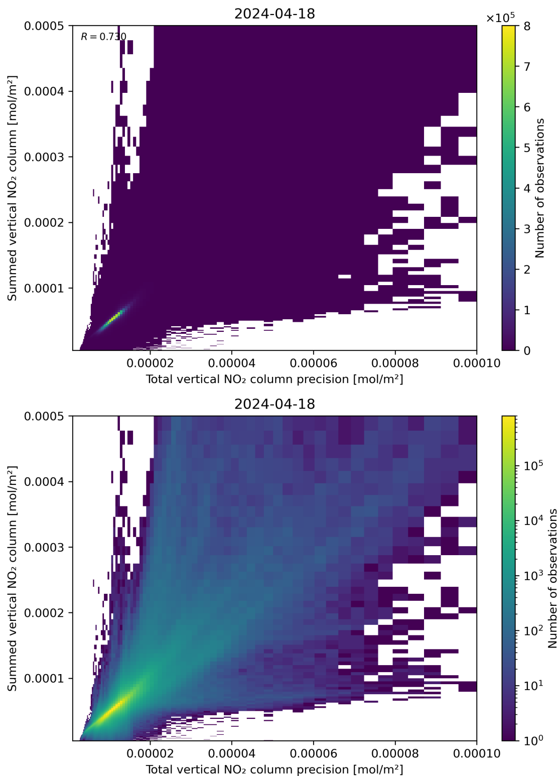
Figure 117: Scatter density plot of “Total vertical NO 2 column precision” against “Summed vertical NO 2 column” for 2024-04-17 to 2024-04-19.
