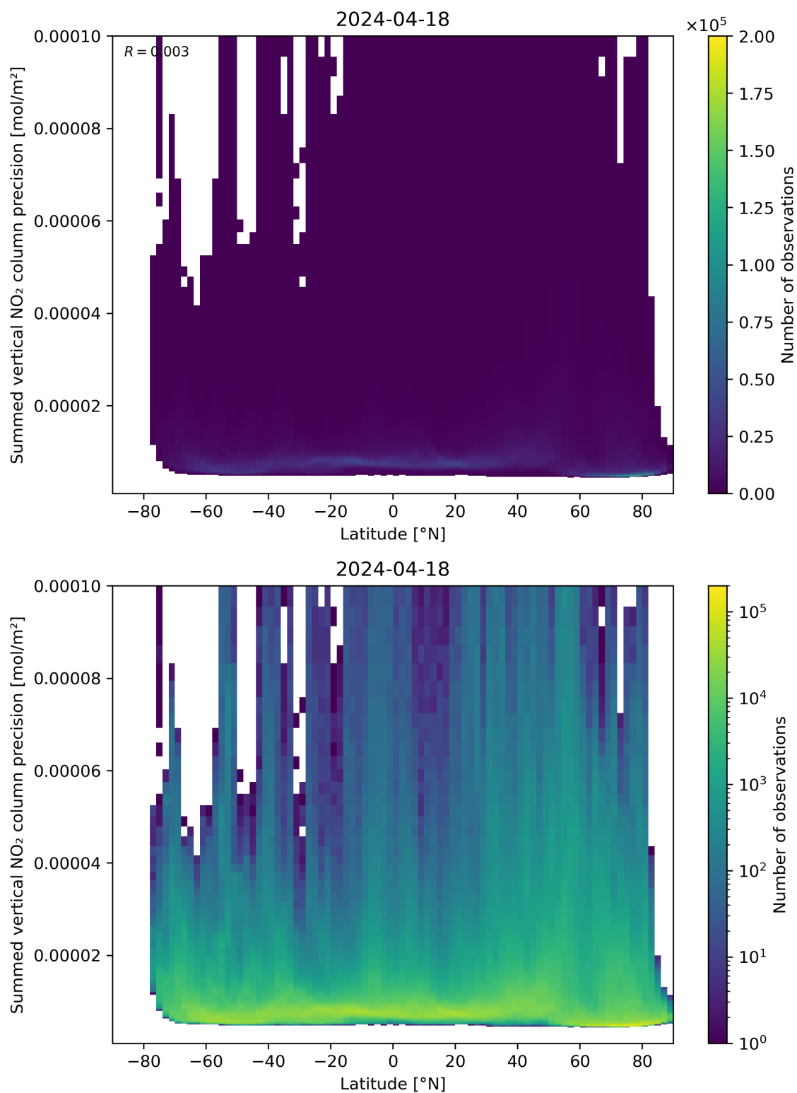
Figure 89: Scatter density plot of “Latitude” against “Summed vertical NO 2 column precision” for 2024-04-17 to 2024-04-19.
