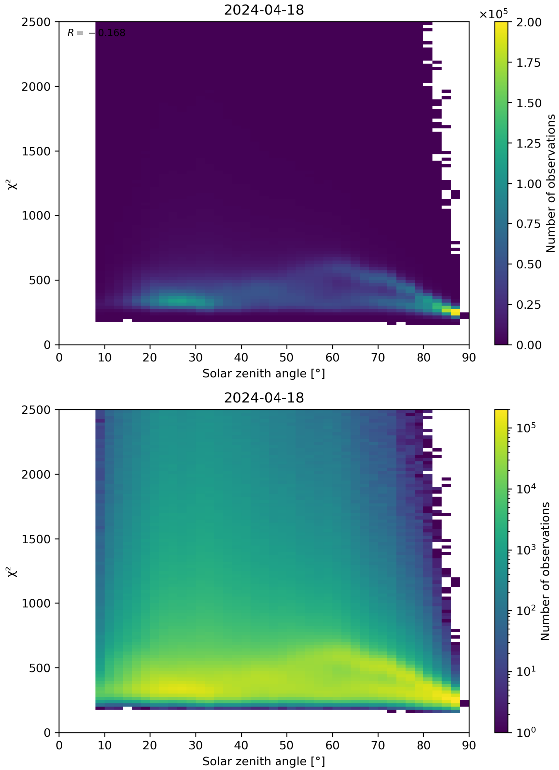
Figure 148: Scatter density plot of “Solar zenith angle” against “ \chi^2 ” for 2024-04-17 to 2024-04-19.
