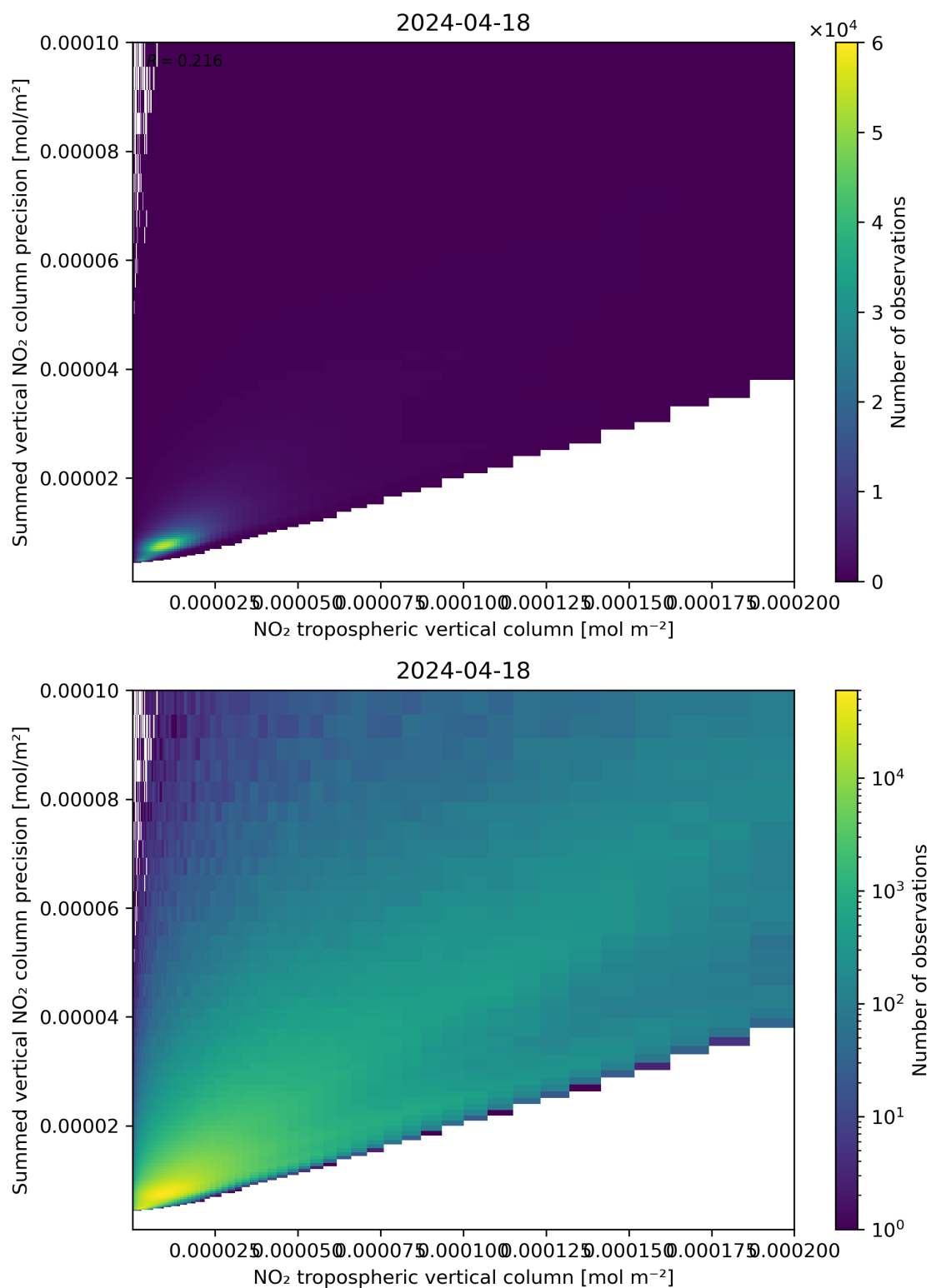
Figure 127: Scatter density plot of “NO 2 tropospheric vertical column” against “Summed vertical NO 2 column precision” for 2024-04-17 to 2024-04-19.
