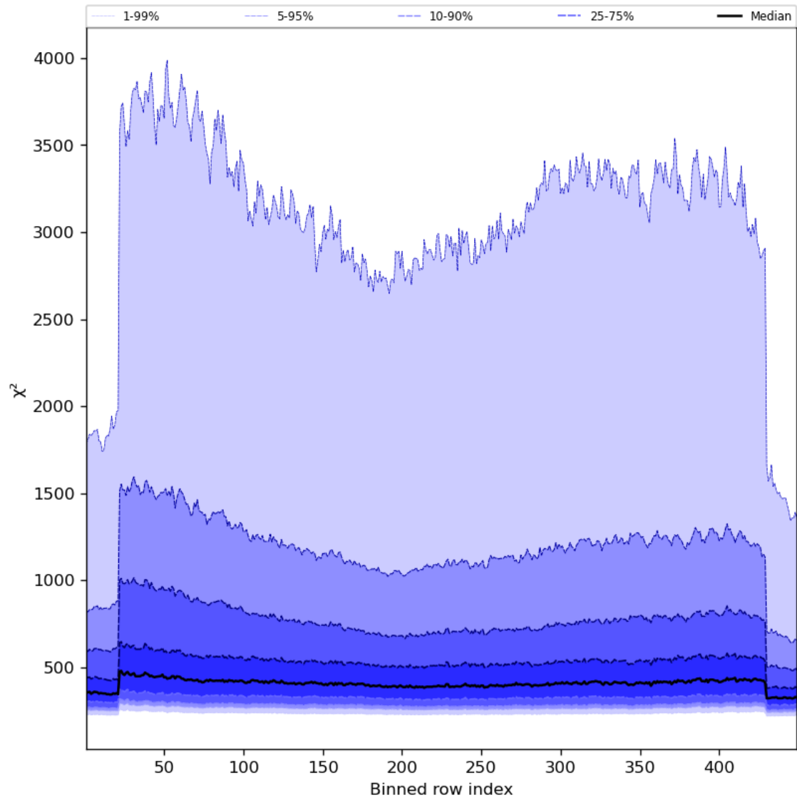
Figure 59: Along track statistics of “ \chi^2 ” for 2024-04-17 to 2024-04-19
