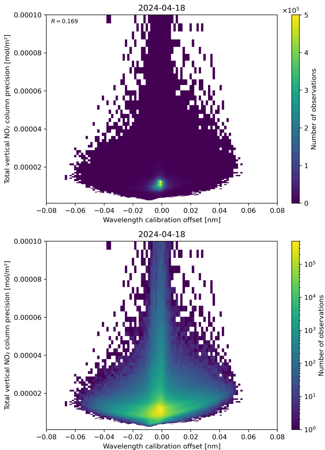
Figure 180: Scatter density plot of “Wavelength calibration offset” against “Total vertical NO 2 column precision” for 2024-04-17 to 2024-04-19.
