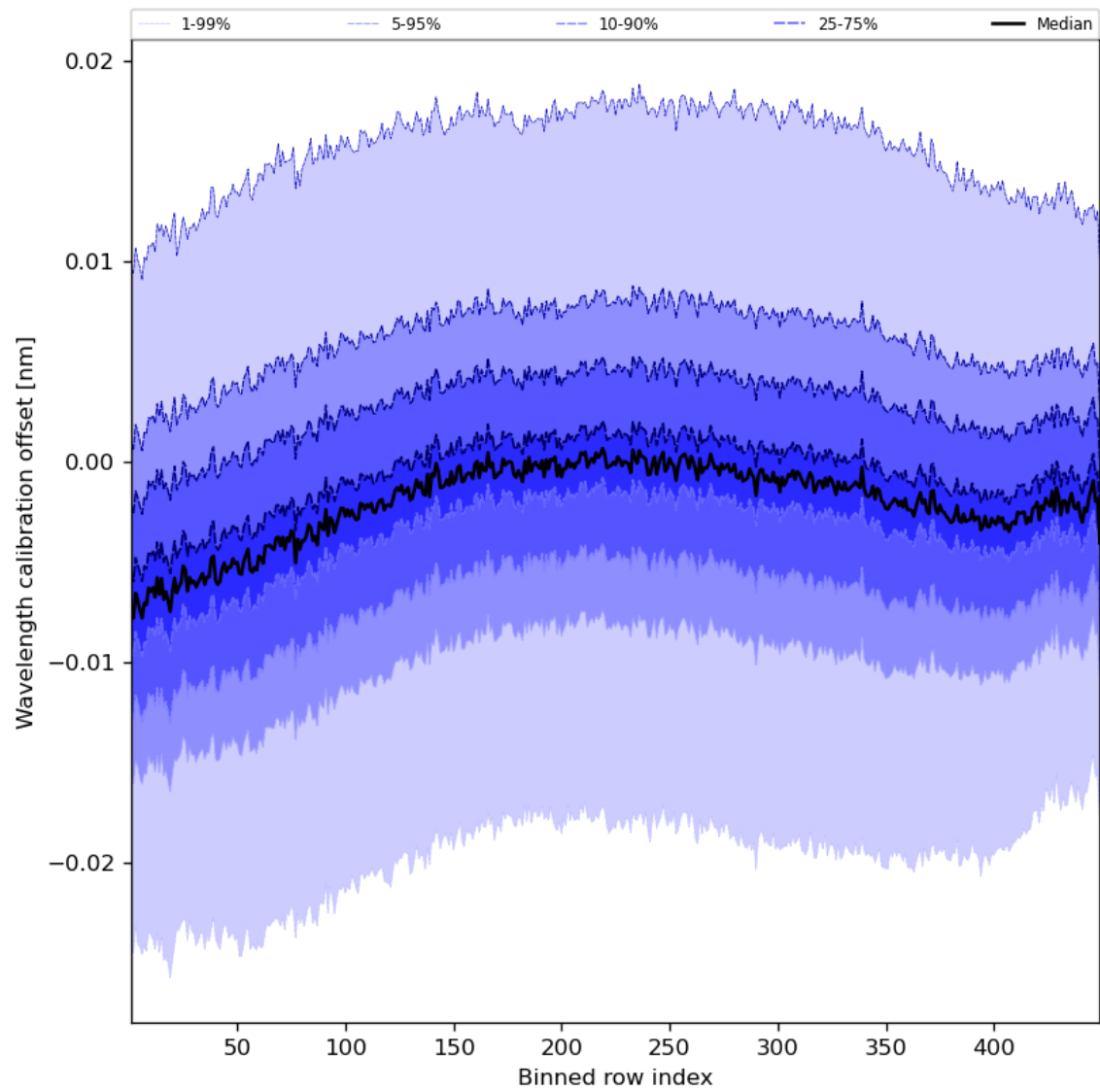
Figure 52: Along track statistics of “Wavelength calibration offset” for 2024-04-17 to 2024-04-19
