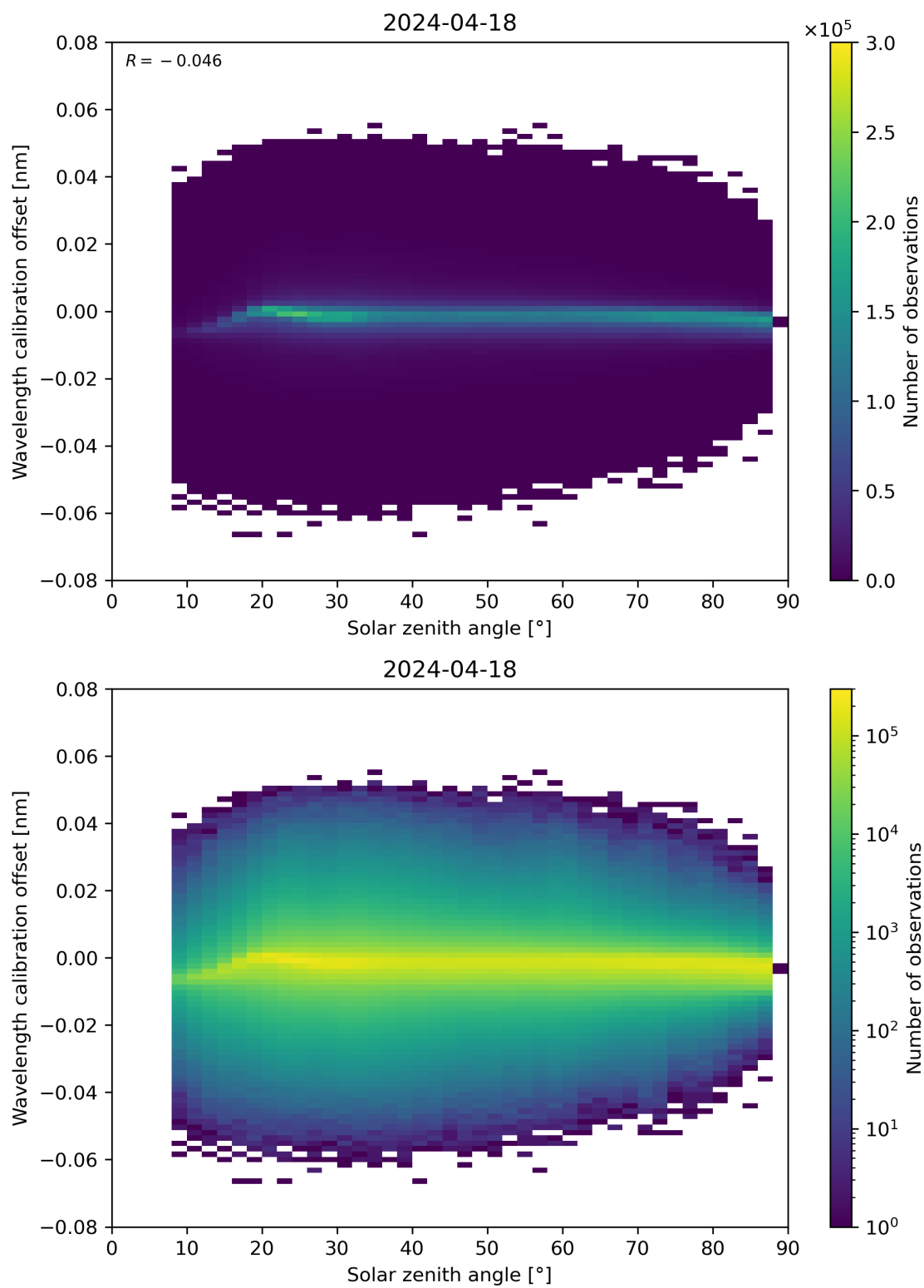
Figure 158: Scatter density plot of “Solar zenith angle” against “Wavelength calibration offset” for 2024-04-17 to 2024-04-19.
