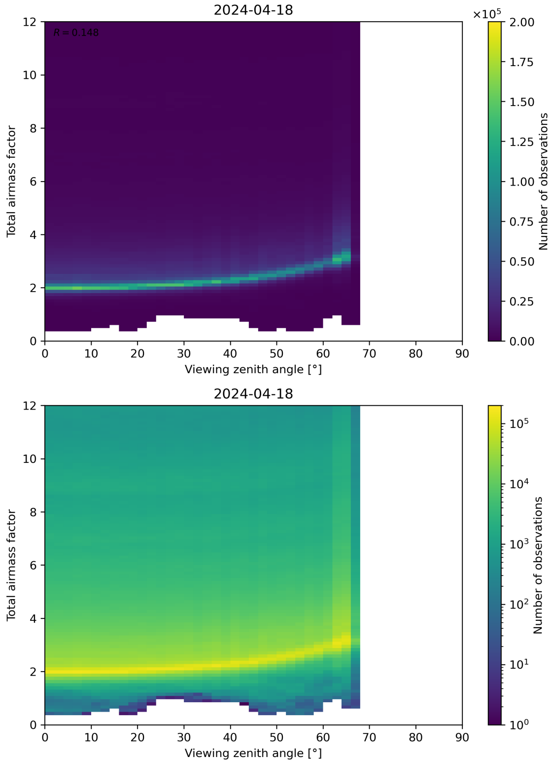
Figure 160: Scatter density plot of “Viewing zenith angle” against “Total airmass factor” for 2024-04-17 to 2024-04-19.
