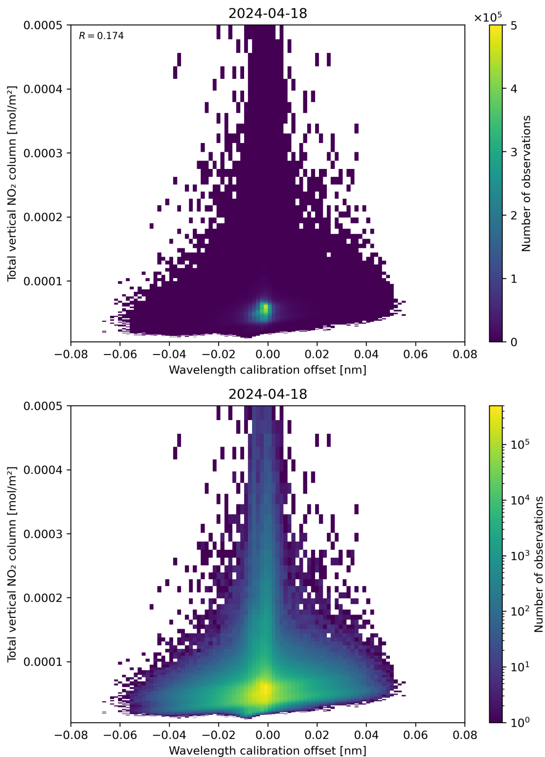
Figure 179: Scatter density plot of “Wavelength calibration offset” against “Total vertical NO 2 column” for 2024-04-17 to 2024-04-19.
