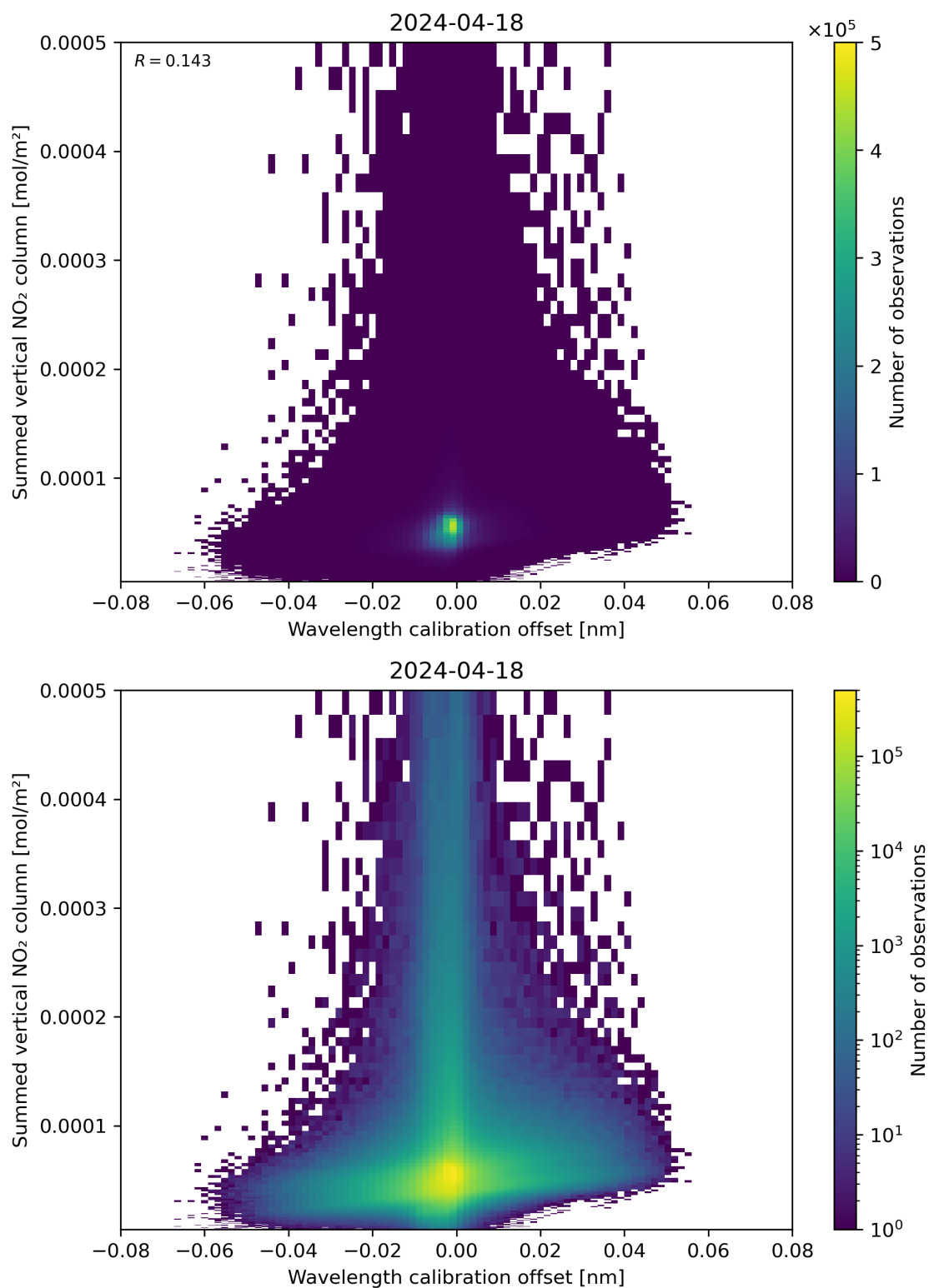
Figure 177: Scatter density plot of “Wavelength calibration offset” against “Summed vertical NO 2 column” for 2024-04-17 to 2024-04-19.
