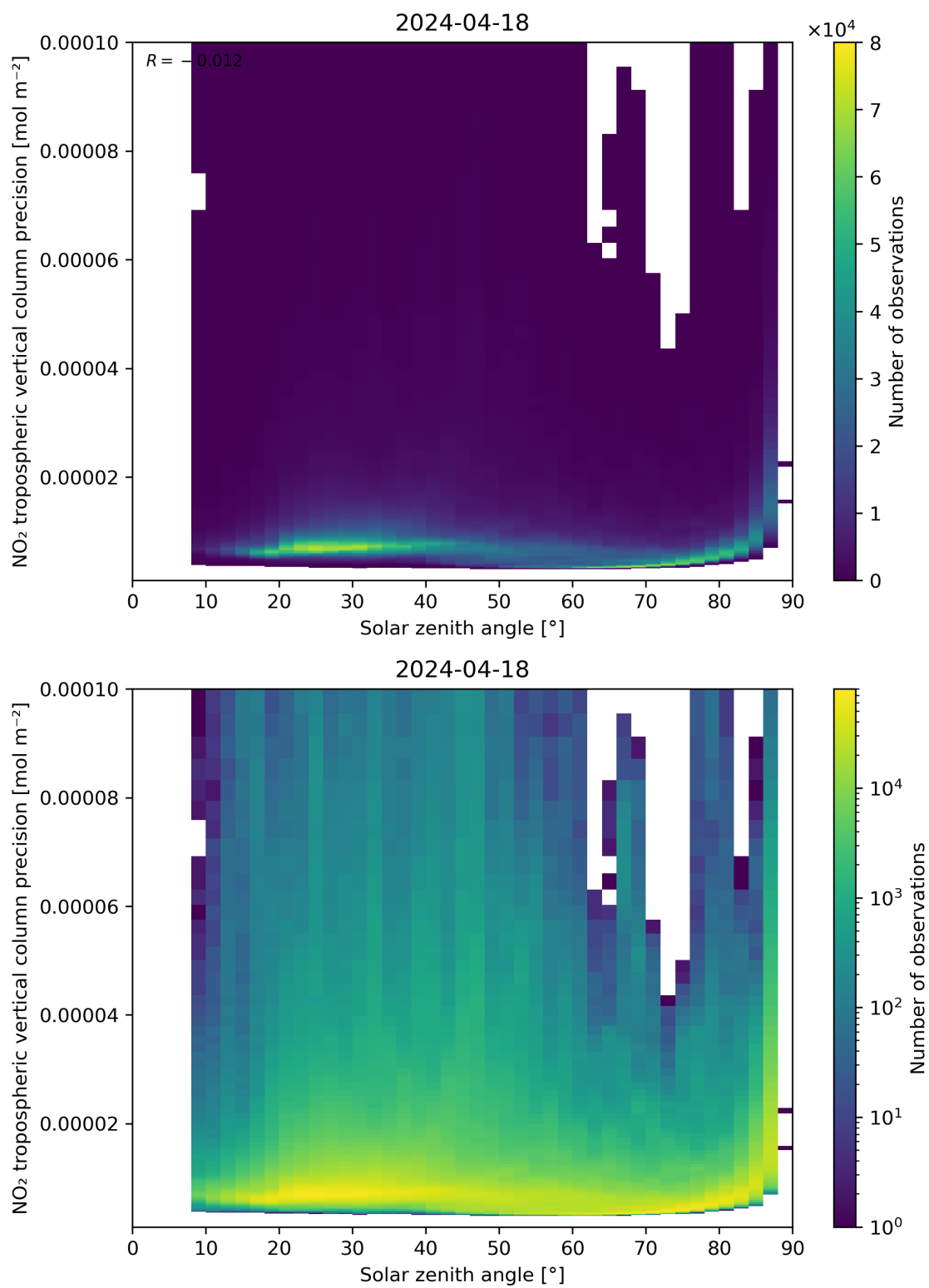
Figure 156: Scatter density plot of “Solar zenith angle” against “NO 2 tropospheric vertical column precision” for 2024-04-17 to 2024-04-19.
