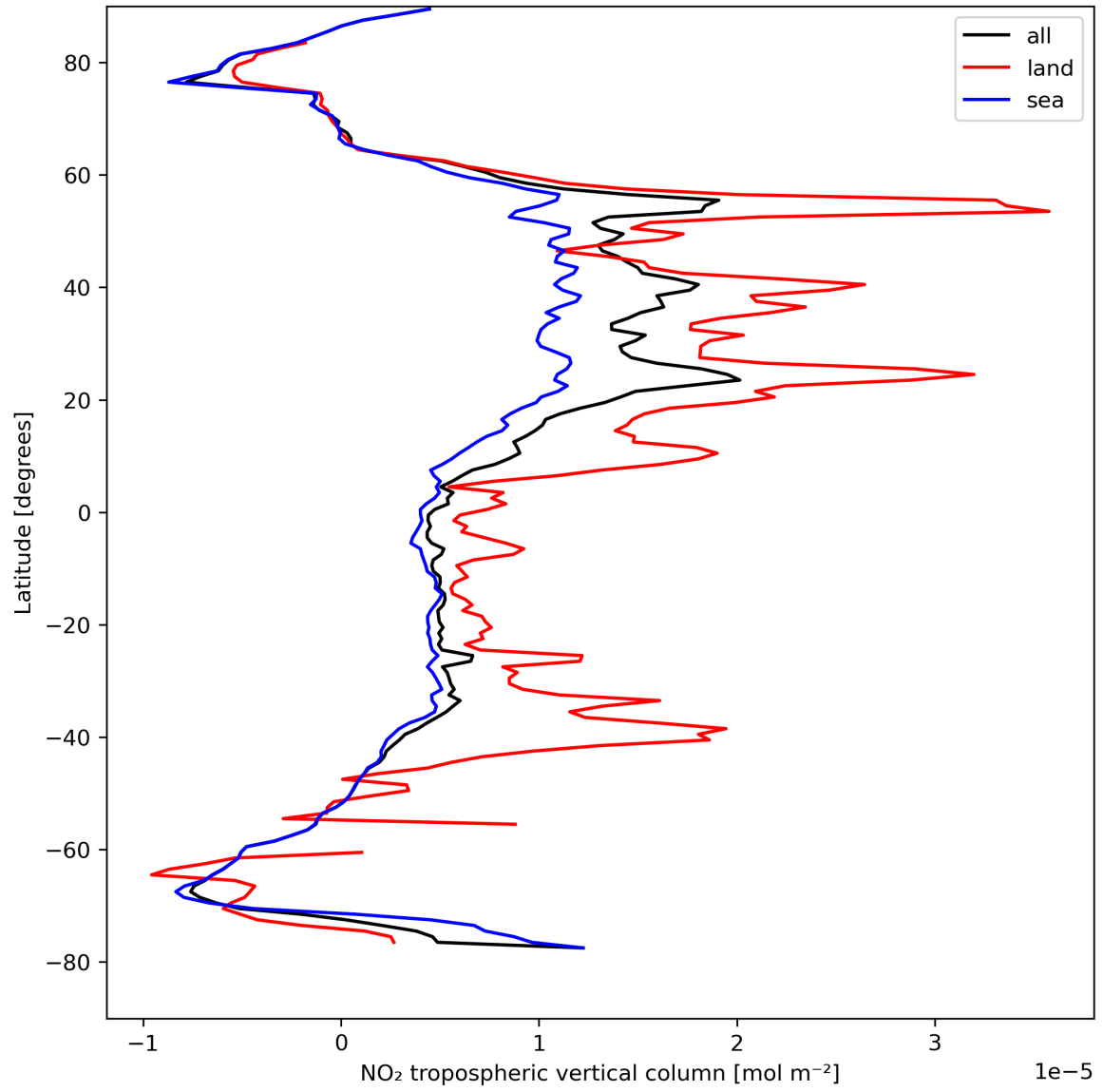
Figure 12: Zonal average of “NO 2 tropospheric vertical column” for 2024-04-17 to 2024-04-19.
