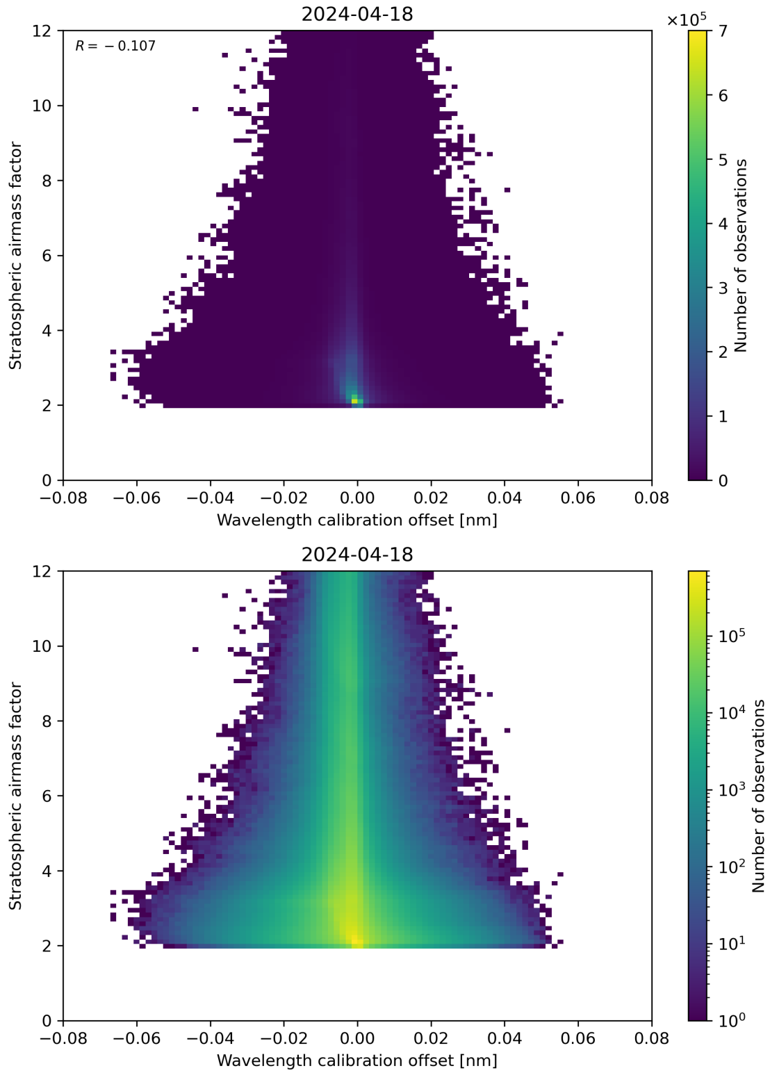
Figure 174: Scatter density plot of “Wavelength calibration offset” against “Stratospheric airmass factor” for 2024-04-17 to 2024-04-19.
