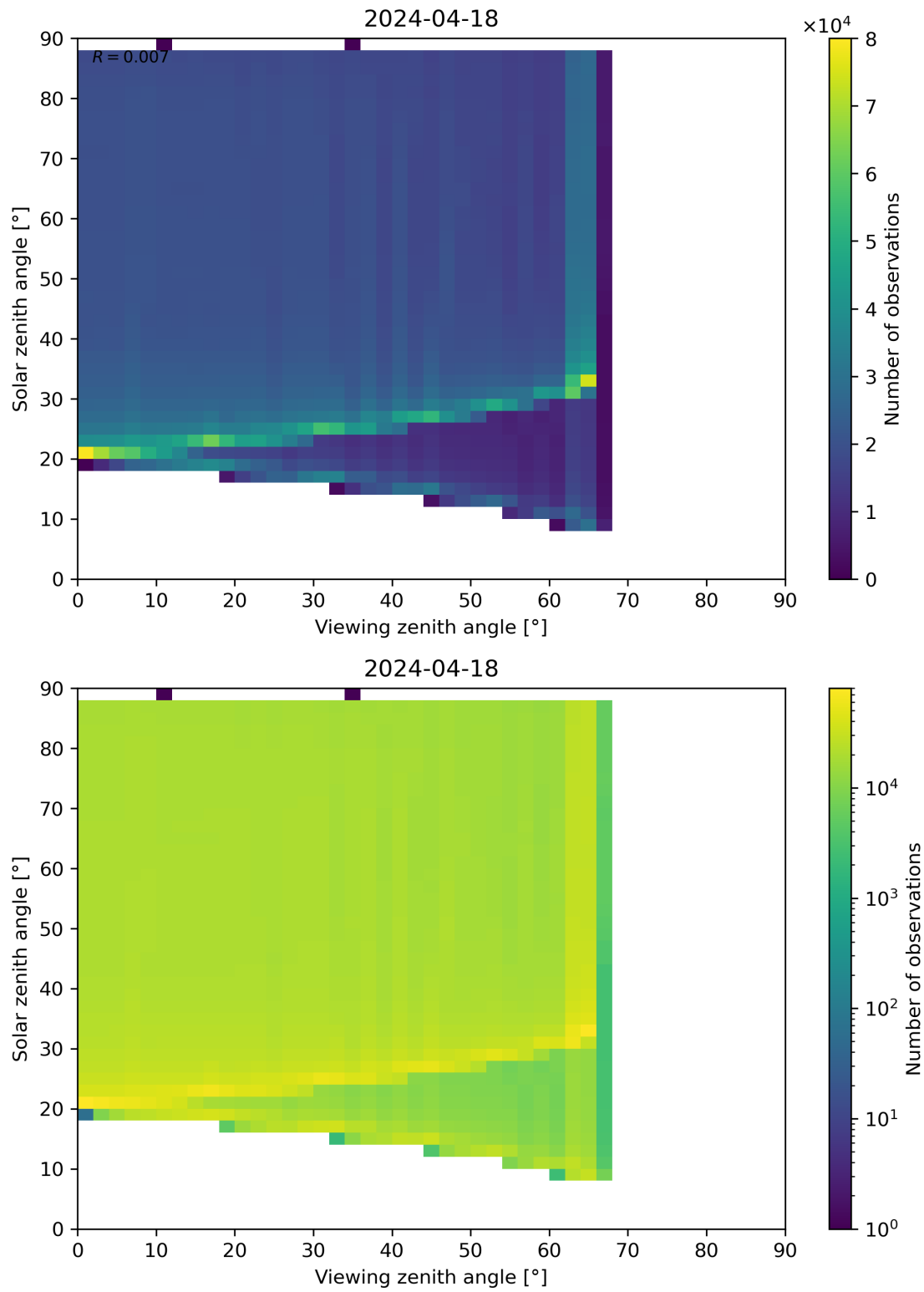
Figure 172: Scatter density plot of “Viewing zenith angle” against “Solar zenith angle” for 2024-04-17 to 2024-04-19.
