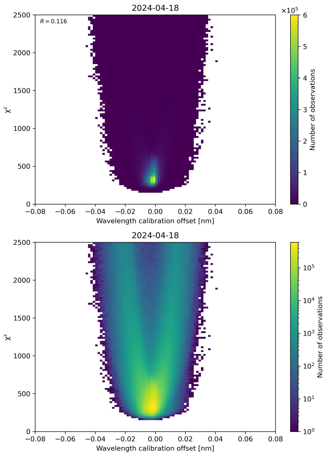
Figure 175: Scatter density plot of “Wavelength calibration offset” against “ \chi^2 ” for 2024-04-17 to 2024-04-19.
