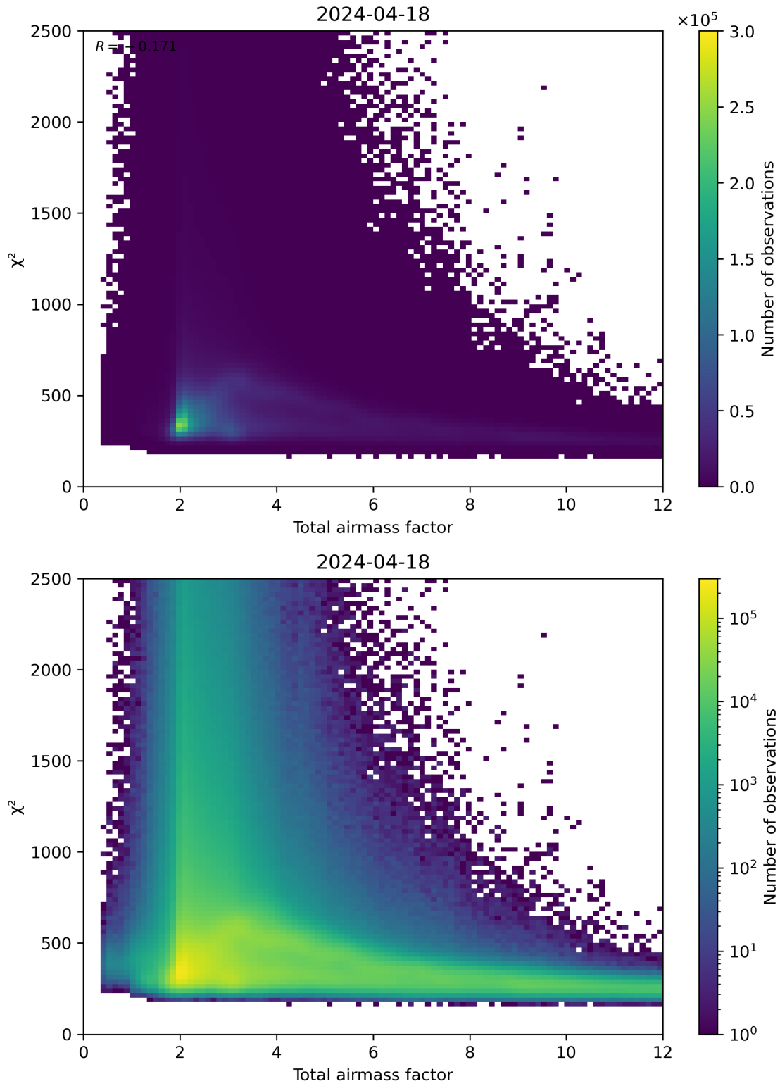
Figure 63: Scatter density plot of “Total airmass factor” against “ \chi^2 ” for 2024-04-17 to 2024-04-19.
