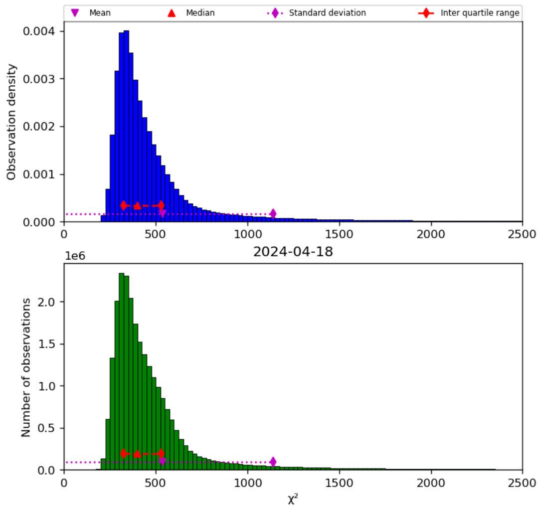
Figure 42: Histogram of “ \chi^2 ” for 2024-04-17 to 2024-04-19
