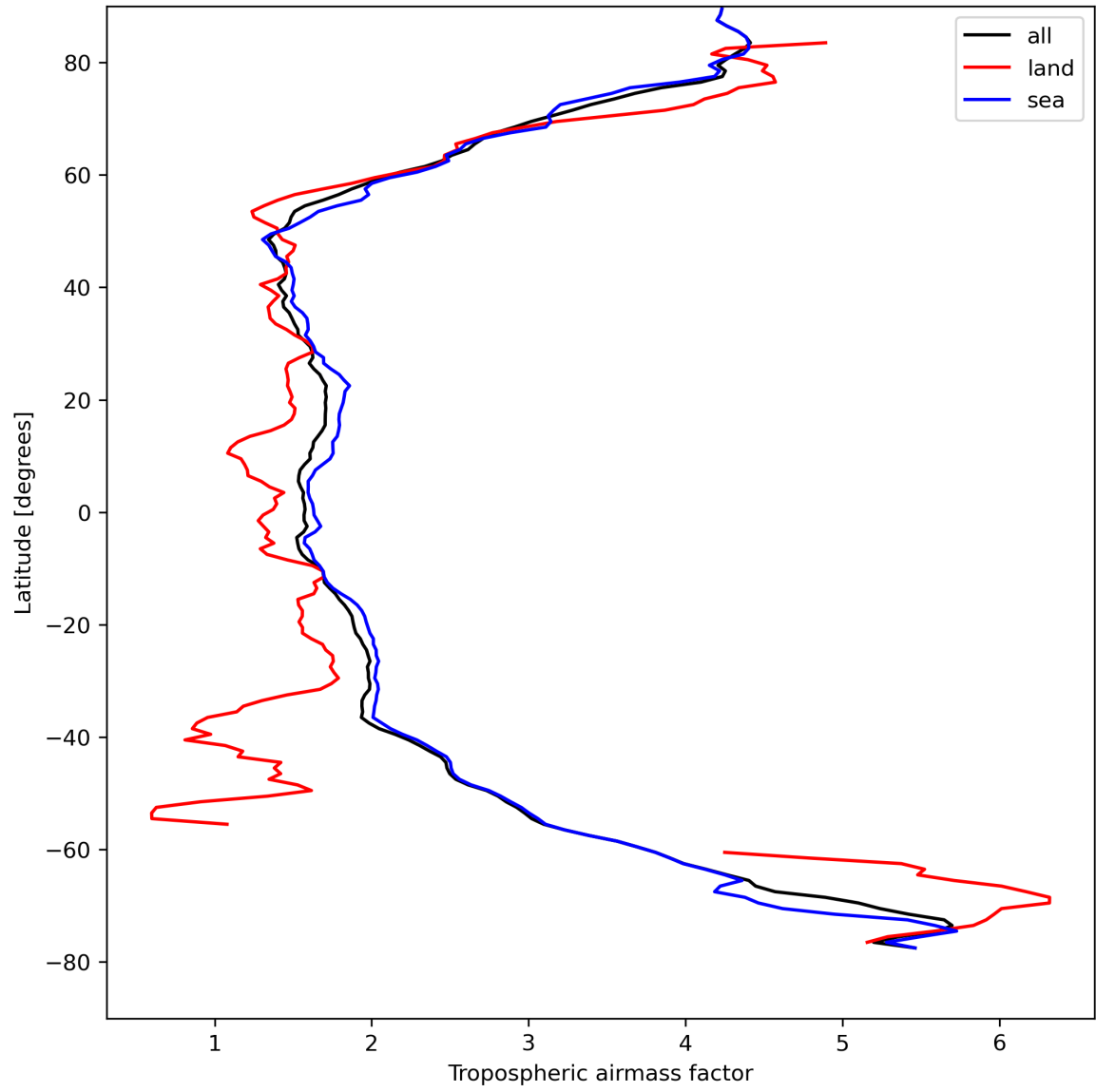
Figure 14: Zonal average of “Tropospheric airmass factor” for 2024-04-17 to 2024-04-19.
