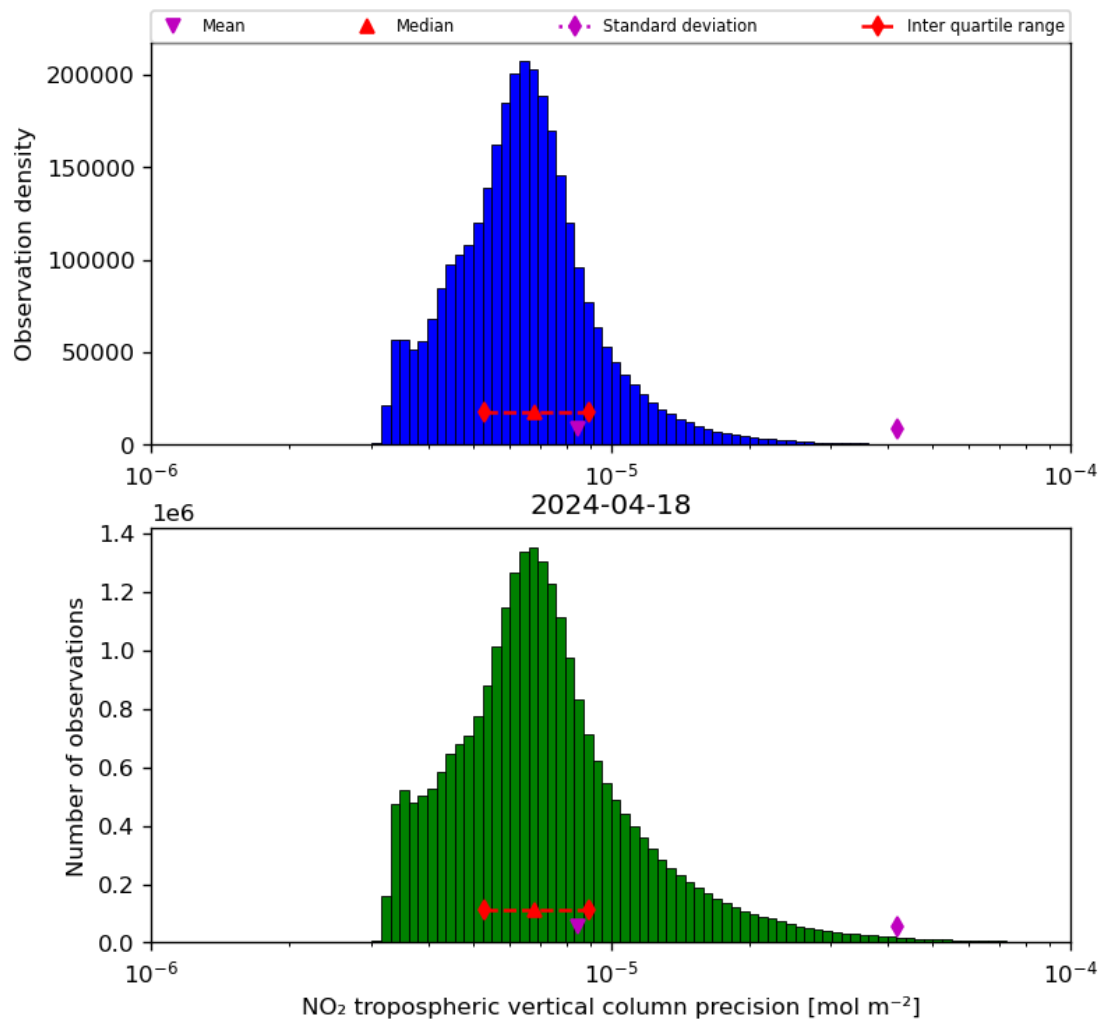
Figure 30: Histogram of “NO 2 tropospheric vertical column precision” for 2024-04-17 to 2024-04-19
