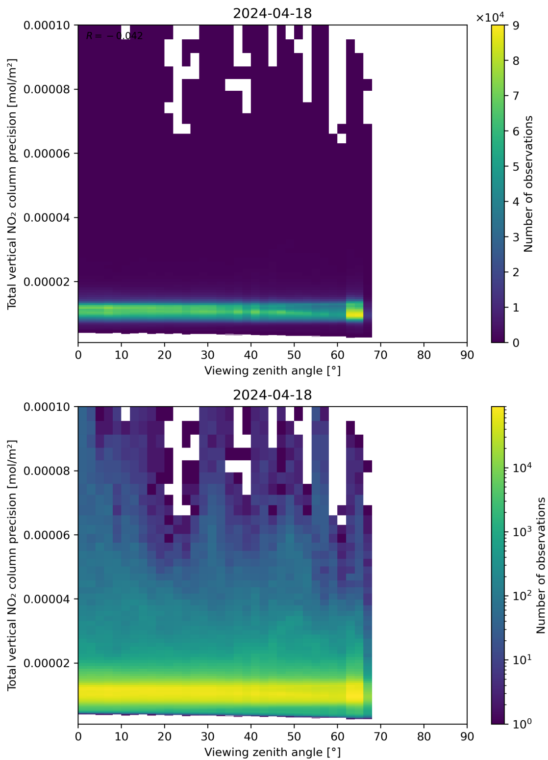
Figure 168: Scatter density plot of “Viewing zenith angle” against “Total vertical NO 2 column precision” for 2024-04-17 to 2024-04-19.
