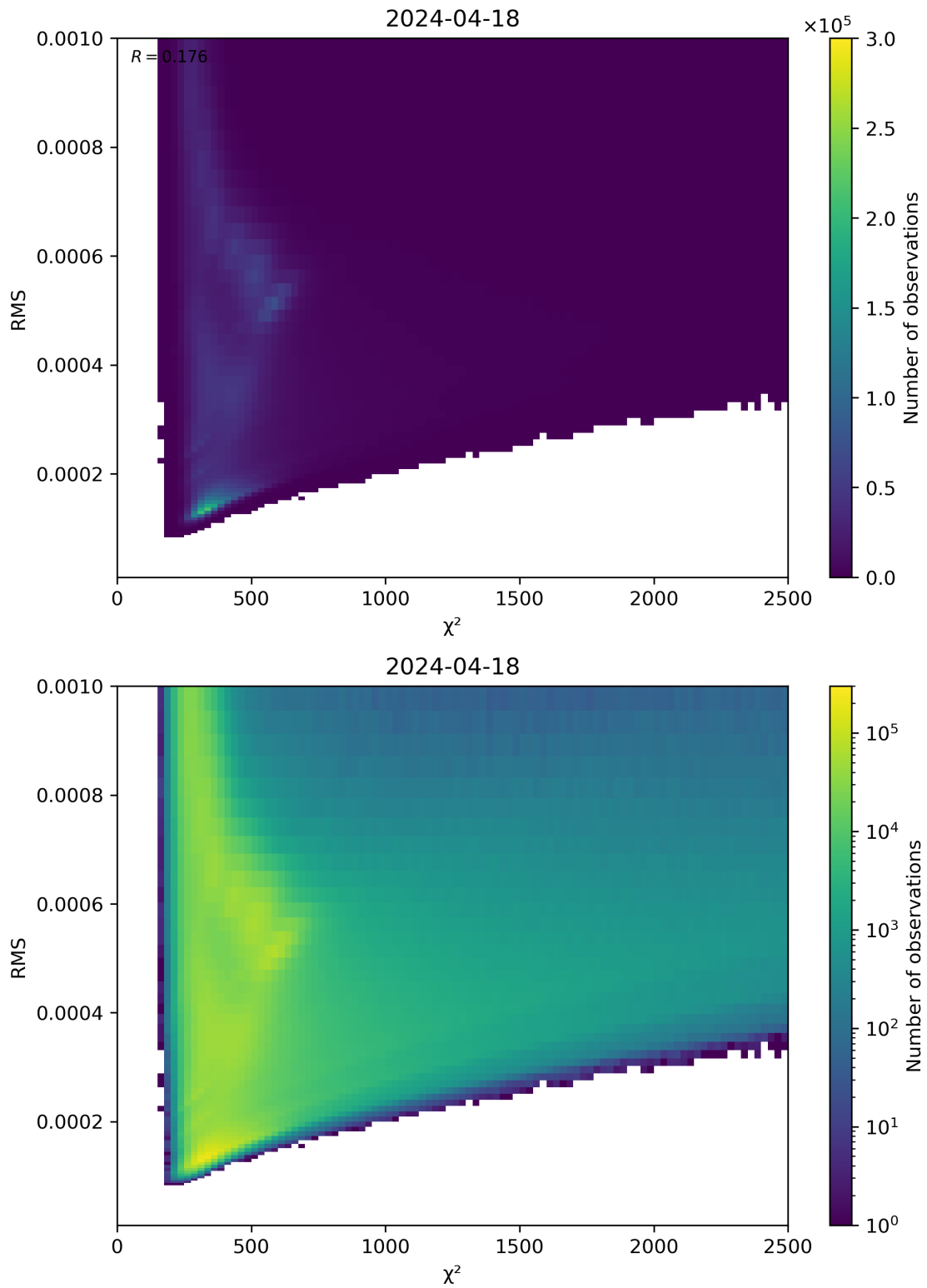
Figure 82: Scatter density plot of “ \chi^2 ” against “RMS” for 2024-04-17 to 2024-04-19.
