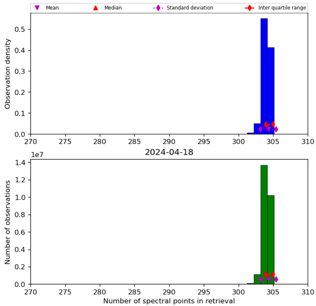
Figure 33: Histogram of “Number of spectral points in retrieval” for 2024-04-17 to 2024-04-19
