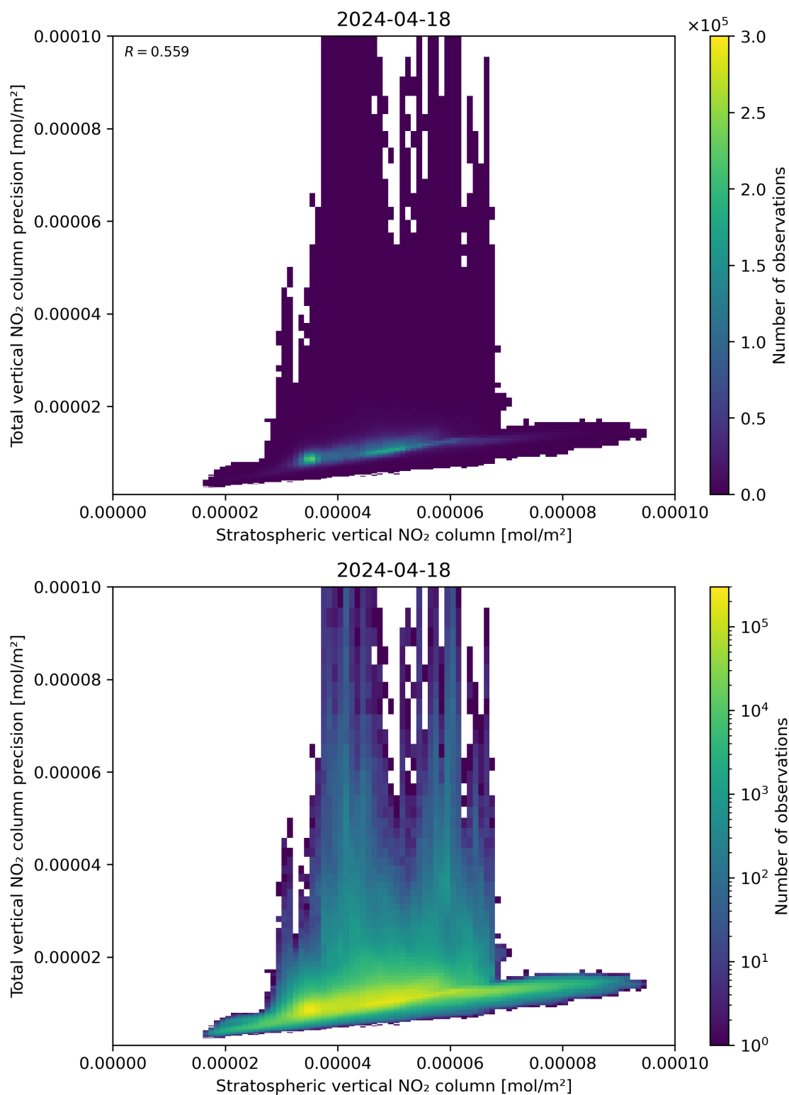
Figure 101: Scatter density plot of “Stratospheric vertical NO 2 column” against “Total vertical NO 2 column precision” for 2024-04-17 to 2024-04-19.
