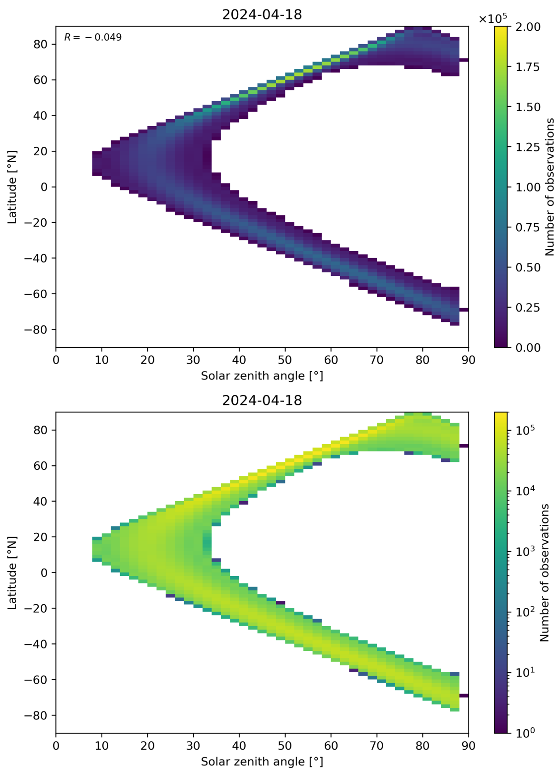
Figure 149: Scatter density plot of “Solar zenith angle” against “Latitude” for 2024-04-17 to 2024-04-19.
