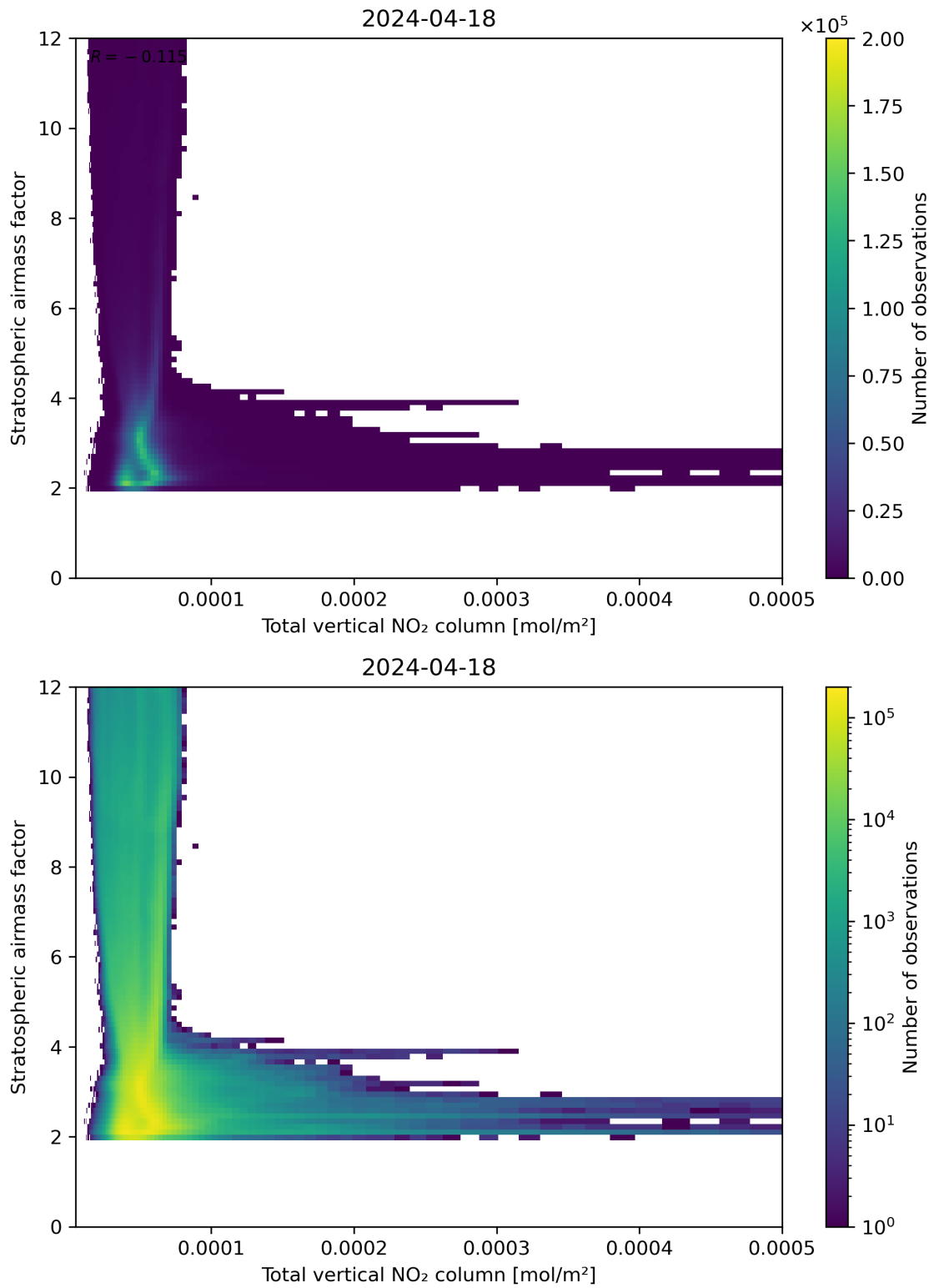
Figure 110: Scatter density plot of “Total vertical NO 2 column” against “Stratospheric airmass factor” for 2024-04-17 to 2024-04-19.
