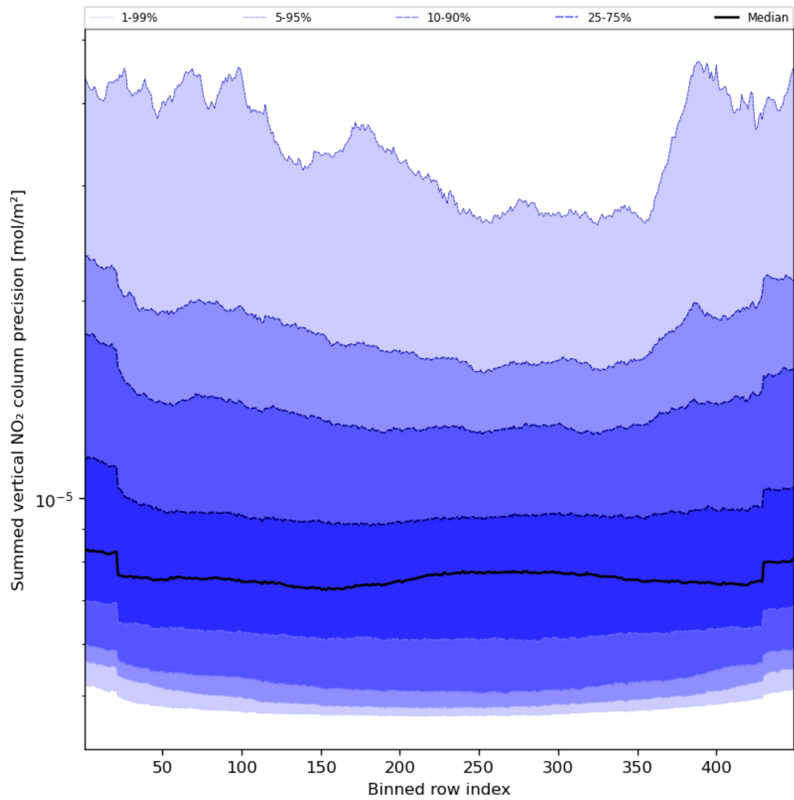
Figure 58: Along track statistics of “Summed vertical NO 2 column precision” for 2024-04-17 to 2024-04-19
