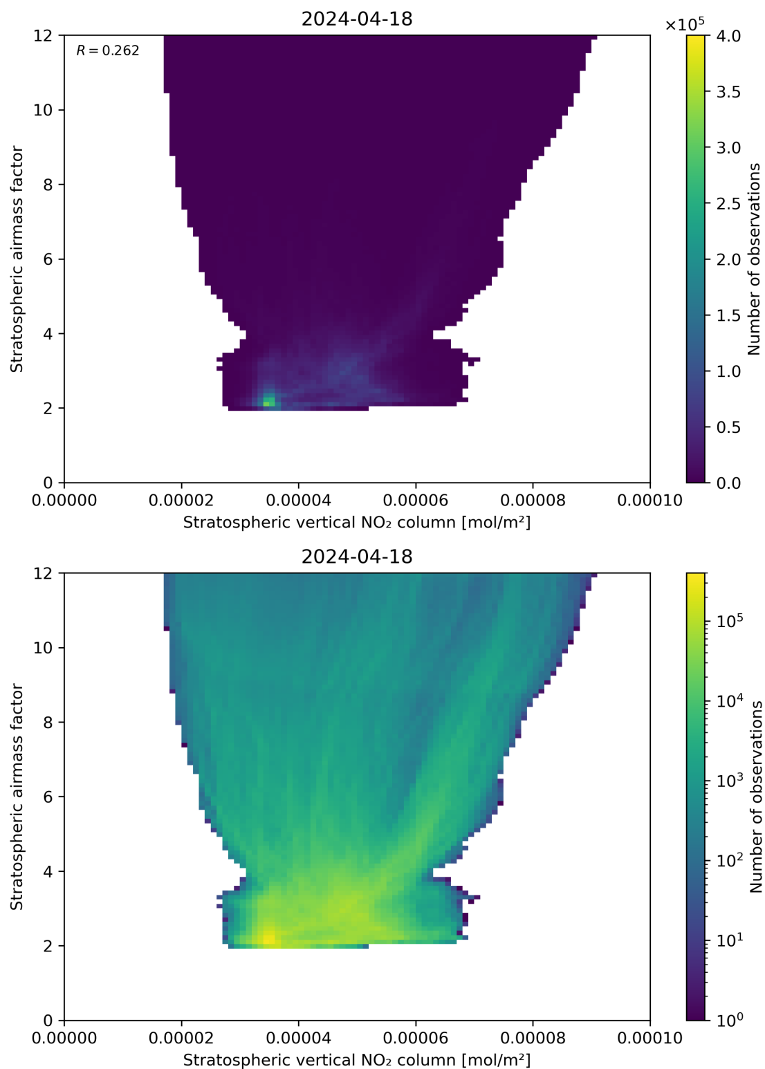
Figure 96: Scatter density plot of “Stratospheric vertical NO 2 column” against “Stratospheric airmass factor” for 2024-04-17 to 2024-04-19.
