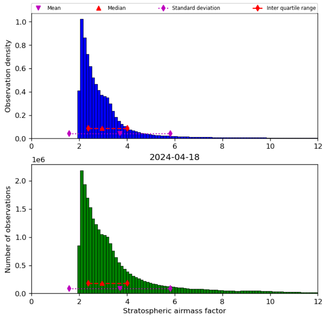
Figure 44: Histogram of “Stratospheric airmass factor” for 2024-04-17 to 2024-04-19
