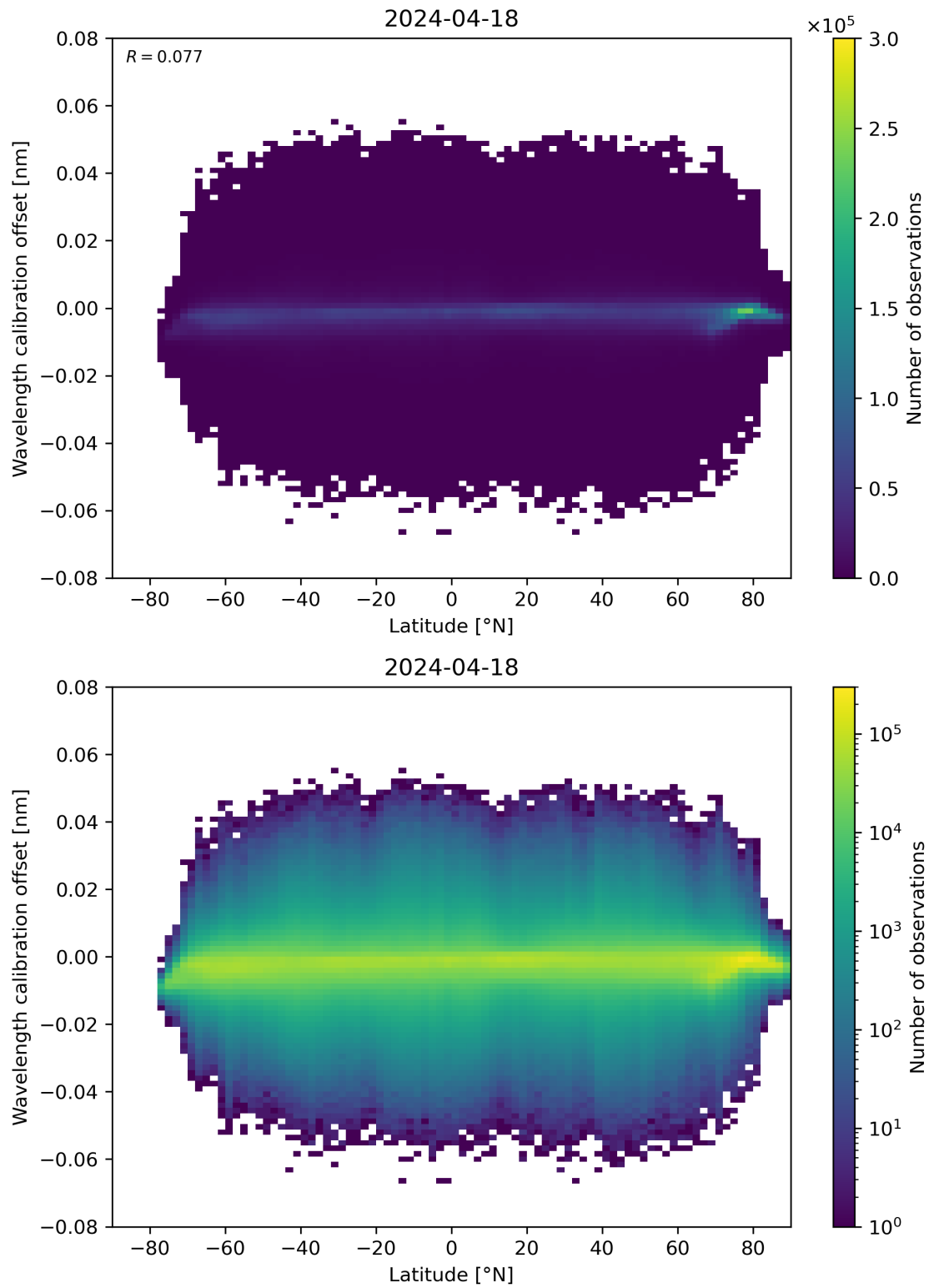
Figure 95: Scatter density plot of “Latitude” against “Wavelength calibration offset” for 2024-04-17 to 2024-04-19.
