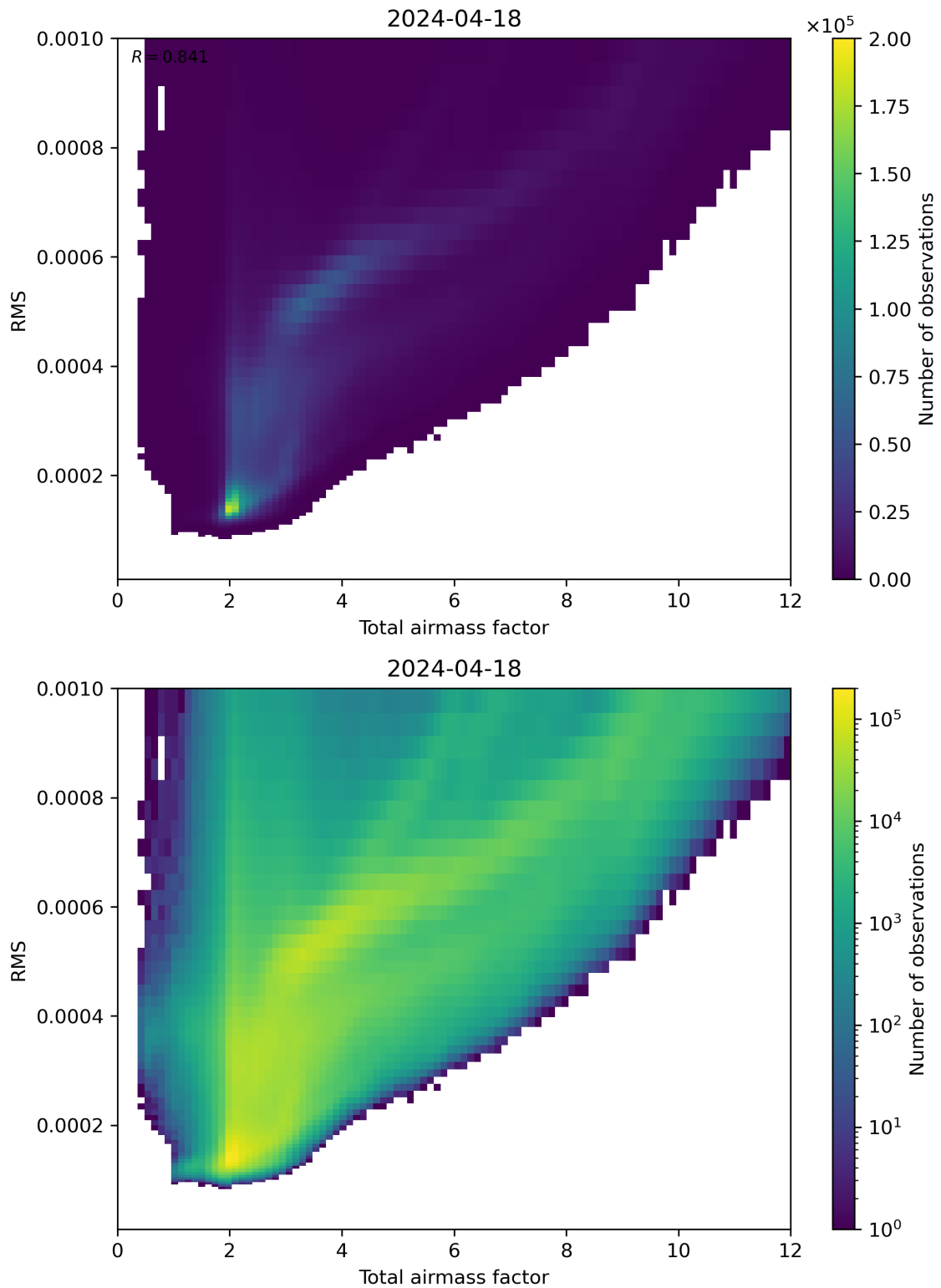
Figure 69: Scatter density plot of “Total airmass factor” against “RMS” for 2024-04-17 to 2024-04-19.
