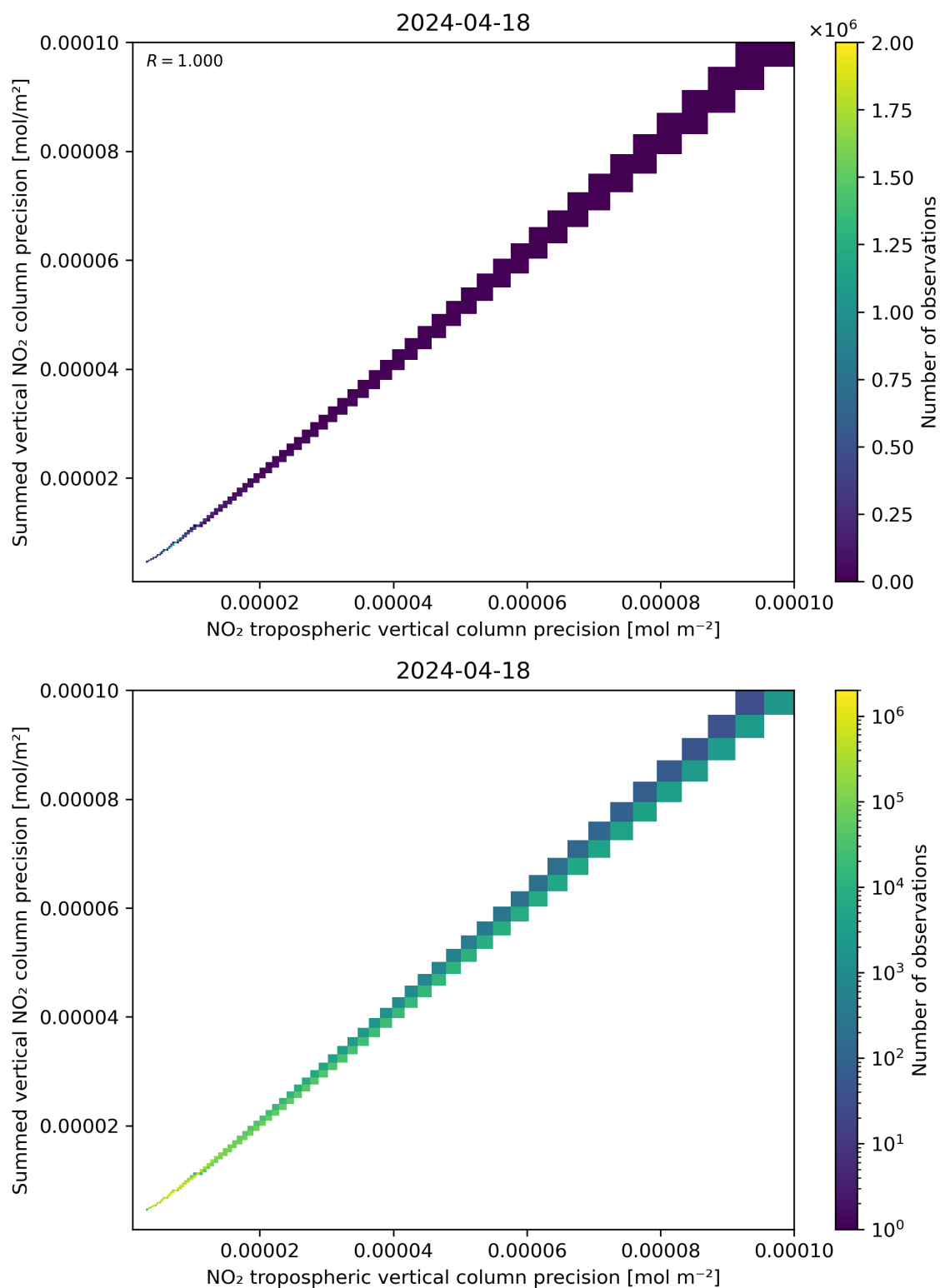
Figure 137: Scatter density plot of “NO 2 tropospheric vertical column precision” against “Summed vertical NO 2 column precision” for 2024-04-17 to 2024-04-19.
