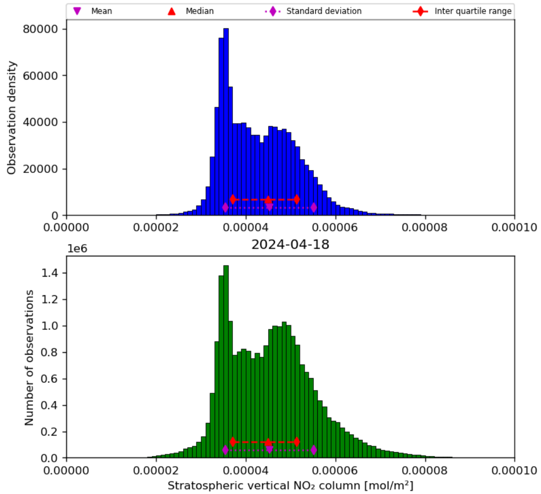
Figure 36: Histogram of “Stratospheric vertical NO 2 column” for 2024-04-17 to 2024-04-19
