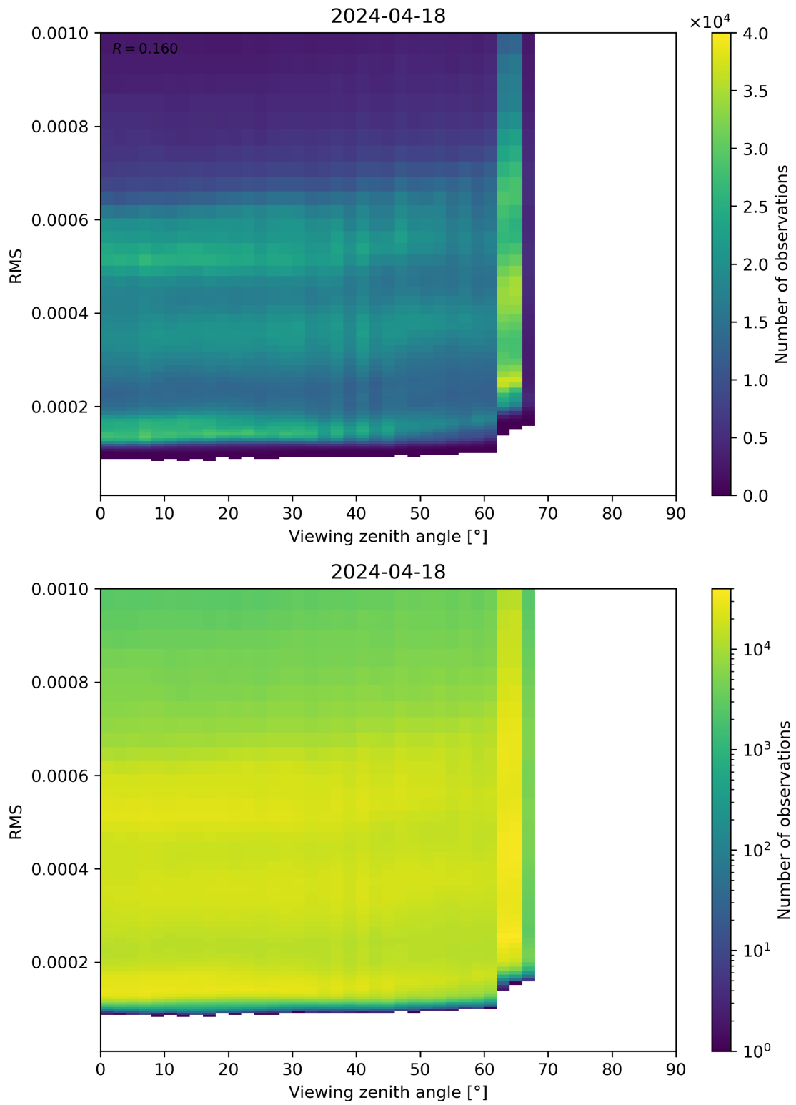
Figure 171: Scatter density plot of “Viewing zenith angle” against “RMS” for 2024-04-17 to 2024-04-19.
