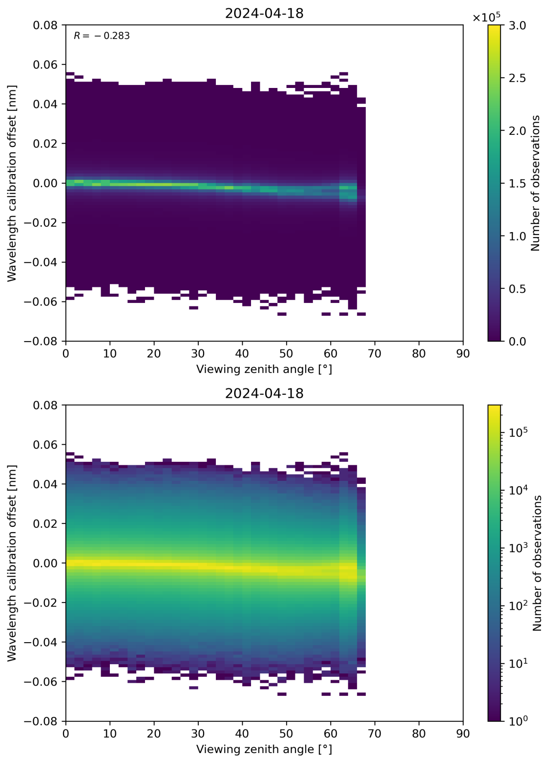
Figure 173: Scatter density plot of “Viewing zenith angle” against “Wavelength calibration offset” for 2024-04-17 to 2024-04-19.
