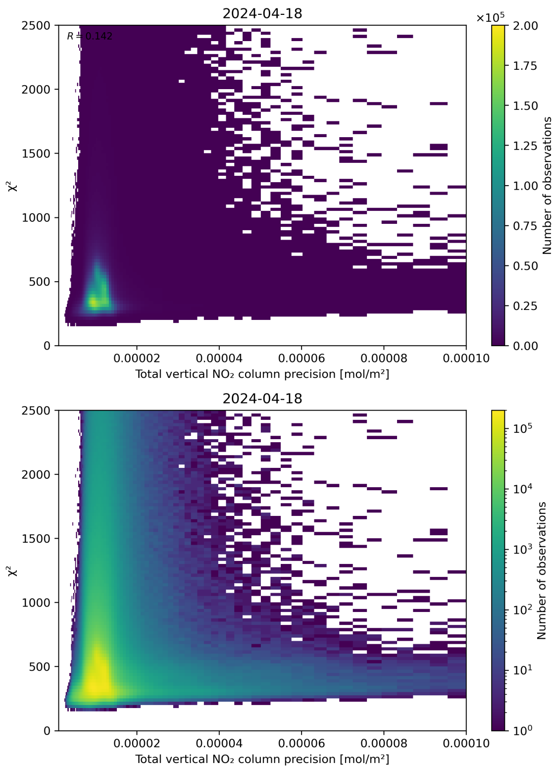
Figure 116: Scatter density plot of “Total vertical NO 2 column precision” against “ \chi^2 ” for 2024-04-17 to 2024-04-19.
