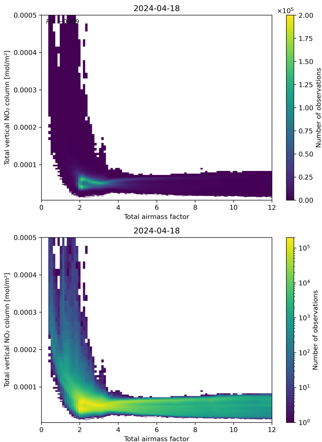
Figure 67: Scatter density plot of “Total airmass factor” against “Total vertical NO 2 column” for 2024-04-17 to 2024-04-19.
