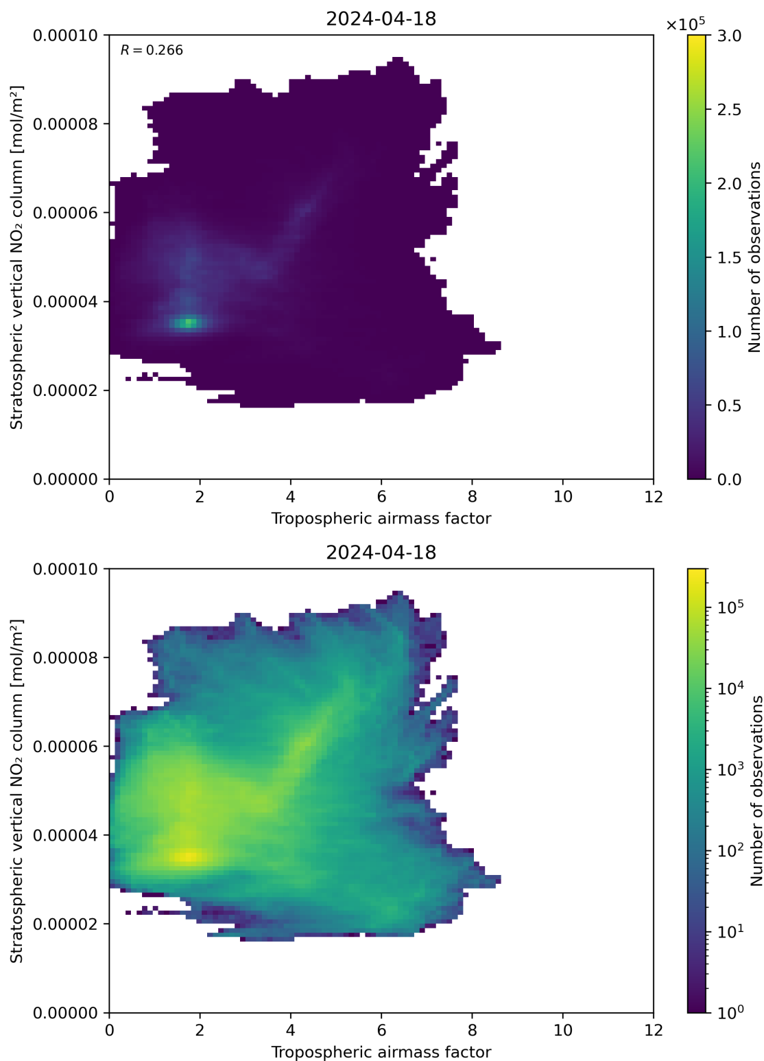
Figure 74: Scatter density plot of “Tropospheric air mass factor” against “Stratospheric vertical \text{NO}_2 column” for 2024-04-17 to 2024-04-19.
