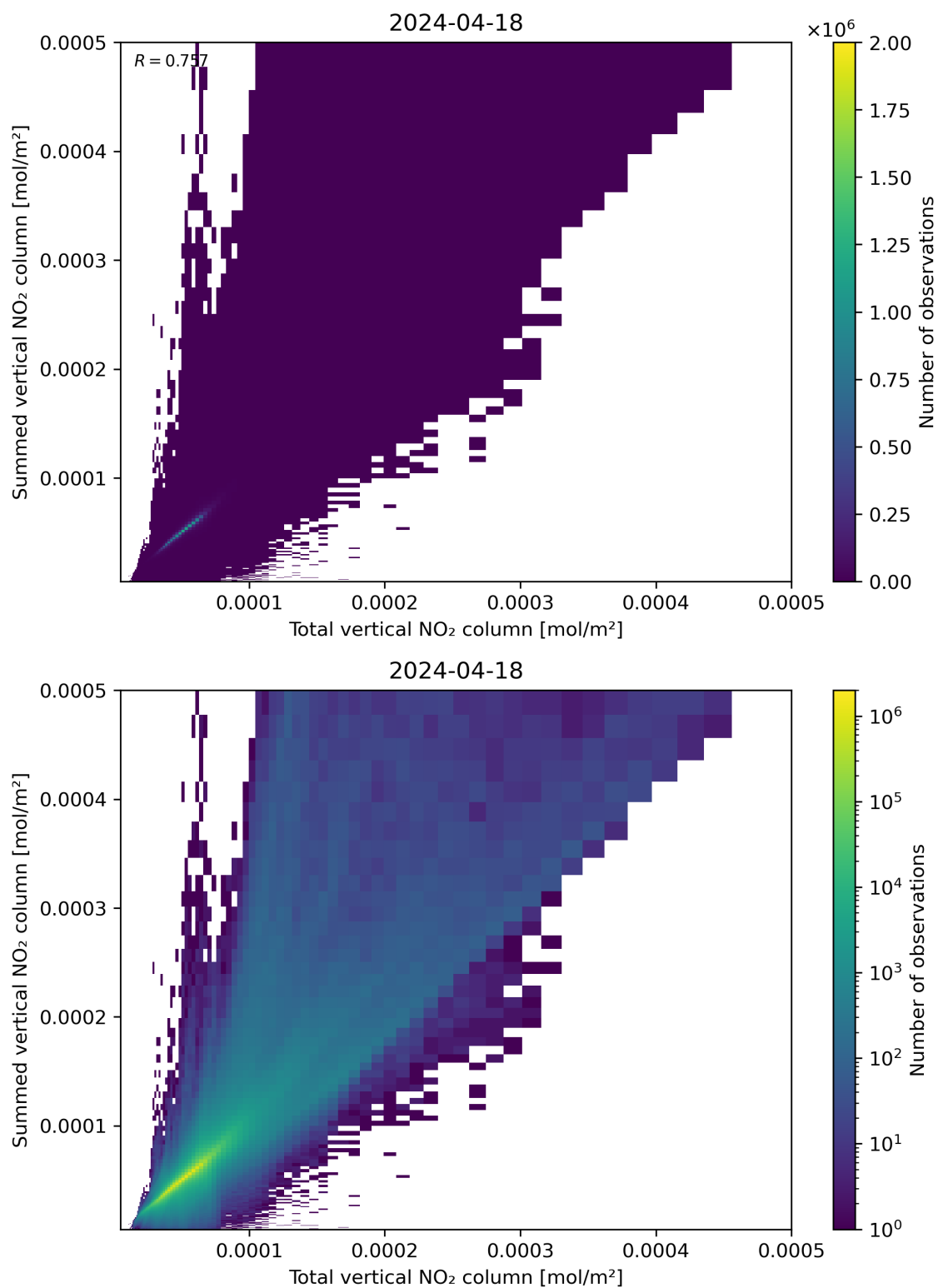
Figure 112: Scatter density plot of “Total vertical NO 2 column” against “Summed vertical NO 2 column” for 2024-04-17 to 2024-04-19.
