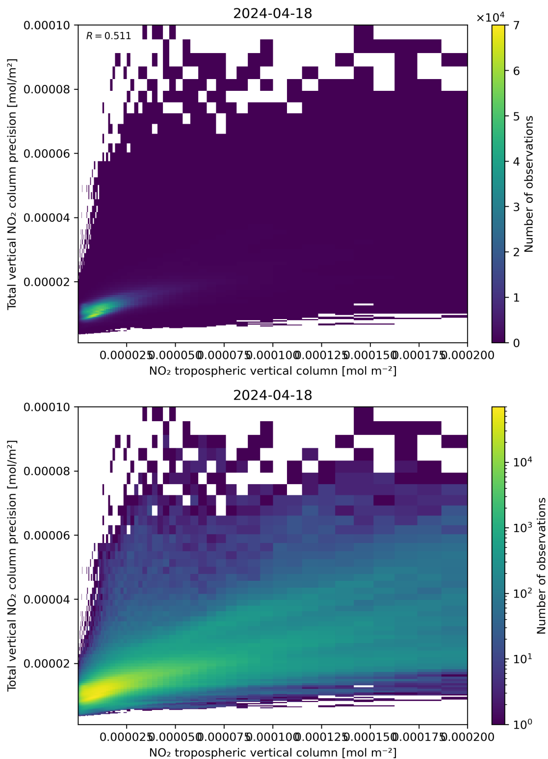
Figure 129: Scatter density plot of “NO 2 tropospheric vertical column” against “Total vertical NO 2 column precision” for 2024-04-17 to 2024-04-19.
