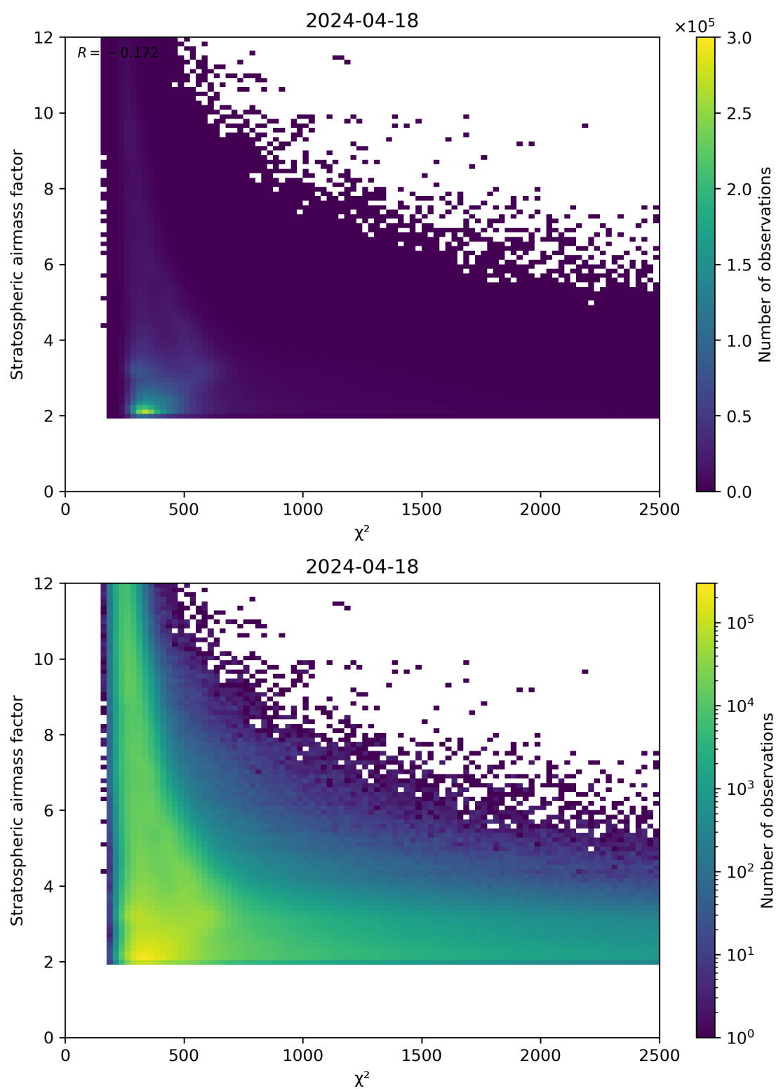
Figure 81: Scatter density plot of “ \chi^2 ” against “Stratospheric airmass factor” for 2024-04-17 to 2024-04-19.
