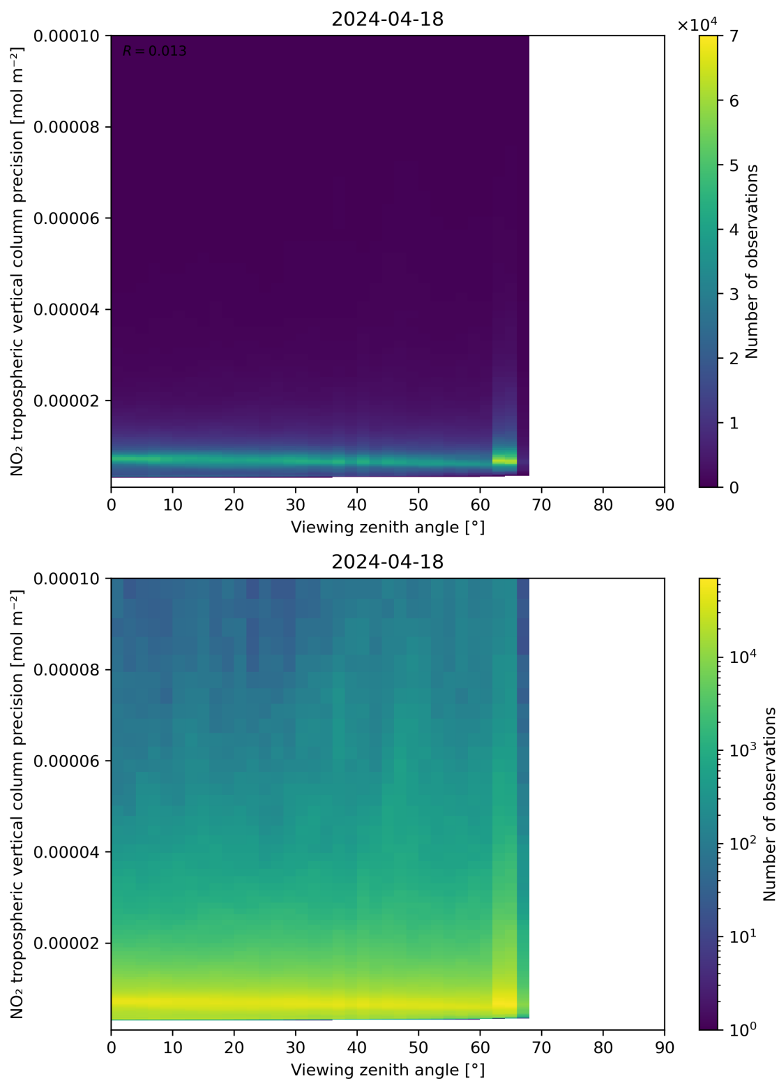
Figure 170: Scatter density plot of “Viewing zenith angle” against “NO 2 tropospheric vertical column precision” for 2024-04-17 to 2024-04-19.
