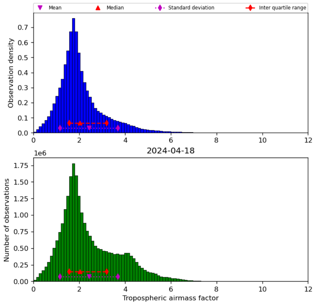
Figure 31: Histogram of “Tropospheric airmass factor” for 2024-04-17 to 2024-04-19
