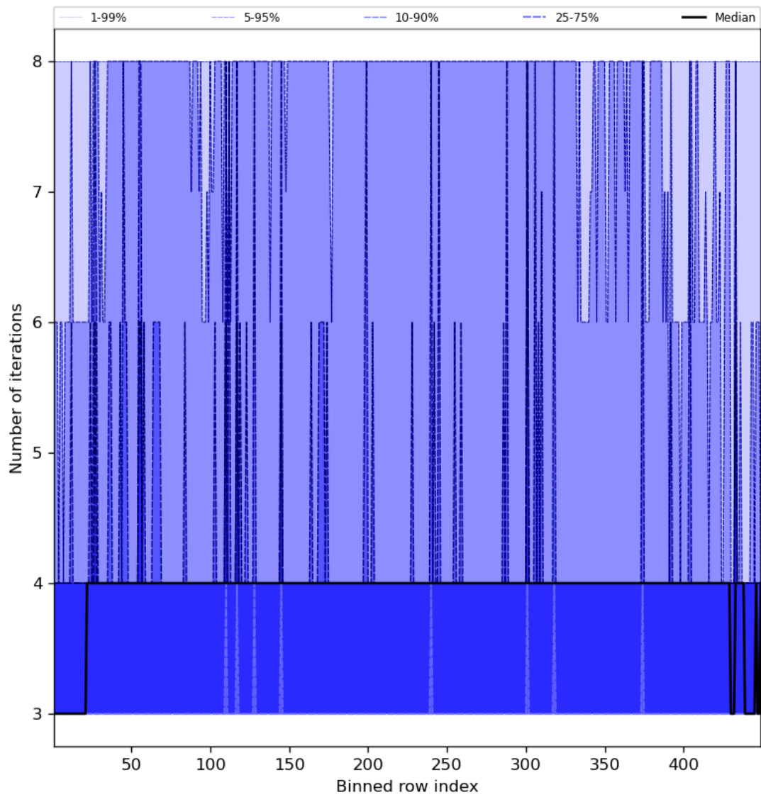
Figure 51: Along track statistics of “Number of iterations” for 2024-04-17 to 2024-04-19
