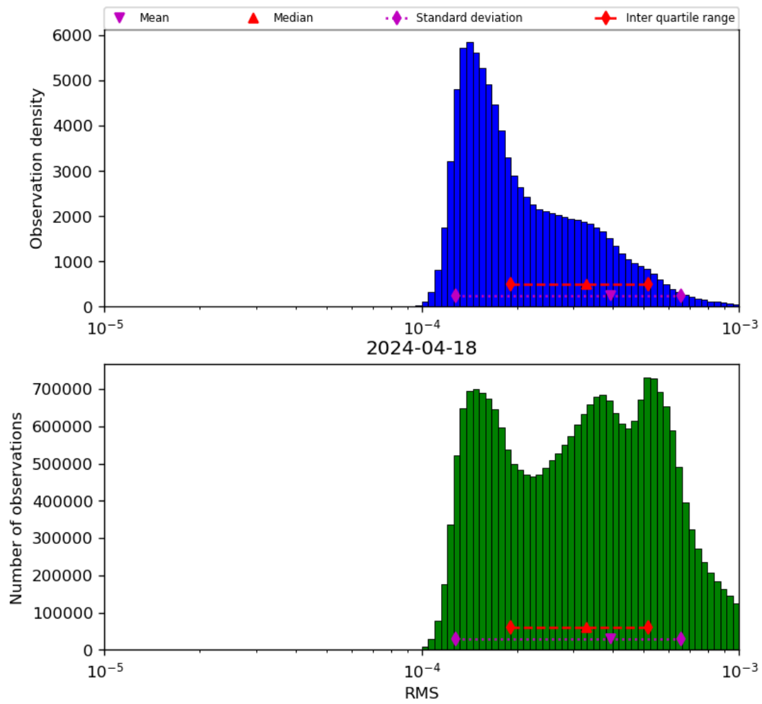
Figure 43: Histogram of “RMS” for 2024-04-17 to 2024-04-19
