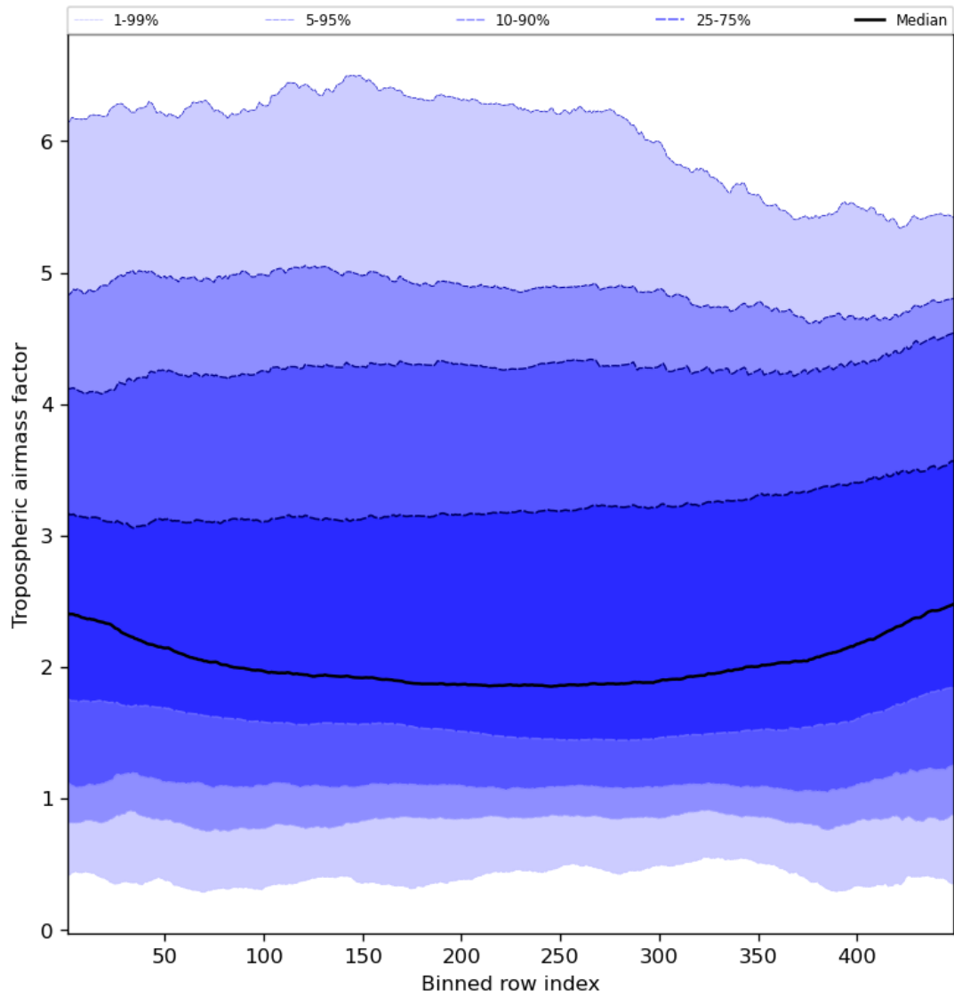
Figure 48: Along track statistics of “Tropospheric air mass factor” for 2024-04-17 to 2024-04-19
