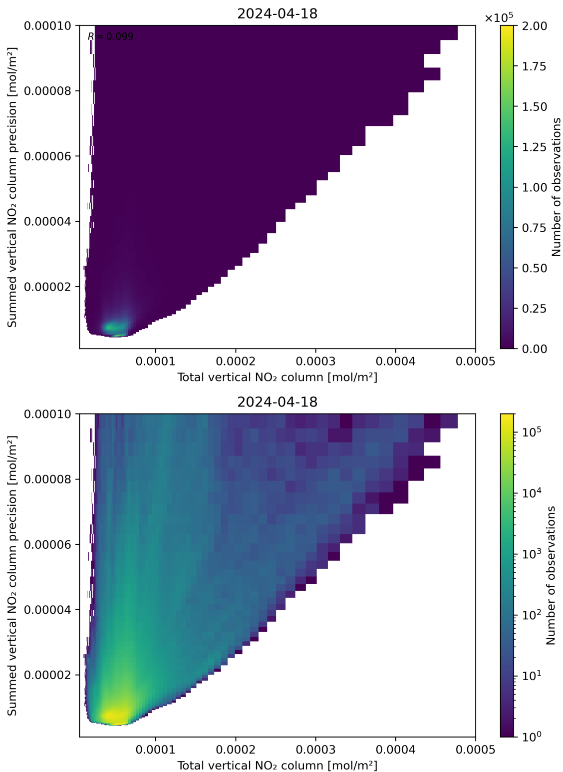
Figure 113: Scatter density plot of “Total vertical NO 2 column” against “Summed vertical NO 2 column precision” for 2024-04-17 to 2024-04-19.
