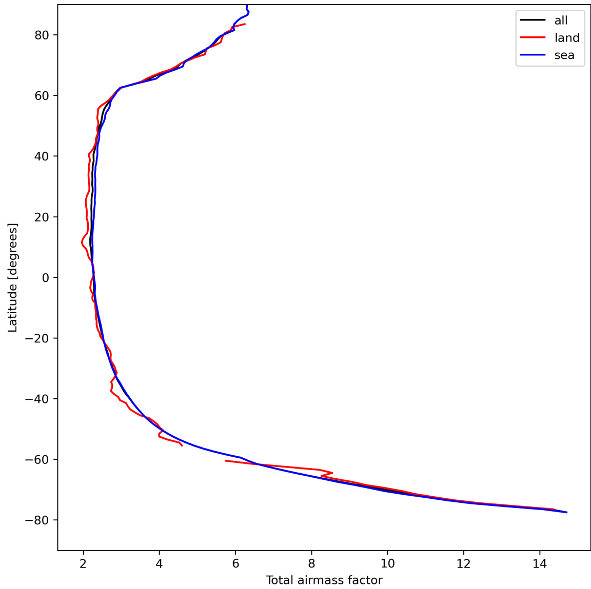
Figure 15: Zonal average of “Total airmass factor” for 2024-04-17 to 2024-04-19.
