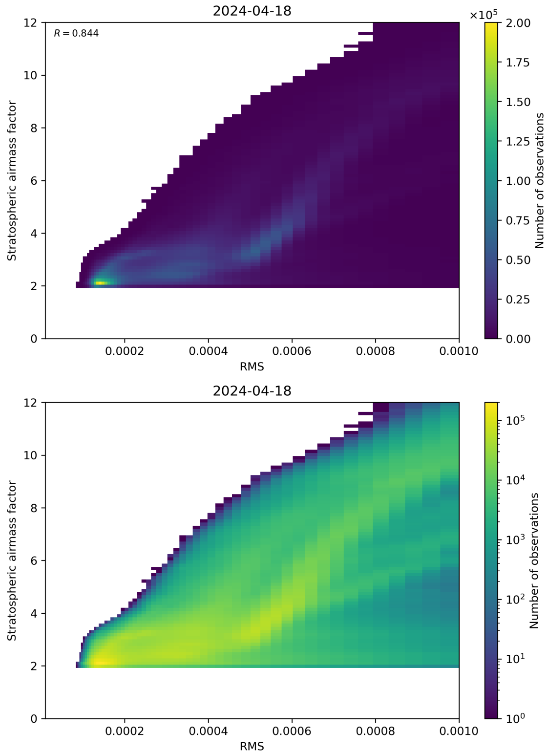
Figure 144: Scatter density plot of “RMS” against “Stratospheric airmass factor” for 2024-04-17 to 2024-04-19.
