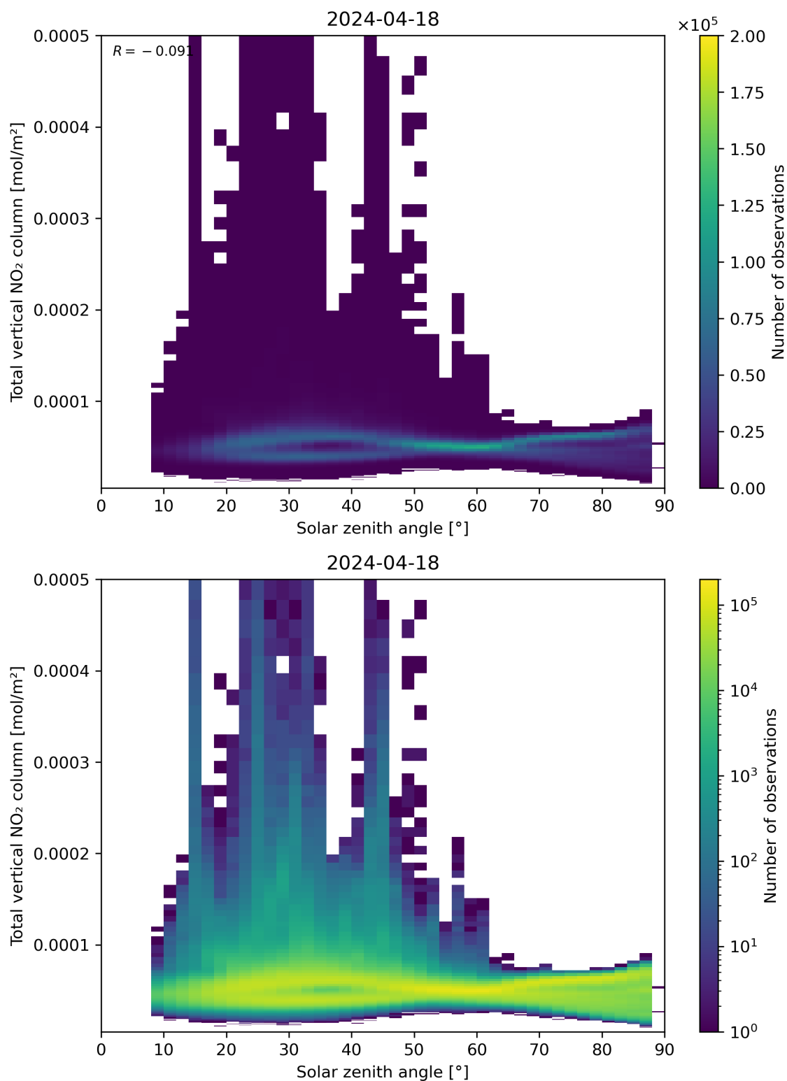
Figure 153: Scatter density plot of “Solar zenith angle” against “Total vertical NO 2 column” for 2024-04-17 to 2024-04-19.
