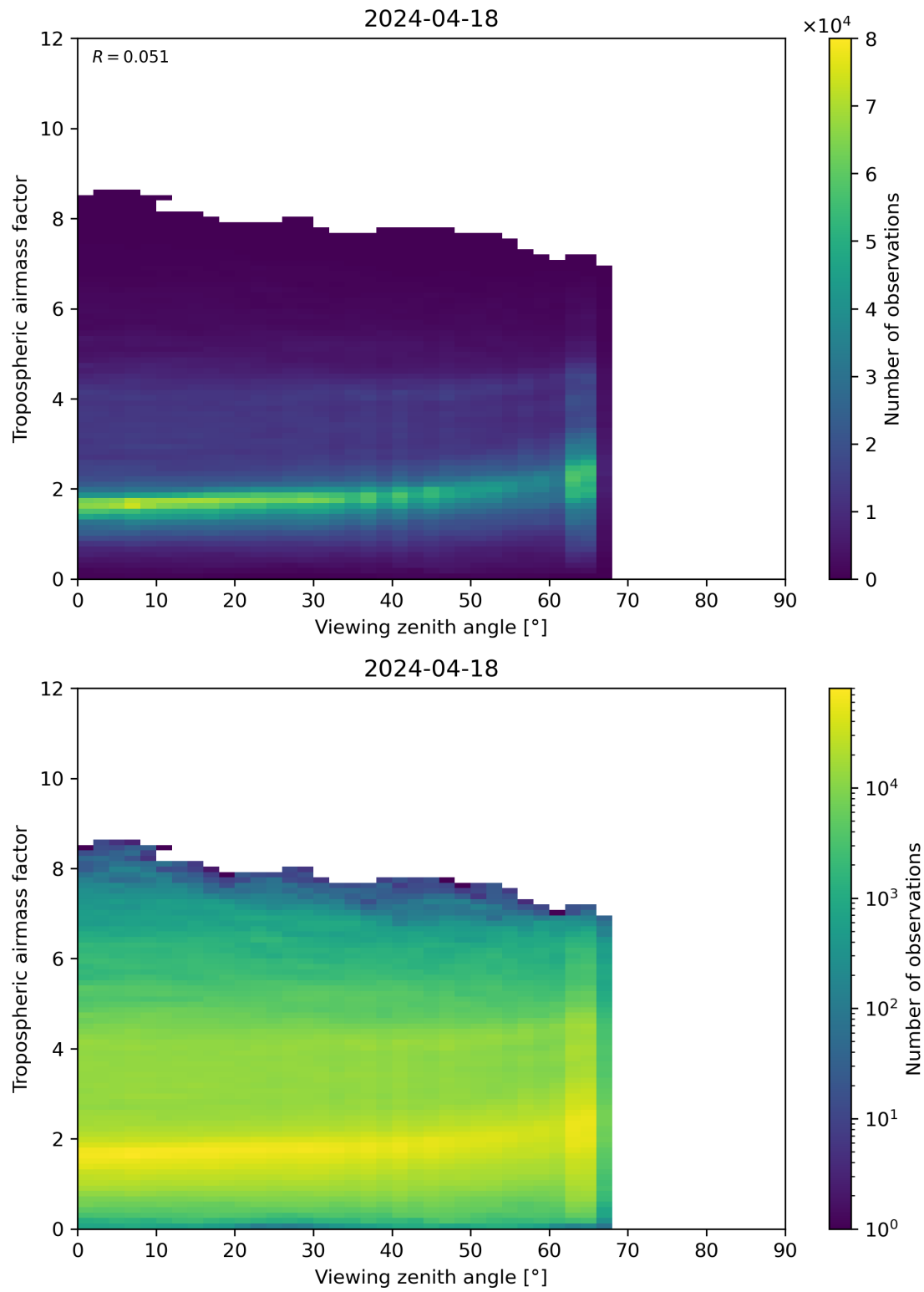
Figure 161: Scatter density plot of “Viewing zenith angle” against “Tropospheric airmass factor” for 2024-04-17 to 2024-04-19.
