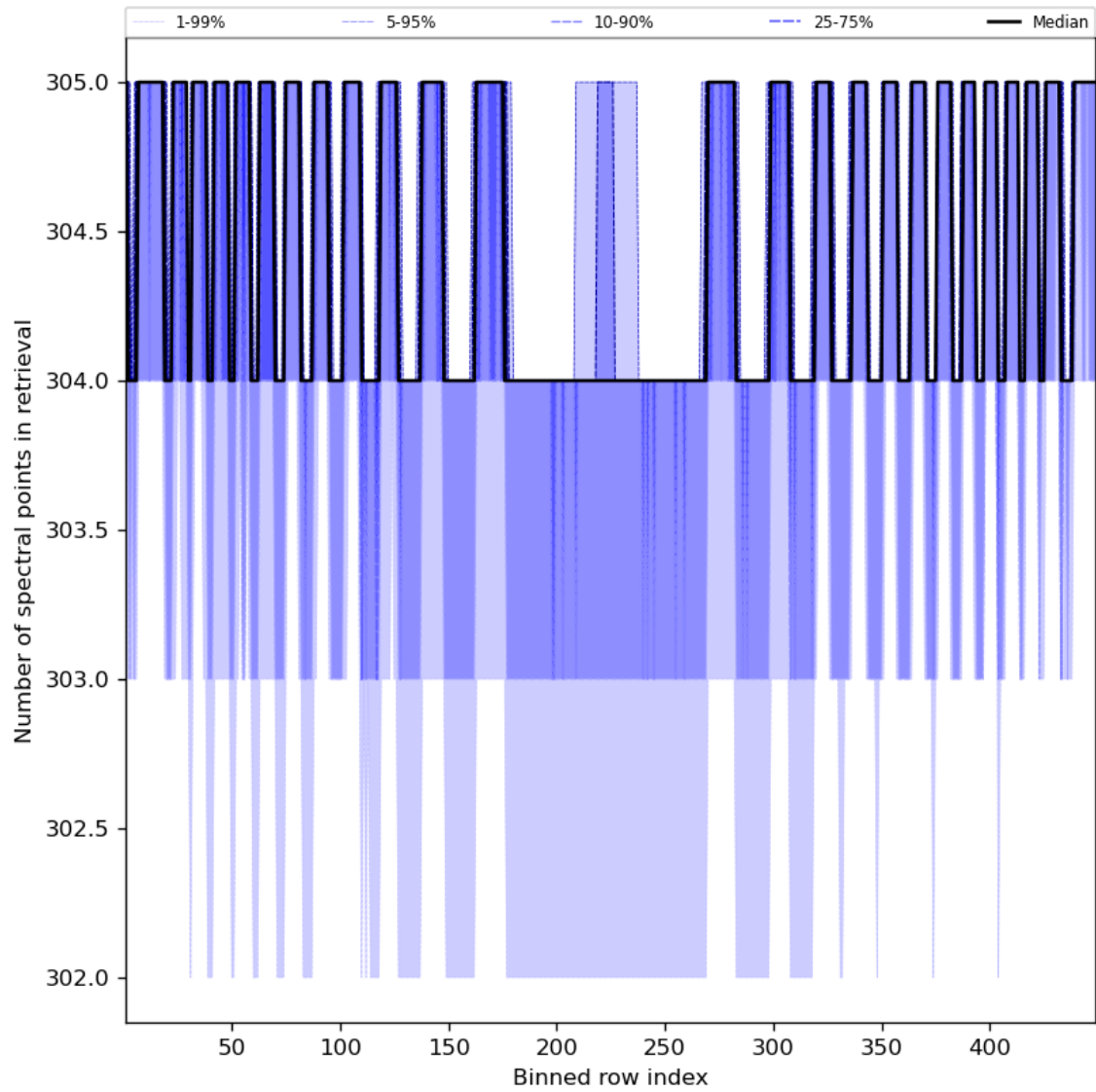
Figure 50: Along track statistics of “Number of spectral points in retrieval” for 2024-04-17 to 2024-04-19
