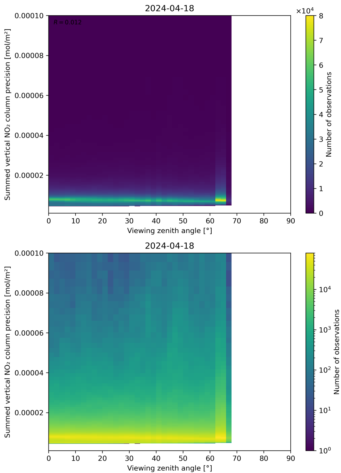
Figure 166: Scatter density plot of “Viewing zenith angle” against “Summed vertical NO 2 column precision” for 2024-04-17 to 2024-04-19.
