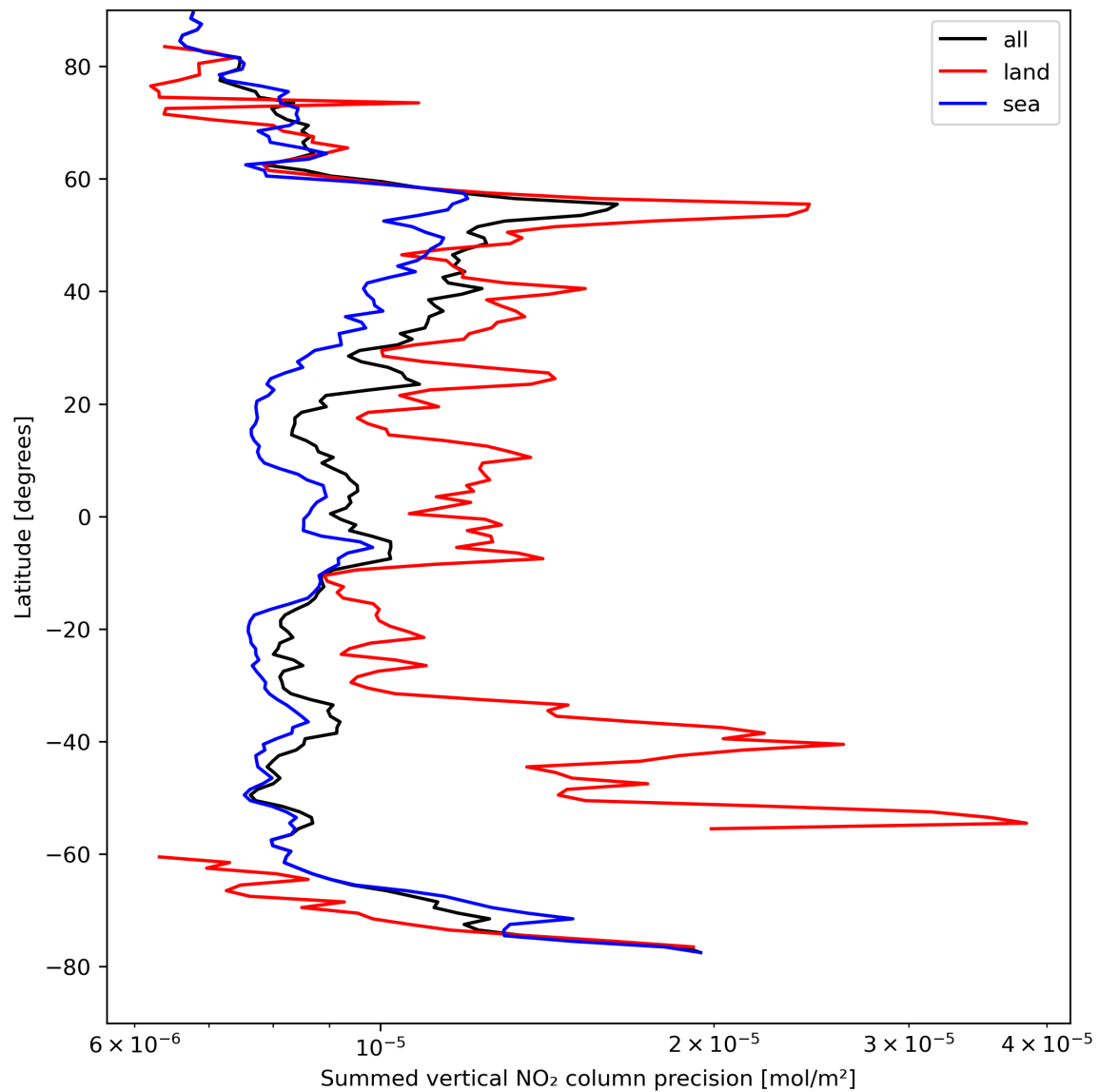
Figure 24: Zonal average of “Summed vertical NO 2 column precision” for 2024-04-17 to 2024-04-19.
