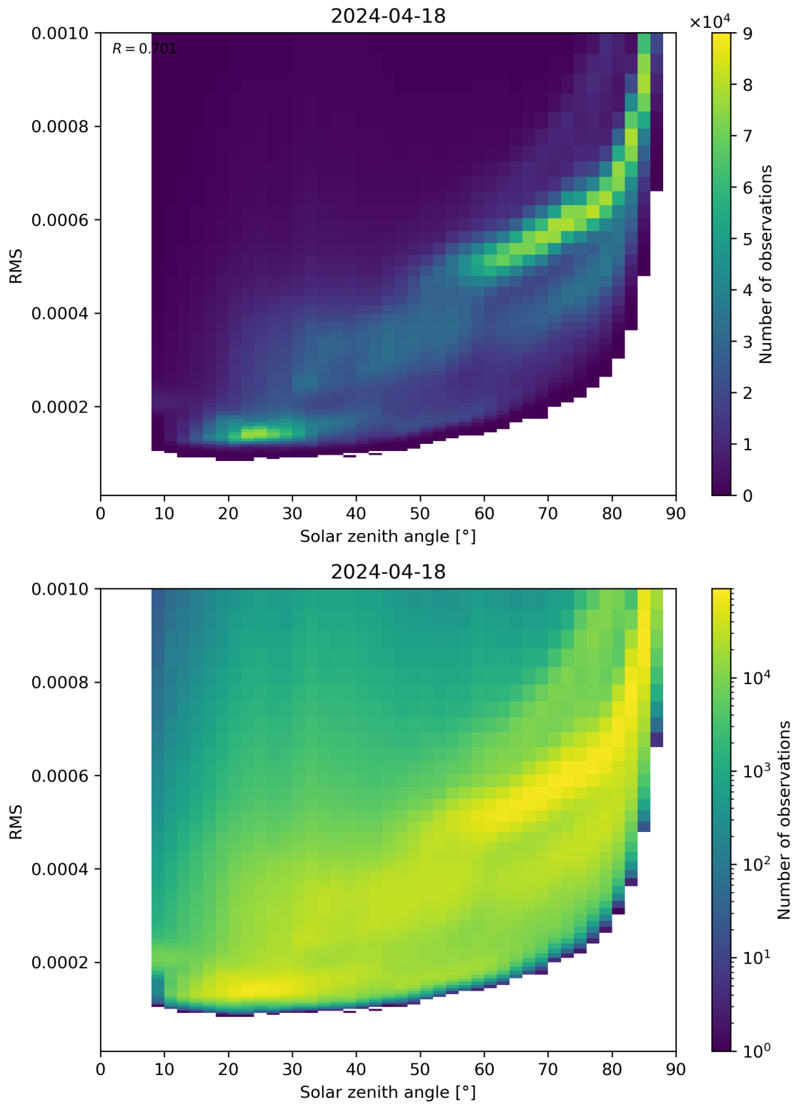
Figure 157: Scatter density plot of “Solar zenith angle” against “RMS” for 2024-04-17 to 2024-04-19.
