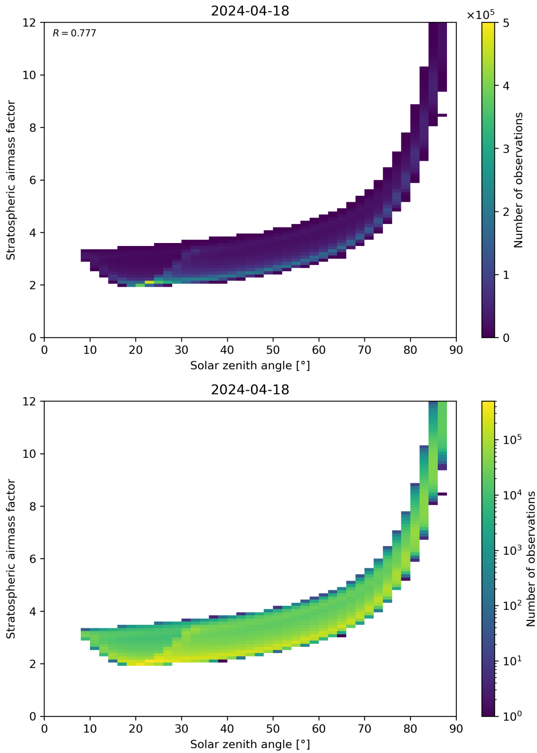
Figure 145: Scatter density plot of “Solar zenith angle” against “Stratospheric airmass factor” for 2024-04-17 to 2024-04-19.
