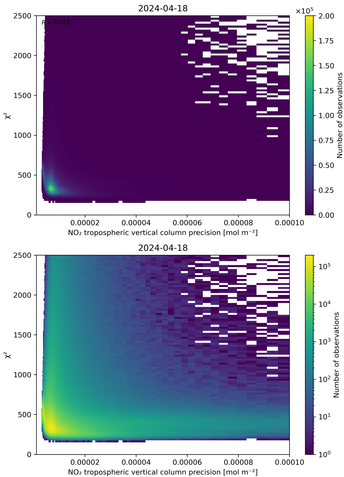
Figure 134: Scatter density plot of “NO 2 tropospheric vertical column precision” against “ \chi^2 ” for 2024-04-17 to 2024-04-19.
