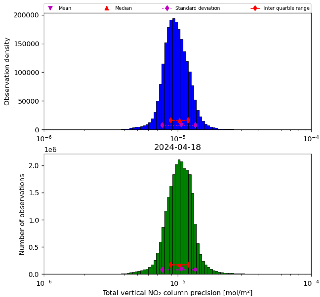
Figure 39: Histogram of "Total vertical NO 2 column precision" for 2024-04-17 to 2024-04-19
