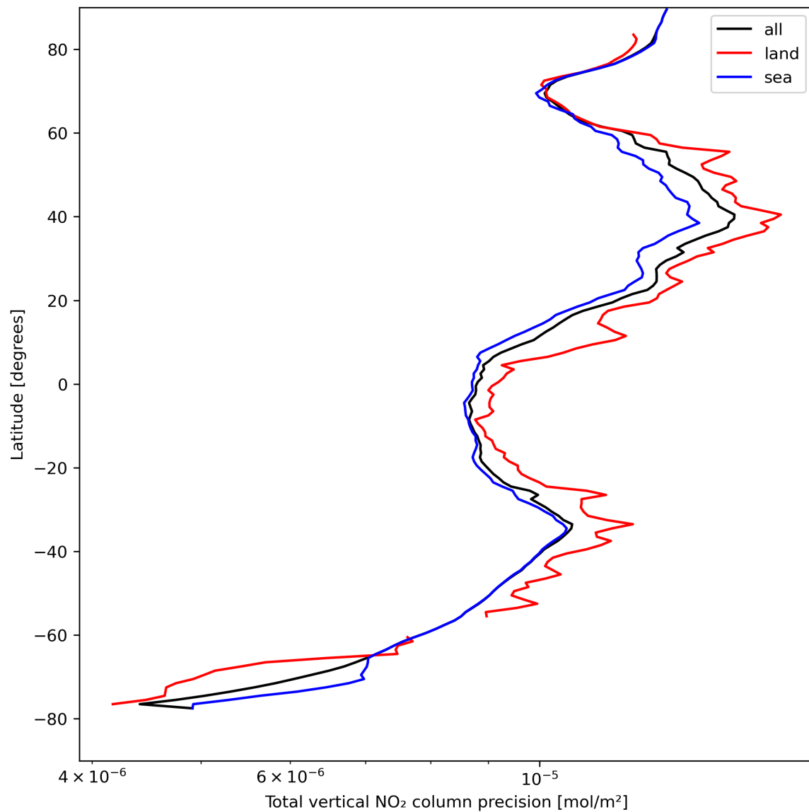
Figure 22: Zonal average of “Total vertical NO 2 column precision” for 2024-04-17 to 2024-04-19.
