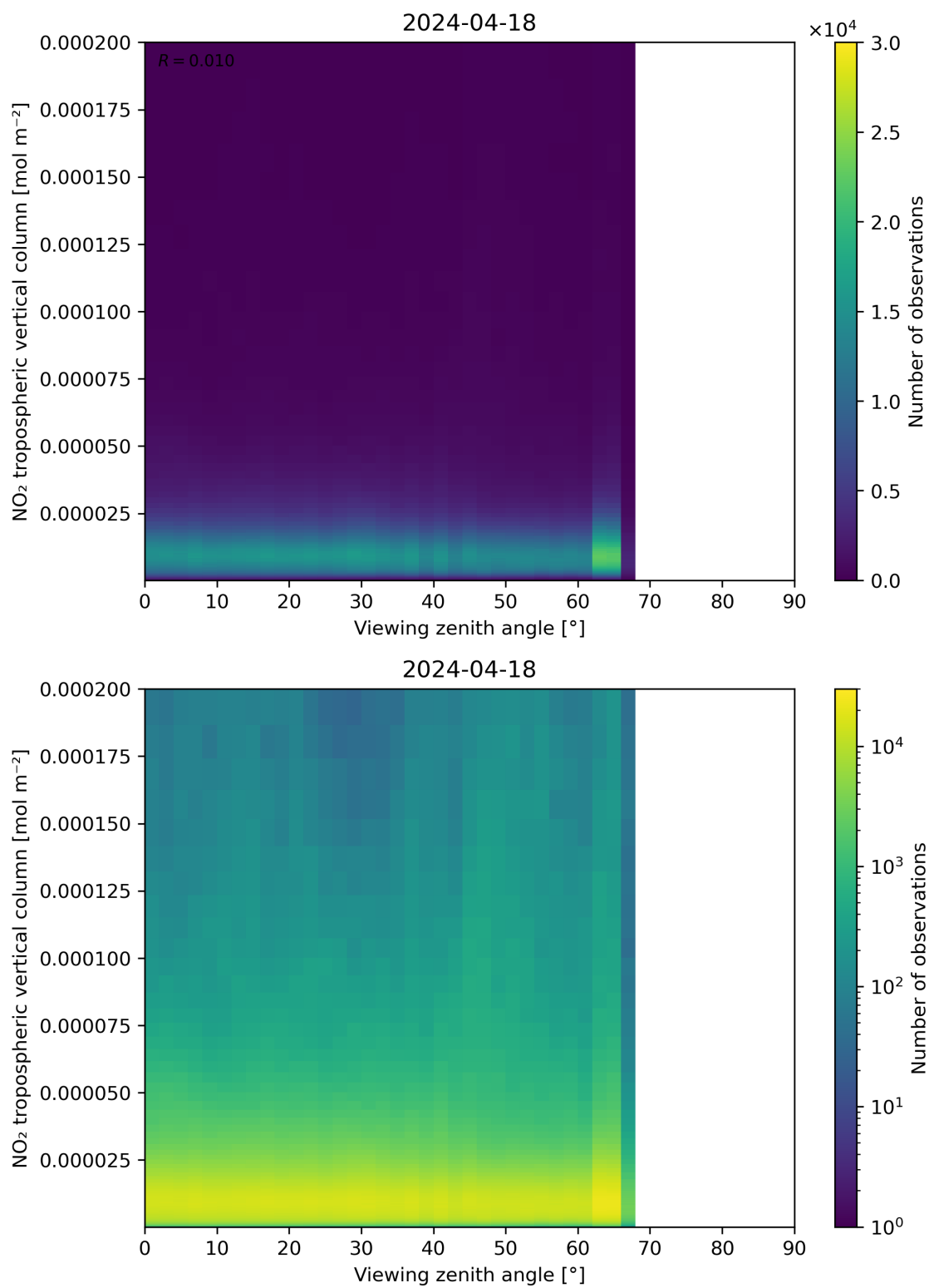
Figure 169: Scatter density plot of “Viewing zenith angle” against “NO 2 tropospheric vertical column” for 2024-04-17 to 2024-04-19.
