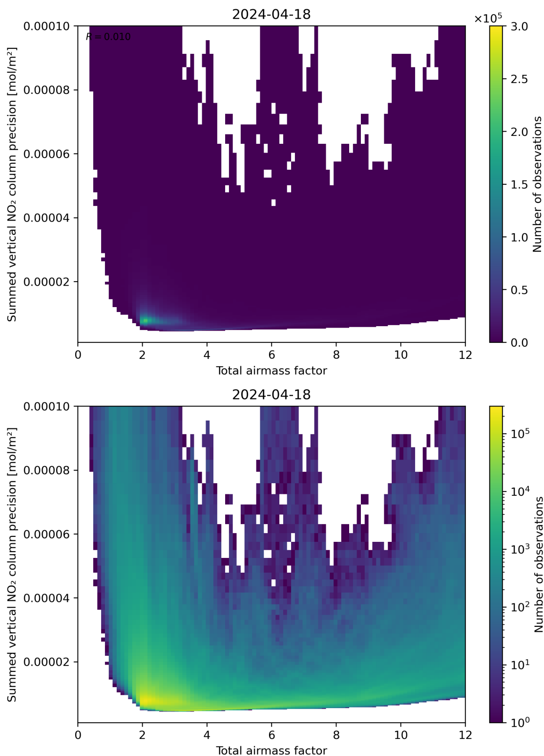
Figure 66: Scatter density plot of “Total airmass factor” against “Summed vertical NO 2 column precision” for 2024-04-17 to 2024-04-19.
