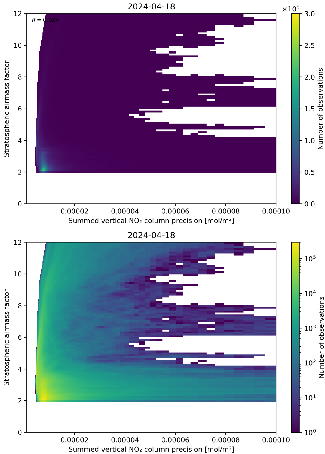
Figure 106: Scatter density plot of “Summed vertical NO 2 column precision” against “Stratospheric airmass factor” for 2024-04-17 to 2024-04-19.
