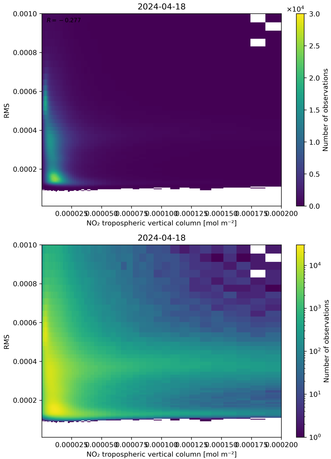
Figure 142: Scatter density plot of “NO 2 tropospheric vertical column” against “RMS” for 2024-04-17 to 2024-04-19.
