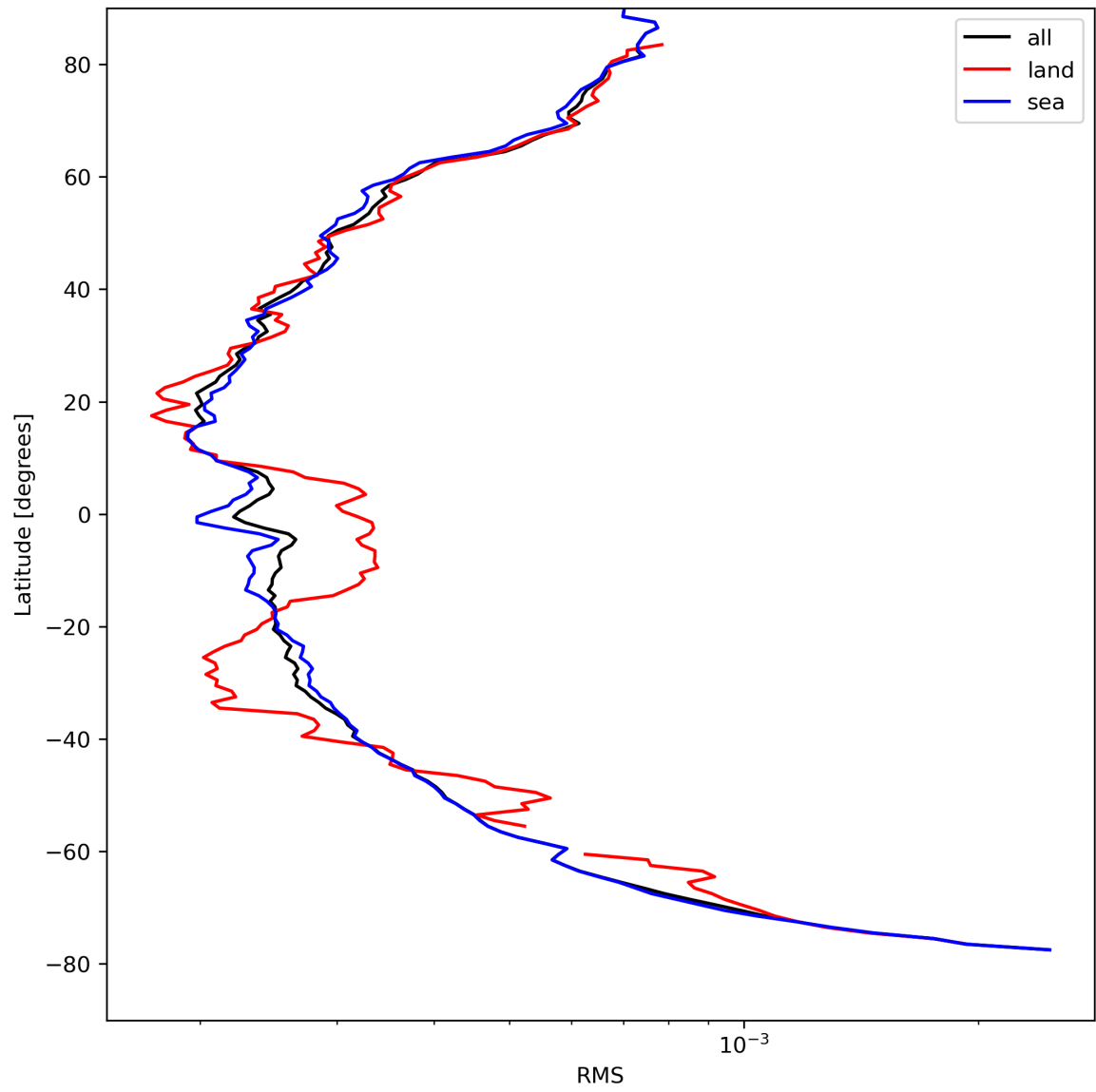
Figure 26: Zonal average of “RMS” for 2024-04-17 to 2024-04-19.
