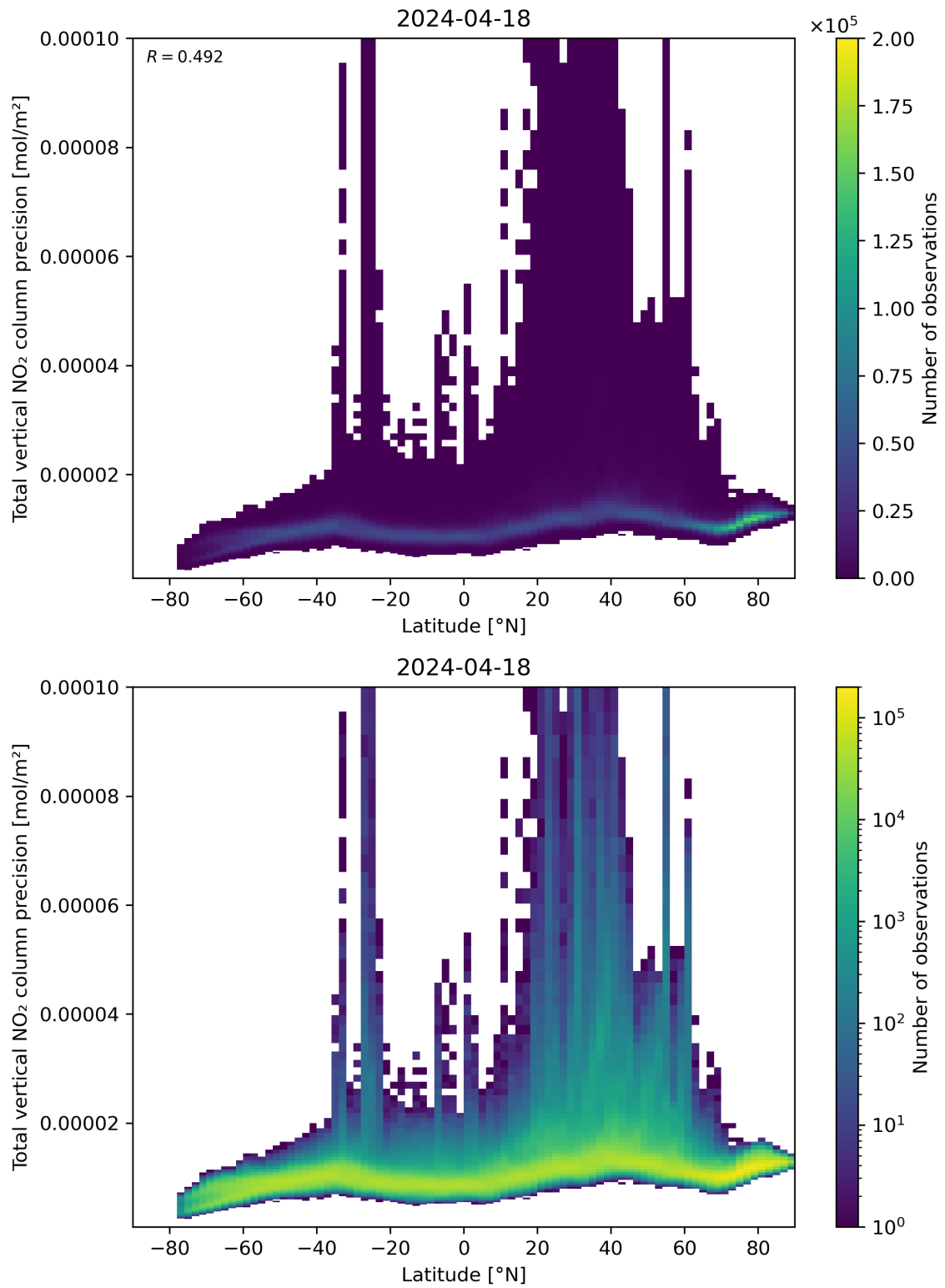
Figure 91: Scatter density plot of “Latitude” against “Total vertical NO 2 column precision” for 2024-04-17 to 2024-04-19.
