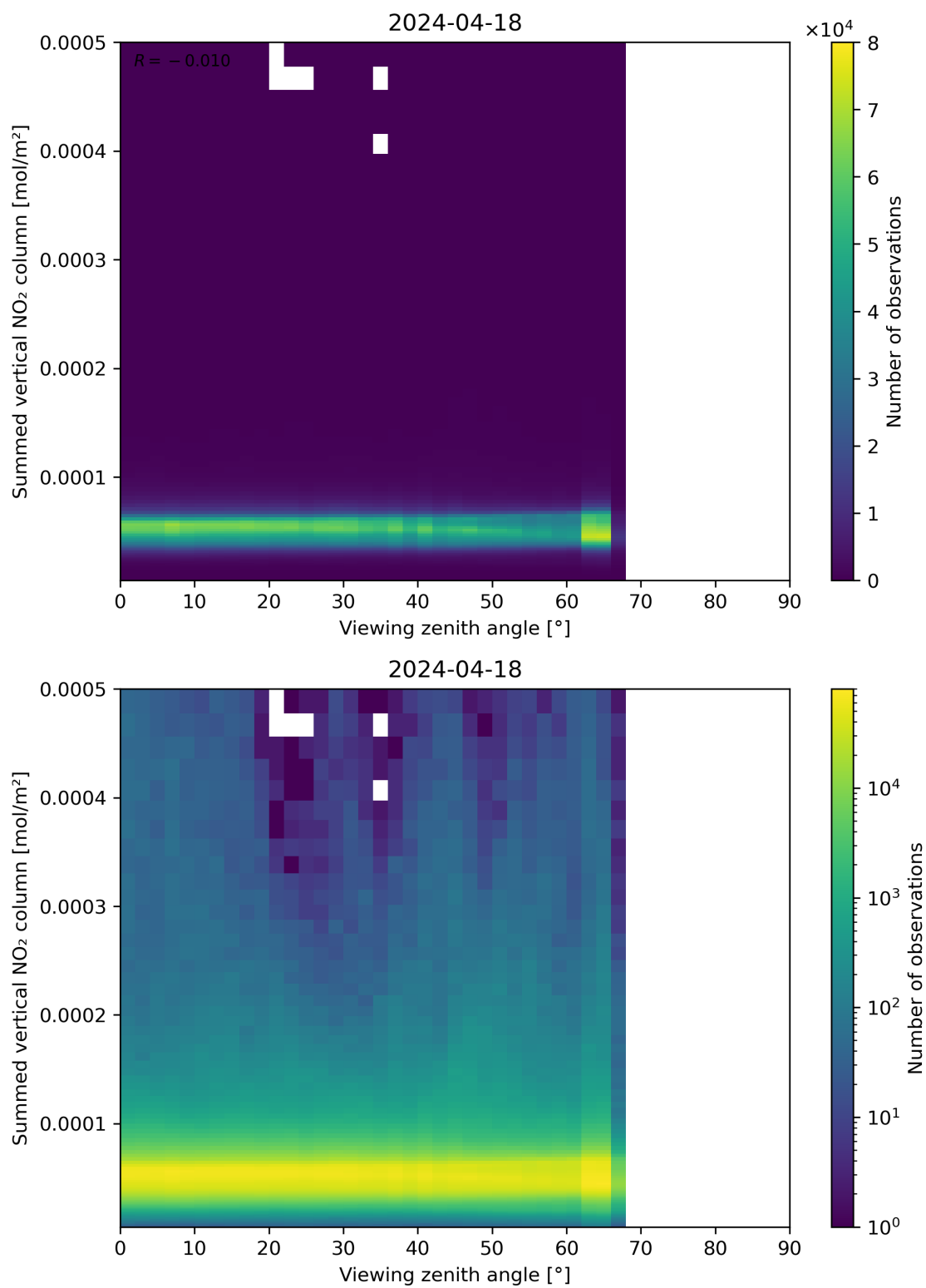
Figure 165: Scatter density plot of “Viewing zenith angle” against “Summed vertical NO 2 column” for 2024-04-17 to 2024-04-19.
