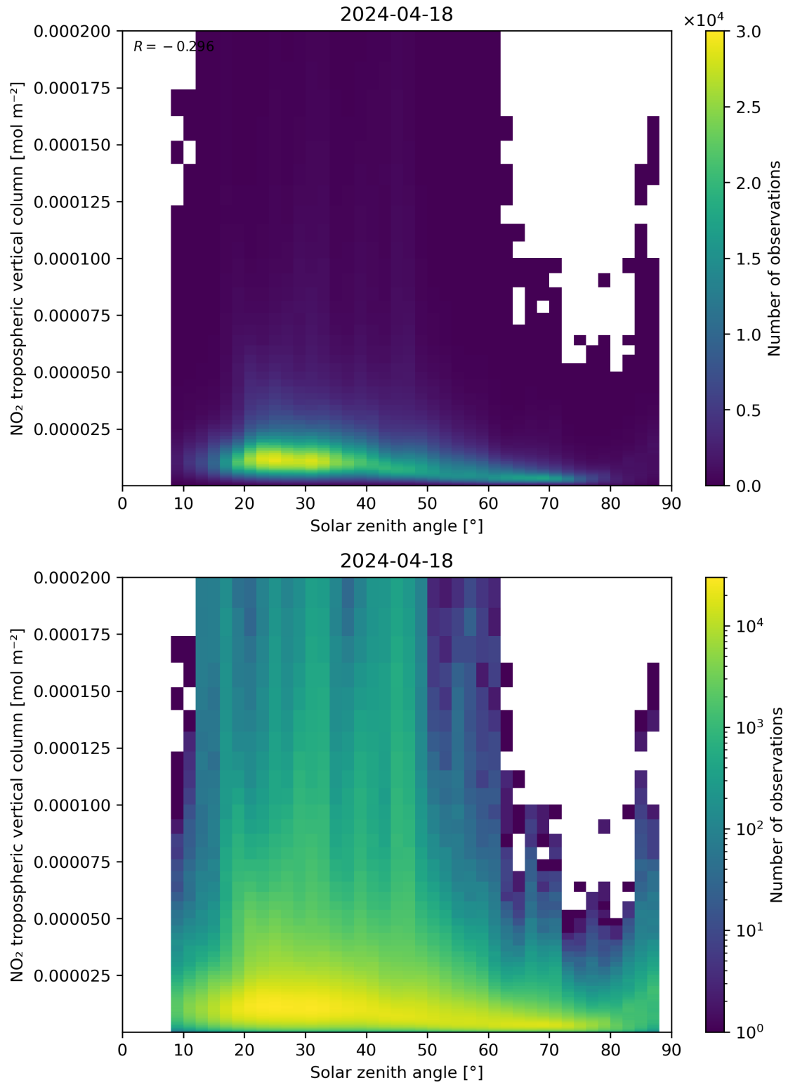
Figure 155: Scatter density plot of “Solar zenith angle” against “NO 2 tropospheric vertical column” for 2024-04-17 to 2024-04-19.
