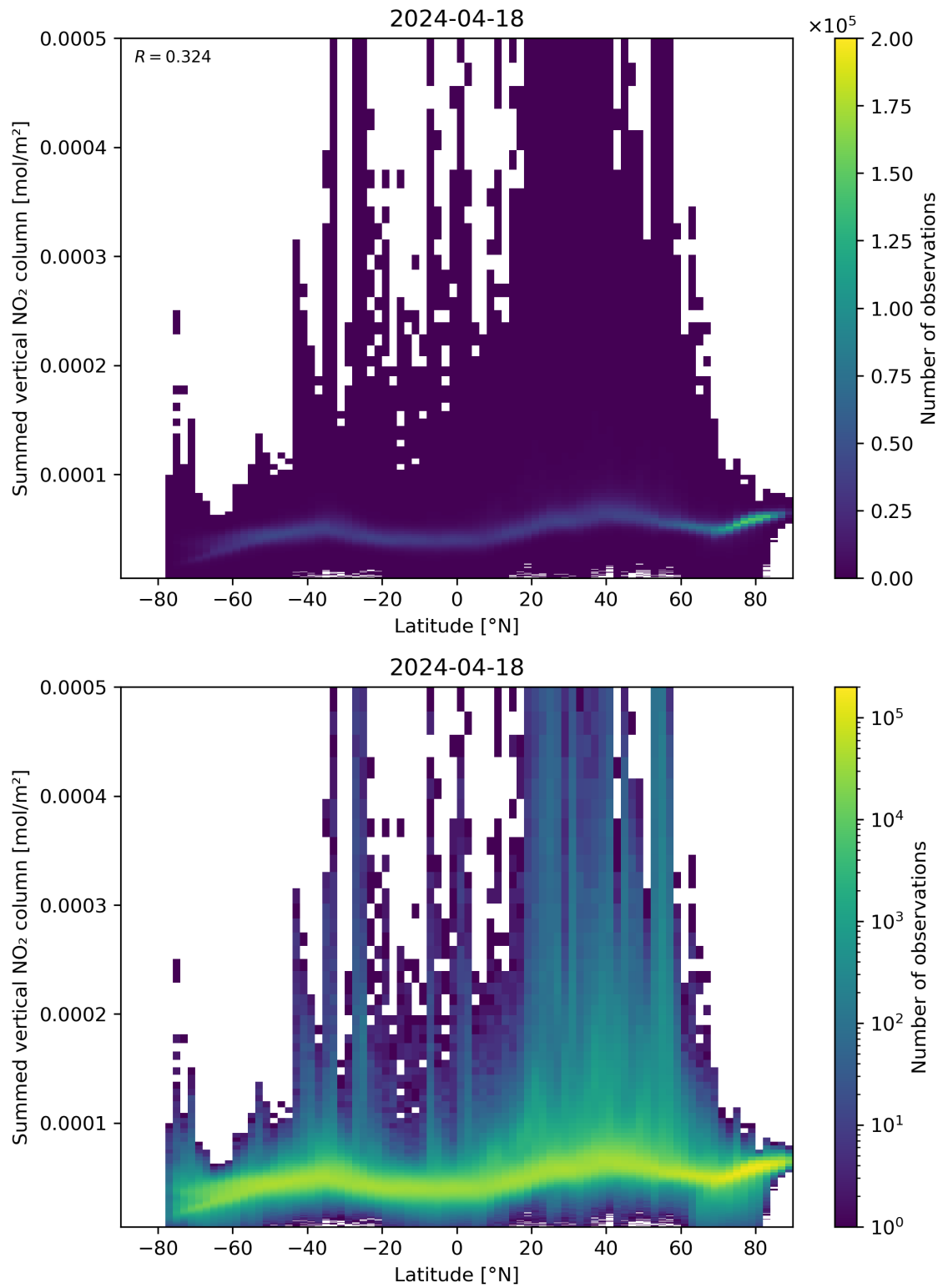
Figure 88: Scatter density plot of “Latitude” against “Summed vertical NO 2 column” for 2024-04-17 to 2024-04-19.
