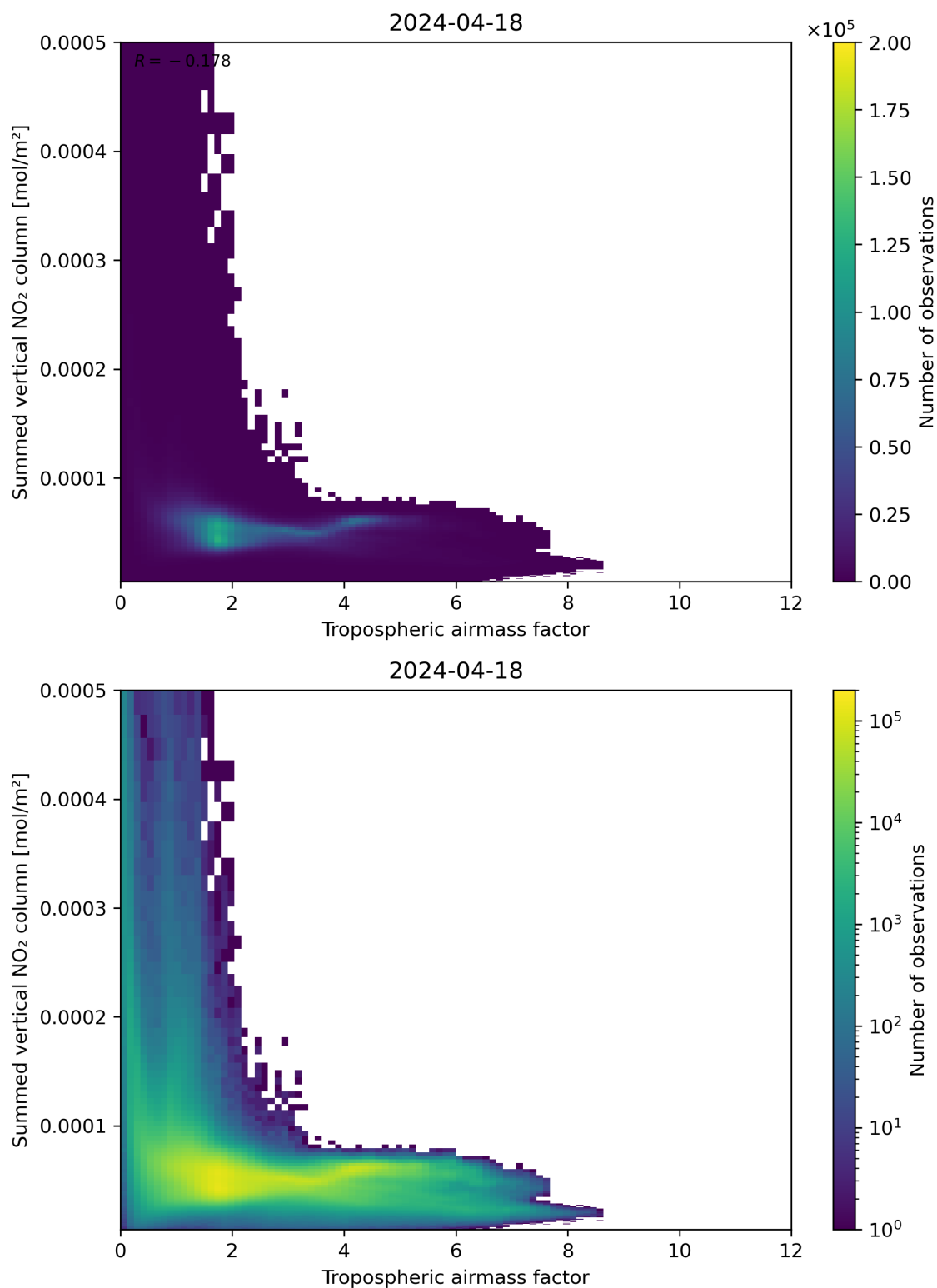
Figure 75: Scatter density plot of “Tropospheric airmass factor” against “Summed vertical NO 2 column” for 2024-04-17 to 2024-04-19.
