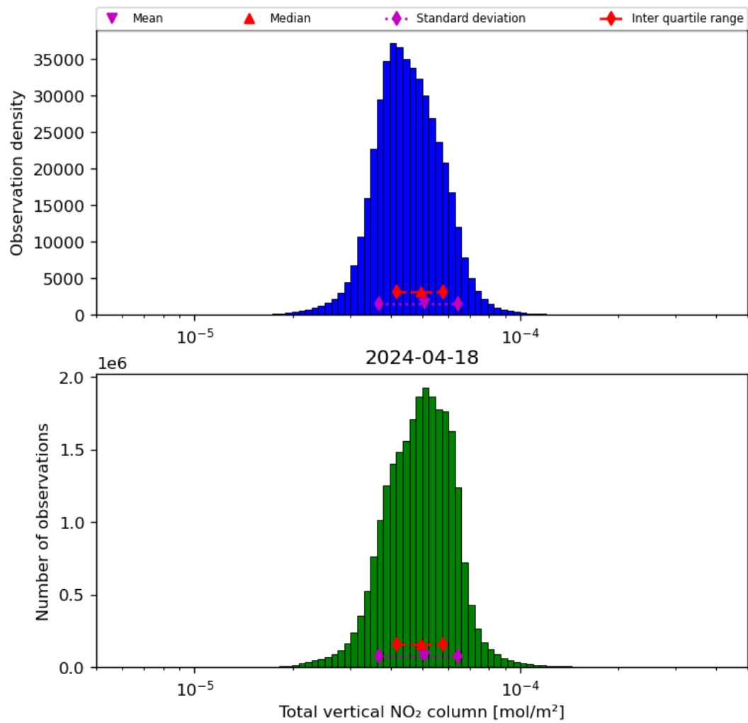
Figure 38: Histogram of “Total vertical NO 2 column” for 2024-04-17 to 2024-04-19
