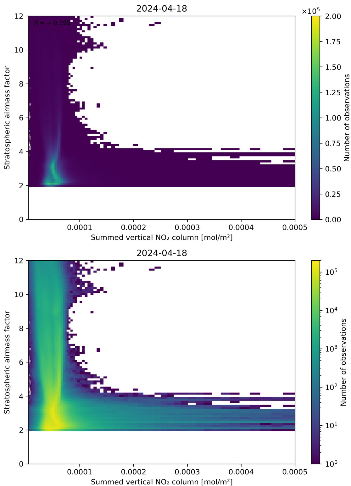
Figure 103: Scatter density plot of “Summed vertical NO 2 column” against “Stratospheric air mass factor” for 2024-04-17 to 2024-04-19.
