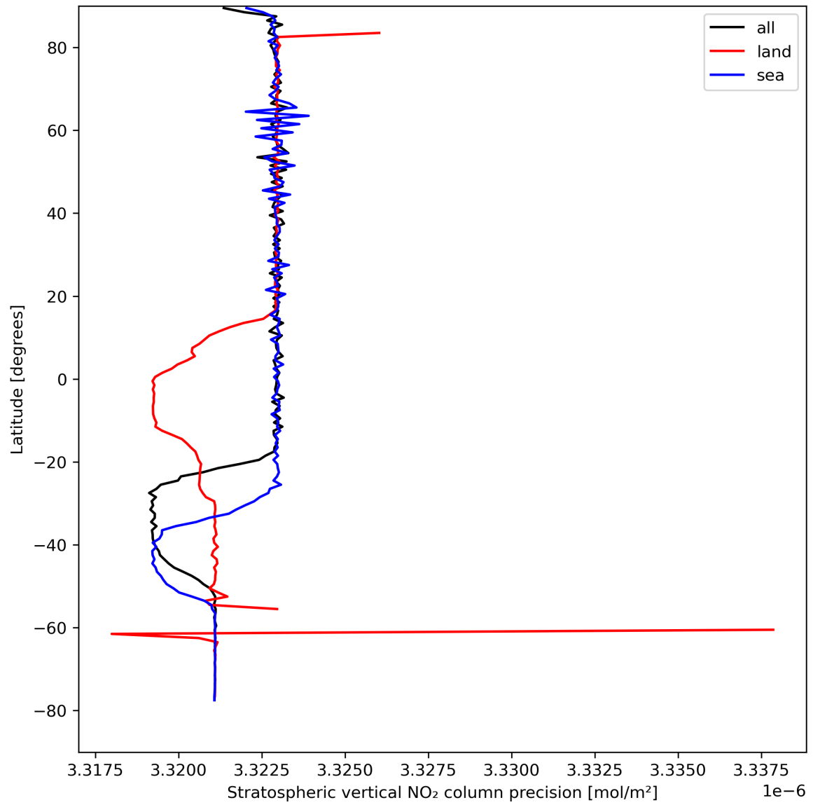
Figure 20: Zonal average of “Stratospheric vertical NO 2 column precision” for 2024-04-17 to 2024-04-19.
