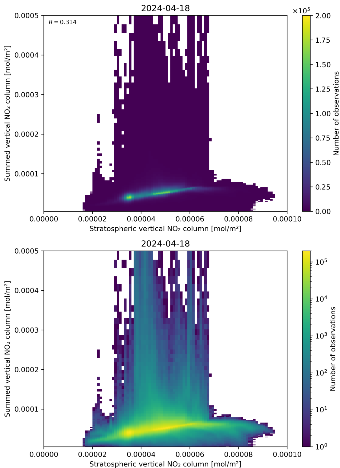
Figure 98: Scatter density plot of “Stratospheric vertical NO 2 column” against “Summed vertical NO 2 column” for 2024-04-17 to 2024-04-19.
