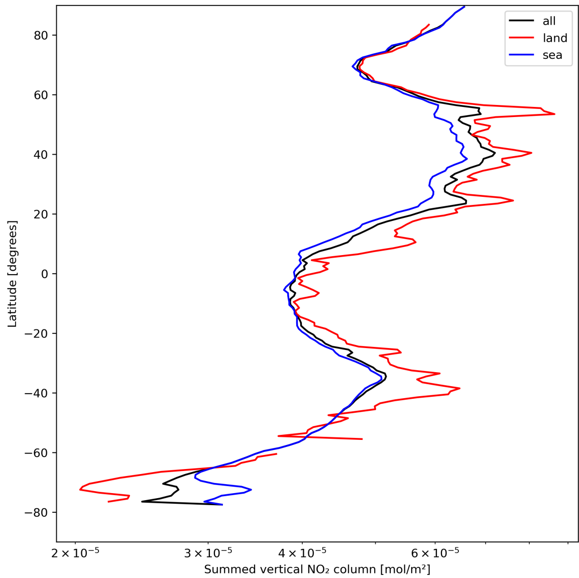
Figure 23: Zonal average of “Summed vertical NO 2 column” for 2024-04-17 to 2024-04-19.
