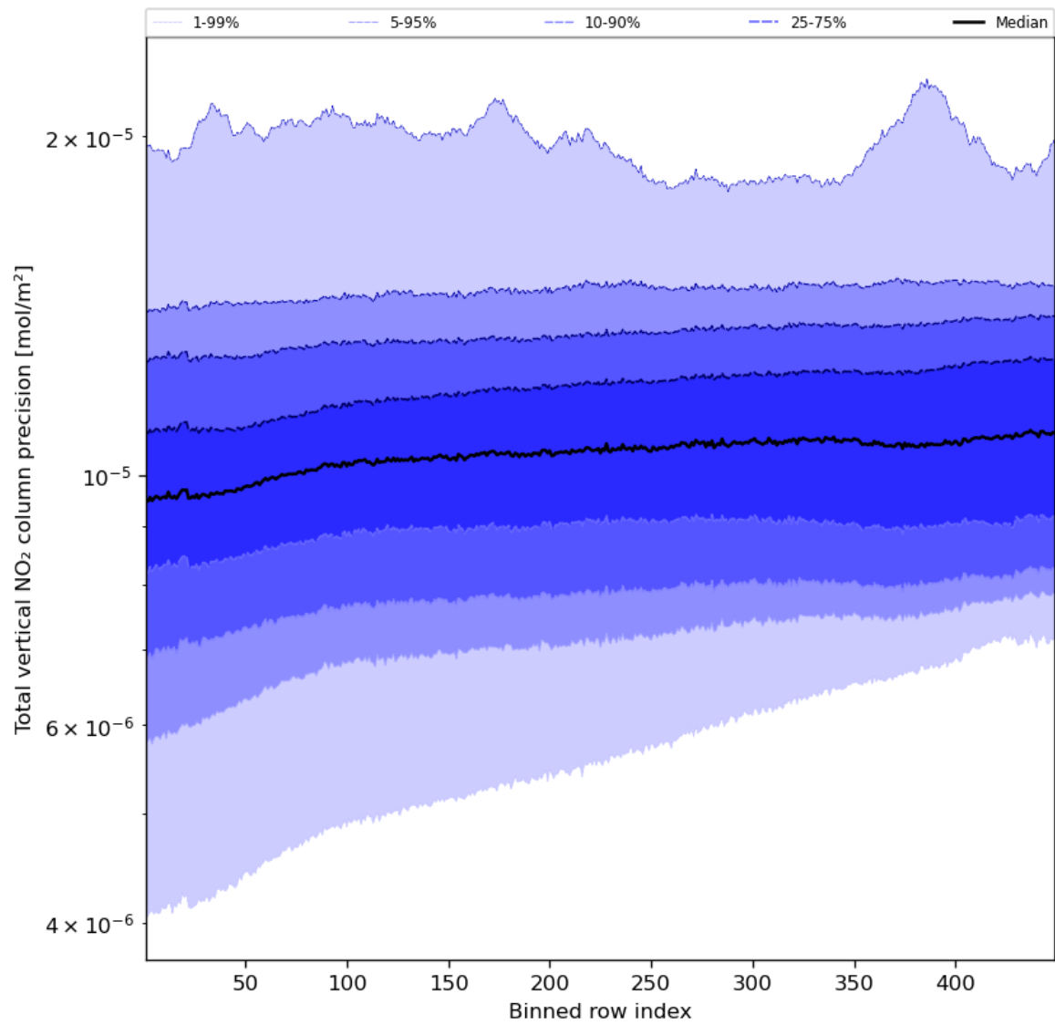
Figure 56: Along track statistics of “Total vertical NO 2 column precision” for 2024-04-17 to 2024-04-19
