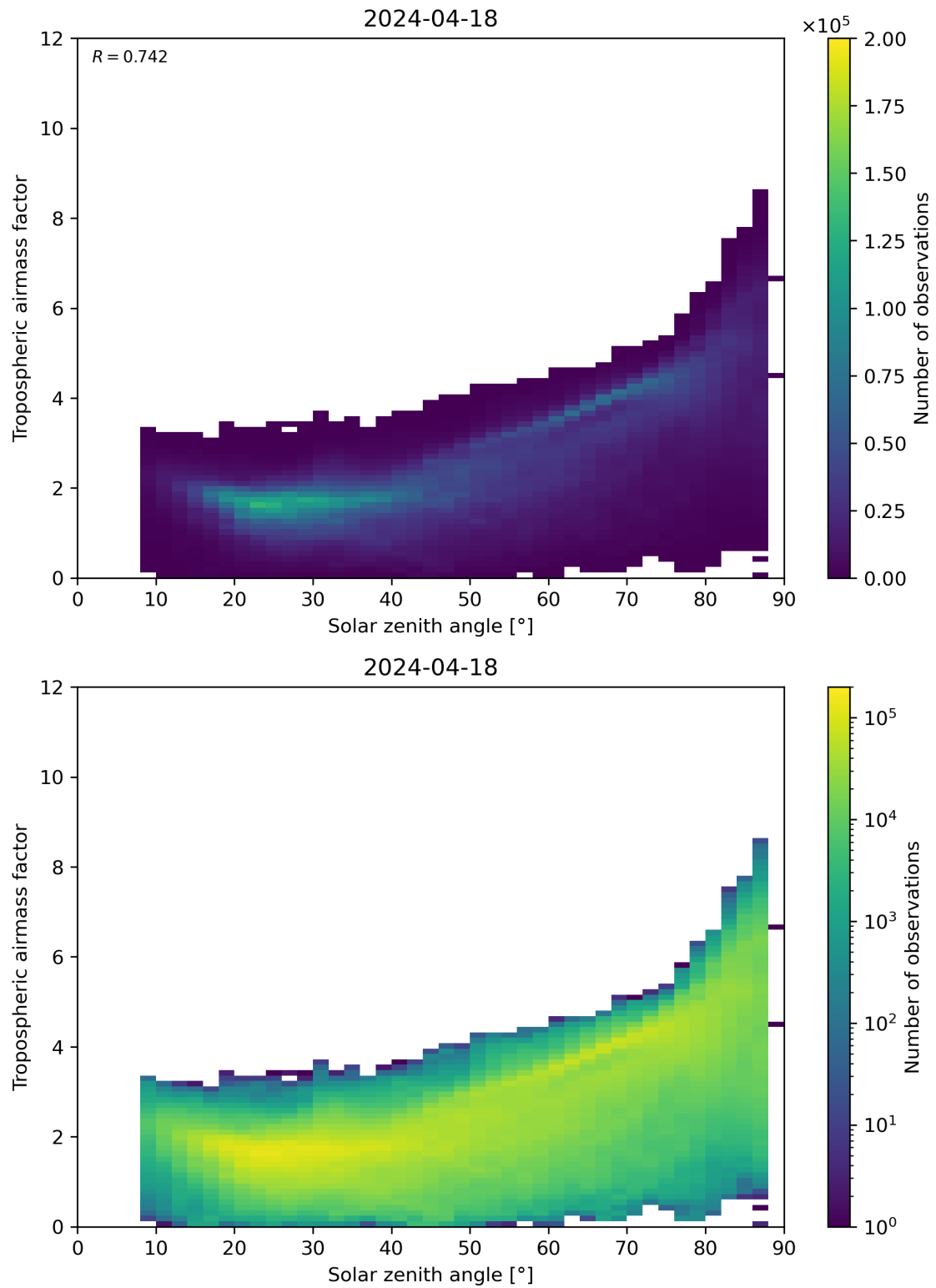
Figure 147: Scatter density plot of “Solar zenith angle” against “Tropospheric airmass factor” for 2024-04-17 to 2024-04-19.
