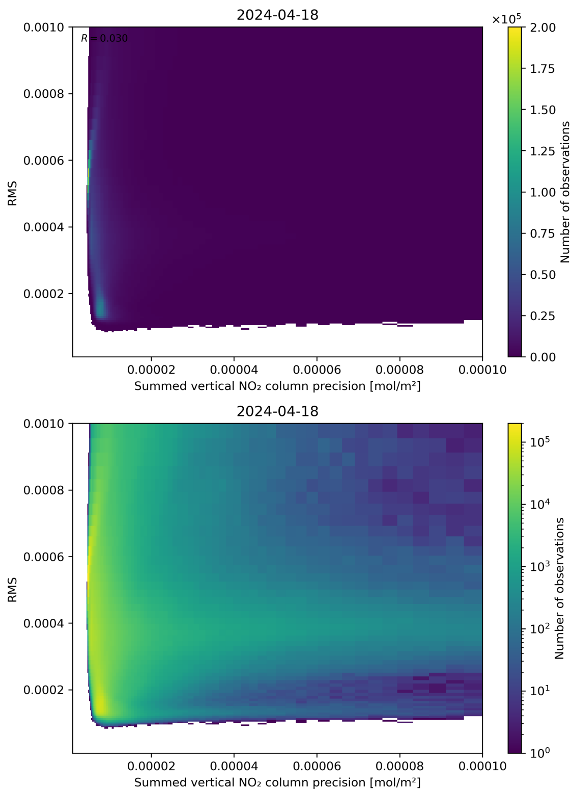
Figure 108: Scatter density plot of “Summed vertical NO 2 column precision” against “RMS” for 2024-04-17 to 2024-04-19.
