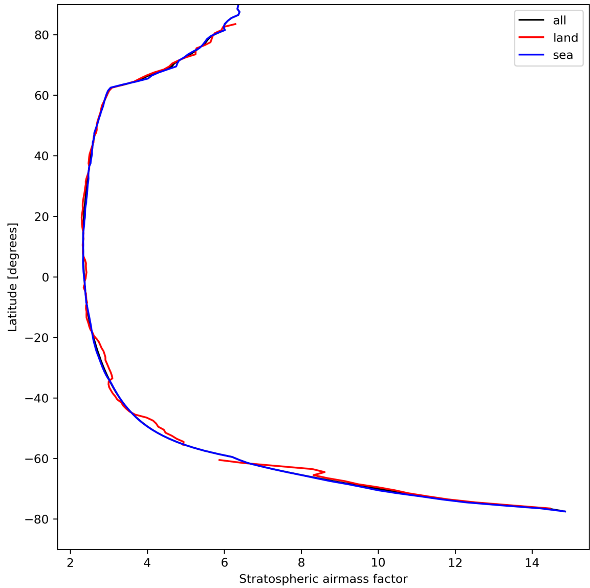
Figure 27: Zonal average of “Stratospheric air mass factor” for 2024-04-17 to 2024-04-19.
