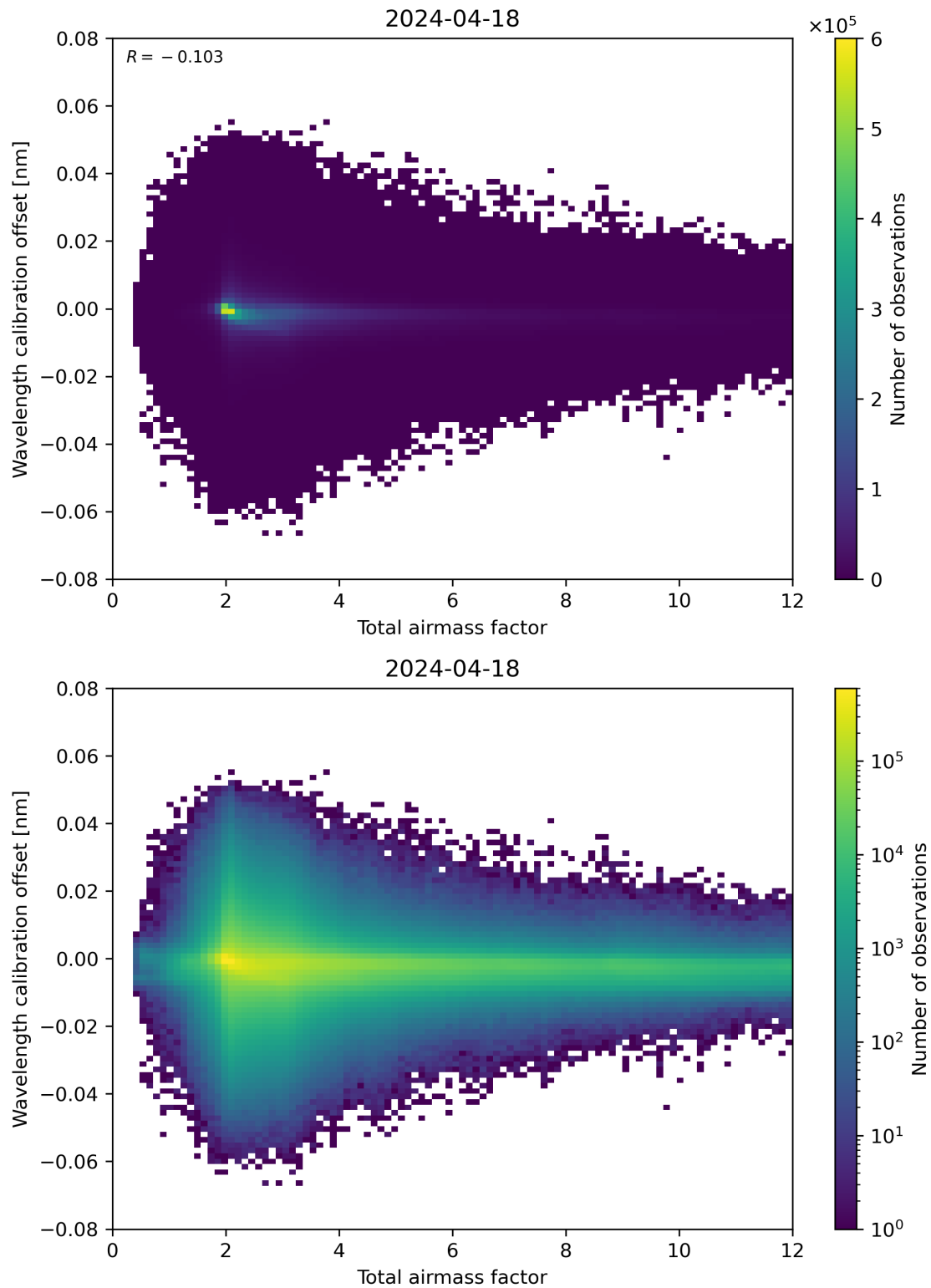
Figure 70: Scatter density plot of “Total airmass factor” against “Wavelength calibration offset” for 2024-04-17 to 2024-04-19.
