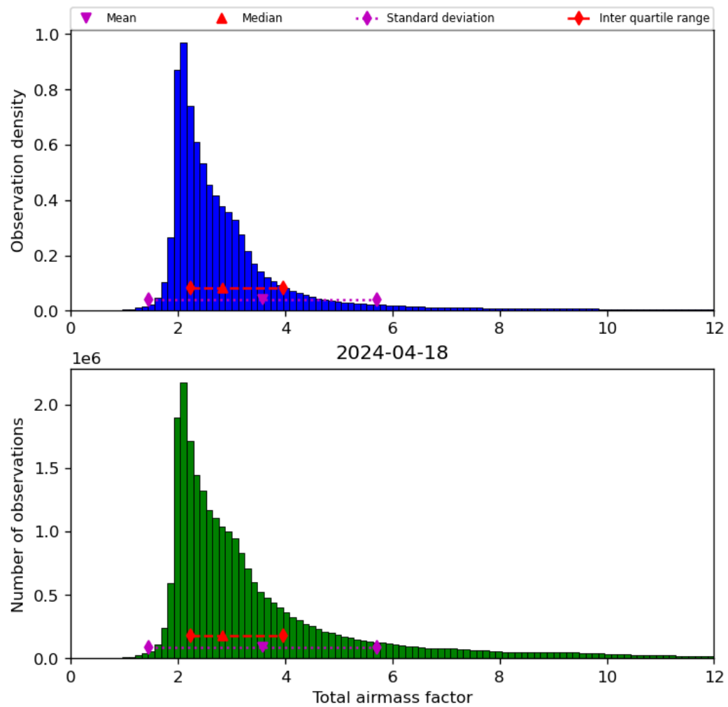
Figure 32: Histogram of “Total airmass factor” for 2024-04-17 to 2024-04-19
