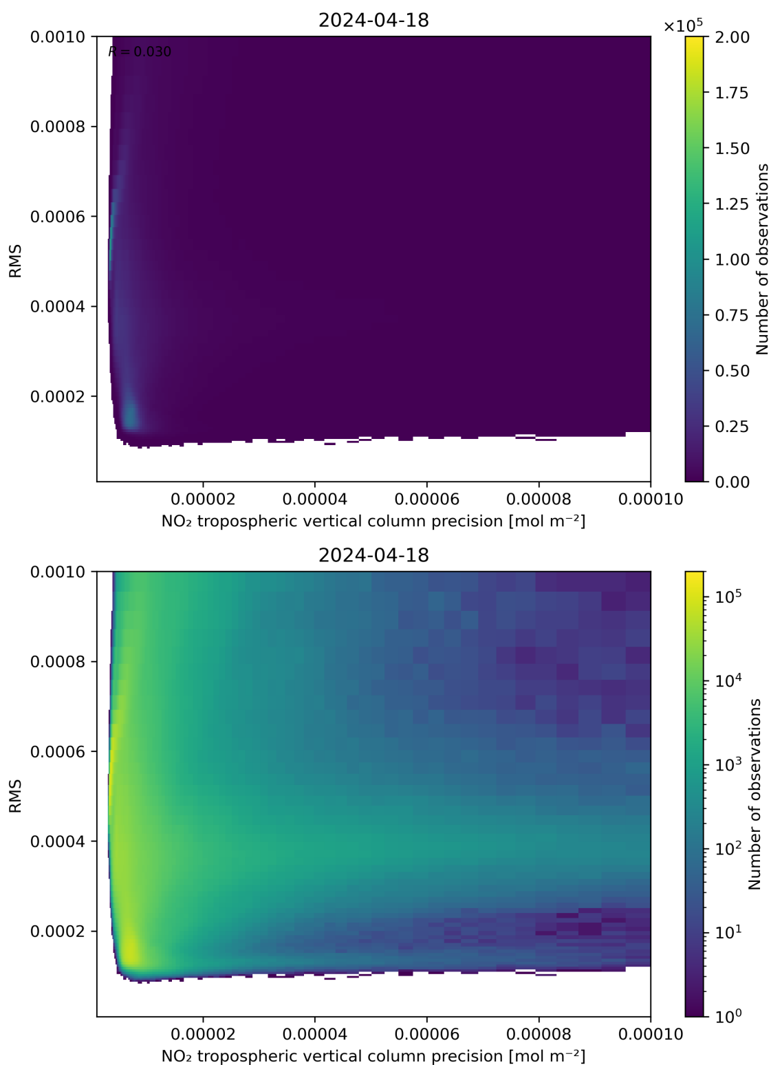
Figure 140: Scatter density plot of “NO 2 tropospheric vertical column precision” against “RMS” for 2024-04-17 to 2024-04-19.
