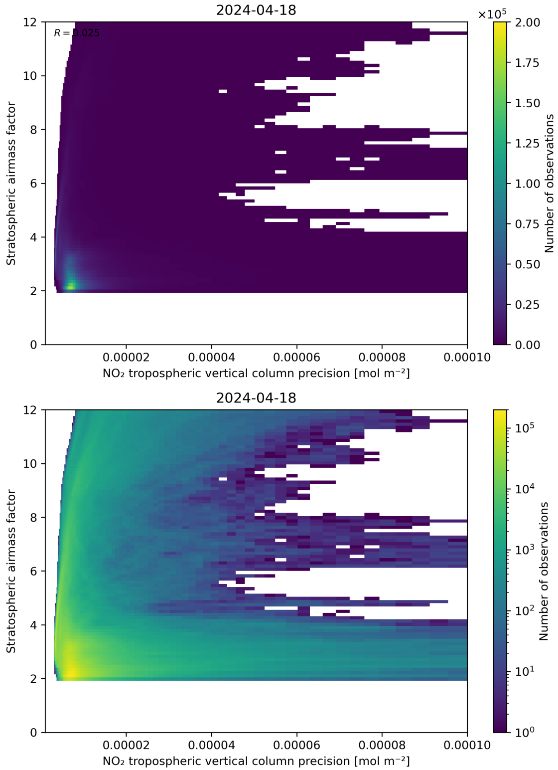
Figure 131: Scatter density plot of “NO 2 tropospheric vertical column precision” against “Stratospheric airmass factor” for 2024-04-17 to 2024-04-19.
