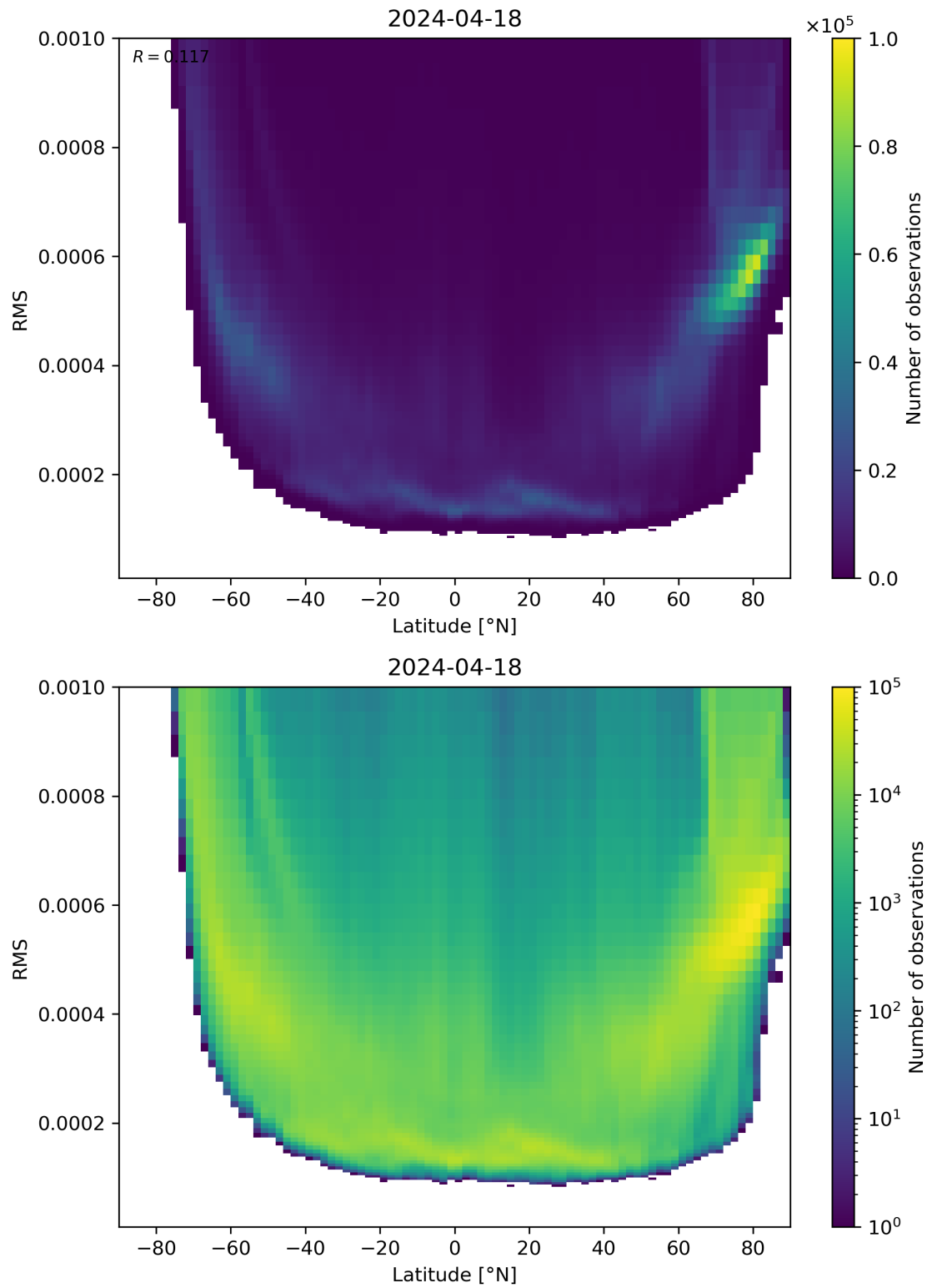
Figure 94: Scatter density plot of “Latitude” against “RMS” for 2024-04-17 to 2024-04-19.
