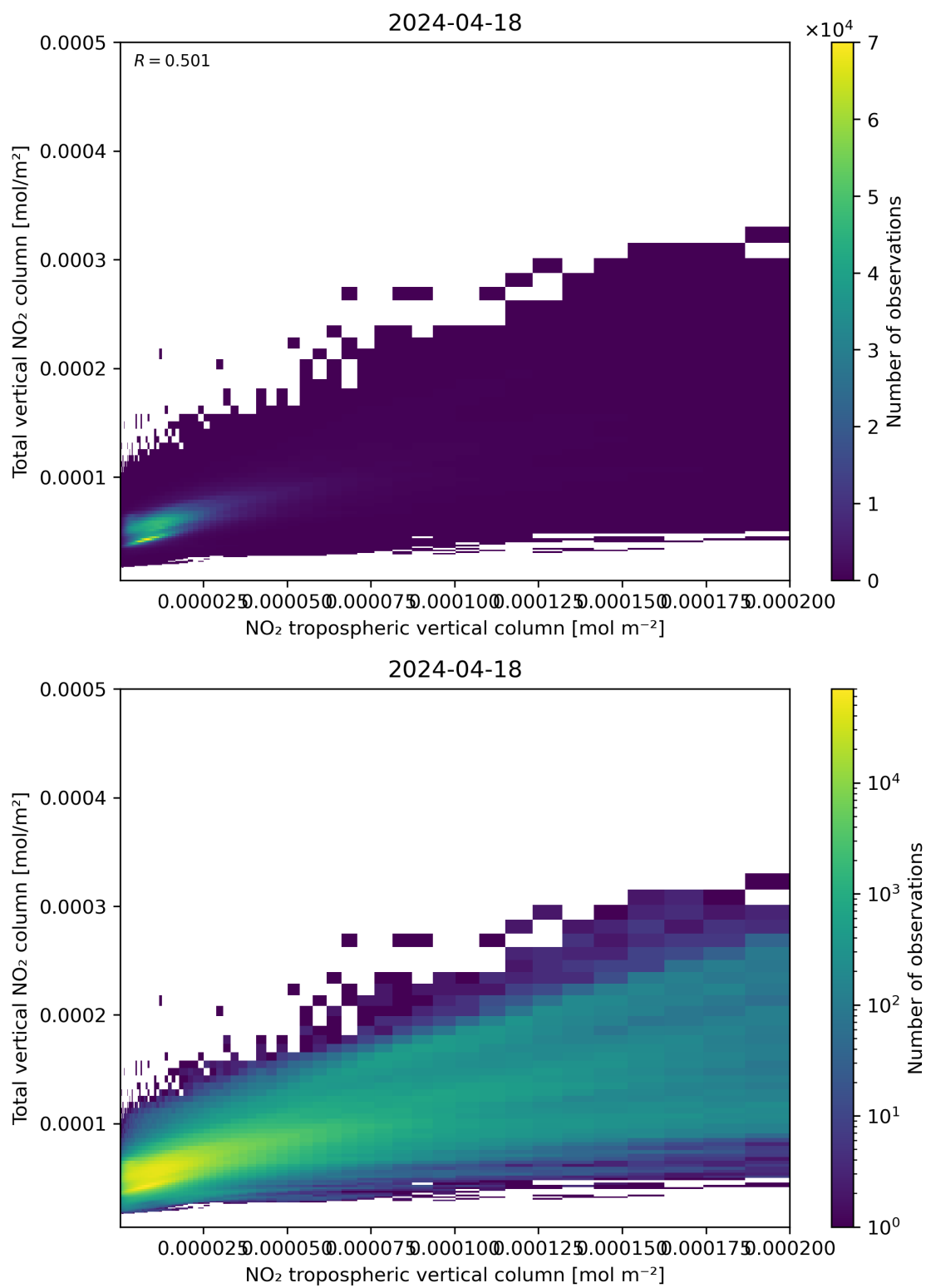
Figure 128: Scatter density plot of “NO 2 tropospheric vertical column” against “Total vertical NO 2 column” for 2024-04-17 to 2024-04-19.
