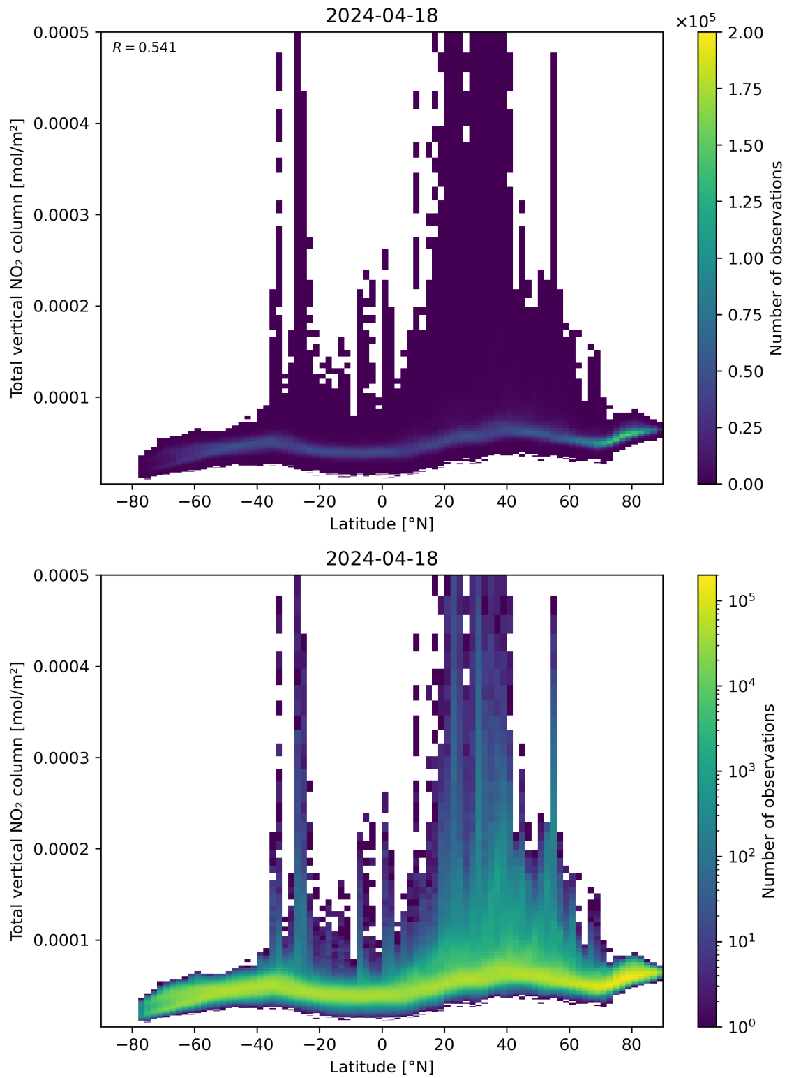
Figure 90: Scatter density plot of “Latitude” against “Total vertical NO 2 column” for 2024-04-17 to 2024-04-19.
