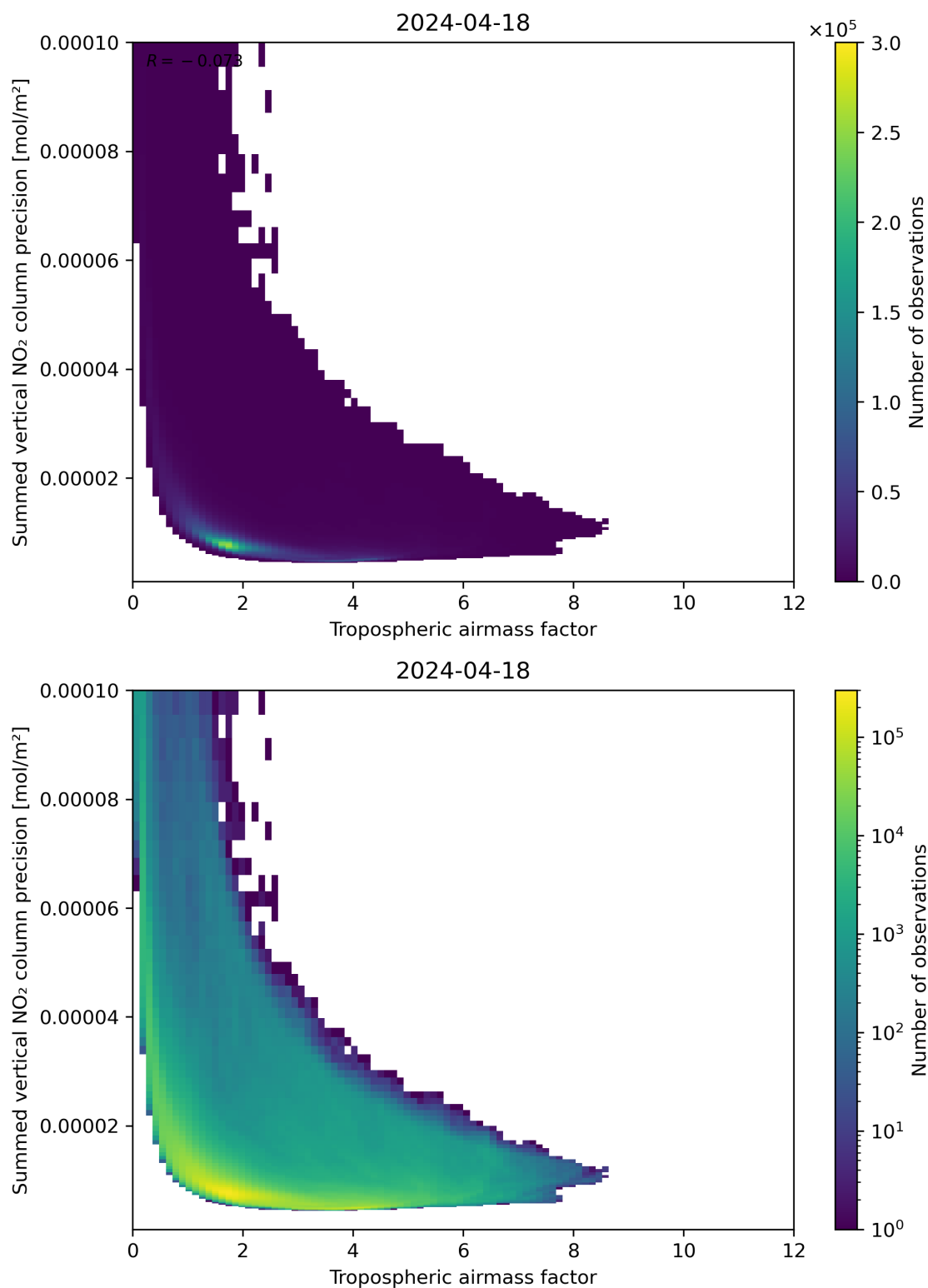
Figure 76: Scatter density plot of “Tropospheric air mass factor” against “Summed vertical NO 2 column precision” for 2024-04-17 to 2024-04-19.
