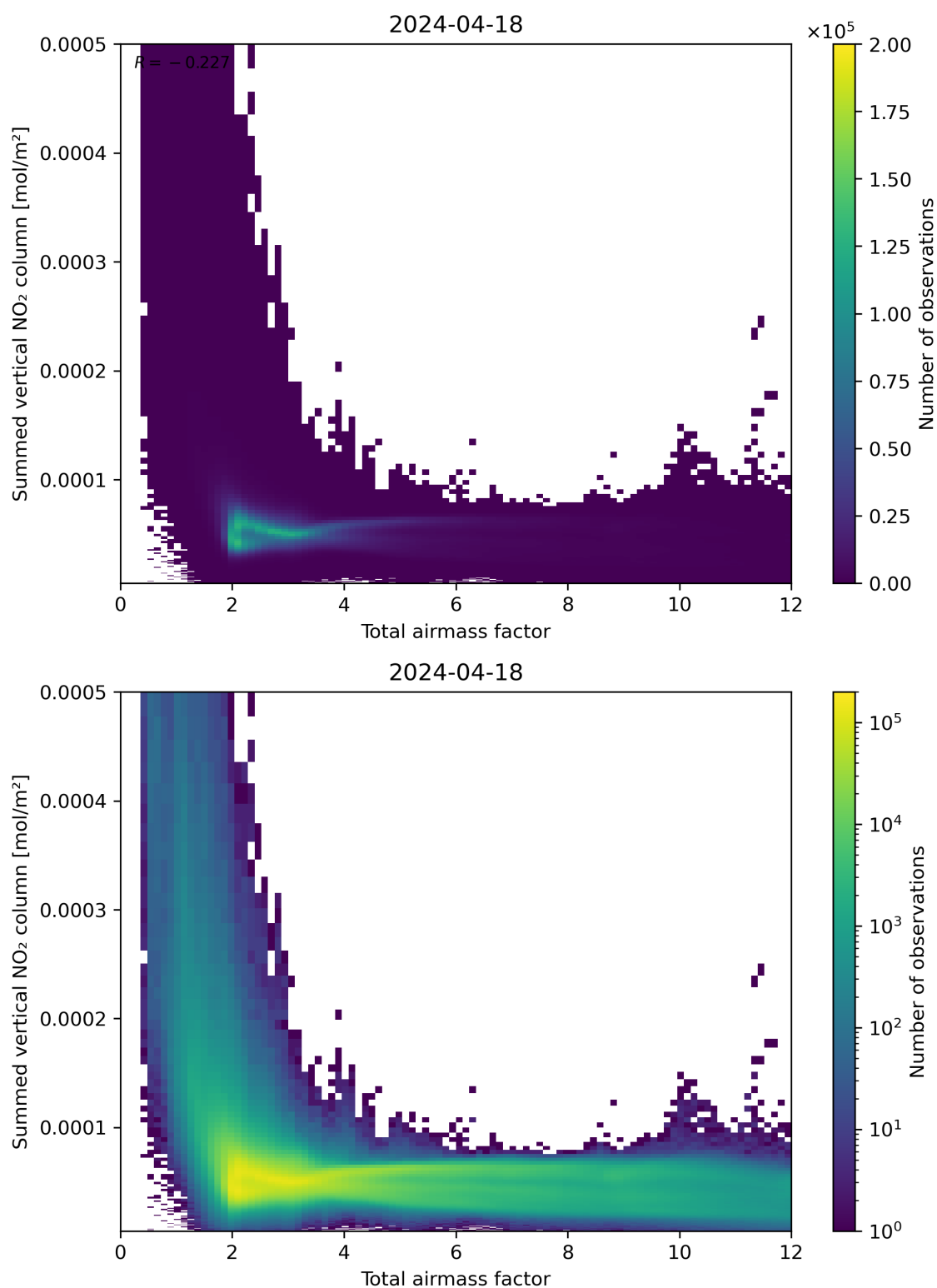
Figure 65: Scatter density plot of “Total airmass factor” against “Summed vertical NO 2 column” for 2024-04-17 to 2024-04-19.
