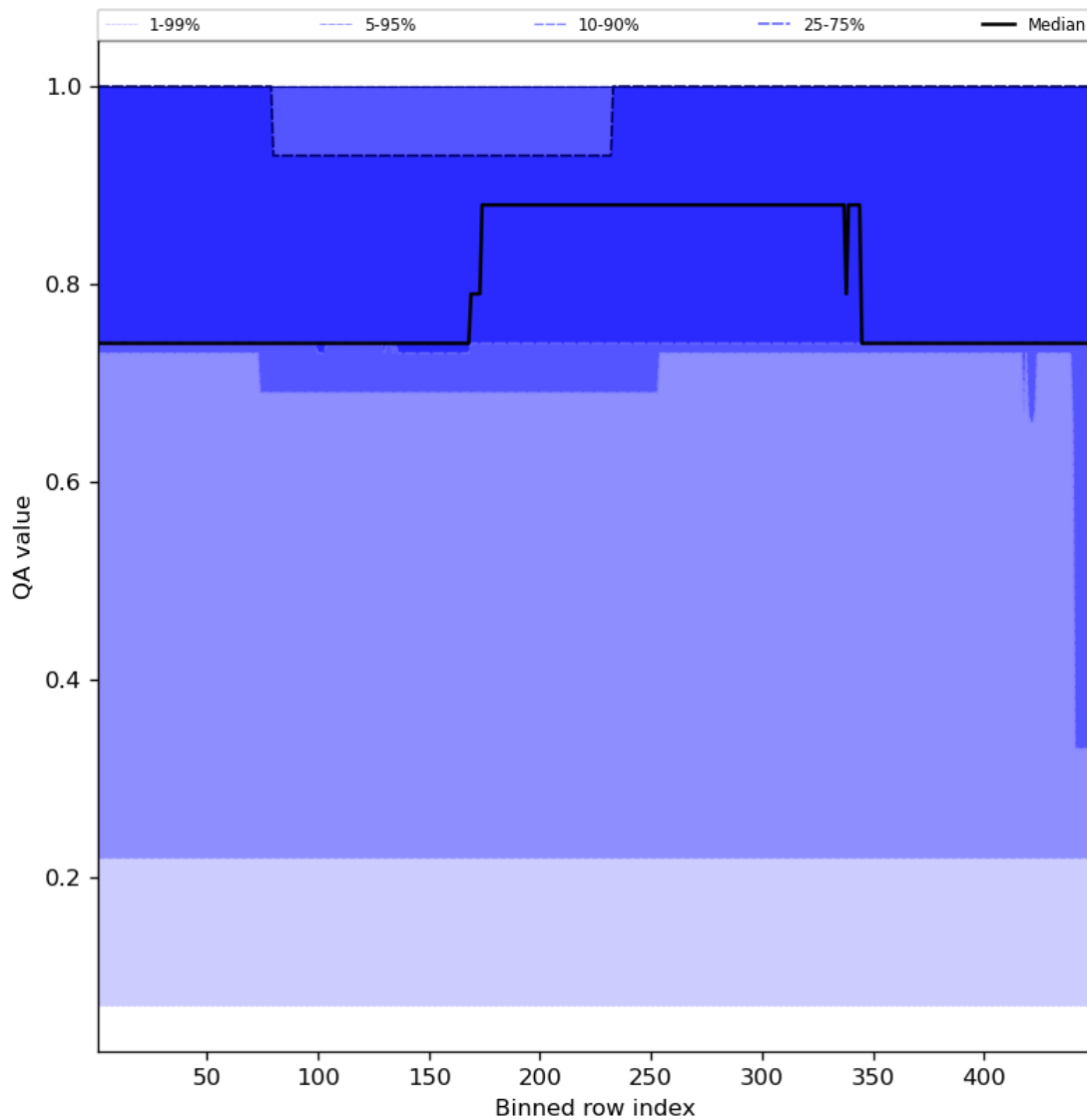
Figure 45: Along track statistics of “QA value” for 2024-04-17 to 2024-04-19
