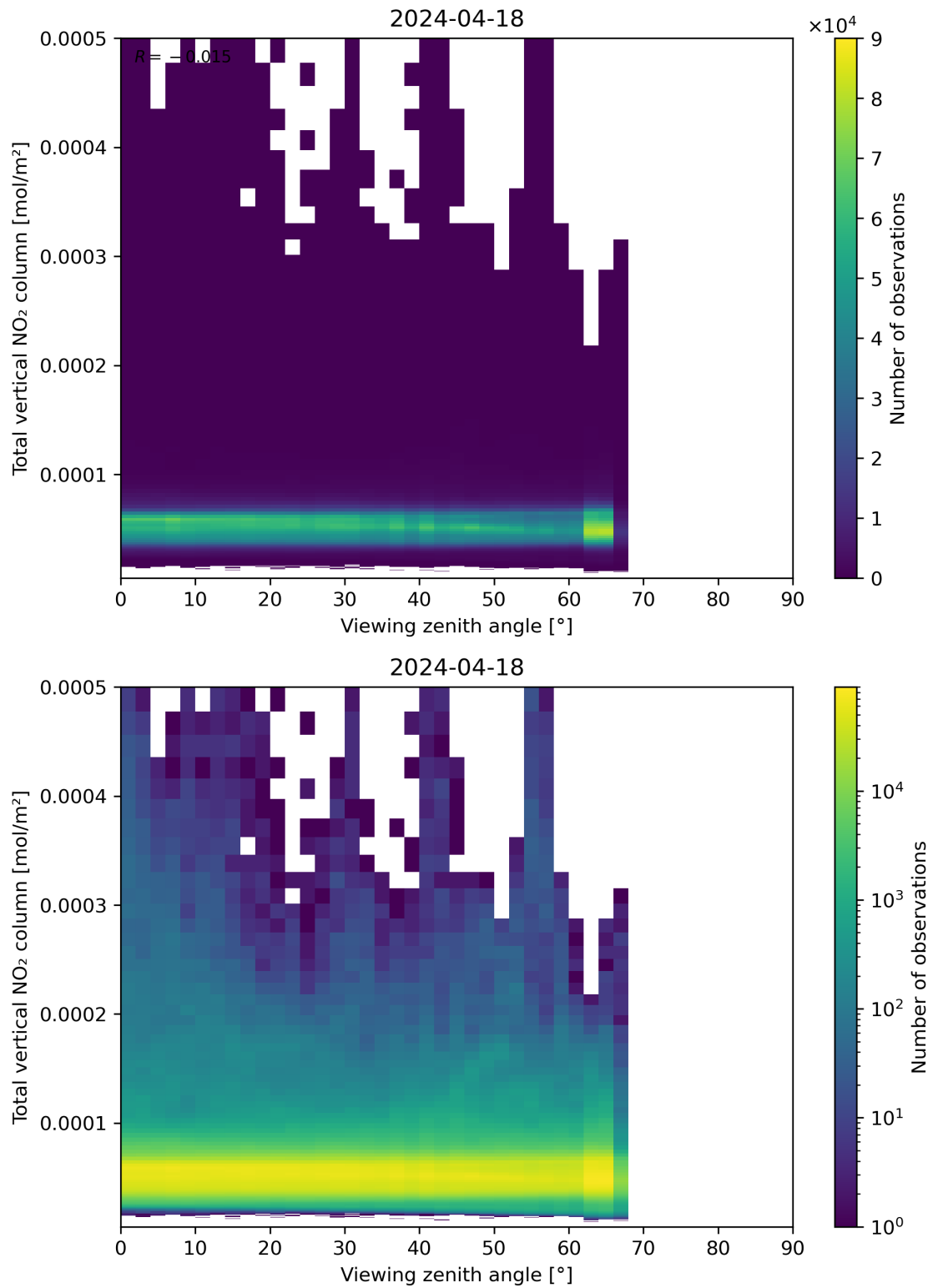
Figure 167: Scatter density plot of “Viewing zenith angle” against “Total vertical NO 2 column” for 2024-04-17 to 2024-04-19.
