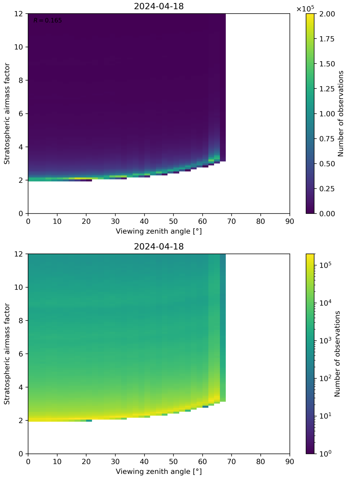
Figure 159: Scatter density plot of “Viewing zenith angle” against “Stratospheric airmass factor” for 2024-04-17 to 2024-04-19.
