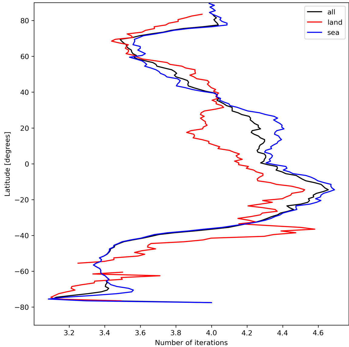
Figure 17: Zonal average of “Number of iterations” for 2024-04-17 to 2024-04-19.
