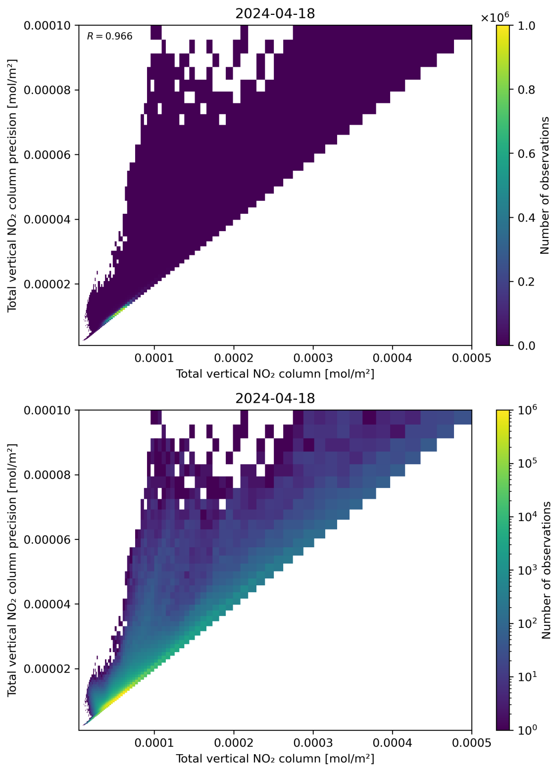
Figure 114: Scatter density plot of “Total vertical NO 2 column” against “Total vertical NO 2 column precision” for 2024-04-17 to 2024-04-19.
