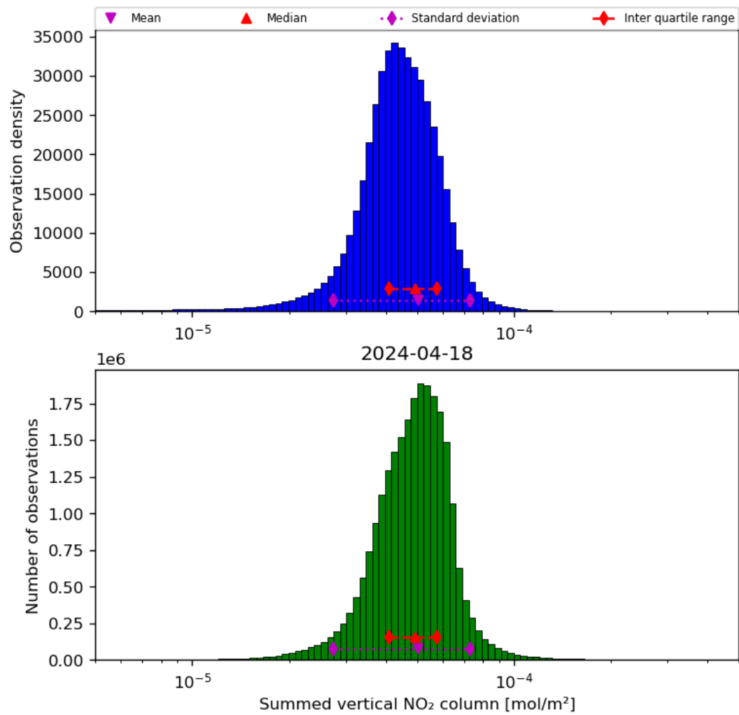
Figure 40: Histogram of “Summed vertical NO 2 column” for 2024-04-17 to 2024-04-19
