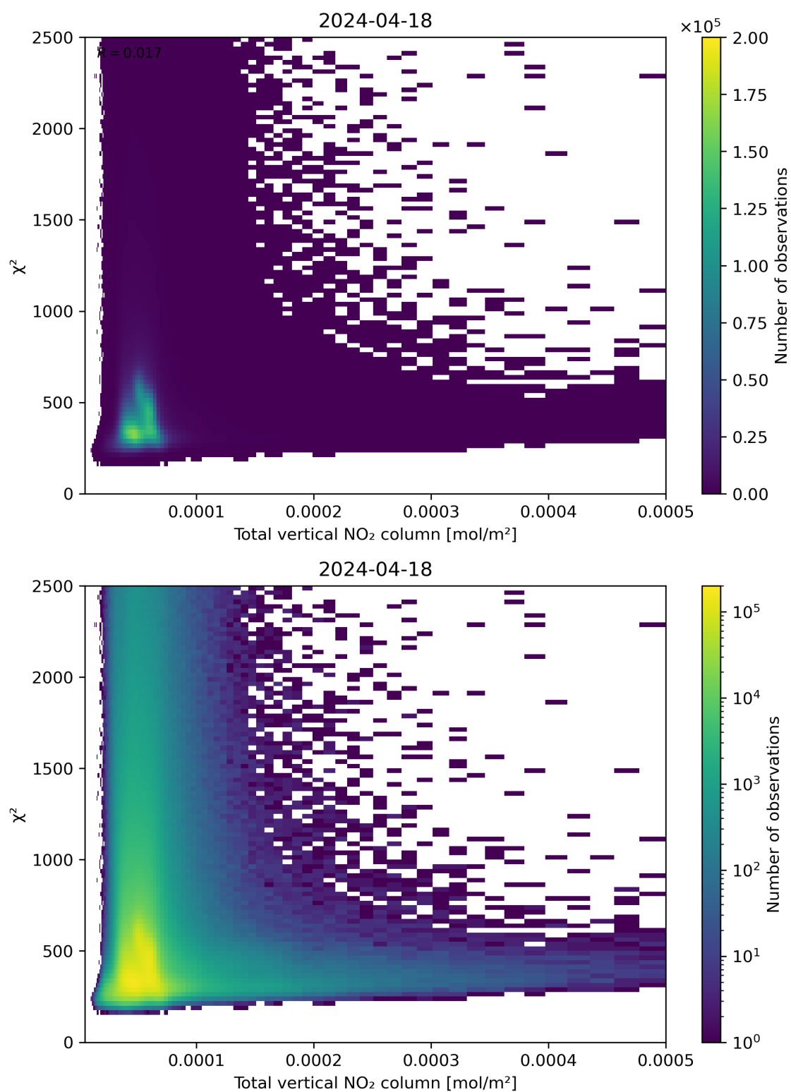
Figure 111: Scatter density plot of “Total vertical NO 2 column” against “ \chi^2 ” for 2024-04-17 to 2024-04-19.
