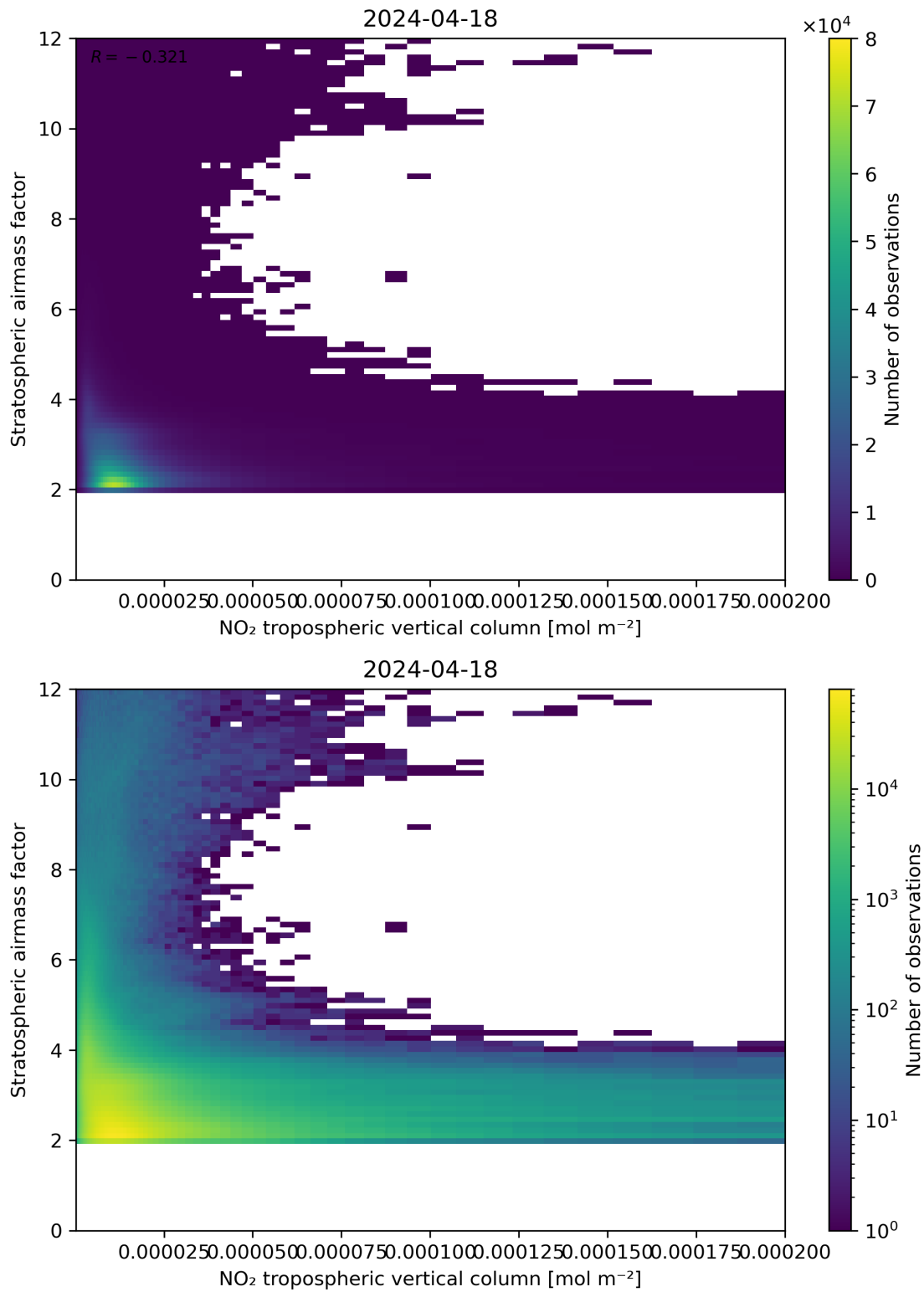
Figure 121: Scatter density plot of “NO 2 tropospheric vertical column” against “Stratospheric air mass factor” for 2024-04-17 to 2024-04-19.
