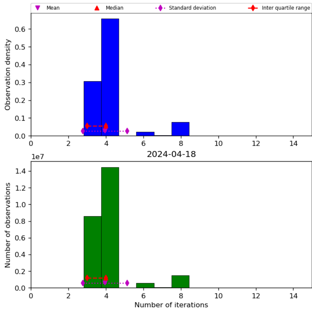
Figure 34: Histogram of “Number of iterations” for 2024-04-17 to 2024-04-19
