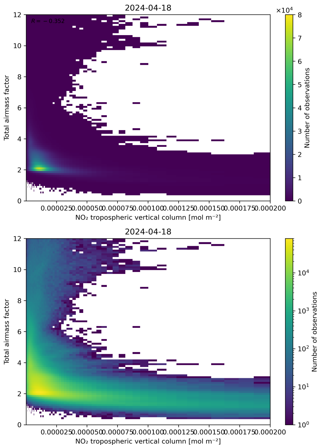
Figure 122: Scatter density plot of “NO 2 tropospheric vertical column” against “Total air mass factor” for 2024-04-17 to 2024-04-19.
