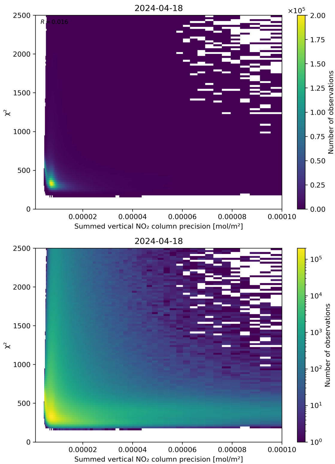
Figure 107: Scatter density plot of “Summed vertical NO 2 column precision” against “ \chi^2 ” for 2024-04-17 to 2024-04-19.
