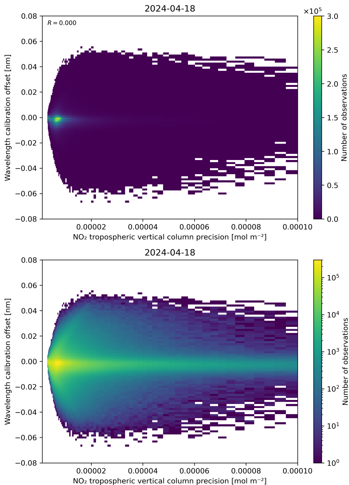
Figure 141: Scatter density plot of “NO 2 tropospheric vertical column precision” against “Wavelength calibration offset” for 2024-04-17 to 2024-04-19.
