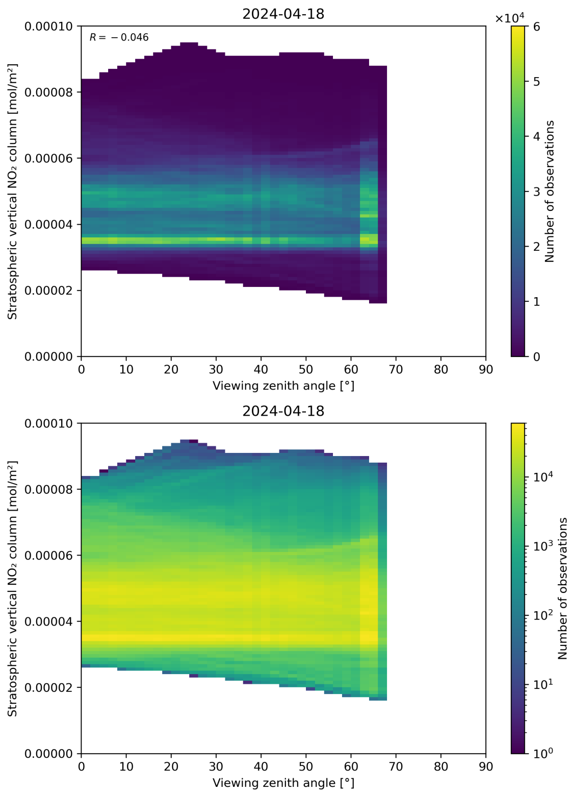
Figure 164: Scatter density plot of “Viewing zenith angle” against “Stratospheric vertical NO 2 column” for 2024-04-17 to 2024-04-19.
