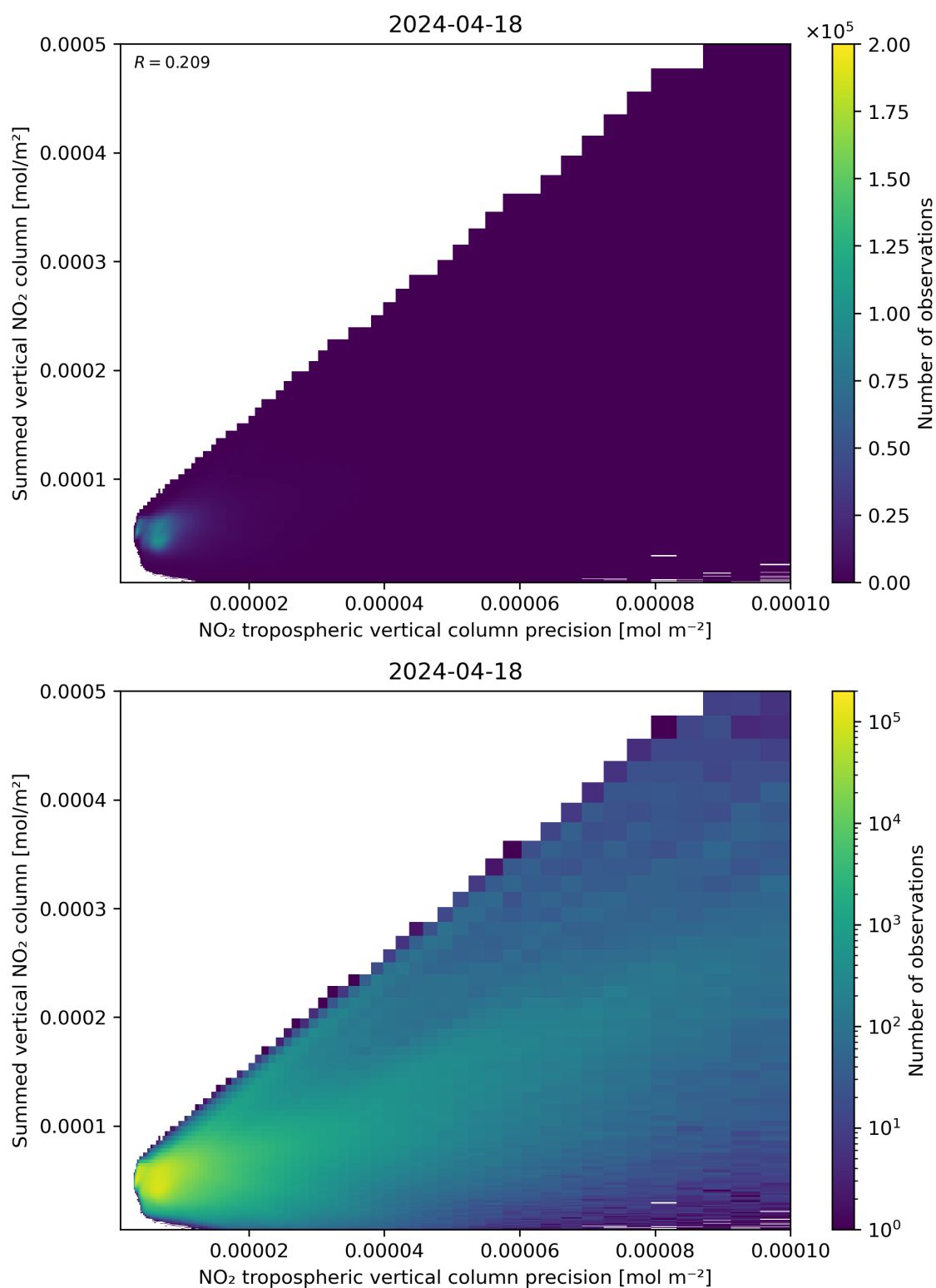
Figure 136: Scatter density plot of “NO 2 tropospheric vertical column precision” against “Summed vertical NO 2 column” for 2024-04-17 to 2024-04-19.
