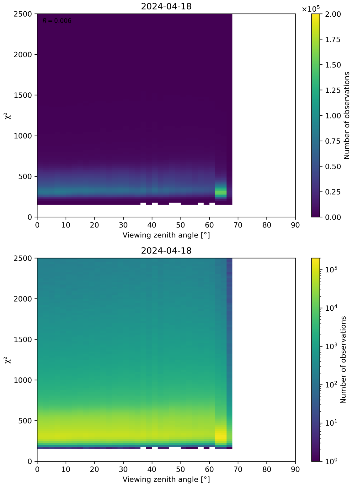
Figure 162: Scatter density plot of “Viewing zenith angle” against “ \chi^2 ” for 2024-04-17 to 2024-04-19.
