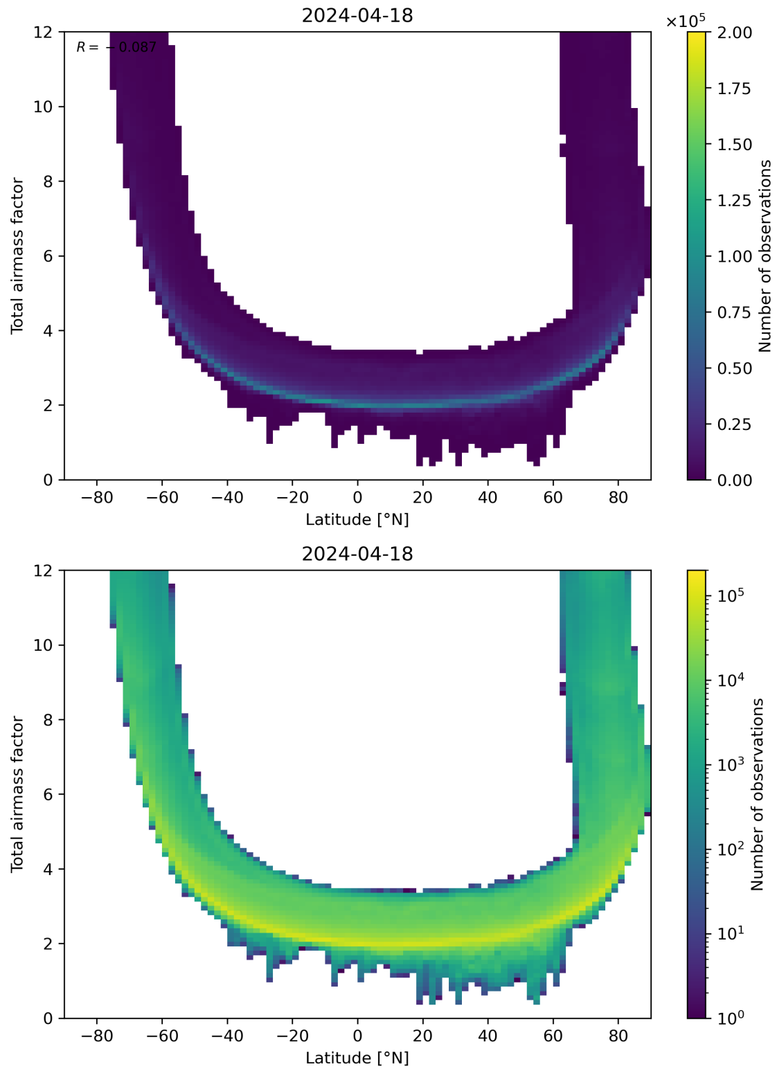
Figure 84: Scatter density plot of “Latitude” against “Total airmass factor” for 2024-04-17 to 2024-04-19.
