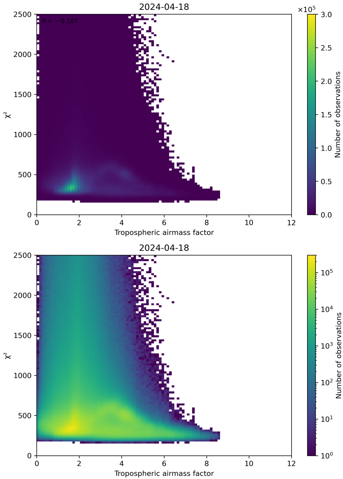
Figure 73: Scatter density plot of “Tropospheric airmass factor” against “ \chi^2 ” for 2024-04-17 to 2024-04-19.
