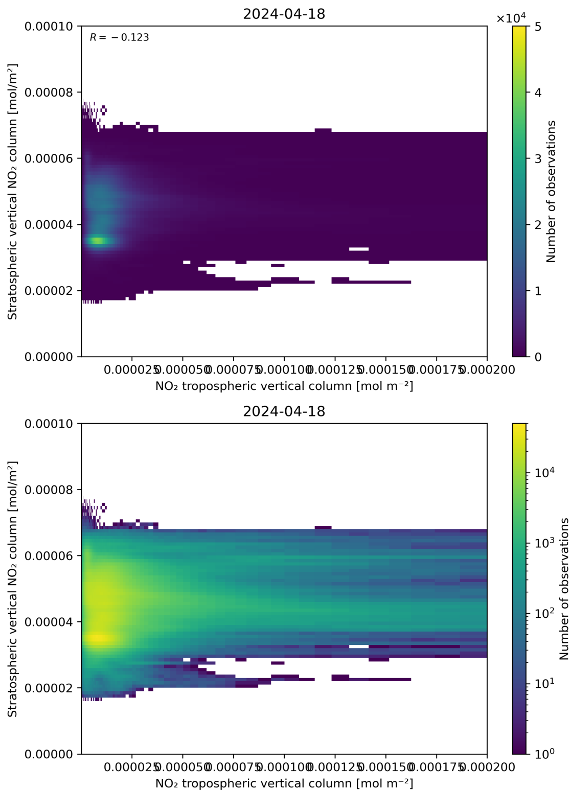
Figure 125: Scatter density plot of “NO 2 tropospheric vertical column” against “Stratospheric vertical NO 2 column” for 2024-04-17 to 2024-04-19.
