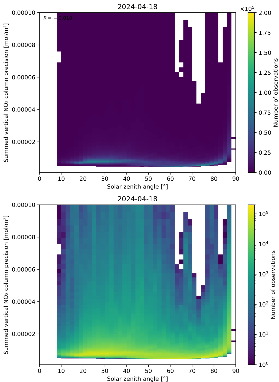
Figure 152: Scatter density plot of “Solar zenith angle” against “Summed vertical NO 2 column precision” for 2024-04-17 to 2024-04-19.
