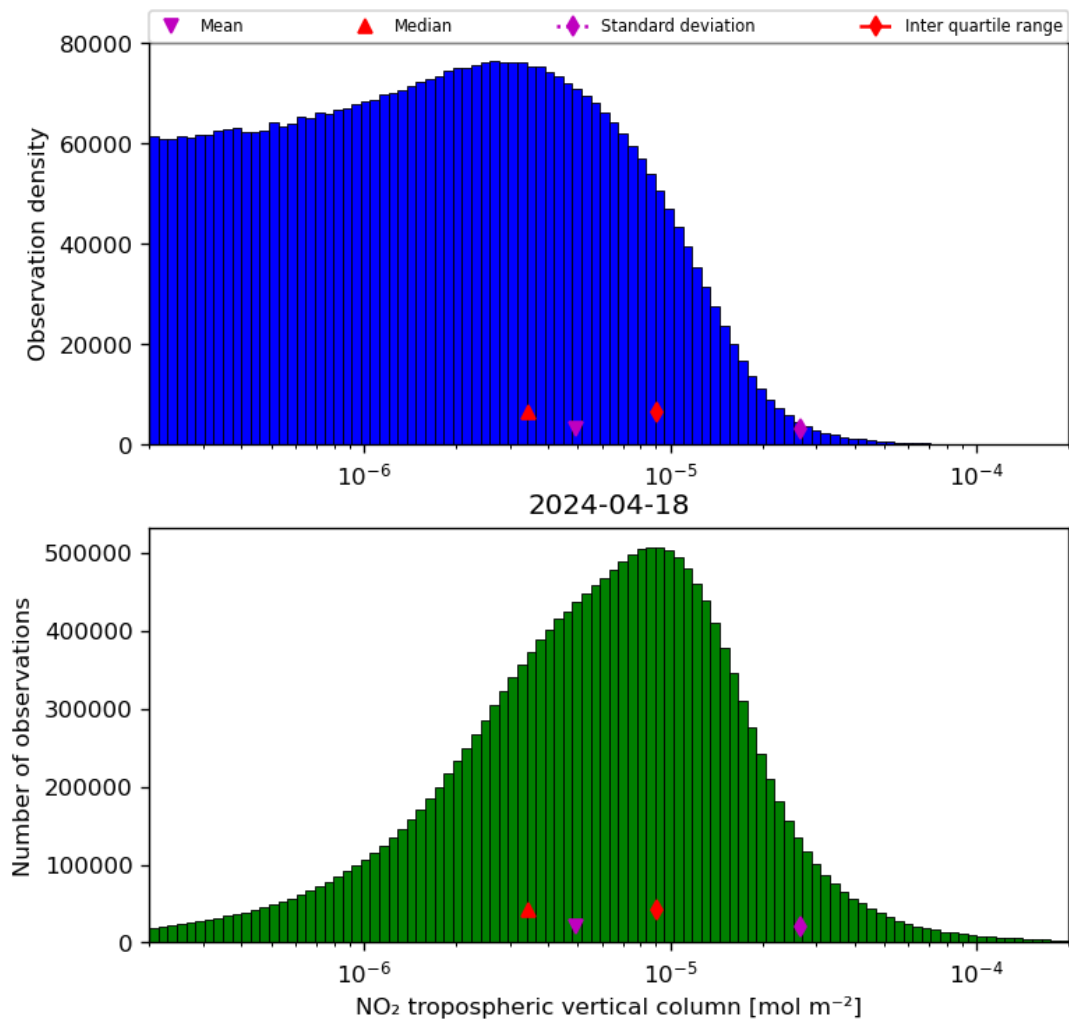
Figure 29: Histogram of “NO 2 tropospheric vertical column” for 2024-04-17 to 2024-04-19
