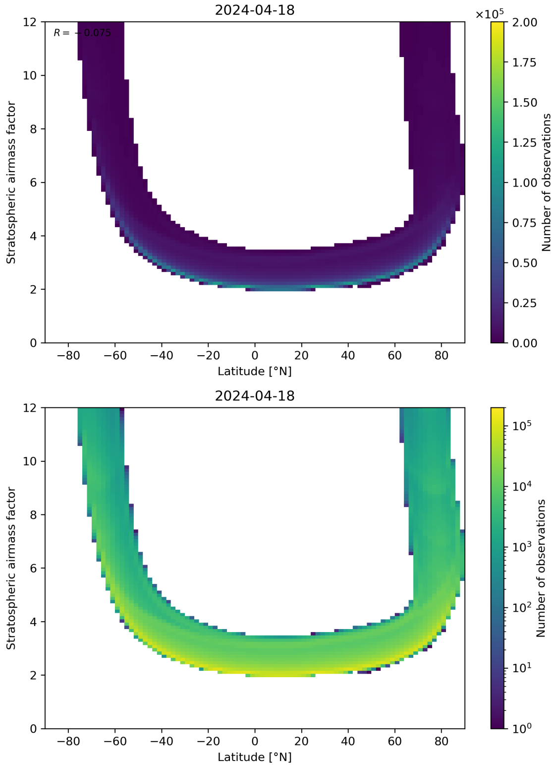
Figure 83: Scatter density plot of “Latitude” against “Stratospheric air mass factor” for 2024-04-17 to 2024-04-19.
