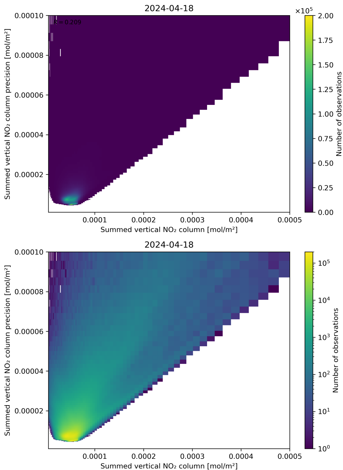
Figure 105: Scatter density plot of “Summed vertical NO 2 column” against “Summed vertical NO 2 column precision” for 2024-04-17 to 2024-04-19.
