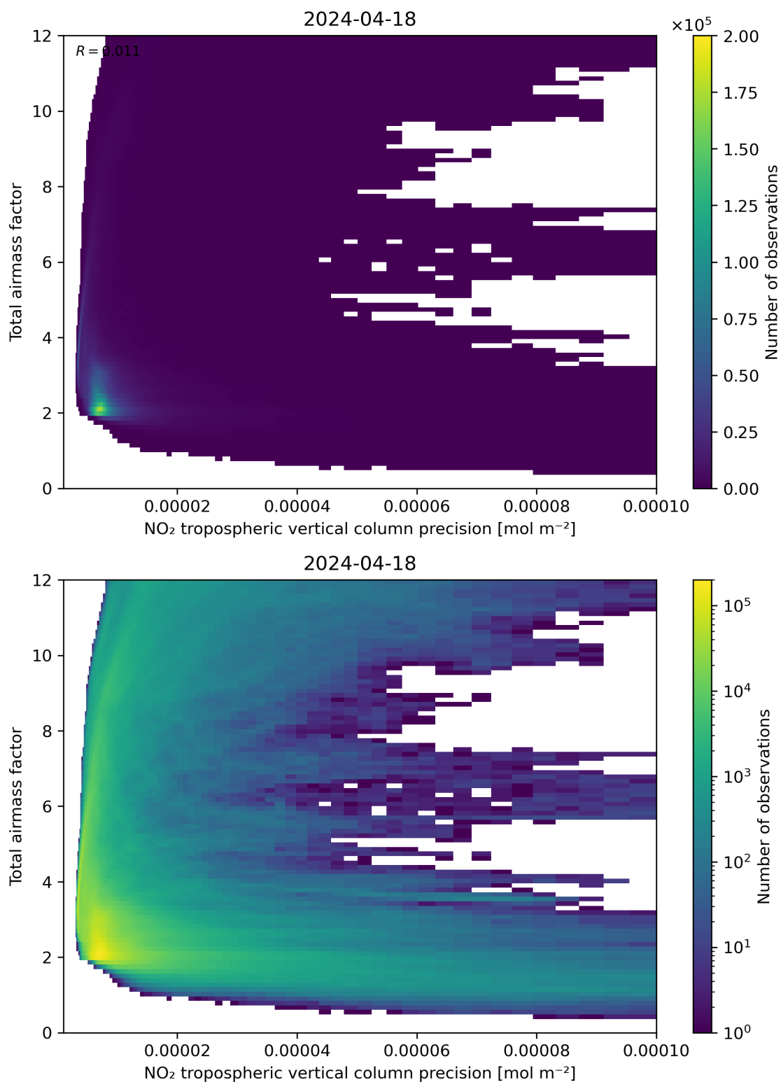
Figure 132: Scatter density plot of “NO 2 tropospheric vertical column precision” against “Total air mass factor” for 2024-04-17 to 2024-04-19.
