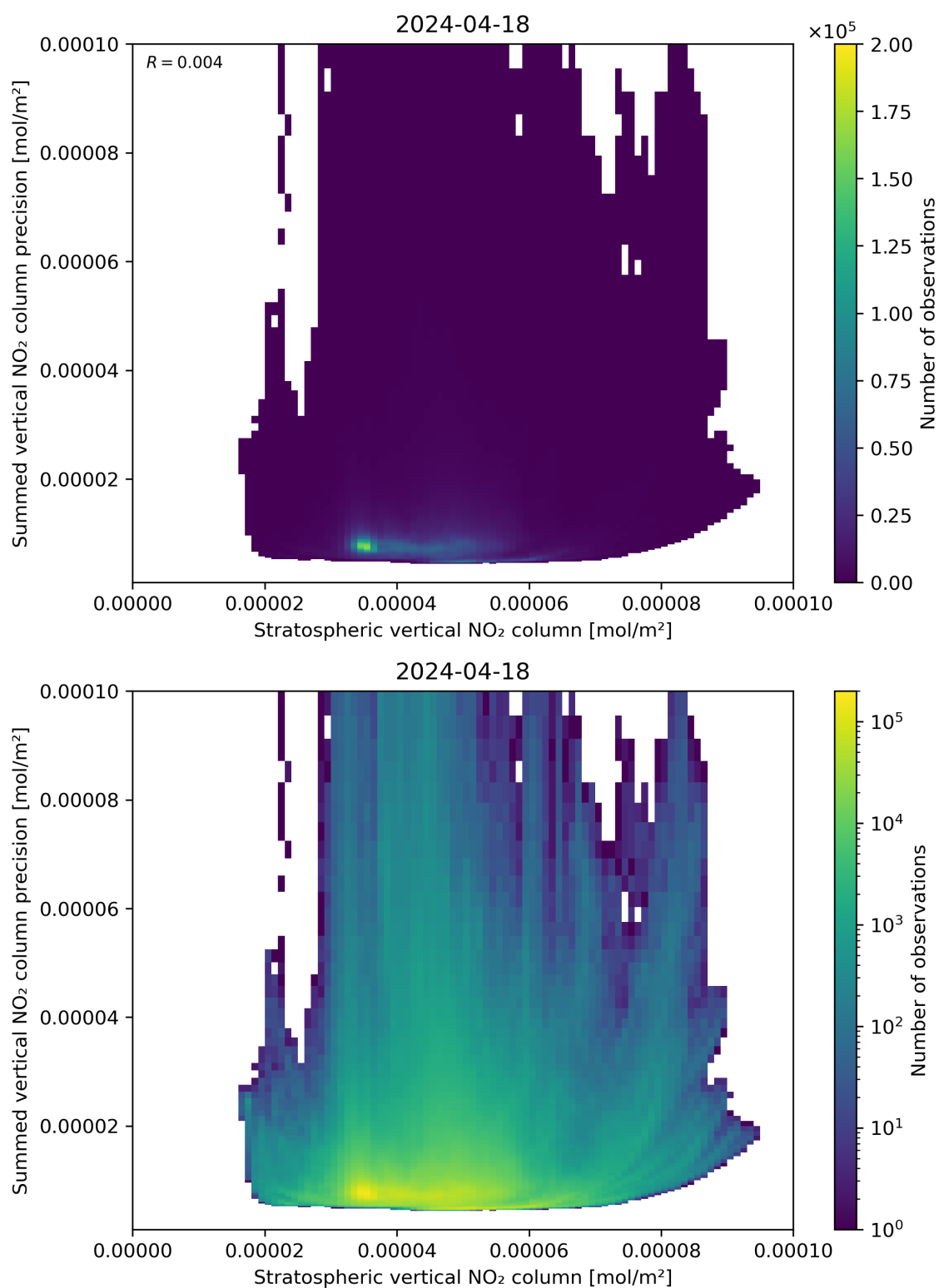
Figure 99: Scatter density plot of “Stratospheric vertical NO 2 column” against “Summed vertical NO 2 column precision” for 2024-04-17 to 2024-04-19.
