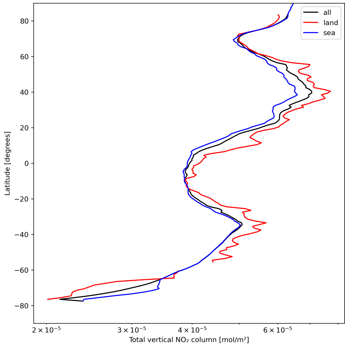
Figure 21: Zonal average of “Total vertical NO 2 column” for 2024-04-17 to 2024-04-19.
