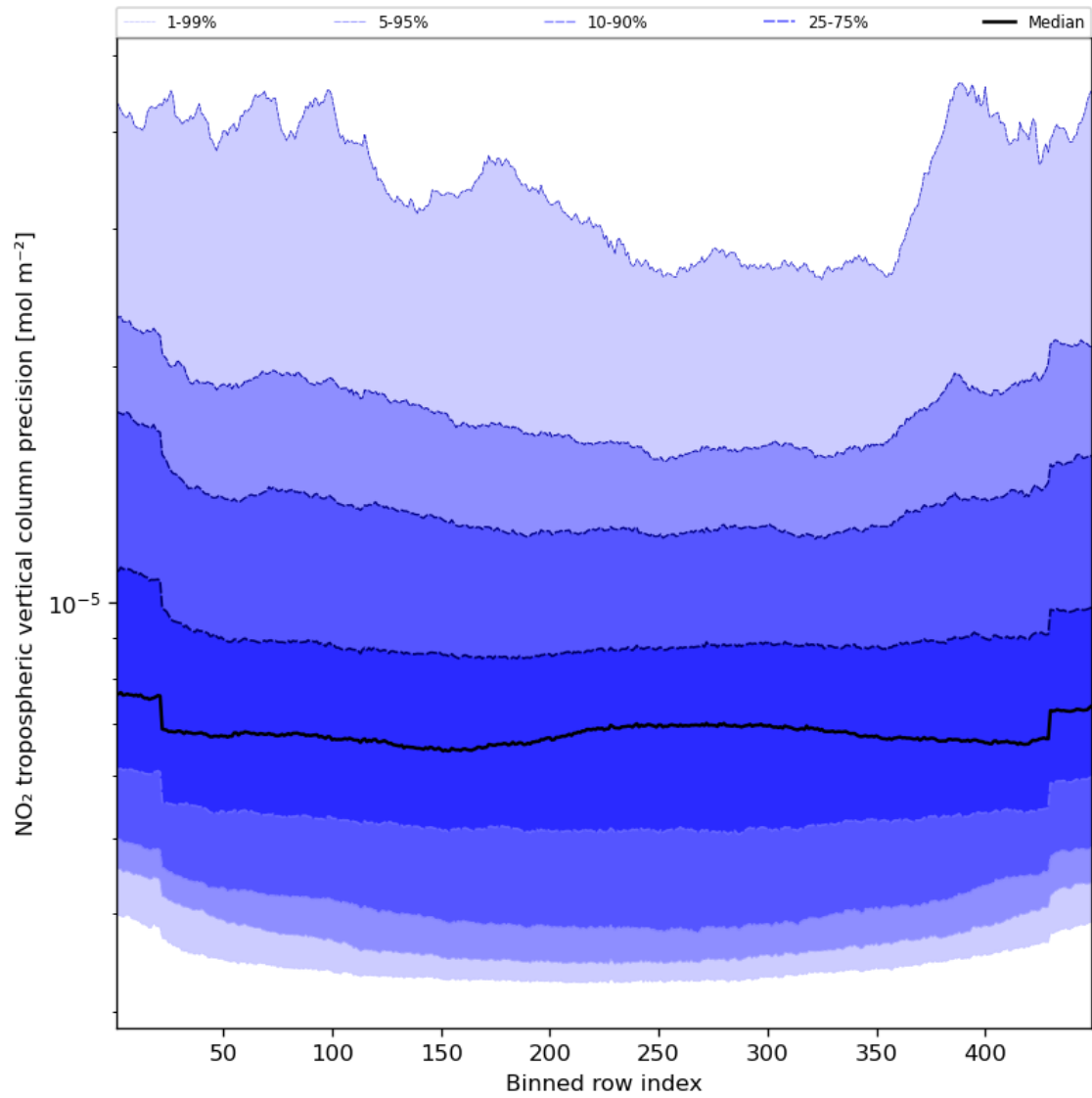
Figure 47: Along track statistics of “NO 2 tropospheric vertical column precision” for 2024-04-17 to 2024-04-19
