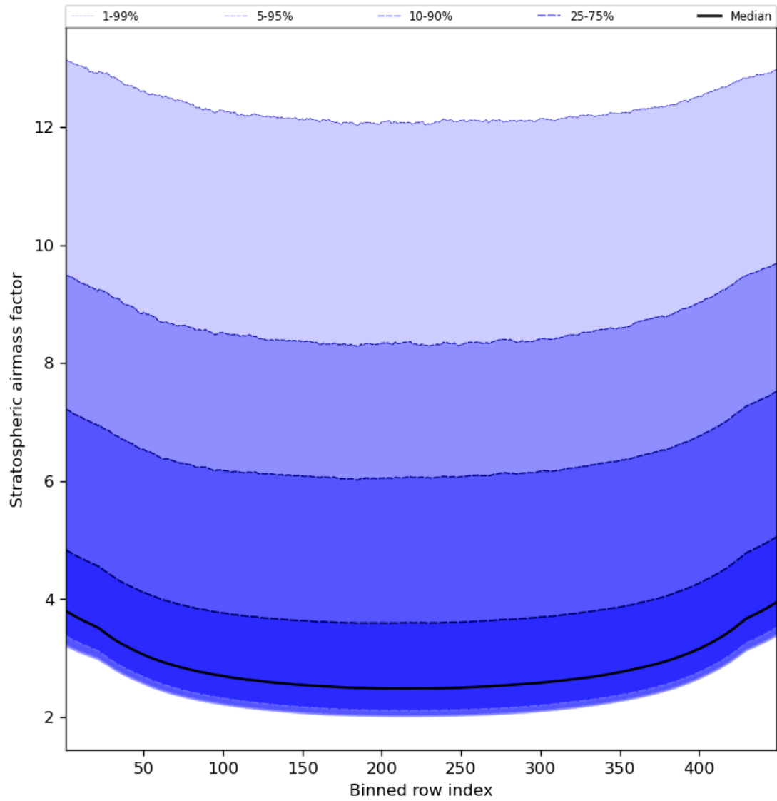
Figure 61: Along track statistics of “Stratospheric air mass factor” for 2024-04-17 to 2024-04-19
