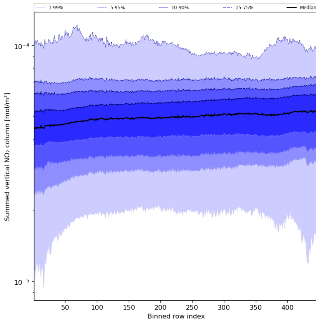
Figure 57: Along track statistics of “Summed vertical NO 2 column” for 2024-04-17 to 2024-04-19
