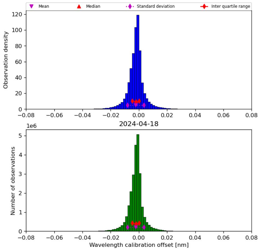
Figure 35: Histogram of “Wavelength calibration offset” for 2024-04-17 to 2024-04-19
