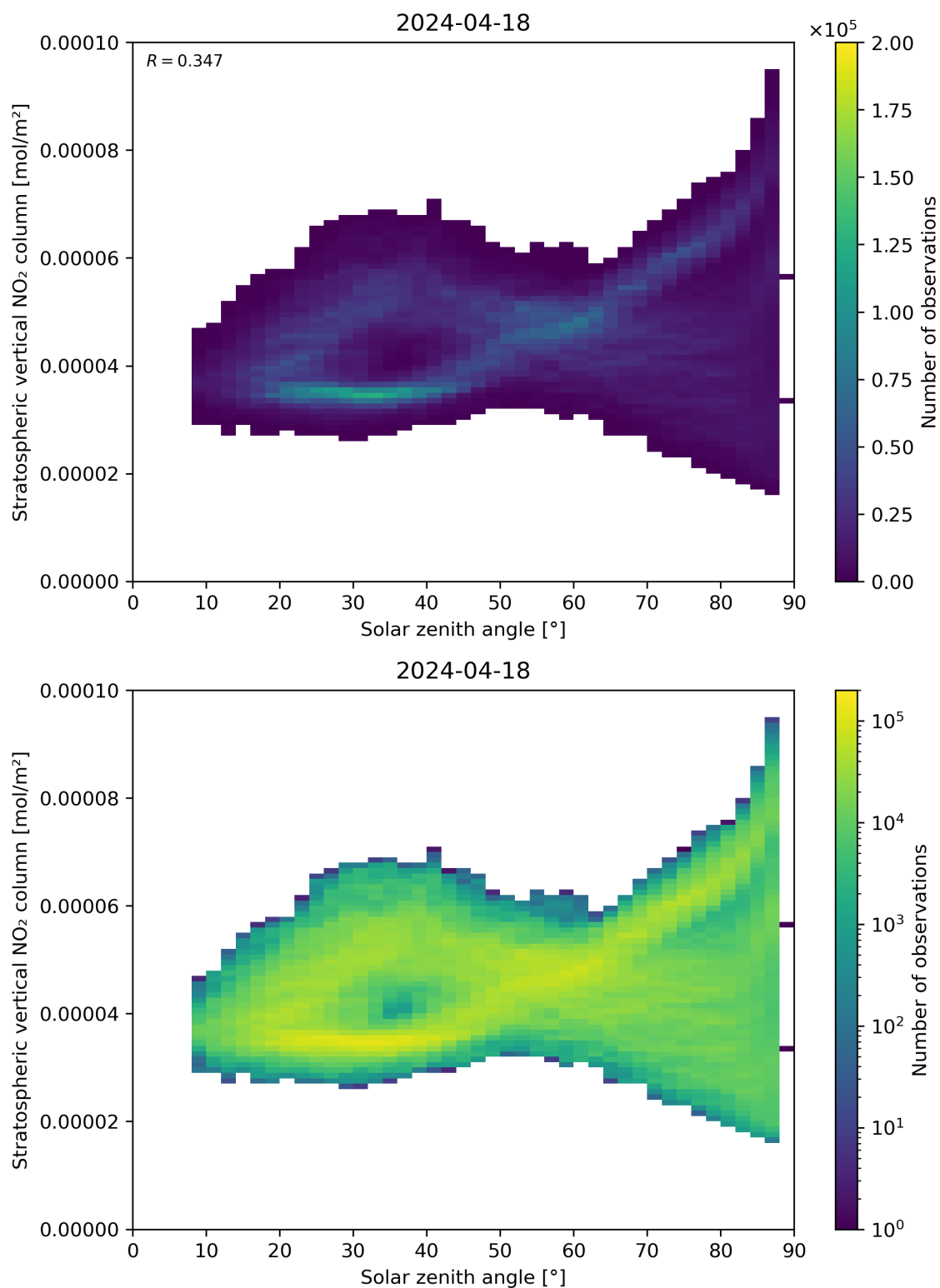
Figure 150: Scatter density plot of “Solar zenith angle” against “Stratospheric vertical NO 2 column” for 2024-04-17 to 2024-04-19.
