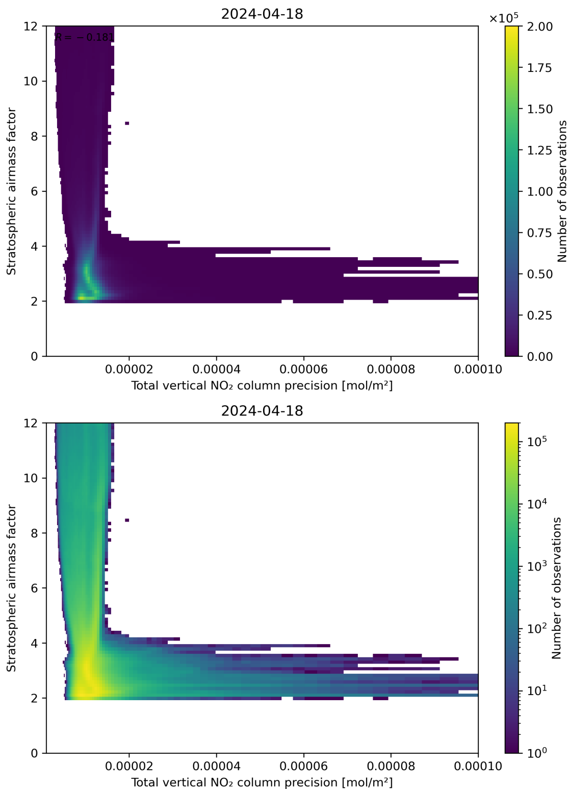
Figure 115: Scatter density plot of “Total vertical NO 2 column precision” against “Stratospheric air mass factor” for 2024-04-17 to 2024-04-19.
