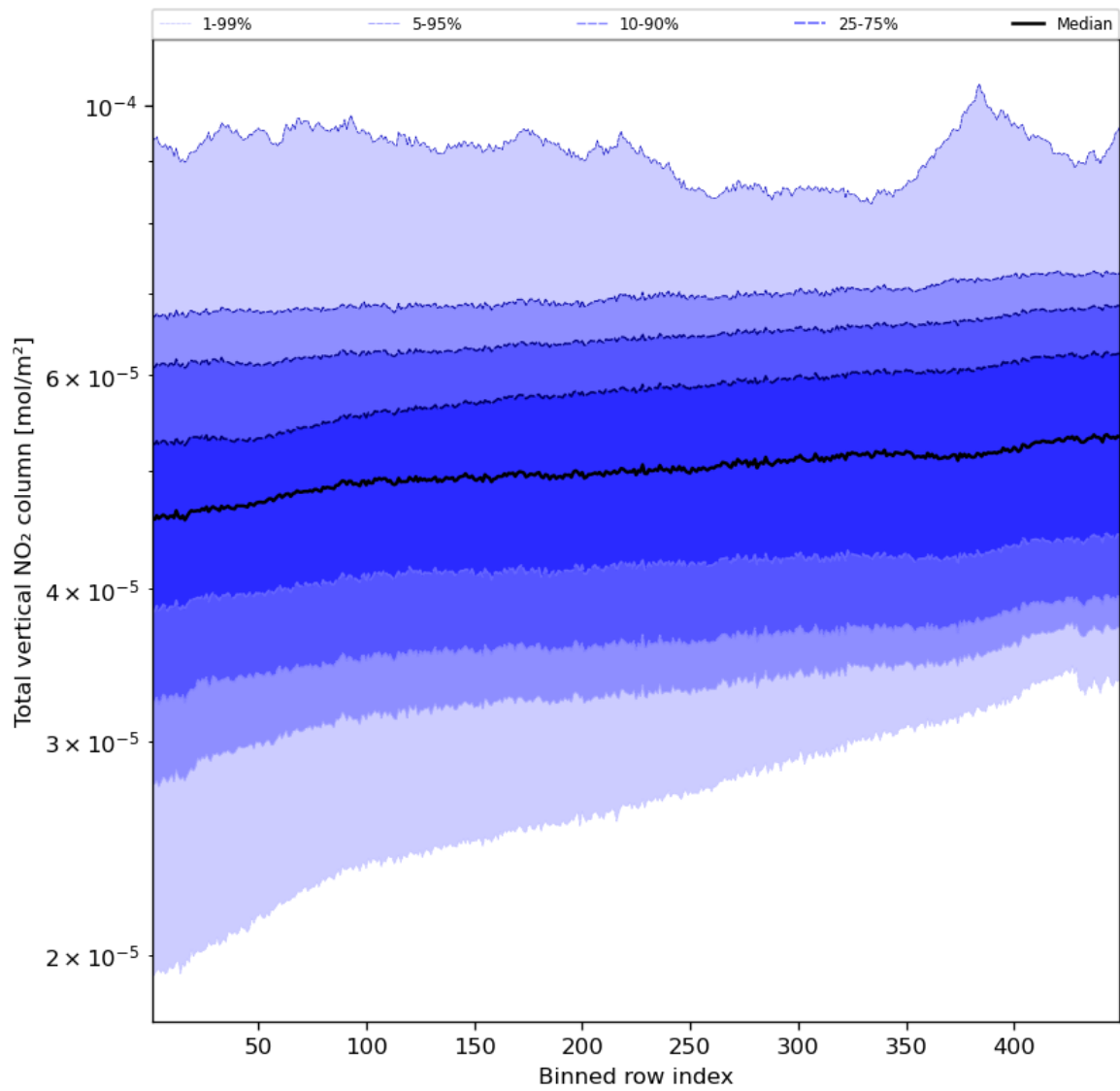
Figure 55: Along track statistics of “Total vertical NO 2 column” for 2024-04-17 to 2024-04-19
