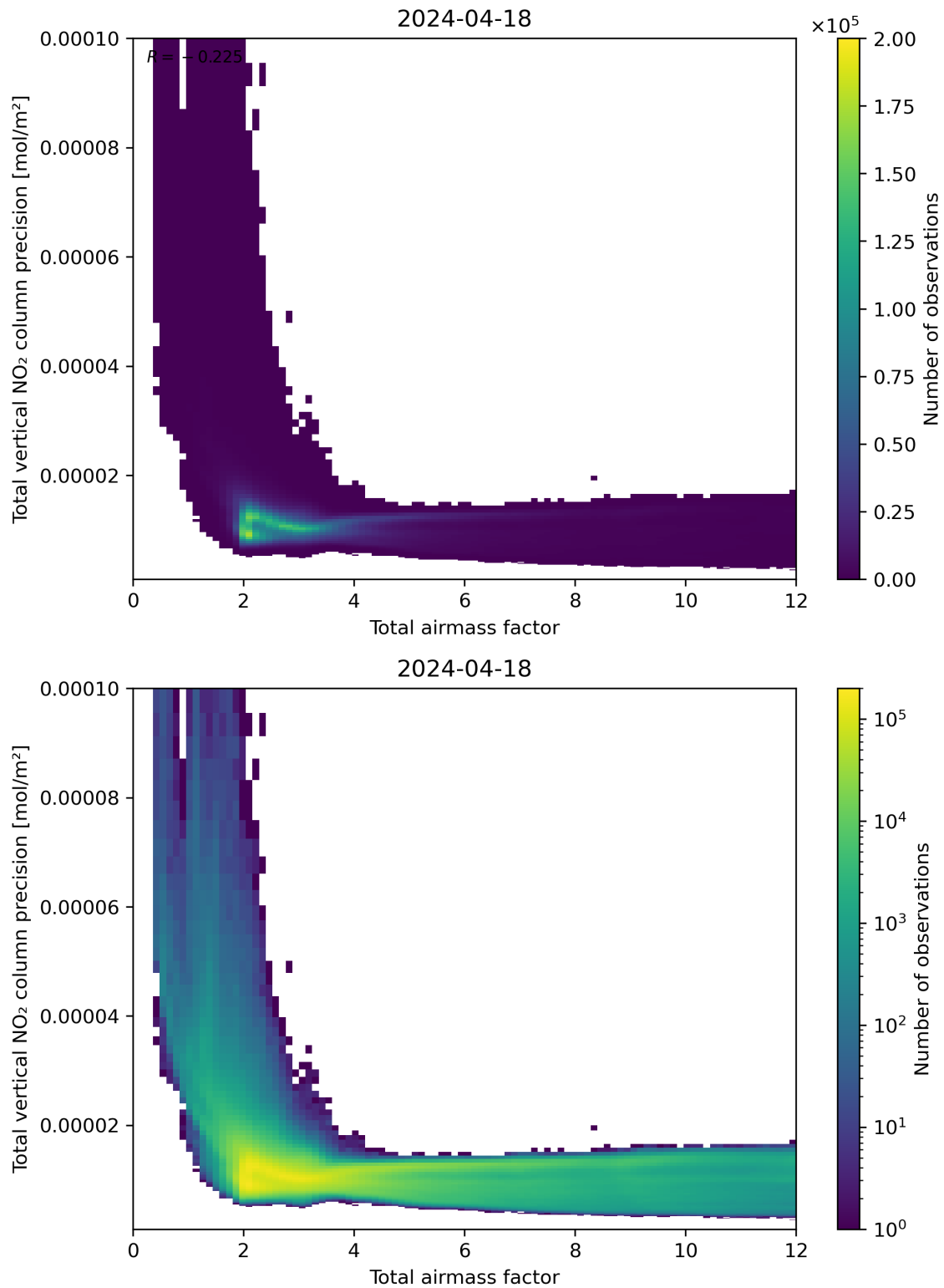
Figure 68: Scatter density plot of “Total airmass factor” against “Total vertical NO 2 column precision” for 2024-04-17 to 2024-04-19.
