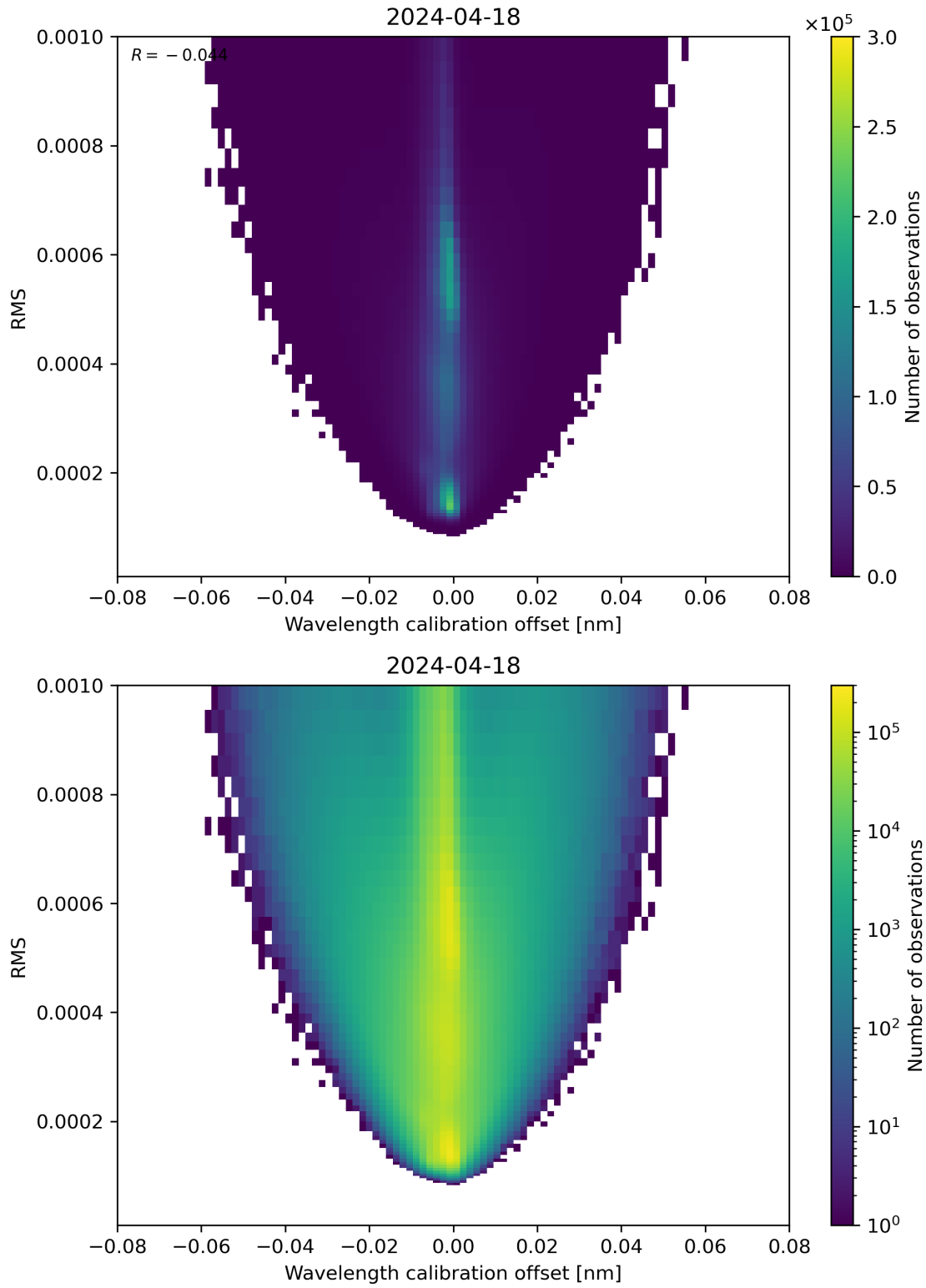
Figure 181: Scatter density plot of “Wavelength calibration offset” against “RMS” for 2024-04-17 to 2024-04-19.
