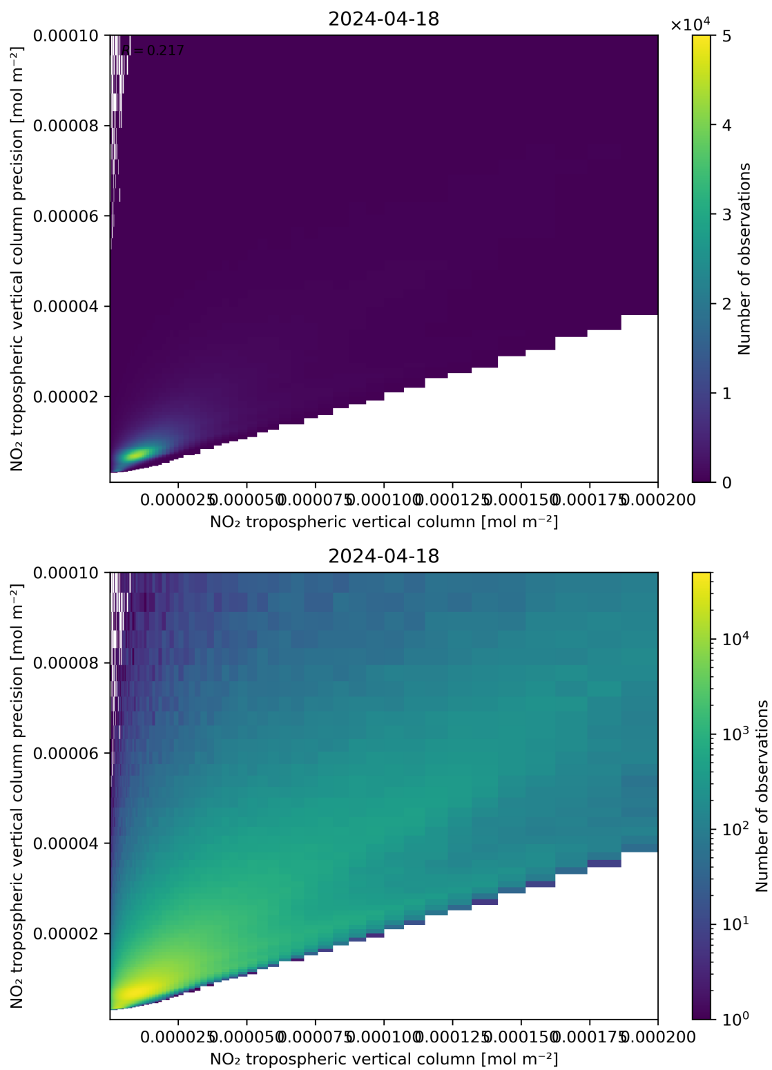
Figure 130: Scatter density plot of “NO 2 tropospheric vertical column” against “NO 2 tropospheric vertical column precision” for 2024-04-17 to 2024-04-19.
