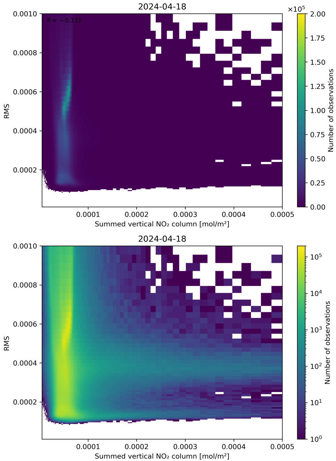
Figure 109: Scatter density plot of “Summed vertical NO 2 column” against “RMS” for 2024-04-17 to 2024-04-19.
