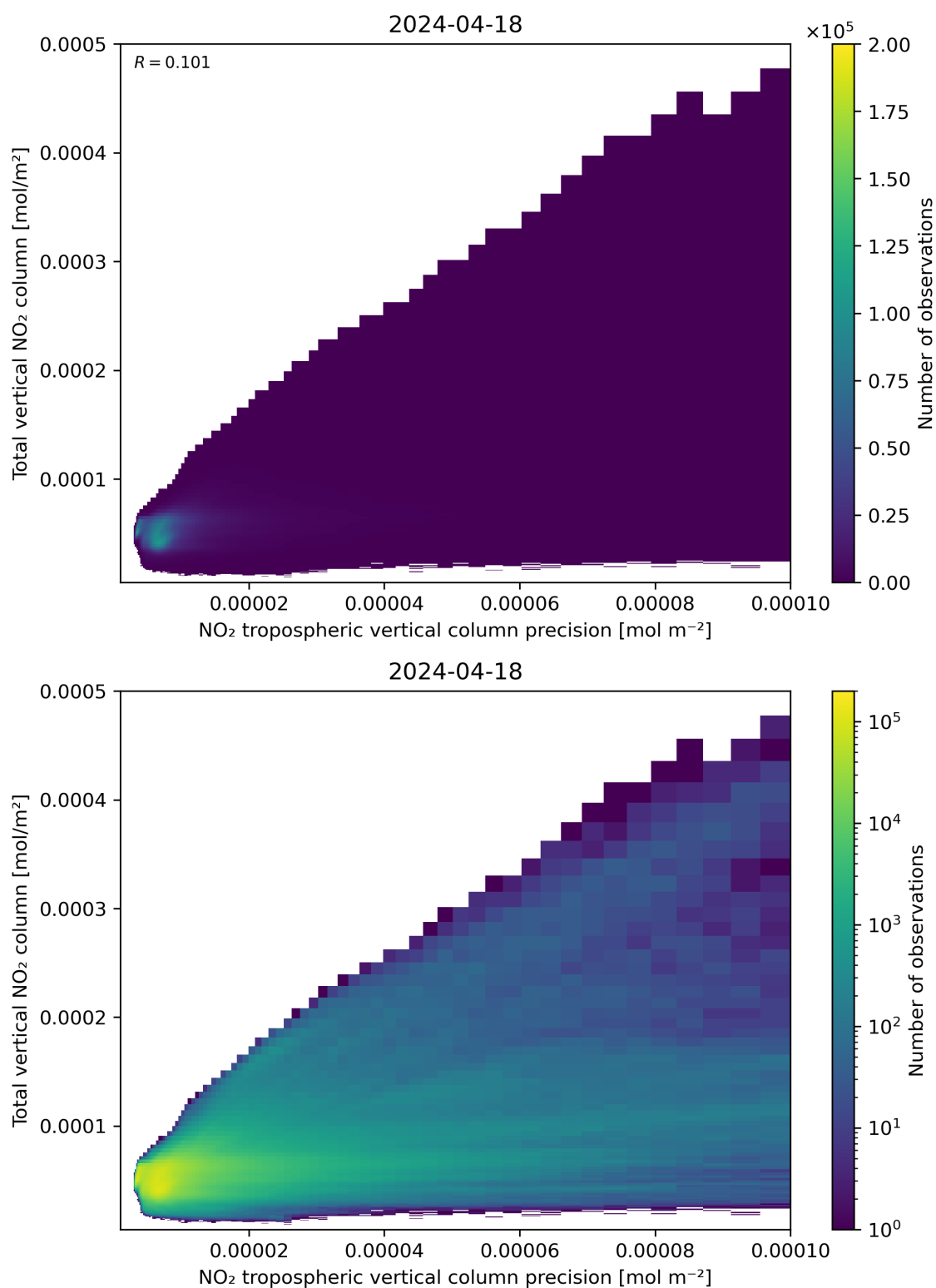
Figure 138: Scatter density plot of “NO 2 tropospheric vertical column precision” against “Total vertical NO 2 column” for 2024-04-17 to 2024-04-19.
