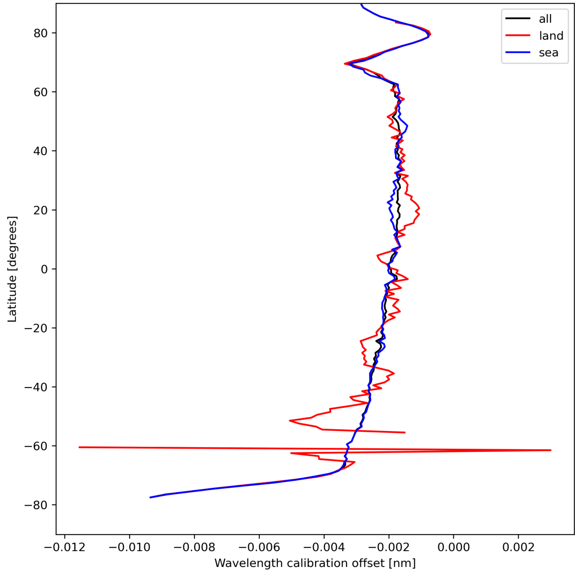
Figure 18: Zonal average of “Wavelength calibration offset” for 2024-04-17 to 2024-04-19.
