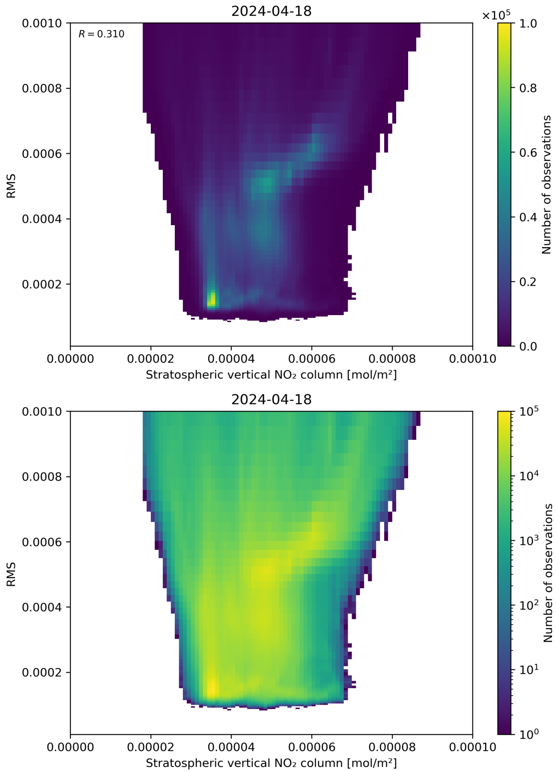
Figure 102: Scatter density plot of “Stratospheric vertical NO 2 column” against “RMS” for 2024-04-17 to 2024-04-19.
