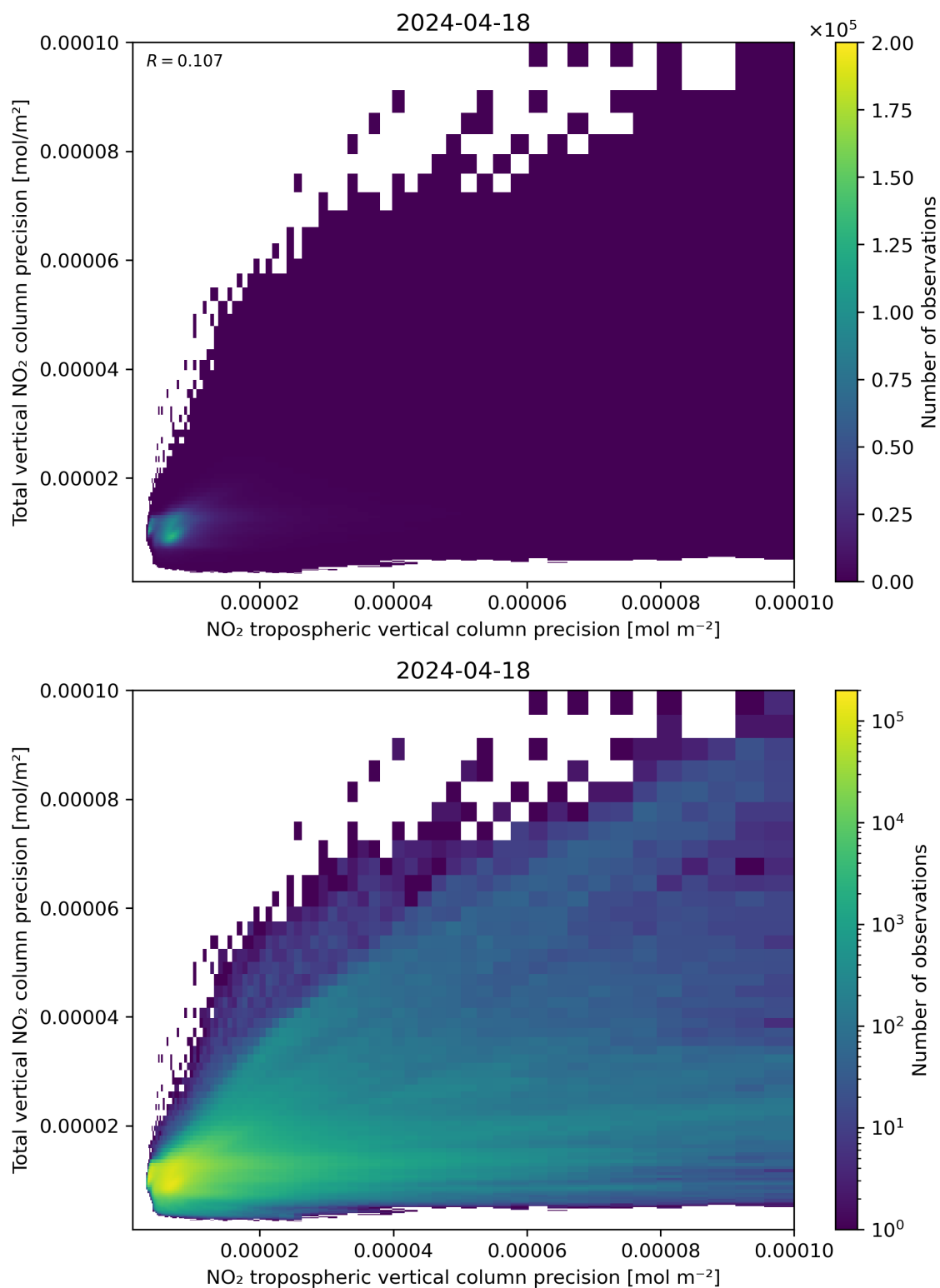
Figure 139: Scatter density plot of “NO 2 tropospheric vertical column precision” against “Total vertical NO 2 column precision” for 2024-04-17 to 2024-04-19.
