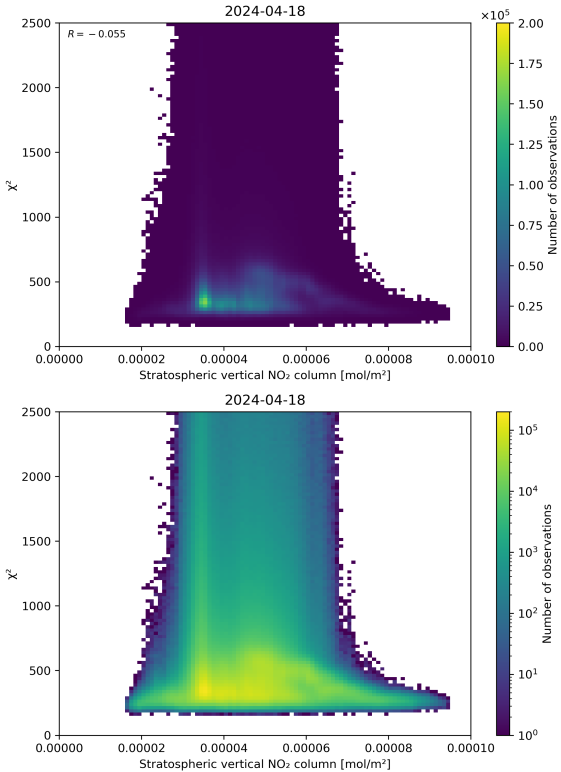
Figure 97: Scatter density plot of “Stratospheric vertical NO 2 column” against “ \chi^2 ” for 2024-04-17 to 2024-04-19.
