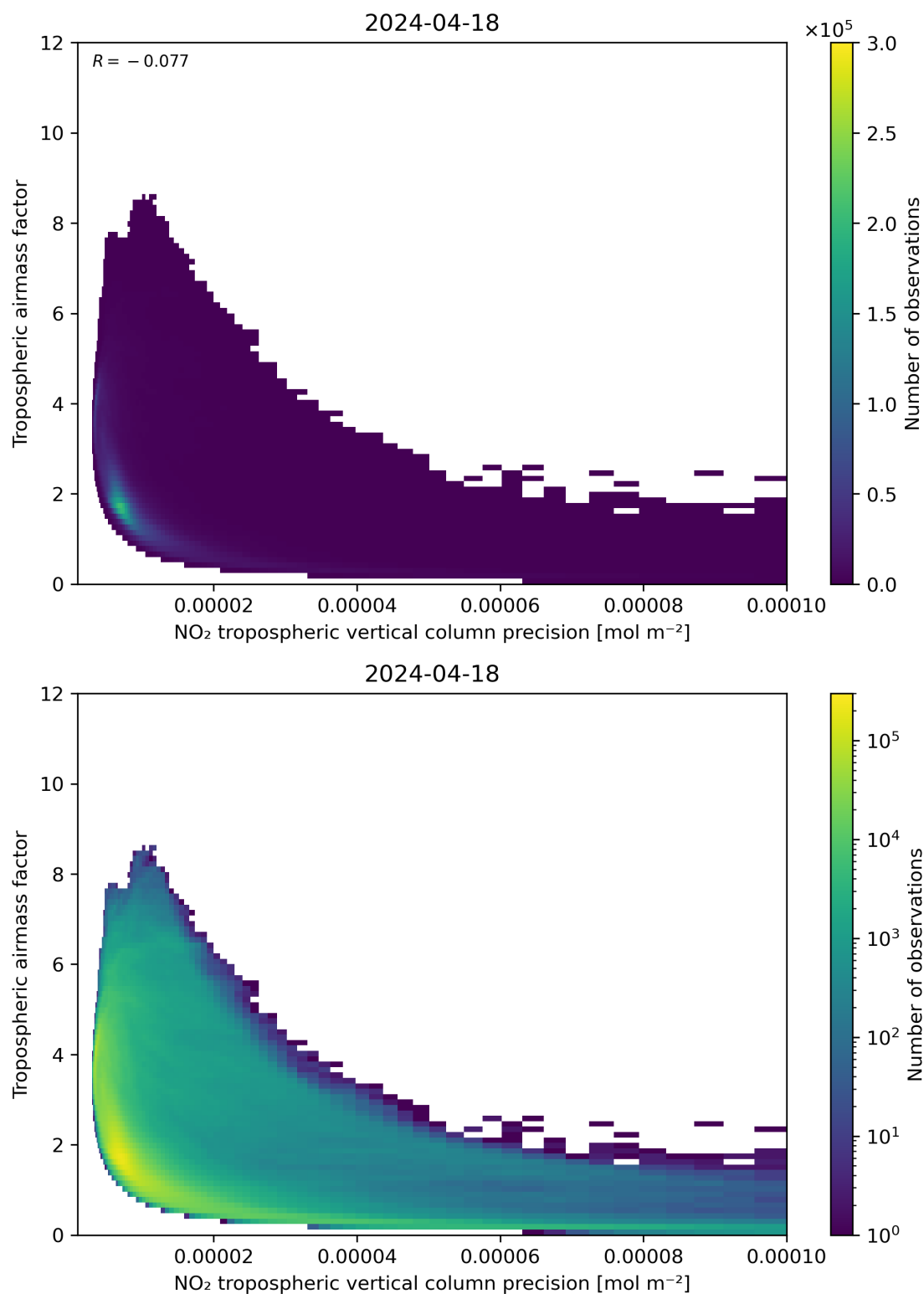
Figure 133: Scatter density plot of “NO 2 tropospheric vertical column precision” against “Tropospheric airmass factor” for 2024-04-17 to 2024-04-19.
