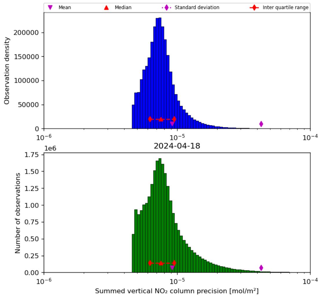
Figure 41: Histogram of "Summed vertical NO 2 column precision" for 2024-04-17 to 2024-04-19
