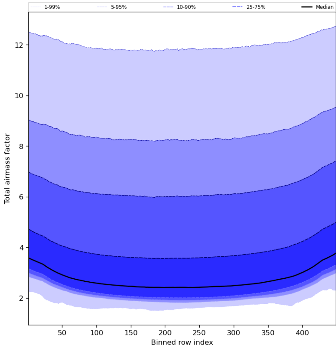
Figure 49: Along track statistics of “Total airmass factor” for 2024-04-17 to 2024-04-19
