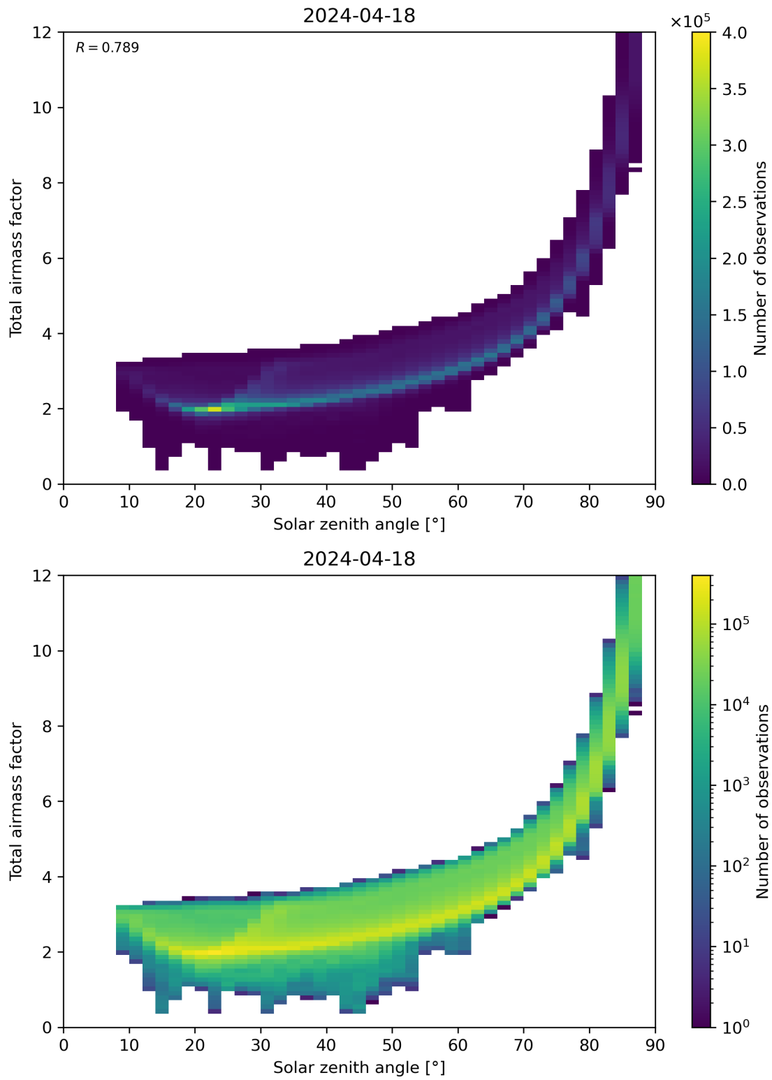
Figure 146: Scatter density plot of “Solar zenith angle” against “Total air mass factor” for 2024-04-17 to 2024-04-19.
