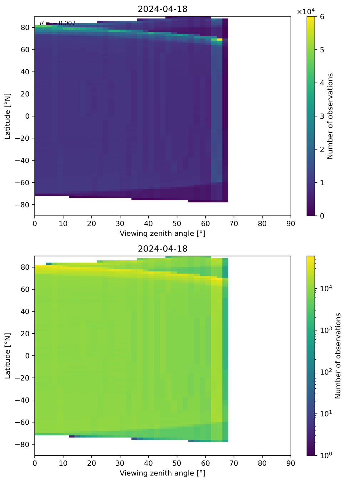
Figure 163: Scatter density plot of “Viewing zenith angle” against “Latitude” for 2024-04-17 to 2024-04-19.
