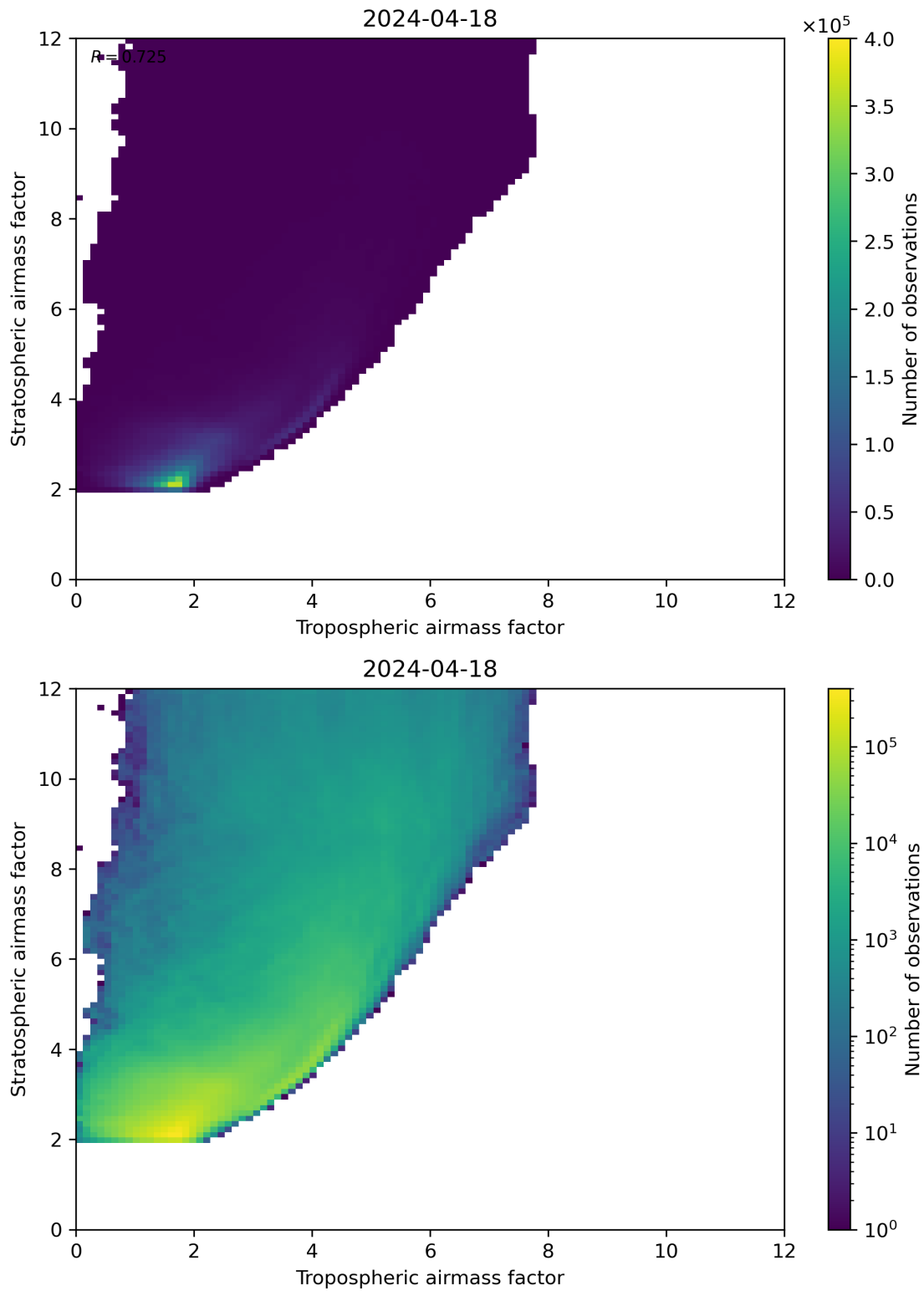
Figure 71: Scatter density plot of “Tropospheric airmass factor” against “Stratospheric airmass factor” for 2024-04-17 to 2024-04-19.
