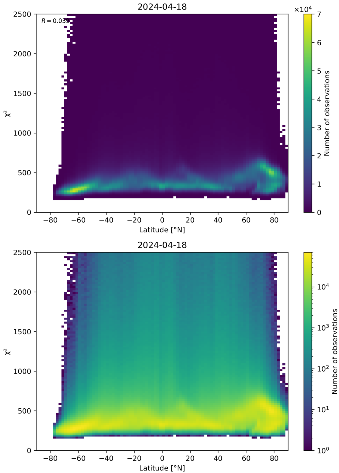
Figure 86: Scatter density plot of “Latitude” against “ \chi^2 ” for 2024-04-17 to 2024-04-19.
