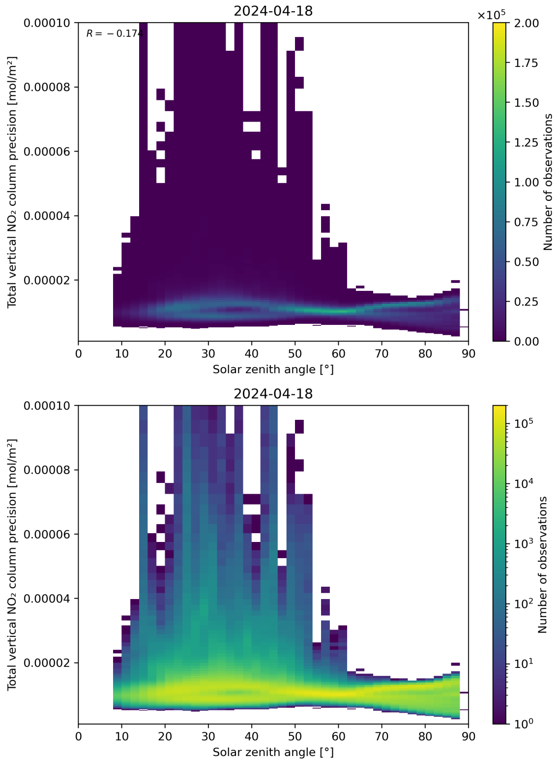
Figure 154: Scatter density plot of “Solar zenith angle” against “Total vertical NO 2 column precision” for 2024-04-17 to 2024-04-19.
