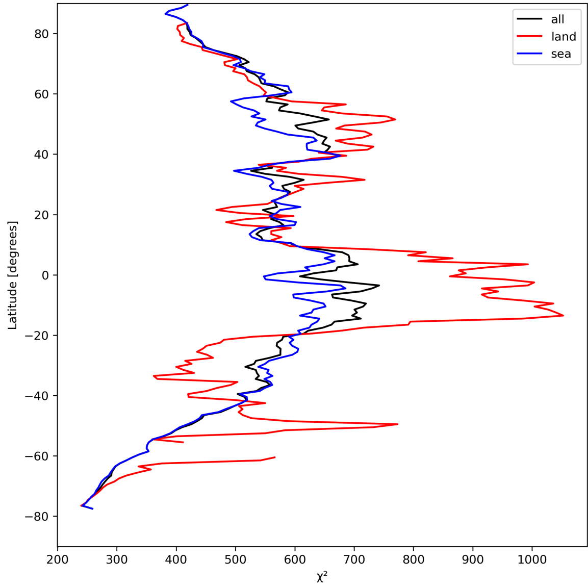
Figure 25: Zonal average of “ \chi^2 ” for 2024-04-17 to 2024-04-19.
