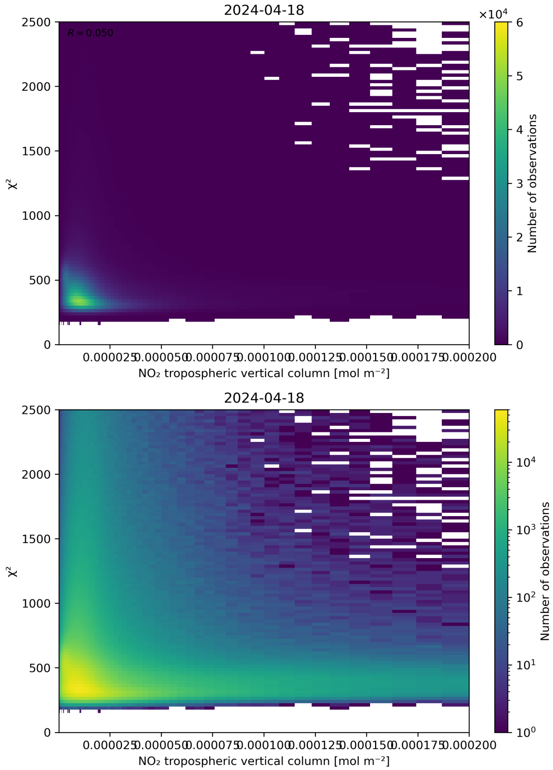
Figure 124: Scatter density plot of “NO 2 tropospheric vertical column” against “ \chi^2 ” for 2024-04-17 to 2024-04-19.
