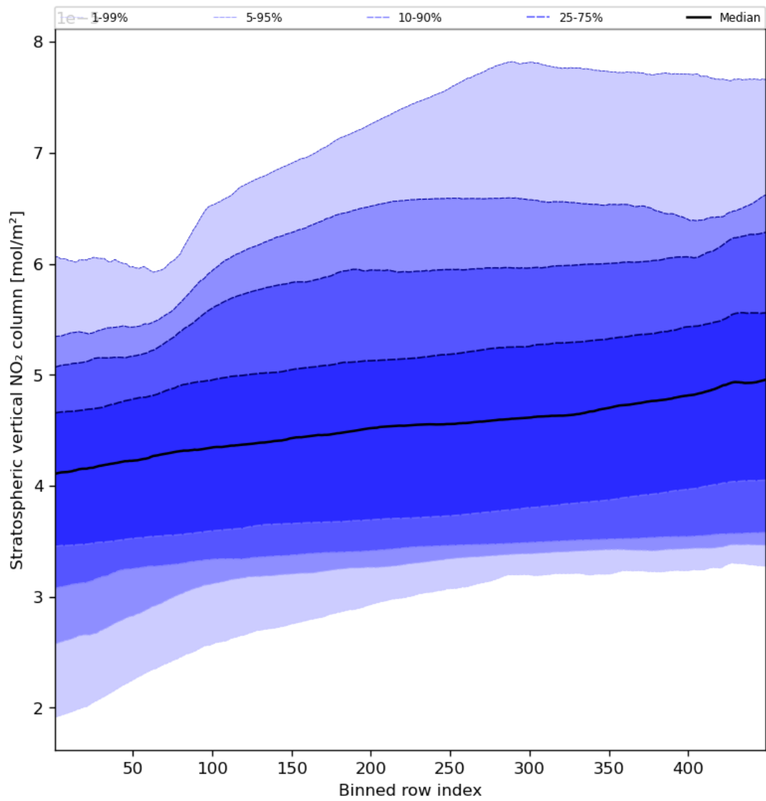
Figure 53: Along track statistics of “Stratospheric vertical NO 2 column” for 2024-04-17 to 2024-04-19
