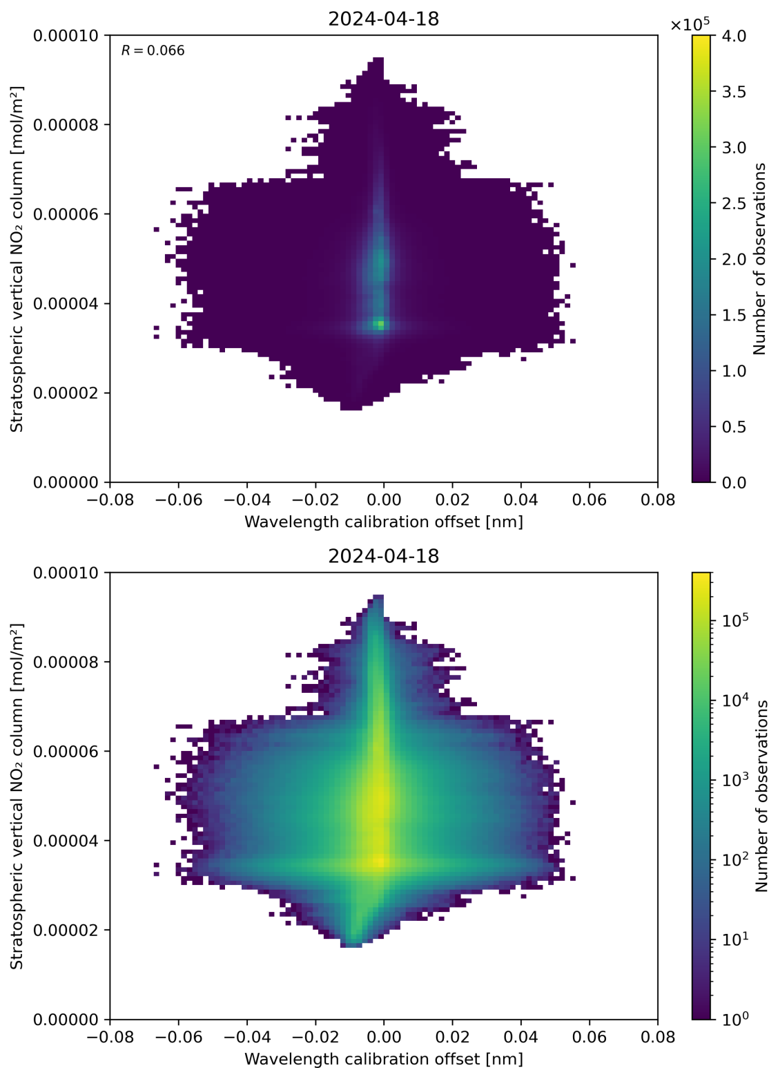
Figure 176: Scatter density plot of “Wavelength calibration offset” against “Stratospheric vertical NO 2 column” for 2024-04-17 to 2024-04-19.
