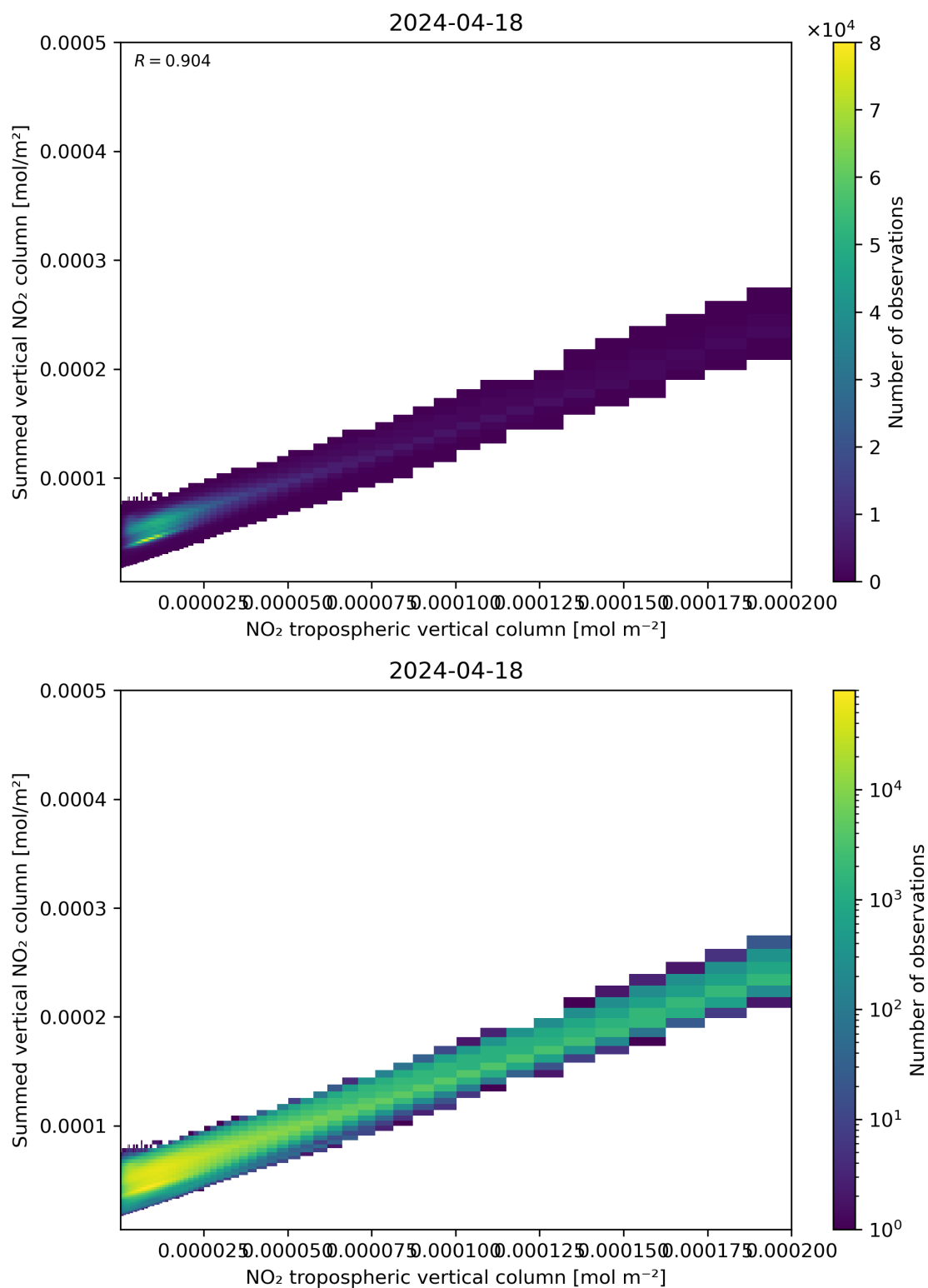
Figure 126: Scatter density plot of “NO 2 tropospheric vertical column” against “Summed vertical NO 2 column” for 2024-04-17 to 2024-04-19.
