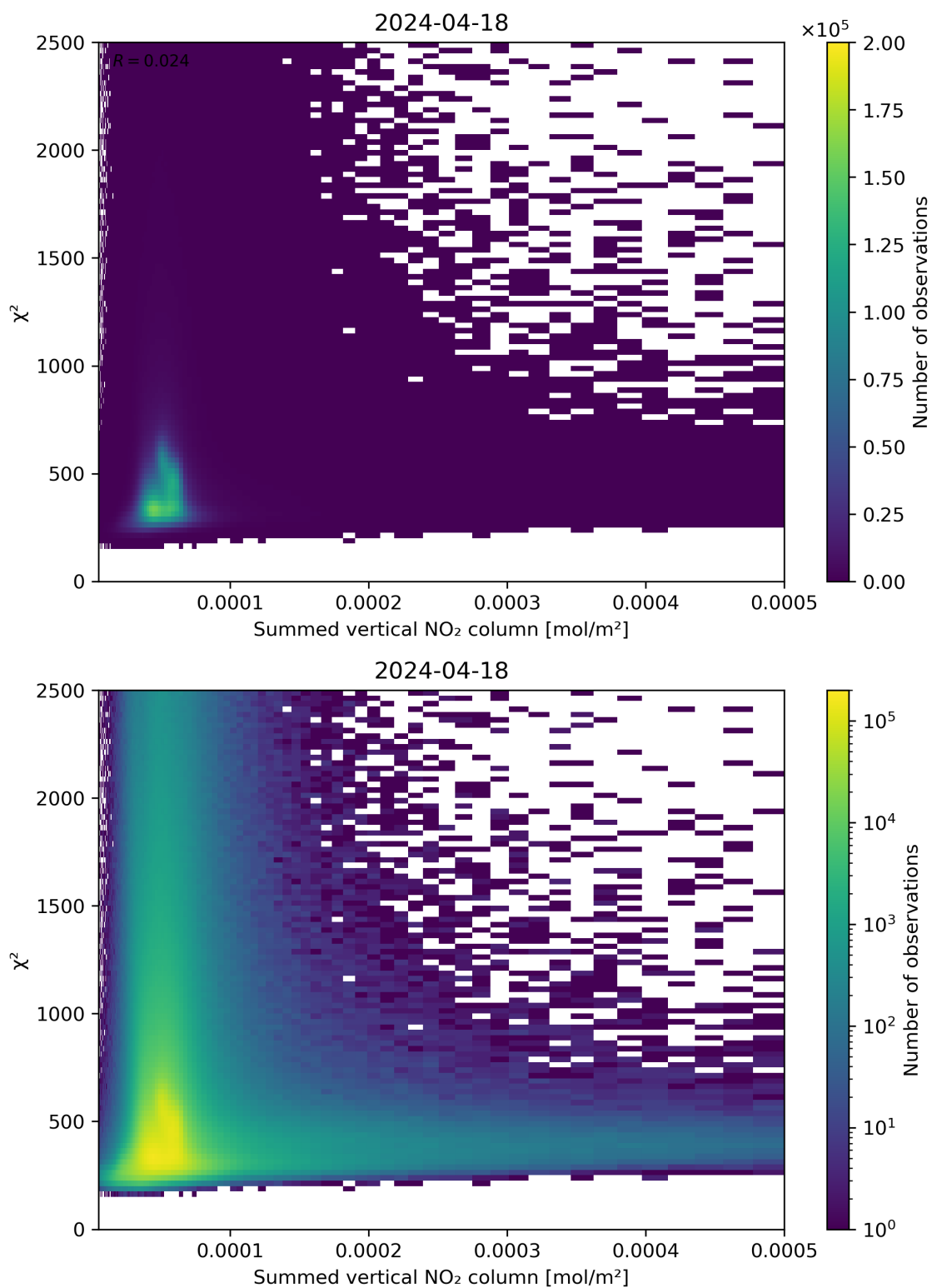
Figure 104: Scatter density plot of “Summed vertical NO 2 column” against “ \chi^2 ” for 2024-04-17 to 2024-04-19.
