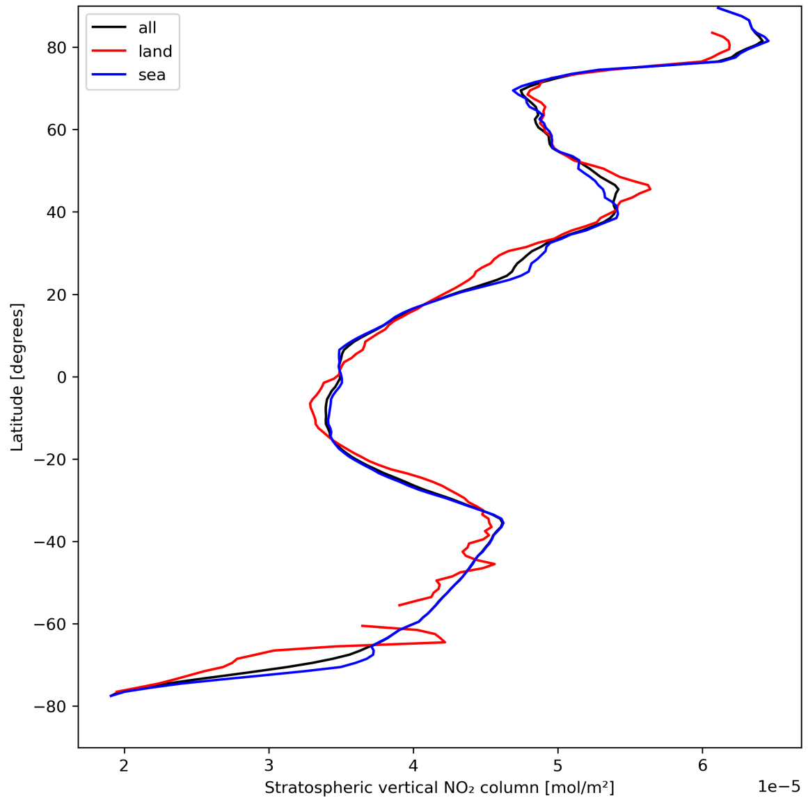
Figure 19: Zonal average of “Stratospheric vertical NO 2 column” for 2024-04-17 to 2024-04-19.
