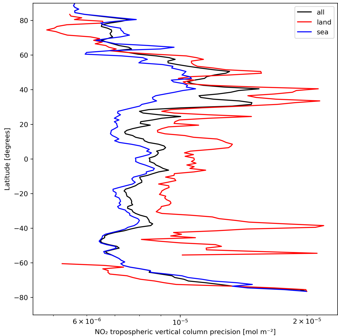
Figure 13: Zonal average of “NO 2 tropospheric vertical column precision” for 2024-04-18 to 2024-04-20.
