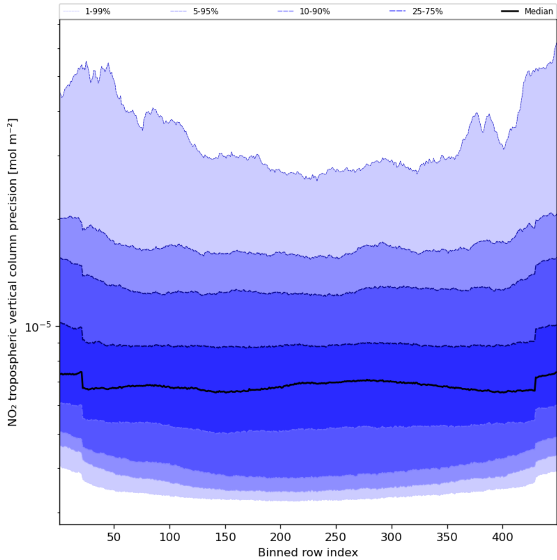
Figure 47: Along track statistics of “NO 2 tropospheric vertical column precision” for 2024-04-18 to 2024-04-20
