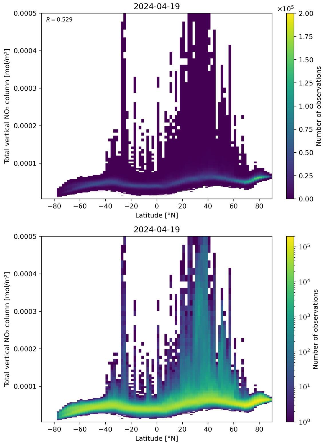
Figure 90: Scatter density plot of “Latitude” against “Total vertical NO 2 column” for 2024-04-18 to 2024-04-20.
