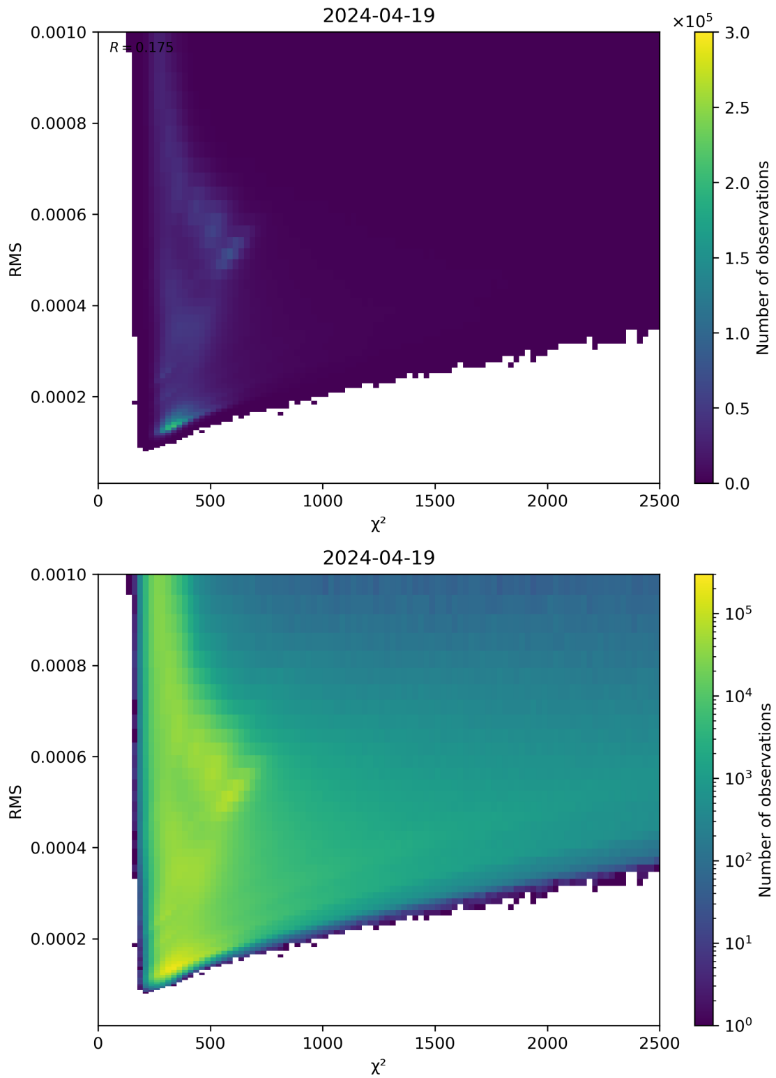
Figure 82: Scatter density plot of “ \chi^2 ” against “RMS” for 2024-04-18 to 2024-04-20.
