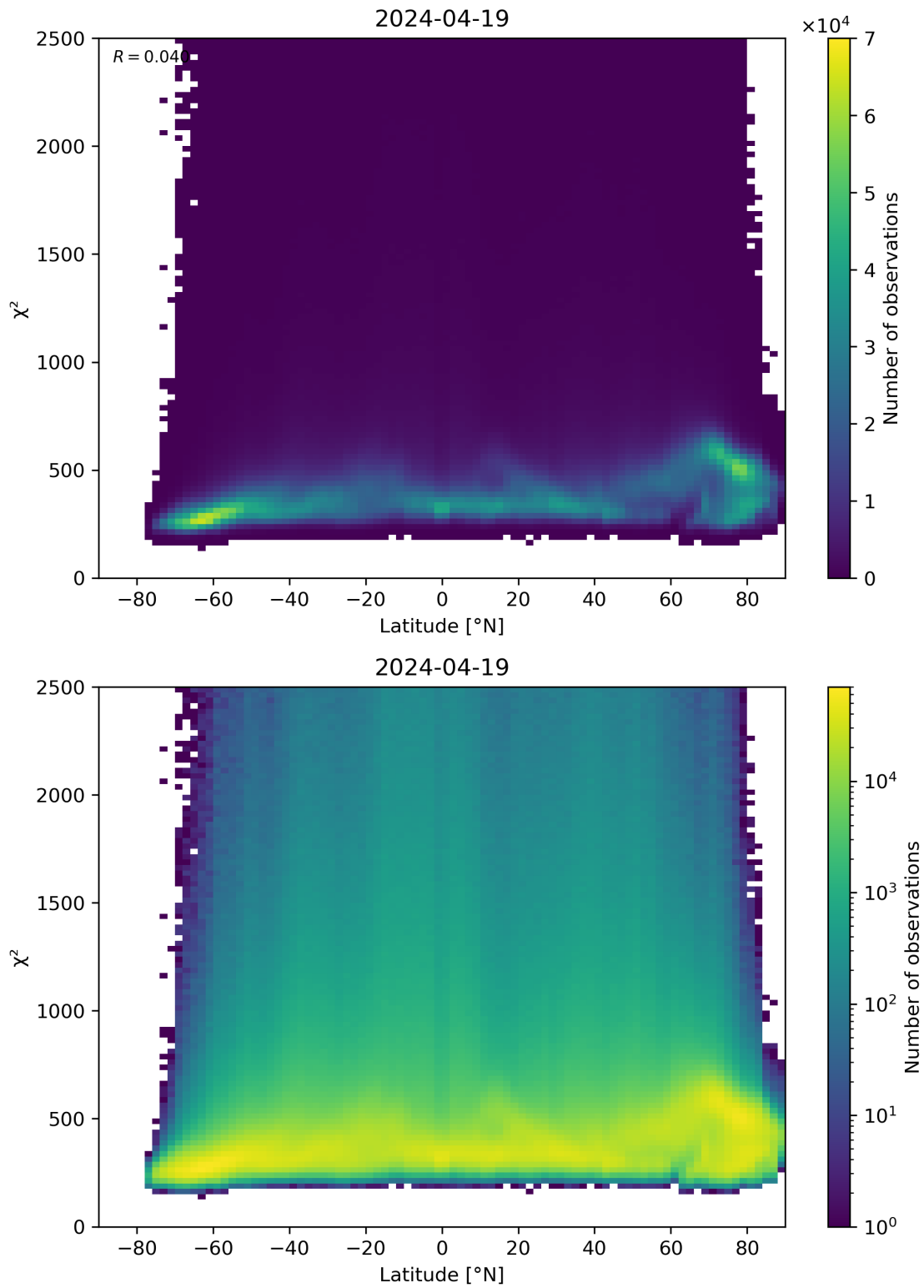
Figure 86: Scatter density plot of “Latitude” against “ \chi^2 ” for 2024-04-18 to 2024-04-20.
