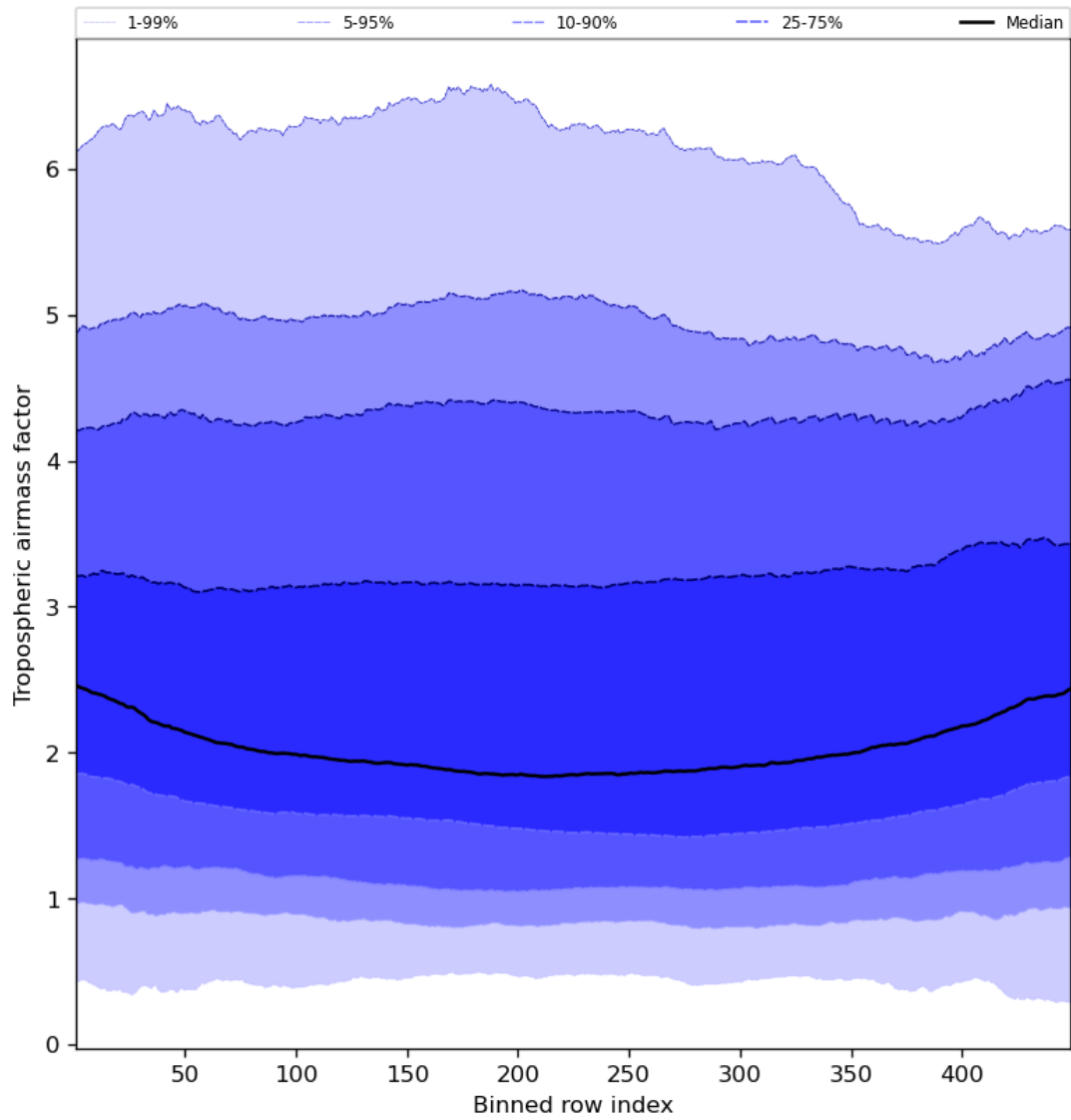
Figure 48: Along track statistics of “Tropospheric air mass factor” for 2024-04-18 to 2024-04-20
