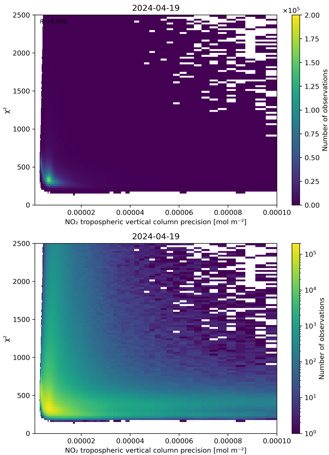
Figure 134: Scatter density plot of “NO 2 tropospheric vertical column precision” against “ \chi^2 ” for 2024-04-18 to 2024-04-20.
