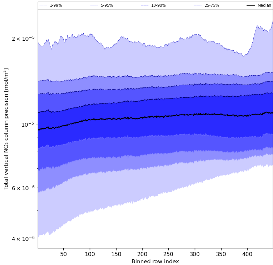
Figure 56: Along track statistics of “Total vertical NO 2 column precision” for 2024-04-18 to 2024-04-20
