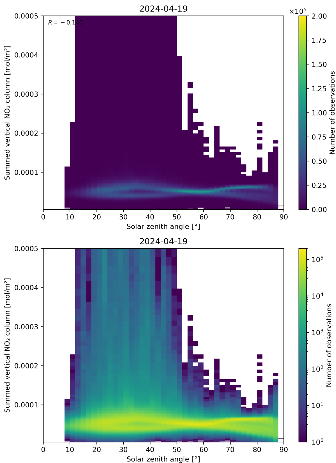
Figure 151: Scatter density plot of “Solar zenith angle” against “Summed vertical NO 2 column” for 2024-04-18 to 2024-04-20.
