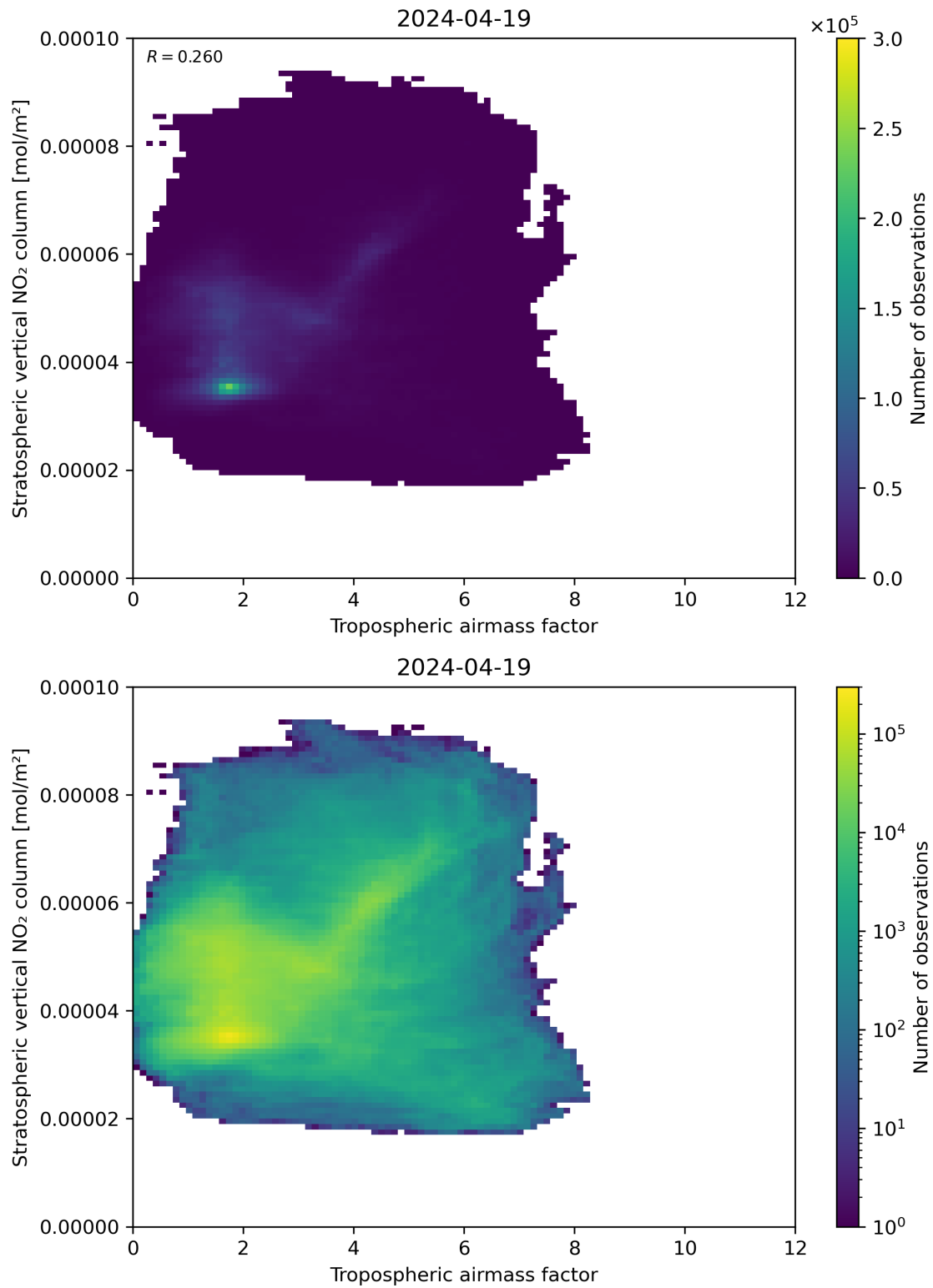
Figure 74: Scatter density plot of “Tropospheric air mass factor” against “Stratospheric vertical NO 2 column” for 2024-04-18 to 2024-04-20.
