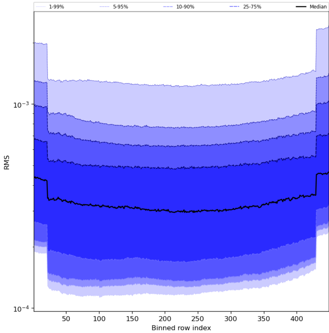
Figure 60: Along track statistics of “RMS” for 2024-04-18 to 2024-04-20
