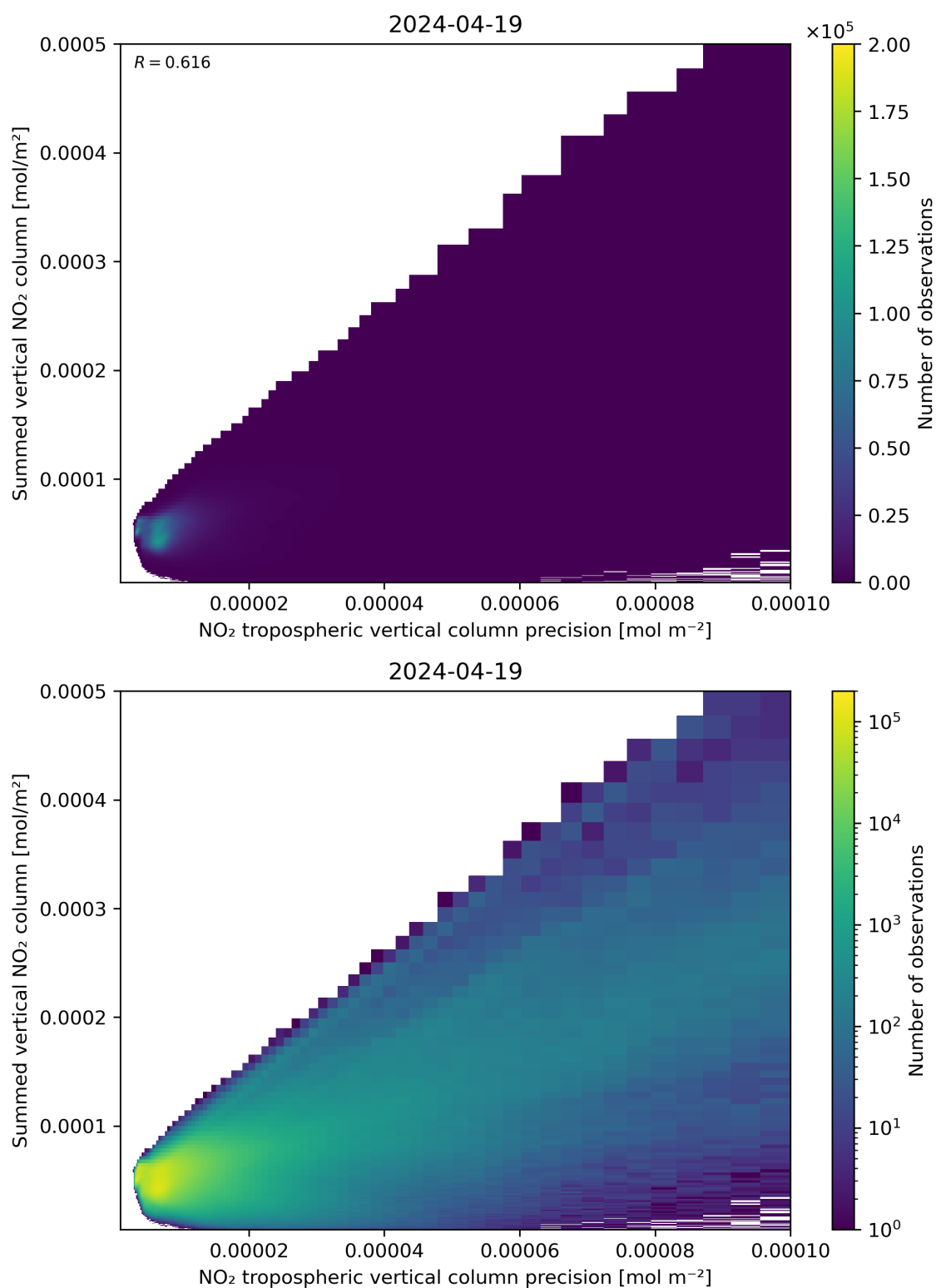
Figure 136: Scatter density plot of “NO 2 tropospheric vertical column precision” against “Summed vertical NO 2 column” for 2024-04-18 to 2024-04-20.
