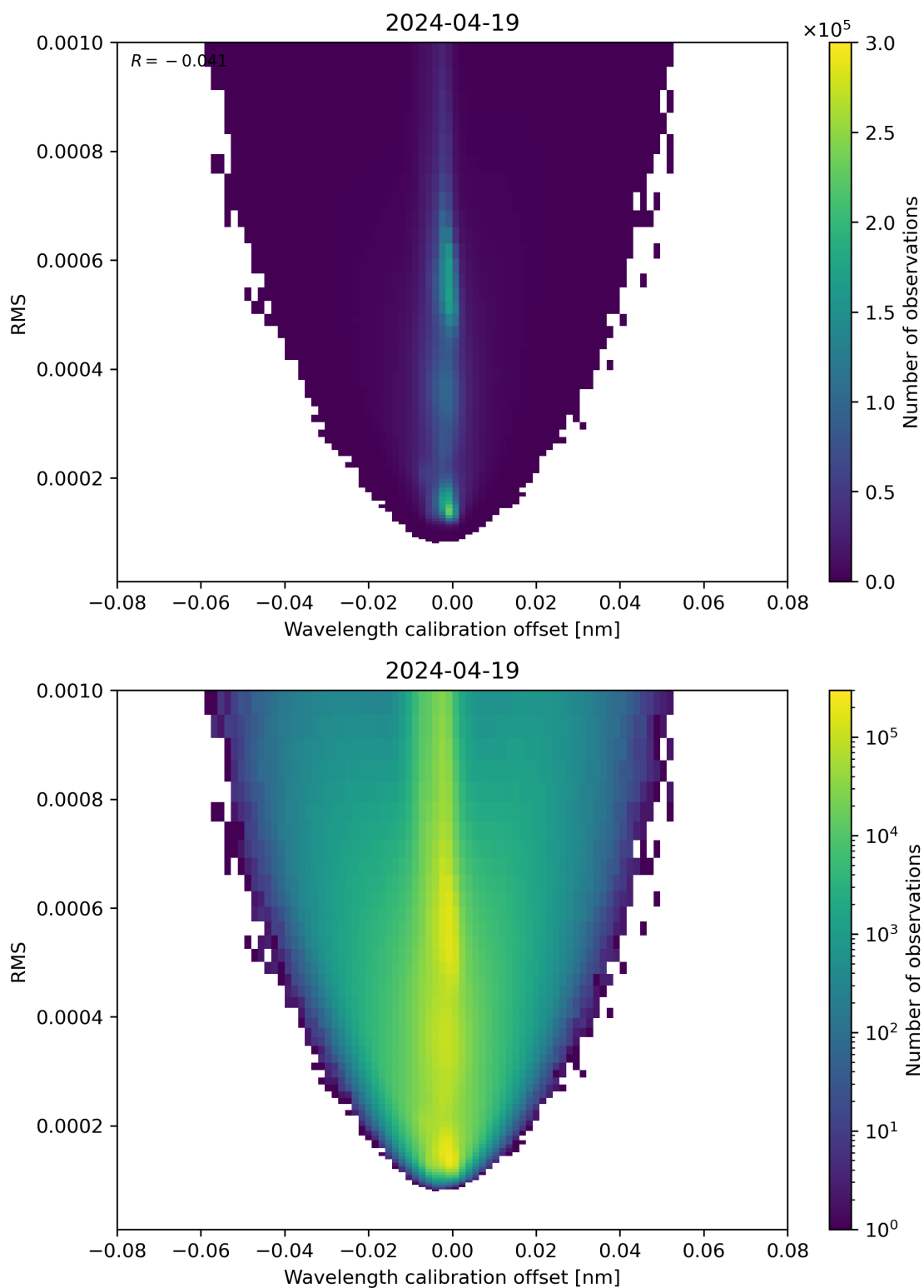
Figure 181: Scatter density plot of “Wavelength calibration offset” against “RMS” for 2024-04-18 to 2024-04-20.
