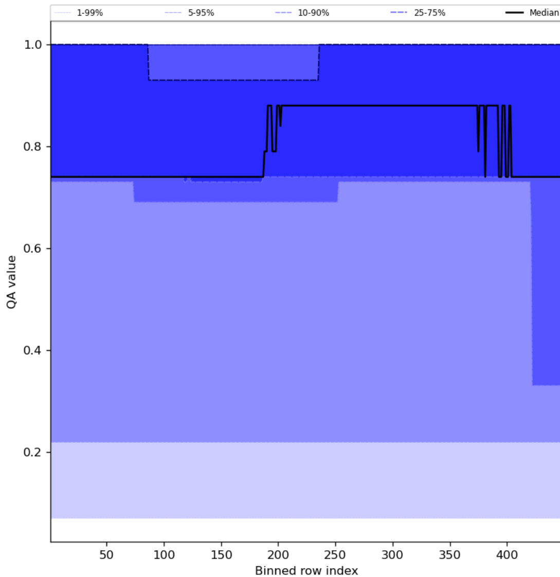
Figure 45: Along track statistics of “QA value” for 2024-04-18 to 2024-04-20
