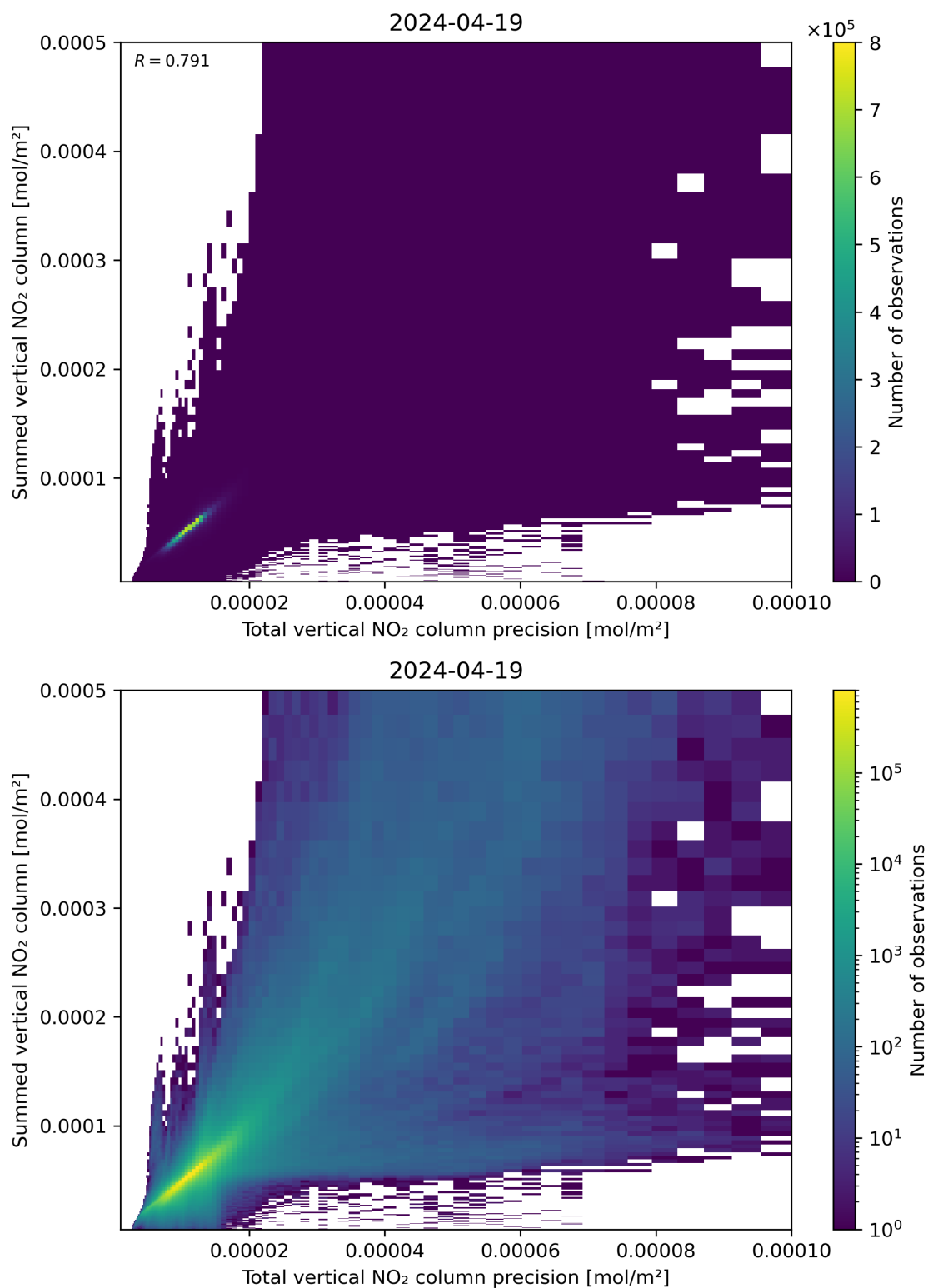
Figure 117: Scatter density plot of “Total vertical NO 2 column precision” against “Summed vertical NO 2 column” for 2024-04-18 to 2024-04-20.
