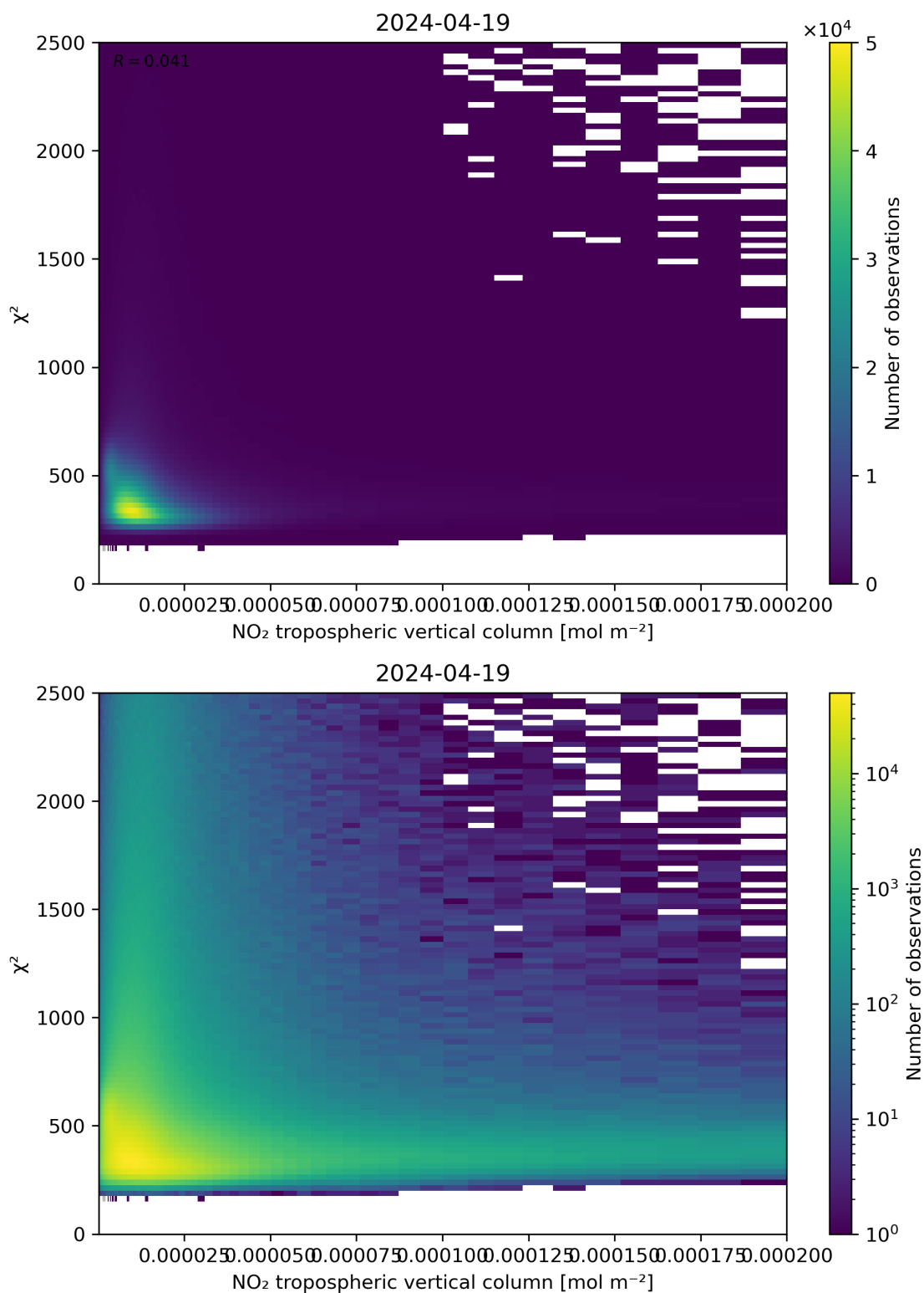
Figure 124: Scatter density plot of “NO 2 tropospheric vertical column” against “ \chi^2 ” for 2024-04-18 to 2024-04-20.
