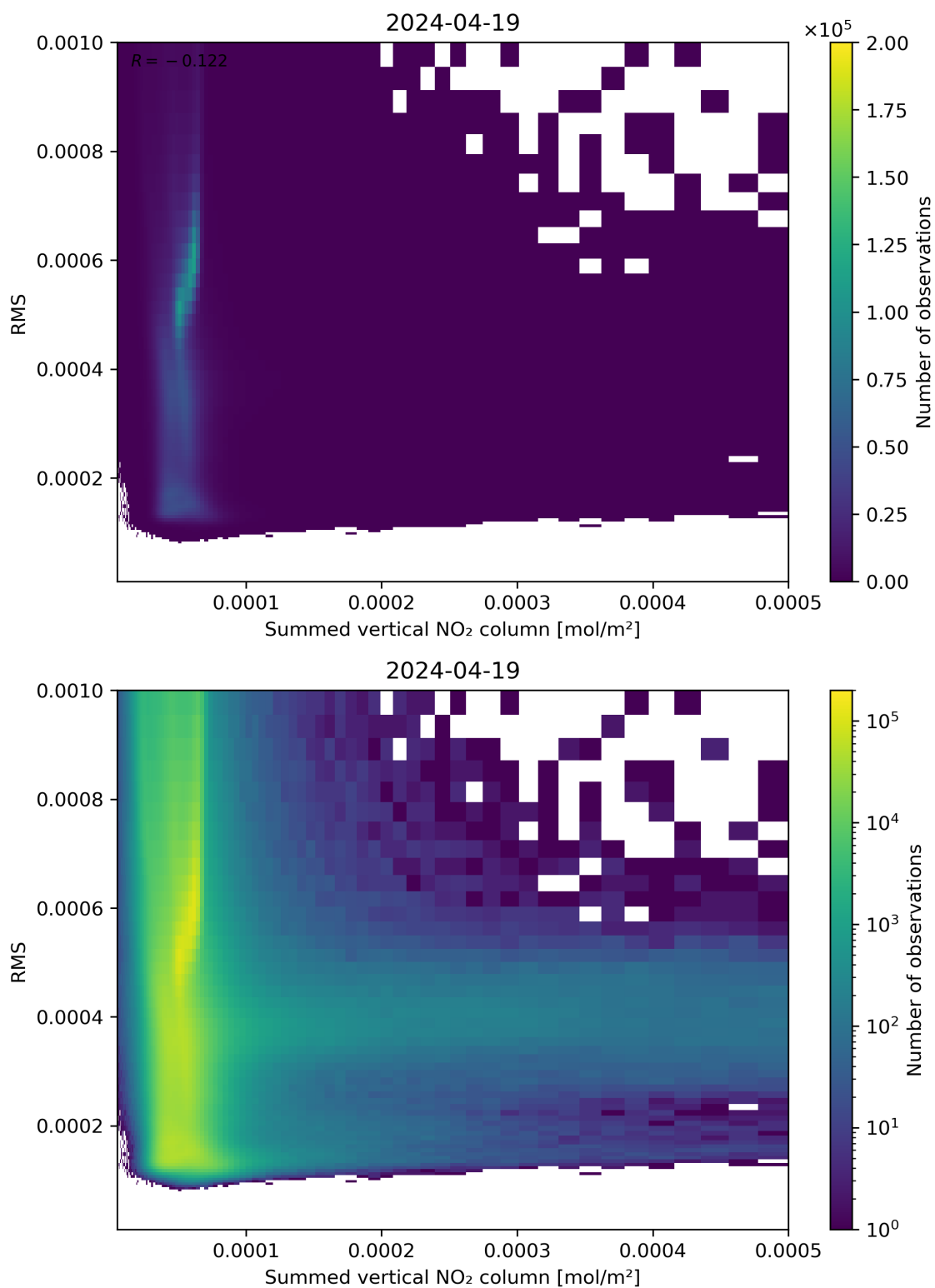
Figure 109: Scatter density plot of “Summed vertical NO 2 column” against “RMS” for 2024-04-18 to 2024-04-20.
