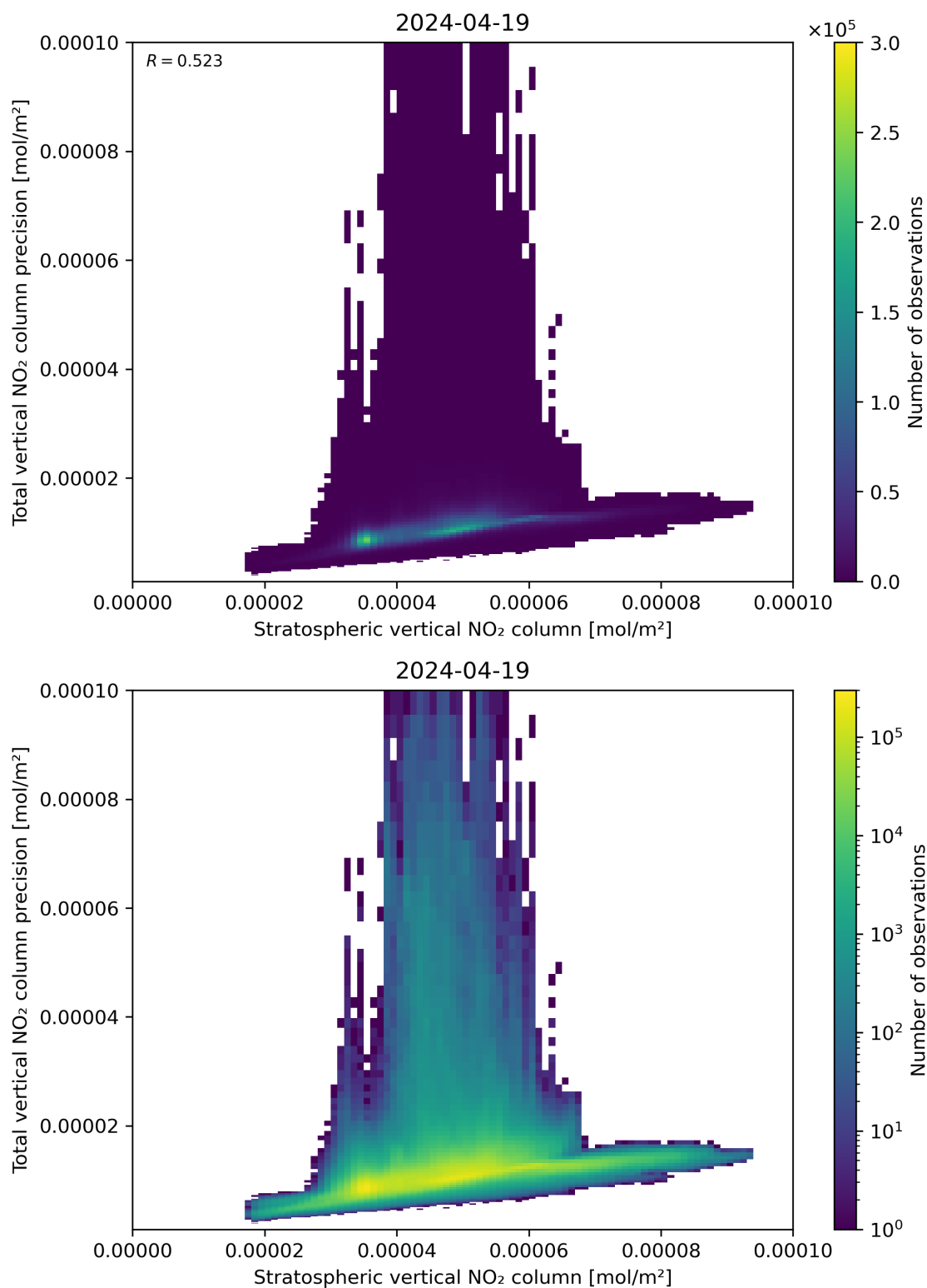
Figure 101: Scatter density plot of “Stratospheric vertical NO 2 column” against “Total vertical NO 2 column precision” for 2024-04-18 to 2024-04-20.
