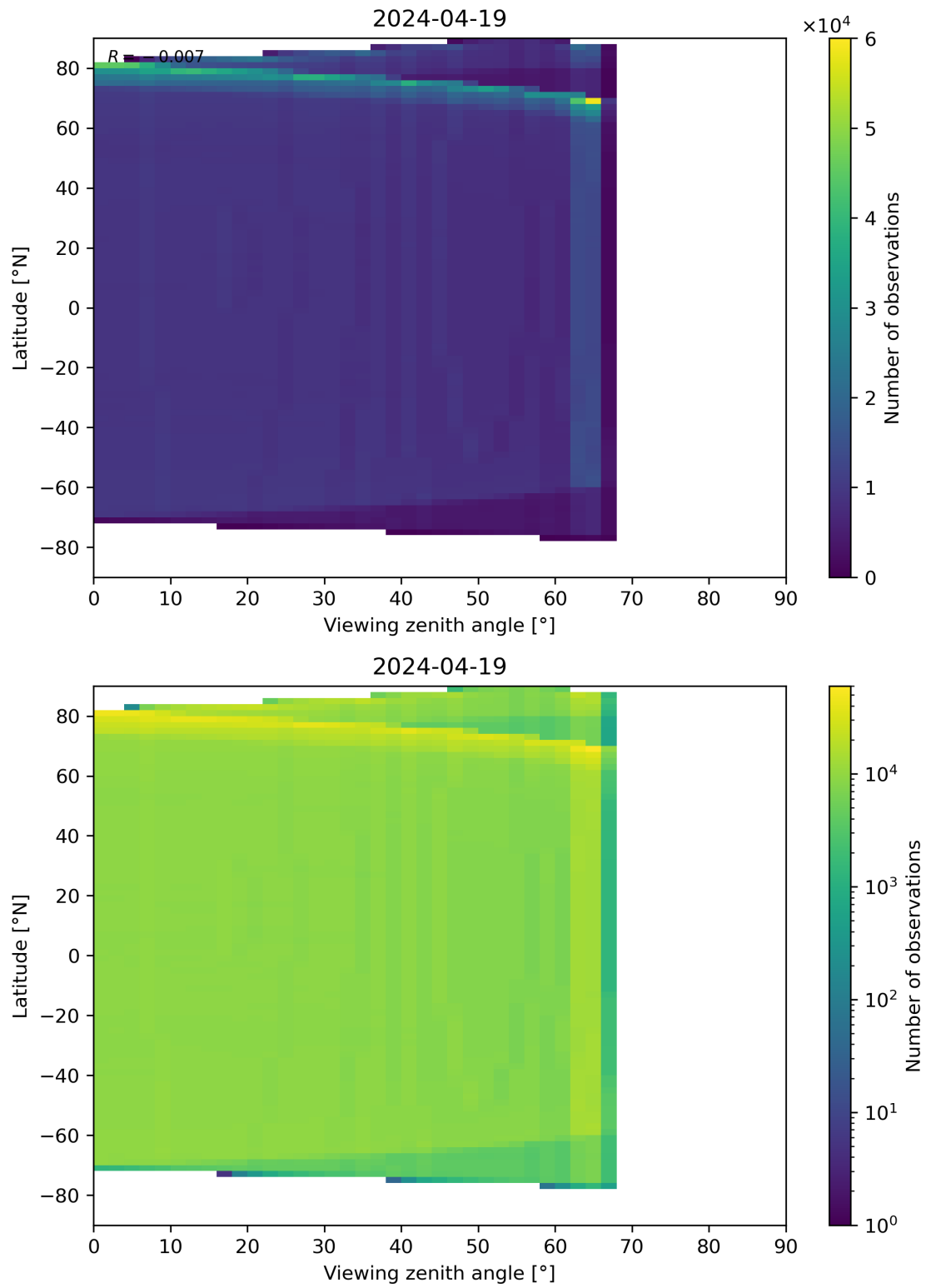
Figure 163: Scatter density plot of “Viewing zenith angle” against “Latitude” for 2024-04-18 to 2024-04-20.
