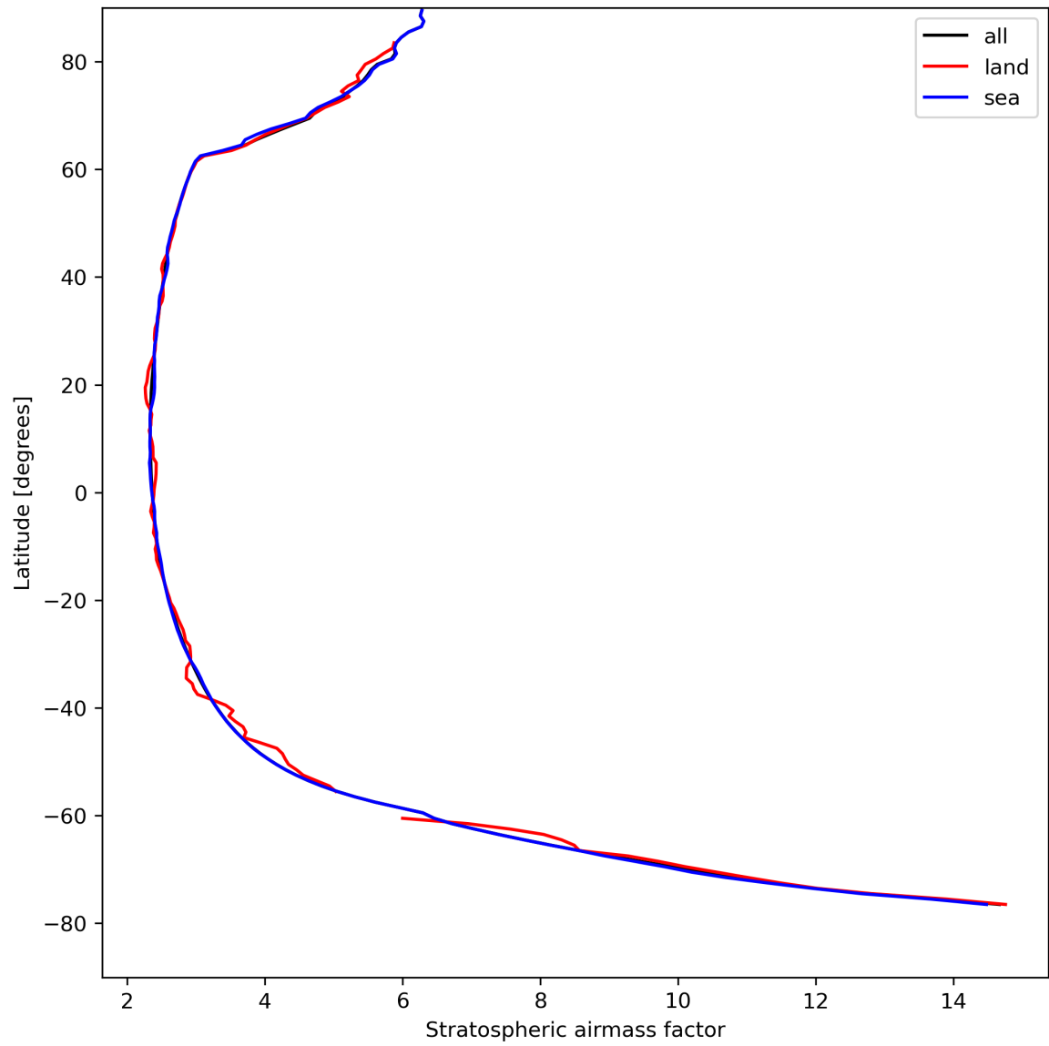
Figure 27: Zonal average of “Stratospheric airmass factor” for 2024-04-18 to 2024-04-20.
