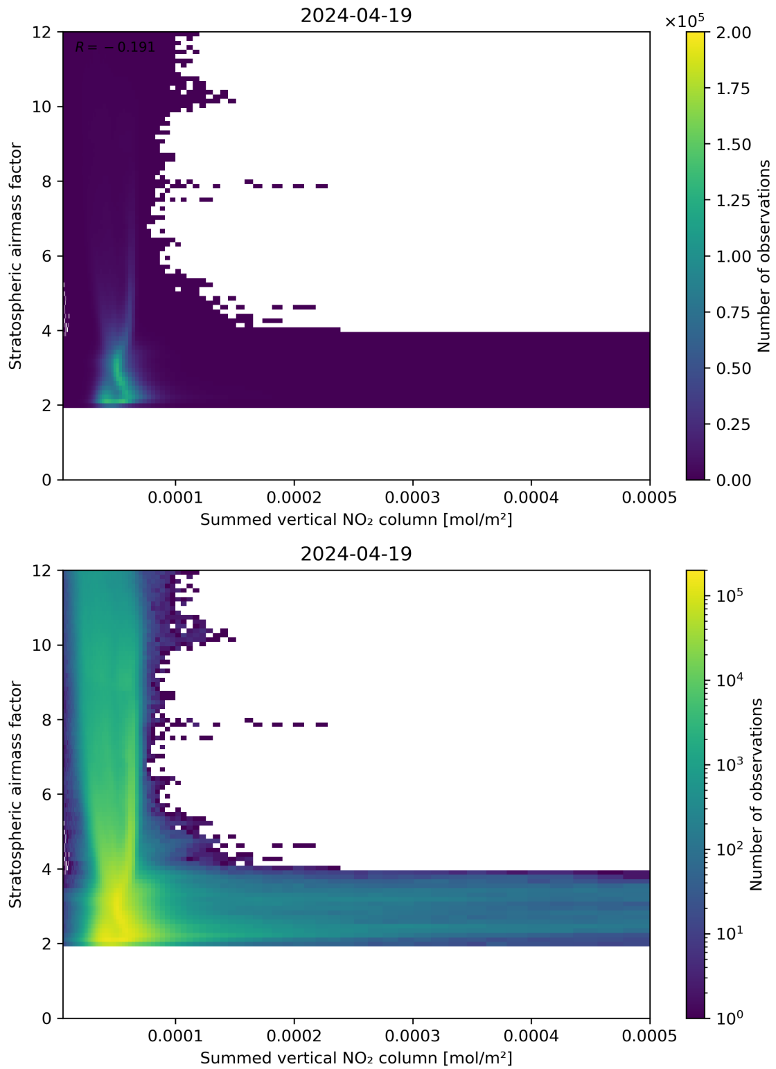
Figure 103: Scatter density plot of “Summed vertical NO 2 column” against “Stratospheric airmass factor” for 2024-04-18 to 2024-04-20.
