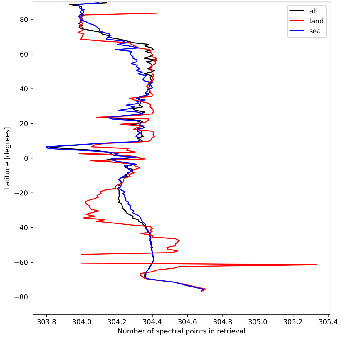
Figure 16: Zonal average of “Number of spectral points in retrieval” for 2024-04-18 to 2024-04-20.
