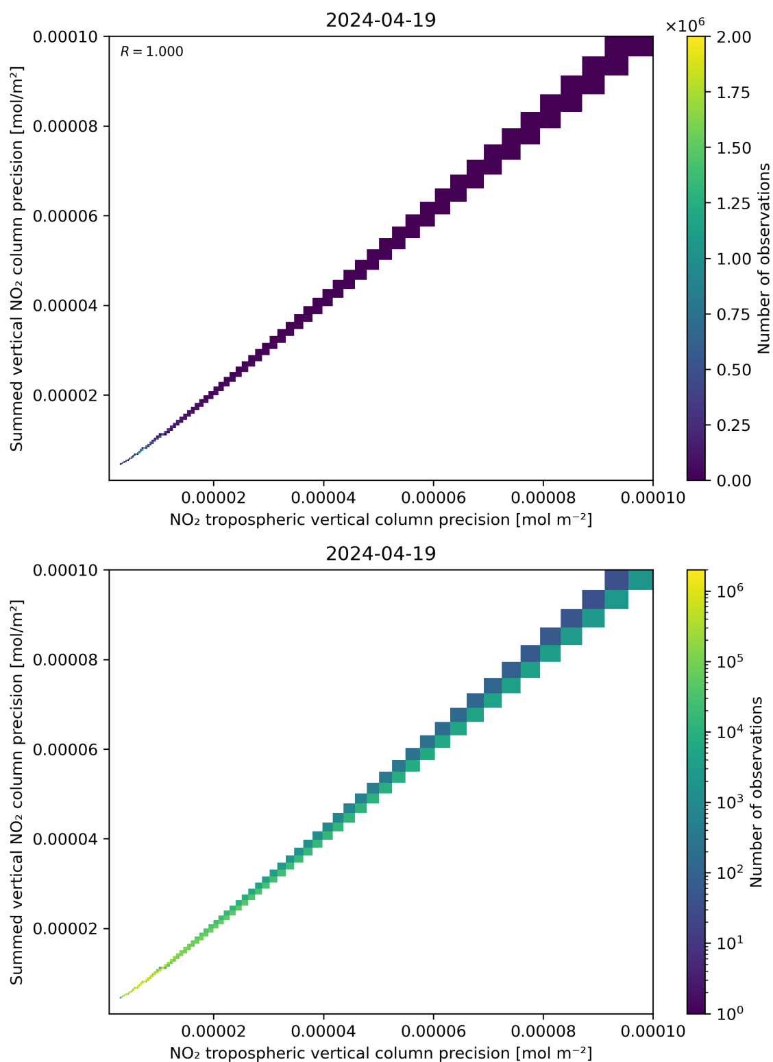
Figure 137: Scatter density plot of “NO 2 tropospheric vertical column precision” against “Summed vertical NO 2 column precision” for 2024-04-18 to 2024-04-20.
