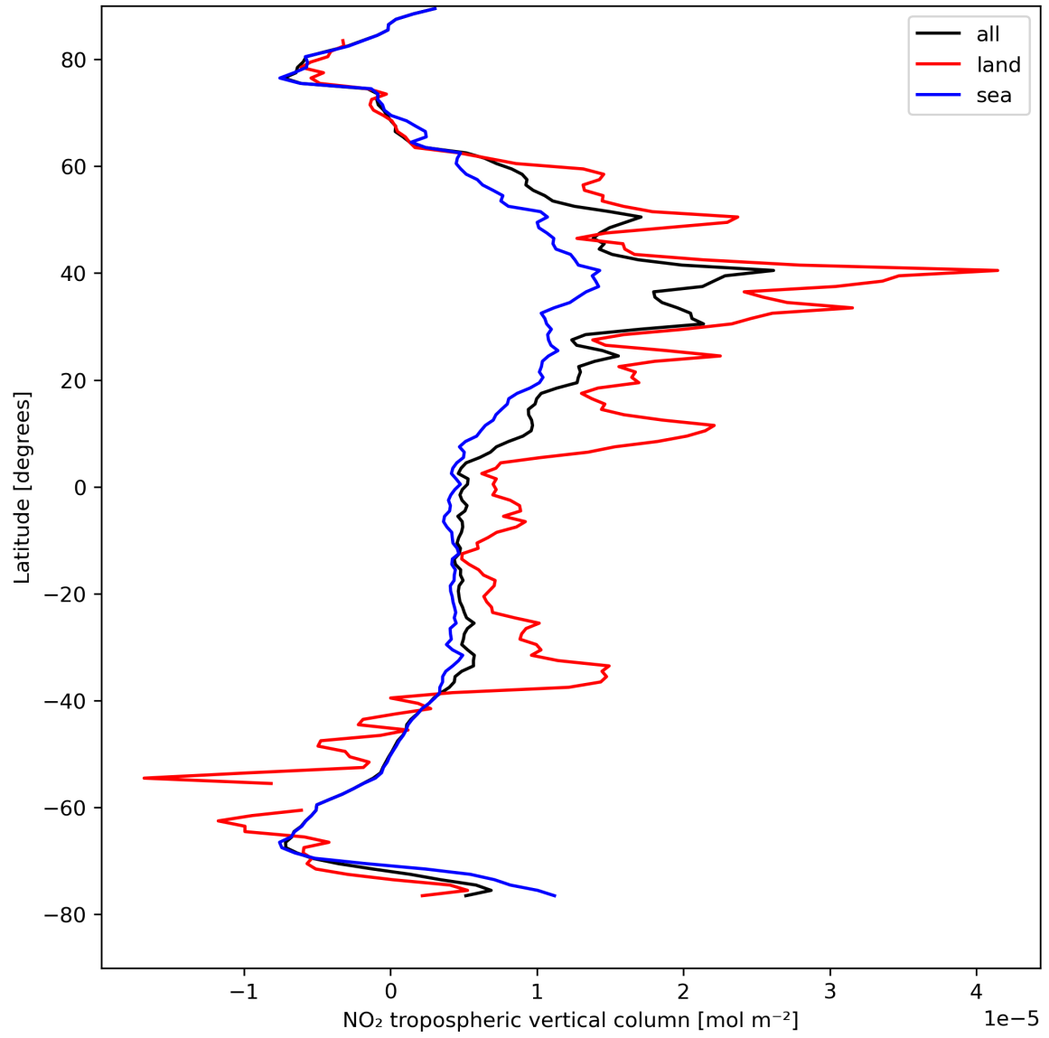
Figure 12: Zonal average of “NO 2 tropospheric vertical column” for 2024-04-18 to 2024-04-20.
