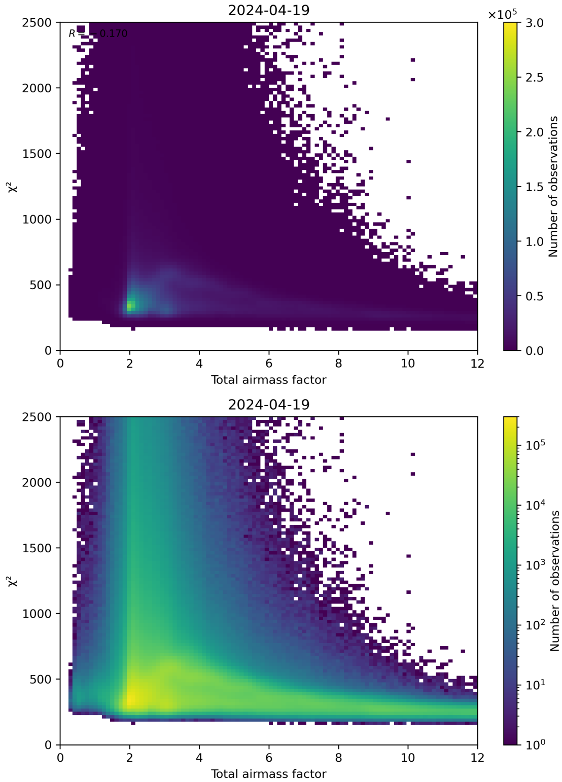
Figure 63: Scatter density plot of “Total airmass factor” against “ \chi^2 ” for 2024-04-18 to 2024-04-20.
