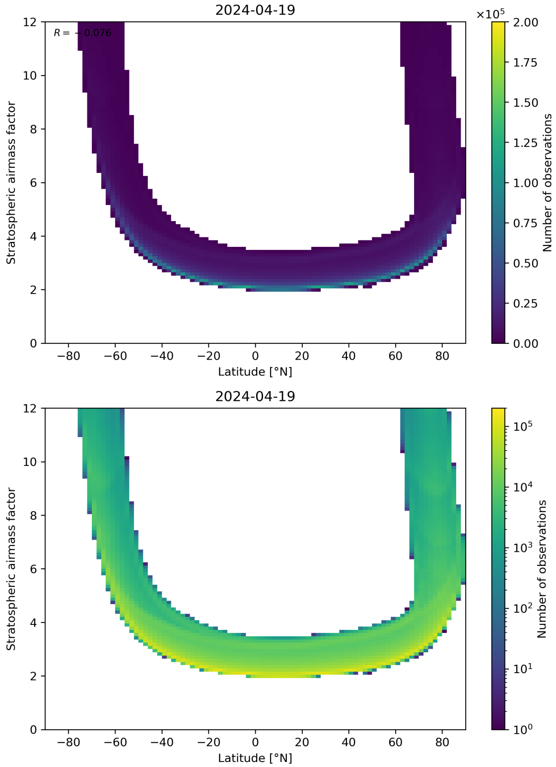
Figure 83: Scatter density plot of “Latitude” against “Stratospheric air mass factor” for 2024-04-18 to 2024-04-20.
