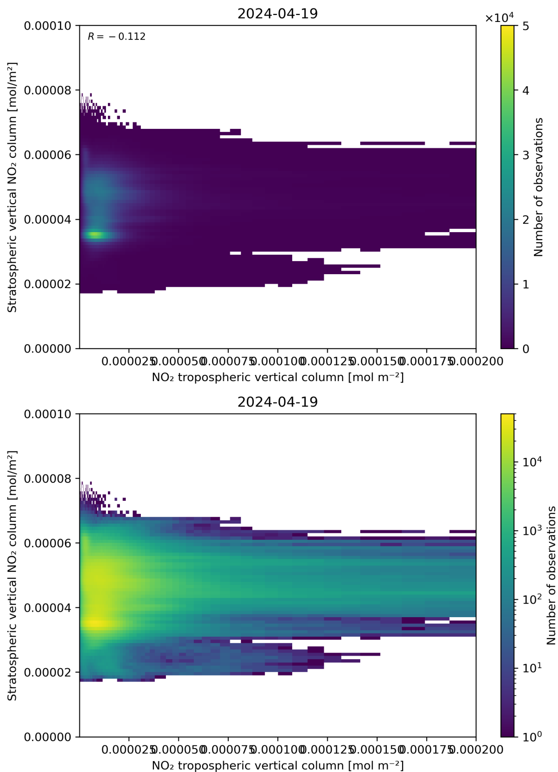
Figure 125: Scatter density plot of “NO 2 tropospheric vertical column” against “Stratospheric vertical NO 2 column” for 2024-04-18 to 2024-04-20.
