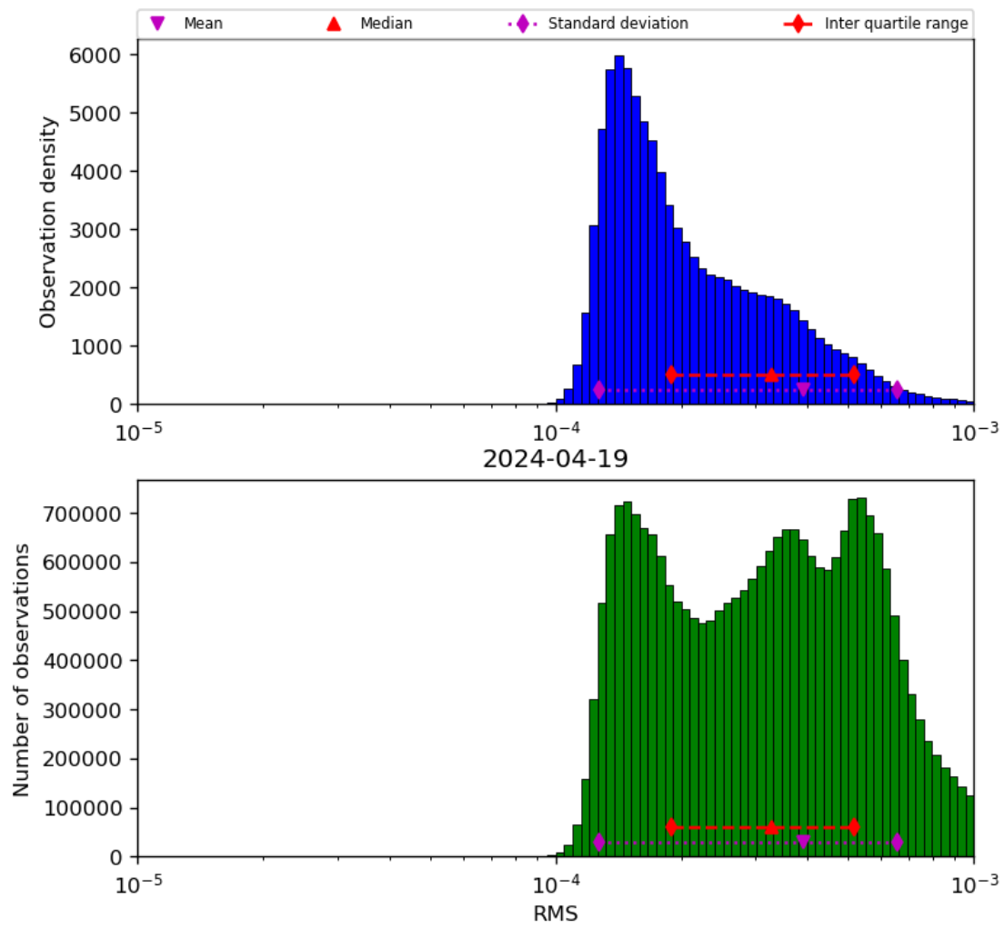
Figure 43: Histogram of “RMS” for 2024-04-18 to 2024-04-20
