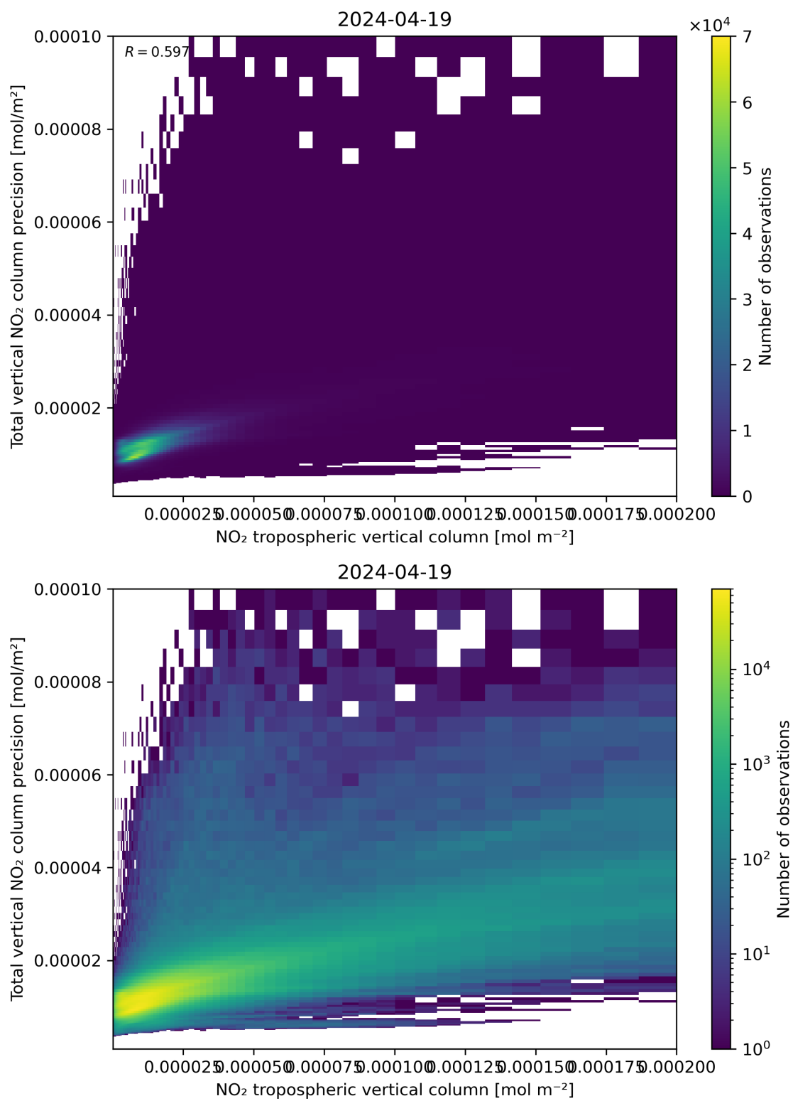
Figure 129: Scatter density plot of “NO 2 tropospheric vertical column” against “Total vertical NO 2 column precision” for 2024-04-18 to 2024-04-20.
