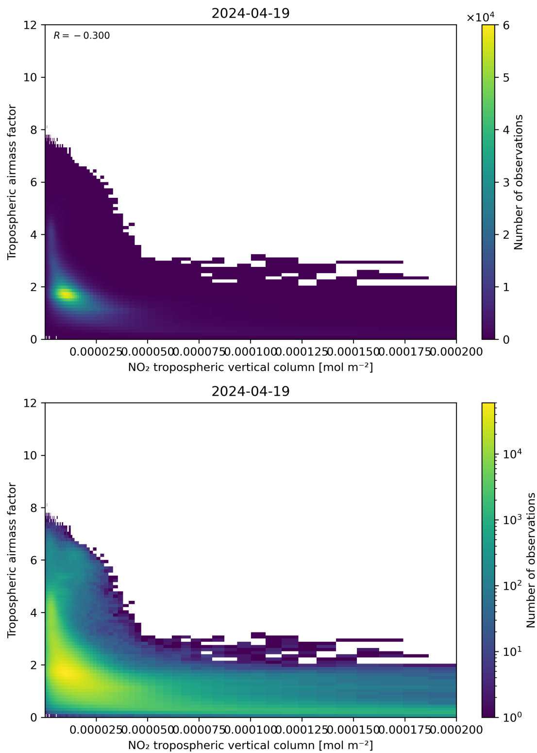
Figure 123: Scatter density plot of “NO 2 tropospheric vertical column” against “Tropospheric air mass factor” for 2024-04-18 to 2024-04-20.
