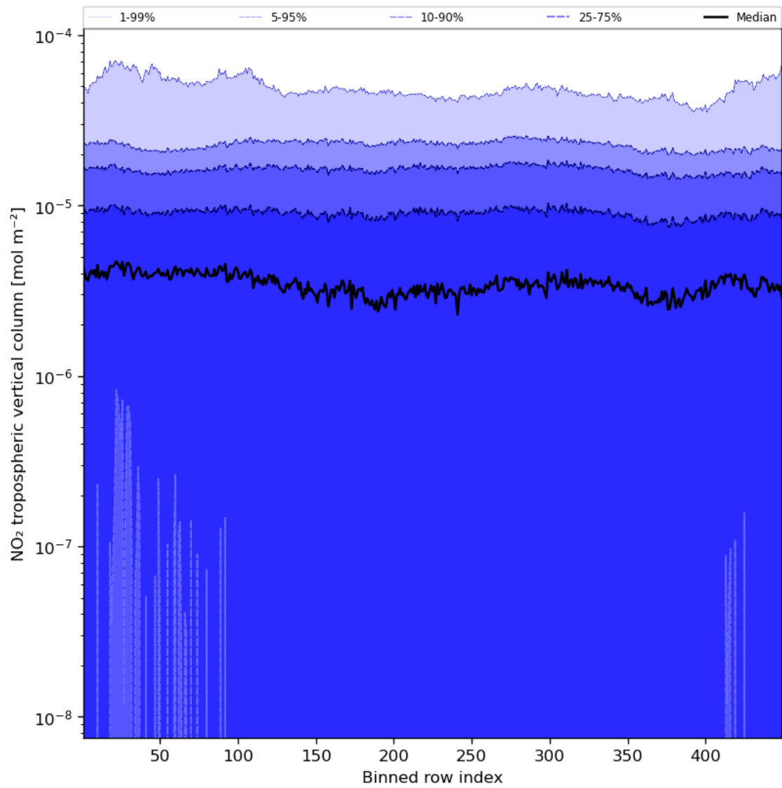
Figure 46: Along track statistics of “NO 2 tropospheric vertical column” for 2024-04-18 to 2024-04-20
