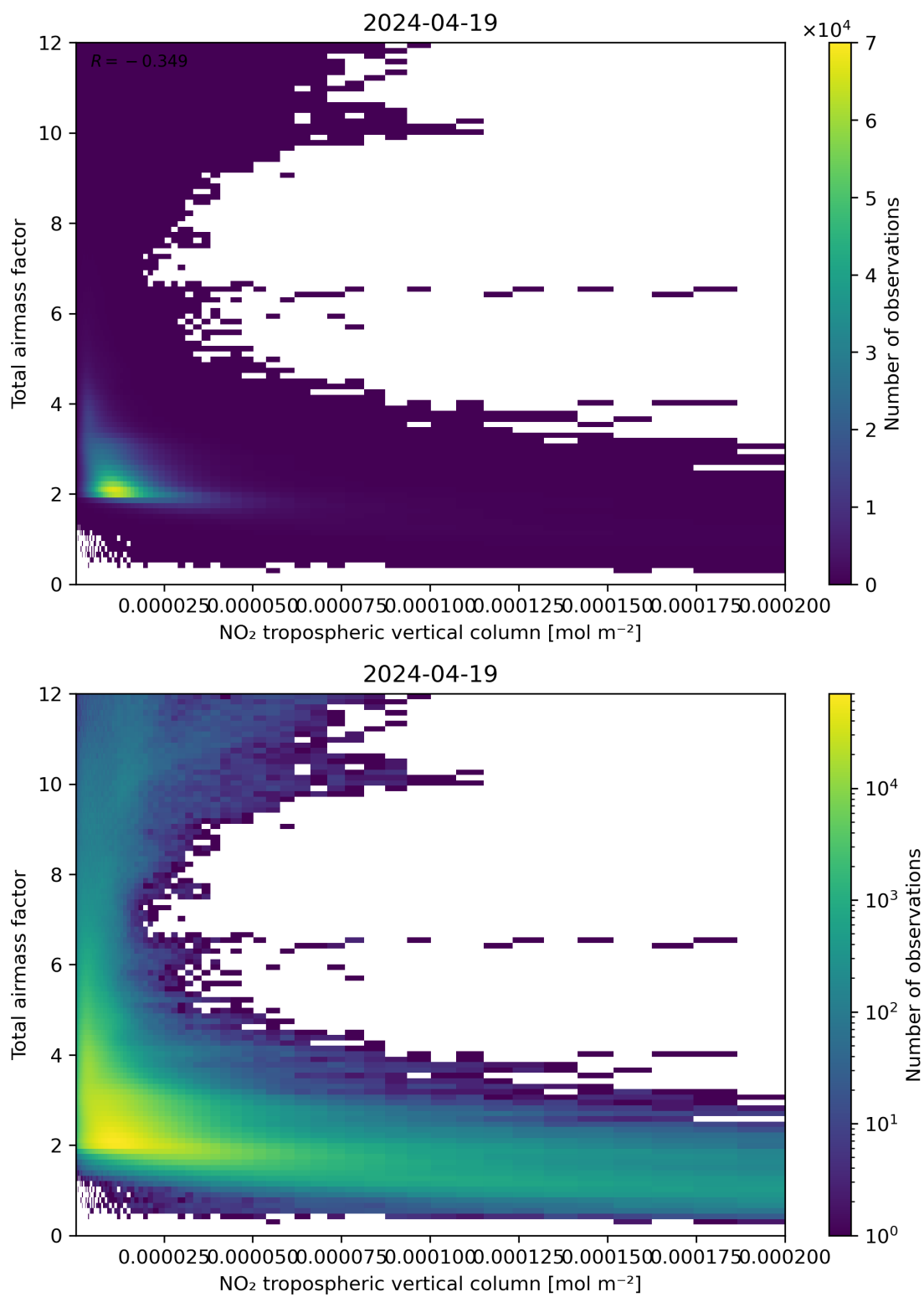
Figure 122: Scatter density plot of “NO 2 tropospheric vertical column” against “Total air mass factor” for 2024-04-18 to 2024-04-20.
