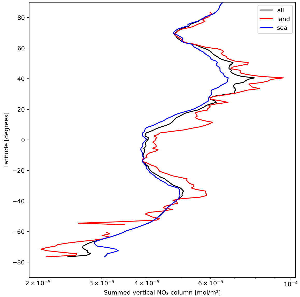
Figure 23: Zonal average of “Summed vertical NO 2 column” for 2024-04-18 to 2024-04-20.
