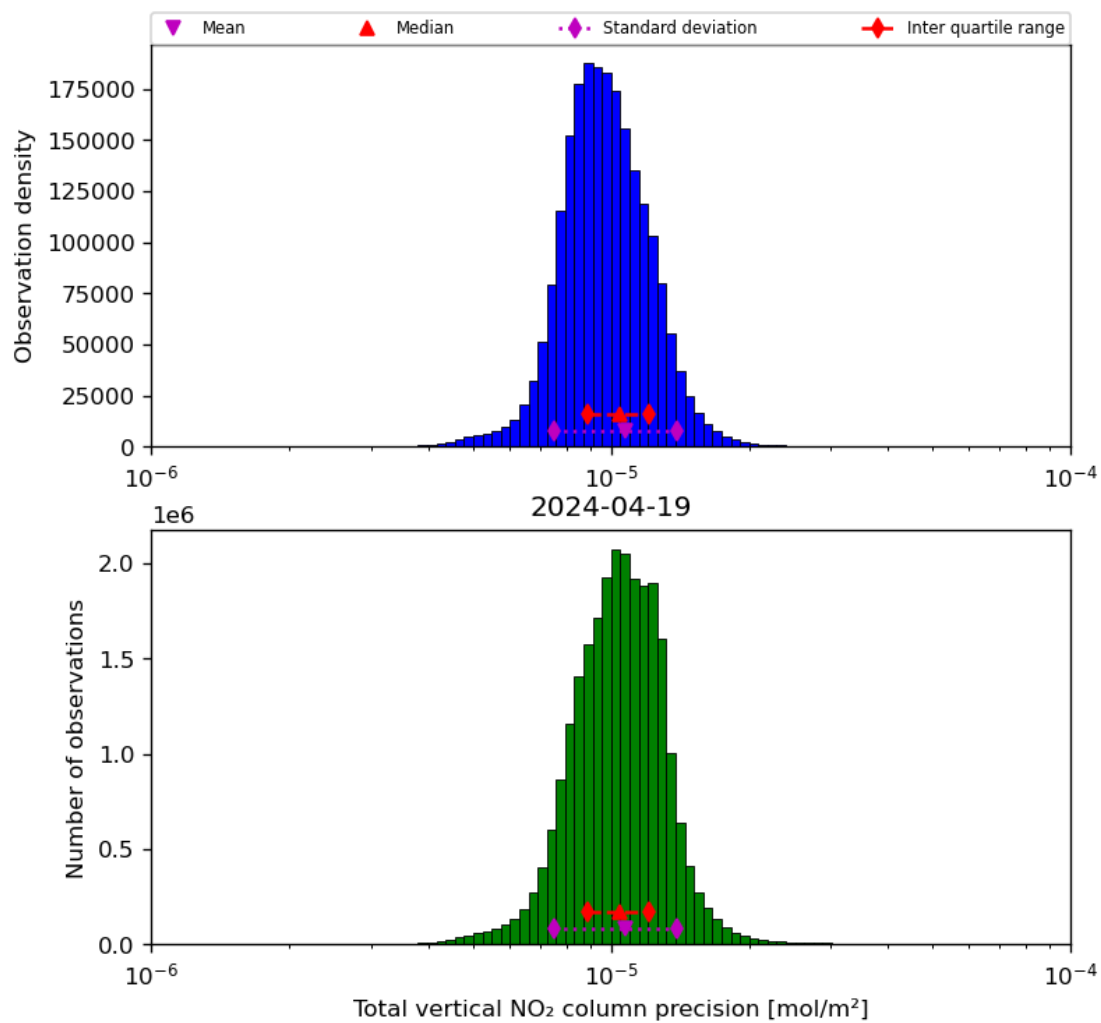
Figure 39: Histogram of “Total vertical NO 2 column precision” for 2024-04-18 to 2024-04-20
