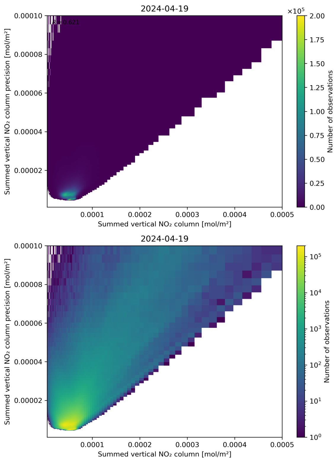
Figure 105: Scatter density plot of “Summed vertical NO 2 column” against “Summed vertical NO 2 column precision” for 2024-04-18 to 2024-04-20.
