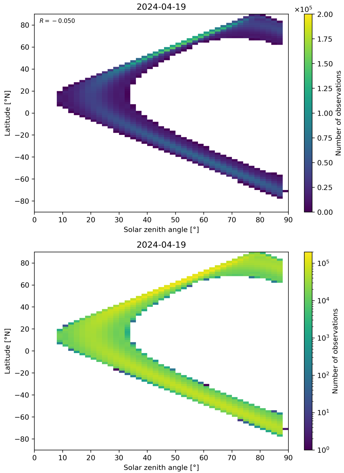
Figure 149: Scatter density plot of “Solar zenith angle” against “Latitude” for 2024-04-18 to 2024-04-20.
