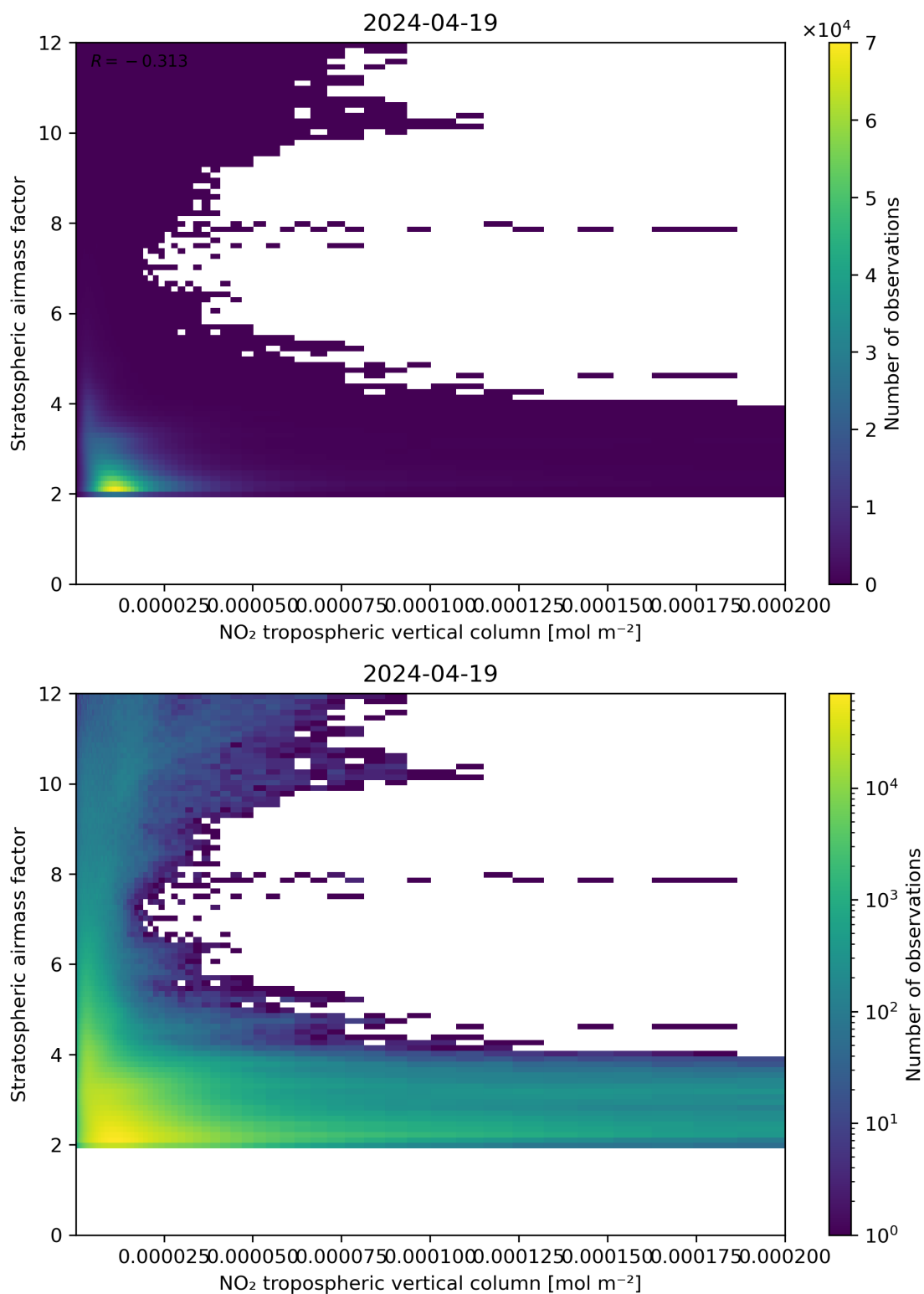
Figure 121: Scatter density plot of “NO 2 tropospheric vertical column” against “Stratospheric air mass factor” for 2024-04-18 to 2024-04-20.
