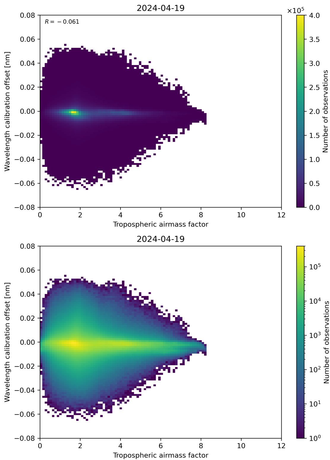
Figure 80: Scatter density plot of “Tropospheric airmass factor” against “Wavelength calibration offset” for 2024-04-18 to 2024-04-20.
