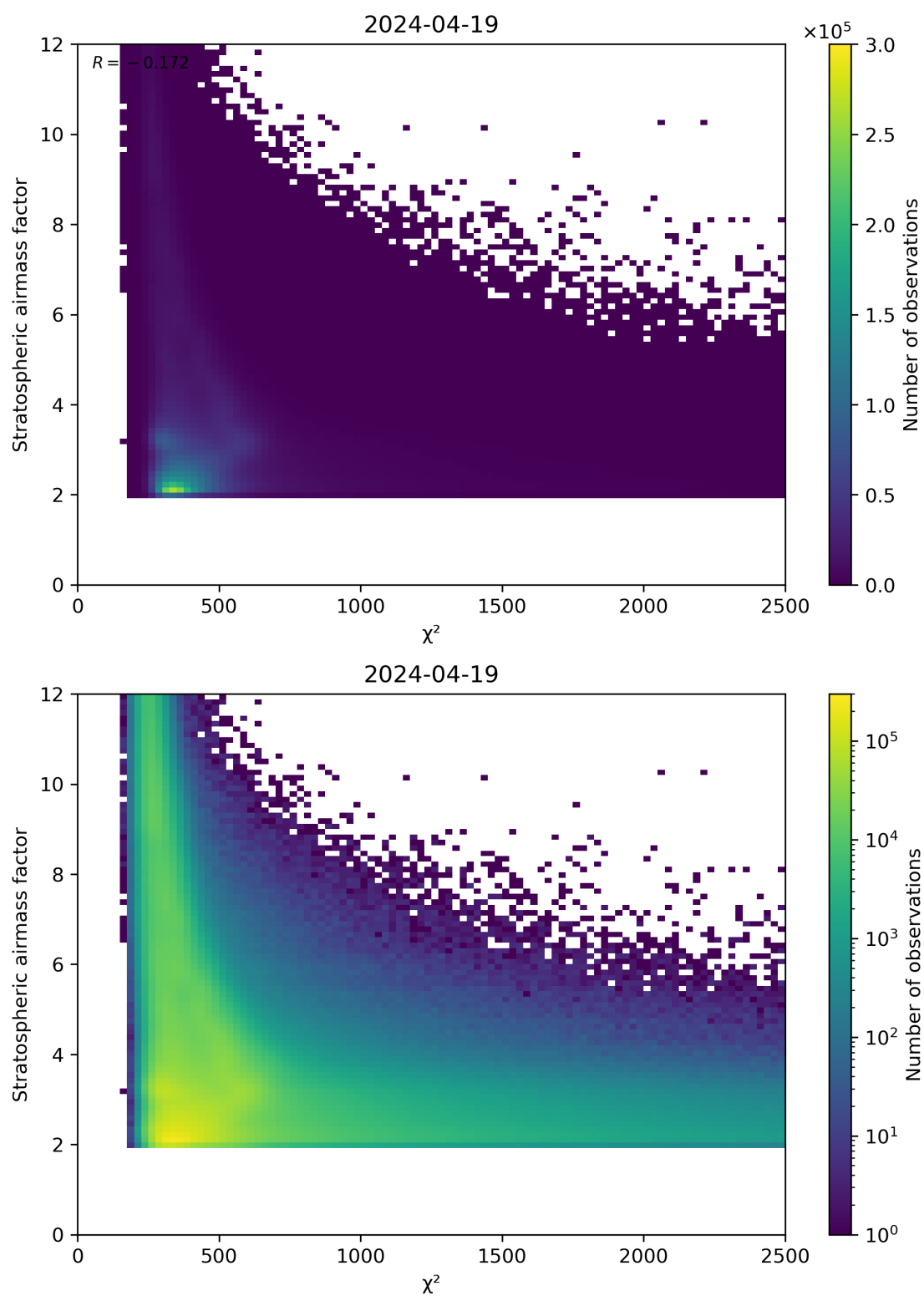
Figure 81: Scatter density plot of “ \chi^2 ” against “Stratospheric airmass factor” for 2024-04-18 to 2024-04-20.
