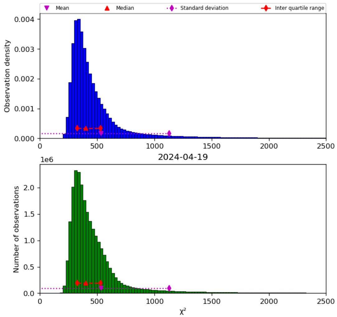
Figure 42: Histogram of “ \chi^2 ” for 2024-04-18 to 2024-04-20
