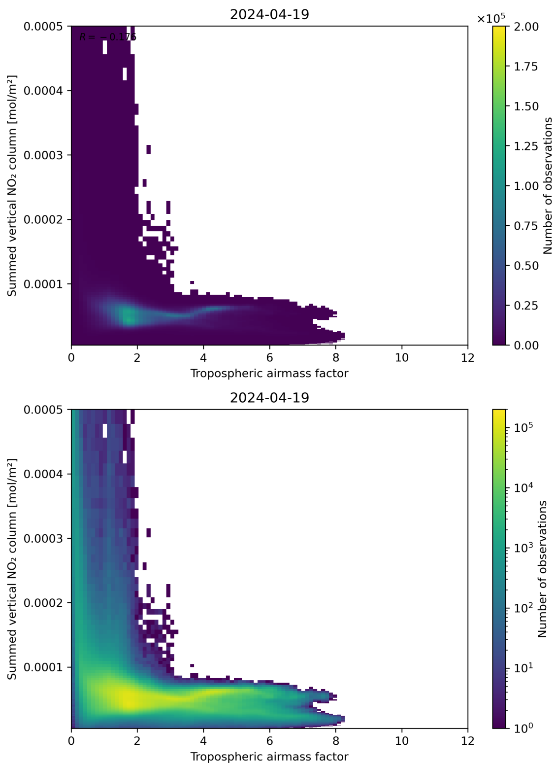
Figure 75: Scatter density plot of “Tropospheric air mass factor” against “Summed vertical NO 2 column” for 2024-04-18 to 2024-04-20.
