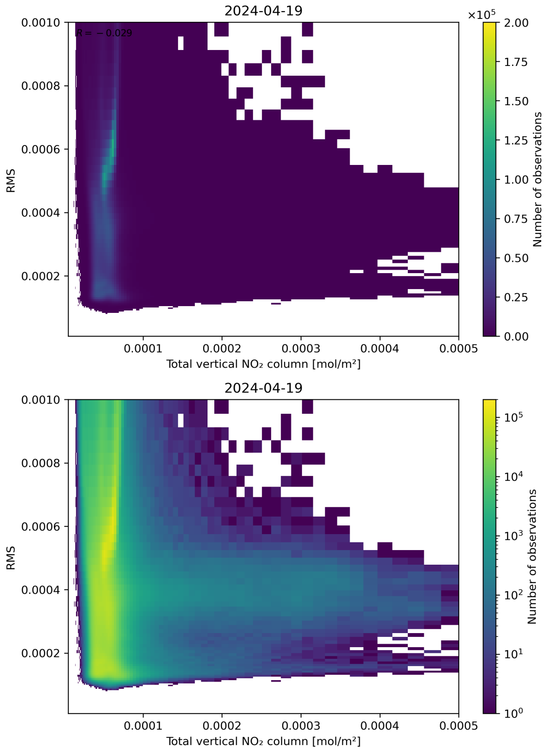
Figure 120: Scatter density plot of “Total vertical NO 2 column” against “RMS” for 2024-04-18 to 2024-04-20.
