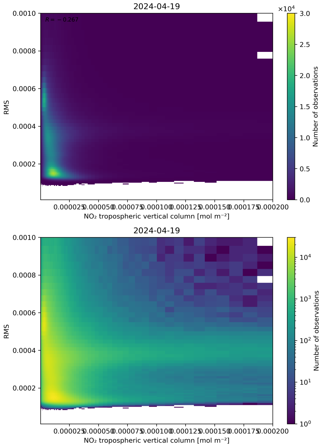
Figure 142: Scatter density plot of “NO 2 tropospheric vertical column” against “RMS” for 2024-04-18 to 2024-04-20.
