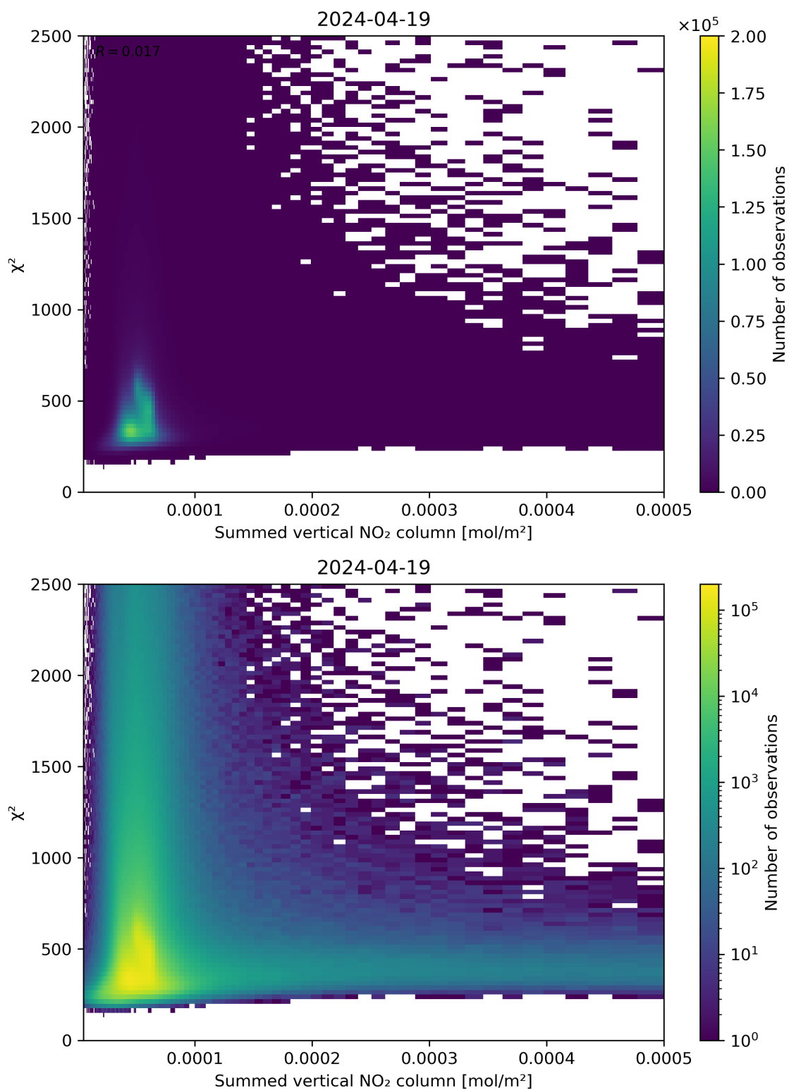
Figure 104: Scatter density plot of “Summed vertical NO 2 column” against “ \chi^2 ” for 2024-04-18 to 2024-04-20.
