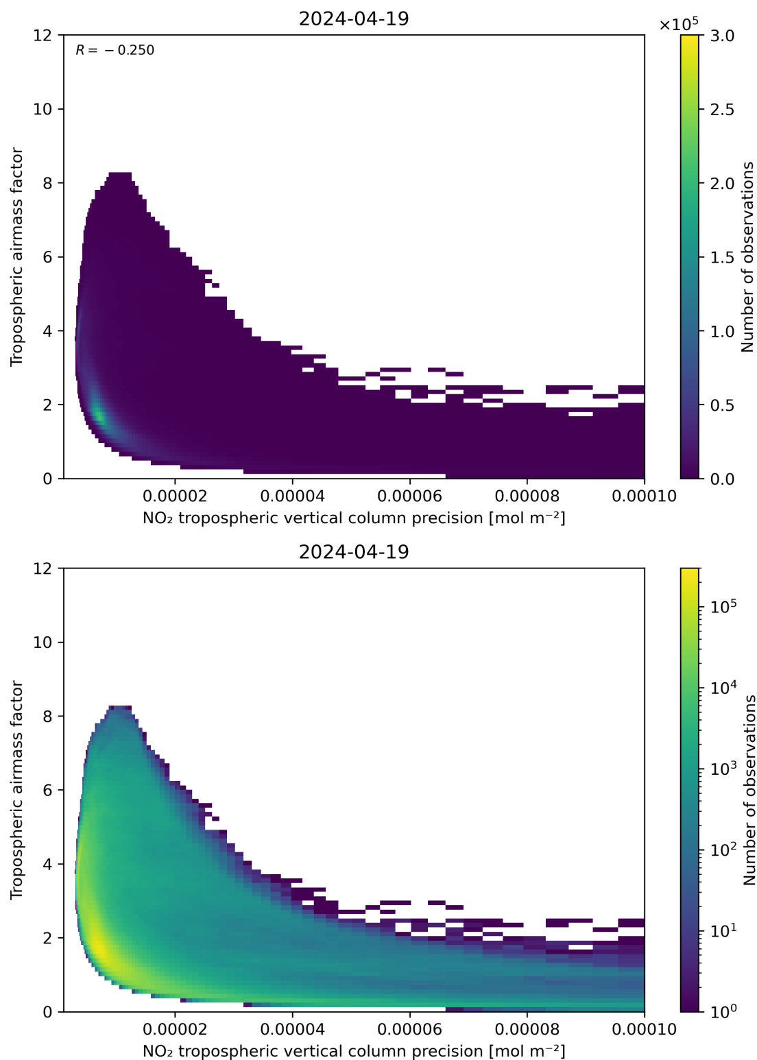
Figure 133: Scatter density plot of “NO 2 tropospheric vertical column precision” against “Tropospheric airmass factor” for 2024-04-18 to 2024-04-20.
