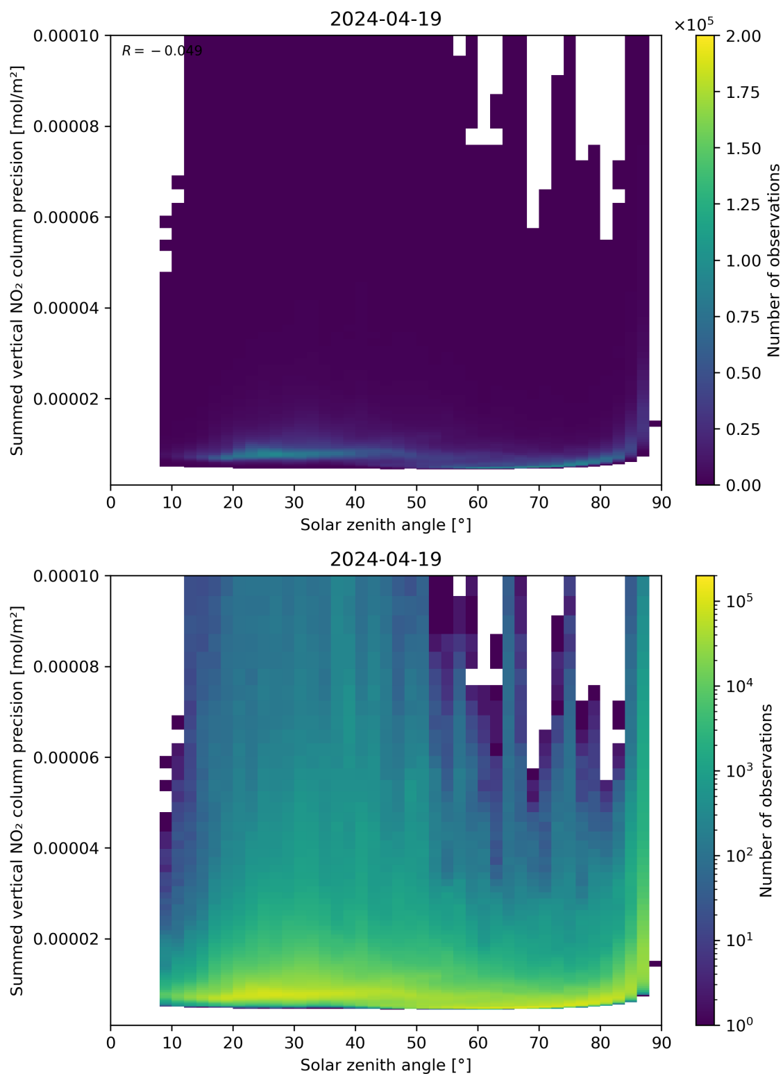
Figure 152: Scatter density plot of “Solar zenith angle” against “Summed vertical NO 2 column precision” for 2024-04-18 to 2024-04-20.
