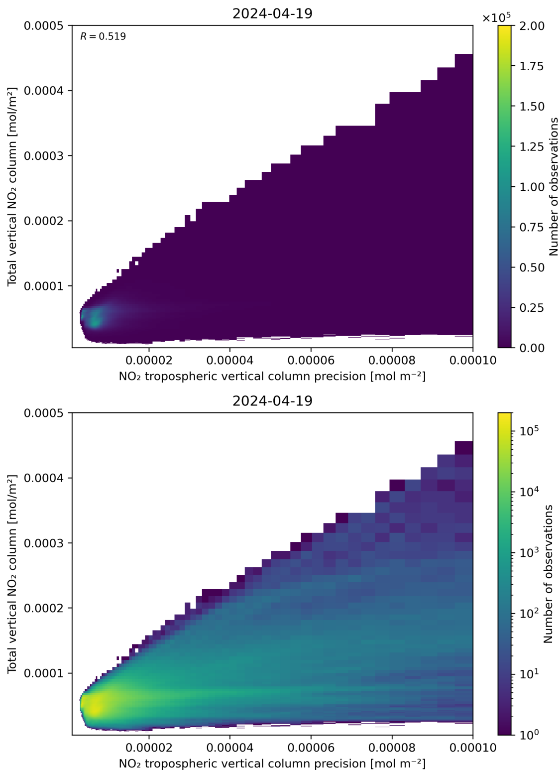
Figure 138: Scatter density plot of “NO 2 tropospheric vertical column precision” against “Total vertical NO 2 column” for 2024-04-18 to 2024-04-20.
