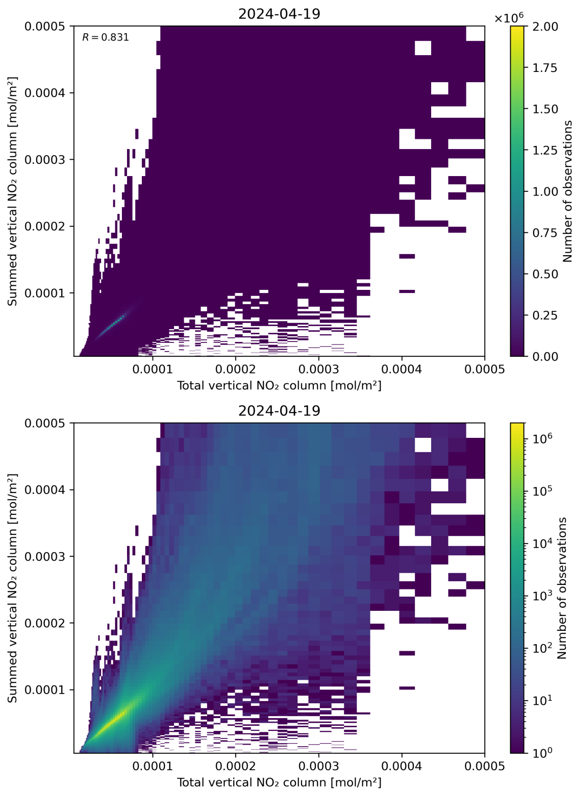
Figure 112: Scatter density plot of “Total vertical NO 2 column” against “Summed vertical NO 2 column” for 2024-04-18 to 2024-04-20.
