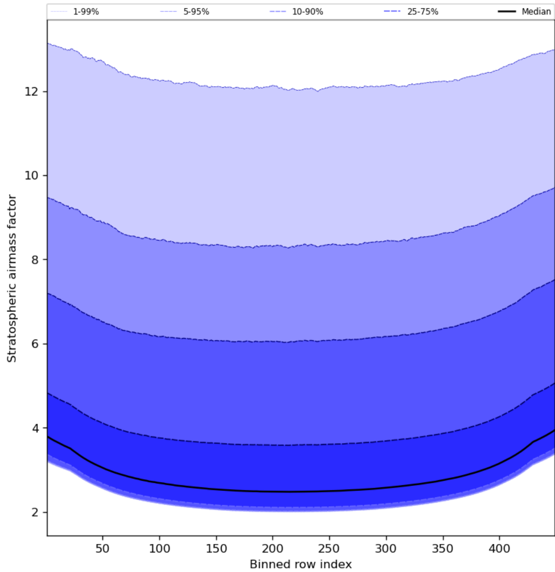
Figure 61: Along track statistics of “Stratospheric airmass factor” for 2024-04-18 to 2024-04-20
