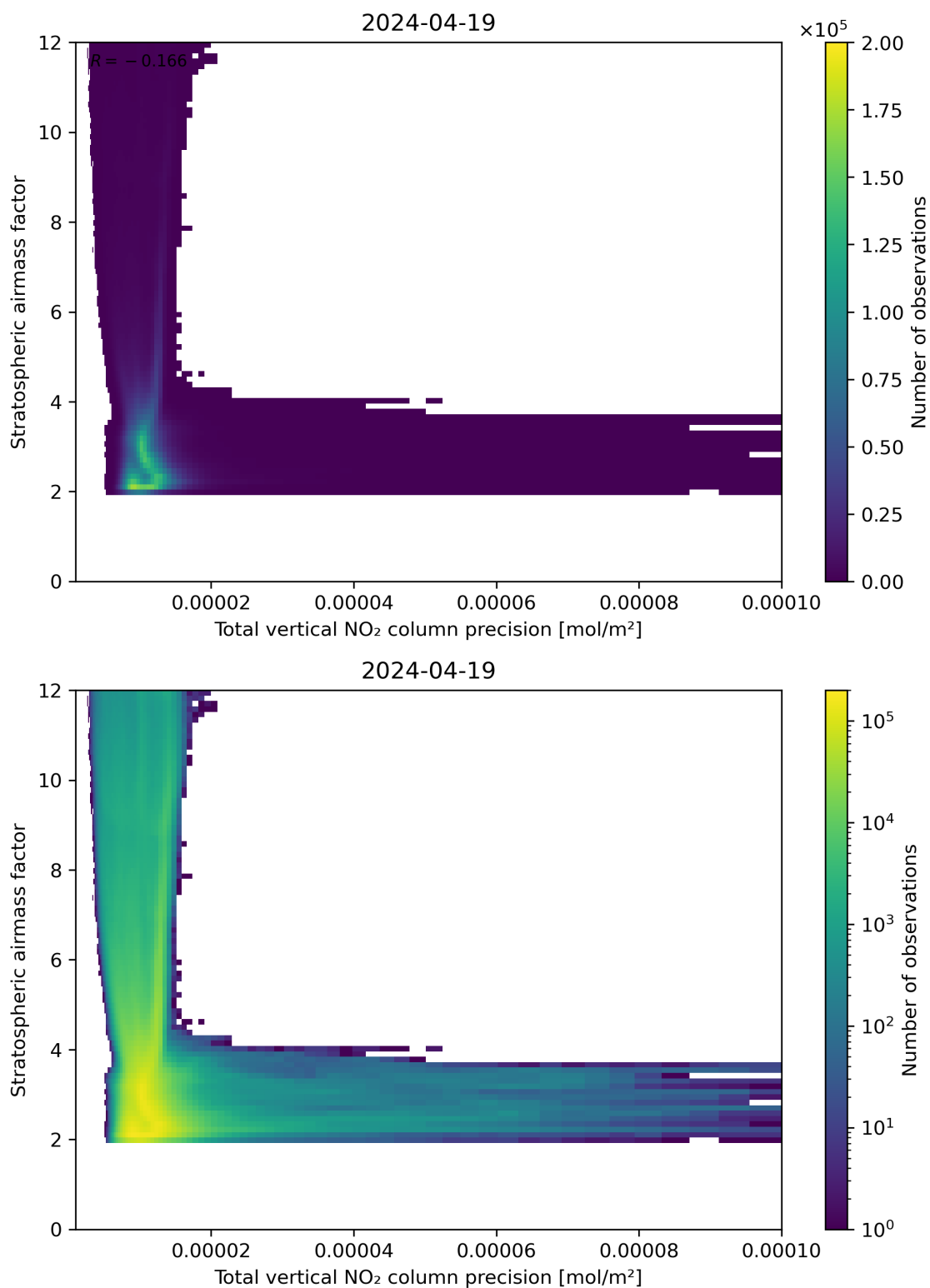
Figure 115: Scatter density plot of “Total vertical NO 2 column precision” against “Stratospheric air mass factor” for 2024-04-18 to 2024-04-20.
