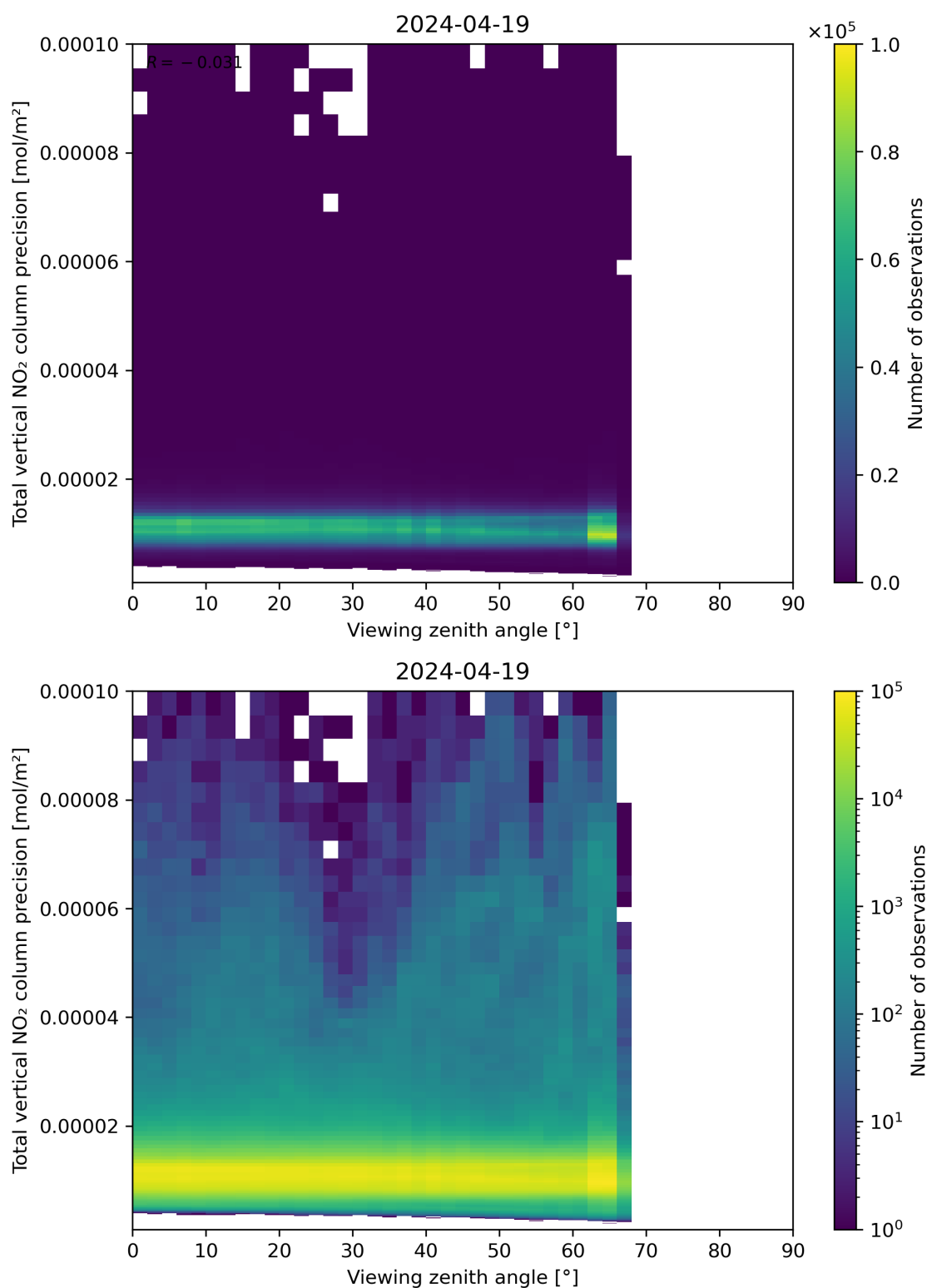
Figure 168: Scatter density plot of “Viewing zenith angle” against “Total vertical NO 2 column precision” for 2024-04-18 to 2024-04-20.
