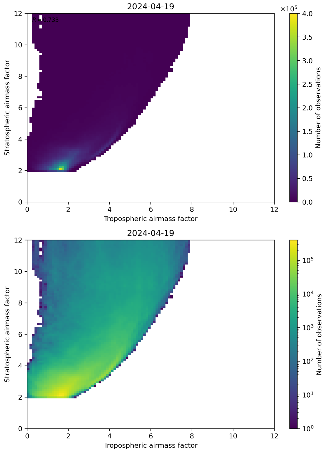
Figure 71: Scatter density plot of “Tropospheric airmass factor” against “Stratospheric airmass factor” for 2024-04-18 to 2024-04-20.
