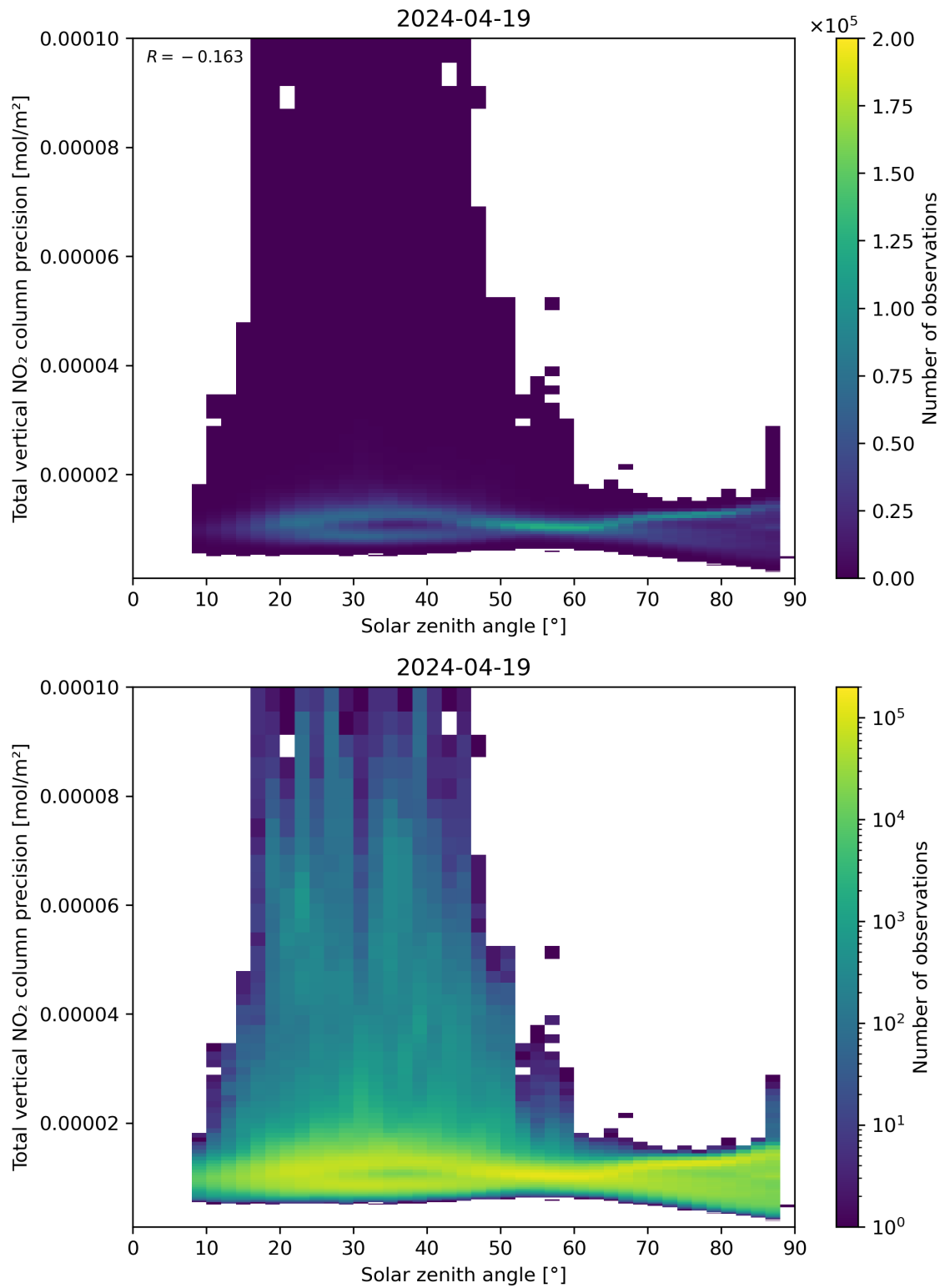
Figure 154: Scatter density plot of “Solar zenith angle” against “Total vertical NO 2 column precision” for 2024-04-18 to 2024-04-20.
