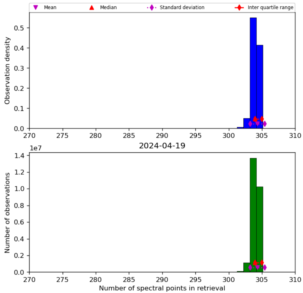
Figure 33: Histogram of “Number of spectral points in retrieval” for 2024-04-18 to 2024-04-20
