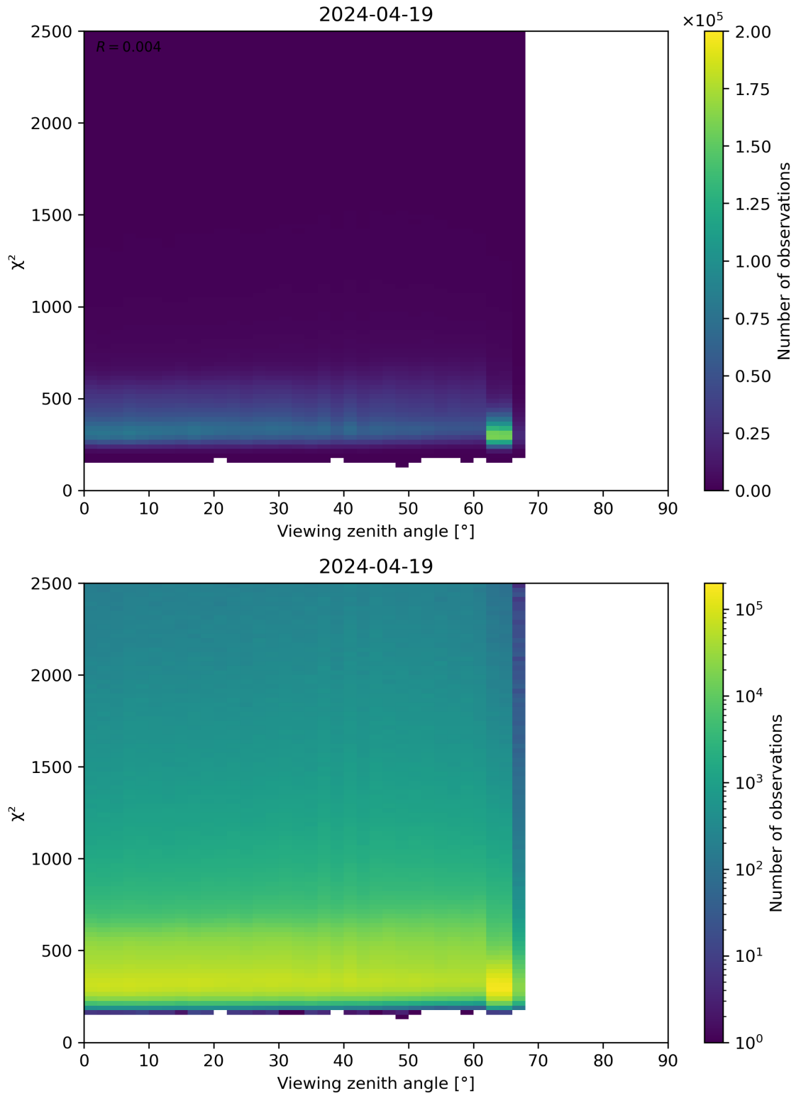
Figure 162: Scatter density plot of “Viewing zenith angle” against “ \chi^2 ” for 2024-04-18 to 2024-04-20.
