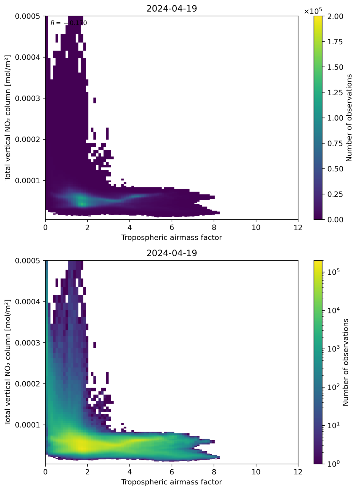
Figure 77: Scatter density plot of “Tropospheric airmass factor” against “Total vertical NO 2 column” for 2024-04-18 to 2024-04-20.
