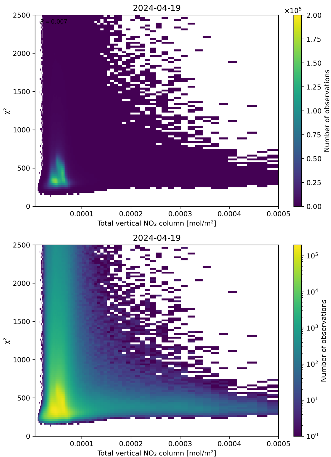
Figure 111: Scatter density plot of “Total vertical NO 2 column” against “ \chi^2 ” for 2024-04-18 to 2024-04-20.
