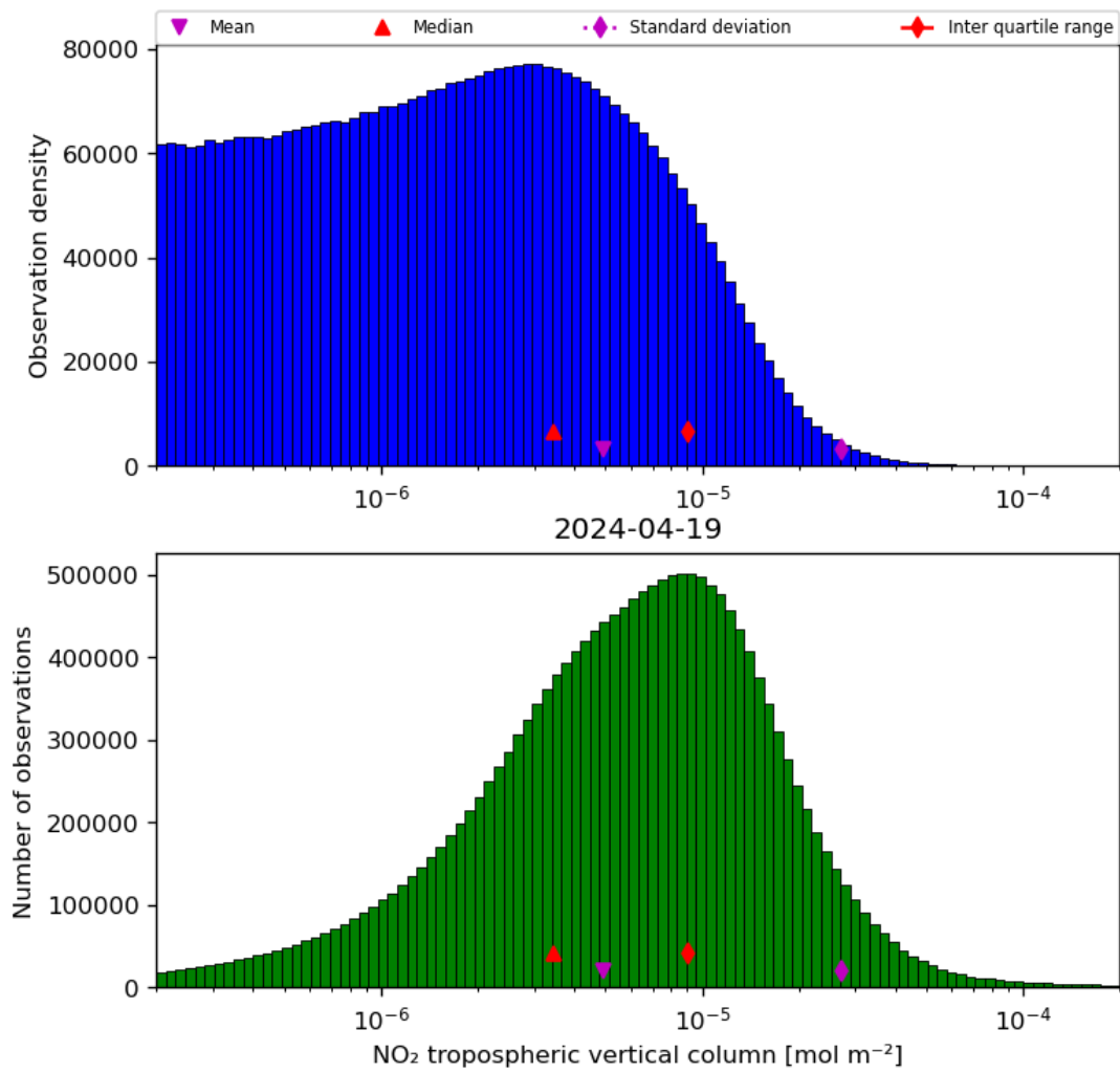
Figure 29: Histogram of “NO 2 tropospheric vertical column” for 2024-04-18 to 2024-04-20
