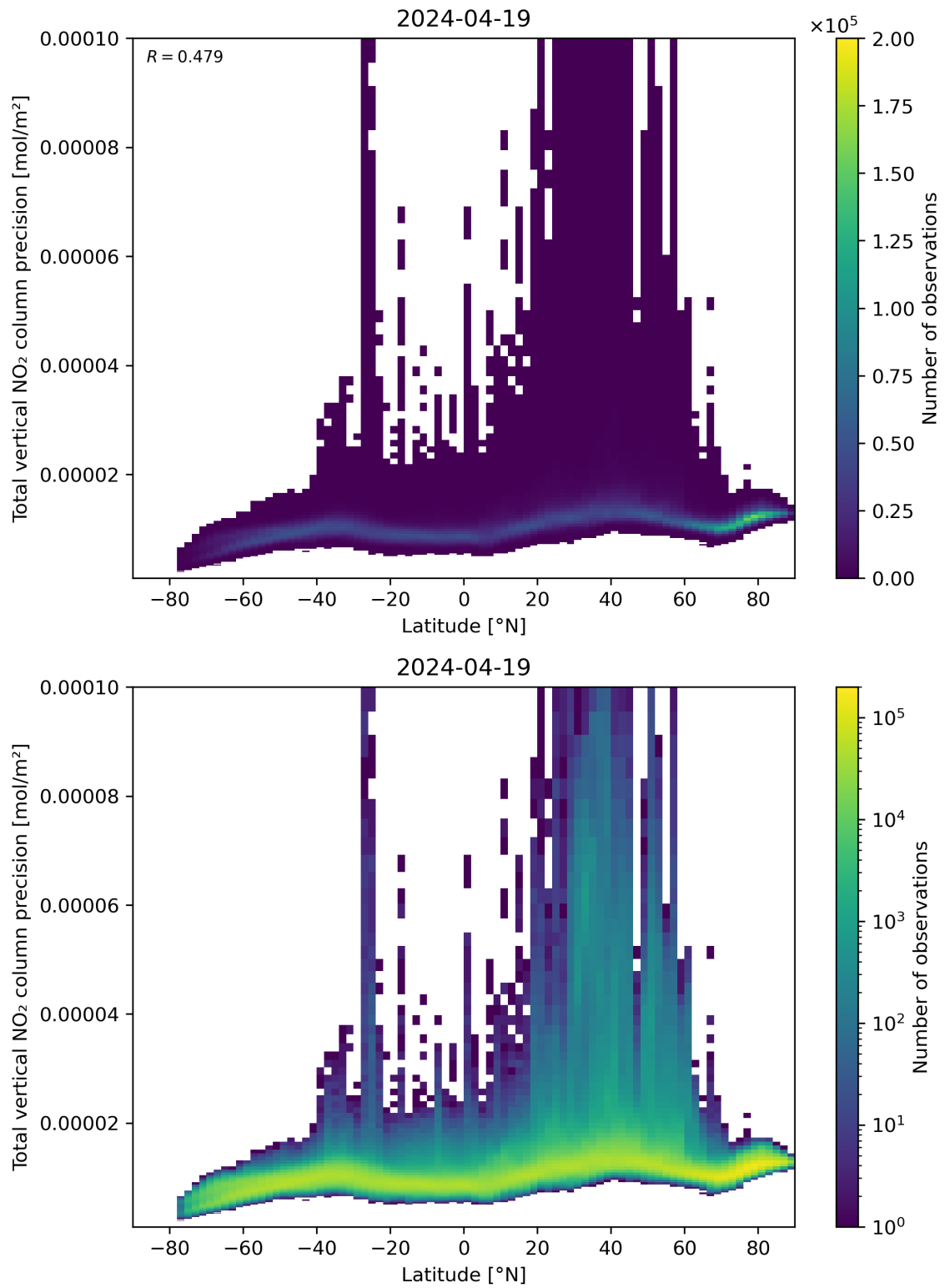
Figure 91: Scatter density plot of “Latitude” against “Total vertical NO 2 column precision” for 2024-04-18 to 2024-04-20.
