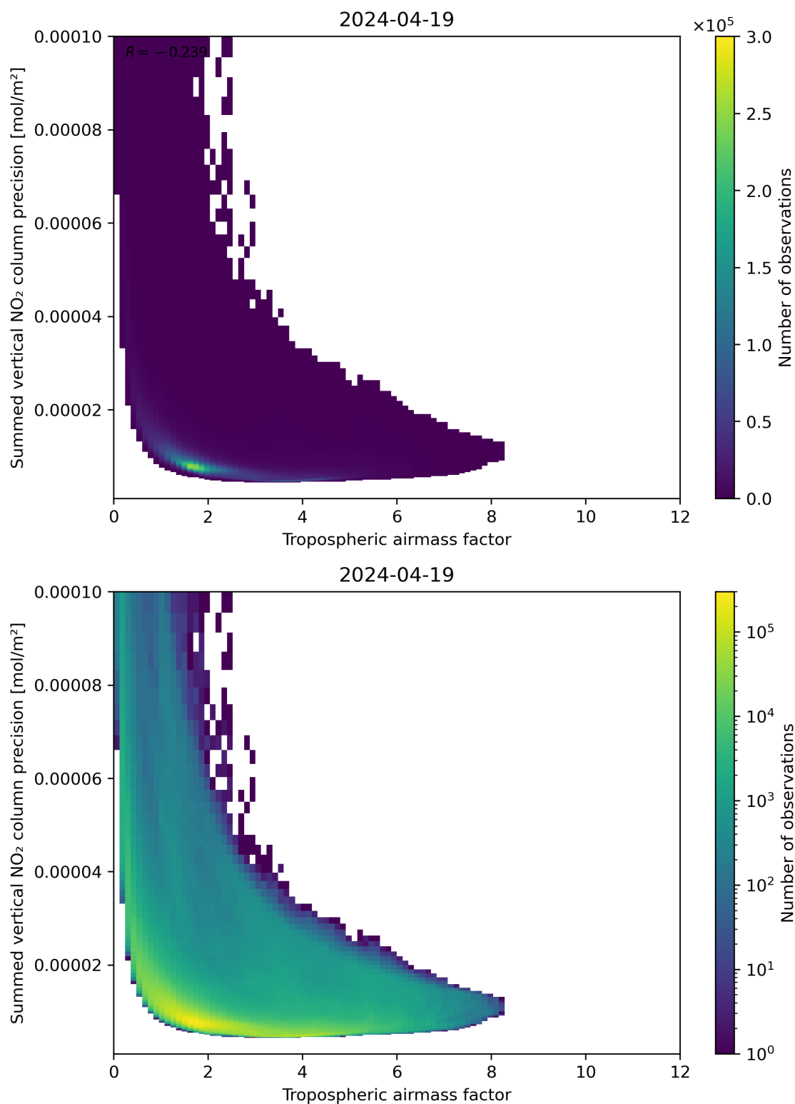
Figure 76: Scatter density plot of “Tropospheric air mass factor” against “Summed vertical NO 2 column precision” for 2024-04-18 to 2024-04-20.
