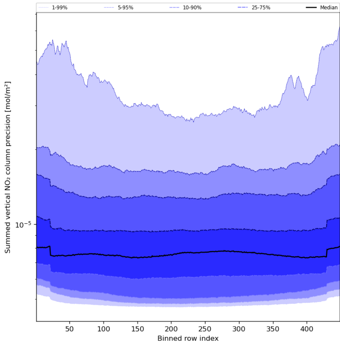
Figure 58: Along track statistics of “Summed vertical NO 2 column precision” for 2024-04-18 to 2024-04-20
