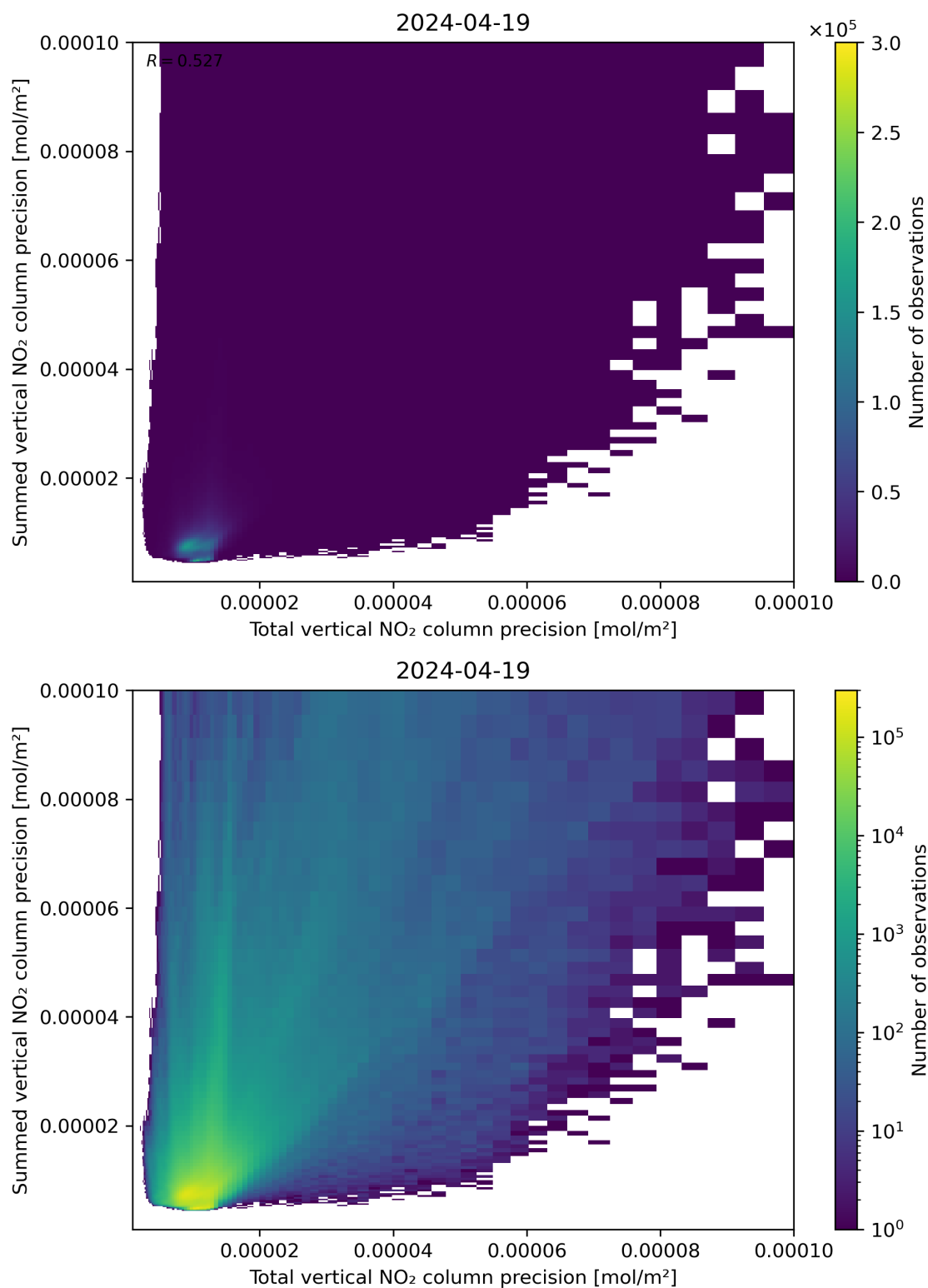
Figure 118: Scatter density plot of “Total vertical NO 2 column precision” against “Summed vertical NO 2 column precision” for 2024-04-18 to 2024-04-20.
