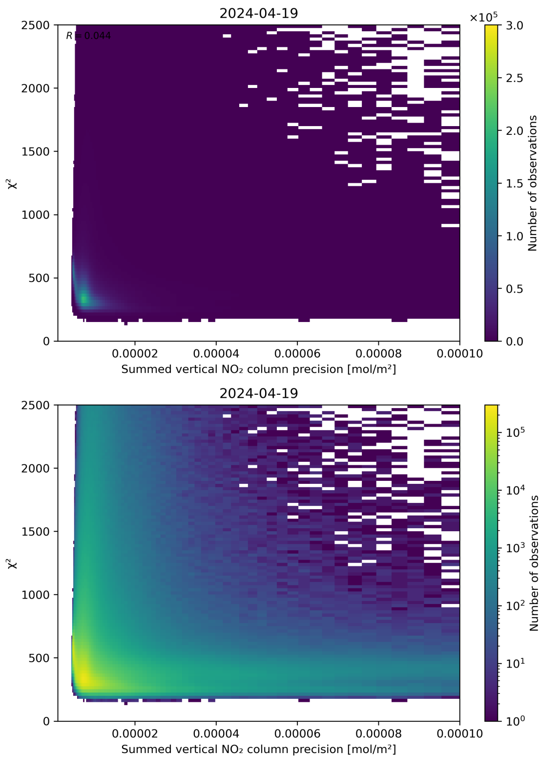
Figure 107: Scatter density plot of “Summed vertical NO 2 column precision” against “ \chi^2 ” for 2024-04-18 to 2024-04-20.
