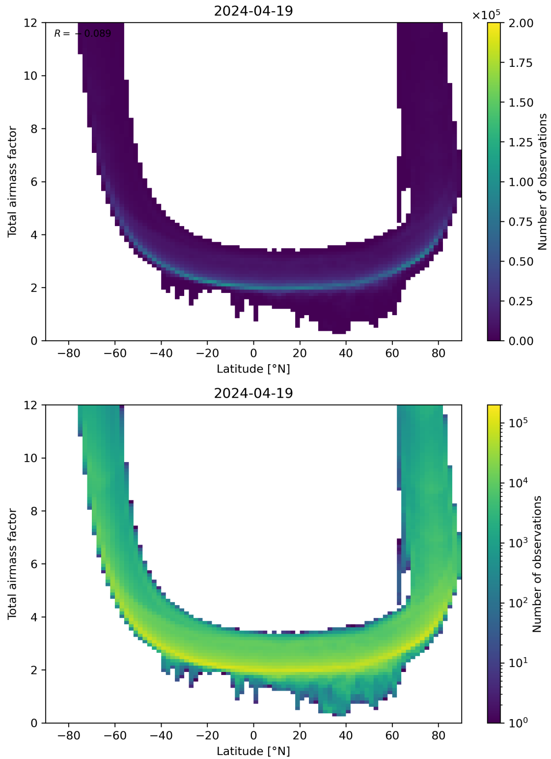
Figure 84: Scatter density plot of “Latitude” against “Total airmass factor” for 2024-04-18 to 2024-04-20.
