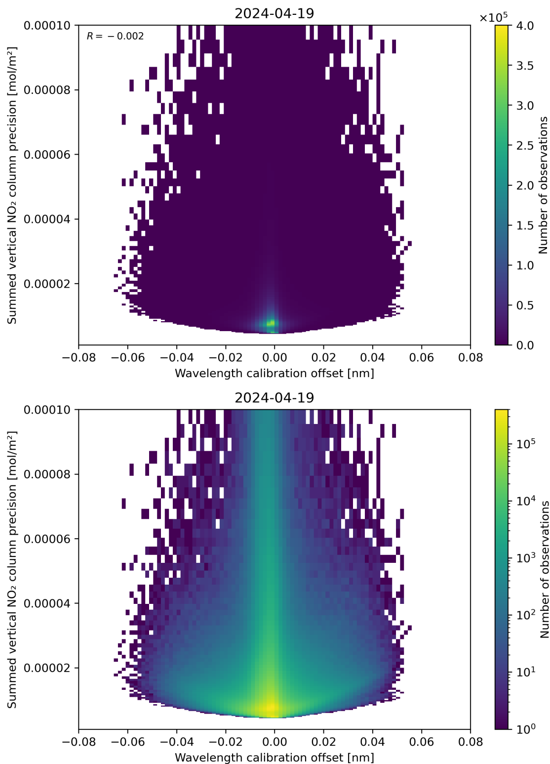
Figure 178: Scatter density plot of “Wavelength calibration offset” against “Summed vertical NO 2 column precision” for 2024-04-18 to 2024-04-20.
