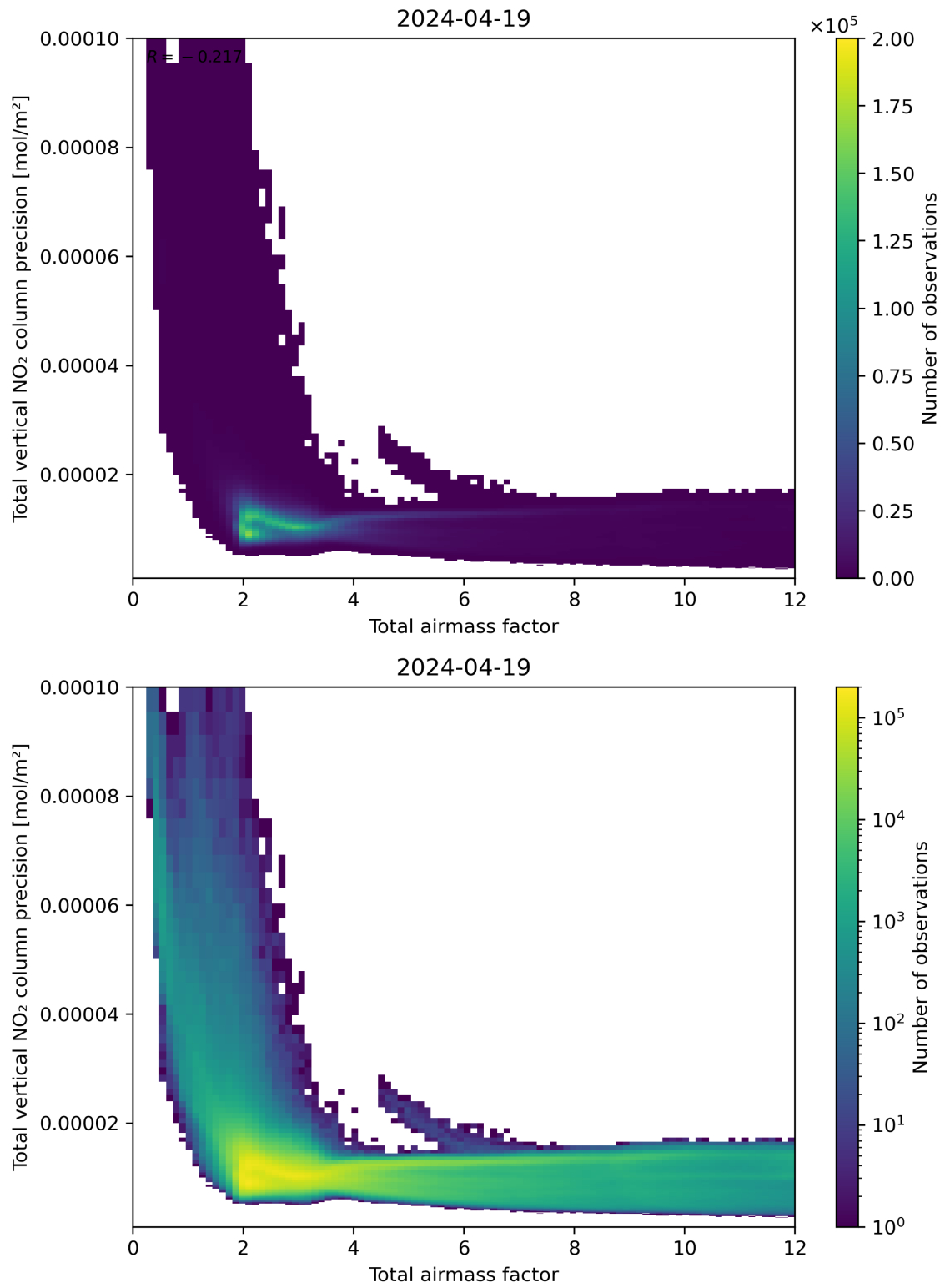
Figure 68: Scatter density plot of “Total airmass factor” against “Total vertical NO 2 column precision” for 2024-04-18 to 2024-04-20.
