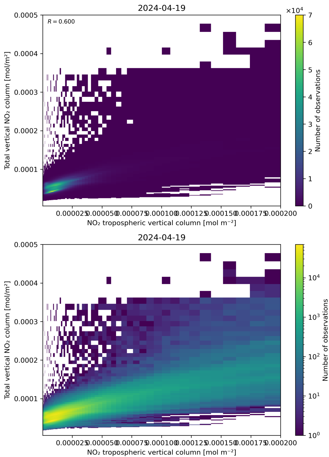
Figure 128: Scatter density plot of “NO 2 tropospheric vertical column” against “Total vertical NO 2 column” for 2024-04-18 to 2024-04-20.
