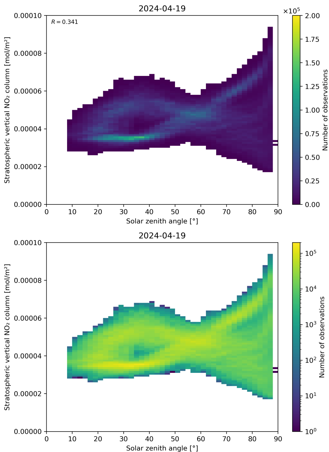
Figure 150: Scatter density plot of “Solar zenith angle” against “Stratospheric vertical NO 2 column” for 2024-04-18 to 2024-04-20.
