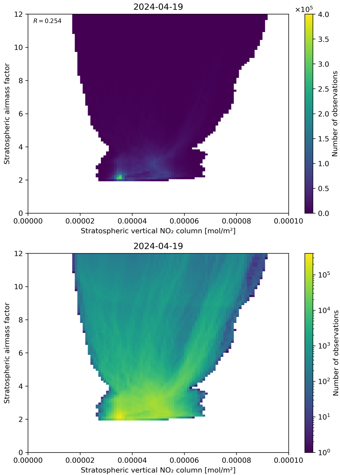
Figure 96: Scatter density plot of “Stratospheric vertical NO 2 column” against “Stratospheric airmass factor” for 2024-04-18 to 2024-04-20.
