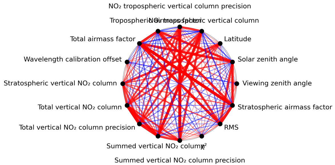
Figure 1: Map of correlation graph for 2024-04-18 to 2024-04-20.
