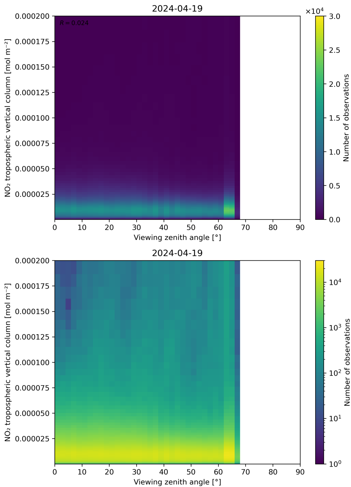
Figure 169: Scatter density plot of “Viewing zenith angle” against “NO 2 tropospheric vertical column” for 2024-04-18 to 2024-04-20.
