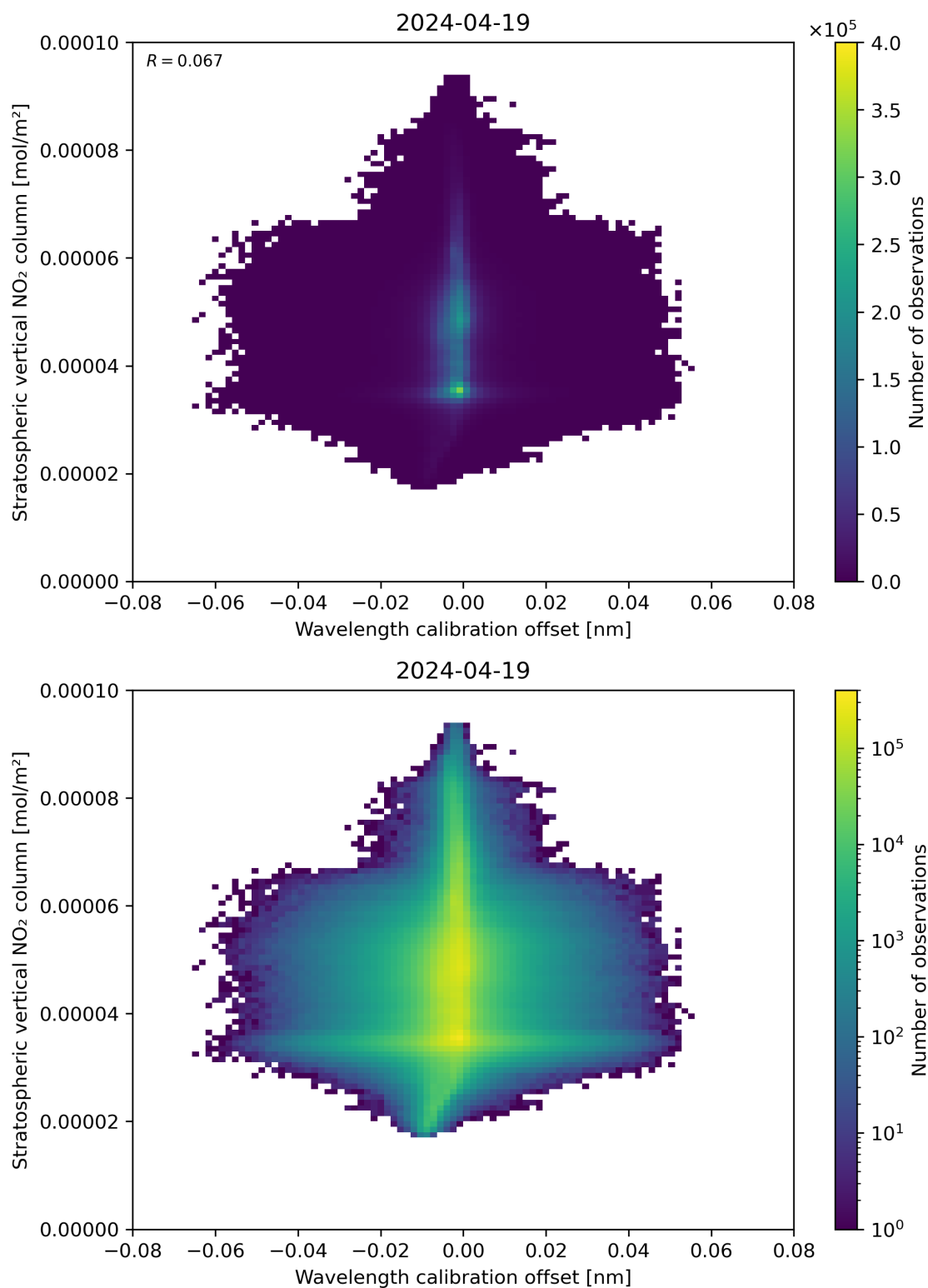
Figure 176: Scatter density plot of “Wavelength calibration offset” against “Stratospheric vertical NO 2 column” for 2024-04-18 to 2024-04-20.
