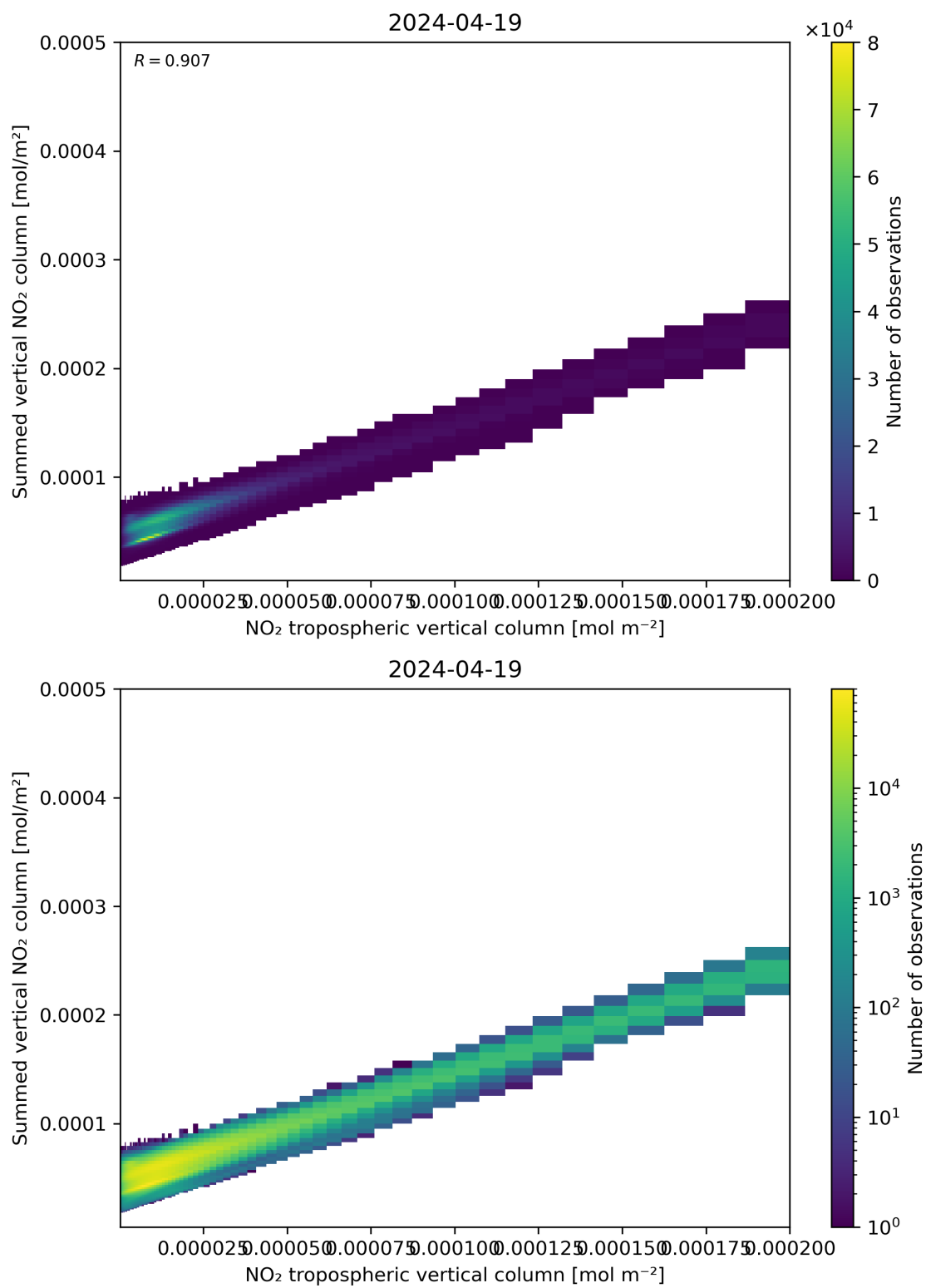
Figure 126: Scatter density plot of “NO 2 tropospheric vertical column” against “Summed vertical NO 2 column” for 2024-04-18 to 2024-04-20.
