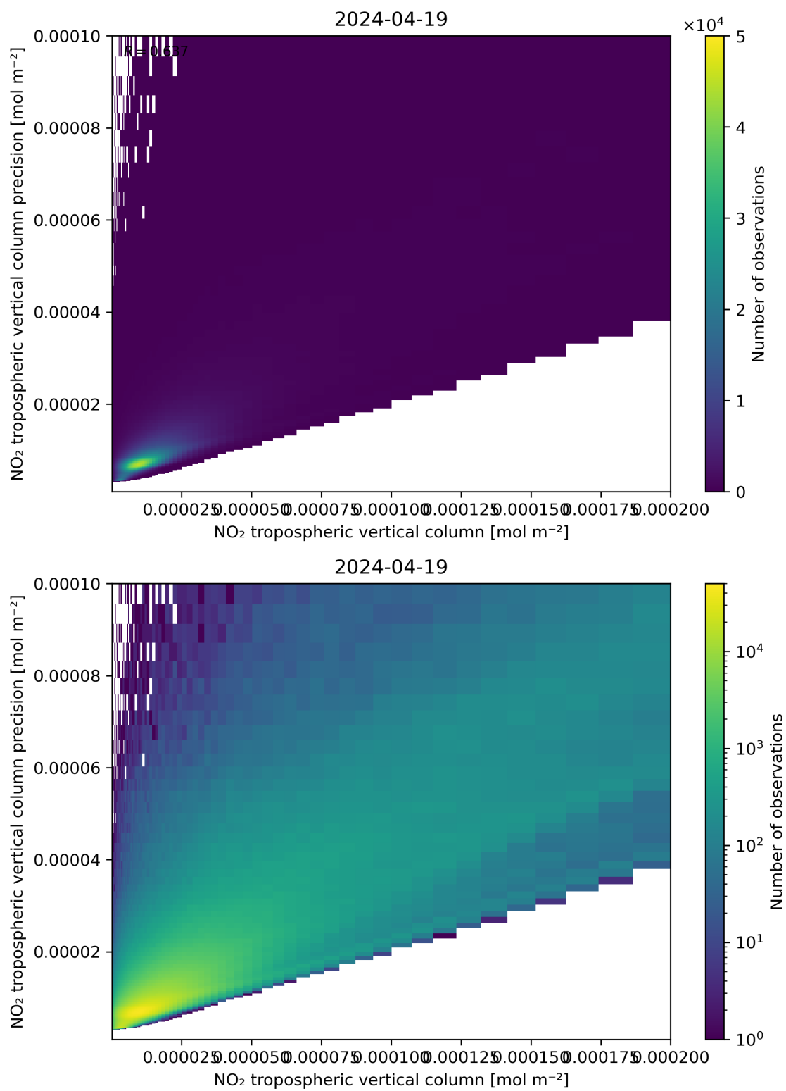
Figure 130: Scatter density plot of “NO 2 tropospheric vertical column” against “NO 2 tropospheric vertical column precision” for 2024-04-18 to 2024-04-20.
