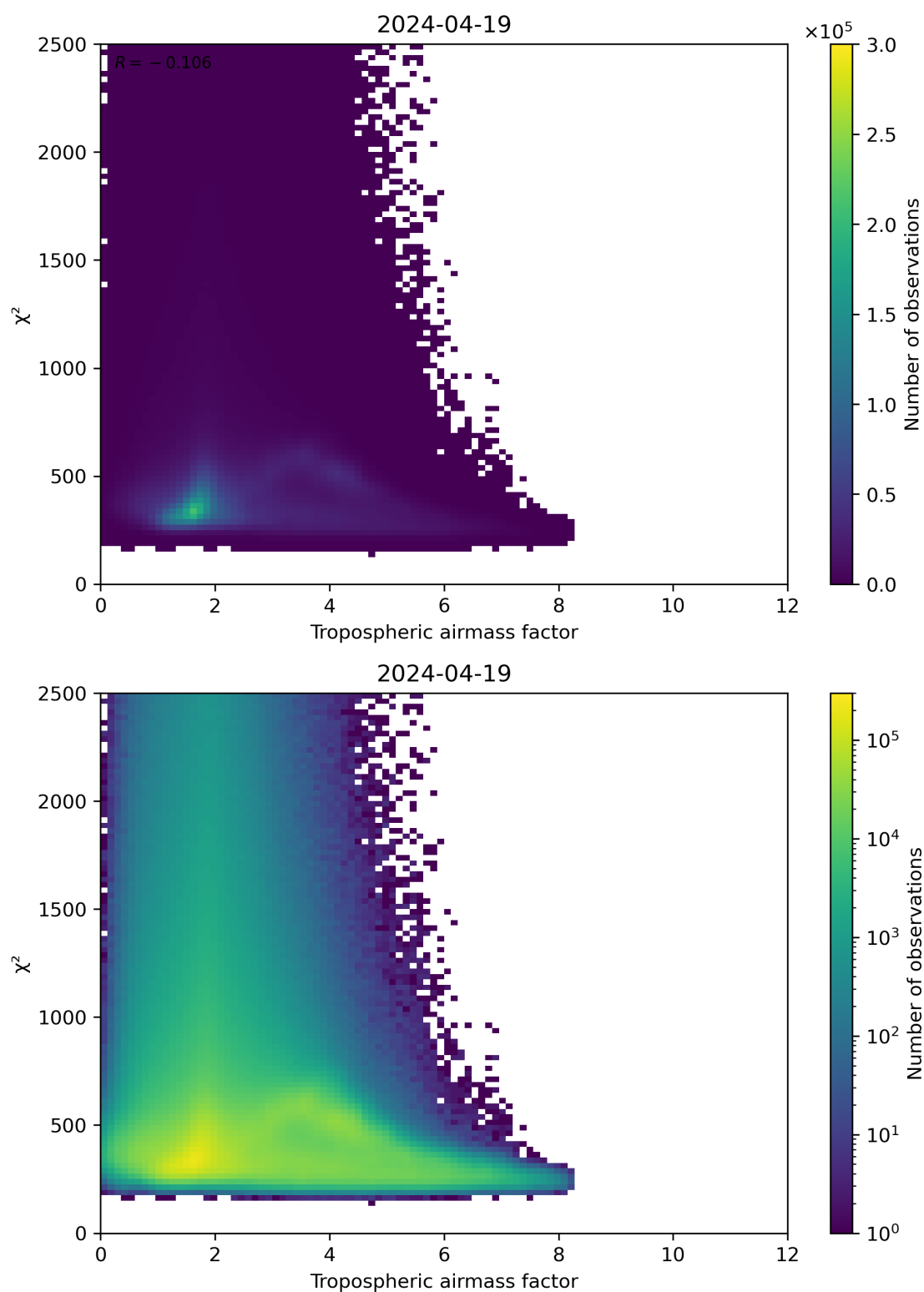
Figure 73: Scatter density plot of “Tropospheric airmass factor” against “ \chi^2 ” for 2024-04-18 to 2024-04-20.
