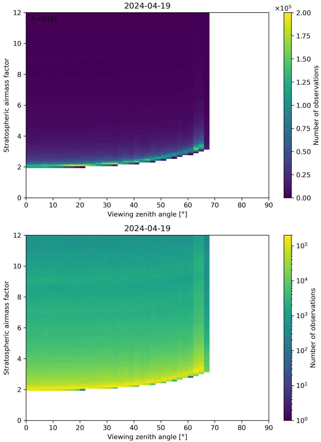
Figure 159: Scatter density plot of “Viewing zenith angle” against “Stratospheric airmass factor” for 2024-04-18 to 2024-04-20.
