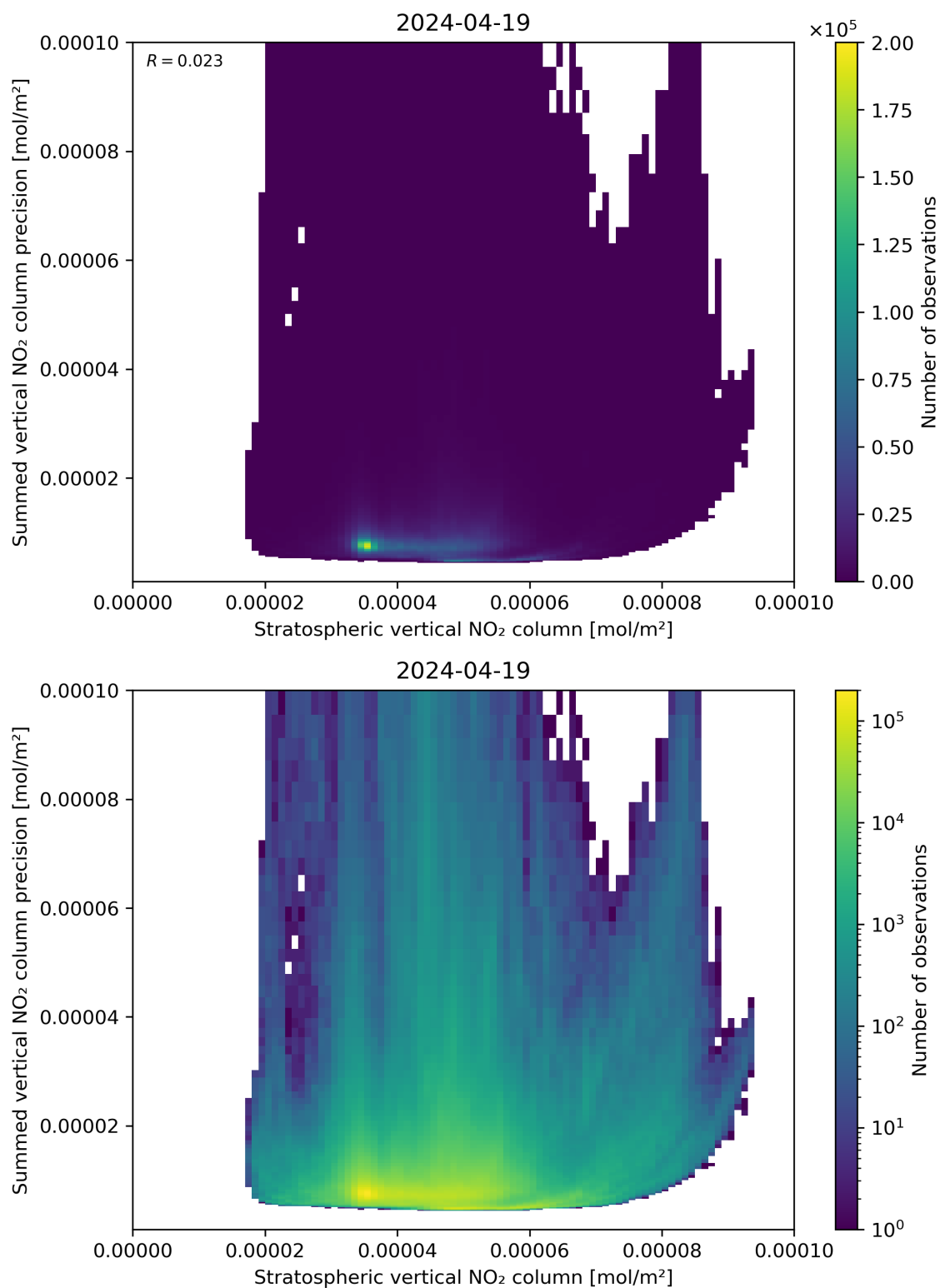
Figure 99: Scatter density plot of “Stratospheric vertical NO 2 column” against “Summed vertical NO 2 column precision” for 2024-04-18 to 2024-04-20.
