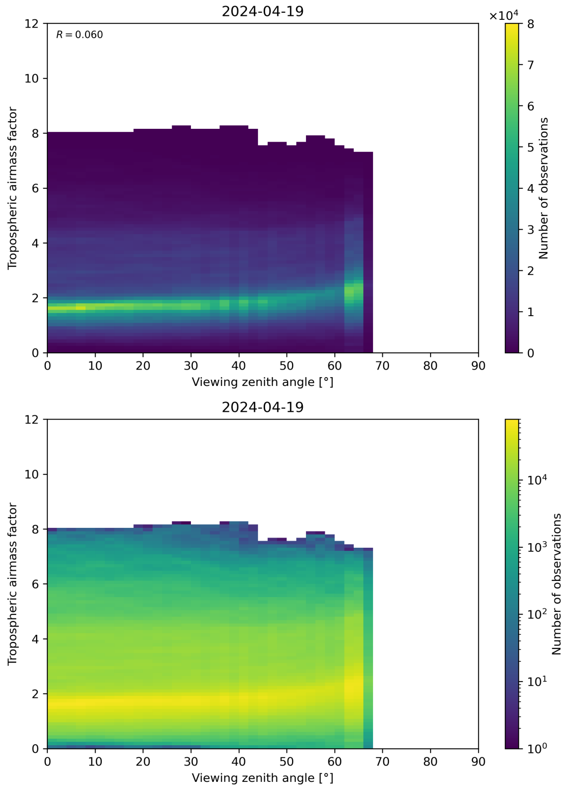
Figure 161: Scatter density plot of “Viewing zenith angle” against “Tropospheric airmass factor” for 2024-04-18 to 2024-04-20.
