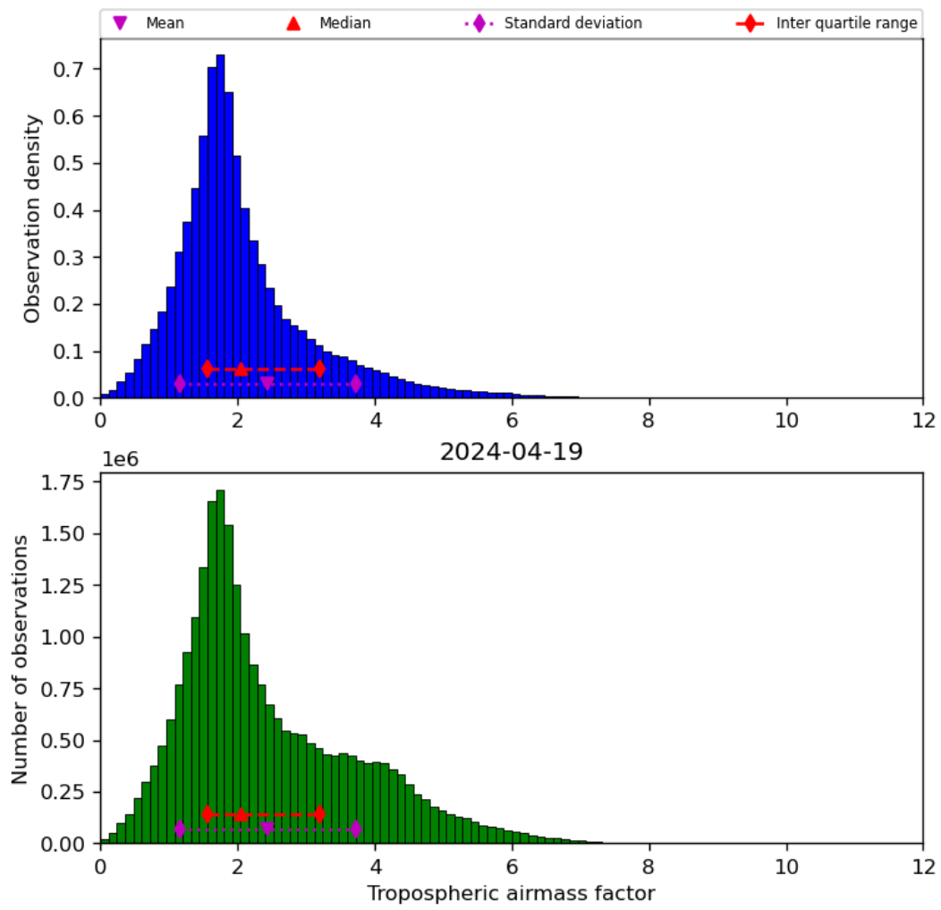
Figure 31: Histogram of “Tropospheric airmass factor” for 2024-04-18 to 2024-04-20
