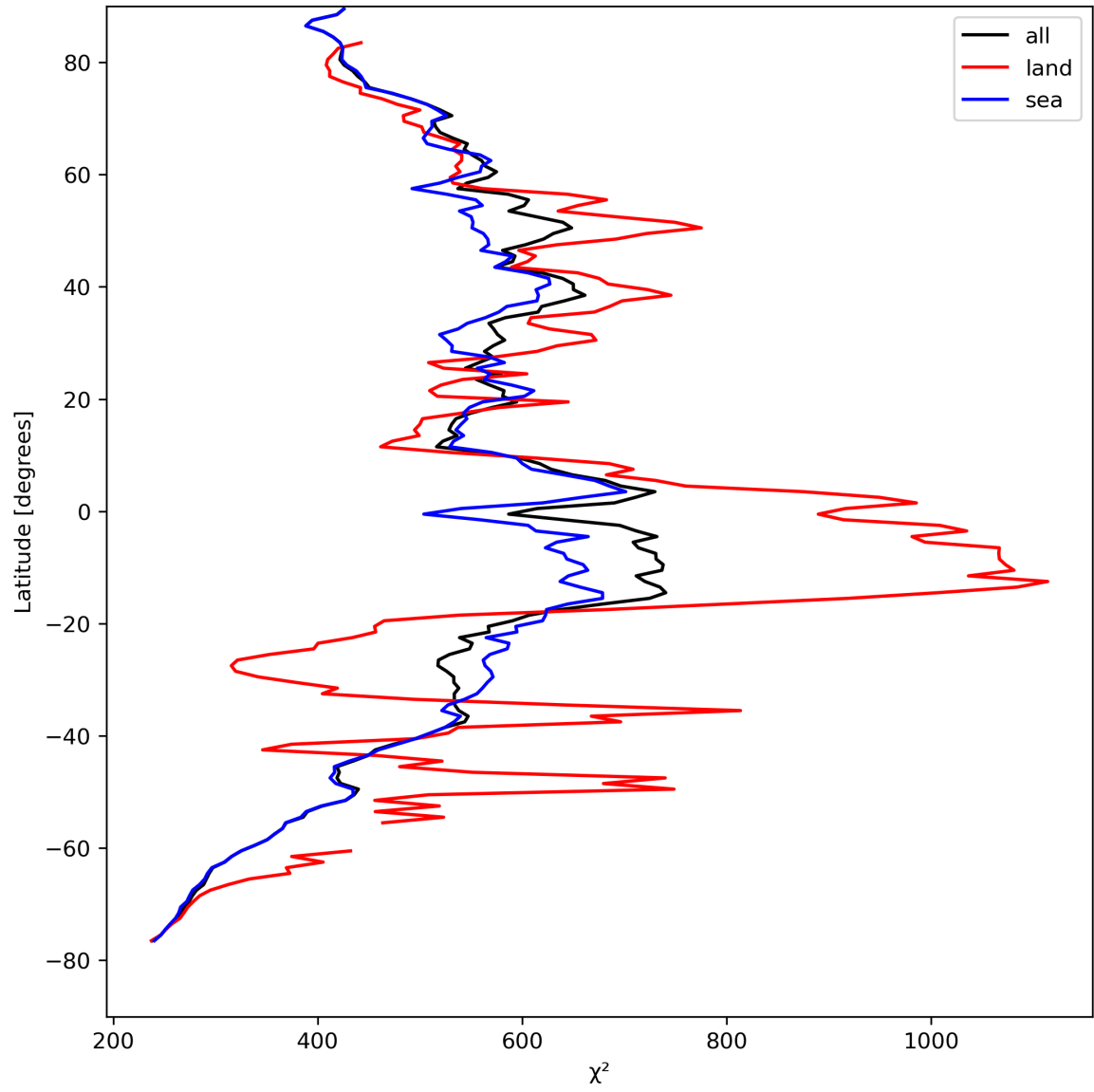
Figure 25: Zonal average of “ \chi^2 ” for 2024-04-18 to 2024-04-20.
