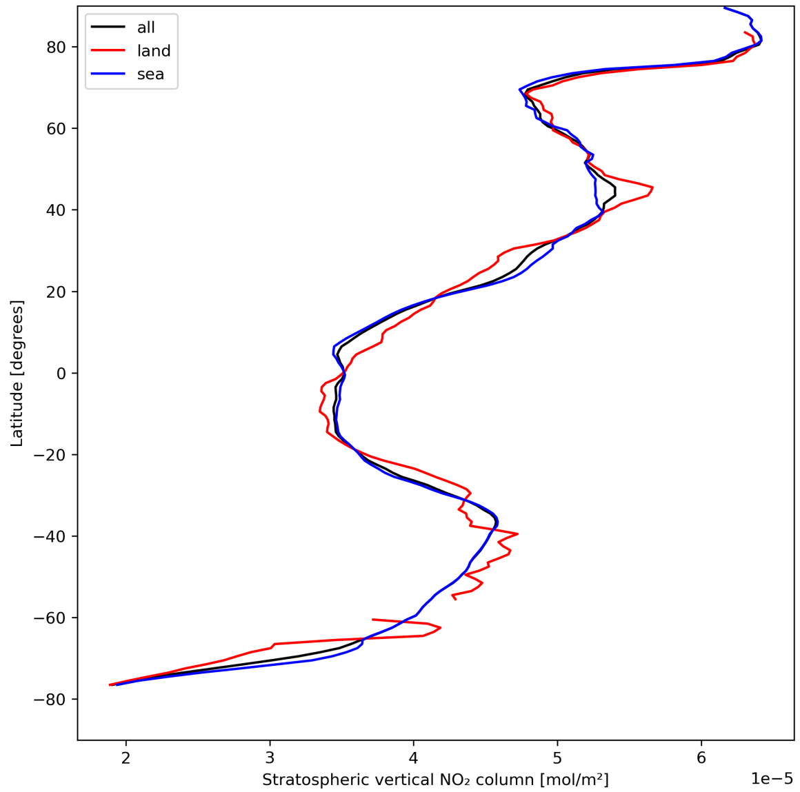
Figure 19: Zonal average of “Stratospheric vertical NO 2 column” for 2024-04-18 to 2024-04-20.
