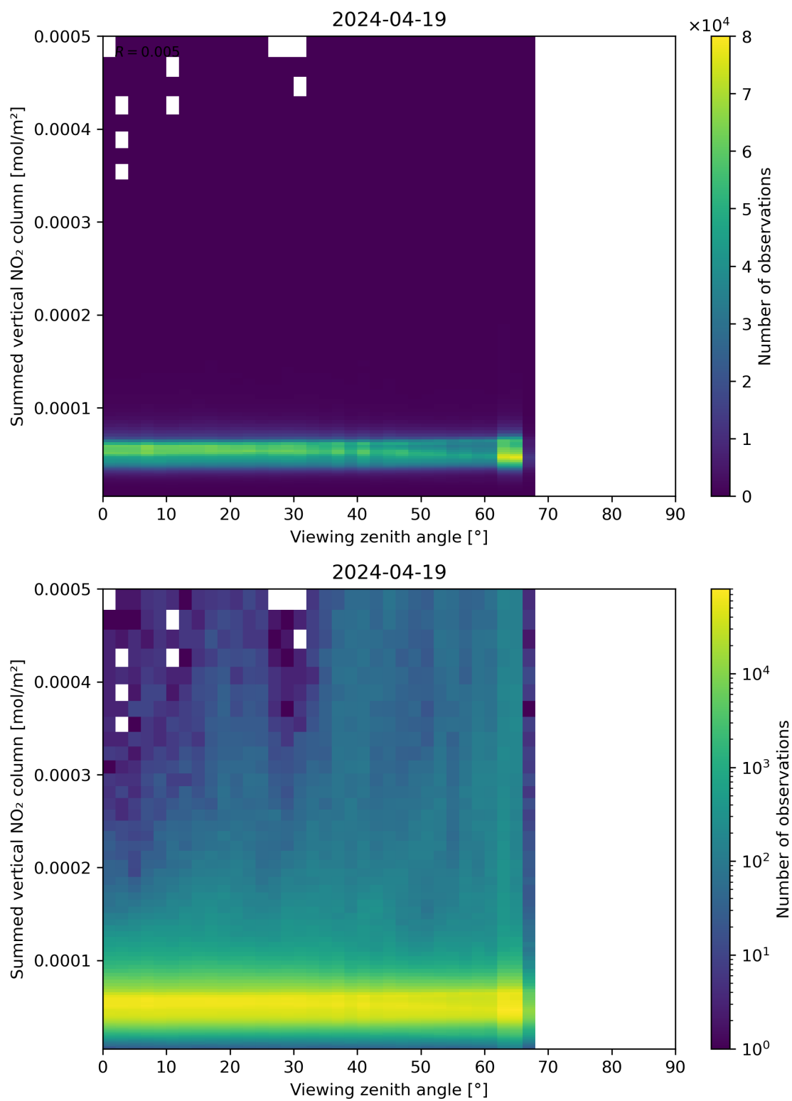
Figure 165: Scatter density plot of “Viewing zenith angle” against “Summed vertical NO 2 column” for 2024-04-18 to 2024-04-20.
