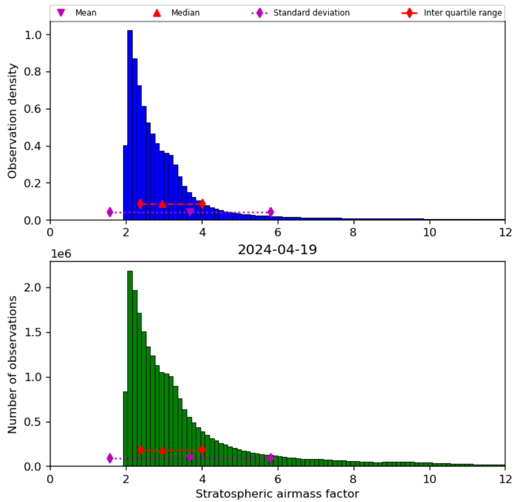
Figure 44: Histogram of “Stratospheric airmass factor” for 2024-04-18 to 2024-04-20
