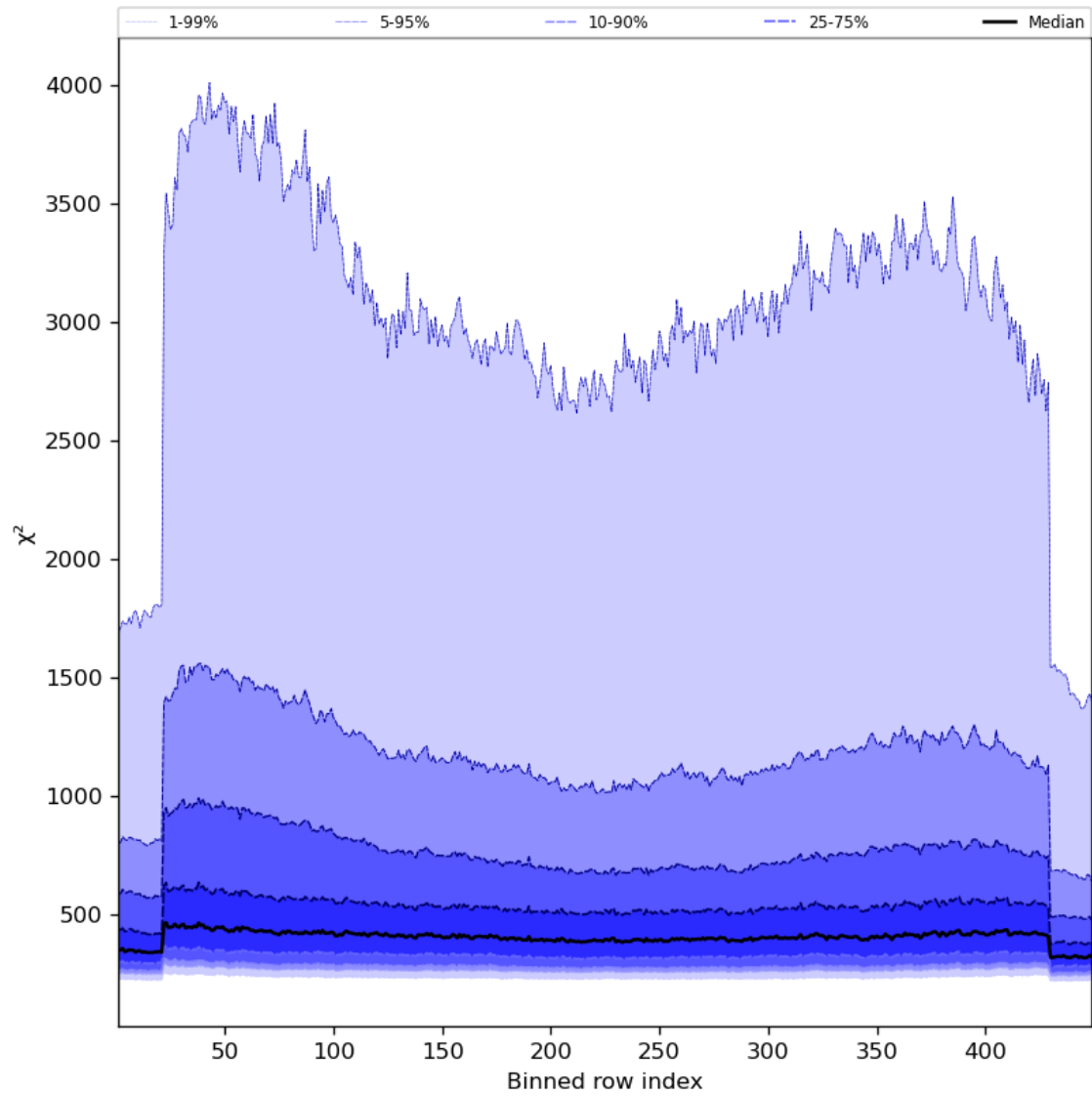
Figure 59: Along track statistics of “ \chi^2 ” for 2024-04-18 to 2024-04-20
