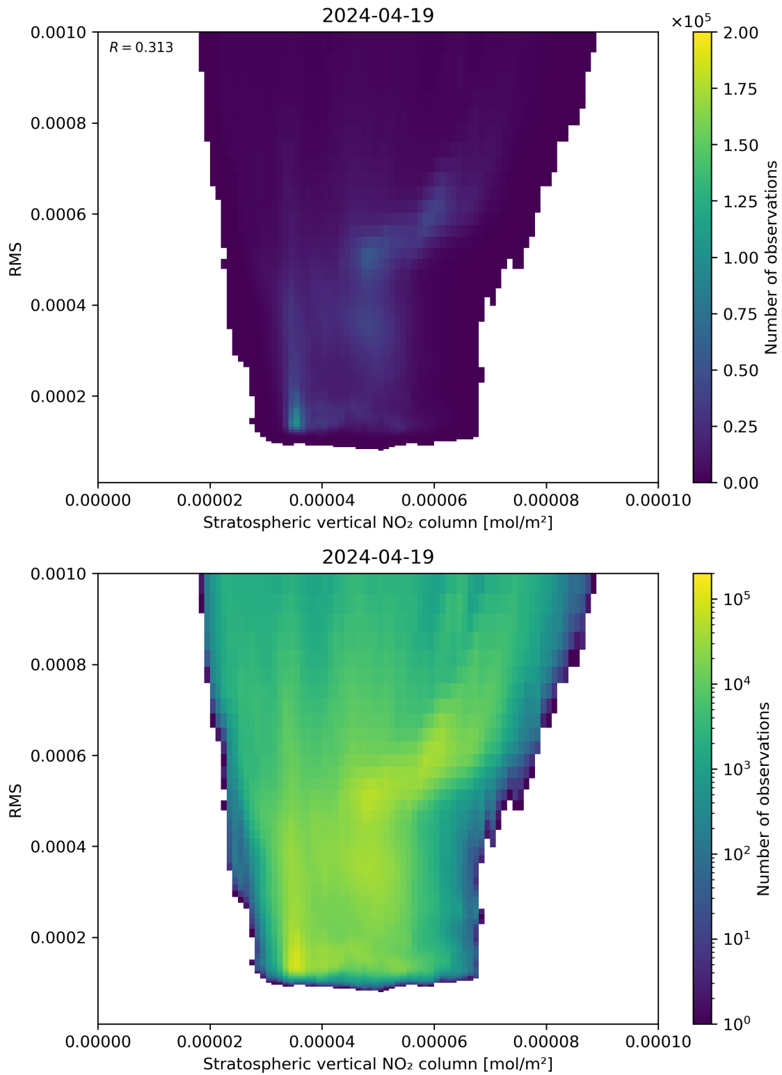
Figure 102: Scatter density plot of “Stratospheric vertical NO 2 column” against “RMS” for 2024-04-18 to 2024-04-20.
