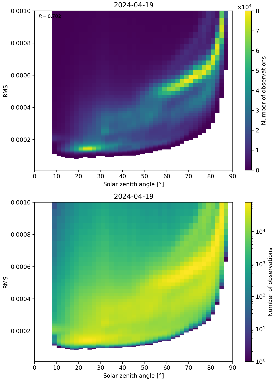
Figure 157: Scatter density plot of “Solar zenith angle” against “RMS” for 2024-04-18 to 2024-04-20.
