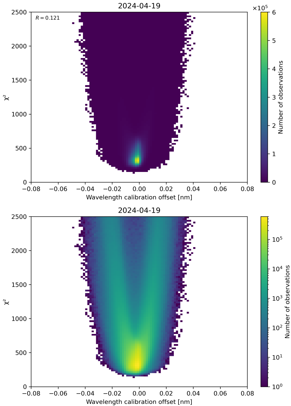
Figure 175: Scatter density plot of “Wavelength calibration offset” against “ \chi^2 ” for 2024-04-18 to 2024-04-20.
