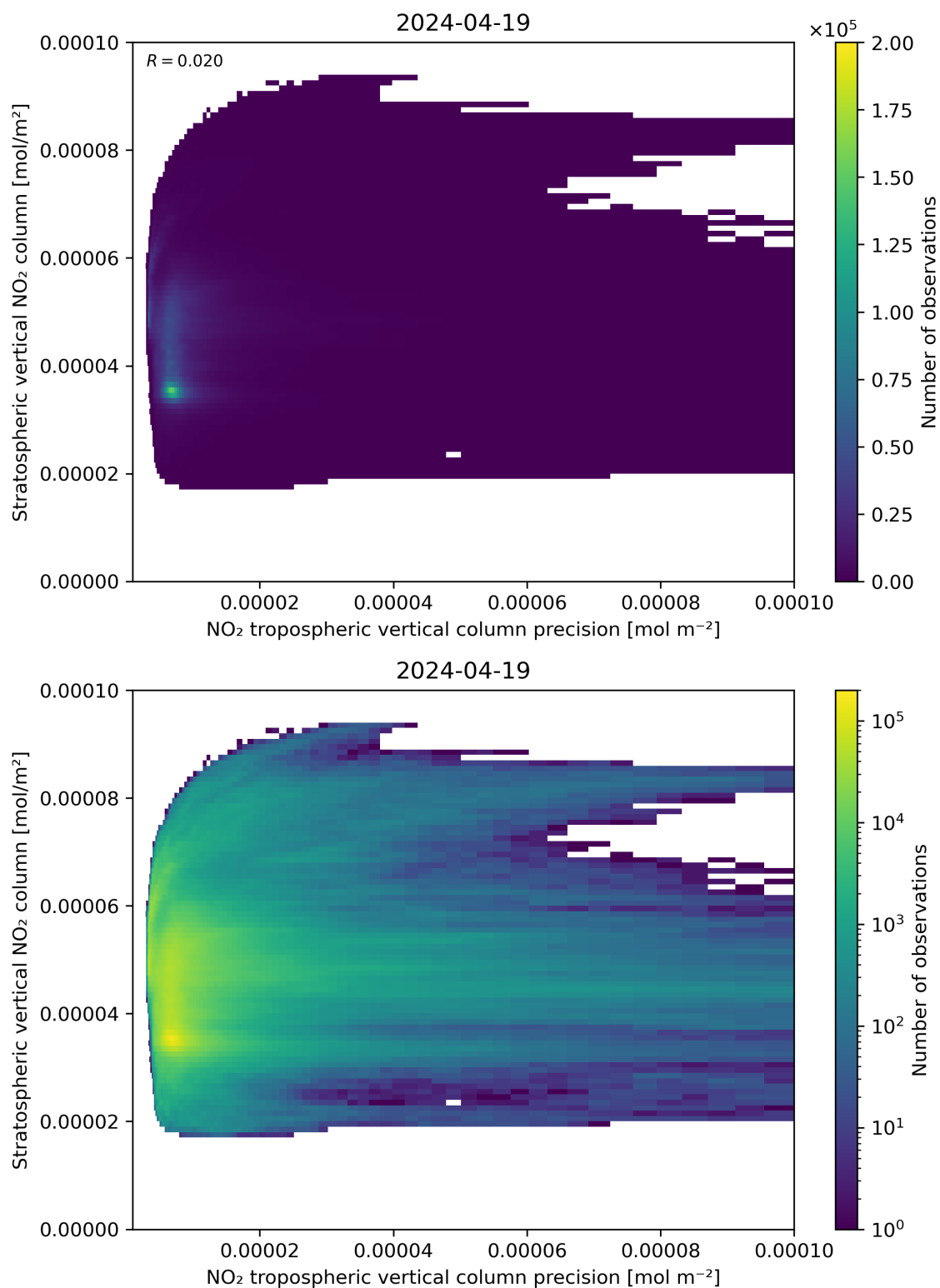
Figure 135: Scatter density plot of “NO 2 tropospheric vertical column precision” against “Stratospheric vertical NO 2 column” for 2024-04-18 to 2024-04-20.
