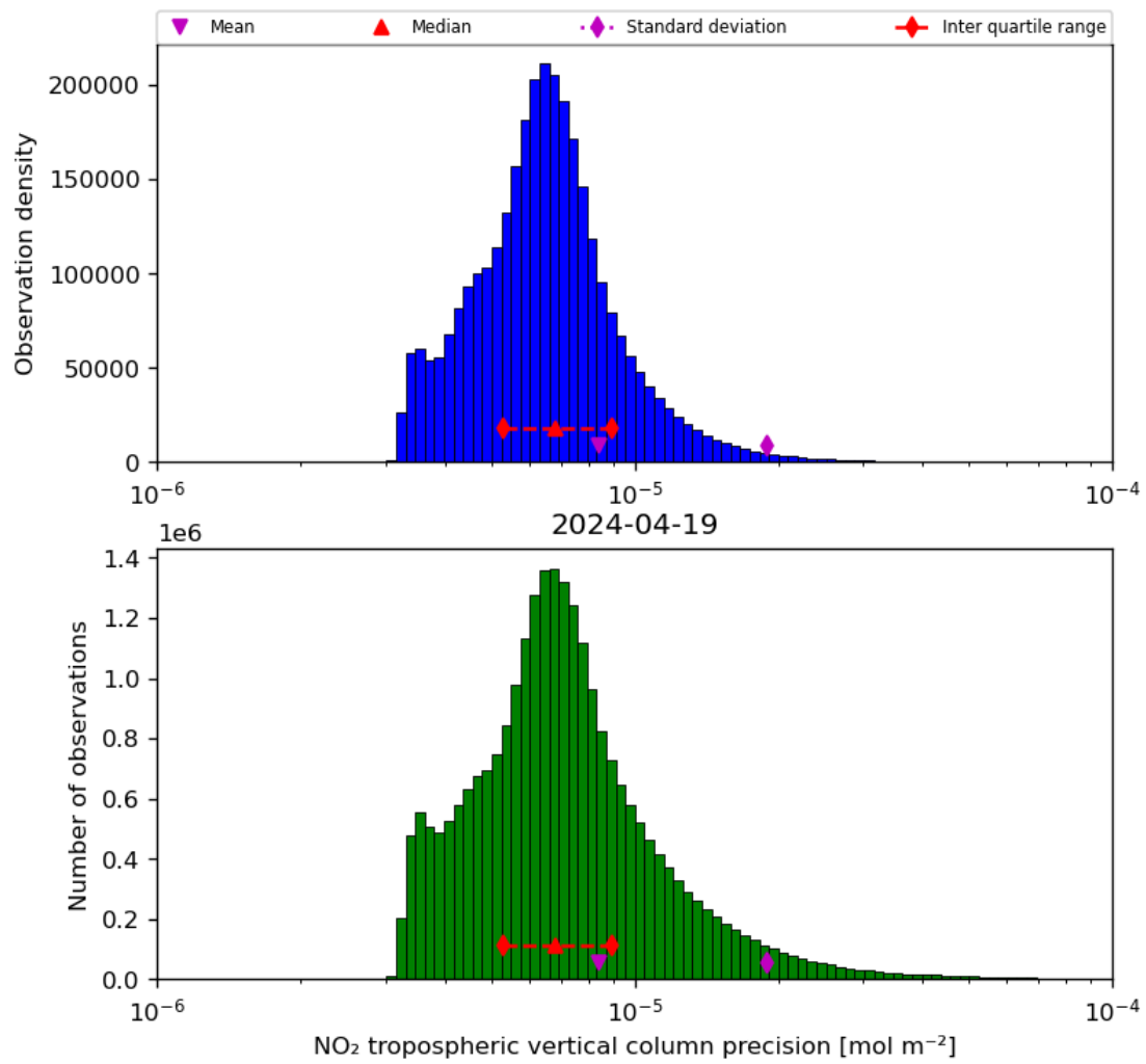
Figure 30: Histogram of “NO 2 tropospheric vertical column precision” for 2024-04-18 to 2024-04-20
