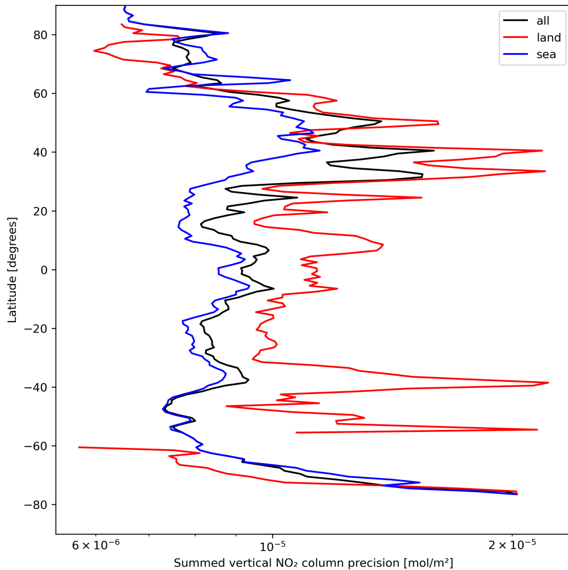
Figure 24: Zonal average of “Summed vertical NO 2 column precision” for 2024-04-18 to 2024-04-20.
