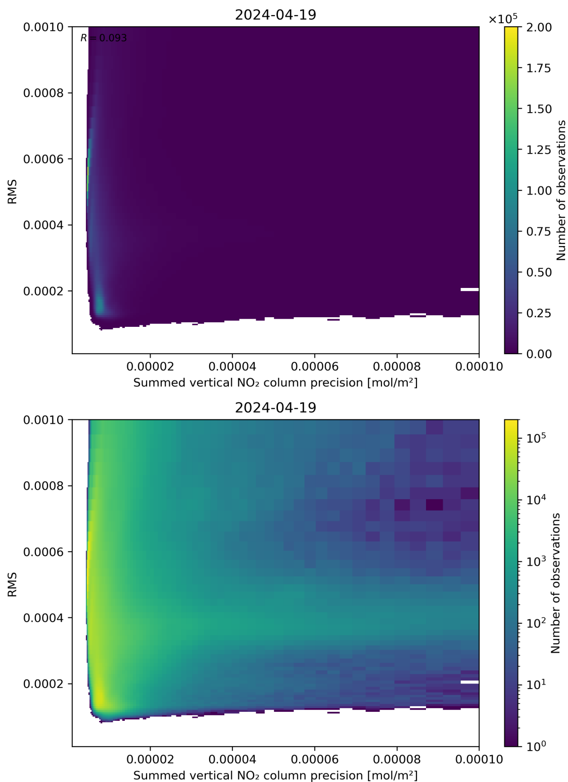
Figure 108: Scatter density plot of “Summed vertical NO 2 column precision” against “RMS” for 2024-04-18 to 2024-04-20.
