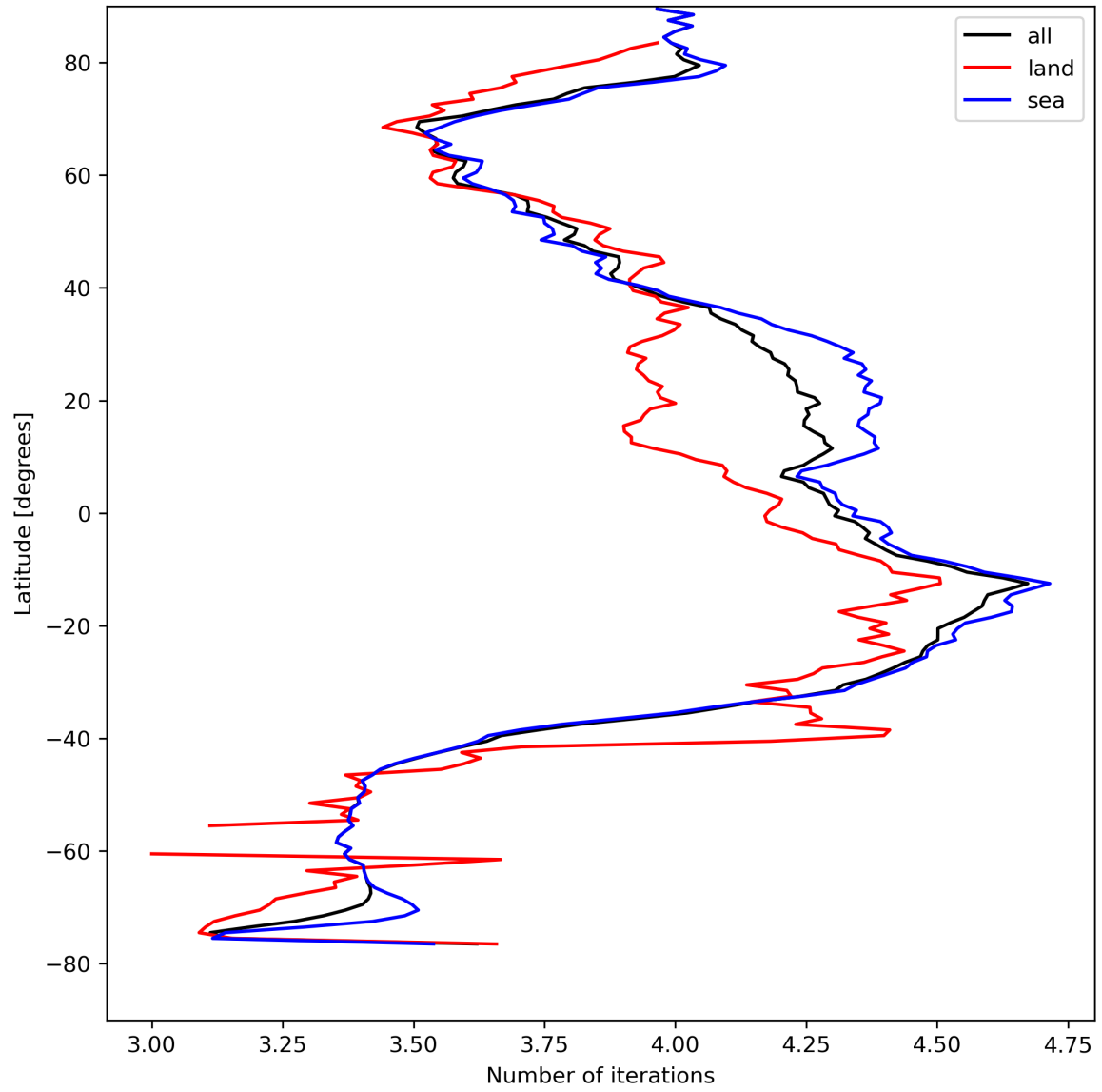
Figure 17: Zonal average of “Number of iterations” for 2024-04-18 to 2024-04-20.
