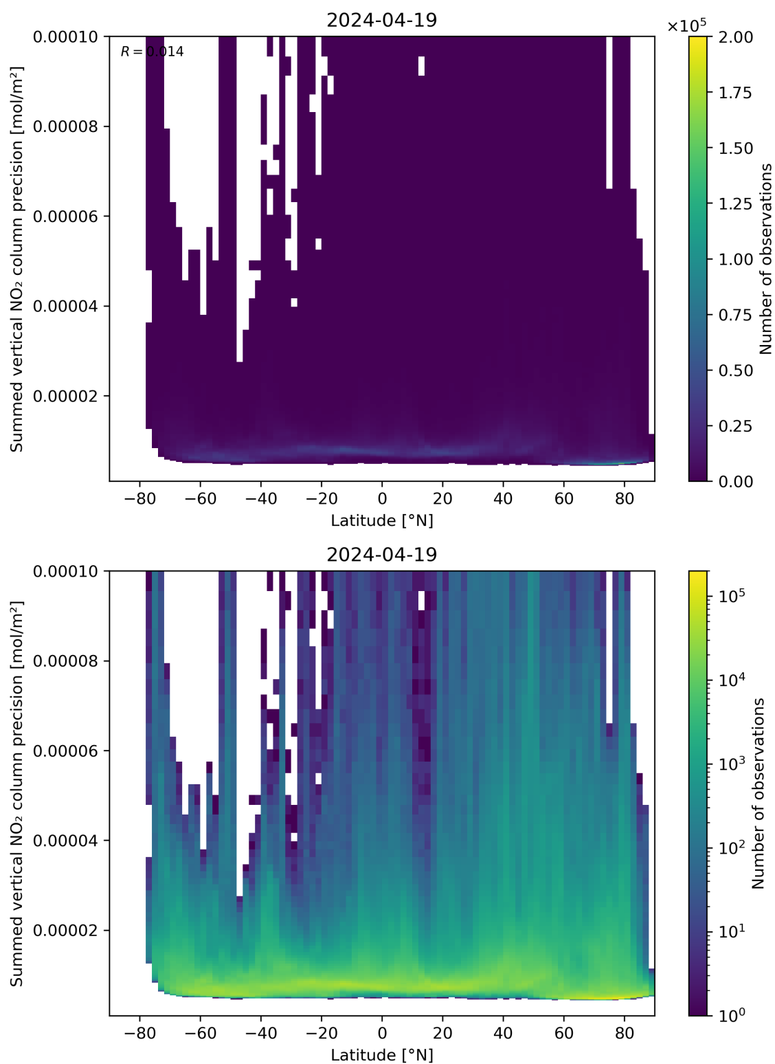
Figure 89: Scatter density plot of “Latitude” against “Summed vertical NO 2 column precision” for 2024-04-18 to 2024-04-20.
