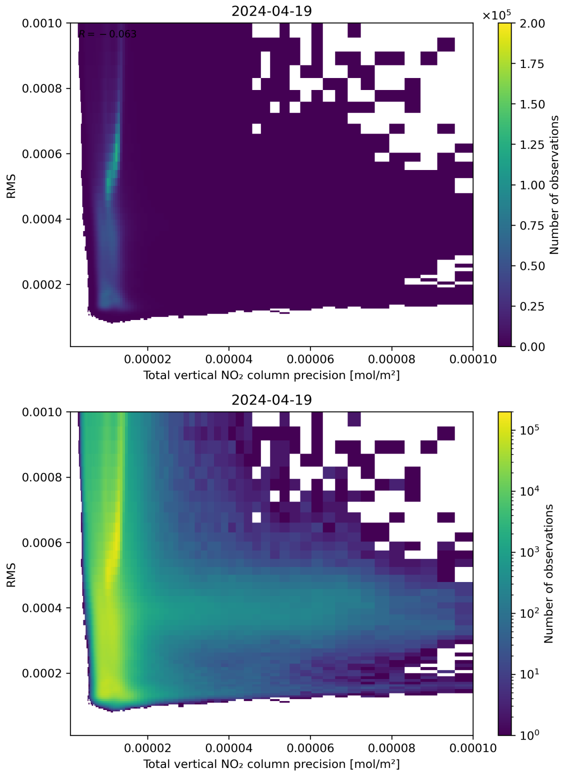
Figure 119: Scatter density plot of “Total vertical NO 2 column precision” against “RMS” for 2024-04-18 to 2024-04-20.
