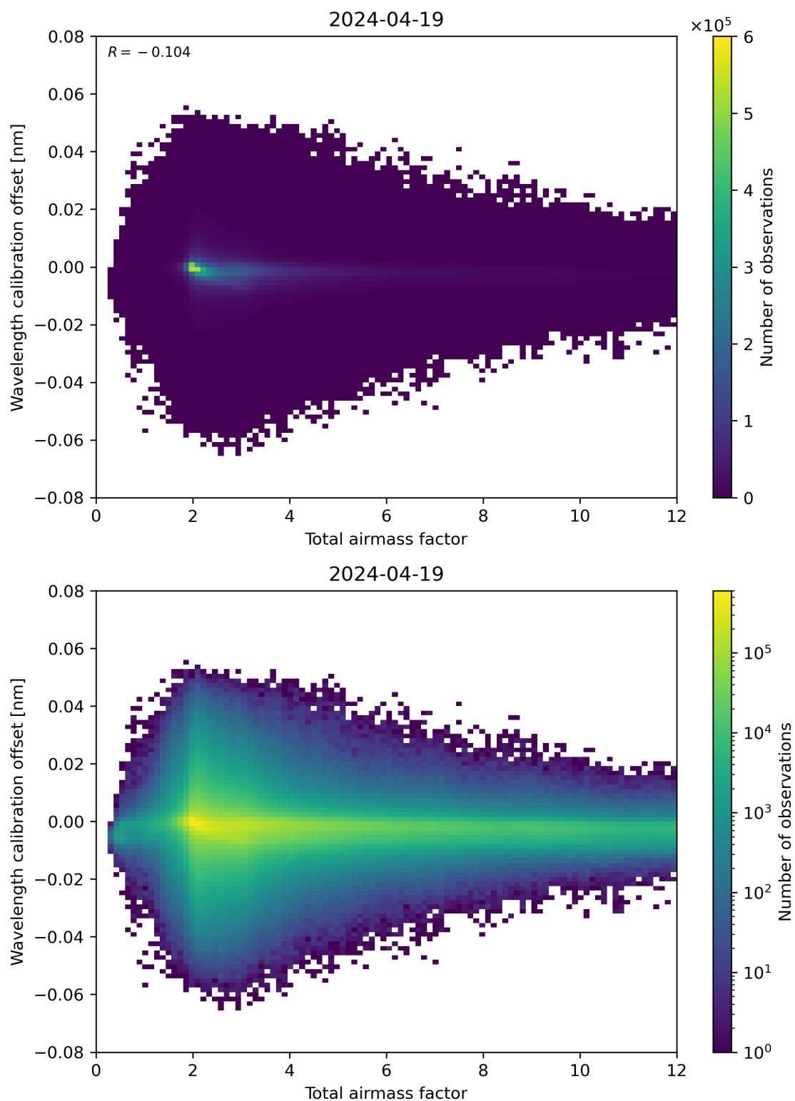
Figure 70: Scatter density plot of “Total airmass factor” against “Wavelength calibration offset” for 2024-04-18 to 2024-04-20.
