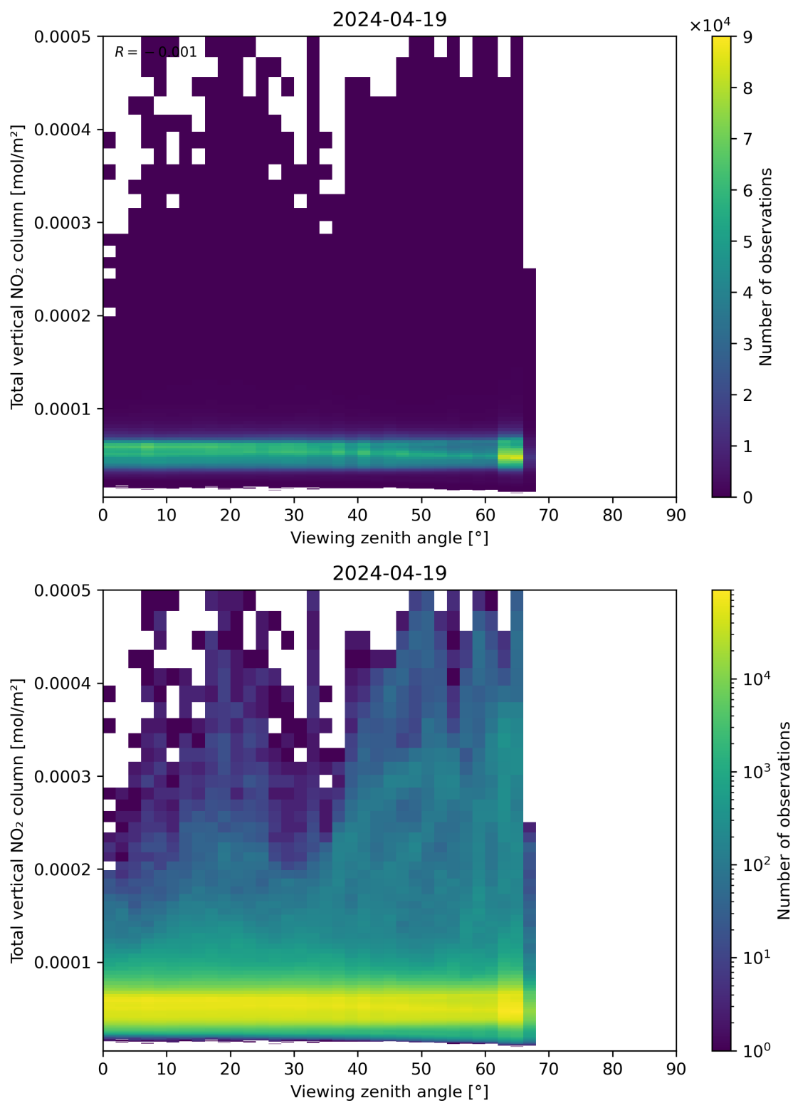
Figure 167: Scatter density plot of “Viewing zenith angle” against “Total vertical NO 2 column” for 2024-04-18 to 2024-04-20.
