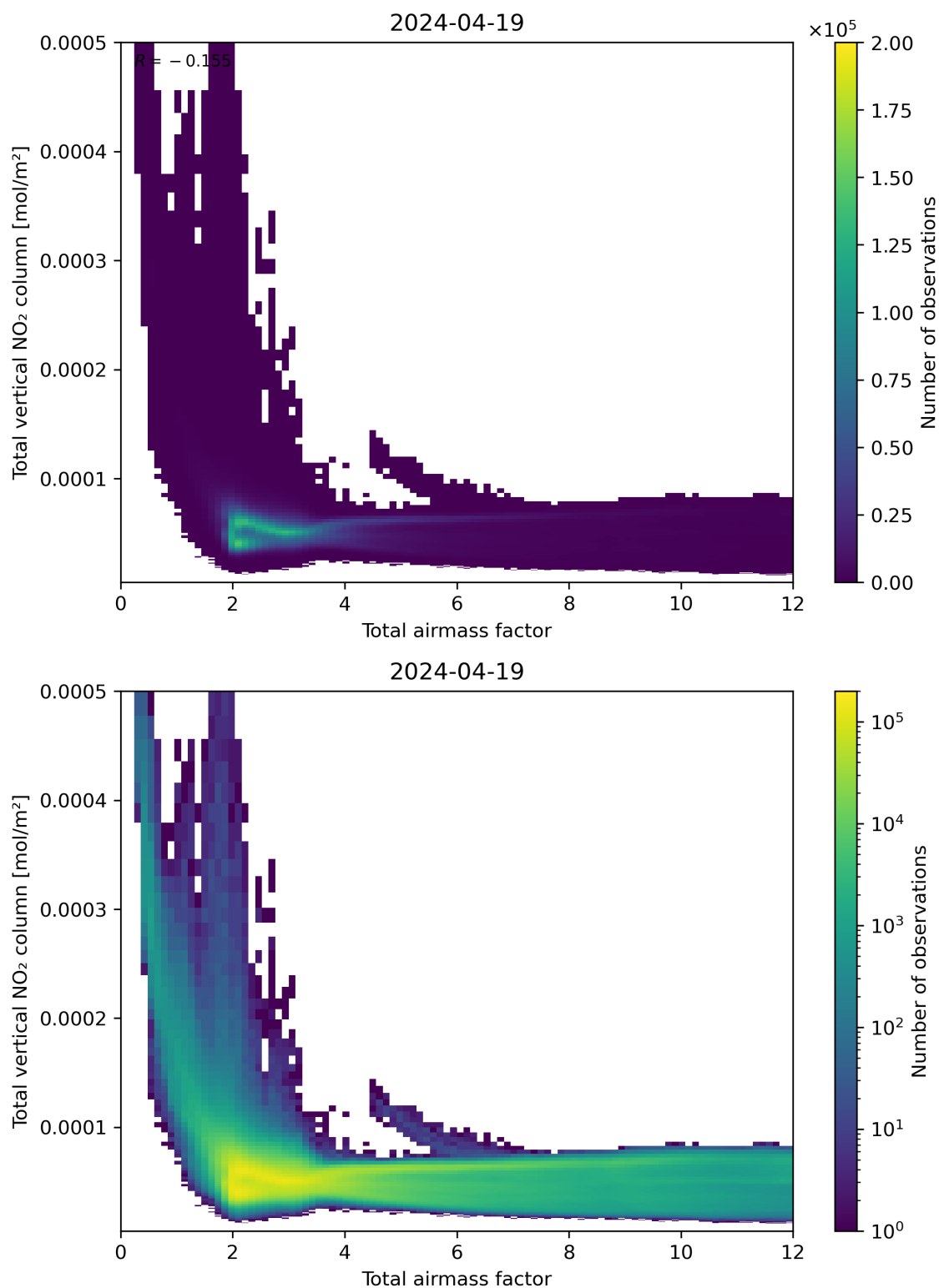
Figure 67: Scatter density plot of “Total airmass factor” against “Total vertical NO 2 column” for 2024-04-18 to 2024-04-20.
