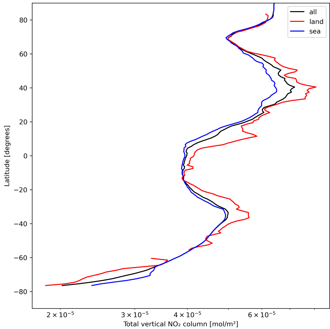
Figure 21: Zonal average of “Total vertical NO 2 column” for 2024-04-18 to 2024-04-20.
