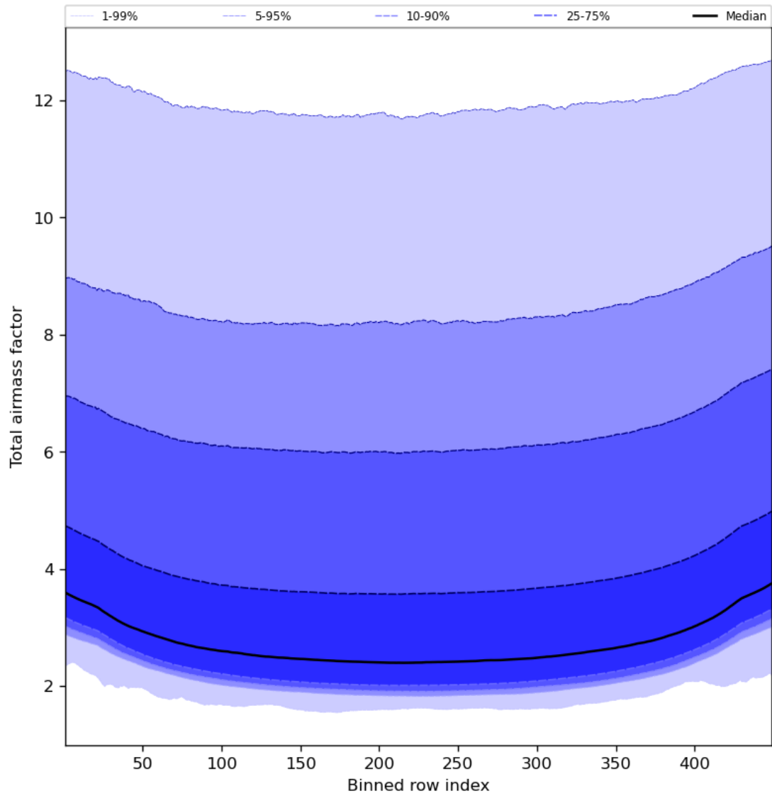
Figure 49: Along track statistics of “Total airmass factor” for 2024-04-18 to 2024-04-20
