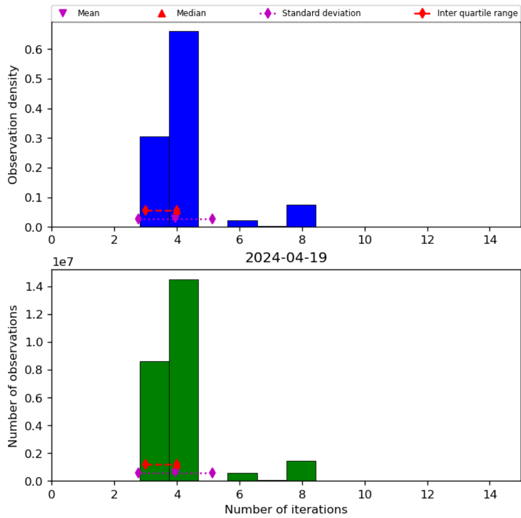
Figure 34: Histogram of “Number of iterations” for 2024-04-18 to 2024-04-20
