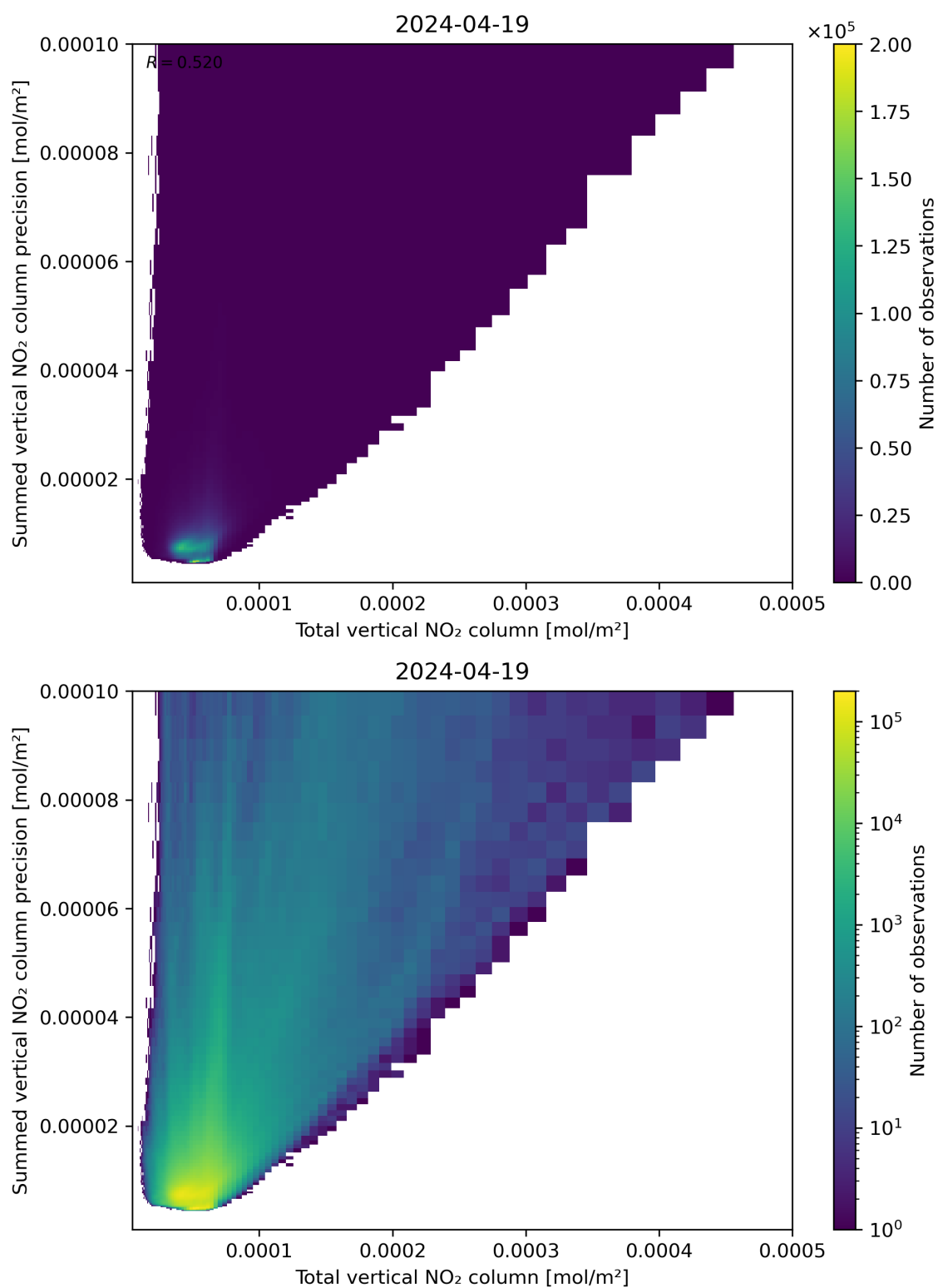
Figure 113: Scatter density plot of “Total vertical NO 2 column” against “Summed vertical NO 2 column precision” for 2024-04-18 to 2024-04-20.
