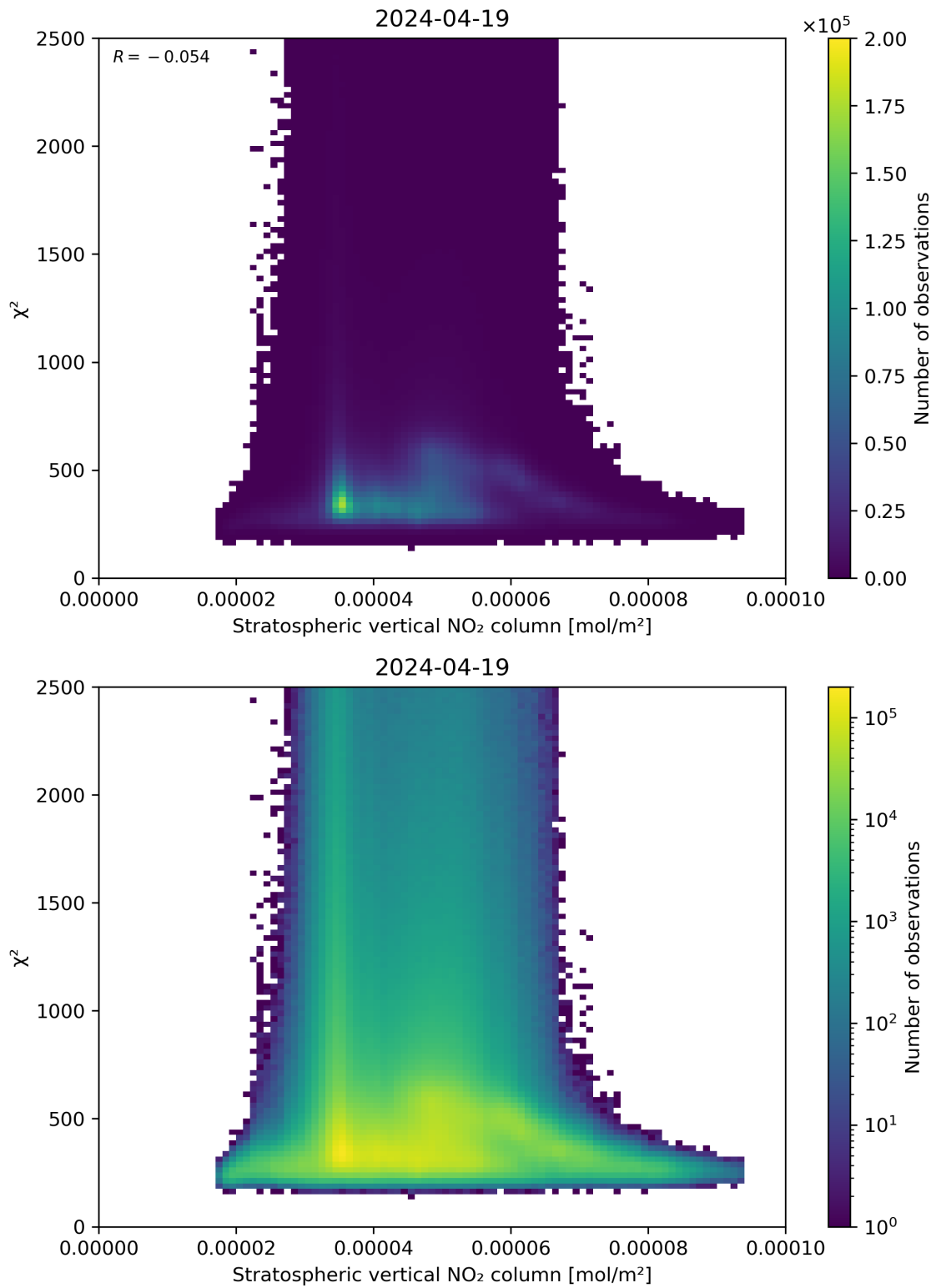
Figure 97: Scatter density plot of “Stratospheric vertical NO 2 column” against “ \chi^2 ” for 2024-04-18 to 2024-04-20.
