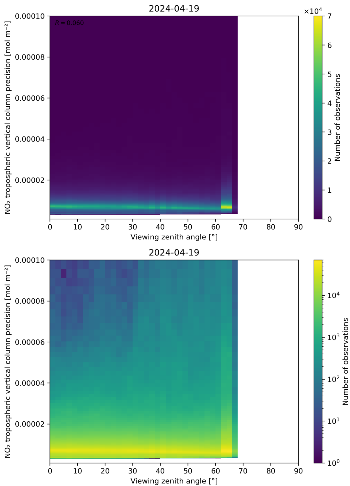
Figure 170: Scatter density plot of “Viewing zenith angle” against “NO 2 tropospheric vertical column precision” for 2024-04-18 to 2024-04-20.
