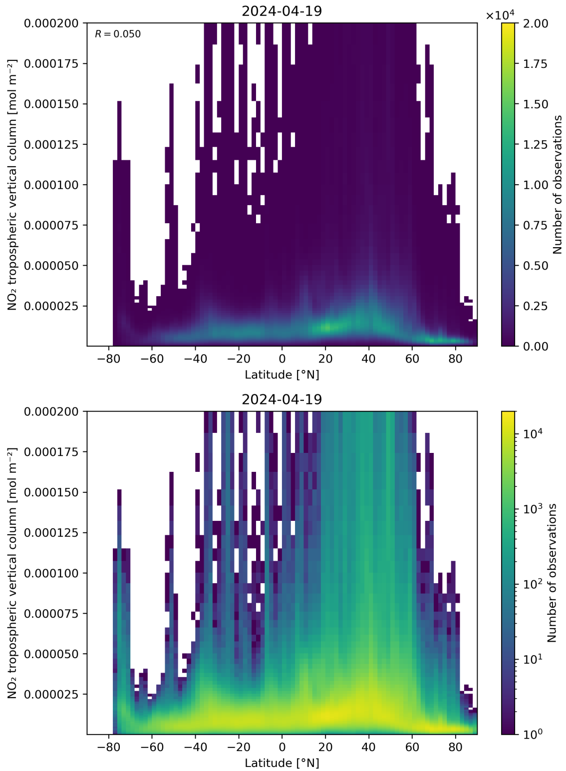
Figure 92: Scatter density plot of “Latitude” against “NO 2 tropospheric vertical column” for 2024-04-18 to 2024-04-20.
