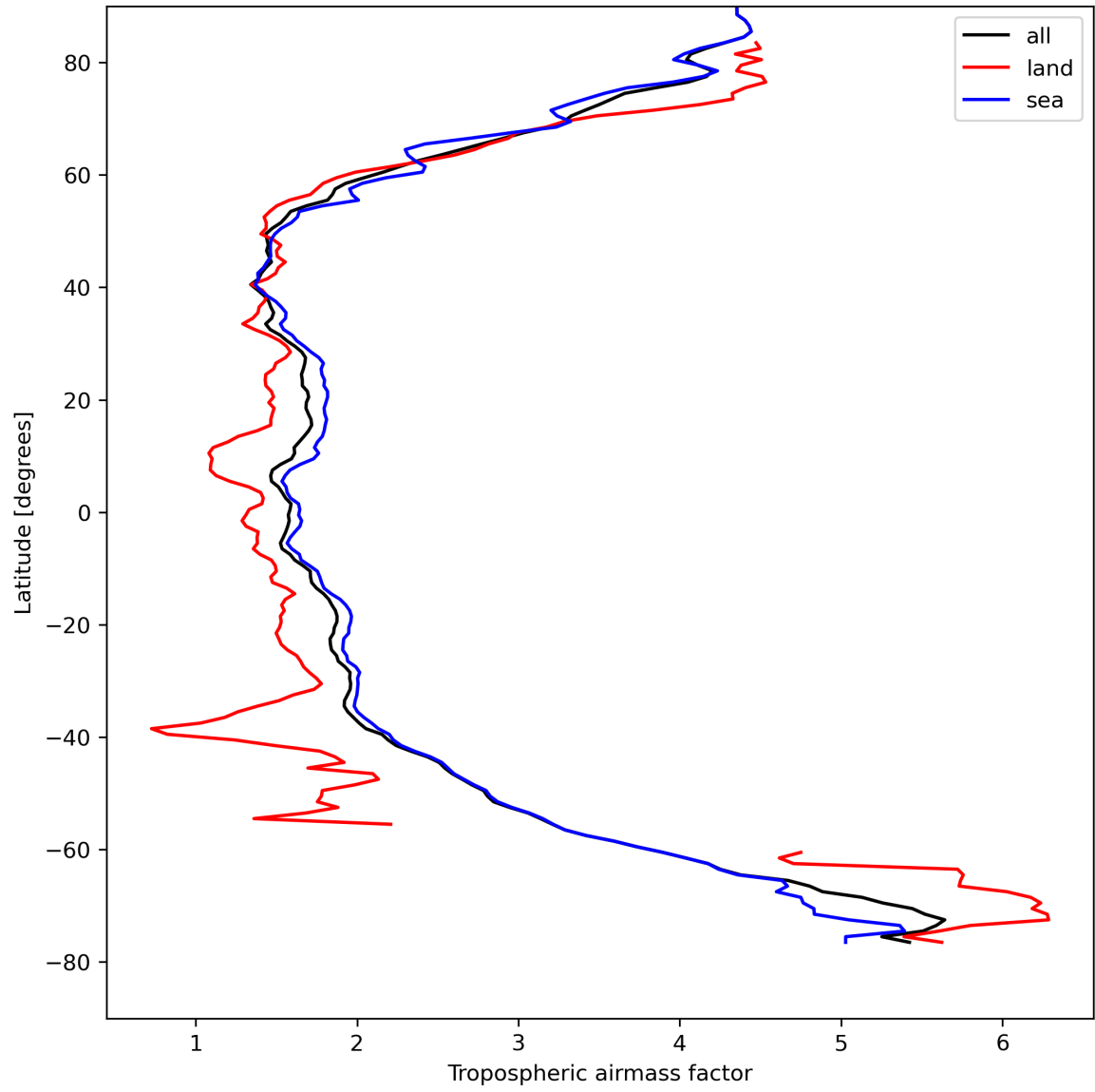
Figure 14: Zonal average of “Tropospheric airmass factor” for 2024-04-18 to 2024-04-20.
