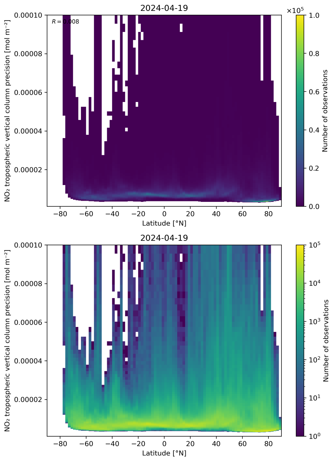
Figure 93: Scatter density plot of “Latitude” against “NO 2 tropospheric vertical column precision” for 2024-04-18 to 2024-04-20.
