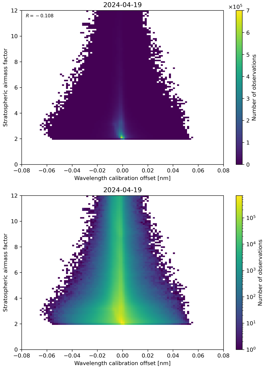
Figure 174: Scatter density plot of “Wavelength calibration offset” against “Stratospheric airmass factor” for 2024-04-18 to 2024-04-20.
