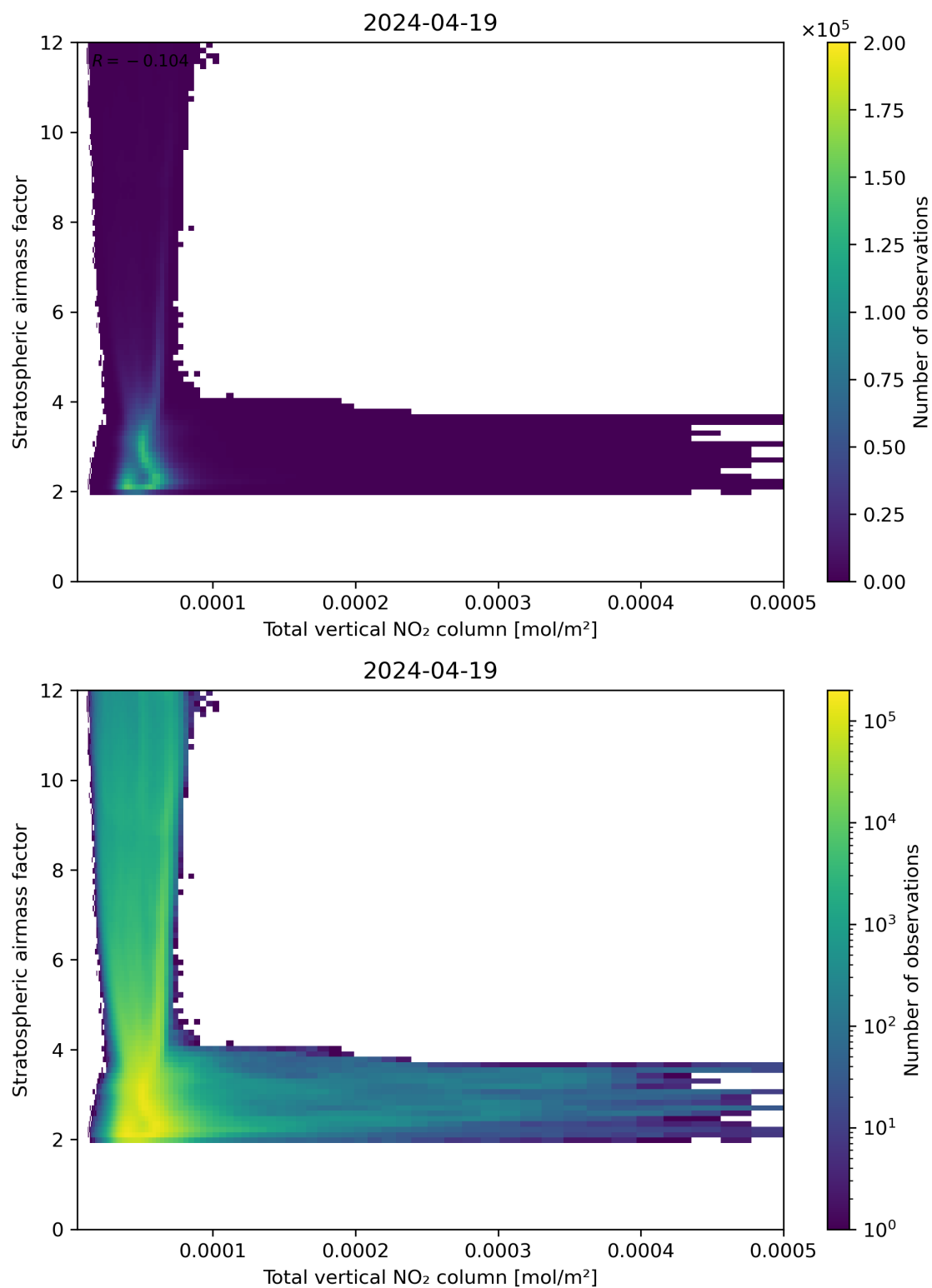
Figure 110: Scatter density plot of “Total vertical NO 2 column” against “Stratospheric air mass factor” for 2024-04-18 to 2024-04-20.
