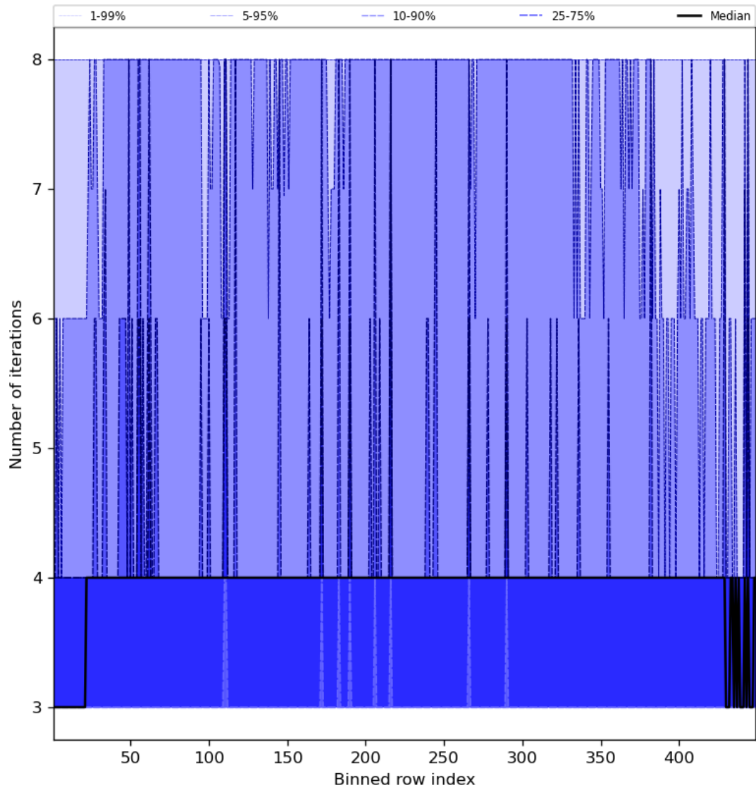
Figure 51: Along track statistics of “Number of iterations” for 2024-04-18 to 2024-04-20
