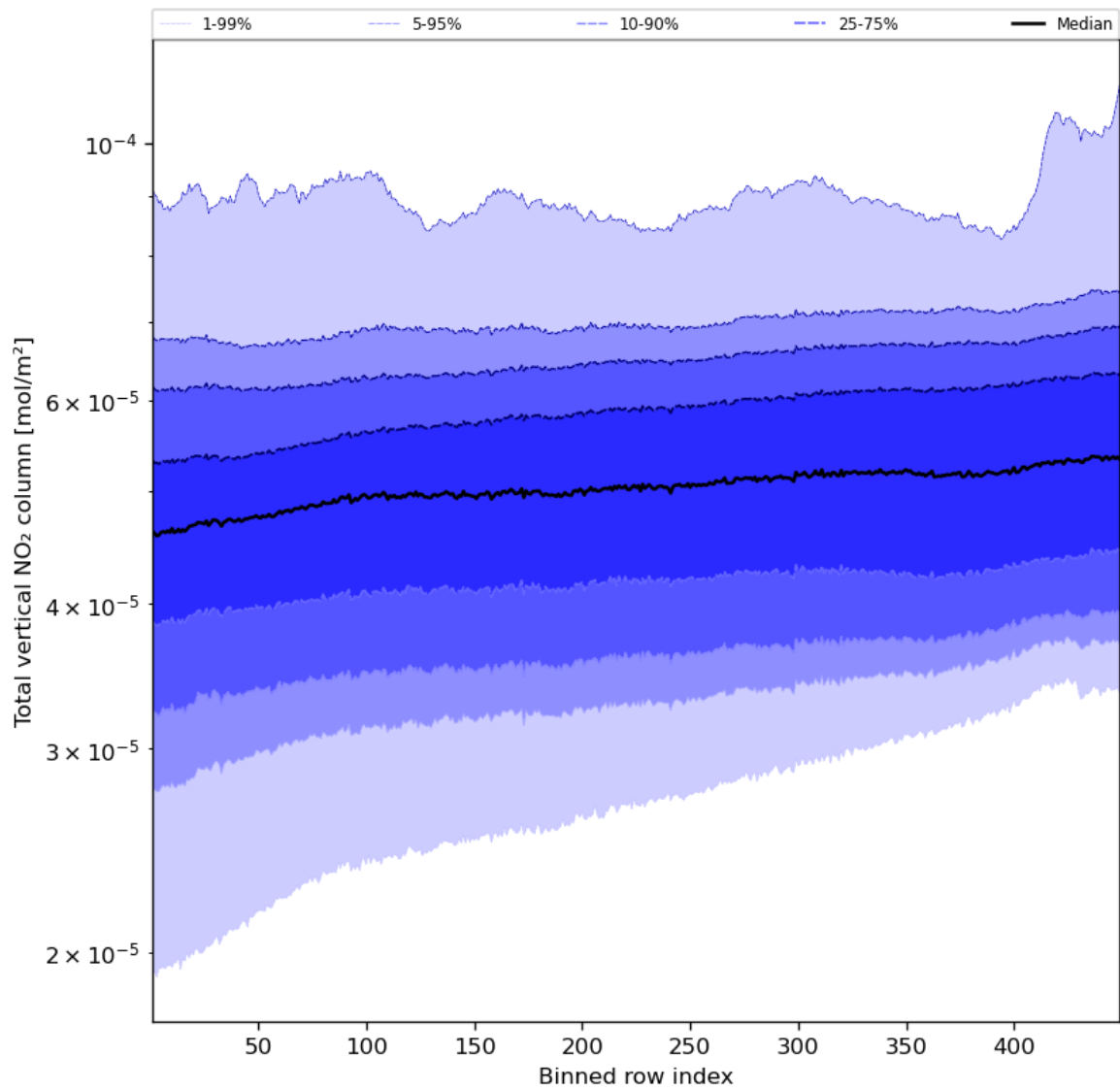
Figure 55: Along track statistics of “Total vertical NO 2 column” for 2024-04-18 to 2024-04-20
