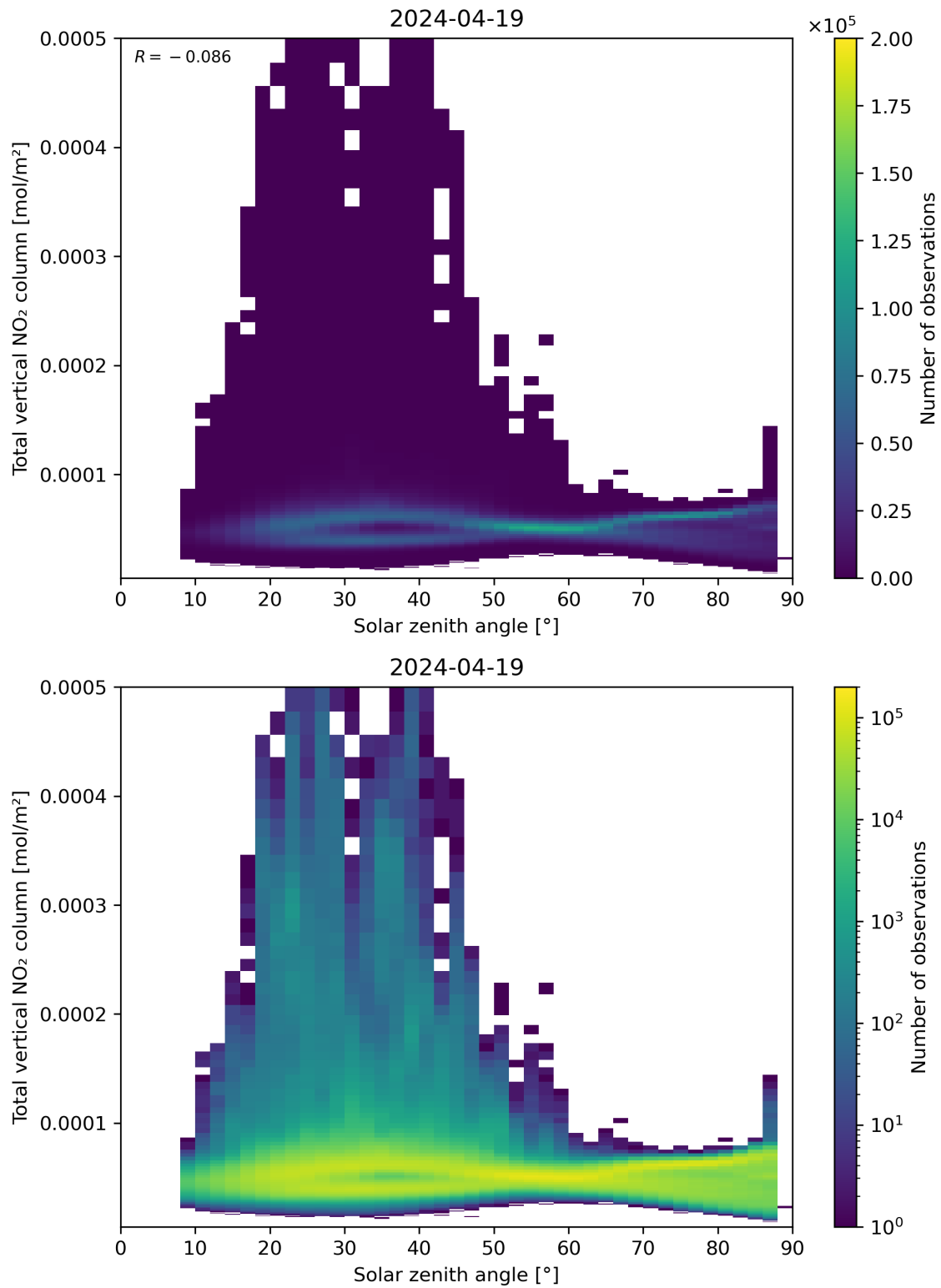
Figure 153: Scatter density plot of “Solar zenith angle” against “Total vertical NO 2 column” for 2024-04-18 to 2024-04-20.
