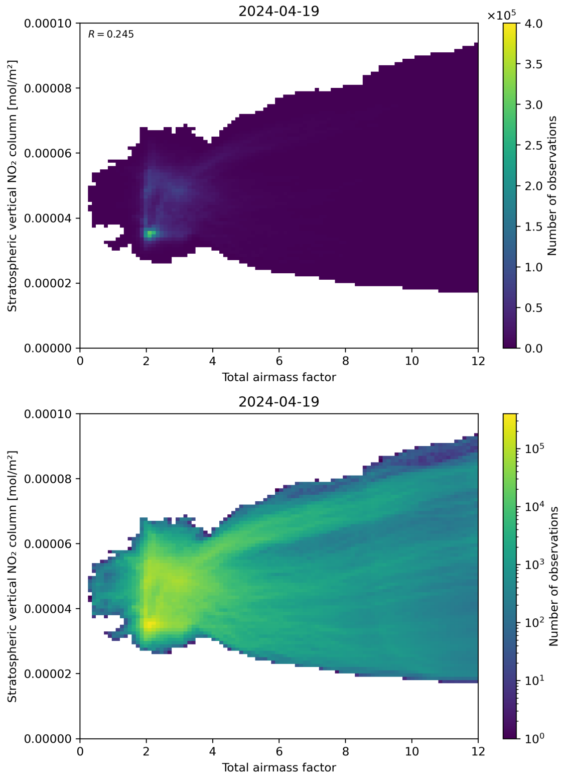
Figure 64: Scatter density plot of “Total airmass factor” against “Stratospheric vertical \text{NO}_2 column” for 2024-04-18 to 2024-04-20.
