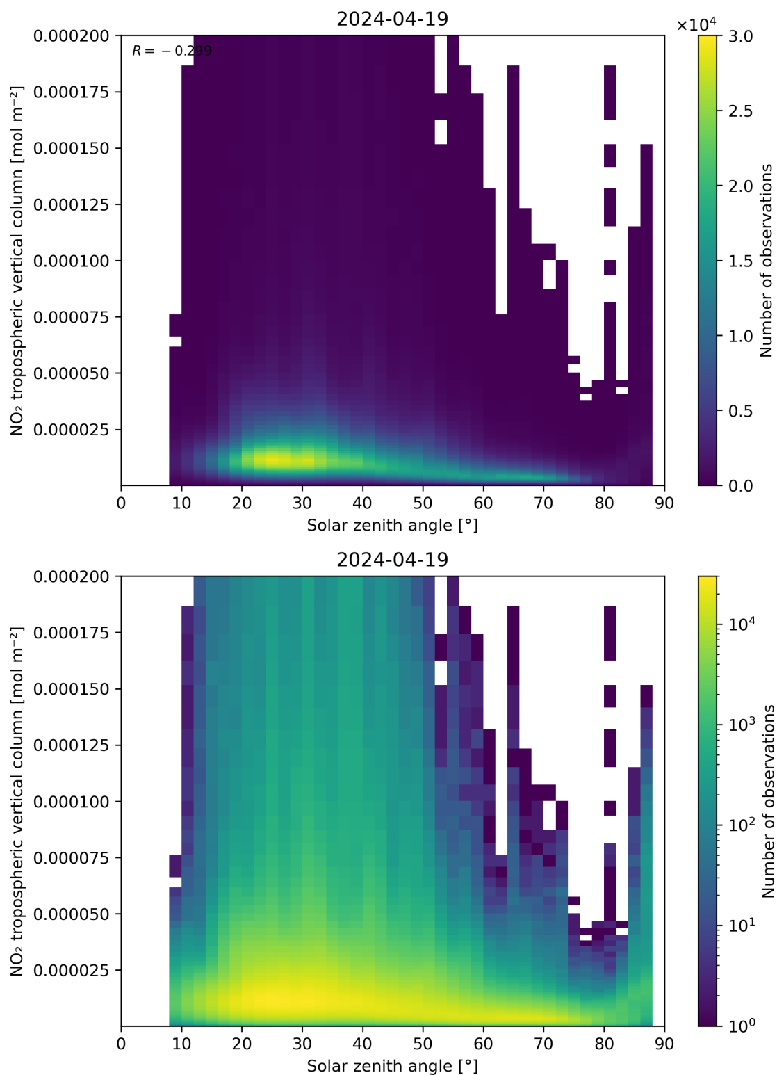
Figure 155: Scatter density plot of “Solar zenith angle” against “NO 2 tropospheric vertical column” for 2024-04-18 to 2024-04-20.
