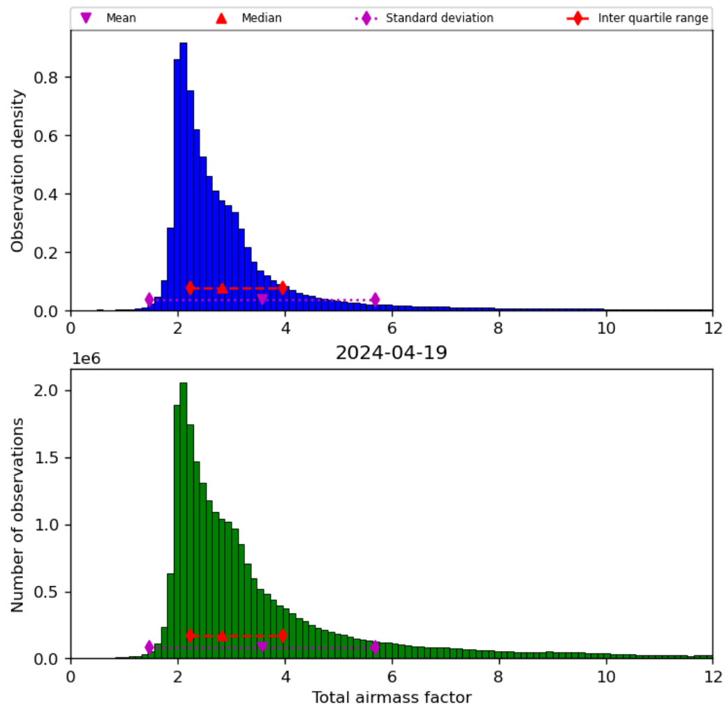
Figure 32: Histogram of “Total airmass factor” for 2024-04-18 to 2024-04-20
