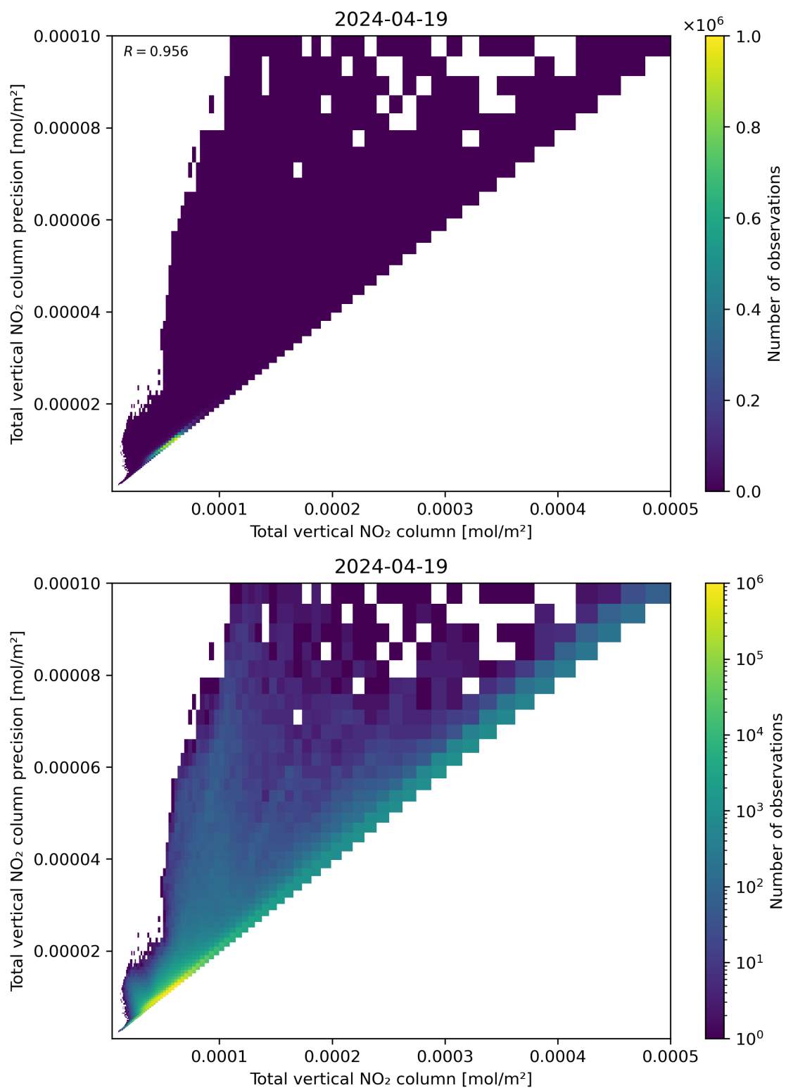
Figure 114: Scatter density plot of “Total vertical NO 2 column” against “Total vertical NO 2 column precision” for 2024-04-18 to 2024-04-20.
