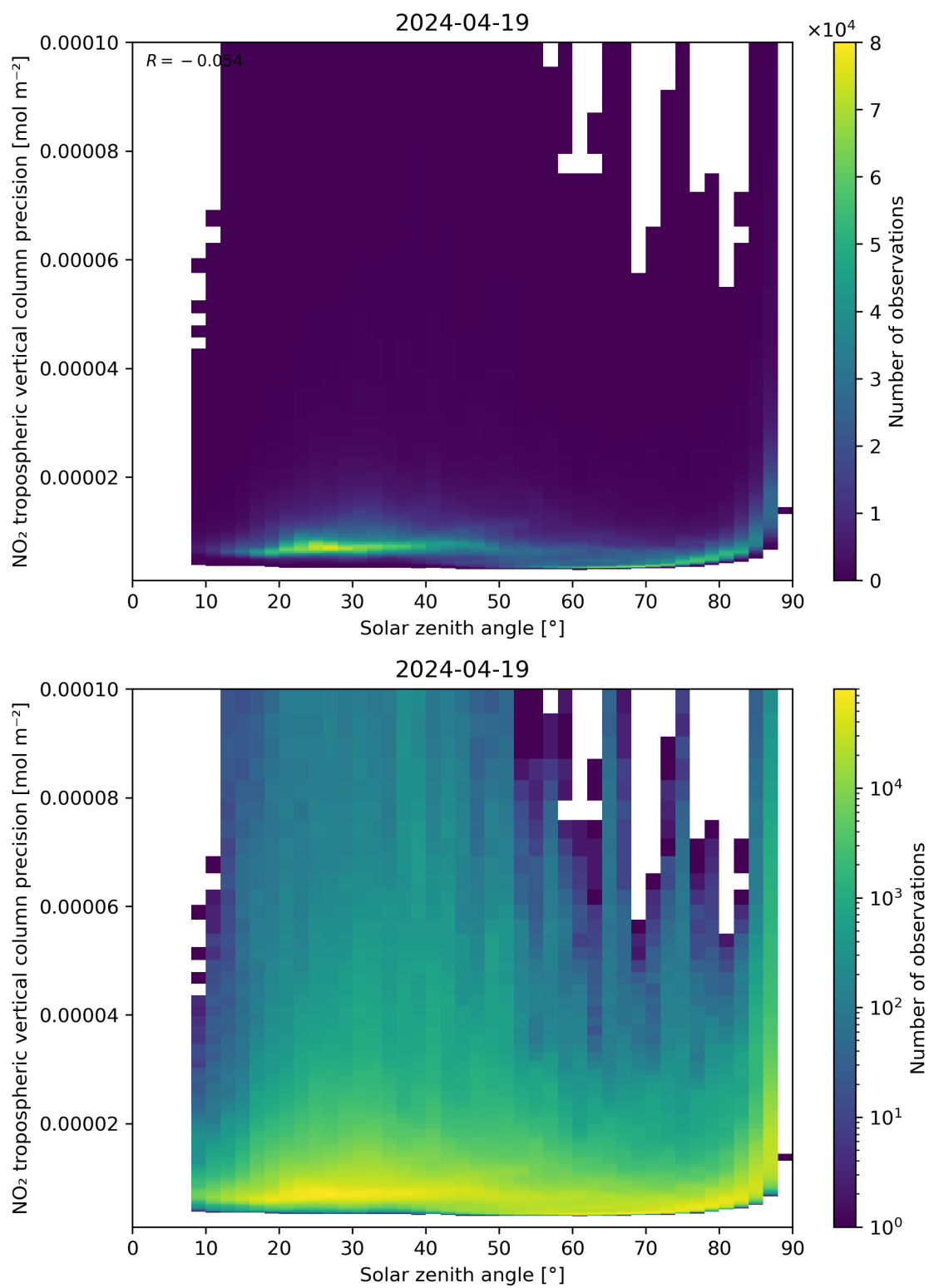
Figure 156: Scatter density plot of “Solar zenith angle” against “NO 2 tropospheric vertical column precision” for 2024-04-18 to 2024-04-20.
