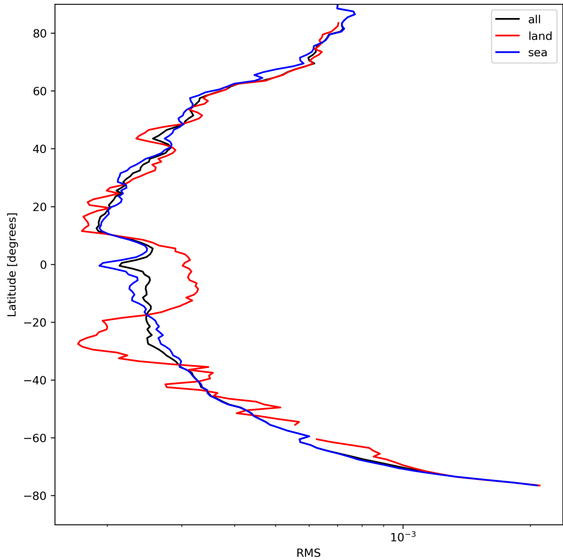
Figure 26: Zonal average of “RMS” for 2024-04-18 to 2024-04-20.
