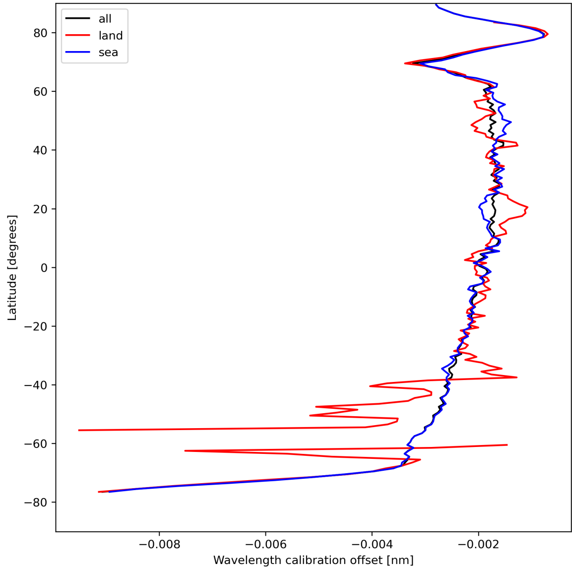
Figure 18: Zonal average of “Wavelength calibration offset” for 2024-04-18 to 2024-04-20.
