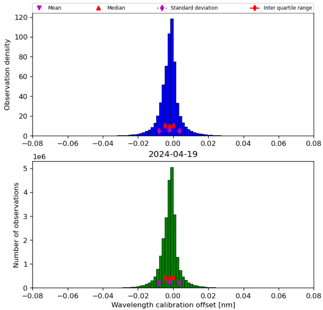
Figure 35: Histogram of “Wavelength calibration offset” for 2024-04-18 to 2024-04-20
