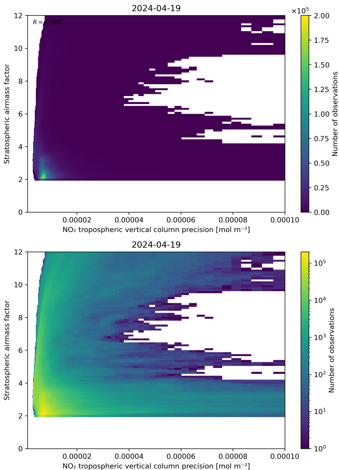
Figure 131: Scatter density plot of “NO 2 tropospheric vertical column precision” against “Stratospheric airmass factor” for 2024-04-18 to 2024-04-20.
