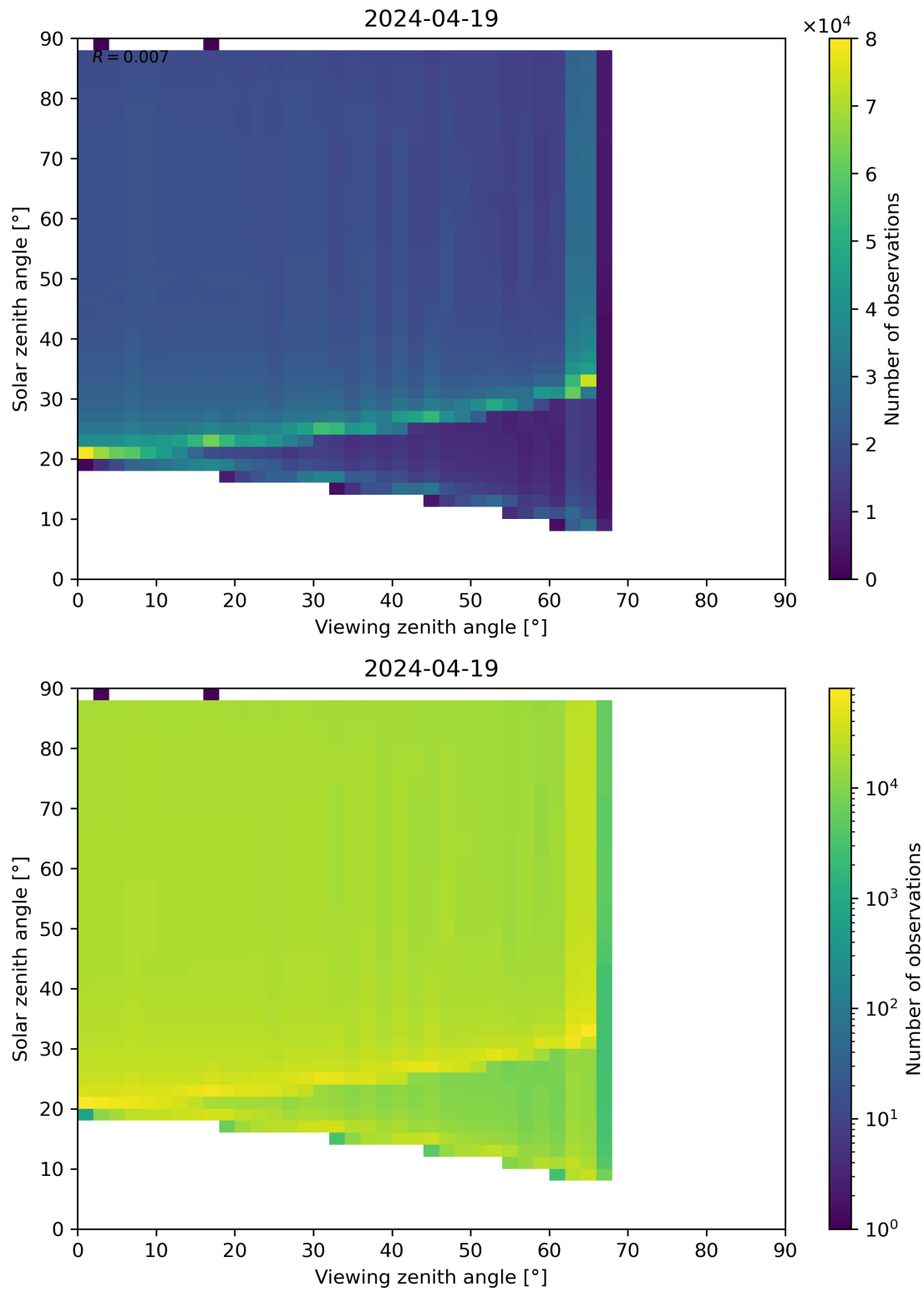
Figure 172: Scatter density plot of “Viewing zenith angle” against “Solar zenith angle” for 2024-04-18 to 2024-04-20.
