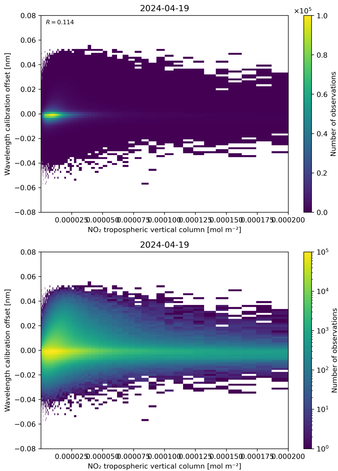
Figure 143: Scatter density plot of “NO 2 tropospheric vertical column” against “Wavelength calibration offset” for 2024-04-18 to 2024-04-20.
