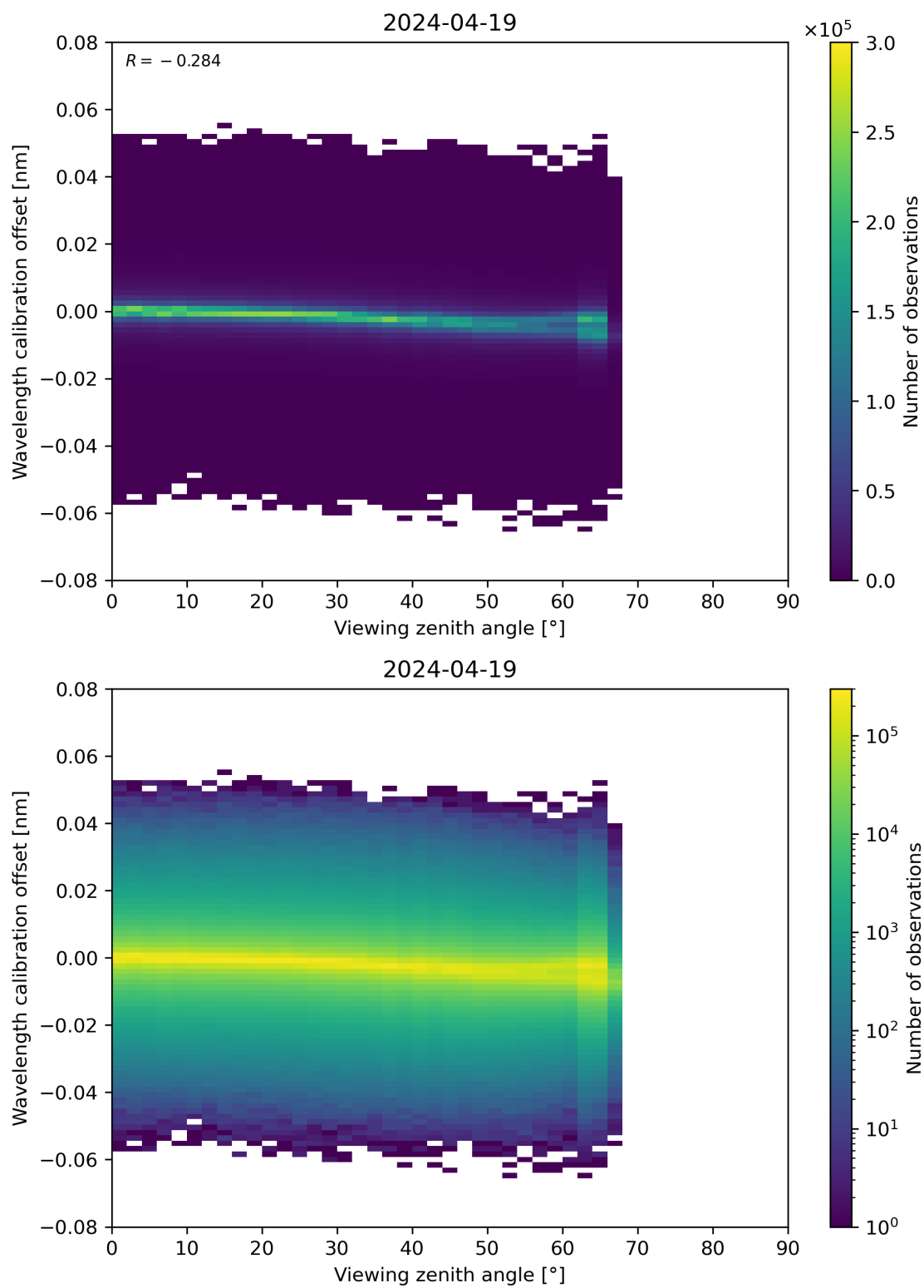
Figure 173: Scatter density plot of “Viewing zenith angle” against “Wavelength calibration offset” for 2024-04-18 to 2024-04-20.
