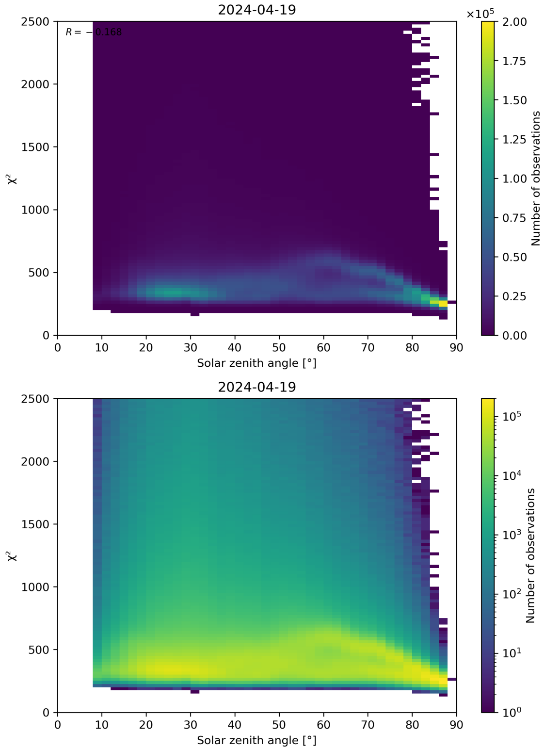
Figure 148: Scatter density plot of “Solar zenith angle” against “ \chi^2 ” for 2024-04-18 to 2024-04-20.
