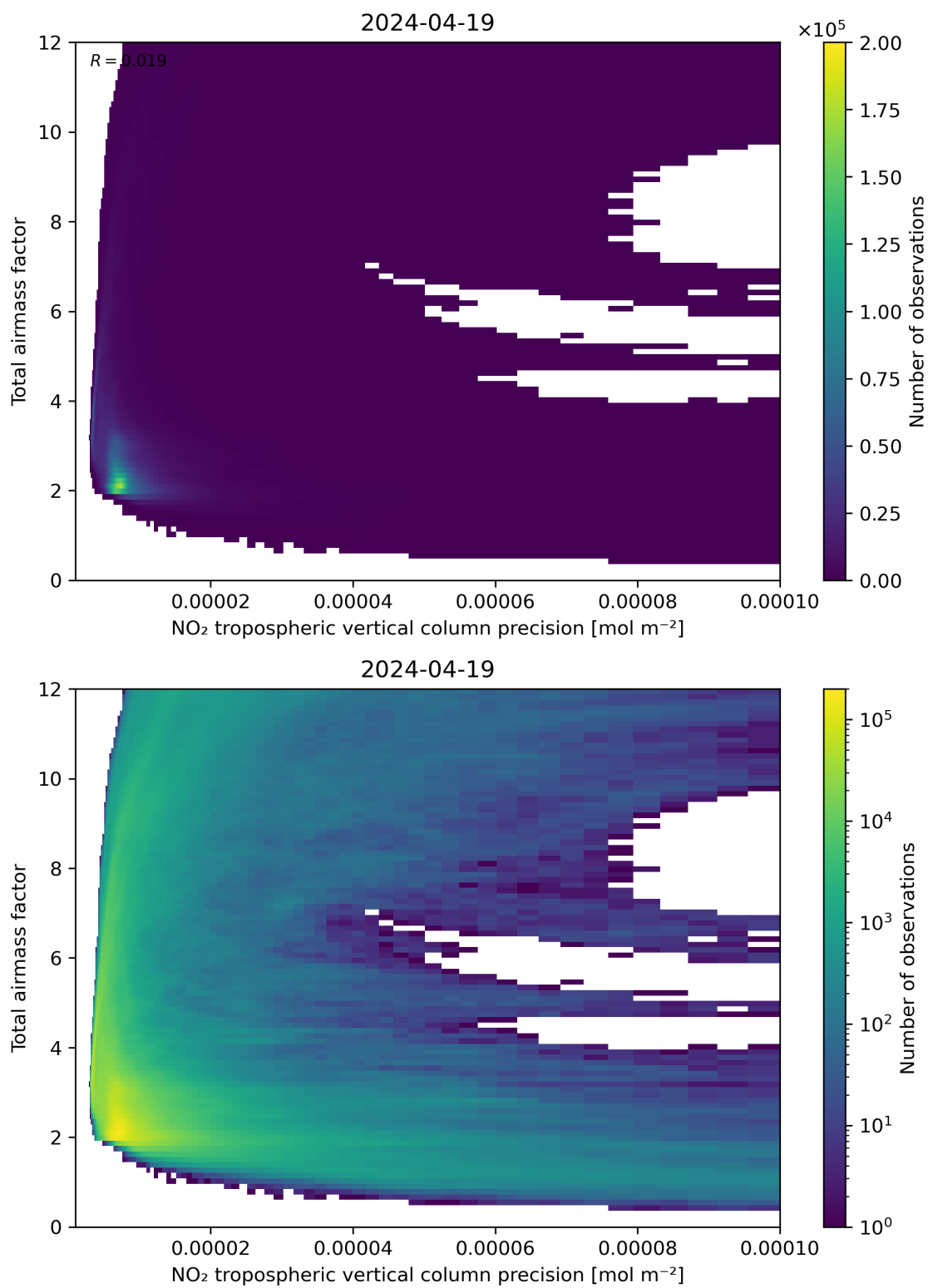
Figure 132: Scatter density plot of “NO 2 tropospheric vertical column precision” against “Total air mass factor” for 2024-04-18 to 2024-04-20.
