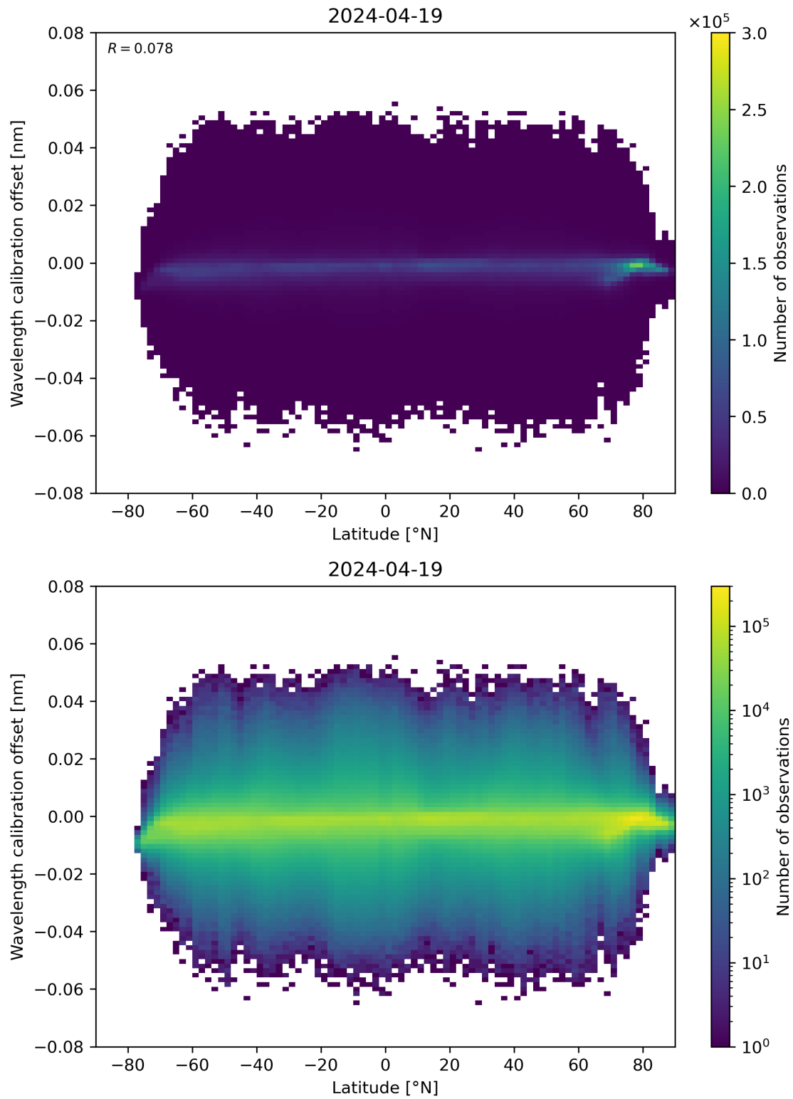
Figure 95: Scatter density plot of “Latitude” against “Wavelength calibration offset” for 2024-04-18 to 2024-04-20.
