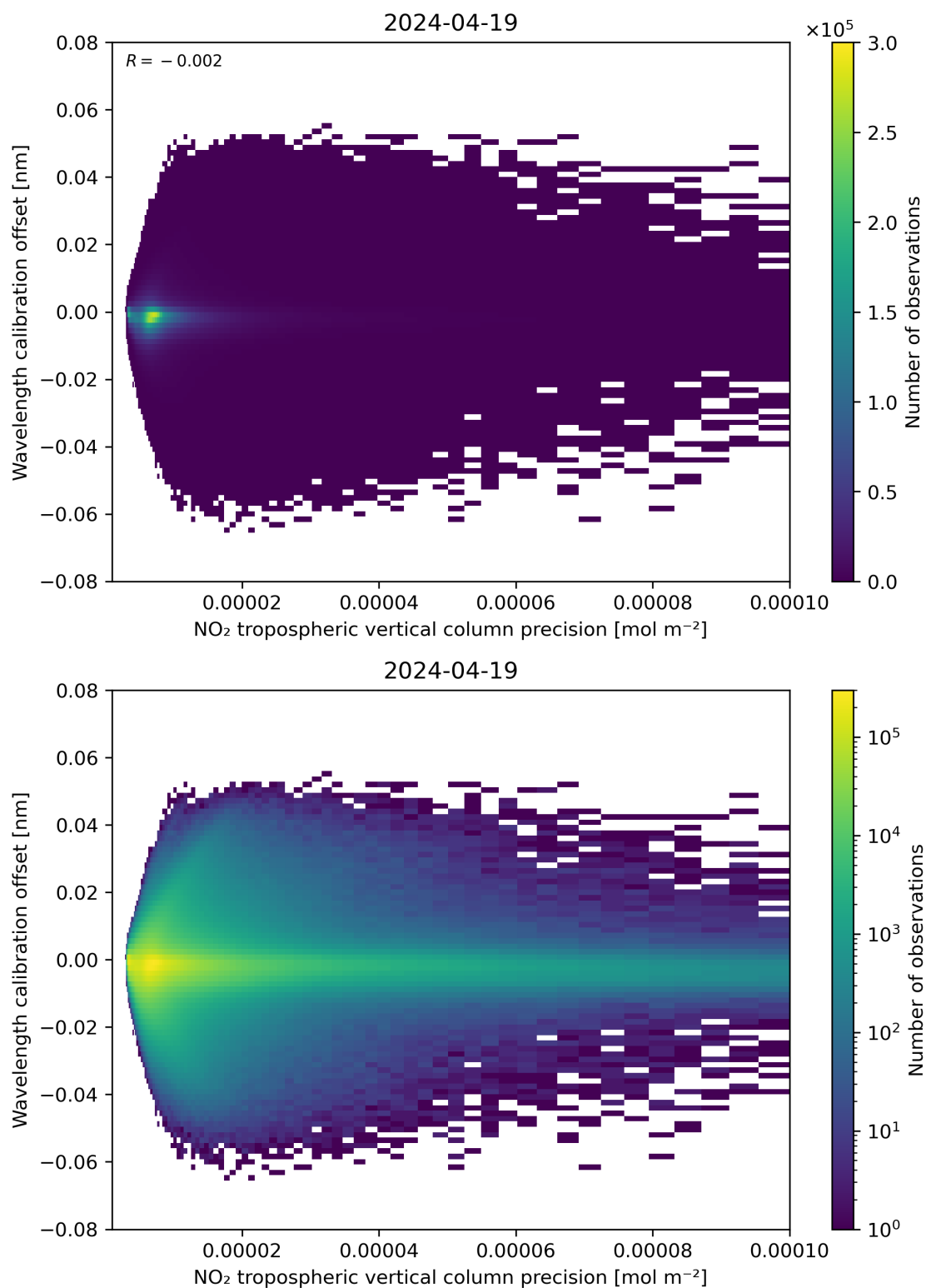
Figure 141: Scatter density plot of “NO 2 tropospheric vertical column precision” against “Wavelength calibration offset” for 2024-04-18 to 2024-04-20.
