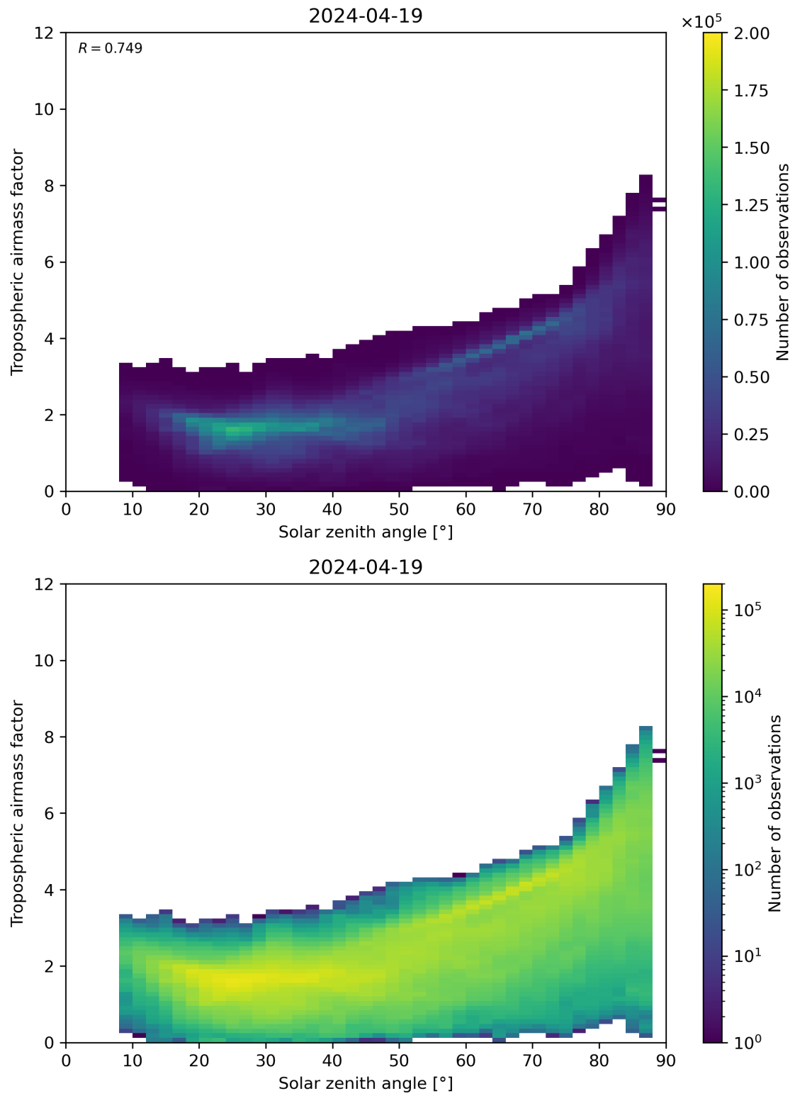
Figure 147: Scatter density plot of “Solar zenith angle” against “Tropospheric airmass factor” for 2024-04-18 to 2024-04-20.
