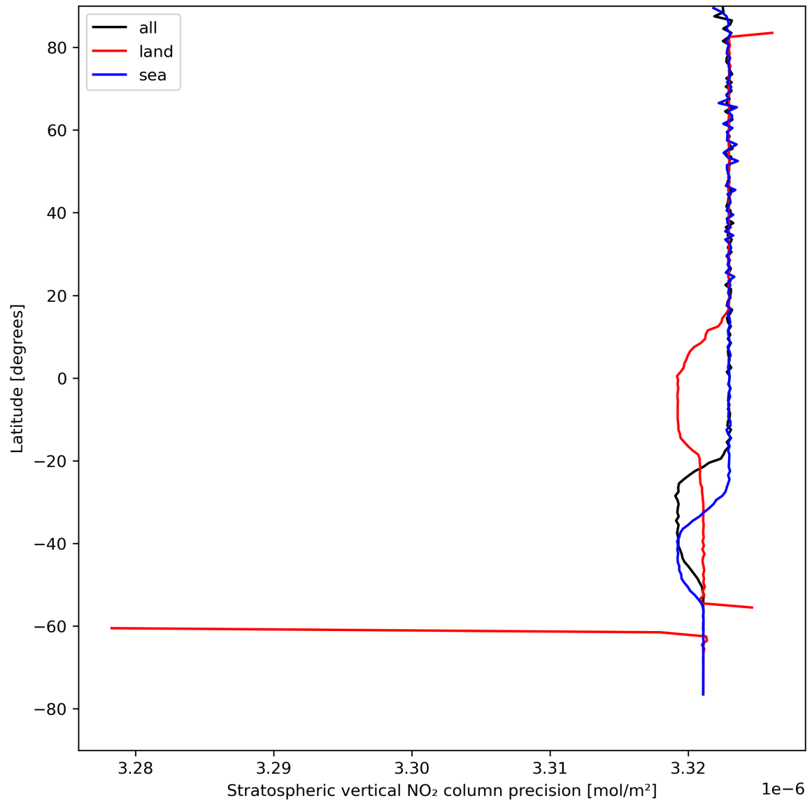
Figure 20: Zonal average of “Stratospheric vertical NO 2 column precision” for 2024-04-18 to 2024-04-20.
