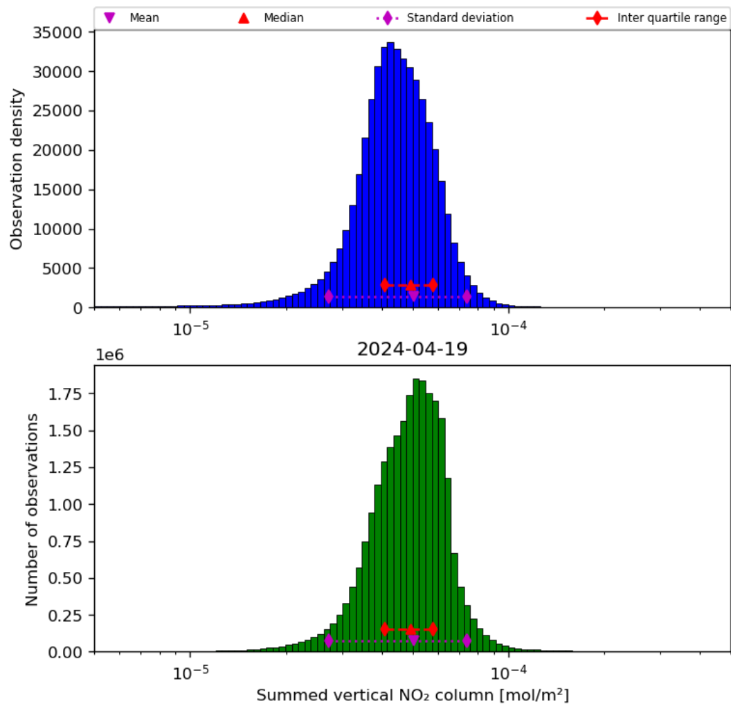
Figure 40: Histogram of “Summed vertical NO 2 column” for 2024-04-18 to 2024-04-20
