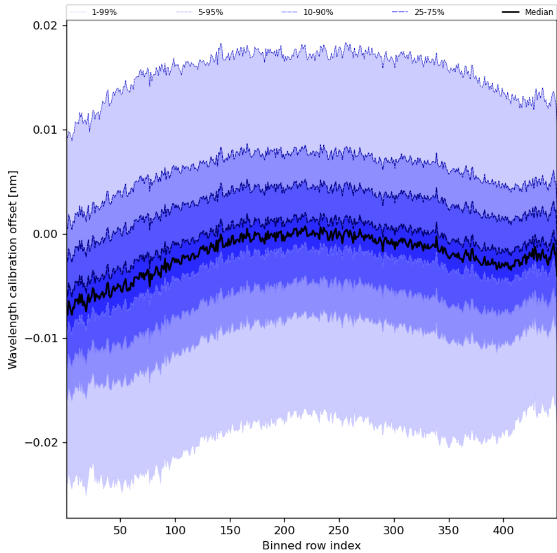
Figure 52: Along track statistics of “Wavelength calibration offset” for 2024-04-18 to 2024-04-20
