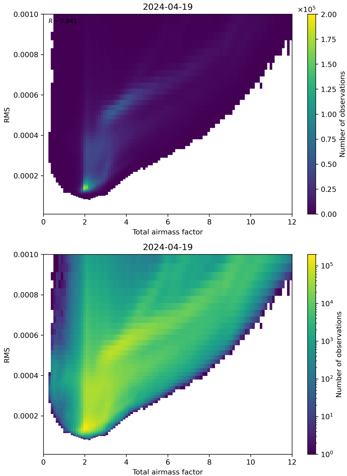
Figure 69: Scatter density plot of “Total airmass factor” against “RMS” for 2024-04-18 to 2024-04-20.
