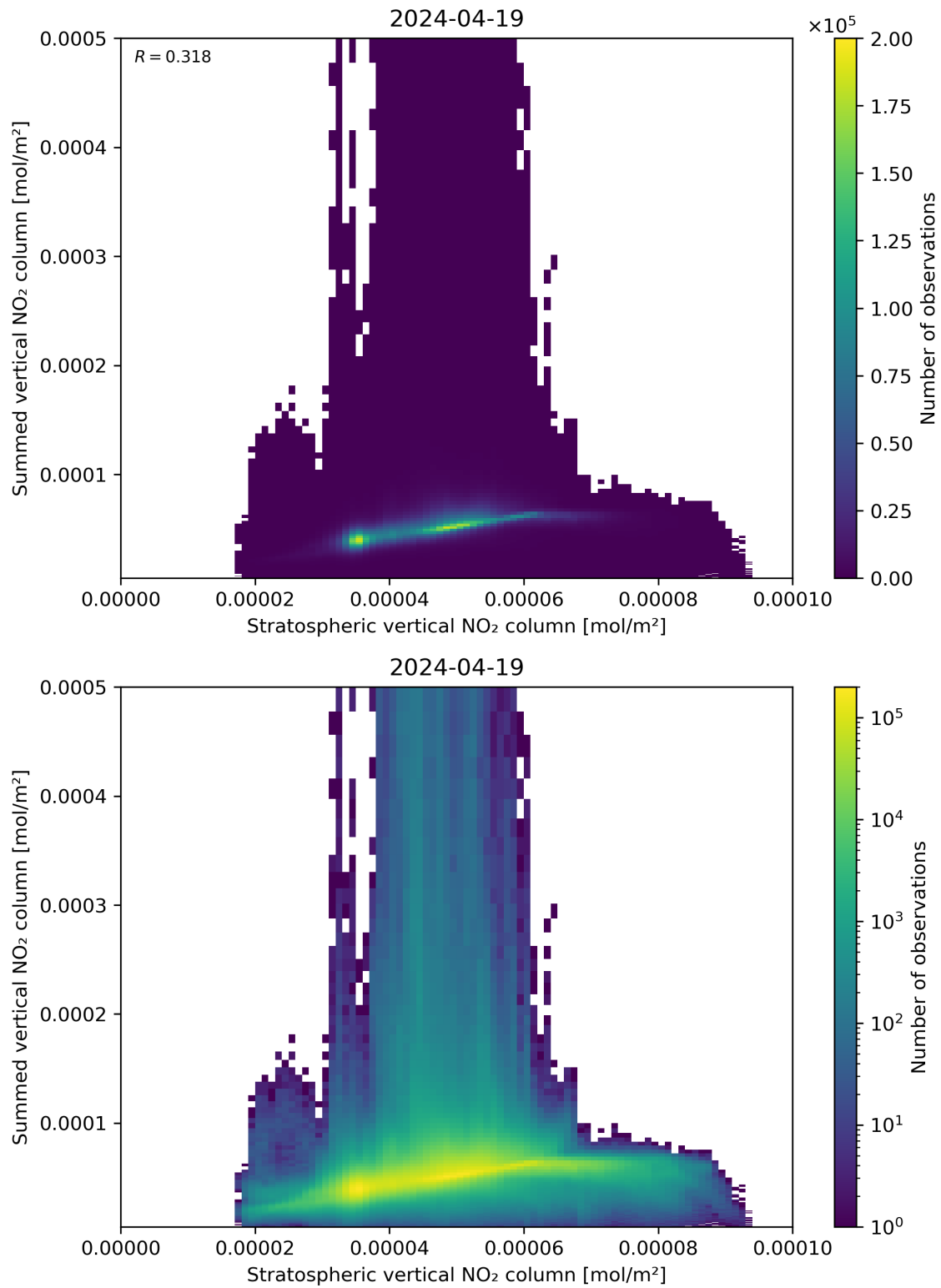
Figure 98: Scatter density plot of “Stratospheric vertical NO 2 column” against “Summed vertical NO 2 column” for 2024-04-18 to 2024-04-20.
