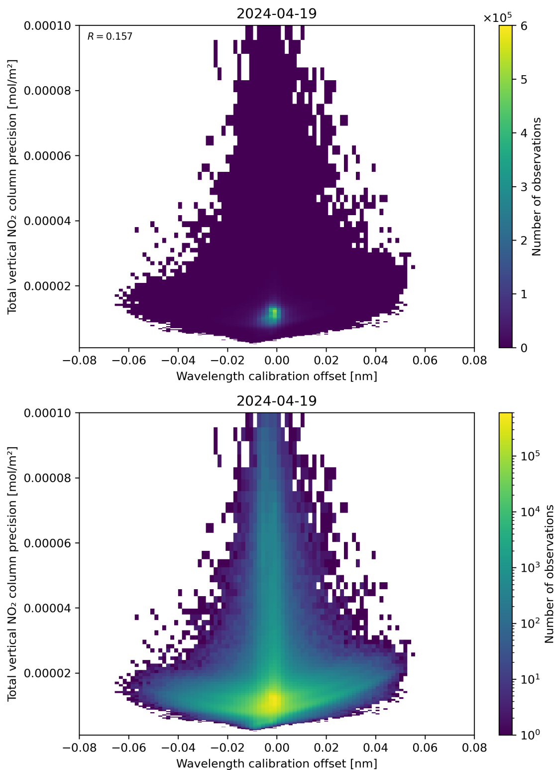
Figure 180: Scatter density plot of “Wavelength calibration offset” against “Total vertical NO 2 column precision” for 2024-04-18 to 2024-04-20.
