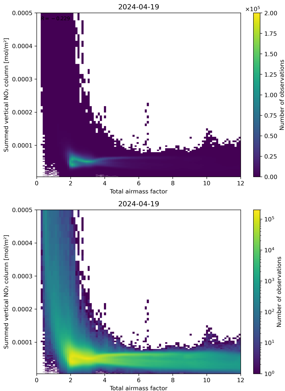
Figure 65: Scatter density plot of “Total airmass factor” against “Summed vertical NO 2 column” for 2024-04-18 to 2024-04-20.
