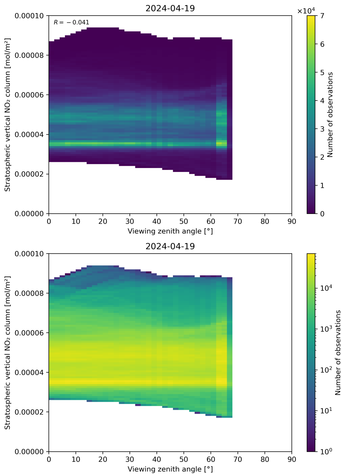
Figure 164: Scatter density plot of “Viewing zenith angle” against “Stratospheric vertical NO 2 column” for 2024-04-18 to 2024-04-20.
