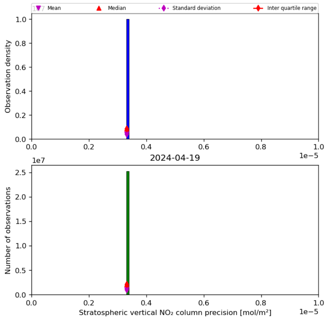
Figure 37: Histogram of “Stratospheric vertical NO 2 column precision” for 2024-04-18 to 2024-04-20
