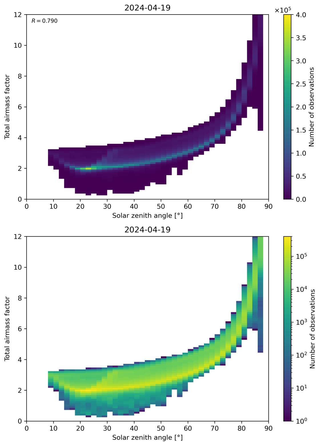
Figure 146: Scatter density plot of “Solar zenith angle” against “Total air mass factor” for 2024-04-18 to 2024-04-20.
