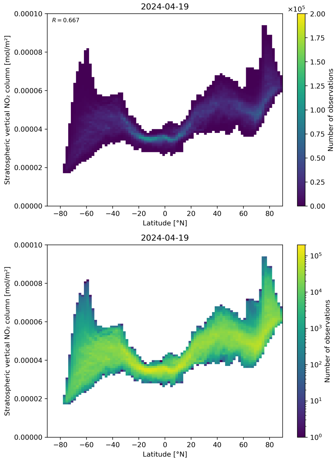
Figure 87: Scatter density plot of “Latitude” against “Stratospheric vertical NO 2 column” for 2024-04-18 to 2024-04-20.
