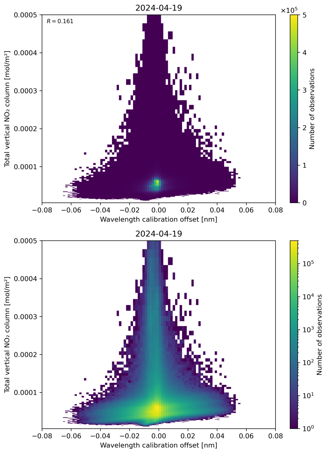
Figure 179: Scatter density plot of “Wavelength calibration offset” against “Total vertical NO 2 column” for 2024-04-18 to 2024-04-20.
