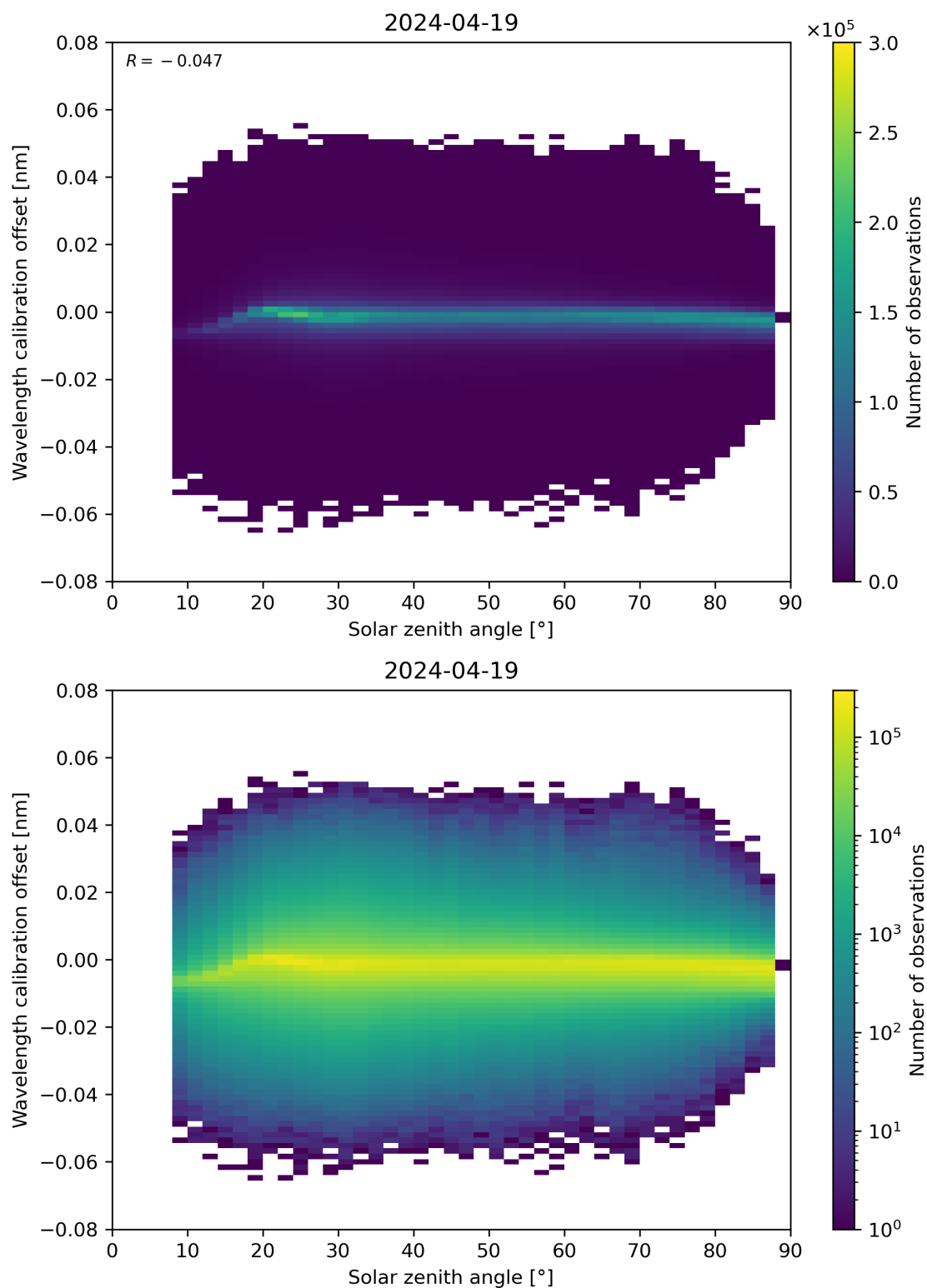
Figure 158: Scatter density plot of “Solar zenith angle” against “Wavelength calibration offset” for 2024-04-18 to 2024-04-20.
