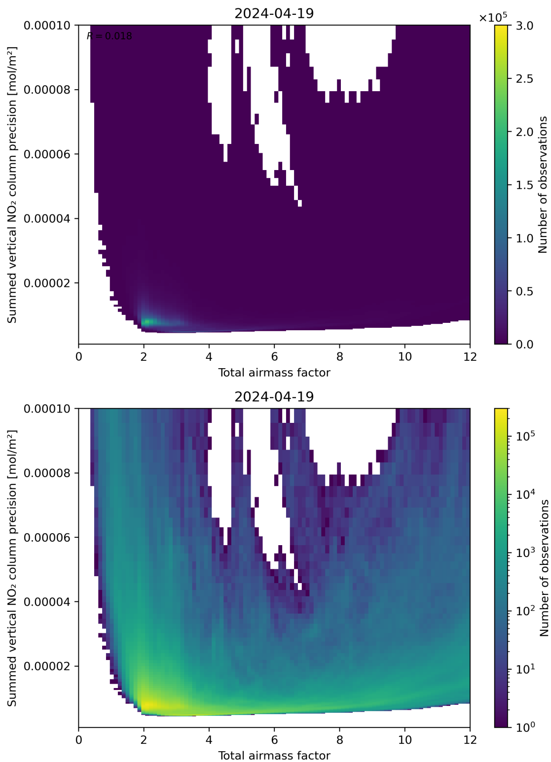
Figure 66: Scatter density plot of “Total airmass factor” against “Summed vertical NO 2 column precision” for 2024-04-18 to 2024-04-20.
