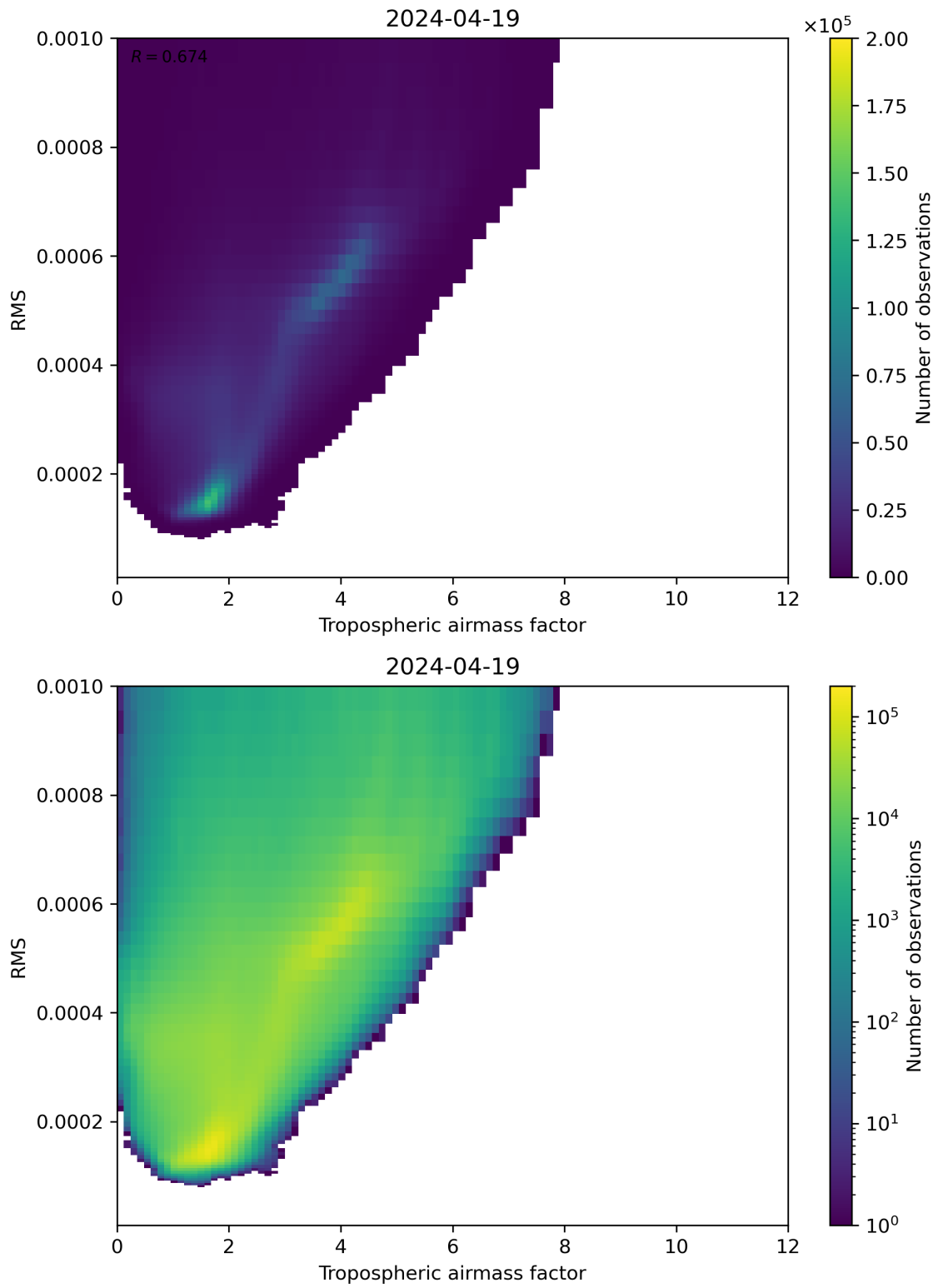
Figure 79: Scatter density plot of “Tropospheric airmass factor” against “RMS” for 2024-04-18 to 2024-04-20.
