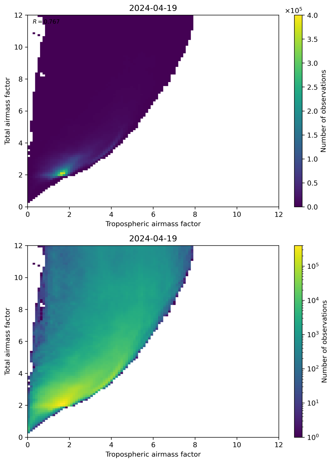
Figure 72: Scatter density plot of “Tropospheric airmass factor” against “Total airmass factor” for 2024-04-18 to 2024-04-20.
