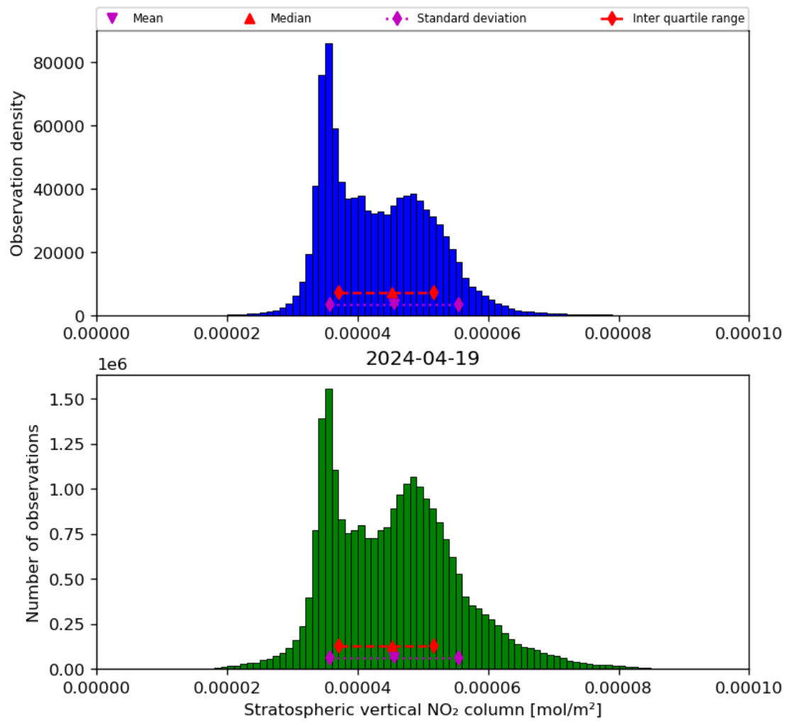
Figure 36: Histogram of “Stratospheric vertical NO 2 column” for 2024-04-18 to 2024-04-20
