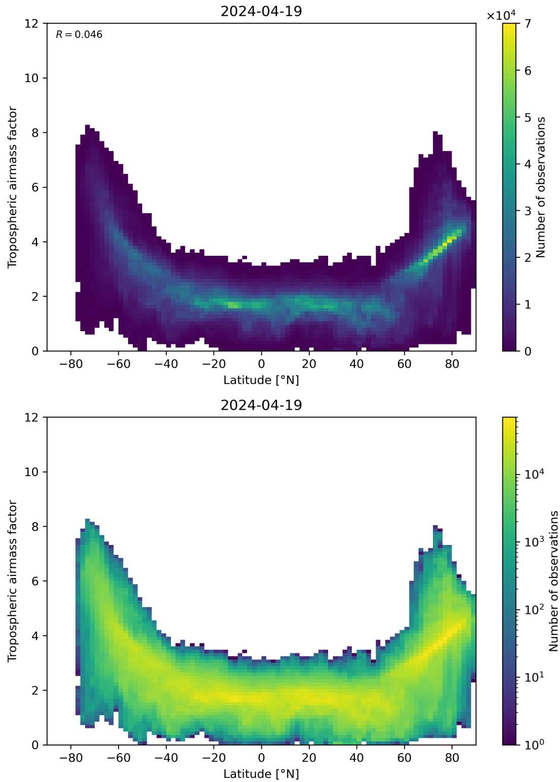
Figure 85: Scatter density plot of “Latitude” against “Tropospheric airmass factor” for 2024-04-18 to 2024-04-20.
