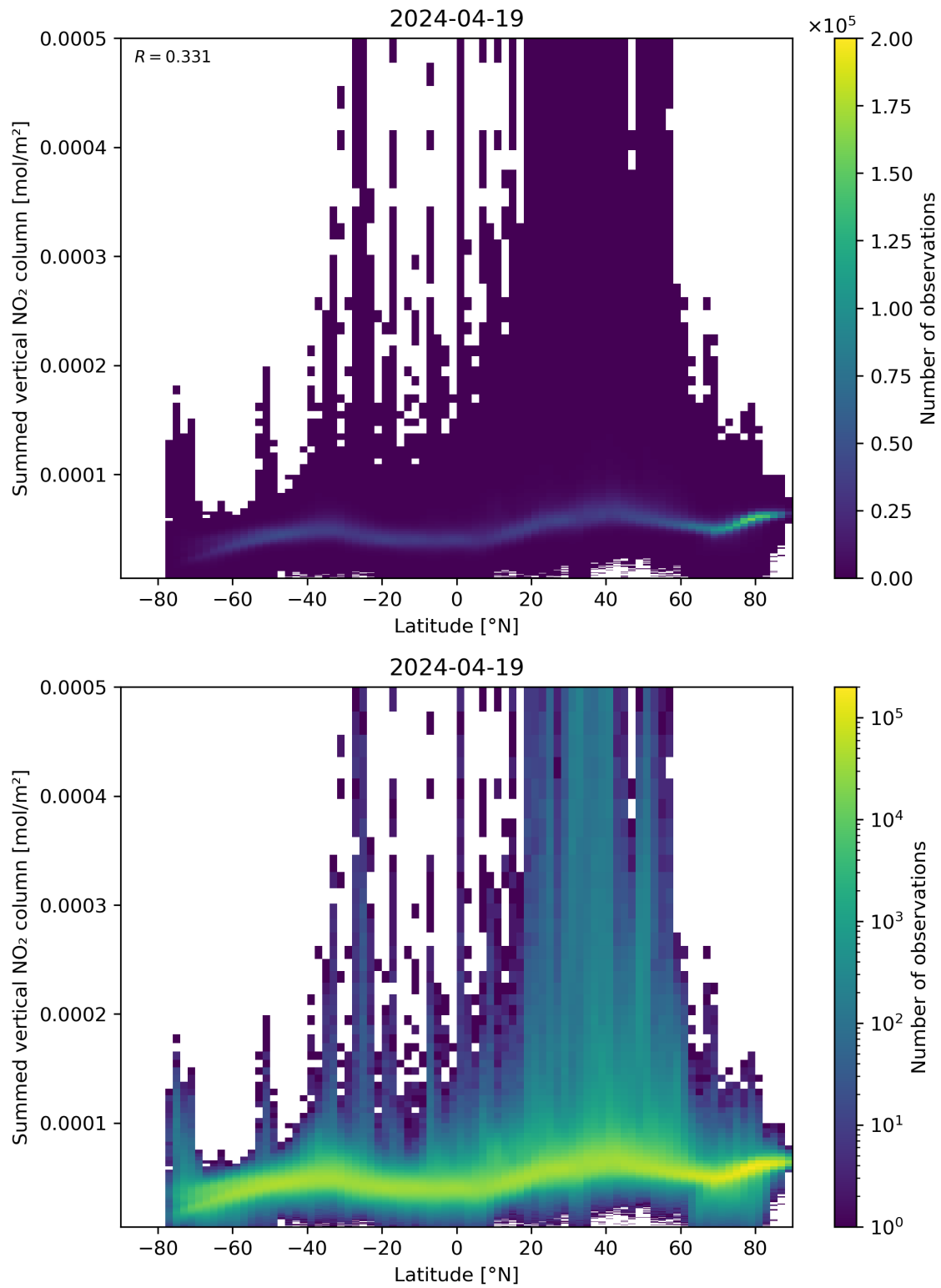
Figure 88: Scatter density plot of “Latitude” against “Summed vertical NO 2 column” for 2024-04-18 to 2024-04-20.
