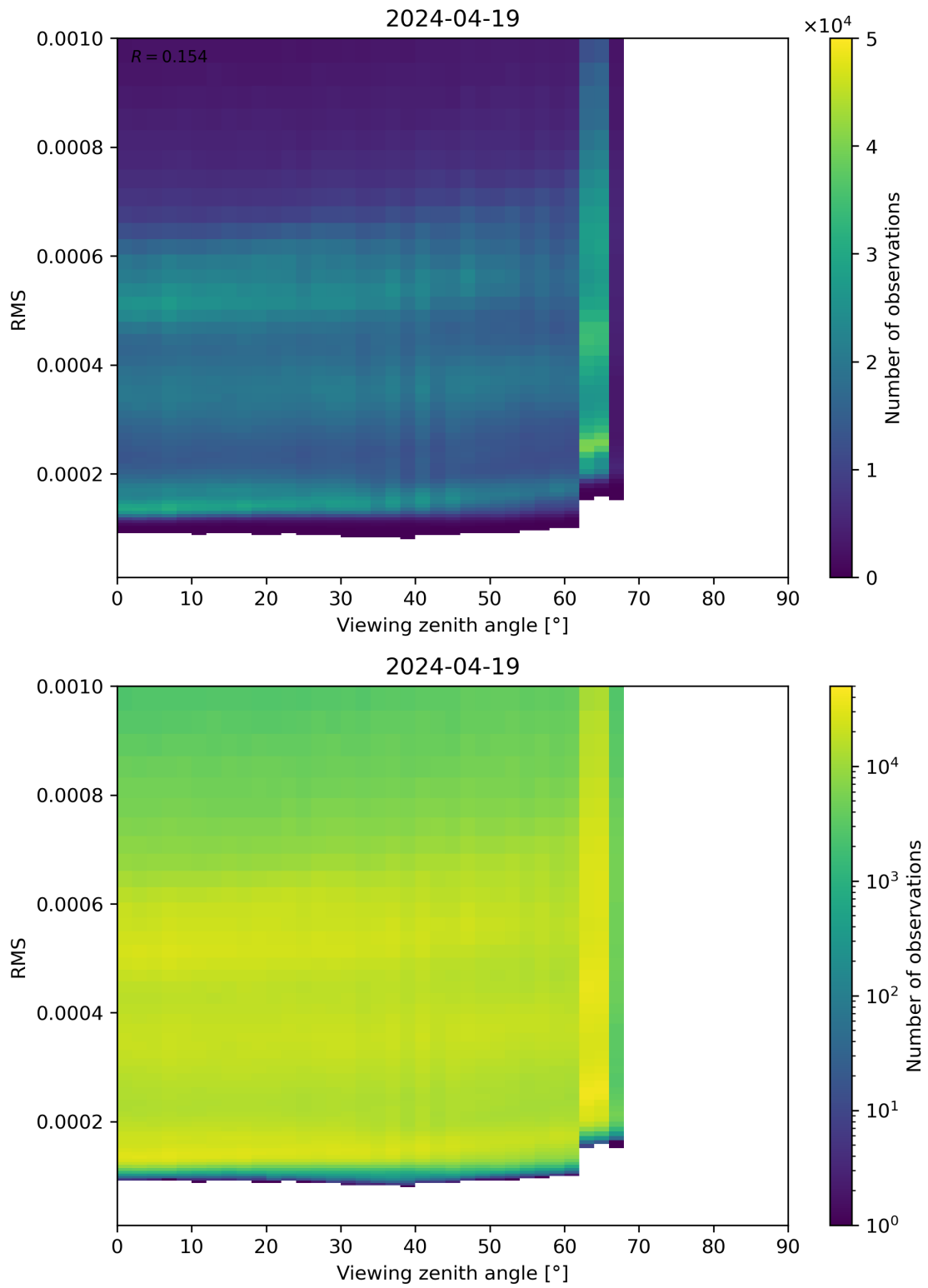
Figure 171: Scatter density plot of “Viewing zenith angle” against “RMS” for 2024-04-18 to 2024-04-20.
