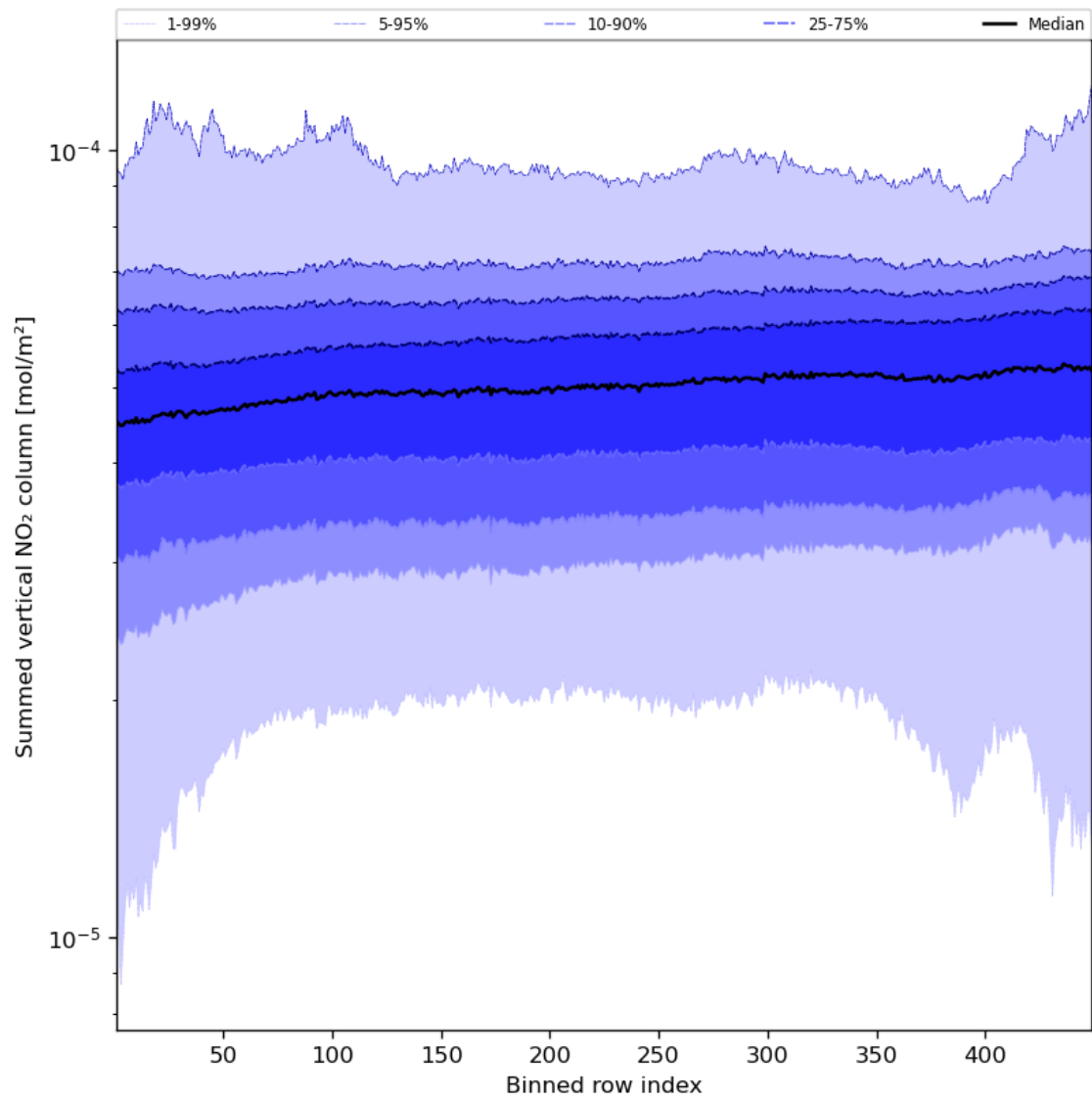
Figure 57: Along track statistics of “Summed vertical NO 2 column” for 2024-04-18 to 2024-04-20
