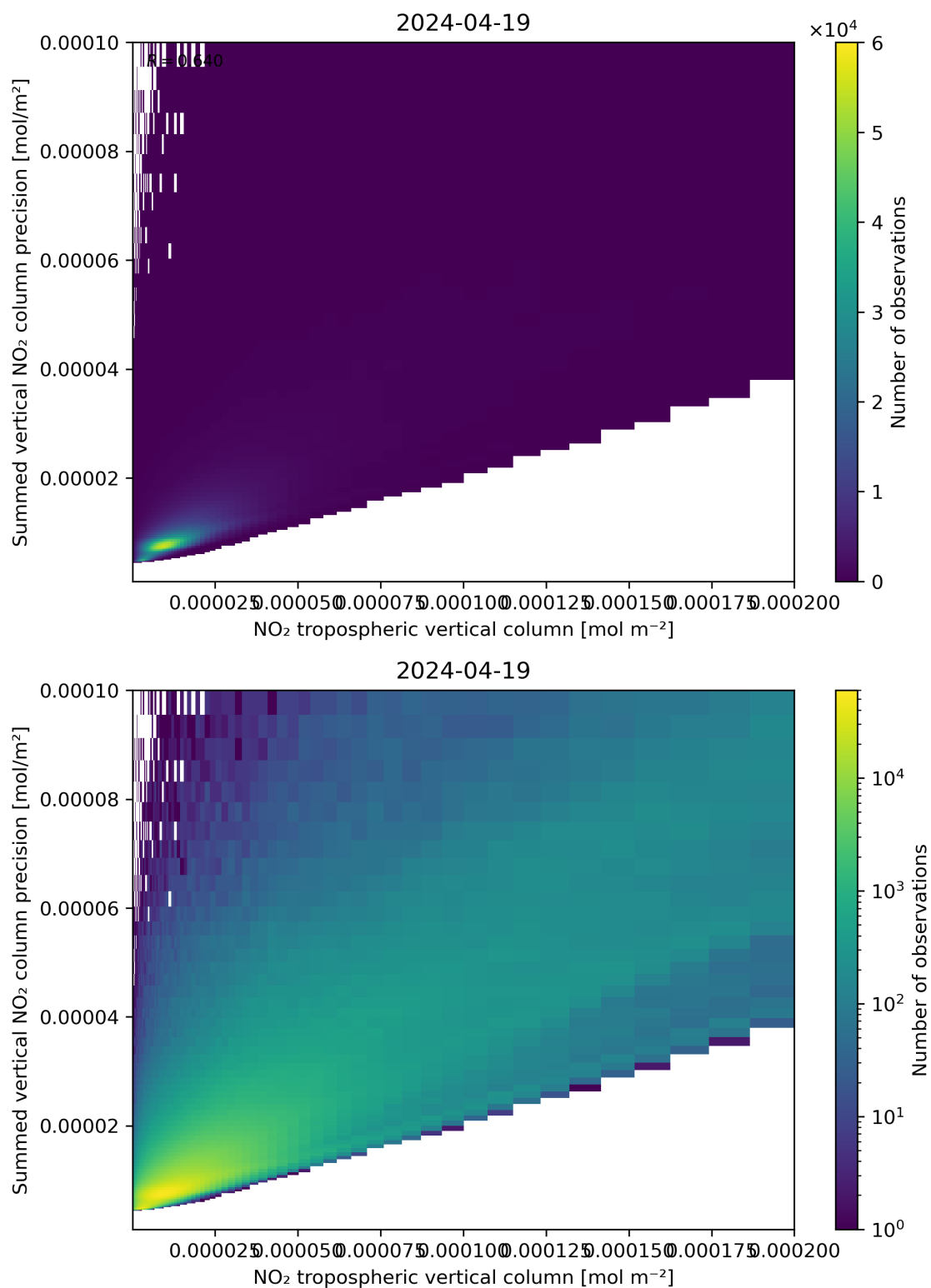
Figure 127: Scatter density plot of “NO 2 tropospheric vertical column” against “Summed vertical NO 2 column precision” for 2024-04-18 to 2024-04-20.
