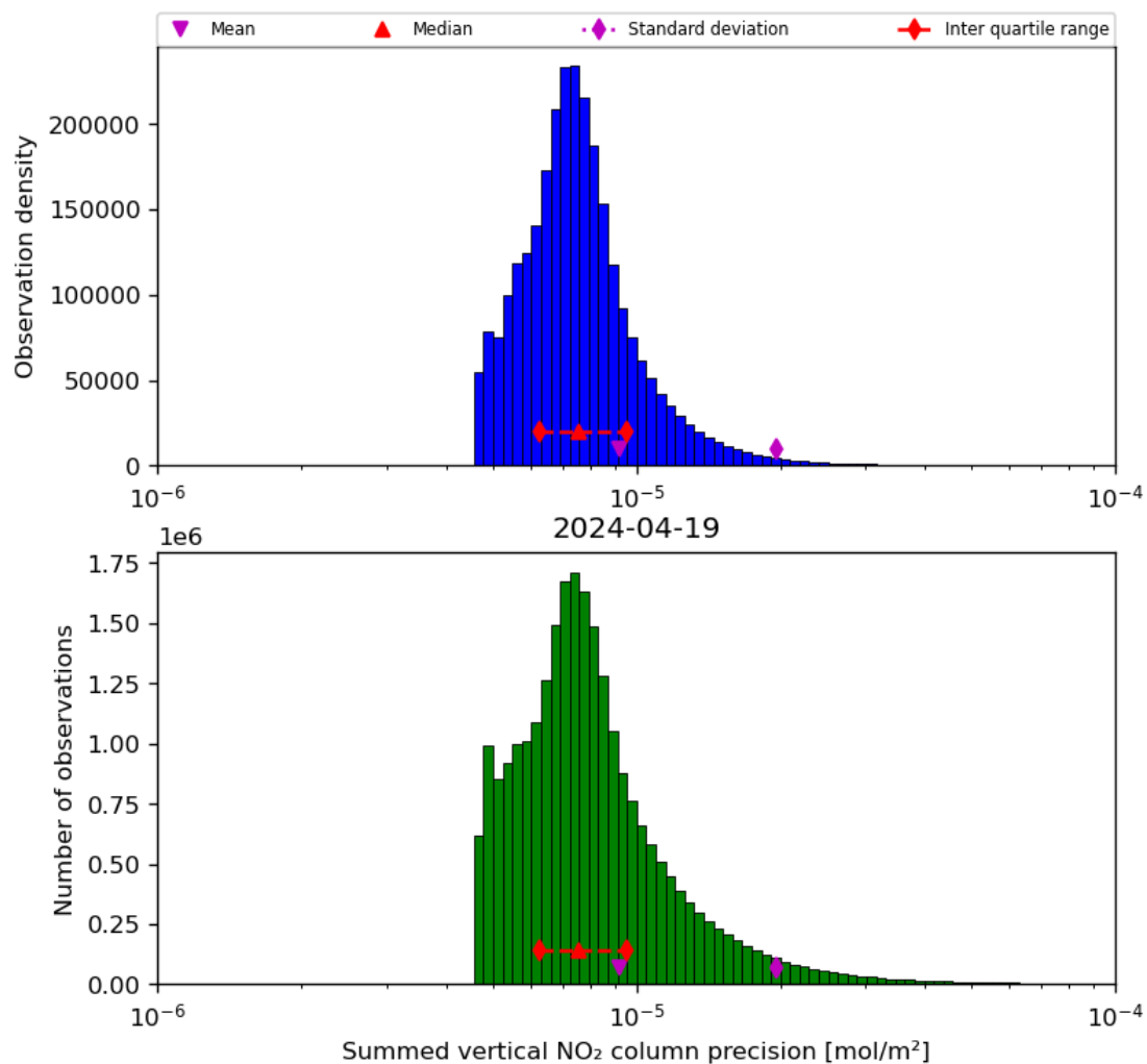
Figure 41: Histogram of “Summed vertical NO 2 column precision” for 2024-04-18 to 2024-04-20
