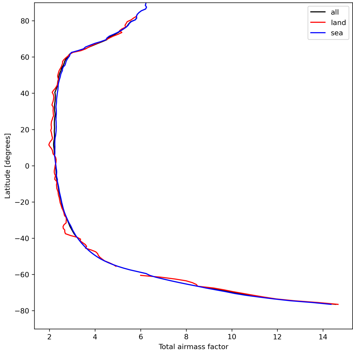
Figure 15: Zonal average of “Total airmass factor” for 2024-04-18 to 2024-04-20.
