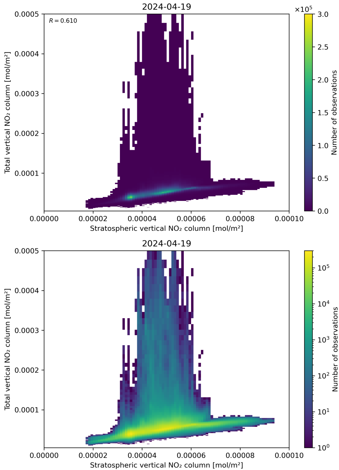
Figure 100: Scatter density plot of “Stratospheric vertical NO 2 column” against “Total vertical NO 2 column” for 2024-04-18 to 2024-04-20.
