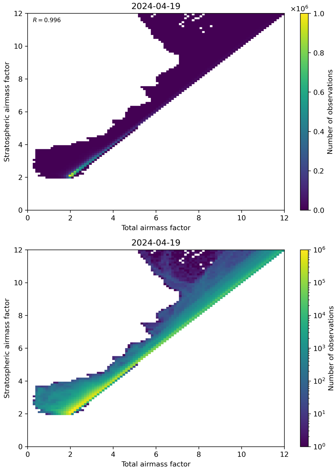
Figure 62: Scatter density plot of “Total airmass factor” against “Stratospheric airmass factor” for 2024-04-18 to 2024-04-20.
