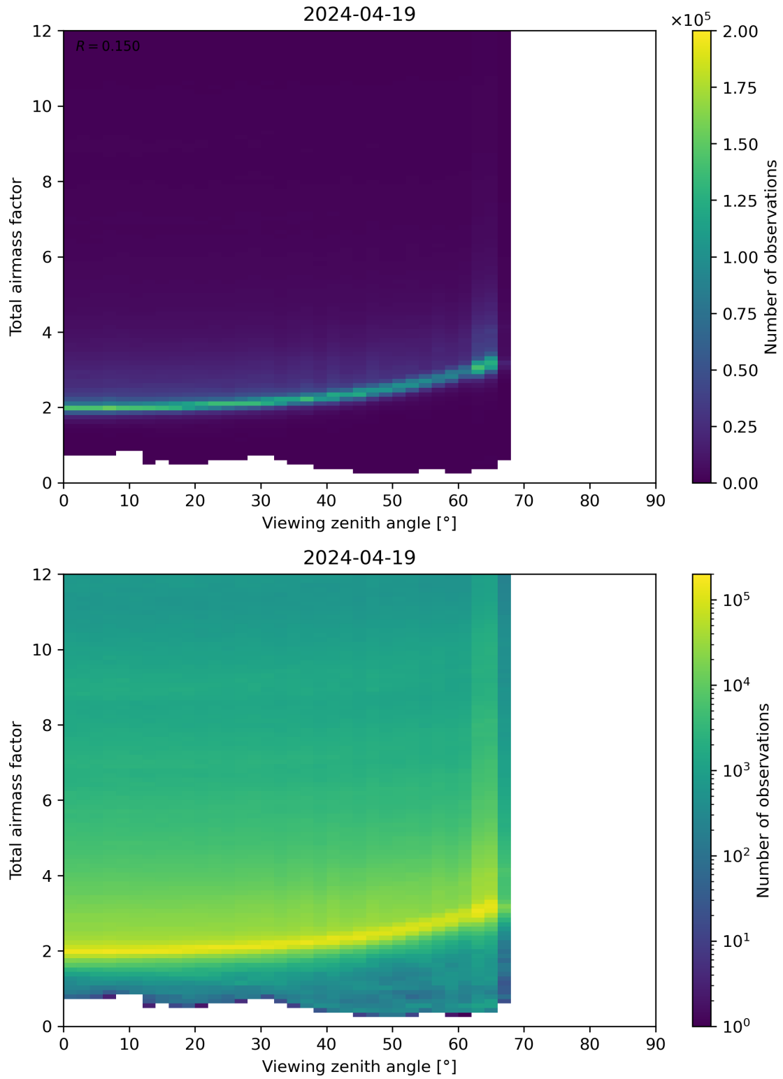
Figure 160: Scatter density plot of “Viewing zenith angle” against “Total airmass factor” for 2024-04-18 to 2024-04-20.
