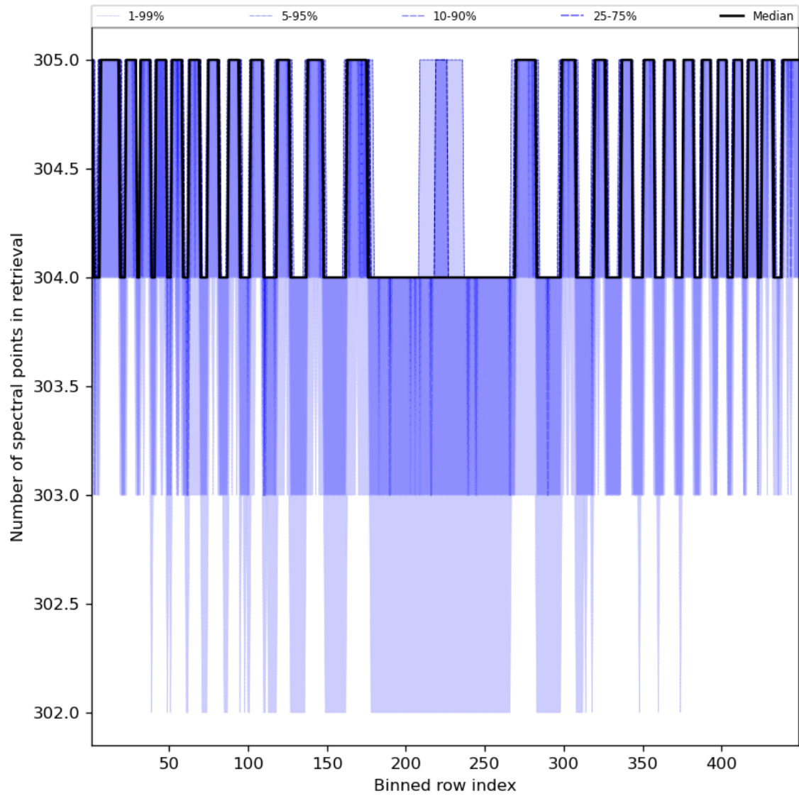
Figure 50: Along track statistics of “Number of spectral points in retrieval” for 2024-04-18 to 2024-04-20
