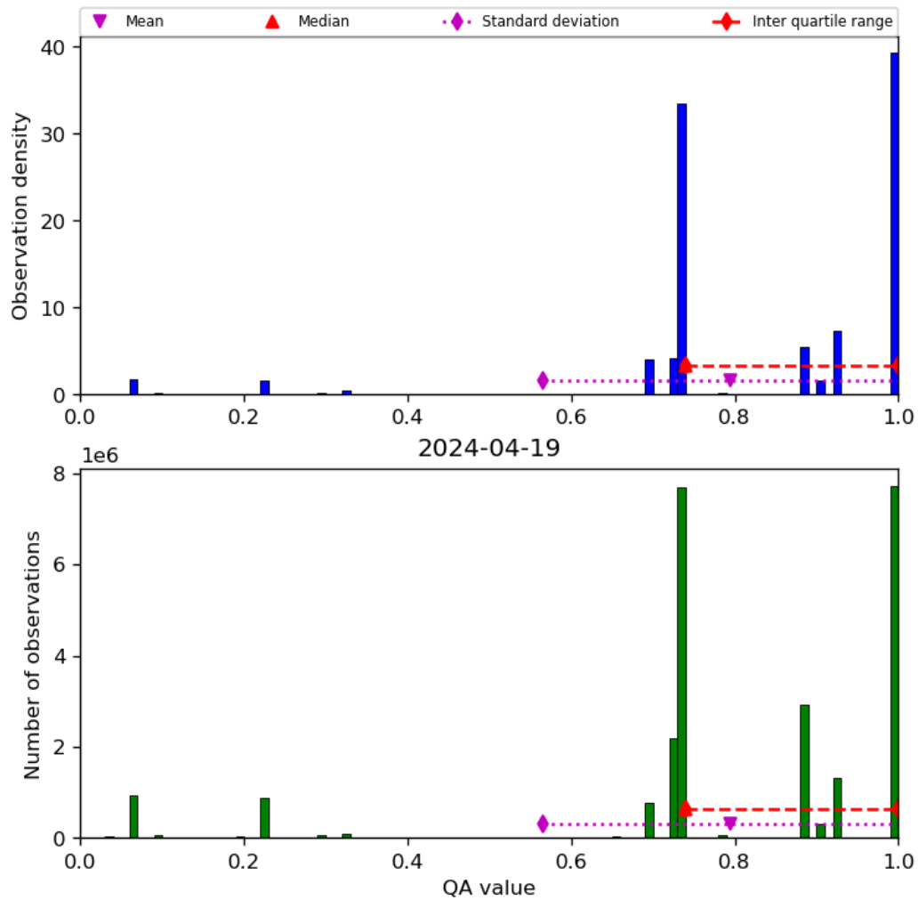
Figure 28: Histogram of “QA value” for 2024-04-18 to 2024-04-20
