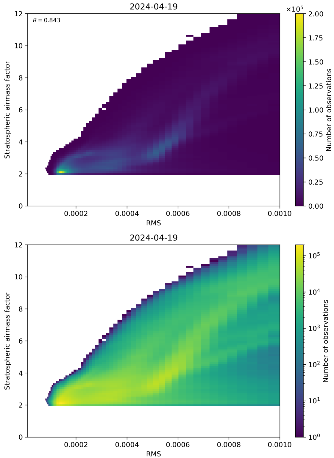
Figure 144: Scatter density plot of “RMS” against “Stratospheric airmass factor” for 2024-04-18 to 2024-04-20.
