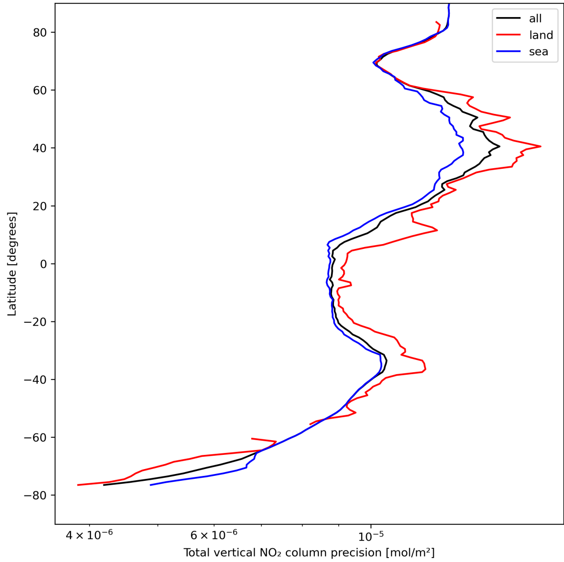
Figure 22: Zonal average of “Total vertical NO 2 column precision” for 2024-04-18 to 2024-04-20.
