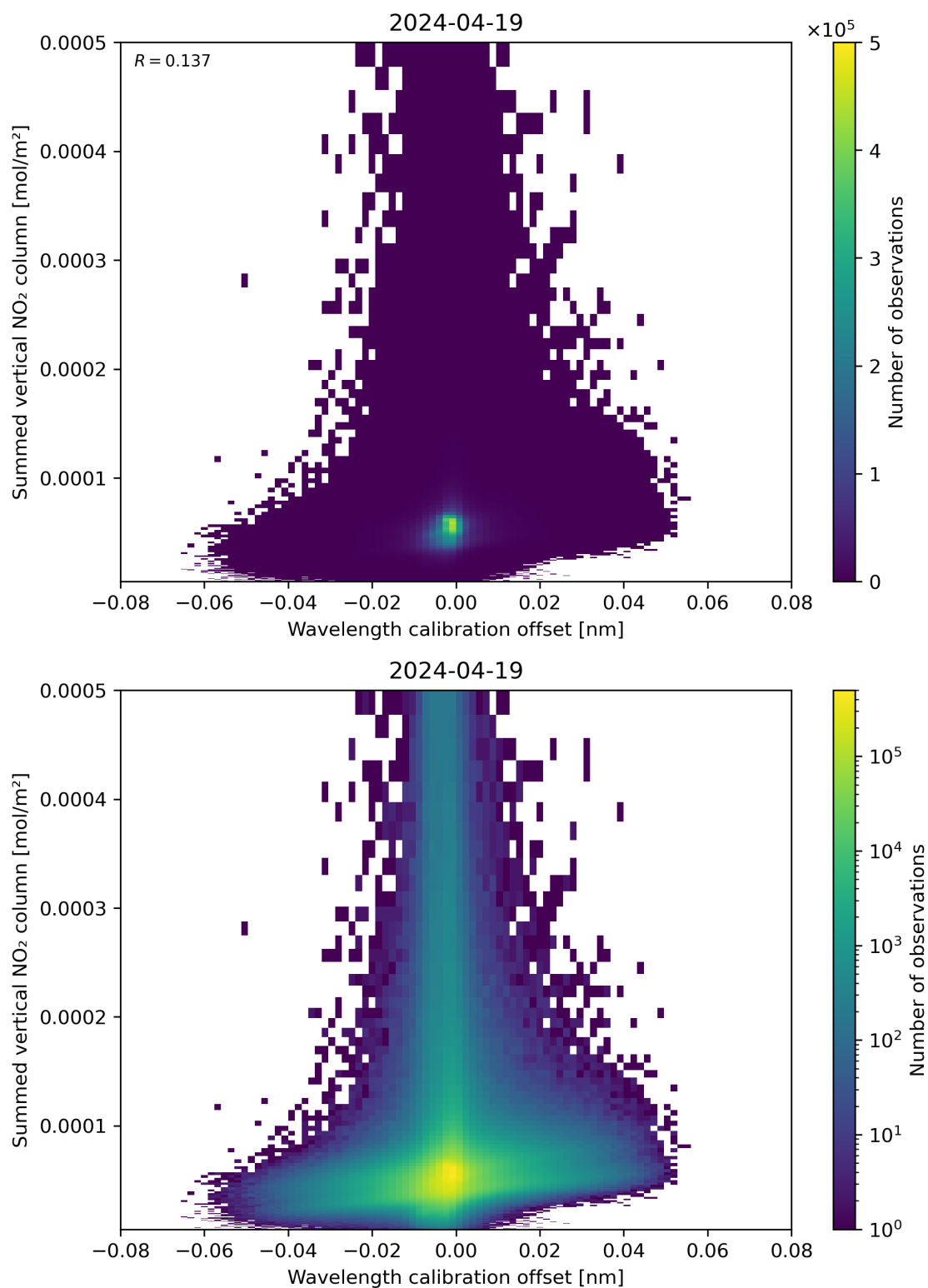
Figure 177: Scatter density plot of “Wavelength calibration offset” against “Summed vertical NO 2 column” for 2024-04-18 to 2024-04-20.
