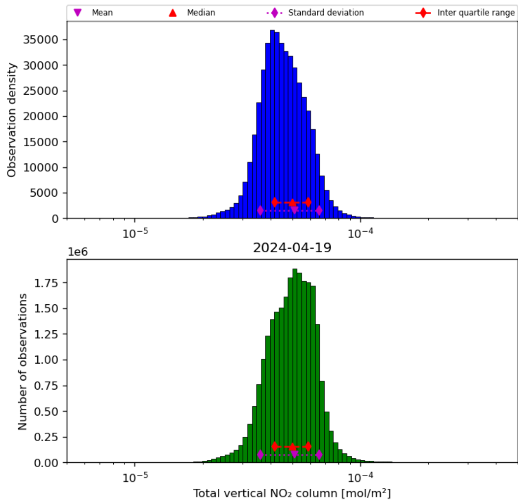
Figure 38: Histogram of “Total vertical NO 2 column” for 2024-04-18 to 2024-04-20
