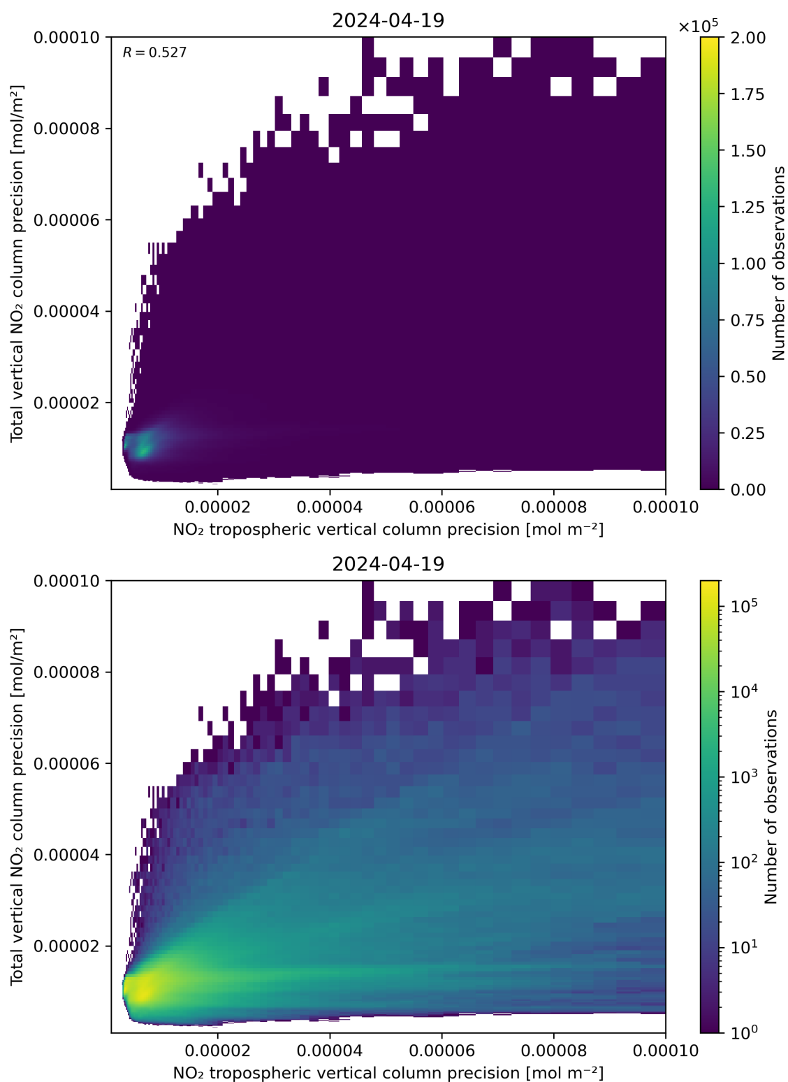
Figure 139: Scatter density plot of “NO 2 tropospheric vertical column precision” against “Total vertical NO 2 column precision” for 2024-04-18 to 2024-04-20.
