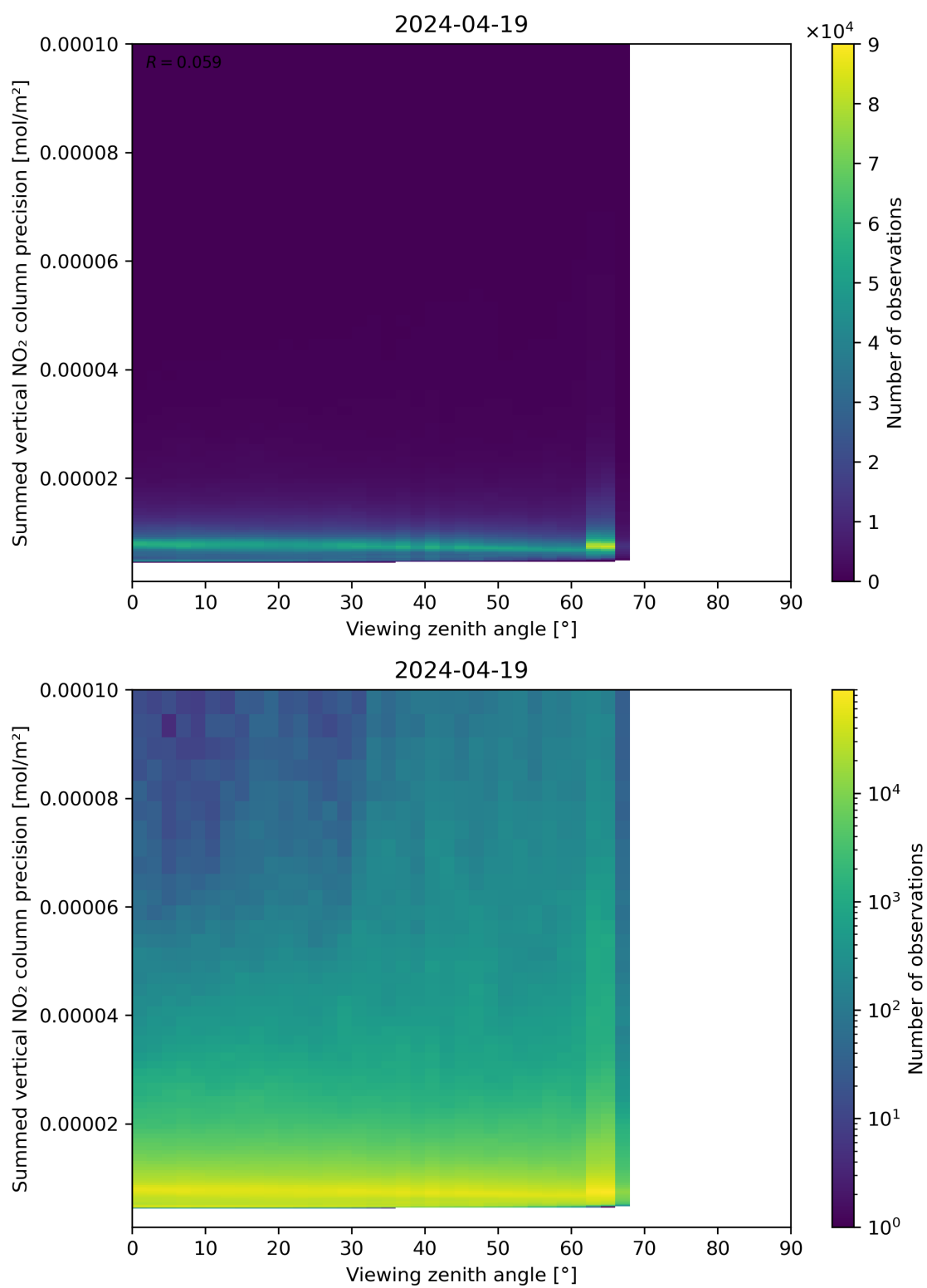
Figure 166: Scatter density plot of “Viewing zenith angle” against “Summed vertical NO 2 column precision” for 2024-04-18 to 2024-04-20.
