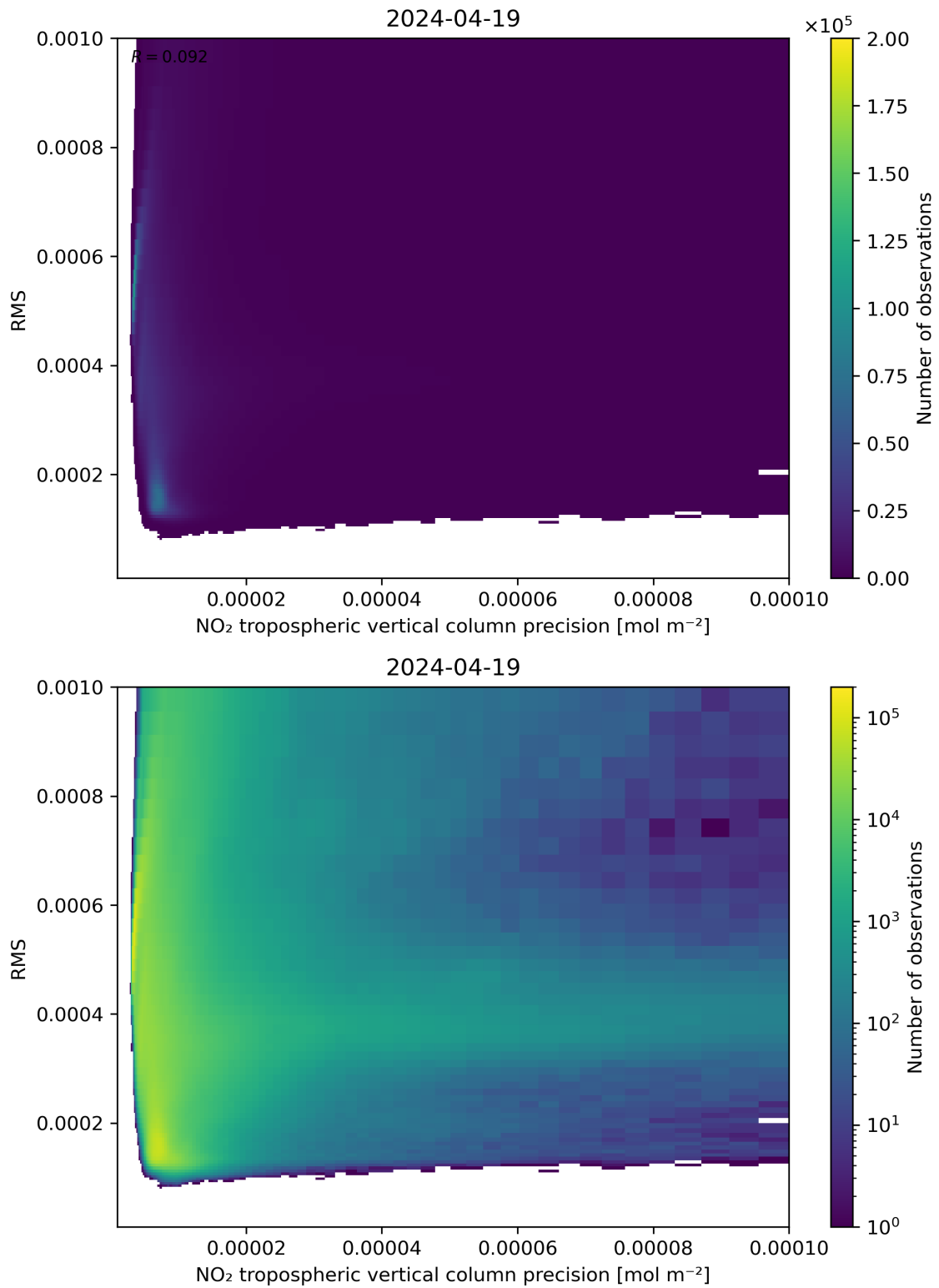
Figure 140: Scatter density plot of “NO 2 tropospheric vertical column precision” against “RMS” for 2024-04-18 to 2024-04-20.
