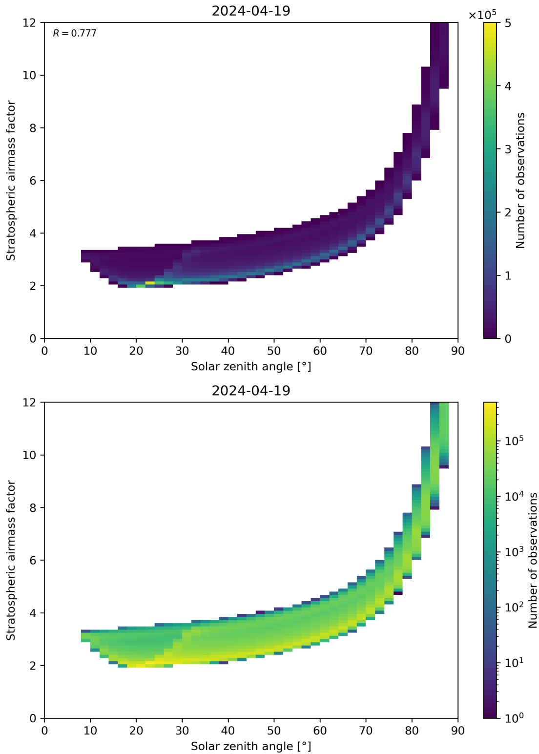
Figure 145: Scatter density plot of “Solar zenith angle” against “Stratospheric airmass factor” for 2024-04-18 to 2024-04-20.
