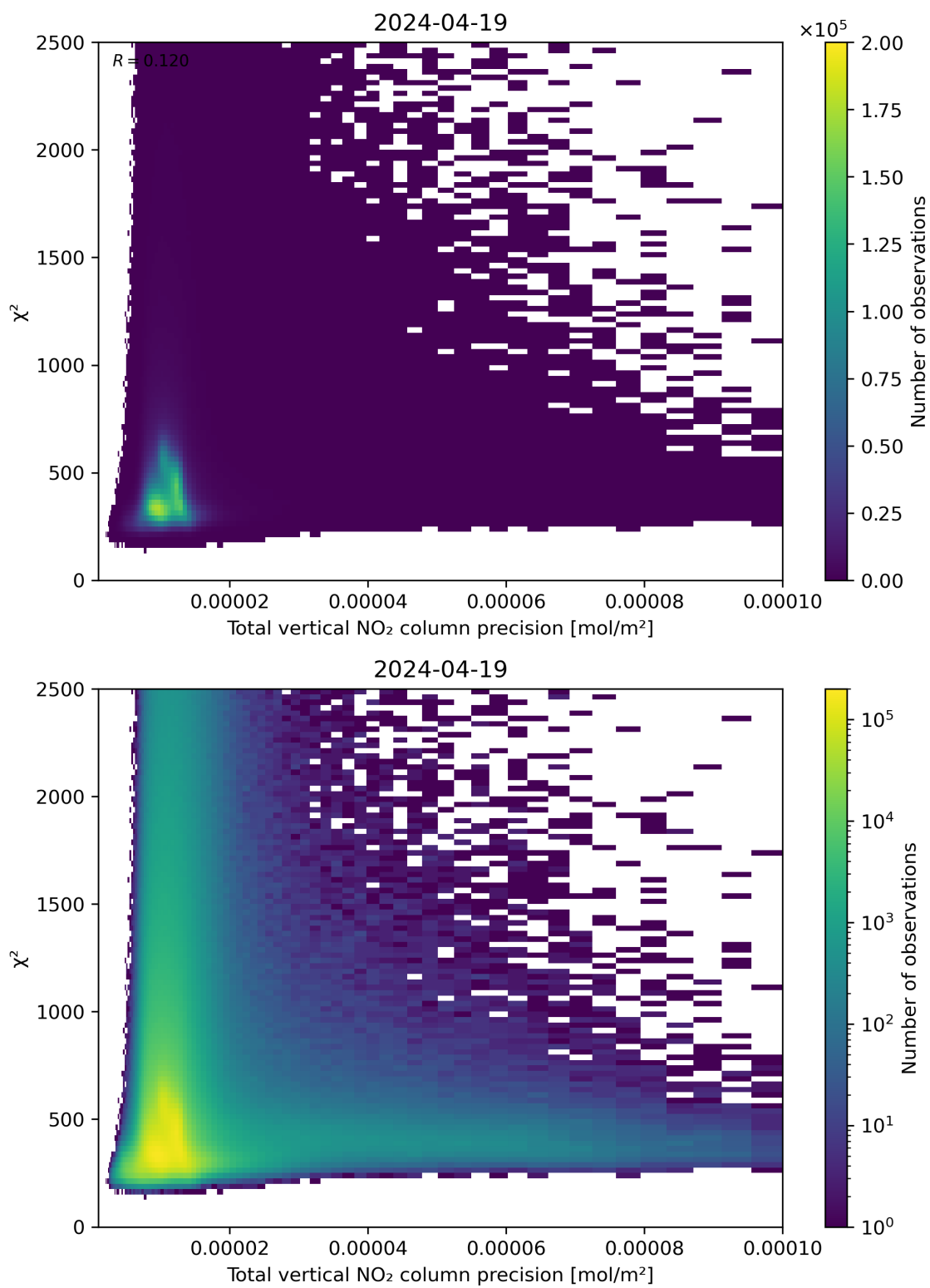
Figure 116: Scatter density plot of “Total vertical NO 2 column precision” against “ \chi^2 ” for 2024-04-18 to 2024-04-20.
