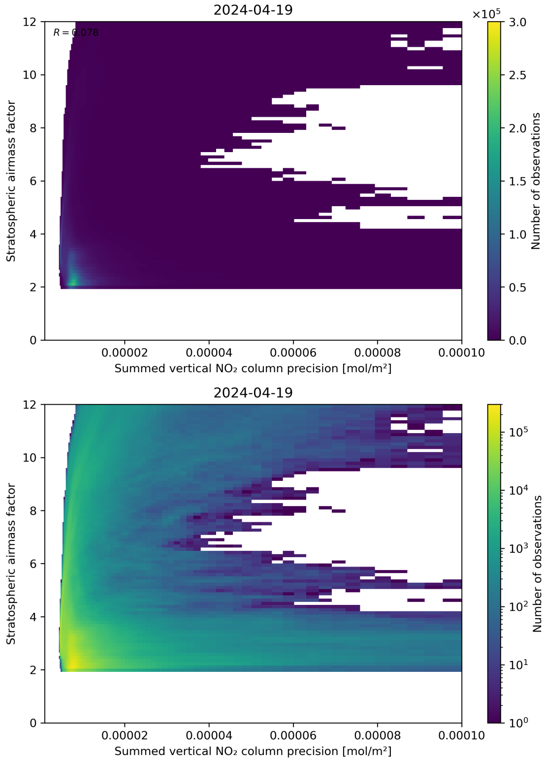
Figure 106: Scatter density plot of “Summed vertical NO 2 column precision” against “Stratospheric airmass factor” for 2024-04-18 to 2024-04-20.
