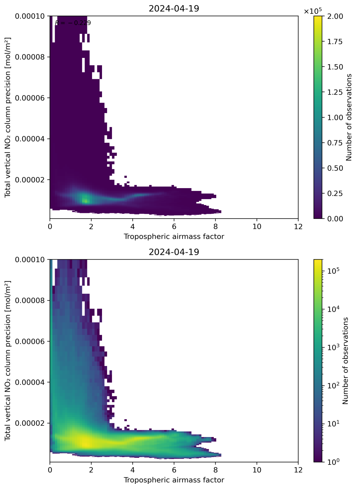
Figure 78: Scatter density plot of “Tropospheric air mass factor” against “Total vertical NO 2 column precision” for 2024-04-18 to 2024-04-20.
