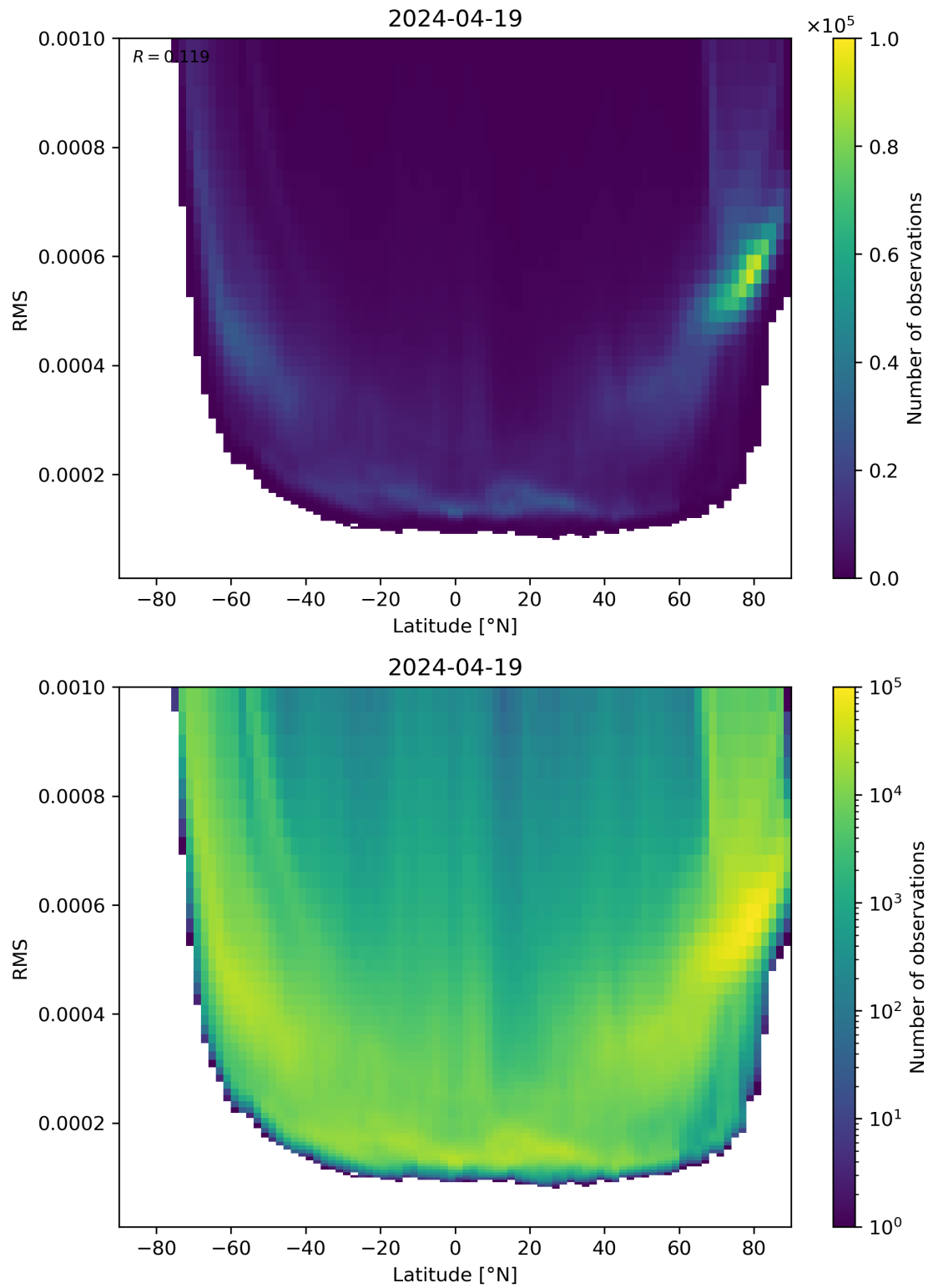
Figure 94: Scatter density plot of “Latitude” against “RMS” for 2024-04-18 to 2024-04-20.
