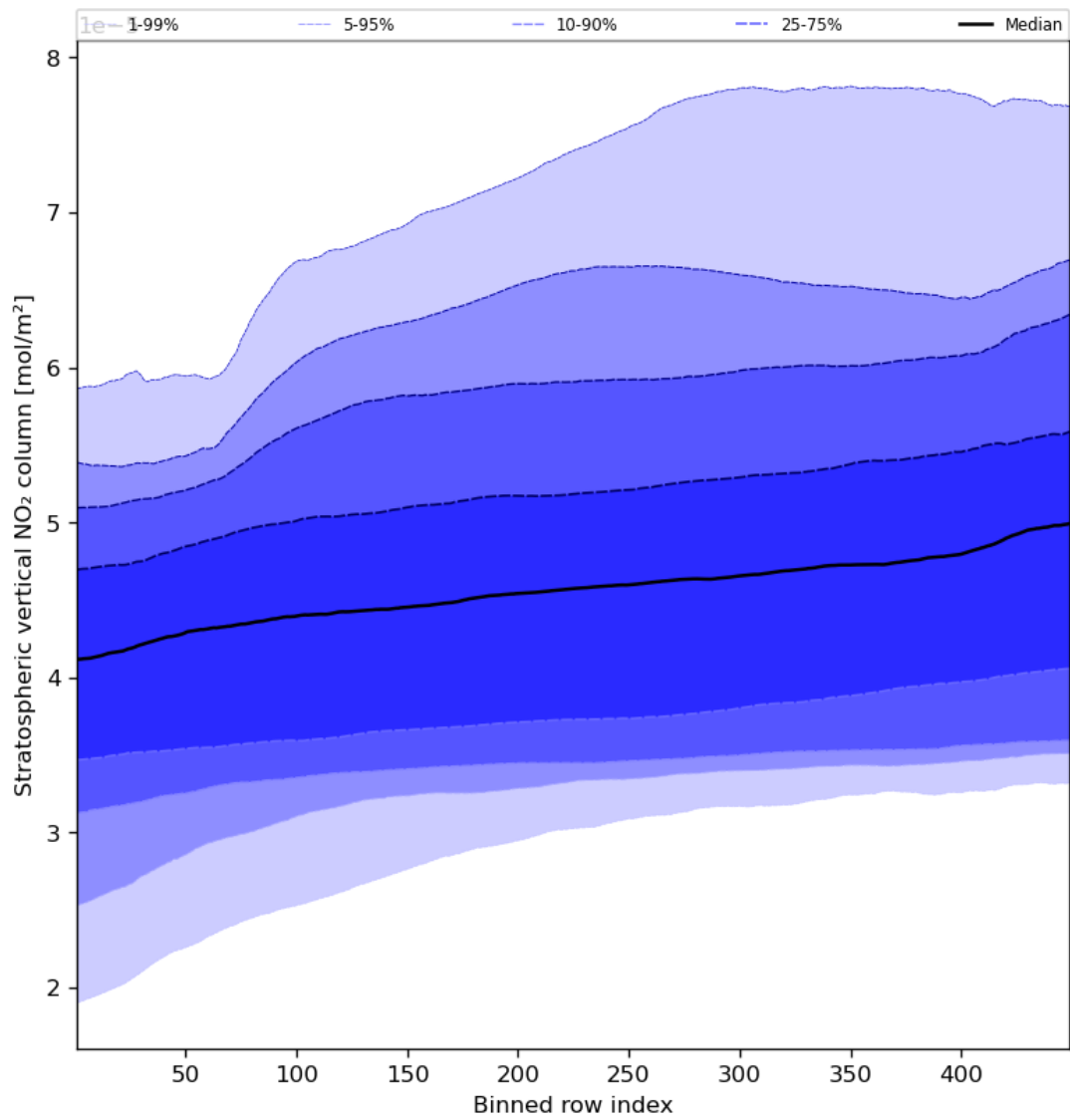
Figure 53: Along track statistics of “Stratospheric vertical NO 2 column” for 2024-04-18 to 2024-04-20
