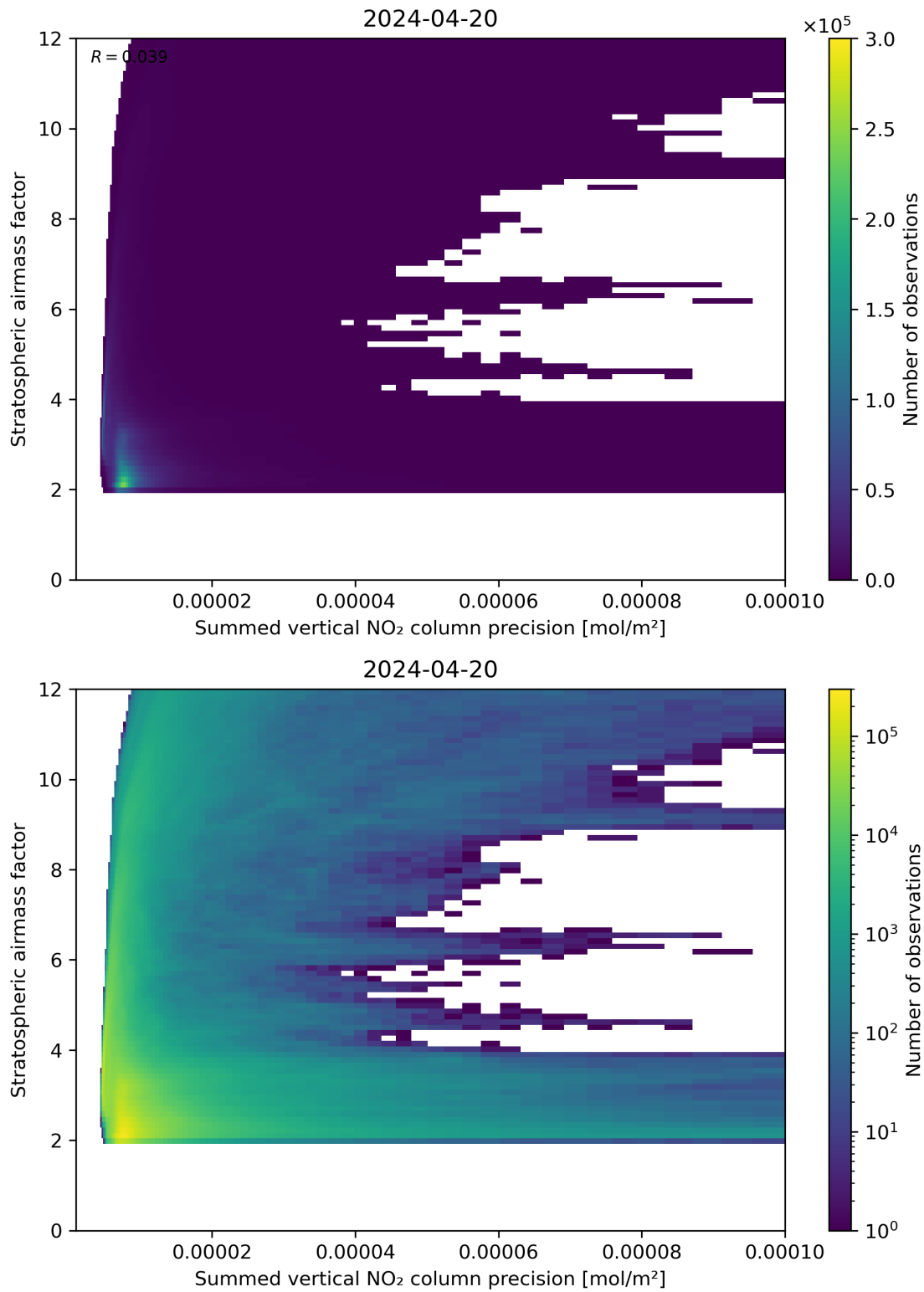
Figure 106: Scatter density plot of “Summed vertical NO 2 column precision” against “Stratospheric airmass factor” for 2024-04-19 to 2024-04-21.
