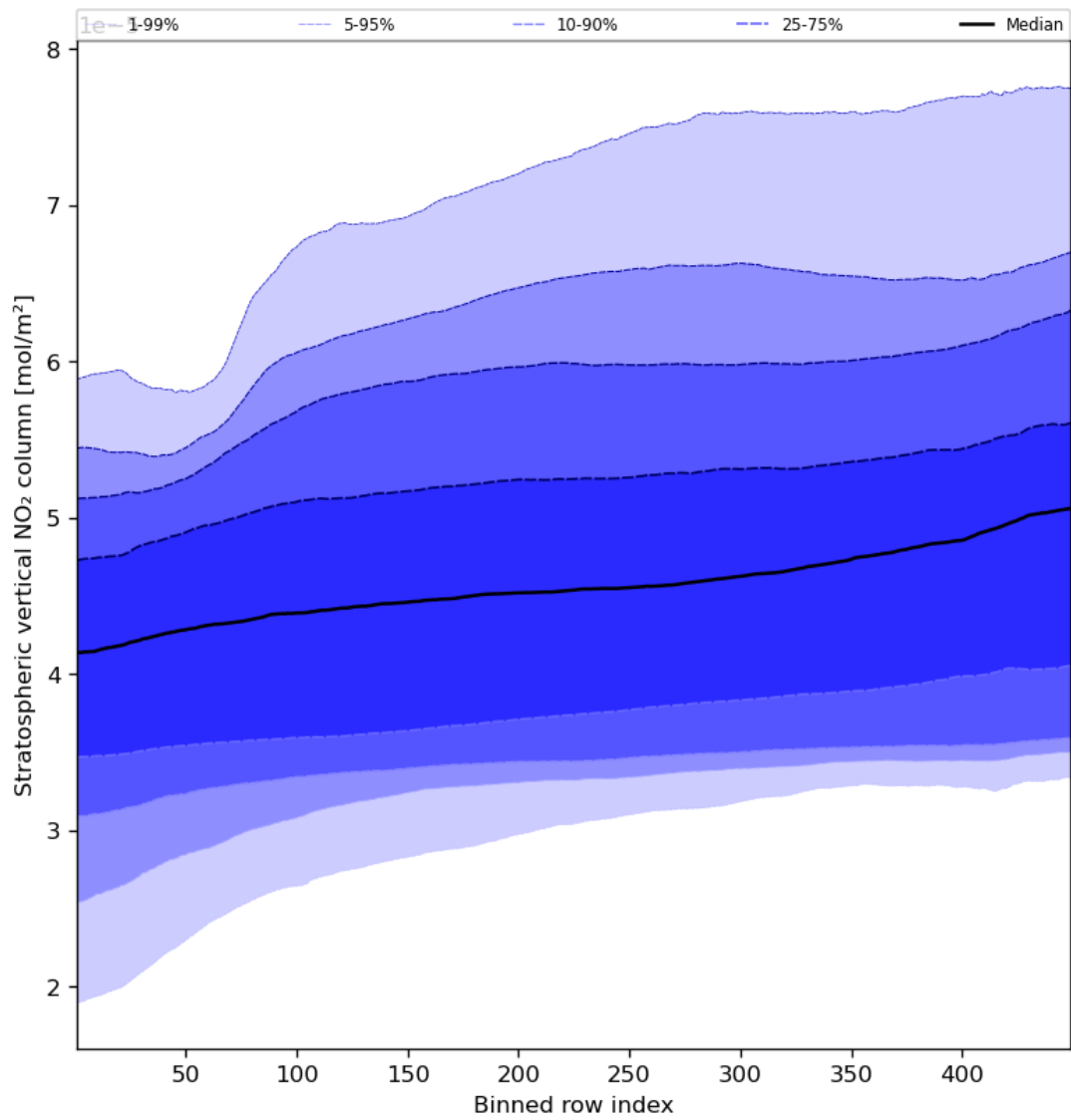
Figure 53: Along track statistics of “Stratospheric vertical NO 2 column” for 2024-04-19 to 2024-04-21
