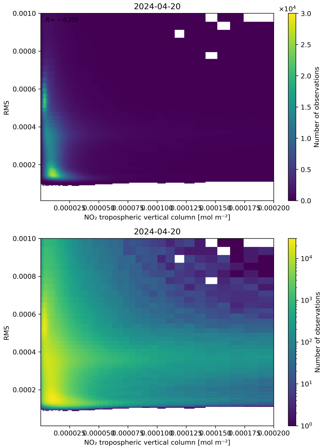
Figure 142: Scatter density plot of “NO 2 tropospheric vertical column” against “RMS” for 2024-04-19 to 2024-04-21.
