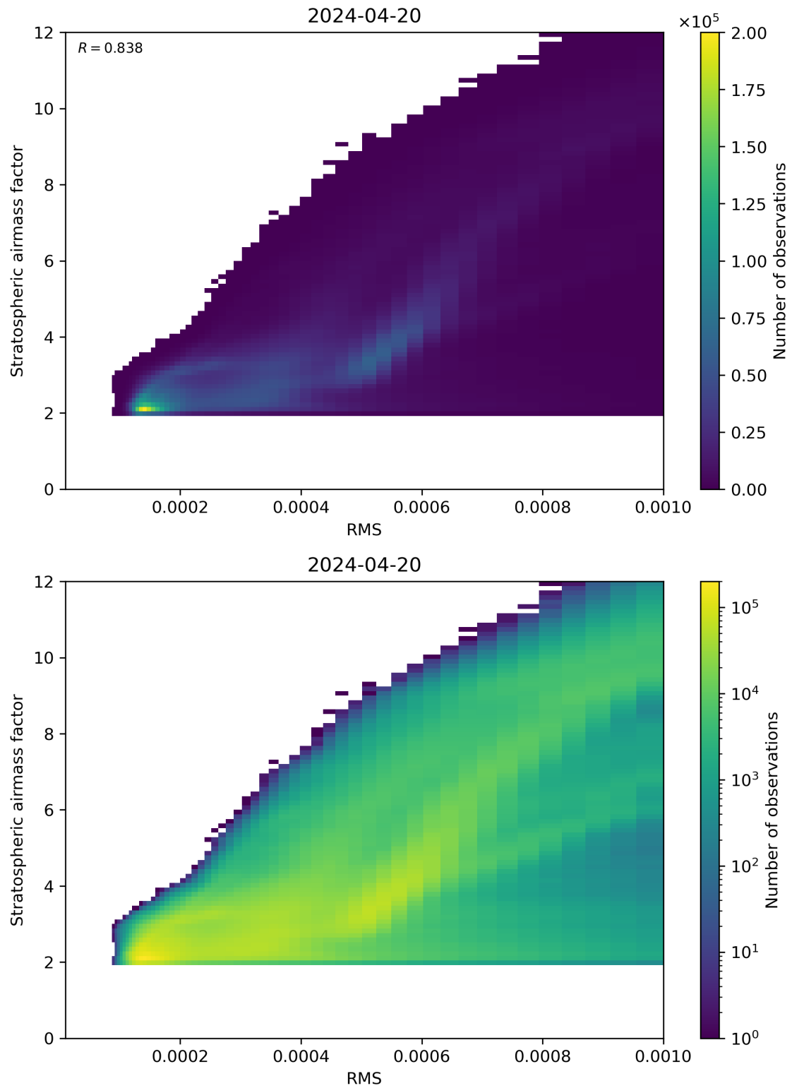
Figure 144: Scatter density plot of “RMS” against “Stratospheric airmass factor” for 2024-04-19 to 2024-04-21.
