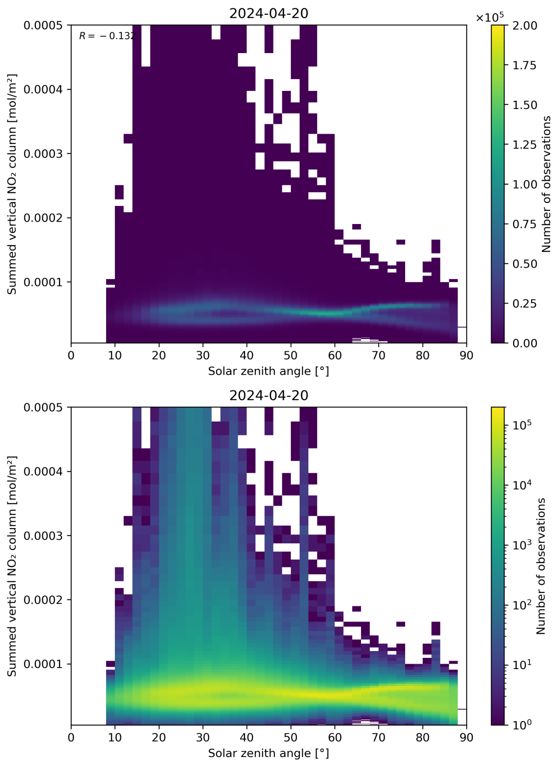
Figure 151: Scatter density plot of “Solar zenith angle” against “Summed vertical NO 2 column” for 2024-04-19 to 2024-04-21.
