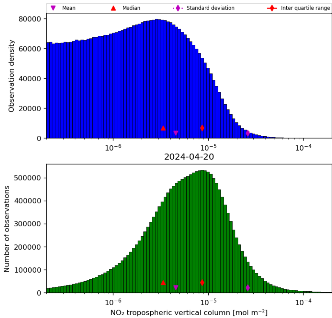
Figure 29: Histogram of “NO 2 tropospheric vertical column” for 2024-04-19 to 2024-04-21
