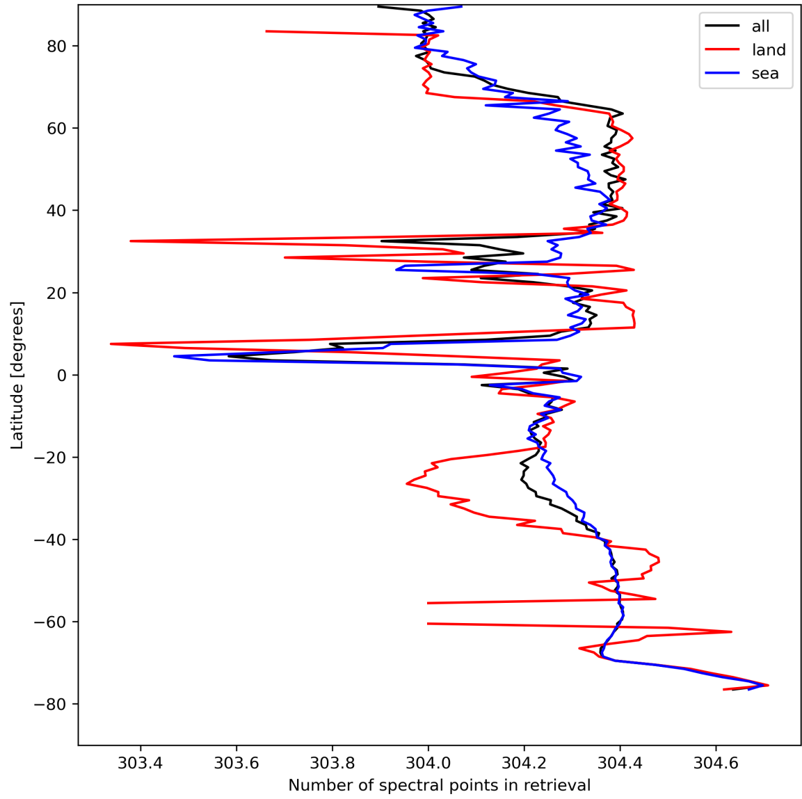
Figure 16: Zonal average of “Number of spectral points in retrieval” for 2024-04-19 to 2024-04-21.
