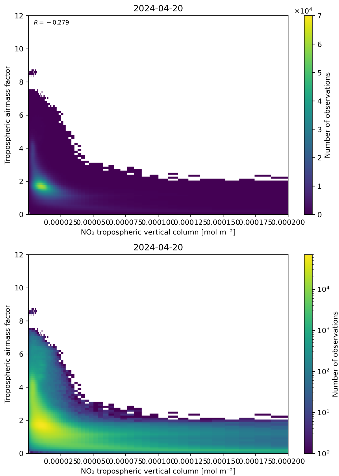
Figure 123: Scatter density plot of “NO 2 tropospheric vertical column” against “Tropospheric air mass factor” for 2024-04-19 to 2024-04-21.
