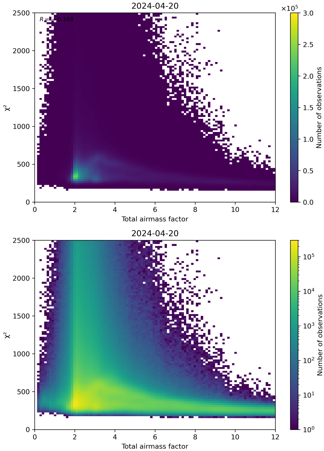
Figure 63: Scatter density plot of “Total airmass factor” against “ \chi^2 ” for 2024-04-19 to 2024-04-21.
