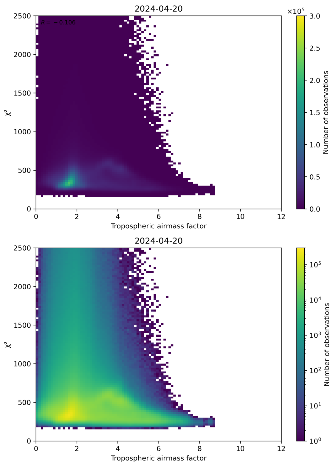
Figure 73: Scatter density plot of “Tropospheric airmass factor” against “ \chi^2 ” for 2024-04-19 to 2024-04-21.
