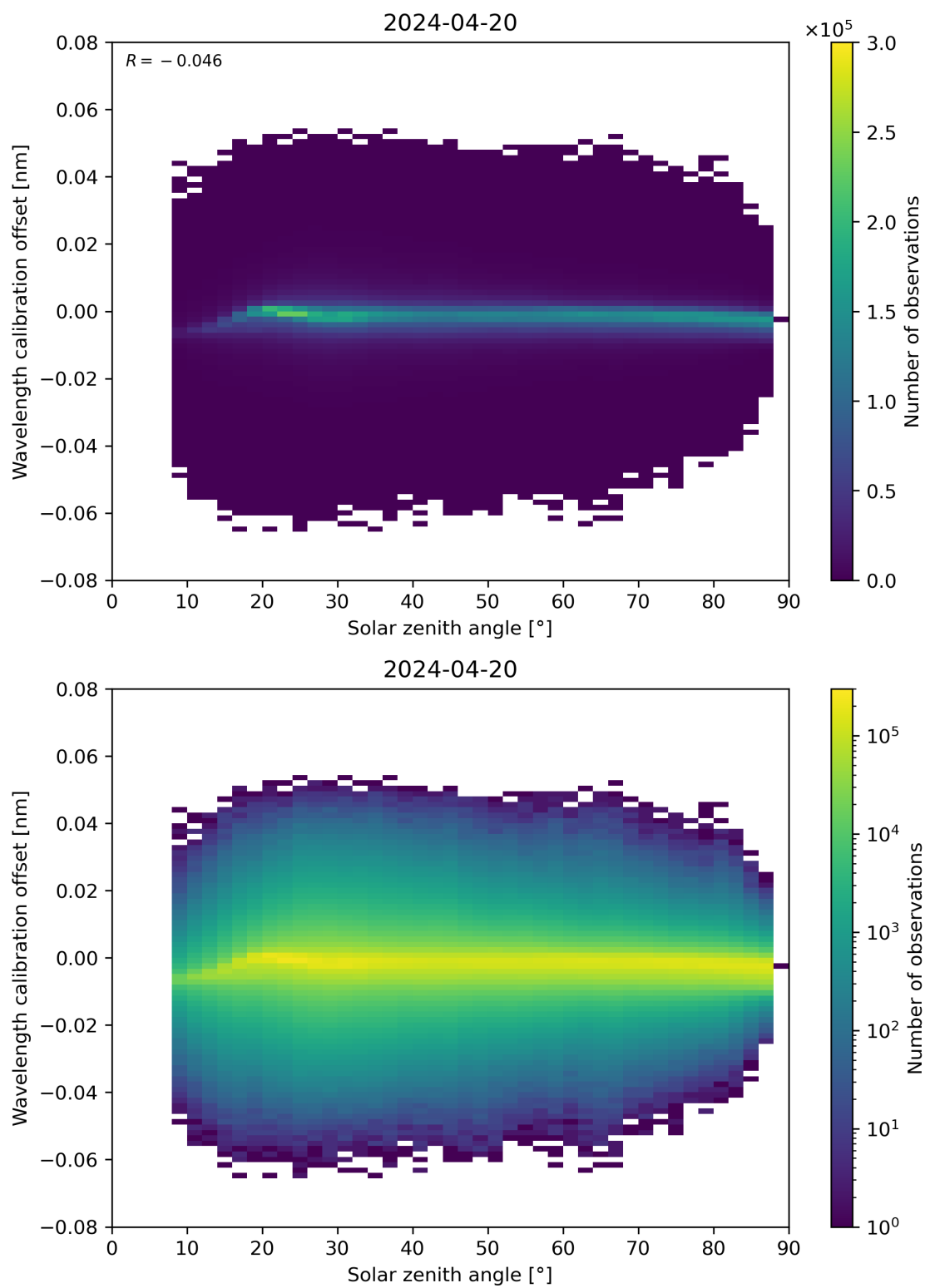
Figure 158: Scatter density plot of “Solar zenith angle” against “Wavelength calibration offset” for 2024-04-19 to 2024-04-21.
