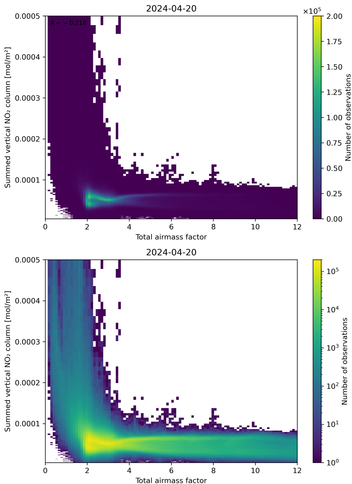
Figure 65: Scatter density plot of “Total airmass factor” against “Summed vertical NO 2 column” for 2024-04-19 to 2024-04-21.
