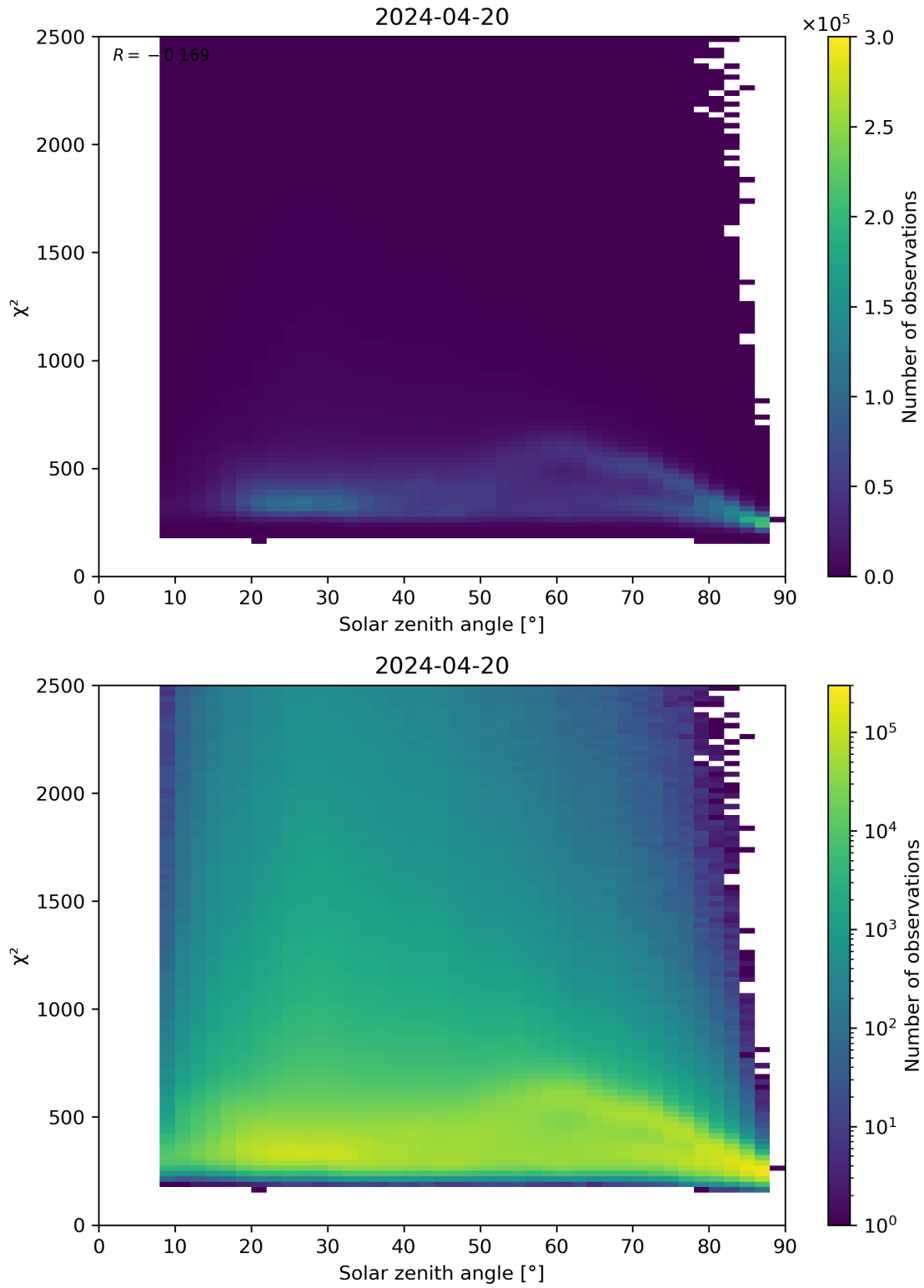
Figure 148: Scatter density plot of “Solar zenith angle” against “ \chi^2 ” for 2024-04-19 to 2024-04-21.
