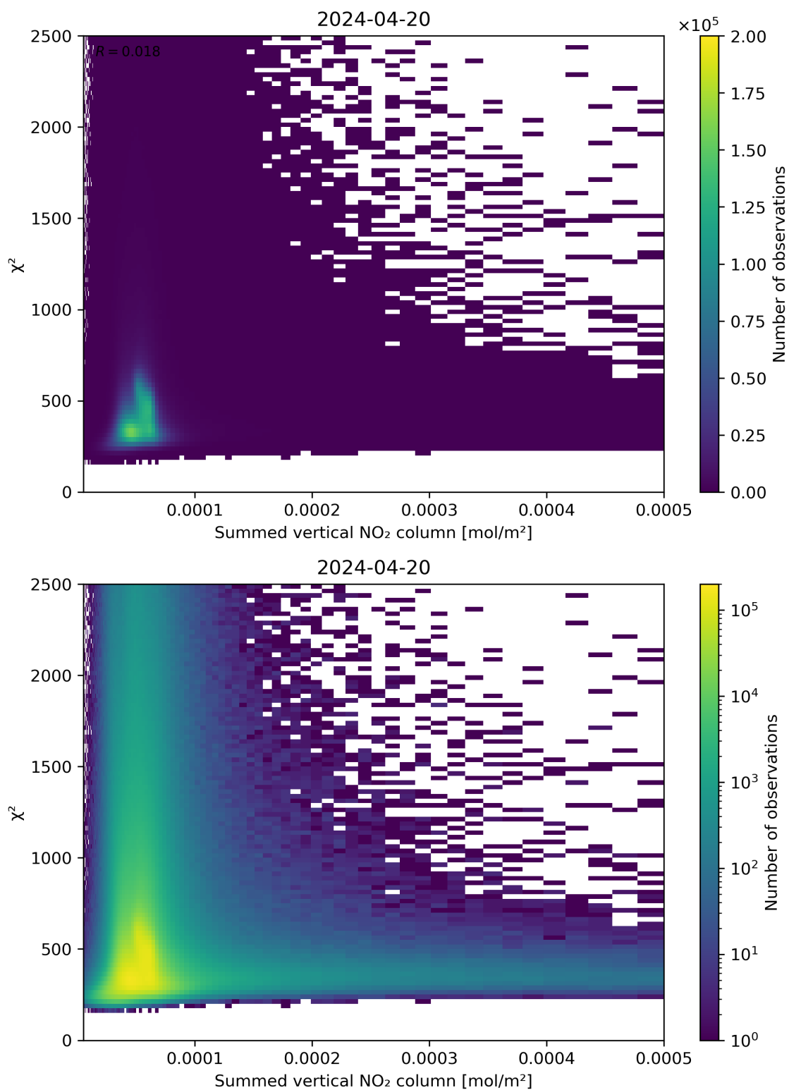
Figure 104: Scatter density plot of “Summed vertical NO 2 column” against “ \chi^2 ” for 2024-04-19 to 2024-04-21.
