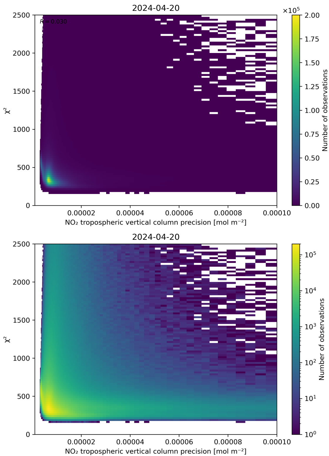
Figure 134: Scatter density plot of “NO 2 tropospheric vertical column precision” against “ \chi^2 ” for 2024-04-19 to 2024-04-21.
