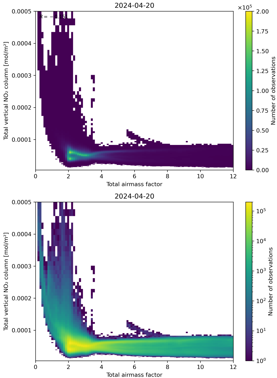
Figure 67: Scatter density plot of “Total airmass factor” against “Total vertical NO 2 column” for 2024-04-19 to 2024-04-21.
