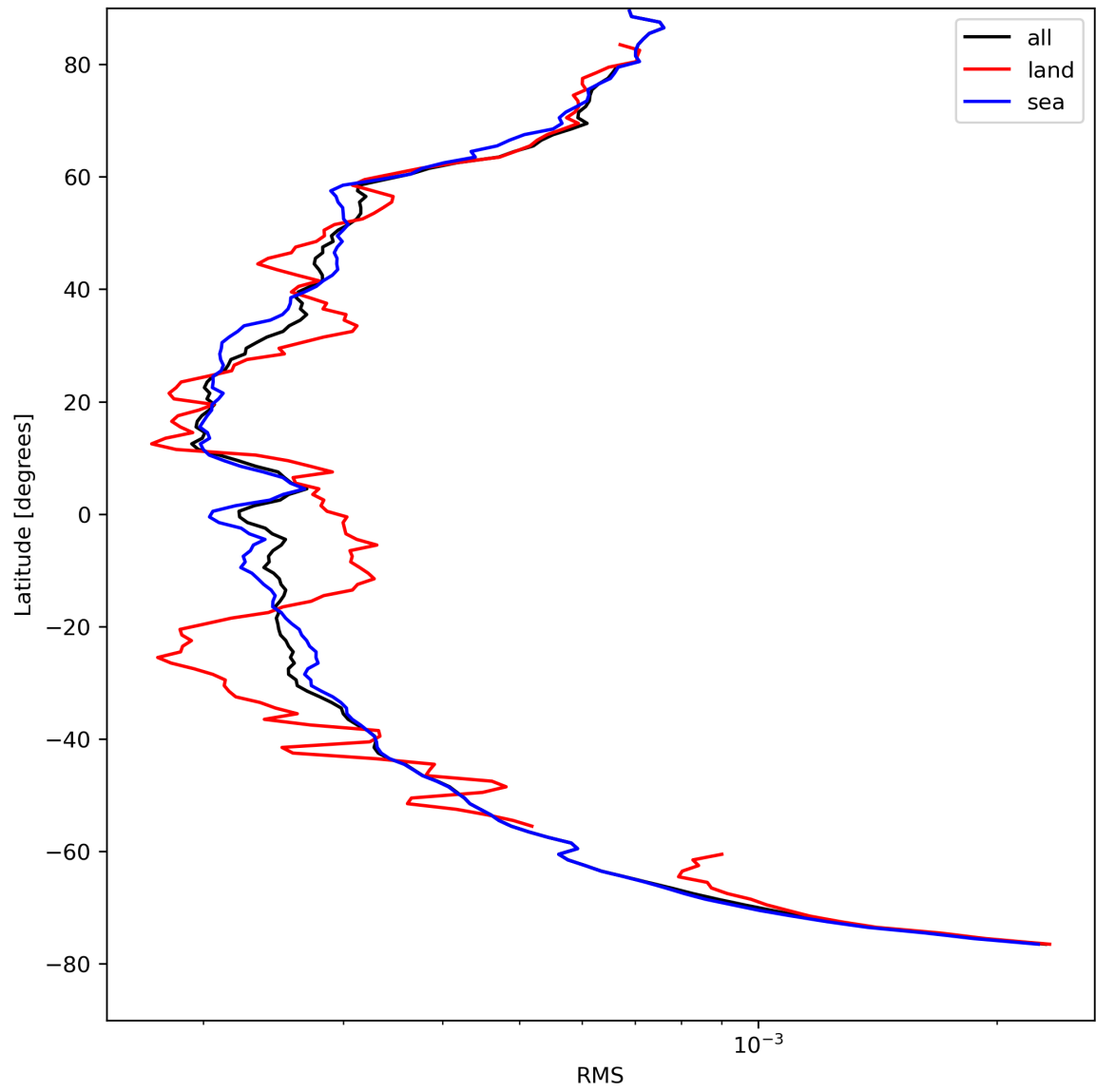
Figure 26: Zonal average of “RMS” for 2024-04-19 to 2024-04-21.
