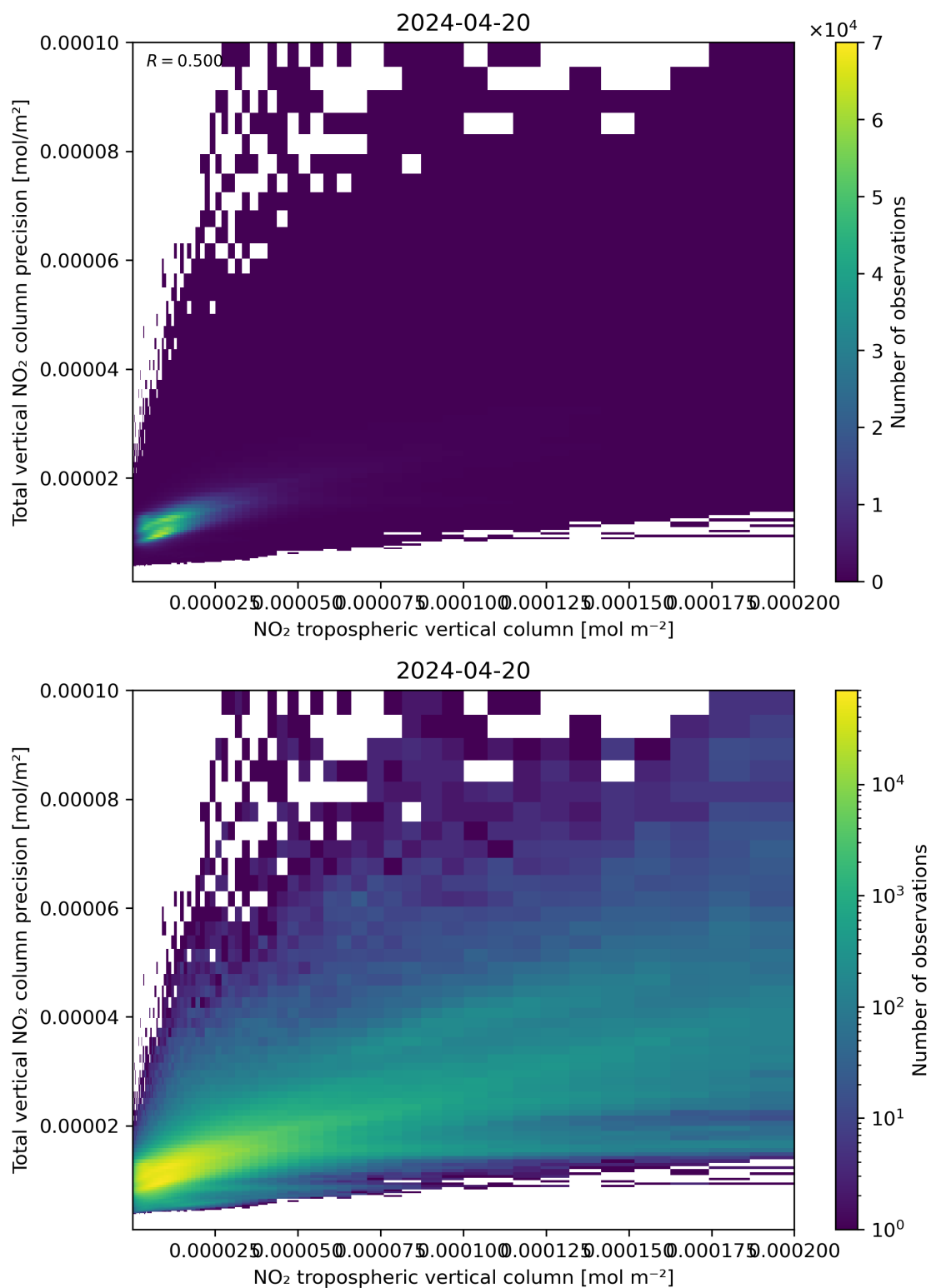
Figure 129: Scatter density plot of “NO 2 tropospheric vertical column” against “Total vertical NO 2 column precision” for 2024-04-19 to 2024-04-21.
