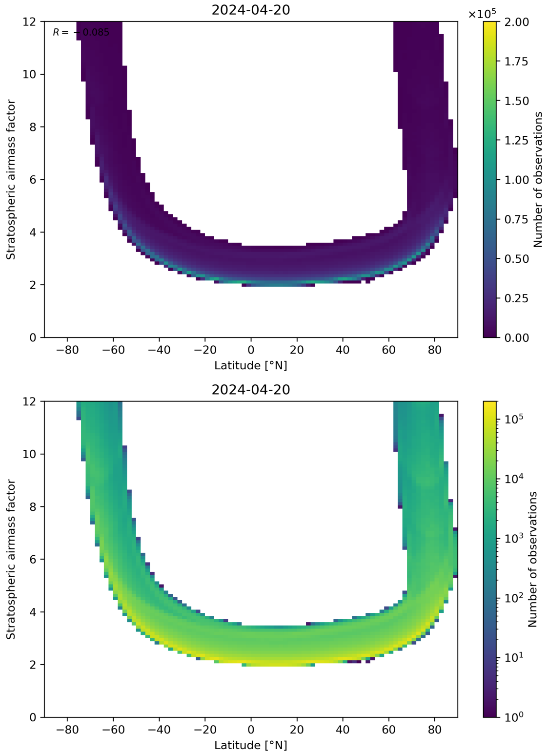
Figure 83: Scatter density plot of “Latitude” against “Stratospheric air mass factor” for 2024-04-19 to 2024-04-21.
