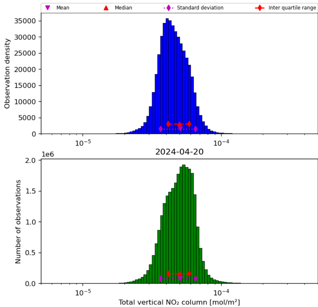
Figure 38: Histogram of “Total vertical NO 2 column” for 2024-04-19 to 2024-04-21
