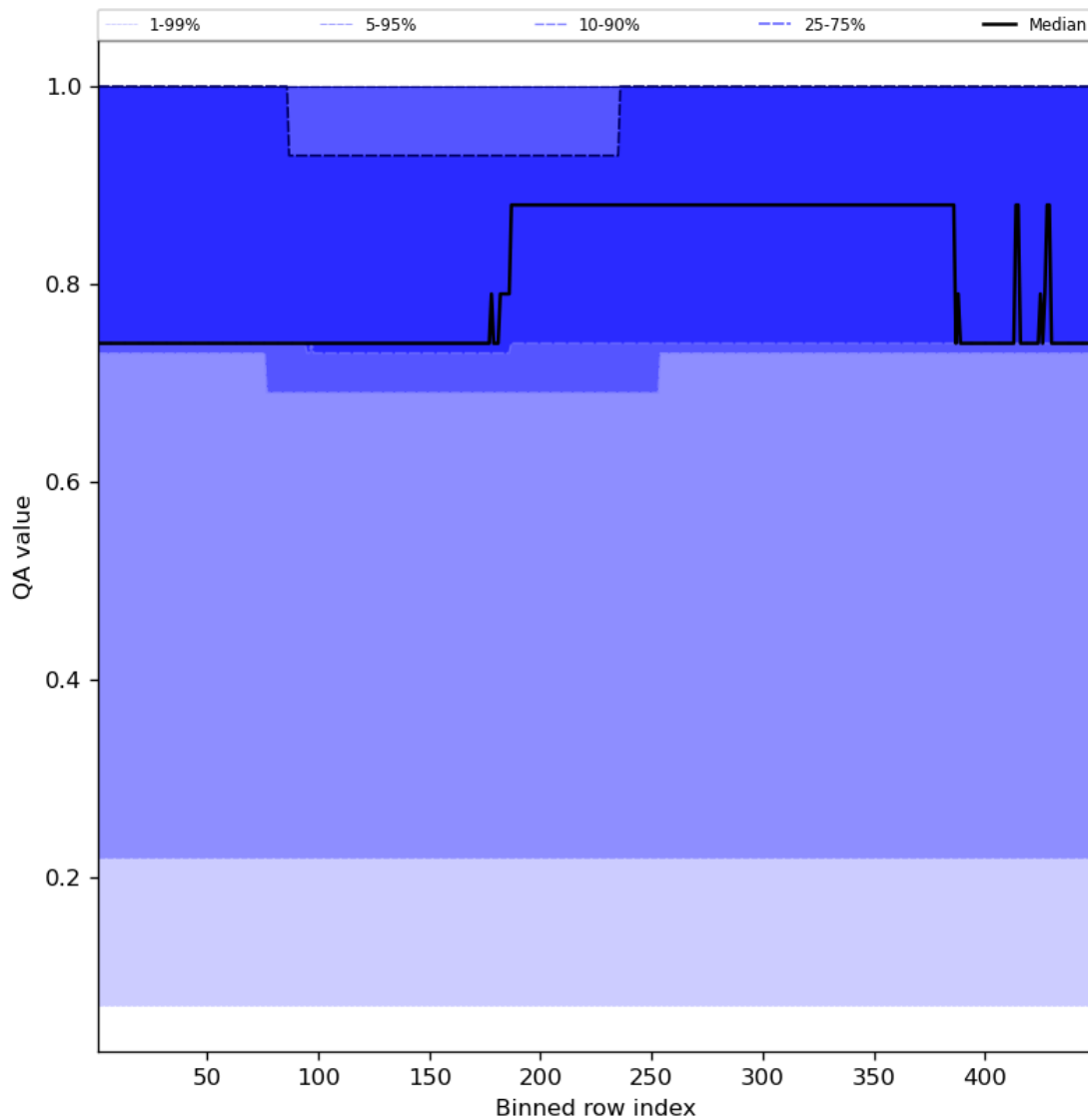
Figure 45: Along track statistics of “QA value” for 2024-04-19 to 2024-04-21
