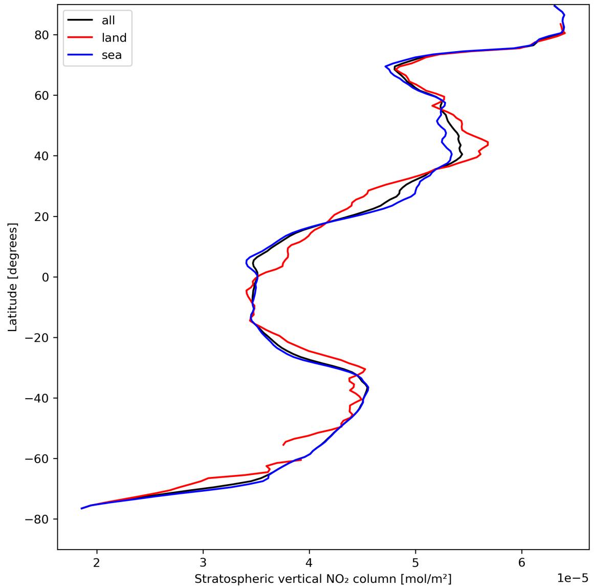
Figure 19: Zonal average of “Stratospheric vertical NO 2 column” for 2024-04-19 to 2024-04-21.
