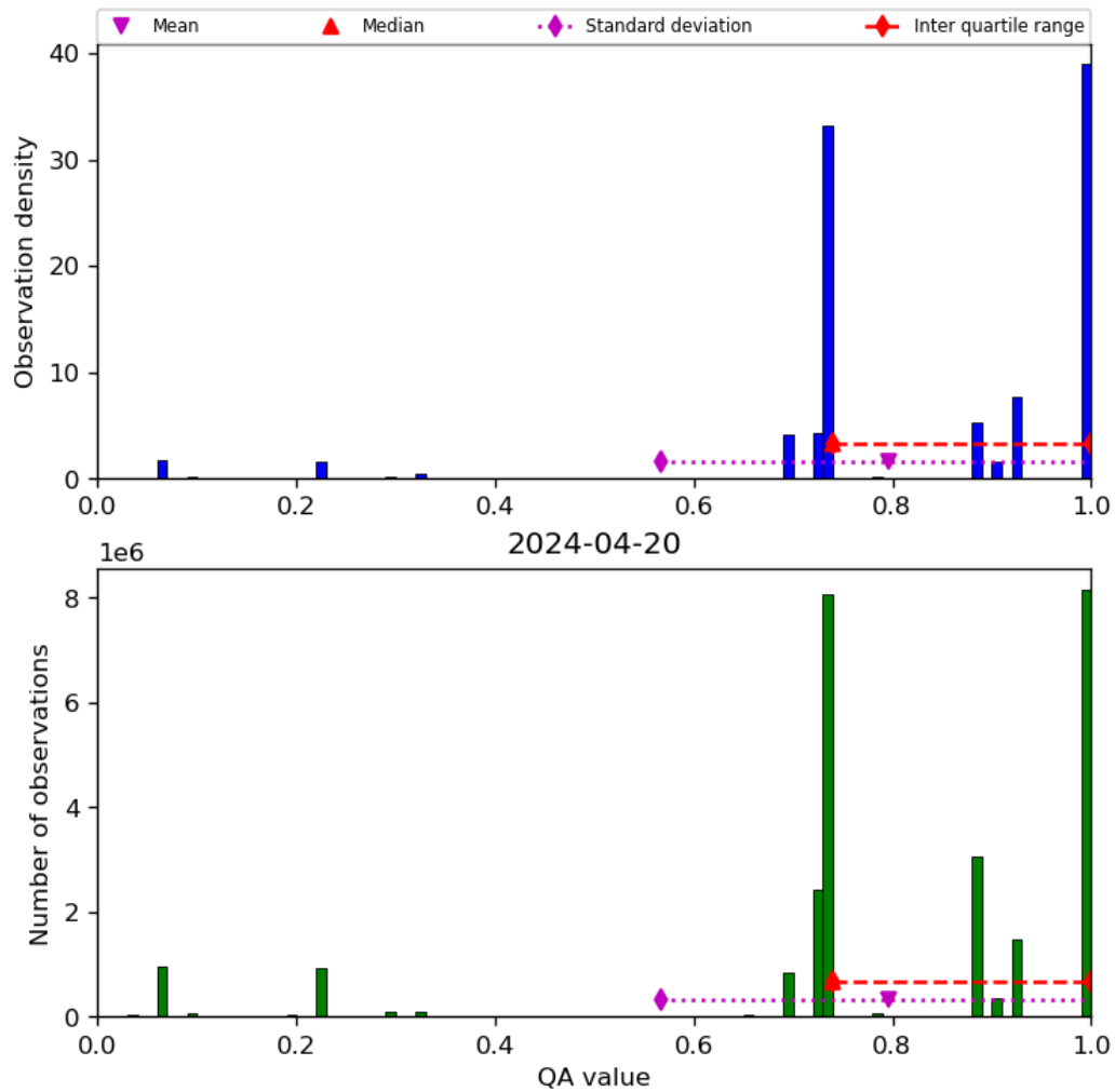
Figure 28: Histogram of “QA value” for 2024-04-19 to 2024-04-21
