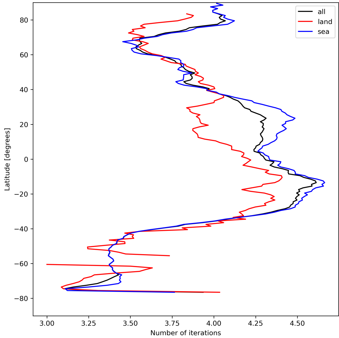
Figure 17: Zonal average of “Number of iterations” for 2024-04-19 to 2024-04-21.
