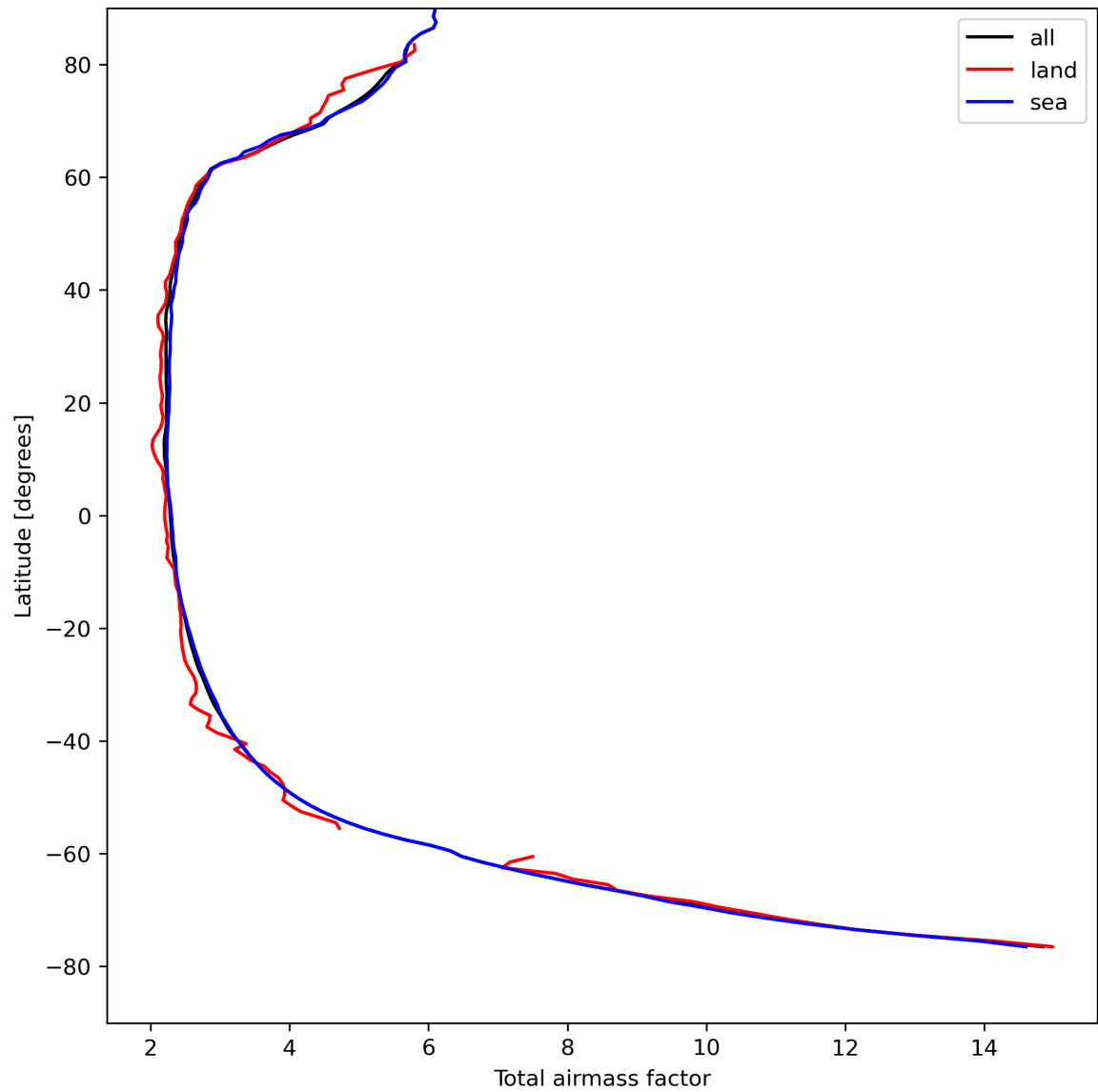
Figure 15: Zonal average of “Total airmass factor” for 2024-04-19 to 2024-04-21.
