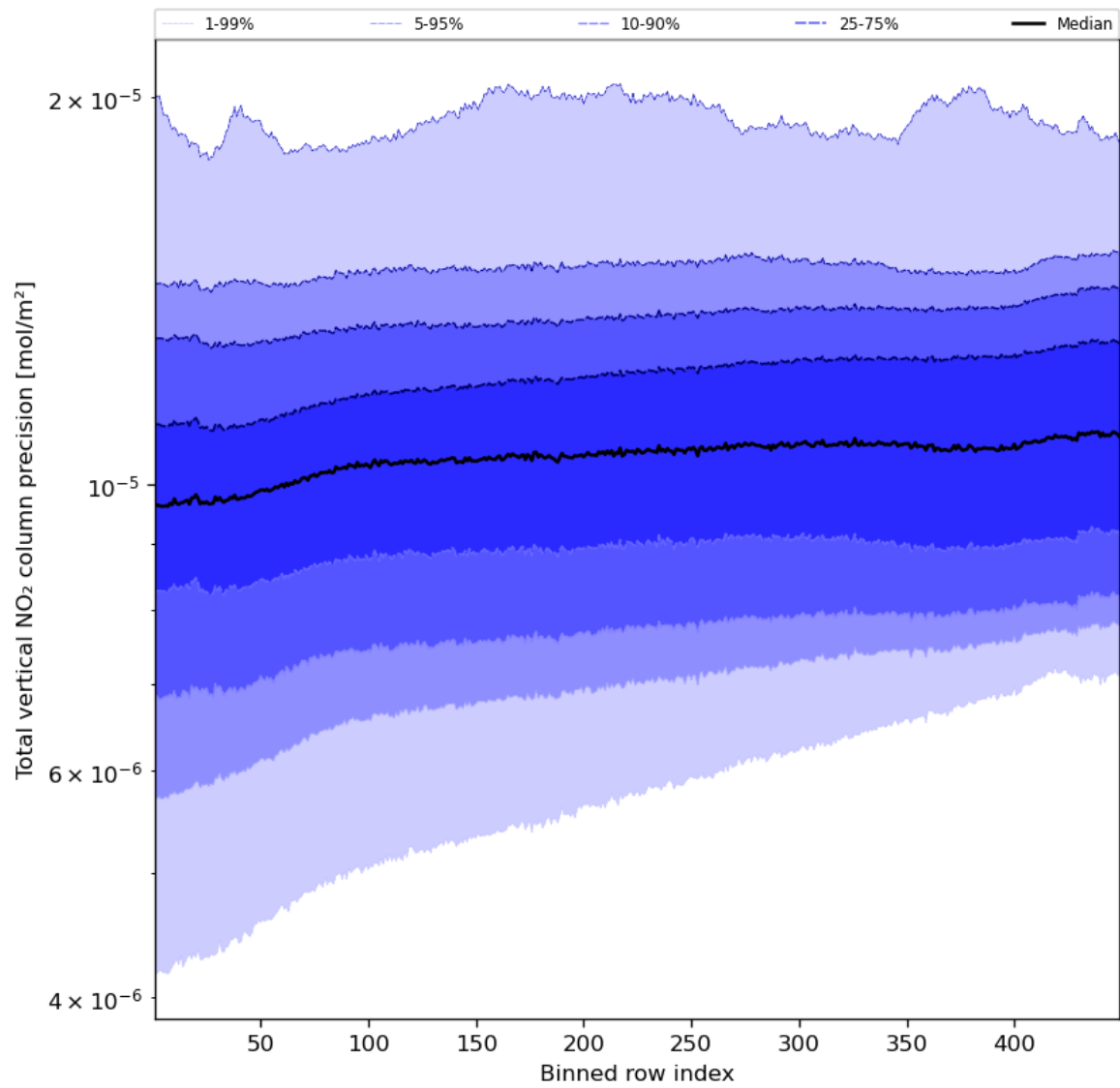
Figure 56: Along track statistics of “Total vertical NO 2 column precision” for 2024-04-19 to 2024-04-21
