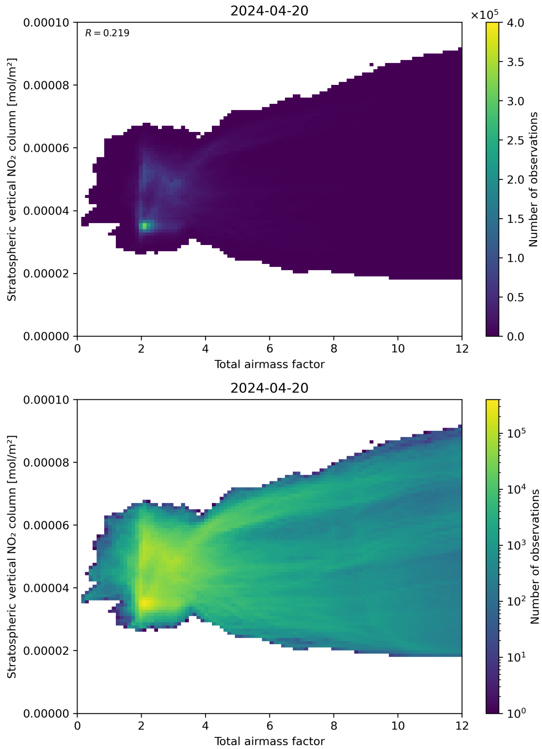
Figure 64: Scatter density plot of “Total airmass factor” against “Stratospheric vertical NO 2 column” for 2024-04-19 to 2024-04-21.
