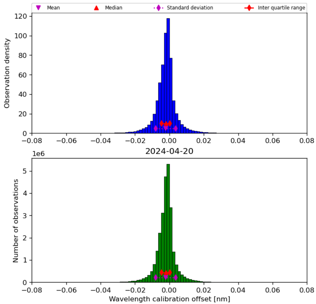
Figure 35: Histogram of “Wavelength calibration offset” for 2024-04-19 to 2024-04-21
