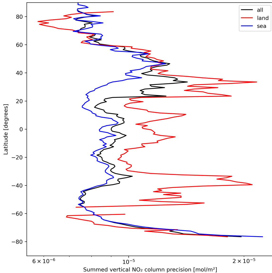
Figure 24: Zonal average of “Summed vertical NO 2 column precision” for 2024-04-19 to 2024-04-21.
