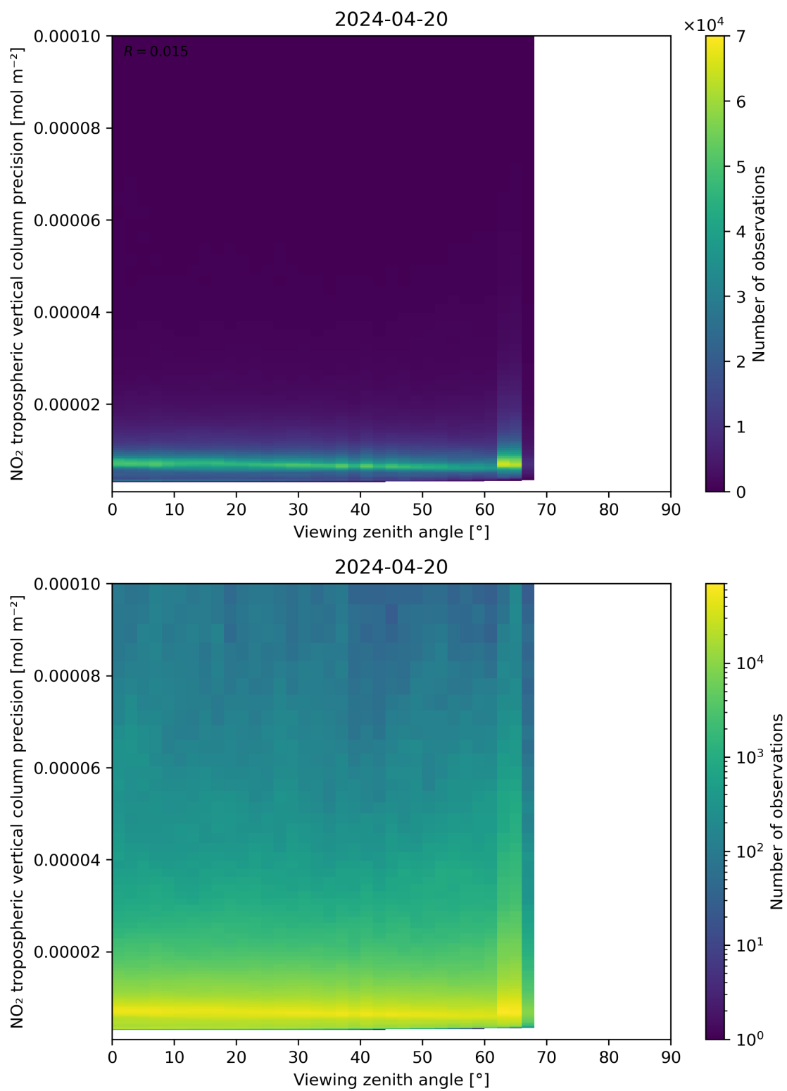
Figure 170: Scatter density plot of “Viewing zenith angle” against “NO 2 tropospheric vertical column precision” for 2024-04-19 to 2024-04-21.
