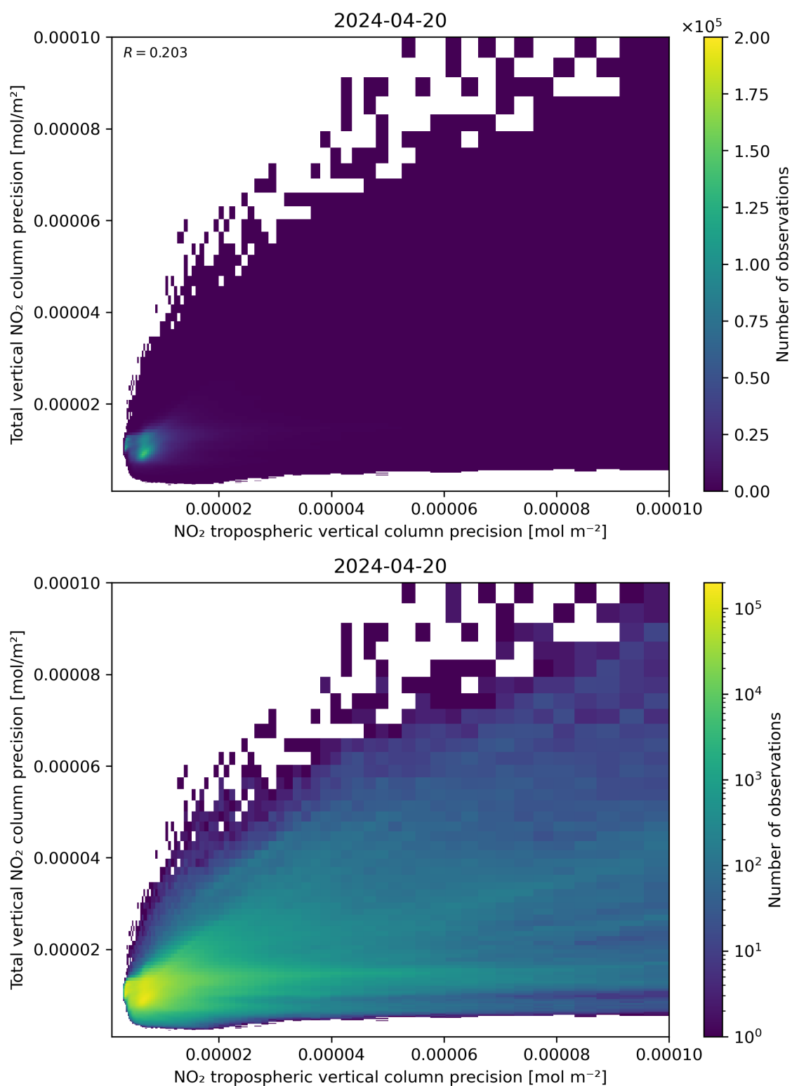
Figure 139: Scatter density plot of “NO 2 tropospheric vertical column precision” against “Total vertical NO 2 column precision” for 2024-04-19 to 2024-04-21.
