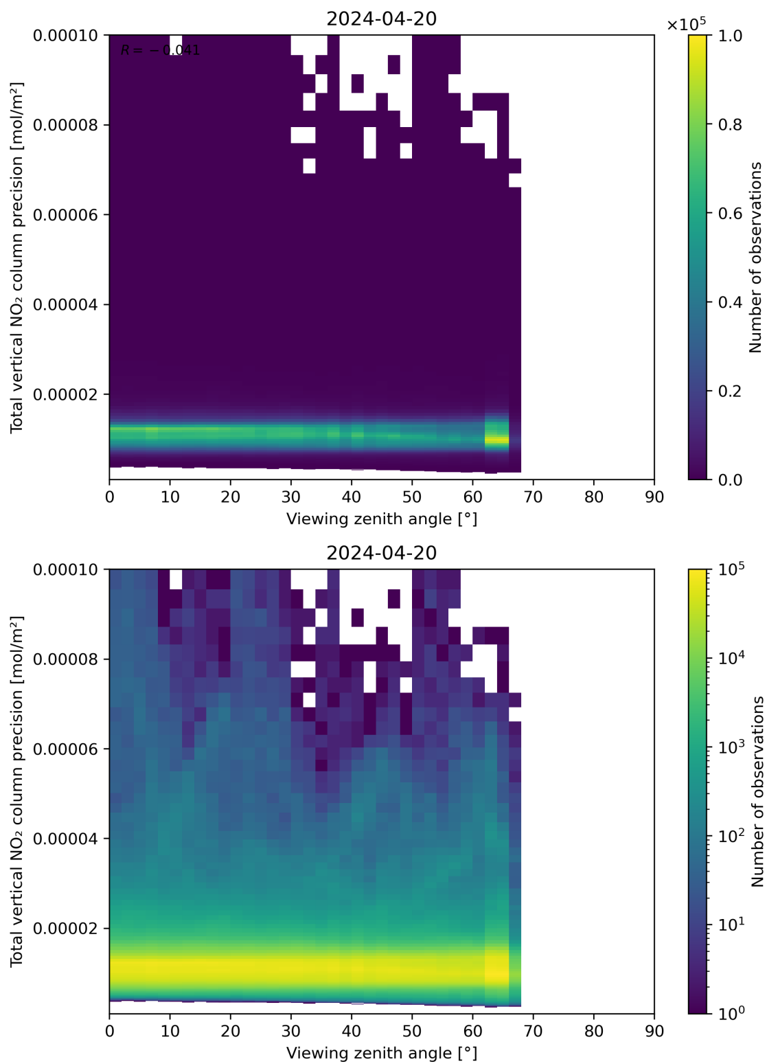
Figure 168: Scatter density plot of “Viewing zenith angle” against “Total vertical NO 2 column precision” for 2024-04-19 to 2024-04-21.
