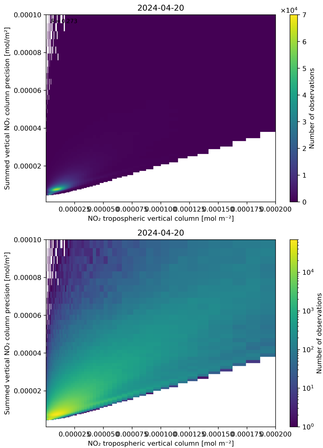
Figure 127: Scatter density plot of “NO 2 tropospheric vertical column” against “Summed vertical NO 2 column precision” for 2024-04-19 to 2024-04-21.
