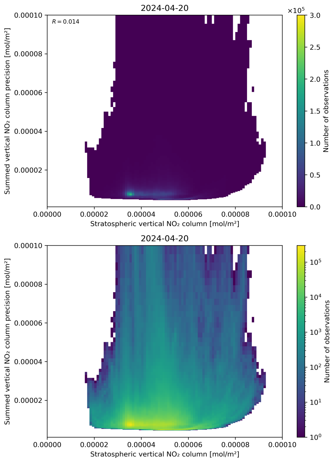
Figure 99: Scatter density plot of “Stratospheric vertical NO 2 column” against “Summed vertical NO 2 column precision” for 2024-04-19 to 2024-04-21.
