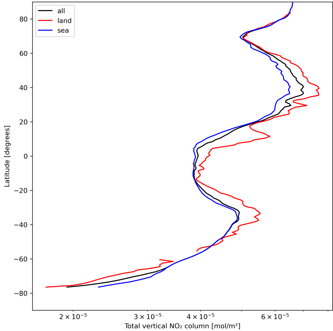
Figure 21: Zonal average of “Total vertical NO 2 column” for 2024-04-19 to 2024-04-21.
