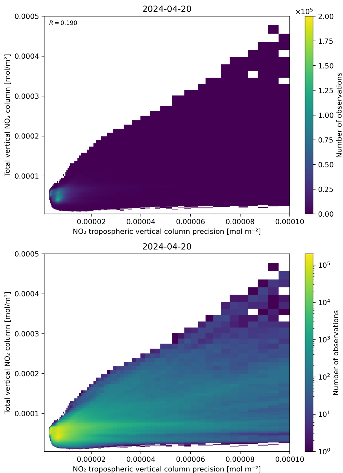
Figure 138: Scatter density plot of “NO 2 tropospheric vertical column precision” against “Total vertical NO 2 column” for 2024-04-19 to 2024-04-21.
