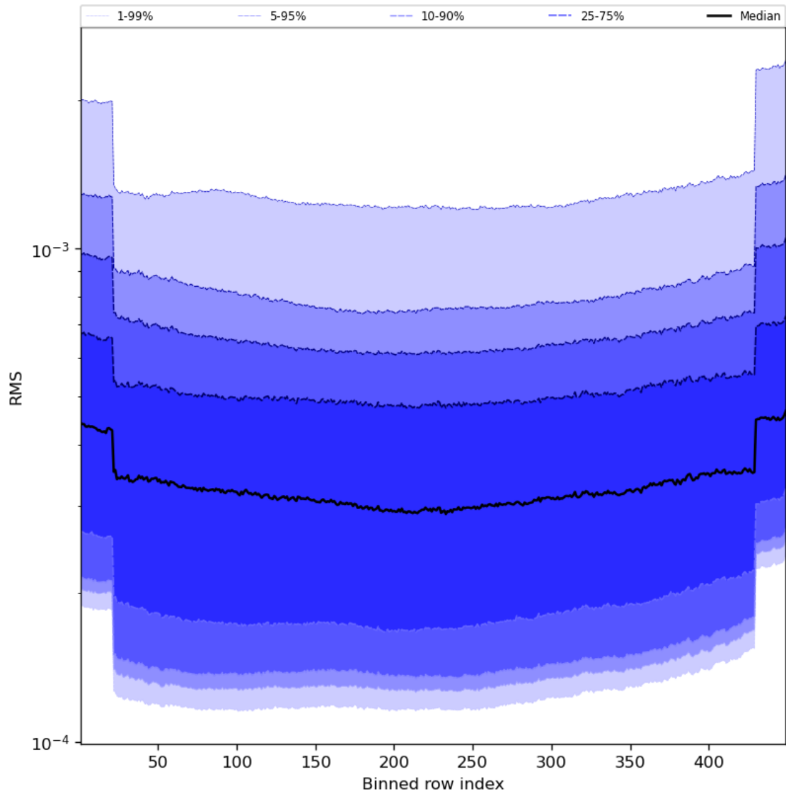
Figure 60: Along track statistics of “RMS” for 2024-04-19 to 2024-04-21
