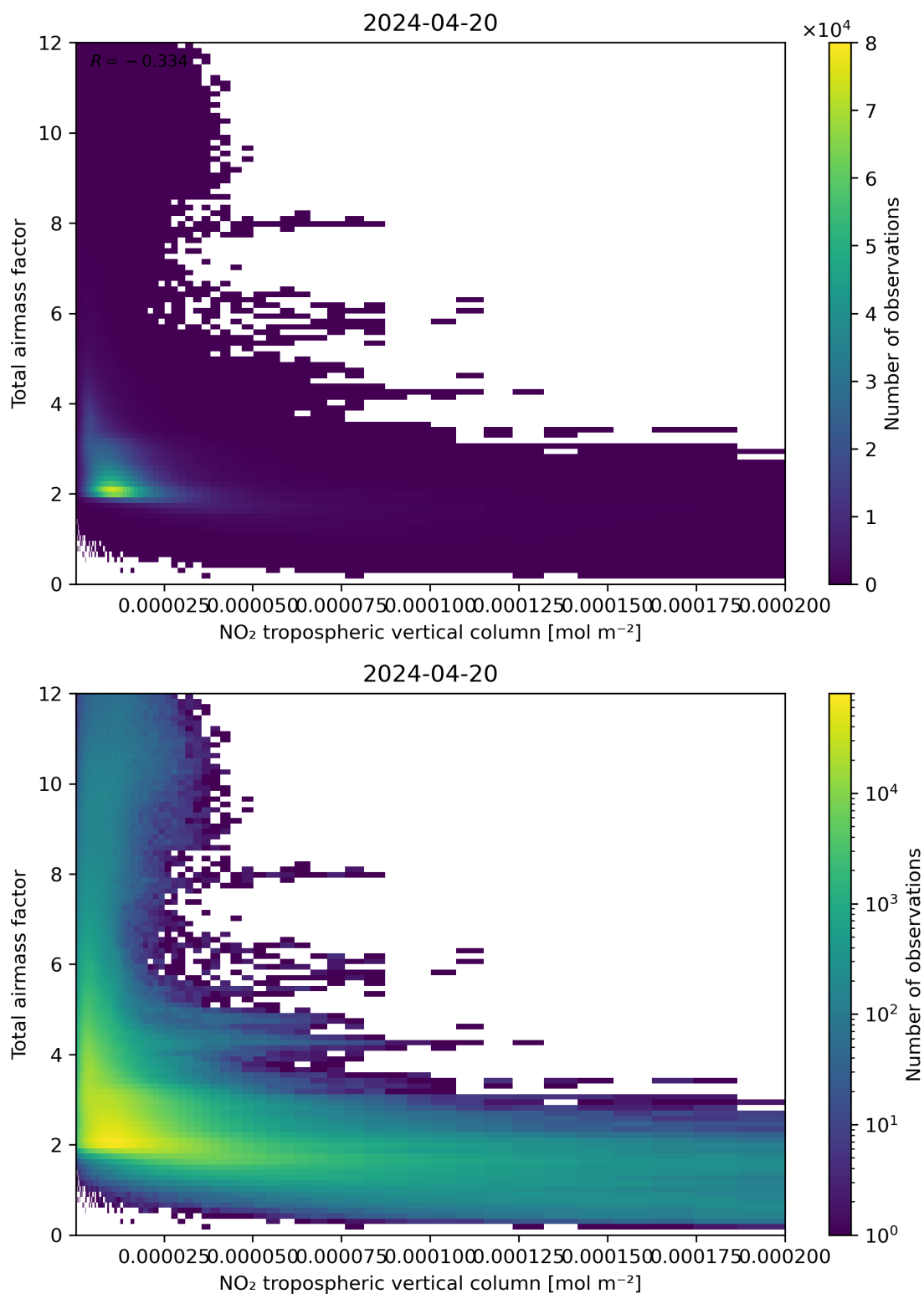
Figure 122: Scatter density plot of “NO 2 tropospheric vertical column” against “Total air mass factor” for 2024-04-19 to 2024-04-21.
