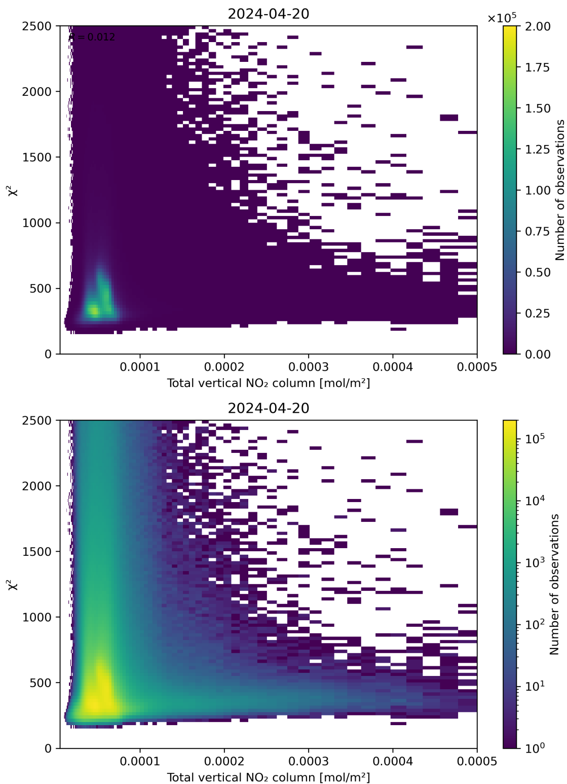
Figure 111: Scatter density plot of “Total vertical NO 2 column” against “ \chi^2 ” for 2024-04-19 to 2024-04-21.
