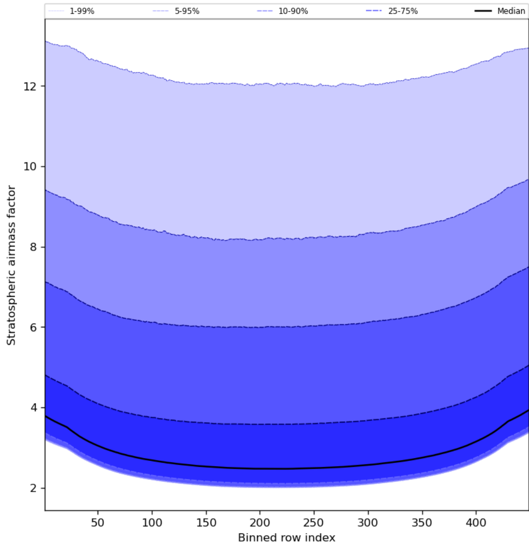
Figure 61: Along track statistics of “Stratospheric airmass factor” for 2024-04-19 to 2024-04-21
