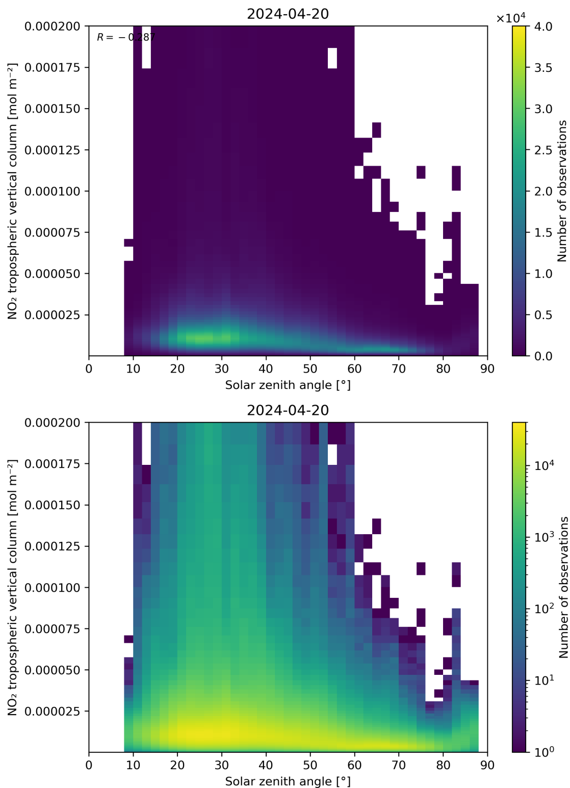
Figure 155: Scatter density plot of “Solar zenith angle” against “NO 2 tropospheric vertical column” for 2024-04-19 to 2024-04-21.
