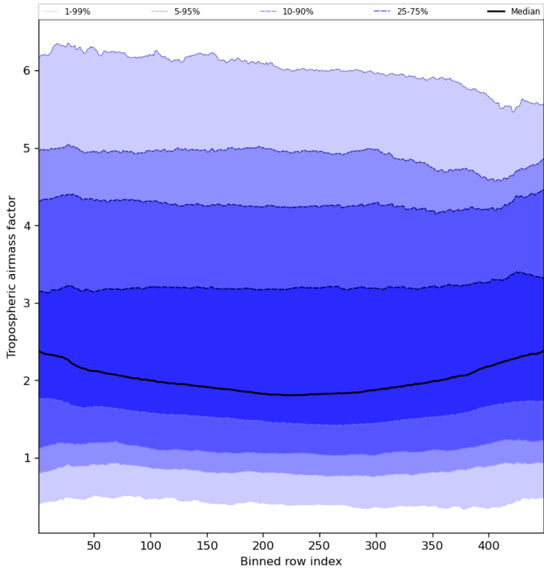
Figure 48: Along track statistics of “Tropospheric air mass factor” for 2024-04-19 to 2024-04-21
