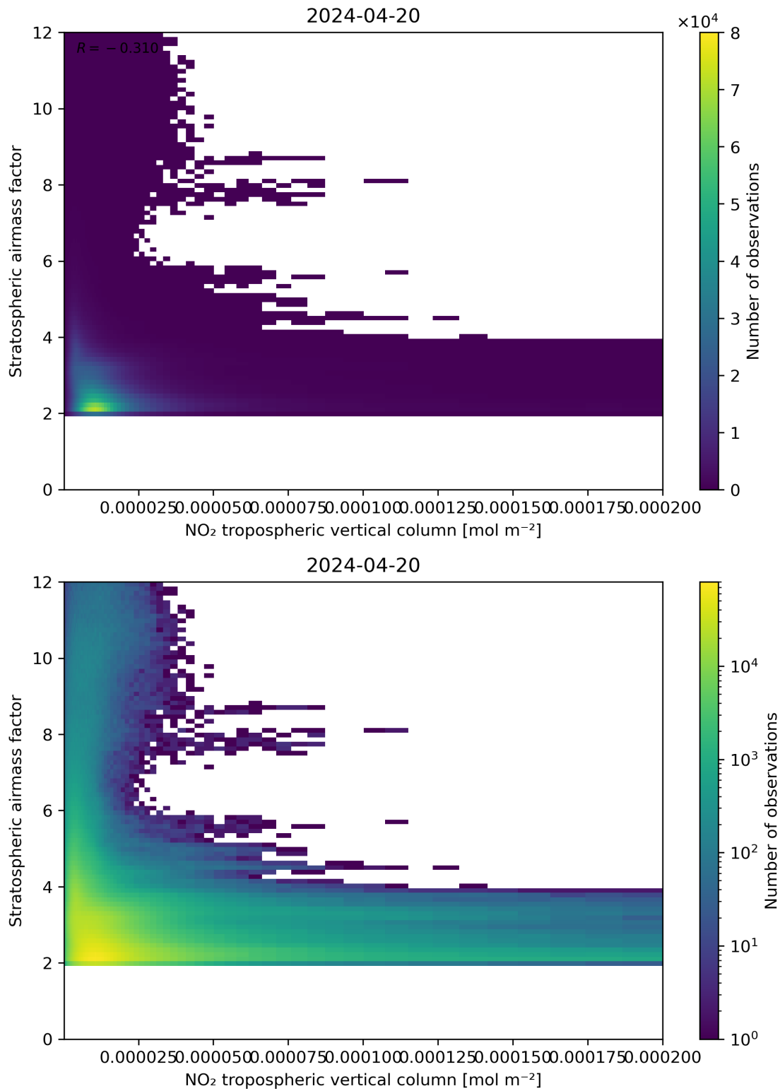
Figure 121: Scatter density plot of “NO 2 tropospheric vertical column” against “Stratospheric air mass factor” for 2024-04-19 to 2024-04-21.
