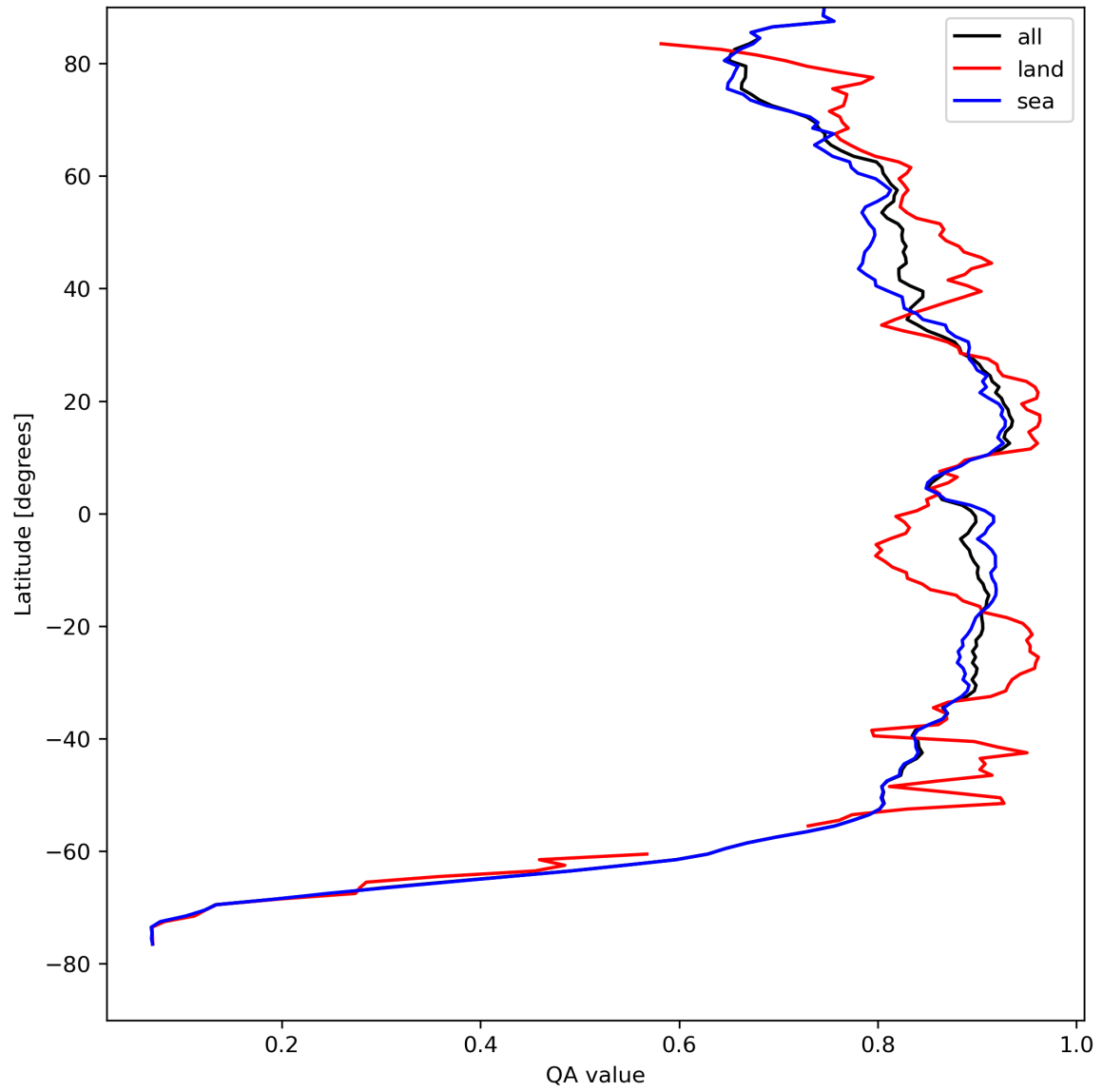
Figure 11: Zonal average of “QA value” for 2024-04-19 to 2024-04-21.
