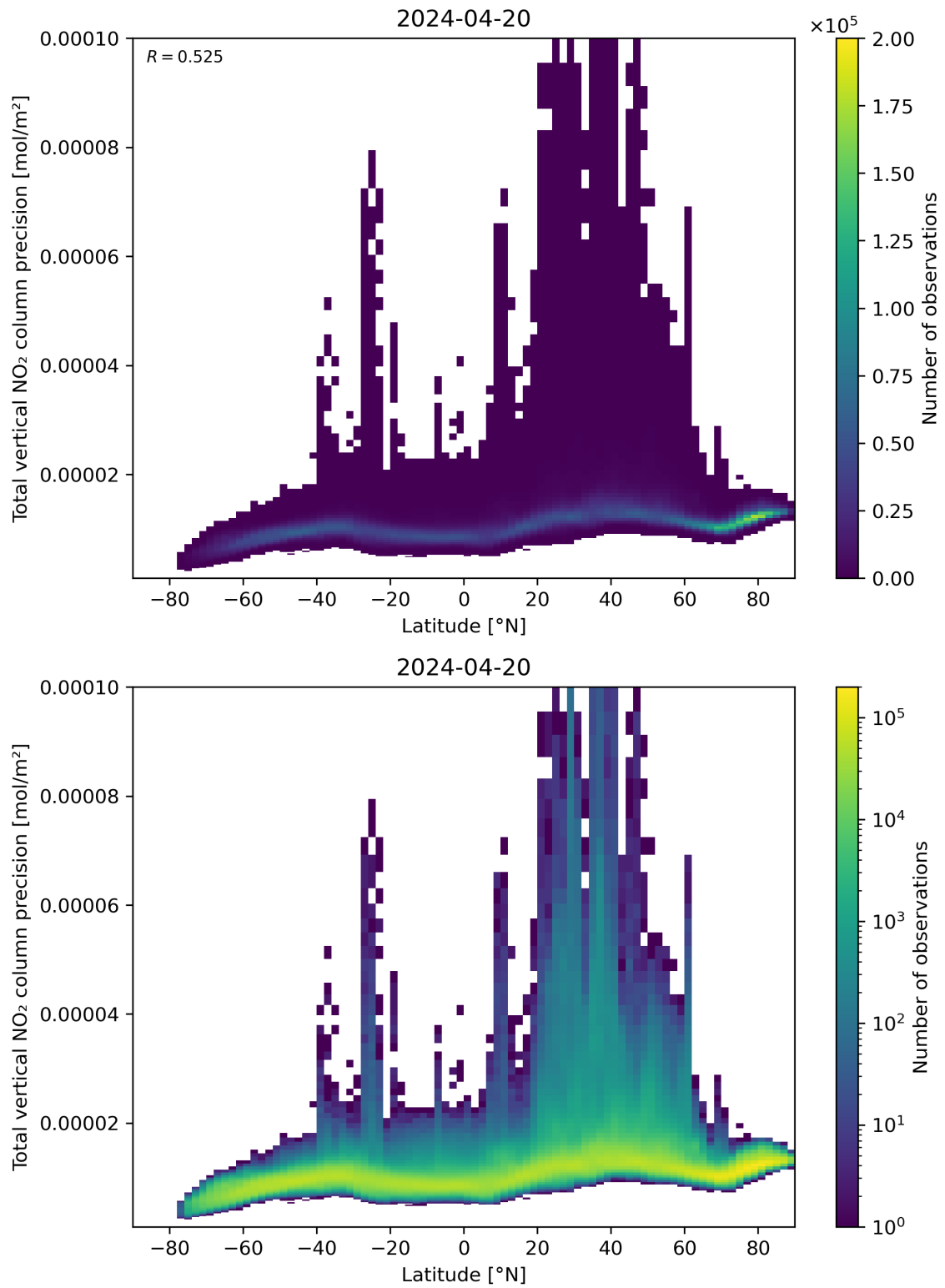
Figure 91: Scatter density plot of “Latitude” against “Total vertical NO 2 column precision” for 2024-04-19 to 2024-04-21.
