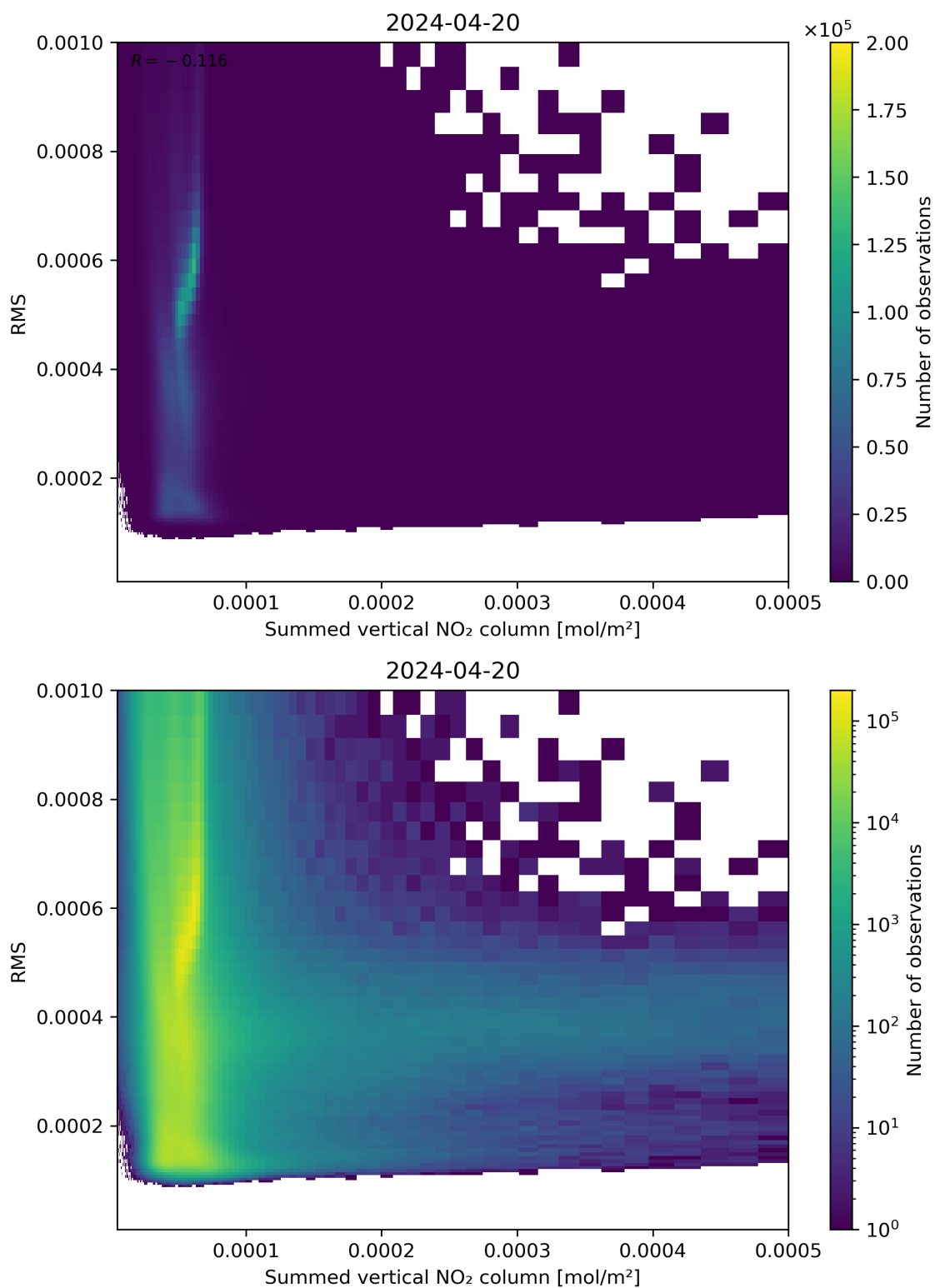
Figure 109: Scatter density plot of “Summed vertical NO 2 column” against “RMS” for 2024-04-19 to 2024-04-21.
