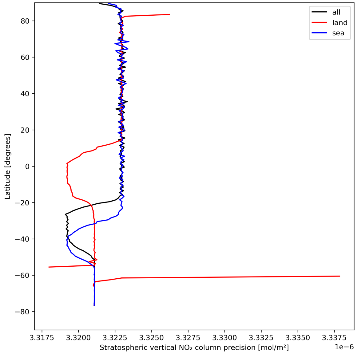
Figure 20: Zonal average of “Stratospheric vertical NO 2 column precision” for 2024-04-19 to 2024-04-21.
