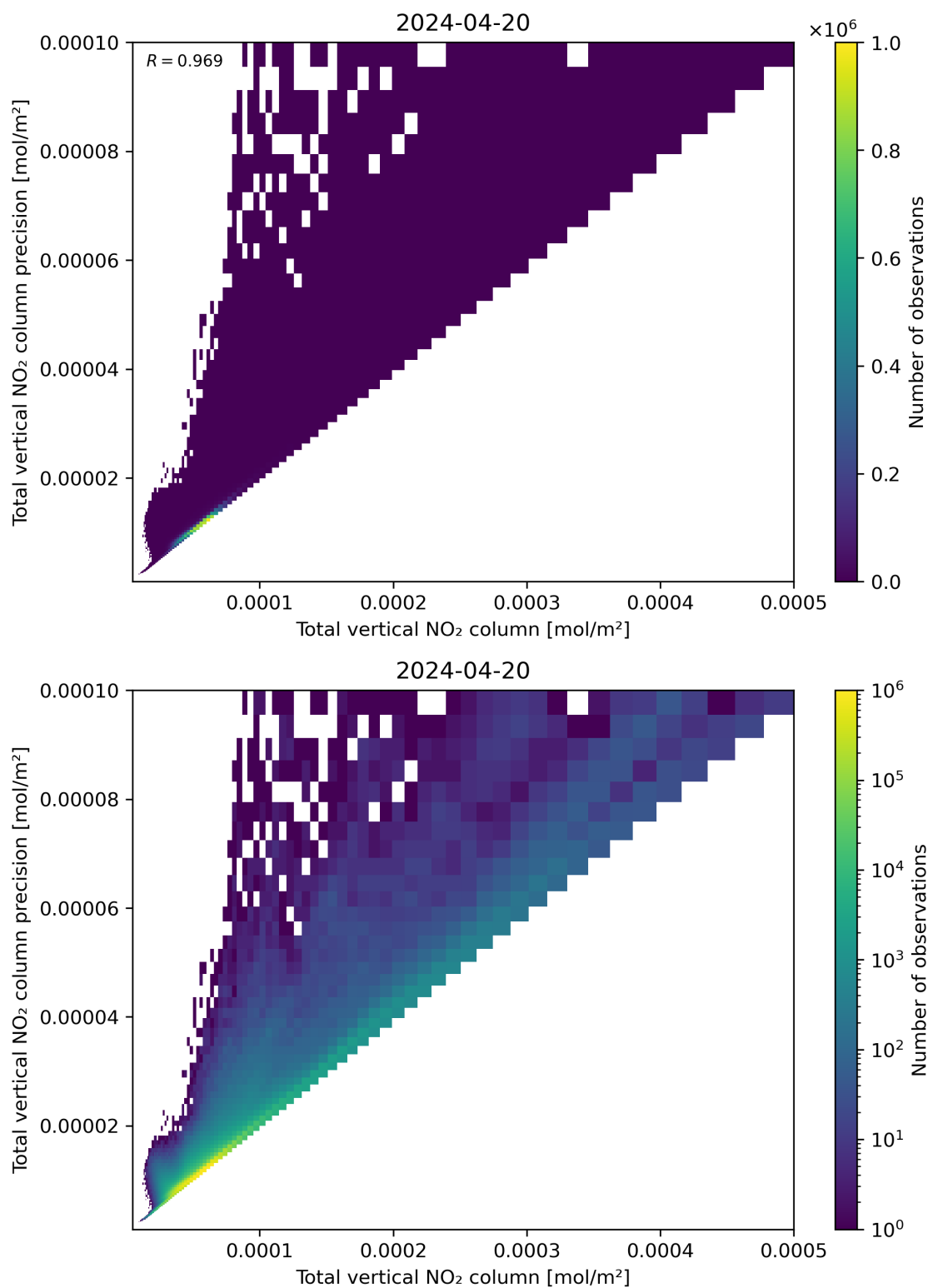
Figure 114: Scatter density plot of “Total vertical NO 2 column” against “Total vertical NO 2 column precision” for 2024-04-19 to 2024-04-21.
