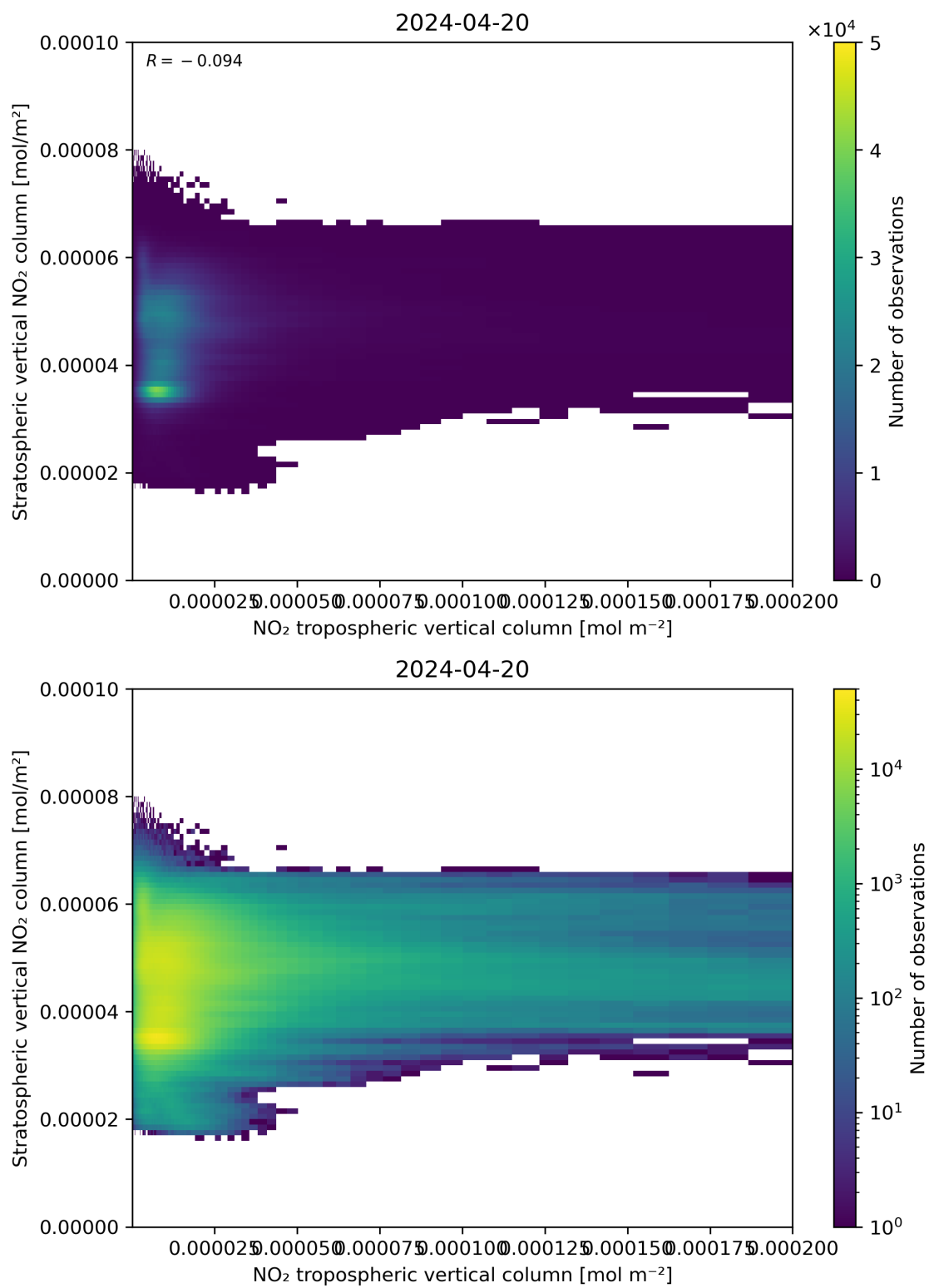
Figure 125: Scatter density plot of “NO 2 tropospheric vertical column” against “Stratospheric vertical NO 2 column” for 2024-04-19 to 2024-04-21.
