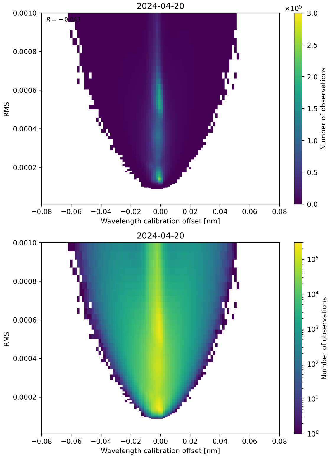
Figure 181: Scatter density plot of “Wavelength calibration offset” against “RMS” for 2024-04-19 to 2024-04-21.
