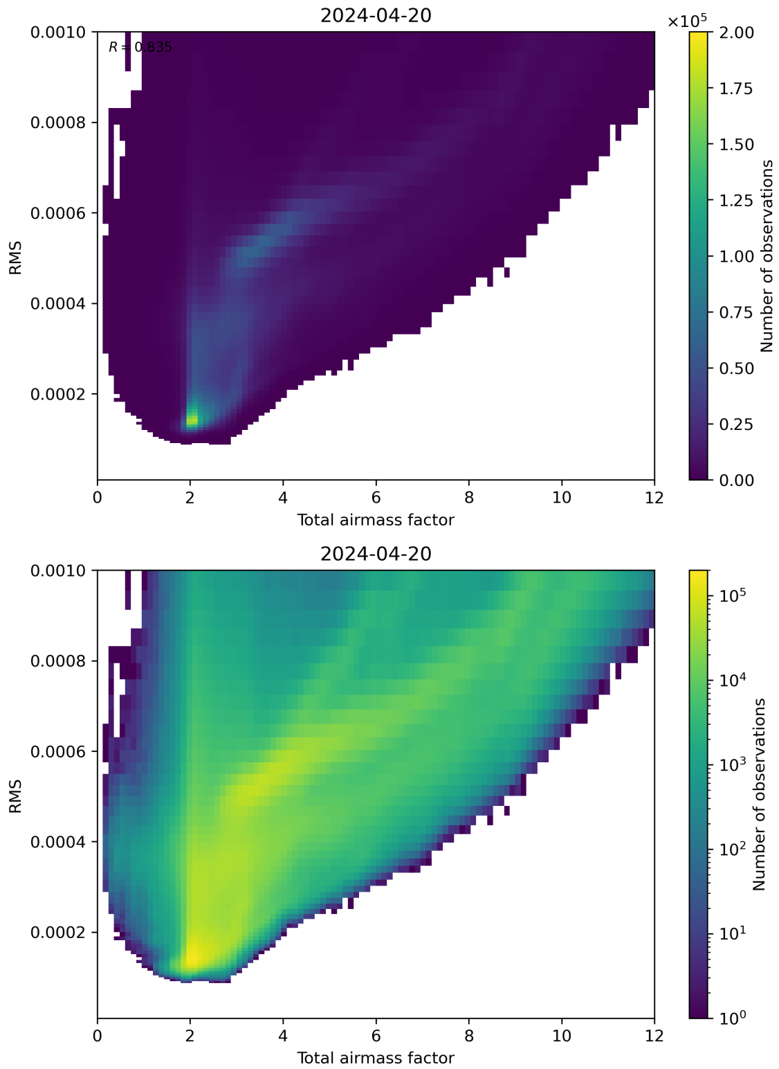
Figure 69: Scatter density plot of “Total airmass factor” against “RMS” for 2024-04-19 to 2024-04-21.
