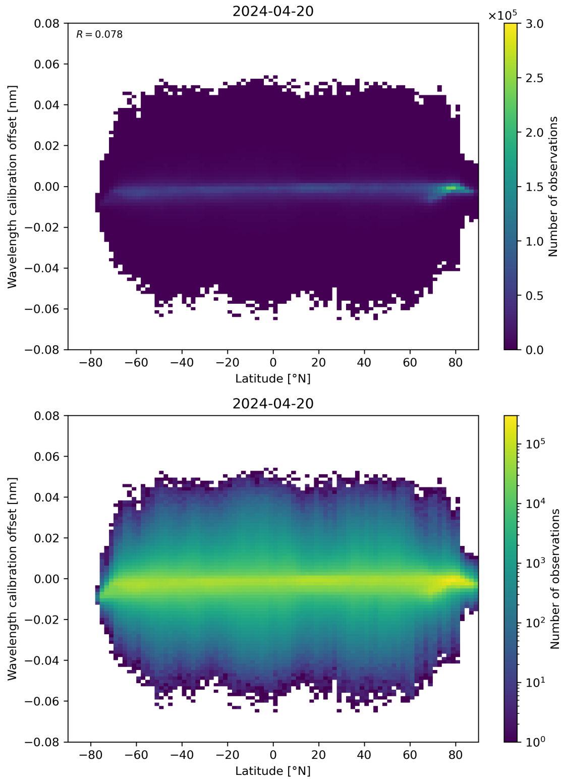
Figure 95: Scatter density plot of “Latitude” against “Wavelength calibration offset” for 2024-04-19 to 2024-04-21.
