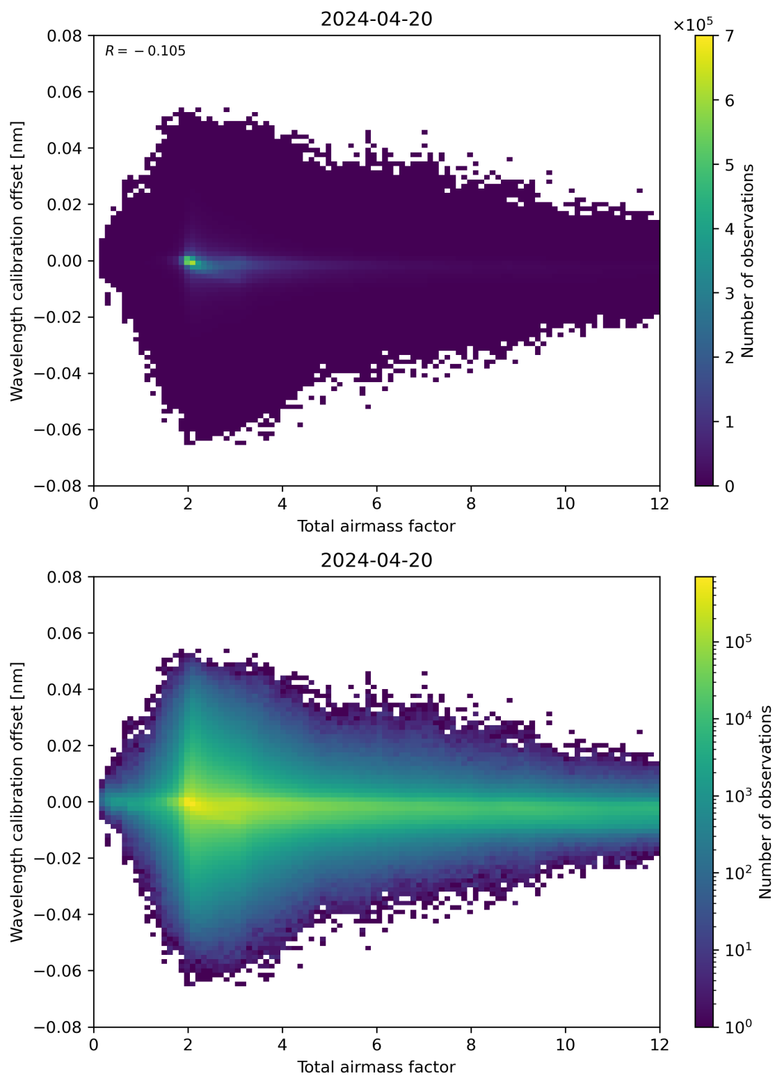
Figure 70: Scatter density plot of “Total airmass factor” against “Wavelength calibration offset” for 2024-04-19 to 2024-04-21.
