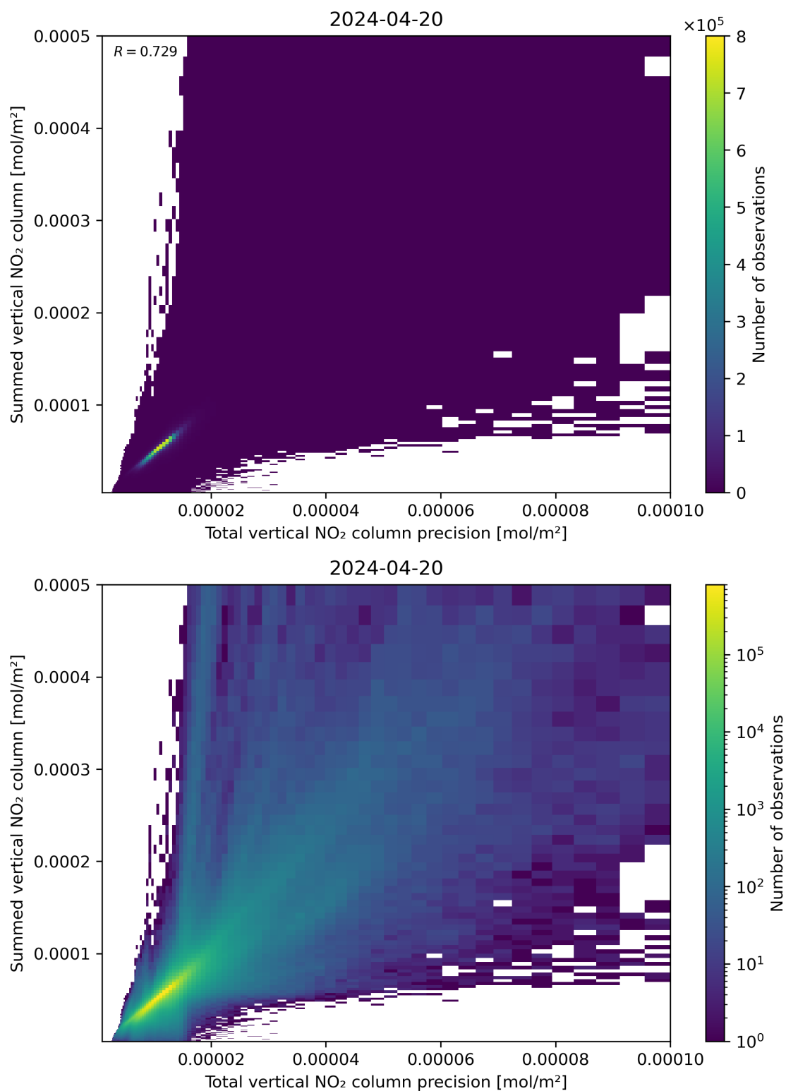
Figure 117: Scatter density plot of “Total vertical NO 2 column precision” against “Summed vertical NO 2 column” for 2024-04-19 to 2024-04-21.
