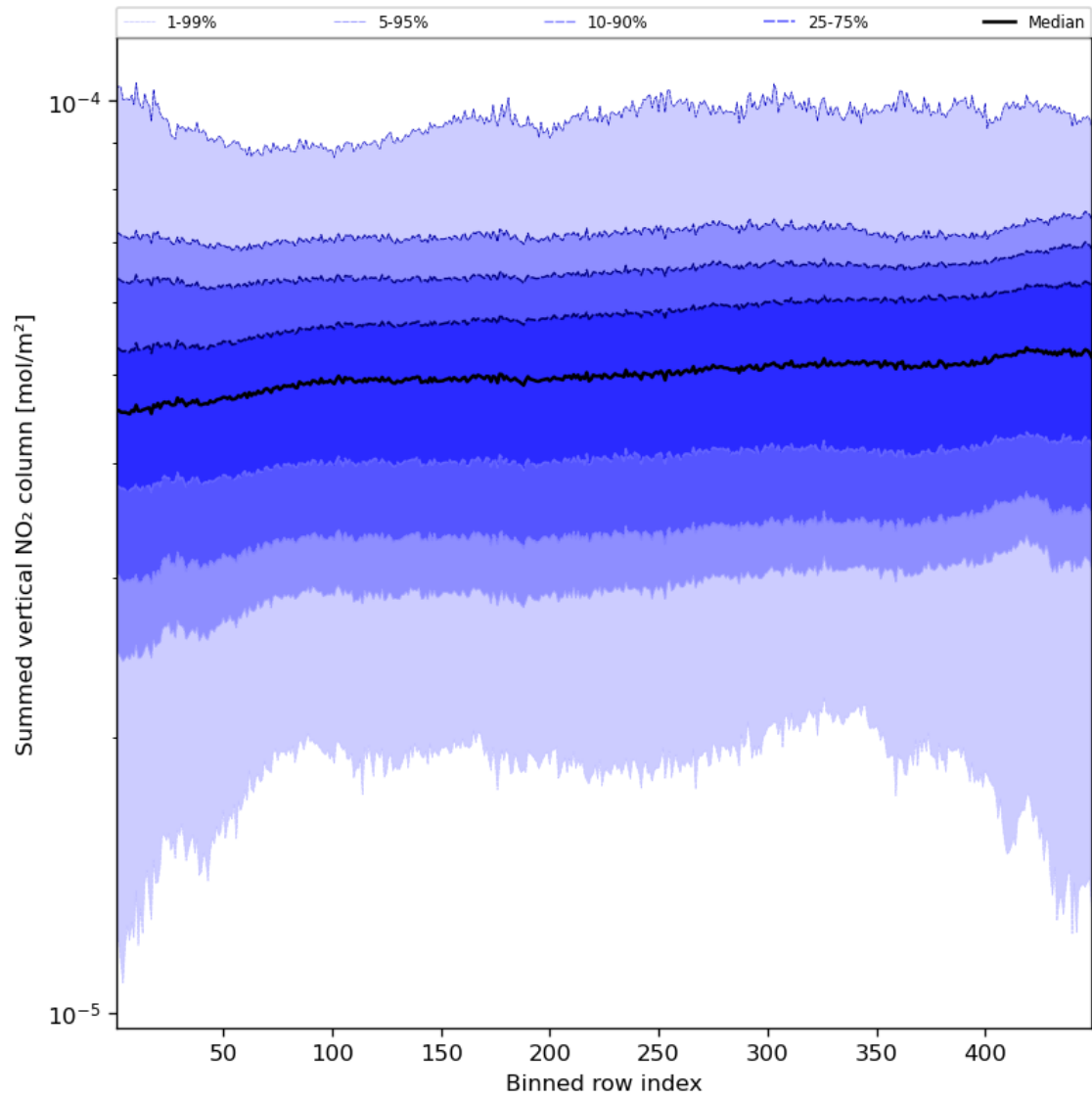
Figure 57: Along track statistics of “Summed vertical NO 2 column” for 2024-04-19 to 2024-04-21
