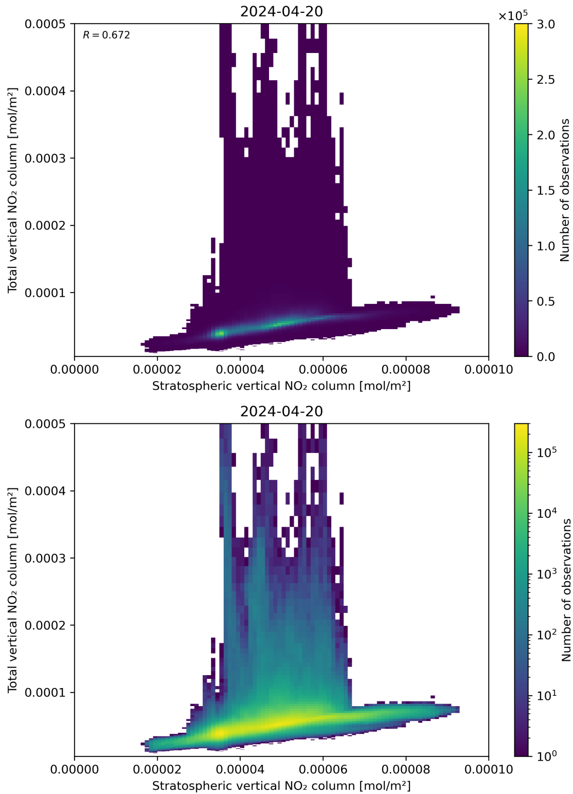
Figure 100: Scatter density plot of “Stratospheric vertical NO 2 column” against “Total vertical NO 2 column” for 2024-04-19 to 2024-04-21.
