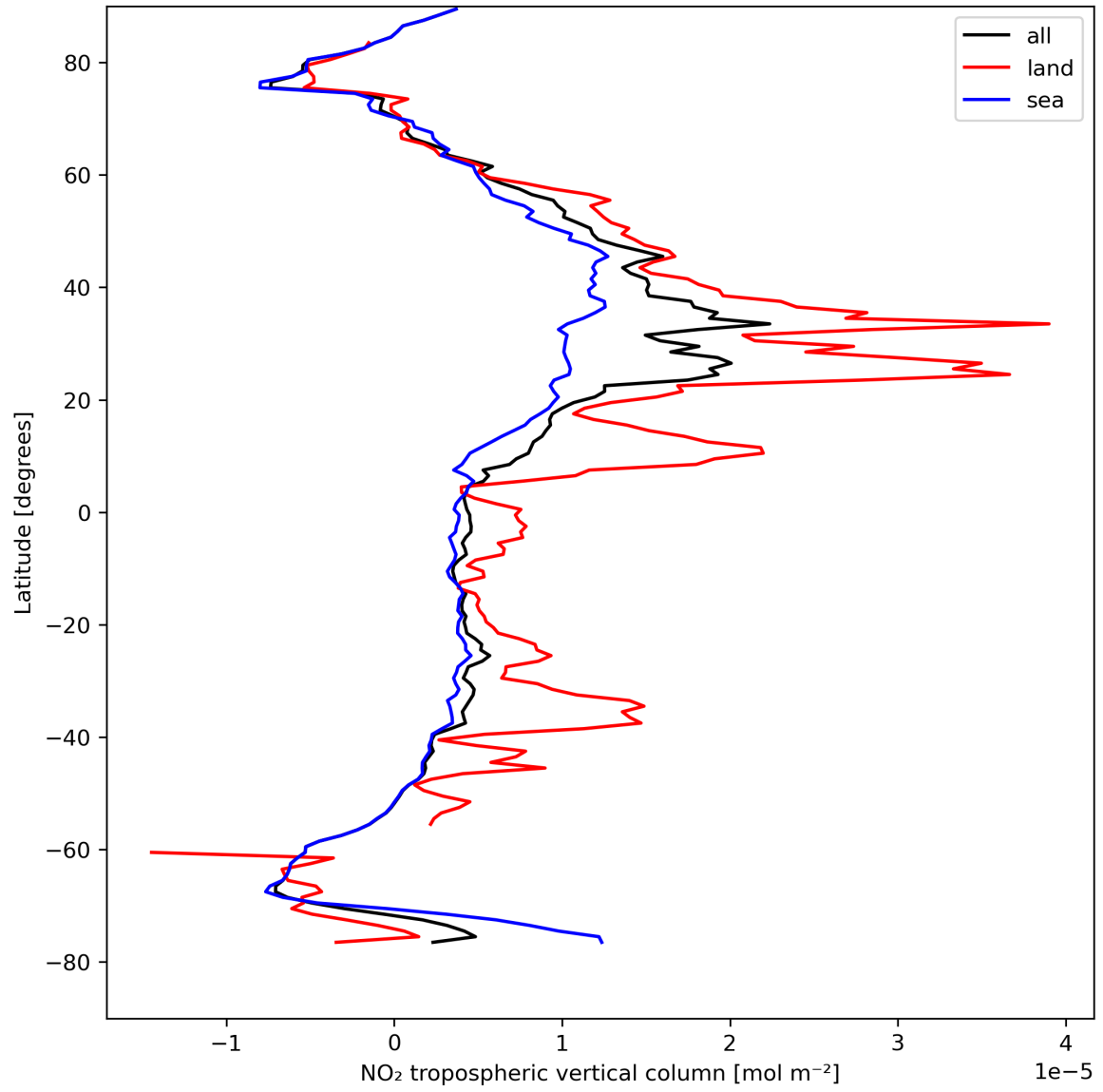
Figure 12: Zonal average of “NO 2 tropospheric vertical column” for 2024-04-19 to 2024-04-21.
