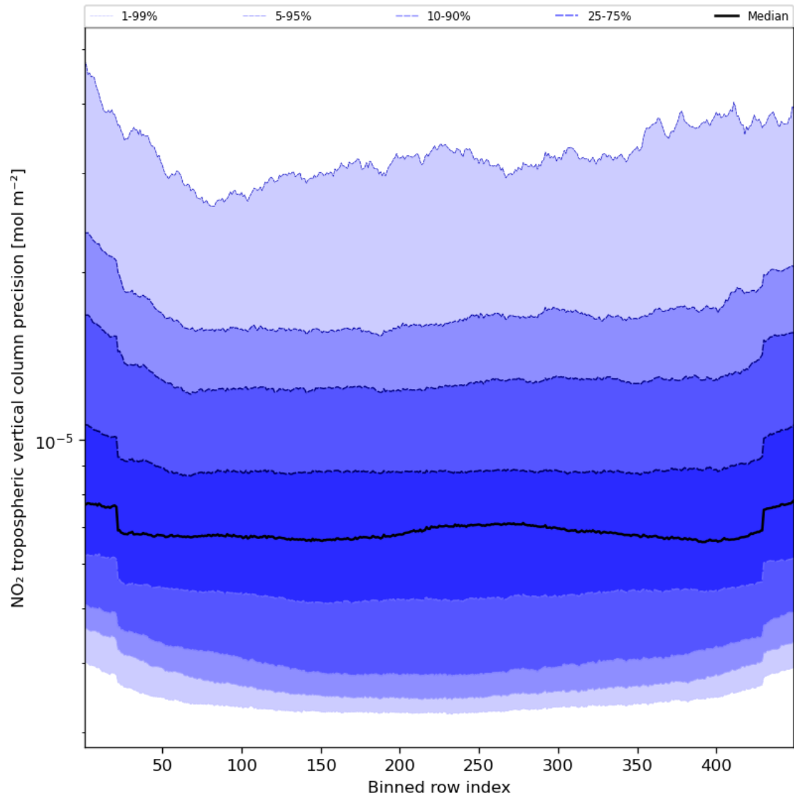
Figure 47: Along track statistics of “NO 2 tropospheric vertical column precision” for 2024-04-19 to 2024-04-21
