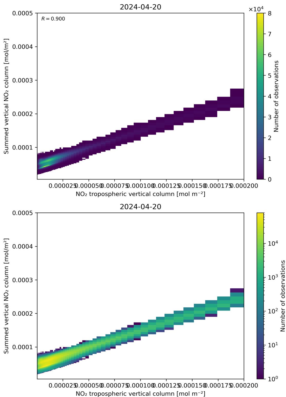
Figure 126: Scatter density plot of “NO 2 tropospheric vertical column” against “Summed vertical NO 2 column” for 2024-04-19 to 2024-04-21.
