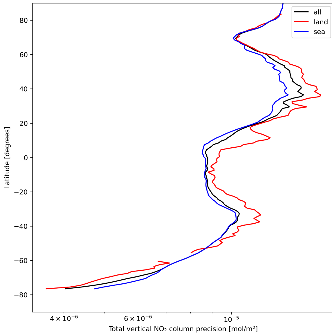
Figure 22: Zonal average of “Total vertical NO 2 column precision” for 2024-04-19 to 2024-04-21.
