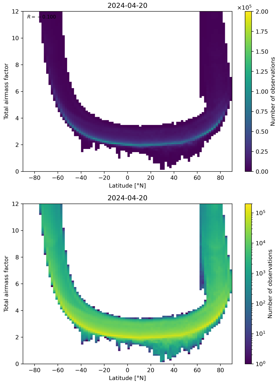
Figure 84: Scatter density plot of “Latitude” against “Total airmass factor” for 2024-04-19 to 2024-04-21.
