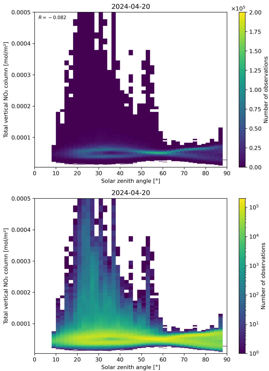
Figure 153: Scatter density plot of “Solar zenith angle” against “Total vertical NO 2 column” for 2024-04-19 to 2024-04-21.
