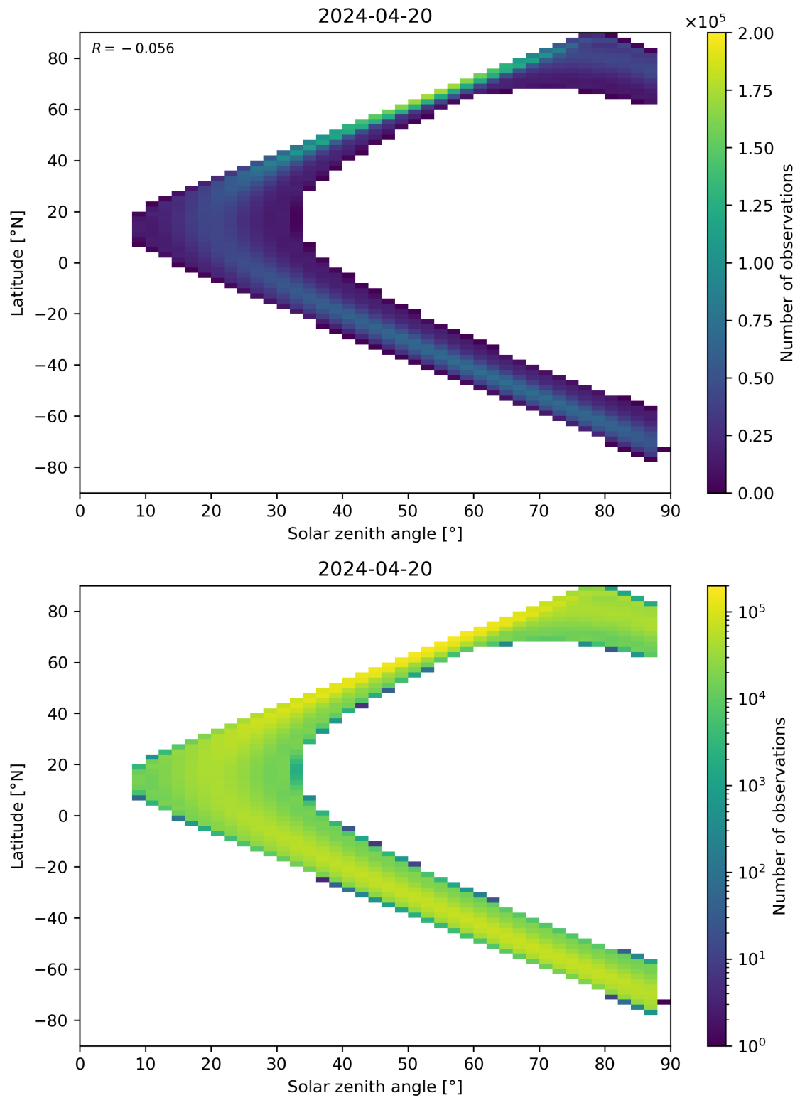
Figure 149: Scatter density plot of “Solar zenith angle” against “Latitude” for 2024-04-19 to 2024-04-21.
