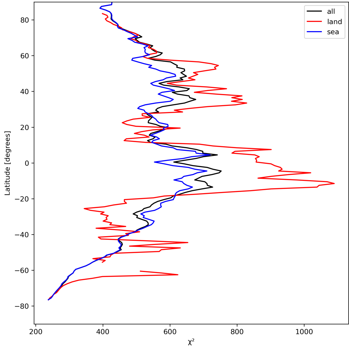
Figure 25: Zonal average of “ \chi^2 ” for 2024-04-19 to 2024-04-21.
