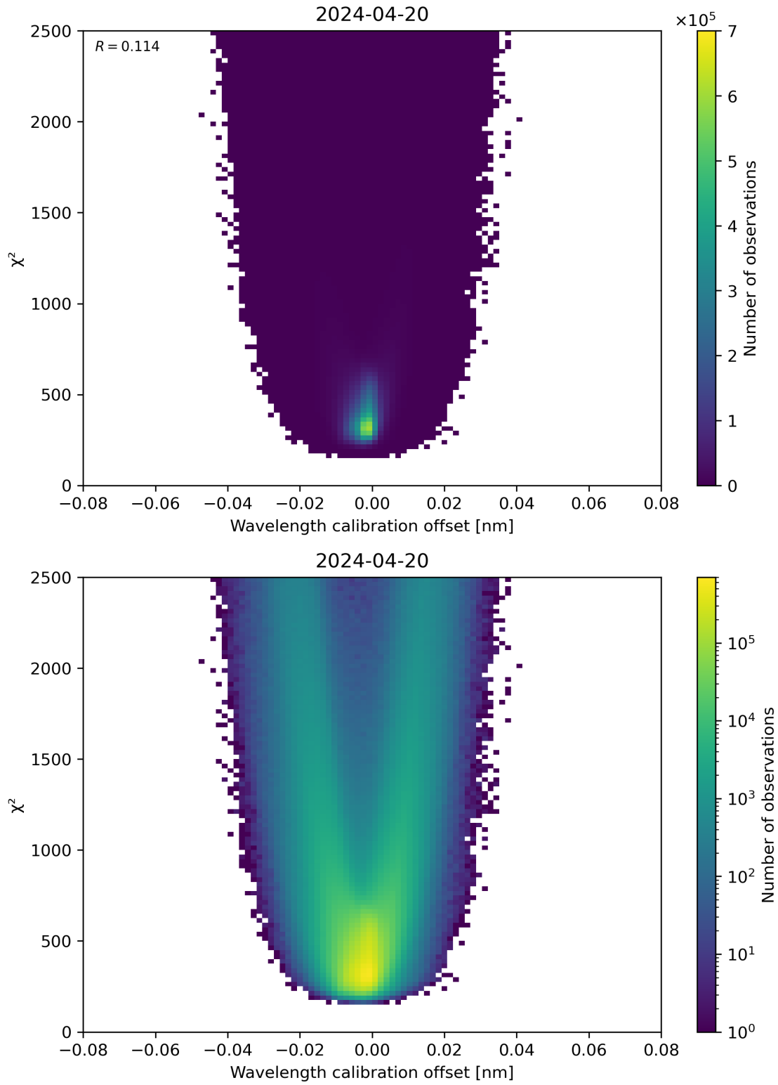
Figure 175: Scatter density plot of “Wavelength calibration offset” against “ \chi^2 ” for 2024-04-19 to 2024-04-21.
