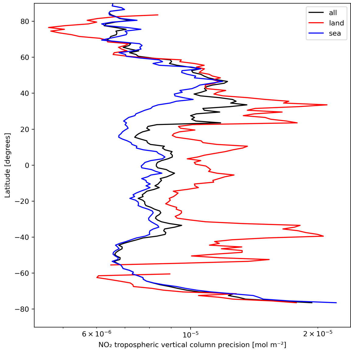
Figure 13: Zonal average of “NO 2 tropospheric vertical column precision” for 2024-04-19 to 2024-04-21.
