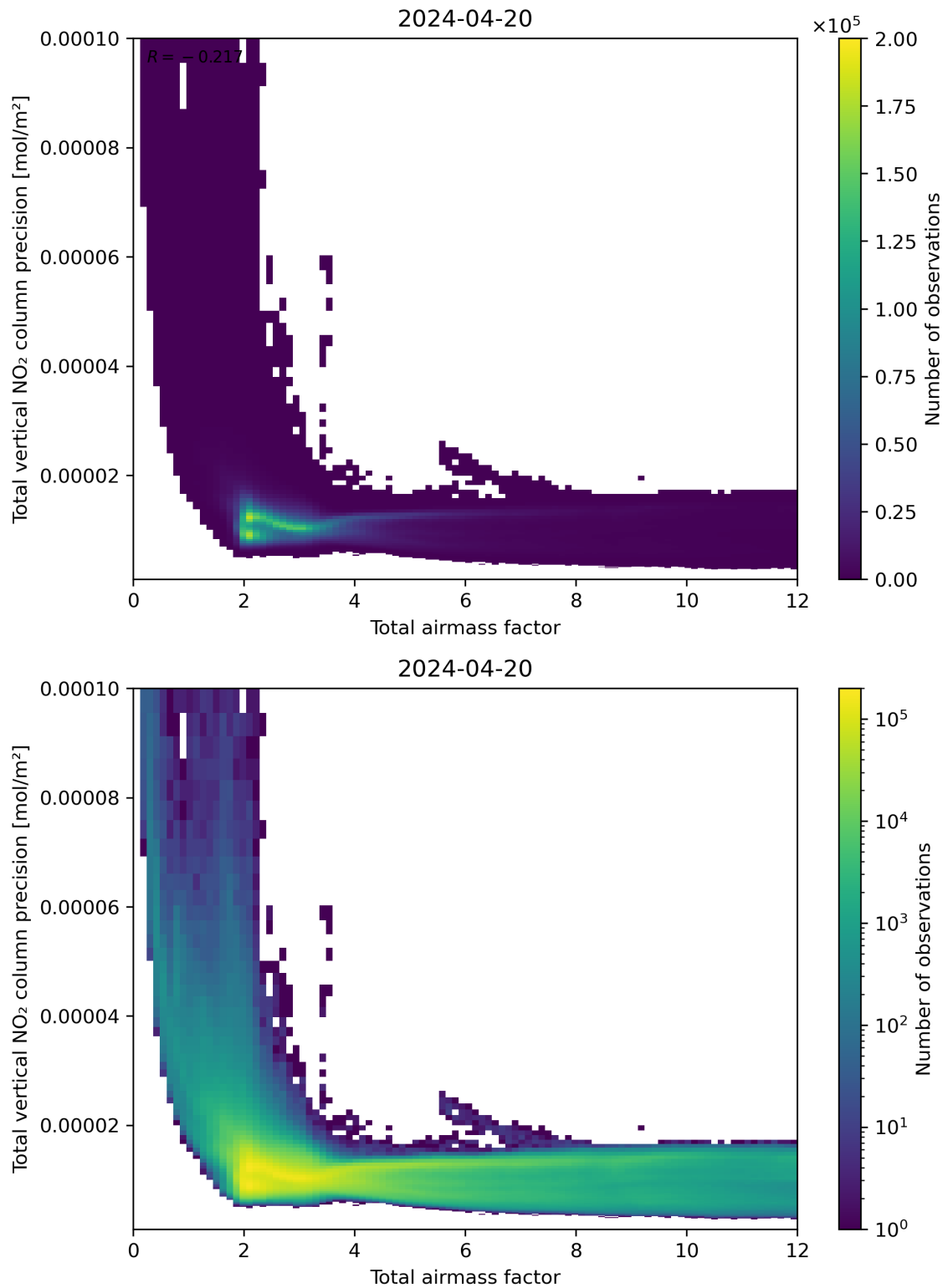
Figure 68: Scatter density plot of “Total airmass factor” against “Total vertical NO 2 column precision” for 2024-04-19 to 2024-04-21.
