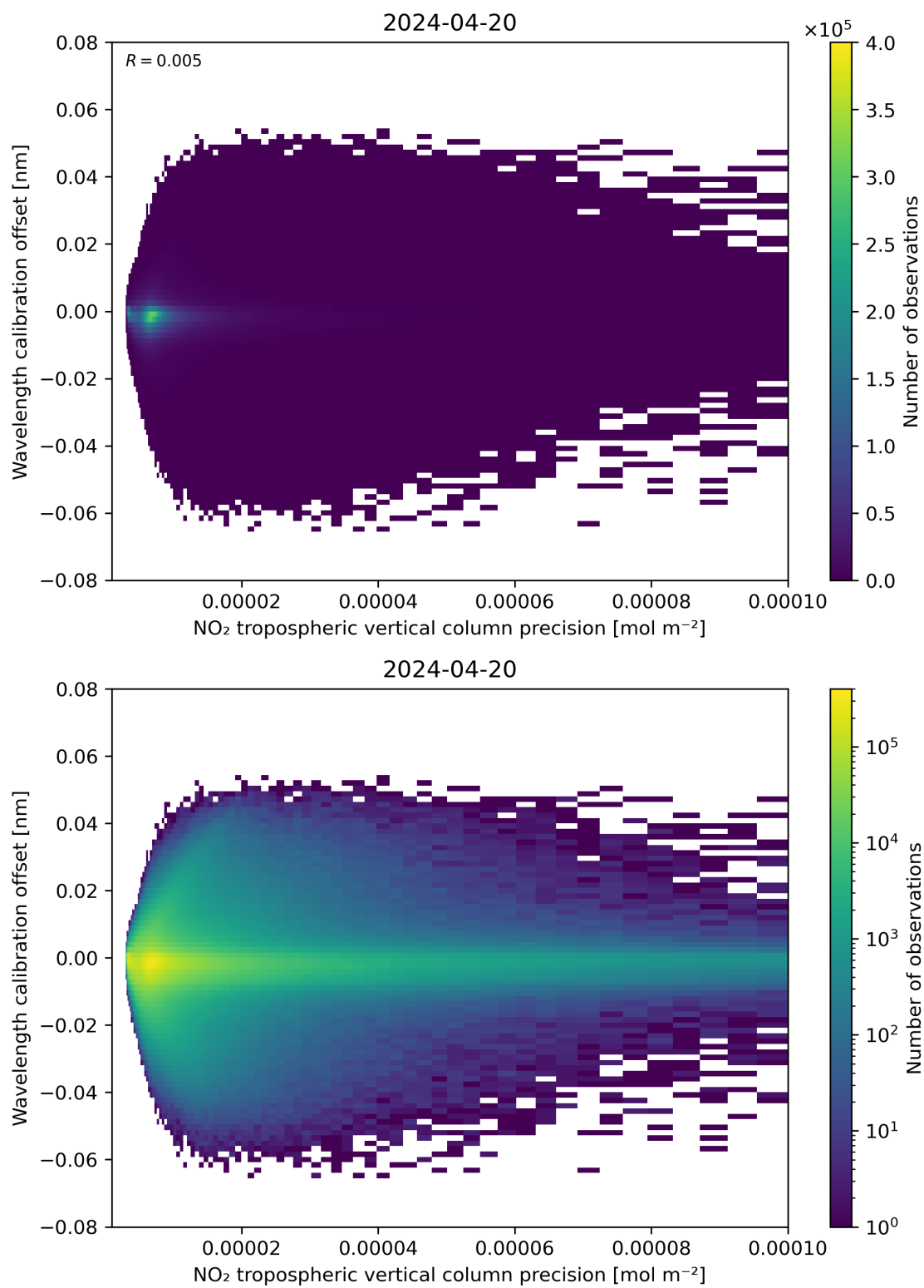
Figure 141: Scatter density plot of “NO 2 tropospheric vertical column precision” against “Wavelength calibration offset” for 2024-04-19 to 2024-04-21.
