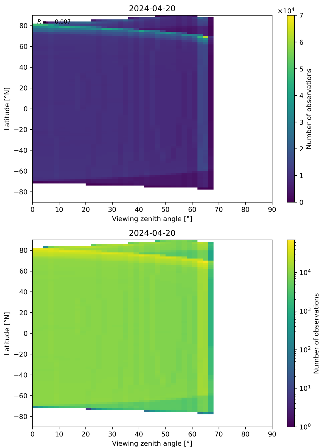
Figure 163: Scatter density plot of “Viewing zenith angle” against “Latitude” for 2024-04-19 to 2024-04-21.
