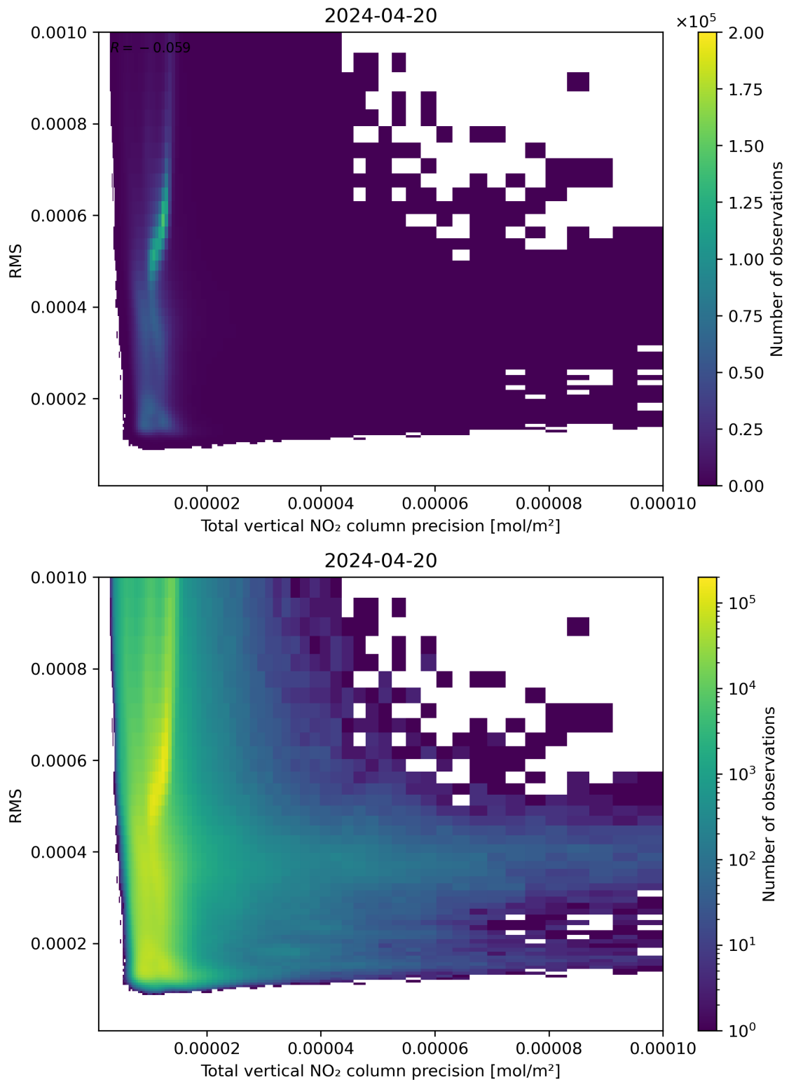
Figure 119: Scatter density plot of “Total vertical NO 2 column precision” against “RMS” for 2024-04-19 to 2024-04-21.
