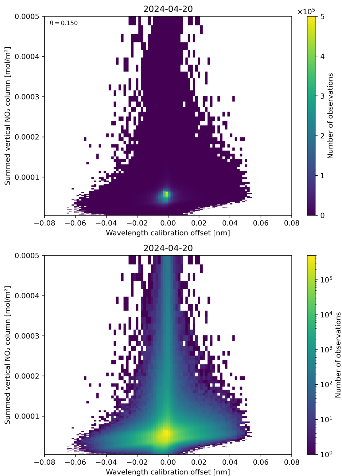
Figure 177: Scatter density plot of “Wavelength calibration offset” against “Summed vertical NO 2 column” for 2024-04-19 to 2024-04-21.
