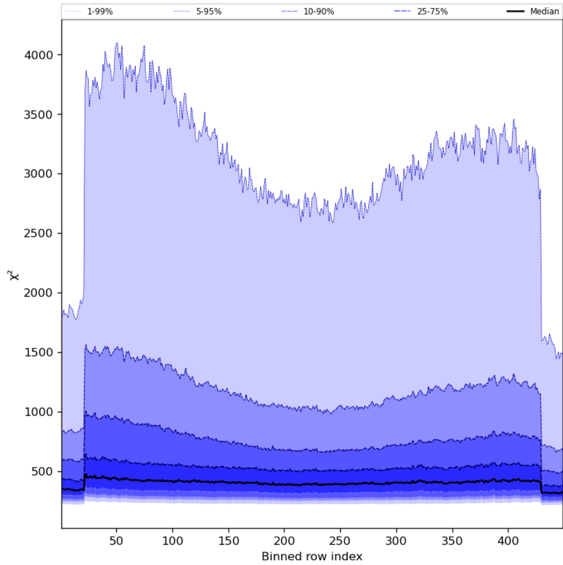
Figure 59: Along track statistics of “ \chi^2 ” for 2024-04-19 to 2024-04-21
