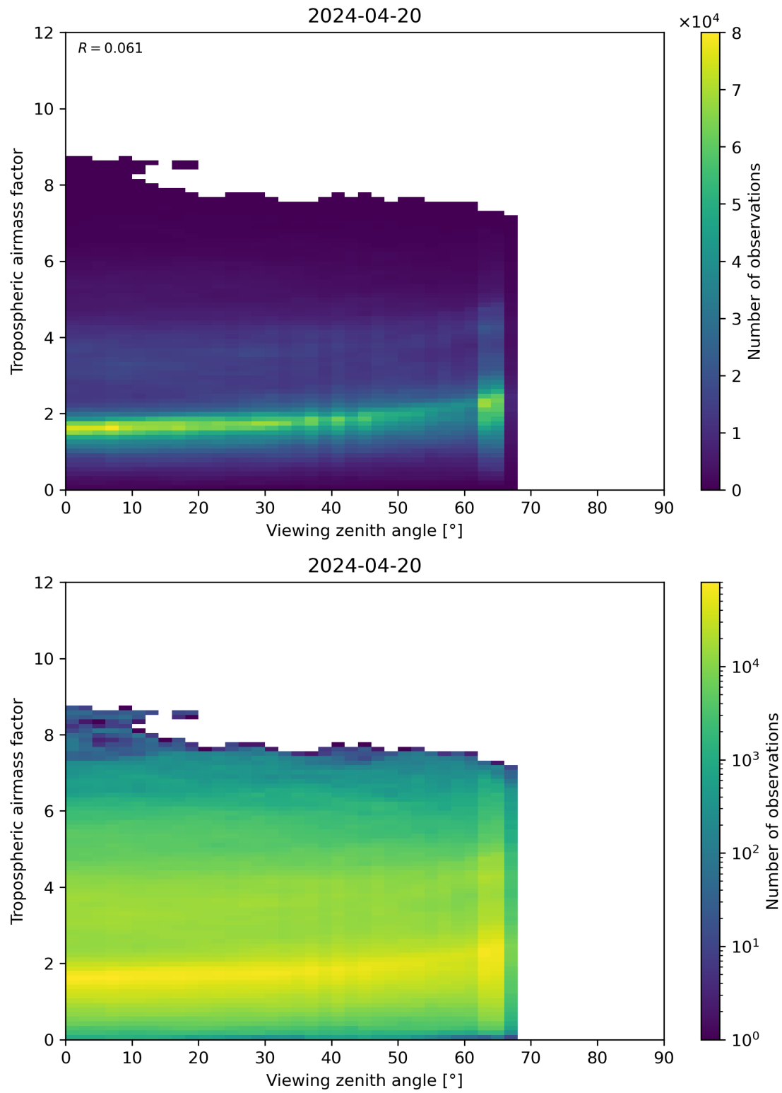
Figure 161: Scatter density plot of “Viewing zenith angle” against “Tropospheric airmass factor” for 2024-04-19 to 2024-04-21.
