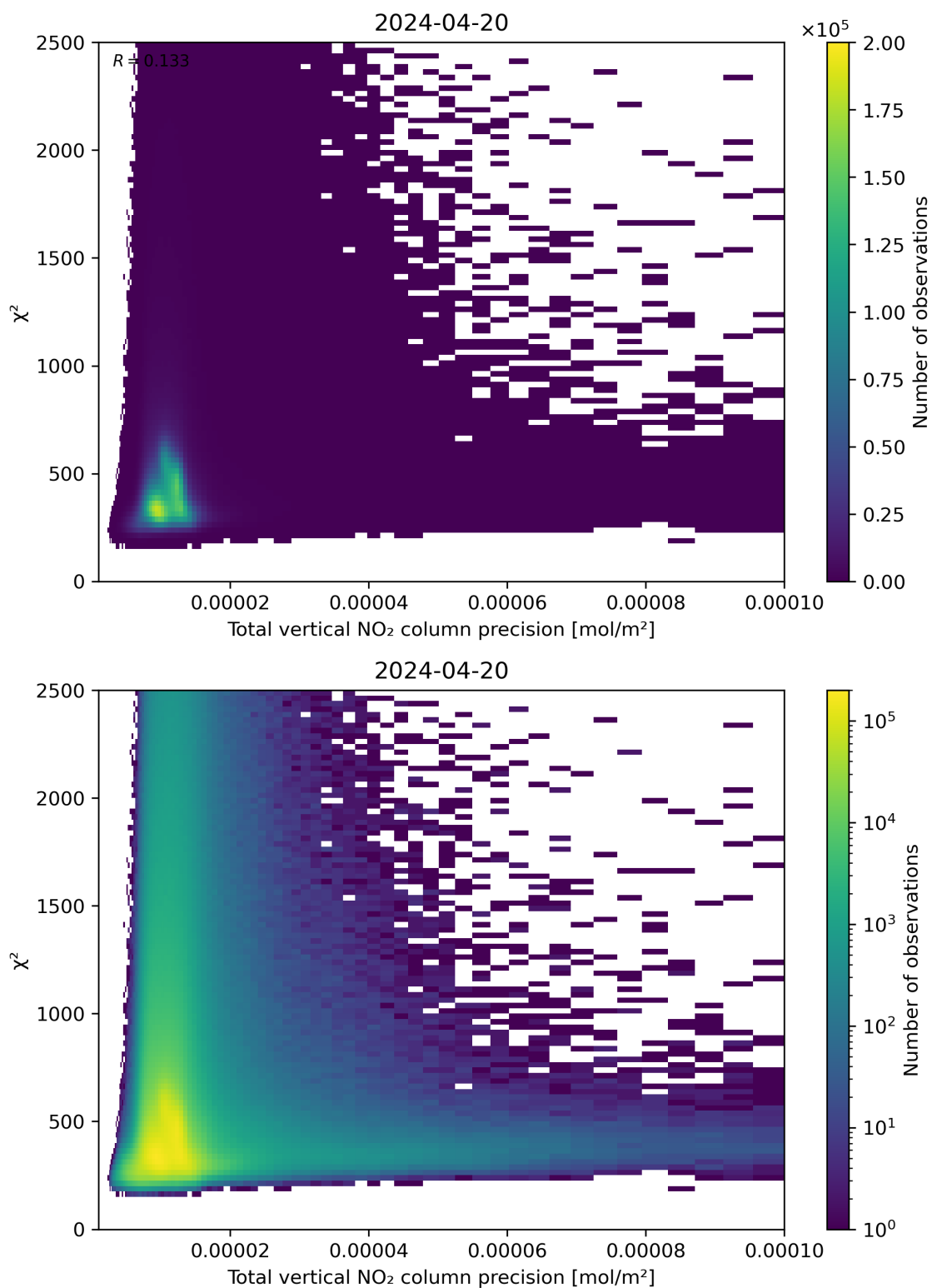
Figure 116: Scatter density plot of “Total vertical NO 2 column precision” against “ \chi^2 ” for 2024-04-19 to 2024-04-21.
