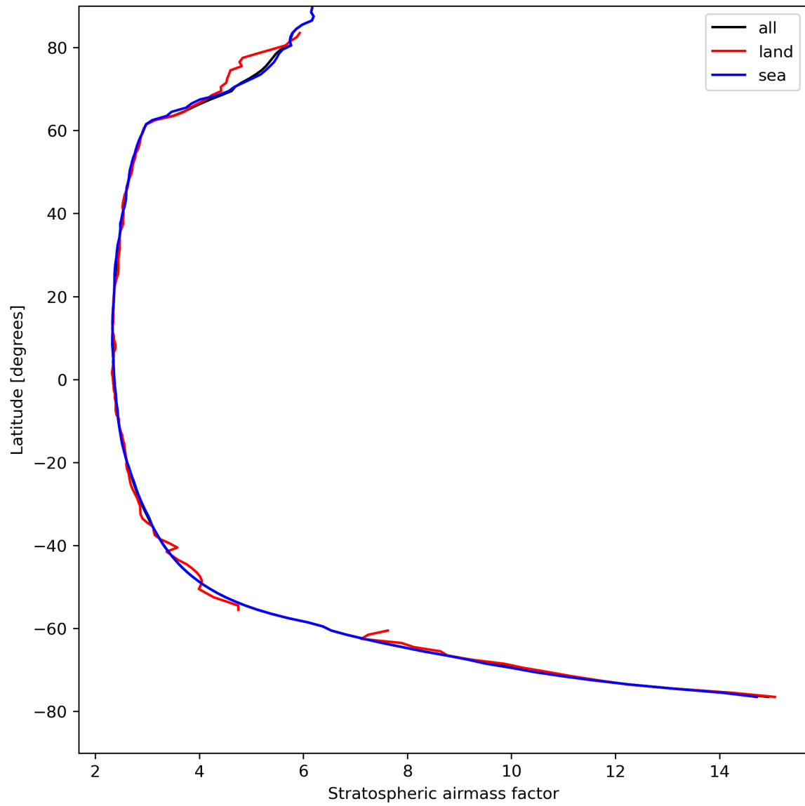
Figure 27: Zonal average of “Stratospheric air mass factor” for 2024-04-19 to 2024-04-21.
