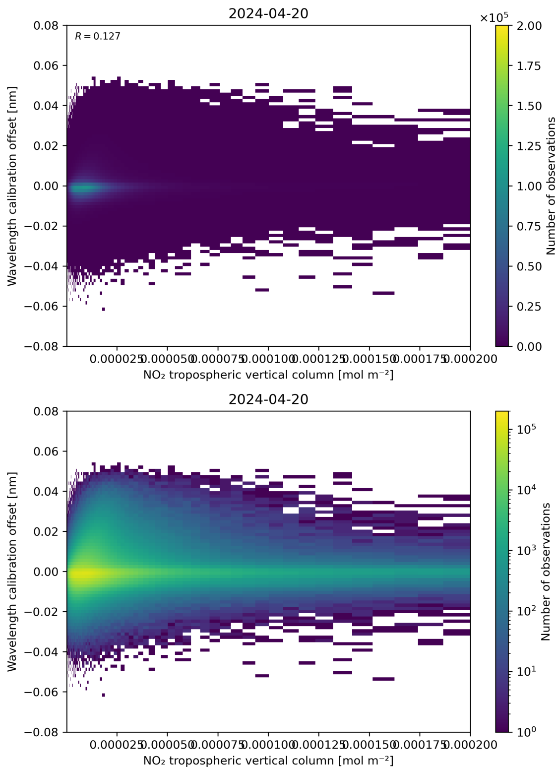
Figure 143: Scatter density plot of “NO 2 tropospheric vertical column” against “Wavelength calibration offset” for 2024-04-19 to 2024-04-21.
