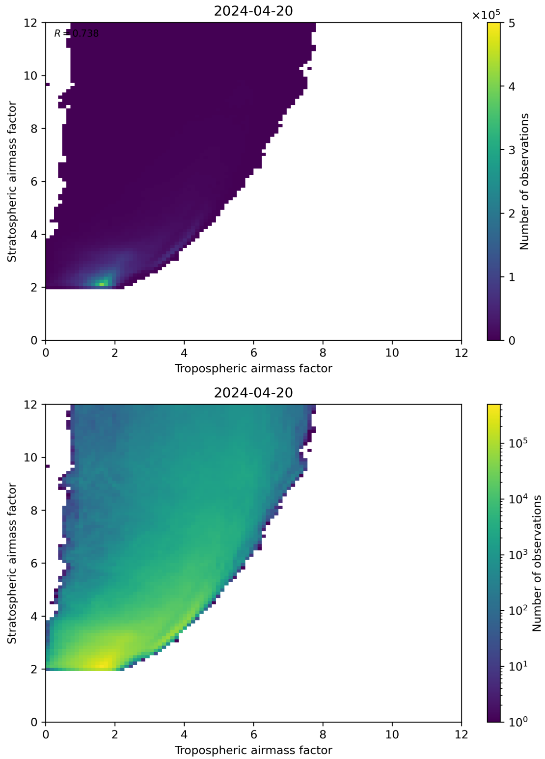
Figure 71: Scatter density plot of “Tropospheric airmass factor” against “Stratospheric airmass factor” for 2024-04-19 to 2024-04-21.
