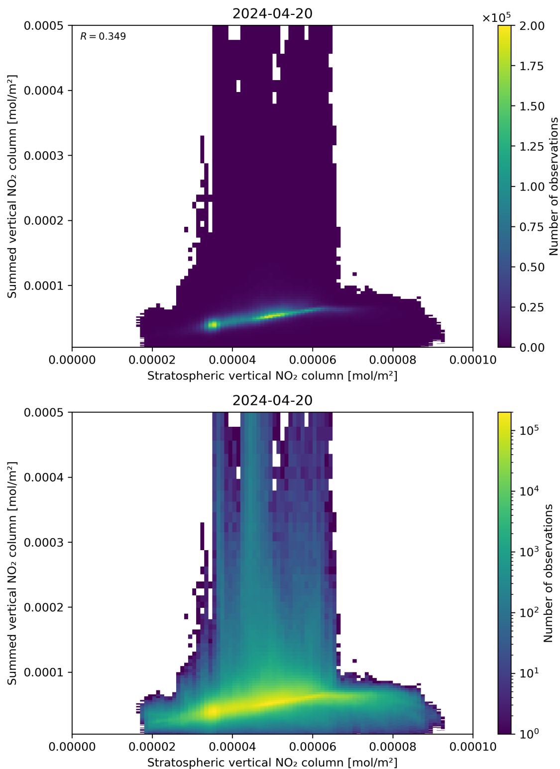
Figure 98: Scatter density plot of “Stratospheric vertical NO 2 column” against “Summed vertical NO 2 column” for 2024-04-19 to 2024-04-21.
