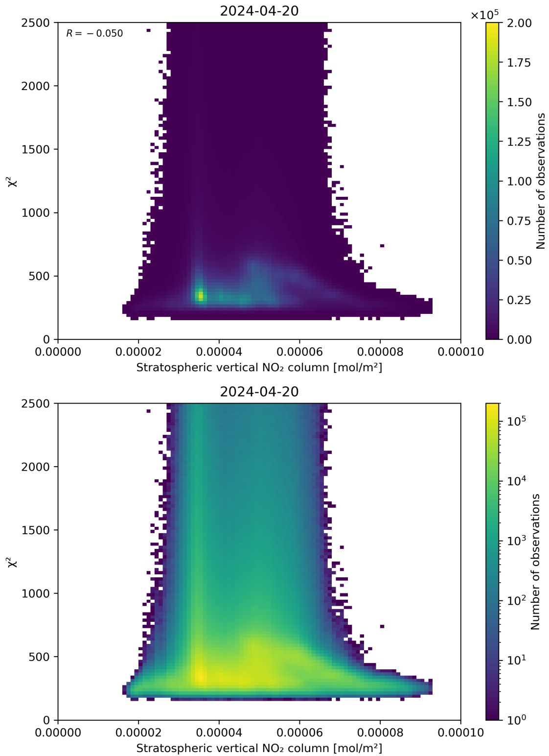
Figure 97: Scatter density plot of “Stratospheric vertical NO 2 column” against “ \chi^2 ” for 2024-04-19 to 2024-04-21.
