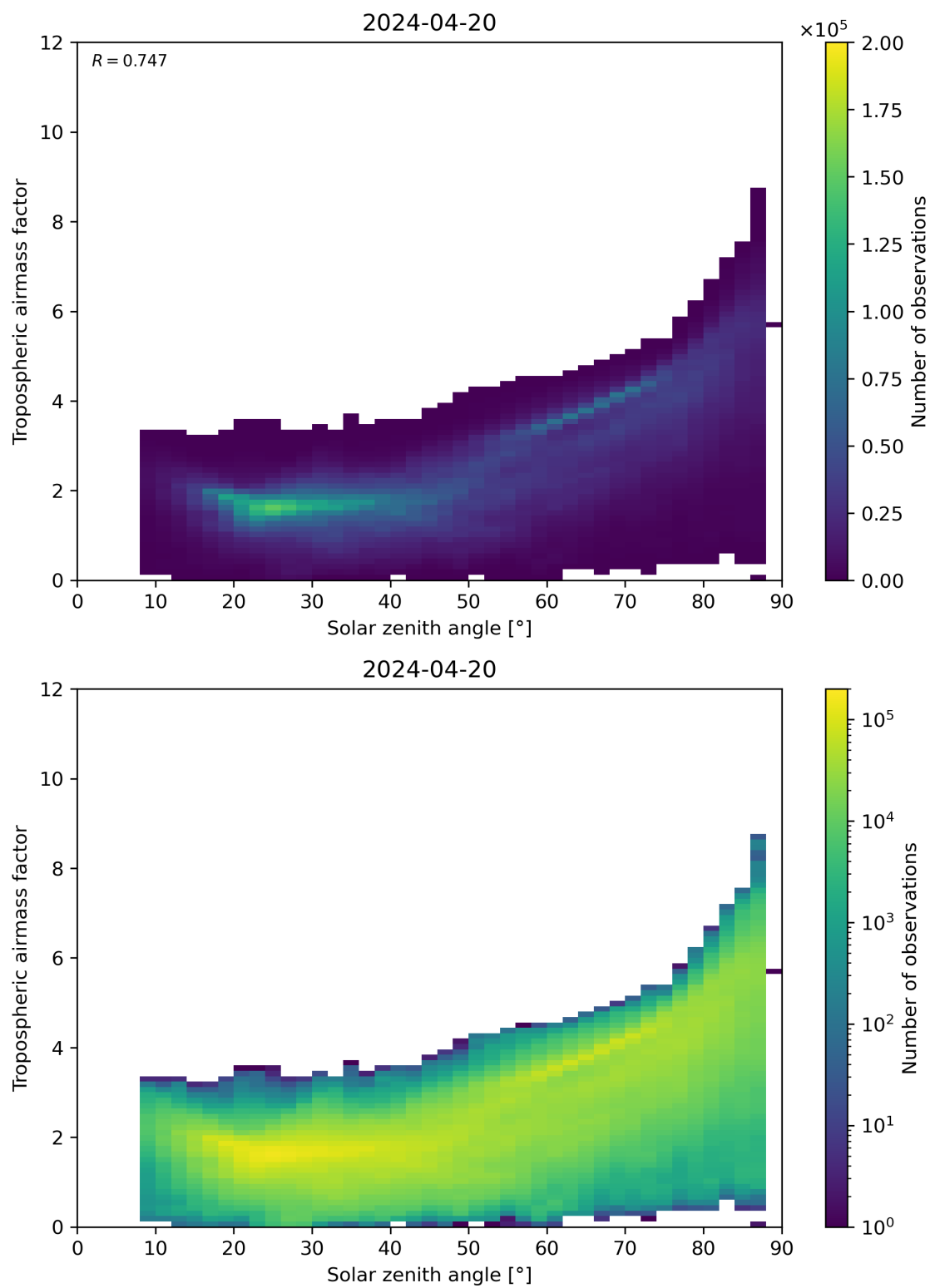
Figure 147: Scatter density plot of “Solar zenith angle” against “Tropospheric airmass factor” for 2024-04-19 to 2024-04-21.
