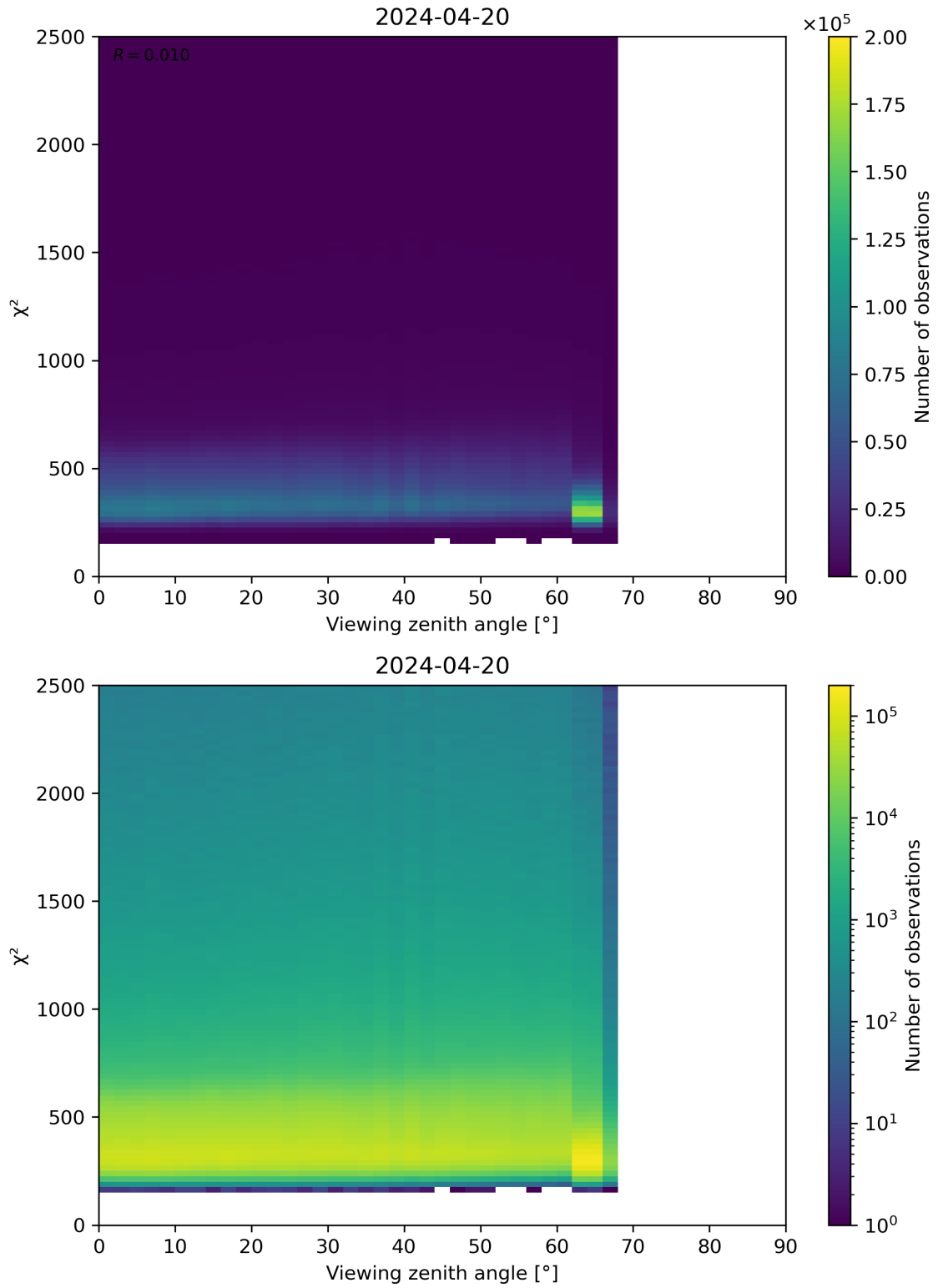
Figure 162: Scatter density plot of “Viewing zenith angle” against “ \chi^2 ” for 2024-04-19 to 2024-04-21.
