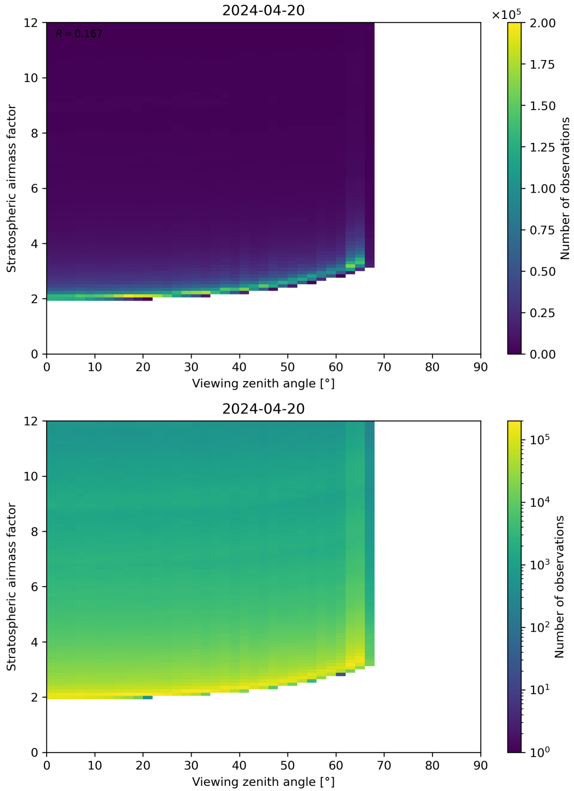
Figure 159: Scatter density plot of “Viewing zenith angle” against “Stratospheric airmass factor” for 2024-04-19 to 2024-04-21.
