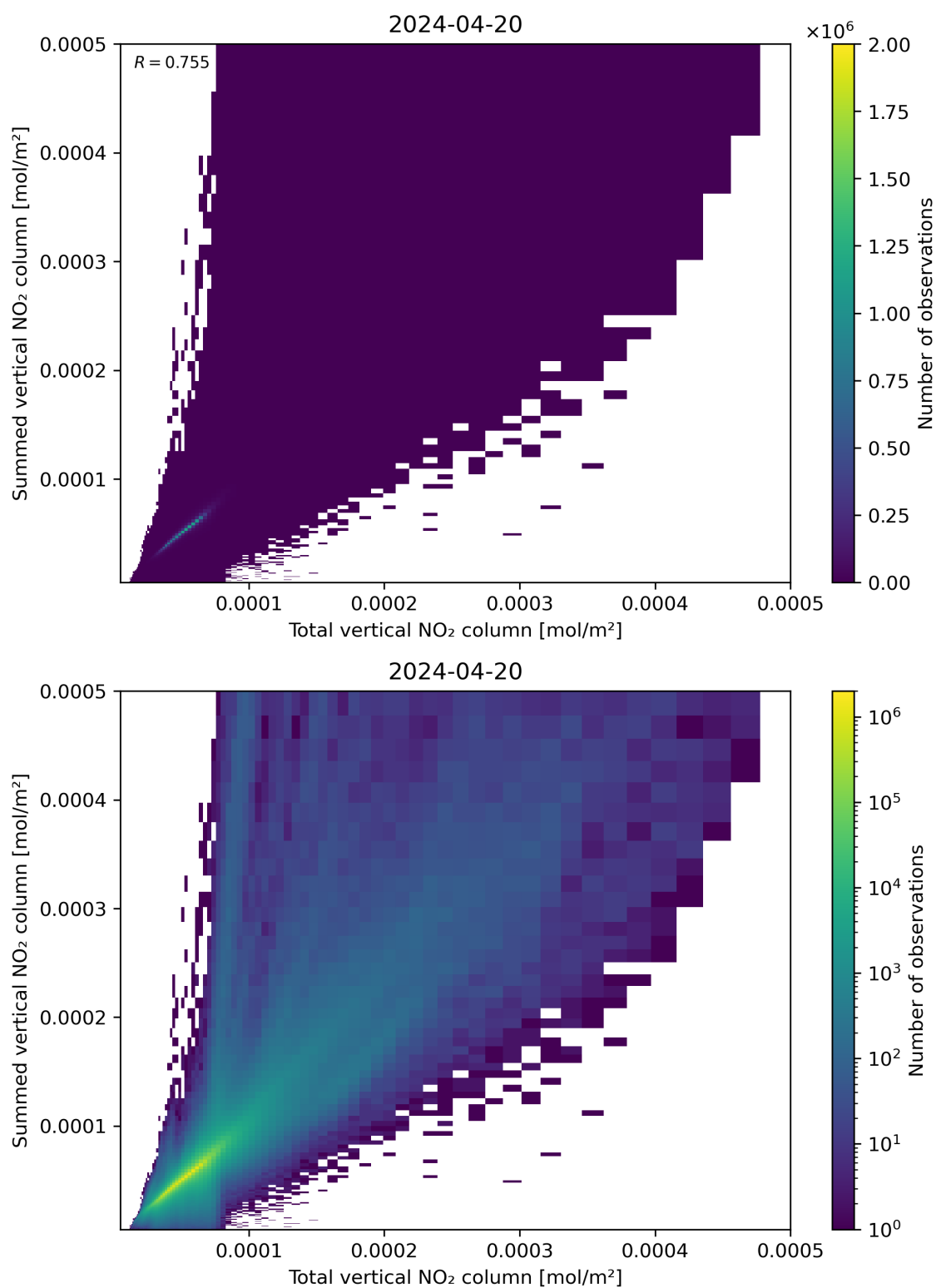
Figure 112: Scatter density plot of “Total vertical NO 2 column” against “Summed vertical NO 2 column” for 2024-04-19 to 2024-04-21.
