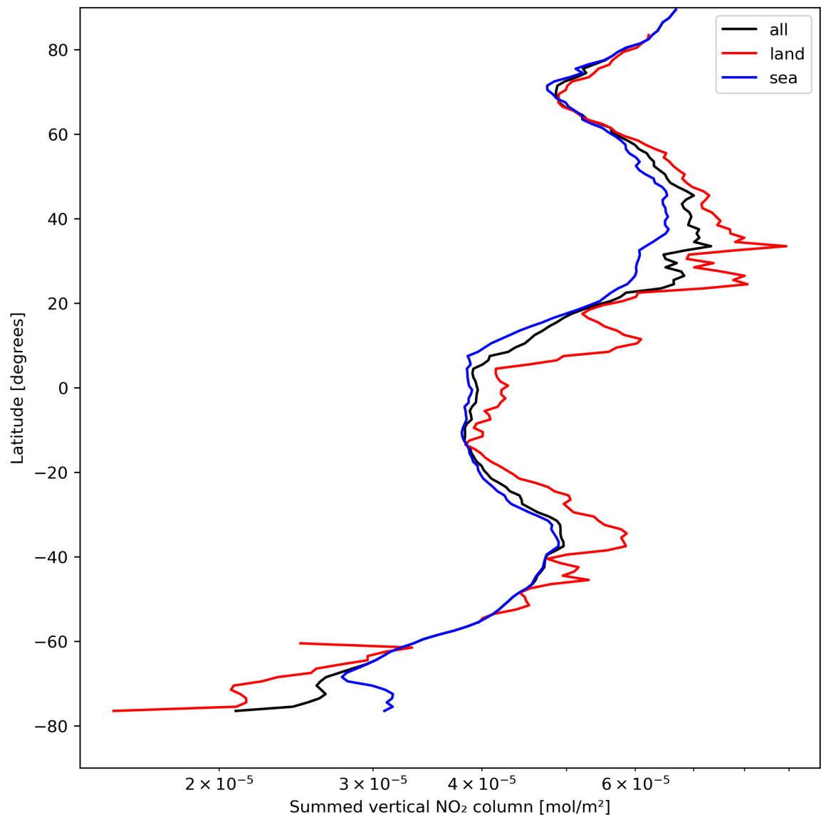
Figure 23: Zonal average of “Summed vertical NO 2 column” for 2024-04-19 to 2024-04-21.
