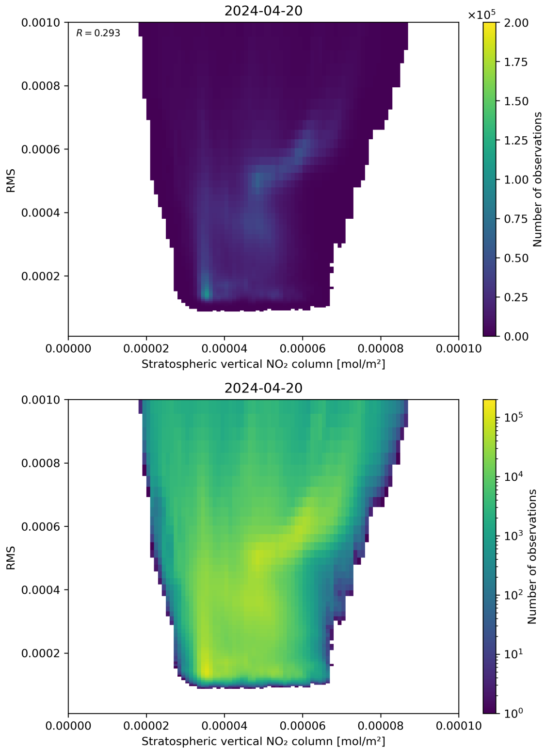
Figure 102: Scatter density plot of “Stratospheric vertical NO 2 column” against “RMS” for 2024-04-19 to 2024-04-21.
