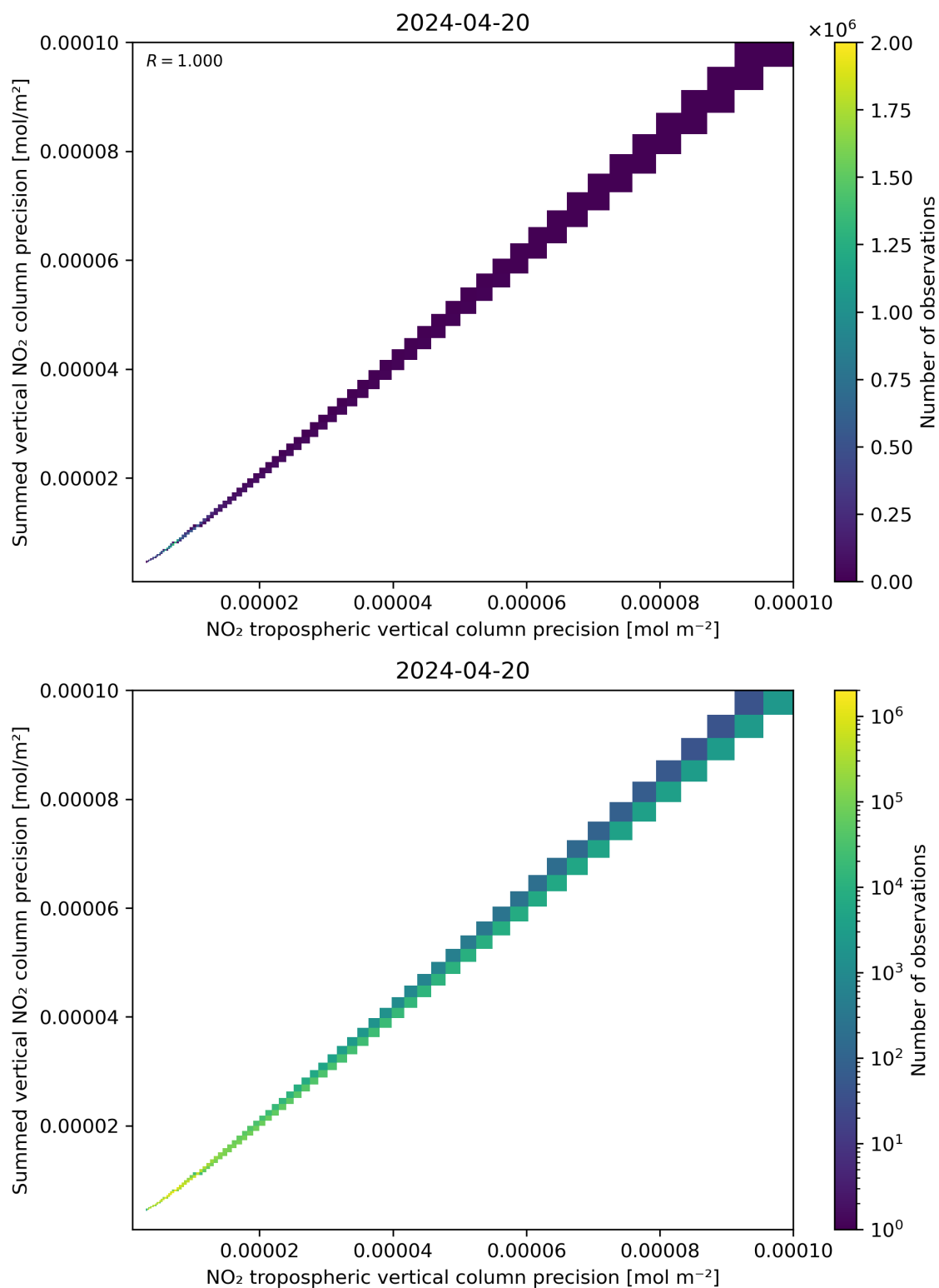
Figure 137: Scatter density plot of “NO 2 tropospheric vertical column precision” against “Summed vertical NO 2 column precision” for 2024-04-19 to 2024-04-21.
