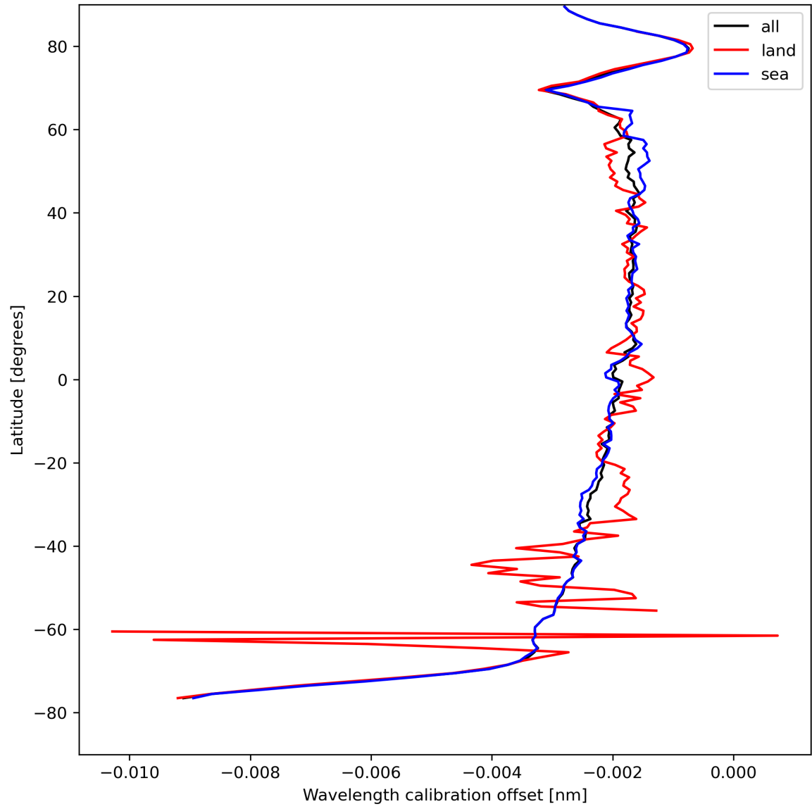
Figure 18: Zonal average of “Wavelength calibration offset” for 2024-04-19 to 2024-04-21.
