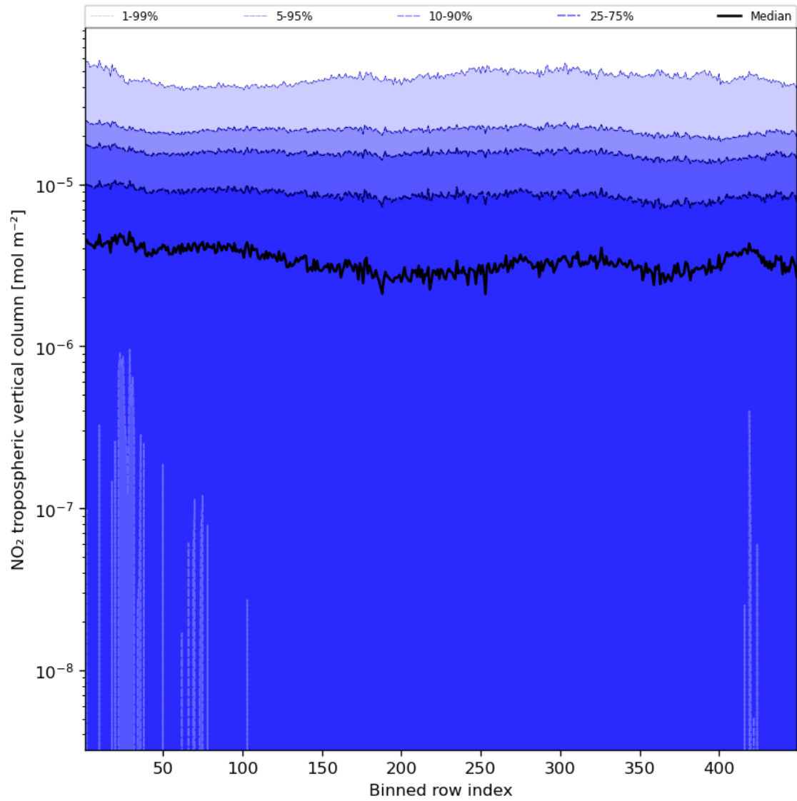
Figure 46: Along track statistics of “NO 2 tropospheric vertical column” for 2024-04-19 to 2024-04-21
