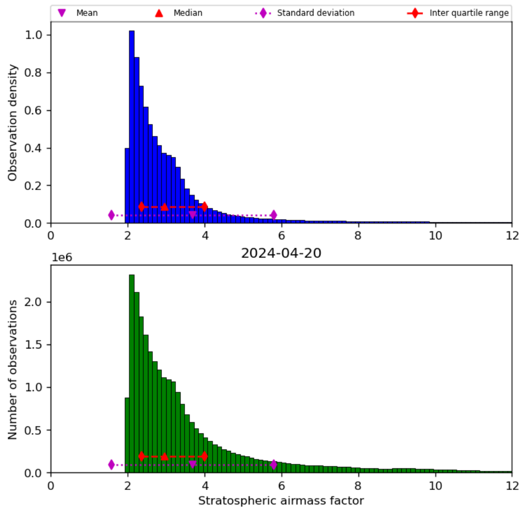
Figure 44: Histogram of “Stratospheric airmass factor” for 2024-04-19 to 2024-04-21
