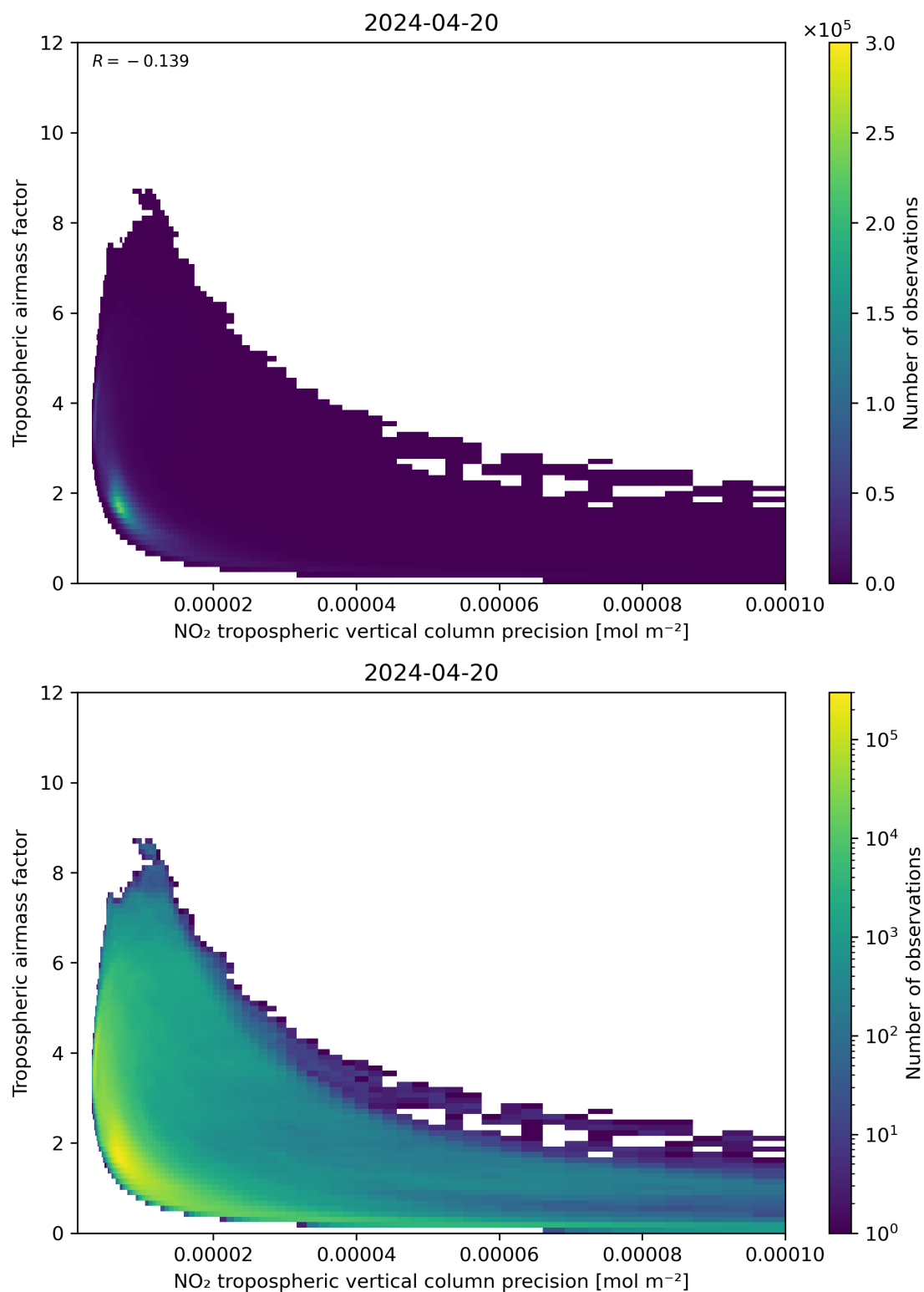
Figure 133: Scatter density plot of “NO 2 tropospheric vertical column precision” against “Tropospheric airmass factor” for 2024-04-19 to 2024-04-21.
