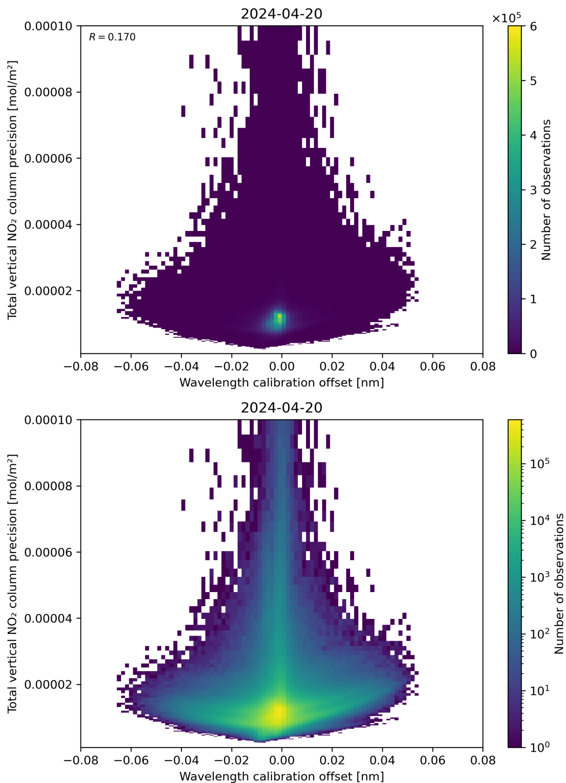
Figure 180: Scatter density plot of “Wavelength calibration offset” against “Total vertical NO 2 column precision” for 2024-04-19 to 2024-04-21.
