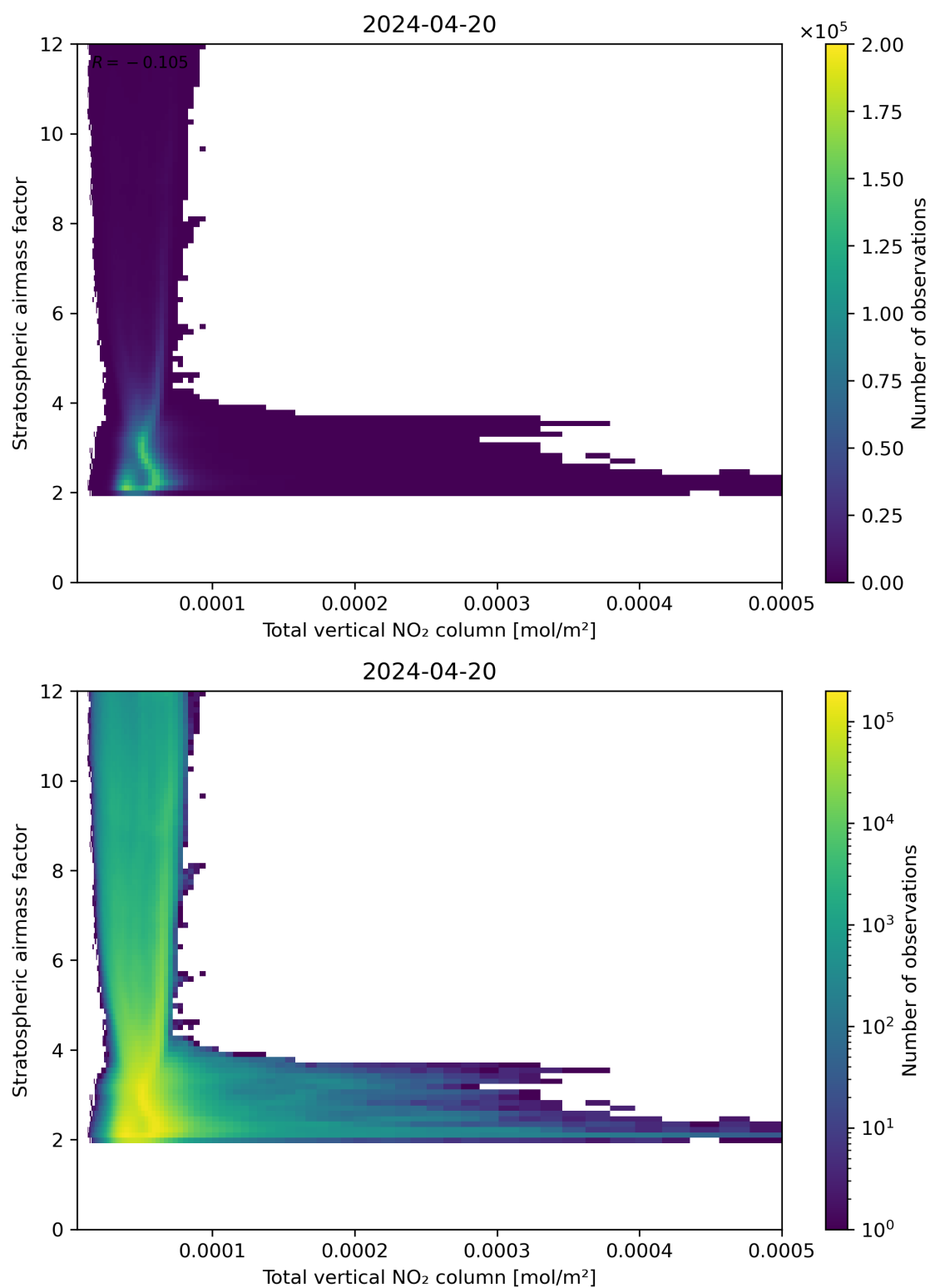
Figure 110: Scatter density plot of “Total vertical NO 2 column” against “Stratospheric airmass factor” for 2024-04-19 to 2024-04-21.
