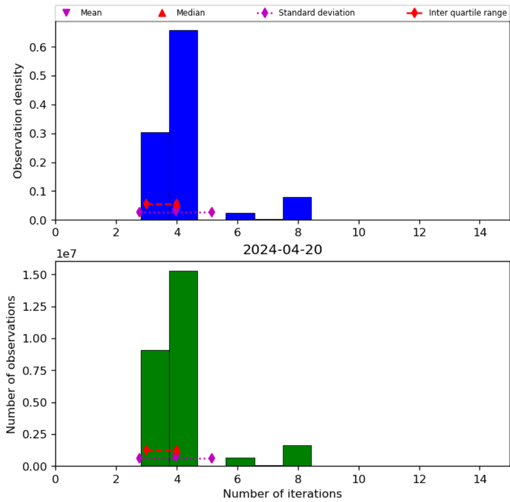
Figure 34: Histogram of “Number of iterations” for 2024-04-19 to 2024-04-21
