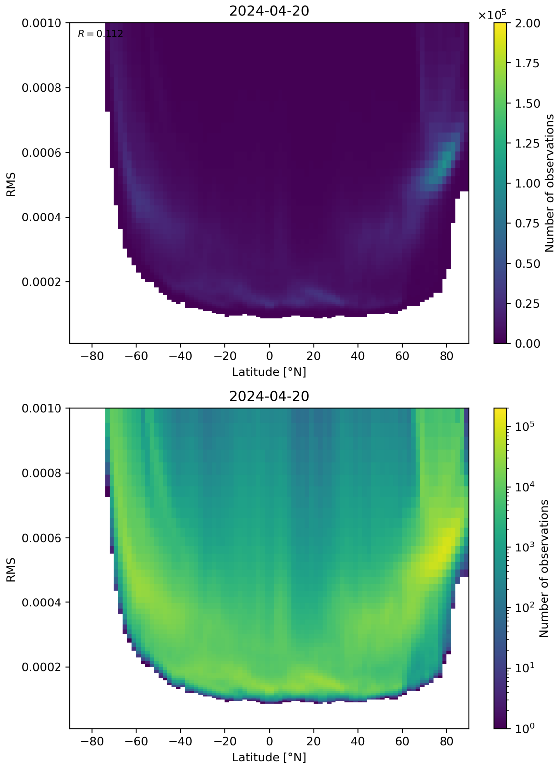
Figure 94: Scatter density plot of “Latitude” against “RMS” for 2024-04-19 to 2024-04-21.
