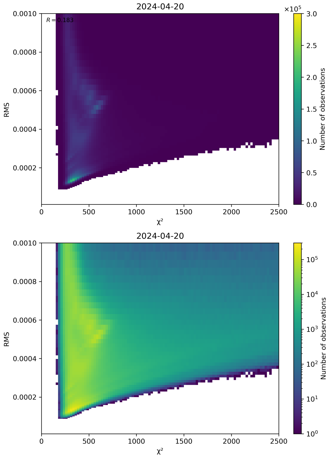
Figure 82: Scatter density plot of “ \chi^2 ” against “RMS” for 2024-04-19 to 2024-04-21.
