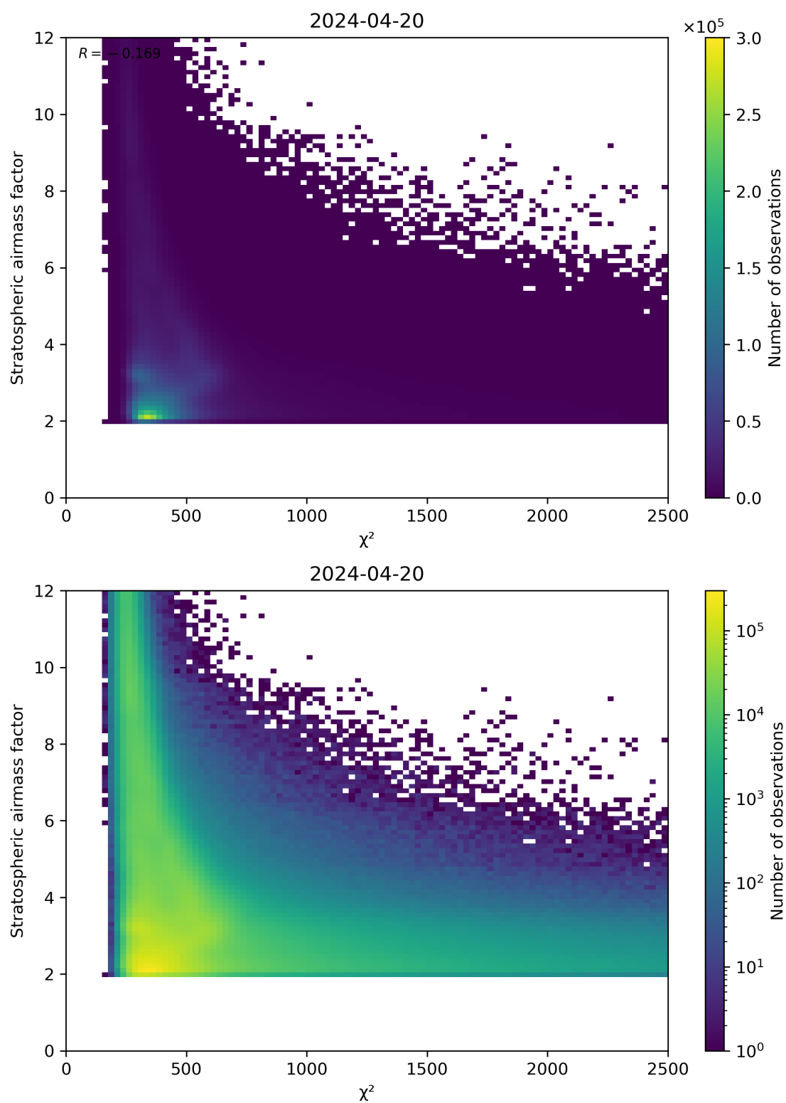
Figure 81: Scatter density plot of “ \chi^2 ” against “Stratospheric air mass factor” for 2024-04-19 to 2024-04-21.
