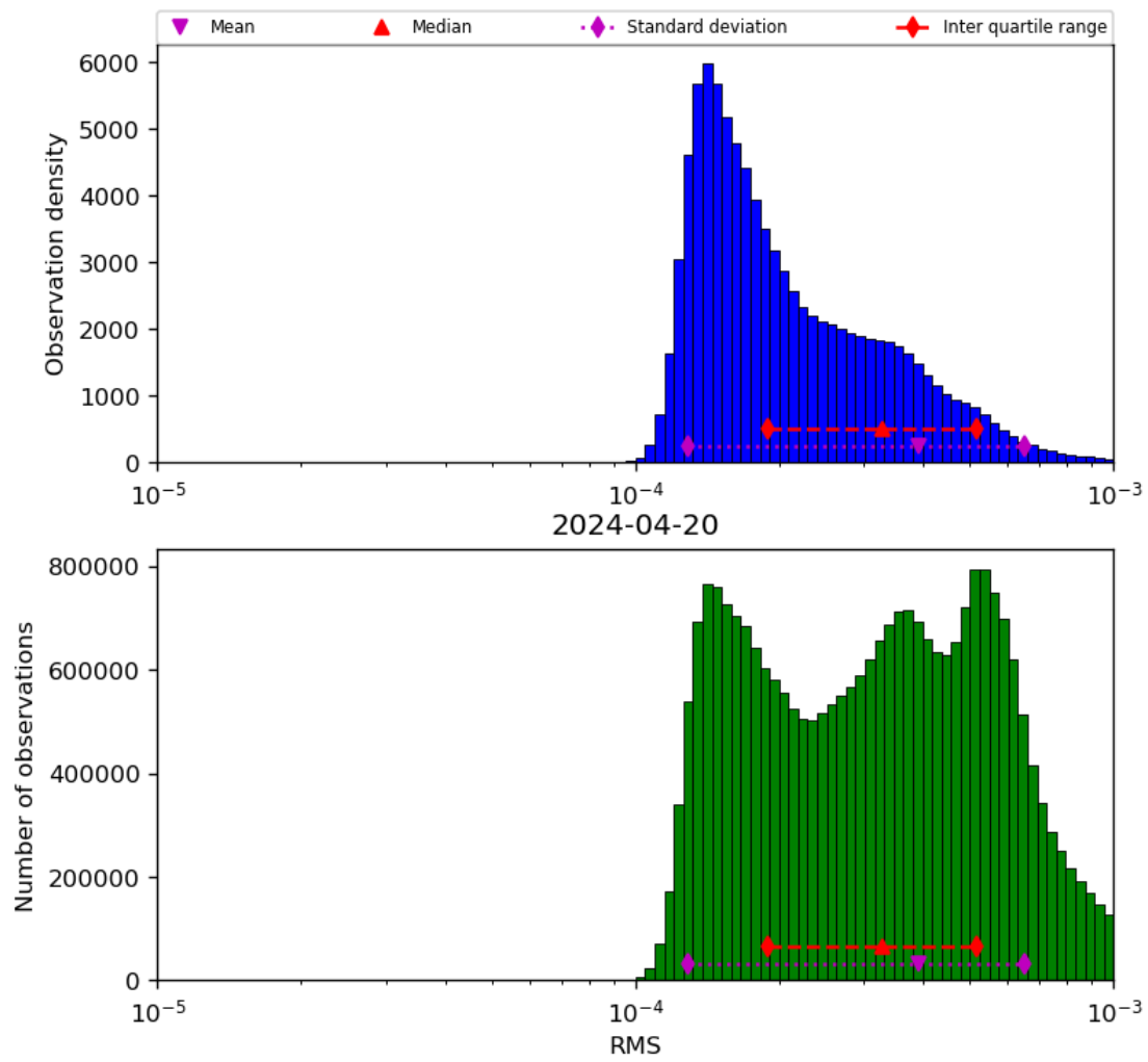
Figure 43: Histogram of “RMS” for 2024-04-19 to 2024-04-21
