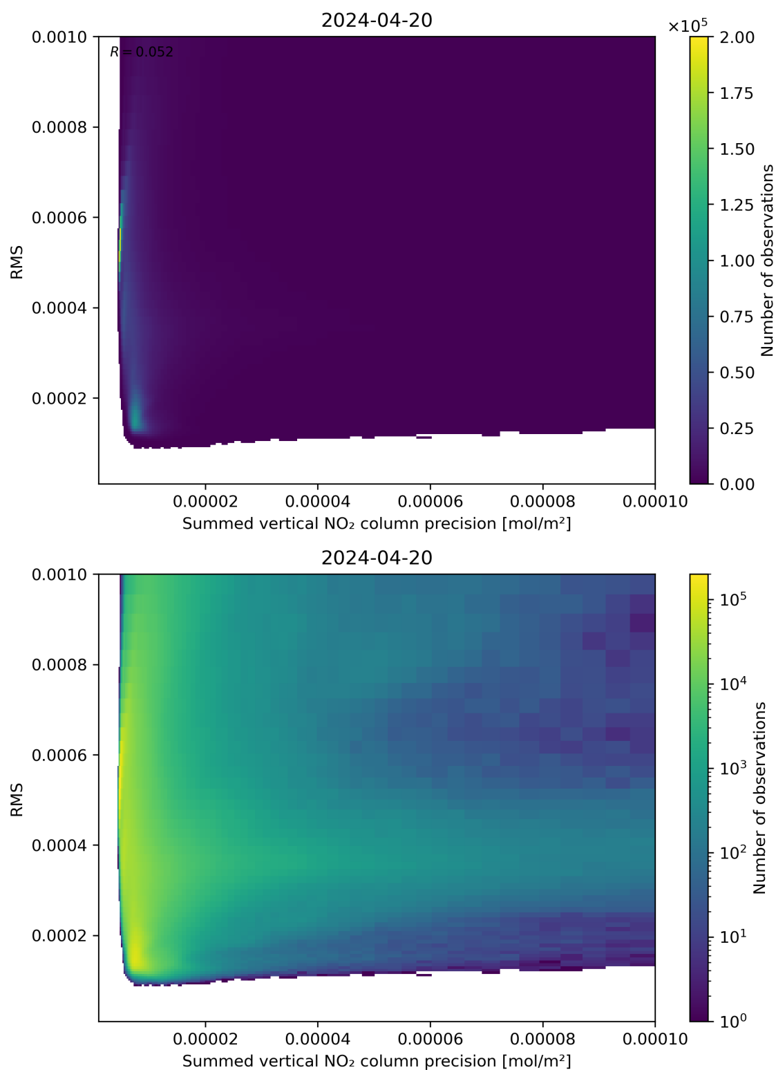
Figure 108: Scatter density plot of “Summed vertical NO 2 column precision” against “RMS” for 2024-04-19 to 2024-04-21.
