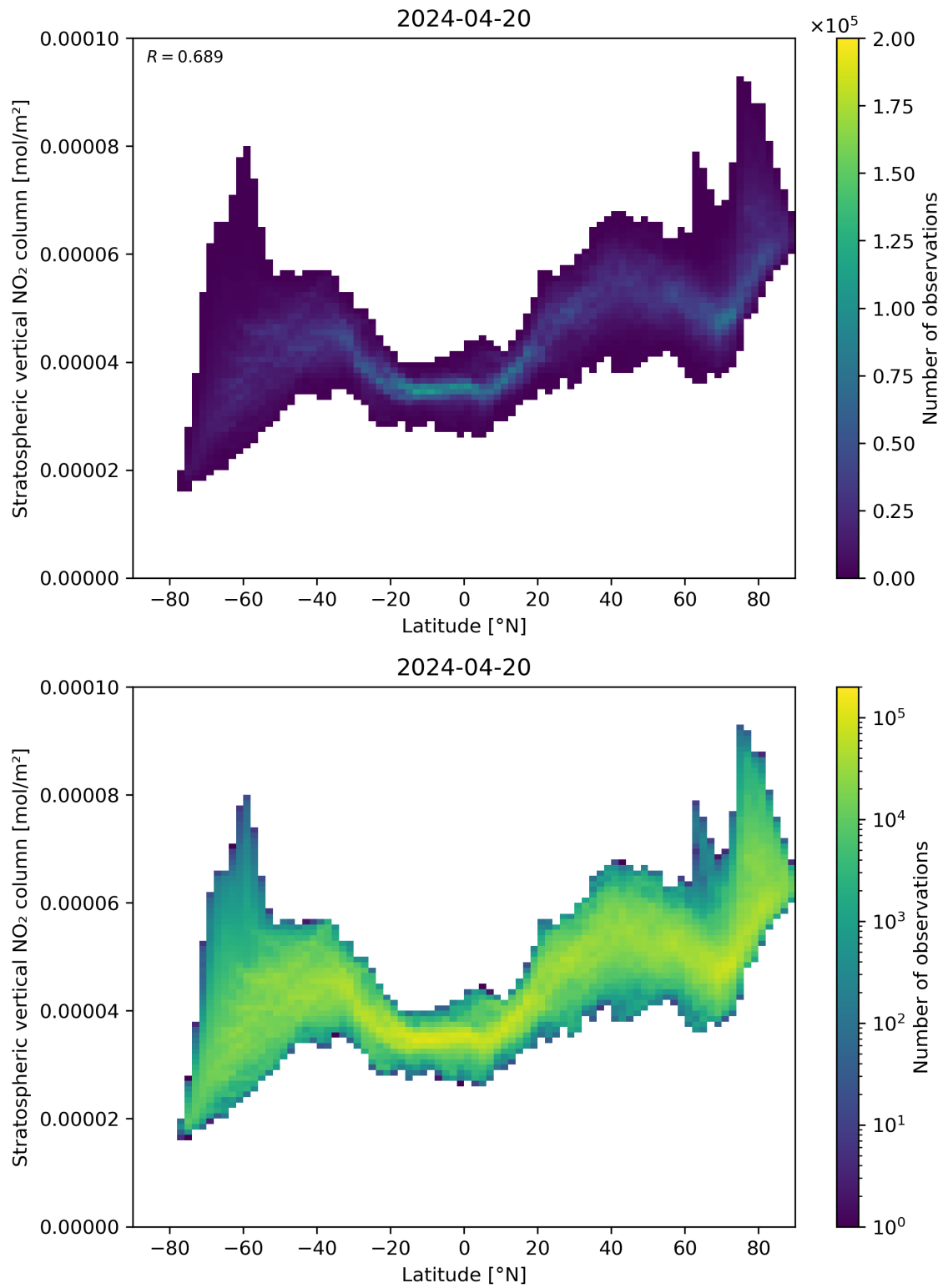
Figure 87: Scatter density plot of “Latitude” against “Stratospheric vertical NO 2 column” for 2024-04-19 to 2024-04-21.
