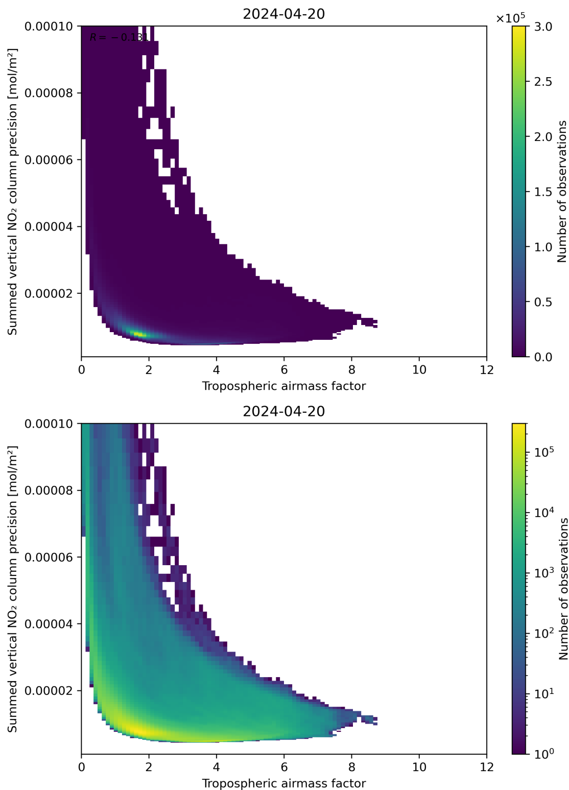
Figure 76: Scatter density plot of “Tropospheric air mass factor” against “Summed vertical NO 2 column precision” for 2024-04-19 to 2024-04-21.
