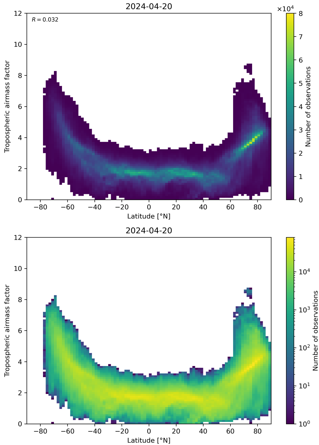
Figure 85: Scatter density plot of “Latitude” against “Tropospheric airmass factor” for 2024-04-19 to 2024-04-21.
