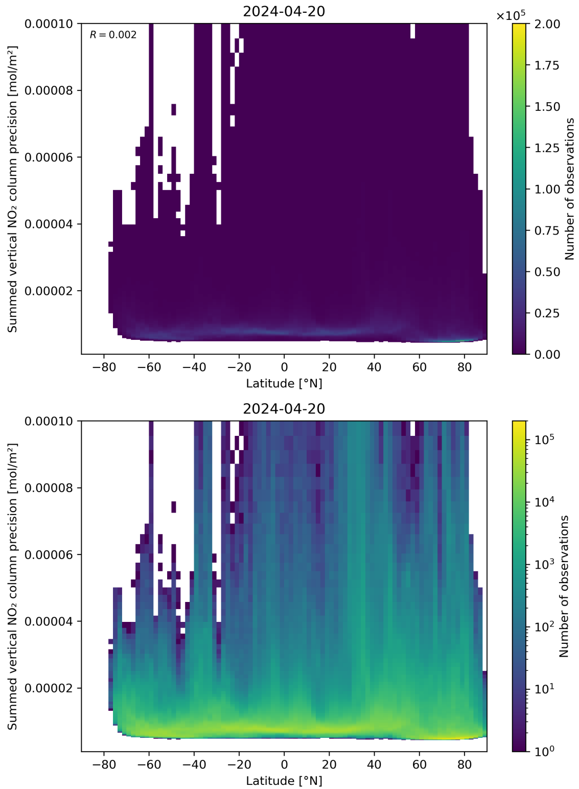
Figure 89: Scatter density plot of “Latitude” against “Summed vertical NO 2 column precision” for 2024-04-19 to 2024-04-21.
