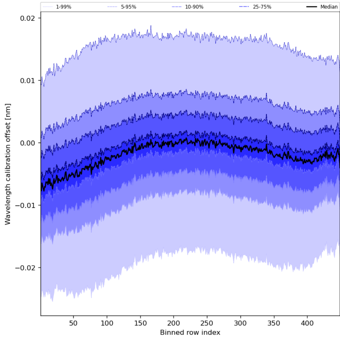
Figure 52: Along track statistics of “Wavelength calibration offset” for 2024-04-19 to 2024-04-21
