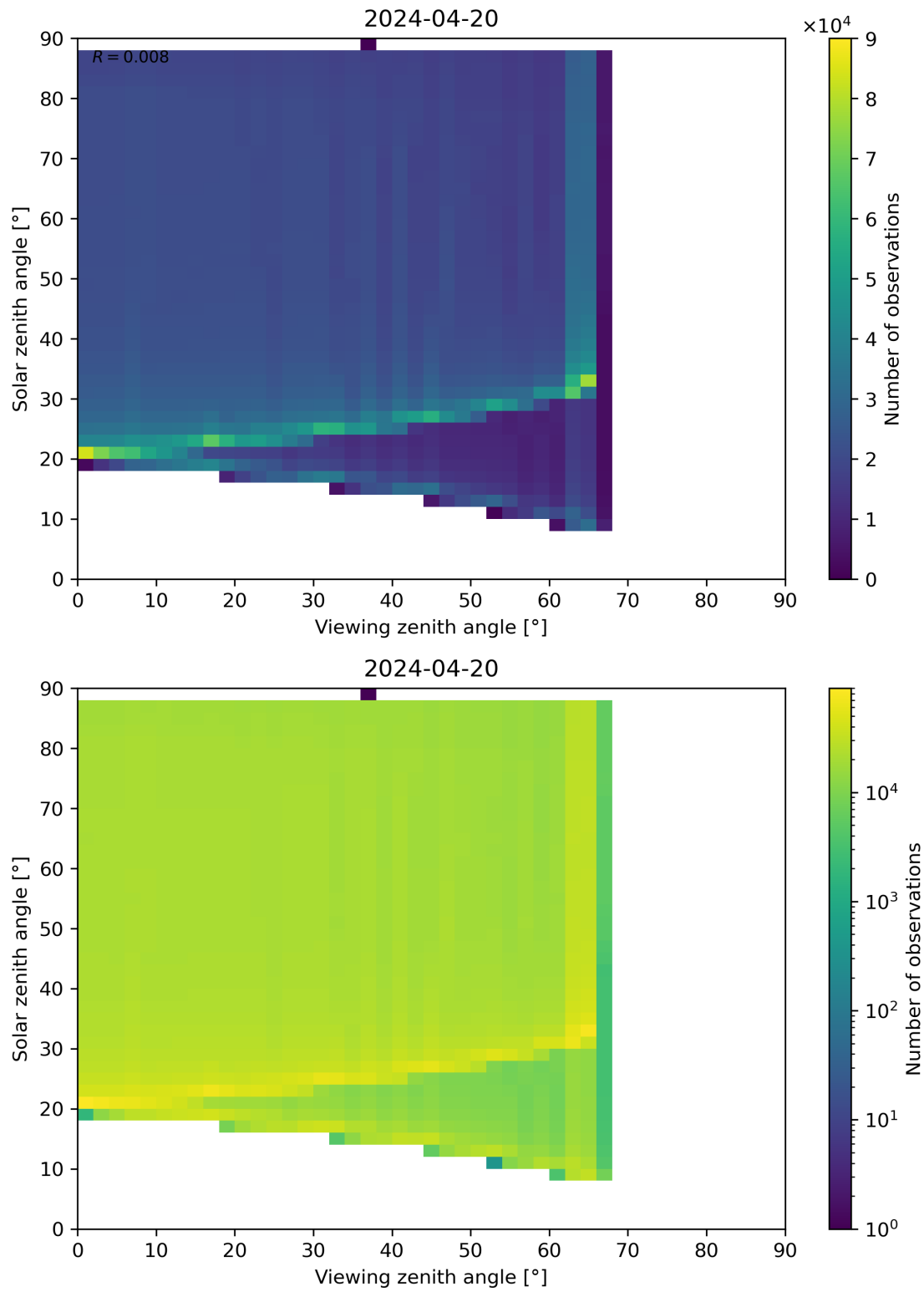
Figure 172: Scatter density plot of “Viewing zenith angle” against “Solar zenith angle” for 2024-04-19 to 2024-04-21.
