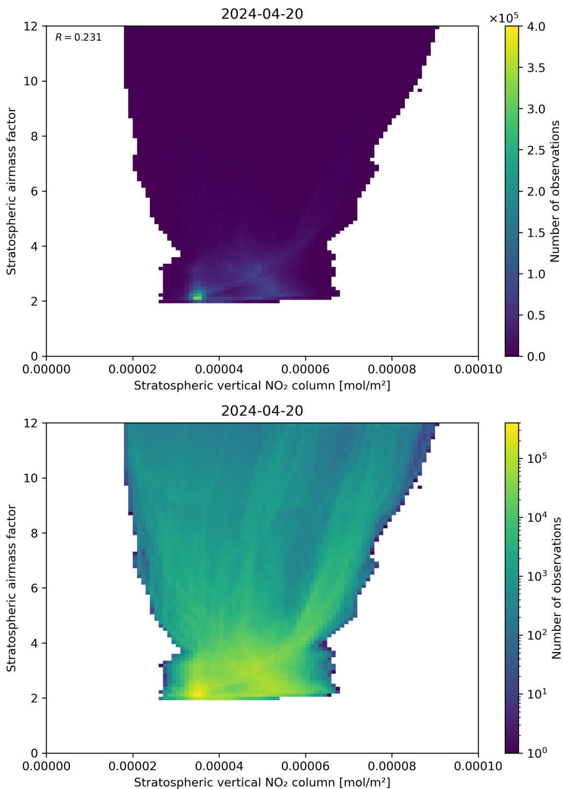
Figure 96: Scatter density plot of “Stratospheric vertical NO 2 column” against “Stratospheric airmass factor” for 2024-04-19 to 2024-04-21.
