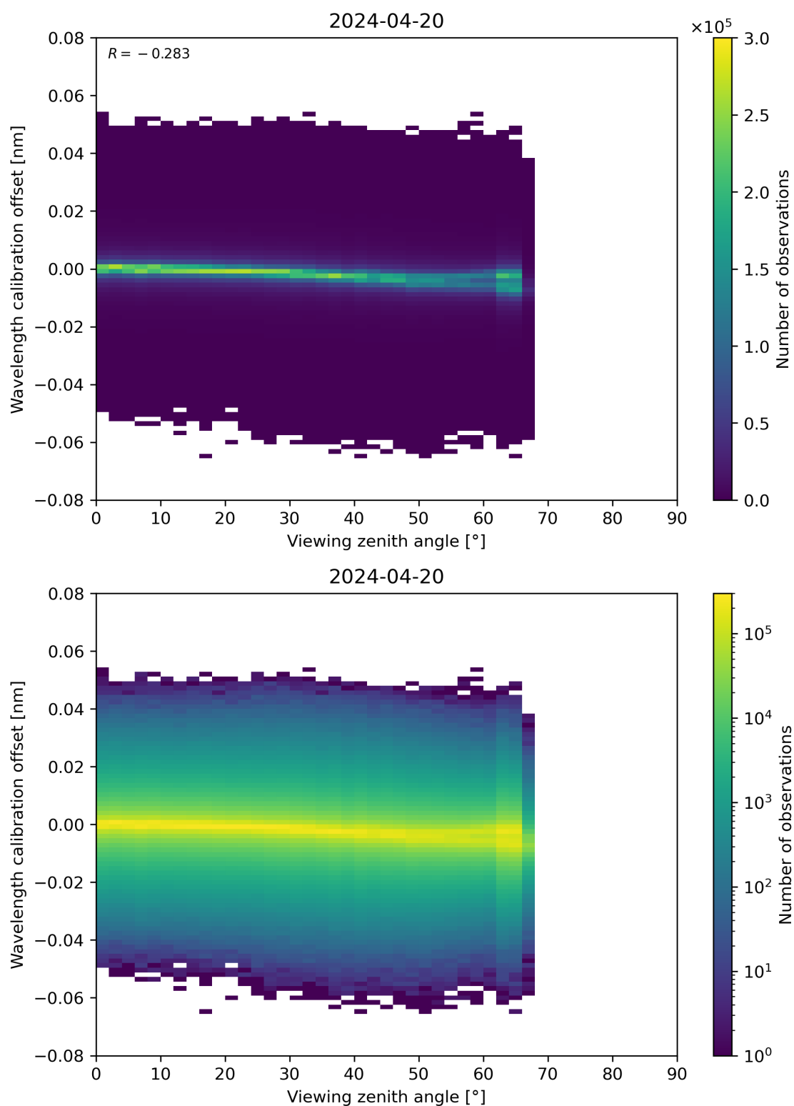
Figure 173: Scatter density plot of “Viewing zenith angle” against “Wavelength calibration offset” for 2024-04-19 to 2024-04-21.
