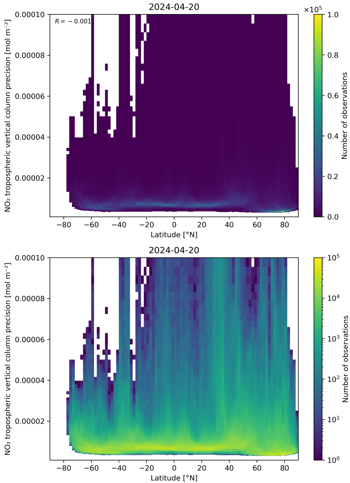
Figure 93: Scatter density plot of “Latitude” against “NO 2 tropospheric vertical column precision” for 2024-04-19 to 2024-04-21.
