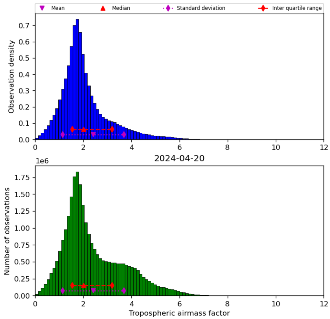
Figure 31: Histogram of “Tropospheric airmass factor” for 2024-04-19 to 2024-04-21
