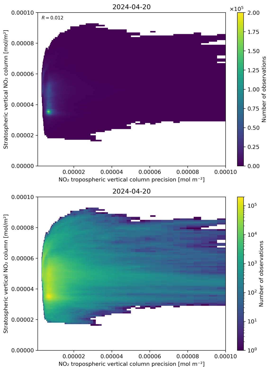
Figure 135: Scatter density plot of “NO 2 tropospheric vertical column precision” against “Stratospheric vertical NO 2 column” for 2024-04-19 to 2024-04-21.
