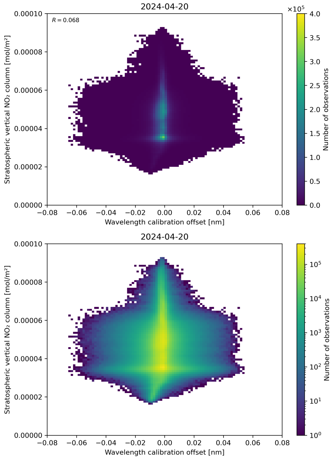
Figure 176: Scatter density plot of “Wavelength calibration offset” against “Stratospheric vertical NO 2 column” for 2024-04-19 to 2024-04-21.
