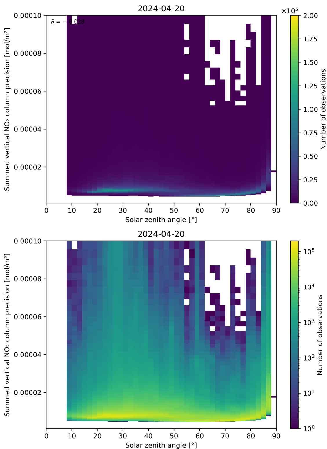
Figure 152: Scatter density plot of “Solar zenith angle” against “Summed vertical NO 2 column precision” for 2024-04-19 to 2024-04-21.
