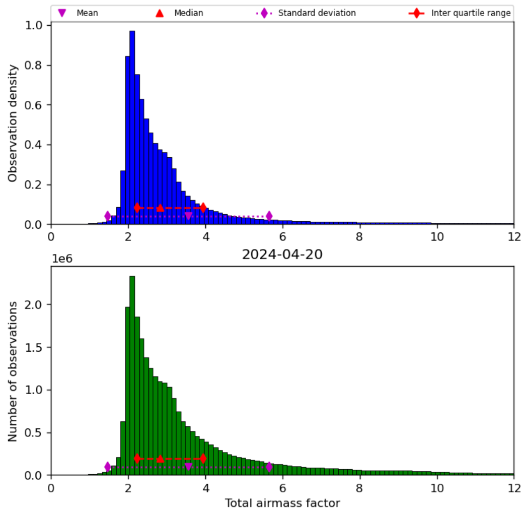
Figure 32: Histogram of “Total airmass factor” for 2024-04-19 to 2024-04-21
