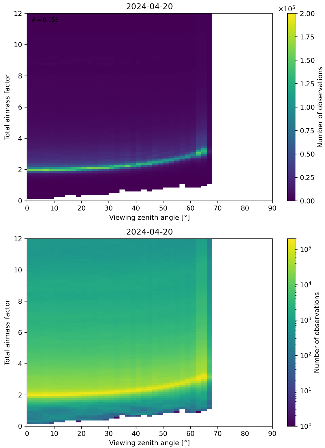
Figure 160: Scatter density plot of “Viewing zenith angle” against “Total airmass factor” for 2024-04-19 to 2024-04-21.
