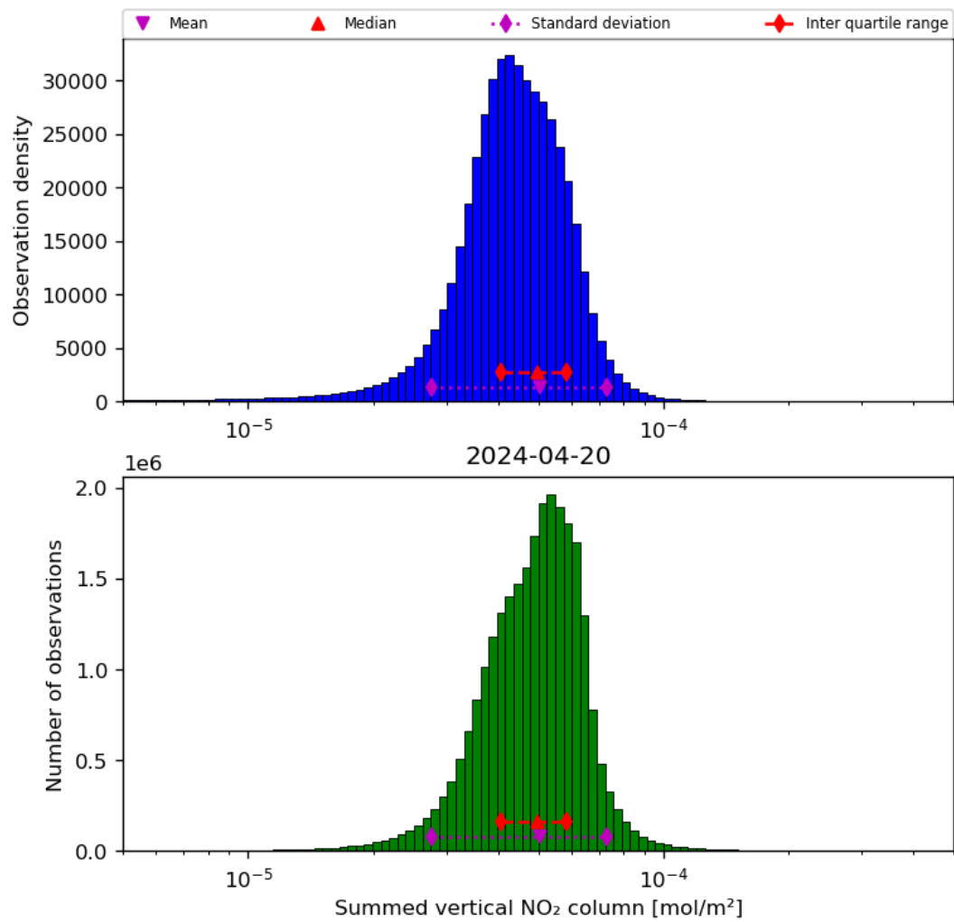
Figure 40: Histogram of “Summed vertical NO 2 column” for 2024-04-19 to 2024-04-21
