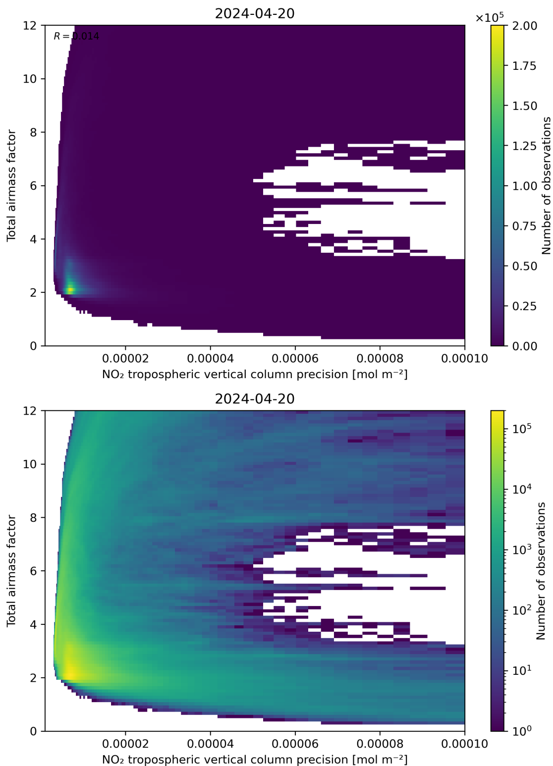
Figure 132: Scatter density plot of “NO 2 tropospheric vertical column precision” against “Total air mass factor” for 2024-04-19 to 2024-04-21.
