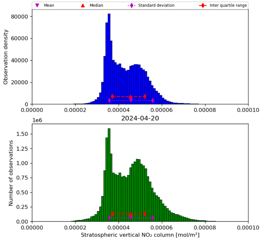
Figure 36: Histogram of “Stratospheric vertical NO 2 column” for 2024-04-19 to 2024-04-21
