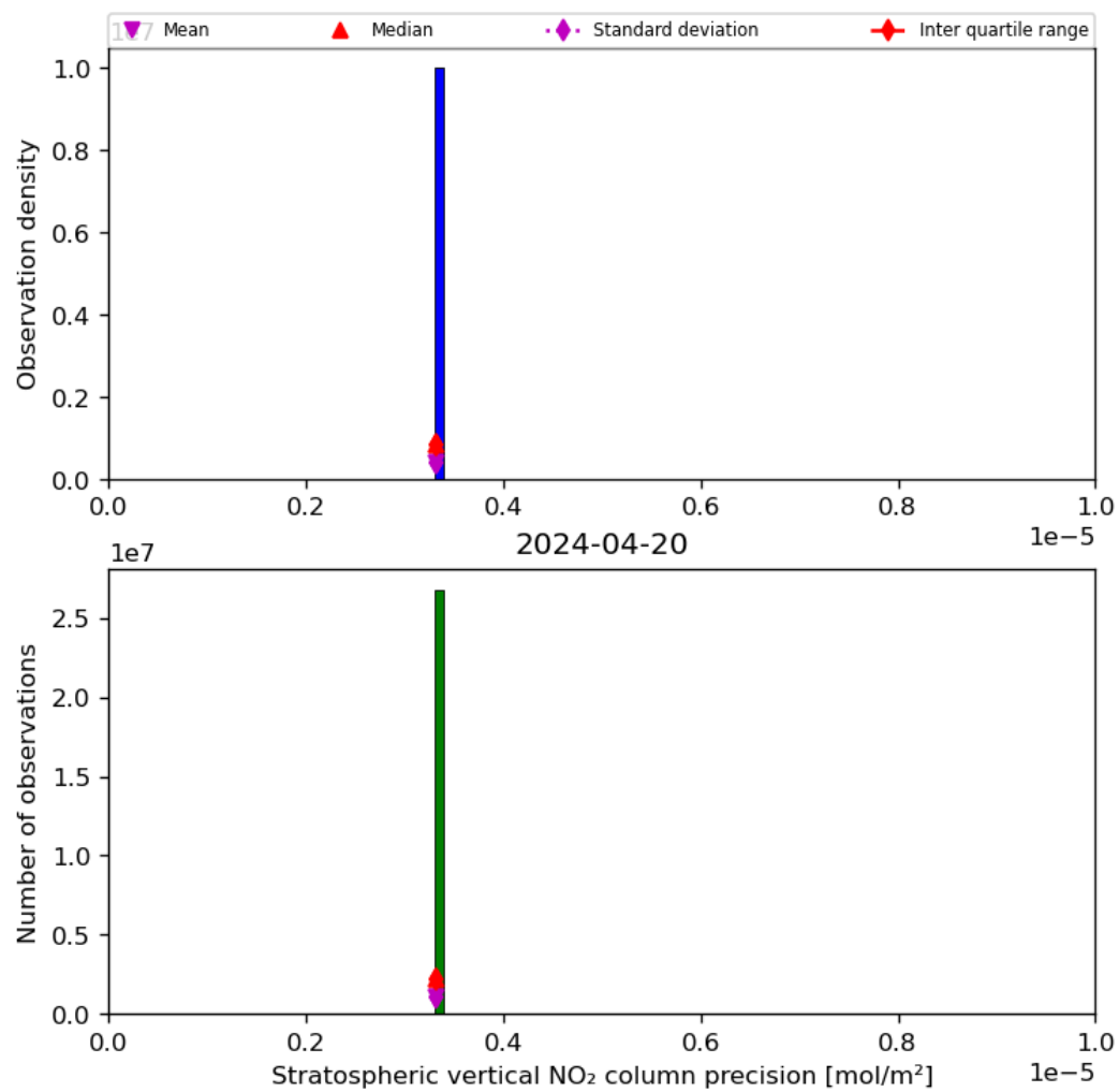
Figure 37: Histogram of “Stratospheric vertical NO 2 column precision” for 2024-04-19 to 2024-04-21
