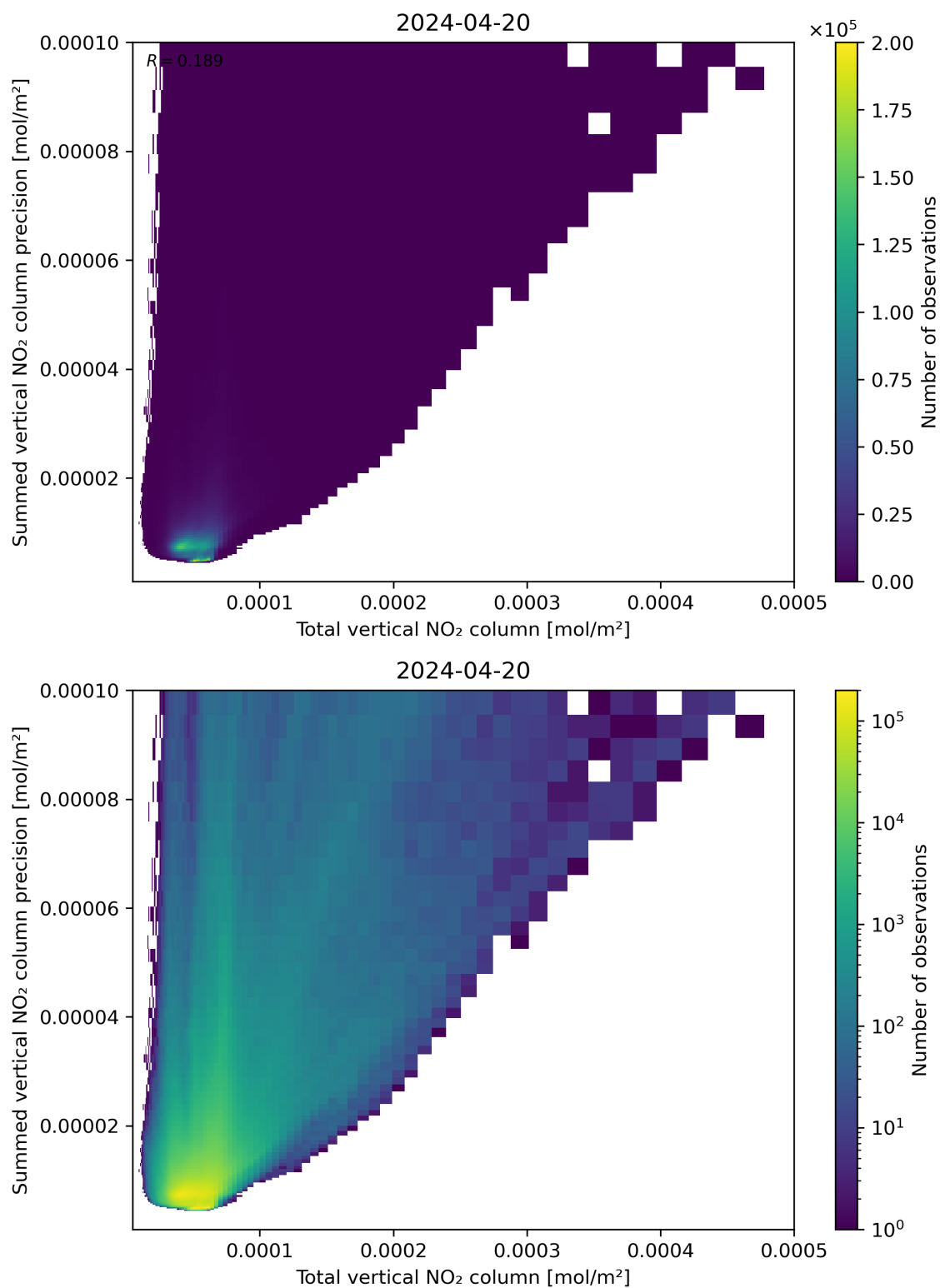
Figure 113: Scatter density plot of “Total vertical NO 2 column” against “Summed vertical NO 2 column precision” for 2024-04-19 to 2024-04-21.
