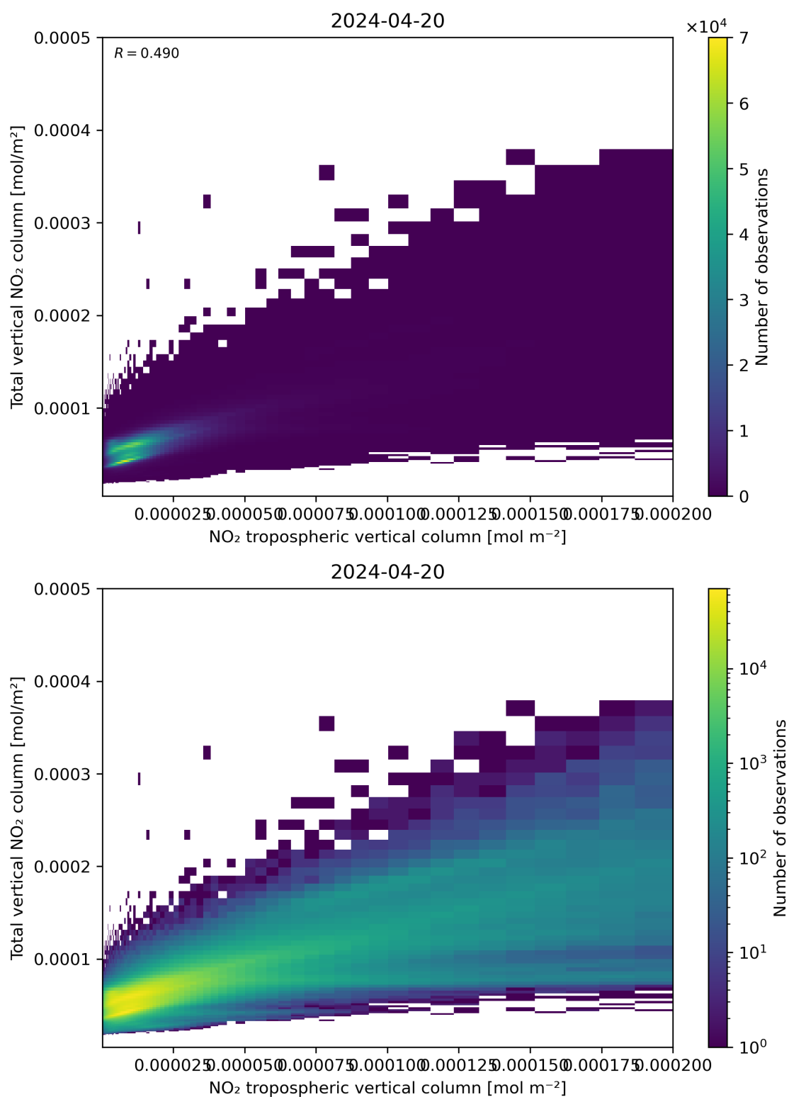
Figure 128: Scatter density plot of “NO 2 tropospheric vertical column” against “Total vertical NO 2 column” for 2024-04-19 to 2024-04-21.
