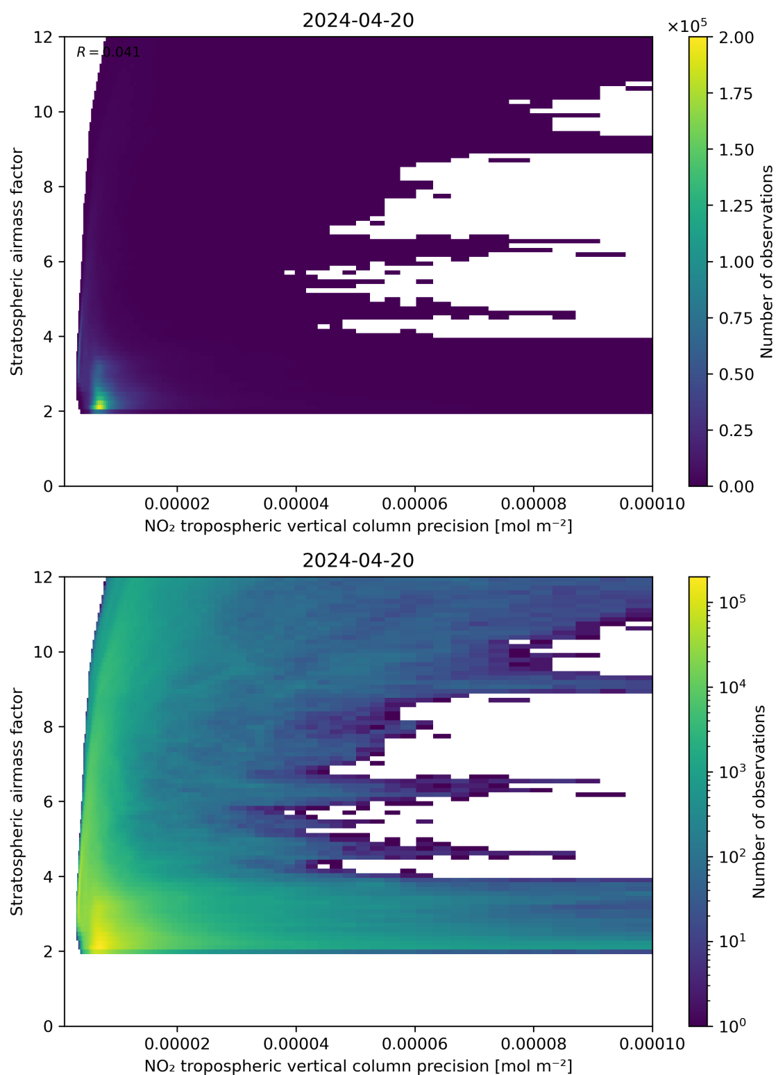
Figure 131: Scatter density plot of “NO 2 tropospheric vertical column precision” against “Stratospheric airmass factor” for 2024-04-19 to 2024-04-21.
