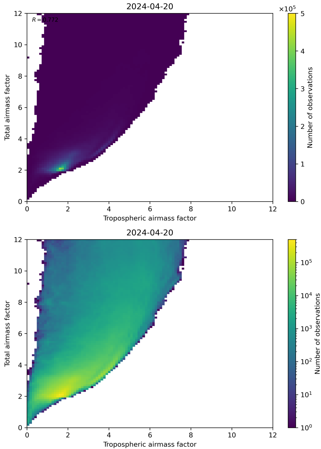
Figure 72: Scatter density plot of “Tropospheric airmass factor” against “Total airmass factor” for 2024-04-19 to 2024-04-21.
