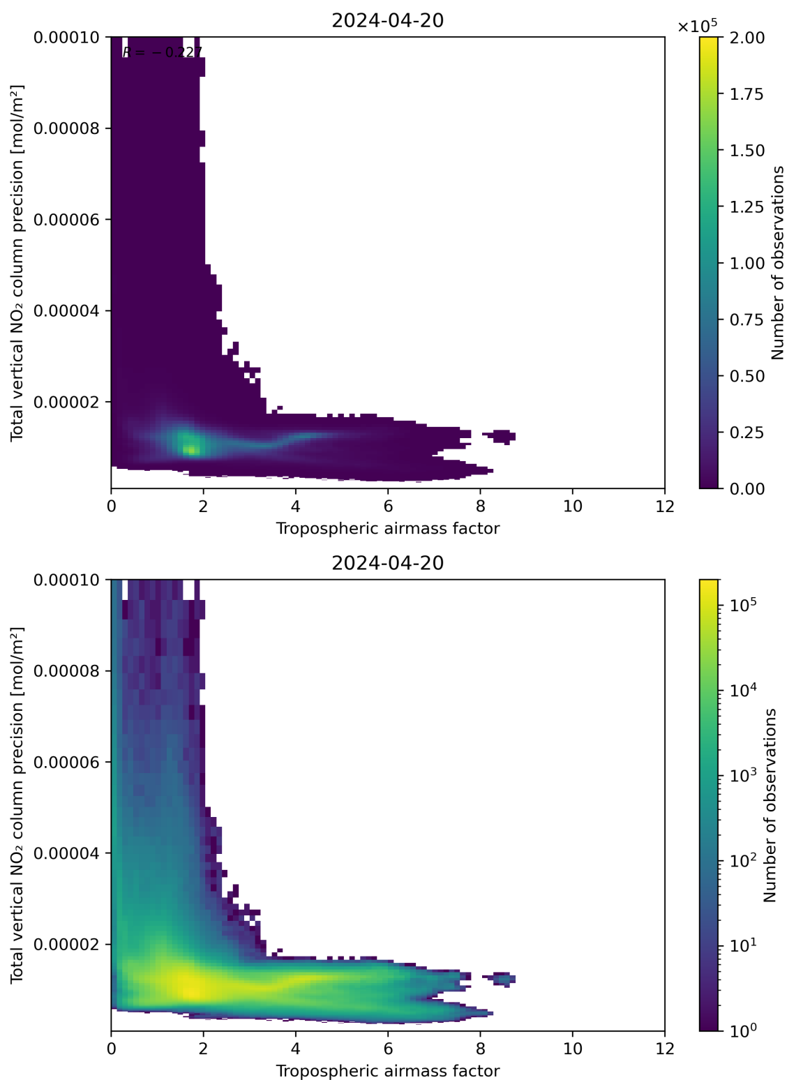
Figure 78: Scatter density plot of “Tropospheric air mass factor” against “Total vertical NO 2 column precision” for 2024-04-19 to 2024-04-21.
