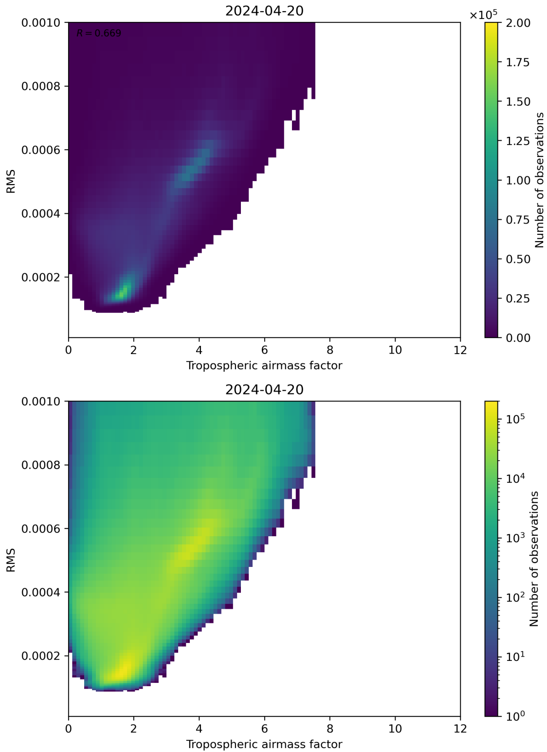
Figure 79: Scatter density plot of “Tropospheric airmass factor” against “RMS” for 2024-04-19 to 2024-04-21.
