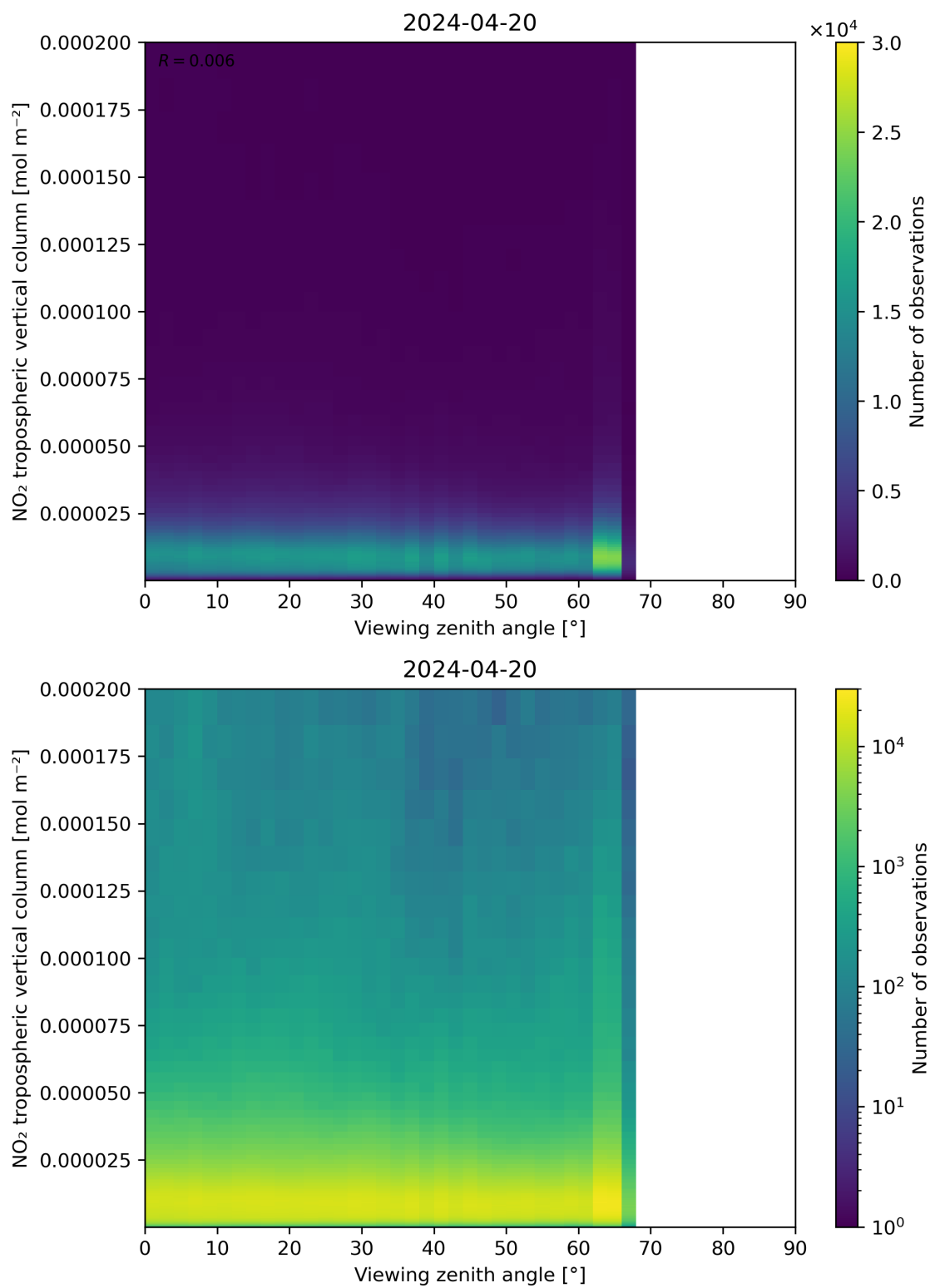
Figure 169: Scatter density plot of “Viewing zenith angle” against “NO 2 tropospheric vertical column” for 2024-04-19 to 2024-04-21.
