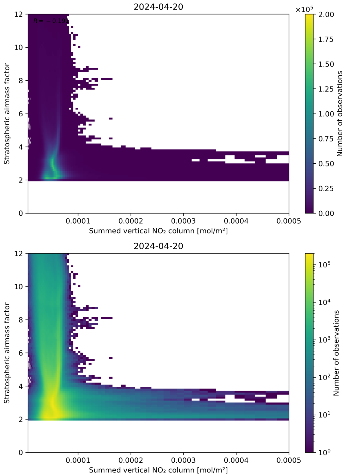
Figure 103: Scatter density plot of “Summed vertical NO 2 column” against “Stratospheric air mass factor” for 2024-04-19 to 2024-04-21.
