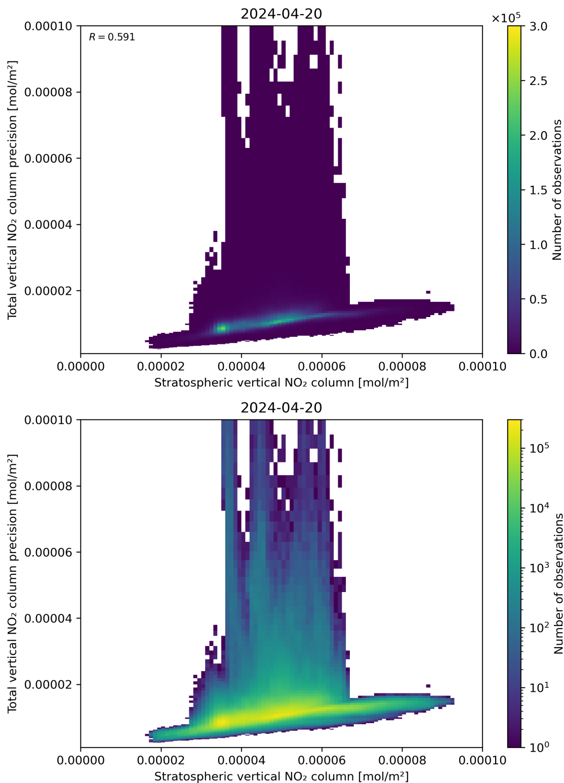
Figure 101: Scatter density plot of “Stratospheric vertical NO 2 column” against “Total vertical NO 2 column precision” for 2024-04-19 to 2024-04-21.
