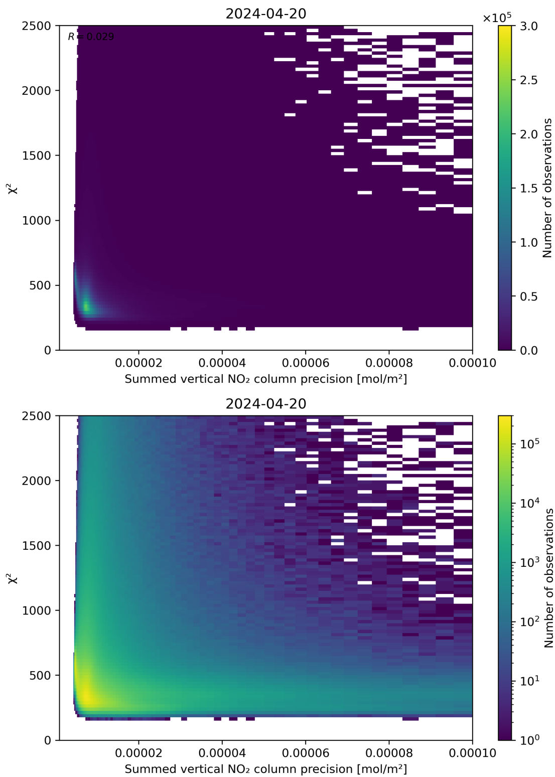
Figure 107: Scatter density plot of “Summed vertical NO 2 column precision” against “ \chi^2 ” for 2024-04-19 to 2024-04-21.
