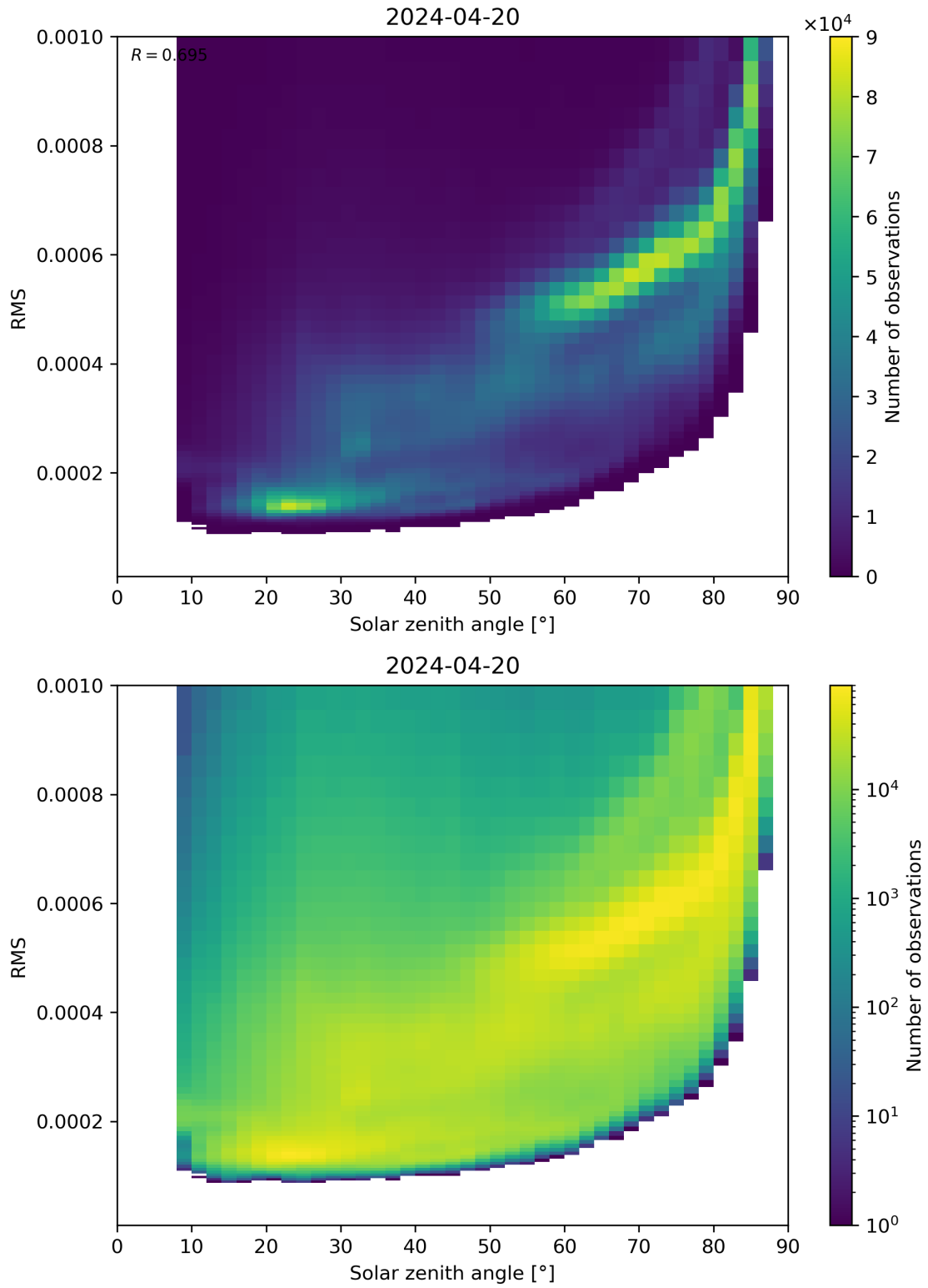
Figure 157: Scatter density plot of “Solar zenith angle” against “RMS” for 2024-04-19 to 2024-04-21.
