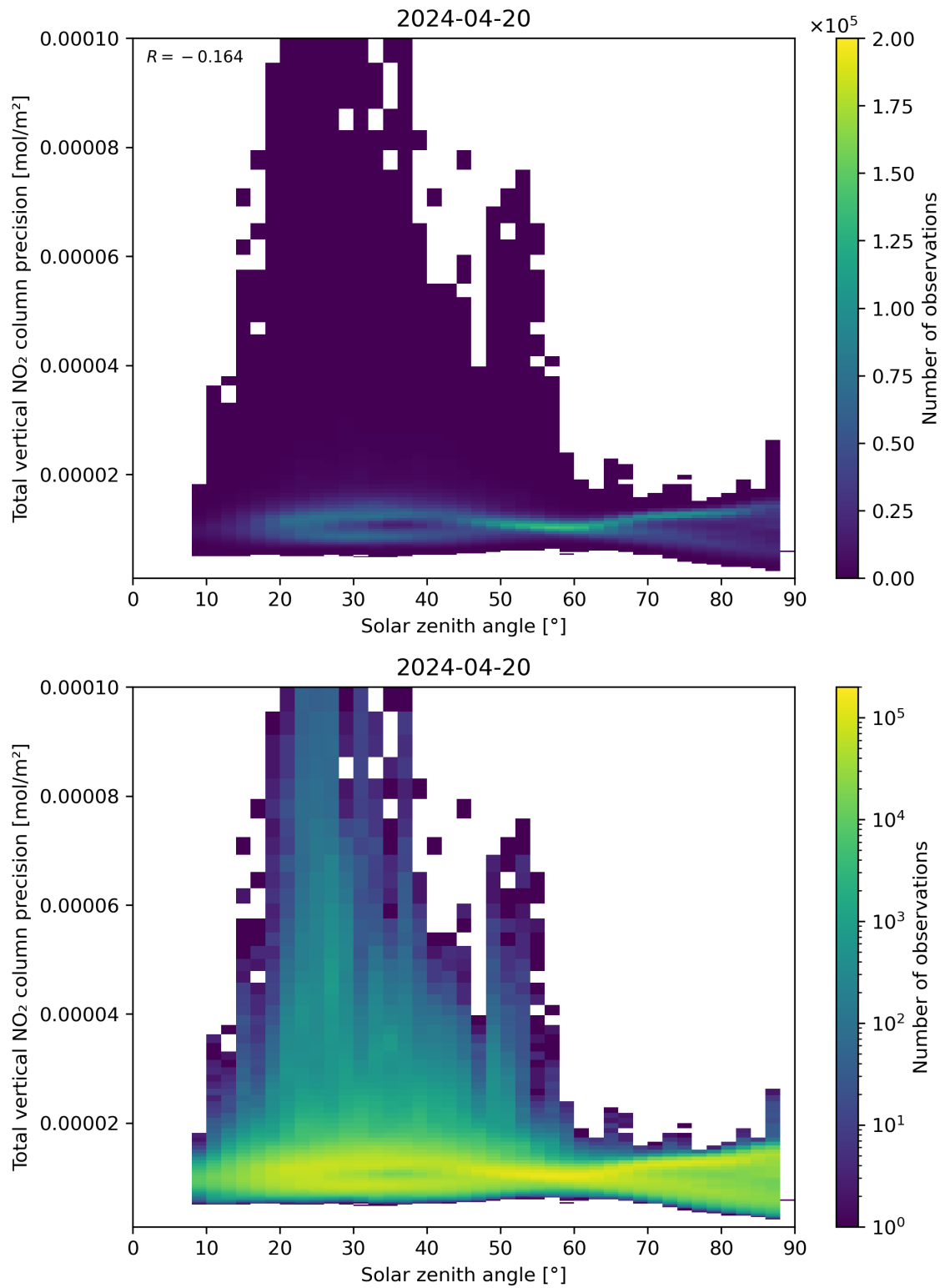
Figure 154: Scatter density plot of “Solar zenith angle” against “Total vertical NO 2 column precision” for 2024-04-19 to 2024-04-21.
