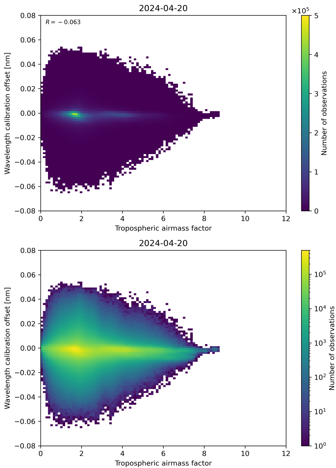
Figure 80: Scatter density plot of “Tropospheric airmass factor” against “Wavelength calibration offset” for 2024-04-19 to 2024-04-21.
