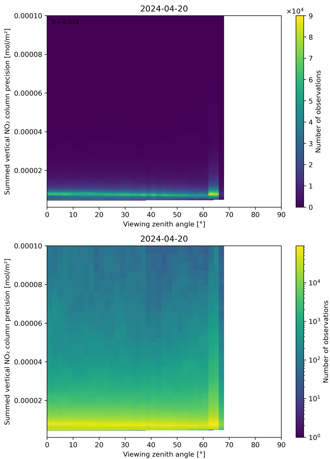
Figure 166: Scatter density plot of “Viewing zenith angle” against “Summed vertical NO 2 column precision” for 2024-04-19 to 2024-04-21.
