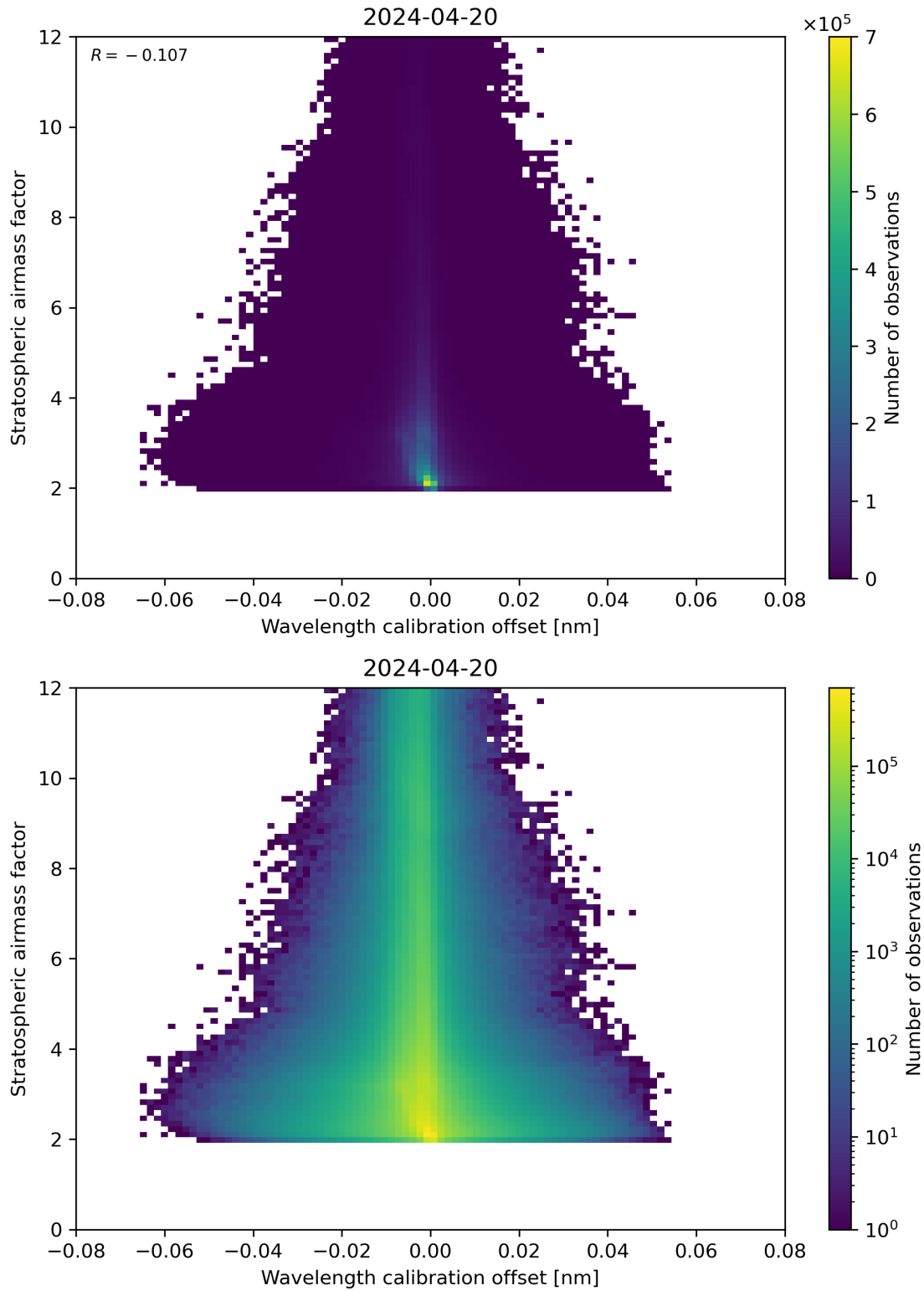
Figure 174: Scatter density plot of “Wavelength calibration offset” against “Stratospheric airmass factor” for 2024-04-19 to 2024-04-21.
