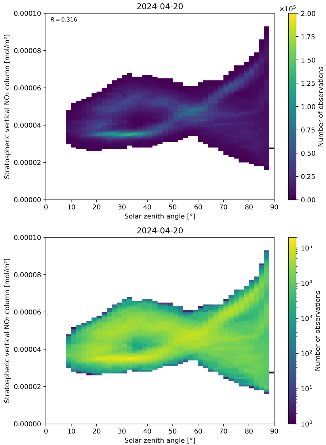
Figure 150: Scatter density plot of “Solar zenith angle” against “Stratospheric vertical NO 2 column” for 2024-04-19 to 2024-04-21.
