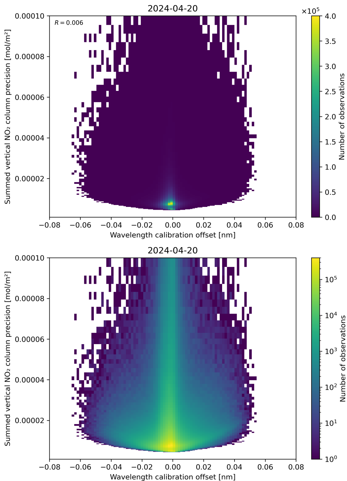
Figure 178: Scatter density plot of “Wavelength calibration offset” against “Summed vertical NO 2 column precision” for 2024-04-19 to 2024-04-21.
