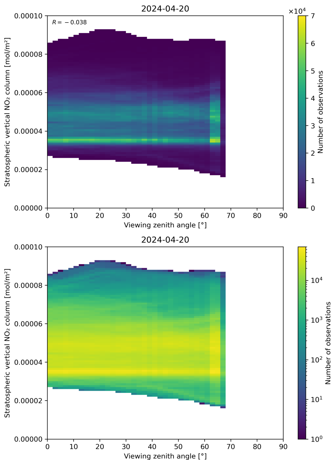
Figure 164: Scatter density plot of “Viewing zenith angle” against “Stratospheric vertical NO 2 column” for 2024-04-19 to 2024-04-21.
