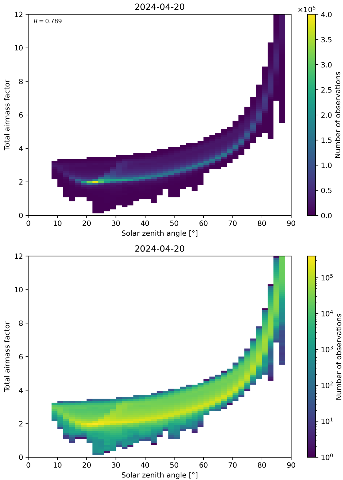
Figure 146: Scatter density plot of “Solar zenith angle” against “Total air mass factor” for 2024-04-19 to 2024-04-21.
