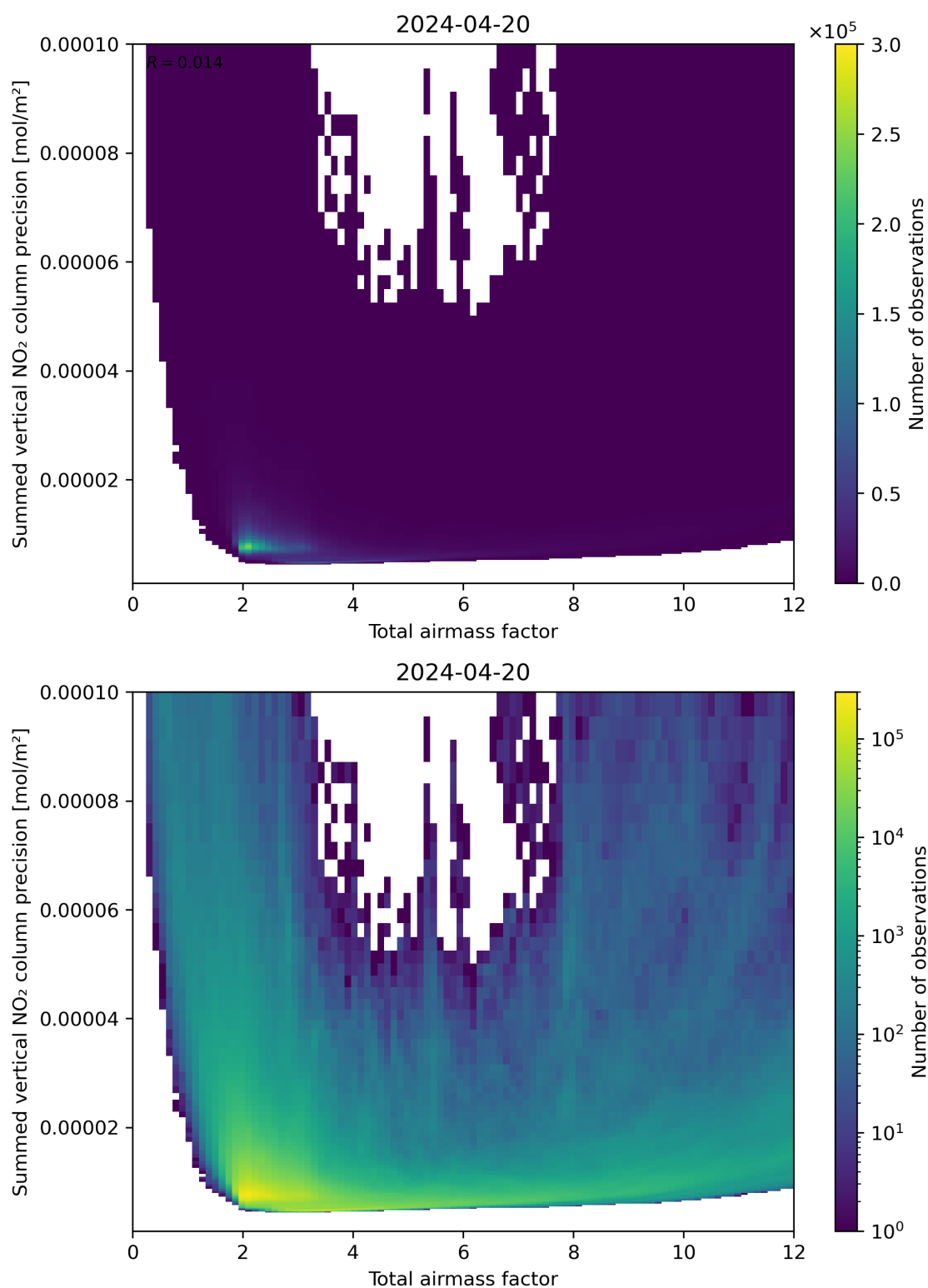
Figure 66: Scatter density plot of “Total airmass factor” against “Summed vertical NO 2 column precision” for 2024-04-19 to 2024-04-21.
