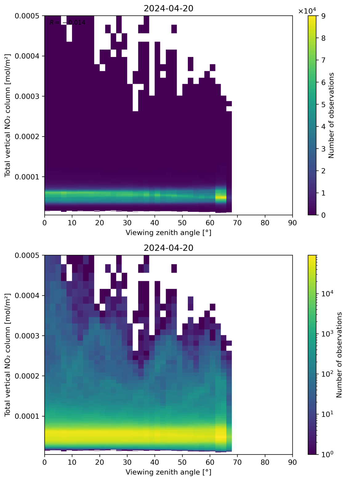
Figure 167: Scatter density plot of “Viewing zenith angle” against “Total vertical NO 2 column” for 2024-04-19 to 2024-04-21.
