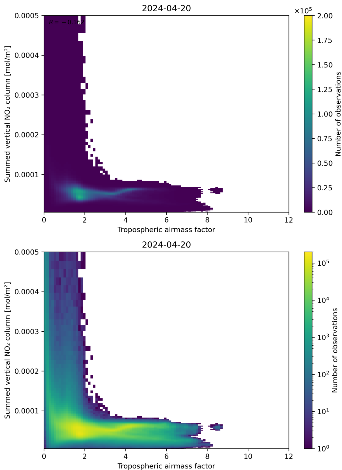
Figure 75: Scatter density plot of “Tropospheric air mass factor” against “Summed vertical NO 2 column” for 2024-04-19 to 2024-04-21.
