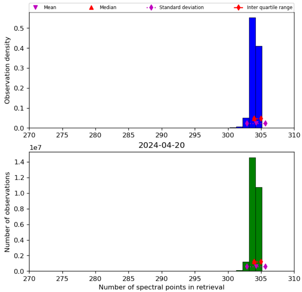
Figure 33: Histogram of "Number of spectral points in retrieval" for 2024-04-19 to 2024-04-21
