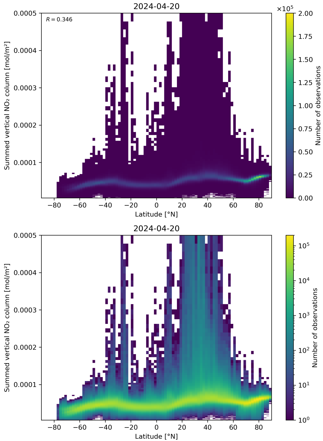
Figure 88: Scatter density plot of “Latitude” against “Summed vertical NO 2 column” for 2024-04-19 to 2024-04-21.
