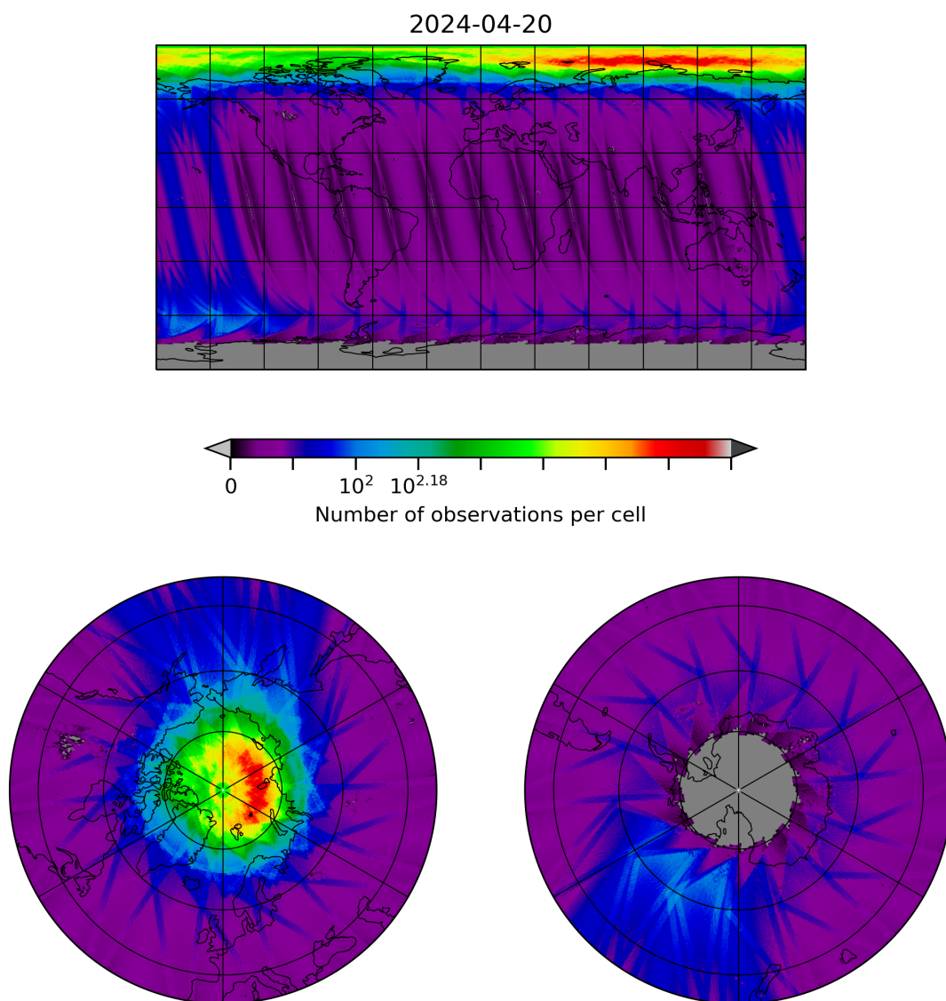
Figure 10: Map of the number of observations for 2024-04-19 to 2024-04-21
