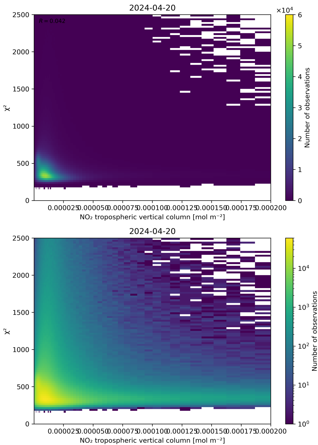
Figure 124: Scatter density plot of “NO 2 tropospheric vertical column” against “ \chi^2 ” for 2024-04-19 to 2024-04-21.
