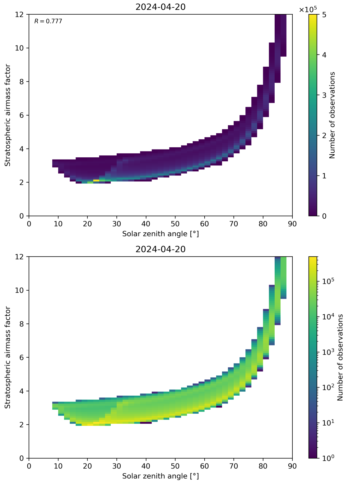
Figure 145: Scatter density plot of “Solar zenith angle” against “Stratospheric airmass factor” for 2024-04-19 to 2024-04-21.
