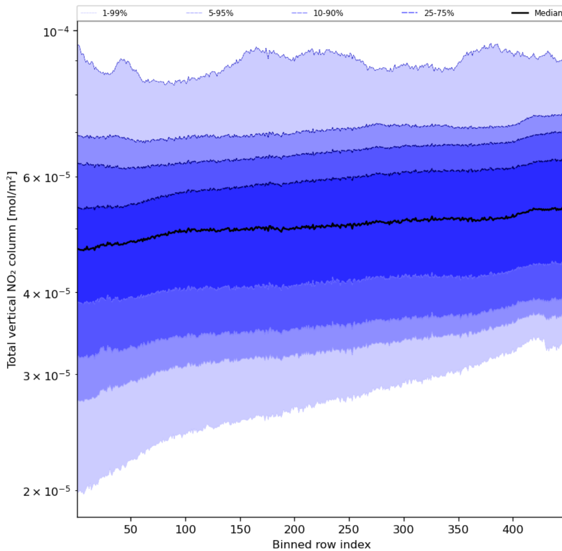
Figure 55: Along track statistics of “Total vertical NO 2 column” for 2024-04-19 to 2024-04-21
