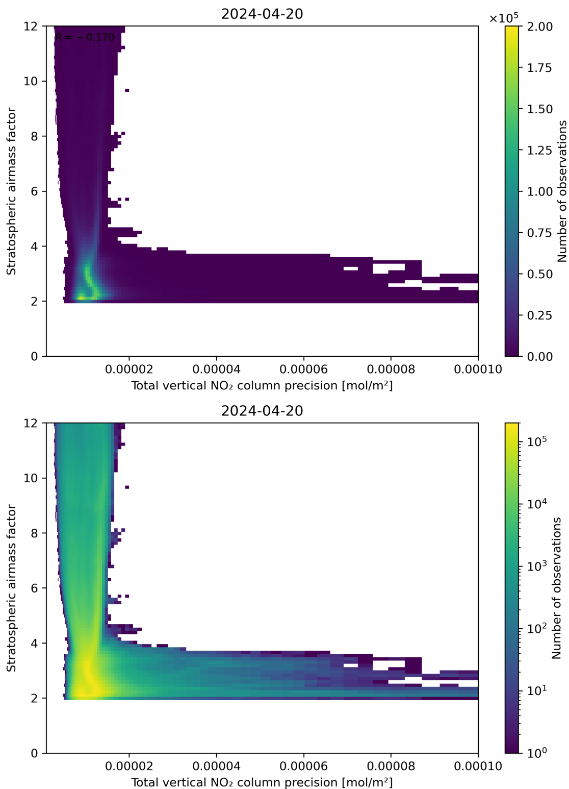
Figure 115: Scatter density plot of “Total vertical NO 2 column precision” against “Stratospheric air mass factor” for 2024-04-19 to 2024-04-21.
