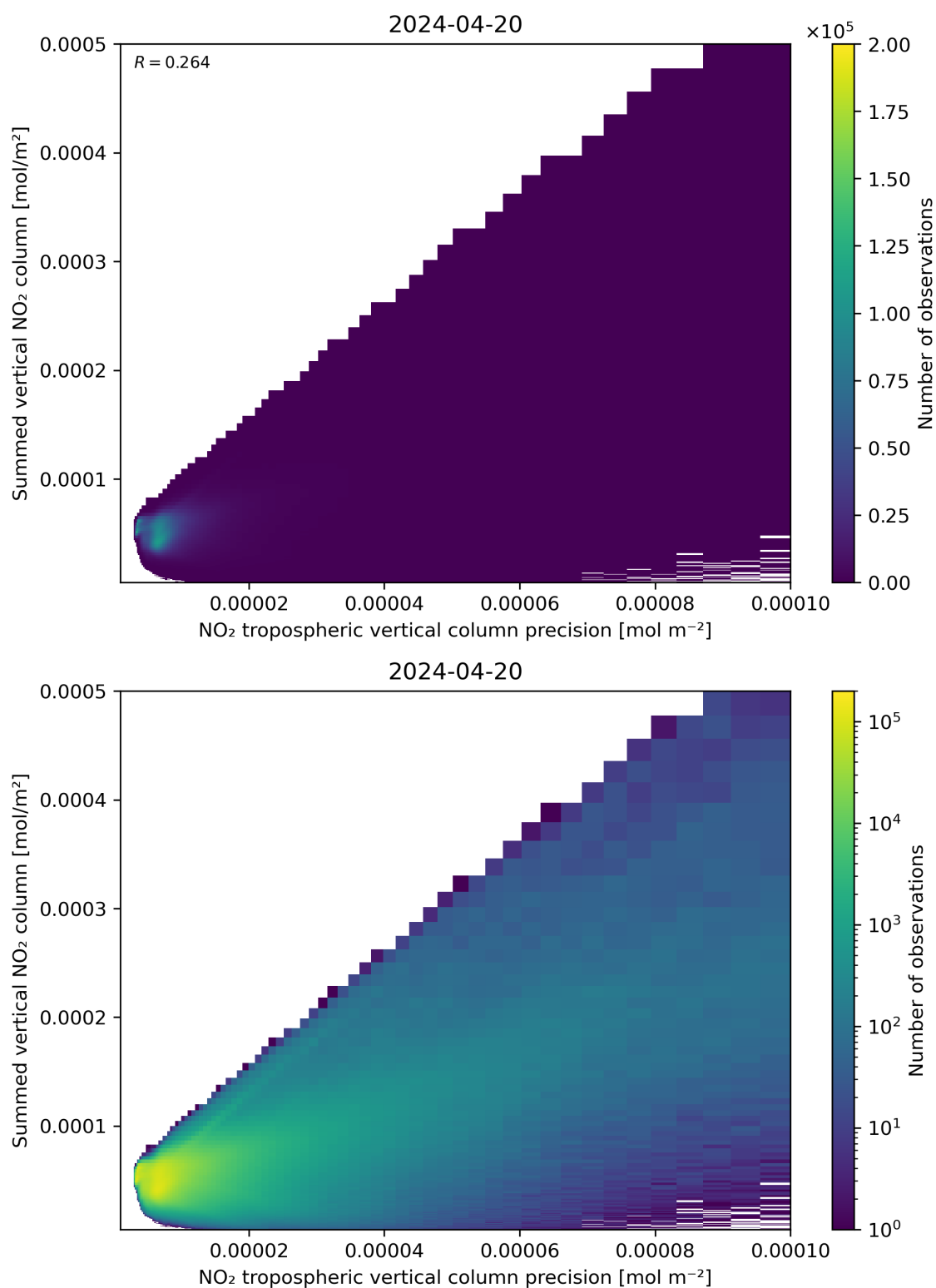
Figure 136: Scatter density plot of “NO 2 tropospheric vertical column precision” against “Summed vertical NO 2 column” for 2024-04-19 to 2024-04-21.
