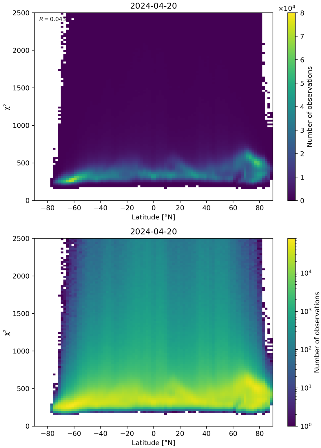
Figure 86: Scatter density plot of “Latitude” against “ \chi^2 ” for 2024-04-19 to 2024-04-21.
