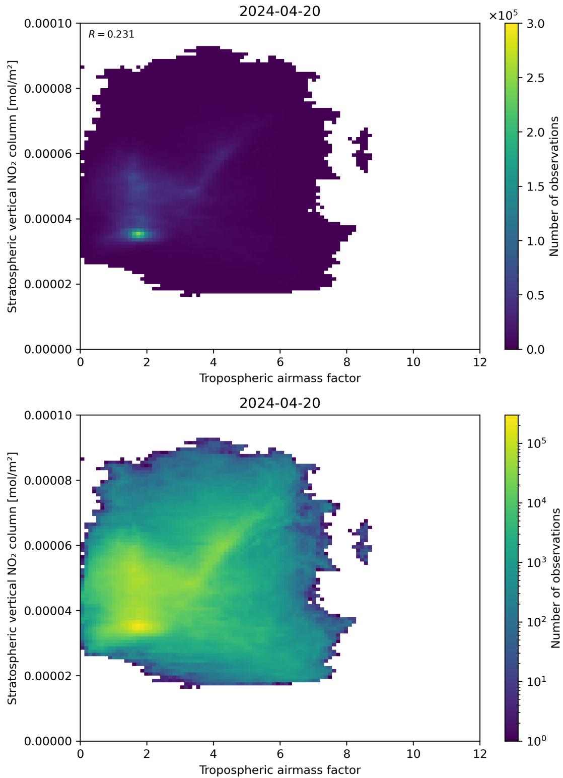
Figure 74: Scatter density plot of “Tropospheric air mass factor” against “Stratospheric vertical NO 2 column” for 2024-04-19 to 2024-04-21.
