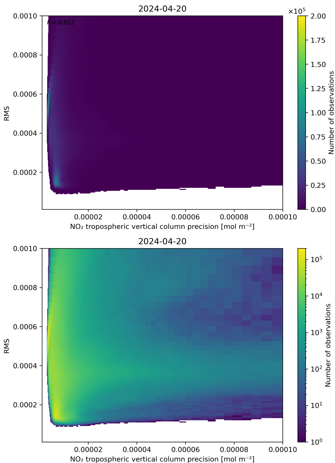
Figure 140: Scatter density plot of “NO 2 tropospheric vertical column precision” against “RMS” for 2024-04-19 to 2024-04-21.
