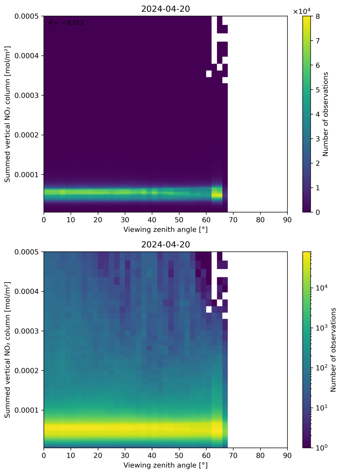
Figure 165: Scatter density plot of “Viewing zenith angle” against “Summed vertical NO 2 column” for 2024-04-19 to 2024-04-21.
