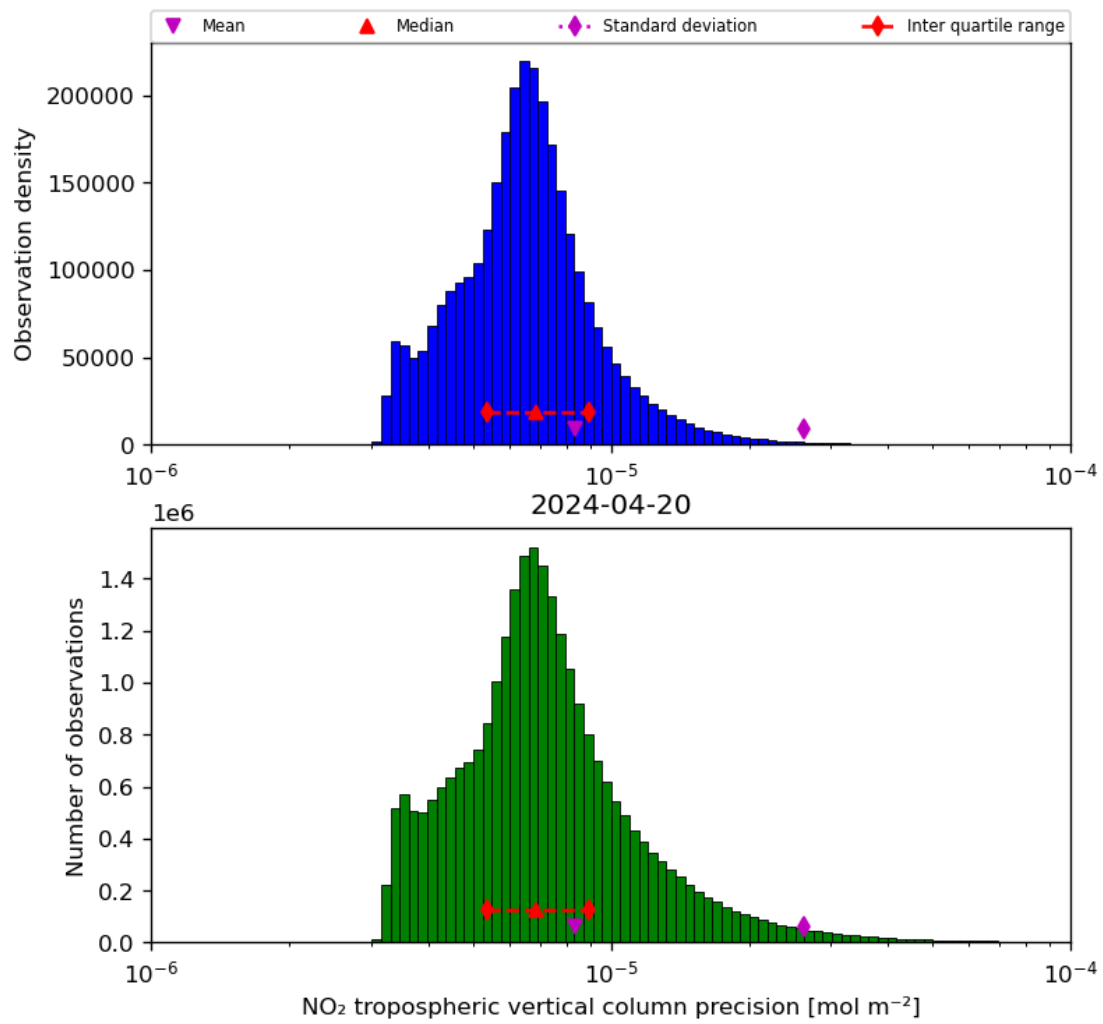
Figure 30: Histogram of “NO 2 tropospheric vertical column precision” for 2024-04-19 to 2024-04-21
