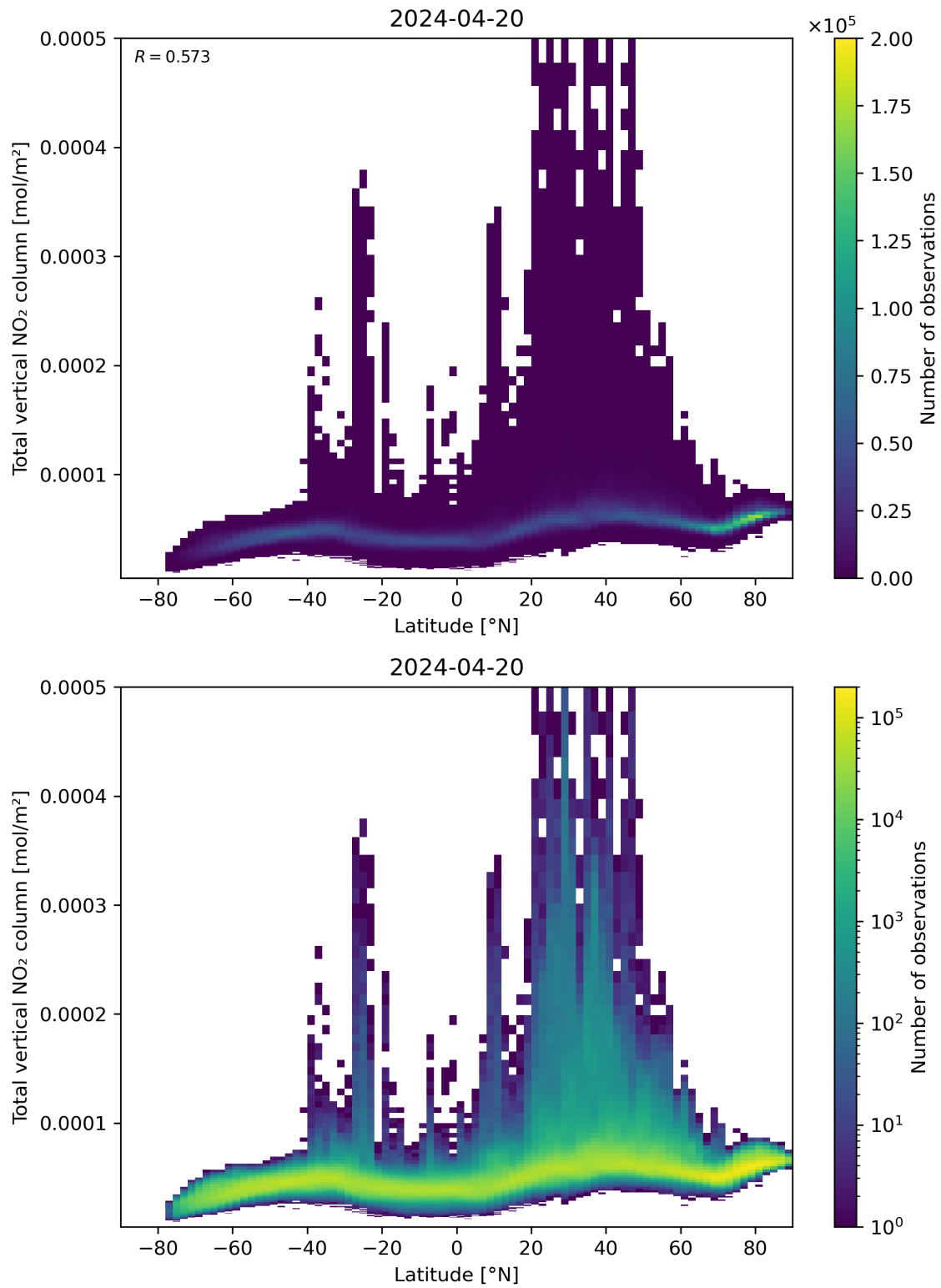
Figure 90: Scatter density plot of “Latitude” against “Total vertical NO 2 column” for 2024-04-19 to 2024-04-21.
