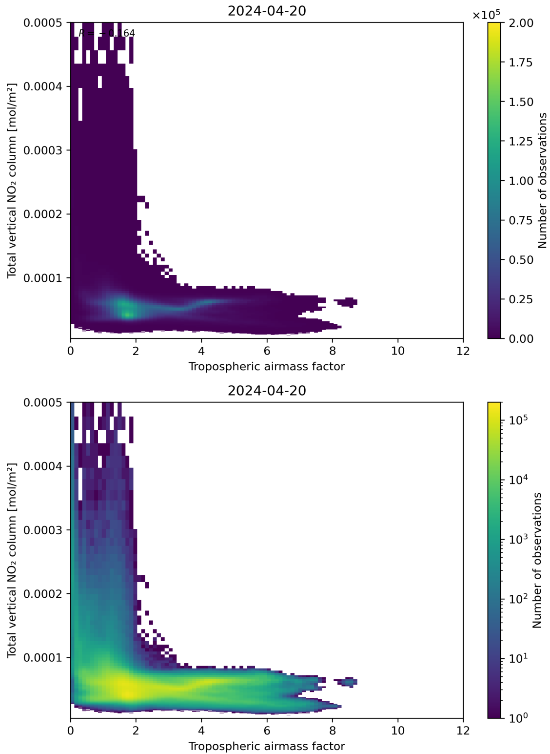
Figure 77: Scatter density plot of “Tropospheric airmass factor” against “Total vertical NO 2 column” for 2024-04-19 to 2024-04-21.
