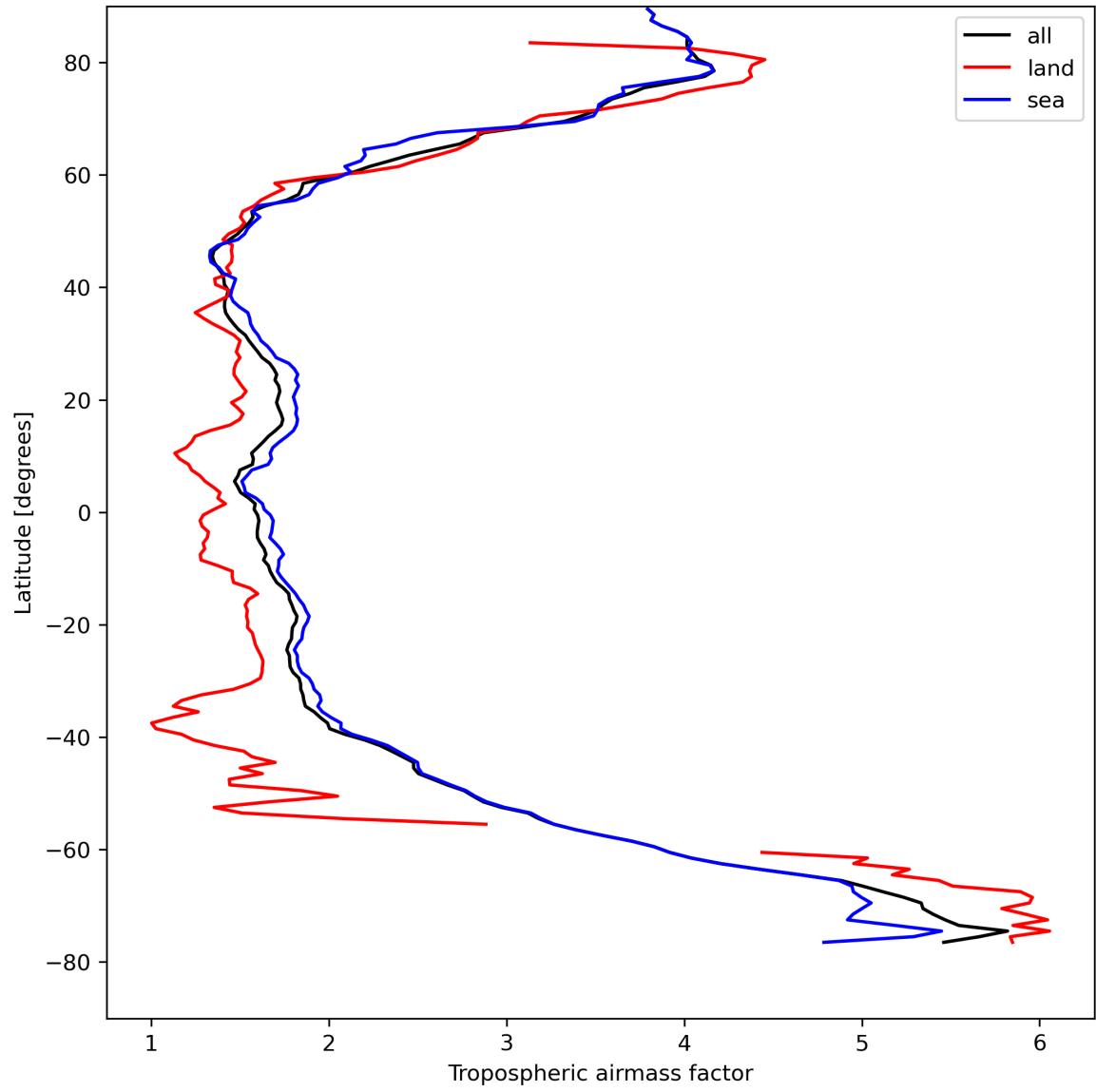
Figure 14: Zonal average of “Tropospheric airmass factor” for 2024-04-19 to 2024-04-21.
