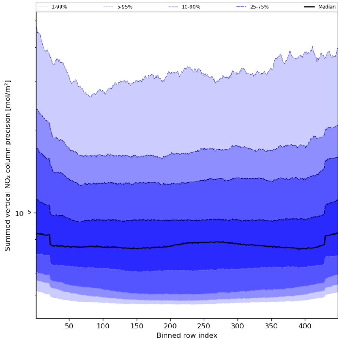
Figure 58: Along track statistics of “Summed vertical NO 2 column precision” for 2024-04-19 to 2024-04-21
