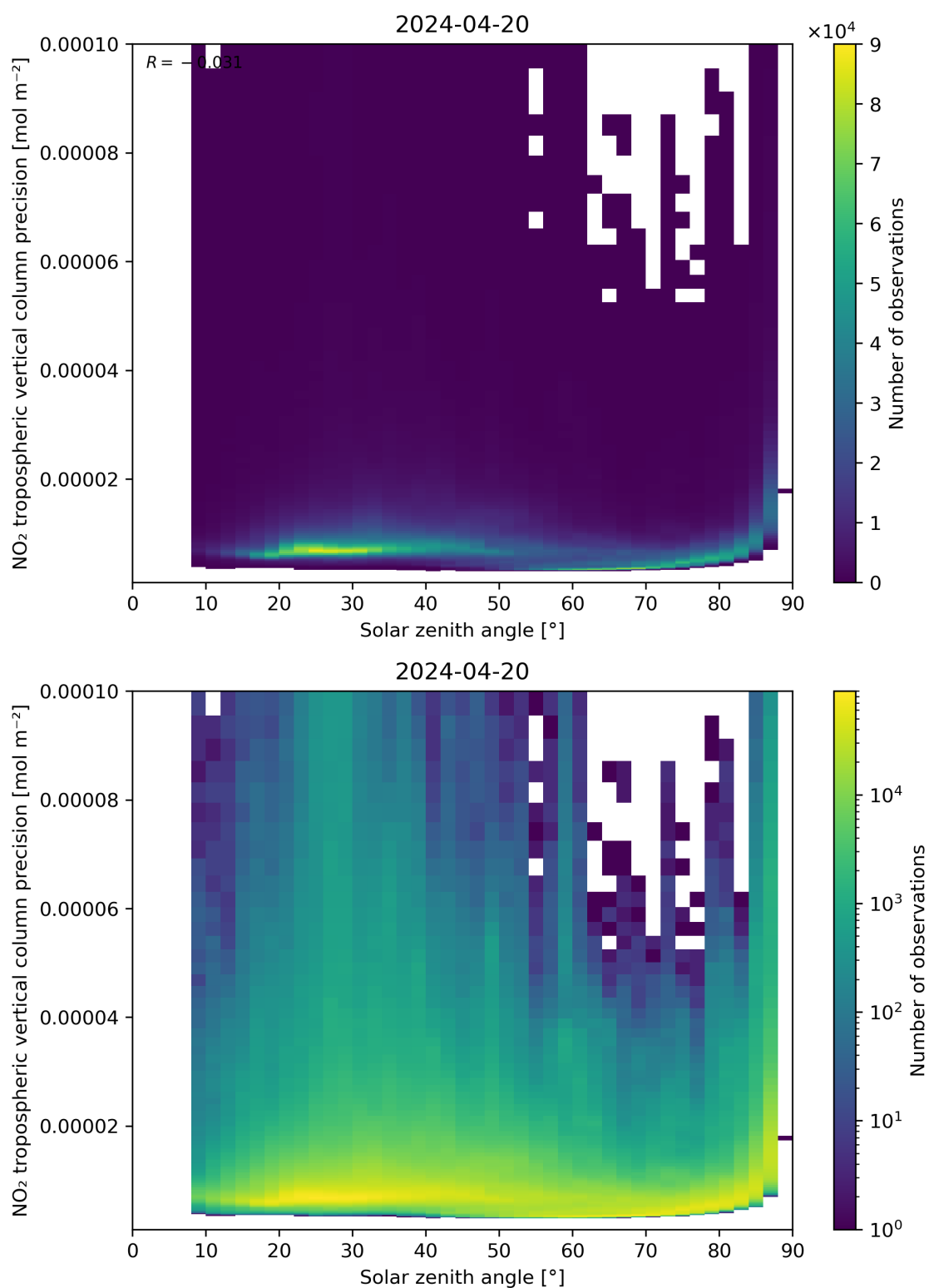
Figure 156: Scatter density plot of “Solar zenith angle” against “NO 2 tropospheric vertical column precision” for 2024-04-19 to 2024-04-21.
