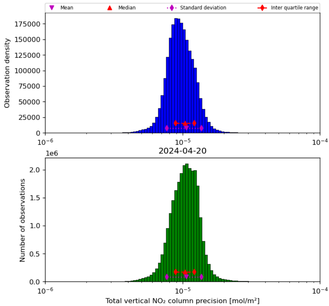
Figure 39: Histogram of “Total vertical NO 2 column precision” for 2024-04-19 to 2024-04-21
