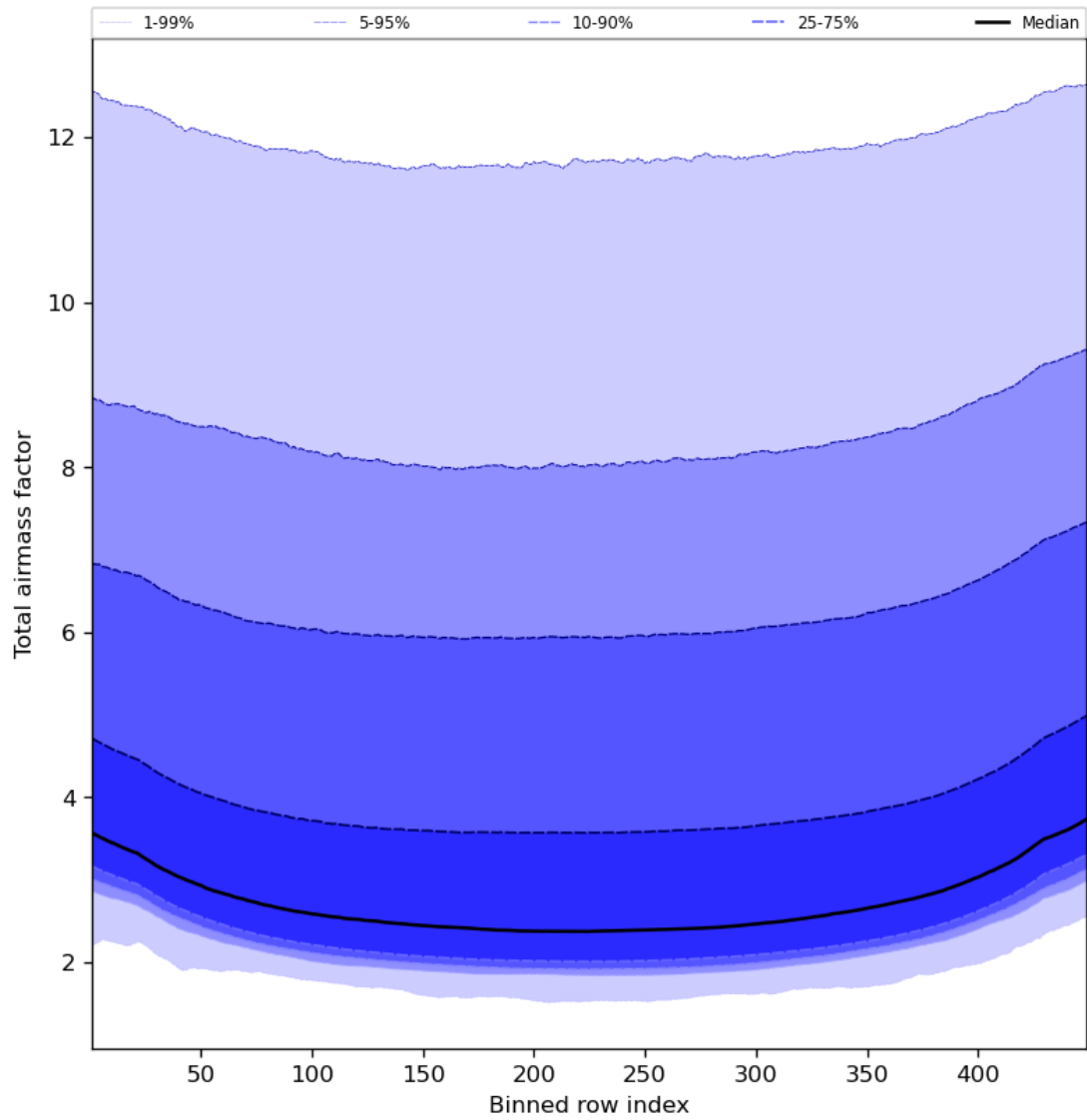
Figure 49: Along track statistics of “Total airmass factor” for 2024-04-19 to 2024-04-21
