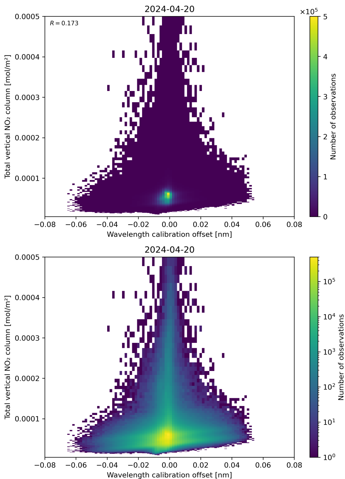
Figure 179: Scatter density plot of “Wavelength calibration offset” against “Total vertical NO 2 column” for 2024-04-19 to 2024-04-21.
