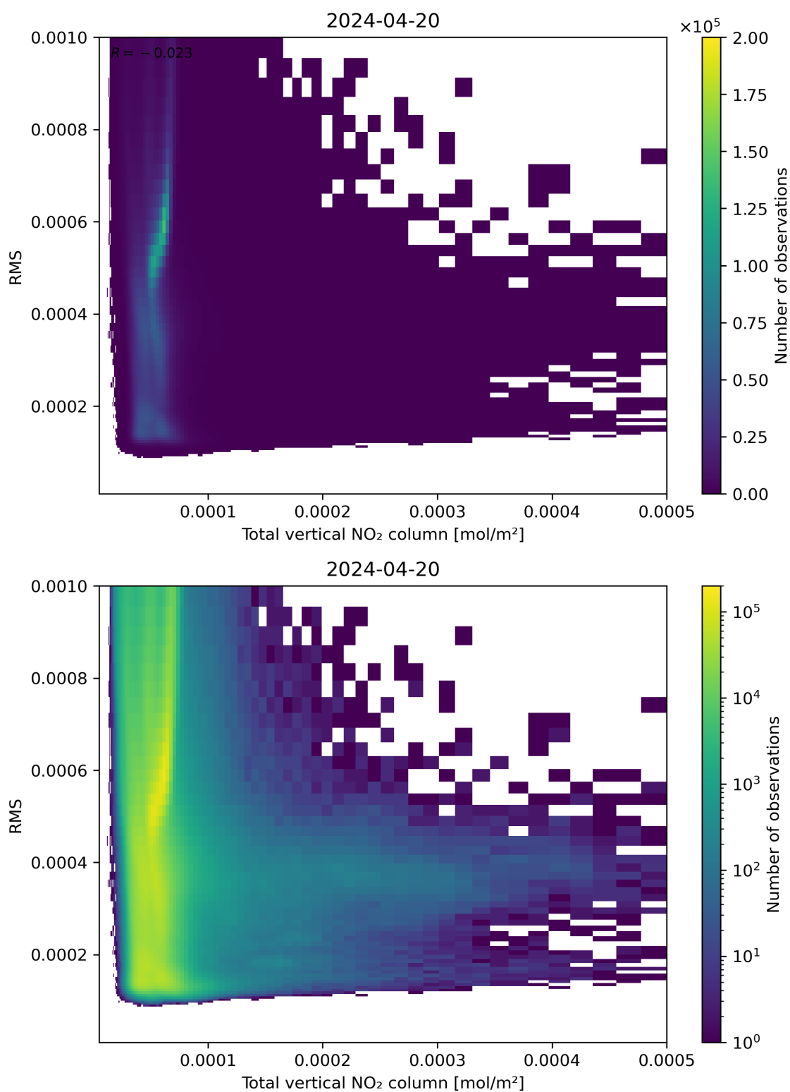
Figure 120: Scatter density plot of “Total vertical NO 2 column” against “RMS” for 2024-04-19 to 2024-04-21.
