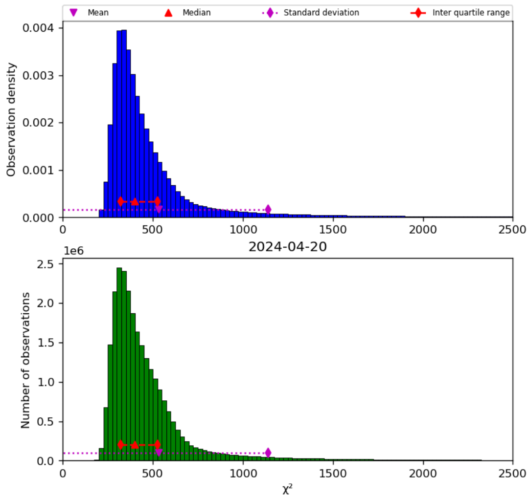
Figure 42: Histogram of “ \chi^2 ” for 2024-04-19 to 2024-04-21
