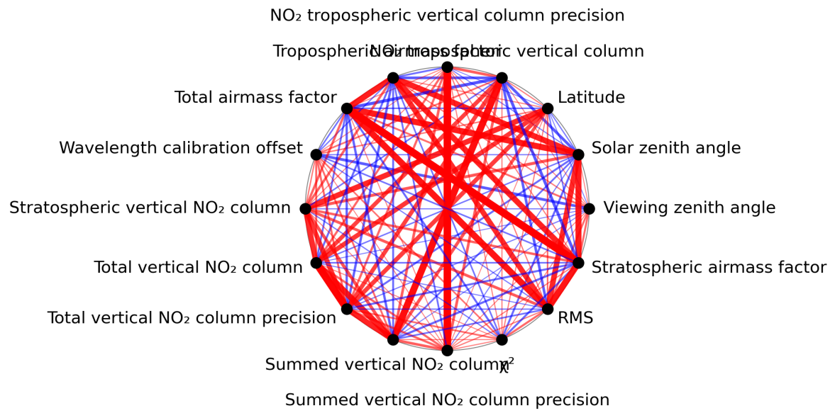
Figure 1: Map of correlation graph for 2024-04-19 to 2024-04-21.
