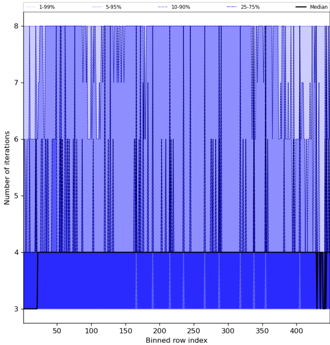
Figure 51: Along track statistics of “Number of iterations” for 2024-04-19 to 2024-04-21
