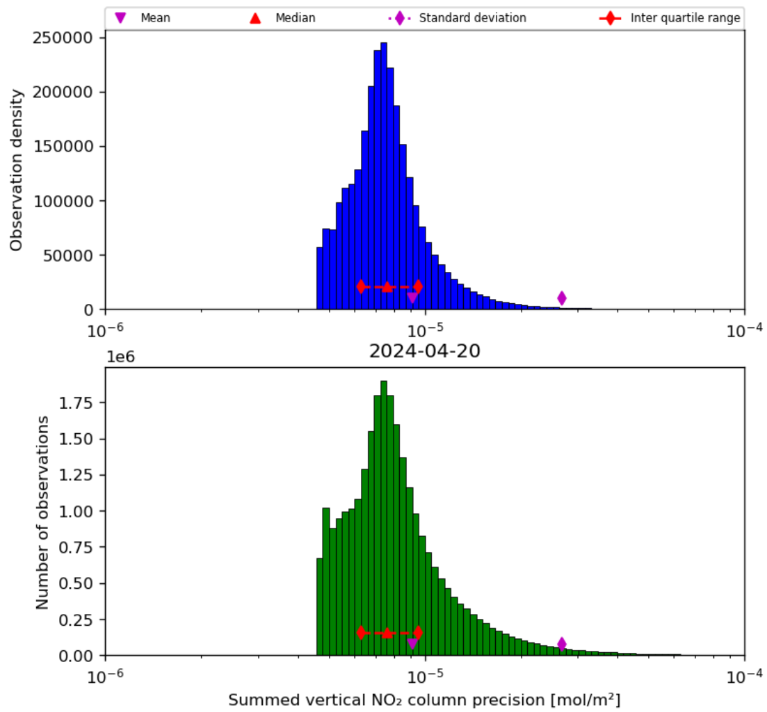
Figure 41: Histogram of “Summed vertical NO 2 column precision” for 2024-04-19 to 2024-04-21
