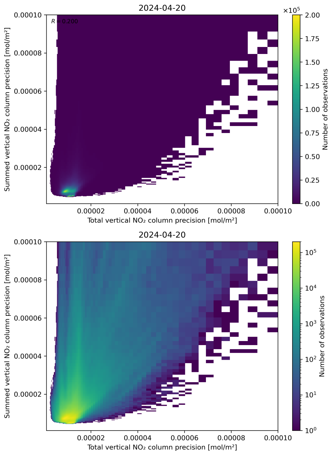
Figure 118: Scatter density plot of “Total vertical NO 2 column precision” against “Summed vertical NO 2 column precision” for 2024-04-19 to 2024-04-21.
