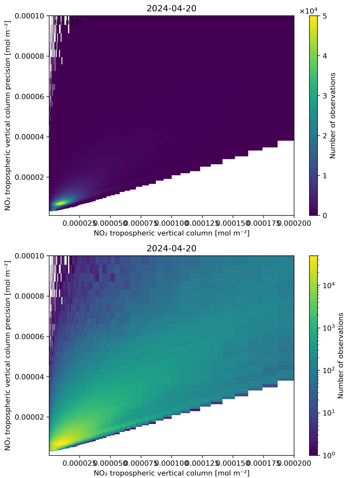
Figure 130: Scatter density plot of “NO 2 tropospheric vertical column” against “NO 2 tropospheric vertical column precision” for 2024-04-19 to 2024-04-21.
