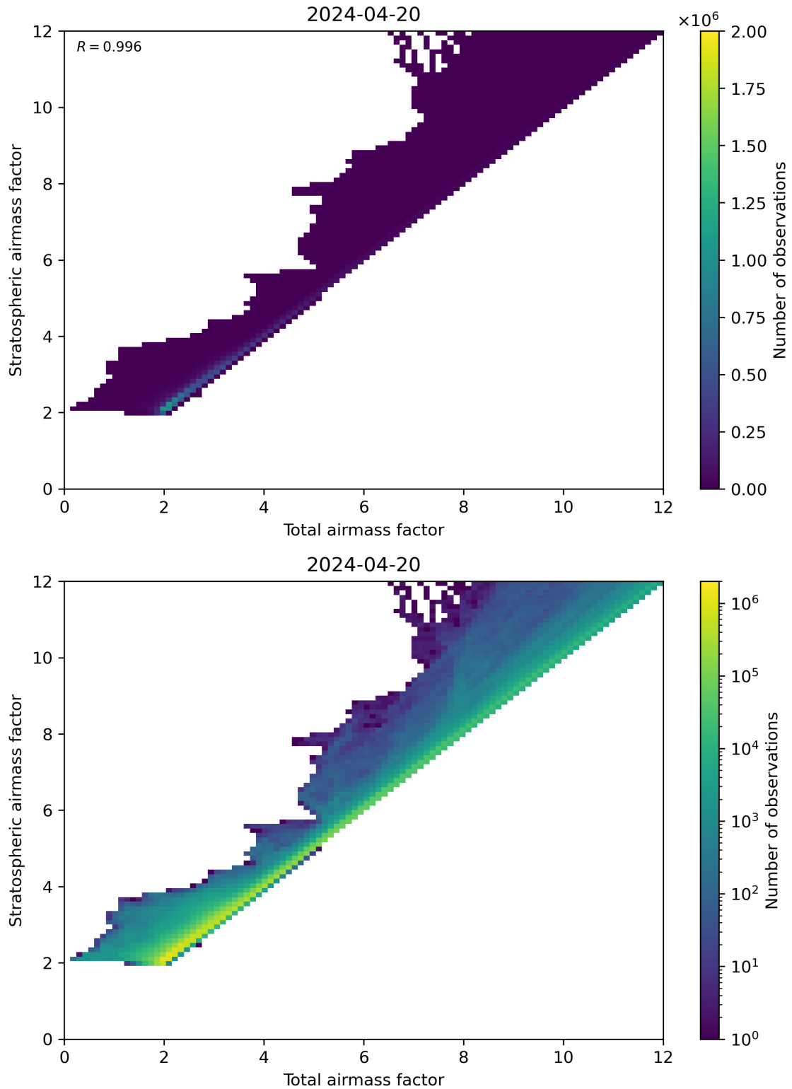
Figure 62: Scatter density plot of “Total airmass factor” against “Stratospheric airmass factor” for 2024-04-19 to 2024-04-21.
