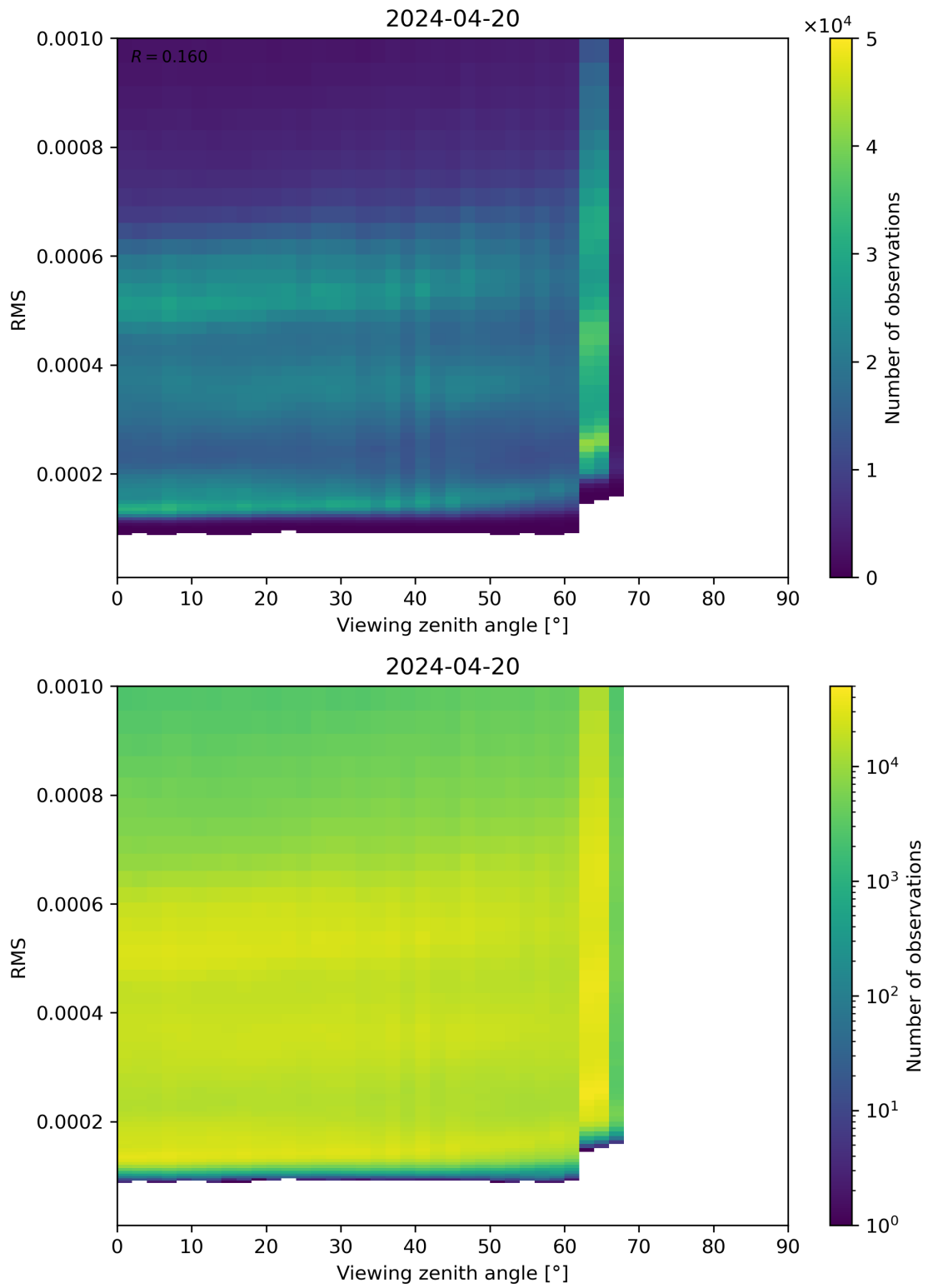
Figure 171: Scatter density plot of “Viewing zenith angle” against “RMS” for 2024-04-19 to 2024-04-21.
