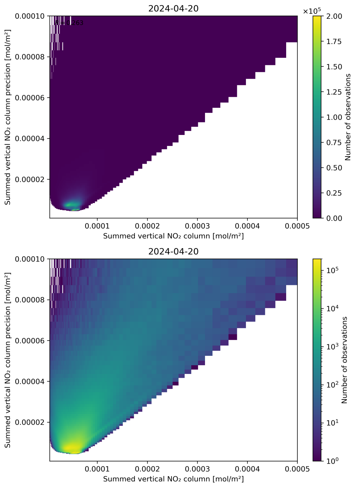
Figure 105: Scatter density plot of “Summed vertical NO 2 column” against “Summed vertical NO 2 column precision” for 2024-04-19 to 2024-04-21.
