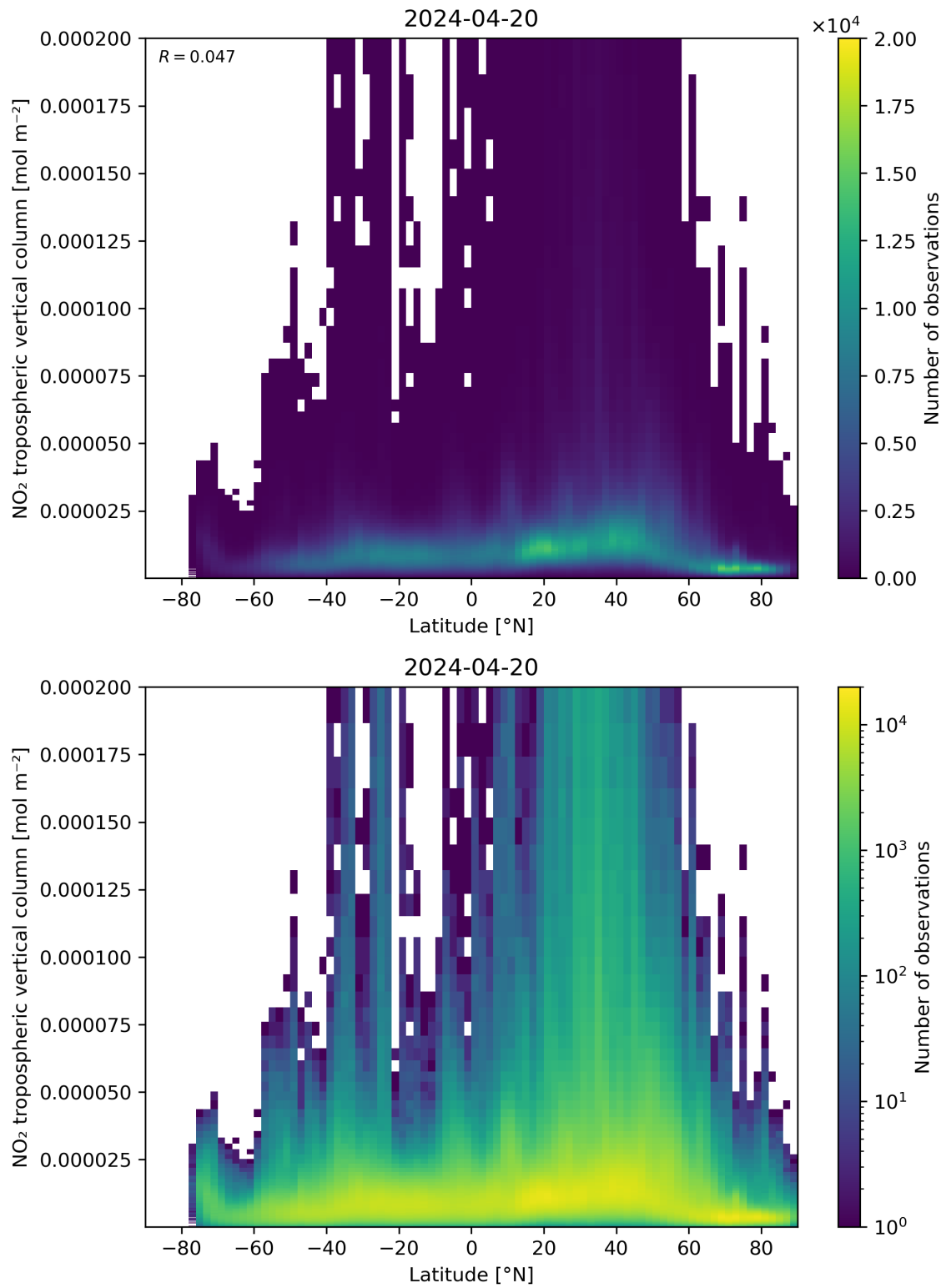
Figure 92: Scatter density plot of “Latitude” against “NO 2 tropospheric vertical column” for 2024-04-19 to 2024-04-21.
