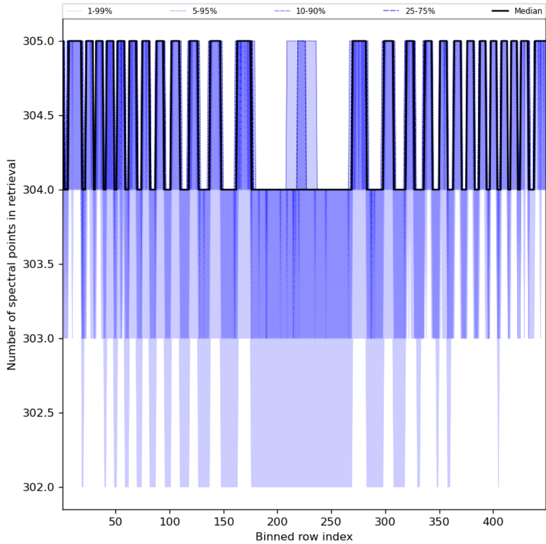
Figure 50: Along track statistics of “Number of spectral points in retrieval” for 2024-04-19 to 2024-04-21
