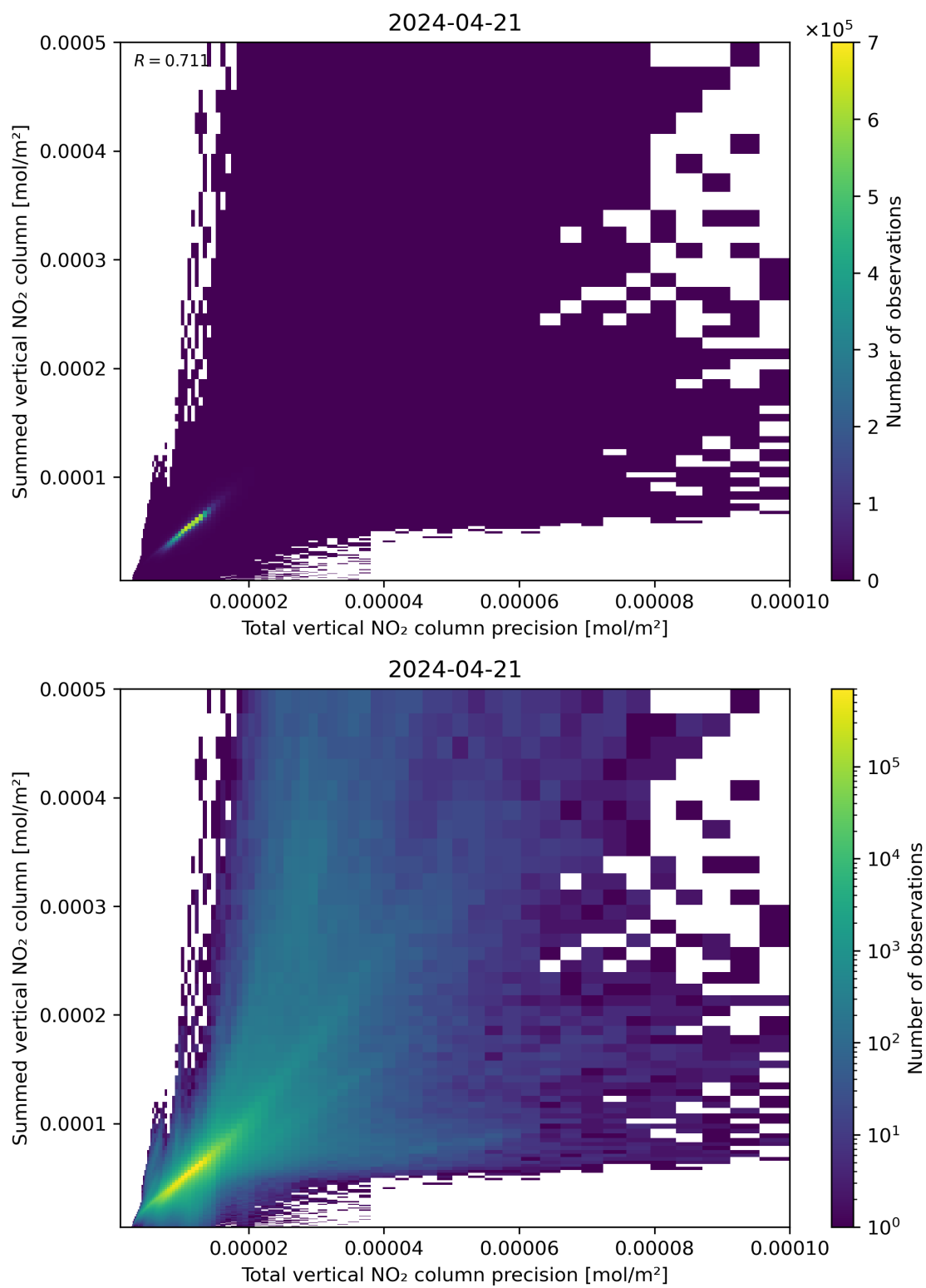
Figure 117: Scatter density plot of “Total vertical NO 2 column precision” against “Summed vertical NO 2 column” for 2024-04-21 to 2024-04-22.
