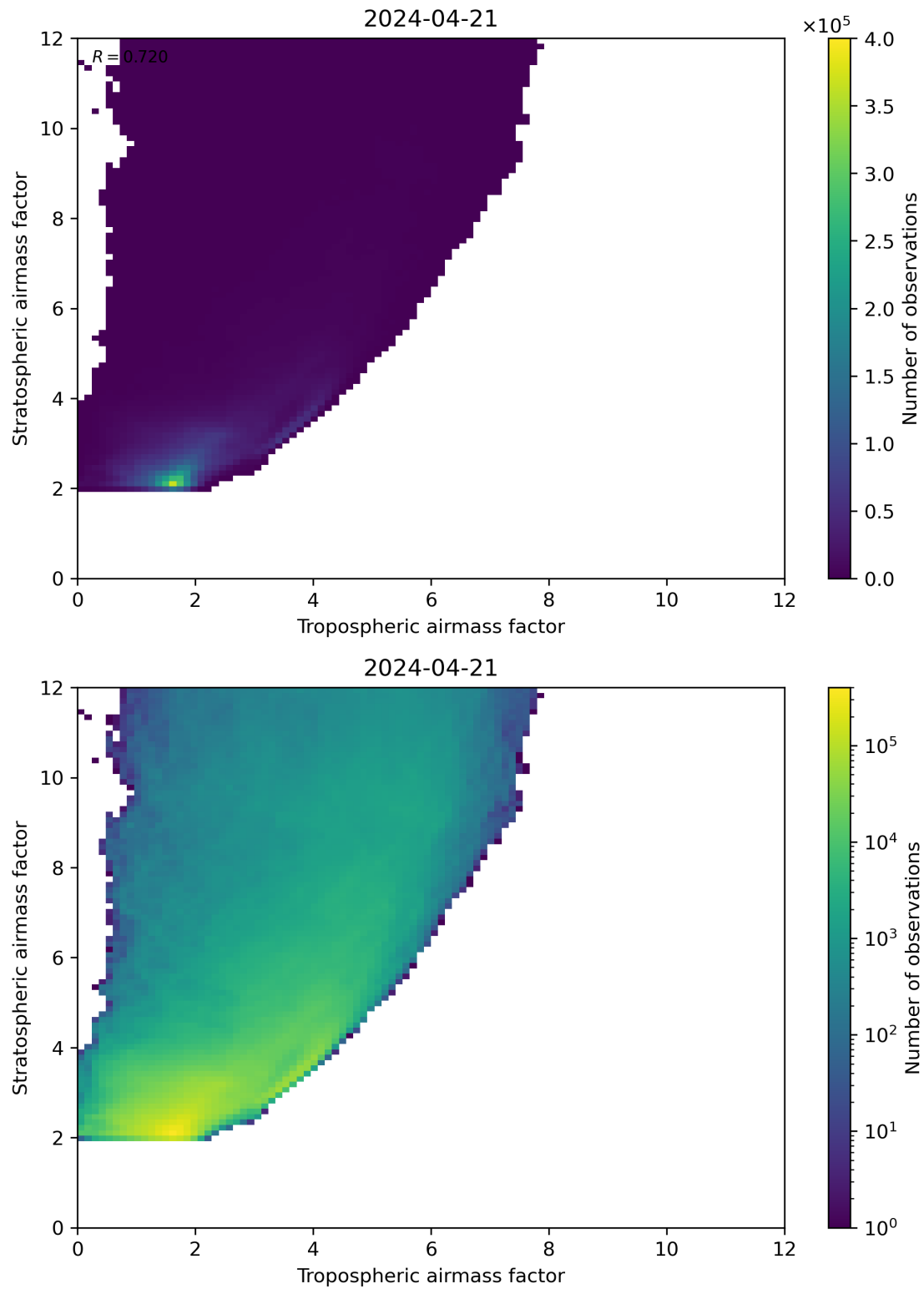
Figure 71: Scatter density plot of “Tropospheric airmass factor” against “Stratospheric airmass factor” for 2024-04-21 to 2024-04-22.
