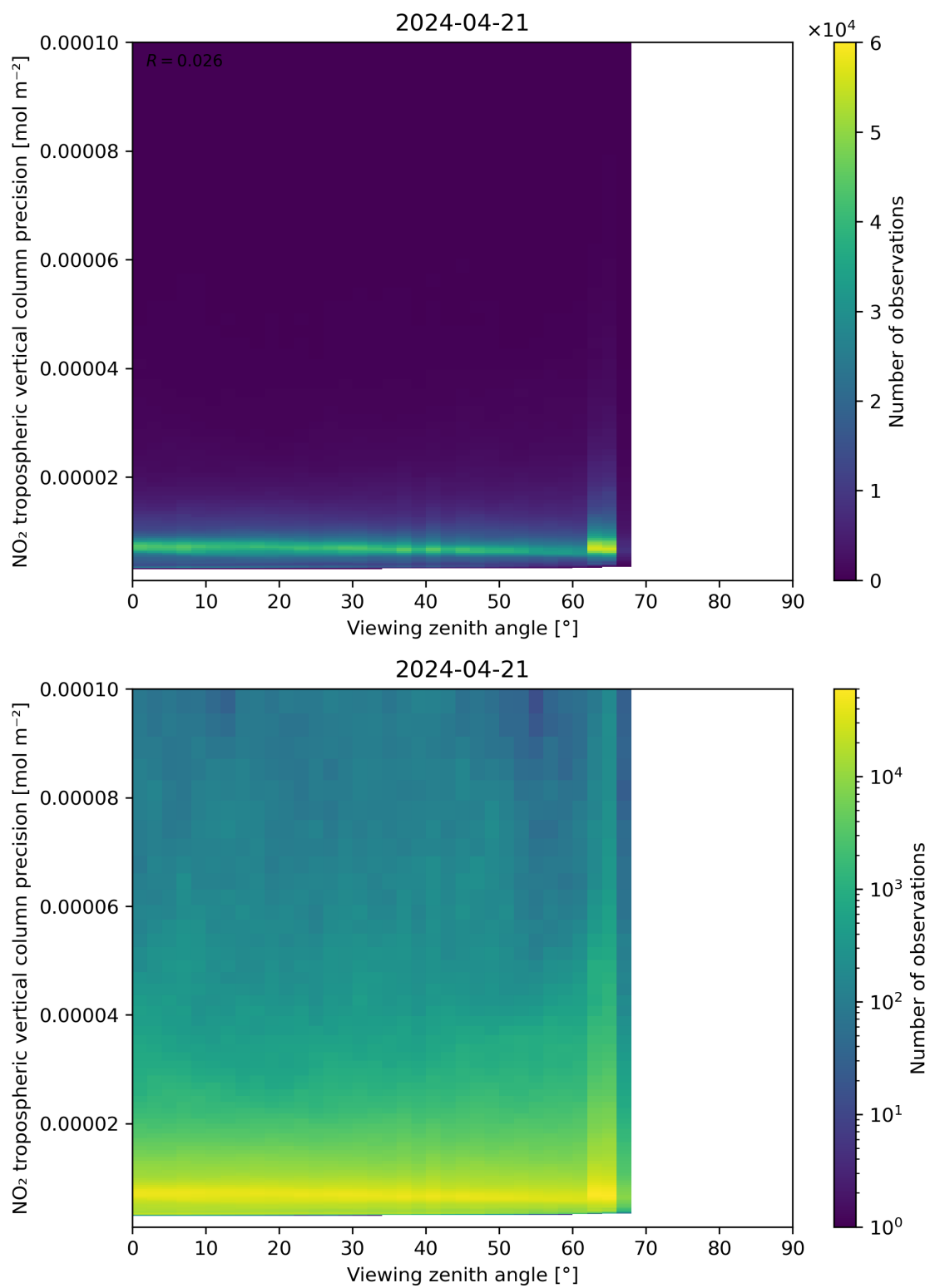
Figure 170: Scatter density plot of “Viewing zenith angle” against “NO 2 tropospheric vertical column precision” for 2024-04-21 to 2024-04-22.
