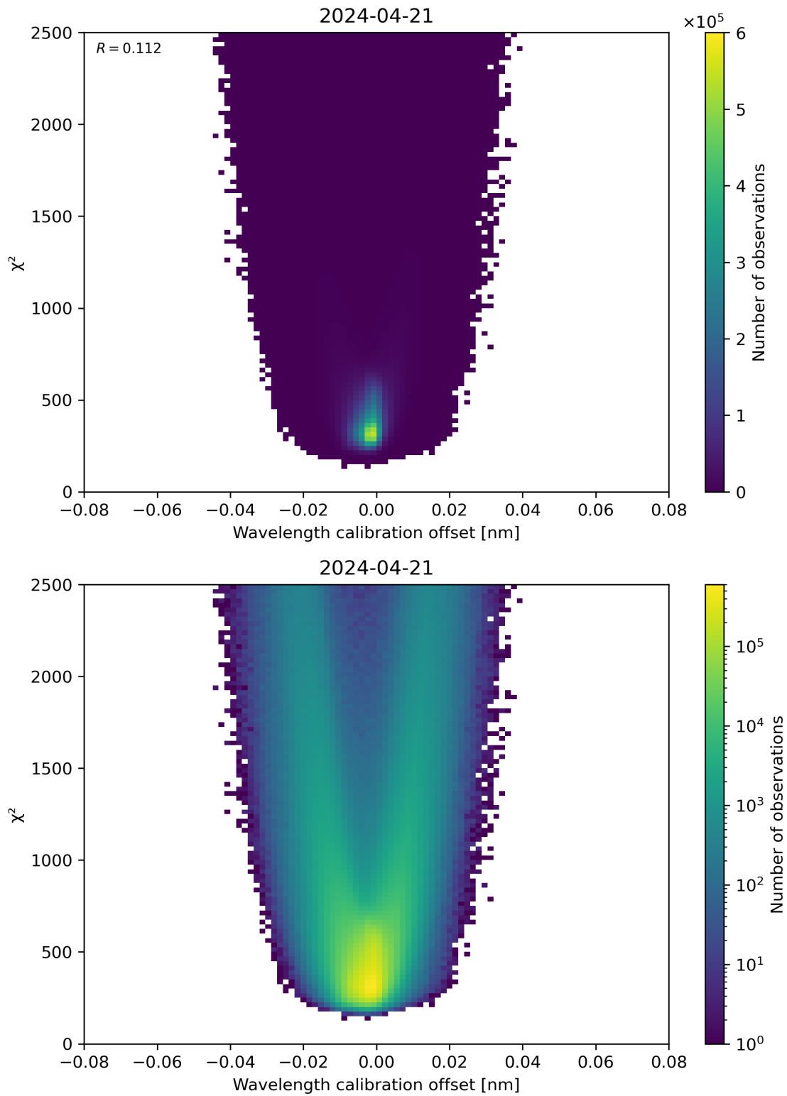
Figure 175: Scatter density plot of “Wavelength calibration offset” against “ \chi^2 ” for 2024-04-21 to 2024-04-22.
