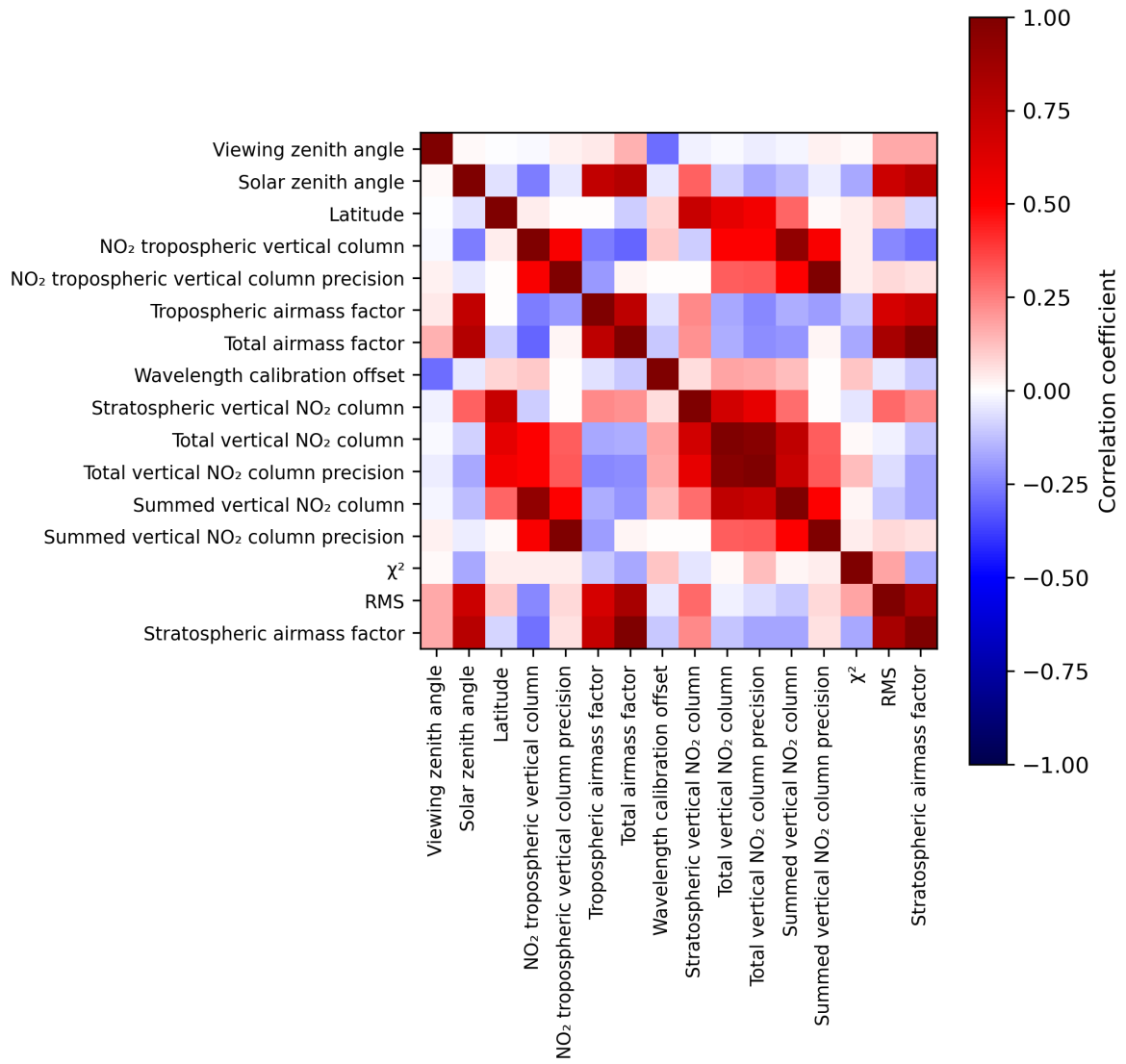
Figure 2: Map of correlation matrix for 2024-04-21 to 2024-04-22.
