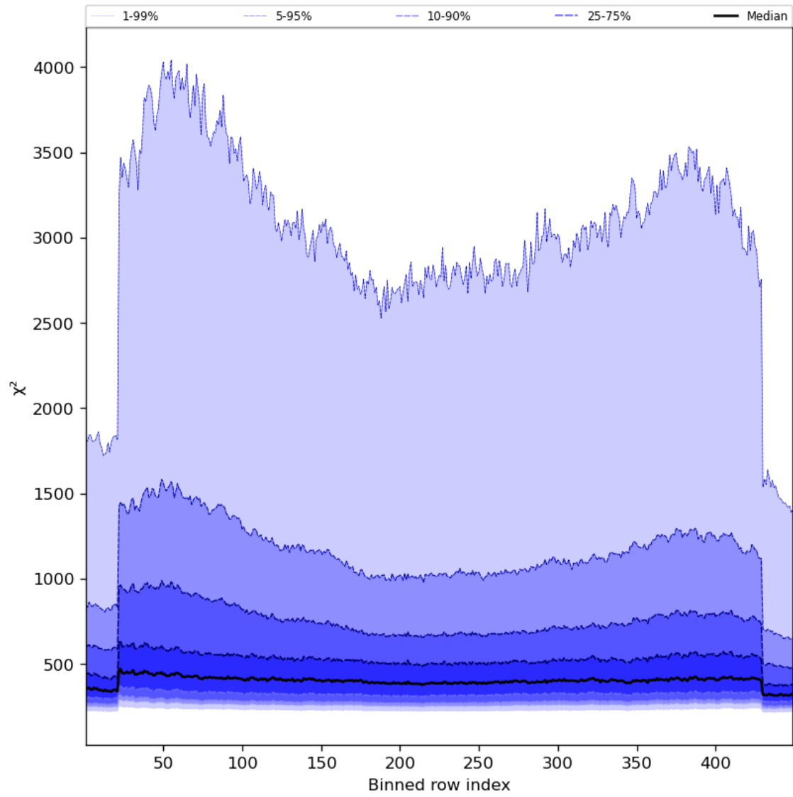
Figure 59: Along track statistics of “ \chi^2 ” for 2024-04-21 to 2024-04-22
