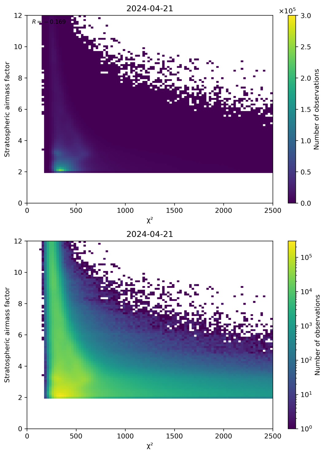
Figure 81: Scatter density plot of " \chi^2 " against "Stratospheric airmass factor" for 2024-04-21 to 2024-04-22.
