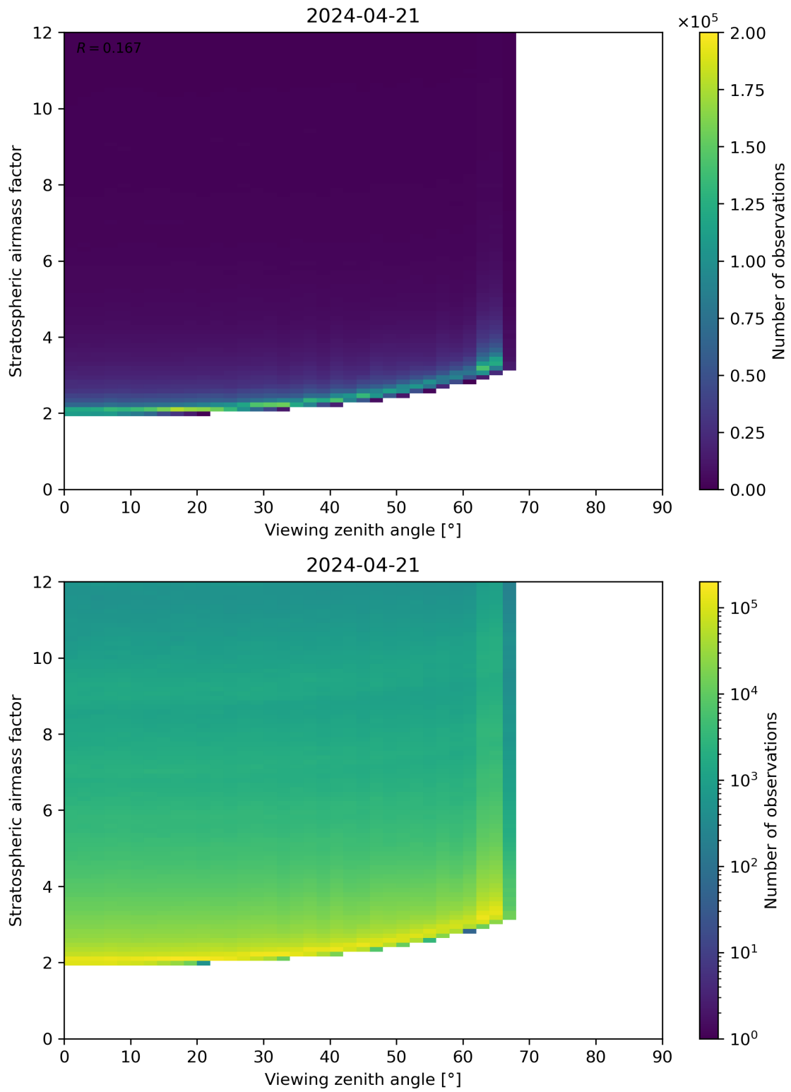
Figure 159: Scatter density plot of “Viewing zenith angle” against “Stratospheric airmass factor” for 2024-04-21 to 2024-04-22.
