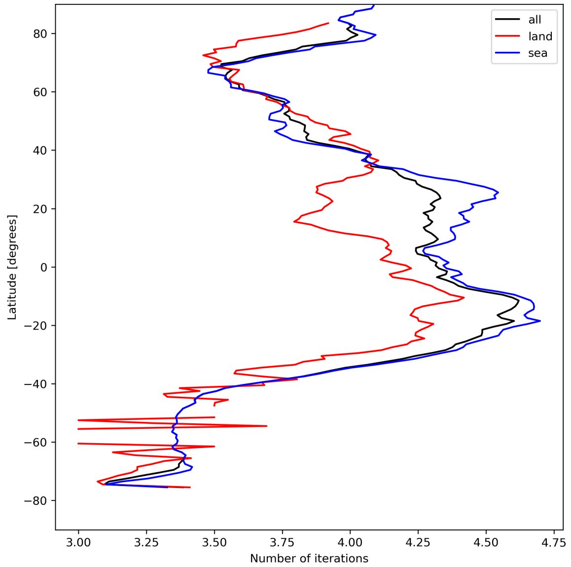
Figure 17: Zonal average of “Number of iterations” for 2024-04-21 to 2024-04-22.
