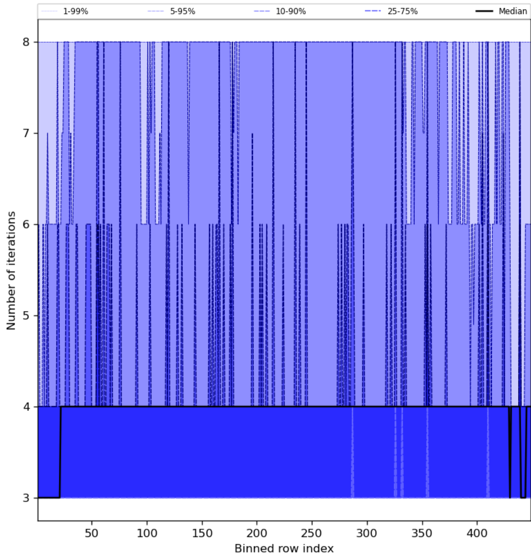
Figure 51: Along track statistics of “Number of iterations” for 2024-04-21 to 2024-04-22
