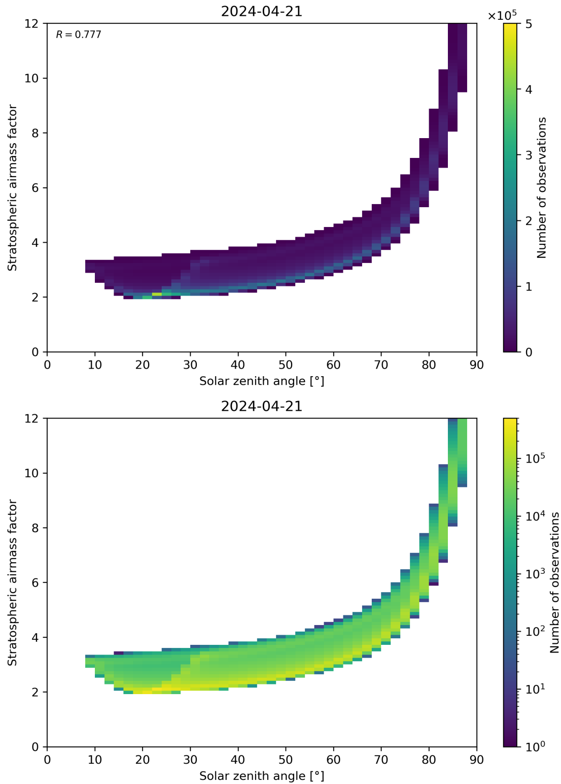
Figure 145: Scatter density plot of “Solar zenith angle” against “Stratospheric airmass factor” for 2024-04-21 to 2024-04-22.
