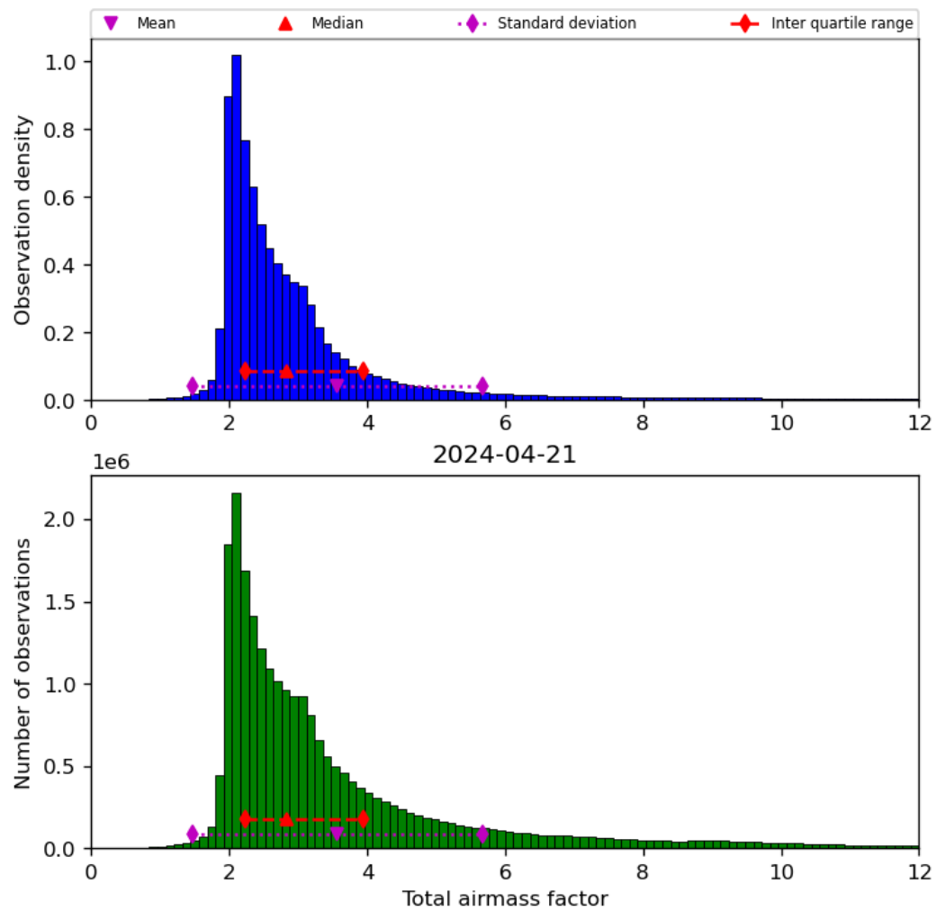
Figure 32: Histogram of “Total airmass factor” for 2024-04-21 to 2024-04-22
