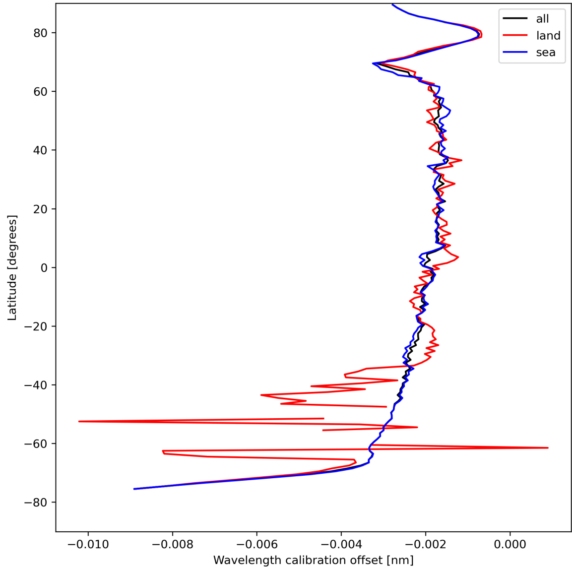
Figure 18: Zonal average of “Wavelength calibration offset” for 2024-04-21 to 2024-04-22.
