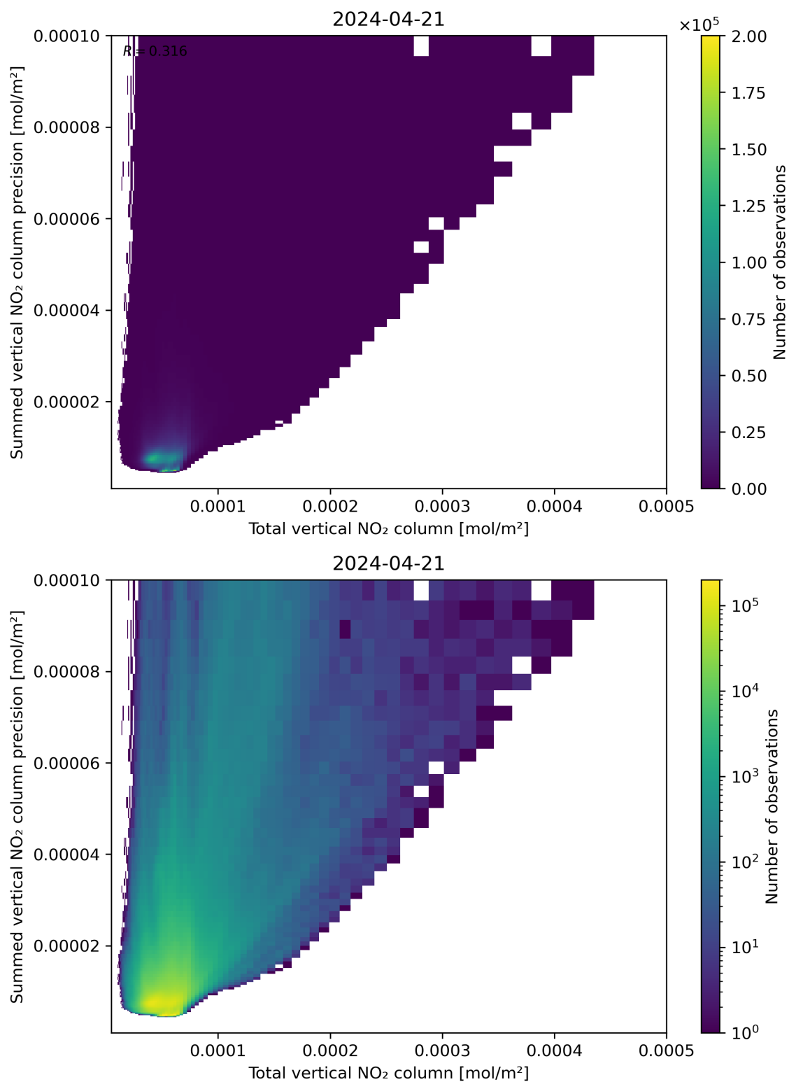
Figure 113: Scatter density plot of “Total vertical NO 2 column” against “Summed vertical NO 2 column precision” for 2024-04-21 to 2024-04-22.
