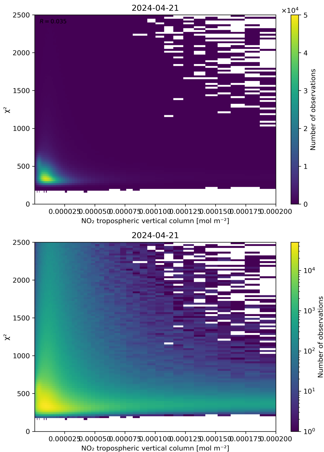
Figure 124: Scatter density plot of “NO 2 tropospheric vertical column” against “ \chi^2 ” for 2024-04-21 to 2024-04-22.
