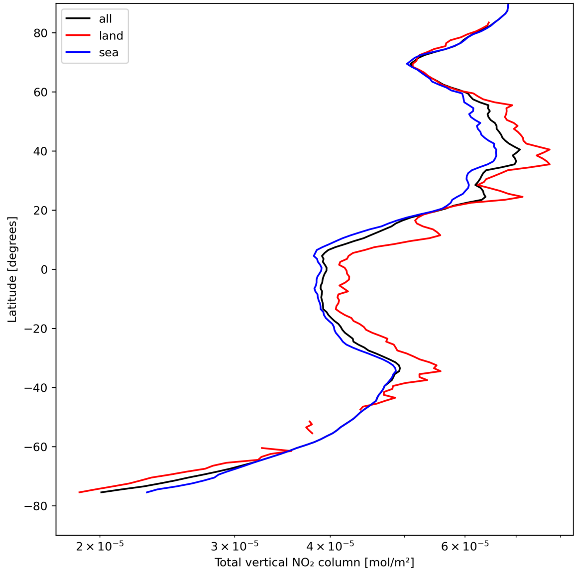
Figure 21: Zonal average of “Total vertical NO 2 column” for 2024-04-21 to 2024-04-22.
