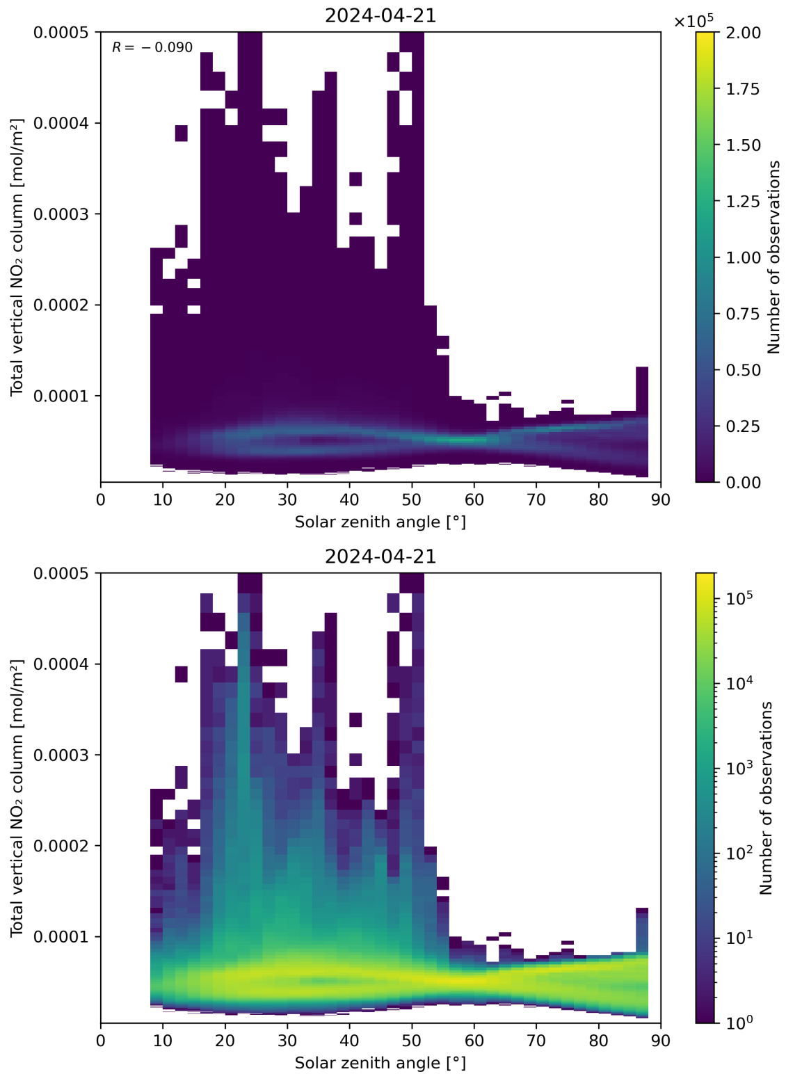
Figure 153: Scatter density plot of “Solar zenith angle” against “Total vertical NO 2 column” for 2024-04-21 to 2024-04-22.
