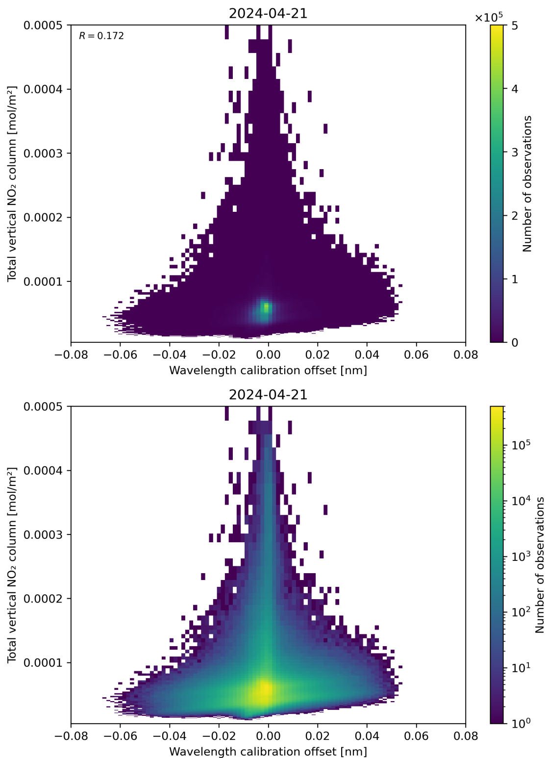
Figure 179: Scatter density plot of “Wavelength calibration offset” against “Total vertical NO 2 column” for 2024-04-21 to 2024-04-22.
