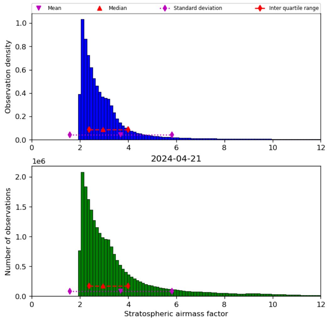
Figure 44: Histogram of “Stratospheric airmass factor” for 2024-04-21 to 2024-04-22
