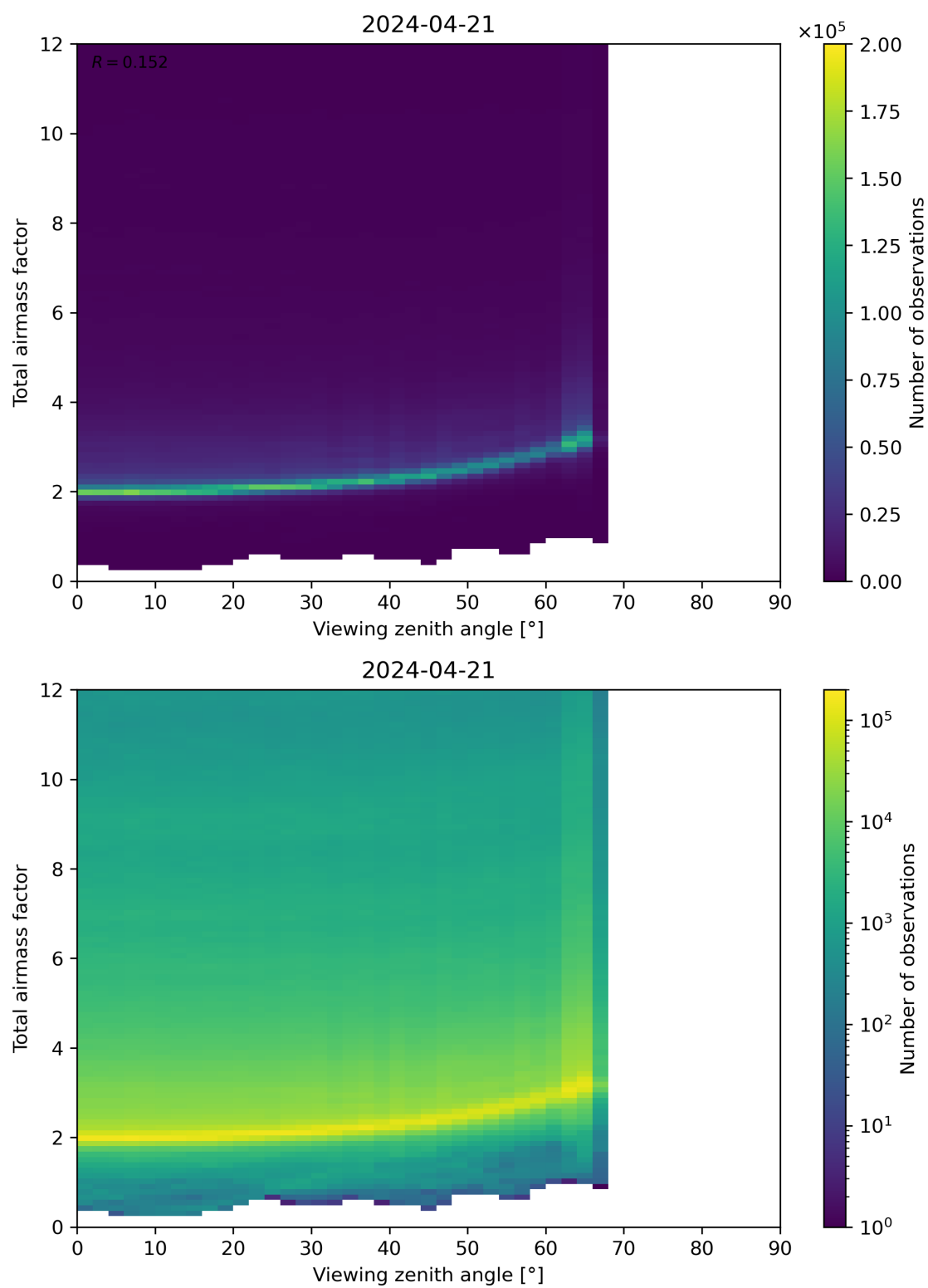
Figure 160: Scatter density plot of “Viewing zenith angle” against “Total airmass factor” for 2024-04-21 to 2024-04-22.
