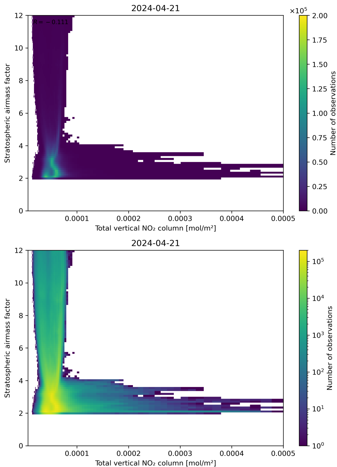
Figure 110: Scatter density plot of “Total vertical NO 2 column” against “Stratospheric airmass factor” for 2024-04-21 to 2024-04-22.
