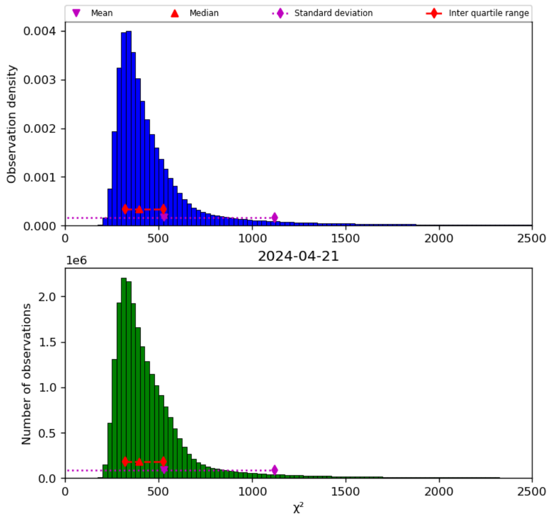
Figure 42: Histogram of “ \chi^2 ” for 2024-04-21 to 2024-04-22
