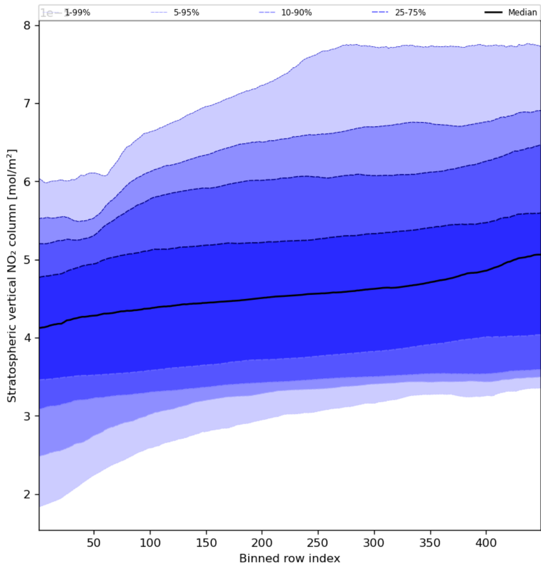
Figure 53: Along track statistics of “Stratospheric vertical NO 2 column” for 2024-04-21 to 2024-04-22
