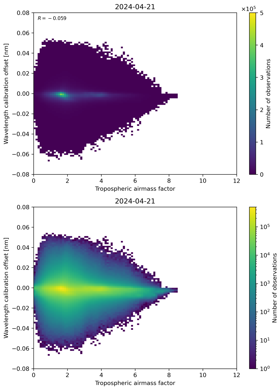
Figure 80: Scatter density plot of “Tropospheric air mass factor” against “Wavelength calibration offset” for 2024-04-21 to 2024-04-22.
