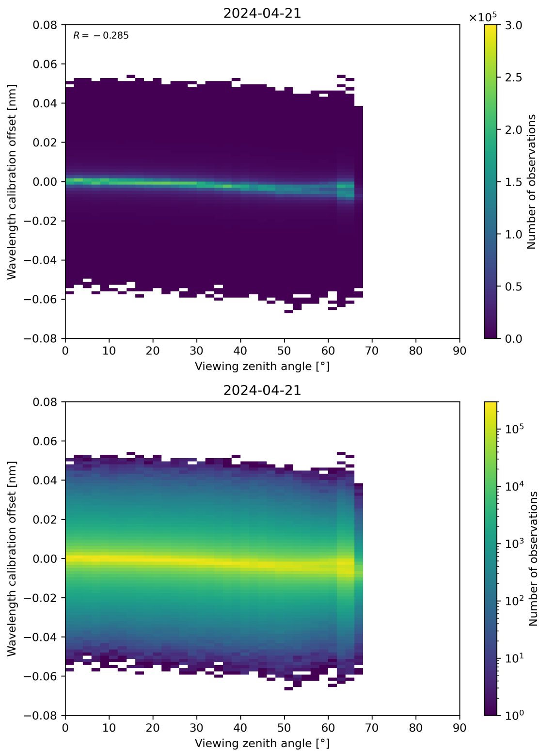
Figure 173: Scatter density plot of “Viewing zenith angle” against “Wavelength calibration offset” for 2024-04-21 to 2024-04-22.
