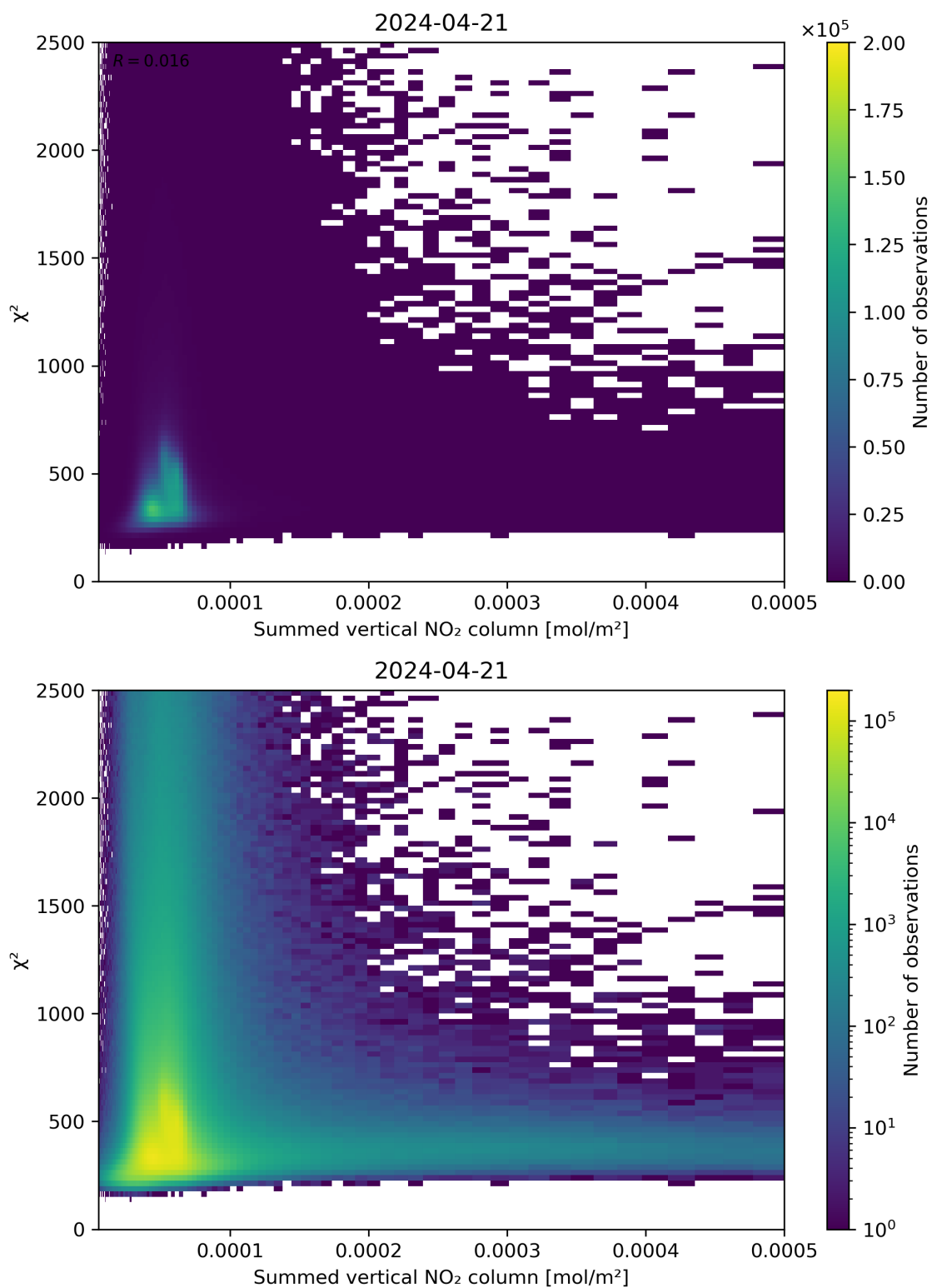
Figure 104: Scatter density plot of “Summed vertical NO 2 column” against “ \chi^2 ” for 2024-04-21 to 2024-04-22.
