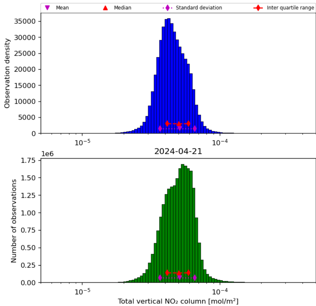
Figure 38: Histogram of “Total vertical NO 2 column” for 2024-04-21 to 2024-04-22
