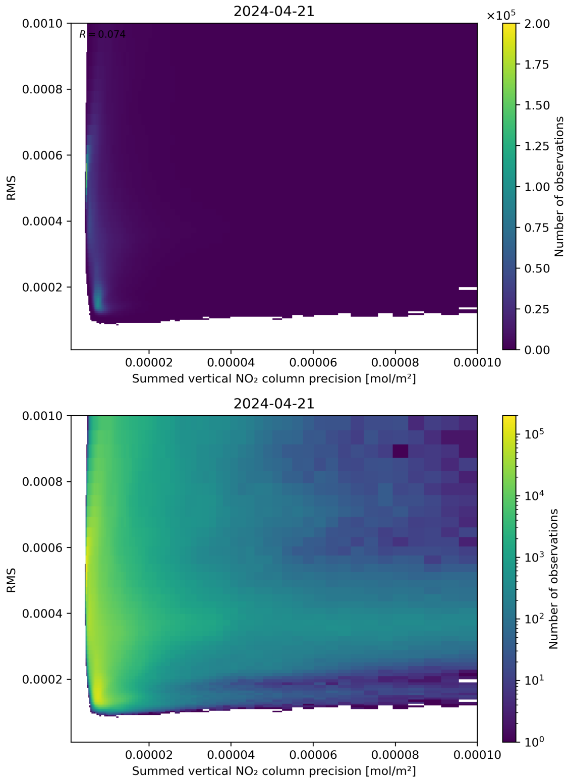
Figure 108: Scatter density plot of “Summed vertical NO 2 column precision” against “RMS” for 2024-04-21 to 2024-04-22.
