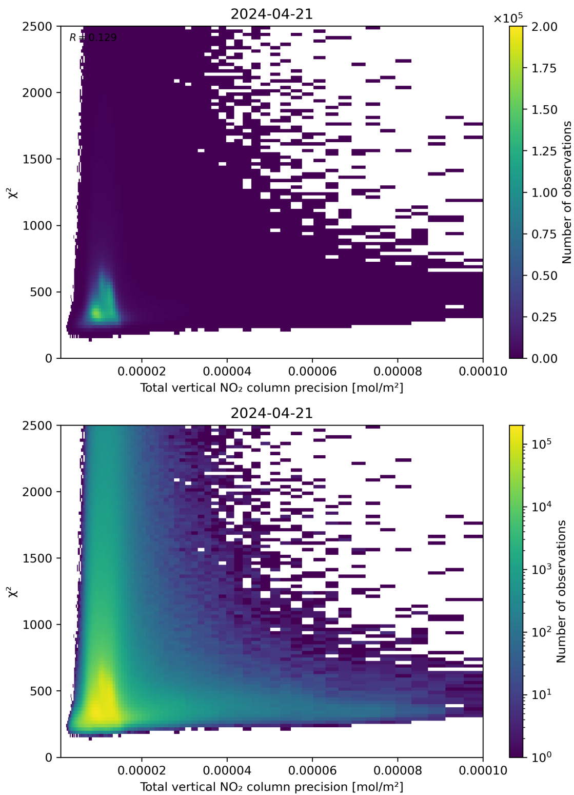
Figure 116: Scatter density plot of “Total vertical NO 2 column precision” against “ \chi^2 ” for 2024-04-21 to 2024-04-22.
