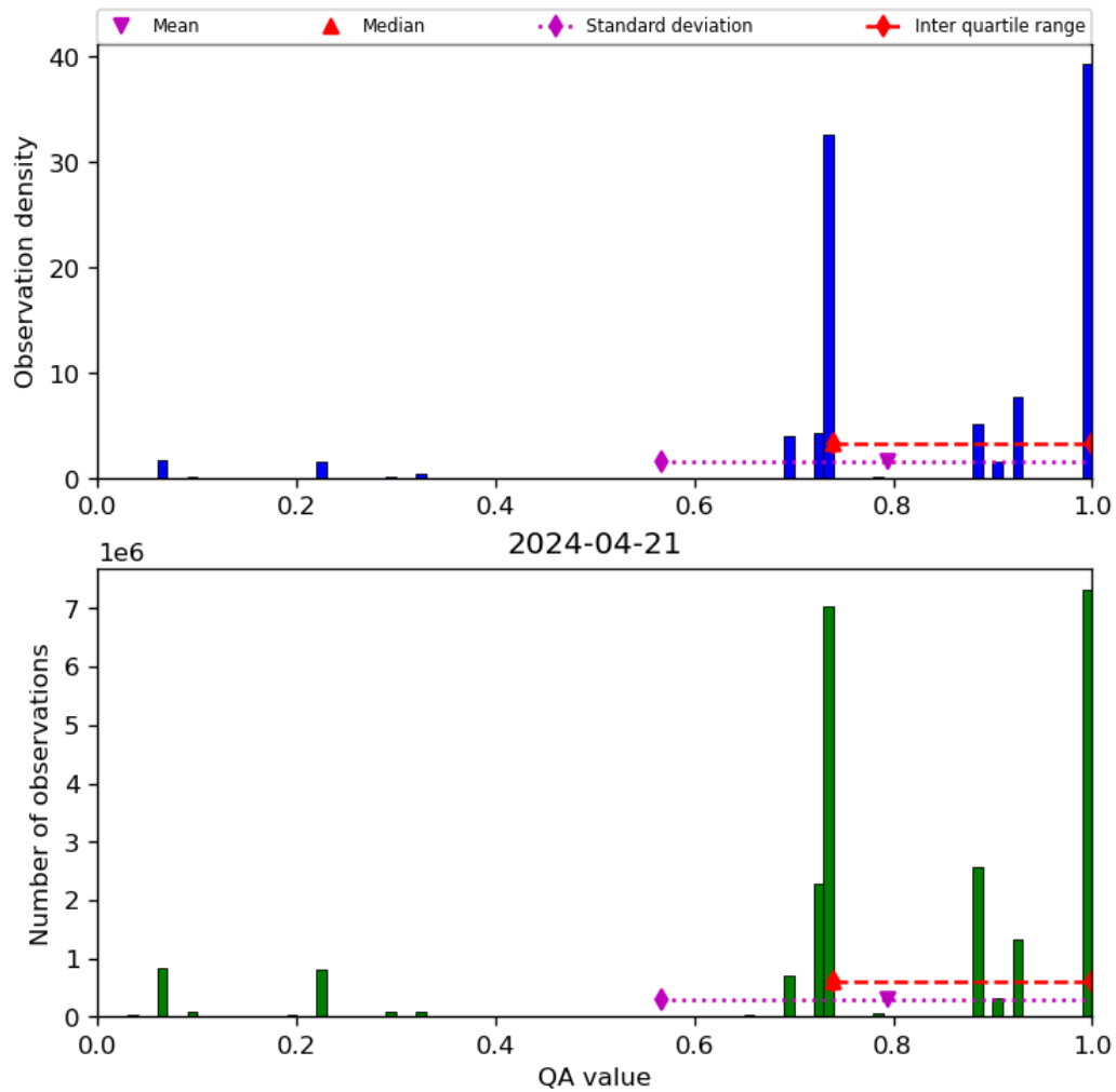
Figure 28: Histogram of “QA value” for 2024-04-21 to 2024-04-22
