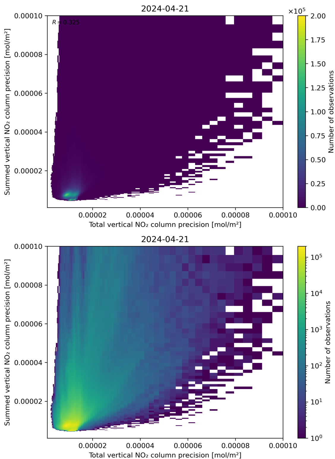
Figure 118: Scatter density plot of “Total vertical NO 2 column precision” against “Summed vertical NO 2 column precision” for 2024-04-21 to 2024-04-22.
