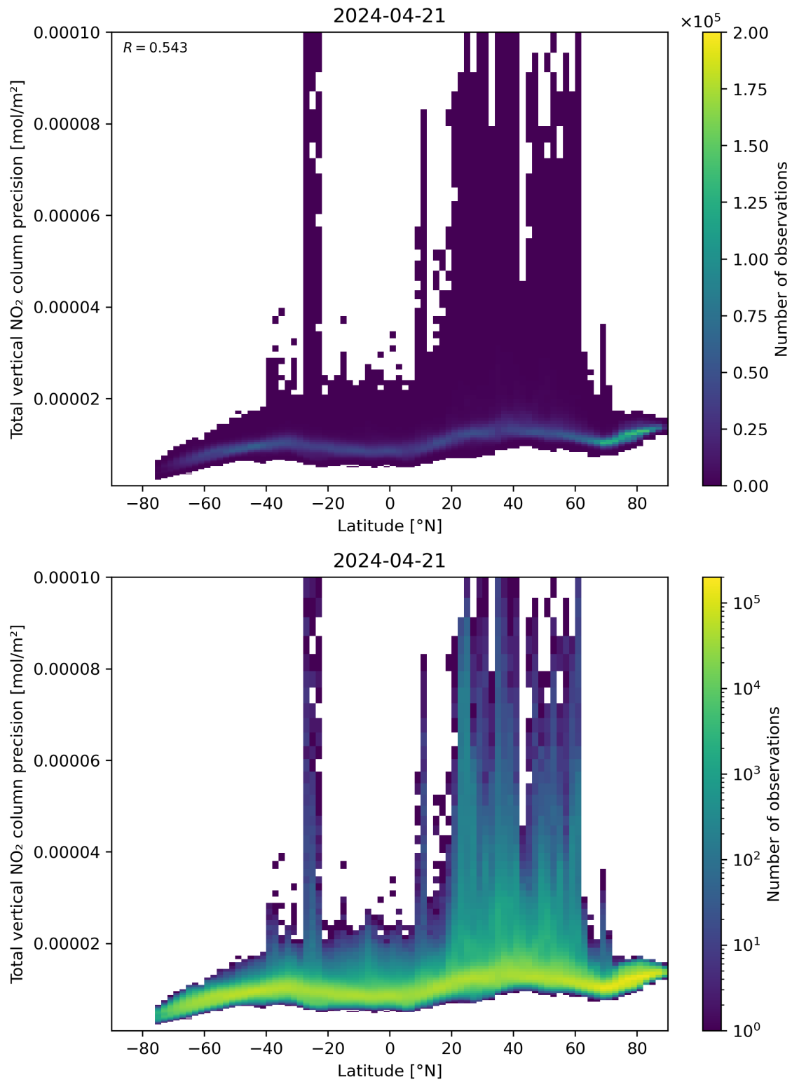
Figure 91: Scatter density plot of “Latitude” against “Total vertical NO 2 column precision” for 2024-04-21 to 2024-04-22.
