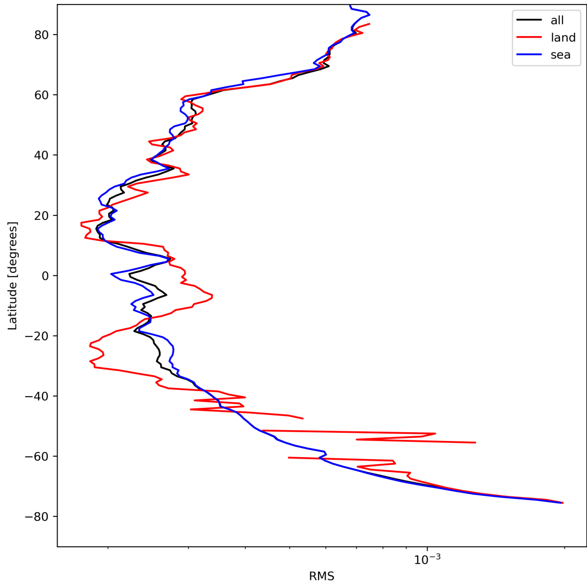
Figure 26: Zonal average of “RMS” for 2024-04-21 to 2024-04-22.
