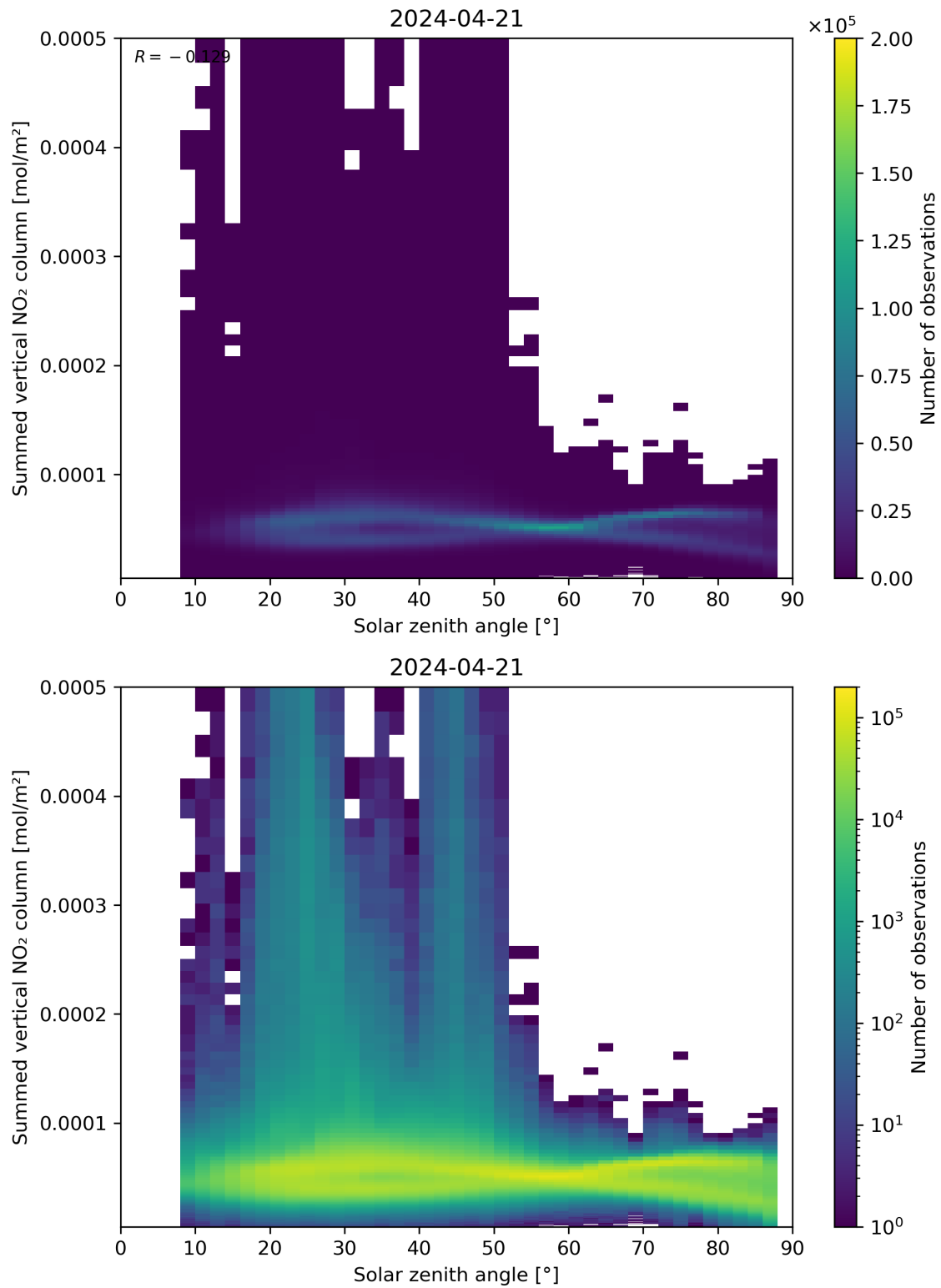
Figure 151: Scatter density plot of “Solar zenith angle” against “Summed vertical NO 2 column” for 2024-04-21 to 2024-04-22.
