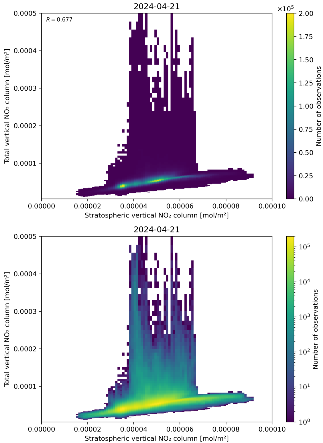
Figure 100: Scatter density plot of “Stratospheric vertical NO 2 column” against “Total vertical NO 2 column” for 2024-04-21 to 2024-04-22.
