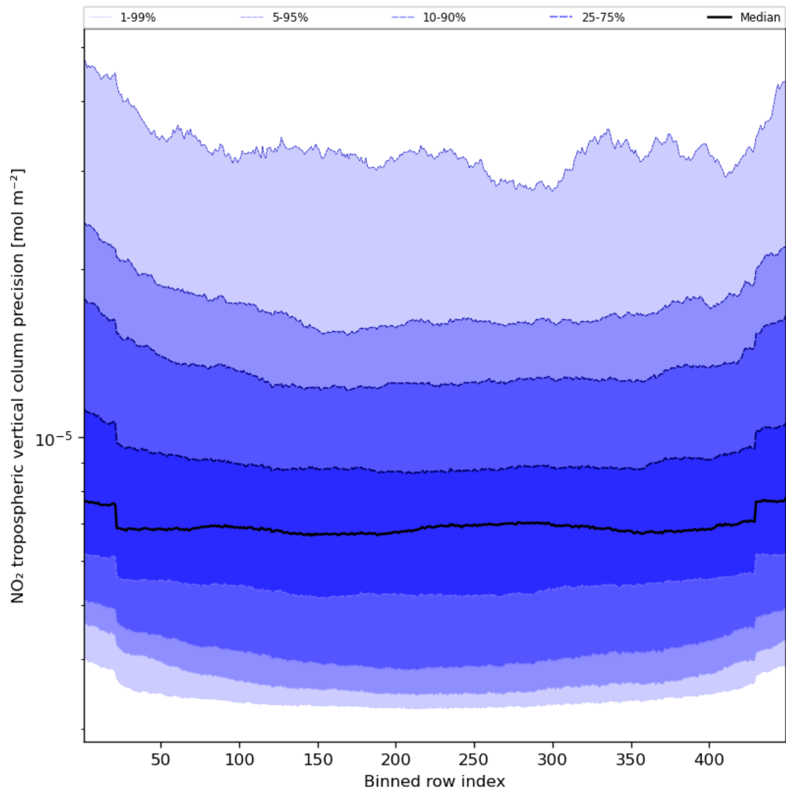
Figure 47: Along track statistics of “NO 2 tropospheric vertical column precision” for 2024-04-21 to 2024-04-22
