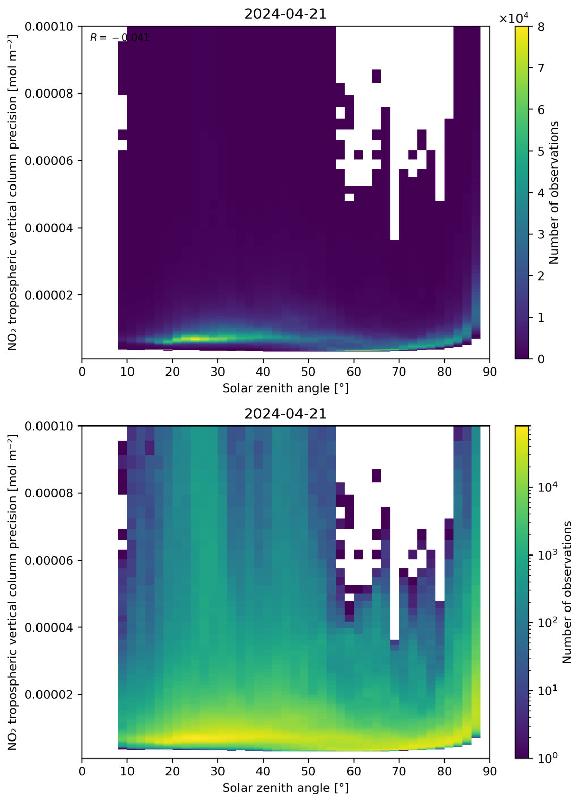
Figure 156: Scatter density plot of “Solar zenith angle” against “NO 2 tropospheric vertical column precision” for 2024-04-21 to 2024-04-22.
