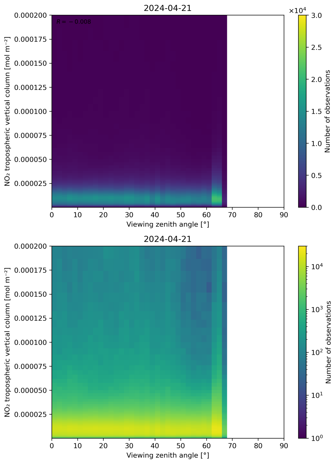
Figure 169: Scatter density plot of “Viewing zenith angle” against “NO 2 tropospheric vertical column” for 2024-04-21 to 2024-04-22.
