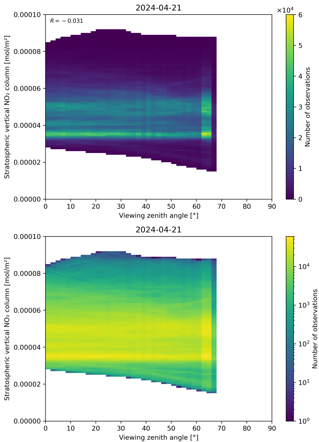
Figure 164: Scatter density plot of “Viewing zenith angle” against “Stratospheric vertical NO 2 column” for 2024-04-21 to 2024-04-22.
