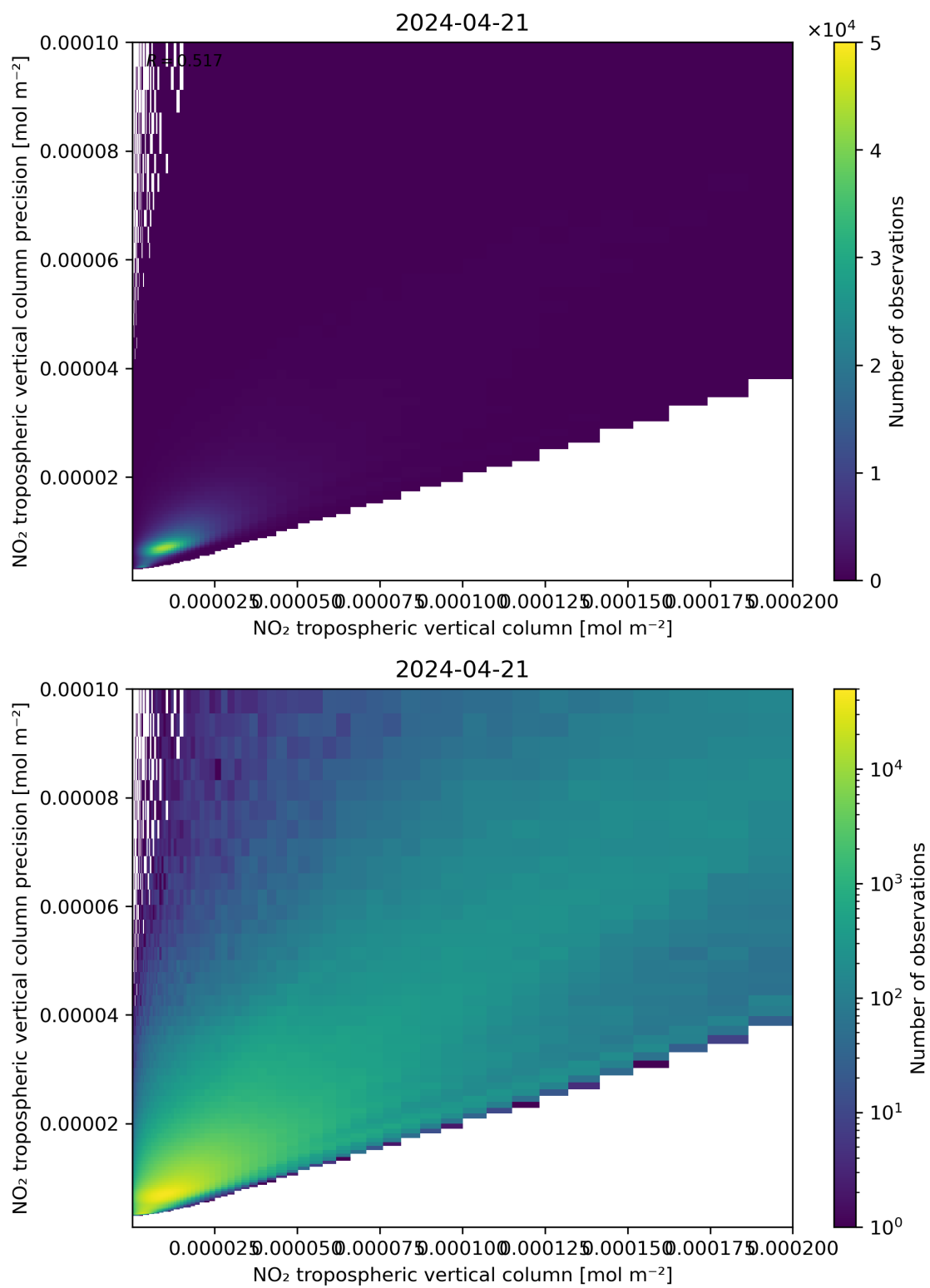
Figure 130: Scatter density plot of “NO 2 tropospheric vertical column” against “NO 2 tropospheric vertical column precision” for 2024-04-21 to 2024-04-22.
