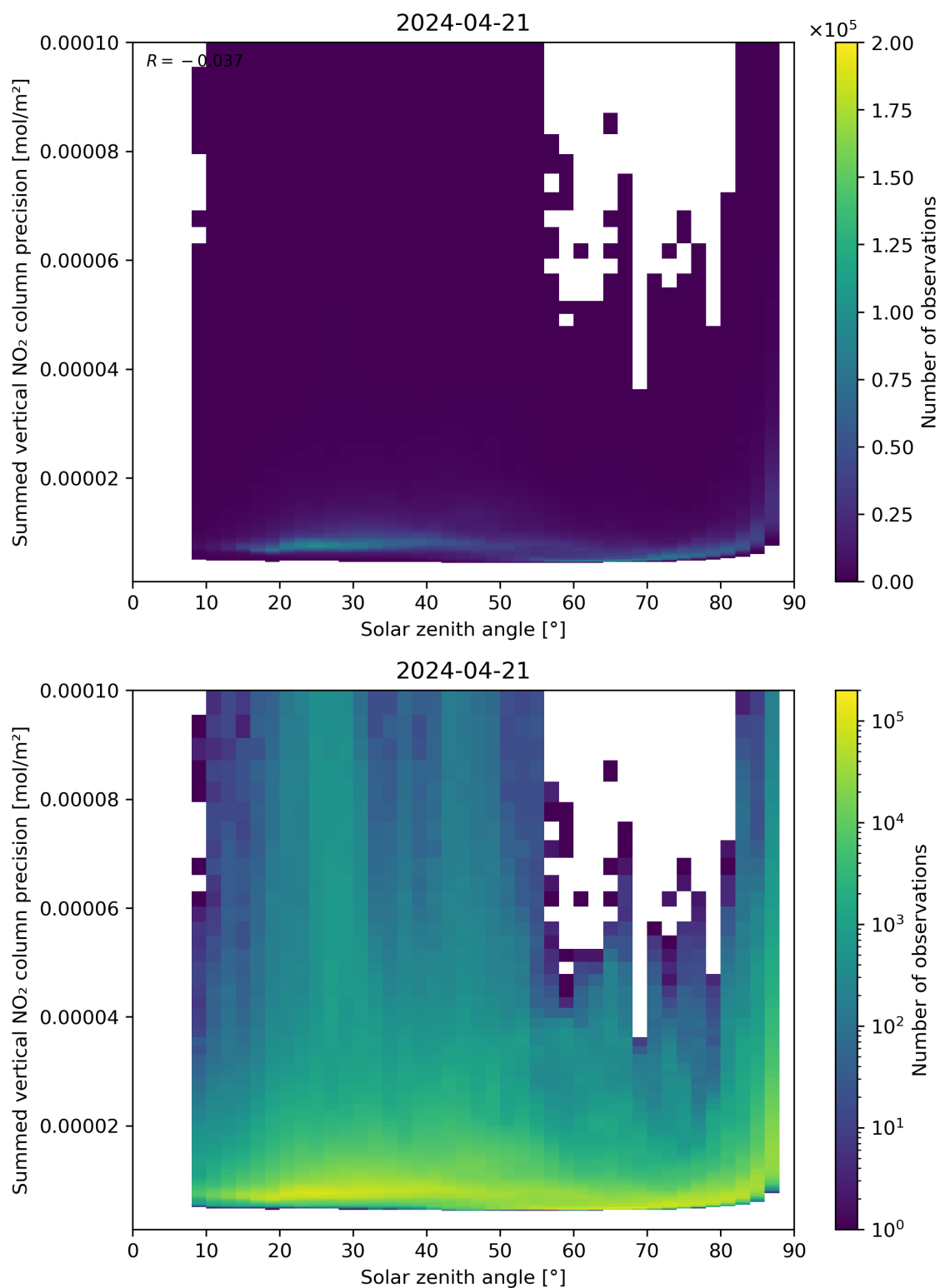
Figure 152: Scatter density plot of “Solar zenith angle” against “Summed vertical NO 2 column precision” for 2024-04-21 to 2024-04-22.
