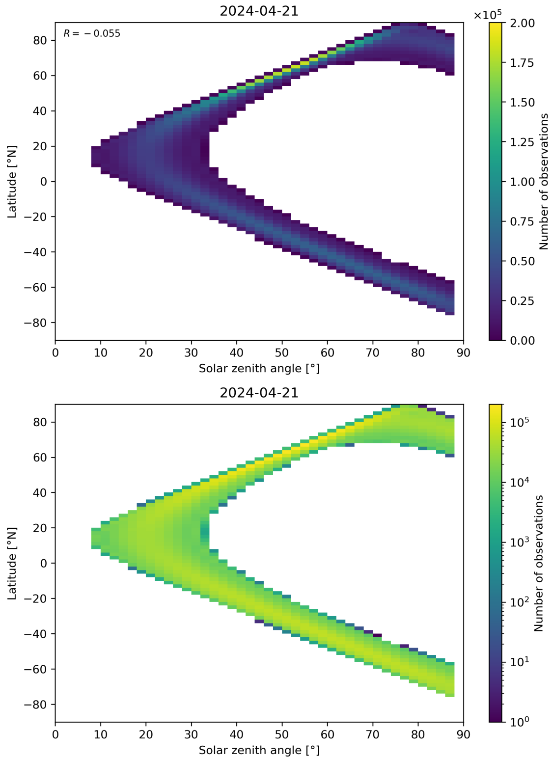
Figure 149: Scatter density plot of “Solar zenith angle” against “Latitude” for 2024-04-21 to 2024-04-22.
