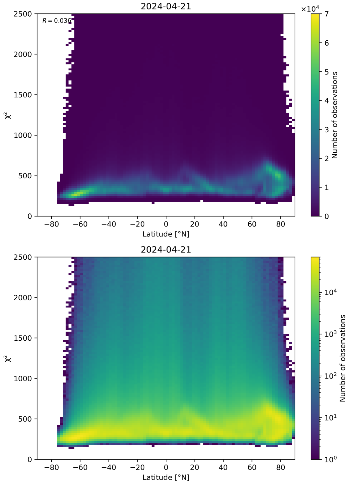
Figure 86: Scatter density plot of “Latitude” against “ \chi^2 ” for 2024-04-21 to 2024-04-22.
