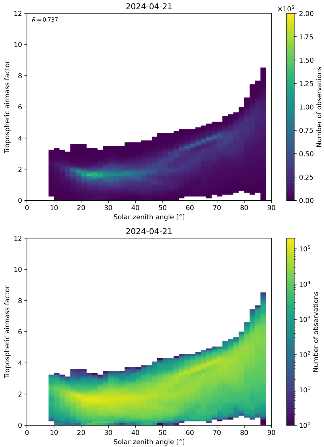
Figure 147: Scatter density plot of “Solar zenith angle” against “Tropospheric airmass factor” for 2024-04-21 to 2024-04-22.
