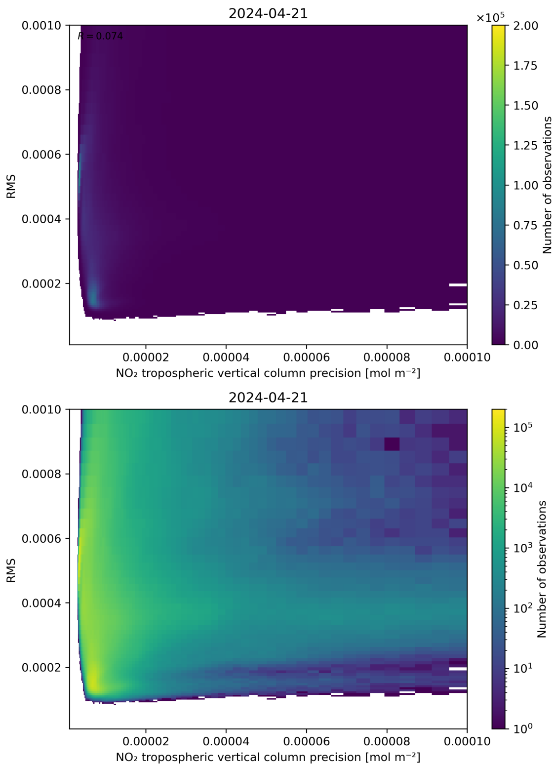
Figure 140: Scatter density plot of “NO 2 tropospheric vertical column precision” against “RMS” for 2024-04-21 to 2024-04-22.
