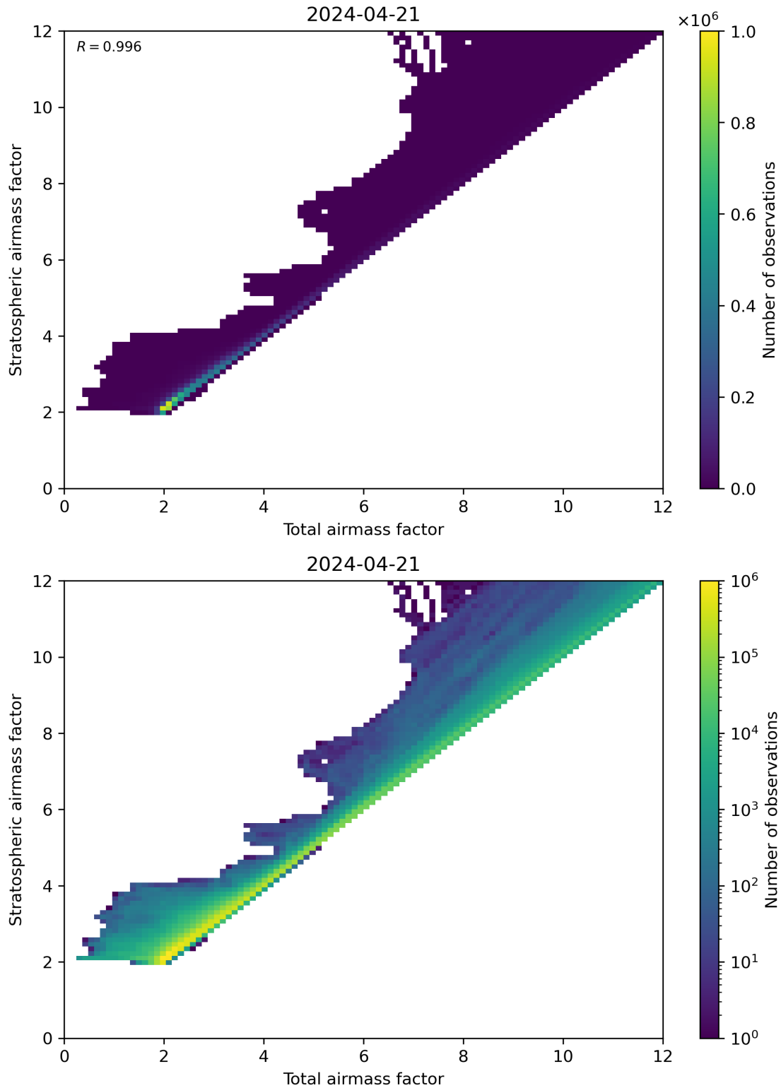
Figure 62: Scatter density plot of “Total airmass factor” against “Stratospheric airmass factor” for 2024-04-21 to 2024-04-22.
