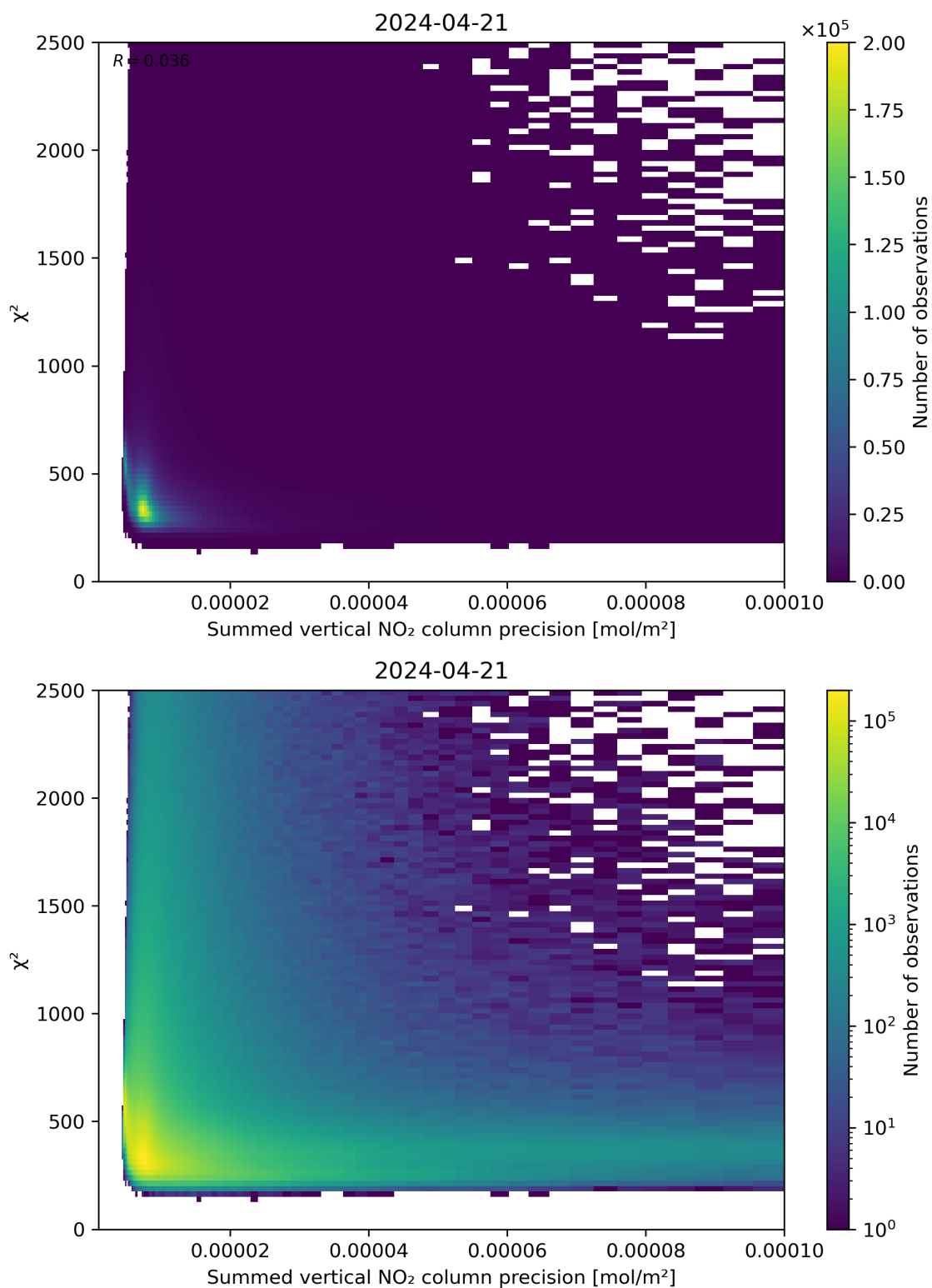
Figure 107: Scatter density plot of “Summed vertical NO 2 column precision” against “ \chi^2 ” for 2024-04-21 to 2024-04-22.
