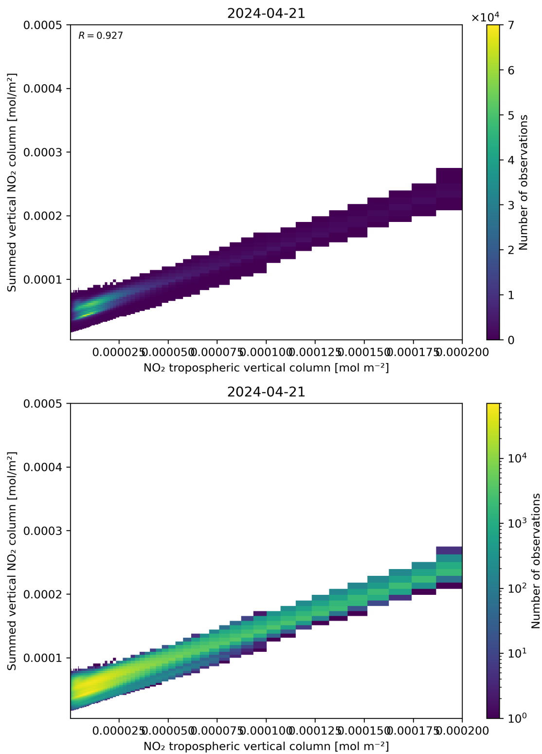
Figure 126: Scatter density plot of “NO 2 tropospheric vertical column” against “Summed vertical NO 2 column” for 2024-04-21 to 2024-04-22.
