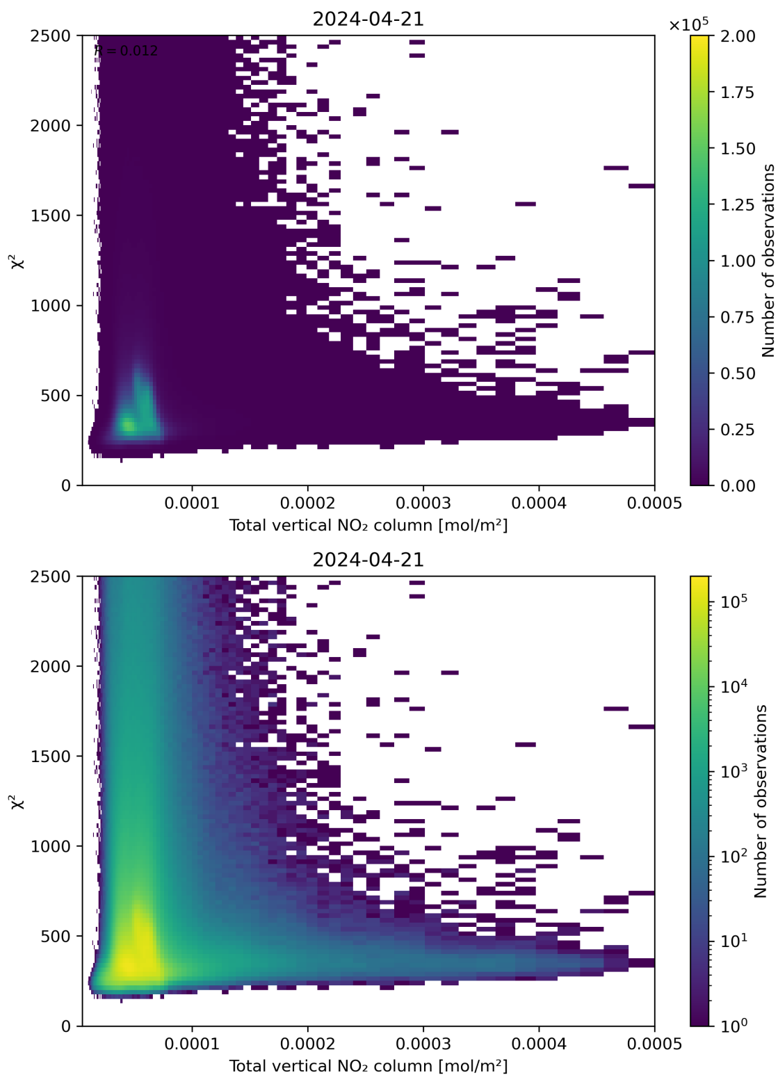
Figure 111: Scatter density plot of “Total vertical NO 2 column” against “ \chi^2 ” for 2024-04-21 to 2024-04-22.
