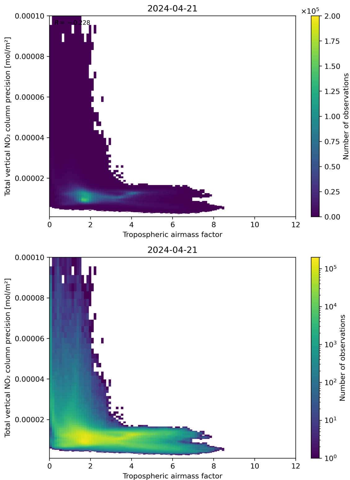
Figure 78: Scatter density plot of “Tropospheric air mass factor” against “Total vertical NO 2 column precision” for 2024-04-21 to 2024-04-22.
