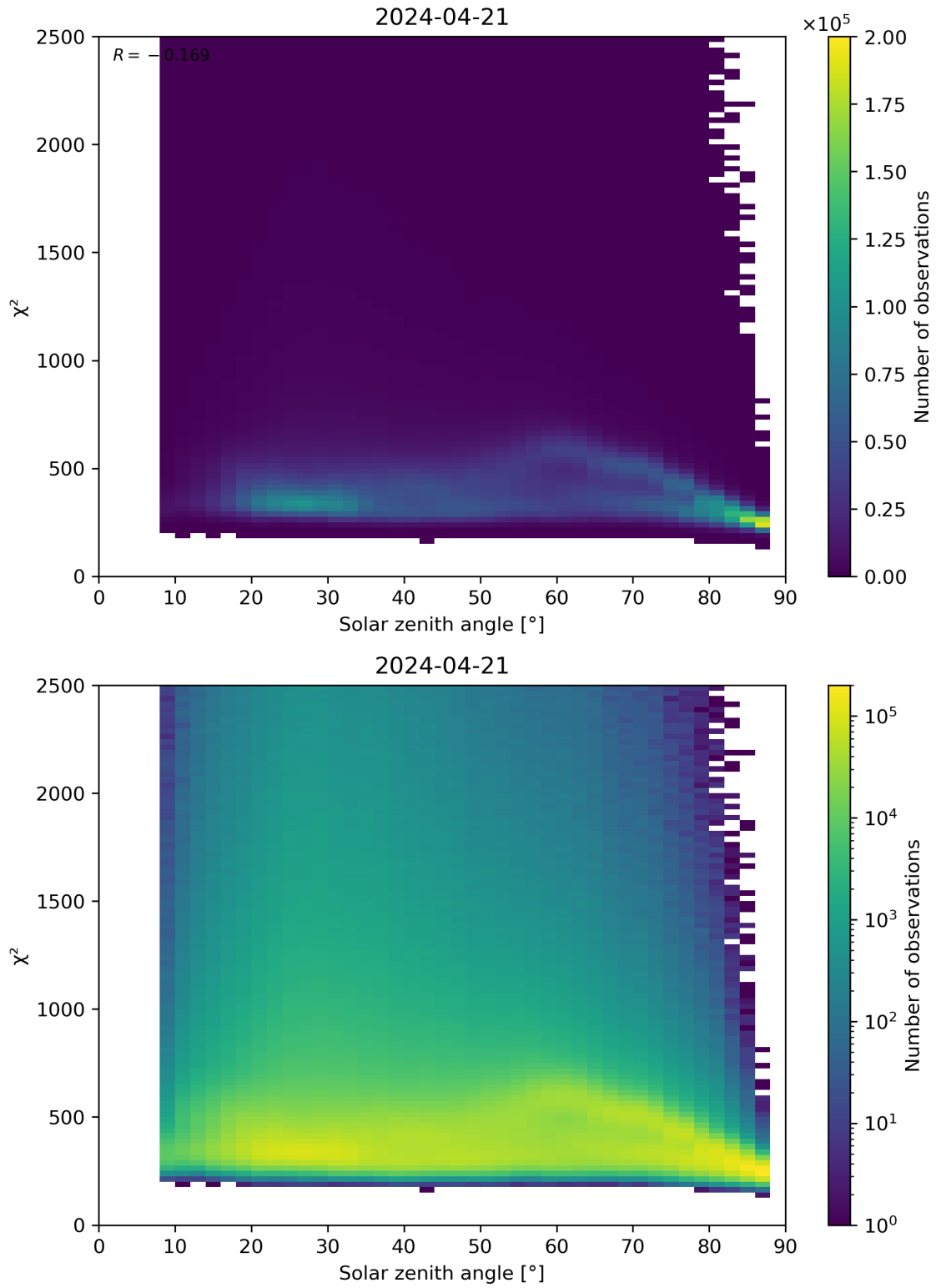
Figure 148: Scatter density plot of “Solar zenith angle” against “ \chi^2 ” for 2024-04-21 to 2024-04-22.
