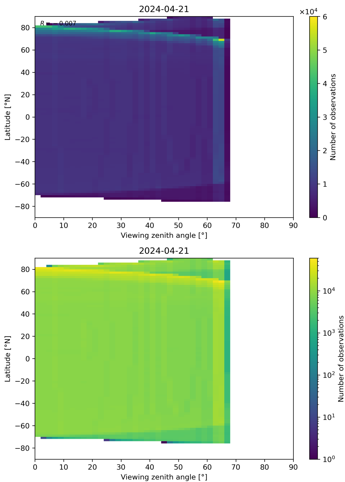
Figure 163: Scatter density plot of “Viewing zenith angle” against “Latitude” for 2024-04-21 to 2024-04-22.
