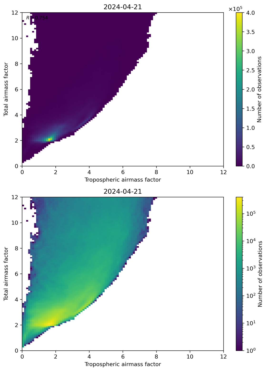
Figure 72: Scatter density plot of “Tropospheric airmass factor” against “Total airmass factor” for 2024-04-21 to 2024-04-22.
