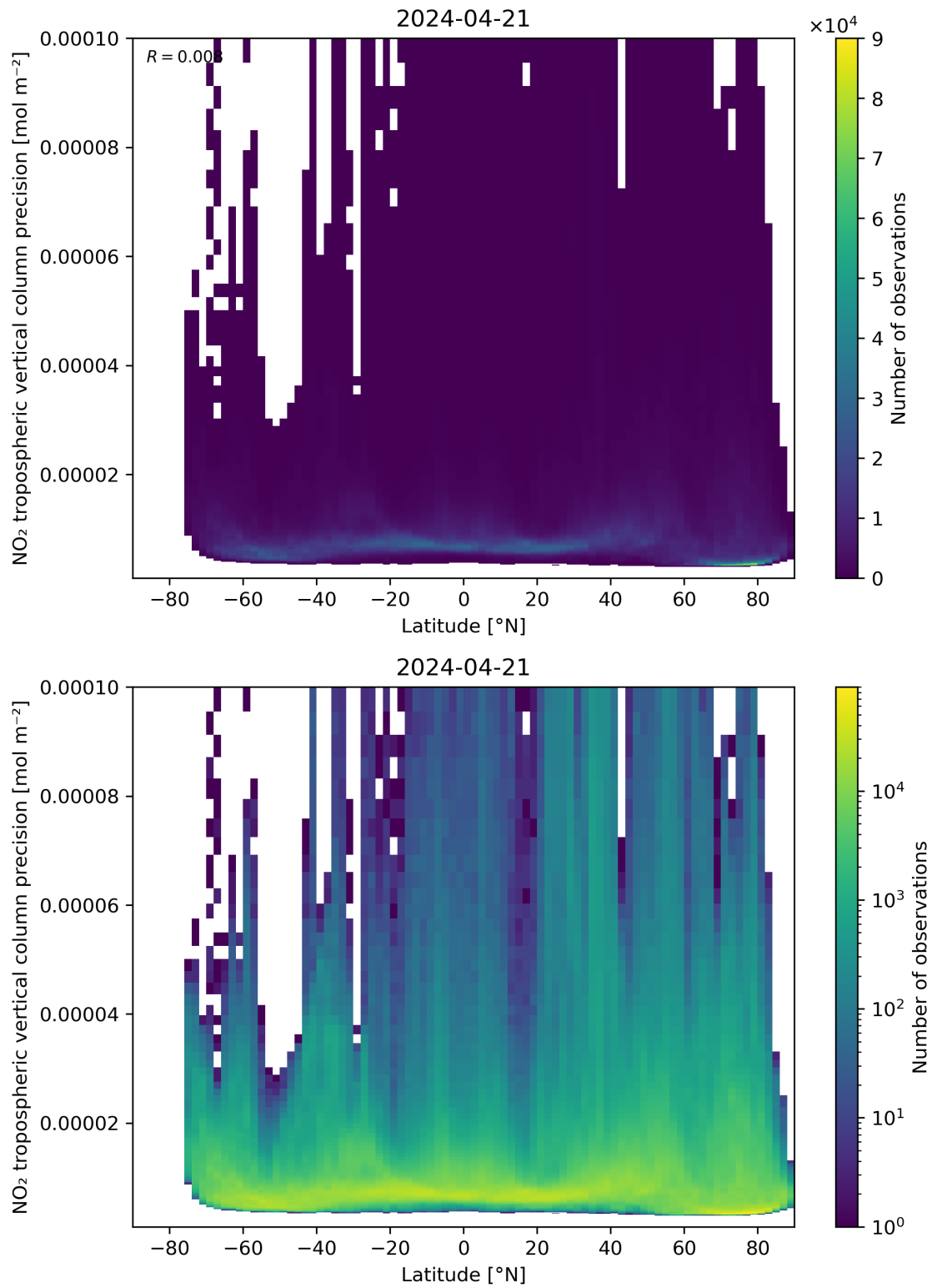
Figure 93: Scatter density plot of “Latitude” against “NO 2 tropospheric vertical column precision” for 2024-04-21 to 2024-04-22.
