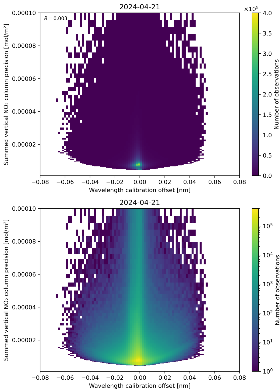
Figure 178: Scatter density plot of “Wavelength calibration offset” against “Summed vertical NO 2 column precision” for 2024-04-21 to 2024-04-22.
