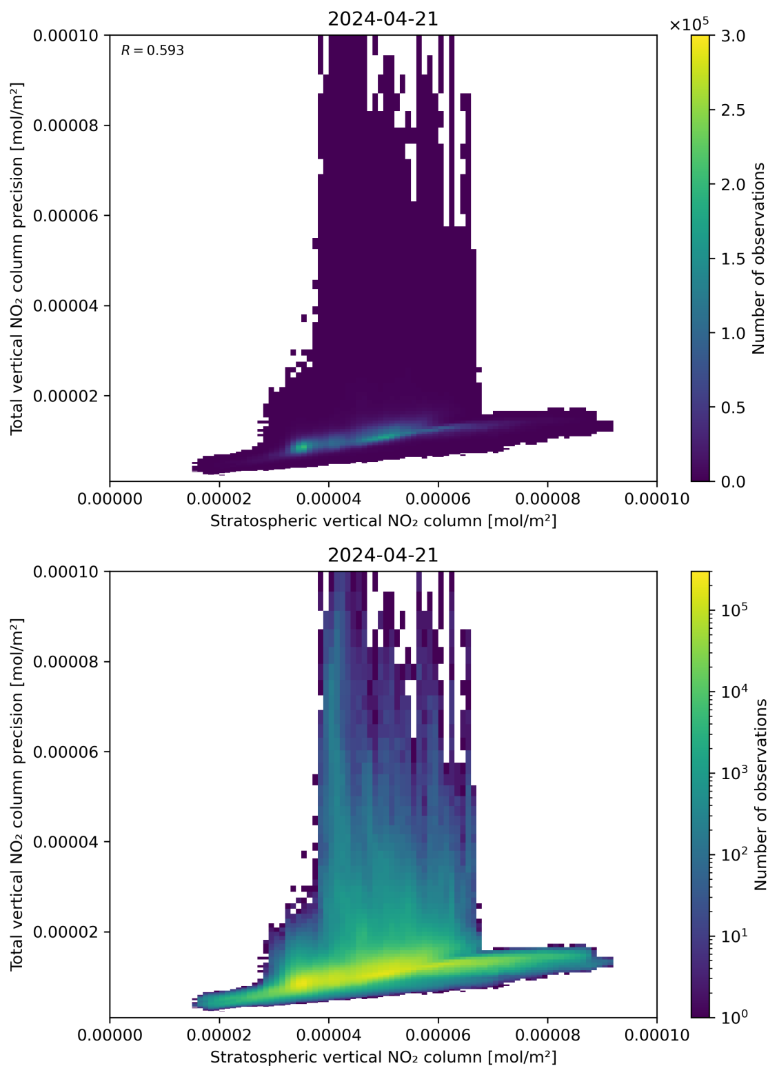
Figure 101: Scatter density plot of “Stratospheric vertical NO 2 column” against “Total vertical NO 2 column precision” for 2024-04-21 to 2024-04-22.
