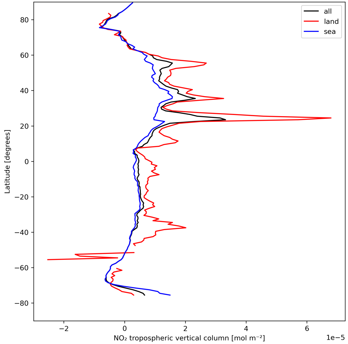
Figure 12: Zonal average of “NO 2 tropospheric vertical column” for 2024-04-21 to 2024-04-22.
