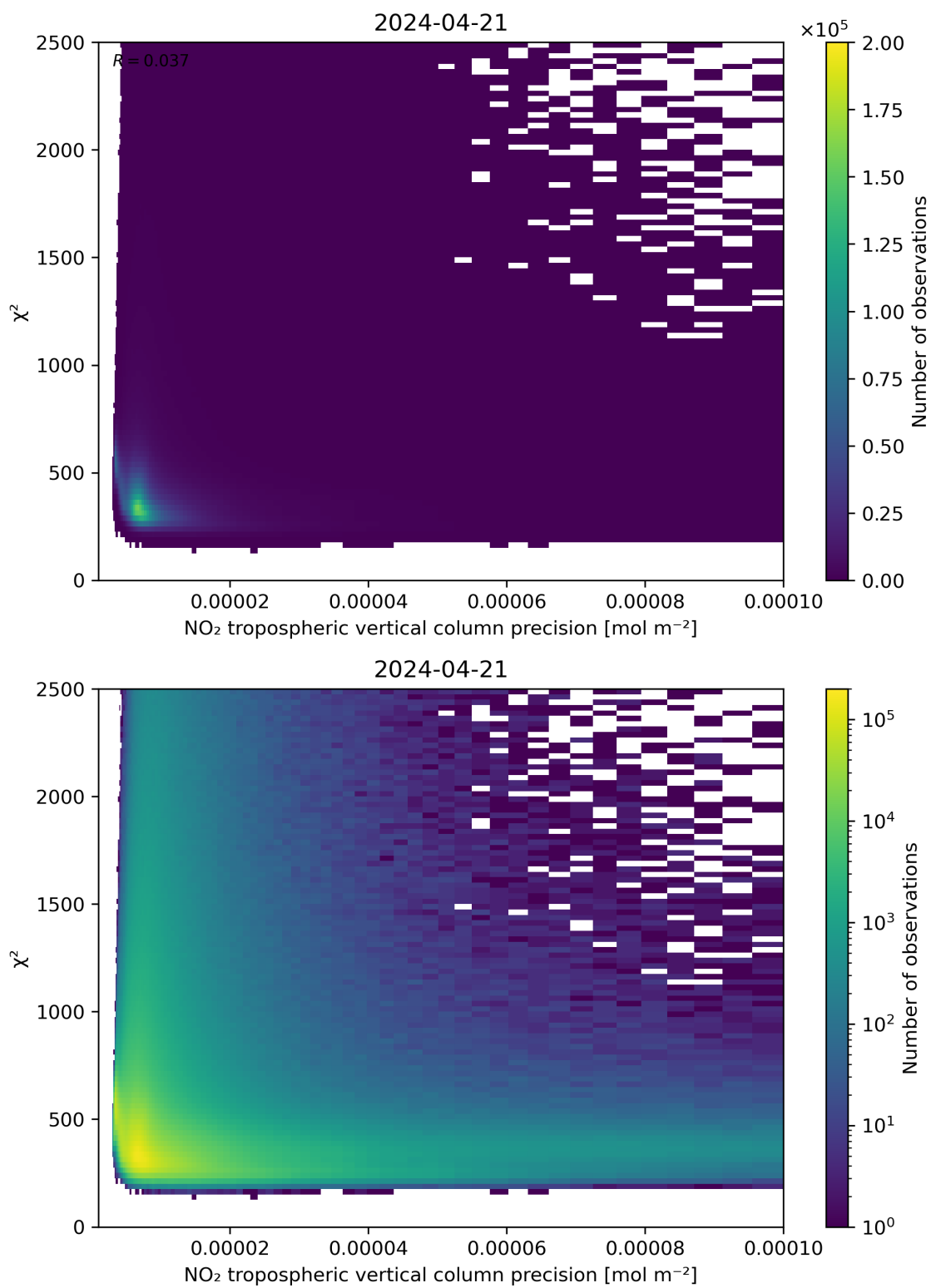
Figure 134: Scatter density plot of “NO 2 tropospheric vertical column precision” against “ \chi^2 ” for 2024-04-21 to 2024-04-22.
