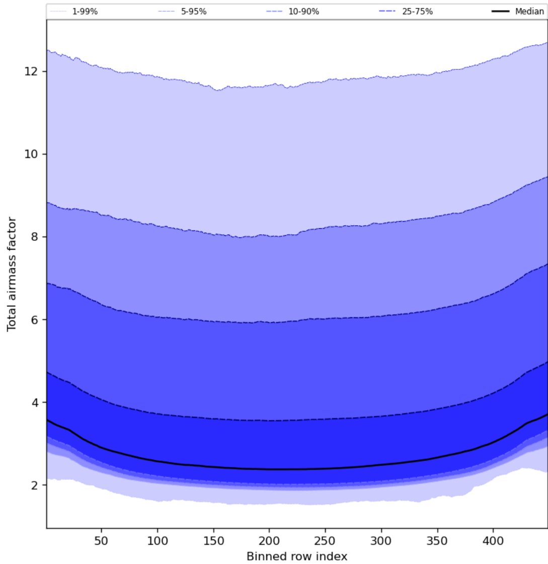
Figure 49: Along track statistics of “Total airmass factor” for 2024-04-21 to 2024-04-22
