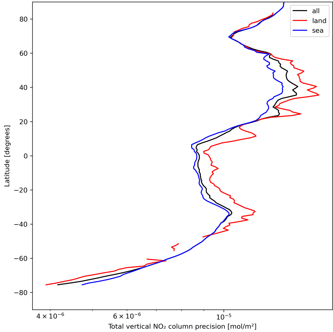
Figure 22: Zonal average of "Total vertical NO 2 column precision" for 2024-04-21 to 2024-04-22.
