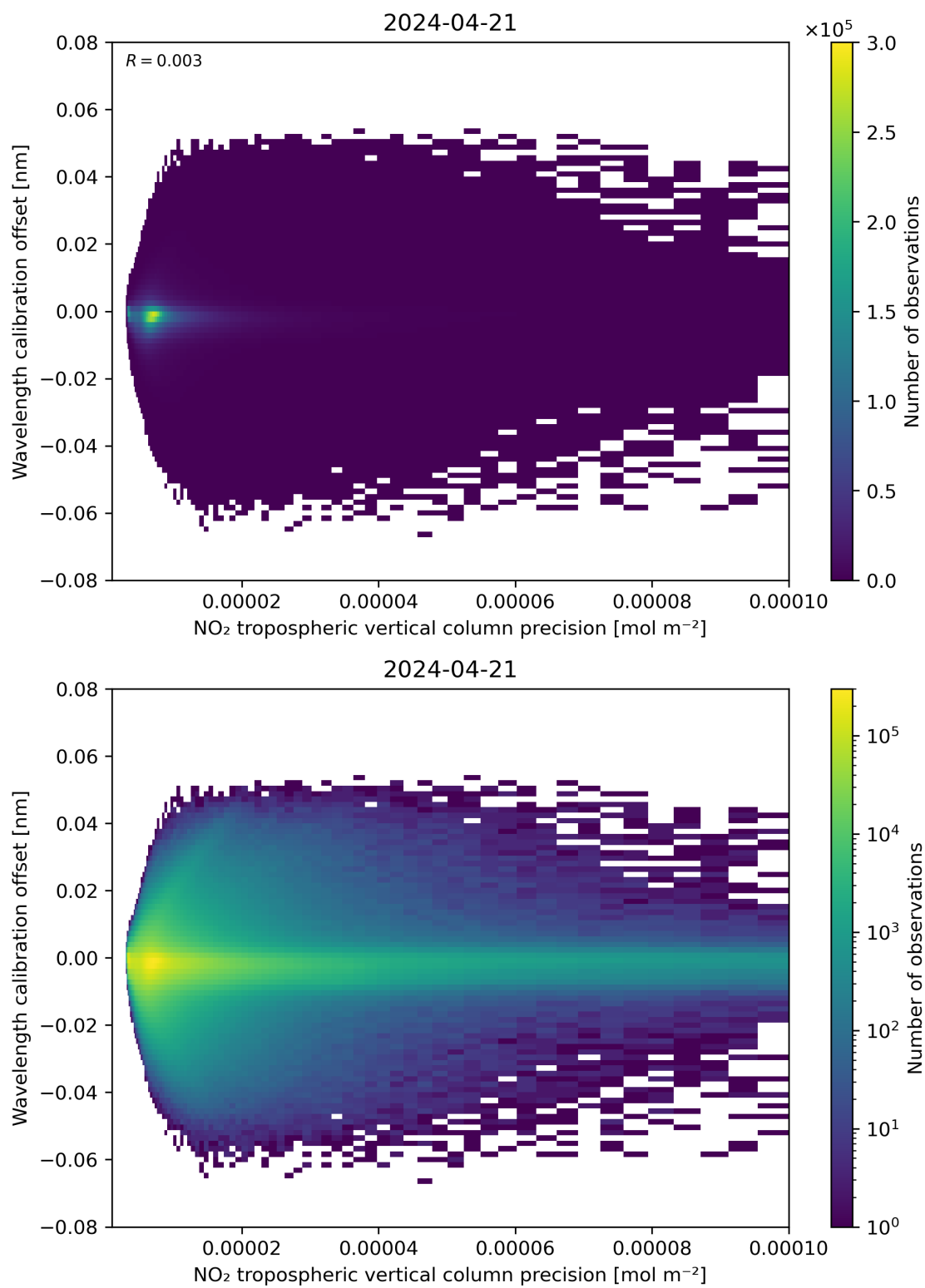
Figure 141: Scatter density plot of “NO 2 tropospheric vertical column precision” against “Wavelength calibration offset” for 2024-04-21 to 2024-04-22.
