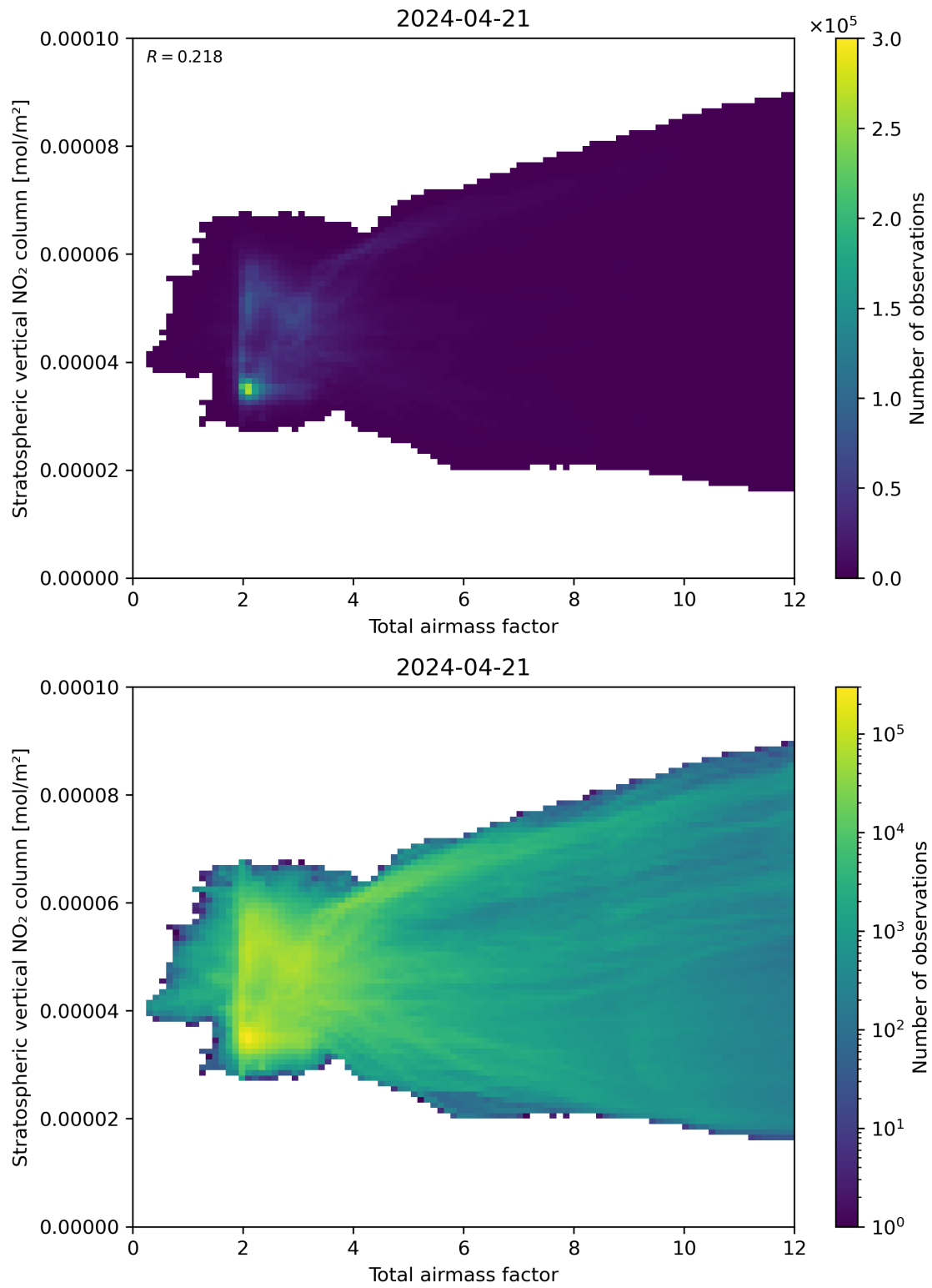
Figure 64: Scatter density plot of “Total airmass factor” against “Stratospheric vertical NO 2 column” for 2024-04-21 to 2024-04-22.
