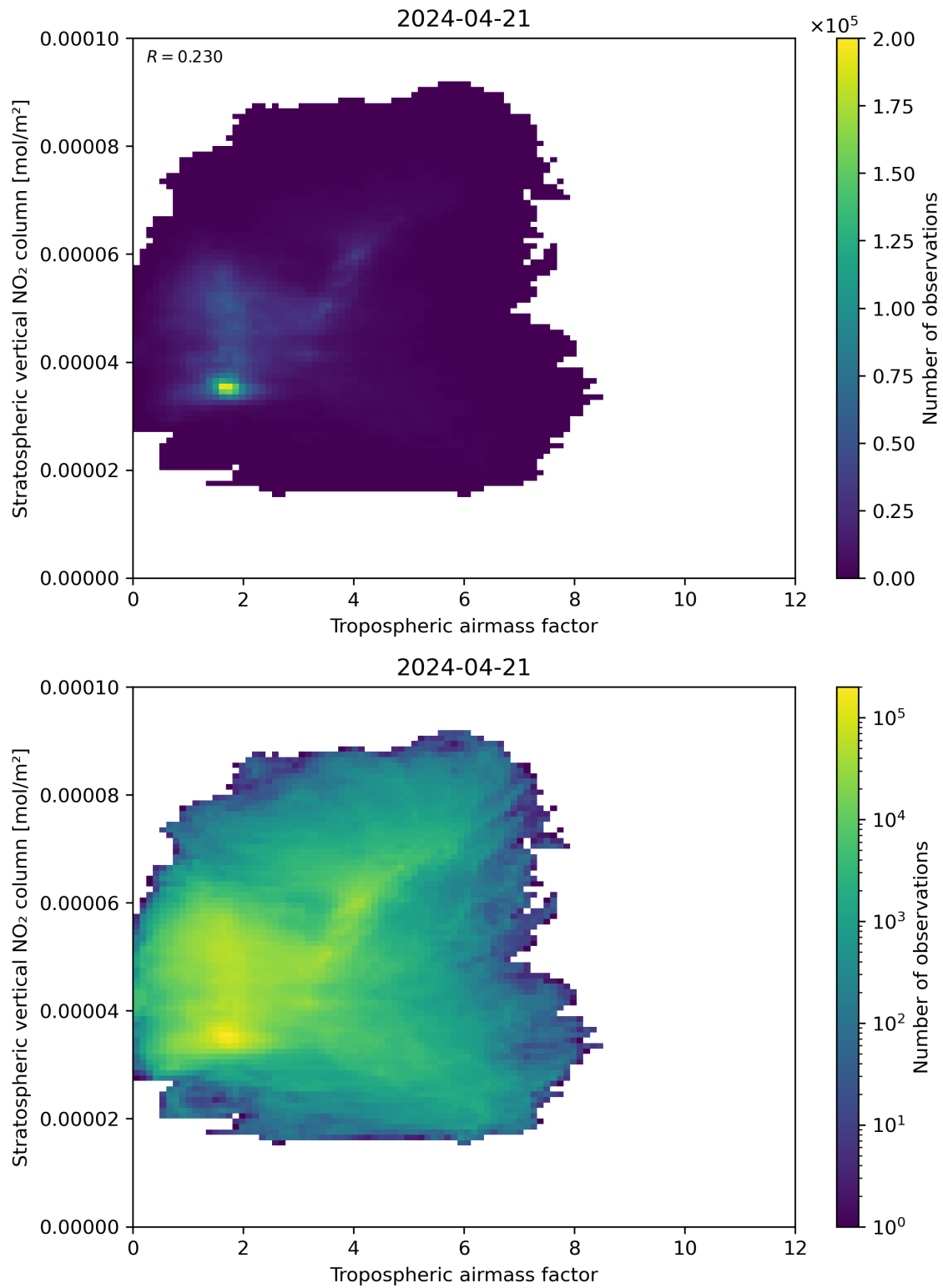
Figure 74: Scatter density plot of “Tropospheric airmass factor” against “Stratospheric vertical \text{NO}_2 column” for 2024-04-21 to 2024-04-22.
