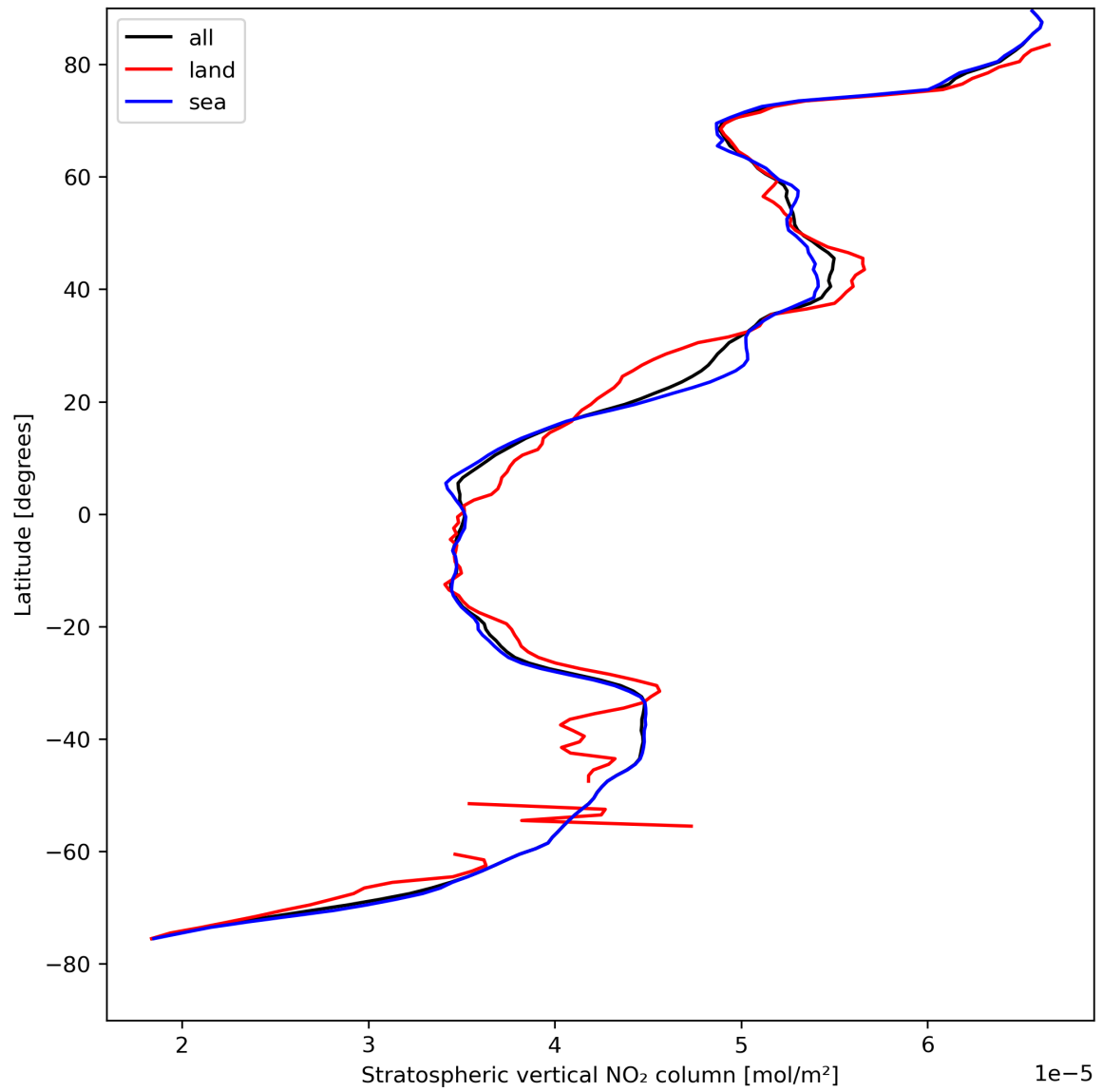
Figure 19: Zonal average of “Stratospheric vertical NO 2 column” for 2024-04-21 to 2024-04-22.
