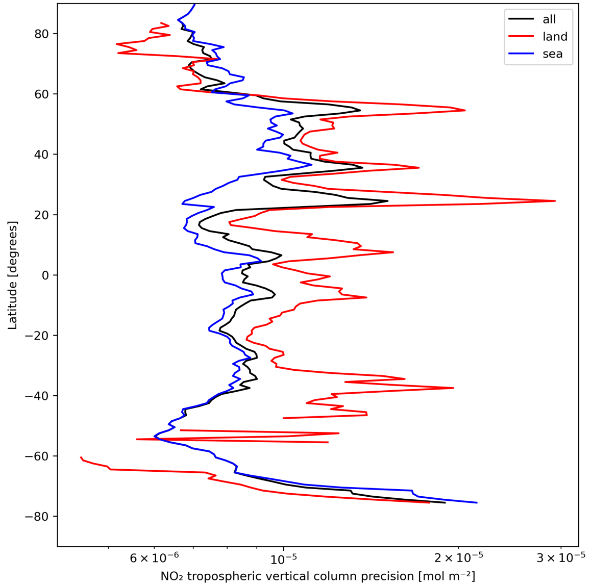
Figure 13: Zonal average of “NO 2 tropospheric vertical column precision” for 2024-04-21 to 2024-04-22.
