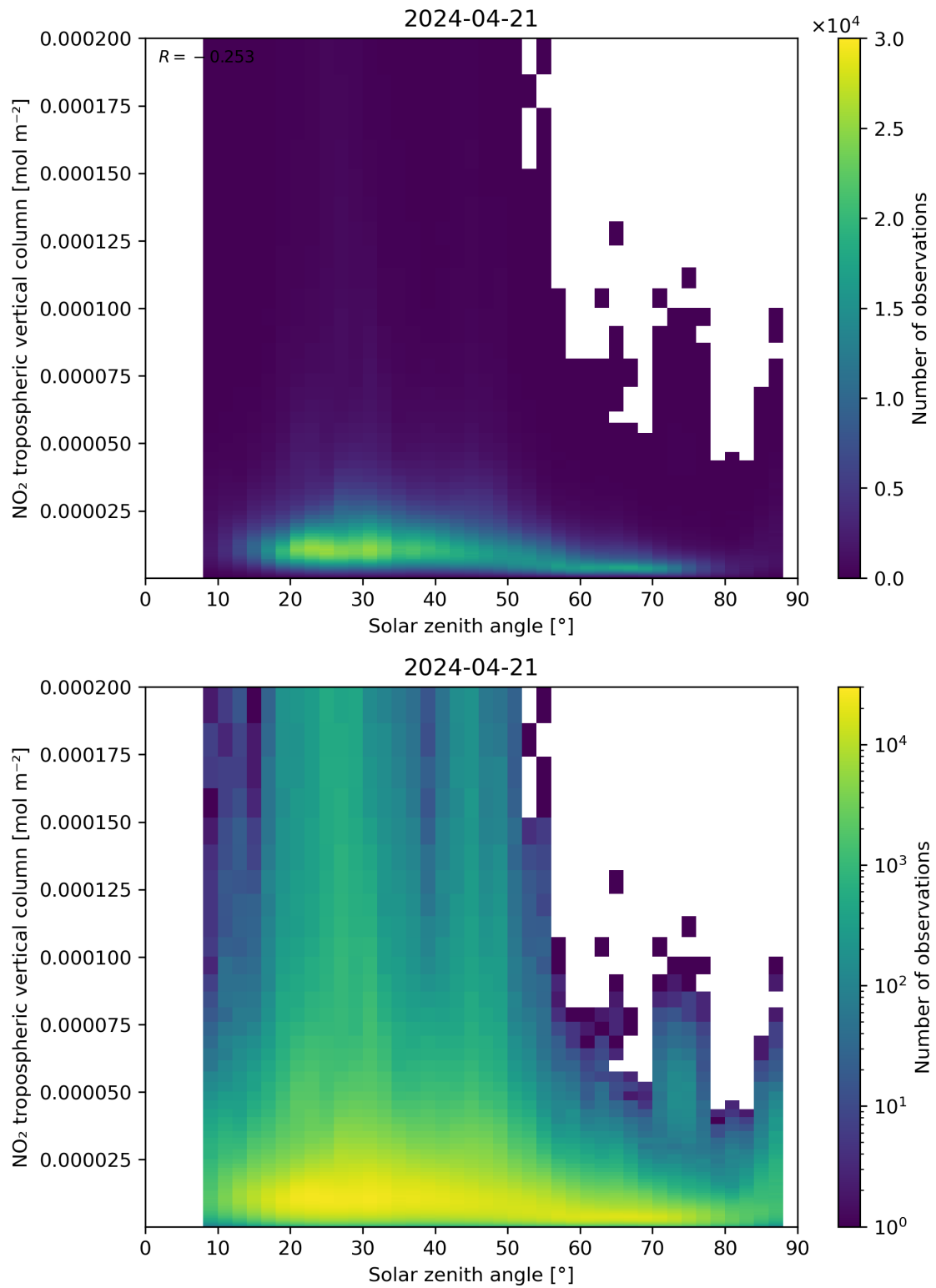
Figure 155: Scatter density plot of “Solar zenith angle” against “NO 2 tropospheric vertical column” for 2024-04-21 to 2024-04-22.
