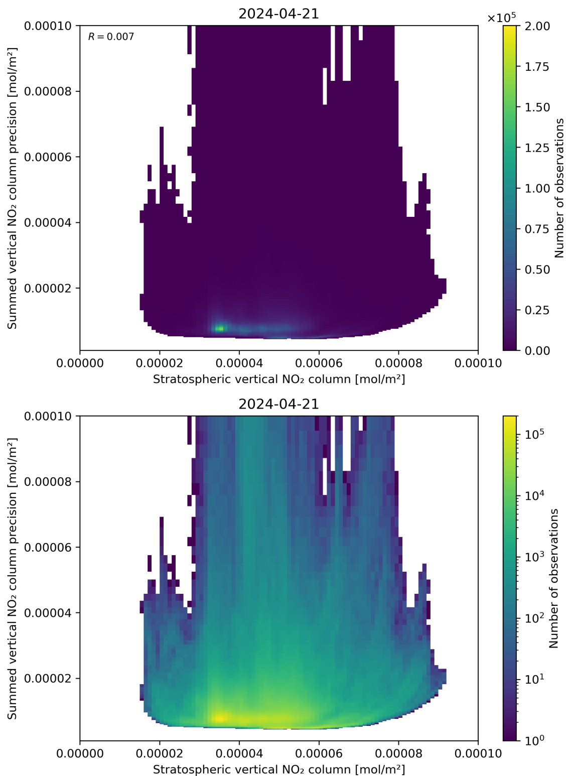
Figure 99: Scatter density plot of “Stratospheric vertical NO 2 column” against “Summed vertical NO 2 column precision” for 2024-04-21 to 2024-04-22.
