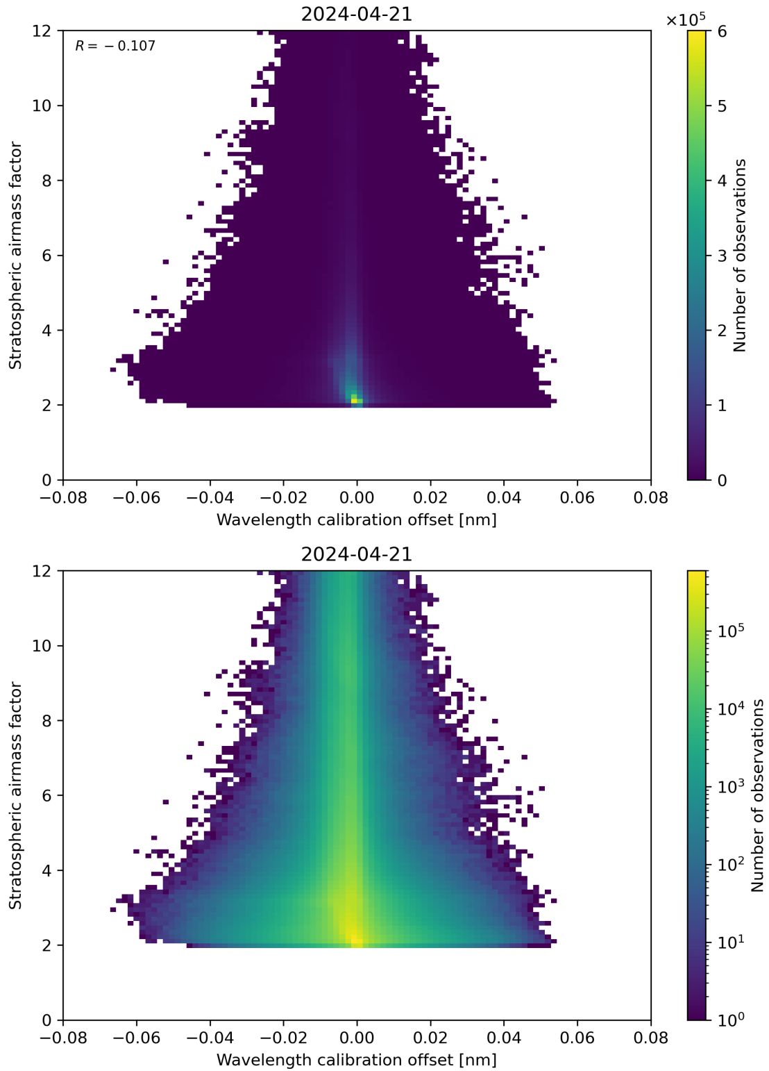
Figure 174: Scatter density plot of “Wavelength calibration offset” against “Stratospheric airmass factor” for 2024-04-21 to 2024-04-22.
