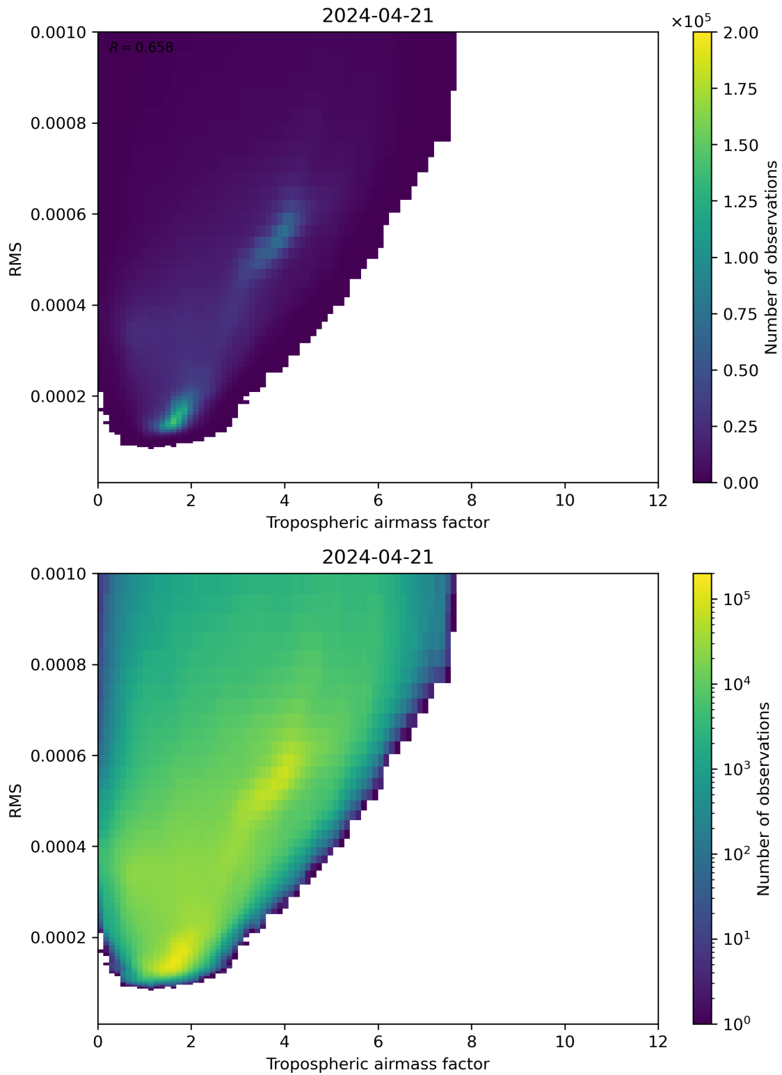
Figure 79: Scatter density plot of “Tropospheric airmass factor” against “RMS” for 2024-04-21 to 2024-04-22.
