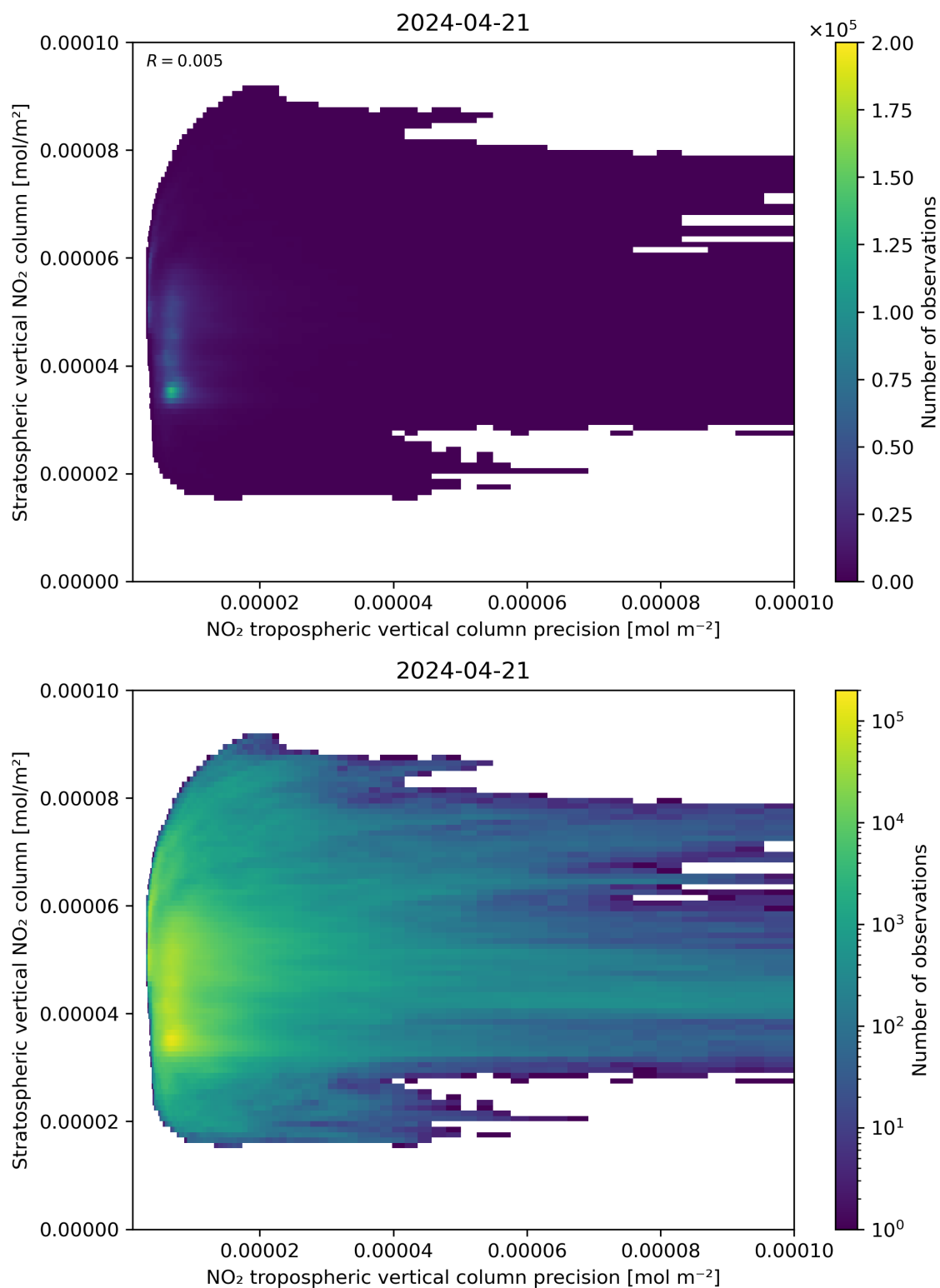
Figure 135: Scatter density plot of “NO 2 tropospheric vertical column precision” against “Stratospheric vertical NO 2 column” for 2024-04-21 to 2024-04-22.
