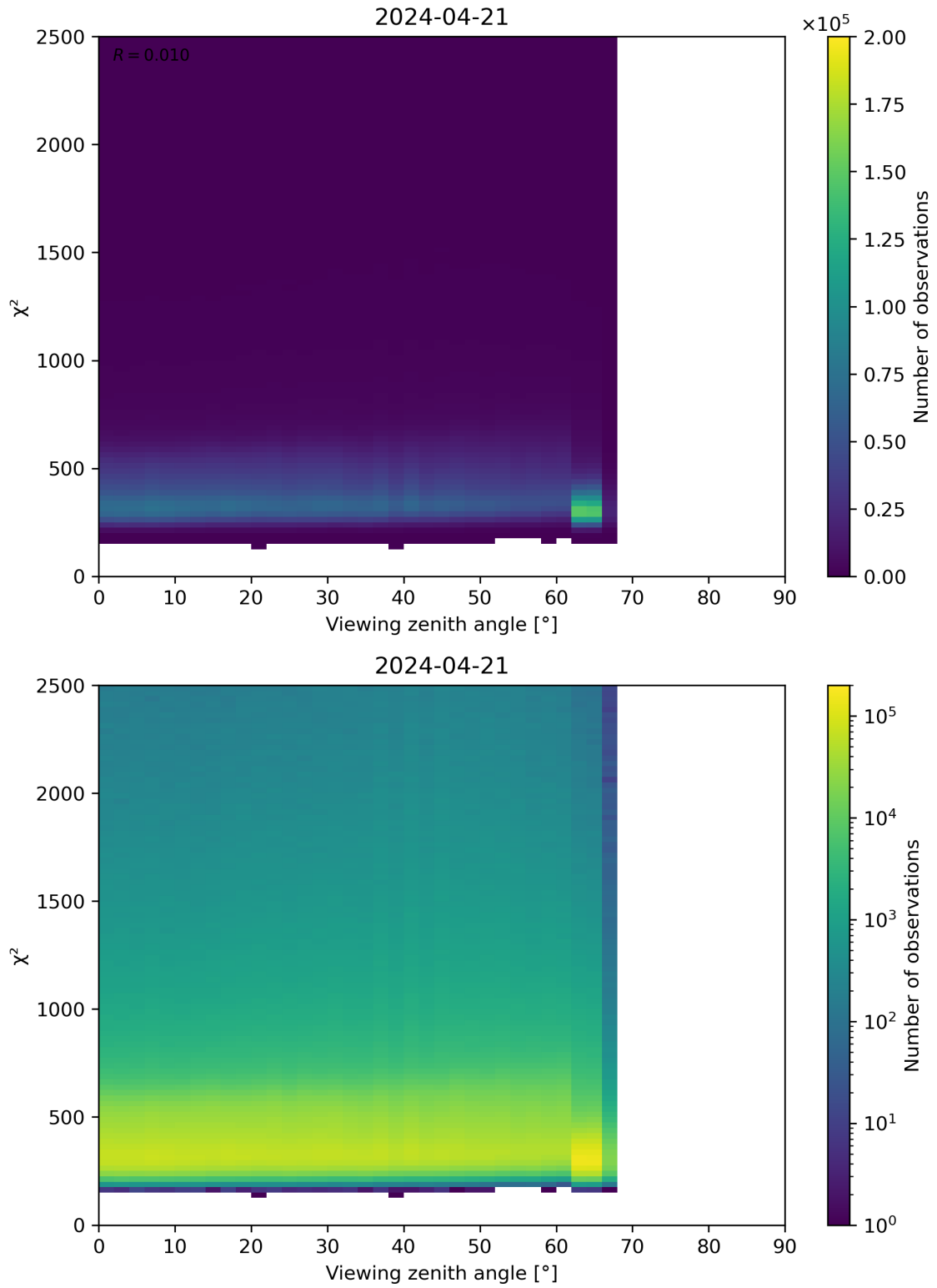
Figure 162: Scatter density plot of “Viewing zenith angle” against “ \chi^2 ” for 2024-04-21 to 2024-04-22.
