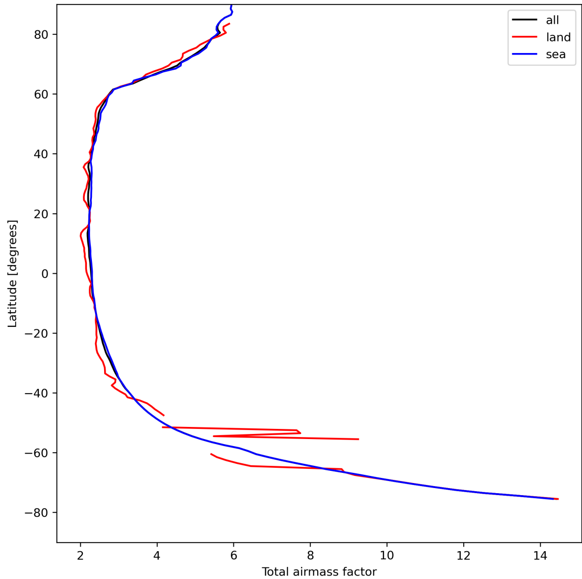
Figure 15: Zonal average of “Total airmass factor” for 2024-04-21 to 2024-04-22.
