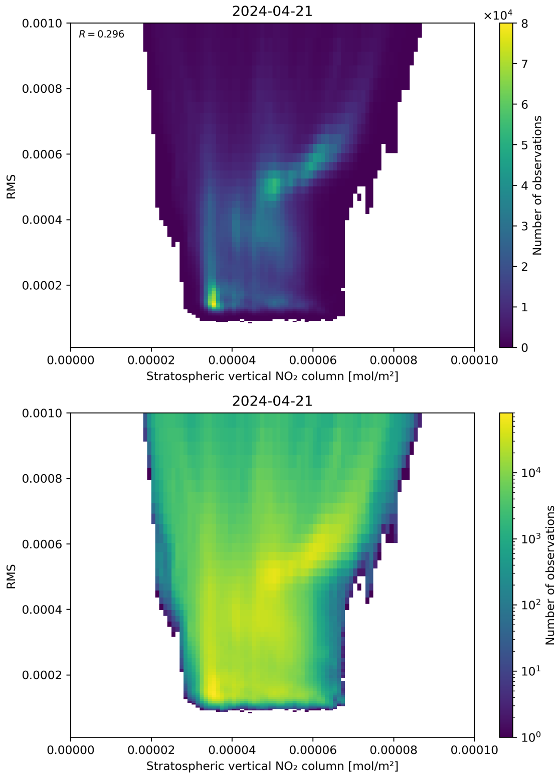
Figure 102: Scatter density plot of “Stratospheric vertical NO 2 column” against “RMS” for 2024-04-21 to 2024-04-22.
