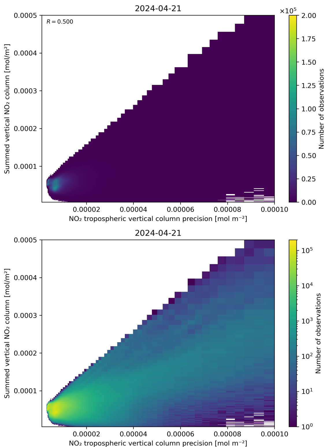
Figure 136: Scatter density plot of “NO 2 tropospheric vertical column precision” against “Summed vertical NO 2 column” for 2024-04-21 to 2024-04-22.
