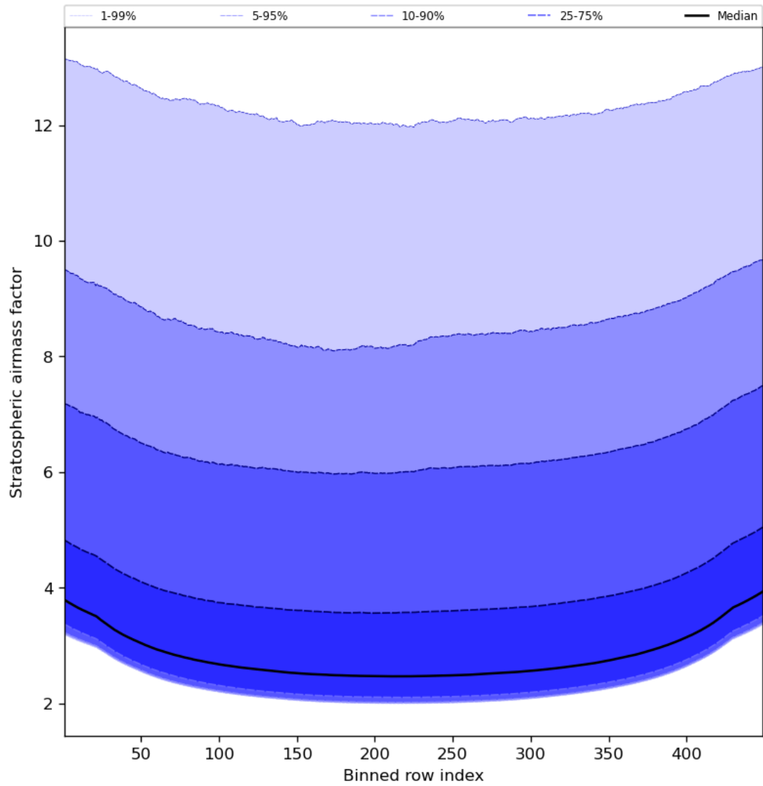
Figure 61: Along track statistics of “Stratospheric airmass factor” for 2024-04-21 to 2024-04-22
