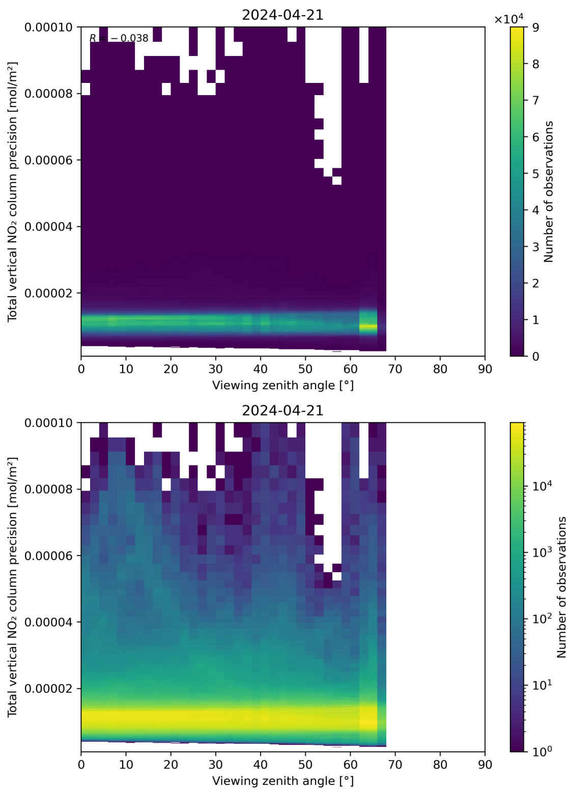
Figure 168: Scatter density plot of “Viewing zenith angle” against “Total vertical NO 2 column precision” for 2024-04-21 to 2024-04-22.
