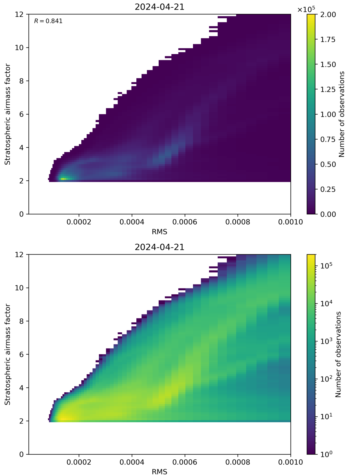
Figure 144: Scatter density plot of “RMS” against “Stratospheric airmass factor” for 2024-04-21 to 2024-04-22.
