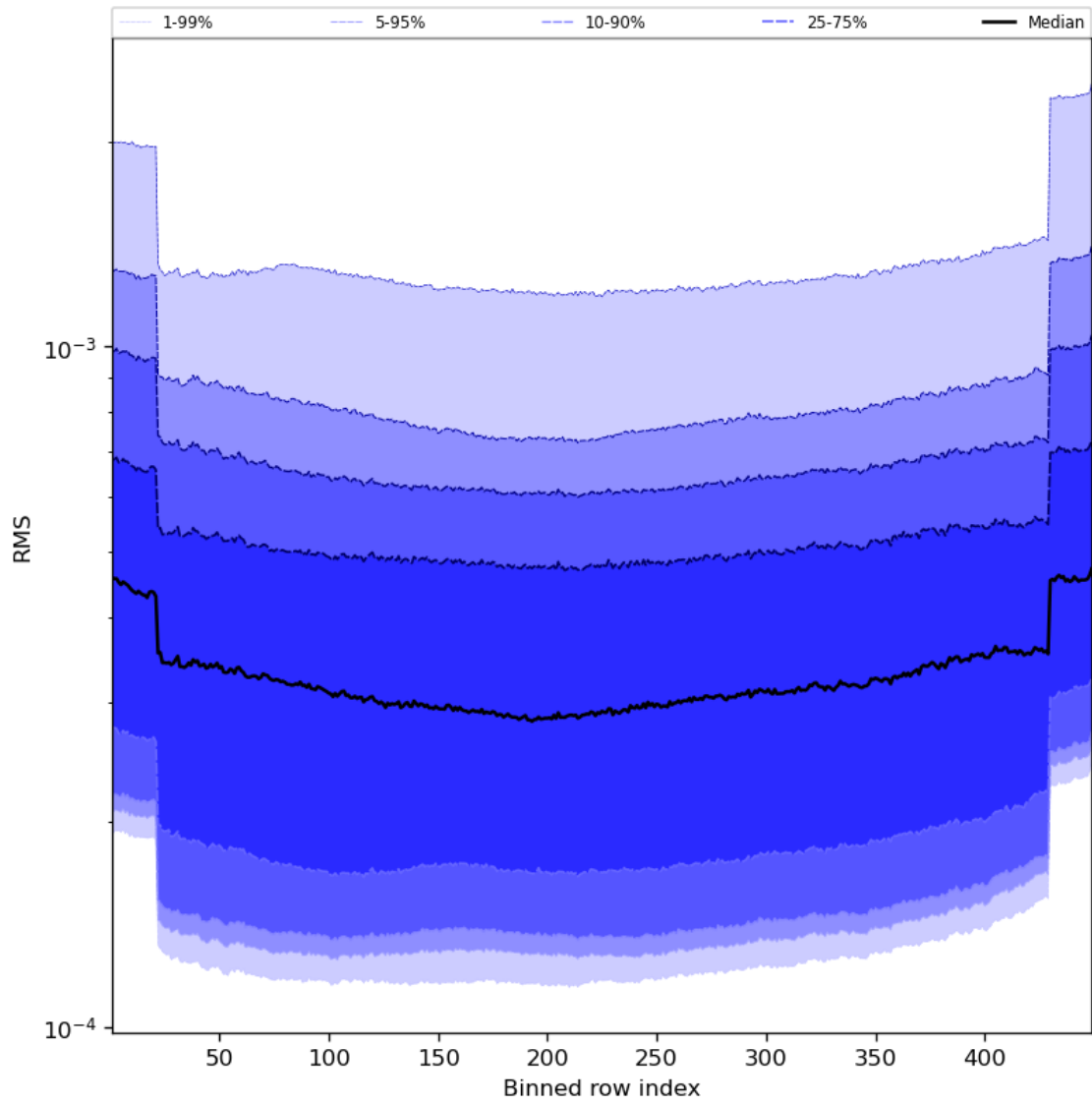
Figure 60: Along track statistics of “RMS” for 2024-04-21 to 2024-04-22
