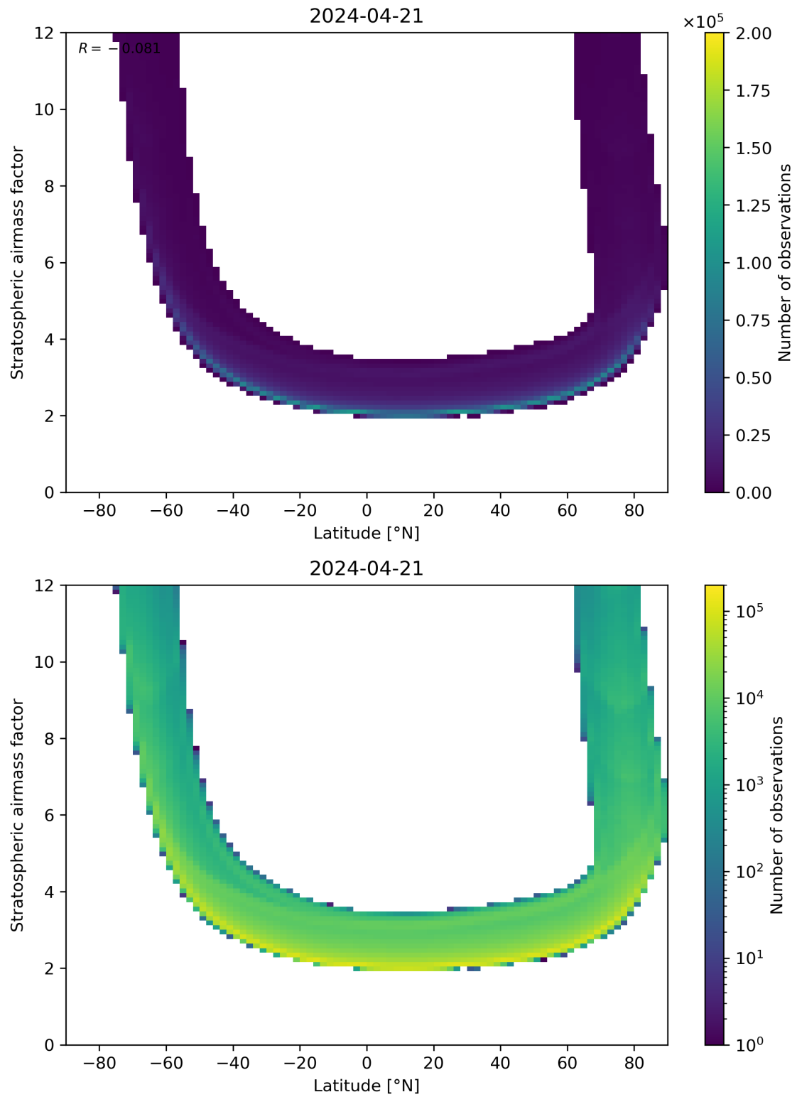
Figure 83: Scatter density plot of “Latitude” against “Stratospheric air mass factor” for 2024-04-21 to 2024-04-22.
