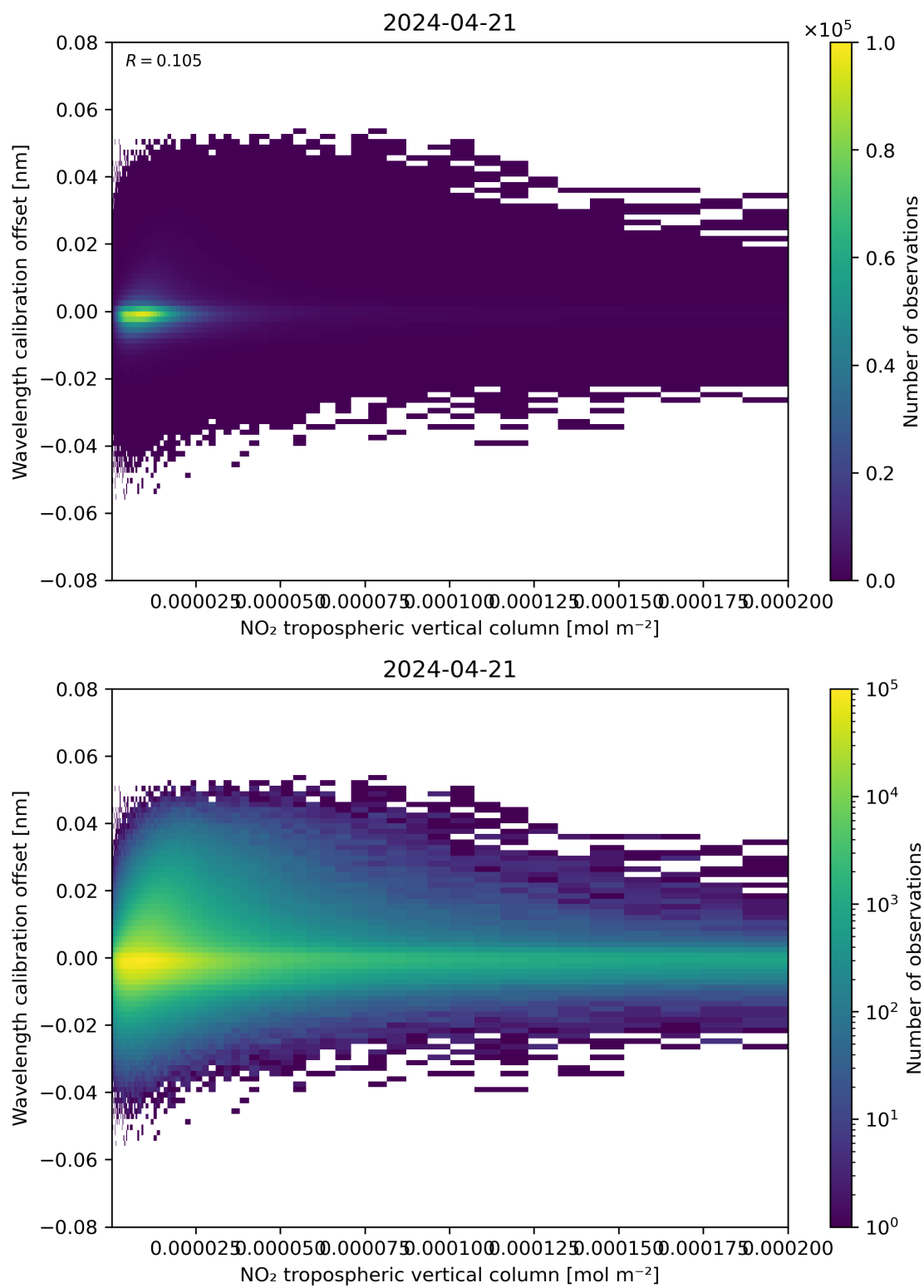
Figure 143: Scatter density plot of “NO 2 tropospheric vertical column” against “Wavelength calibration offset” for 2024-04-21 to 2024-04-22.
