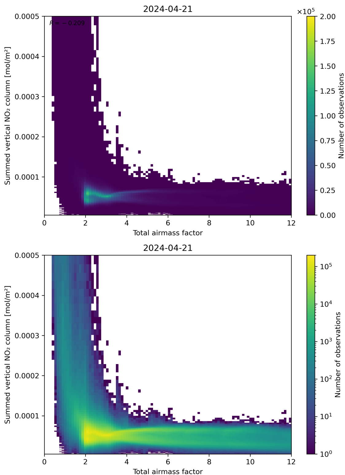
Figure 65: Scatter density plot of “Total airmass factor” against “Summed vertical NO 2 column” for 2024-04-21 to 2024-04-22.
