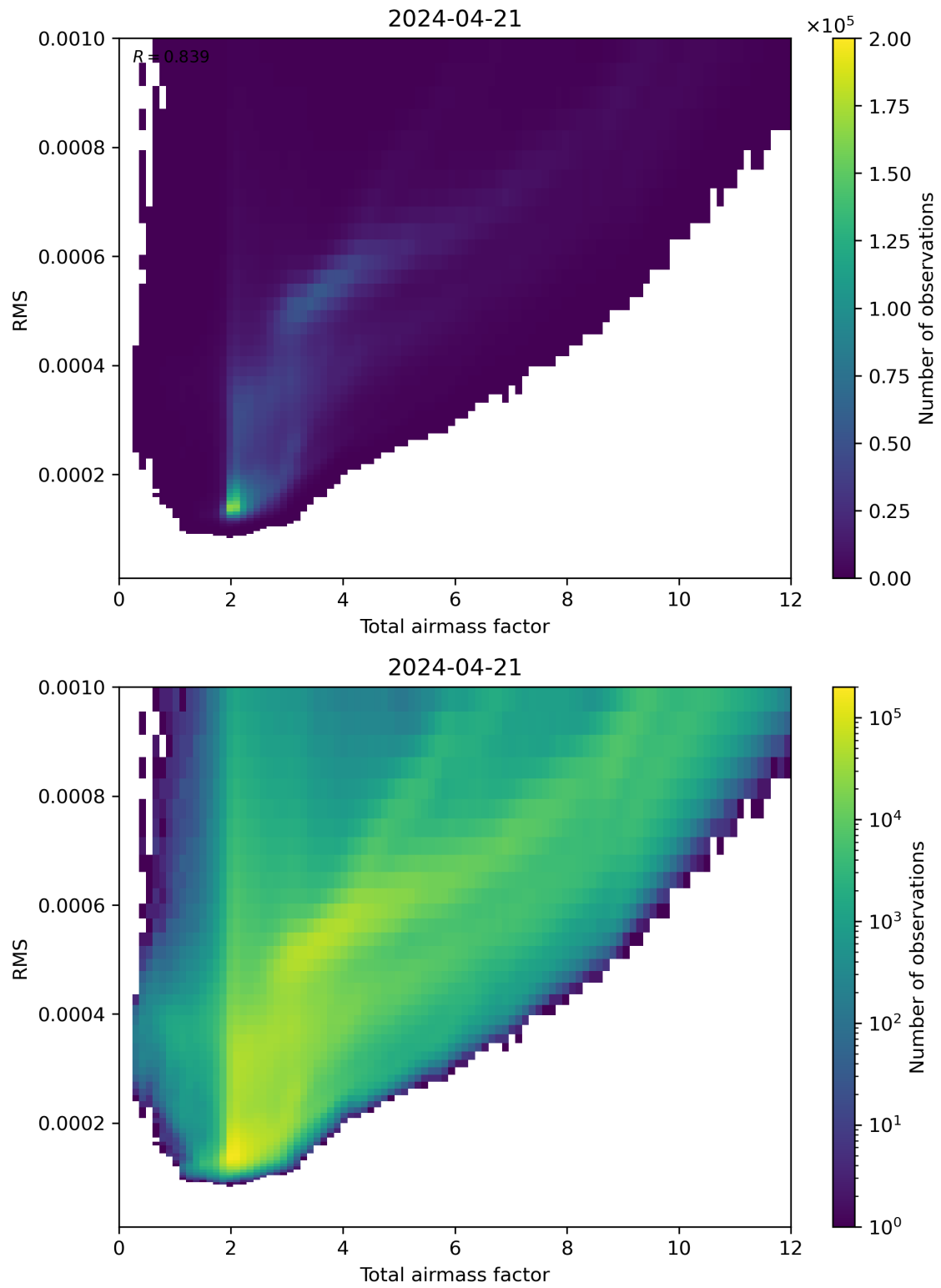
Figure 69: Scatter density plot of “Total airmass factor” against “RMS” for 2024-04-21 to 2024-04-22.
