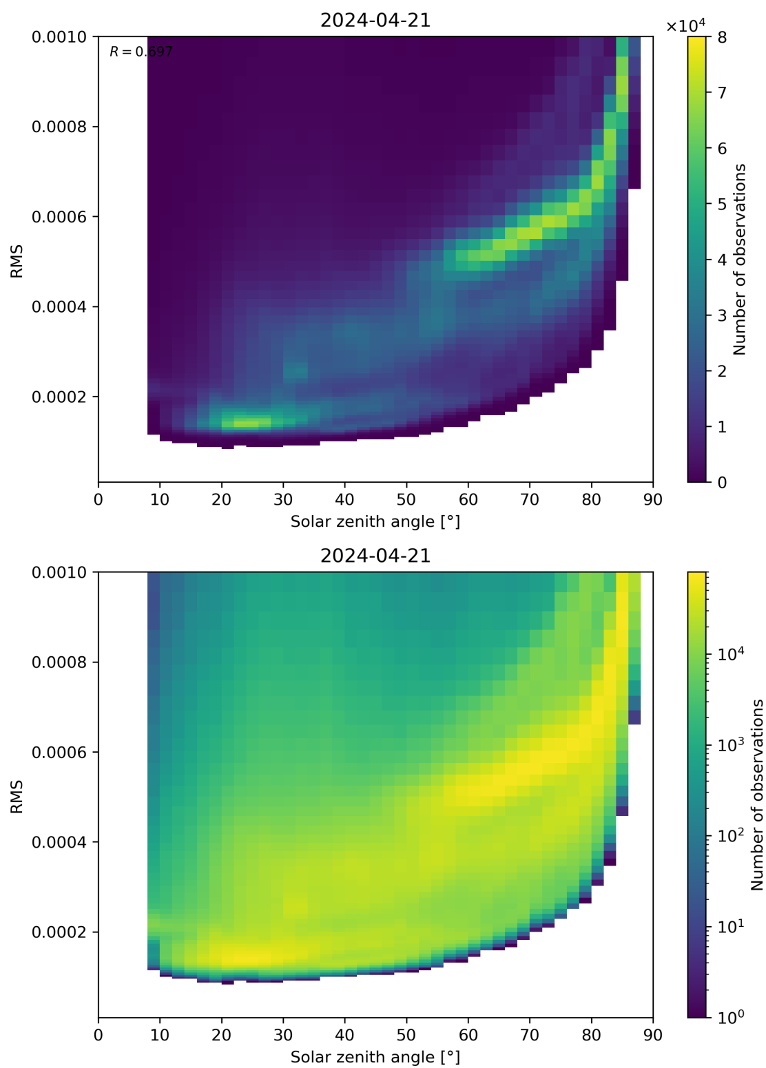
Figure 157: Scatter density plot of “Solar zenith angle” against “RMS” for 2024-04-21 to 2024-04-22.
