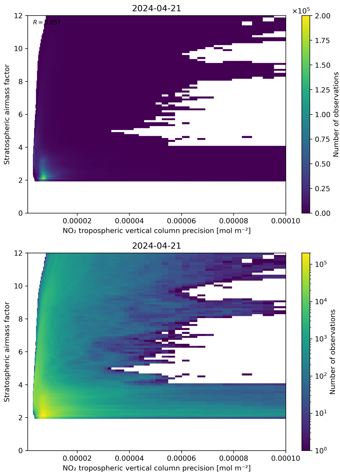
Figure 131: Scatter density plot of “NO 2 tropospheric vertical column precision” against “Stratospheric airmass factor” for 2024-04-21 to 2024-04-22.
