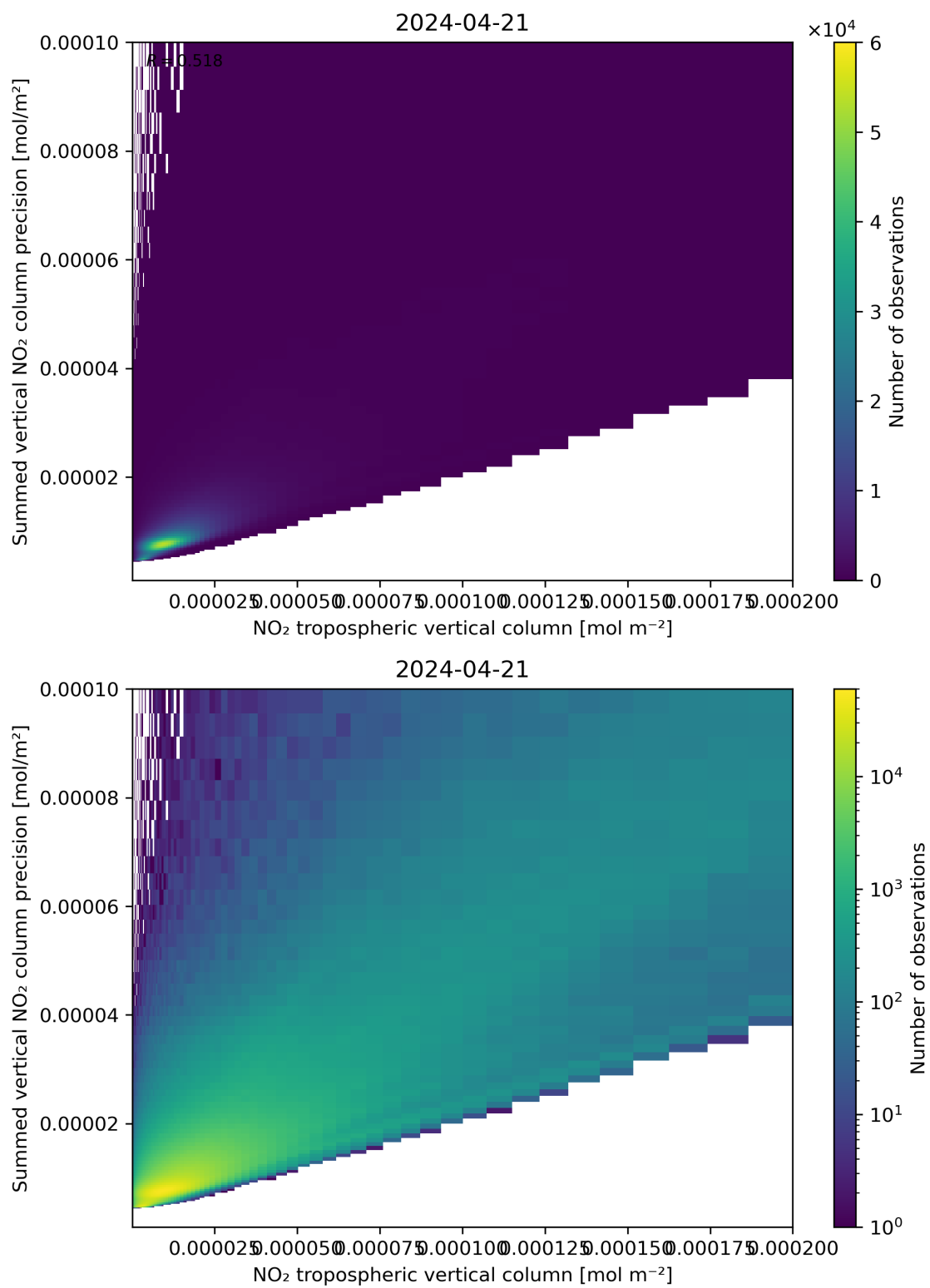
Figure 127: Scatter density plot of “NO 2 tropospheric vertical column” against “Summed vertical NO 2 column precision” for 2024-04-21 to 2024-04-22.
