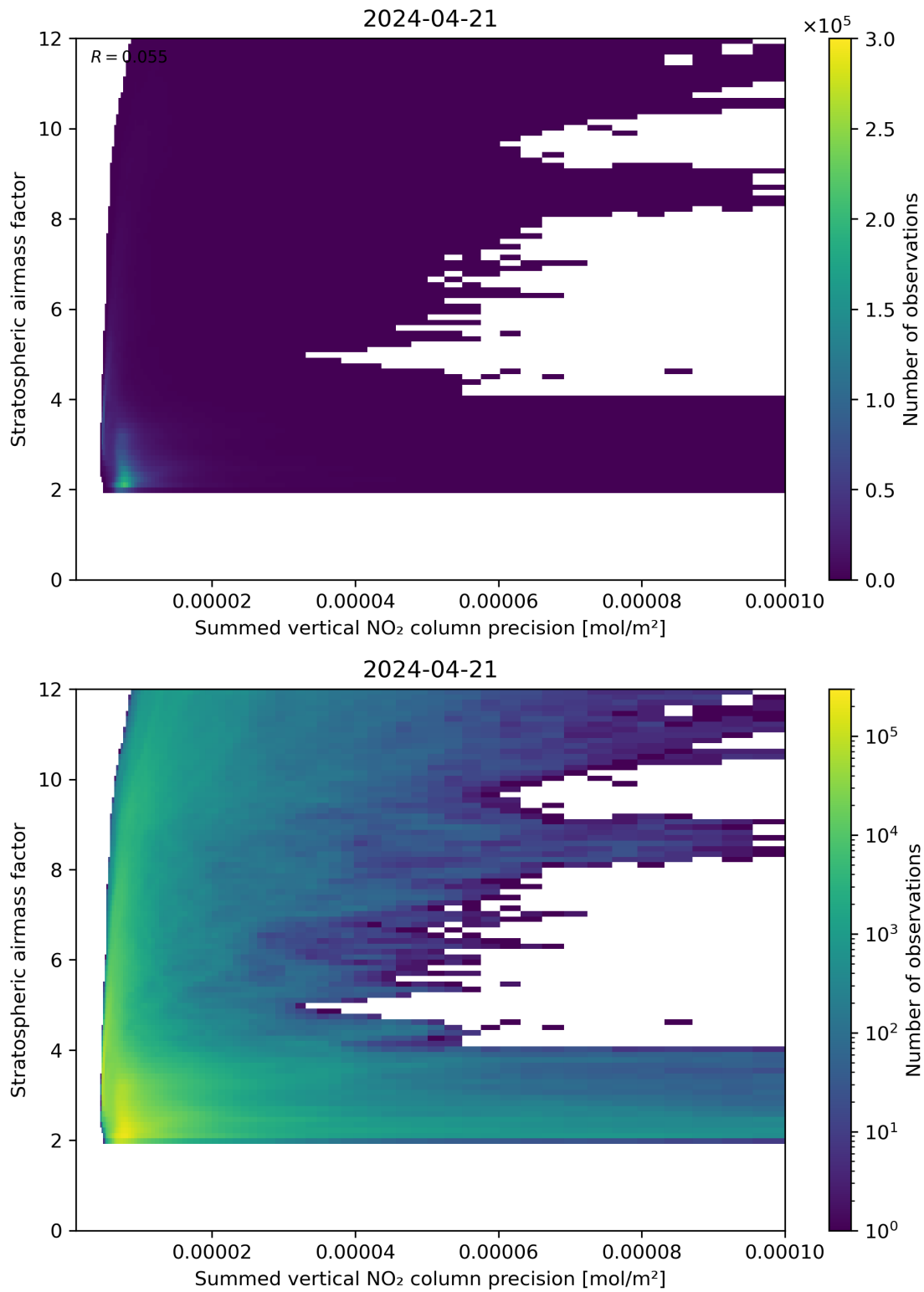
Figure 106: Scatter density plot of “Summed vertical NO 2 column precision” against “Stratospheric airmass factor” for 2024-04-21 to 2024-04-22.
