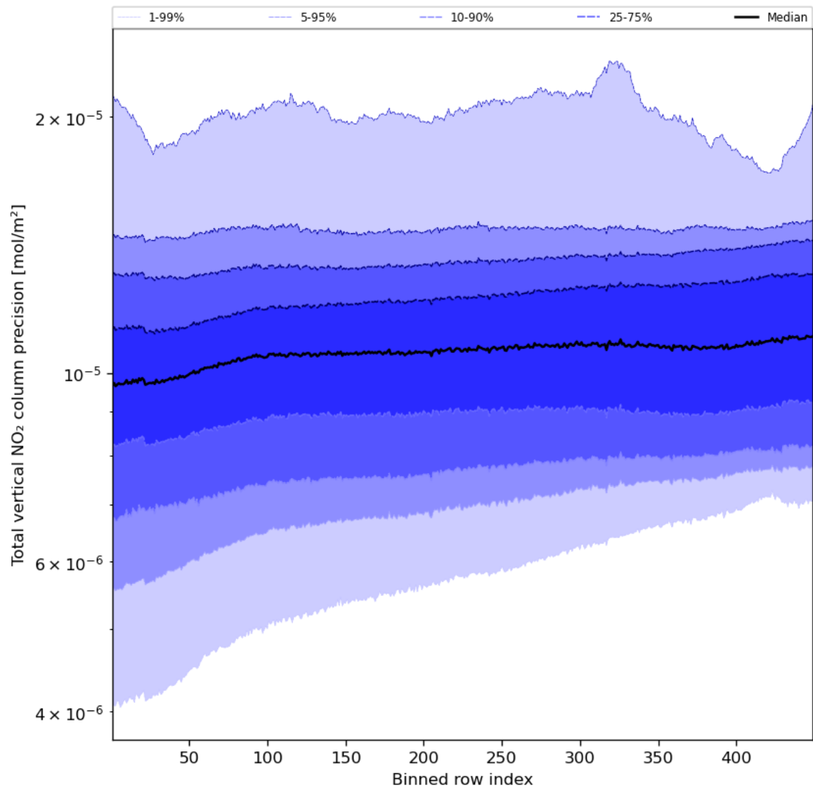
Figure 56: Along track statistics of “Total vertical NO 2 column precision” for 2024-04-21 to 2024-04-22
