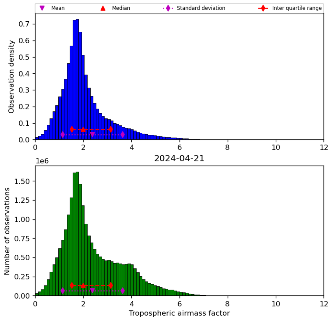
Figure 31: Histogram of “Tropospheric airmass factor” for 2024-04-21 to 2024-04-22
