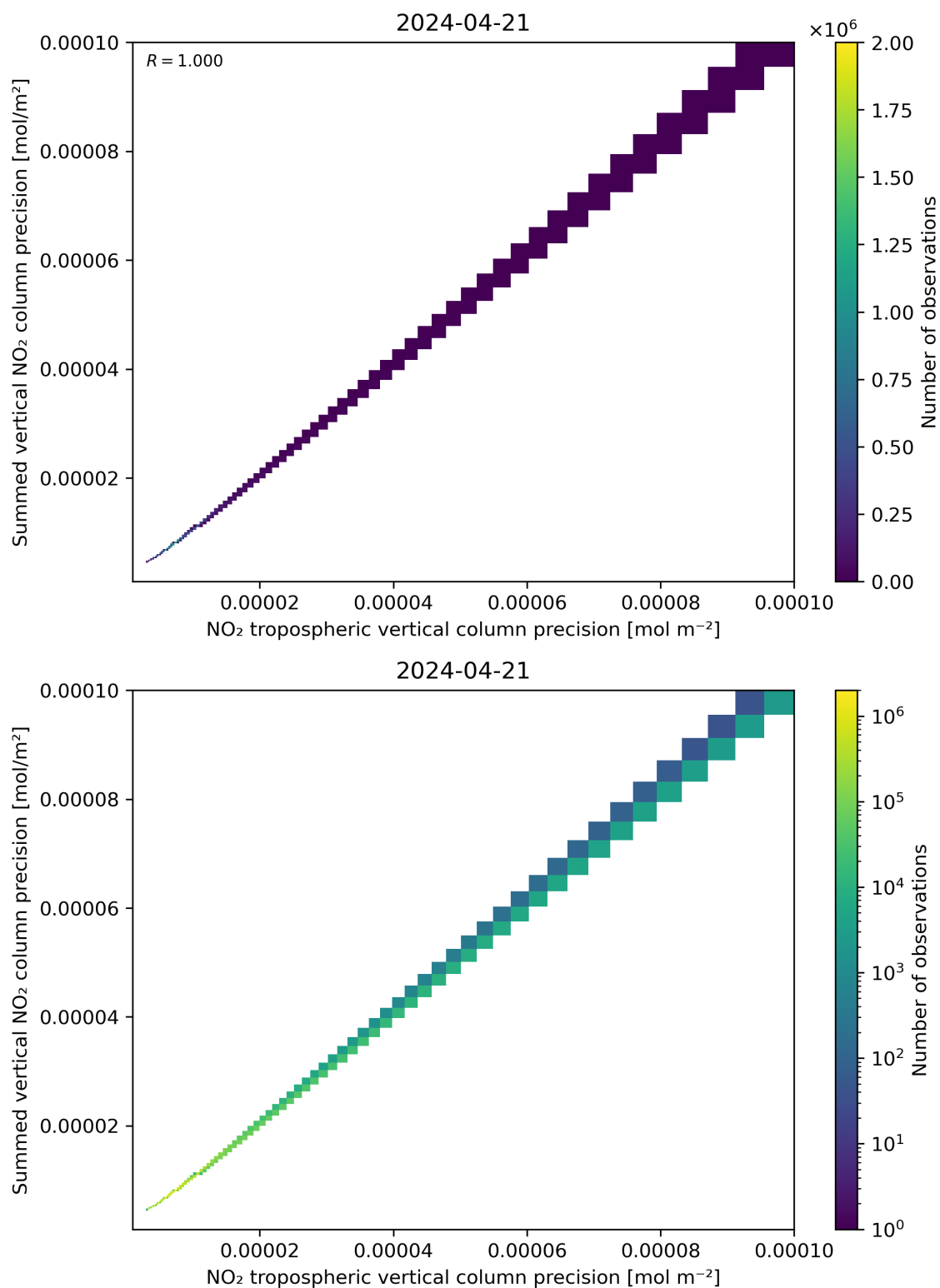
Figure 137: Scatter density plot of “NO 2 tropospheric vertical column precision” against “Summed vertical NO 2 column precision” for 2024-04-21 to 2024-04-22.
