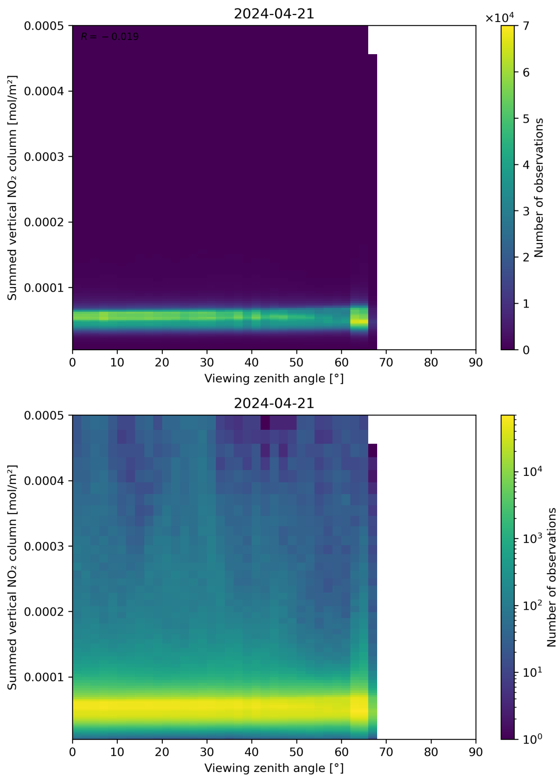
Figure 165: Scatter density plot of “Viewing zenith angle” against “Summed vertical NO 2 column” for 2024-04-21 to 2024-04-22.
