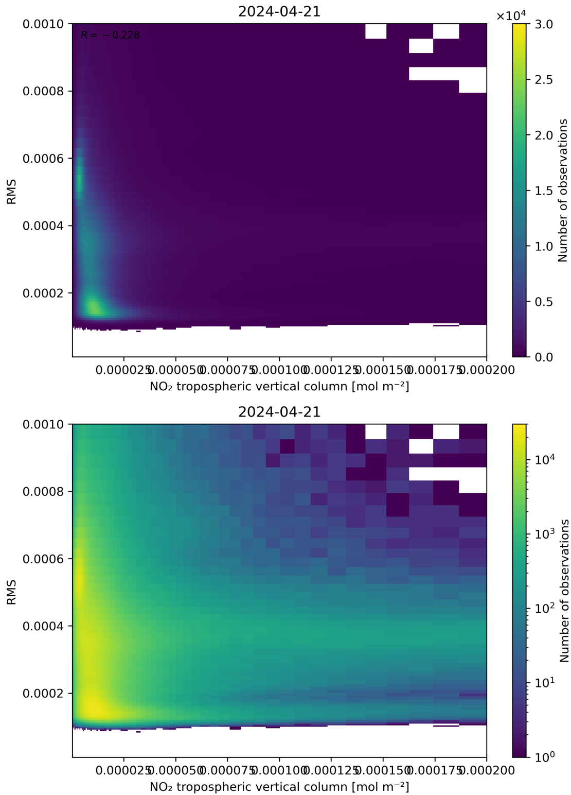
Figure 142: Scatter density plot of “NO 2 tropospheric vertical column” against “RMS” for 2024-04-21 to 2024-04-22.
