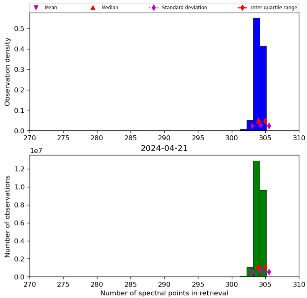
Figure 33: Histogram of “Number of spectral points in retrieval” for 2024-04-21 to 2024-04-22
