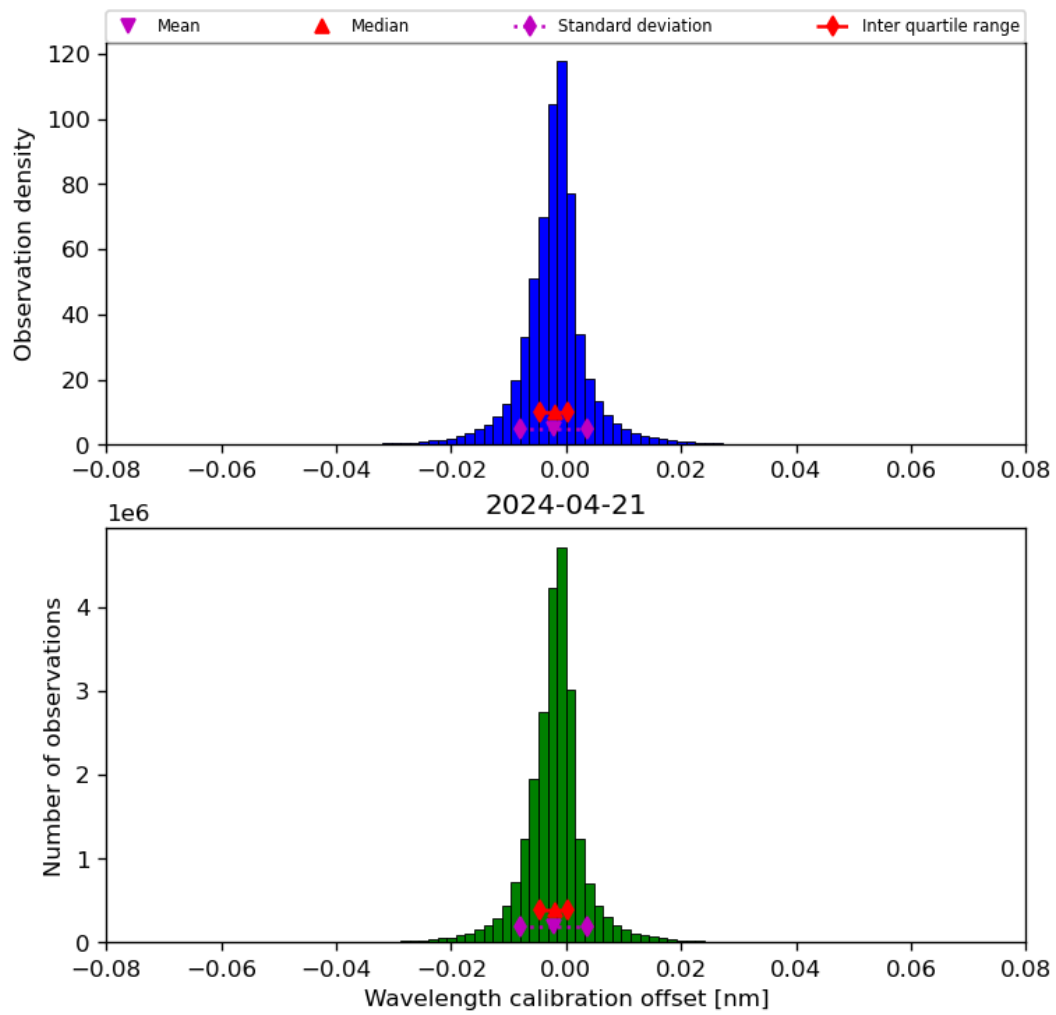
Figure 35: Histogram of “Wavelength calibration offset” for 2024-04-21 to 2024-04-22
