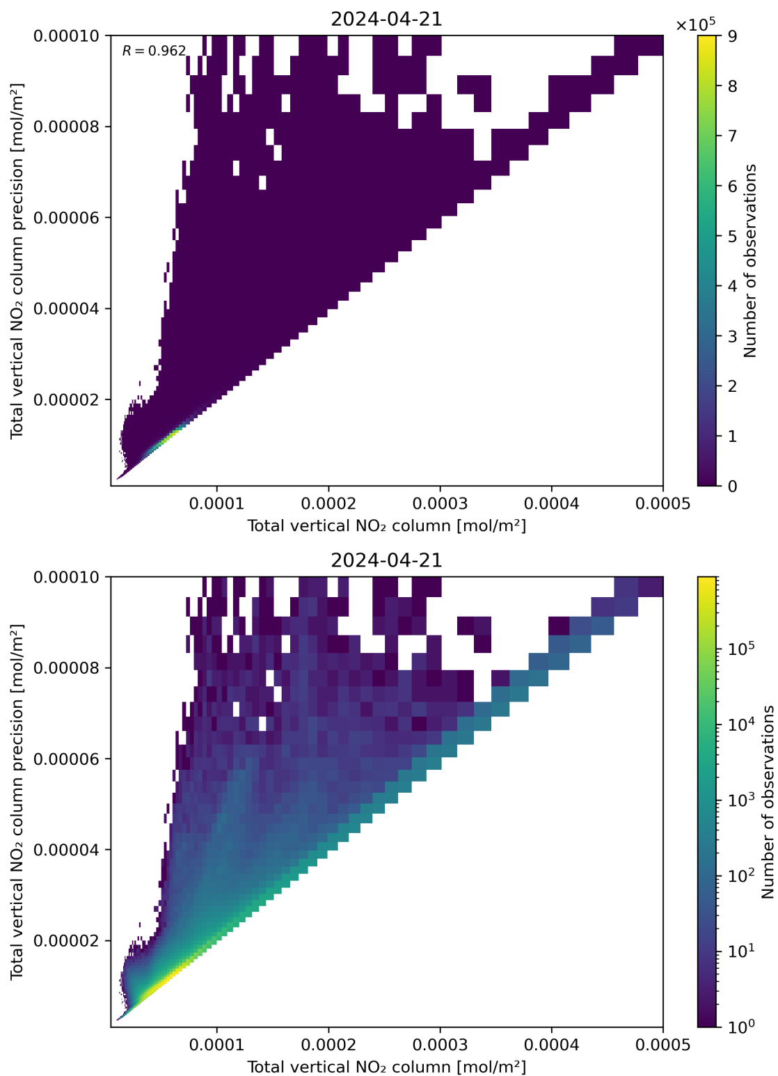
Figure 114: Scatter density plot of “Total vertical NO 2 column” against “Total vertical NO 2 column precision” for 2024-04-21 to 2024-04-22.
