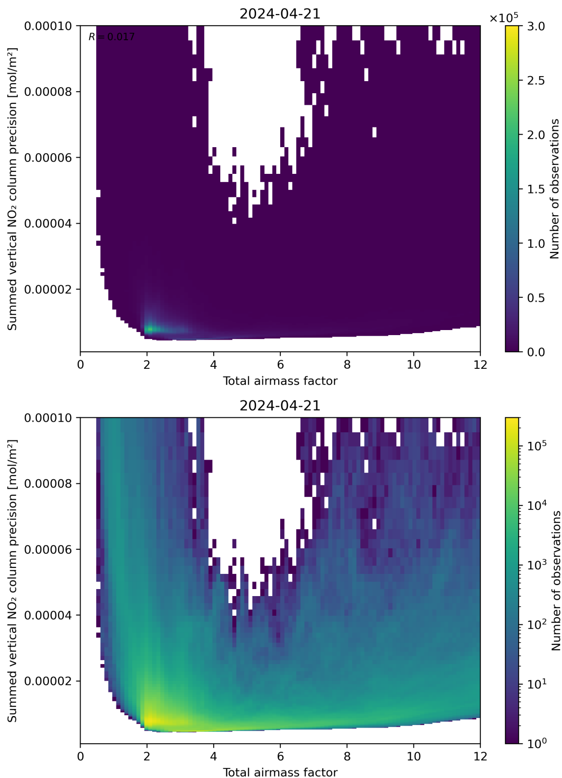
Figure 66: Scatter density plot of “Total airmass factor” against “Summed vertical NO 2 column precision” for 2024-04-21 to 2024-04-22.
