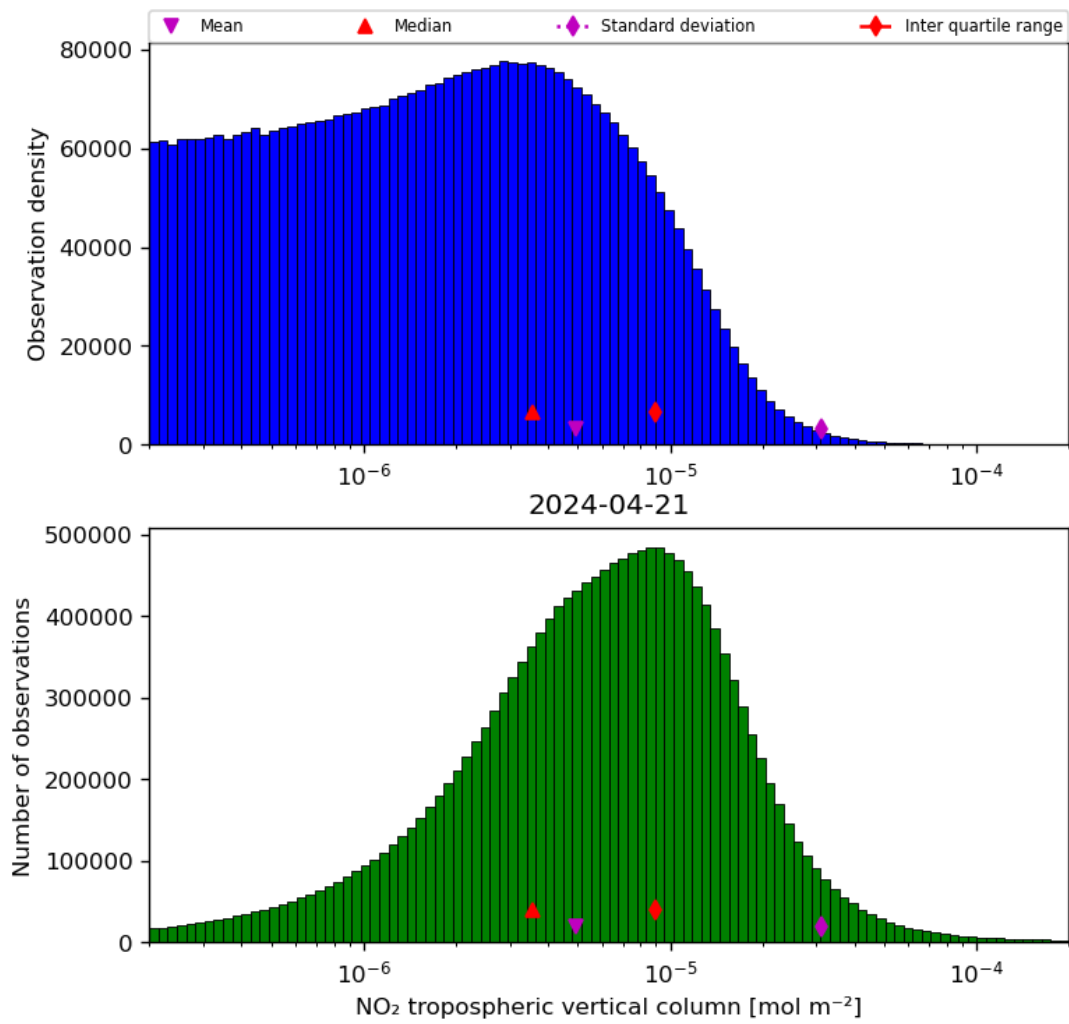
Figure 29: Histogram of “NO 2 tropospheric vertical column” for 2024-04-21 to 2024-04-22
