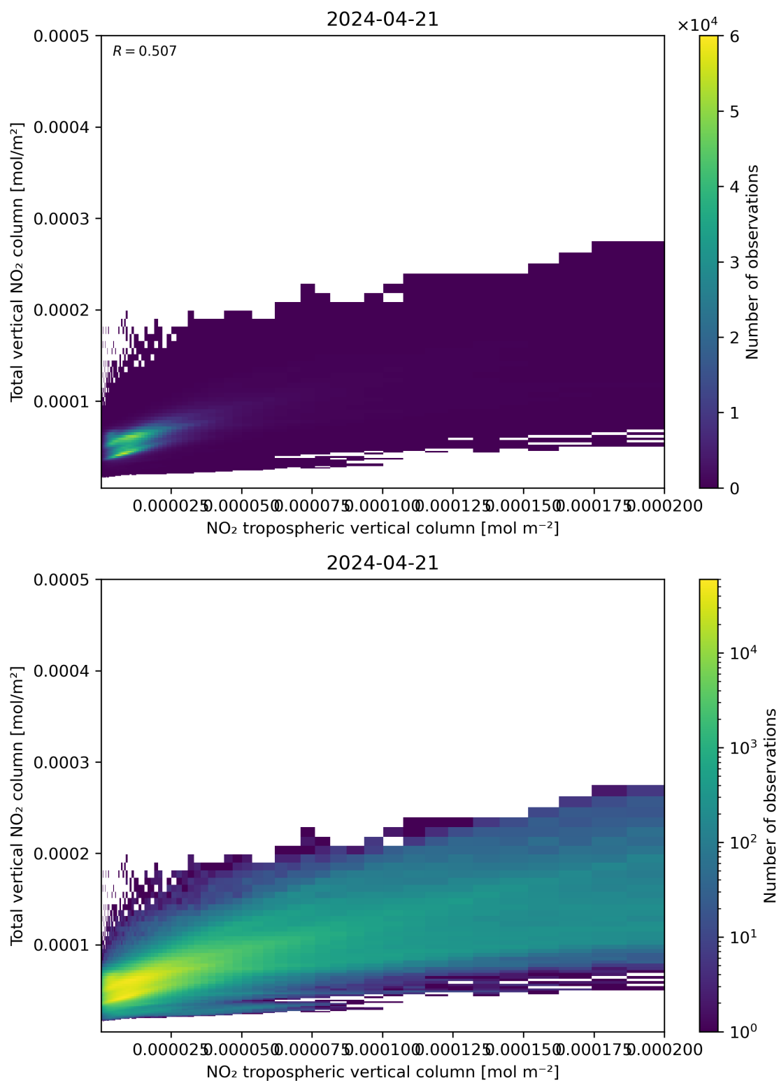
Figure 128: Scatter density plot of “NO 2 tropospheric vertical column” against “Total vertical NO 2 column” for 2024-04-21 to 2024-04-22.
