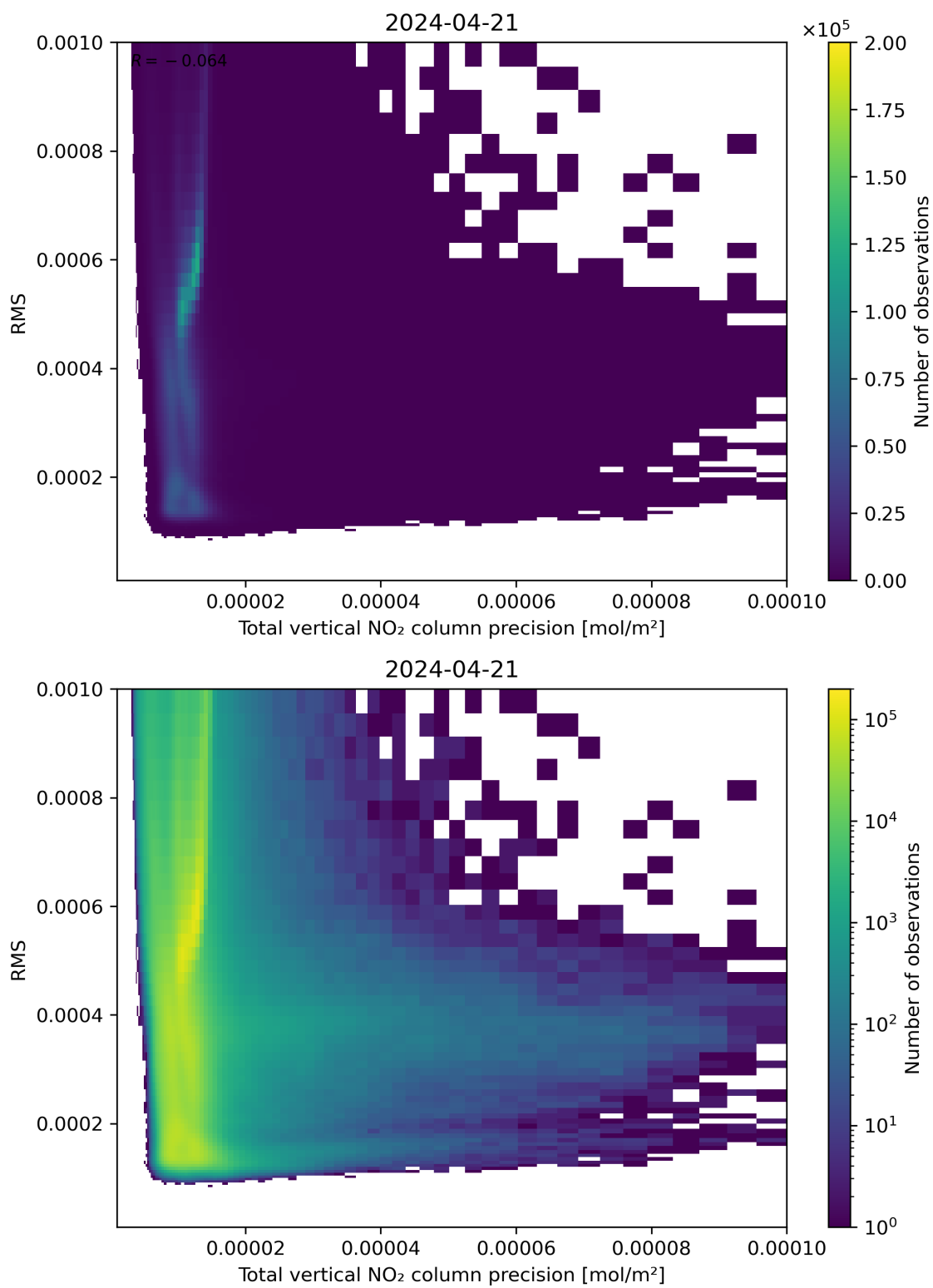
Figure 119: Scatter density plot of “Total vertical NO 2 column precision” against “RMS” for 2024-04-21 to 2024-04-22.
