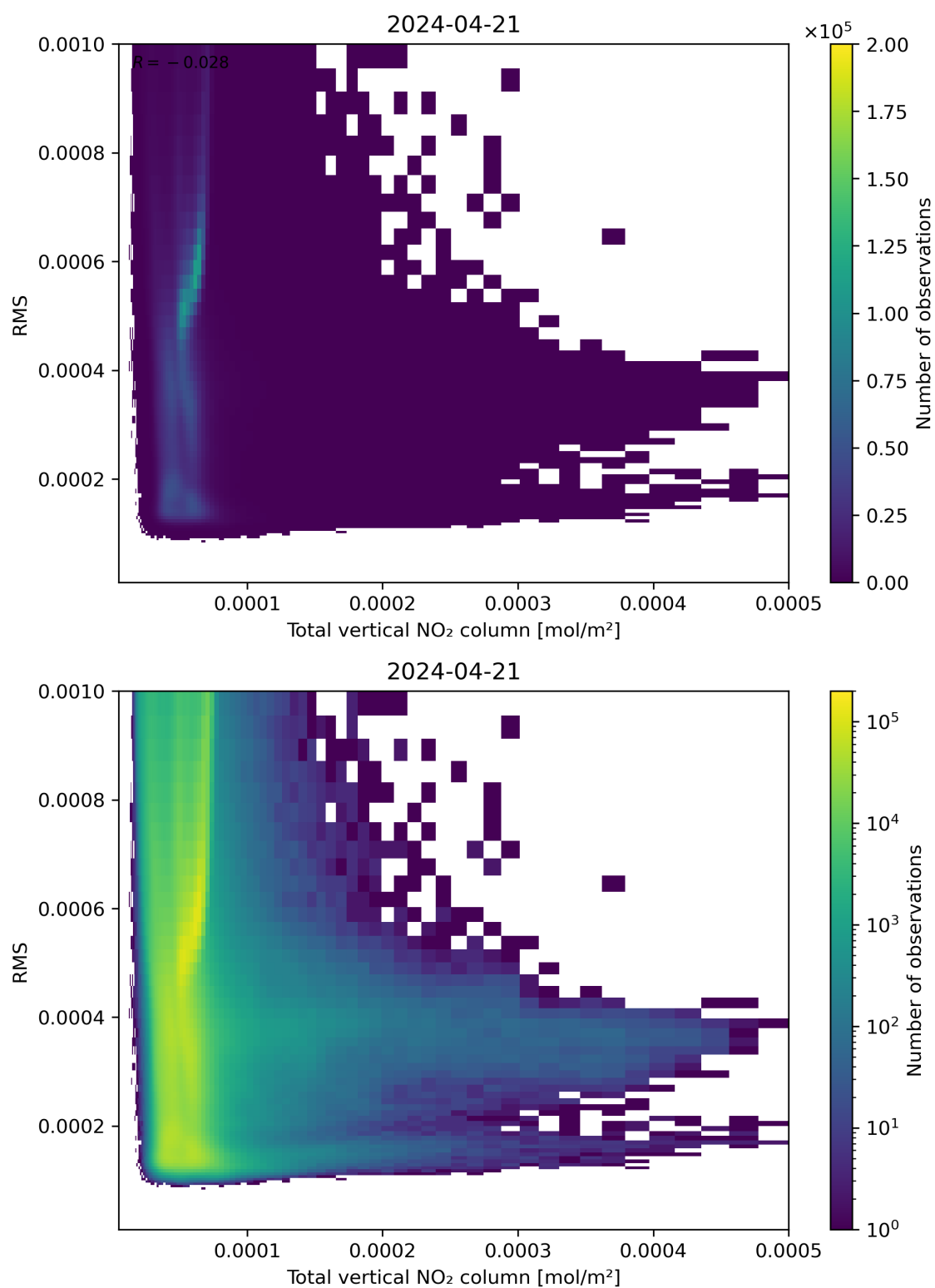
Figure 120: Scatter density plot of “Total vertical NO 2 column” against “RMS” for 2024-04-21 to 2024-04-22.
