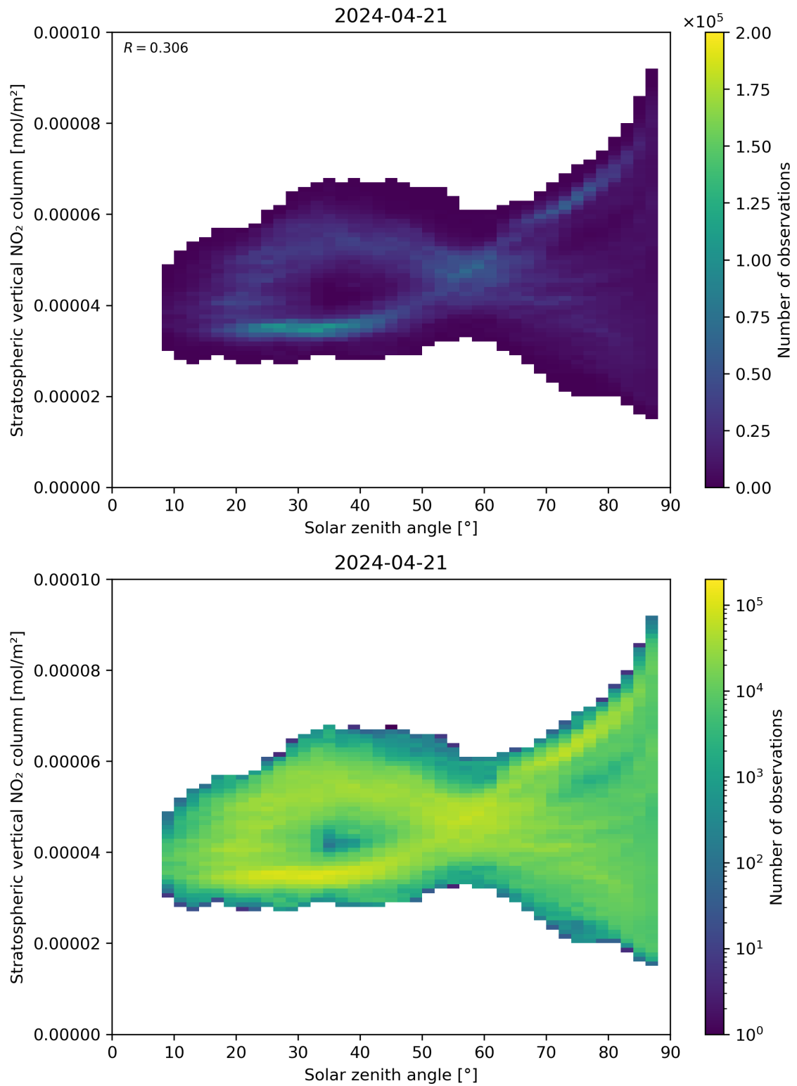
Figure 150: Scatter density plot of “Solar zenith angle” against “Stratospheric vertical NO 2 column” for 2024-04-21 to 2024-04-22.
