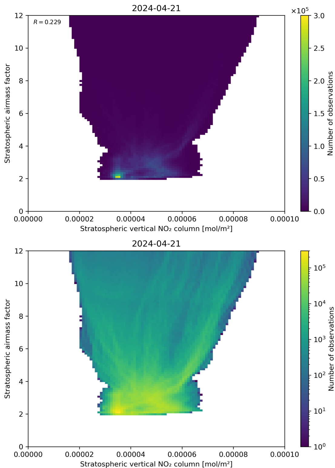
Figure 96: Scatter density plot of “Stratospheric vertical NO 2 column” against “Stratospheric airmass factor” for 2024-04-21 to 2024-04-22.
