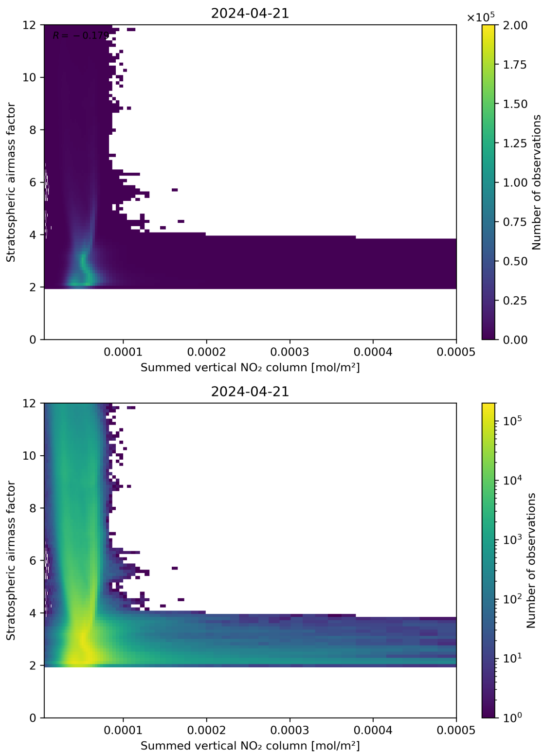
Figure 103: Scatter density plot of “Summed vertical NO 2 column” against “Stratospheric air mass factor” for 2024-04-21 to 2024-04-22.
