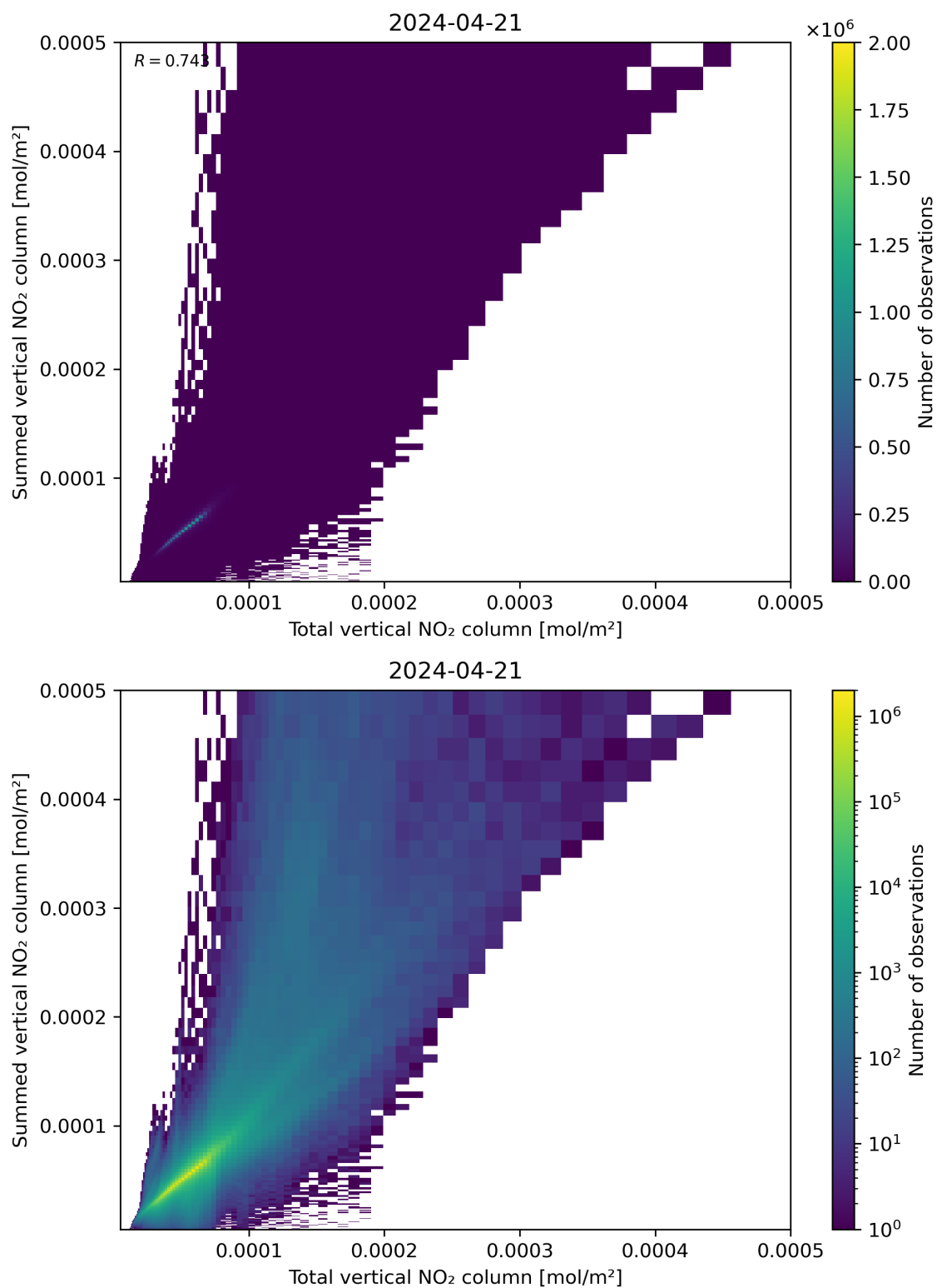
Figure 112: Scatter density plot of “Total vertical NO 2 column” against “Summed vertical NO 2 column” for 2024-04-21 to 2024-04-22.
