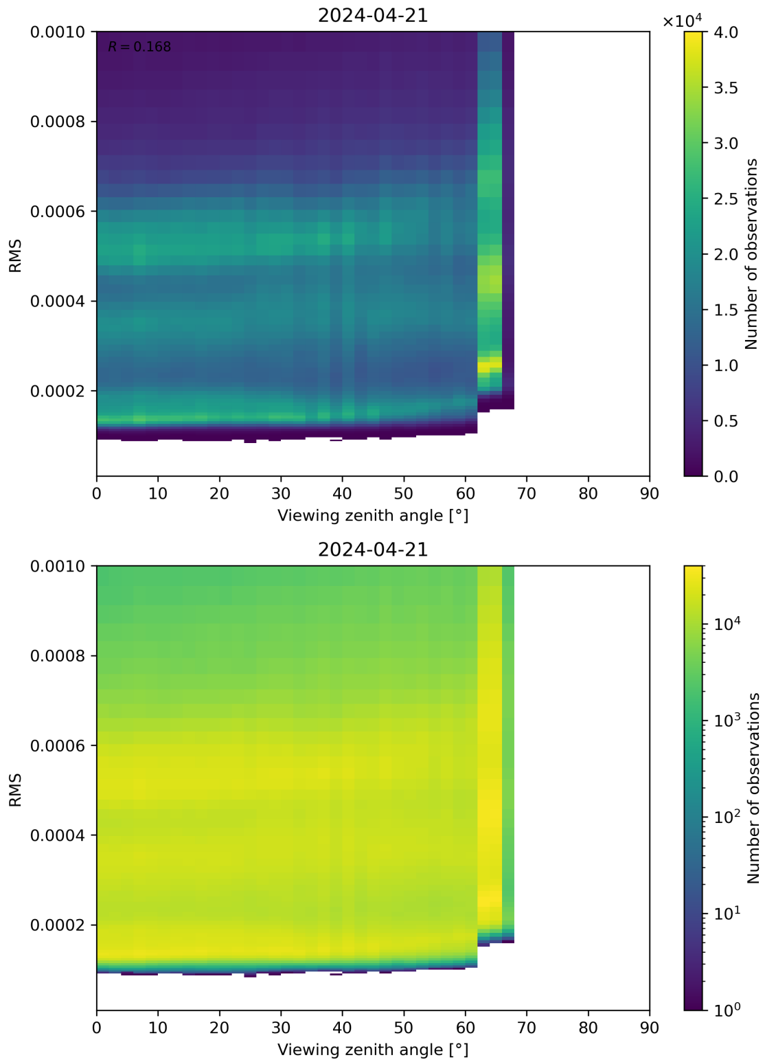
Figure 171: Scatter density plot of “Viewing zenith angle” against “RMS” for 2024-04-21 to 2024-04-22.
