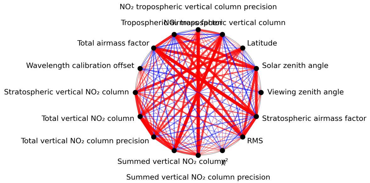
Figure 1: Map of correlation graph for 2024-04-21 to 2024-04-22.
