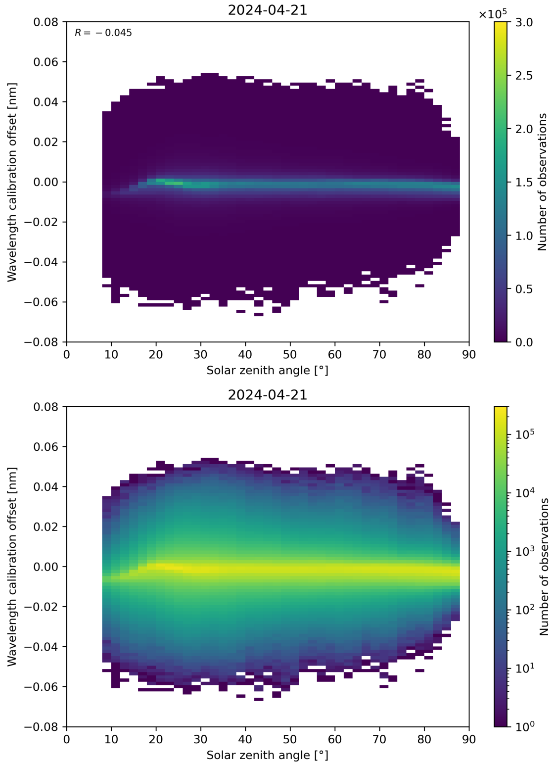
Figure 158: Scatter density plot of “Solar zenith angle” against “Wavelength calibration offset” for 2024-04-21 to 2024-04-22.
