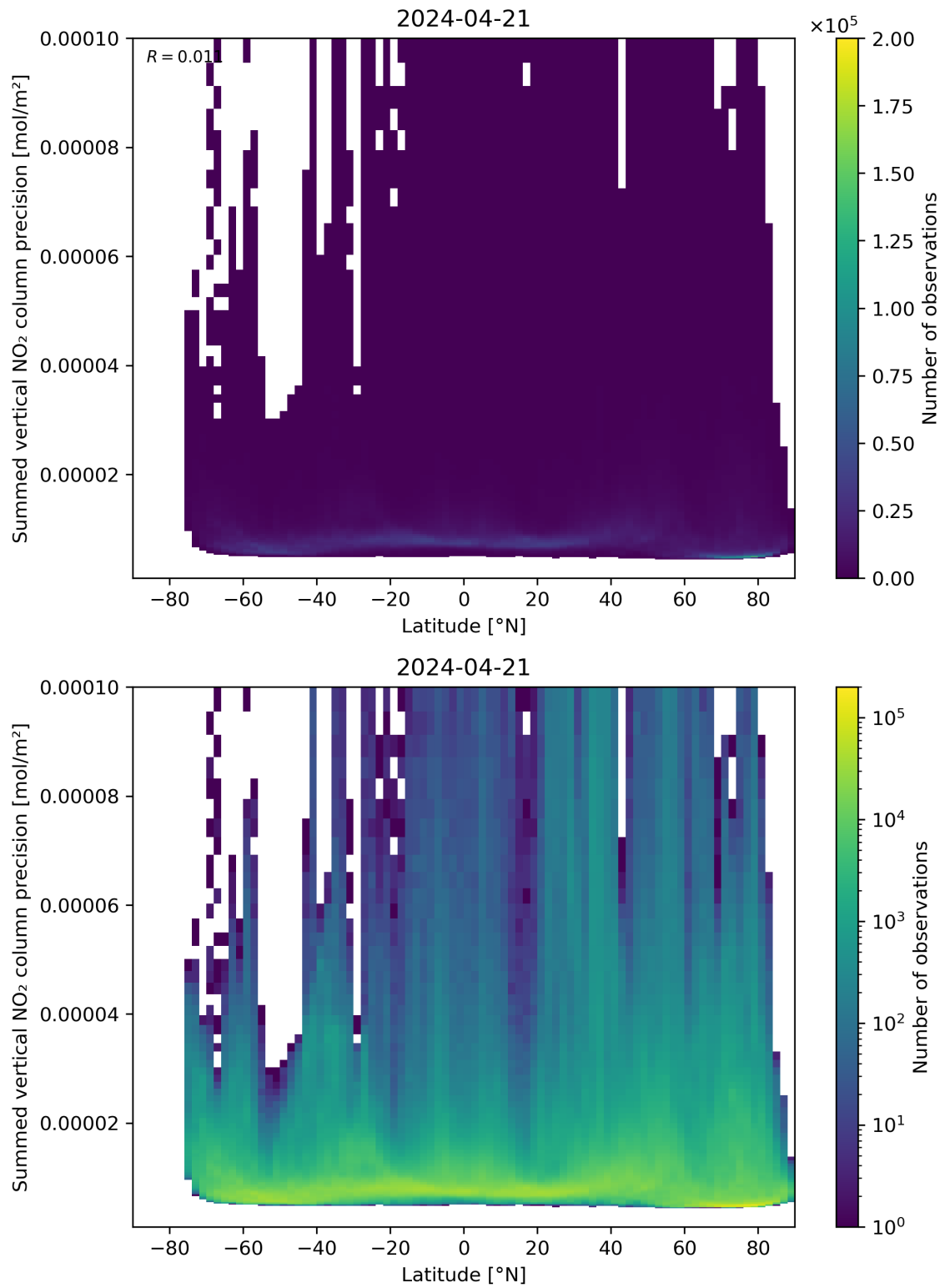
Figure 89: Scatter density plot of “Latitude” against “Summed vertical NO 2 column precision” for 2024-04-21 to 2024-04-22.
