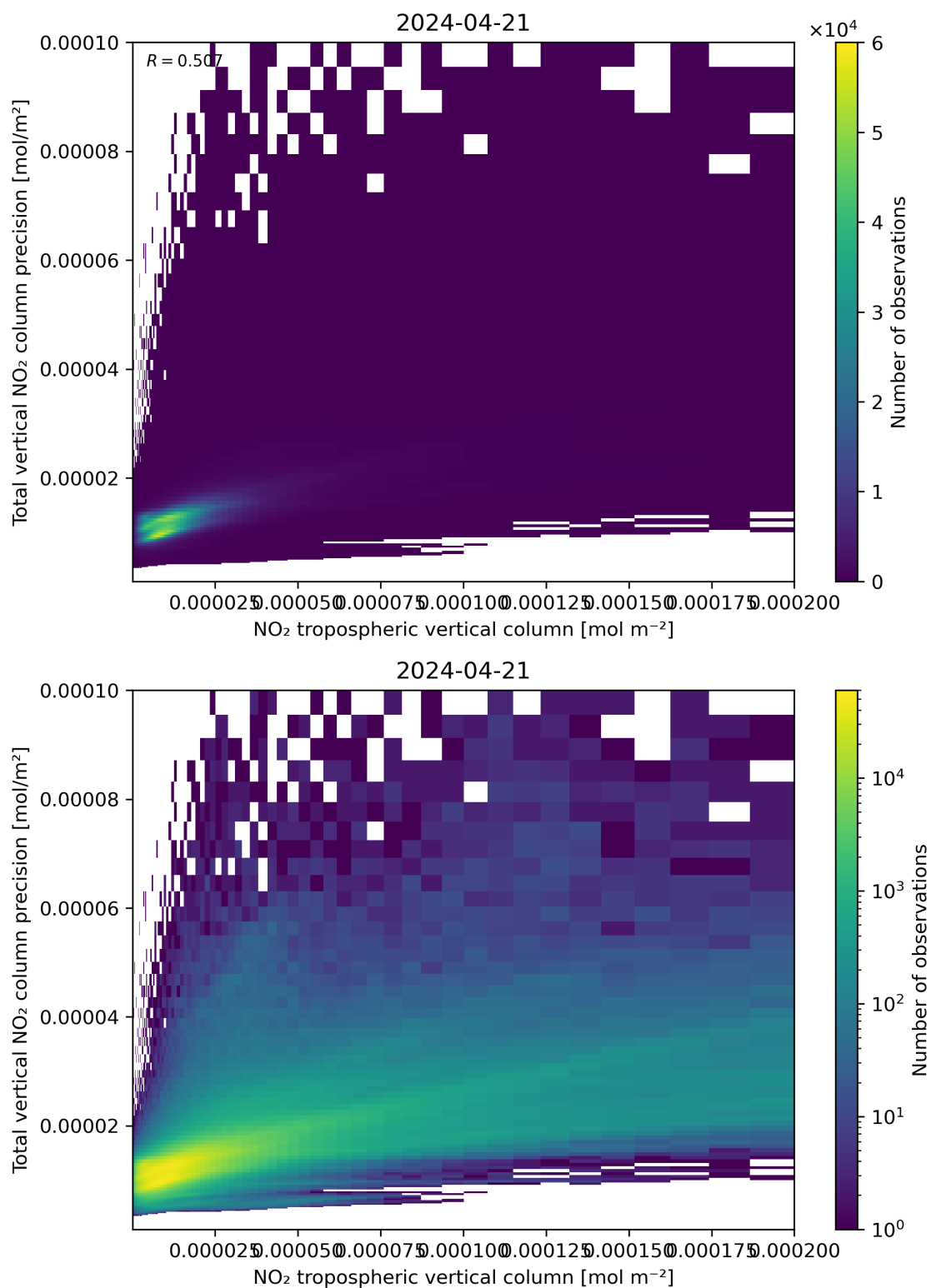
Figure 129: Scatter density plot of “NO 2 tropospheric vertical column” against “Total vertical NO 2 column precision” for 2024-04-21 to 2024-04-22.
