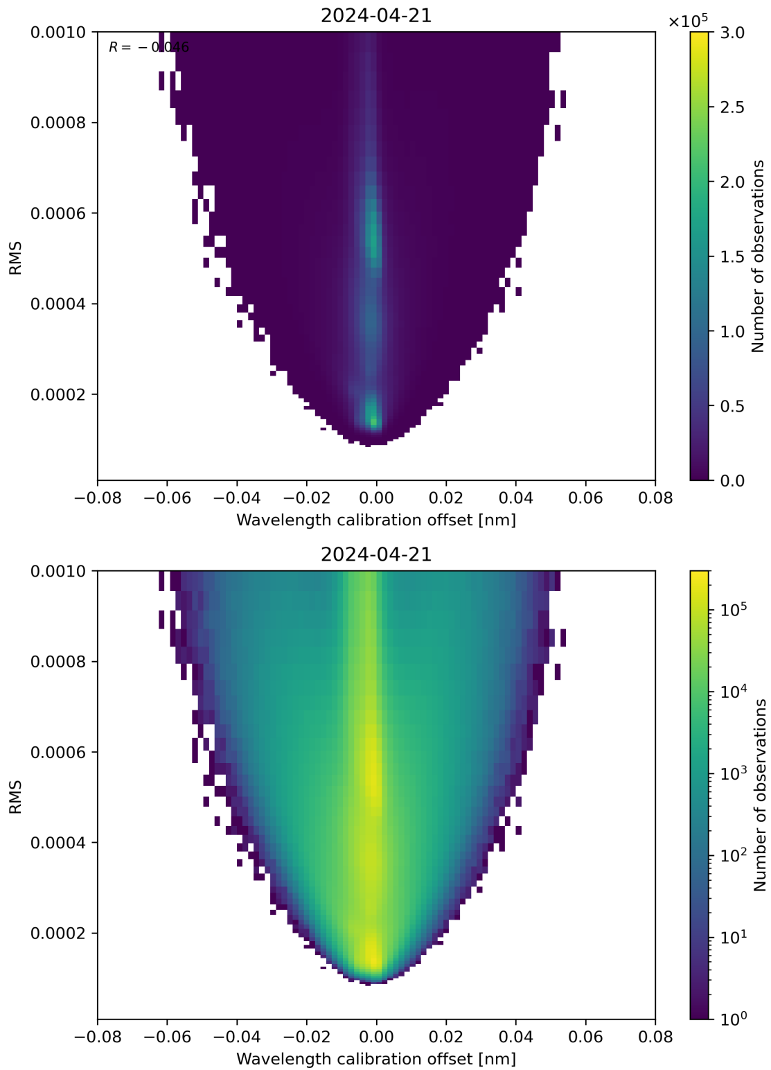
Figure 181: Scatter density plot of “Wavelength calibration offset” against “RMS” for 2024-04-21 to 2024-04-22.
