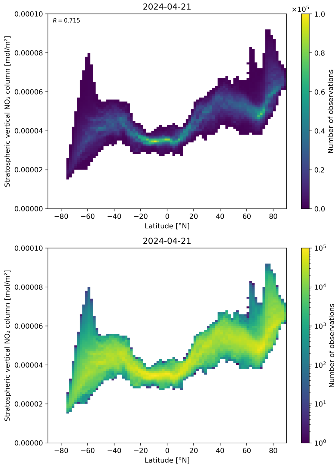
Figure 87: Scatter density plot of “Latitude” against “Stratospheric vertical \text{NO}_2 column” for 2024-04-21 to 2024-04-22.
