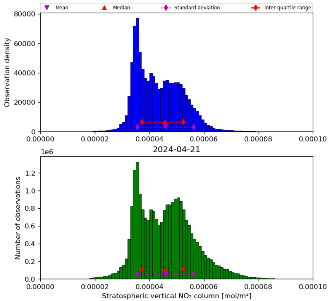
Figure 36: Histogram of “Stratospheric vertical NO 2 column” for 2024-04-21 to 2024-04-22
