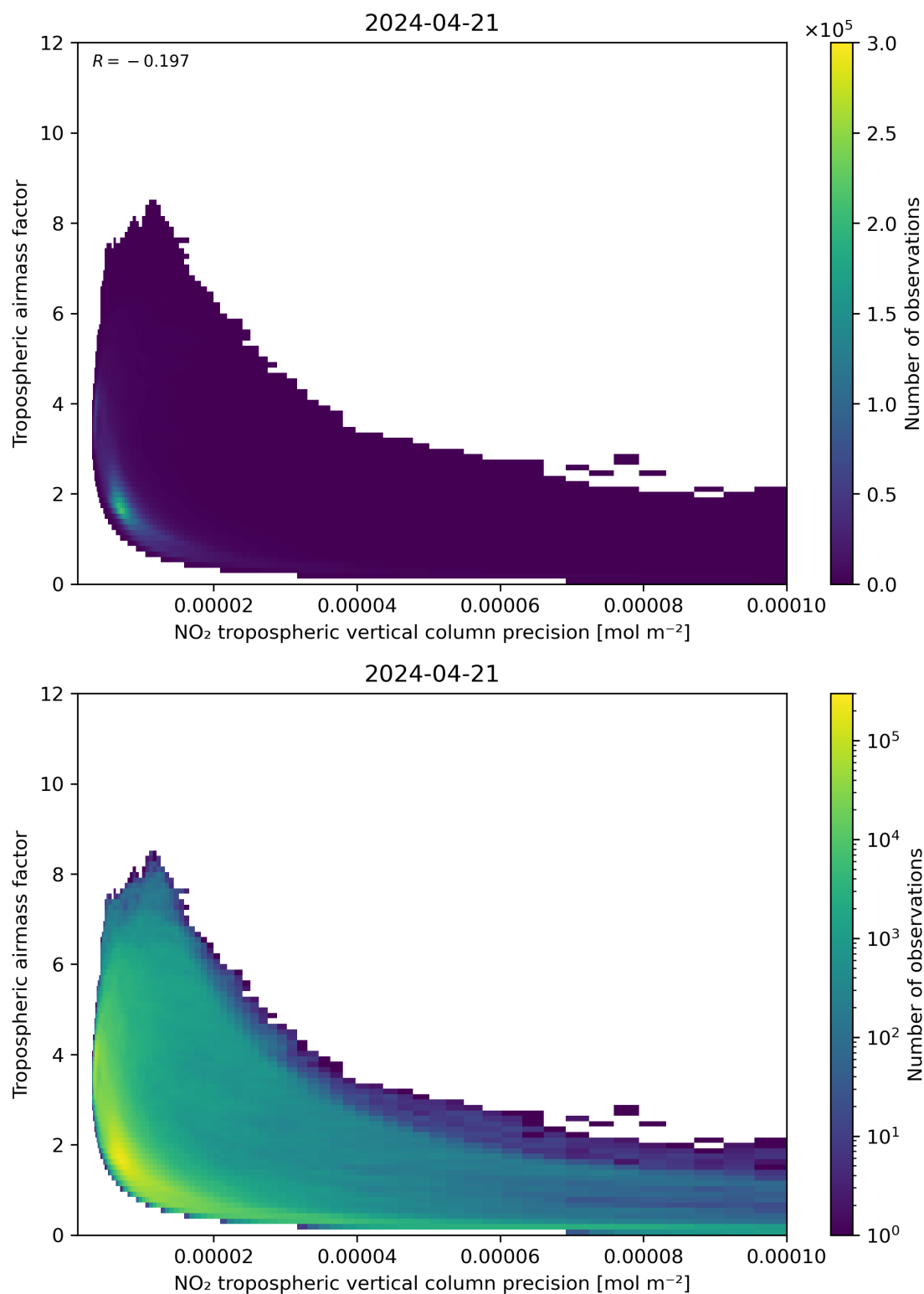
Figure 133: Scatter density plot of “NO 2 tropospheric vertical column precision” against “Tropospheric airmass factor” for 2024-04-21 to 2024-04-22.
