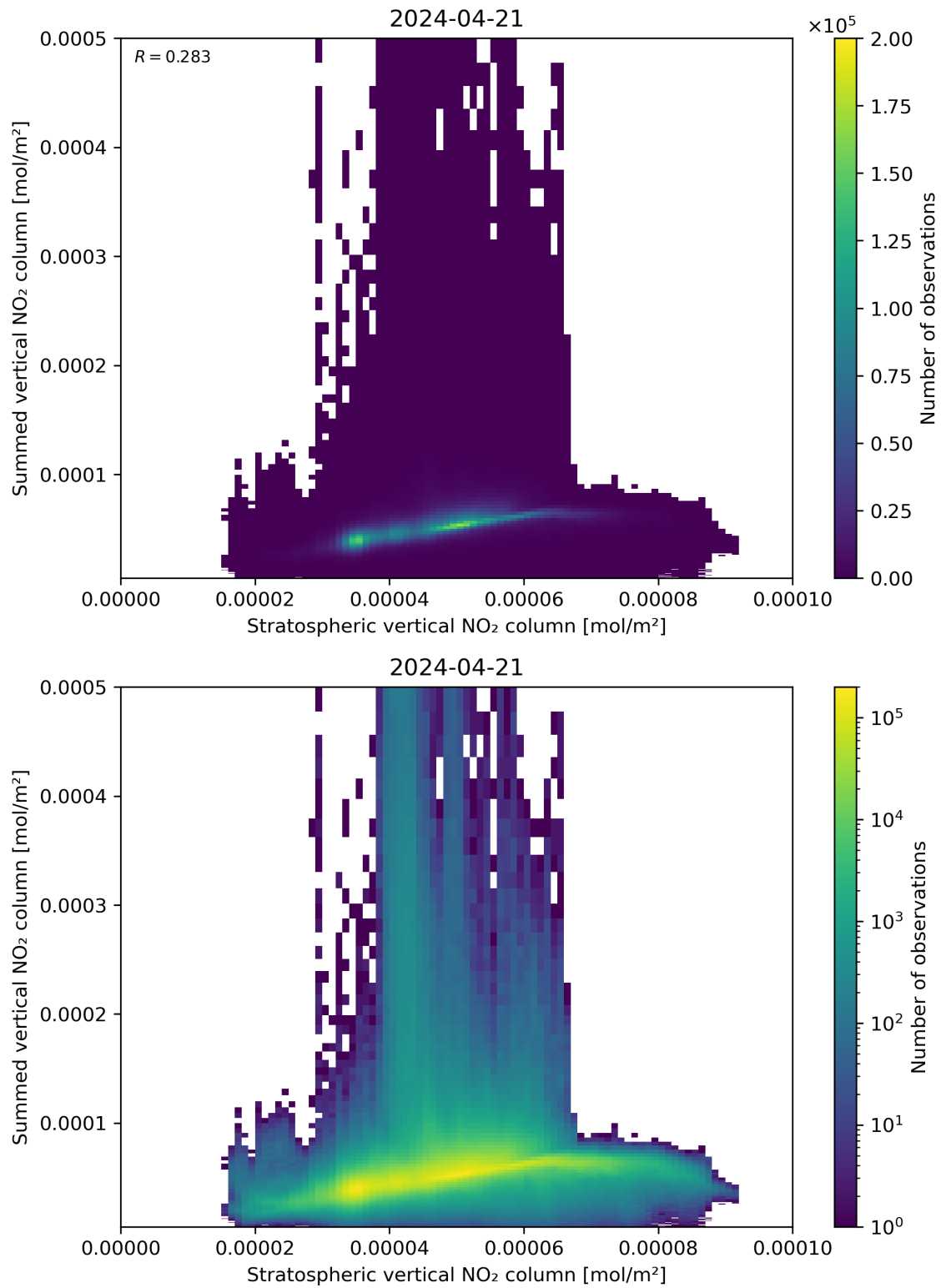
Figure 98: Scatter density plot of “Stratospheric vertical NO 2 column” against “Summed vertical NO 2 column” for 2024-04-21 to 2024-04-22.
