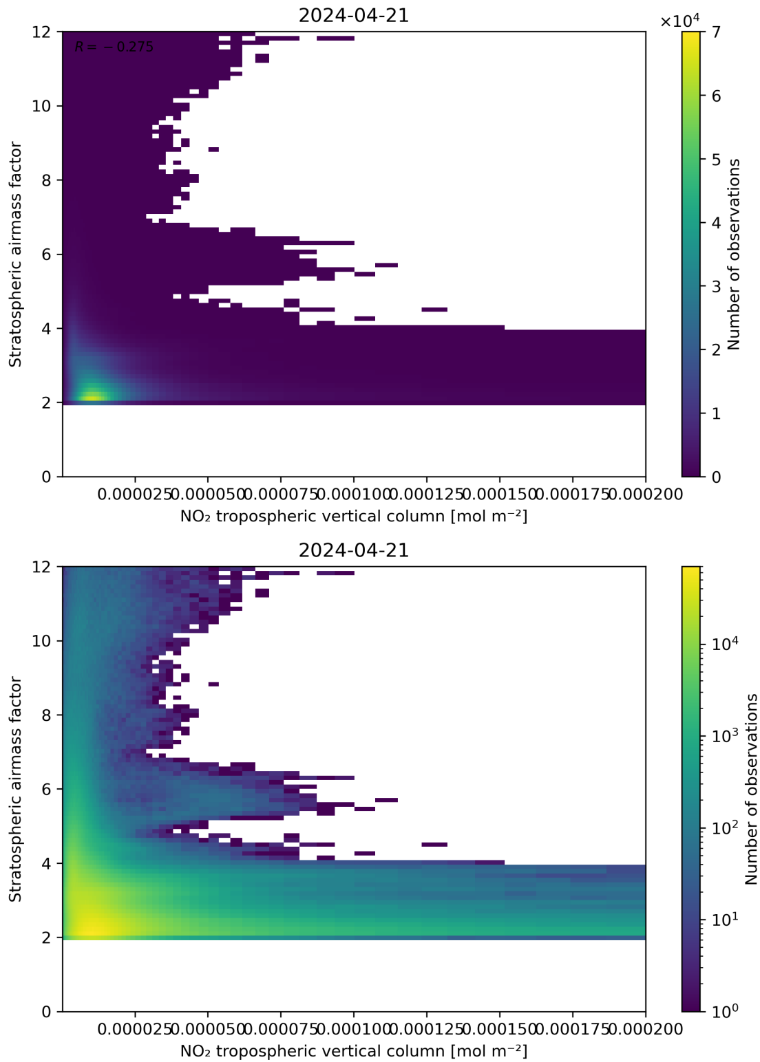
Figure 121: Scatter density plot of “NO 2 tropospheric vertical column” against “Stratospheric air mass factor” for 2024-04-21 to 2024-04-22.
