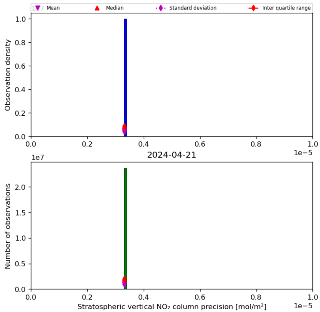
Figure 37: Histogram of “Stratospheric vertical NO 2 column precision” for 2024-04-21 to 2024-04-22
