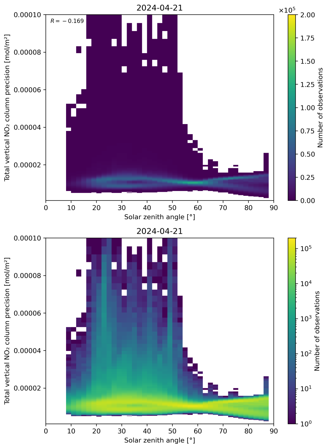
Figure 154: Scatter density plot of “Solar zenith angle” against “Total vertical NO 2 column precision” for 2024-04-21 to 2024-04-22.
