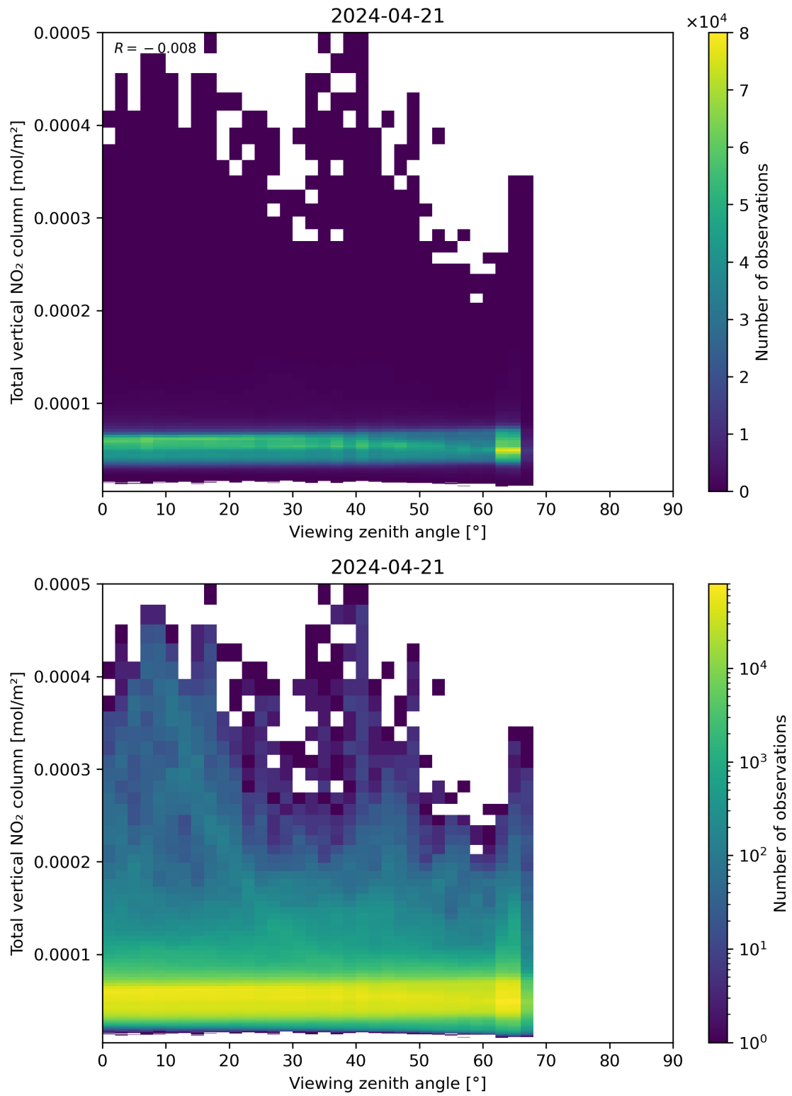
Figure 167: Scatter density plot of “Viewing zenith angle” against “Total vertical NO 2 column” for 2024-04-21 to 2024-04-22.
