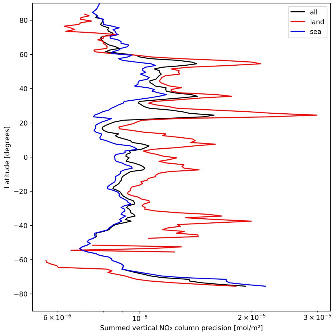
Figure 24: Zonal average of “Summed vertical NO 2 column precision” for 2024-04-21 to 2024-04-22.
