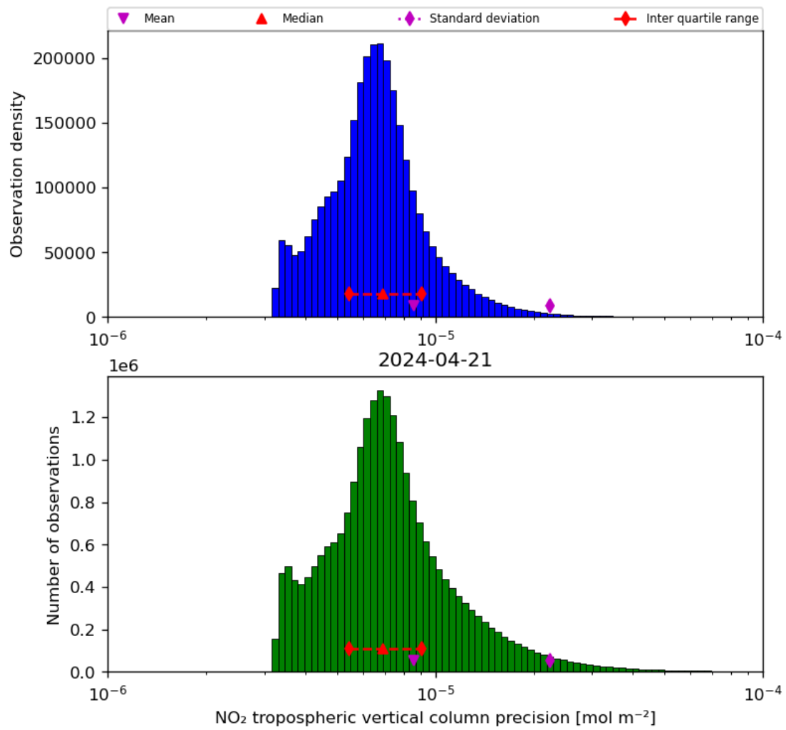
Figure 30: Histogram of “NO 2 tropospheric vertical column precision” for 2024-04-21 to 2024-04-22
