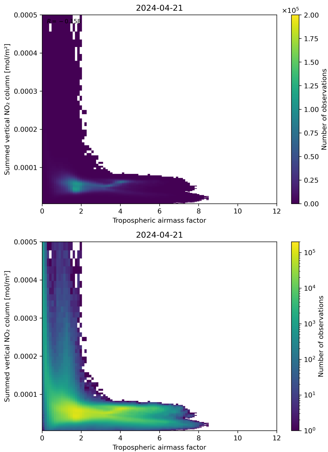
Figure 75: Scatter density plot of “Tropospheric airmass factor” against “Summed vertical NO 2 column” for 2024-04-21 to 2024-04-22.
