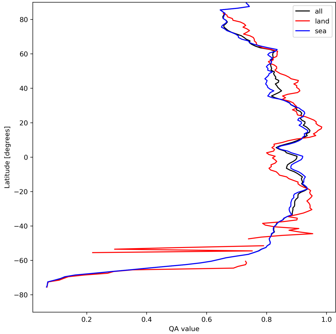
Figure 11: Zonal average of “QA value” for 2024-04-21 to 2024-04-22.
