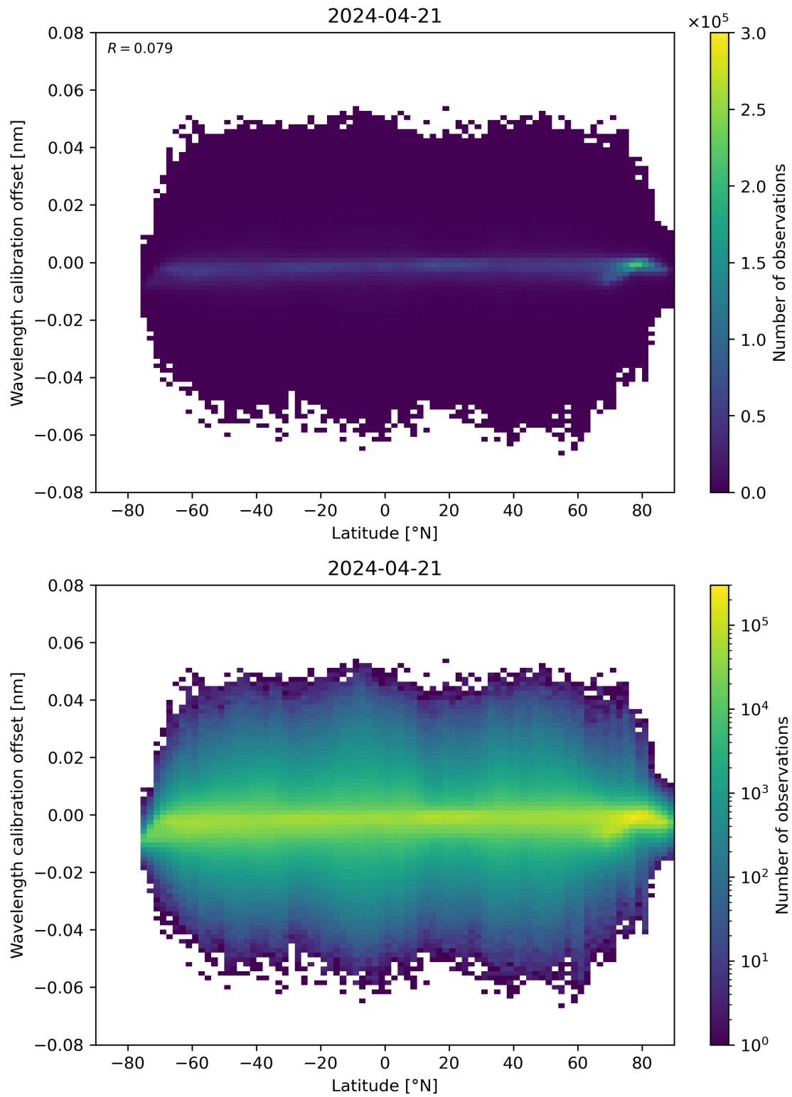
Figure 95: Scatter density plot of “Latitude” against “Wavelength calibration offset” for 2024-04-21 to 2024-04-22.
