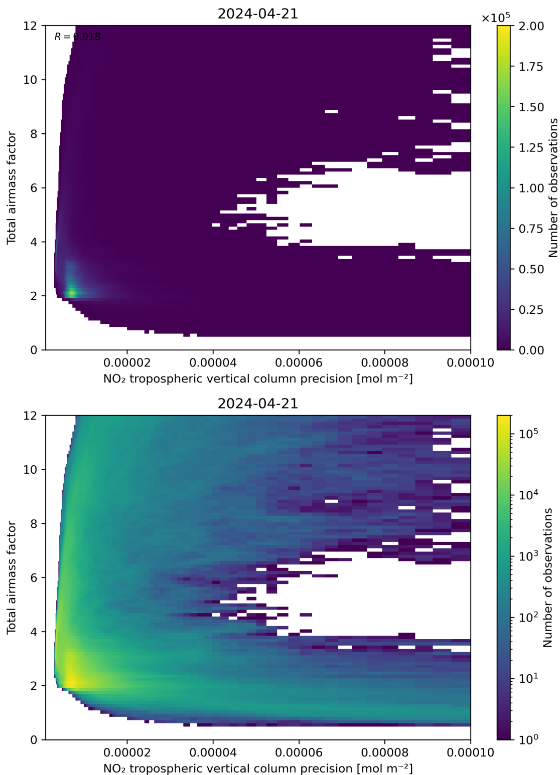
Figure 132: Scatter density plot of “NO 2 tropospheric vertical column precision” against “Total air mass factor” for 2024-04-21 to 2024-04-22.
