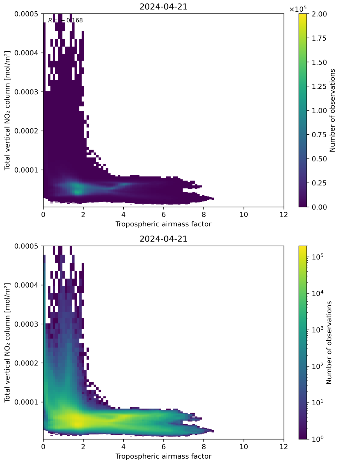
Figure 77: Scatter density plot of “Tropospheric airmass factor” against “Total vertical NO 2 column” for 2024-04-21 to 2024-04-22.
