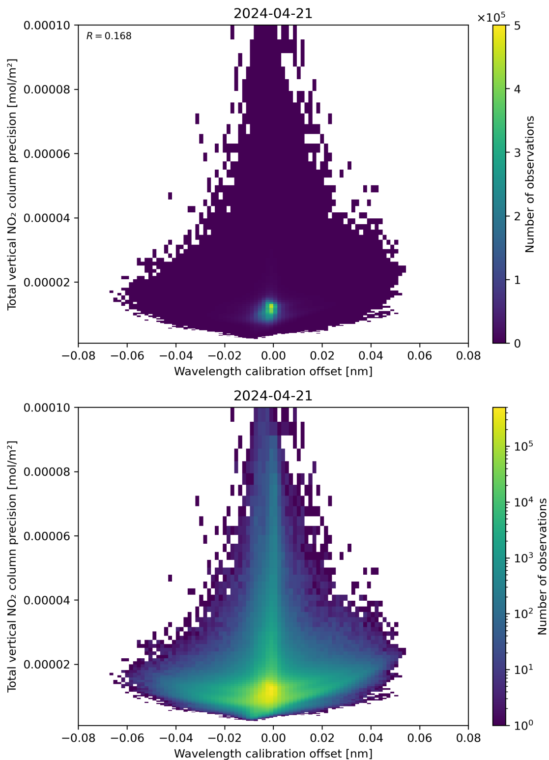
Figure 180: Scatter density plot of “Wavelength calibration offset” against “Total vertical NO 2 column precision” for 2024-04-21 to 2024-04-22.
