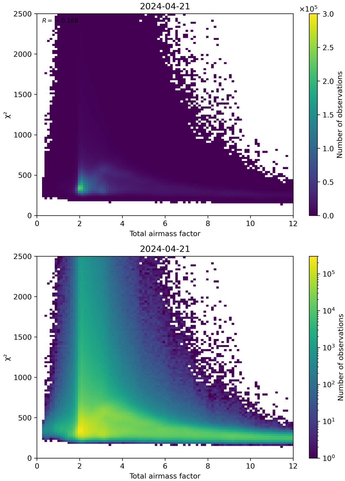
Figure 63: Scatter density plot of “Total airmass factor” against “ \chi^2 ” for 2024-04-21 to 2024-04-22.
