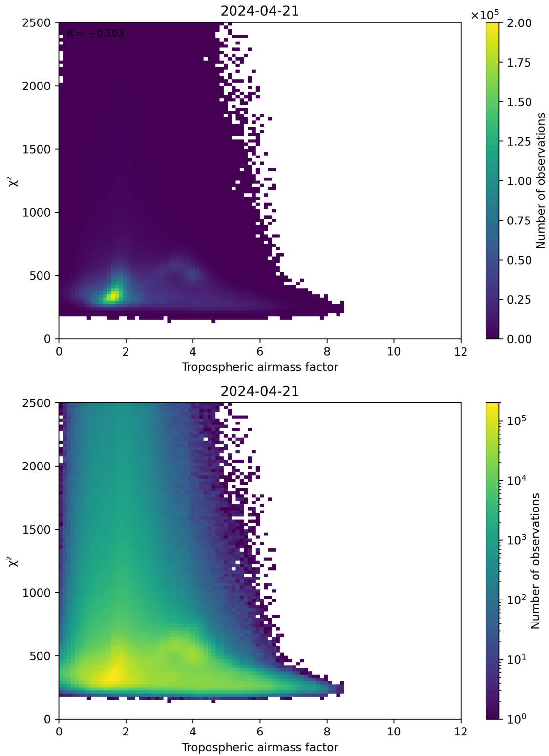
Figure 73: Scatter density plot of “Tropospheric airmass factor” against “ \chi^2 ” for 2024-04-21 to 2024-04-22.
