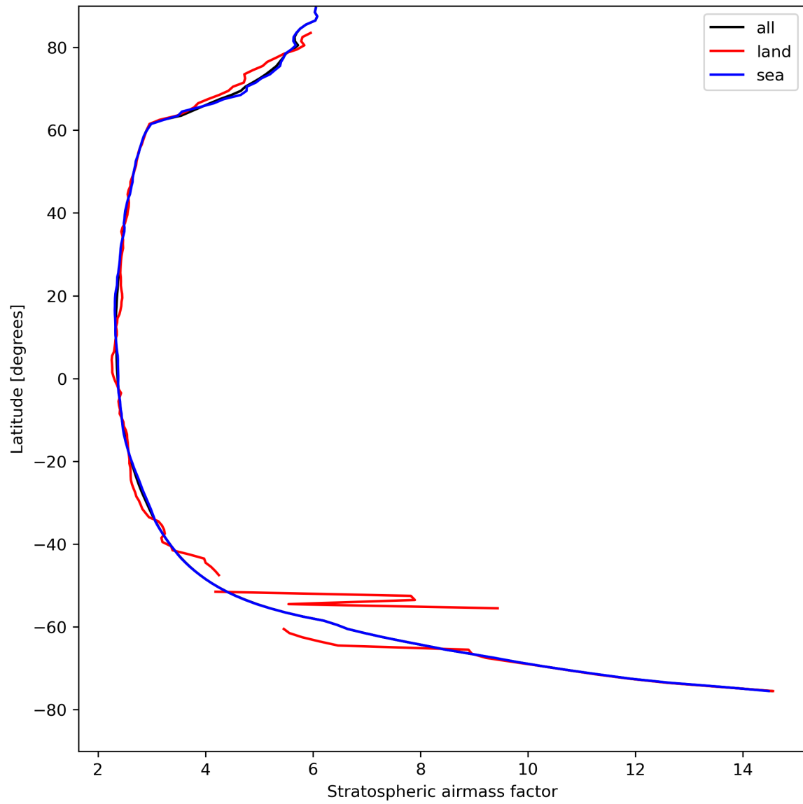
Figure 27: Zonal average of “Stratospheric air mass factor” for 2024-04-21 to 2024-04-22.
