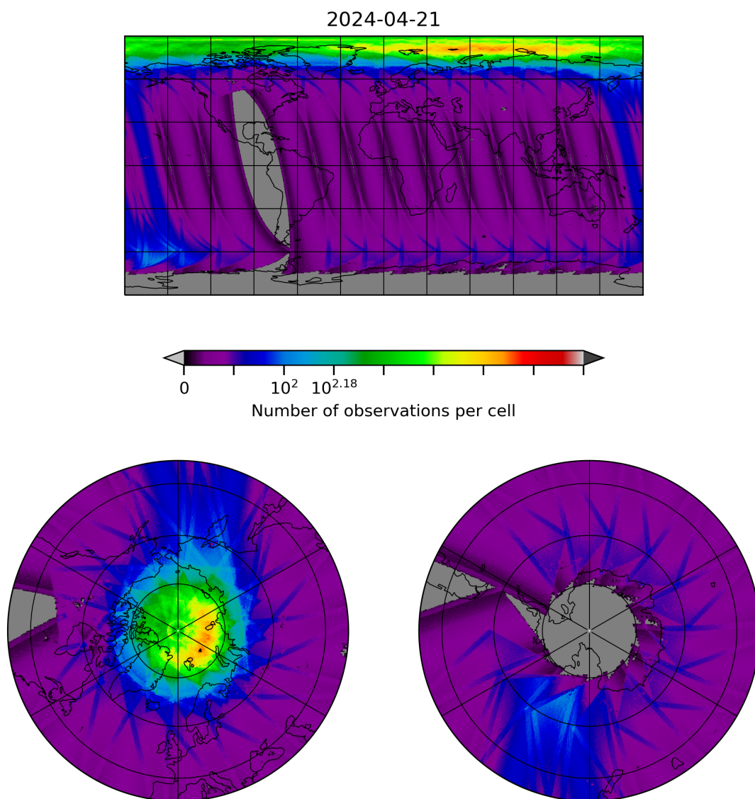
Figure 10: Map of the number of observations for 2024-04-21 to 2024-04-22
