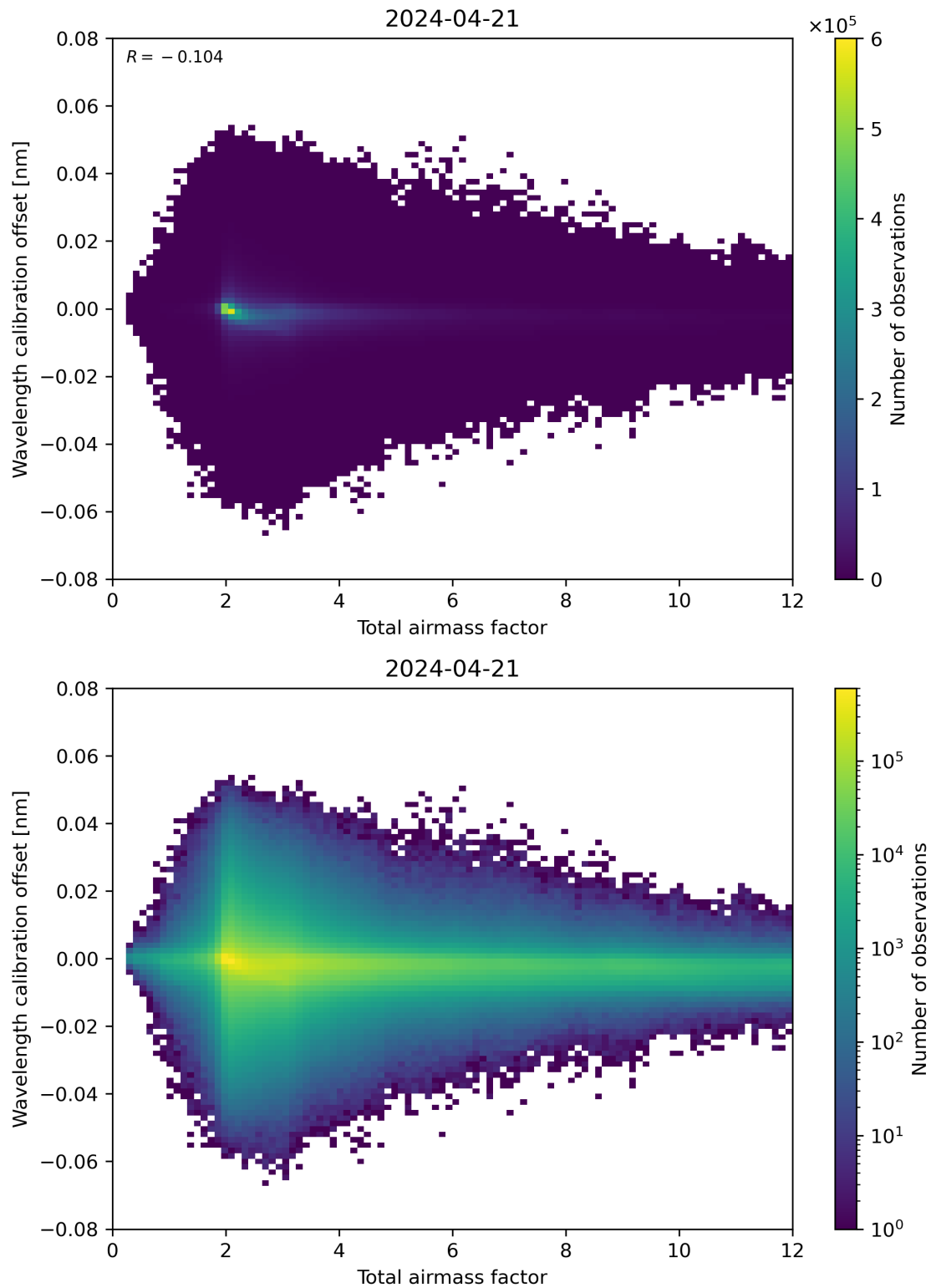
Figure 70: Scatter density plot of “Total airmass factor” against “Wavelength calibration offset” for 2024-04-21 to 2024-04-22.
