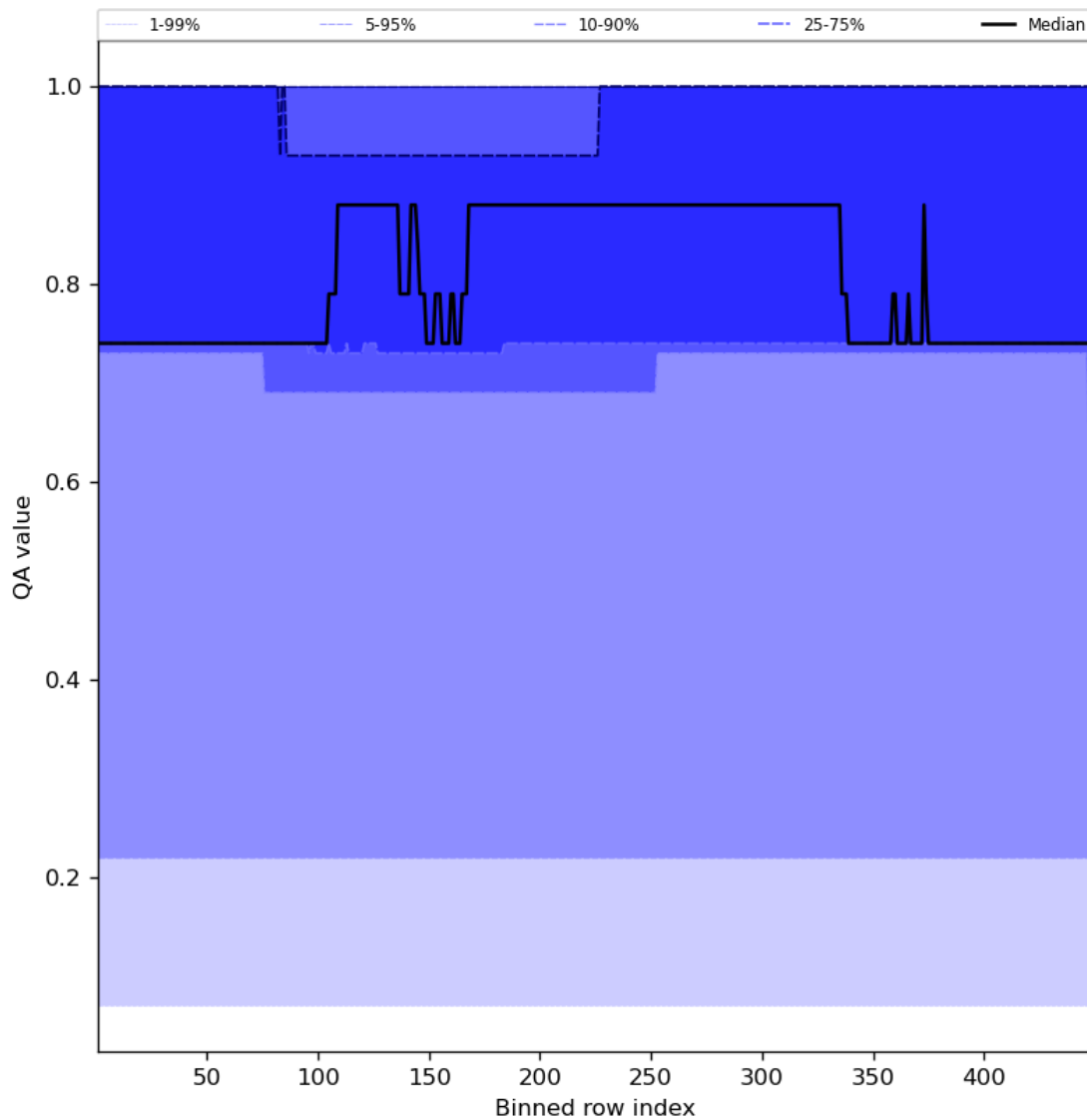
Figure 45: Along track statistics of “QA value” for 2024-04-21 to 2024-04-22
