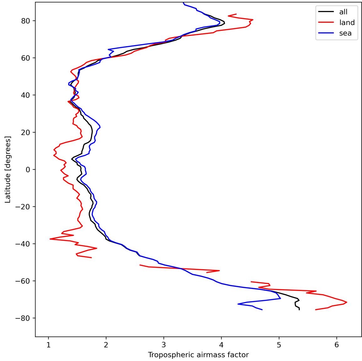
Figure 14: Zonal average of “Tropospheric airmass factor” for 2024-04-21 to 2024-04-22.
