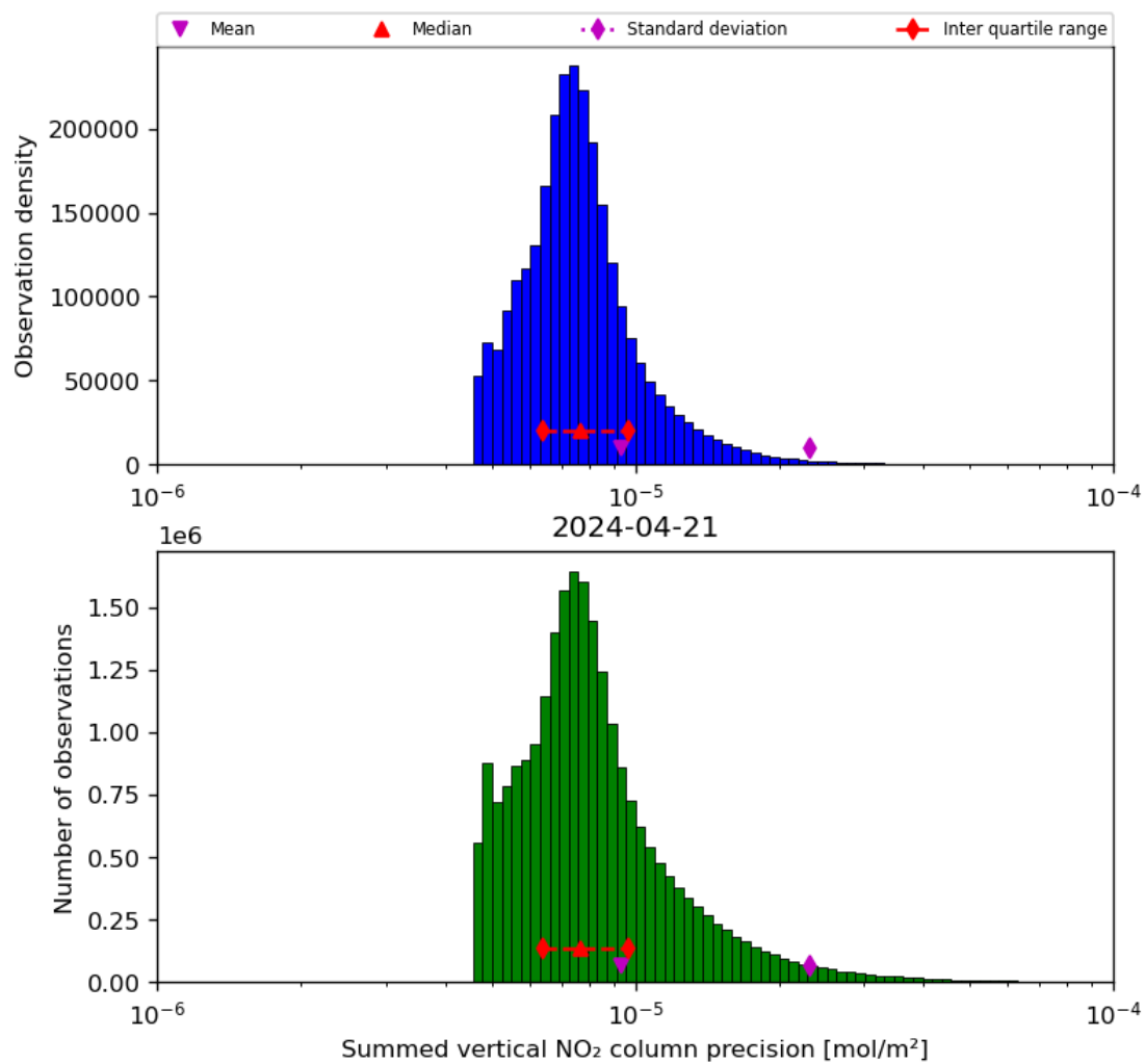
Figure 41: Histogram of “Summed vertical NO 2 column precision” for 2024-04-21 to 2024-04-22
