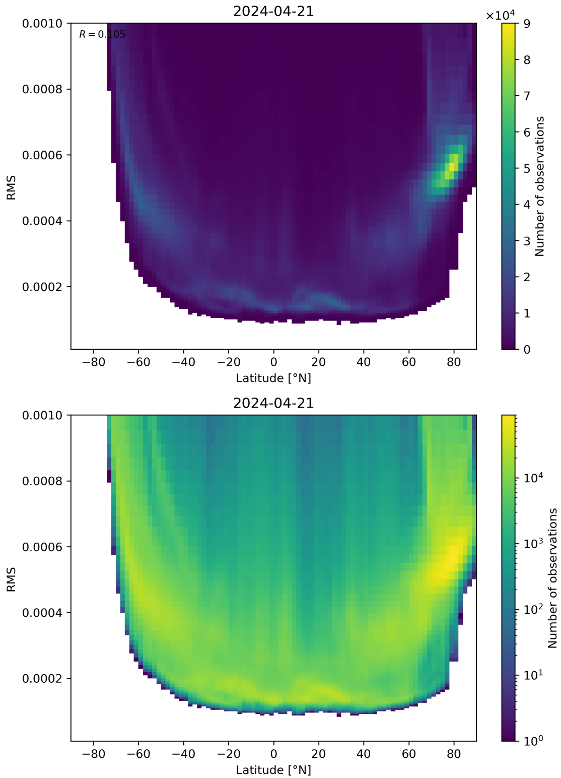
Figure 94: Scatter density plot of “Latitude” against “RMS” for 2024-04-21 to 2024-04-22.
