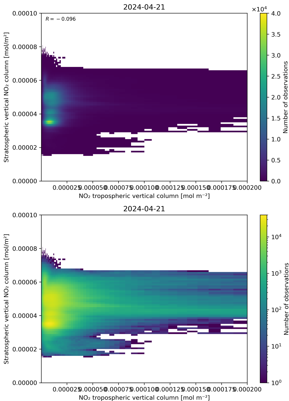
Figure 125: Scatter density plot of “NO 2 tropospheric vertical column” against “Stratospheric vertical NO 2 column” for 2024-04-21 to 2024-04-22.
