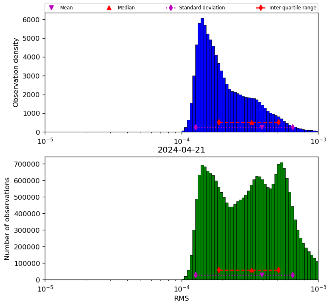
Figure 43: Histogram of “RMS” for 2024-04-21 to 2024-04-22
