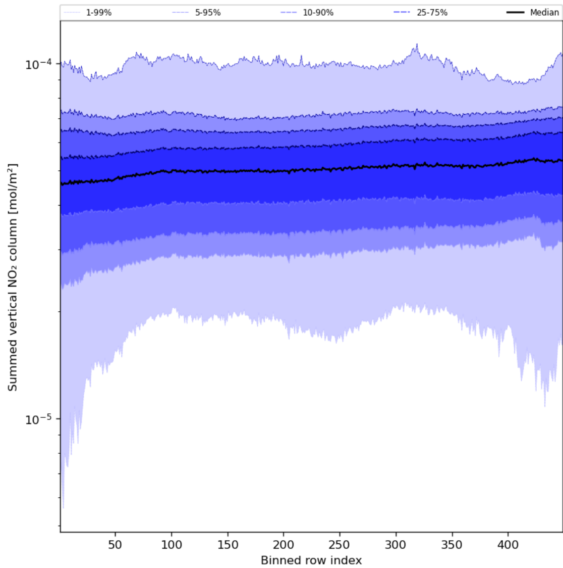
Figure 57: Along track statistics of “Summed vertical NO 2 column” for 2024-04-21 to 2024-04-22
