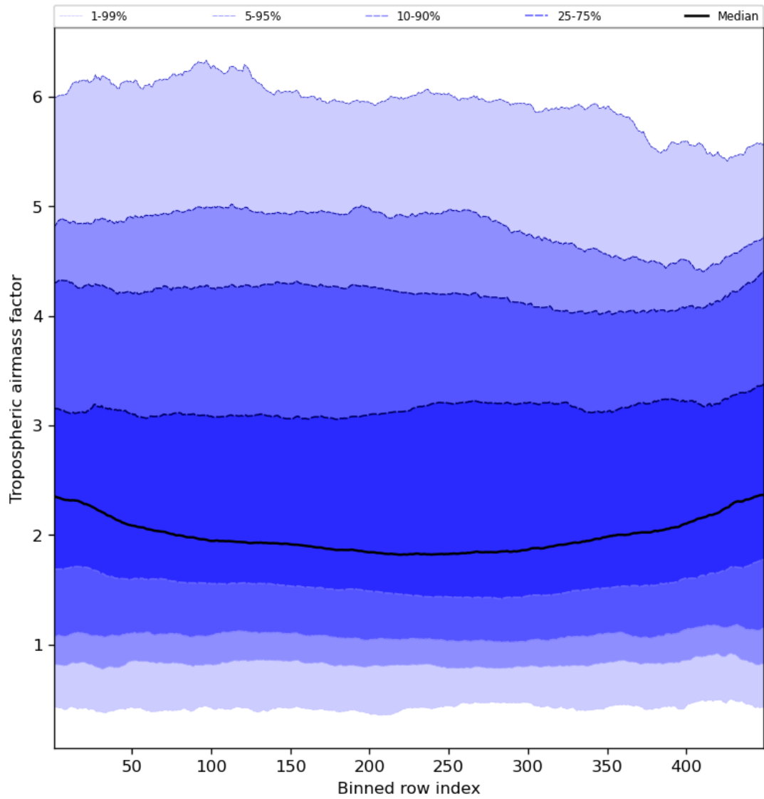
Figure 48: Along track statistics of “Tropospheric airmass factor” for 2024-04-21 to 2024-04-22
