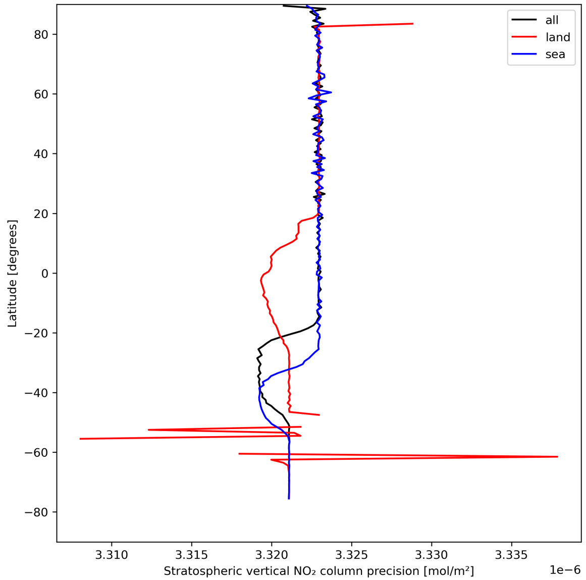
Figure 20: Zonal average of “Stratospheric vertical NO 2 column precision” for 2024-04-21 to 2024-04-22.
