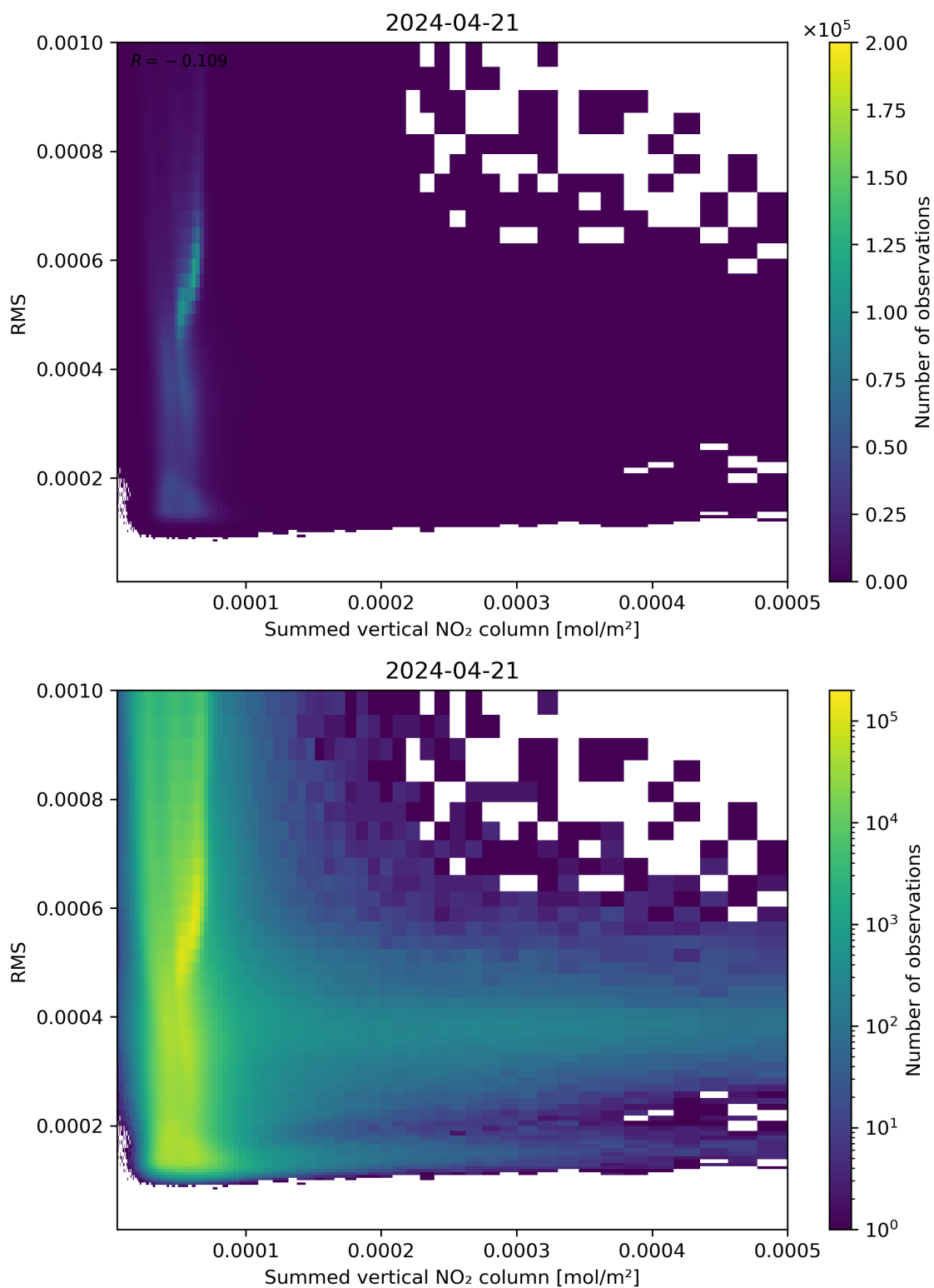
Figure 109: Scatter density plot of “Summed vertical NO 2 column” against “RMS” for 2024-04-21 to 2024-04-22.
