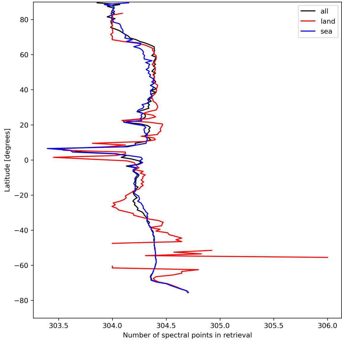
Figure 16: Zonal average of “Number of spectral points in retrieval” for 2024-04-21 to 2024-04-22.
