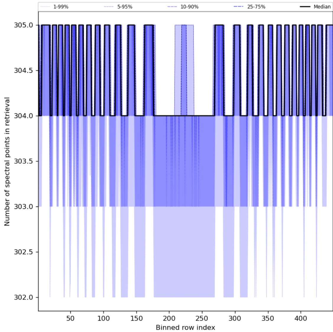
Figure 50: Along track statistics of “Number of spectral points in retrieval” for 2024-04-21 to 2024-04-22
