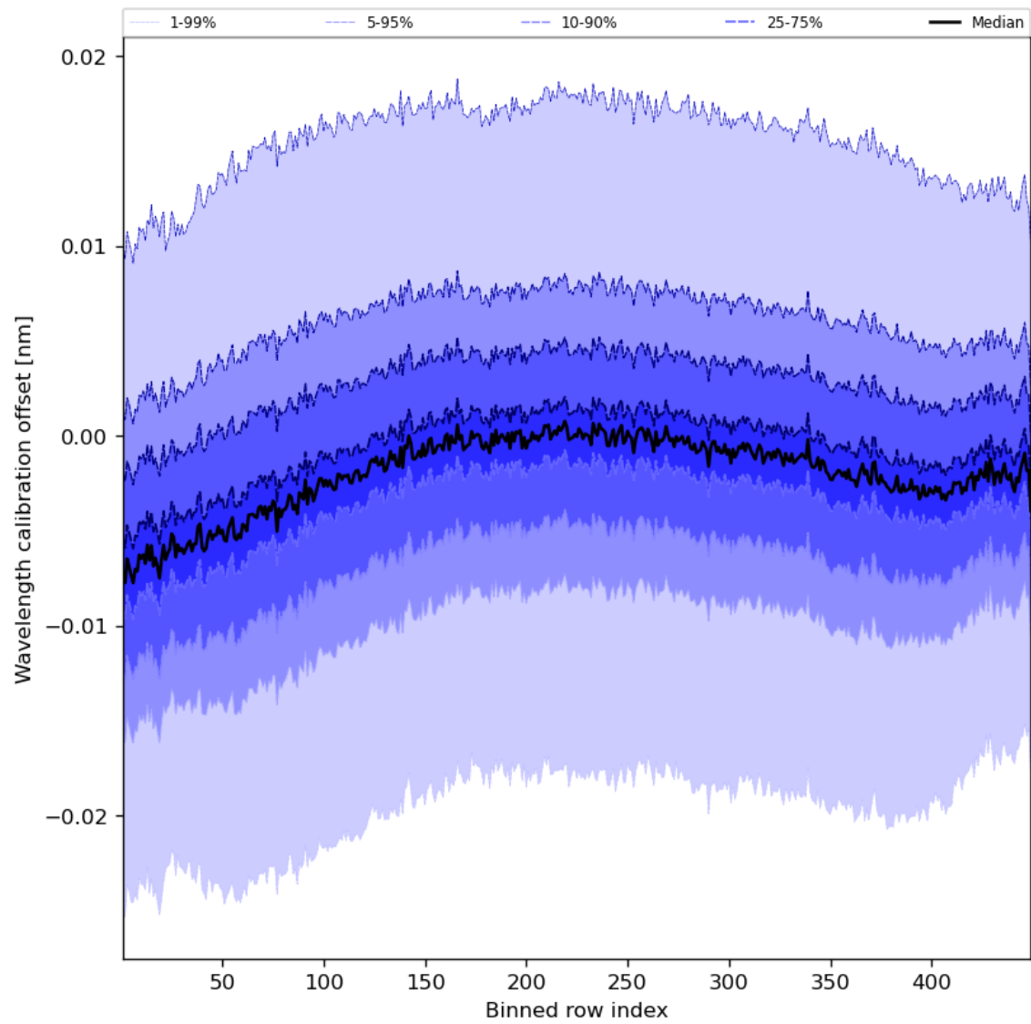
Figure 52: Along track statistics of “Wavelength calibration offset” for 2024-04-21 to 2024-04-22
