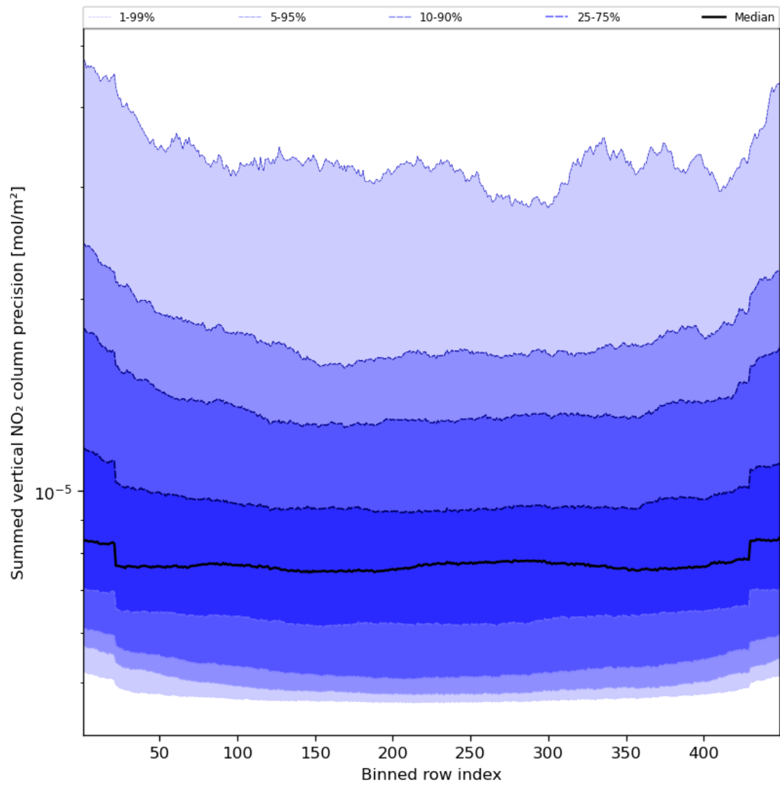
Figure 58: Along track statistics of “Summed vertical NO 2 column precision” for 2024-04-21 to 2024-04-22
