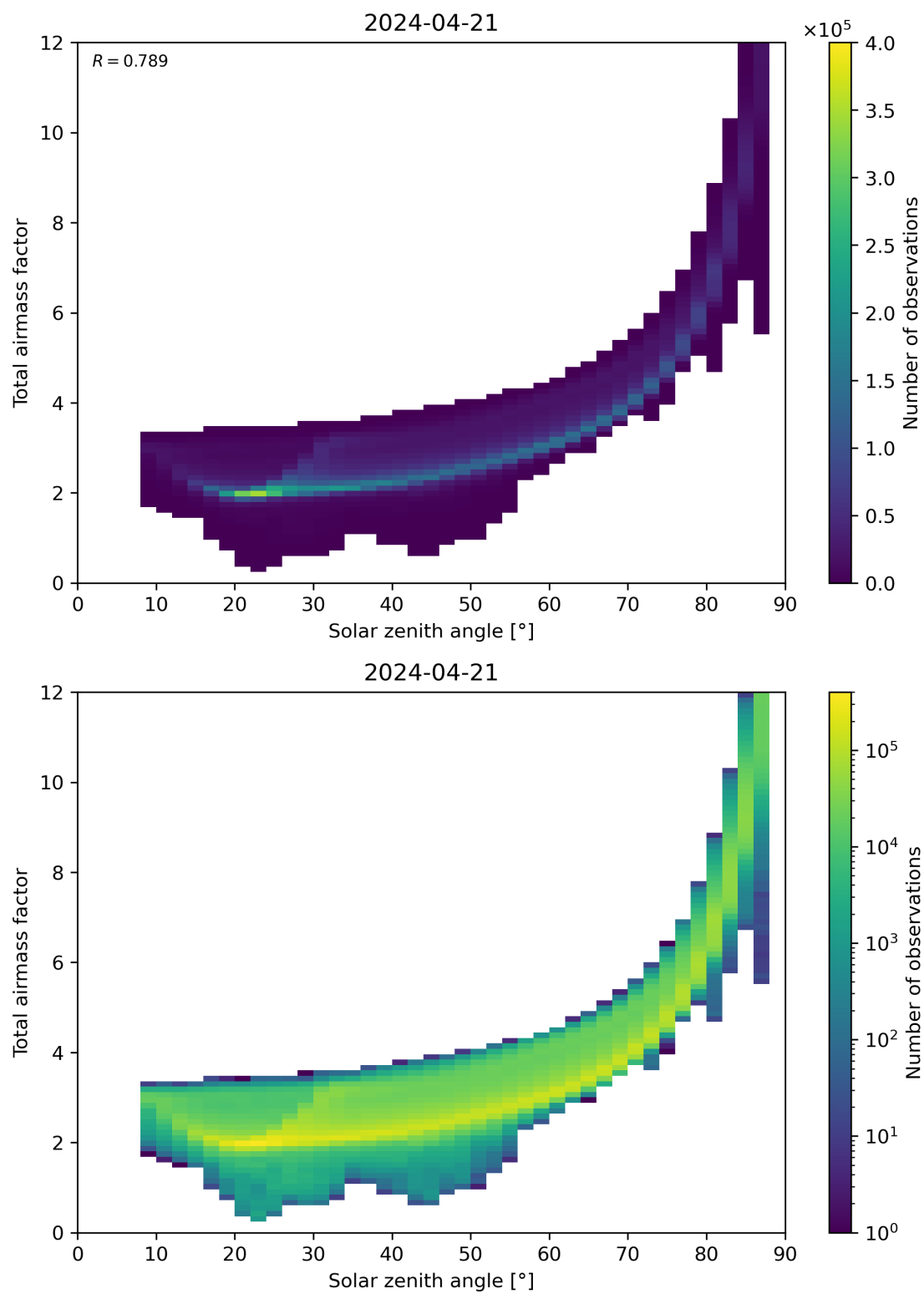
Figure 146: Scatter density plot of “Solar zenith angle” against “Total airmass factor” for 2024-04-21 to 2024-04-22.
