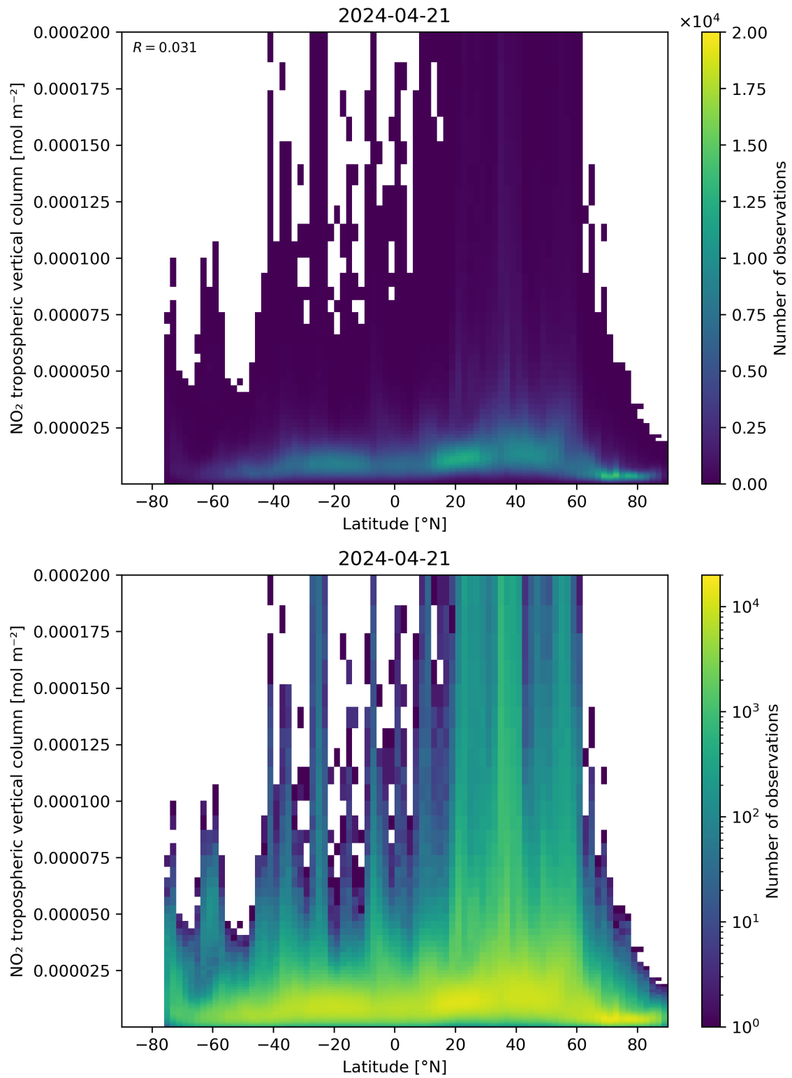
Figure 92: Scatter density plot of “Latitude” against “NO 2 tropospheric vertical column” for 2024-04-21 to 2024-04-22.
