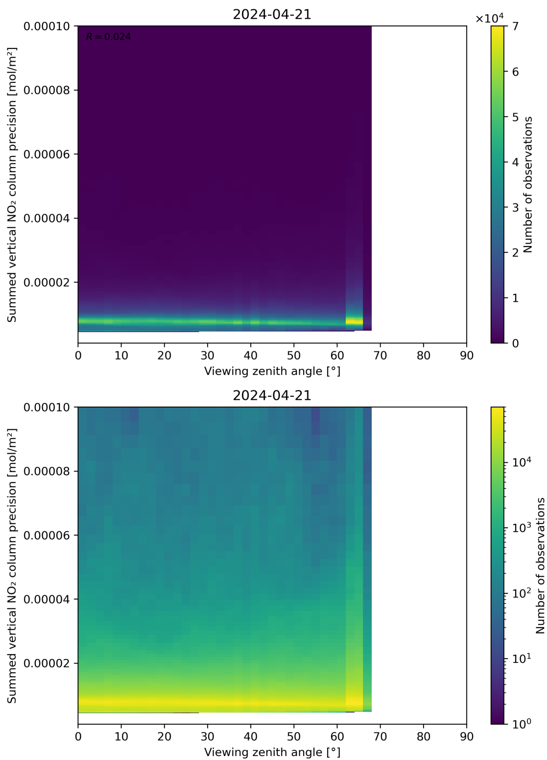
Figure 166: Scatter density plot of “Viewing zenith angle” against “Summed vertical NO 2 column precision” for 2024-04-21 to 2024-04-22.
