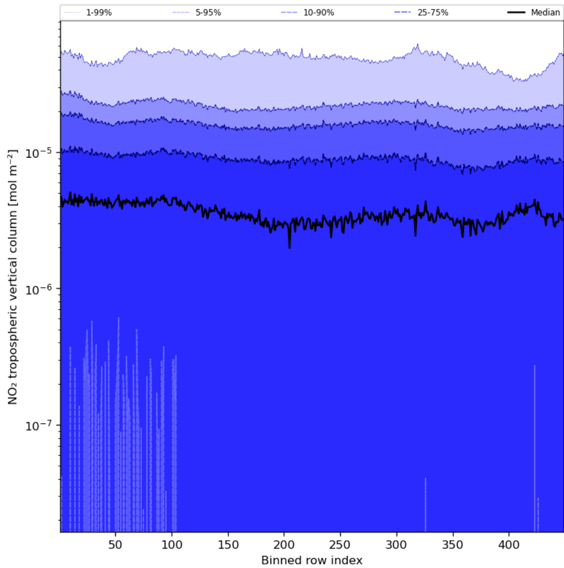
Figure 46: Along track statistics of “NO 2 tropospheric vertical column” for 2024-04-21 to 2024-04-22
