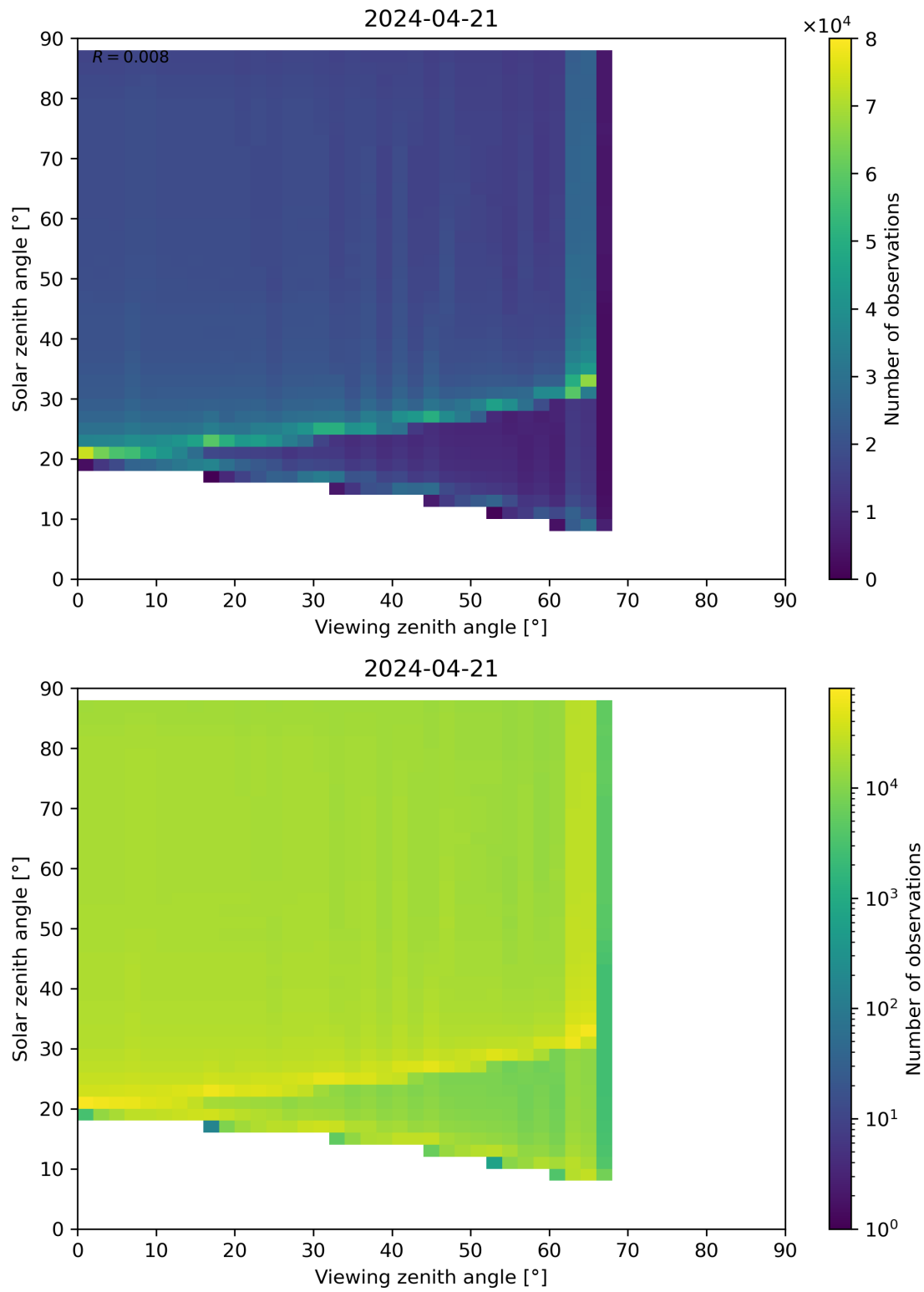
Figure 172: Scatter density plot of “Viewing zenith angle” against “Solar zenith angle” for 2024-04-21 to 2024-04-22.
