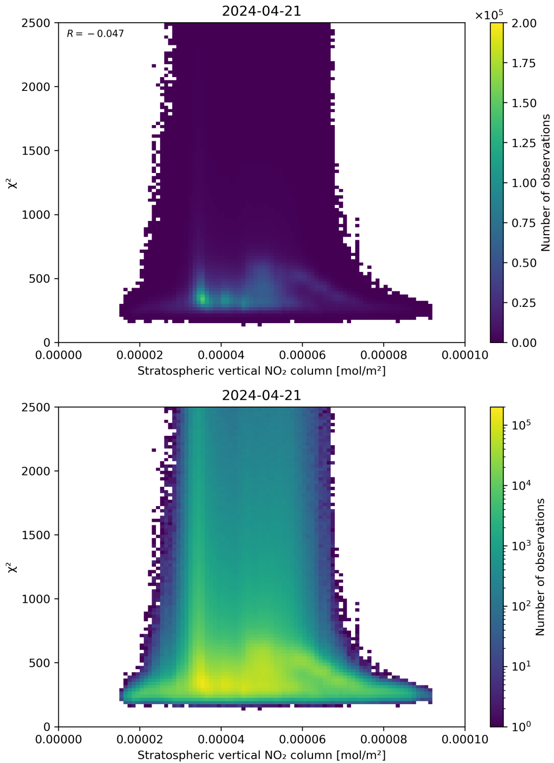
Figure 97: Scatter density plot of “Stratospheric vertical NO 2 column” against “ \chi^2 ” for 2024-04-21 to 2024-04-22.
