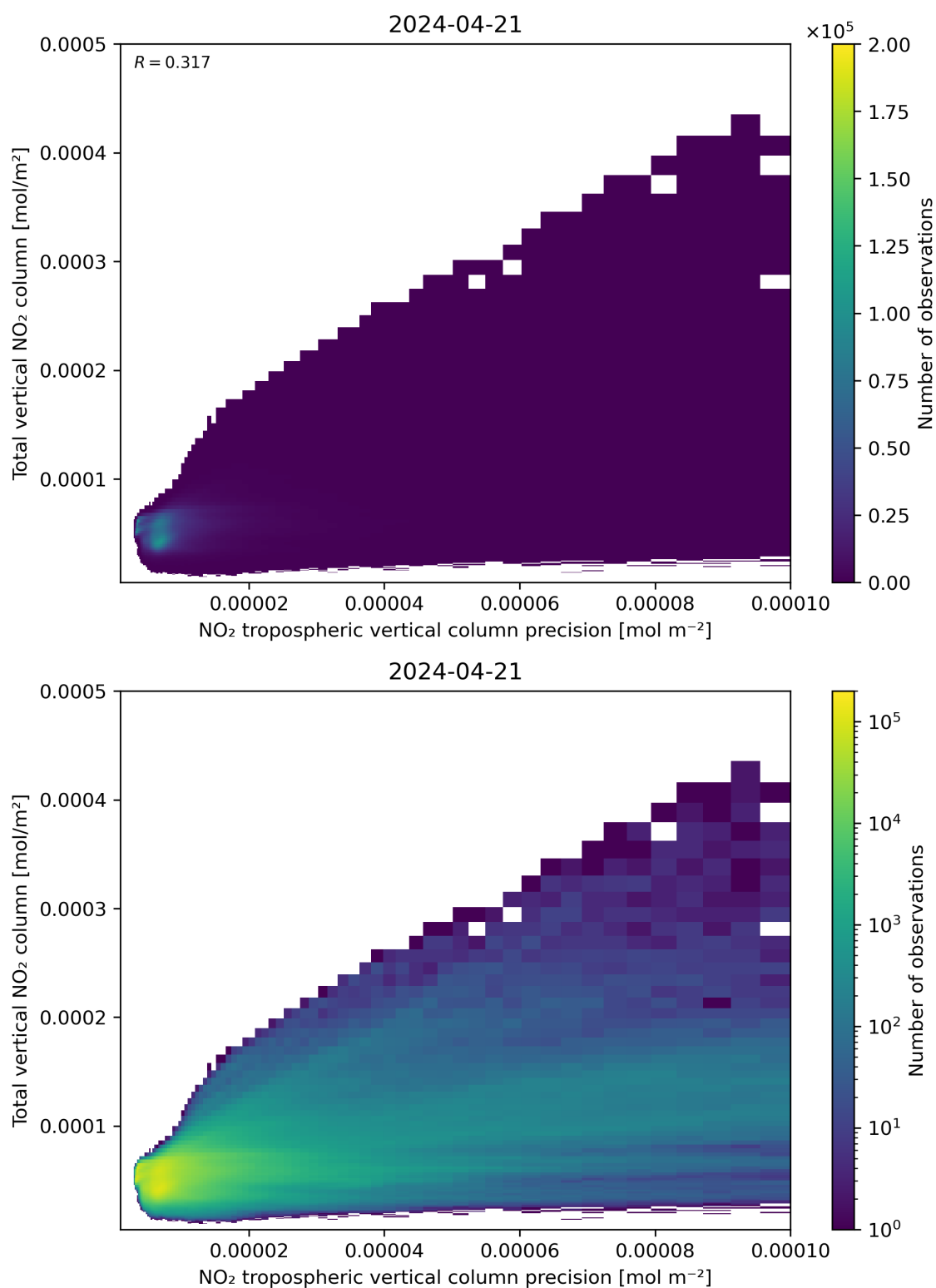
Figure 138: Scatter density plot of “NO 2 tropospheric vertical column precision” against “Total vertical NO 2 column” for 2024-04-21 to 2024-04-22.
