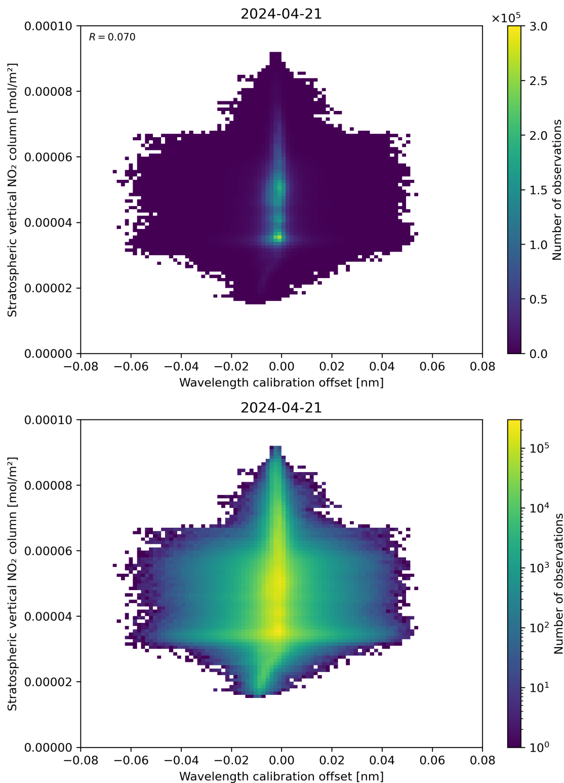
Figure 176: Scatter density plot of “Wavelength calibration offset” against “Stratospheric vertical NO 2 column” for 2024-04-21 to 2024-04-22.
