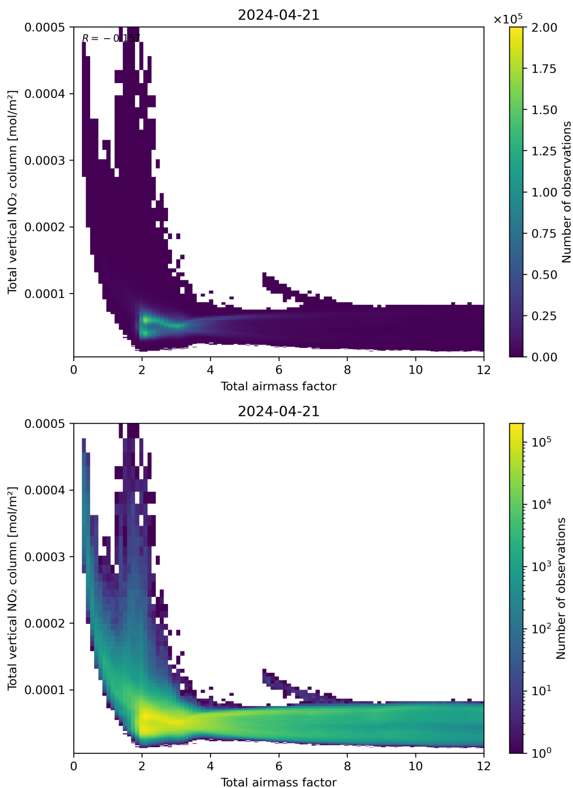
Figure 67: Scatter density plot of “Total airmass factor” against “Total vertical NO 2 column” for 2024-04-21 to 2024-04-22.
