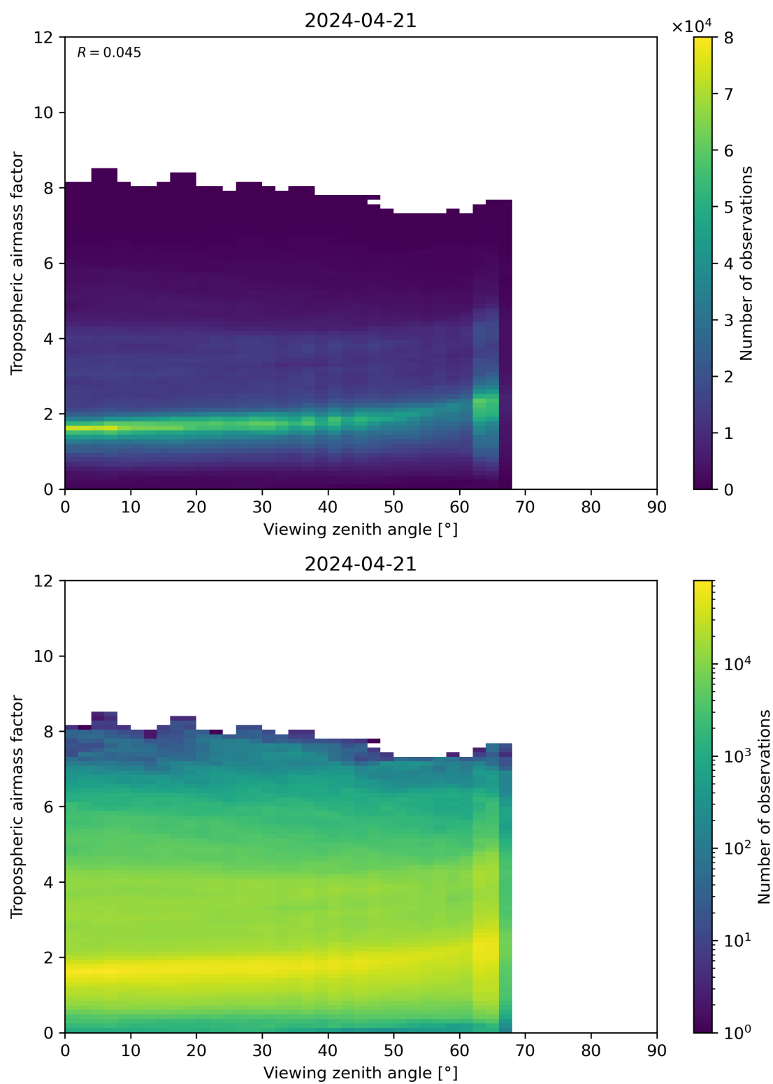
Figure 161: Scatter density plot of “Viewing zenith angle” against “Tropospheric airmass factor” for 2024-04-21 to 2024-04-22.
