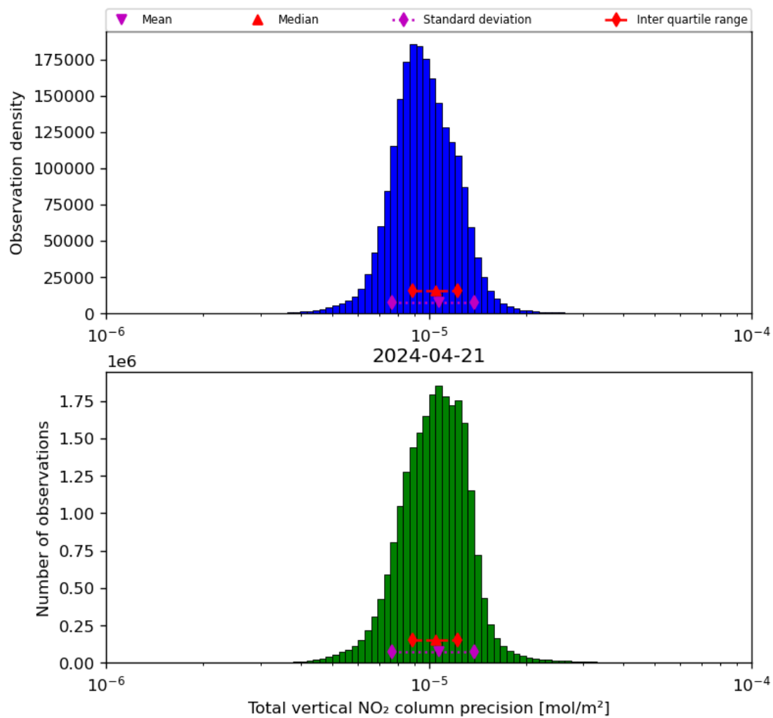
Figure 39: Histogram of “Total vertical NO 2 column precision” for 2024-04-21 to 2024-04-22
