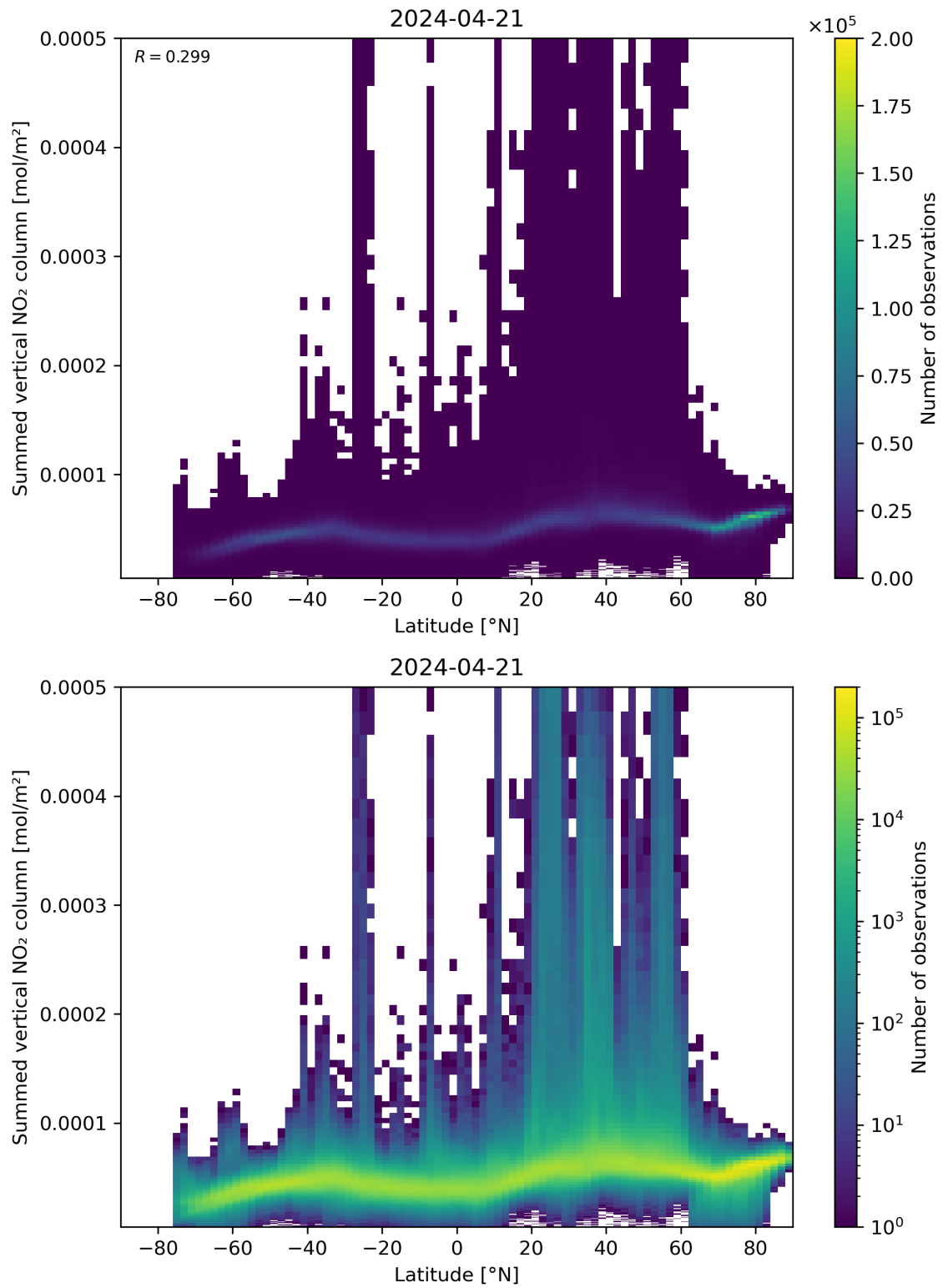
Figure 88: Scatter density plot of “Latitude” against “Summed vertical NO 2 column” for 2024-04-21 to 2024-04-22.
