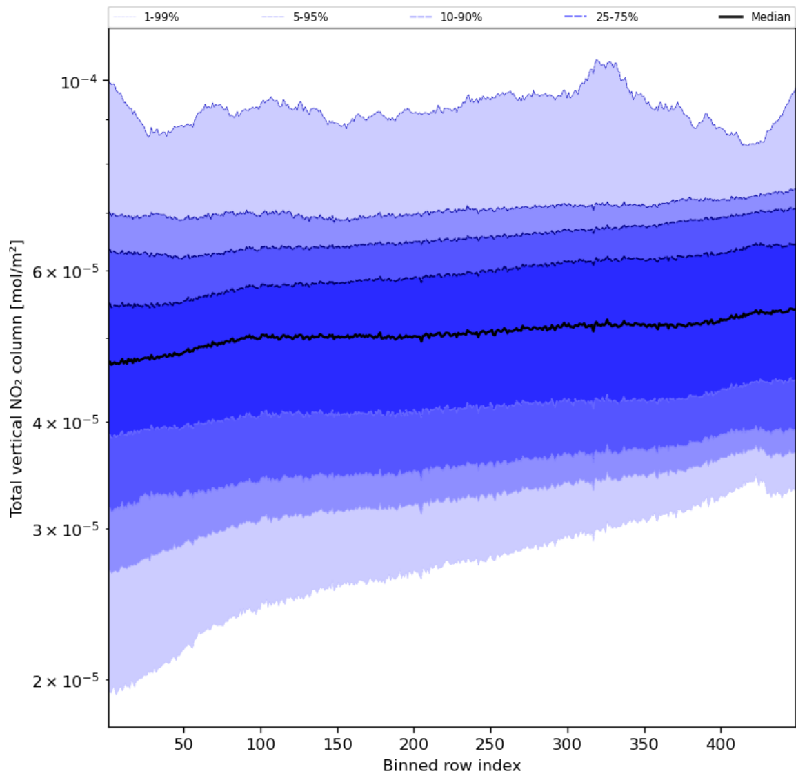
Figure 55: Along track statistics of “Total vertical NO 2 column” for 2024-04-21 to 2024-04-22
