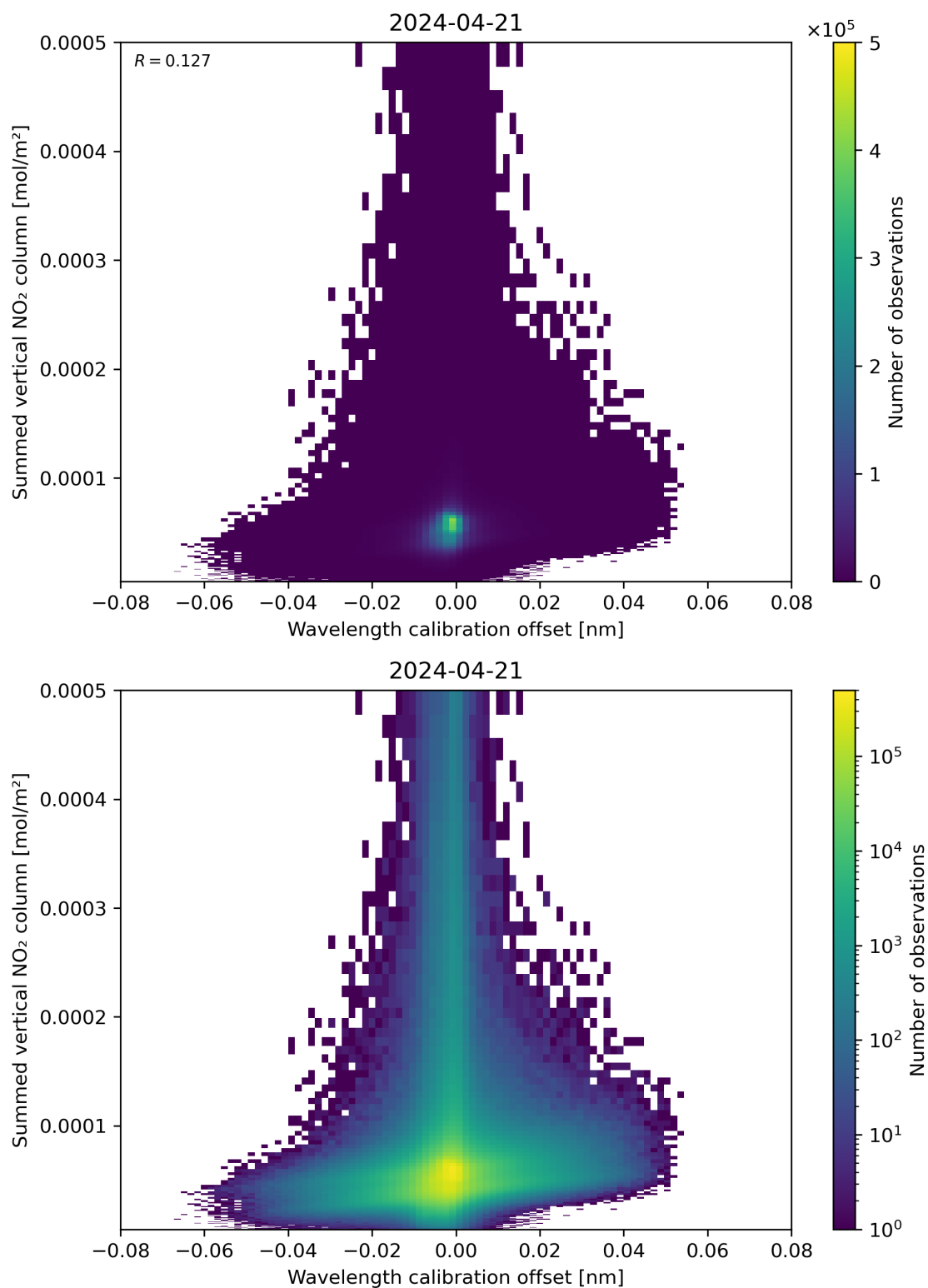
Figure 177: Scatter density plot of “Wavelength calibration offset” against “Summed vertical NO 2 column” for 2024-04-21 to 2024-04-22.
