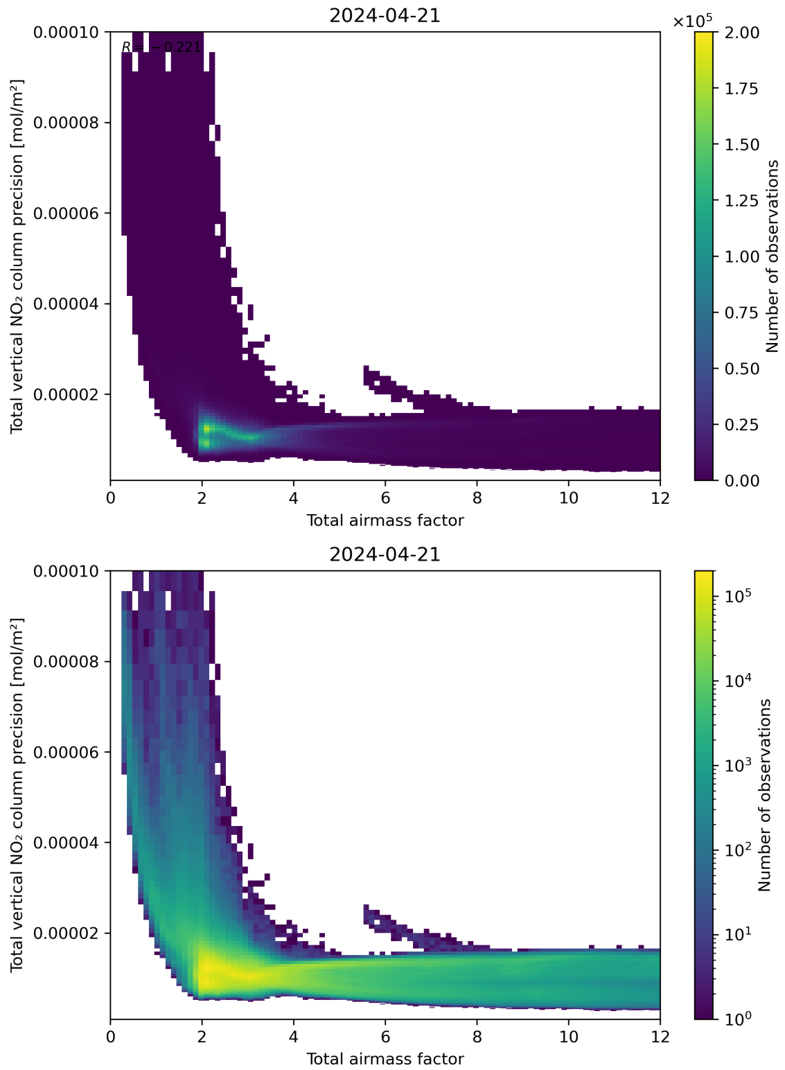
Figure 68: Scatter density plot of “Total airmass factor” against “Total vertical NO 2 column precision” for 2024-04-21 to 2024-04-22.
