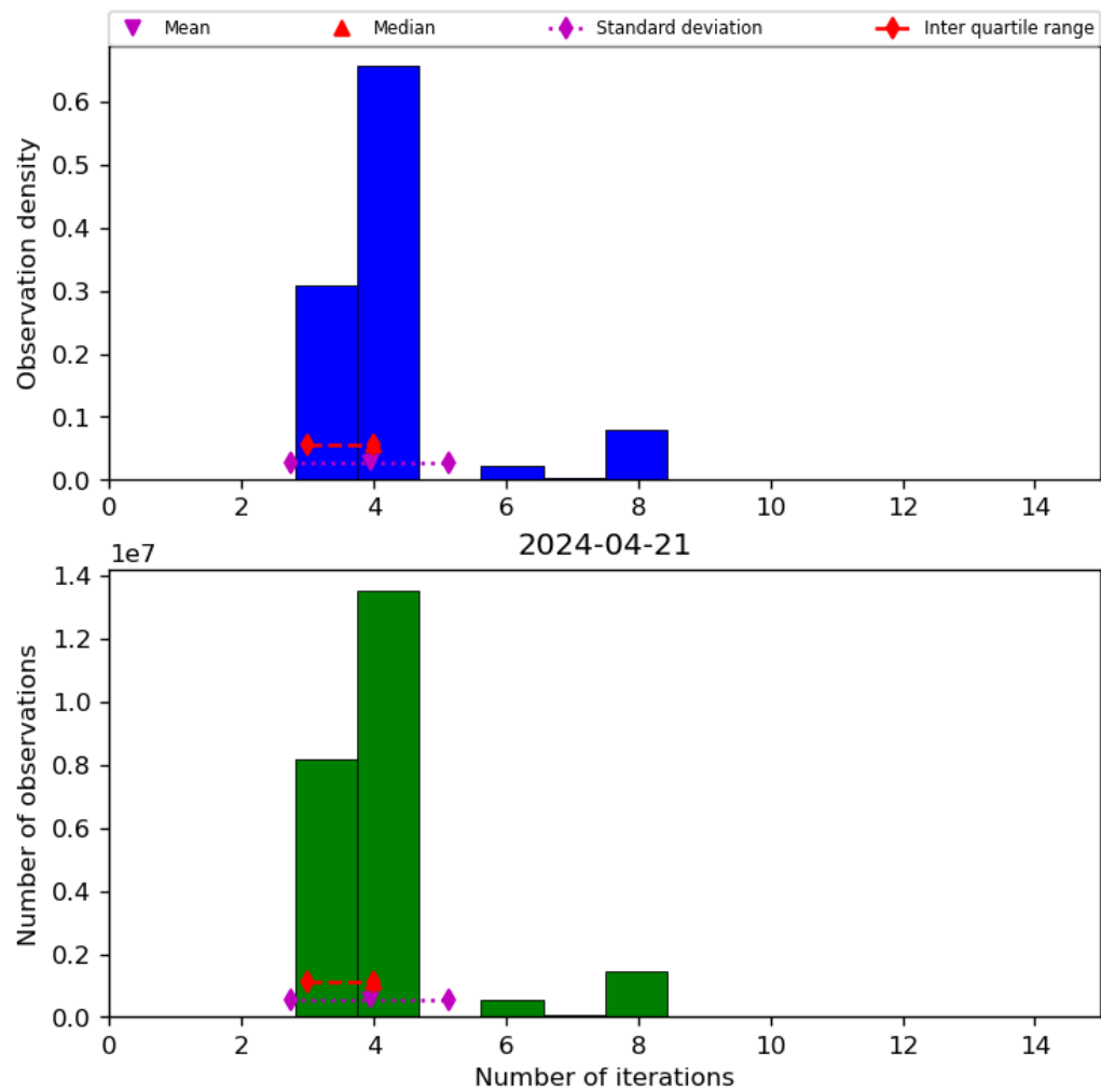
Figure 34: Histogram of “Number of iterations” for 2024-04-21 to 2024-04-22
