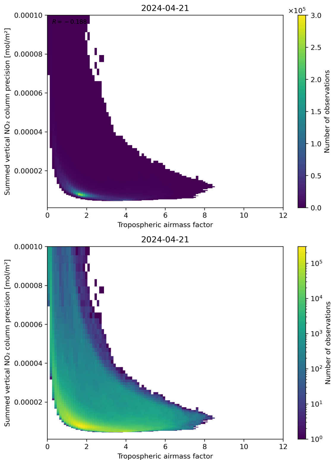
Figure 76: Scatter density plot of “Tropospheric air mass factor” against “Summed vertical NO 2 column precision” for 2024-04-21 to 2024-04-22.
