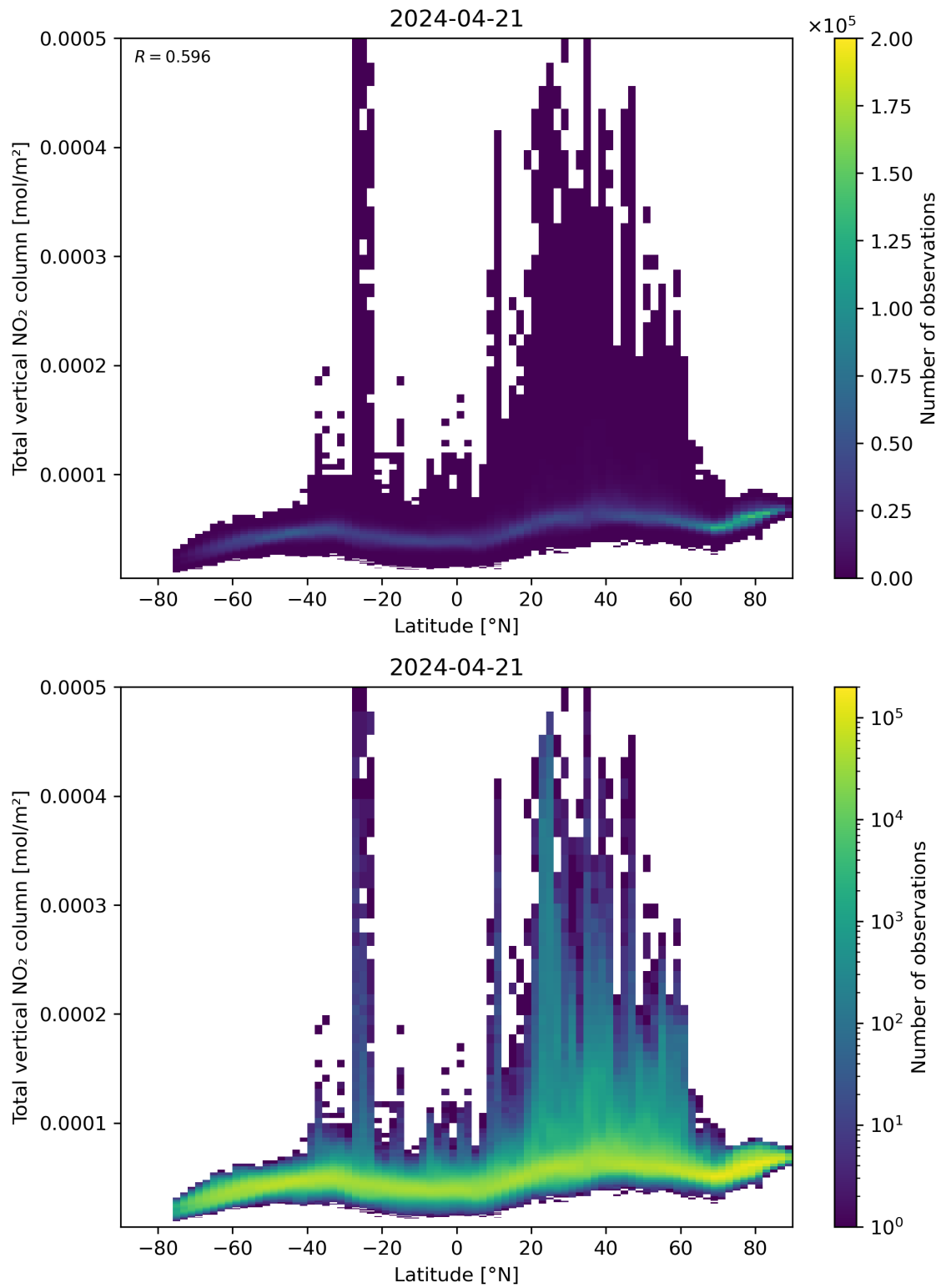
Figure 90: Scatter density plot of “Latitude” against “Total vertical NO 2 column” for 2024-04-21 to 2024-04-22.
