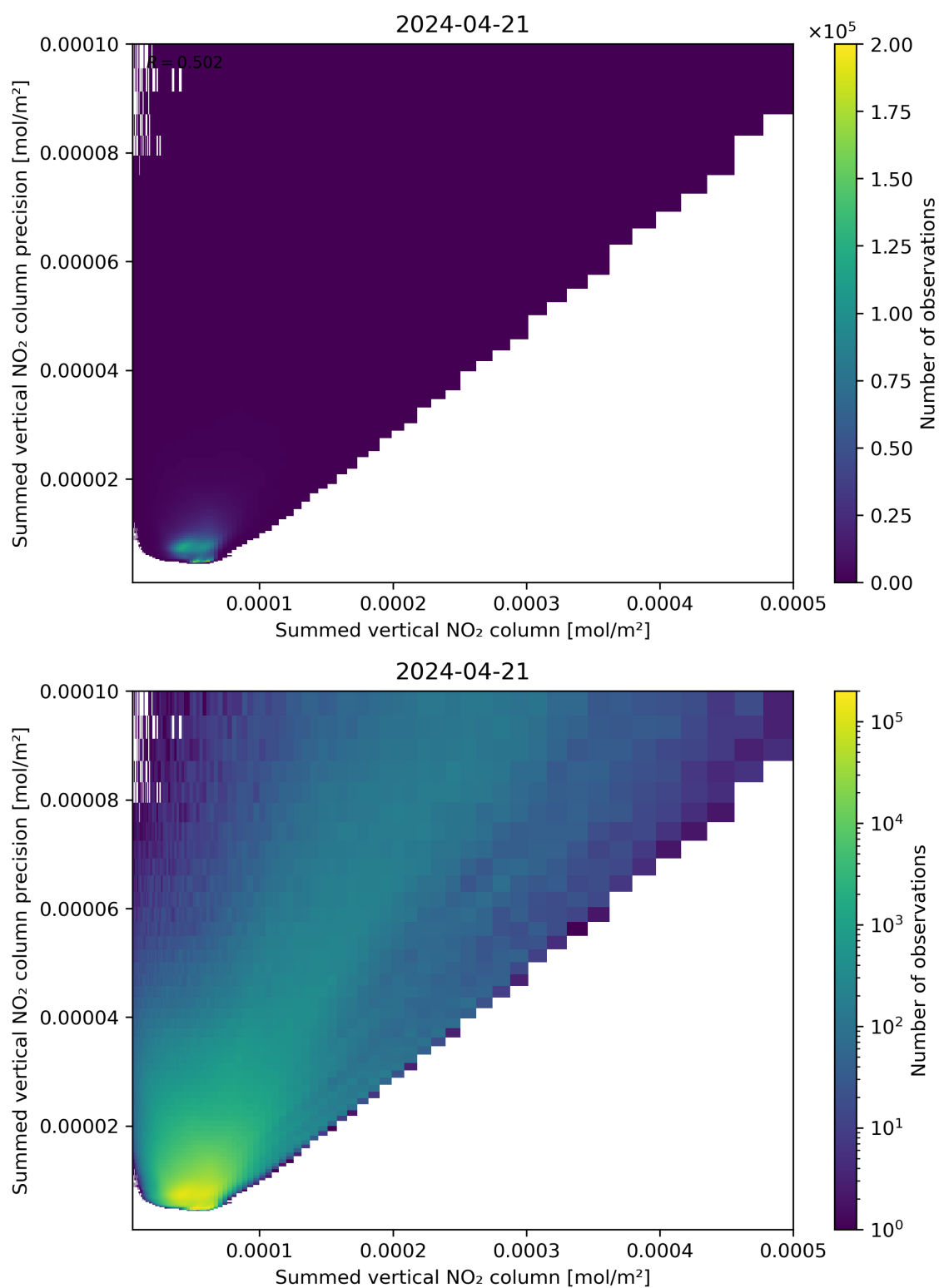
Figure 105: Scatter density plot of “Summed vertical NO 2 column” against “Summed vertical NO 2 column precision” for 2024-04-21 to 2024-04-22.
