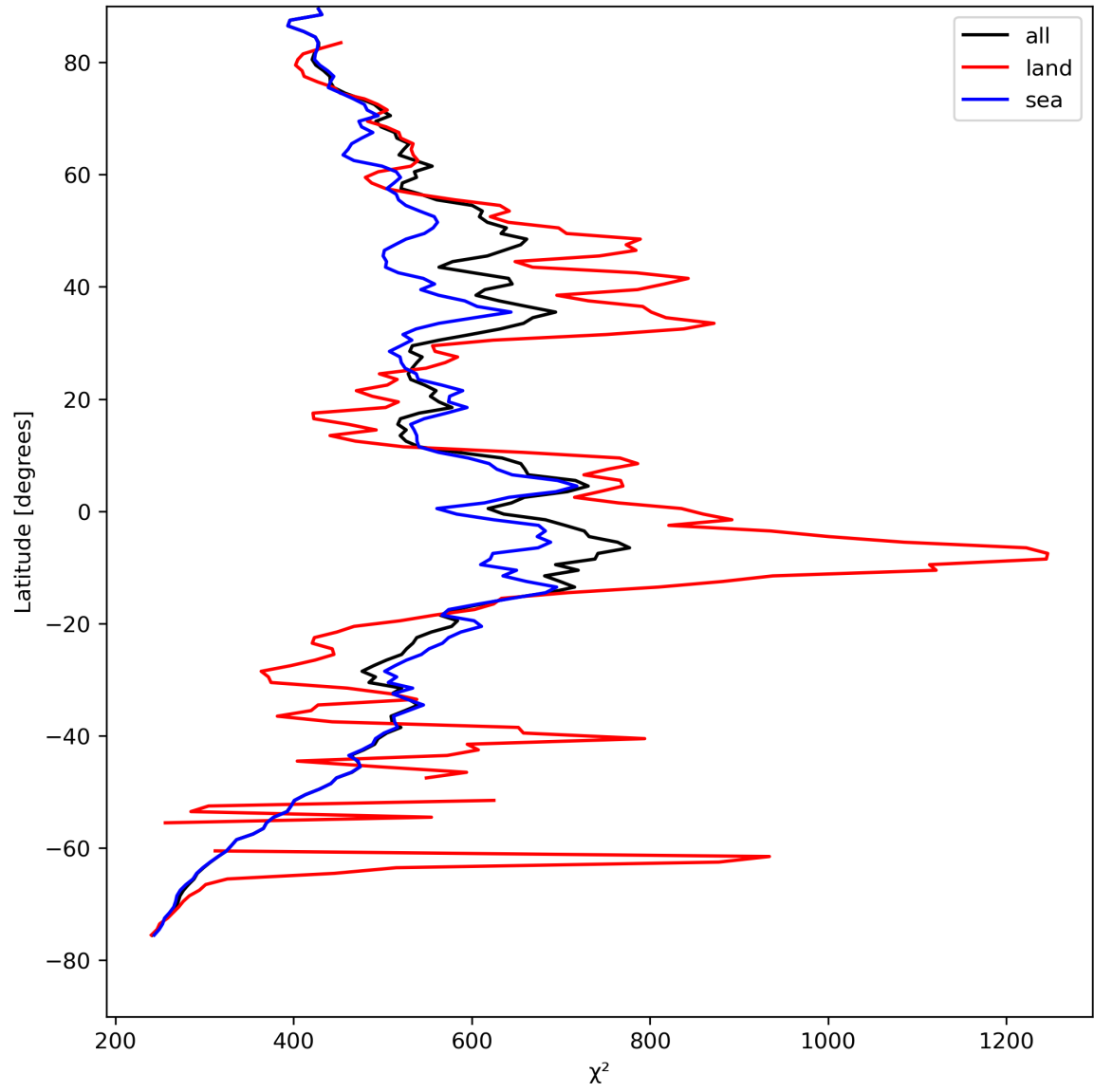
Figure 25: Zonal average of “ \chi^2 ” for 2024-04-21 to 2024-04-22.
