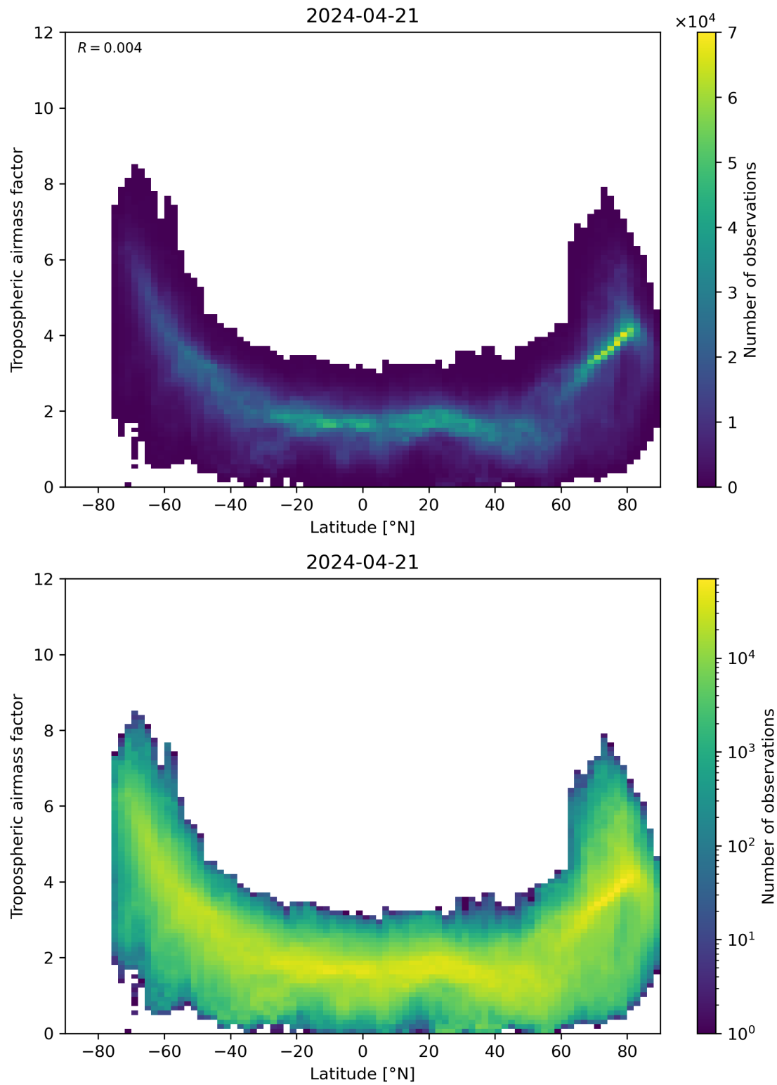
Figure 85: Scatter density plot of “Latitude” against “Tropospheric air mass factor” for 2024-04-21 to 2024-04-22.
