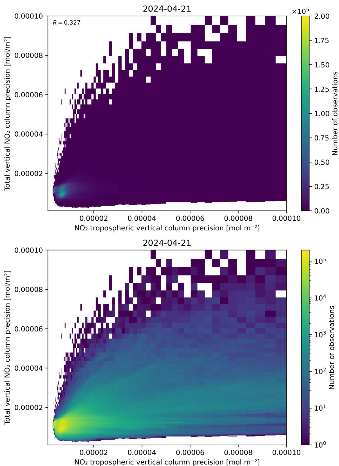
Figure 139: Scatter density plot of “NO 2 tropospheric vertical column precision” against “Total vertical NO 2 column precision” for 2024-04-21 to 2024-04-22.
