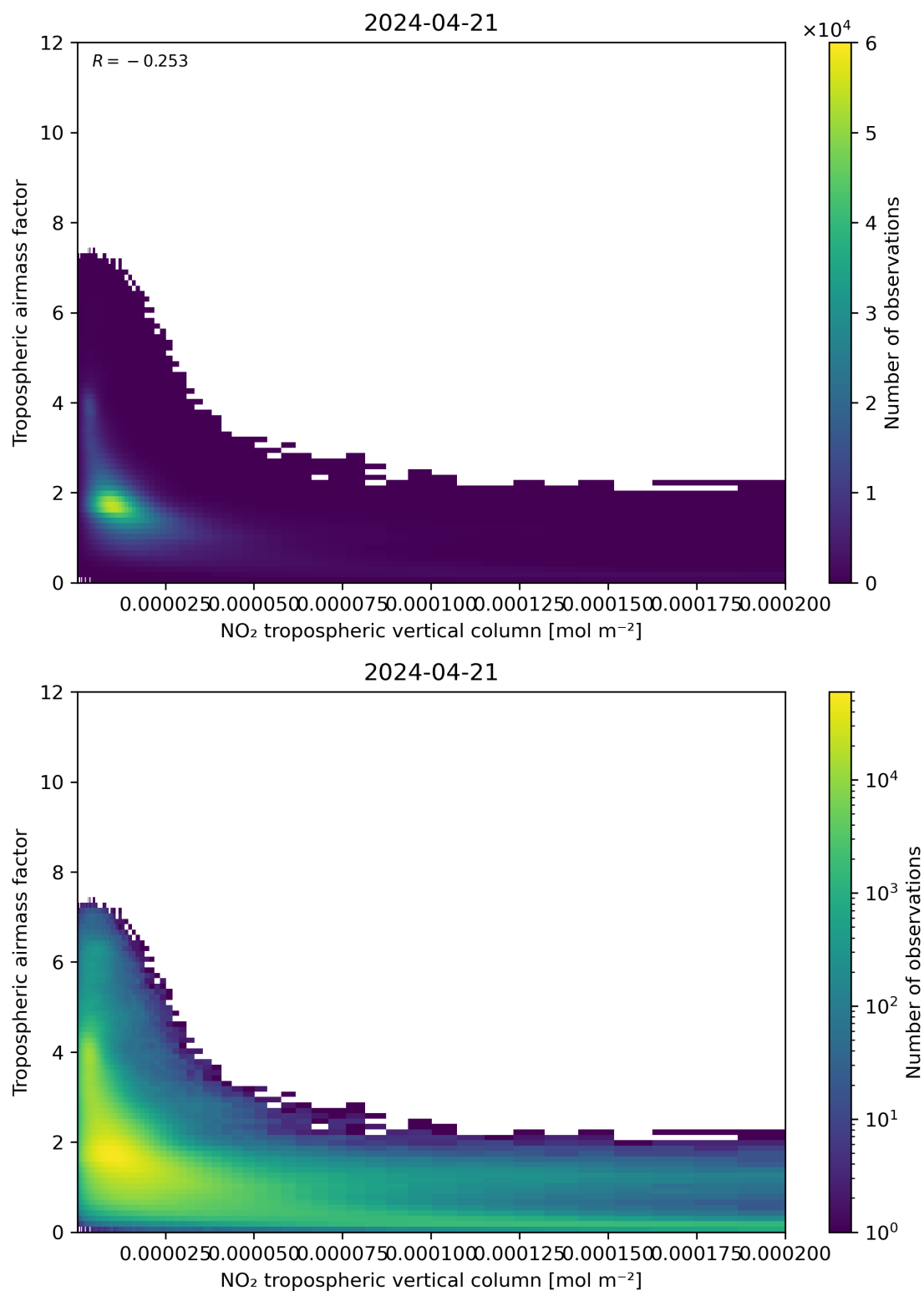
Figure 123: Scatter density plot of “NO 2 tropospheric vertical column” against “Tropospheric air mass factor” for 2024-04-21 to 2024-04-22.
