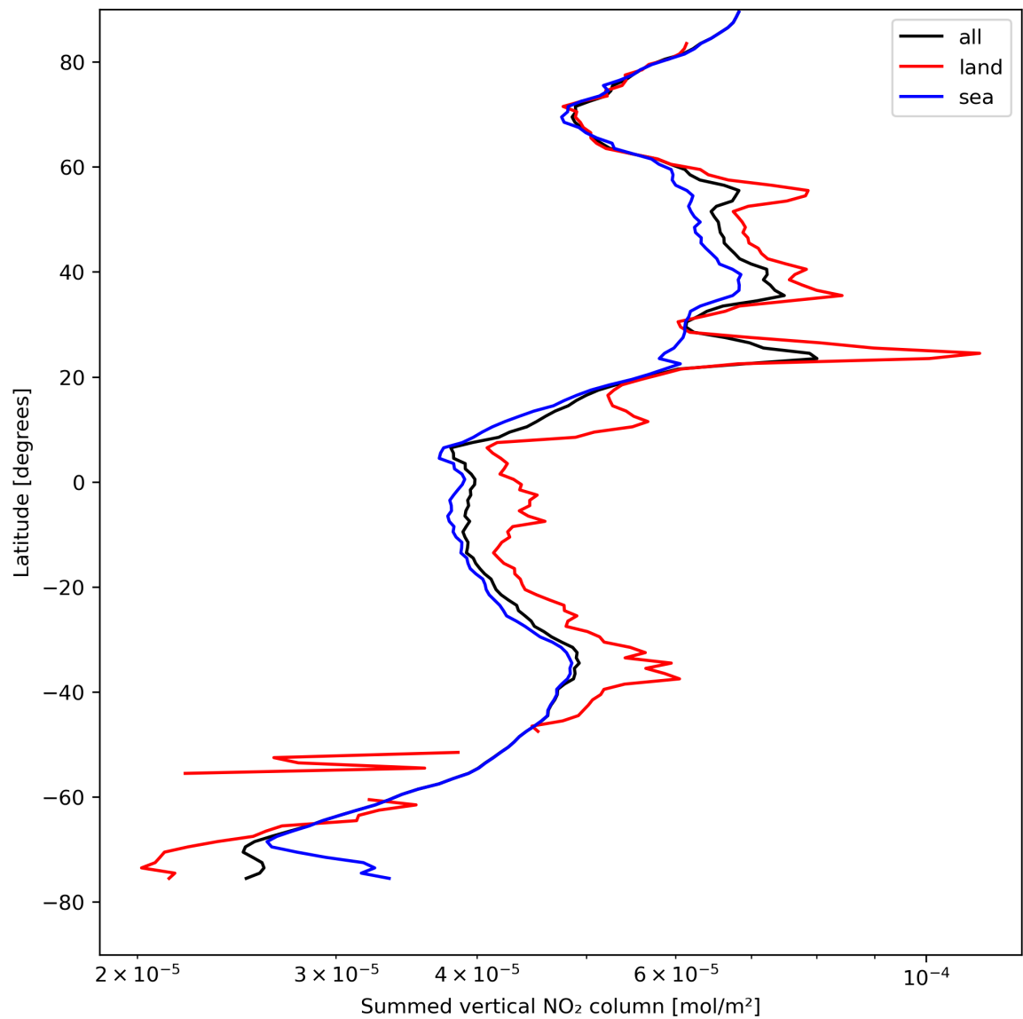
Figure 23: Zonal average of “Summed vertical NO 2 column” for 2024-04-21 to 2024-04-22.
