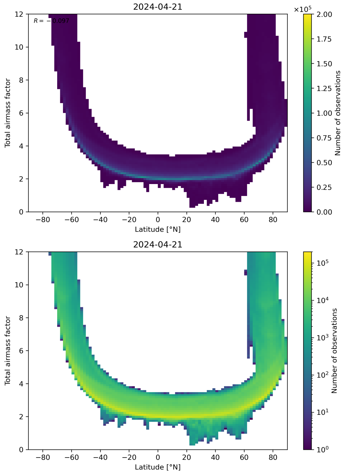
Figure 84: Scatter density plot of “Latitude” against “Total airmass factor” for 2024-04-21 to 2024-04-22.
