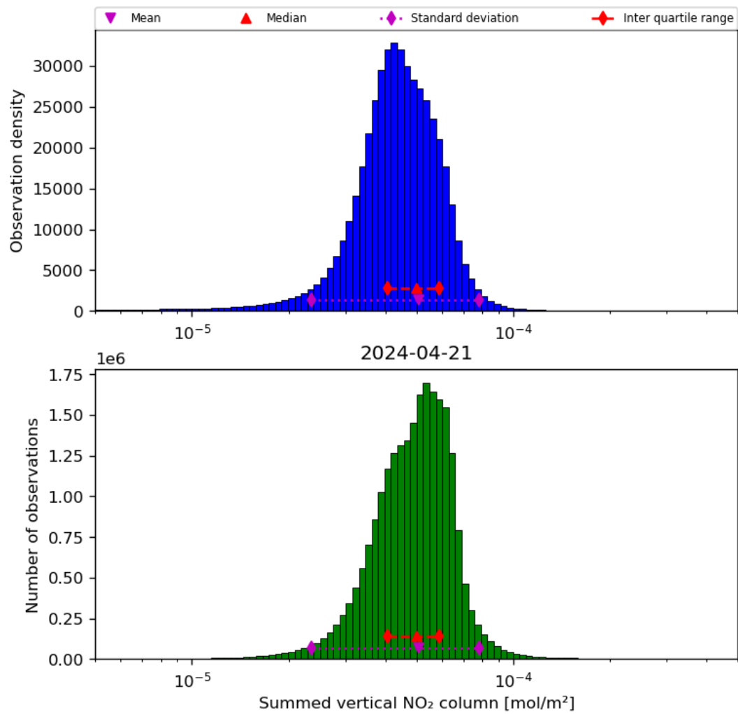
Figure 40: Histogram of “Summed vertical NO 2 column” for 2024-04-21 to 2024-04-22
