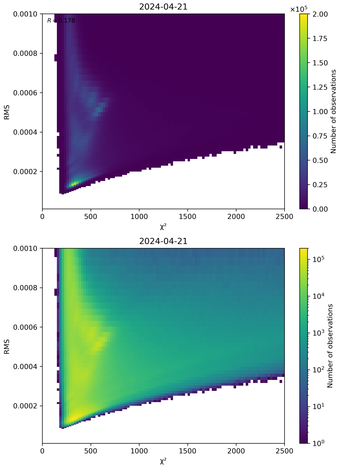
Figure 82: Scatter density plot of “ \chi^2 ” against “RMS” for 2024-04-21 to 2024-04-22.
