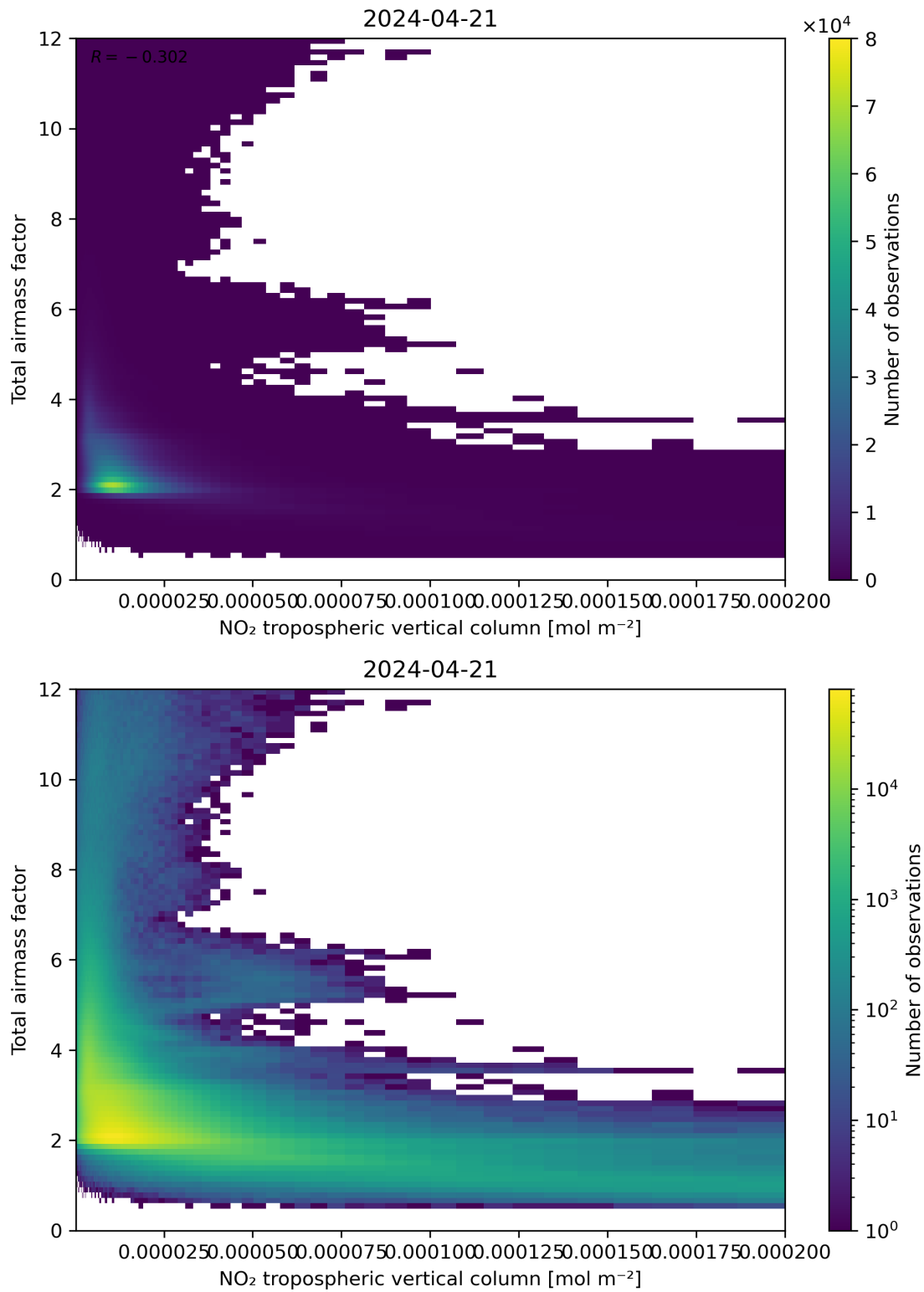
Figure 122: Scatter density plot of “NO 2 tropospheric vertical column” against “Total air mass factor” for 2024-04-21 to 2024-04-22.
