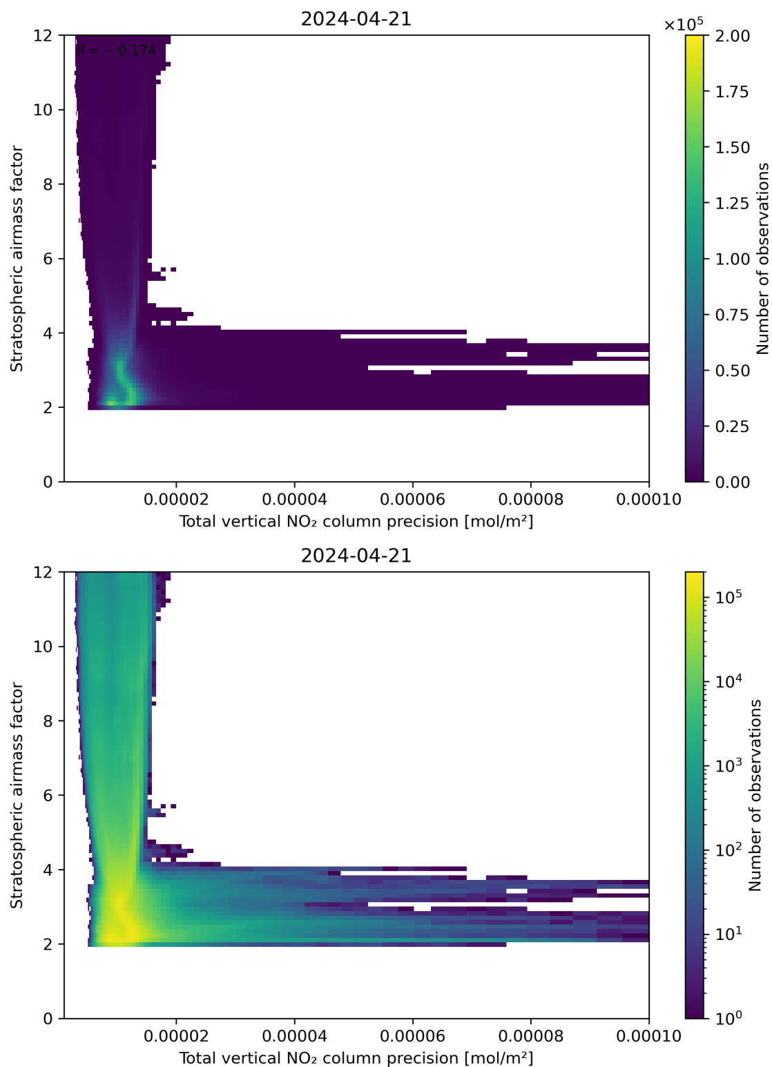
Figure 115: Scatter density plot of “Total vertical NO 2 column precision” against “Stratospheric air mass factor” for 2024-04-21 to 2024-04-22.
