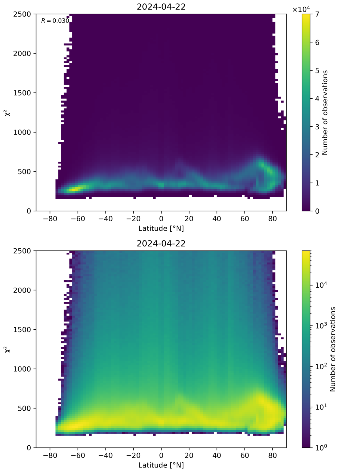
Figure 86: Scatter density plot of “Latitude” against “ \chi^2 ” for 2024-04-21 to 2024-04-23.
