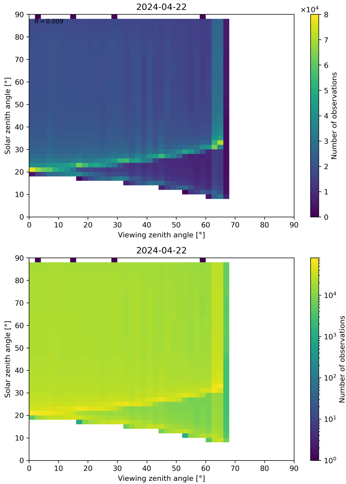
Figure 172: Scatter density plot of “Viewing zenith angle” against “Solar zenith angle” for 2024-04-21 to 2024-04-23.
