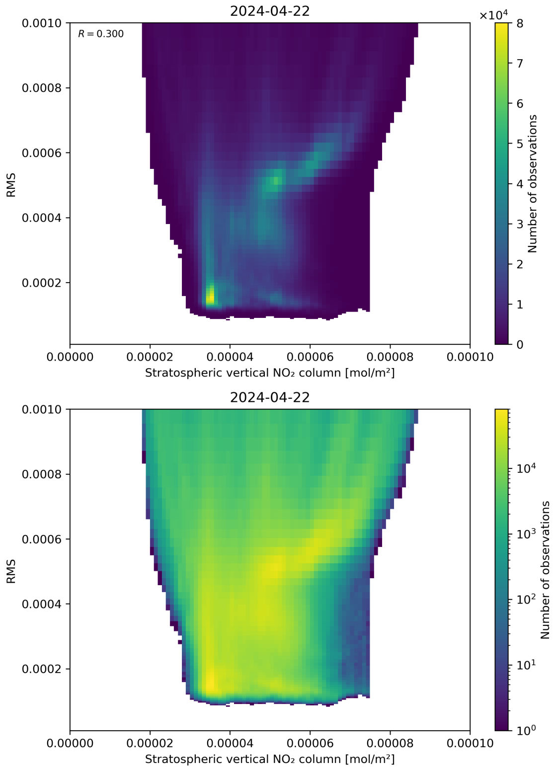
Figure 102: Scatter density plot of “Stratospheric vertical NO 2 column” against “RMS” for 2024-04-21 to 2024-04-23.
