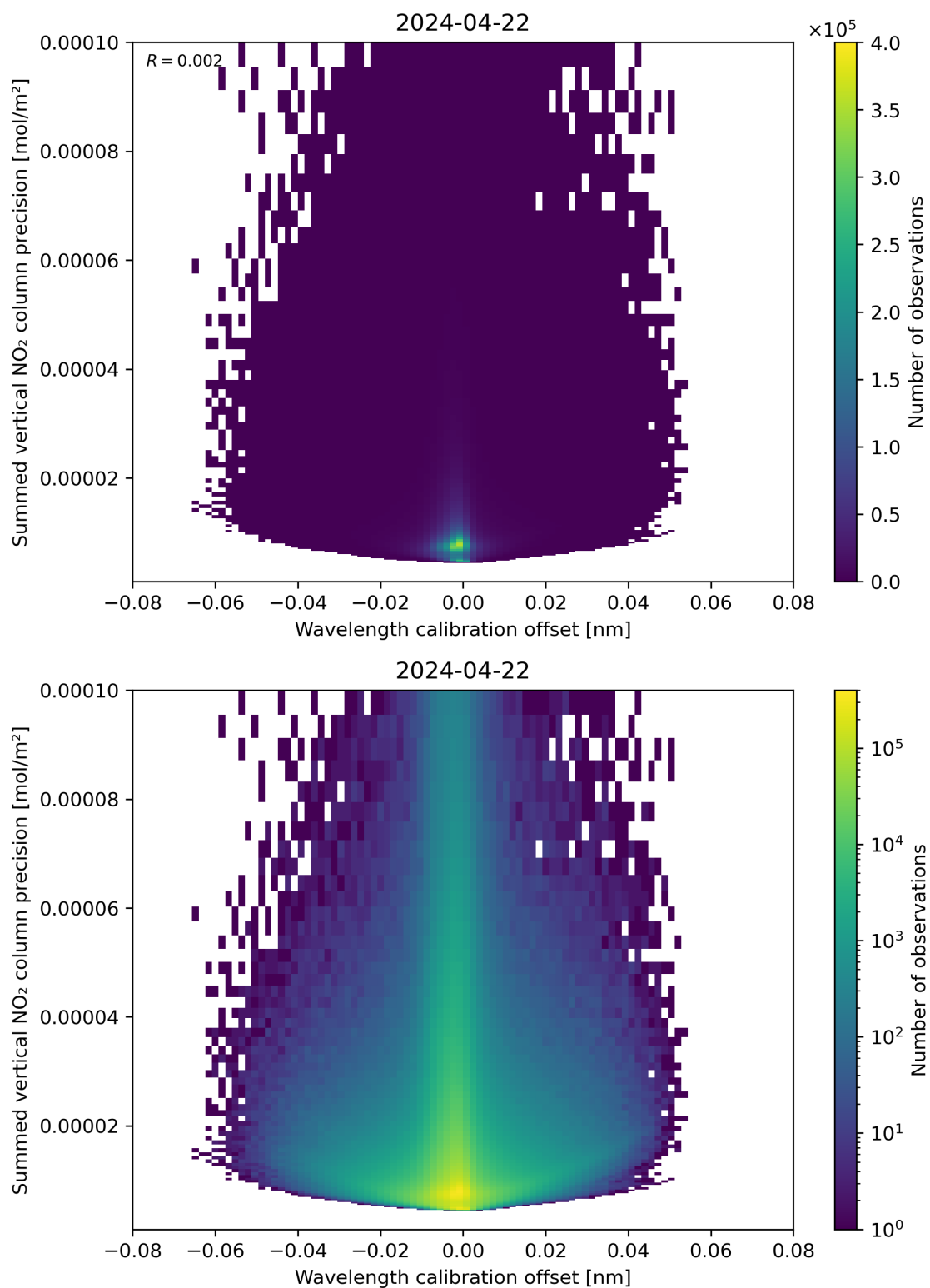
Figure 178: Scatter density plot of “Wavelength calibration offset” against “Summed vertical NO 2 column precision” for 2024-04-21 to 2024-04-23.
