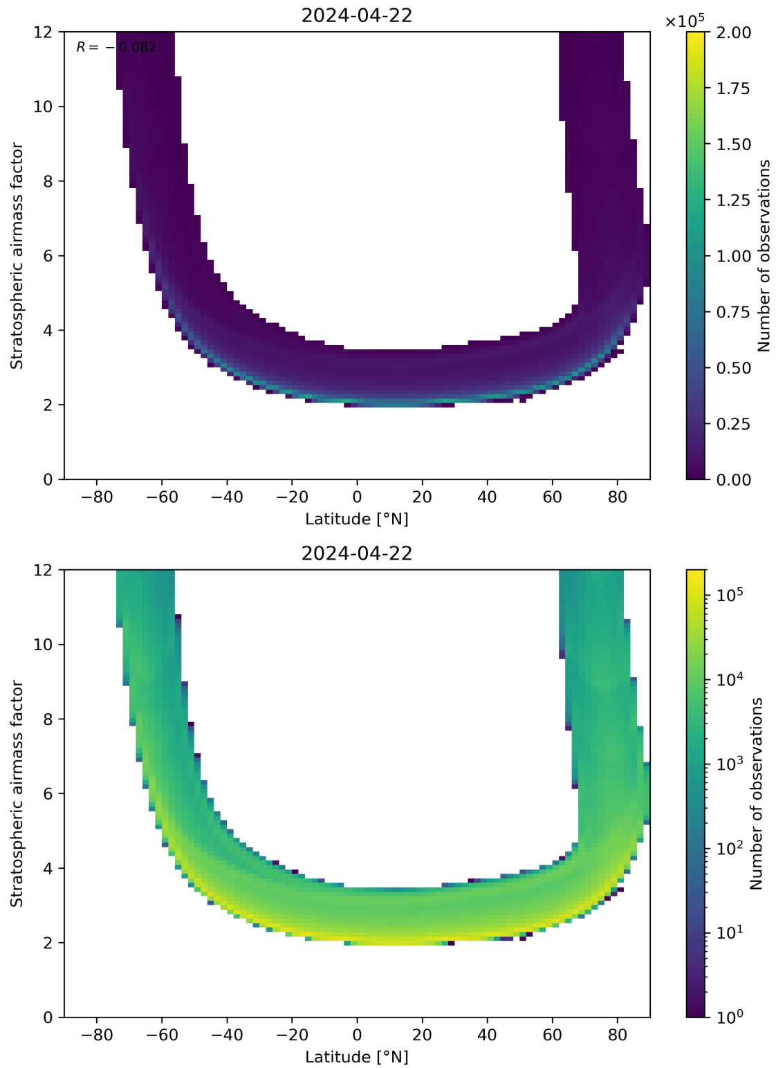
Figure 83: Scatter density plot of “Latitude” against “Stratospheric air mass factor” for 2024-04-21 to 2024-04-23.
