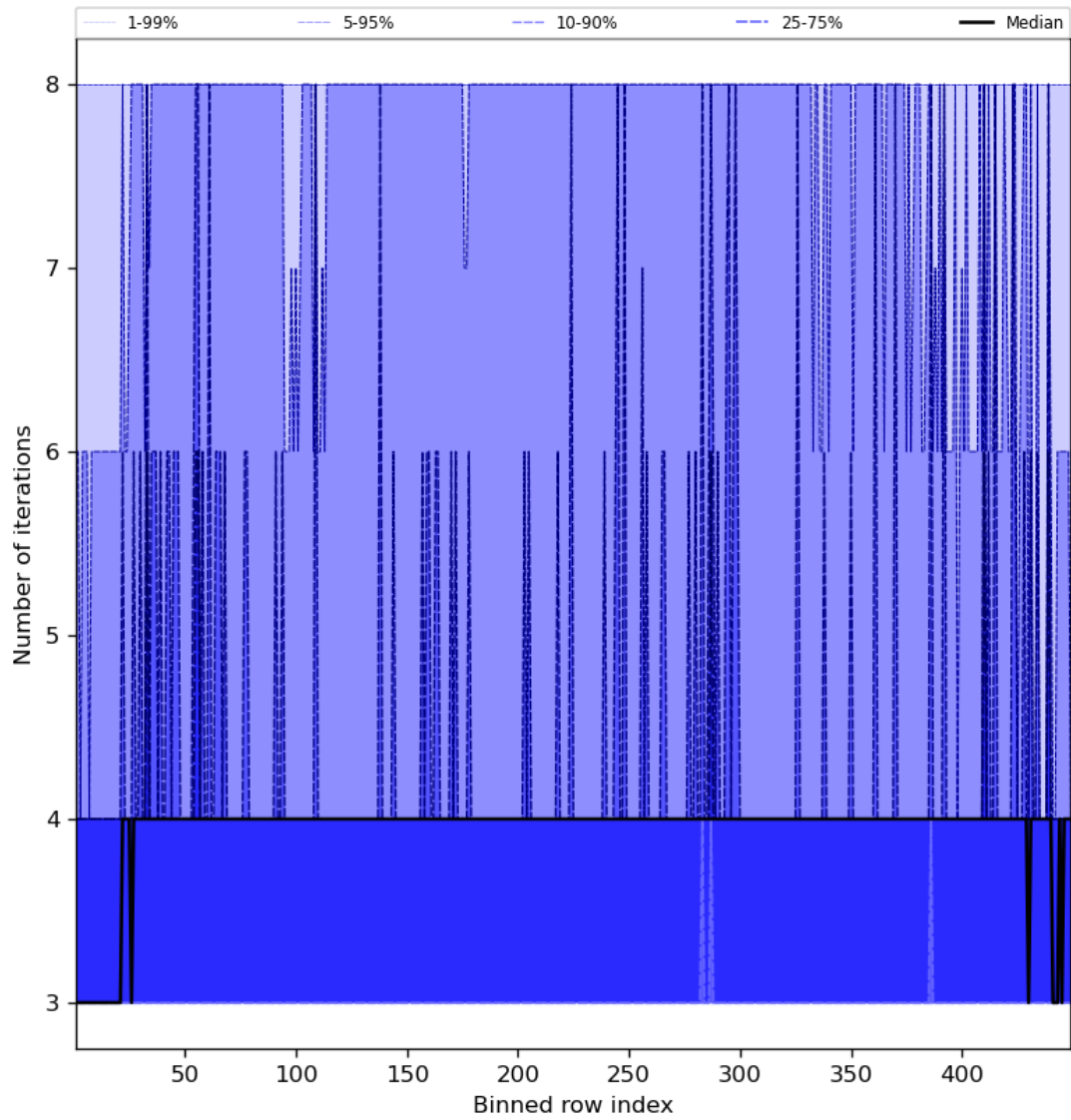
Figure 51: Along track statistics of “Number of iterations” for 2024-04-21 to 2024-04-23
