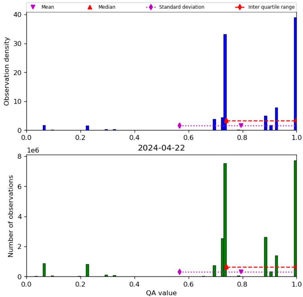
Figure 28: Histogram of “QA value” for 2024-04-21 to 2024-04-23
