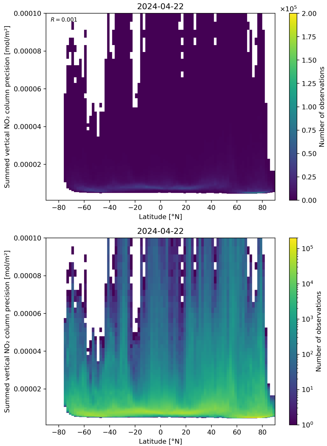
Figure 89: Scatter density plot of “Latitude” against “Summed vertical NO 2 column precision” for 2024-04-21 to 2024-04-23.
