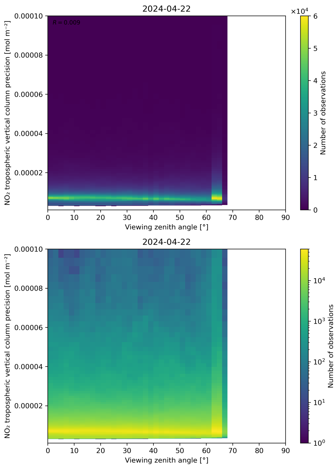
Figure 170: Scatter density plot of “Viewing zenith angle” against “NO 2 tropospheric vertical column precision” for 2024-04-21 to 2024-04-23.
