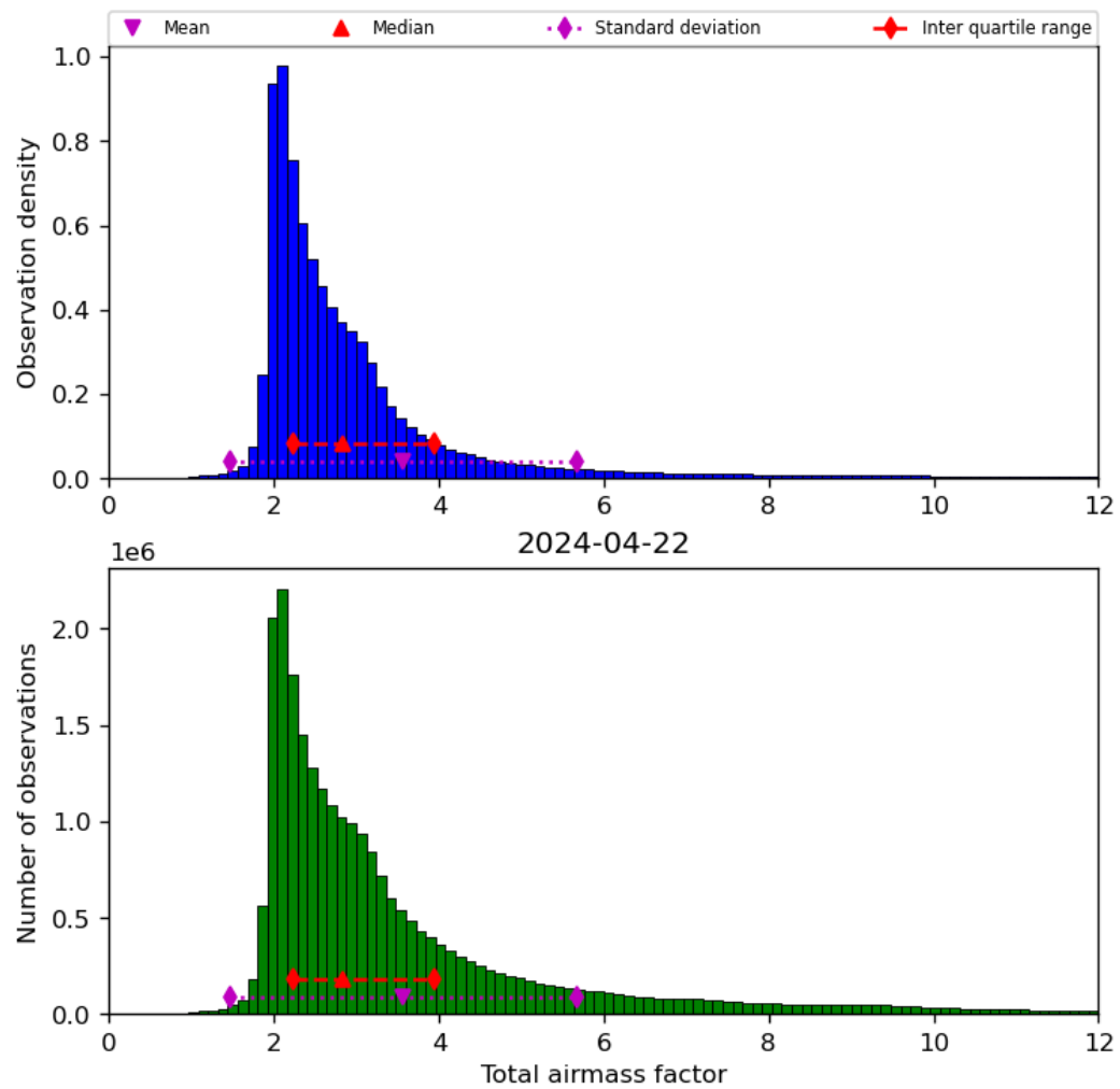
Figure 32: Histogram of “Total airmass factor” for 2024-04-21 to 2024-04-23
