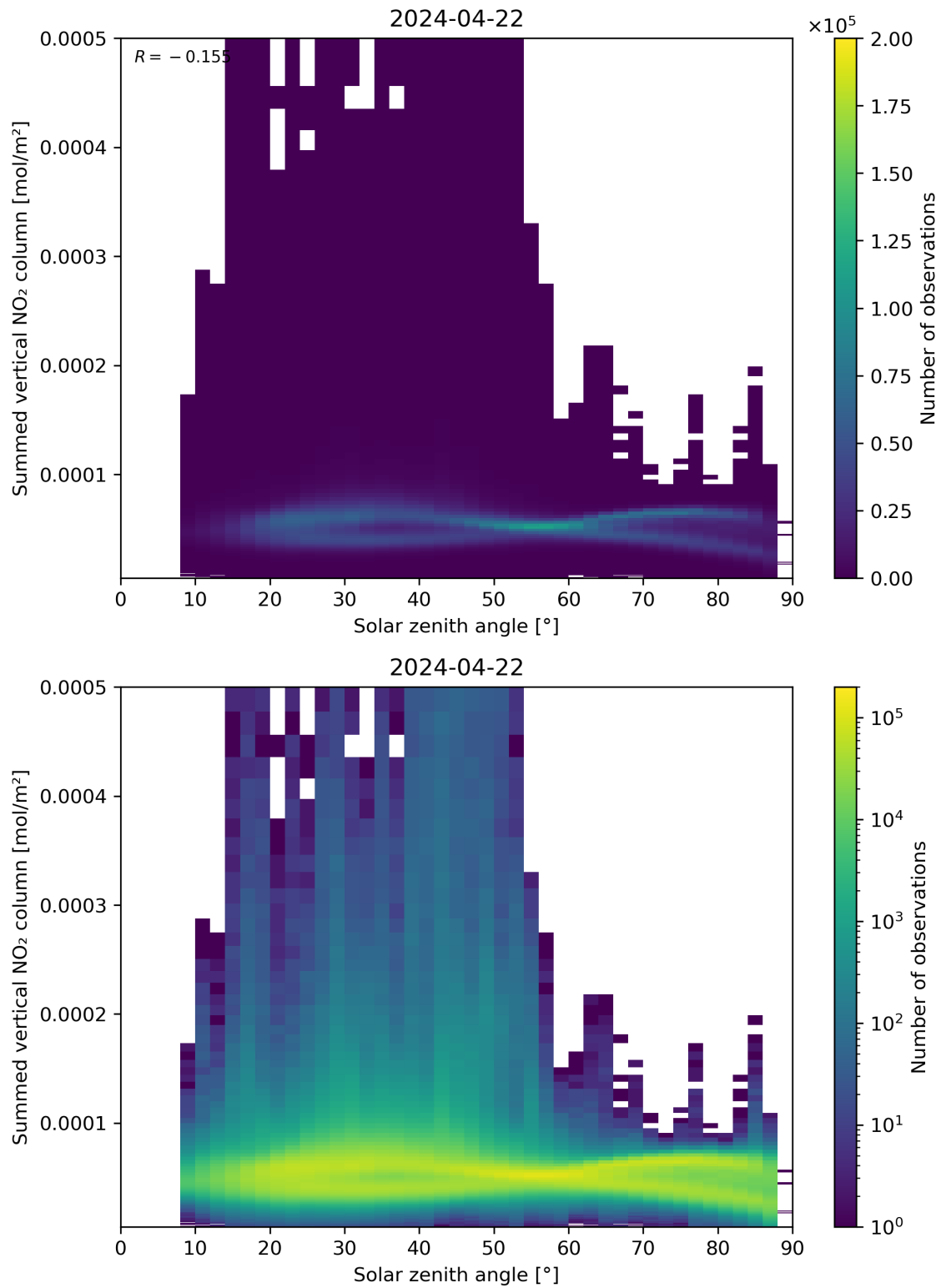
Figure 151: Scatter density plot of “Solar zenith angle” against “Summed vertical NO 2 column” for 2024-04-21 to 2024-04-23.
