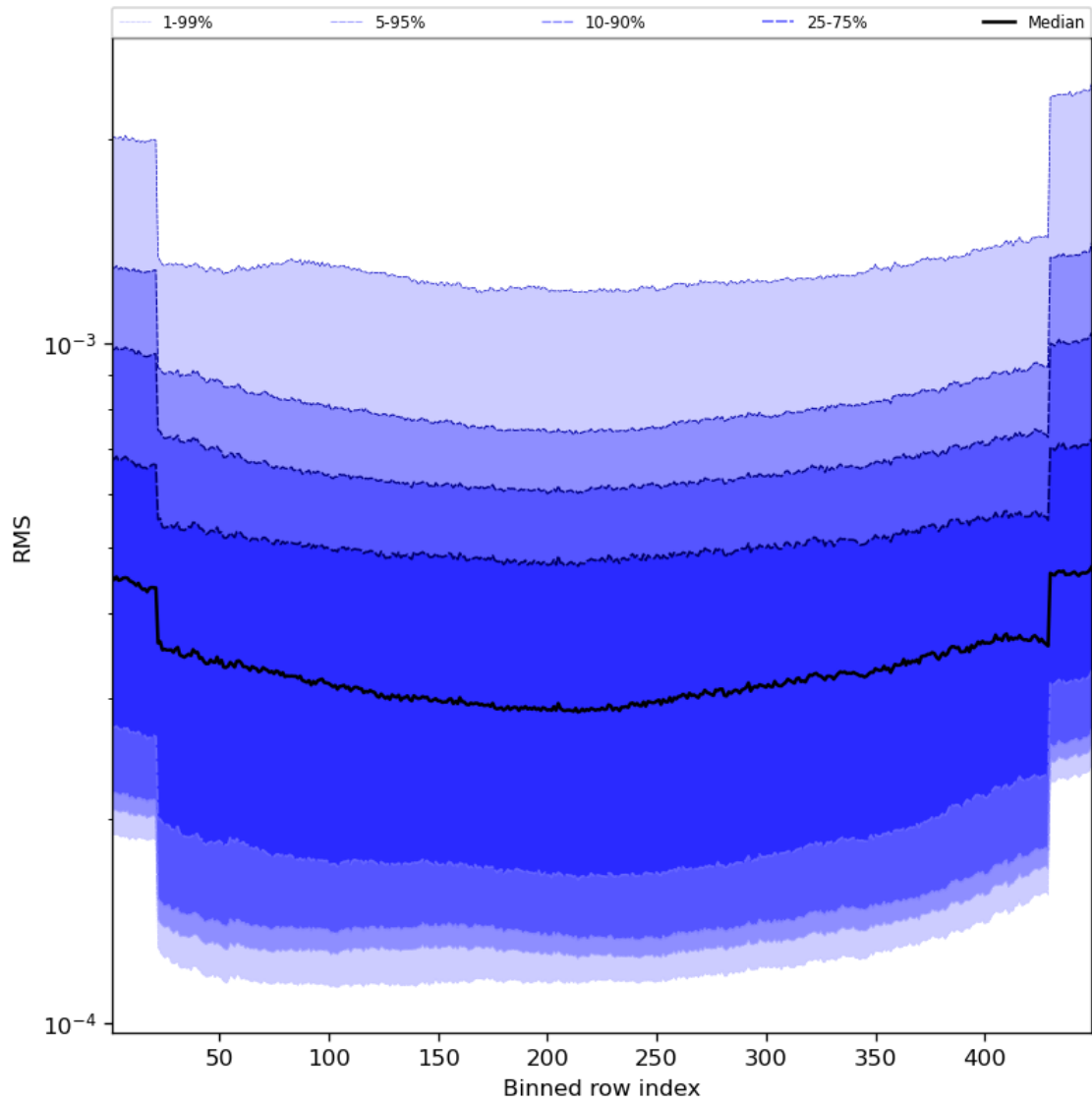
Figure 60: Along track statistics of “RMS” for 2024-04-21 to 2024-04-23
