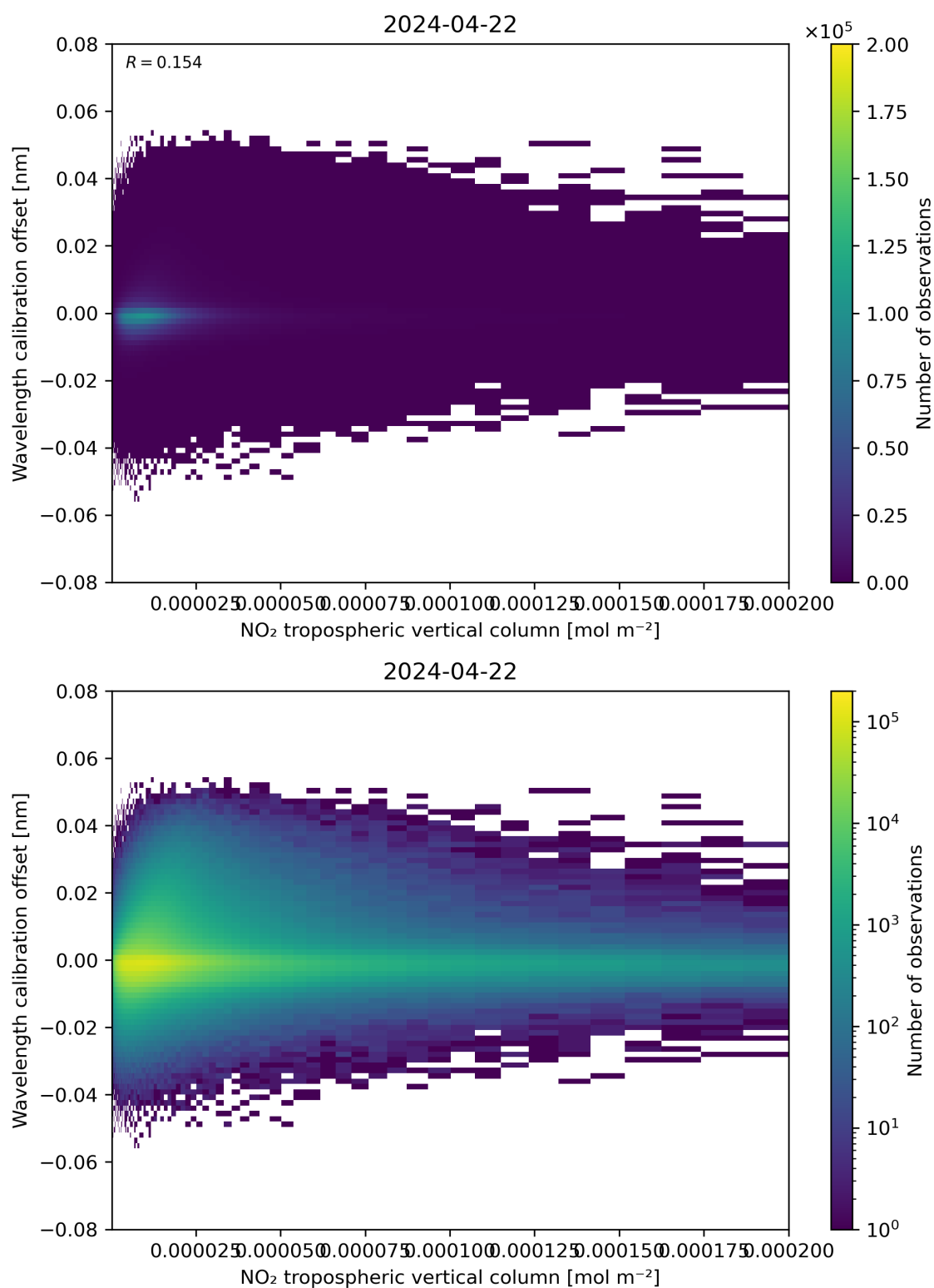
Figure 143: Scatter density plot of “NO 2 tropospheric vertical column” against “Wavelength calibration offset” for 2024-04-21 to 2024-04-23.
