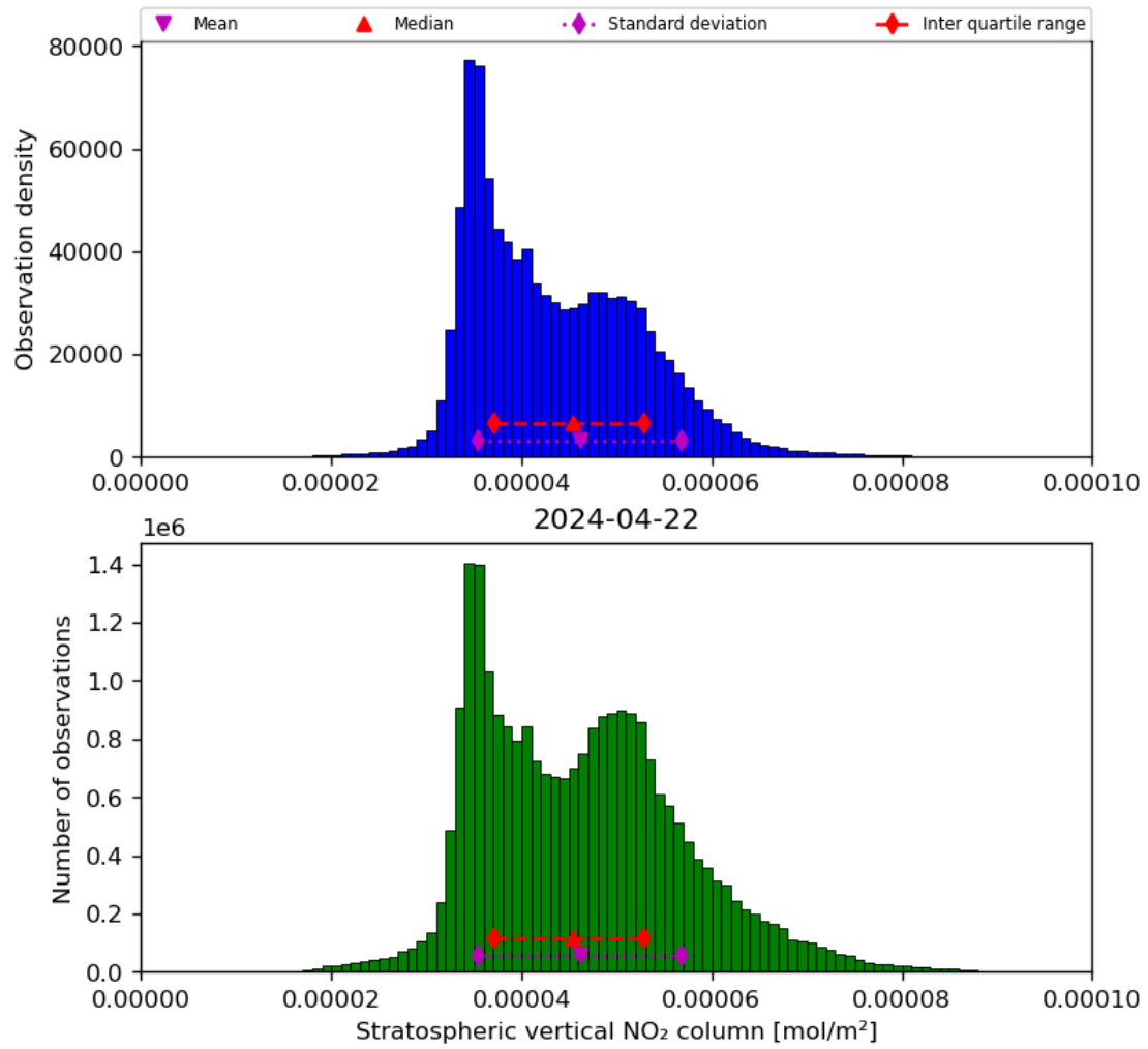
Figure 36: Histogram of “Stratospheric vertical NO 2 column” for 2024-04-21 to 2024-04-23
