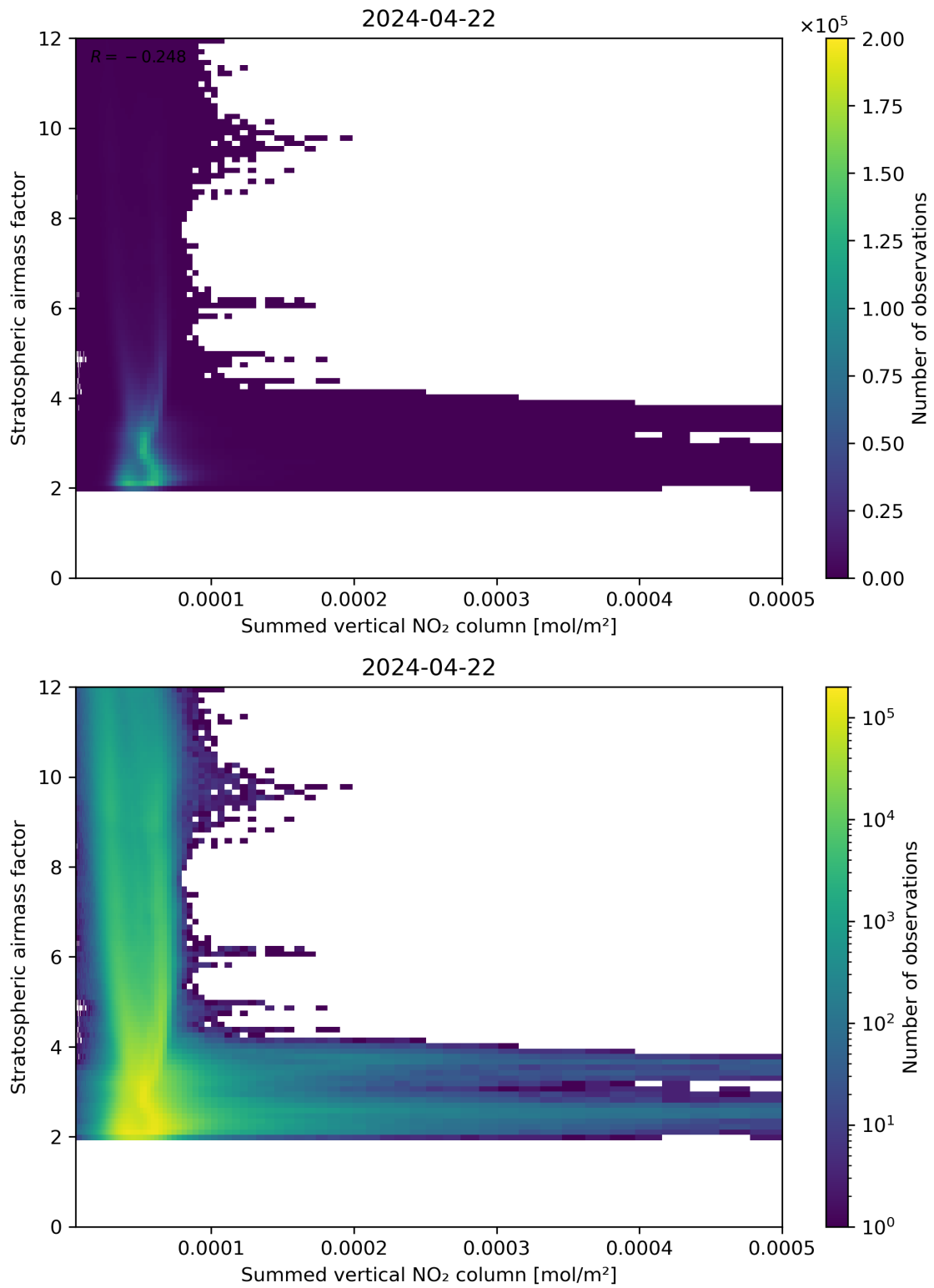
Figure 103: Scatter density plot of “Summed vertical NO 2 column” against “Stratospheric air mass factor” for 2024-04-21 to 2024-04-23.
