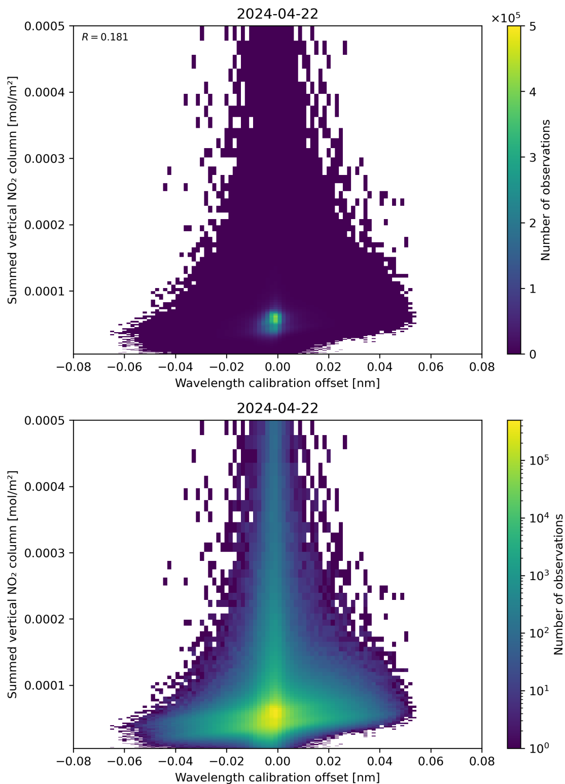
Figure 177: Scatter density plot of “Wavelength calibration offset” against “Summed vertical NO 2 column” for 2024-04-21 to 2024-04-23.
