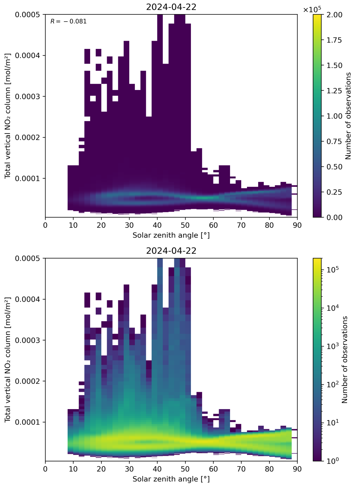
Figure 153: Scatter density plot of “Solar zenith angle” against “Total vertical NO 2 column” for 2024-04-21 to 2024-04-23.
