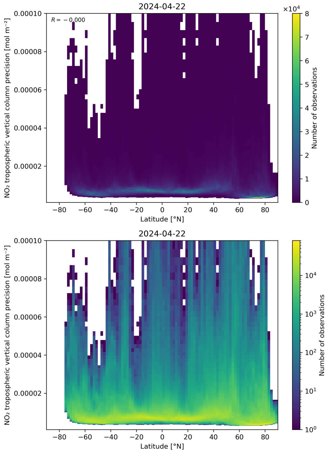
Figure 93: Scatter density plot of “Latitude” against “NO 2 tropospheric vertical column precision” for 2024-04-21 to 2024-04-23.
