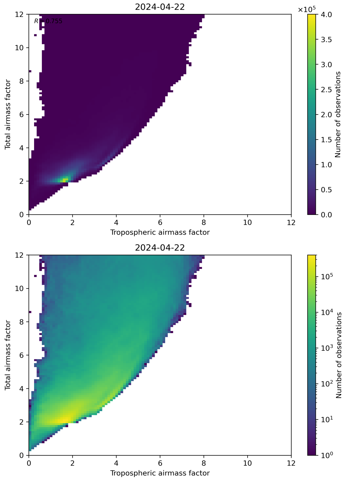
Figure 72: Scatter density plot of “Tropospheric airmass factor” against “Total airmass factor” for 2024-04-21 to 2024-04-23.
