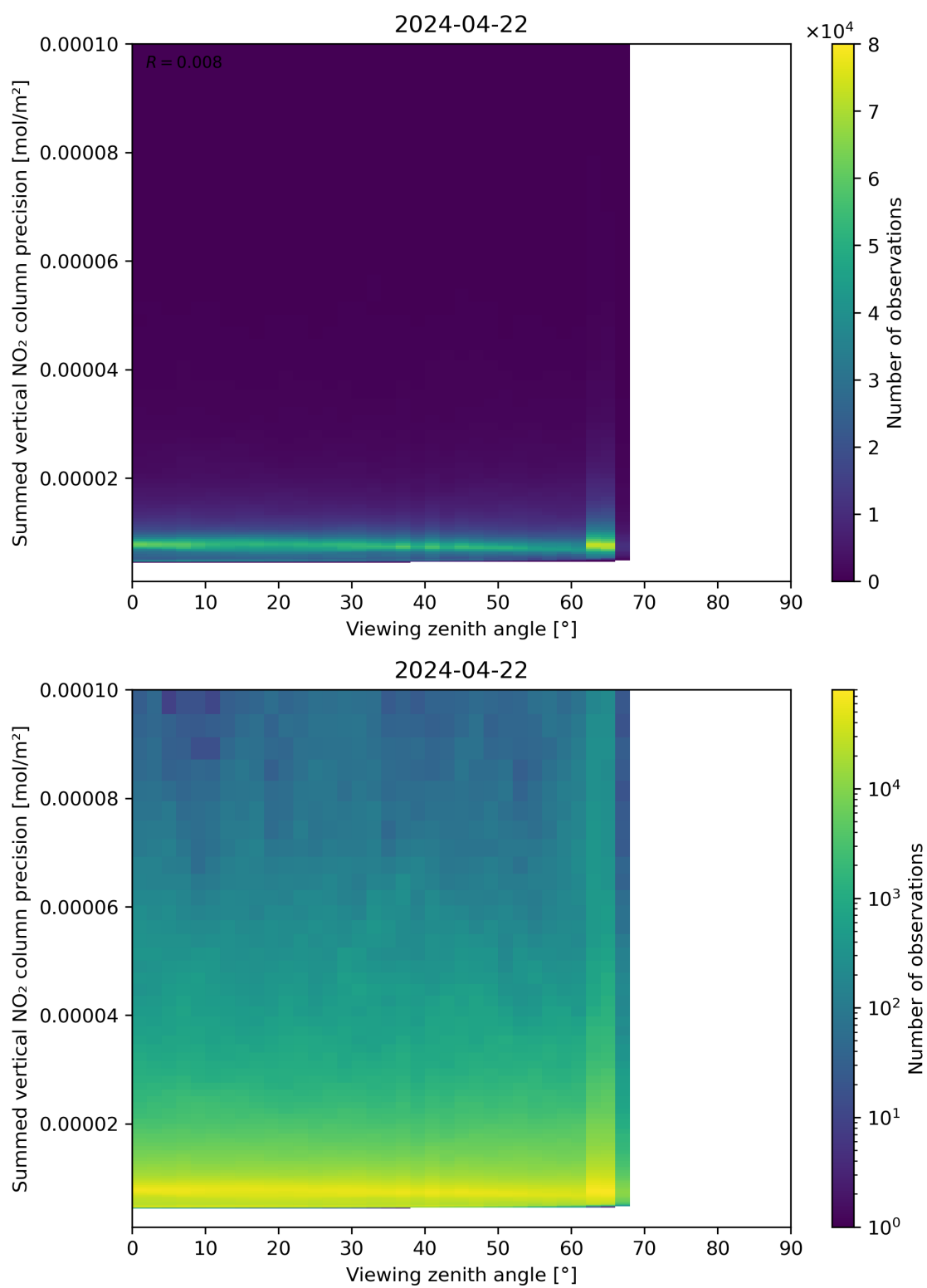
Figure 166: Scatter density plot of “Viewing zenith angle” against “Summed vertical NO 2 column precision” for 2024-04-21 to 2024-04-23.
