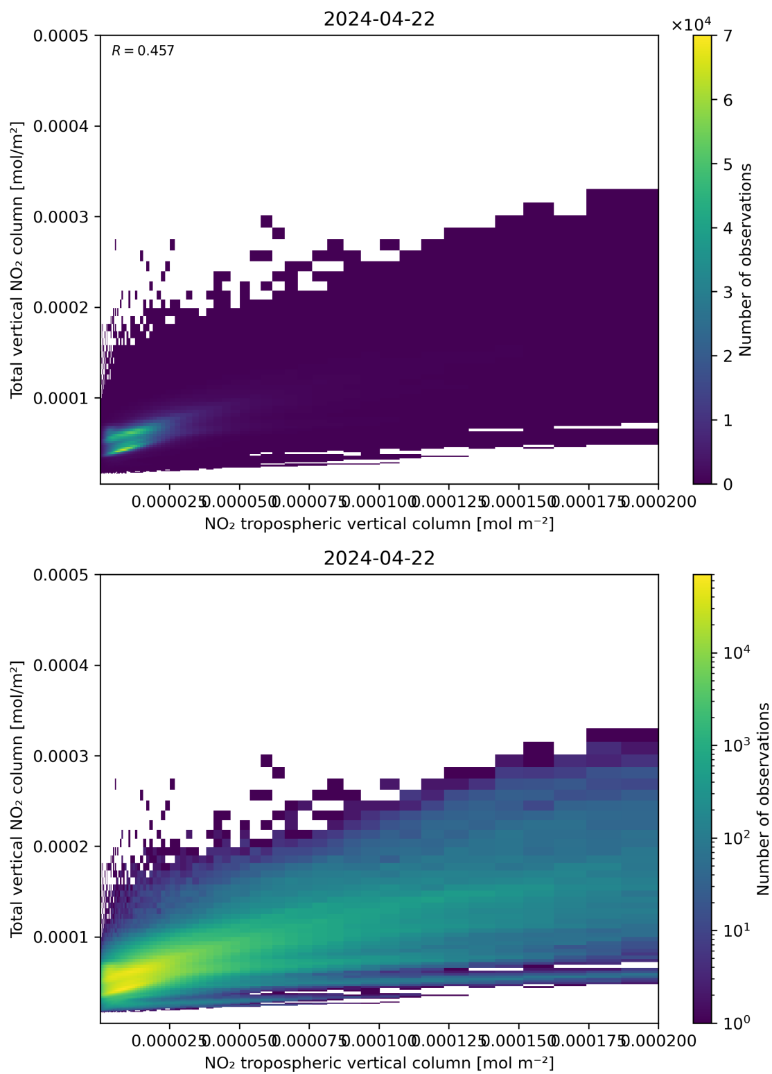
Figure 128: Scatter density plot of “NO 2 tropospheric vertical column” against “Total vertical NO 2 column” for 2024-04-21 to 2024-04-23.
