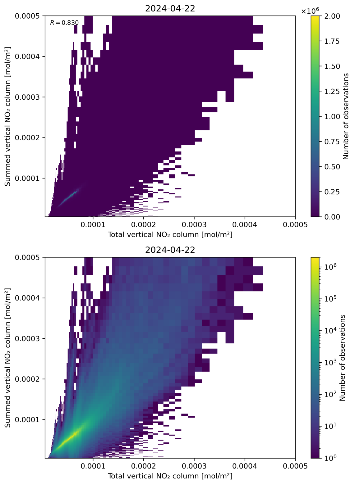
Figure 112: Scatter density plot of “Total vertical NO 2 column” against “Summed vertical NO 2 column” for 2024-04-21 to 2024-04-23.
