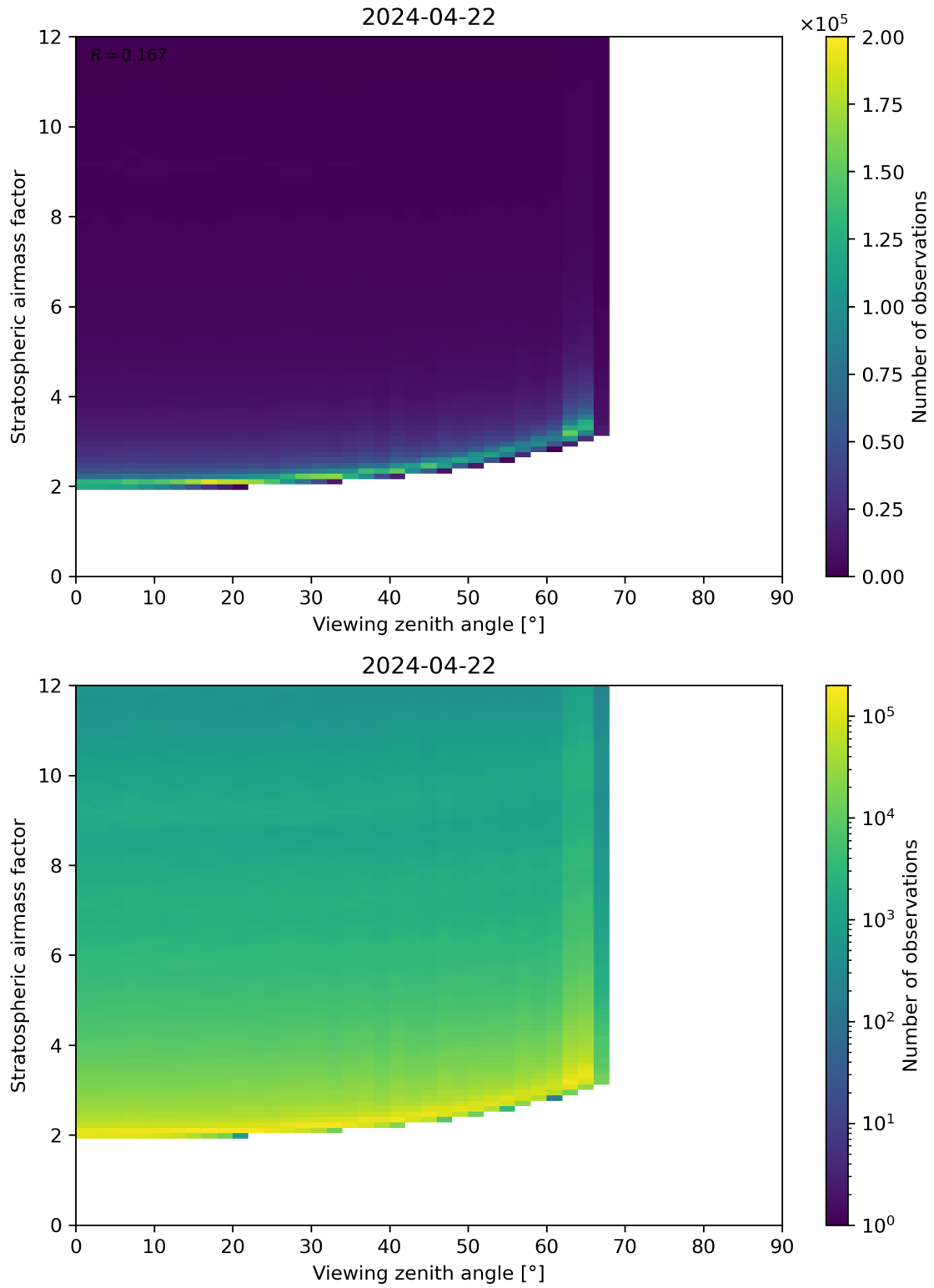
Figure 159: Scatter density plot of “Viewing zenith angle” against “Stratospheric airmass factor” for 2024-04-21 to 2024-04-23.
