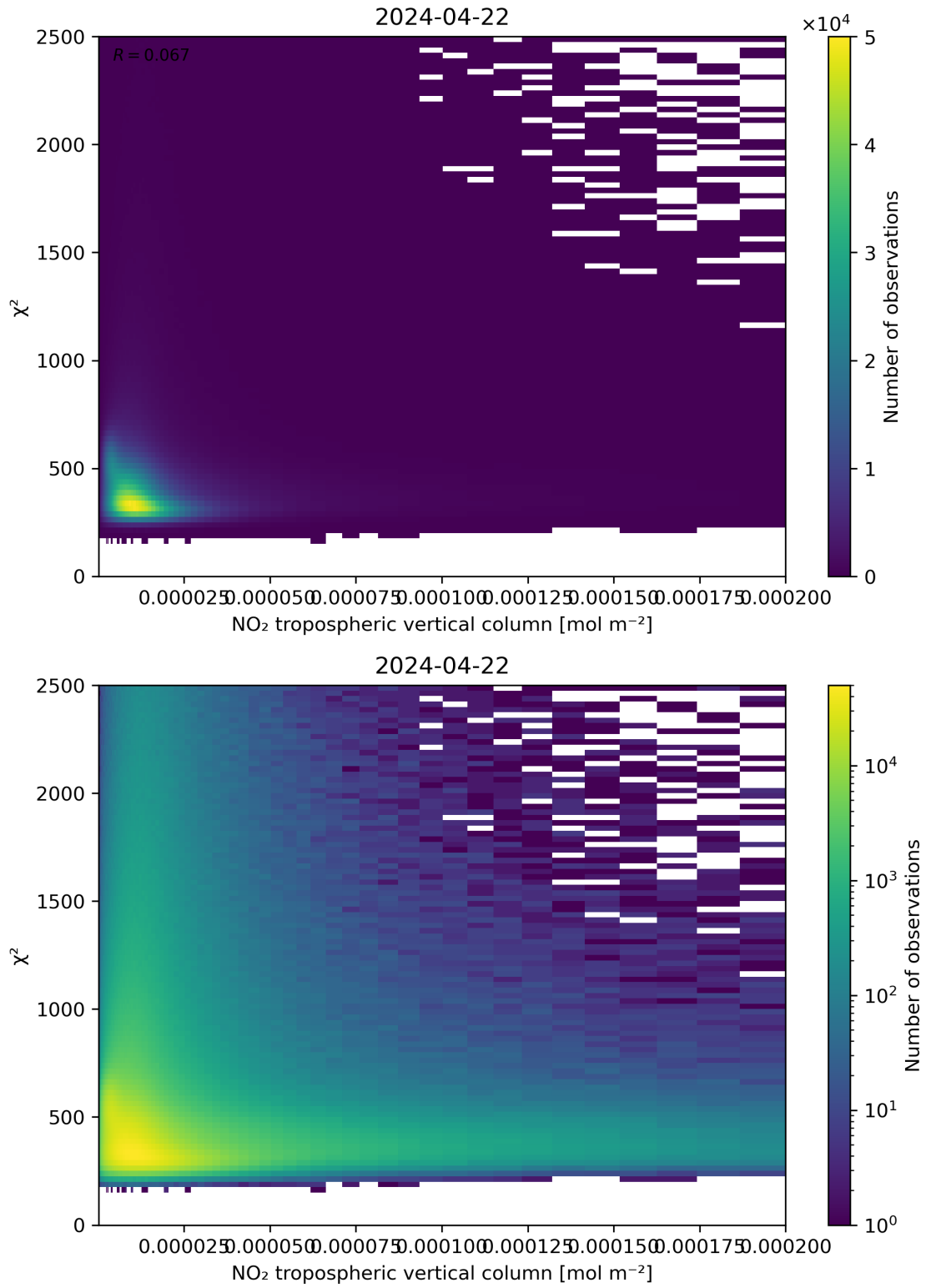
Figure 124: Scatter density plot of “NO 2 tropospheric vertical column” against “ \chi^2 ” for 2024-04-21 to 2024-04-23.
