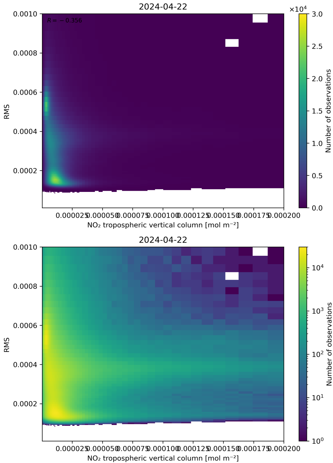
Figure 142: Scatter density plot of “NO 2 tropospheric vertical column” against “RMS” for 2024-04-21 to 2024-04-23.
