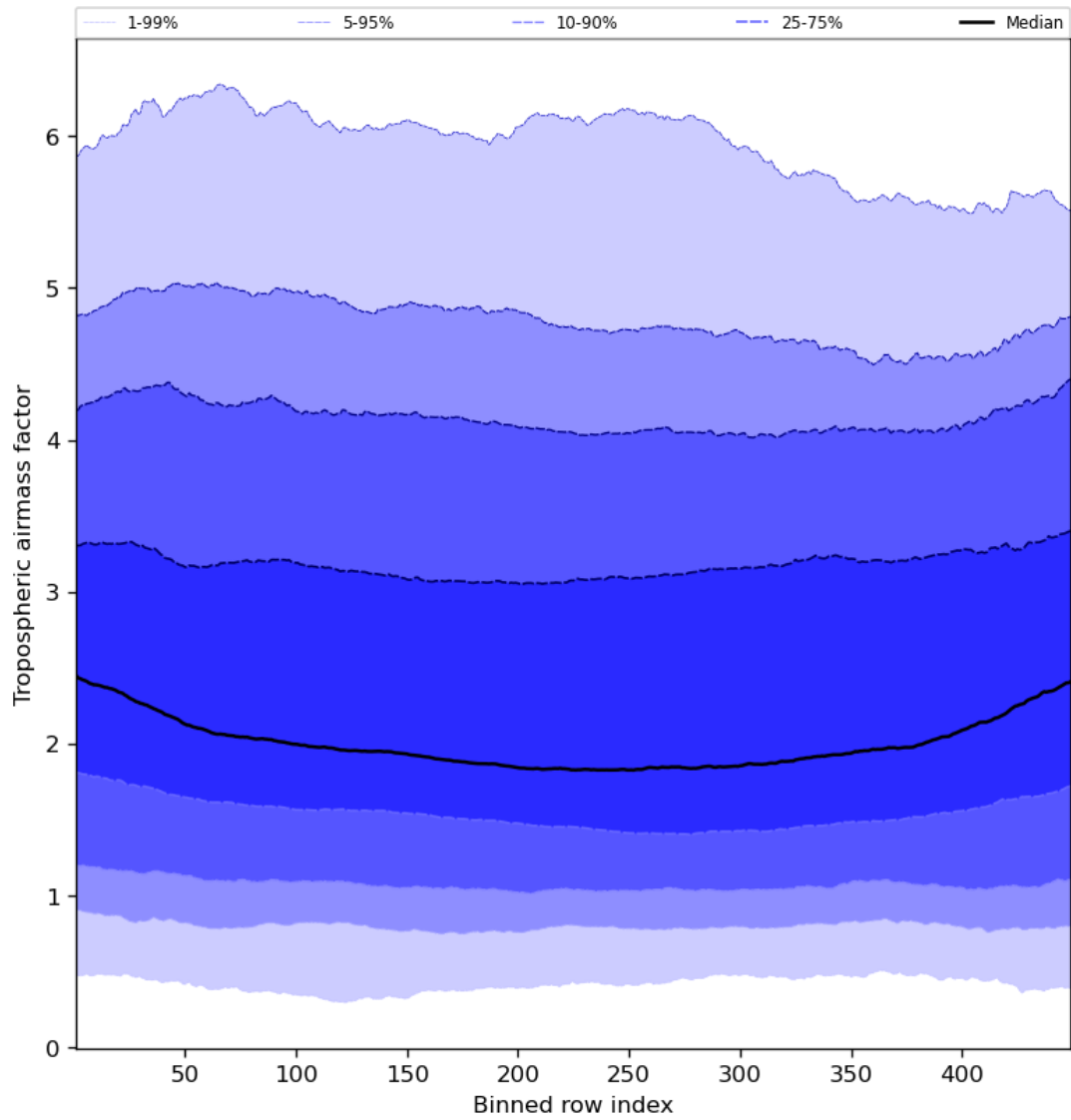
Figure 48: Along track statistics of “Tropospheric airmass factor” for 2024-04-21 to 2024-04-23
