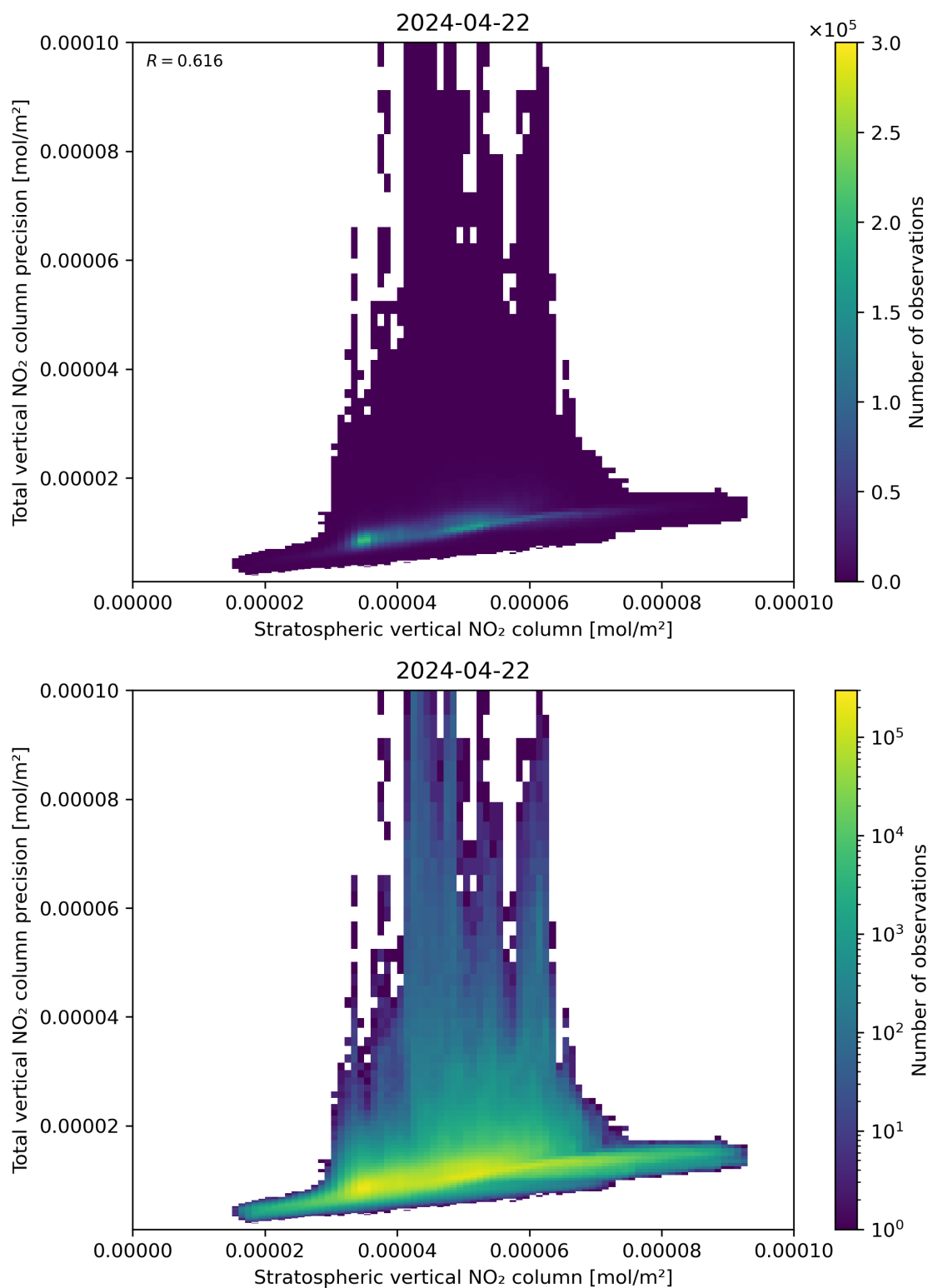
Figure 101: Scatter density plot of “Stratospheric vertical NO 2 column” against “Total vertical NO 2 column precision” for 2024-04-21 to 2024-04-23.
