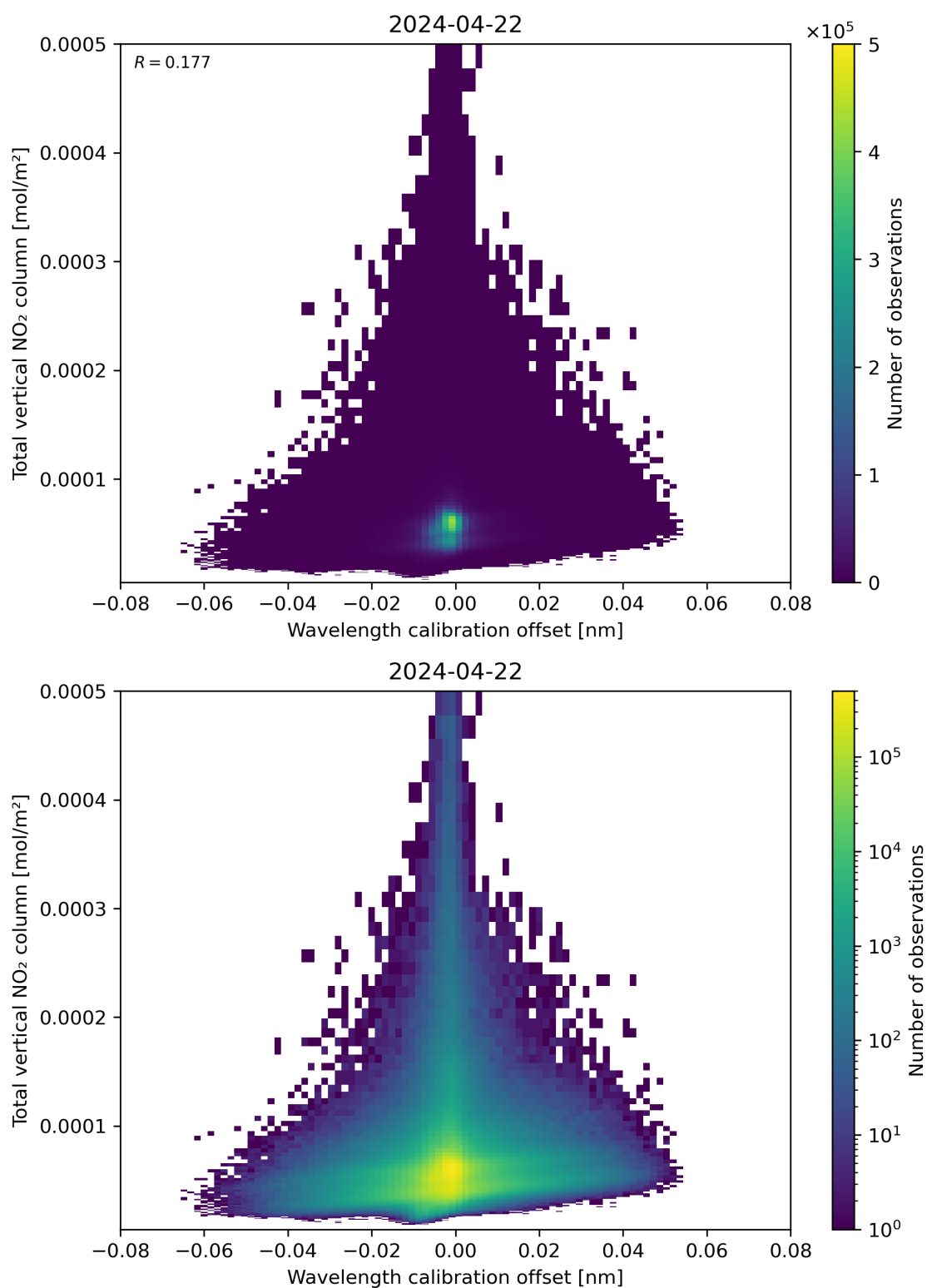
Figure 179: Scatter density plot of “Wavelength calibration offset” against “Total vertical NO 2 column” for 2024-04-21 to 2024-04-23.
