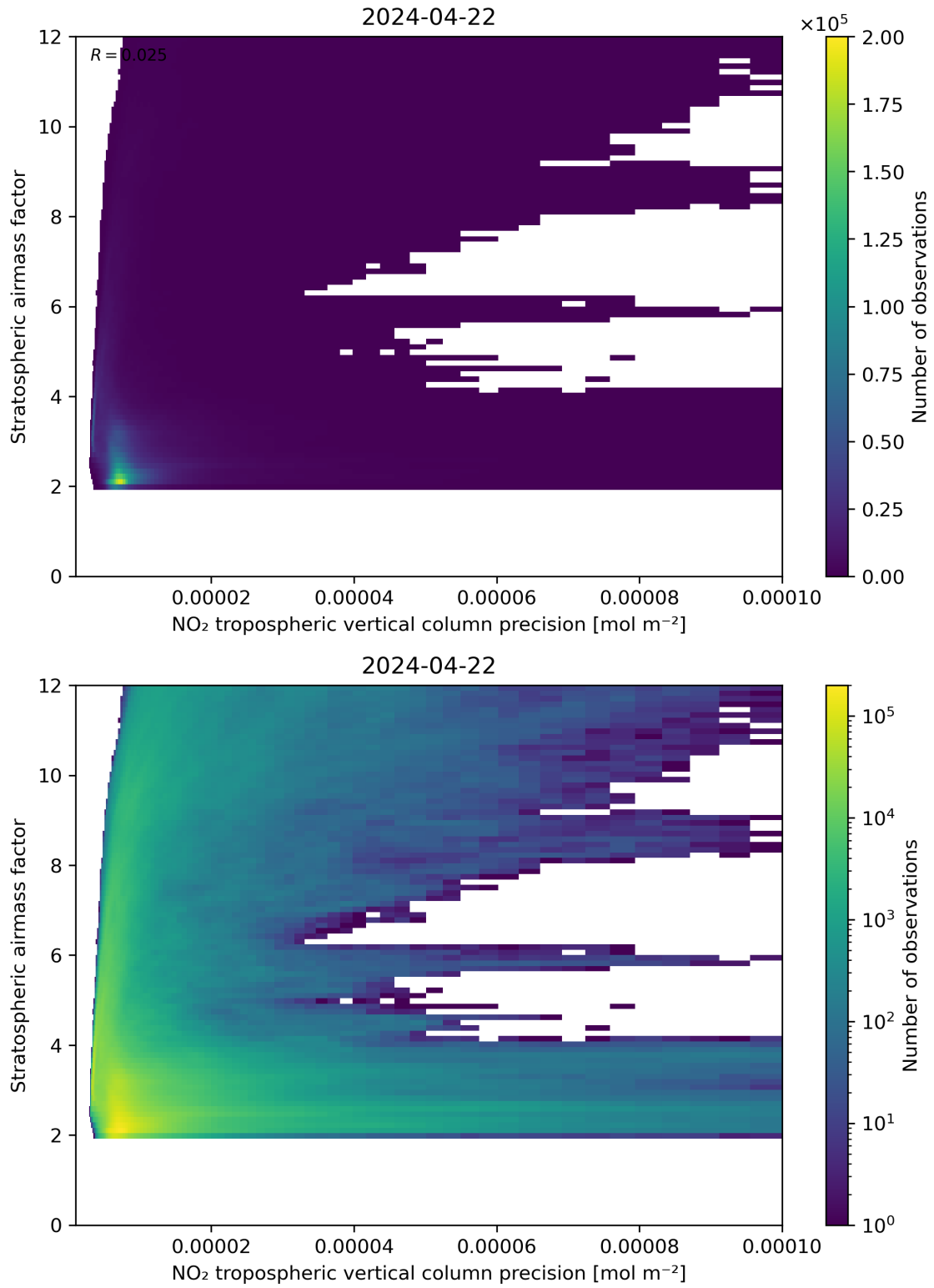
Figure 131: Scatter density plot of “NO 2 tropospheric vertical column precision” against “Stratospheric airmass factor” for 2024-04-21 to 2024-04-23.
