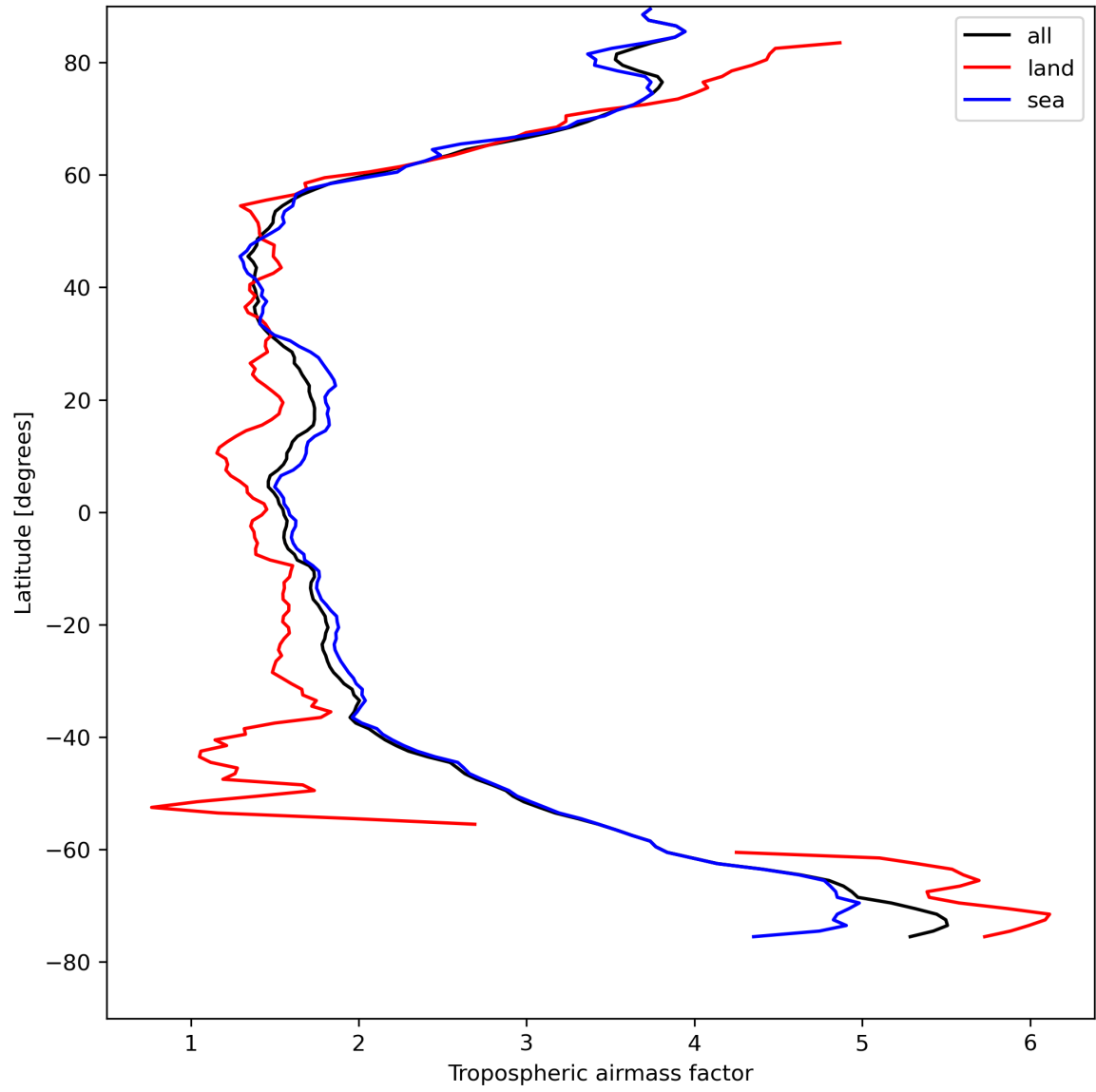
Figure 14: Zonal average of “Tropospheric airmass factor” for 2024-04-21 to 2024-04-23.
