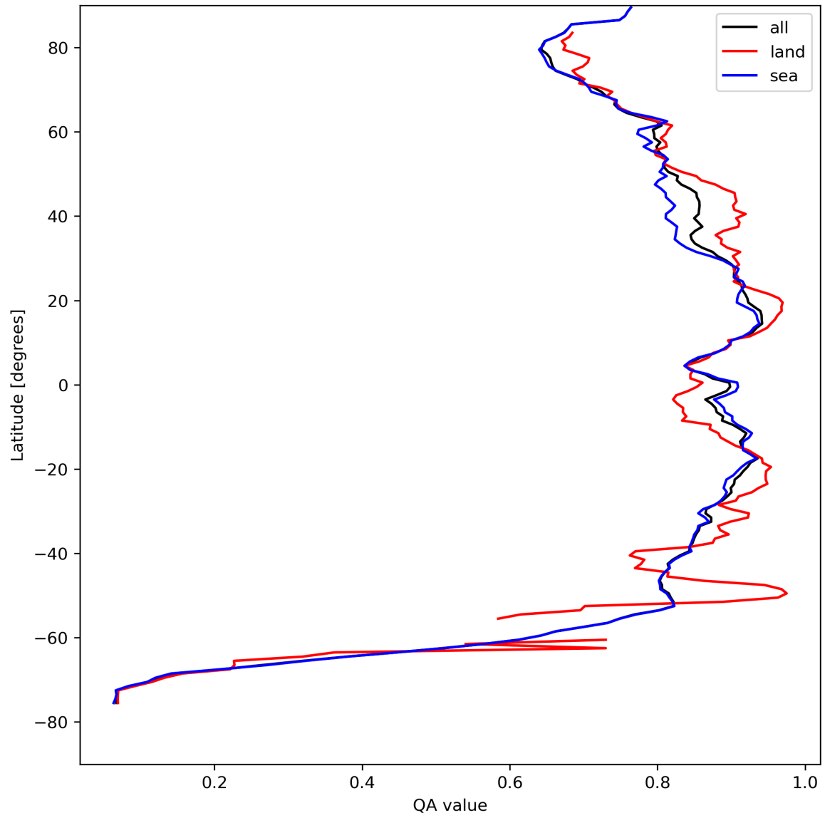
Figure 11: Zonal average of “QA value” for 2024-04-21 to 2024-04-23.
