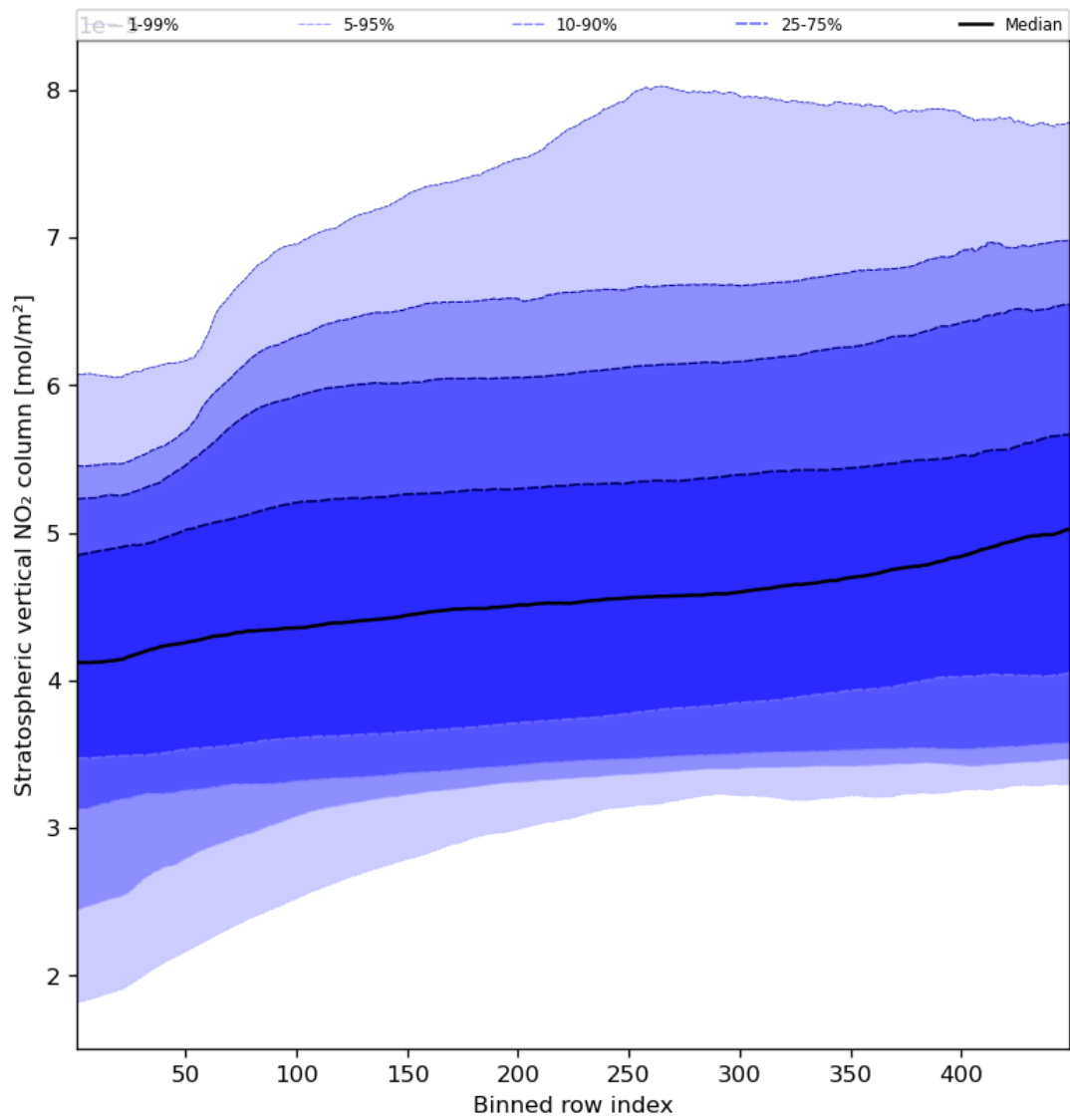
Figure 53: Along track statistics of “Stratospheric vertical NO 2 column” for 2024-04-21 to 2024-04-23
