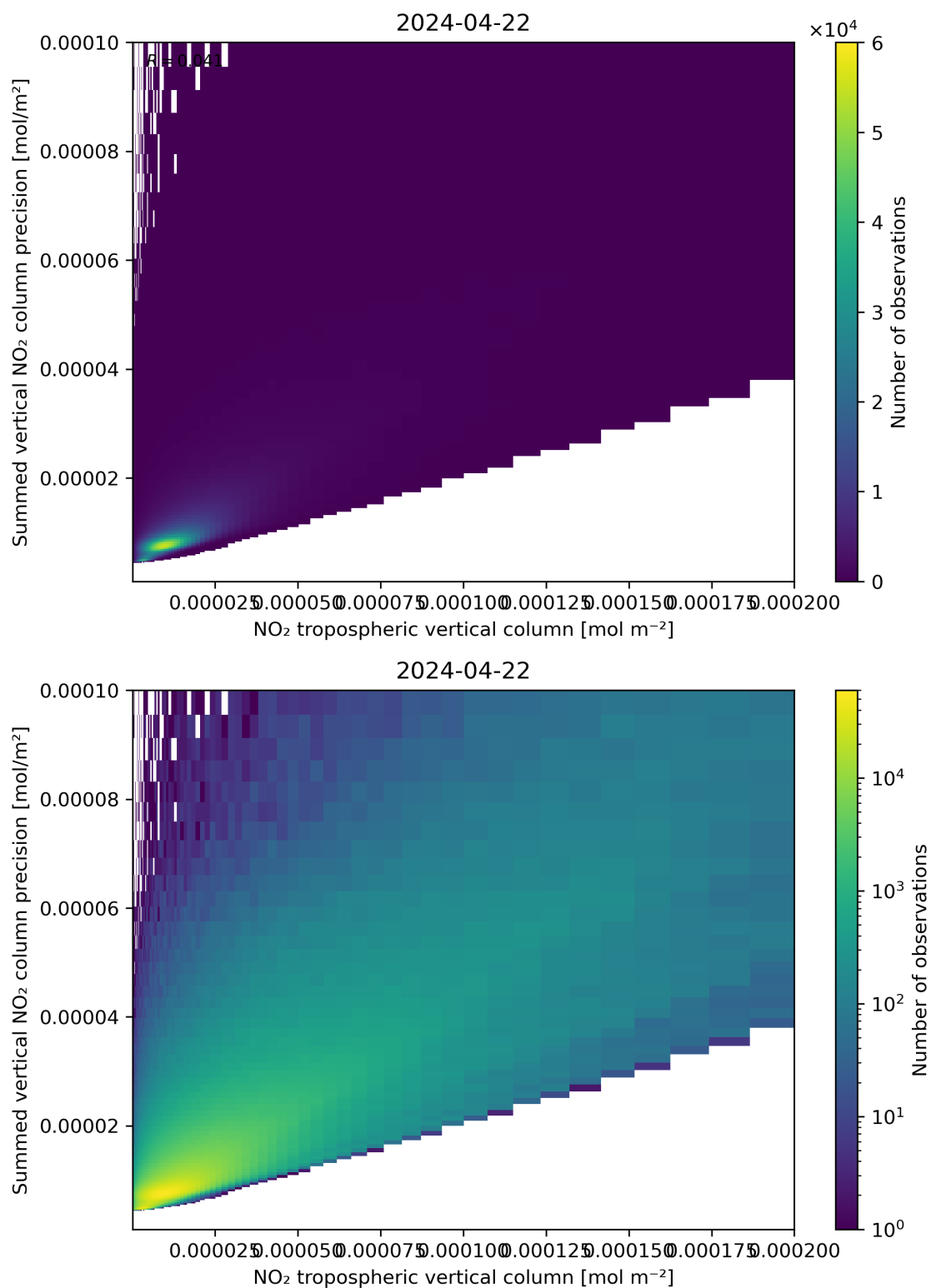
Figure 127: Scatter density plot of “NO 2 tropospheric vertical column” against “Summed vertical NO 2 column precision” for 2024-04-21 to 2024-04-23.
