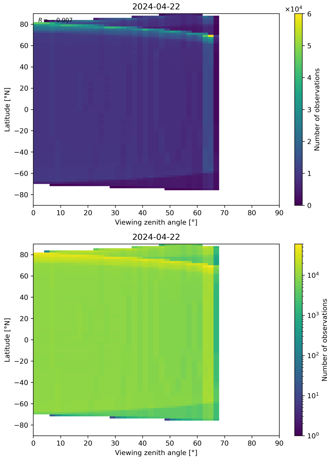
Figure 163: Scatter density plot of “Viewing zenith angle” against “Latitude” for 2024-04-21 to 2024-04-23.
