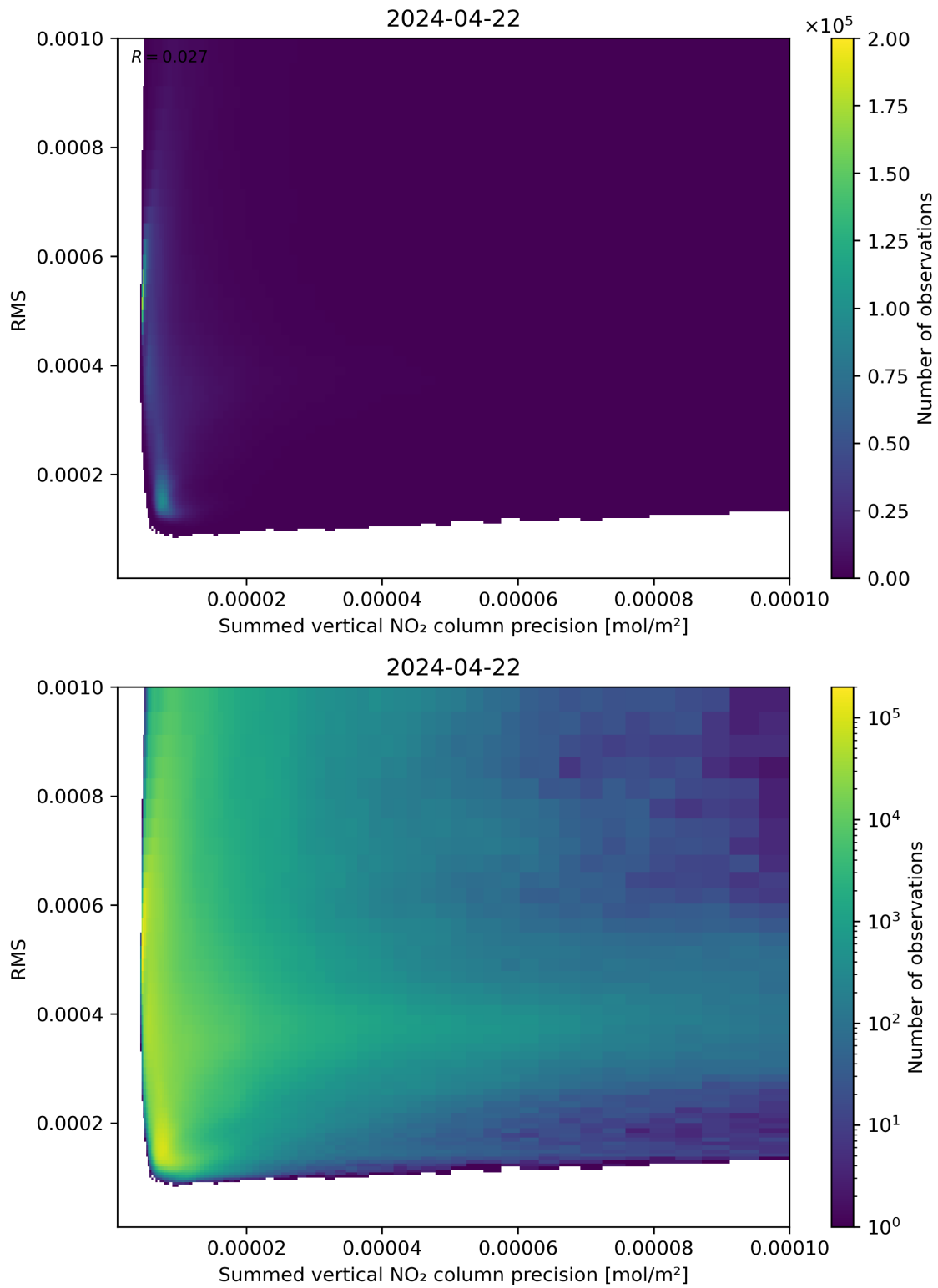
Figure 108: Scatter density plot of “Summed vertical NO 2 column precision” against “RMS” for 2024-04-21 to 2024-04-23.
