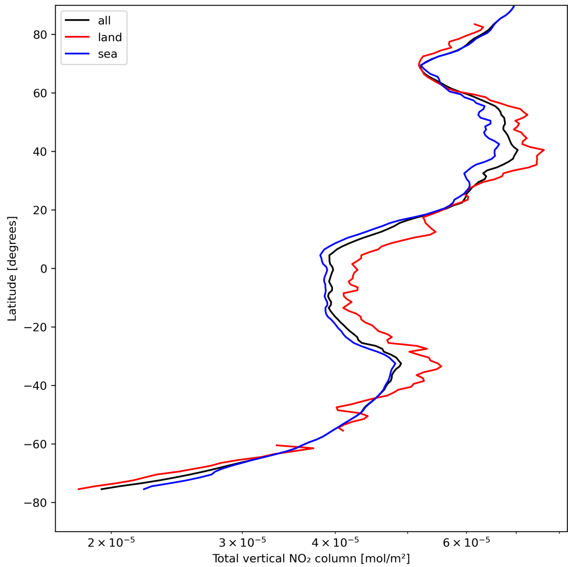
Figure 21: Zonal average of “Total vertical NO 2 column” for 2024-04-21 to 2024-04-23.
