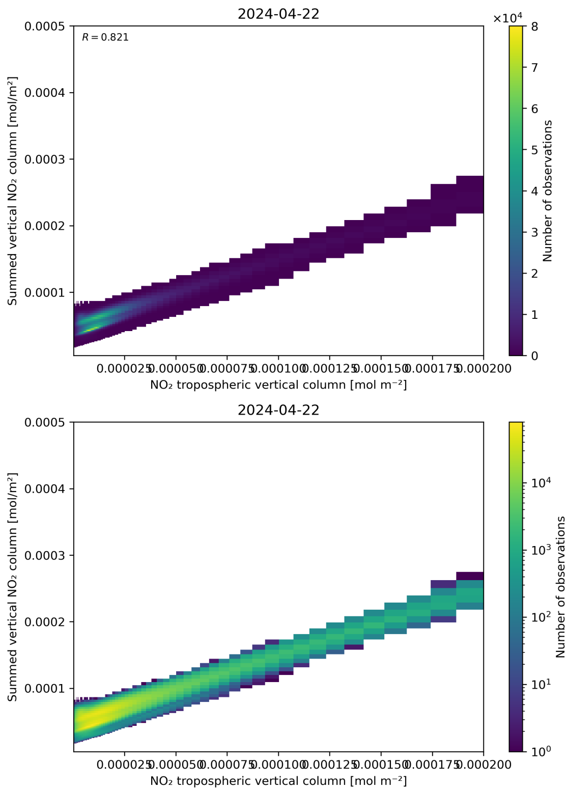
Figure 126: Scatter density plot of “NO 2 tropospheric vertical column” against “Summed vertical NO 2 column” for 2024-04-21 to 2024-04-23.
