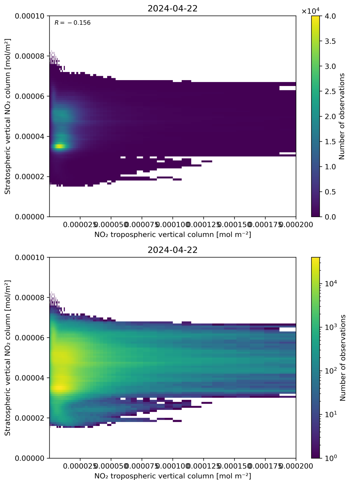
Figure 125: Scatter density plot of “NO 2 tropospheric vertical column” against “Stratospheric vertical NO 2 column” for 2024-04-21 to 2024-04-23.
