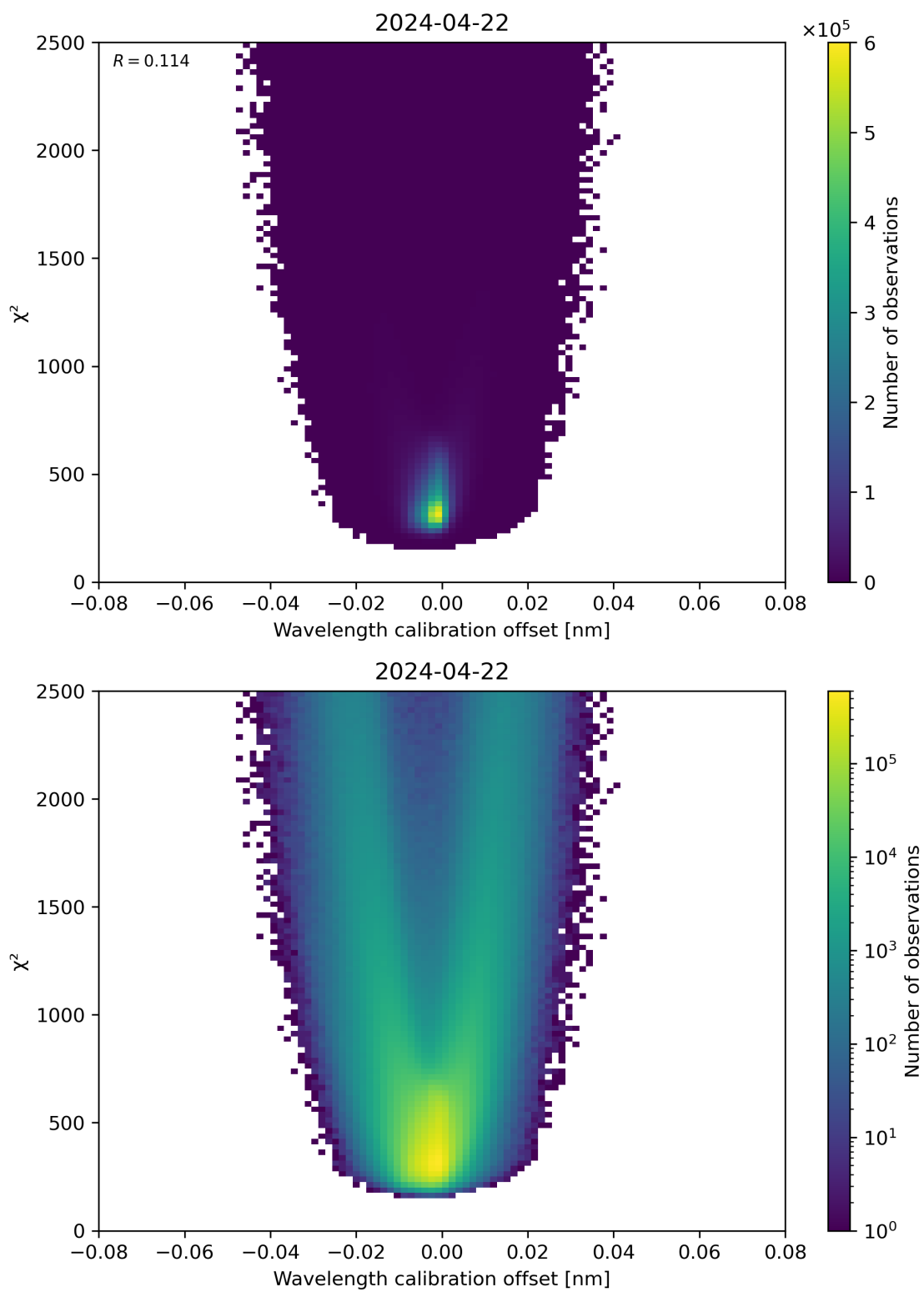
Figure 175: Scatter density plot of “Wavelength calibration offset” against “ \chi^2 ” for 2024-04-21 to 2024-04-23.
