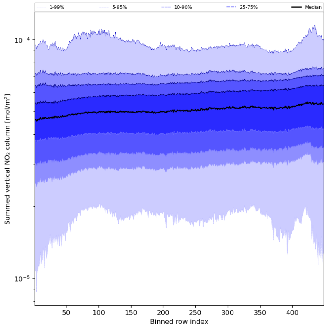
Figure 57: Along track statistics of “Summed vertical NO 2 column” for 2024-04-21 to 2024-04-23
