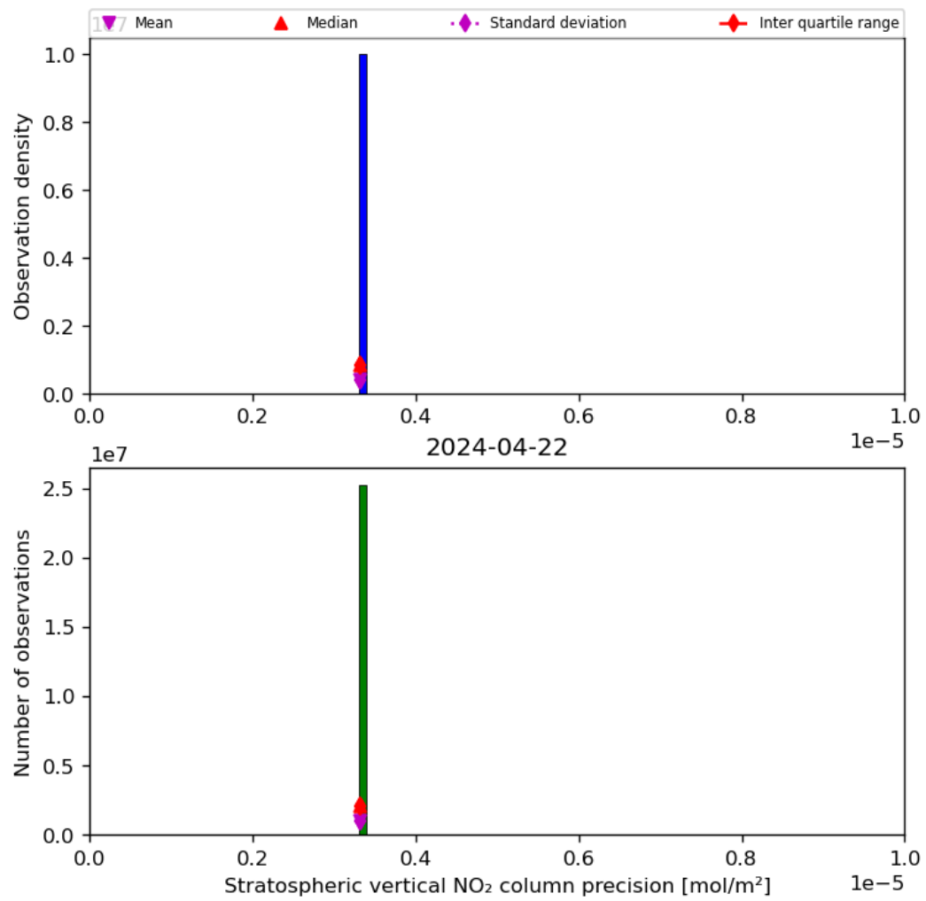
Figure 37: Histogram of “Stratospheric vertical NO 2 column precision” for 2024-04-21 to 2024-04-23
