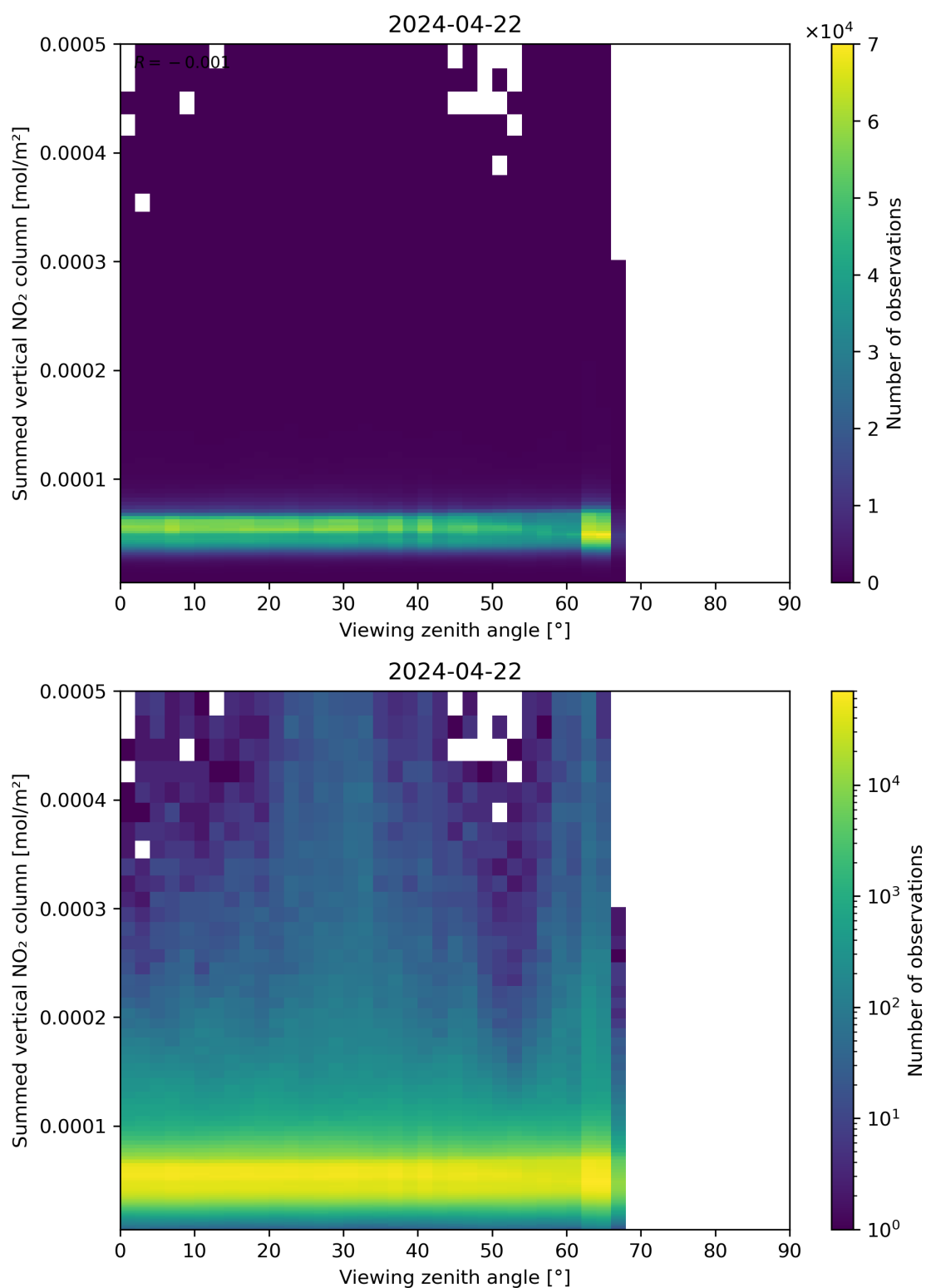
Figure 165: Scatter density plot of “Viewing zenith angle” against “Summed vertical NO 2 column” for 2024-04-21 to 2024-04-23.
