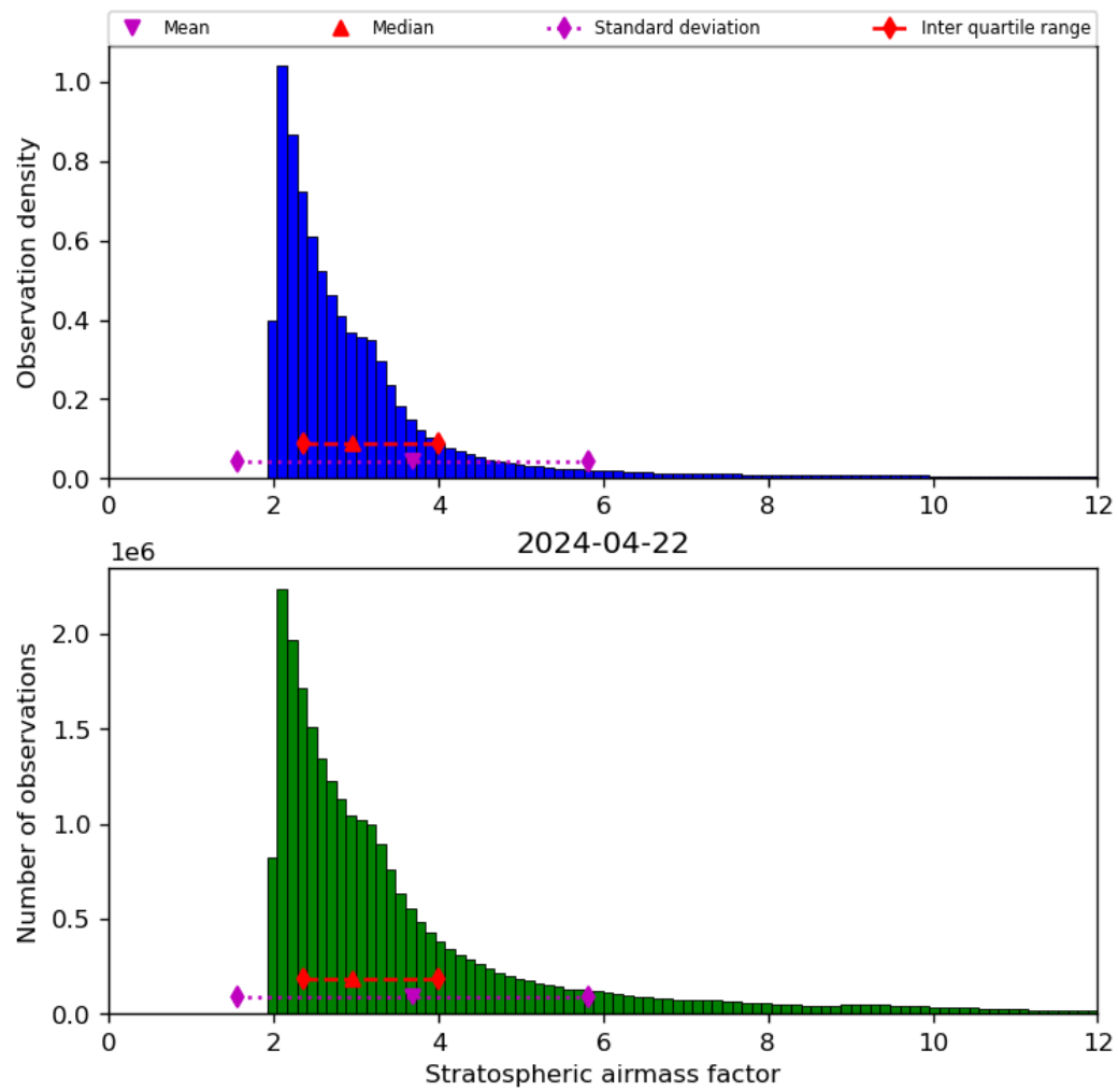
Figure 44: Histogram of “Stratospheric airmass factor” for 2024-04-21 to 2024-04-23
