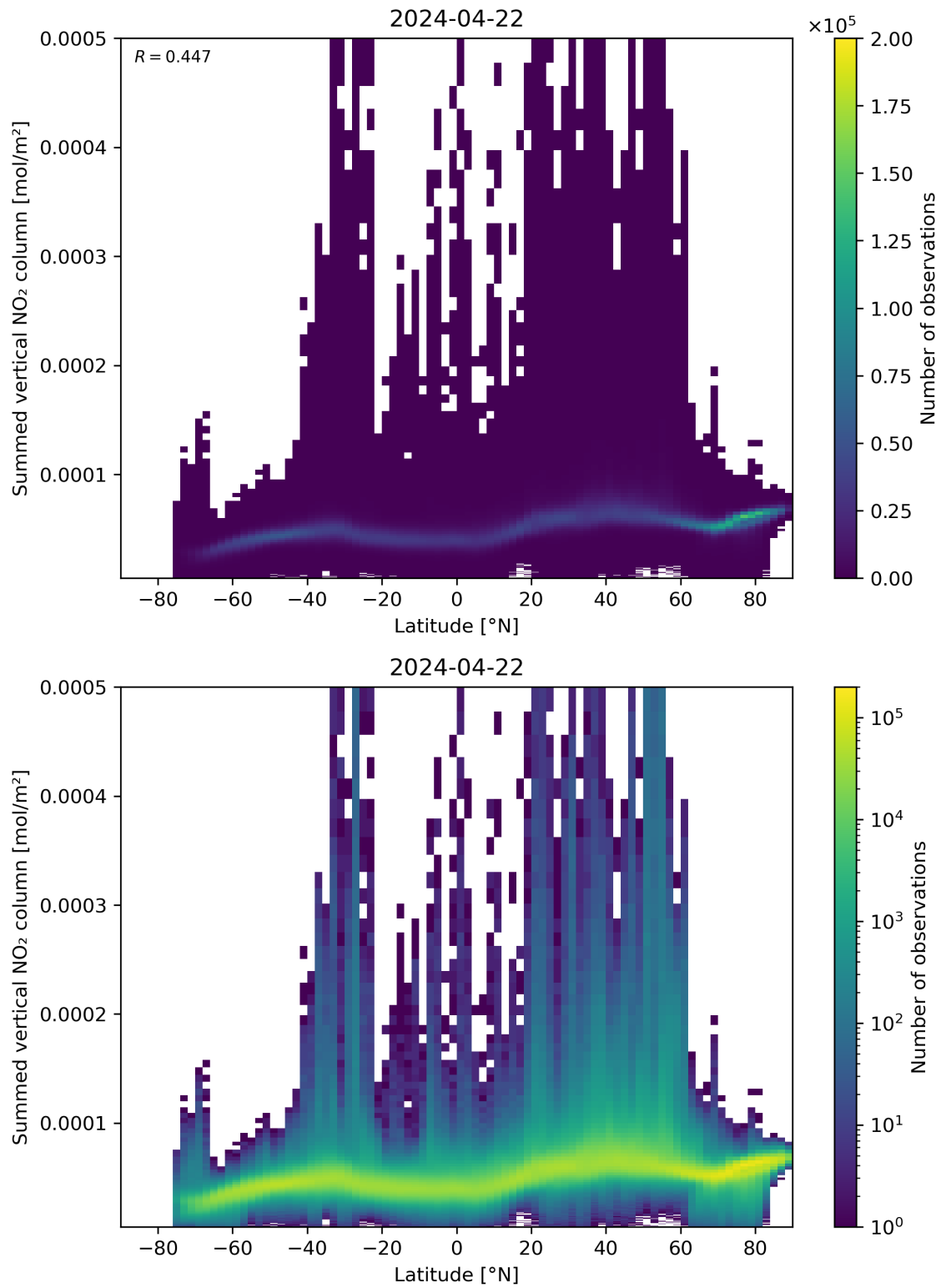
Figure 88: Scatter density plot of “Latitude” against “Summed vertical NO 2 column” for 2024-04-21 to 2024-04-23.
