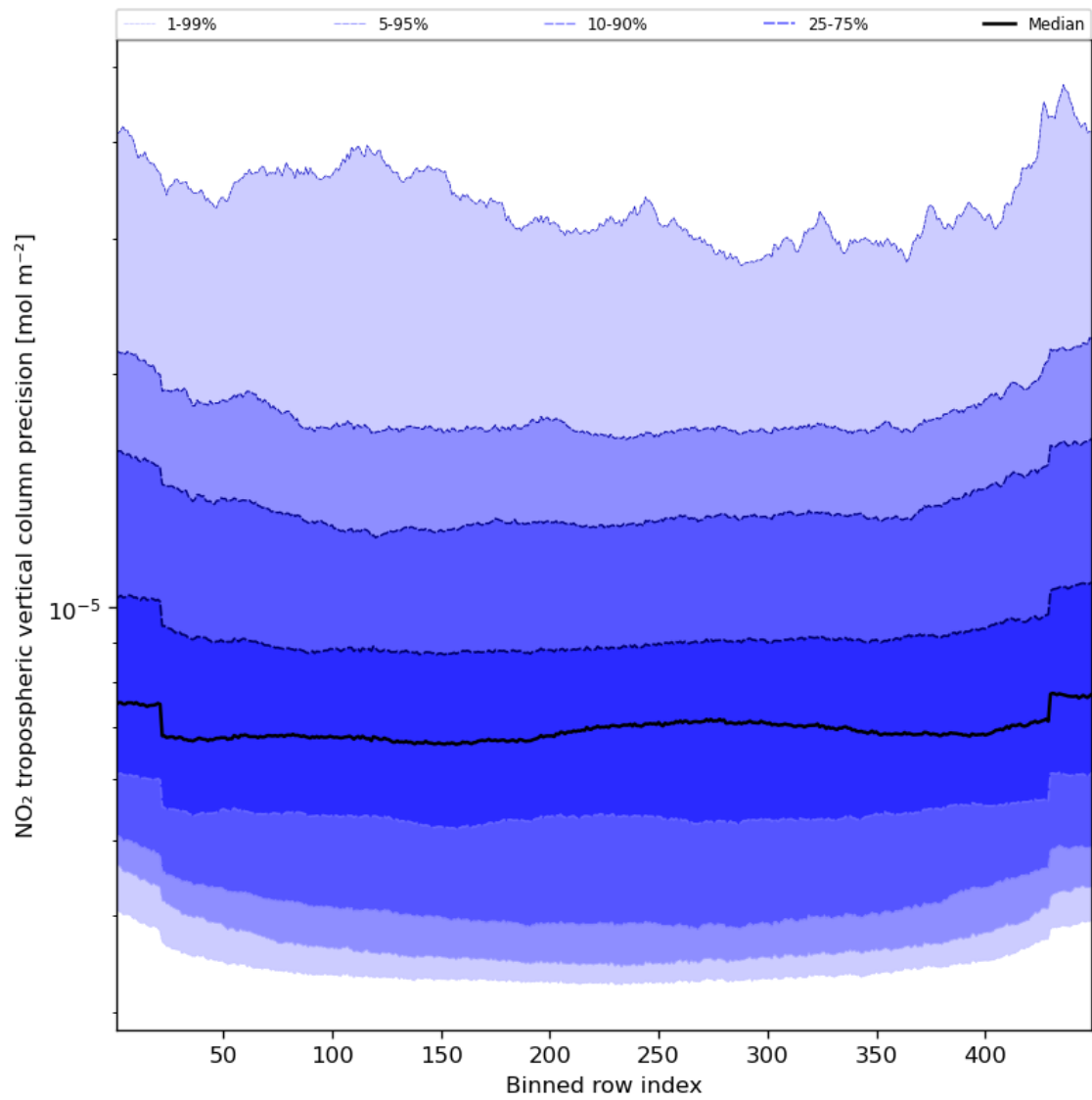
Figure 47: Along track statistics of “NO 2 tropospheric vertical column precision” for 2024-04-21 to 2024-04-23
