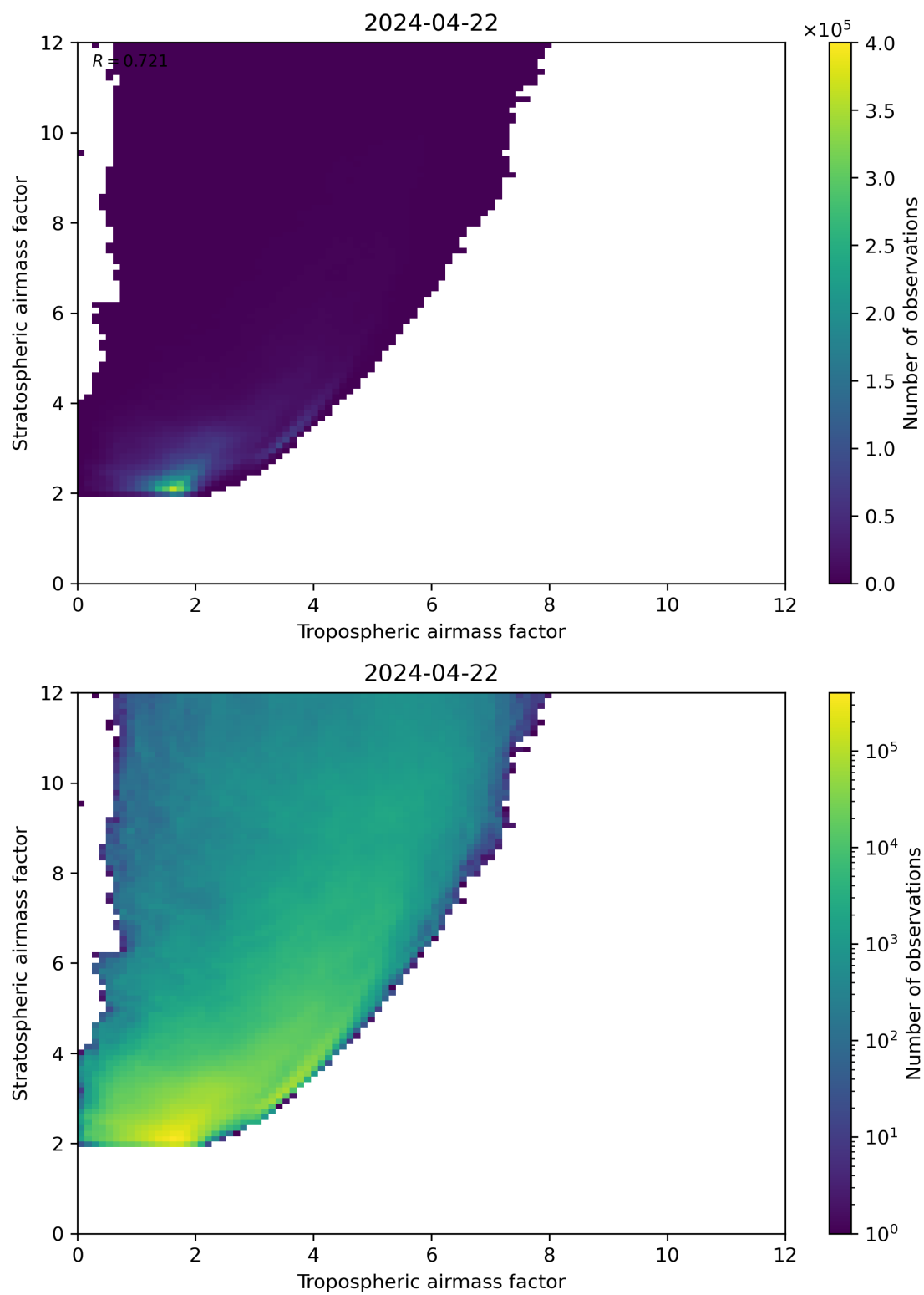
Figure 71: Scatter density plot of “Tropospheric airmass factor” against “Stratospheric airmass factor” for 2024-04-21 to 2024-04-23.
