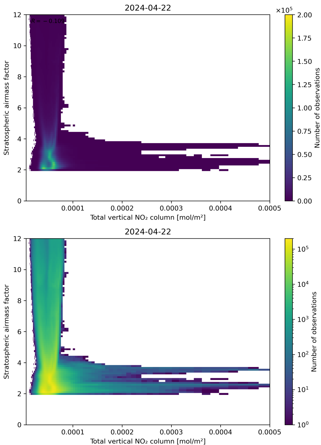
Figure 110: Scatter density plot of “Total vertical NO 2 column” against “Stratospheric airmass factor” for 2024-04-21 to 2024-04-23.
