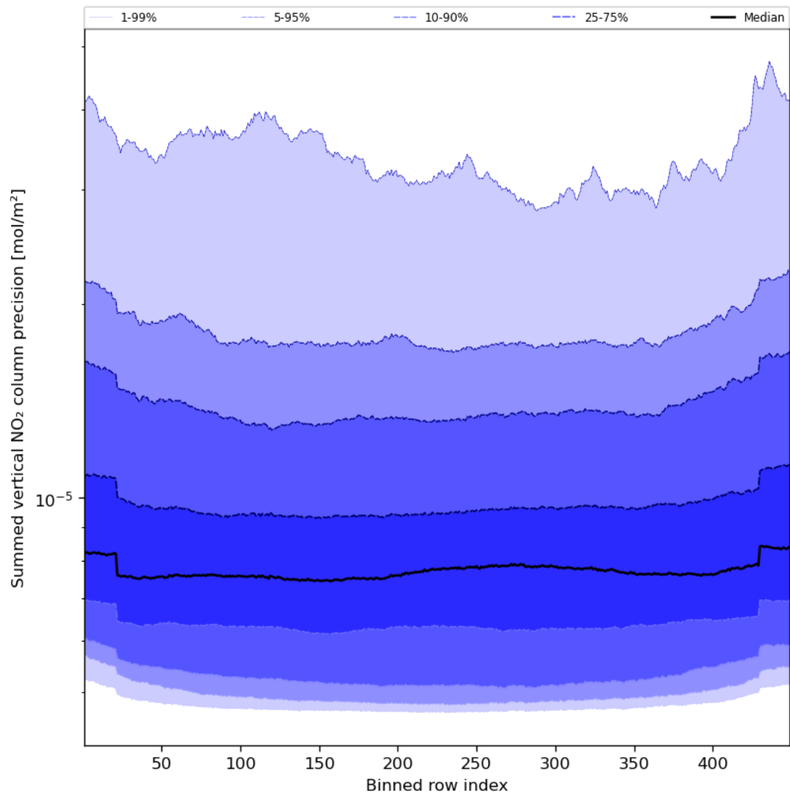
Figure 58: Along track statistics of “Summed vertical NO 2 column precision” for 2024-04-21 to 2024-04-23
