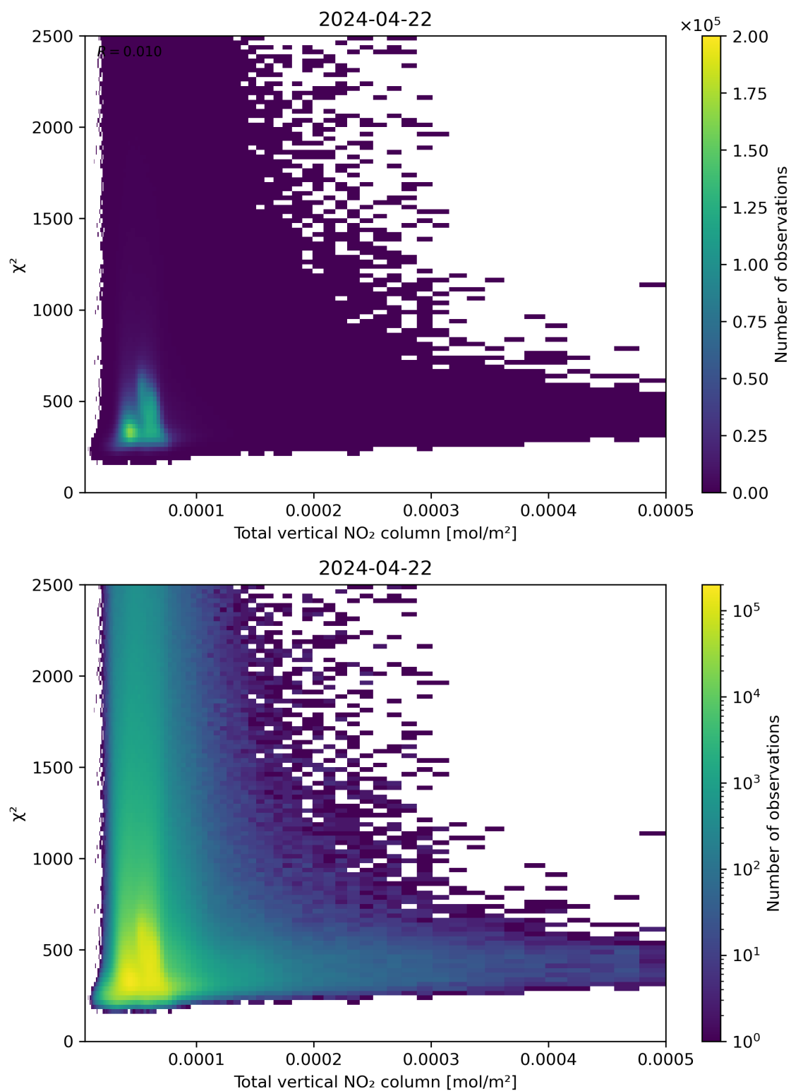
Figure 111: Scatter density plot of “Total vertical NO 2 column” against “ \chi^2 ” for 2024-04-21 to 2024-04-23.
