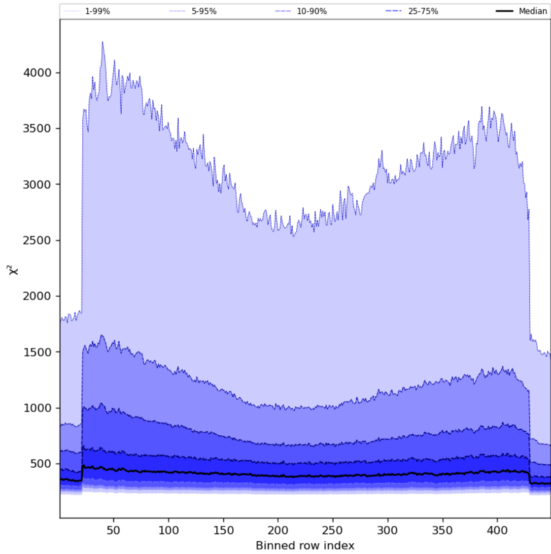
Figure 59: Along track statistics of “ \chi^2 ” for 2024-04-21 to 2024-04-23
