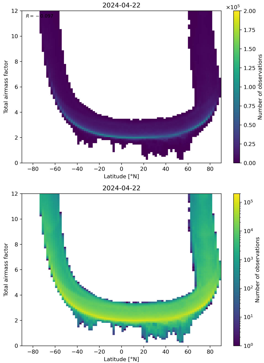
Figure 84: Scatter density plot of “Latitude” against “Total airmass factor” for 2024-04-21 to 2024-04-23.
