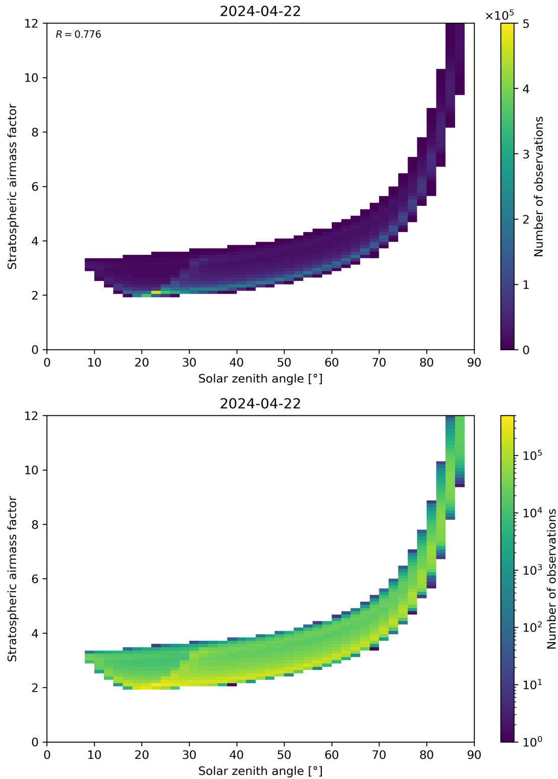
Figure 145: Scatter density plot of “Solar zenith angle” against “Stratospheric airmass factor” for 2024-04-21 to 2024-04-23.
