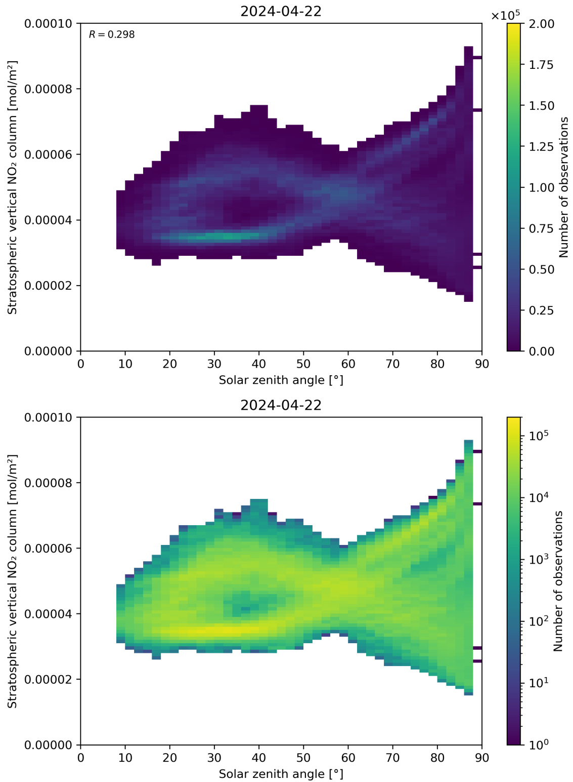
Figure 150: Scatter density plot of “Solar zenith angle” against “Stratospheric vertical NO 2 column” for 2024-04-21 to 2024-04-23.
