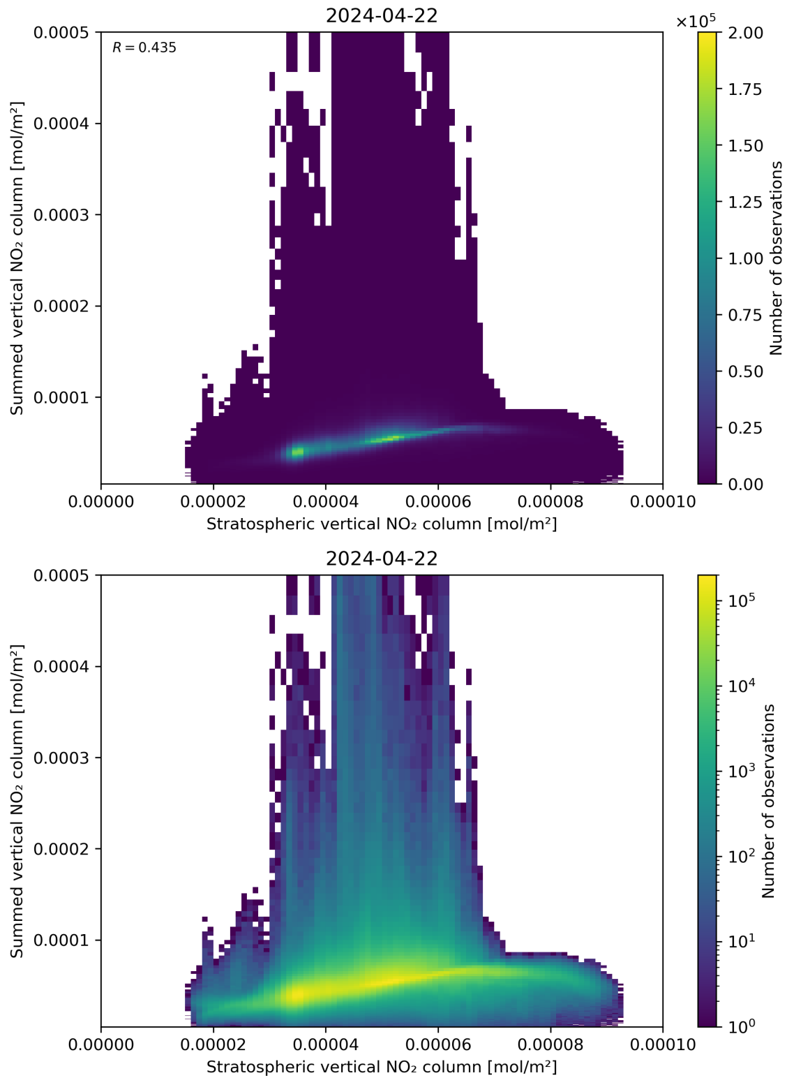
Figure 98: Scatter density plot of “Stratospheric vertical NO 2 column” against “Summed vertical NO 2 column” for 2024-04-21 to 2024-04-23.
