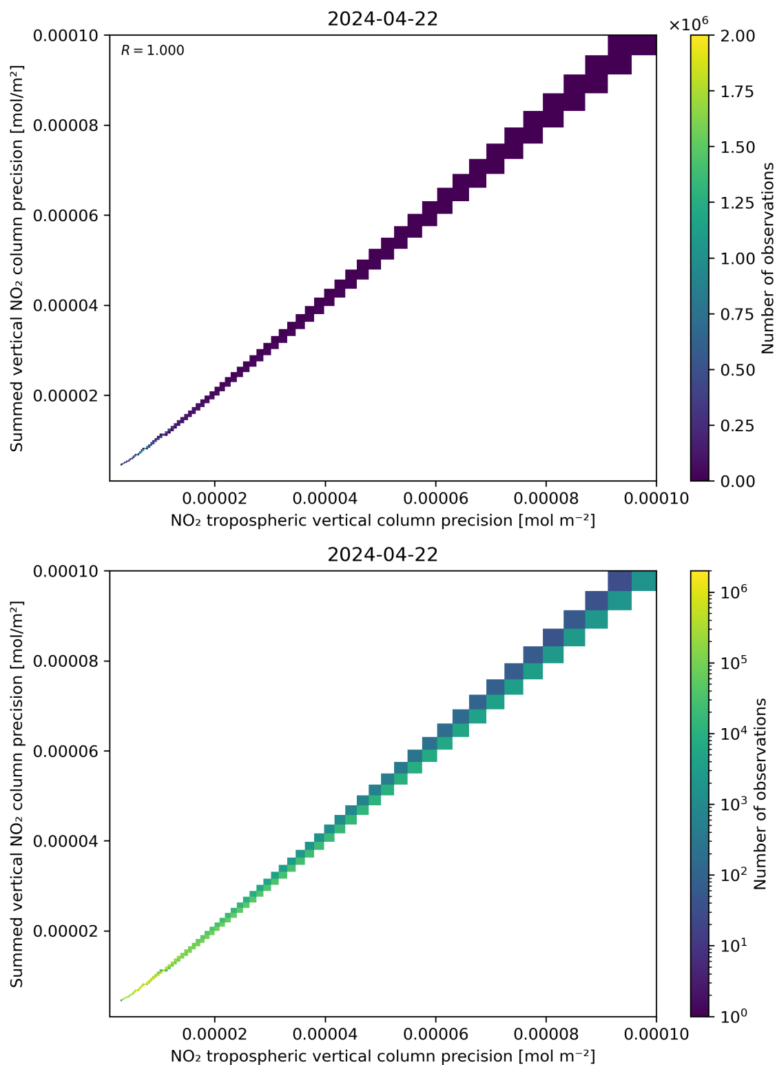
Figure 137: Scatter density plot of “NO 2 tropospheric vertical column precision” against “Summed vertical NO 2 column precision” for 2024-04-21 to 2024-04-23.
