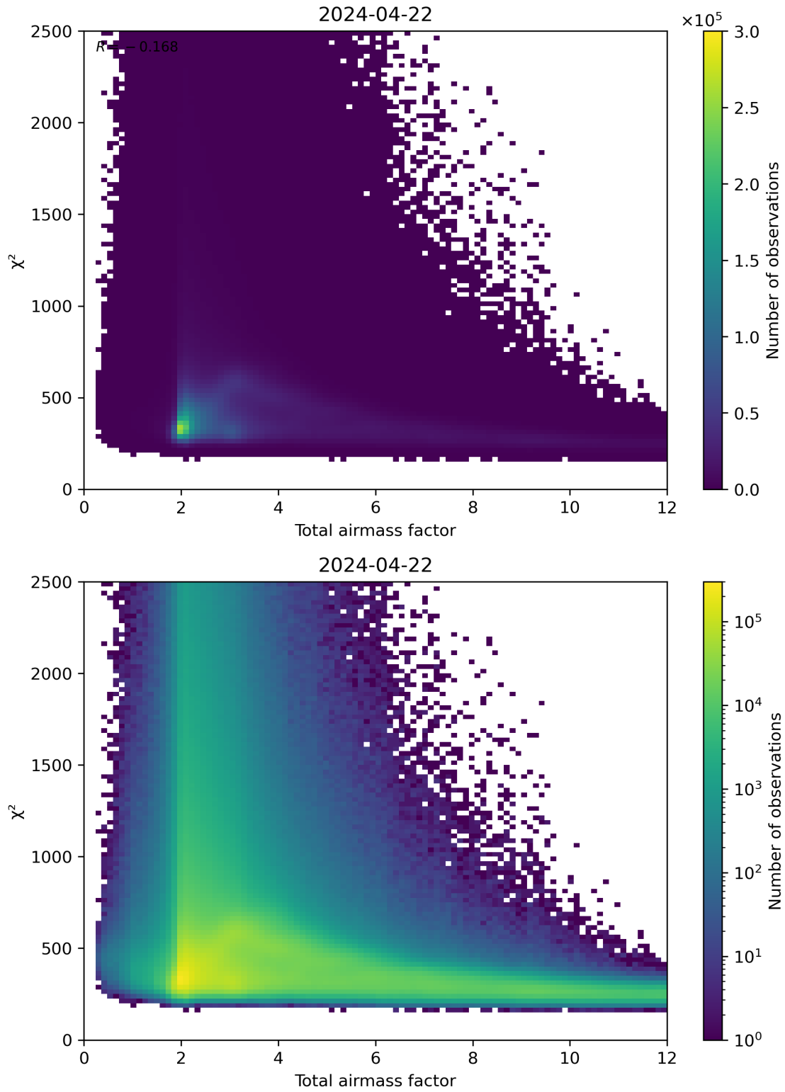
Figure 63: Scatter density plot of “Total airmass factor” against “ \chi^2 ” for 2024-04-21 to 2024-04-23.
