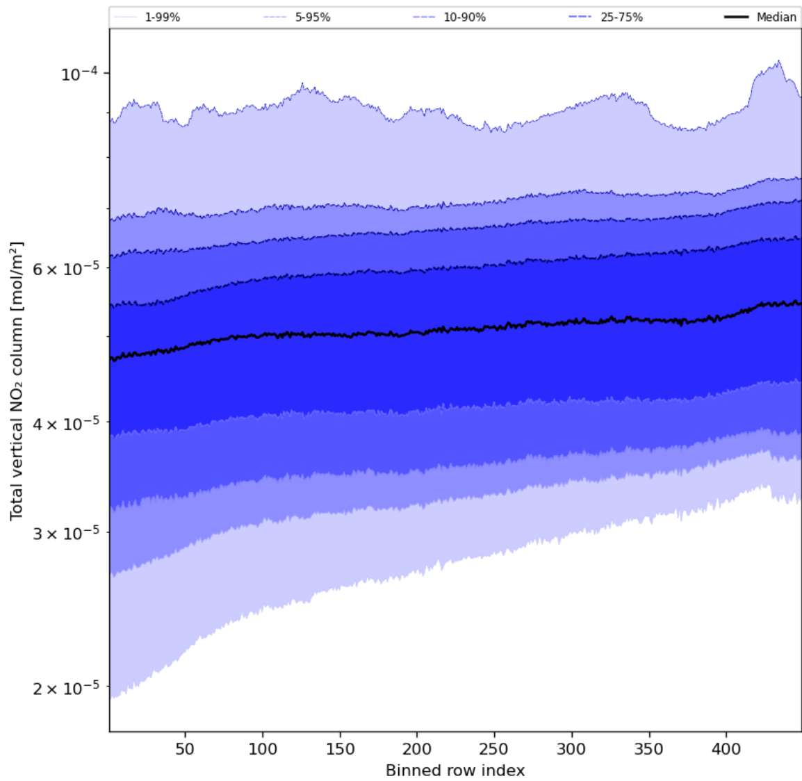
Figure 55: Along track statistics of “Total vertical NO 2 column” for 2024-04-21 to 2024-04-23
