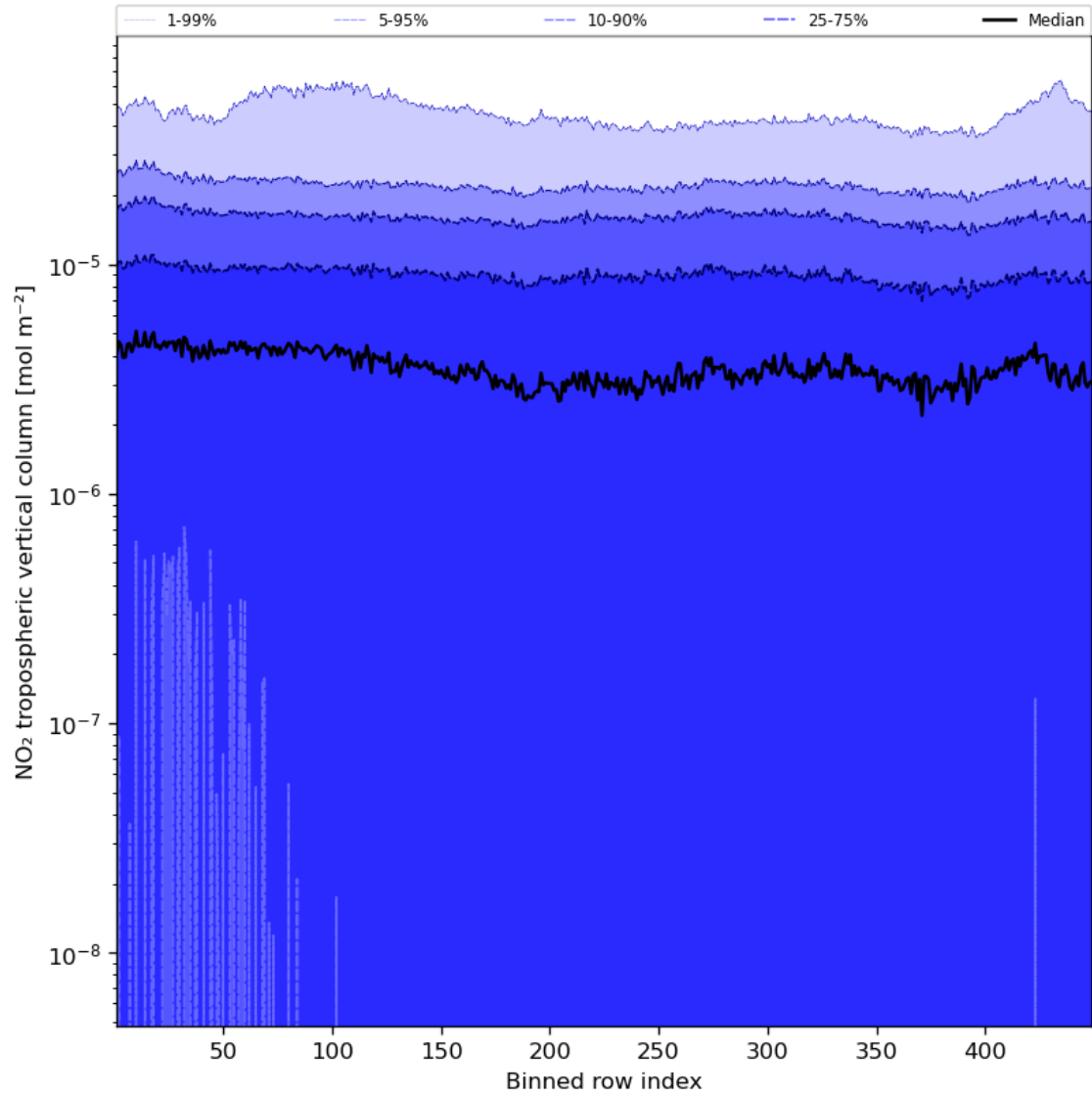
Figure 46: Along track statistics of “NO 2 tropospheric vertical column” for 2024-04-21 to 2024-04-23
