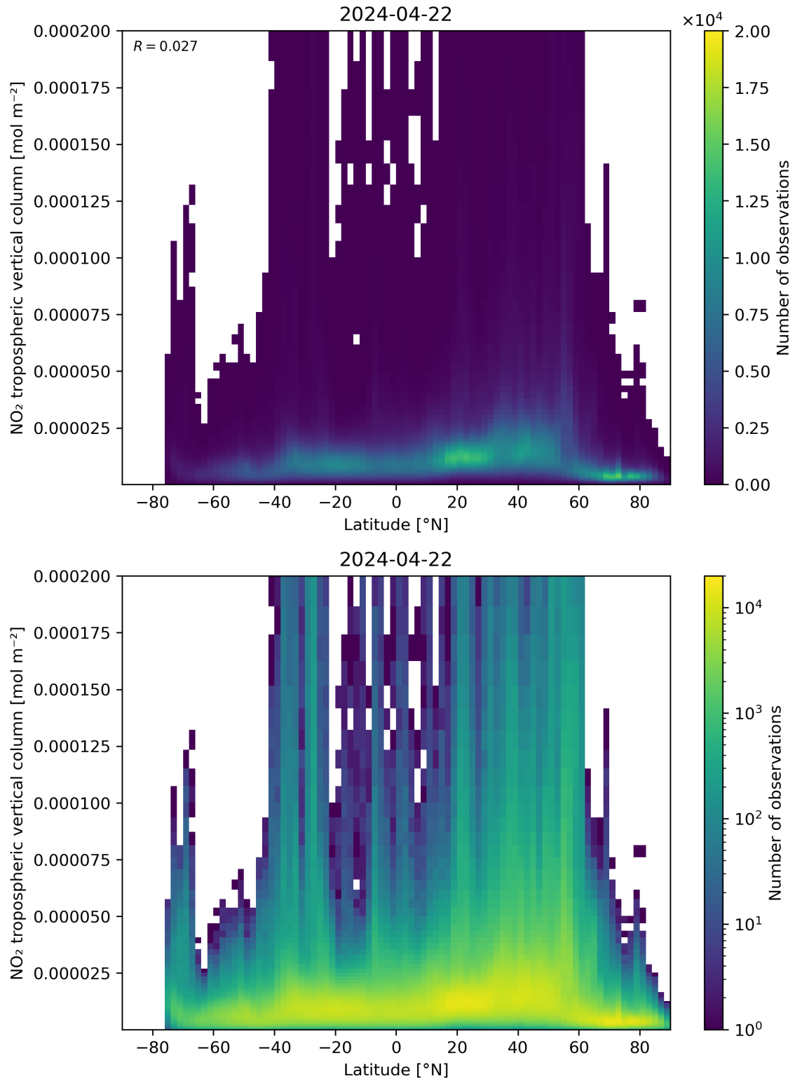
Figure 92: Scatter density plot of “Latitude” against “NO 2 tropospheric vertical column” for 2024-04-21 to 2024-04-23.
