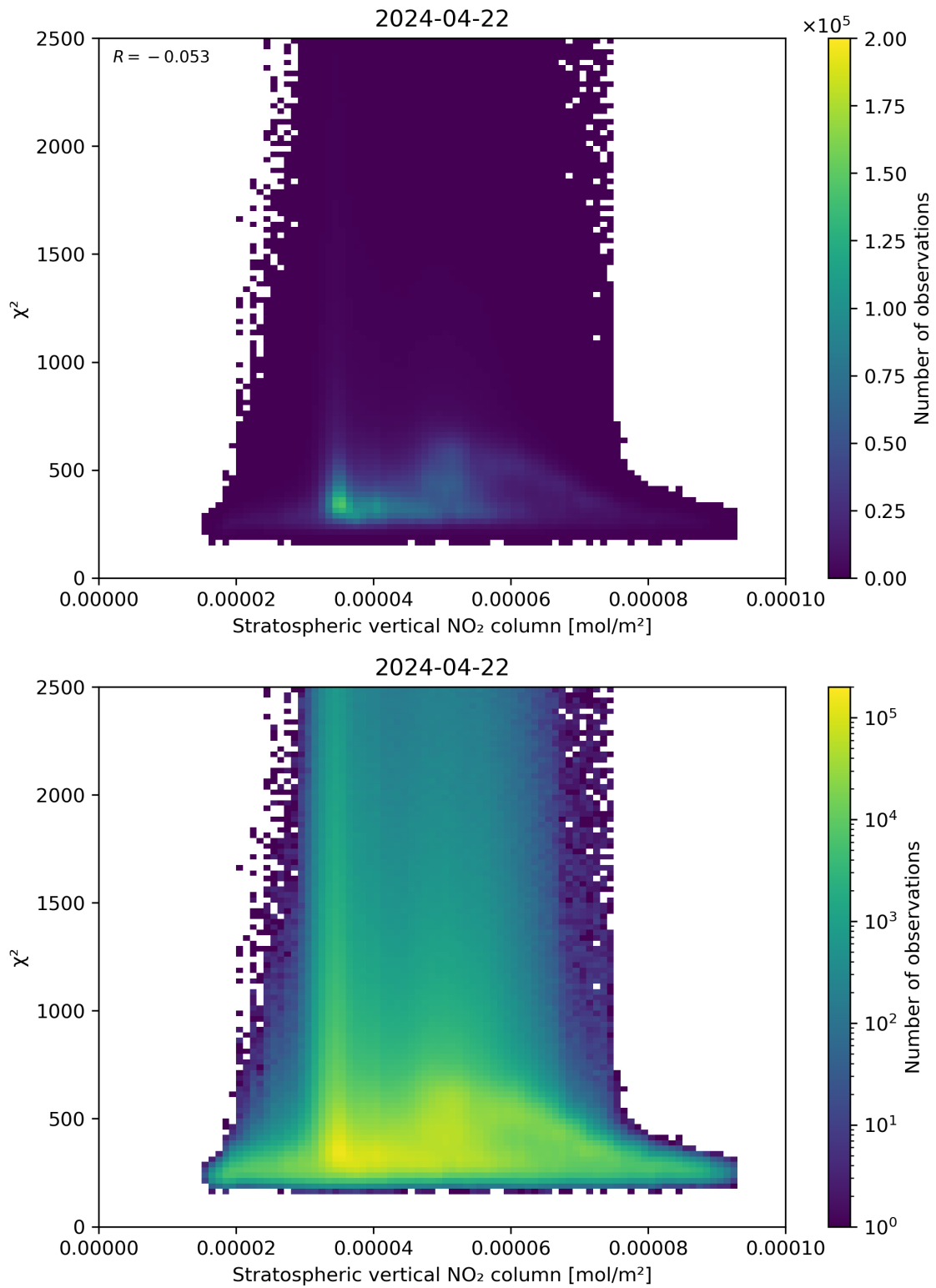
Figure 97: Scatter density plot of “Stratospheric vertical NO 2 column” against “ \chi^2 ” for 2024-04-21 to 2024-04-23.
