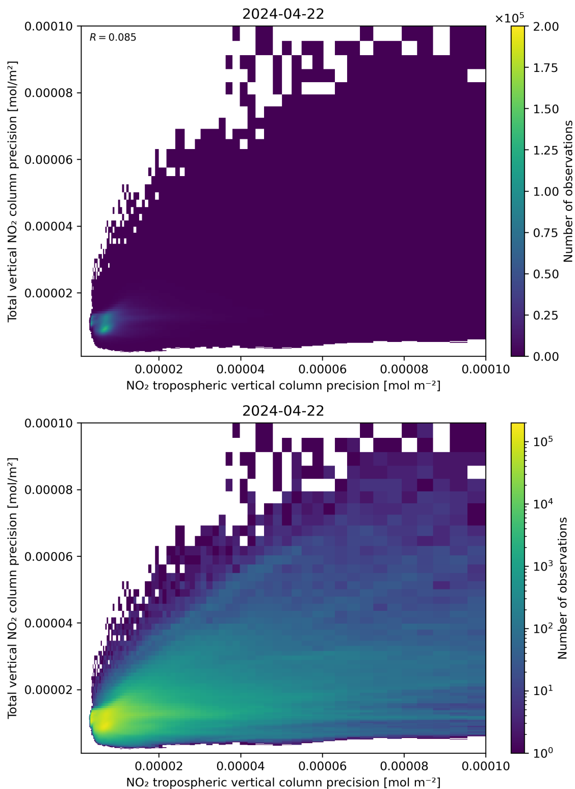
Figure 139: Scatter density plot of “NO 2 tropospheric vertical column precision” against “Total vertical NO 2 column precision” for 2024-04-21 to 2024-04-23.
