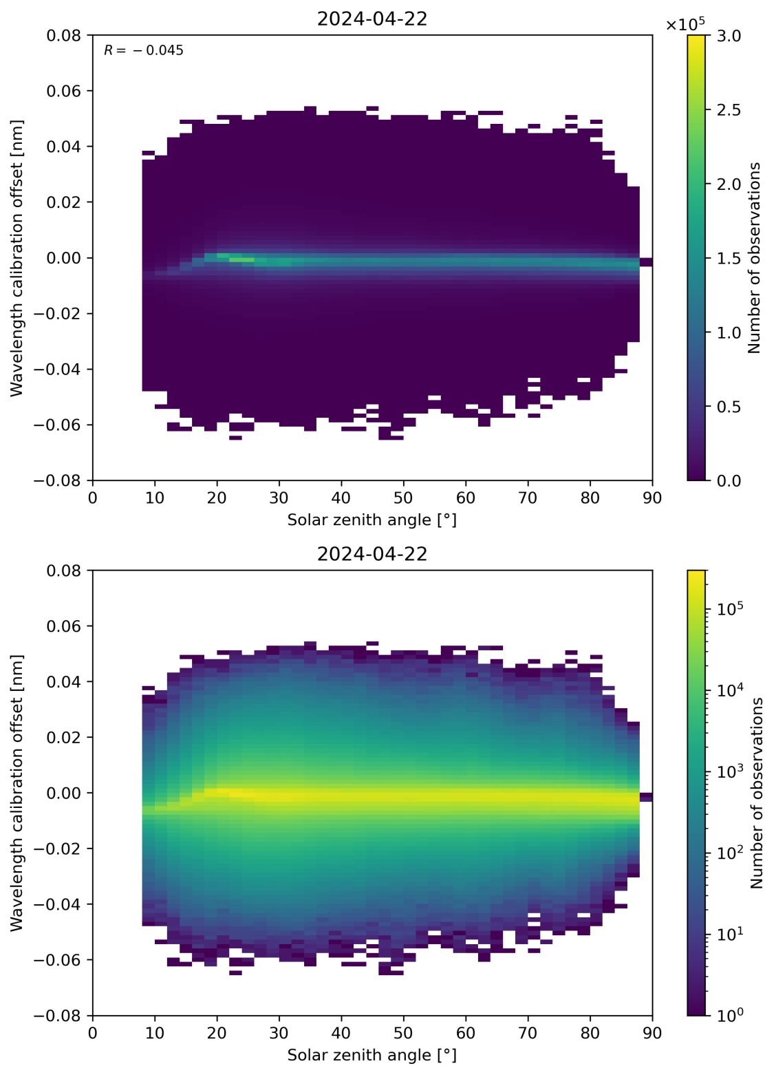
Figure 158: Scatter density plot of “Solar zenith angle” against “Wavelength calibration offset” for 2024-04-21 to 2024-04-23.
