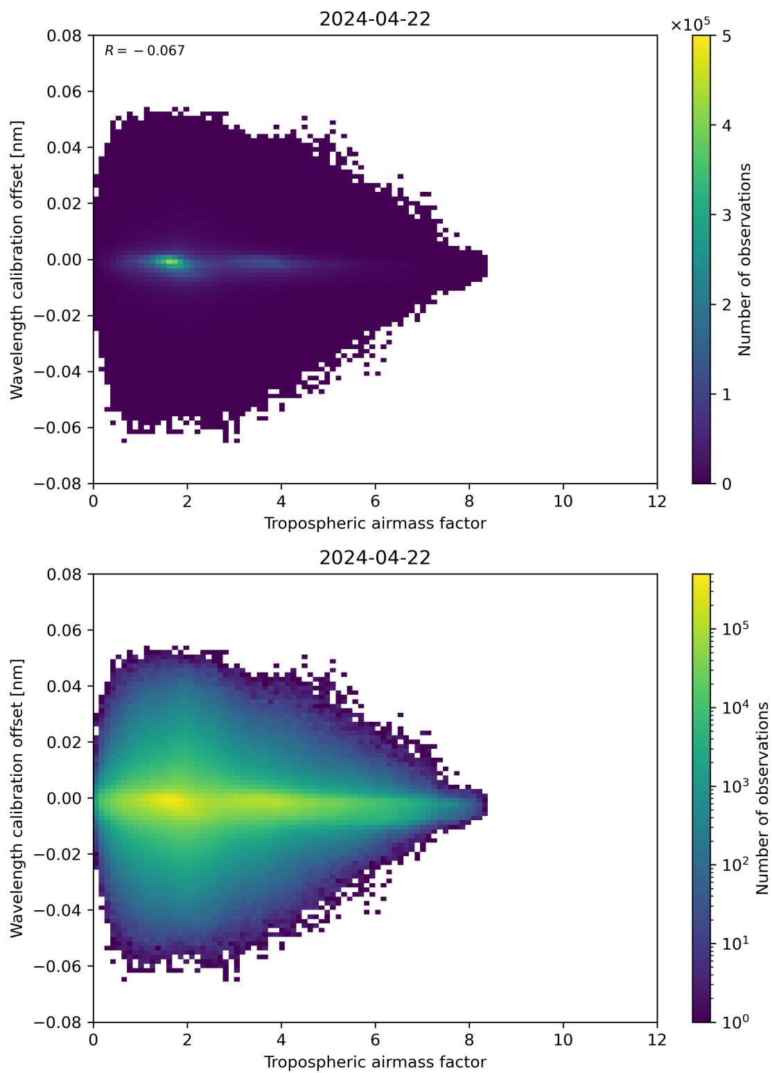
Figure 80: Scatter density plot of “Tropospheric airmass factor” against “Wavelength calibration offset” for 2024-04-21 to 2024-04-23.
