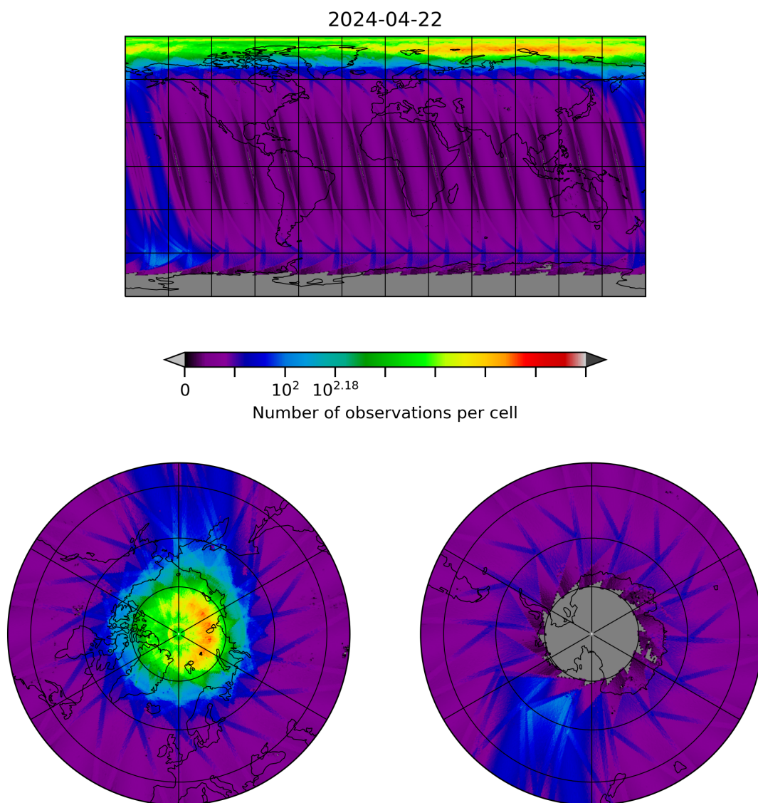
Figure 10: Map of the number of observations for 2024-04-21 to 2024-04-23
