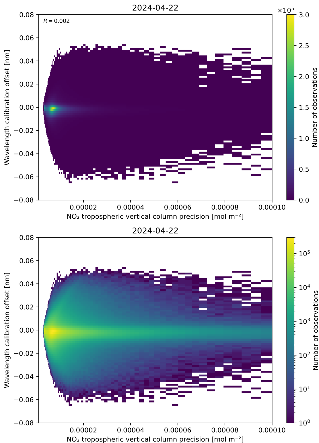
Figure 141: Scatter density plot of “NO 2 tropospheric vertical column precision” against “Wavelength calibration offset” for 2024-04-21 to 2024-04-23.
