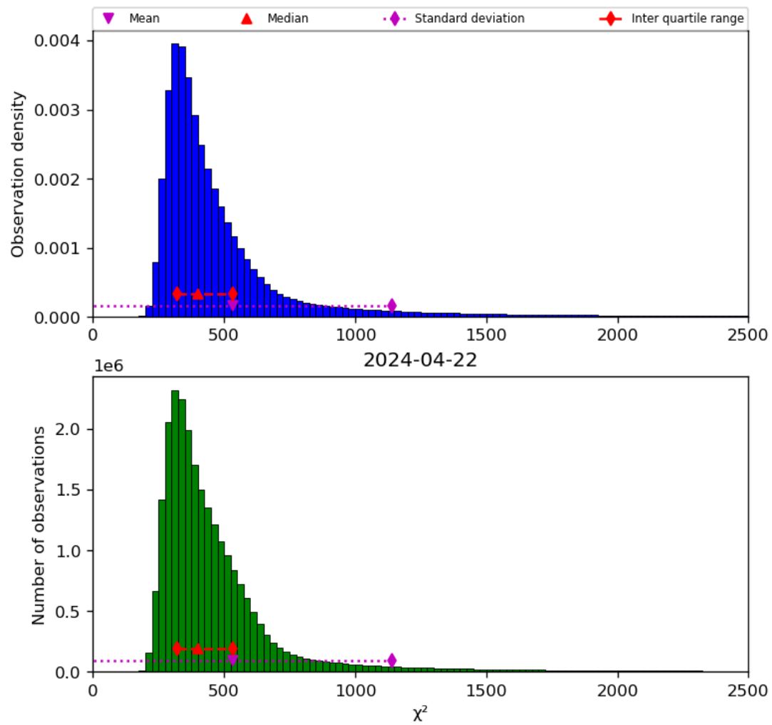
Figure 42: Histogram of “ \chi^2 ” for 2024-04-21 to 2024-04-23
