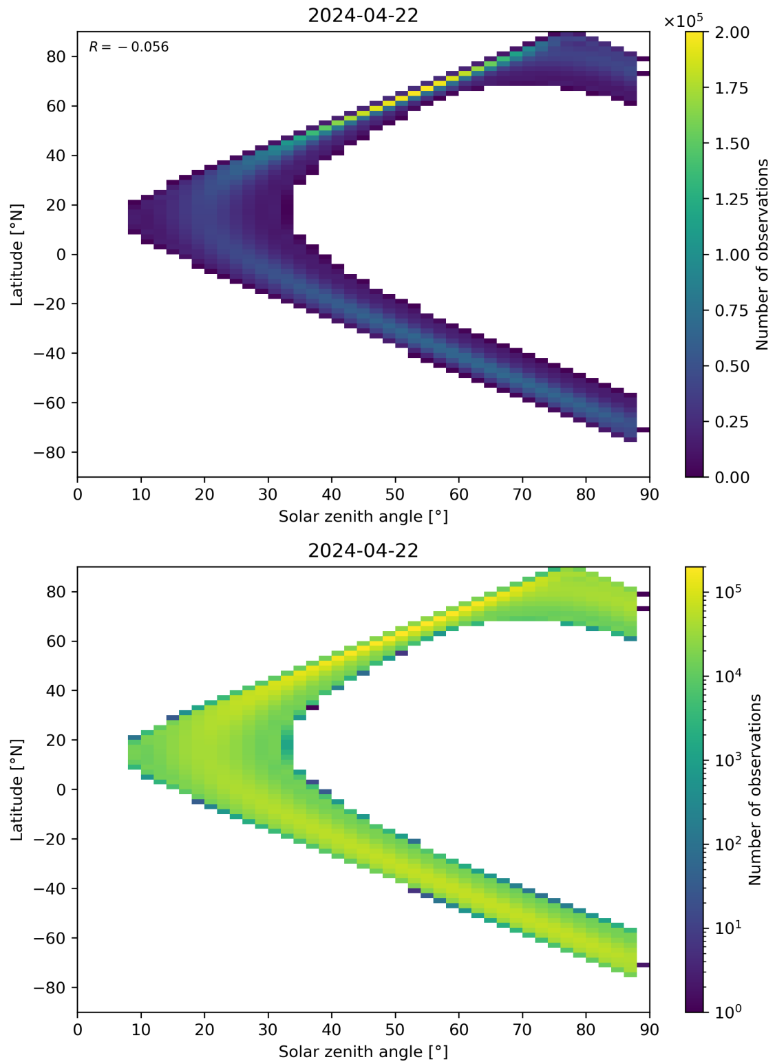
Figure 149: Scatter density plot of “Solar zenith angle” against “Latitude” for 2024-04-21 to 2024-04-23.
