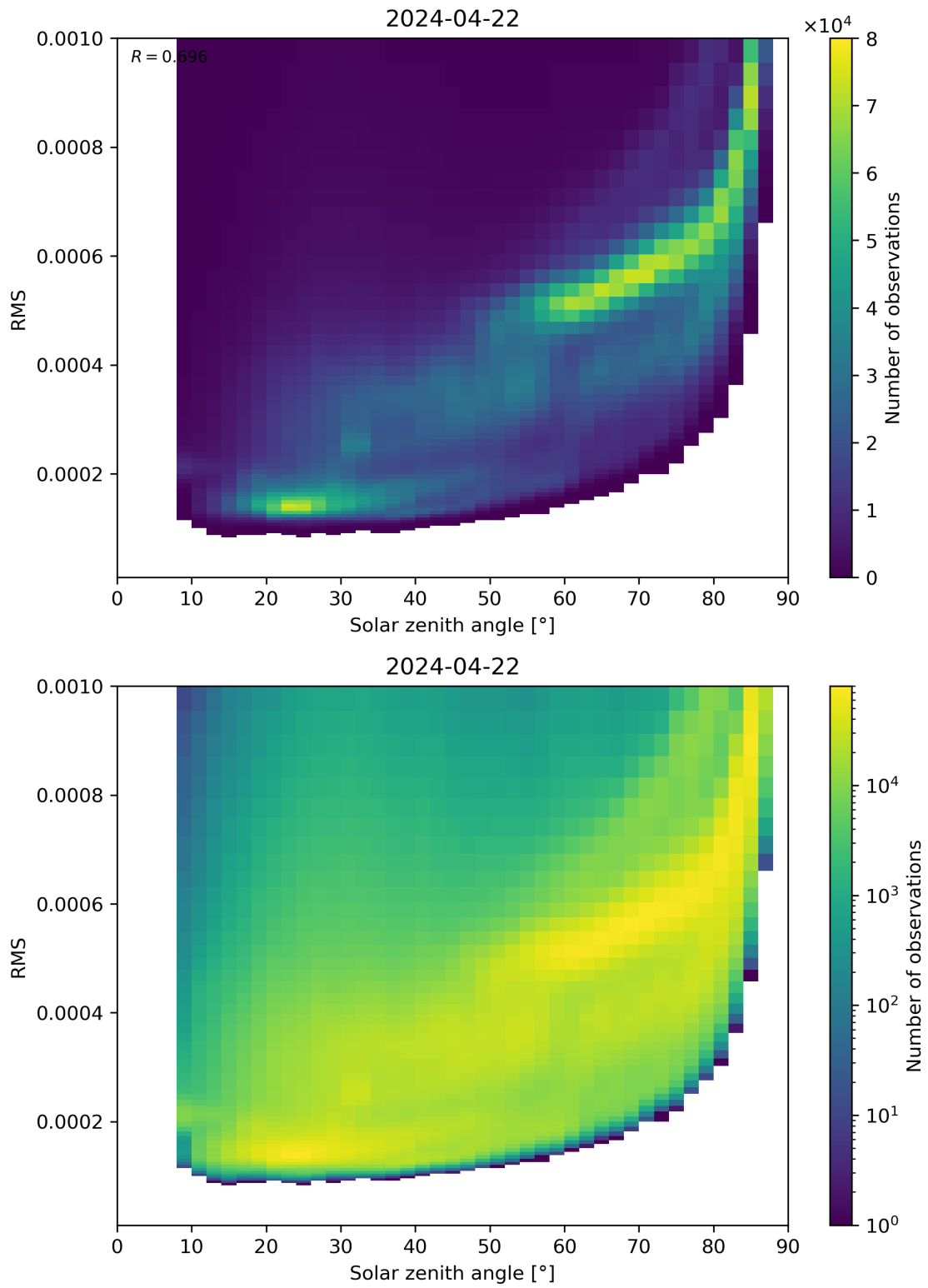
Figure 157: Scatter density plot of “Solar zenith angle” against “RMS” for 2024-04-21 to 2024-04-23.
