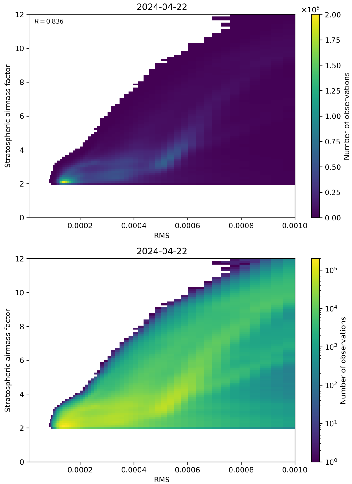
Figure 144: Scatter density plot of “RMS” against “Stratospheric airmass factor” for 2024-04-21 to 2024-04-23.
