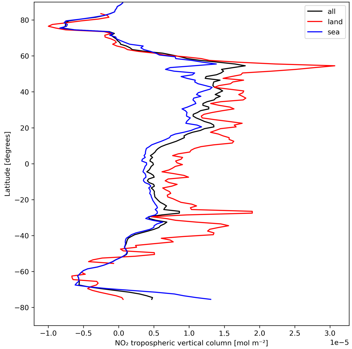
Figure 12: Zonal average of “NO 2 tropospheric vertical column” for 2024-04-21 to 2024-04-23.
