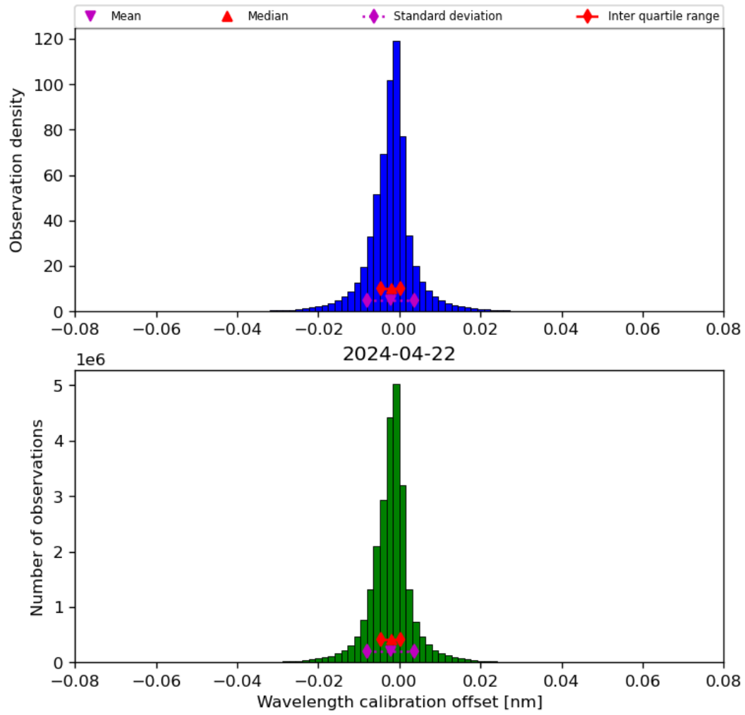
Figure 35: Histogram of “Wavelength calibration offset” for 2024-04-21 to 2024-04-23
