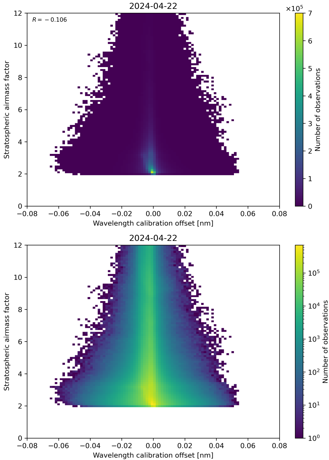
Figure 174: Scatter density plot of “Wavelength calibration offset” against “Stratospheric airmass factor” for 2024-04-21 to 2024-04-23.
