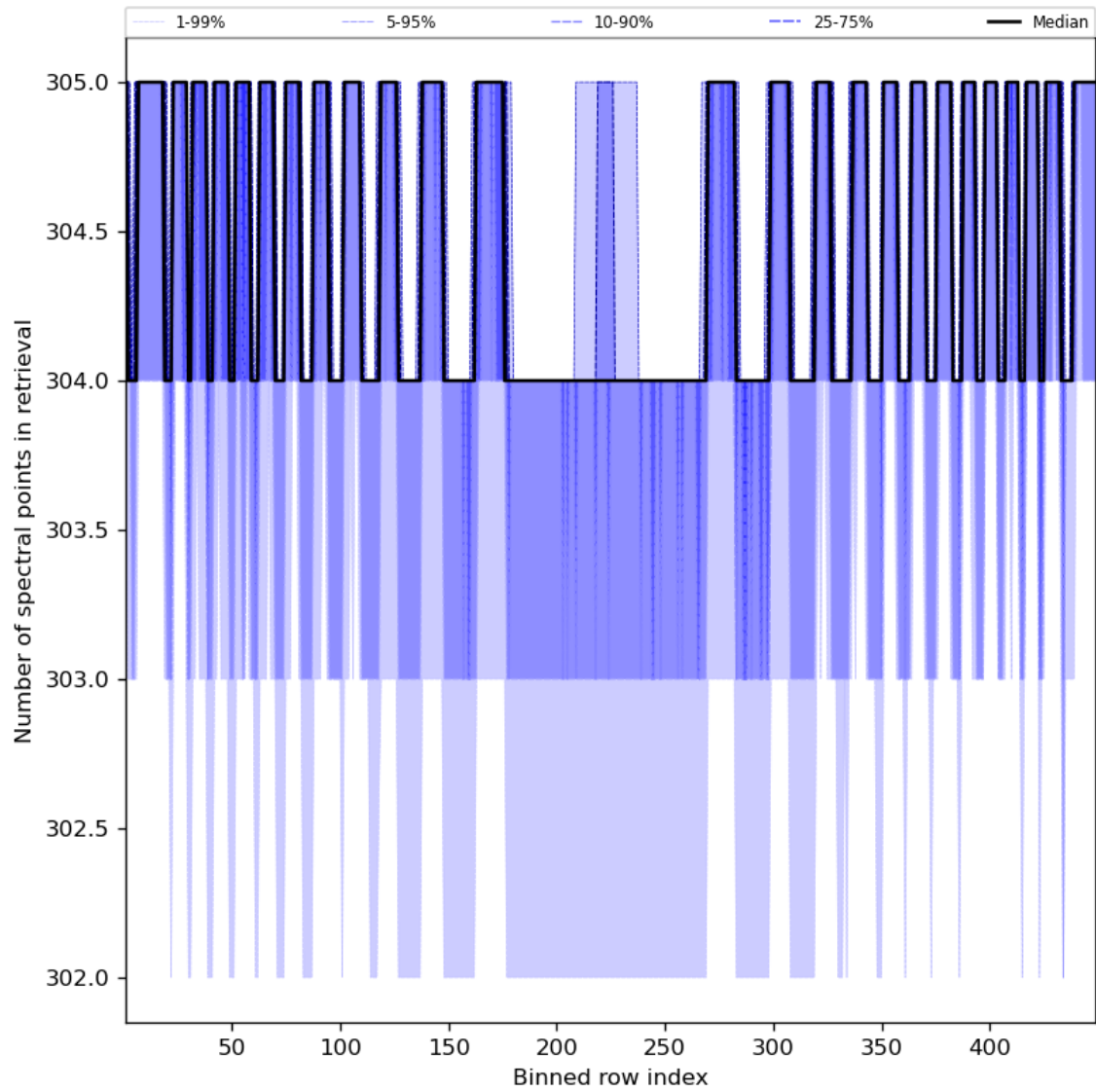
Figure 50: Along track statistics of “Number of spectral points in retrieval” for 2024-04-21 to 2024-04-23
