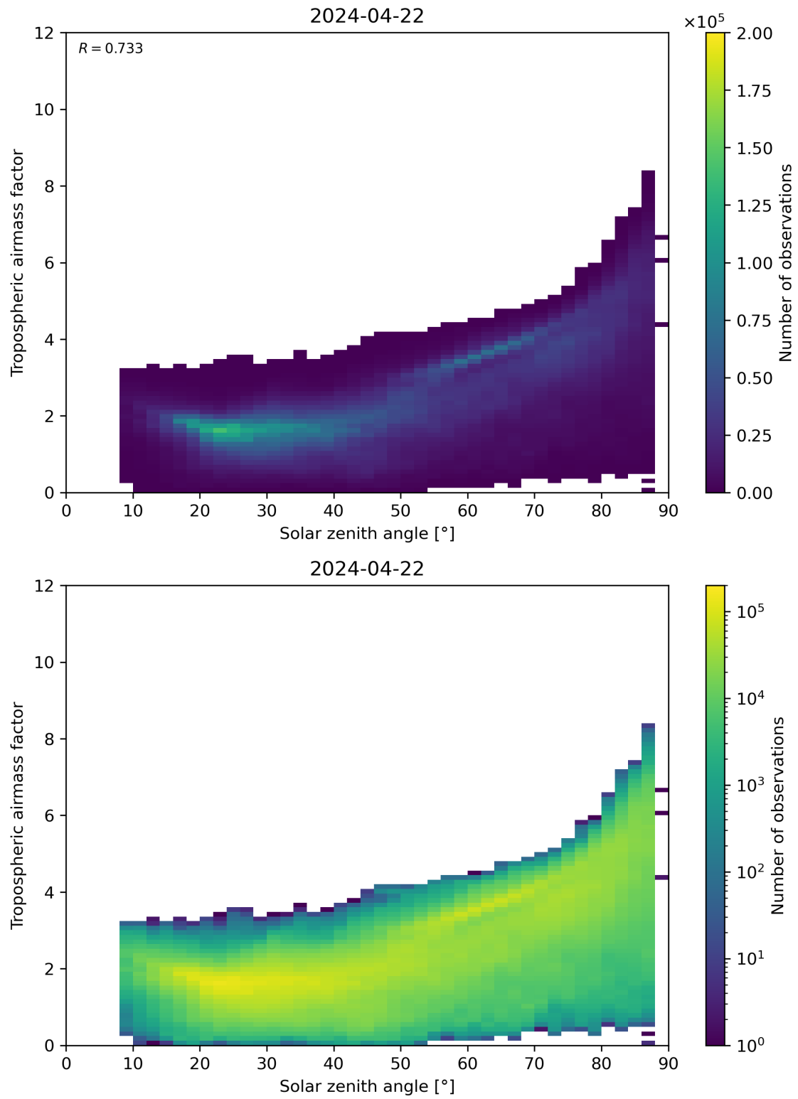
Figure 147: Scatter density plot of “Solar zenith angle” against “Tropospheric airmass factor” for 2024-04-21 to 2024-04-23.
