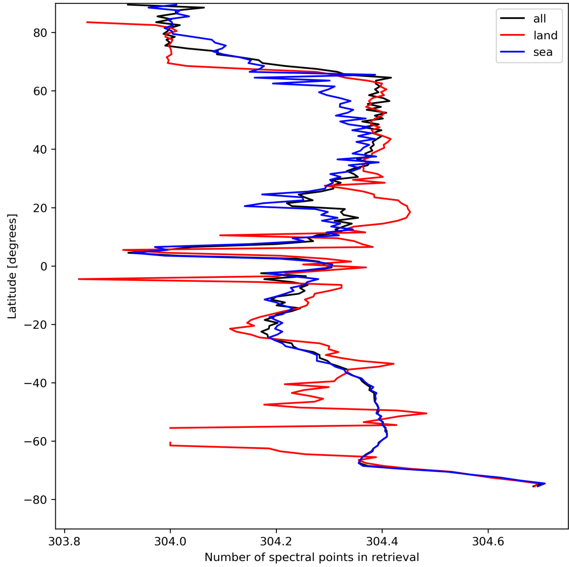
Figure 16: Zonal average of “Number of spectral points in retrieval” for 2024-04-21 to 2024-04-23.
