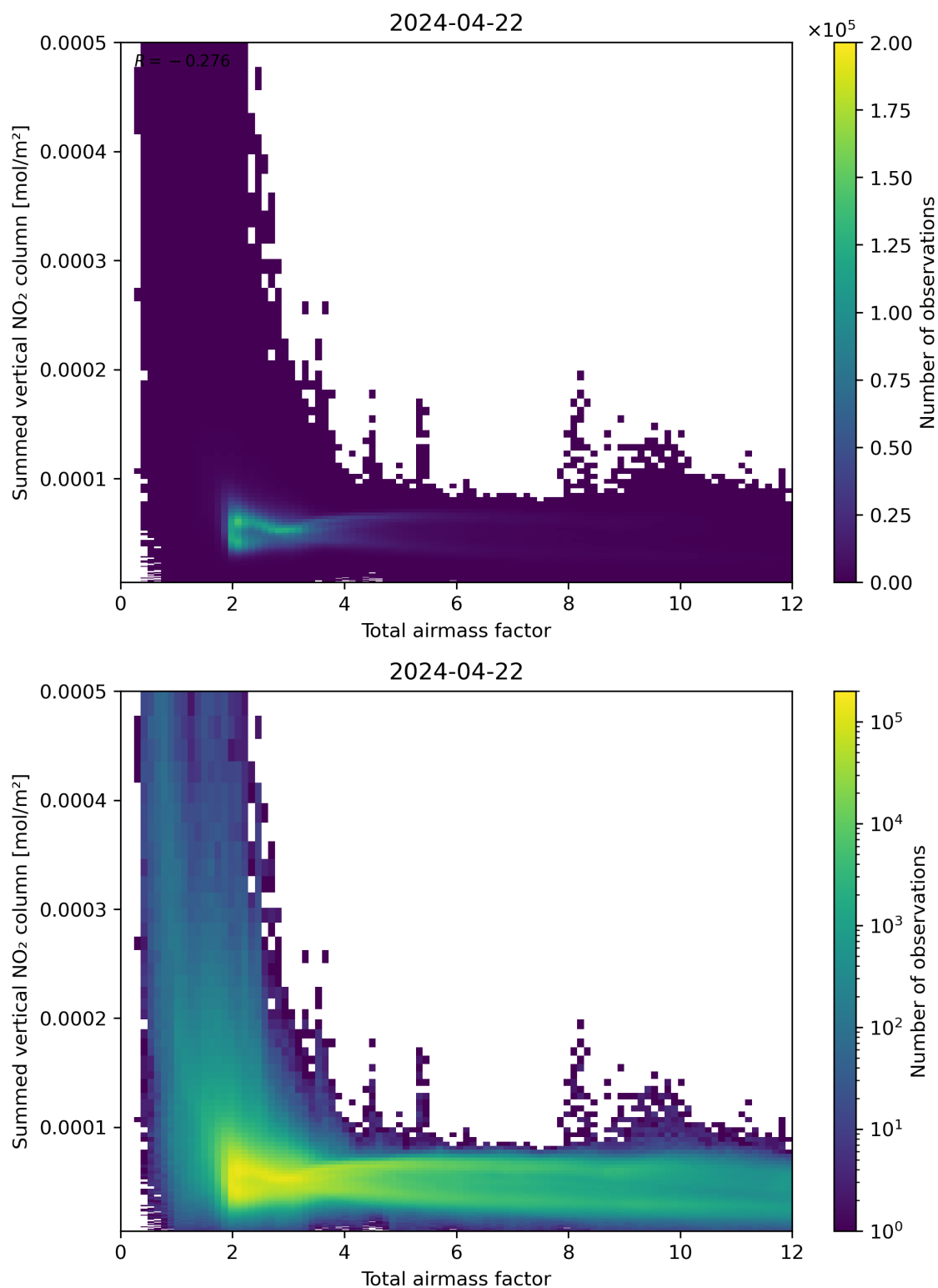
Figure 65: Scatter density plot of “Total airmass factor” against “Summed vertical NO 2 column” for 2024-04-21 to 2024-04-23.
