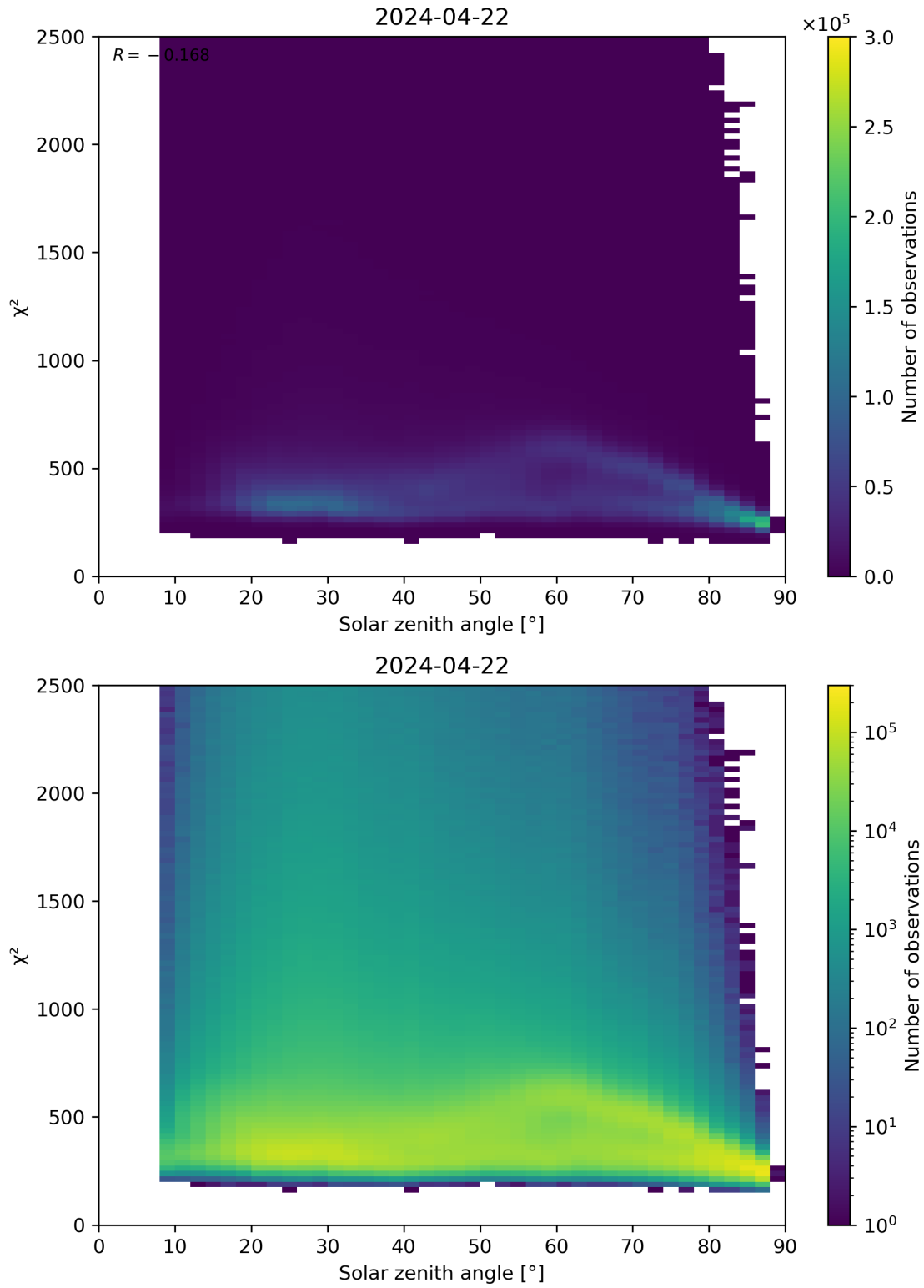
Figure 148: Scatter density plot of “Solar zenith angle” against “ \chi^2 ” for 2024-04-21 to 2024-04-23.
