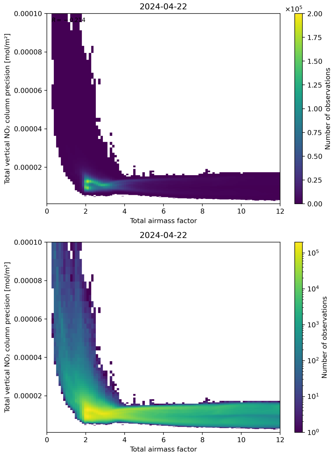
Figure 68: Scatter density plot of “Total airmass factor” against “Total vertical NO 2 column precision” for 2024-04-21 to 2024-04-23.
