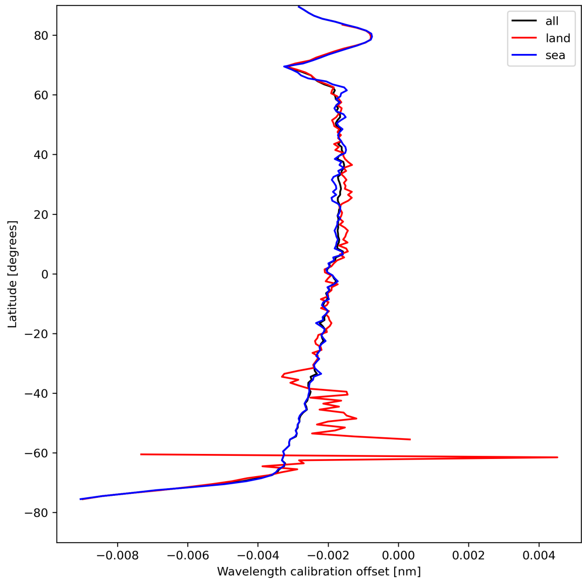
Figure 18: Zonal average of “Wavelength calibration offset” for 2024-04-21 to 2024-04-23.
