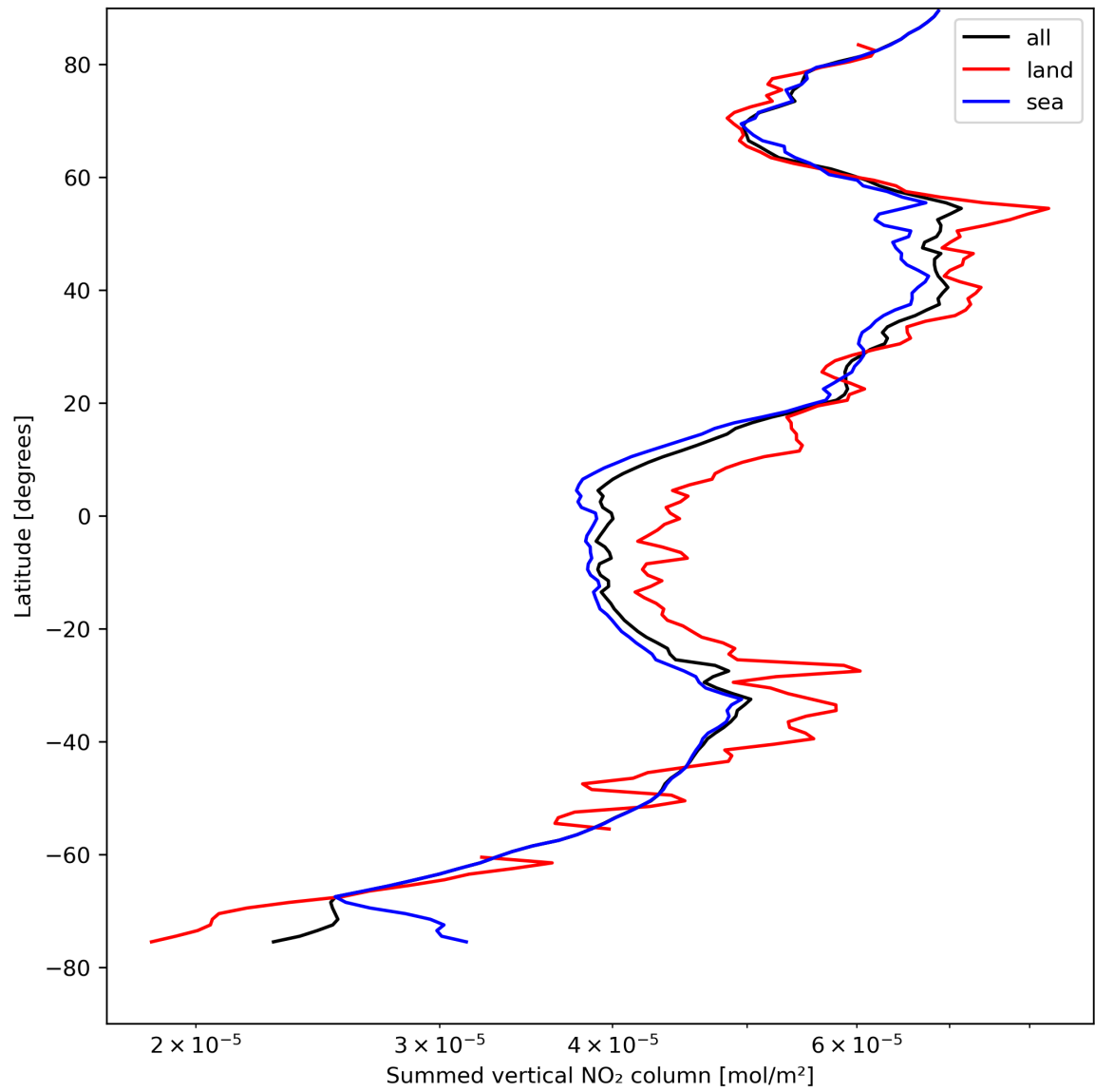
Figure 23: Zonal average of “Summed vertical NO 2 column” for 2024-04-21 to 2024-04-23.
