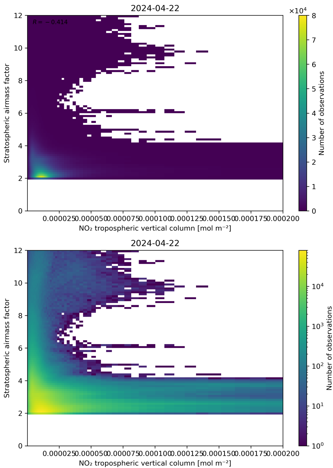
Figure 121: Scatter density plot of “NO 2 tropospheric vertical column” against “Stratospheric air mass factor” for 2024-04-21 to 2024-04-23.
