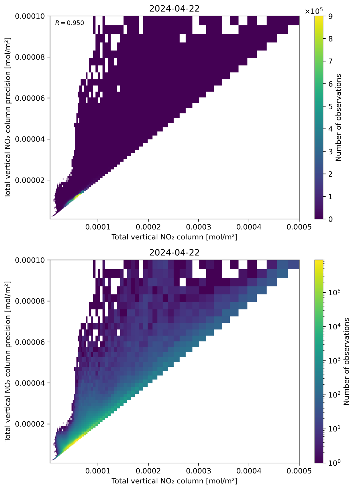
Figure 114: Scatter density plot of “Total vertical NO 2 column” against “Total vertical NO 2 column precision” for 2024-04-21 to 2024-04-23.
