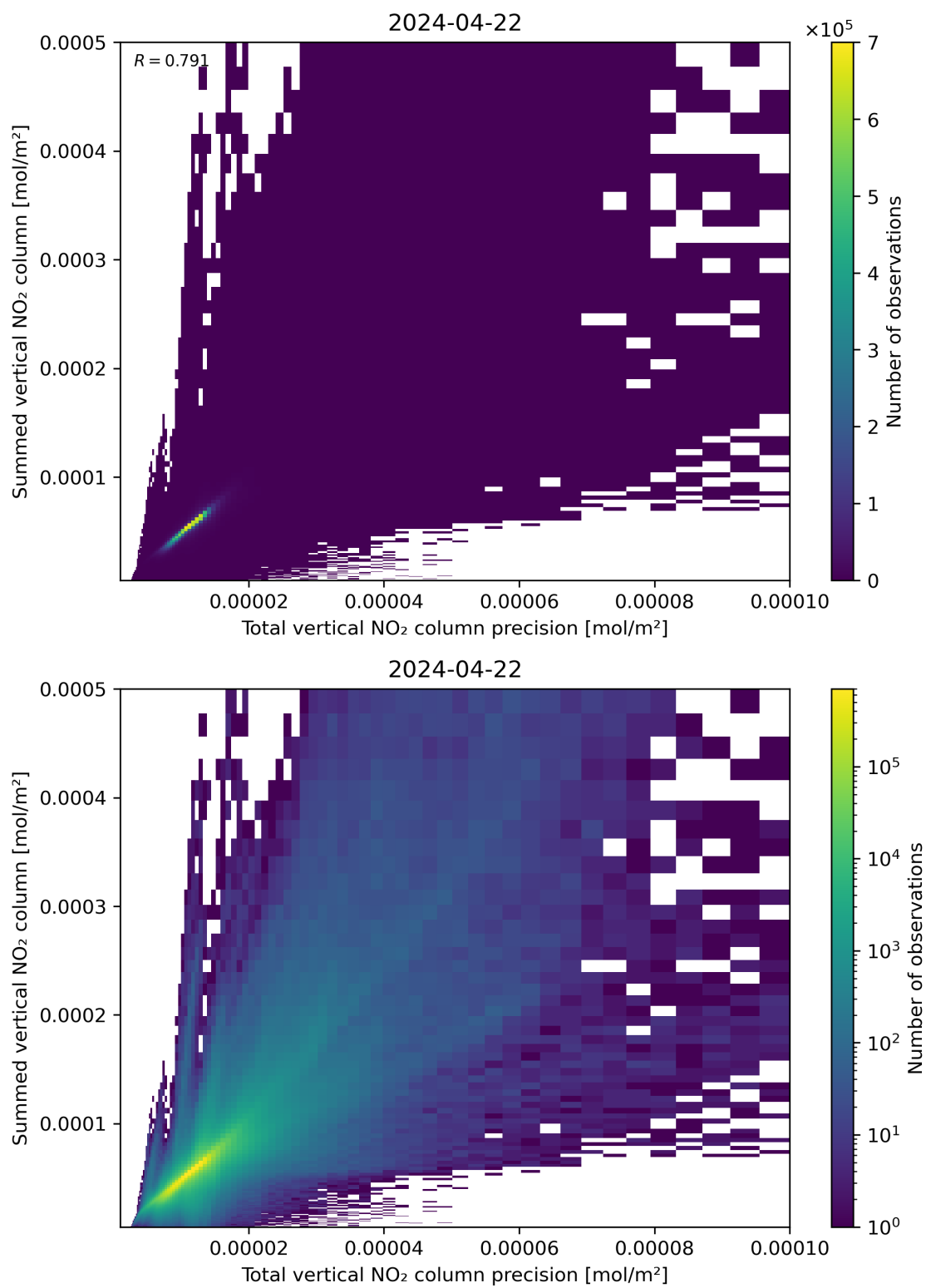
Figure 117: Scatter density plot of “Total vertical NO 2 column precision” against “Summed vertical NO 2 column” for 2024-04-21 to 2024-04-23.
