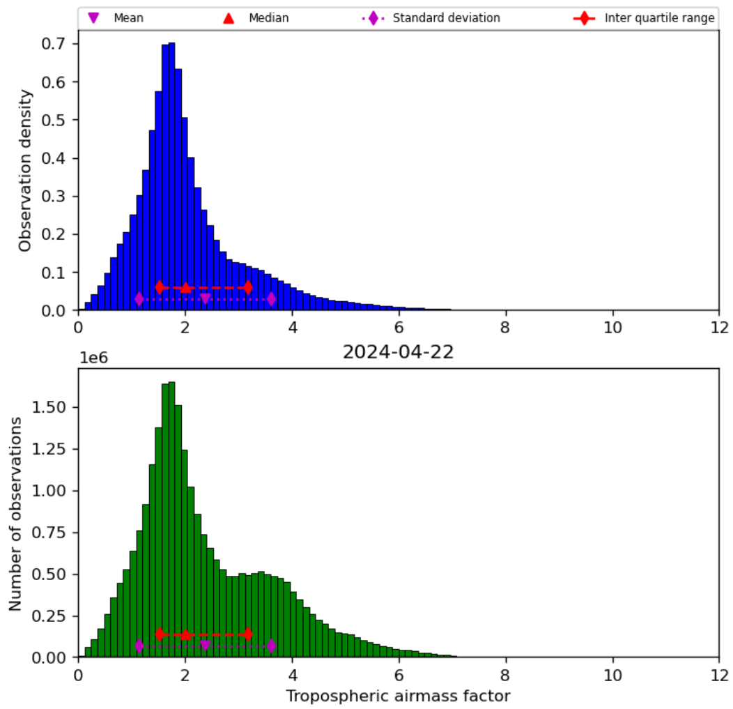
Figure 31: Histogram of “Tropospheric airmass factor” for 2024-04-21 to 2024-04-23
