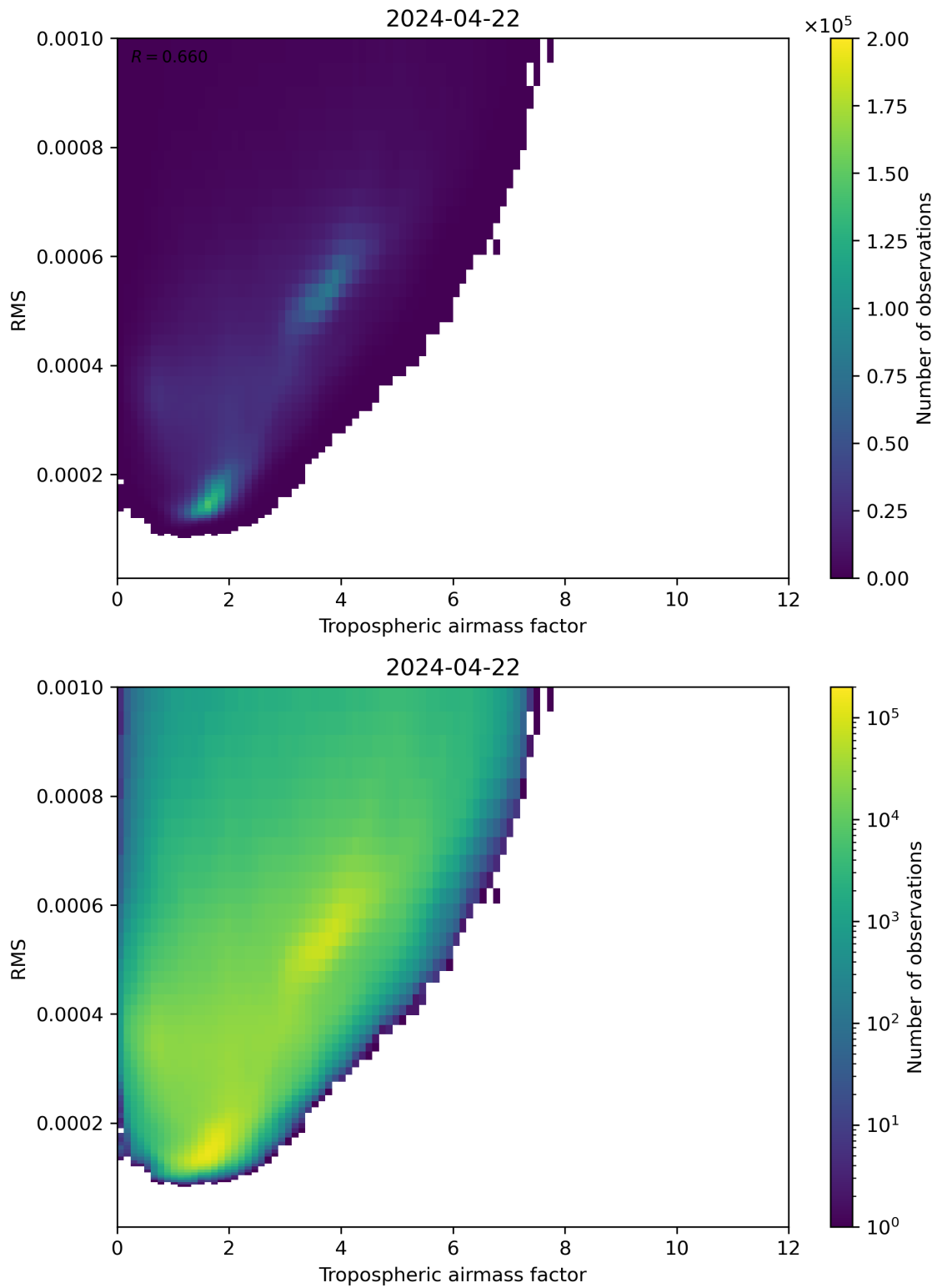
Figure 79: Scatter density plot of “Tropospheric airmass factor” against “RMS” for 2024-04-21 to 2024-04-23.
