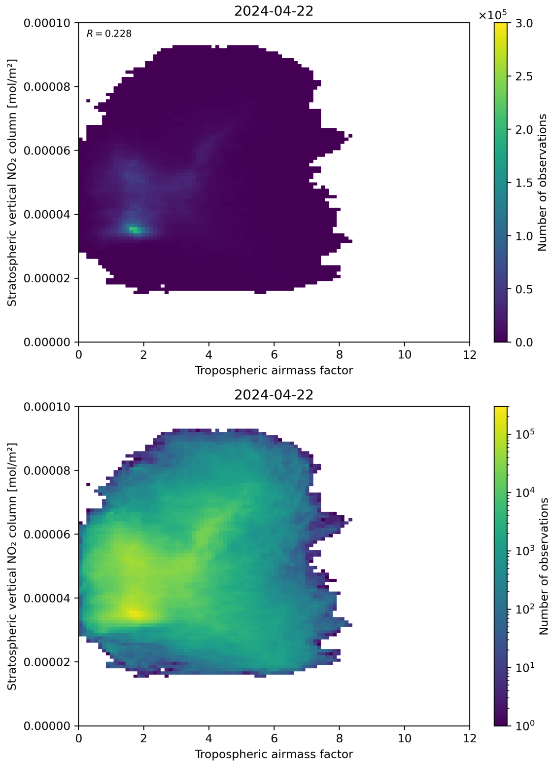
Figure 74: Scatter density plot of “Tropospheric air mass factor” against “Stratospheric vertical NO 2 column” for 2024-04-21 to 2024-04-23.
