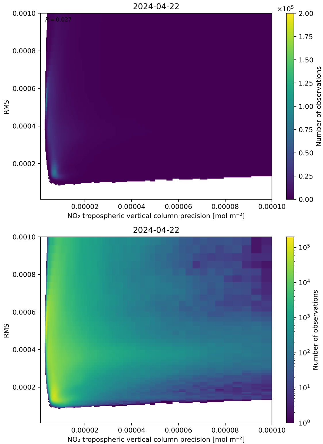
Figure 140: Scatter density plot of “NO 2 tropospheric vertical column precision” against “RMS” for 2024-04-21 to 2024-04-23.
