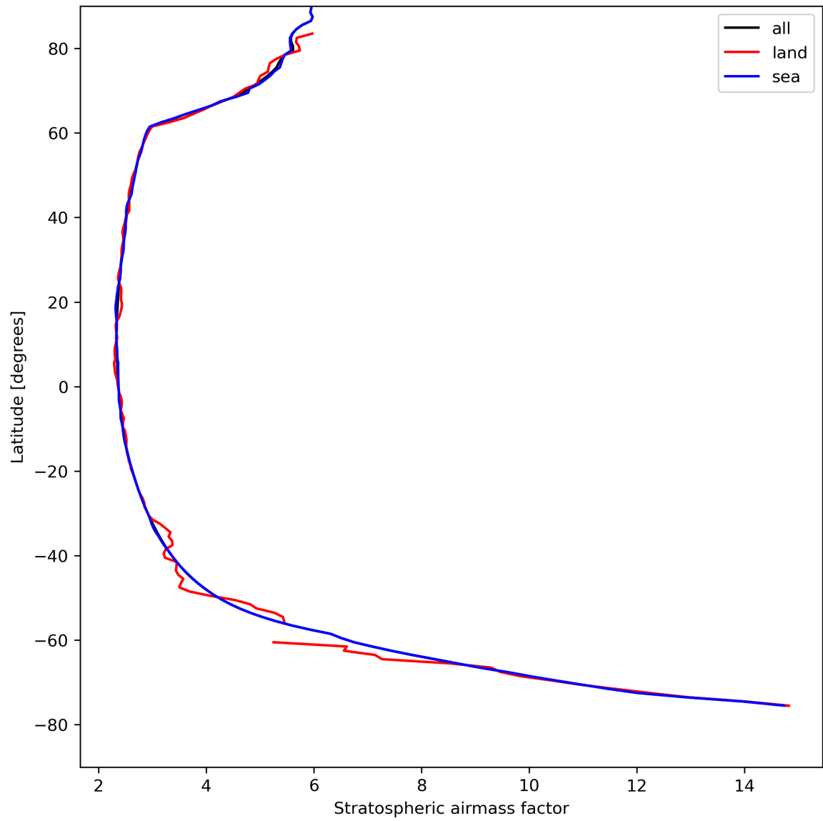
Figure 27: Zonal average of “Stratospheric air mass factor” for 2024-04-21 to 2024-04-23.
