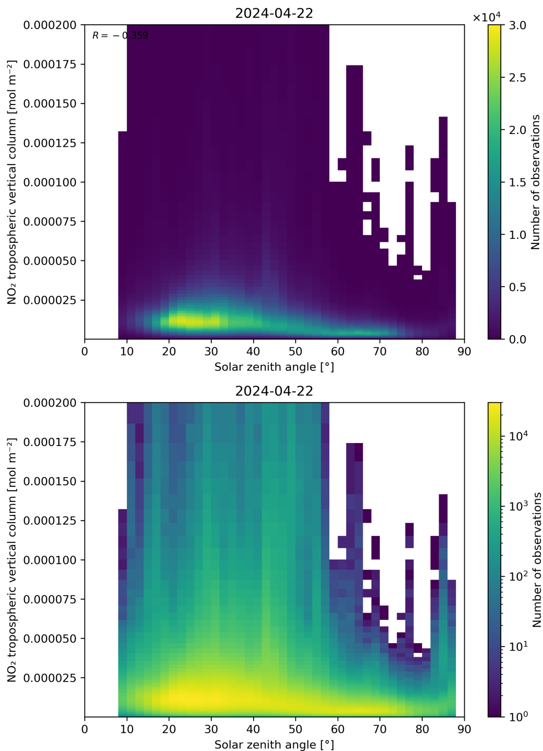
Figure 155: Scatter density plot of “Solar zenith angle” against “NO 2 tropospheric vertical column” for 2024-04-21 to 2024-04-23.
