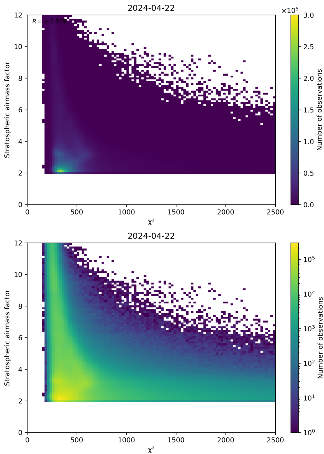
Figure 81: Scatter density plot of “ \chi^2 ” against “Stratospheric airmass factor” for 2024-04-21 to 2024-04-23.
