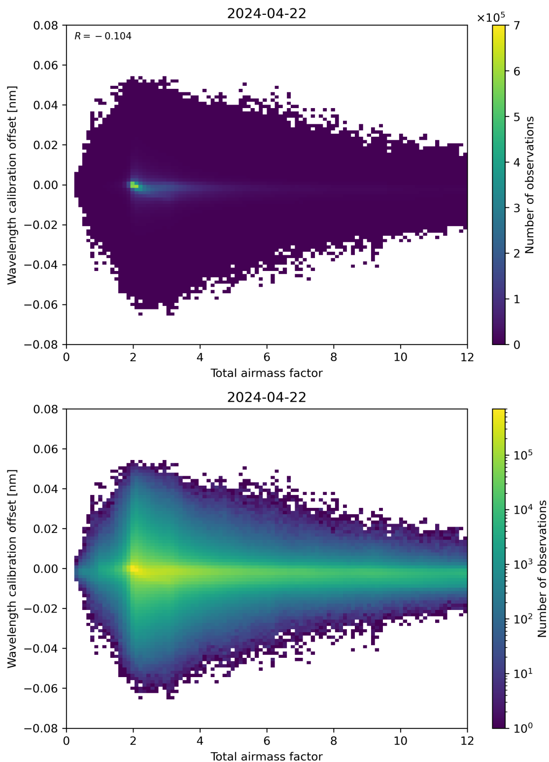
Figure 70: Scatter density plot of “Total airmass factor” against “Wavelength calibration offset” for 2024-04-21 to 2024-04-23.
