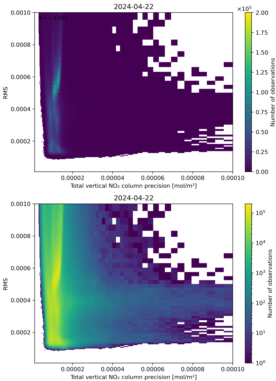
Figure 119: Scatter density plot of “Total vertical NO 2 column precision” against “RMS” for 2024-04-21 to 2024-04-23.
