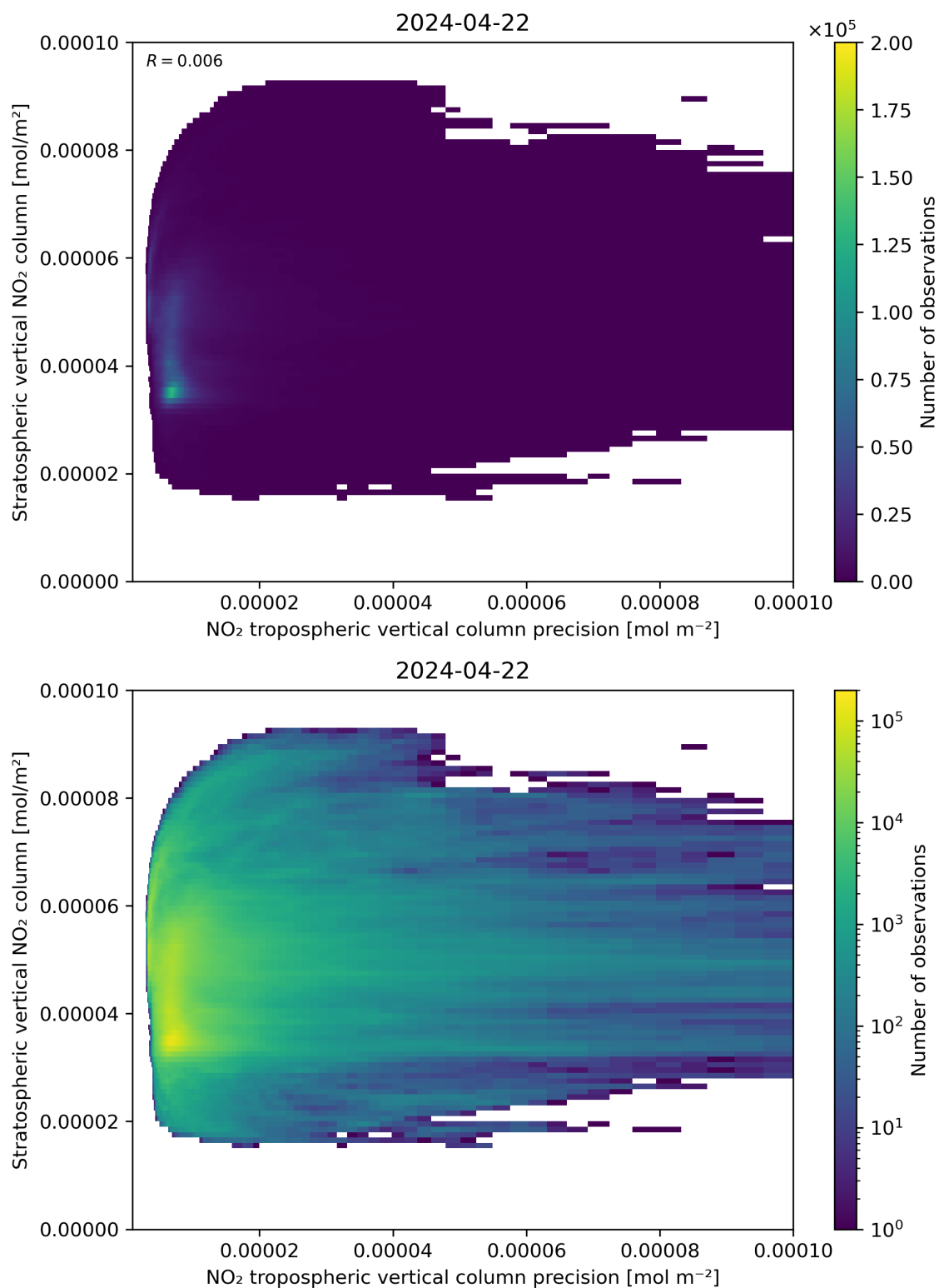
Figure 135: Scatter density plot of “NO 2 tropospheric vertical column precision” against “Stratospheric vertical NO 2 column” for 2024-04-21 to 2024-04-23.
