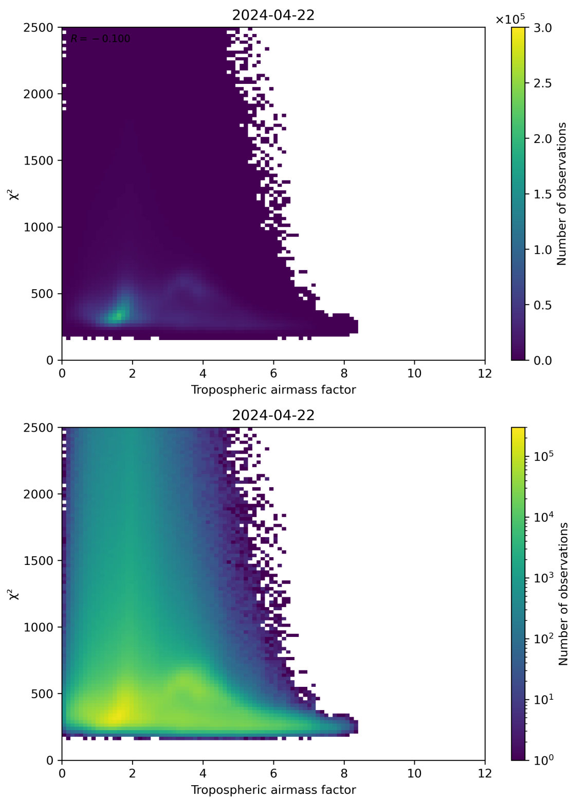
Figure 73: Scatter density plot of “Tropospheric airmass factor” against “ \chi^2 ” for 2024-04-21 to 2024-04-23.
