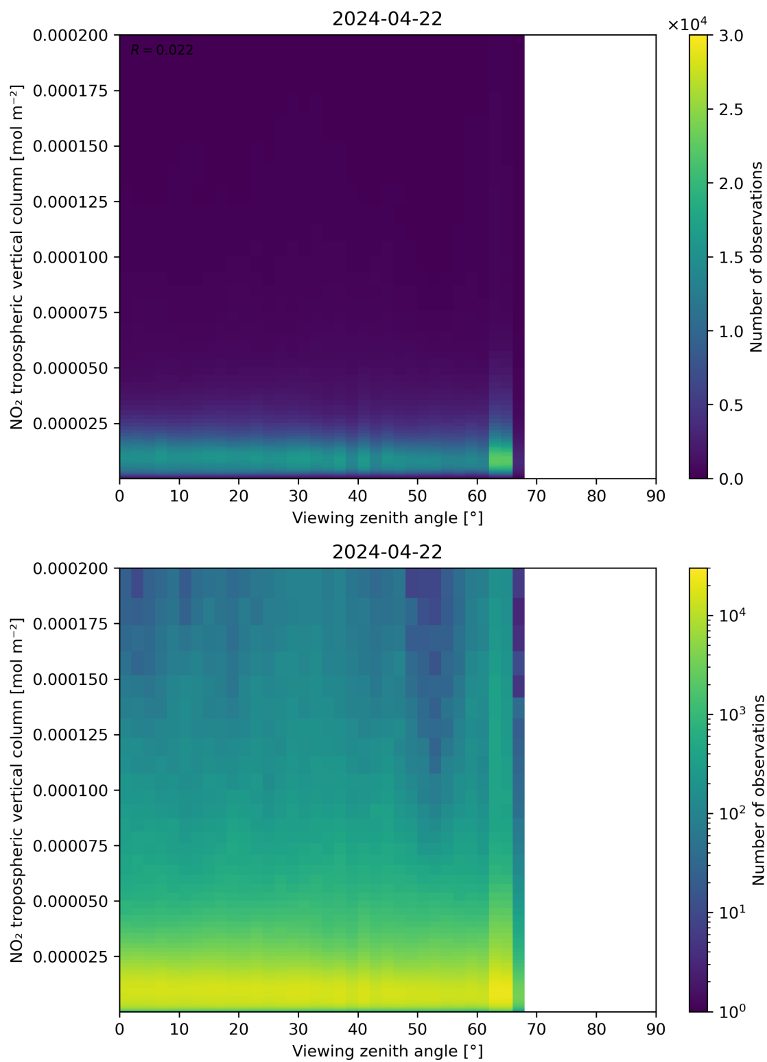
Figure 169: Scatter density plot of “Viewing zenith angle” against “NO 2 tropospheric vertical column” for 2024-04-21 to 2024-04-23.
