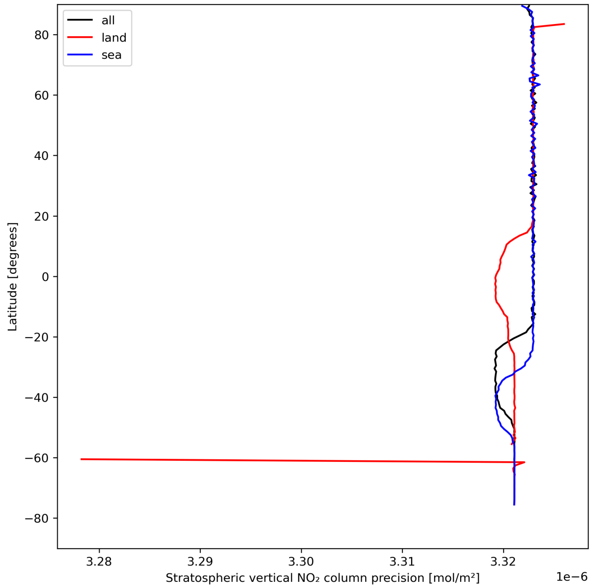
Figure 20: Zonal average of “Stratospheric vertical NO 2 column precision” for 2024-04-21 to 2024-04-23.
