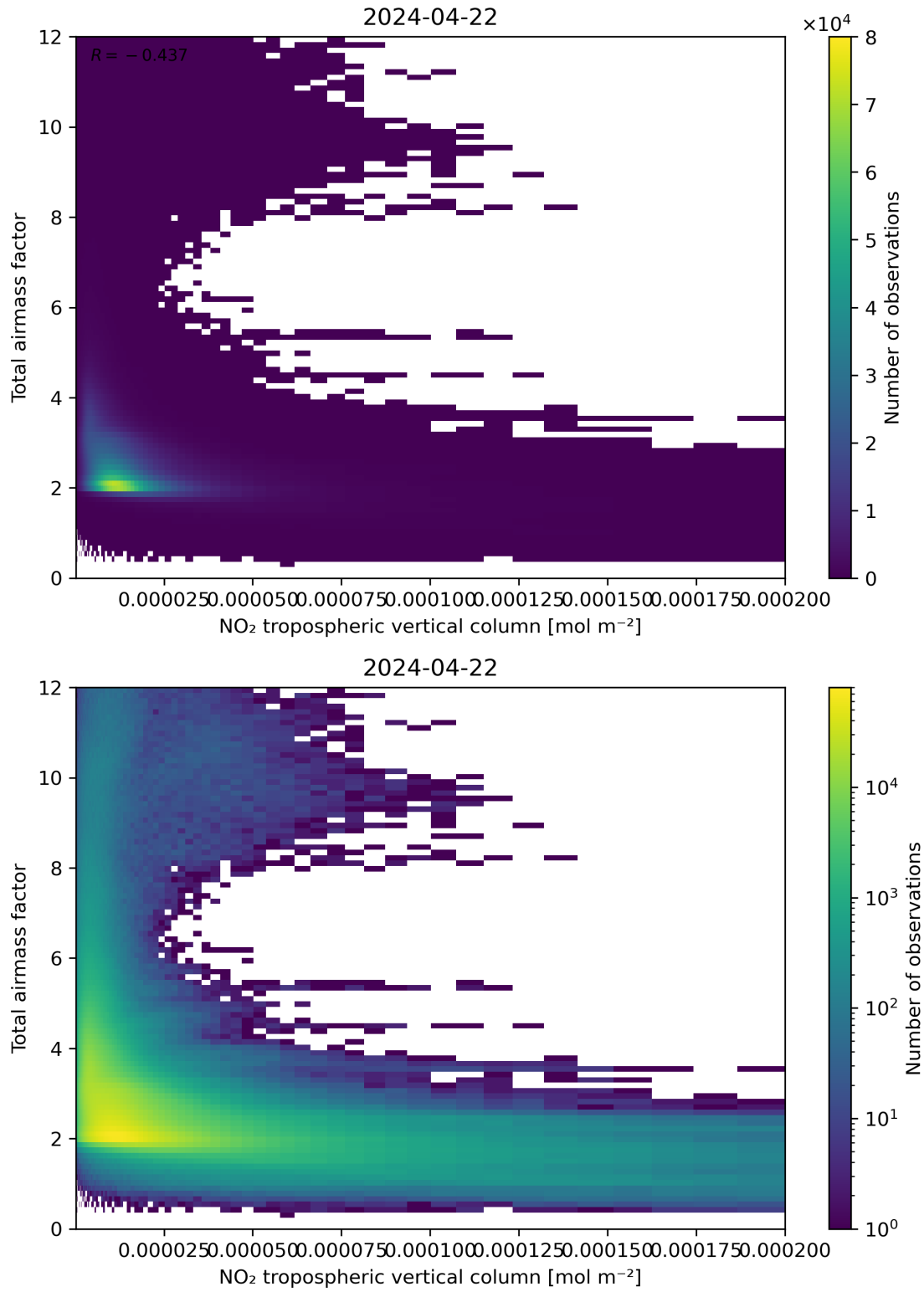
Figure 122: Scatter density plot of “NO 2 tropospheric vertical column” against “Total air mass factor” for 2024-04-21 to 2024-04-23.
