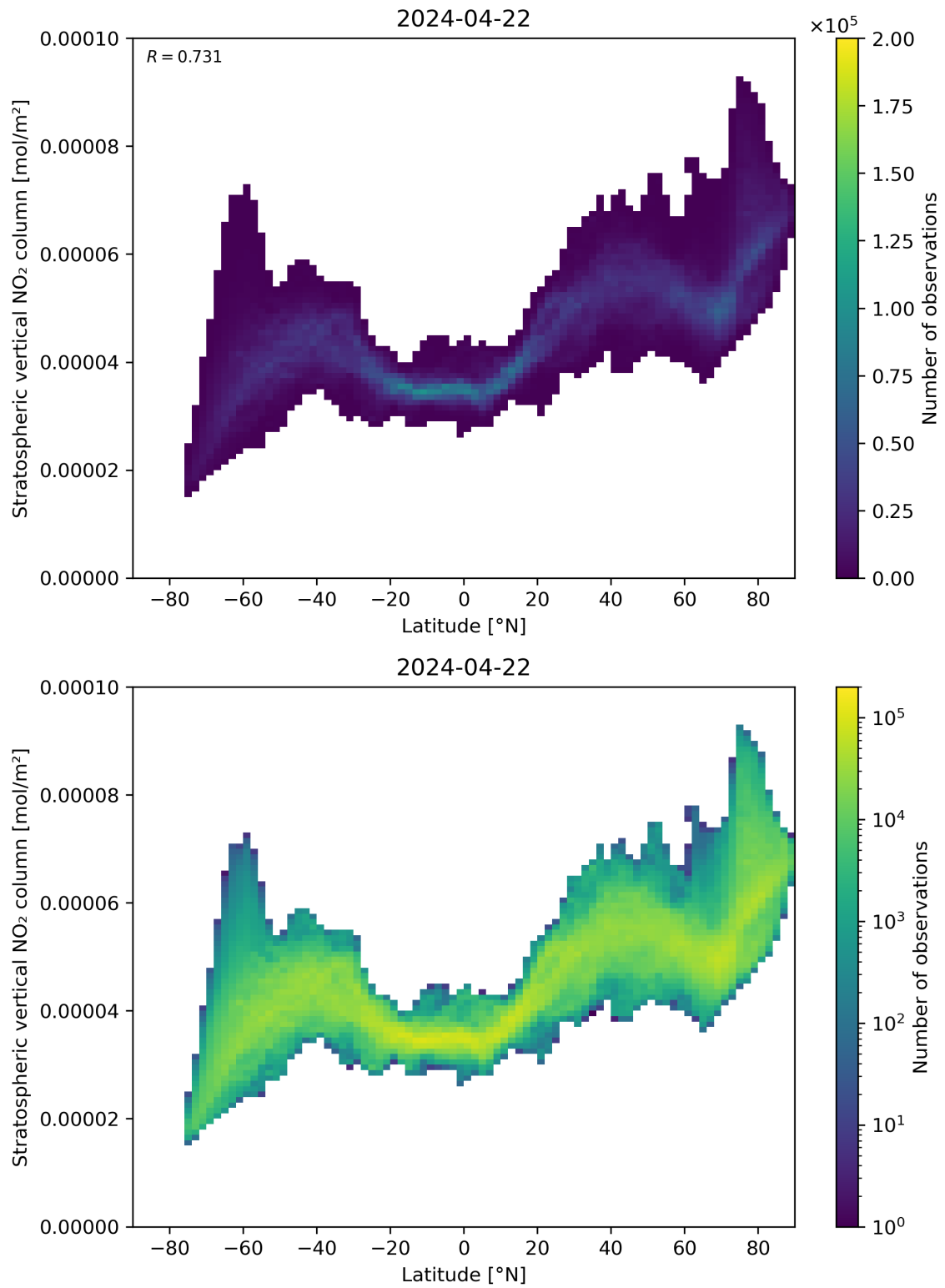
Figure 87: Scatter density plot of “Latitude” against “Stratospheric vertical NO 2 column” for 2024-04-21 to 2024-04-23.
