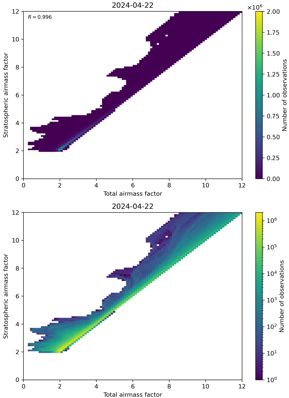
Figure 62: Scatter density plot of “Total airmass factor” against “Stratospheric airmass factor” for 2024-04-21 to 2024-04-23.
