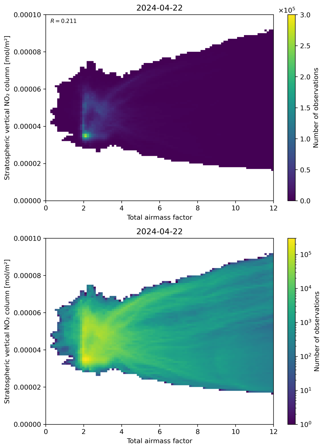
Figure 64: Scatter density plot of “Total airmass factor” against “Stratospheric vertical NO 2 column” for 2024-04-21 to 2024-04-23.
