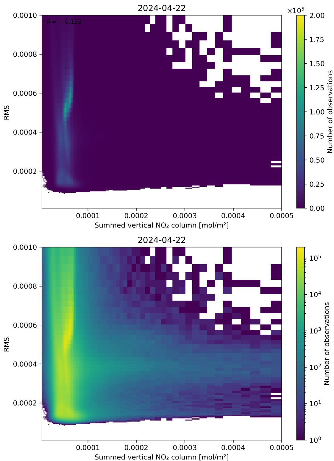
Figure 109: Scatter density plot of “Summed vertical NO 2 column” against “RMS” for 2024-04-21 to 2024-04-23.
