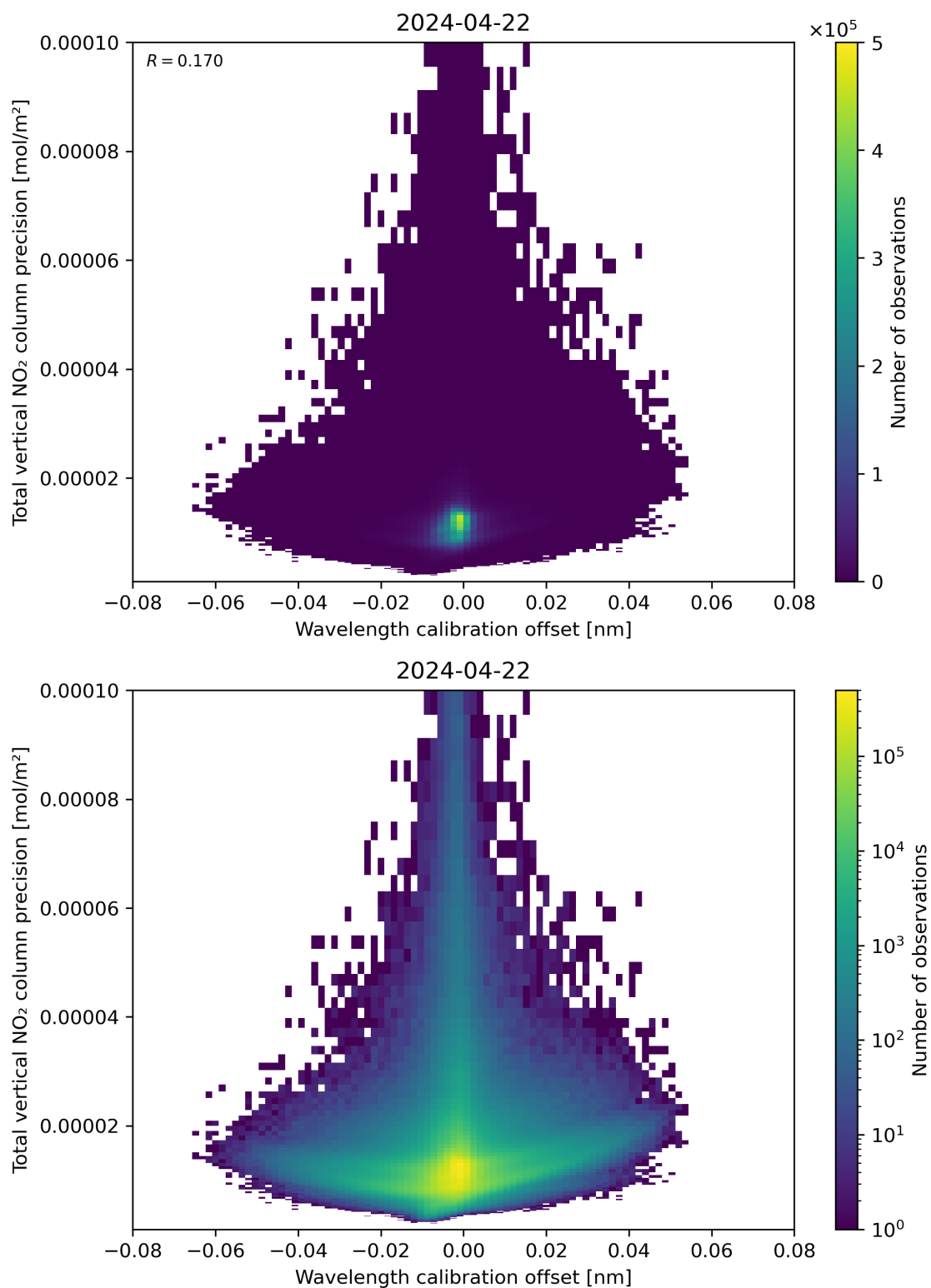
Figure 180: Scatter density plot of “Wavelength calibration offset” against “Total vertical NO 2 column precision” for 2024-04-21 to 2024-04-23.
