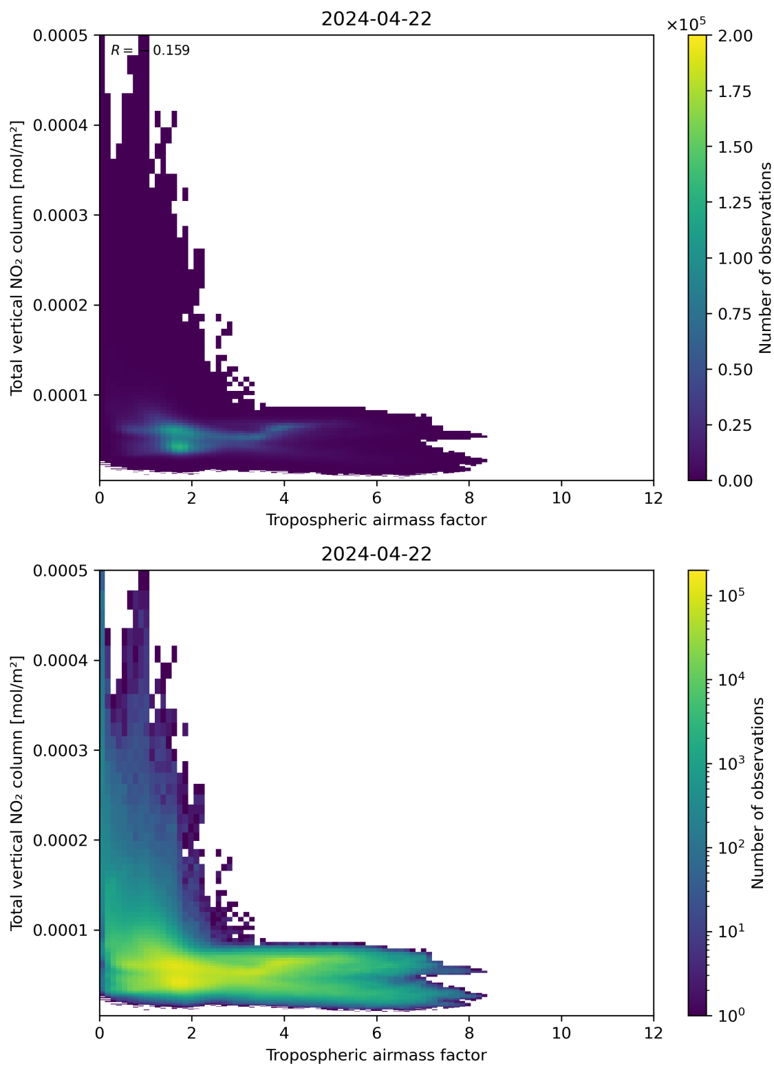
Figure 77: Scatter density plot of “Tropospheric airmass factor” against “Total vertical NO 2 column” for 2024-04-21 to 2024-04-23.
