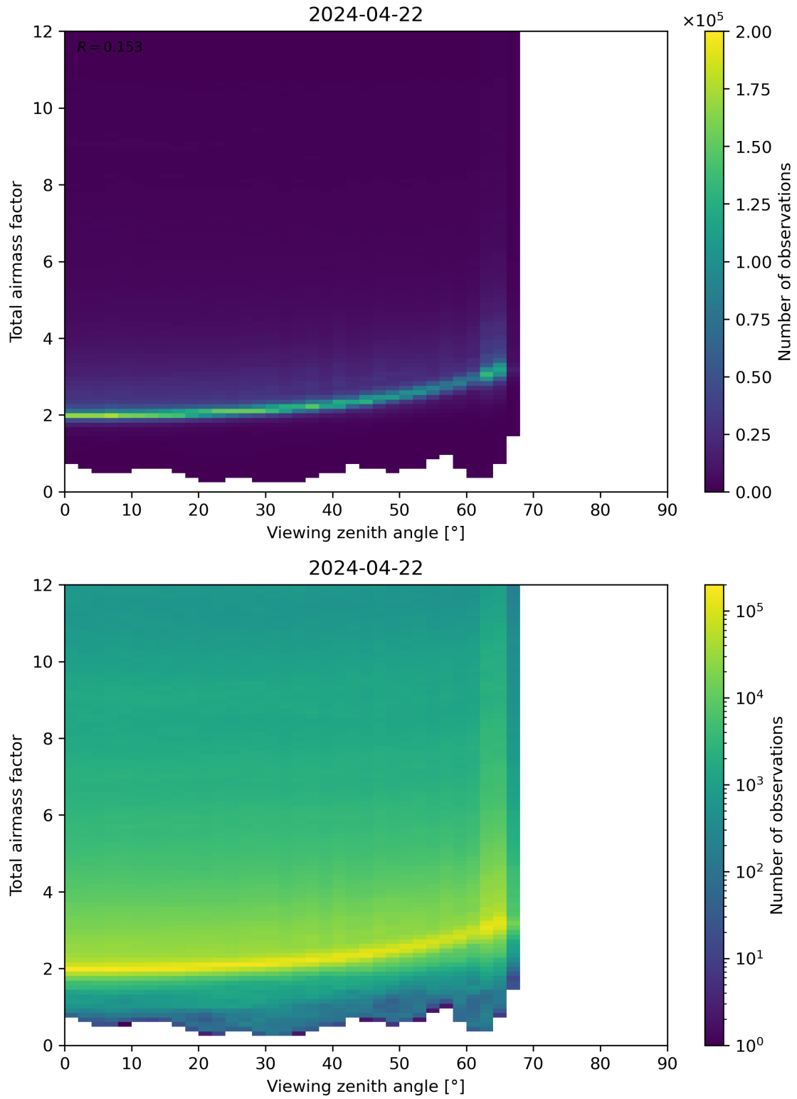
Figure 160: Scatter density plot of “Viewing zenith angle” against “Total airmass factor” for 2024-04-21 to 2024-04-23.
