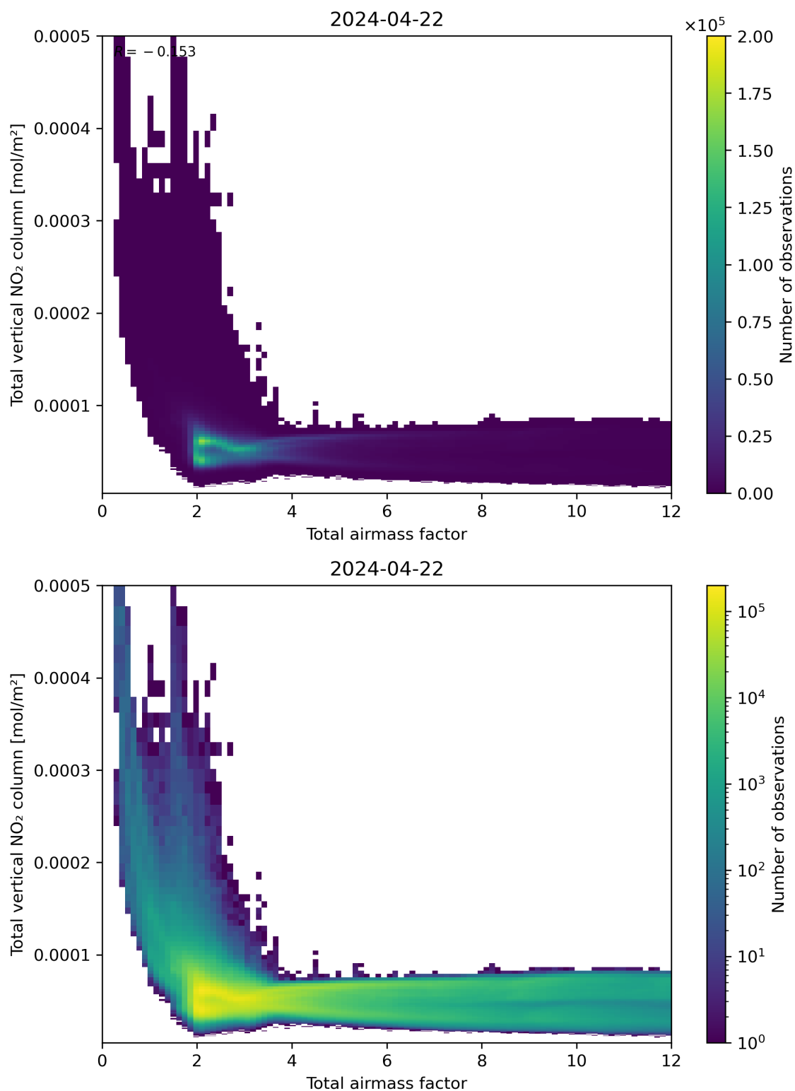
Figure 67: Scatter density plot of “Total air mass factor” against “Total vertical NO 2 column” for 2024-04-21 to 2024-04-23.
