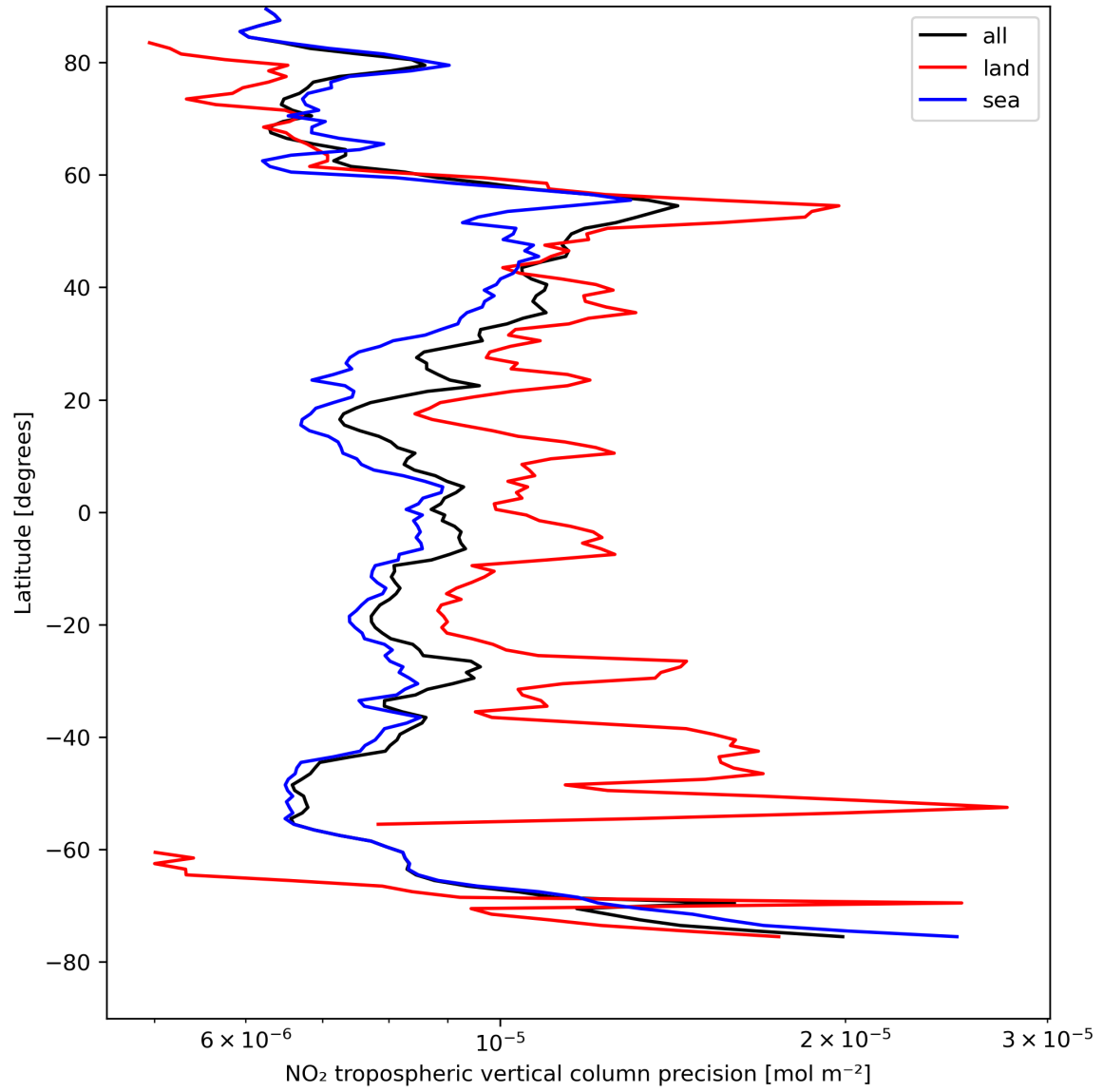
Figure 13: Zonal average of “NO 2 tropospheric vertical column precision” for 2024-04-21 to 2024-04-23.
