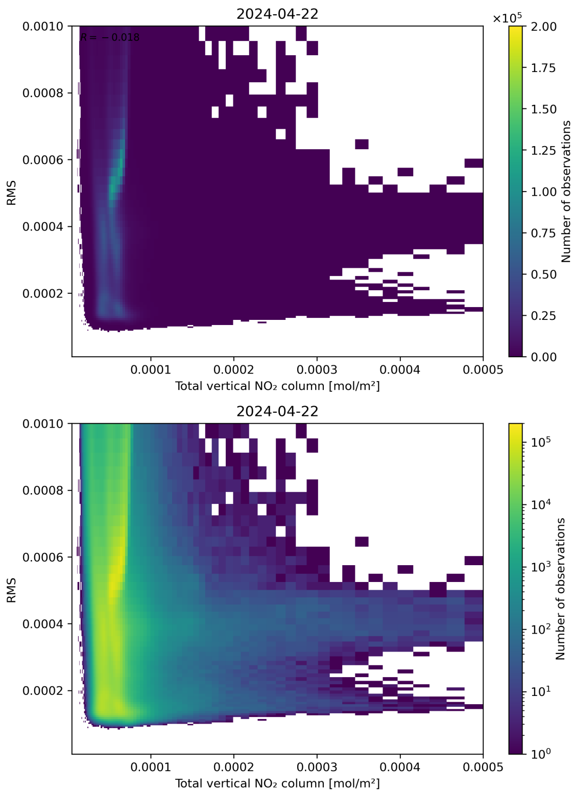
Figure 120: Scatter density plot of “Total vertical NO 2 column” against “RMS” for 2024-04-21 to 2024-04-23.
