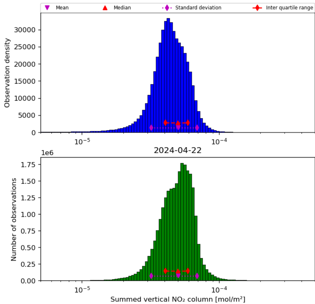
Figure 40: Histogram of “Summed vertical NO 2 column” for 2024-04-21 to 2024-04-23
