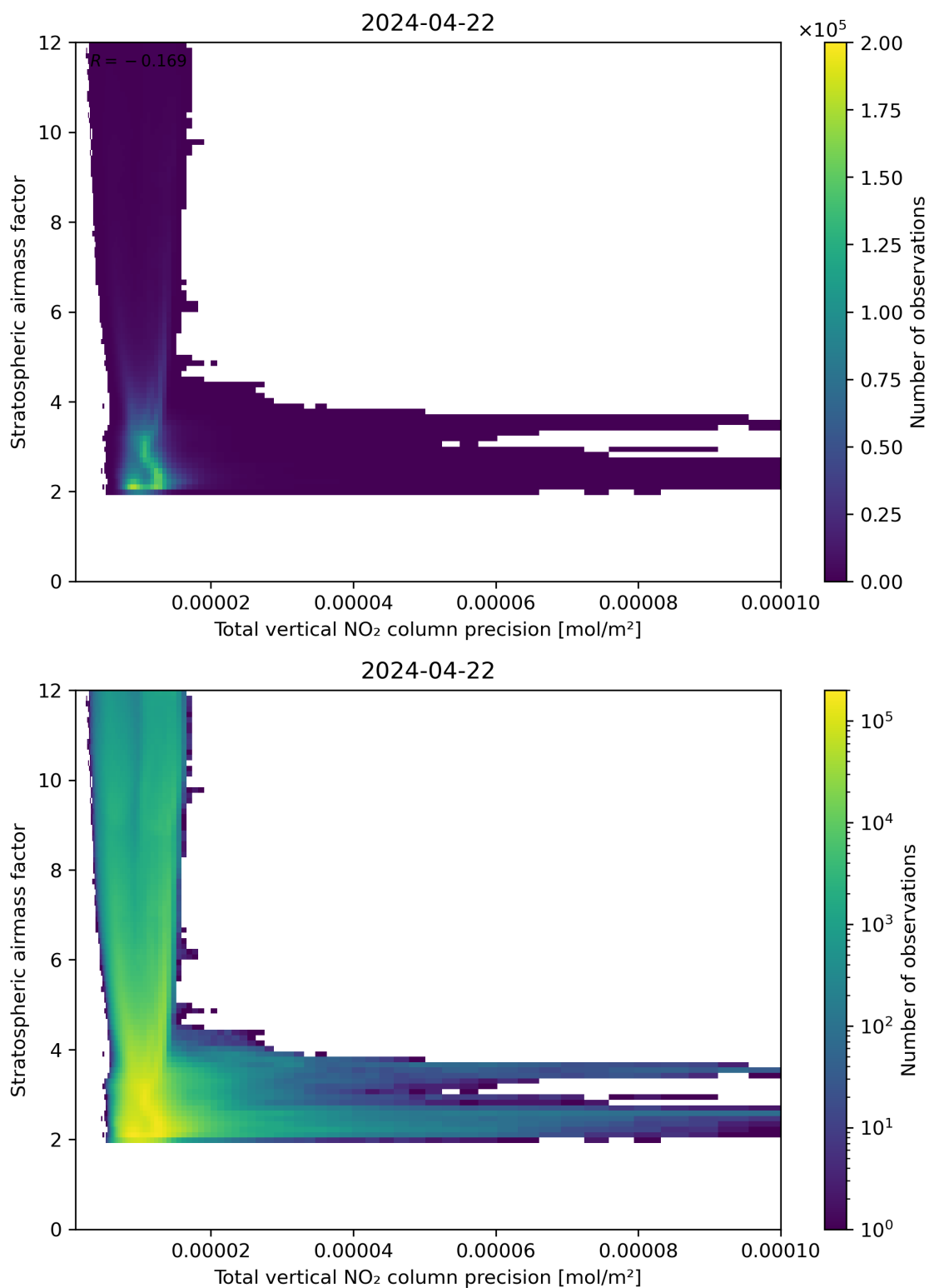
Figure 115: Scatter density plot of “Total vertical NO 2 column precision” against “Stratospheric airmass factor” for 2024-04-21 to 2024-04-23.
