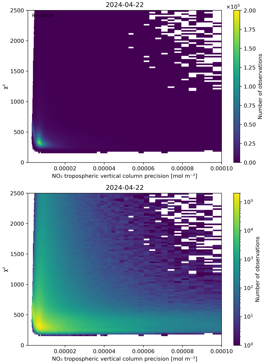
Figure 134: Scatter density plot of “NO 2 tropospheric vertical column precision” against “ \chi^2 ” for 2024-04-21 to 2024-04-23.
