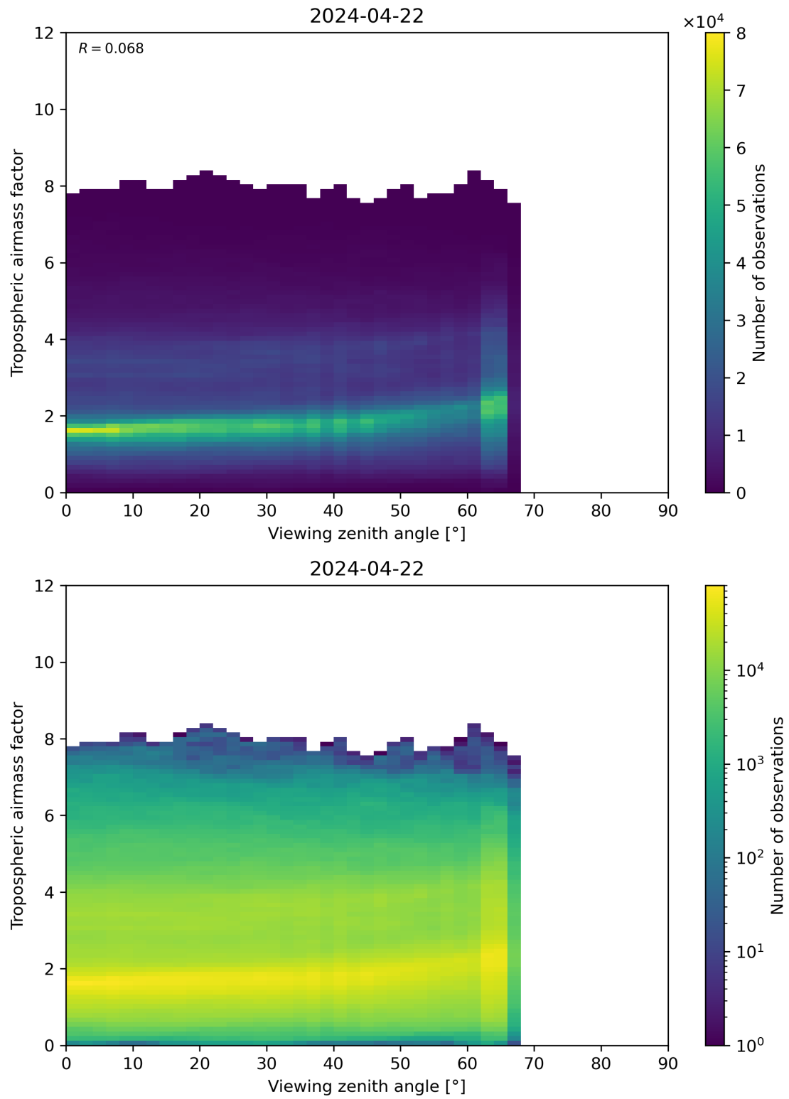
Figure 161: Scatter density plot of “Viewing zenith angle” against “Tropospheric airmass factor” for 2024-04-21 to 2024-04-23.
