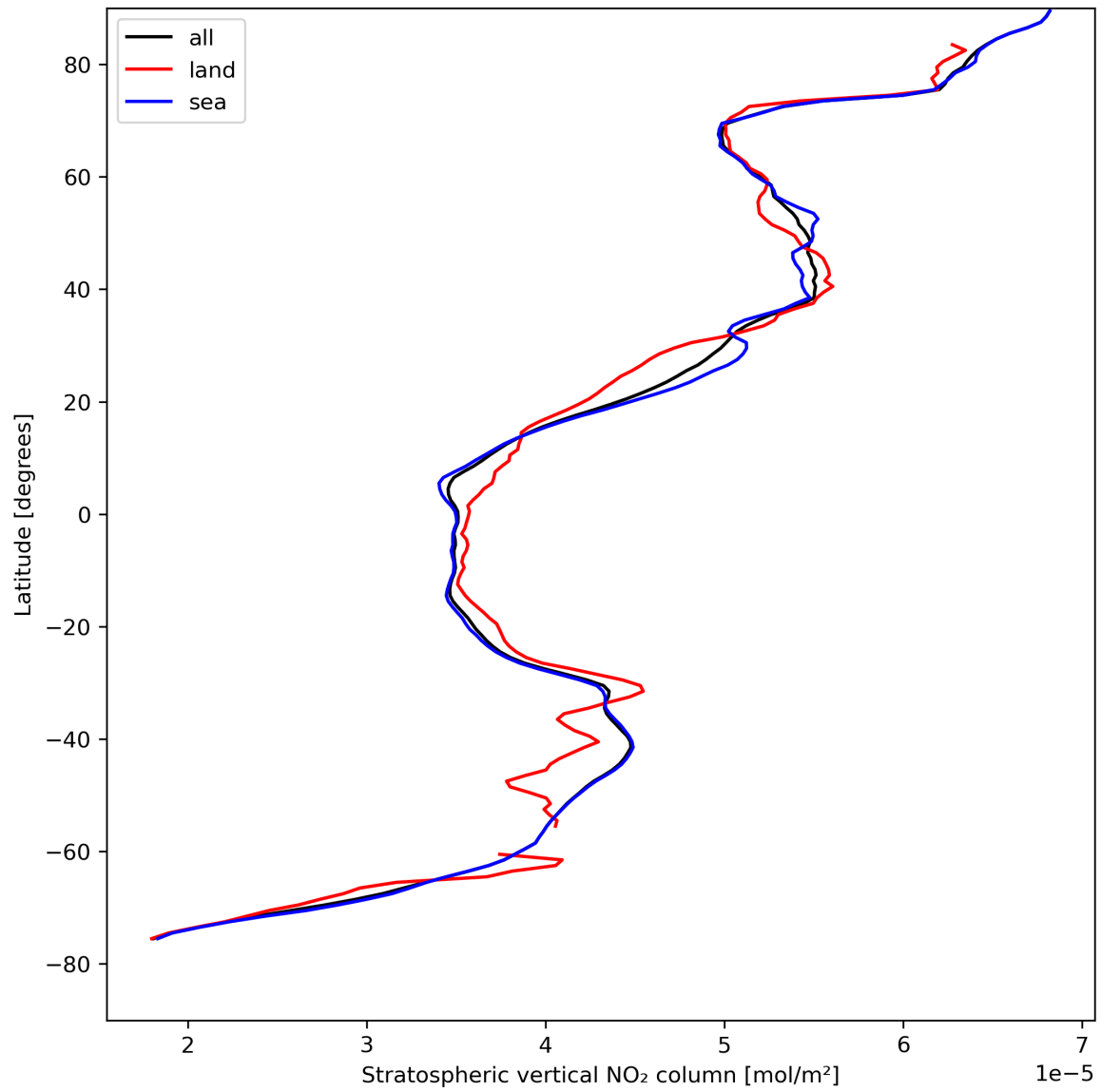
Figure 19: Zonal average of “Stratospheric vertical NO 2 column” for 2024-04-21 to 2024-04-23.
