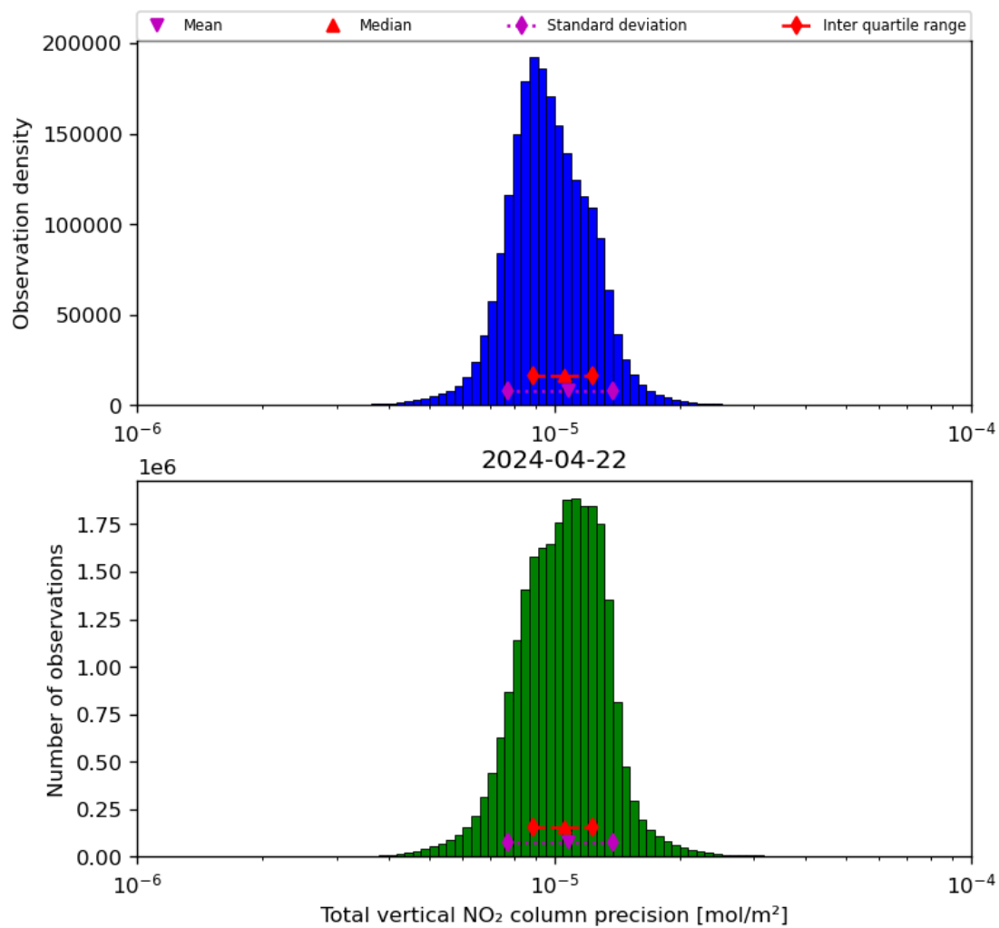
Figure 39: Histogram of “Total vertical NO 2 column precision” for 2024-04-21 to 2024-04-23
