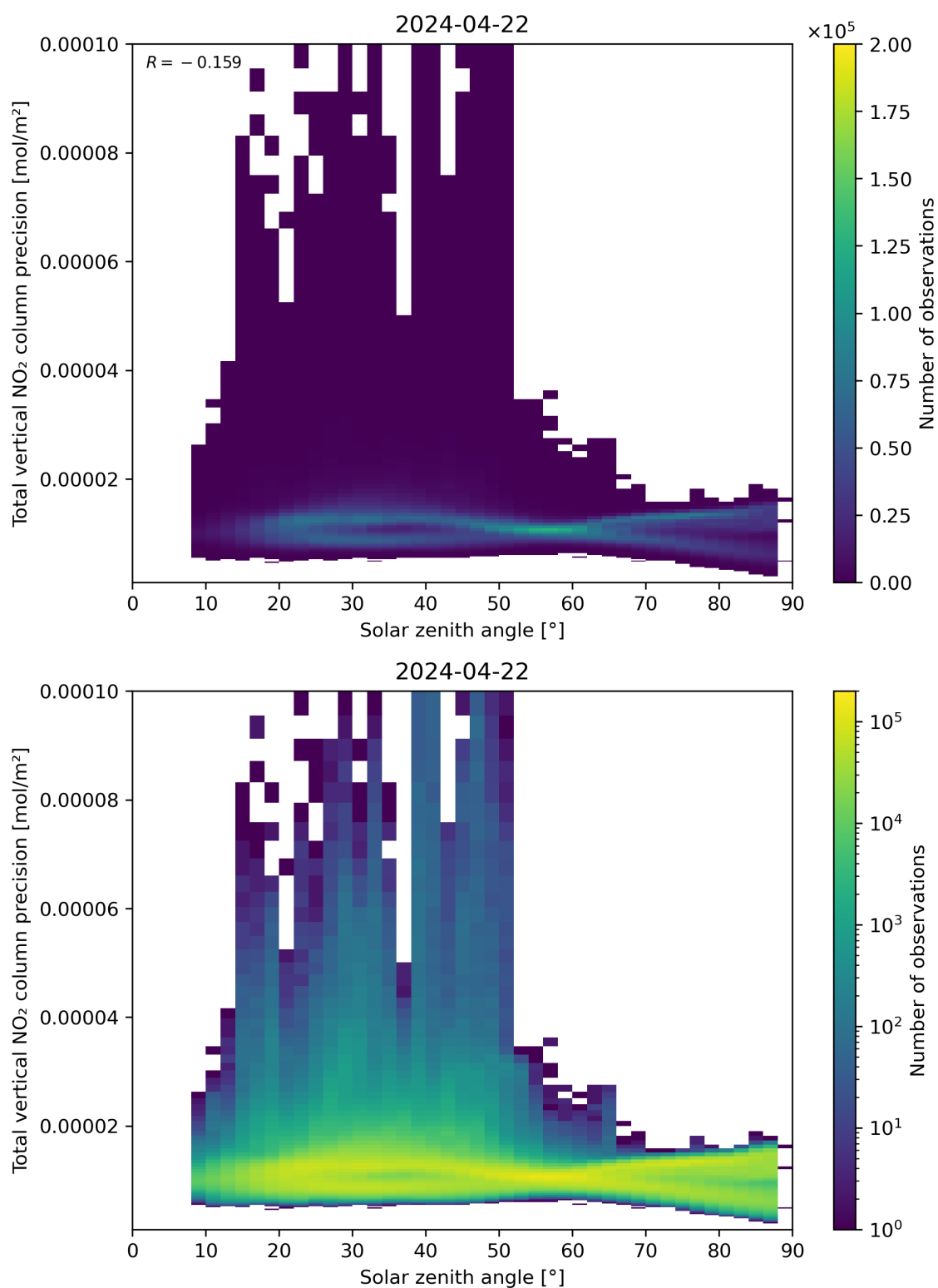
Figure 154: Scatter density plot of “Solar zenith angle” against “Total vertical NO 2 column precision” for 2024-04-21 to 2024-04-23.
