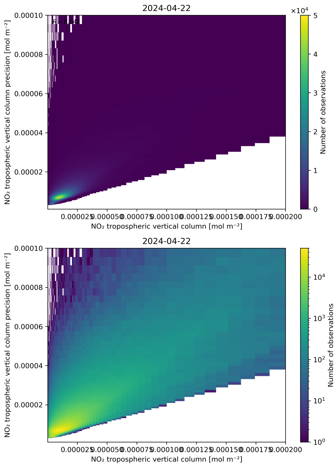
Figure 130: Scatter density plot of “NO 2 tropospheric vertical column” against “NO 2 tropospheric vertical column precision” for 2024-04-21 to 2024-04-23.
