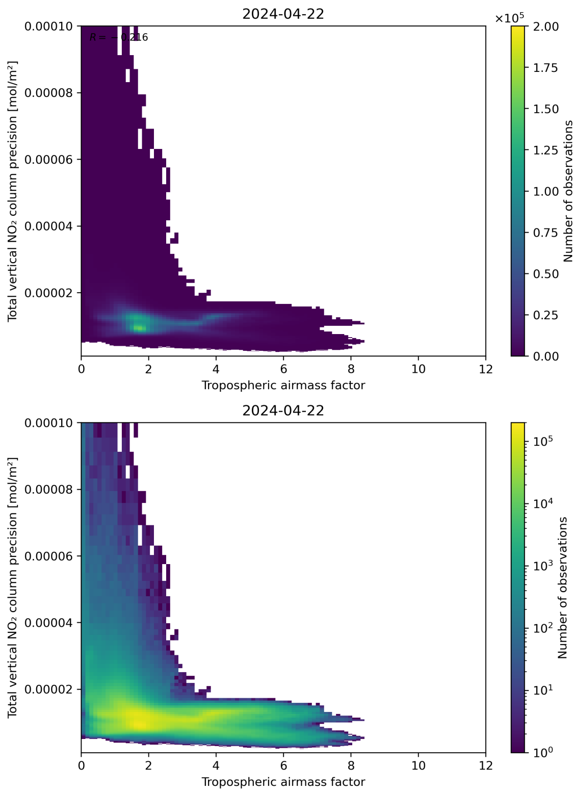
Figure 78: Scatter density plot of “Tropospheric air mass factor” against “Total vertical NO 2 column precision” for 2024-04-21 to 2024-04-23.
