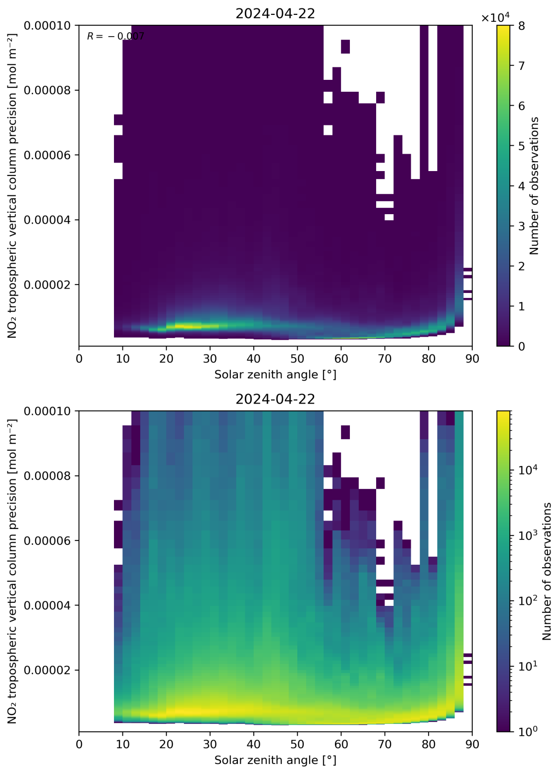
Figure 156: Scatter density plot of “Solar zenith angle” against “NO 2 tropospheric vertical column precision” for 2024-04-21 to 2024-04-23.
