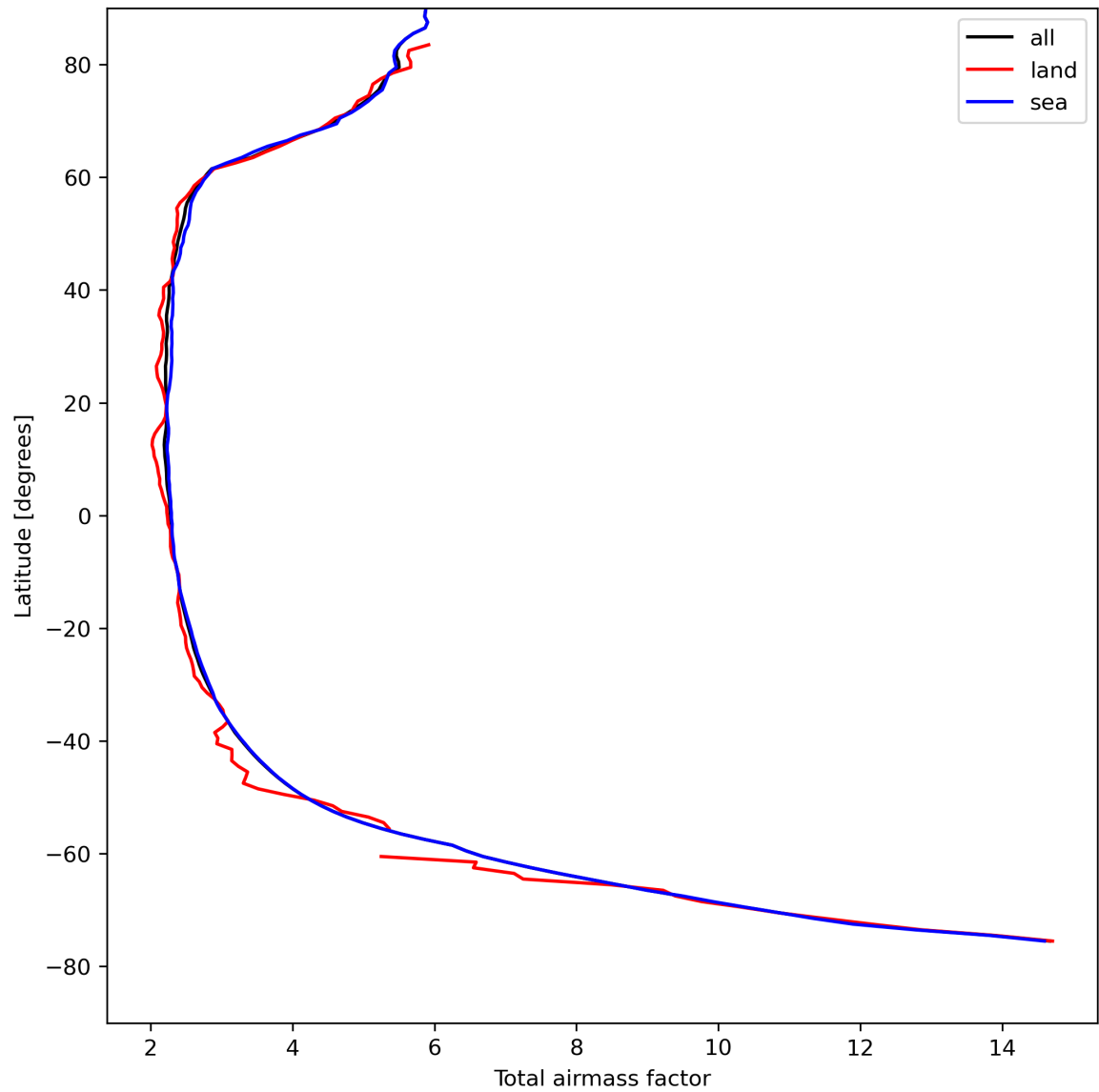
Figure 15: Zonal average of “Total airmass factor” for 2024-04-21 to 2024-04-23.
