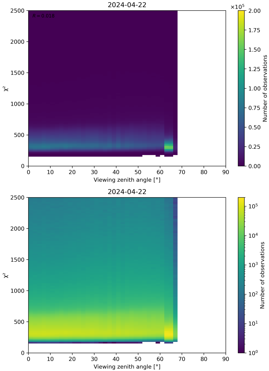
Figure 162: Scatter density plot of “Viewing zenith angle” against “ \chi^2 ” for 2024-04-21 to 2024-04-23.
