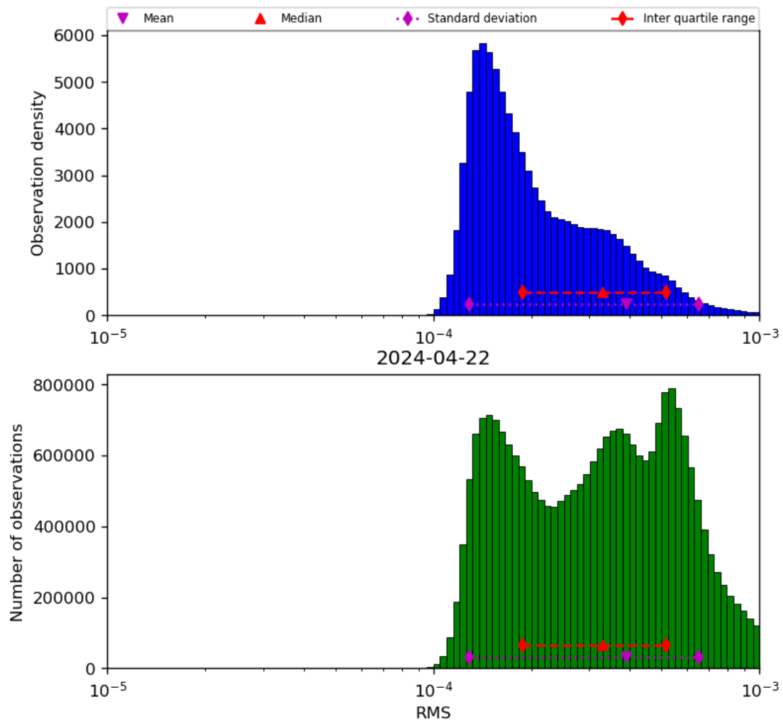
Figure 43: Histogram of “RMS” for 2024-04-21 to 2024-04-23
