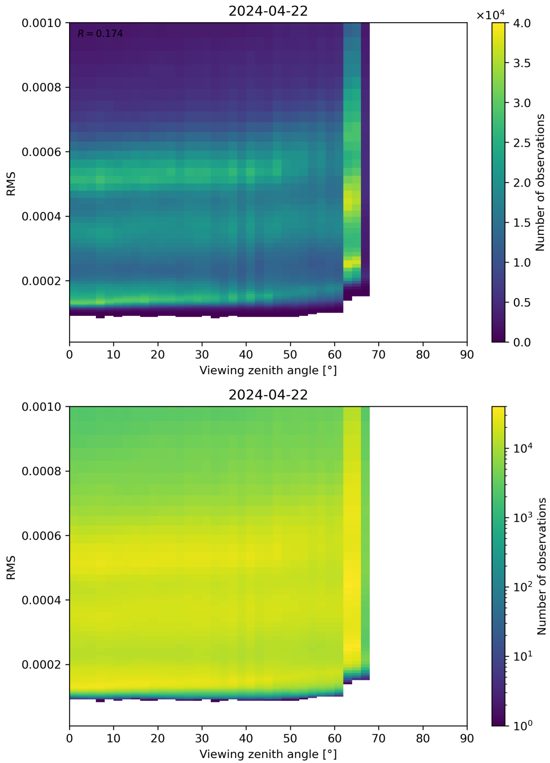
Figure 171: Scatter density plot of “Viewing zenith angle” against “RMS” for 2024-04-21 to 2024-04-23.
