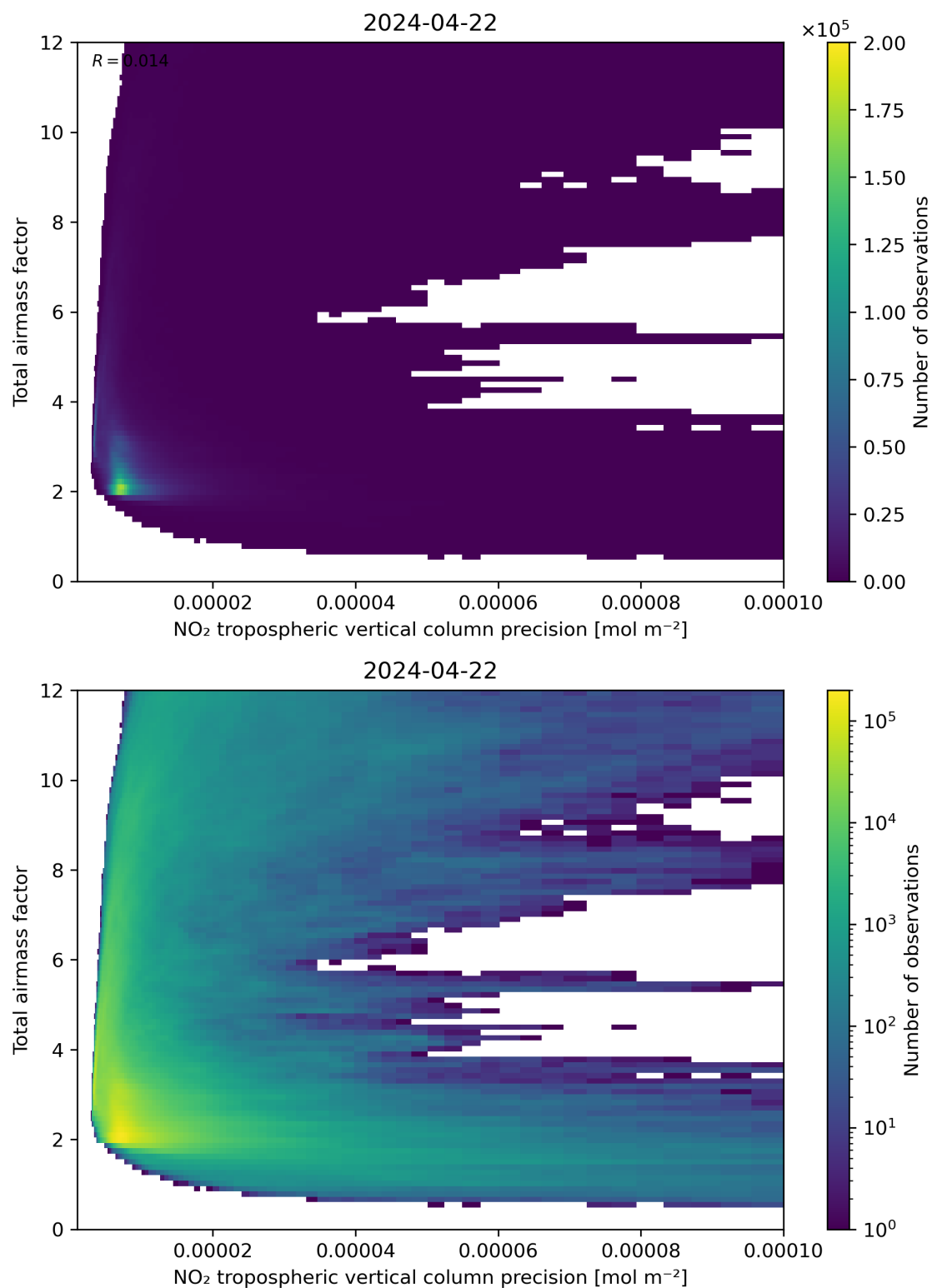
Figure 132: Scatter density plot of “NO 2 tropospheric vertical column precision” against “Total air mass factor” for 2024-04-21 to 2024-04-23.
