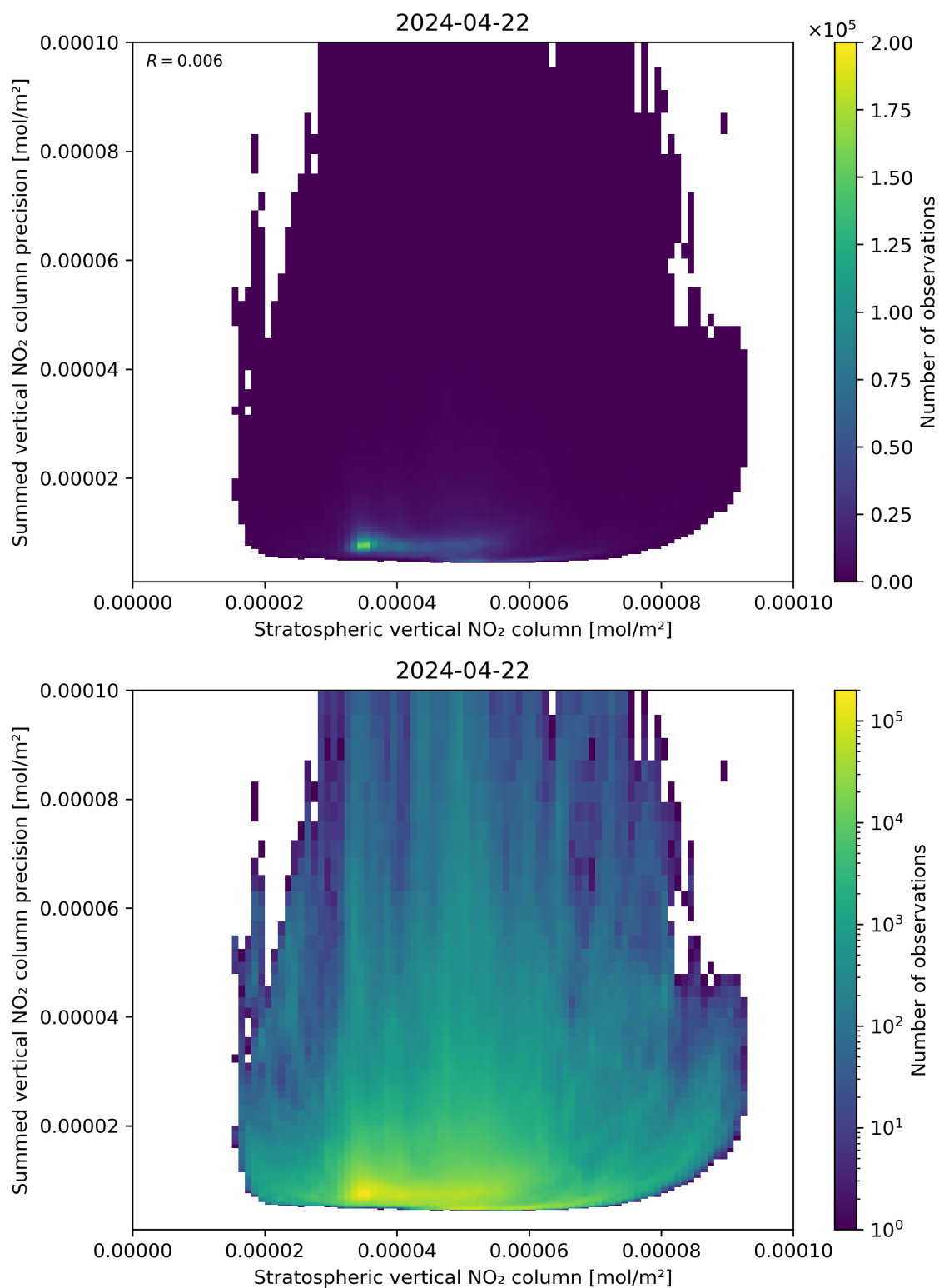
Figure 99: Scatter density plot of “Stratospheric vertical NO 2 column” against “Summed vertical NO 2 column precision” for 2024-04-21 to 2024-04-23.
