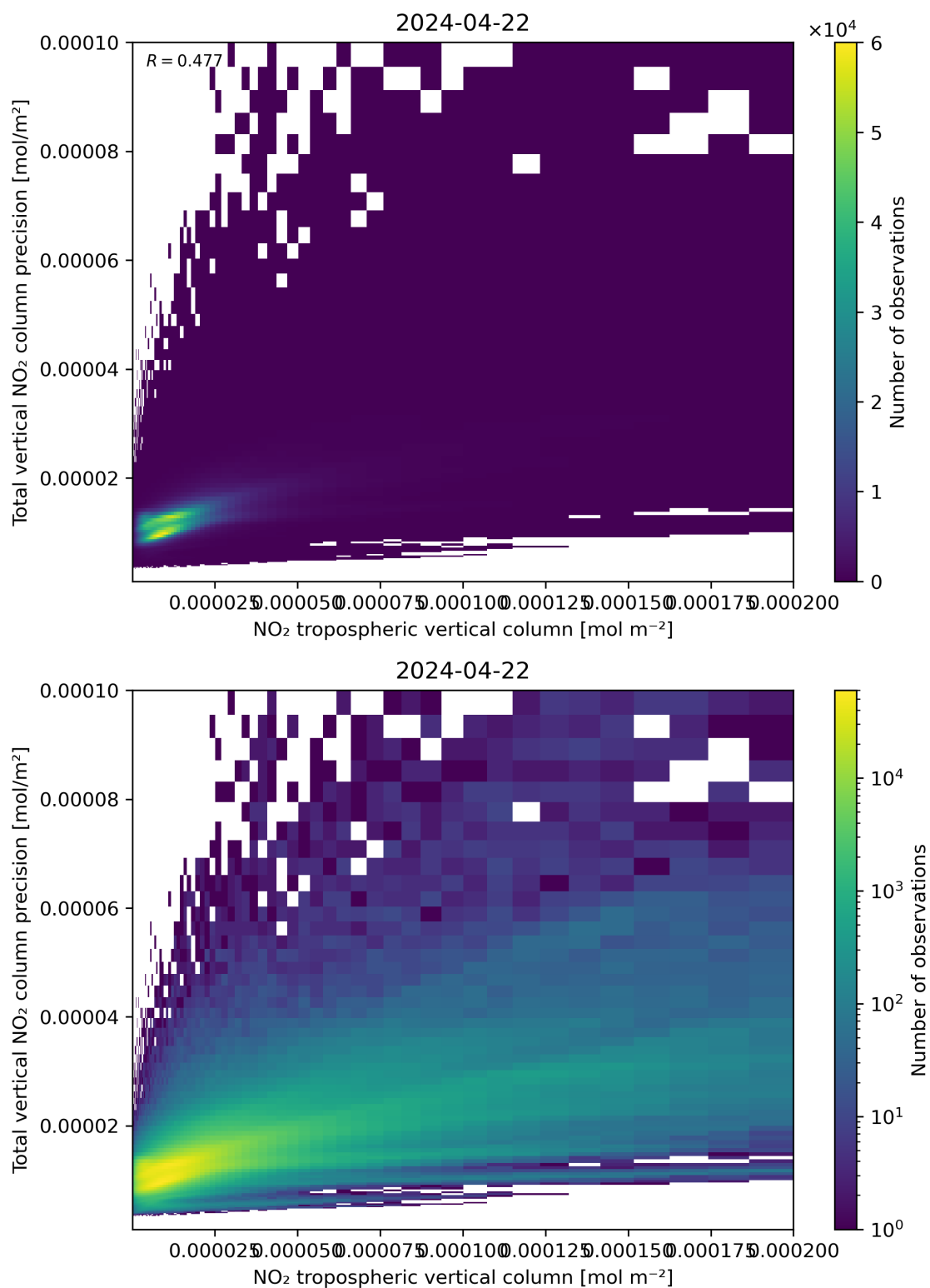
Figure 129: Scatter density plot of “NO 2 tropospheric vertical column” against “Total vertical NO 2 column precision” for 2024-04-21 to 2024-04-23.
