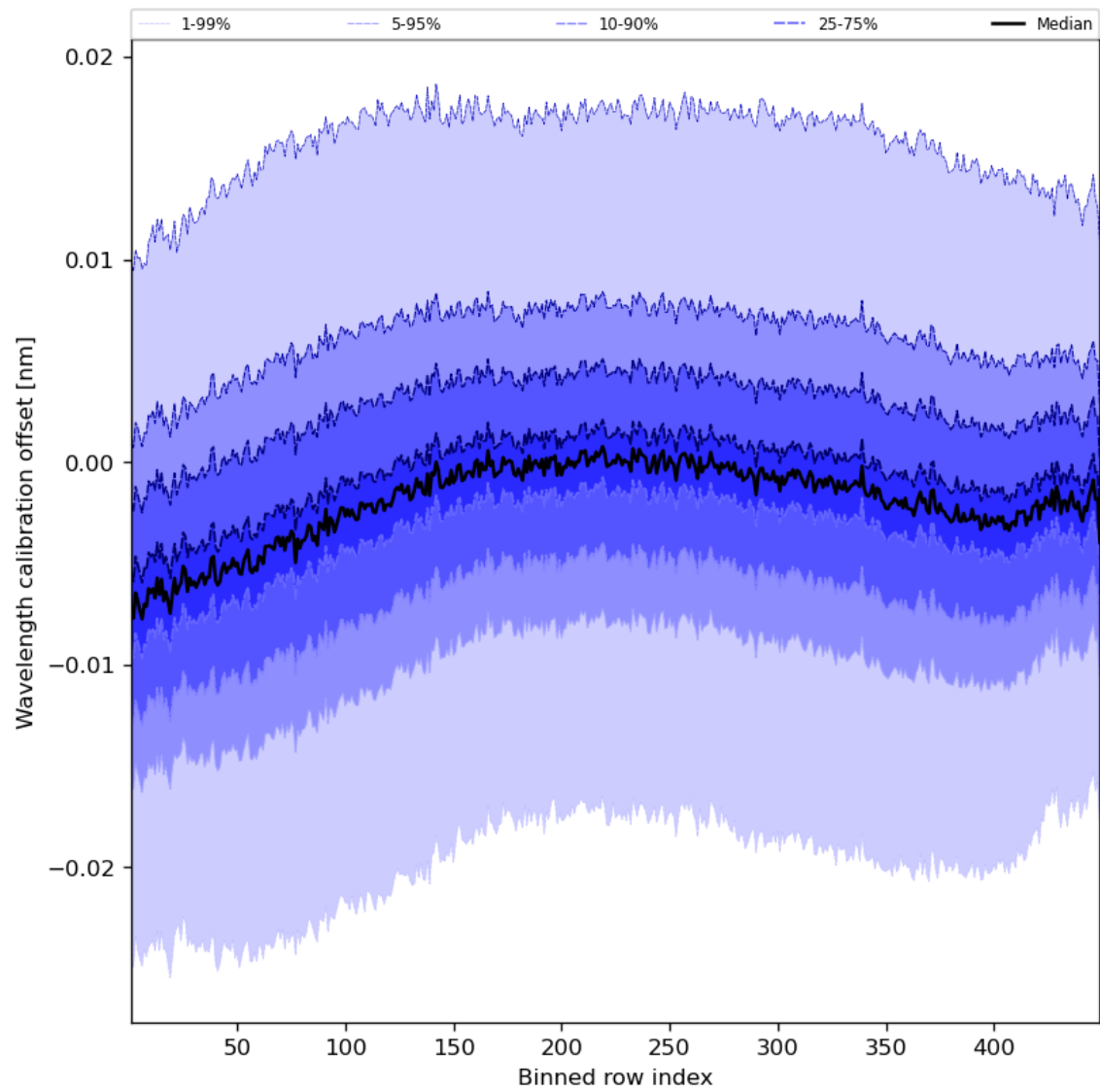
Figure 52: Along track statistics of “Wavelength calibration offset” for 2024-04-21 to 2024-04-23
