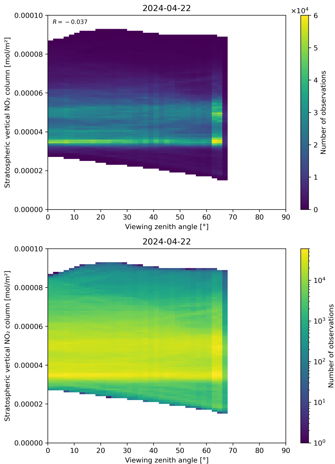
Figure 164: Scatter density plot of “Viewing zenith angle” against “Stratospheric vertical NO 2 column” for 2024-04-21 to 2024-04-23.
