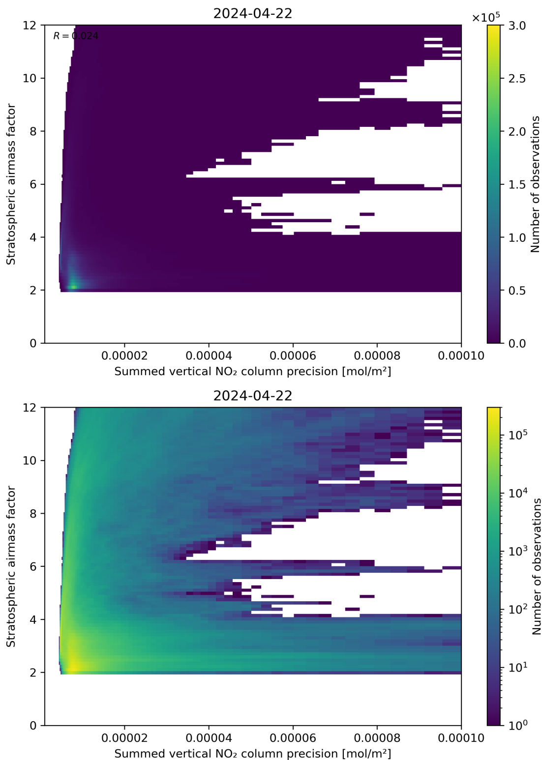
Figure 106: Scatter density plot of “Summed vertical NO 2 column precision” against “Stratospheric airmass factor” for 2024-04-21 to 2024-04-23.
