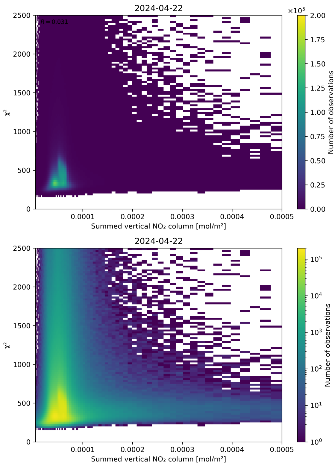
Figure 104: Scatter density plot of “Summed vertical NO 2 column” against “ \chi^2 ” for 2024-04-21 to 2024-04-23.
