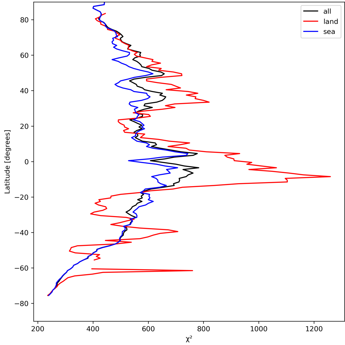
Figure 25: Zonal average of “ \chi^2 ” for 2024-04-21 to 2024-04-23.
