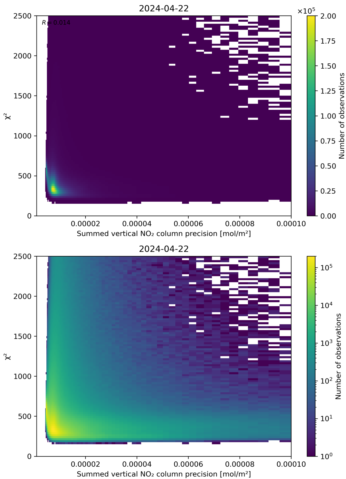
Figure 107: Scatter density plot of “Summed vertical NO 2 column precision” against “ \chi^2 ” for 2024-04-21 to 2024-04-23.
