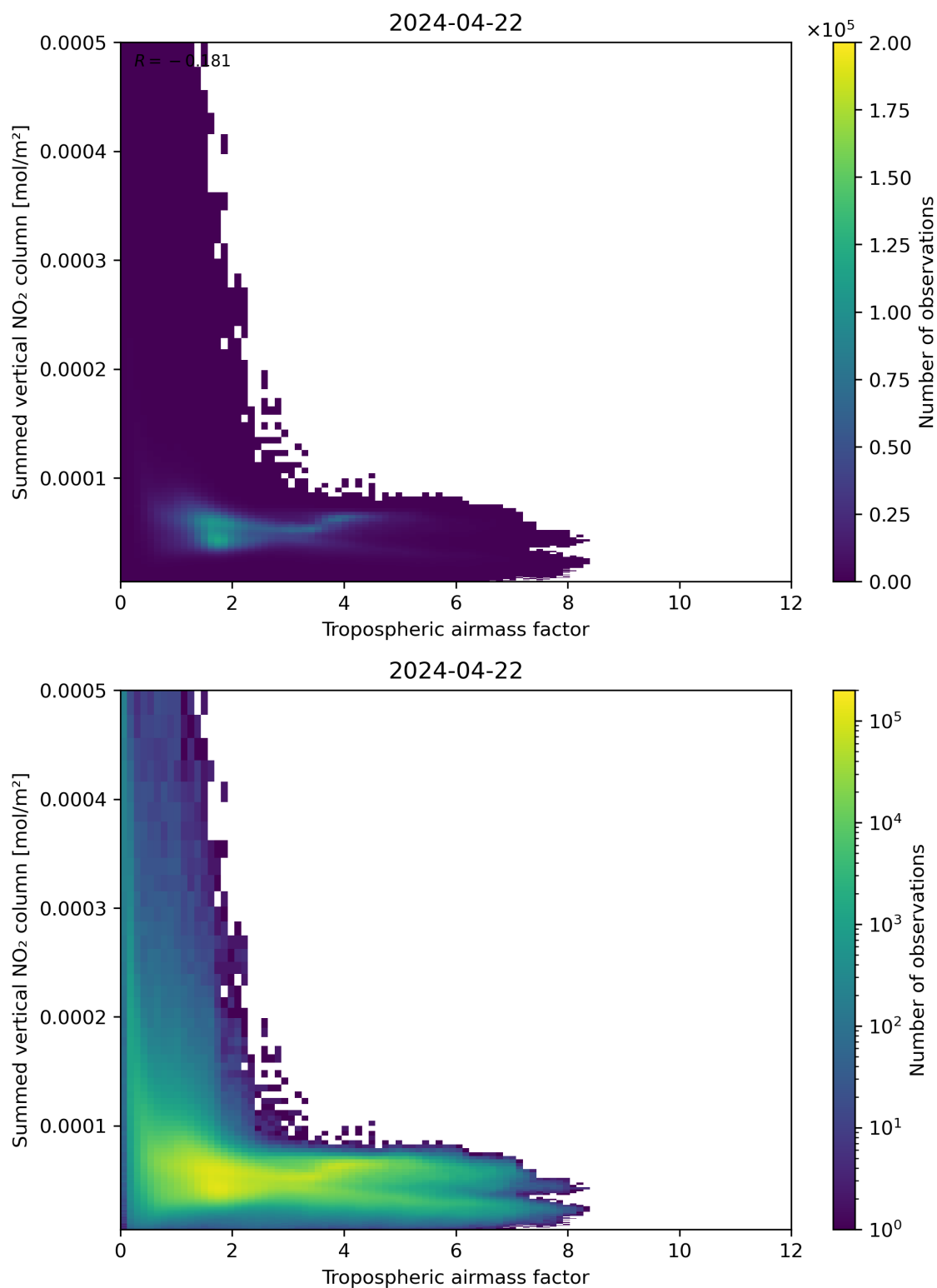
Figure 75: Scatter density plot of “Tropospheric airmass factor” against “Summed vertical NO 2 column” for 2024-04-21 to 2024-04-23.
