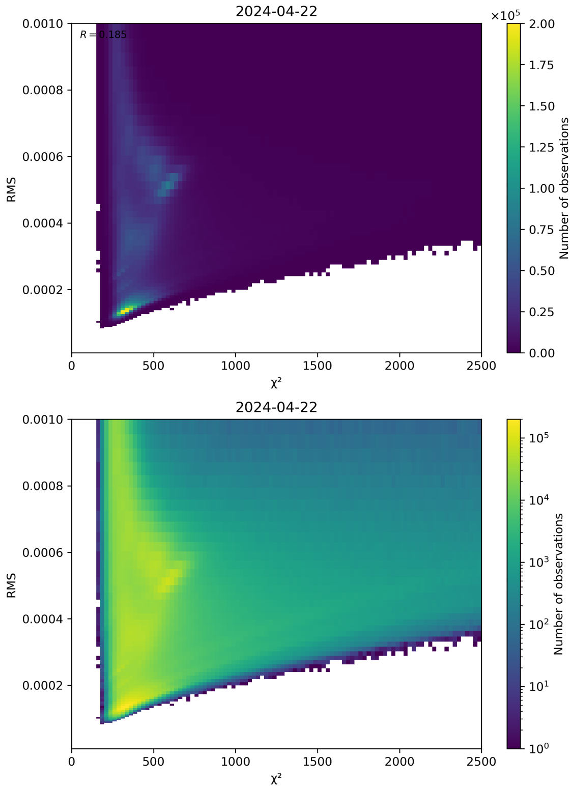
Figure 82: Scatter density plot of “ \chi^2 ” against “RMS” for 2024-04-21 to 2024-04-23.
