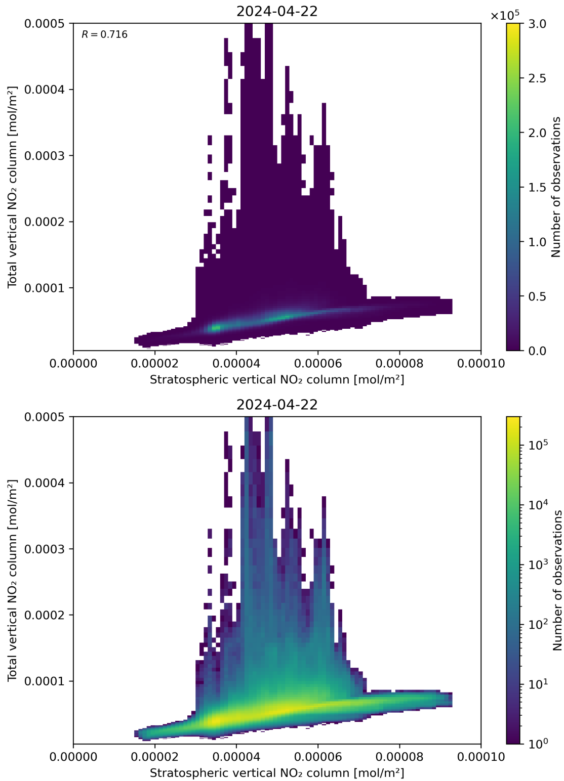
Figure 100: Scatter density plot of “Stratospheric vertical NO 2 column” against “Total vertical NO 2 column” for 2024-04-21 to 2024-04-23.
