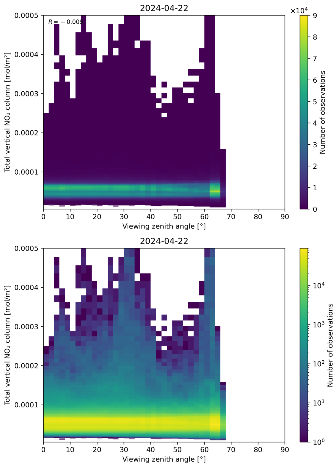
Figure 167: Scatter density plot of “Viewing zenith angle” against “Total vertical NO 2 column” for 2024-04-21 to 2024-04-23.
