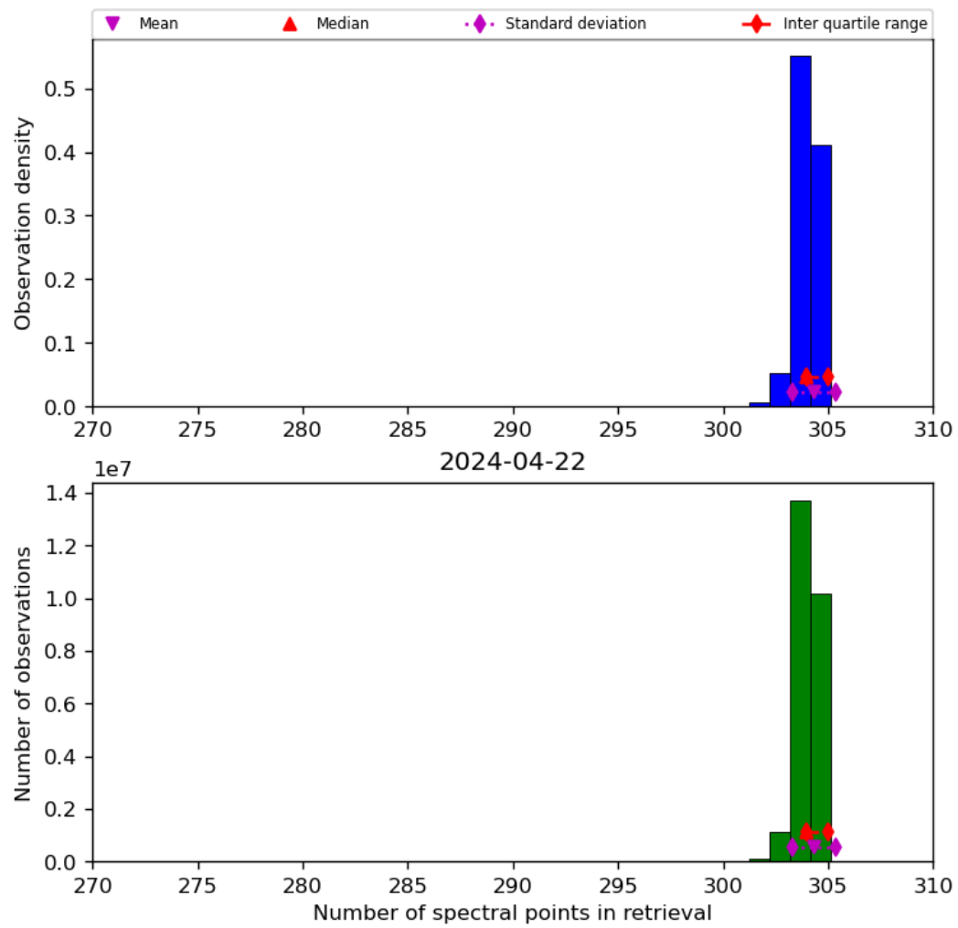
Figure 33: Histogram of “Number of spectral points in retrieval” for 2024-04-21 to 2024-04-23
