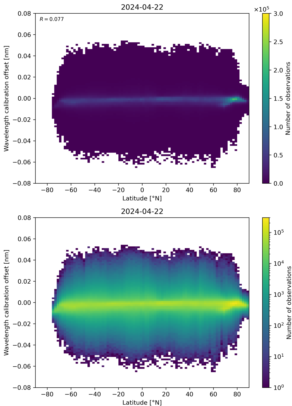
Figure 95: Scatter density plot of “Latitude” against “Wavelength calibration offset” for 2024-04-21 to 2024-04-23.
