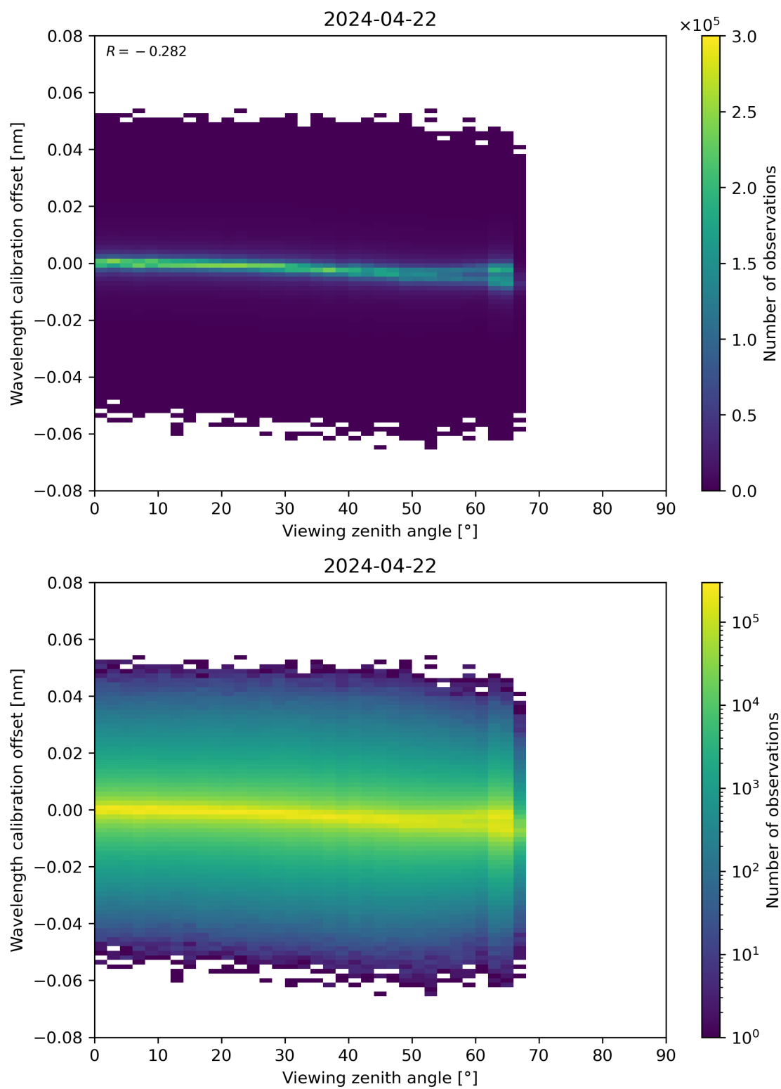
Figure 173: Scatter density plot of “Viewing zenith angle” against “Wavelength calibration offset” for 2024-04-21 to 2024-04-23.
