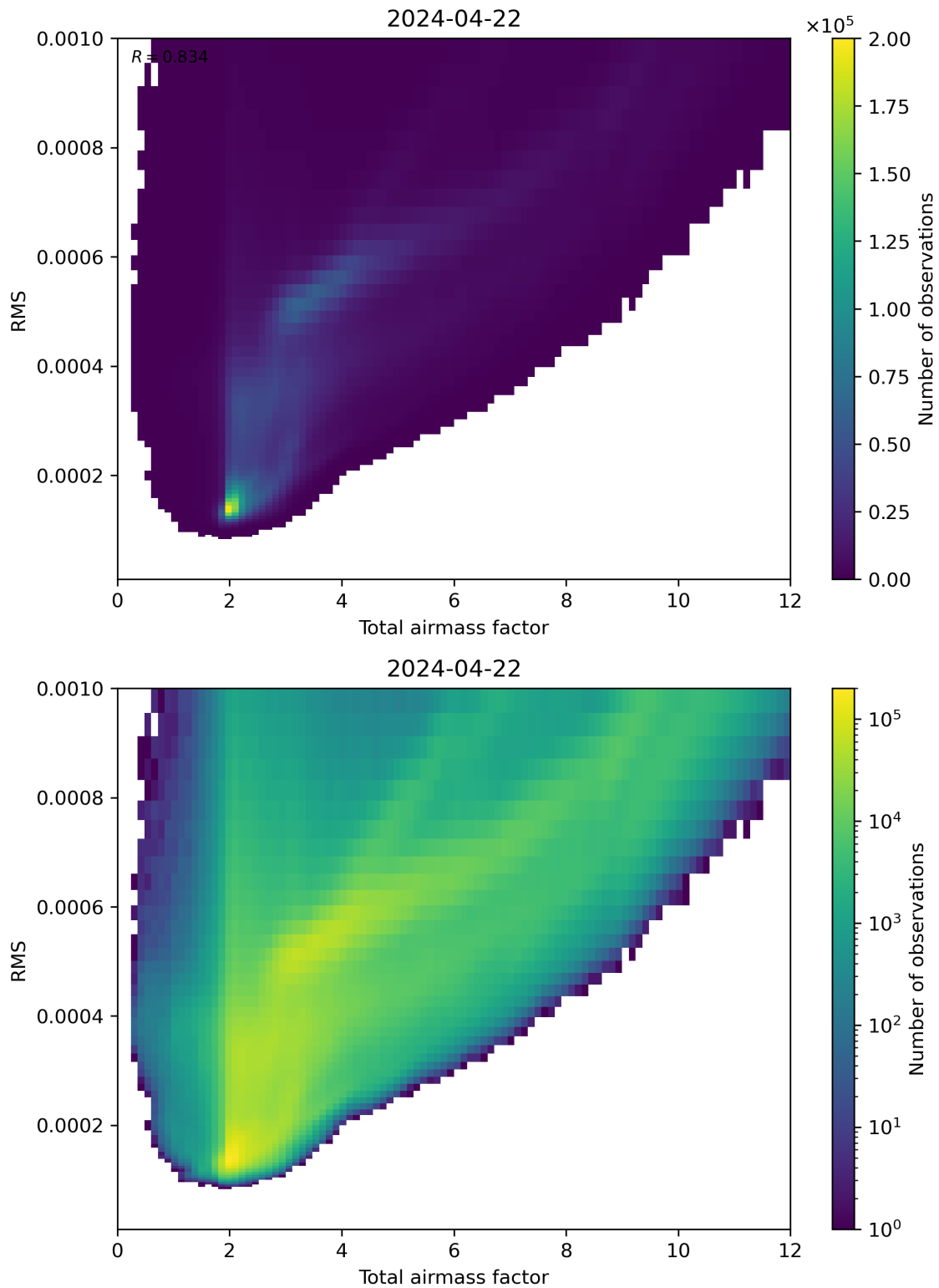
Figure 69: Scatter density plot of “Total airmass factor” against “RMS” for 2024-04-21 to 2024-04-23.
