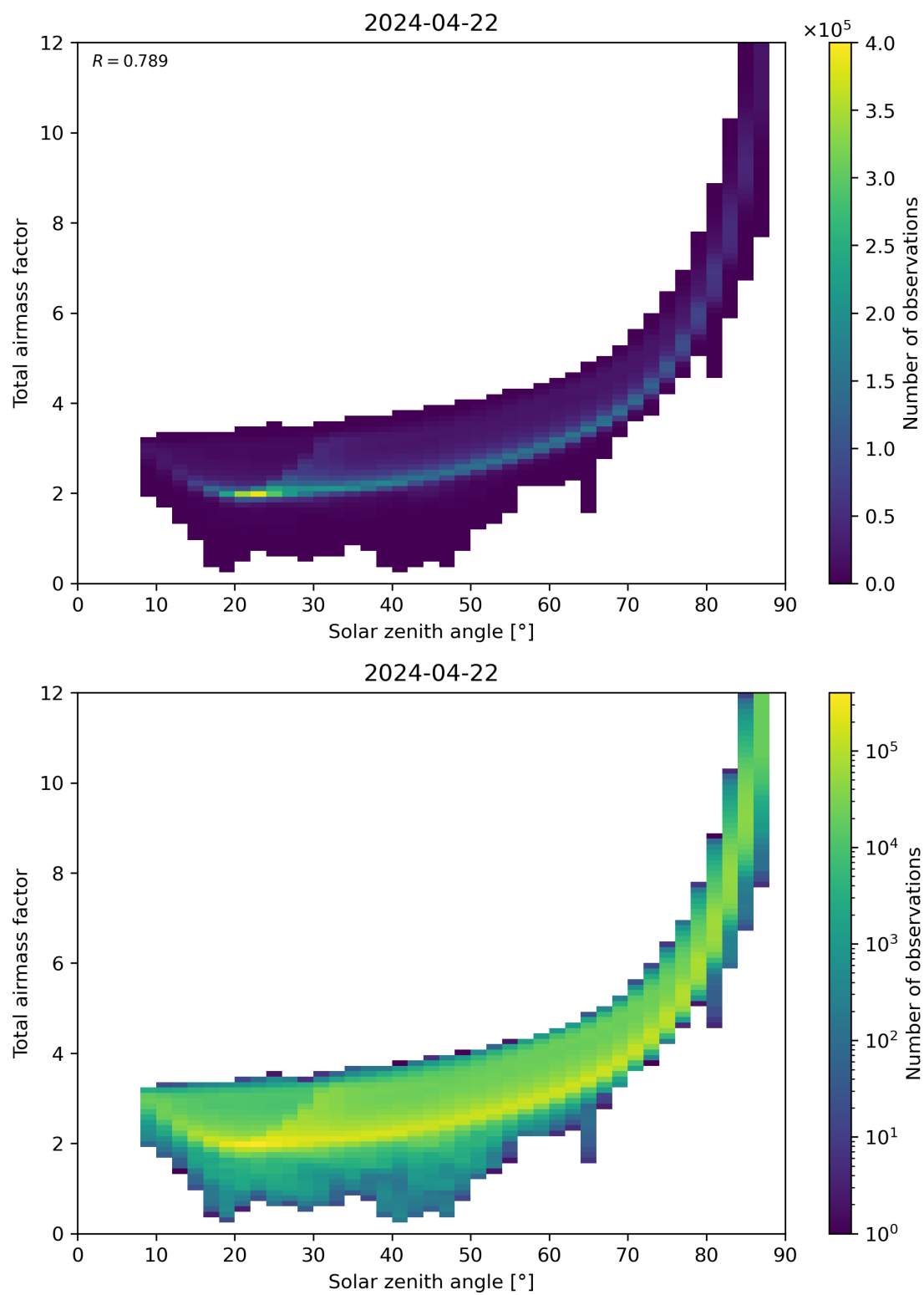
Figure 146: Scatter density plot of “Solar zenith angle” against “Total air mass factor” for 2024-04-21 to 2024-04-23.
