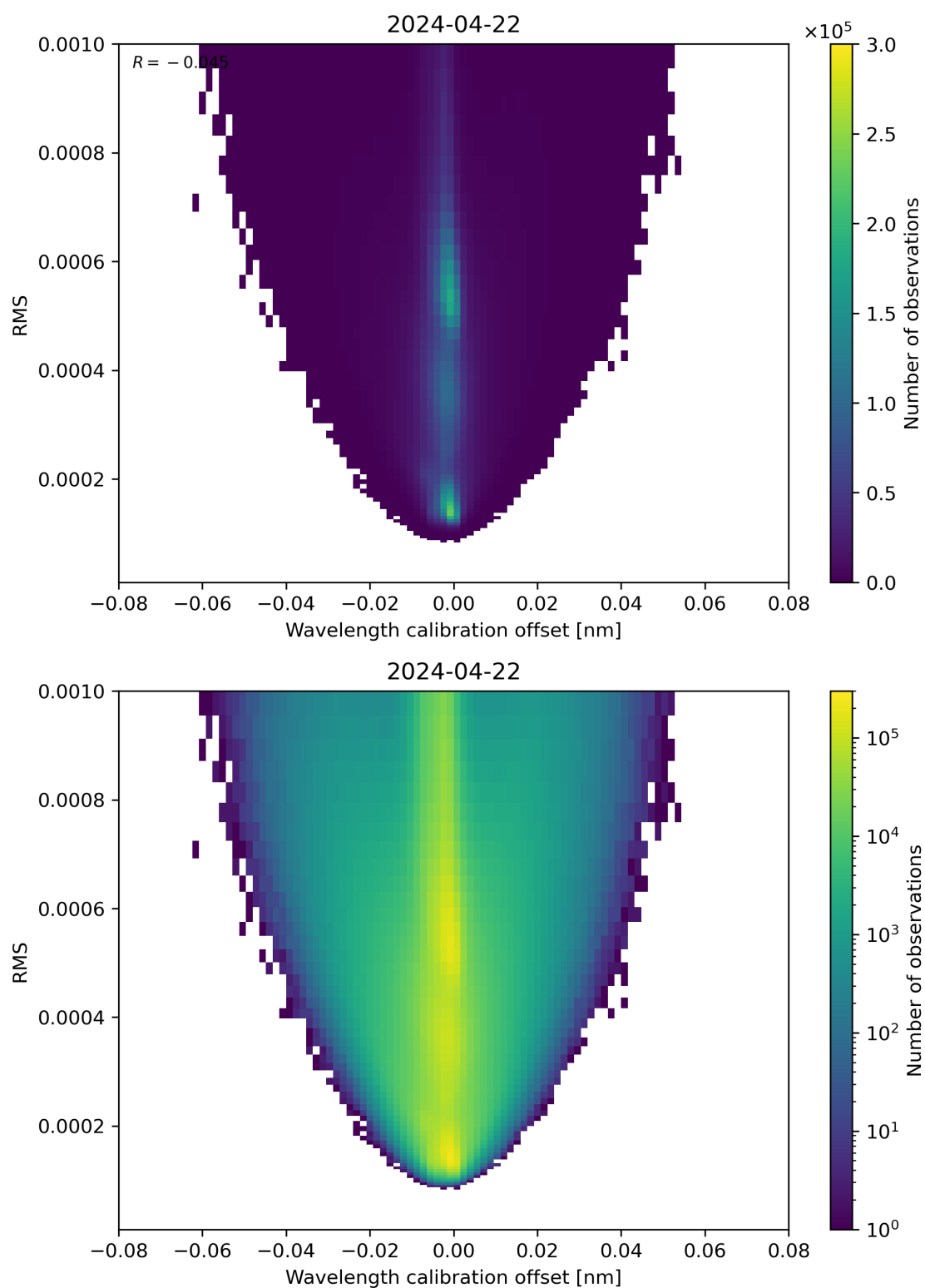
Figure 181: Scatter density plot of “Wavelength calibration offset” against “RMS” for 2024-04-21 to 2024-04-23.
