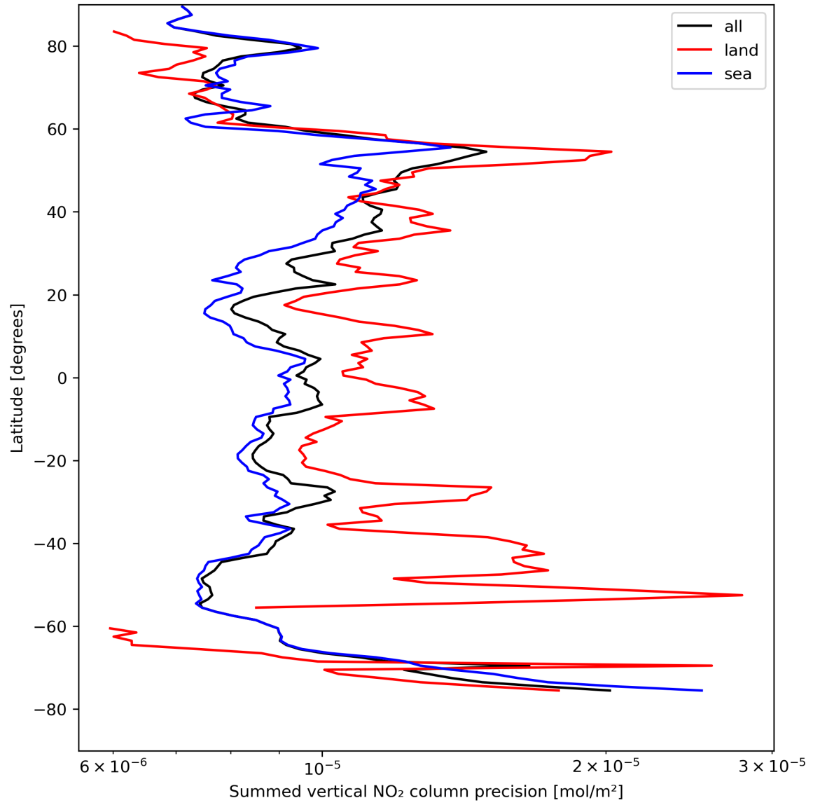
Figure 24: Zonal average of “Summed vertical NO 2 column precision” for 2024-04-21 to 2024-04-23.
