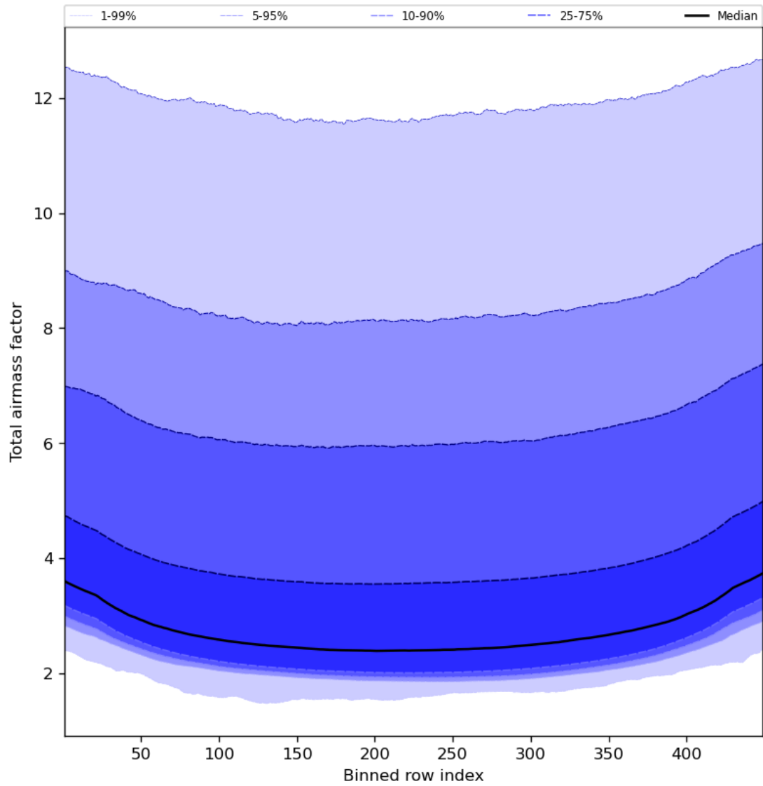
Figure 49: Along track statistics of “Total airmass factor” for 2024-04-21 to 2024-04-23
