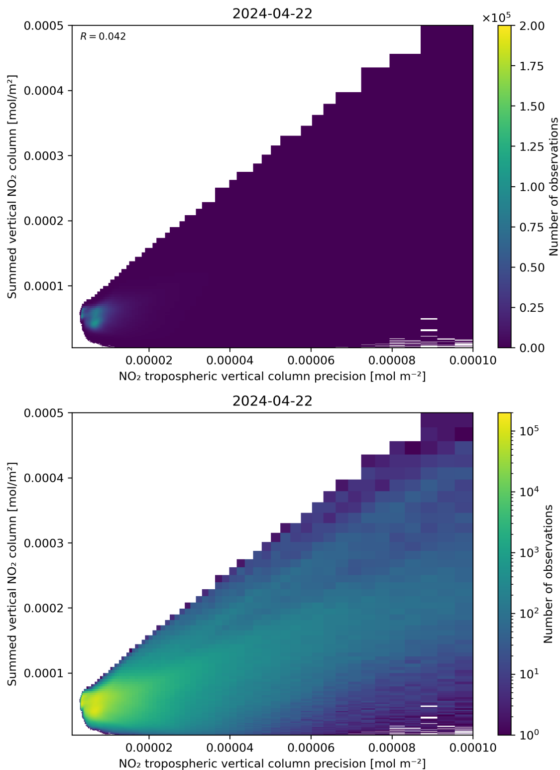
Figure 136: Scatter density plot of “NO 2 tropospheric vertical column precision” against “Summed vertical NO 2 column” for 2024-04-21 to 2024-04-23.
