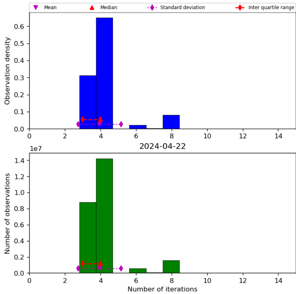
Figure 34: Histogram of “Number of iterations” for 2024-04-21 to 2024-04-23
