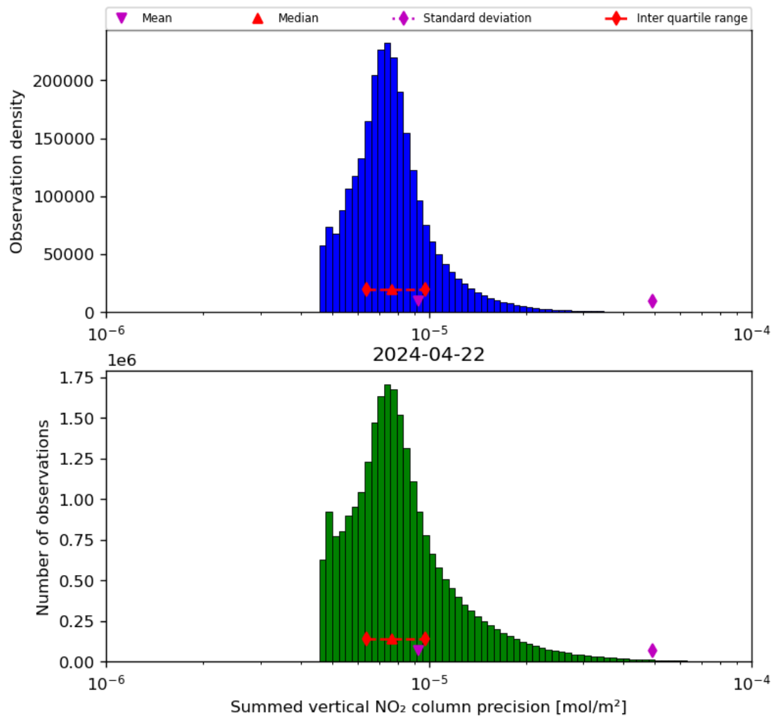
Figure 41: Histogram of “Summed vertical NO 2 column precision” for 2024-04-21 to 2024-04-23
