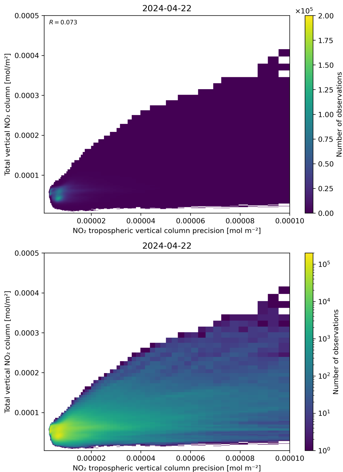
Figure 138: Scatter density plot of “NO 2 tropospheric vertical column precision” against “Total vertical NO 2 column” for 2024-04-21 to 2024-04-23.
