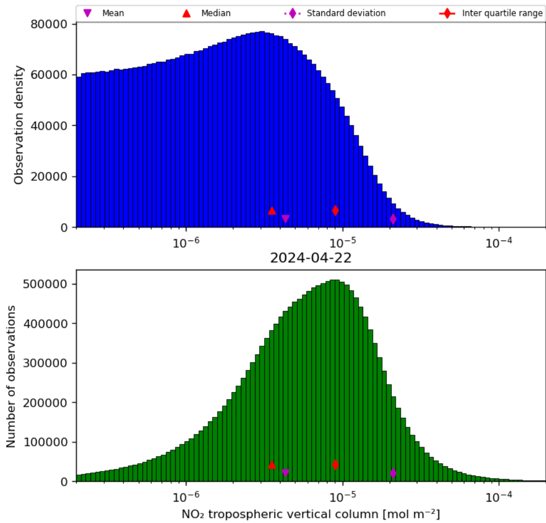
Figure 29: Histogram of “NO 2 tropospheric vertical column” for 2024-04-21 to 2024-04-23
