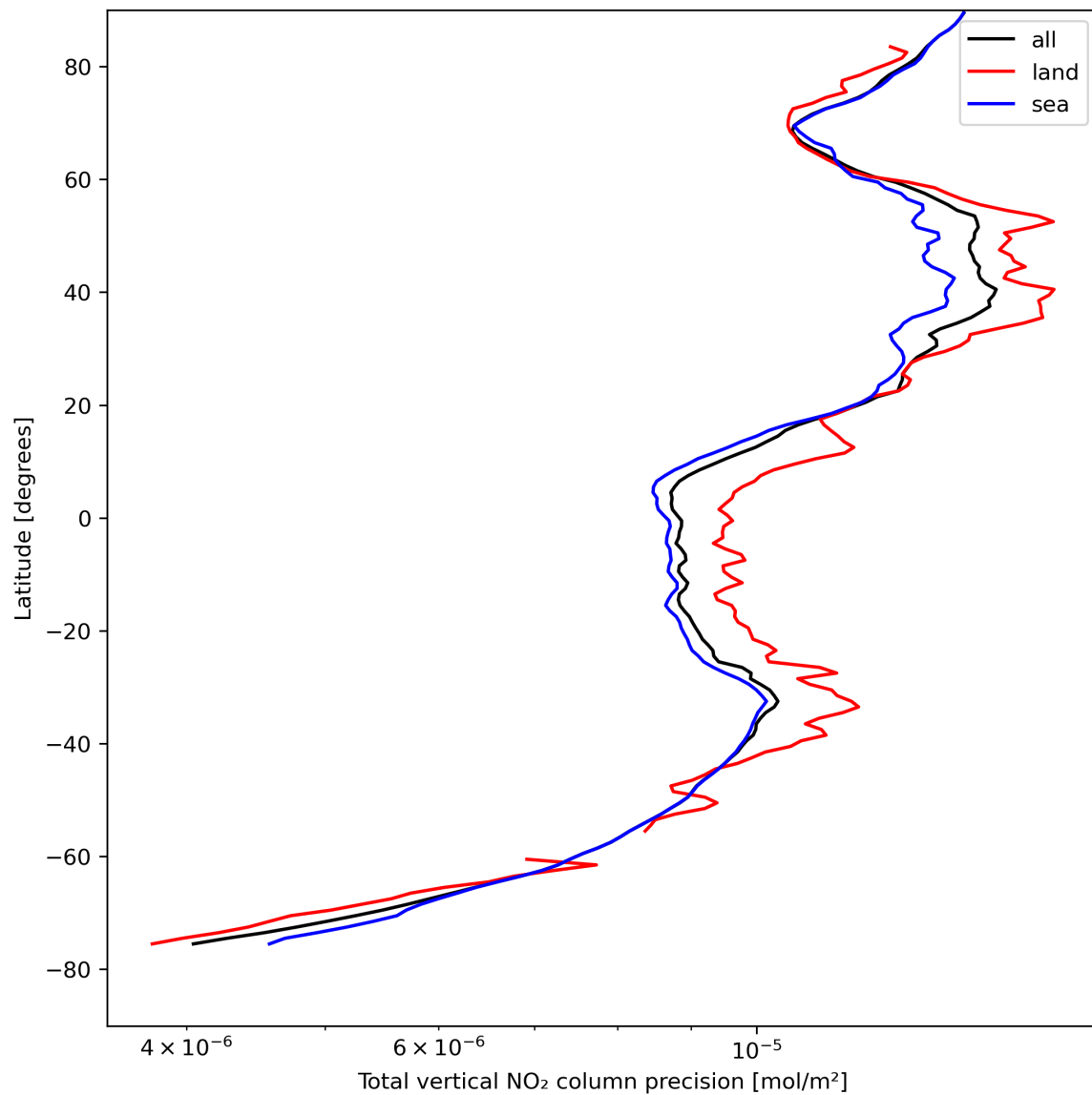
Figure 22: Zonal average of “Total vertical NO 2 column precision” for 2024-04-21 to 2024-04-23.
