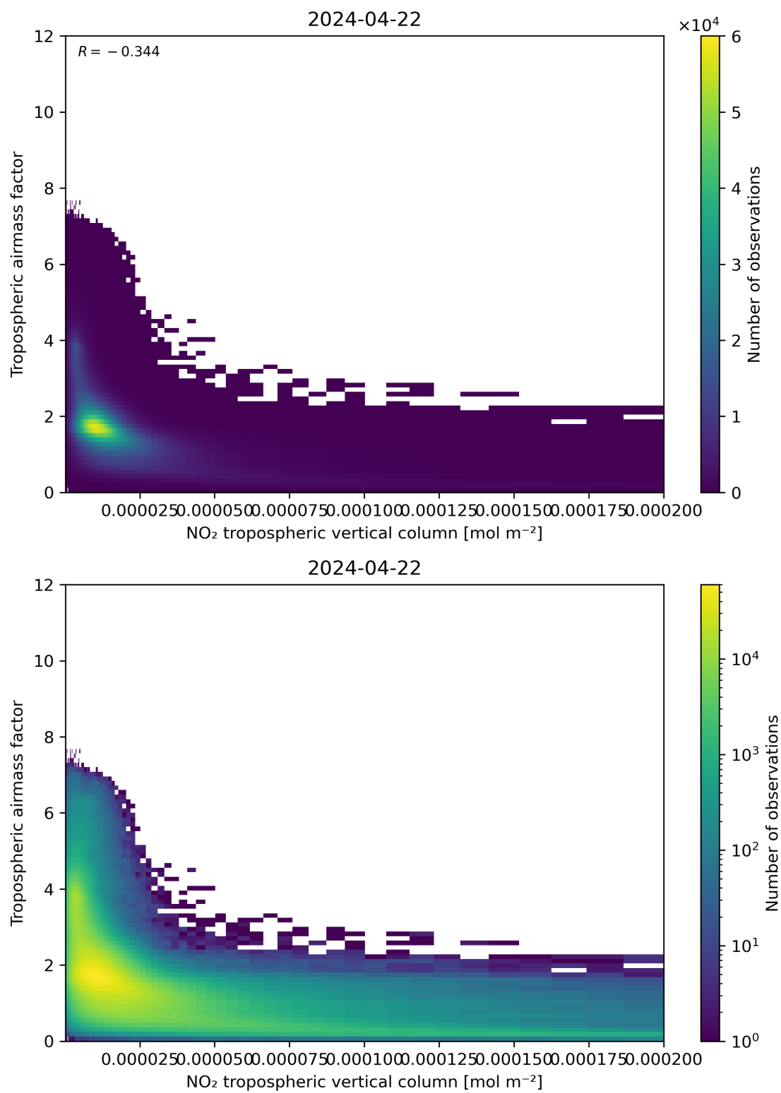
Figure 123: Scatter density plot of “NO 2 tropospheric vertical column” against “Tropospheric airmass factor” for 2024-04-21 to 2024-04-23.
