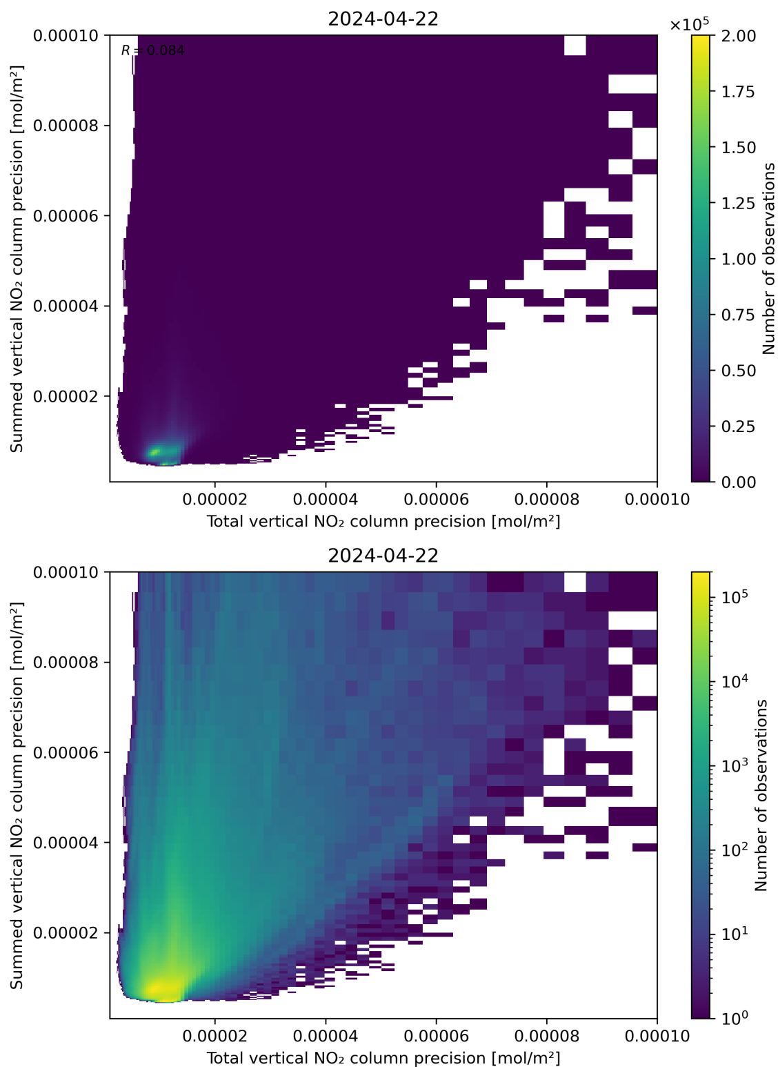
Figure 118: Scatter density plot of “Total vertical NO 2 column precision” against “Summed vertical NO 2 column precision” for 2024-04-21 to 2024-04-23.
