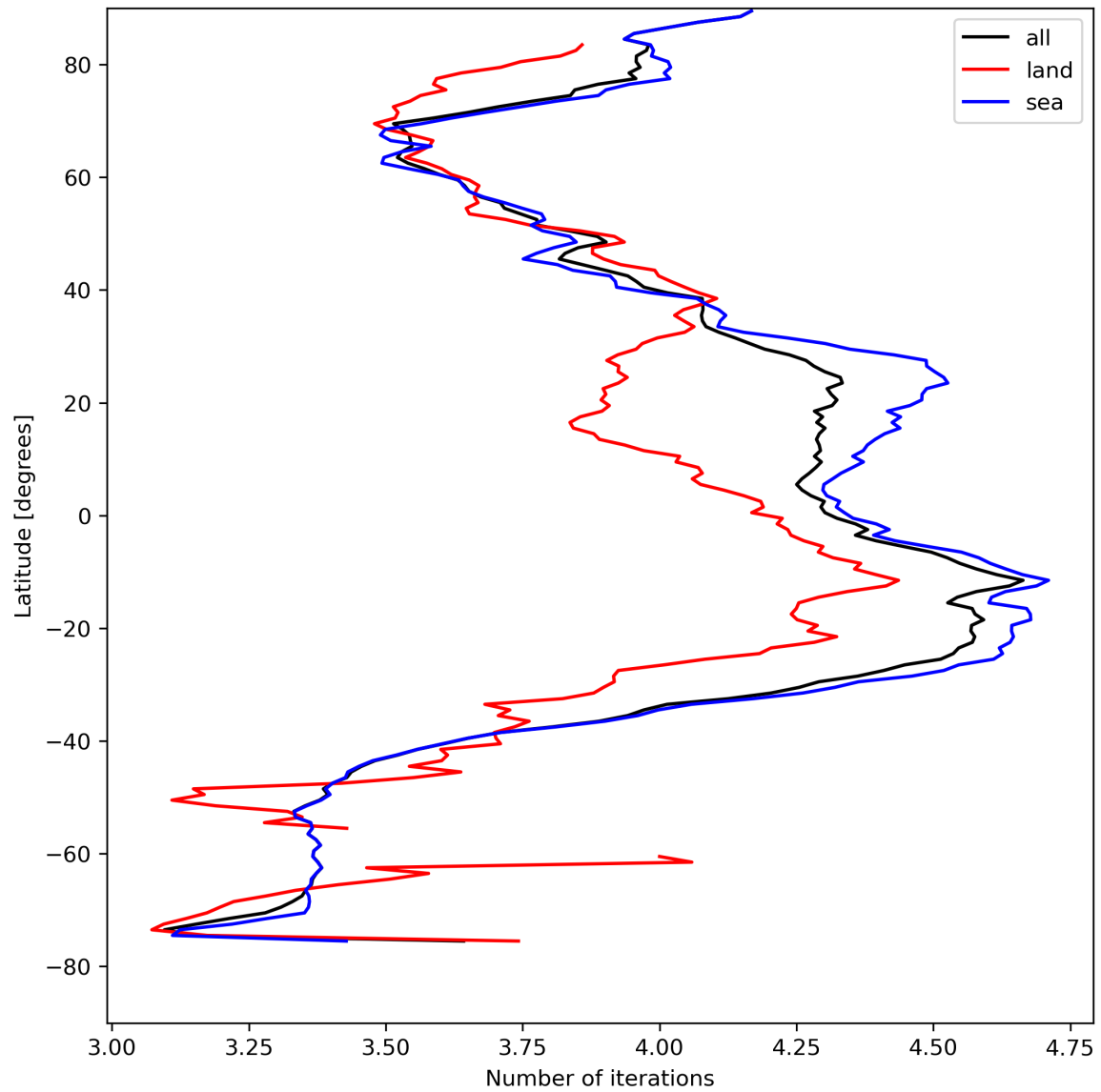
Figure 17: Zonal average of “Number of iterations” for 2024-04-21 to 2024-04-23.
