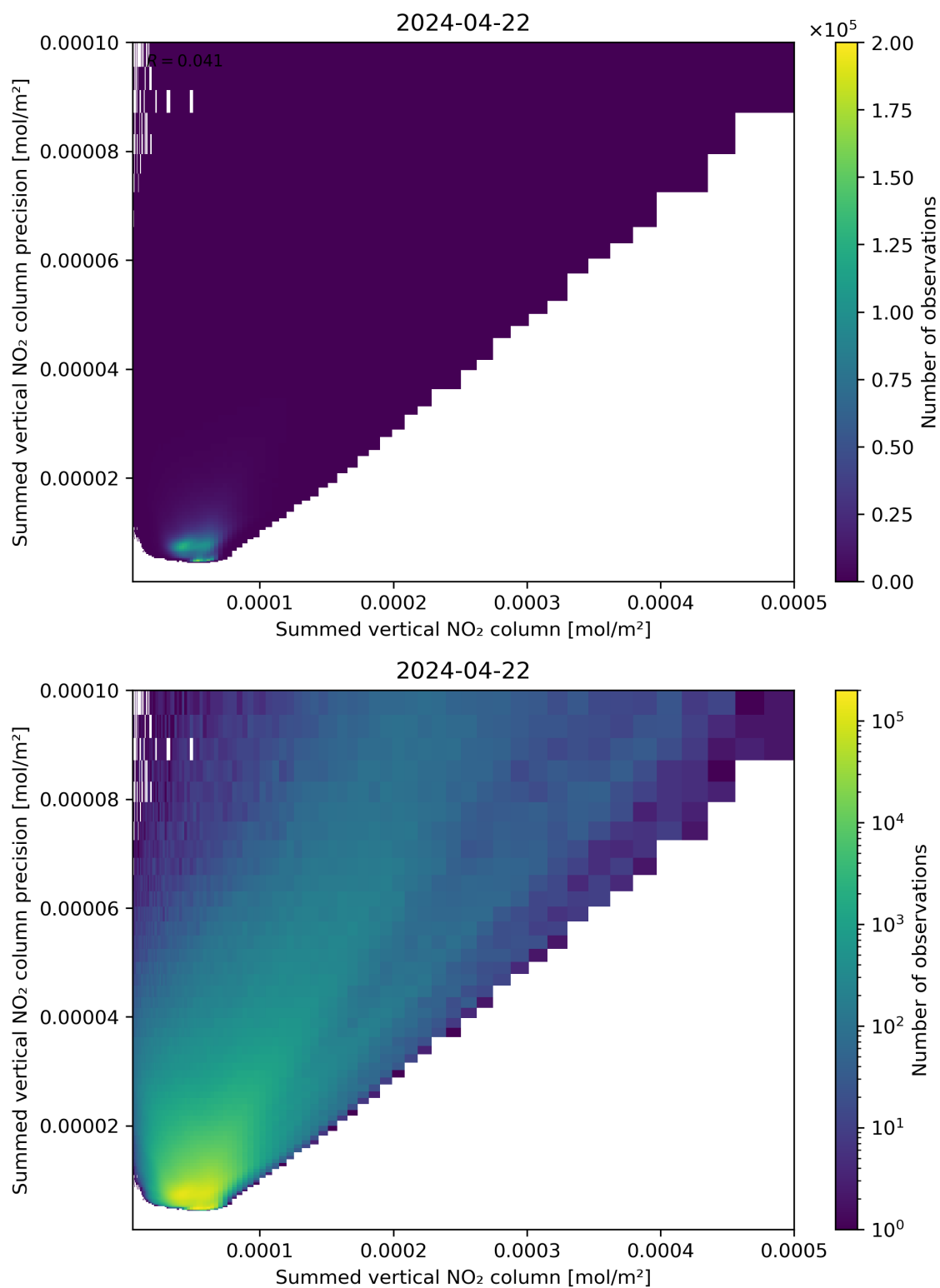
Figure 105: Scatter density plot of “Summed vertical NO 2 column” against “Summed vertical NO 2 column precision” for 2024-04-21 to 2024-04-23.
