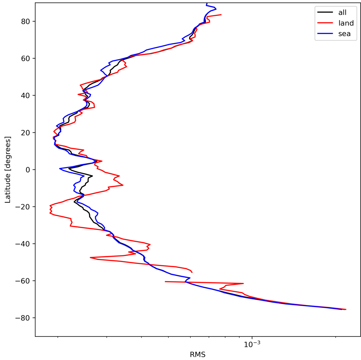
Figure 26: Zonal average of “RMS” for 2024-04-21 to 2024-04-23.
