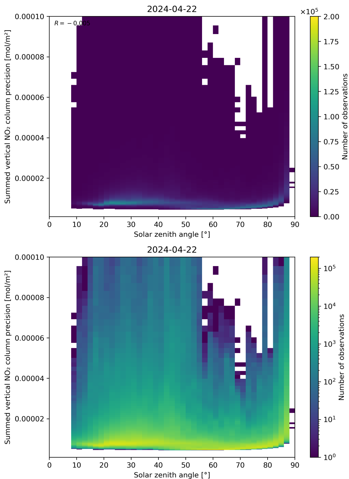
Figure 152: Scatter density plot of “Solar zenith angle” against “Summed vertical NO 2 column precision” for 2024-04-21 to 2024-04-23.
