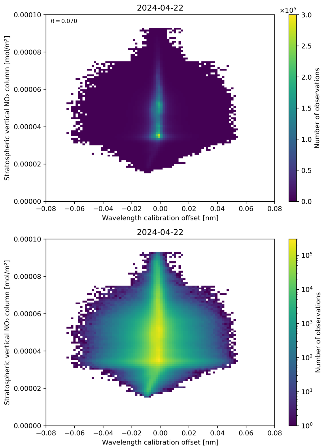
Figure 176: Scatter density plot of “Wavelength calibration offset” against “Stratospheric vertical NO 2 column” for 2024-04-21 to 2024-04-23.
