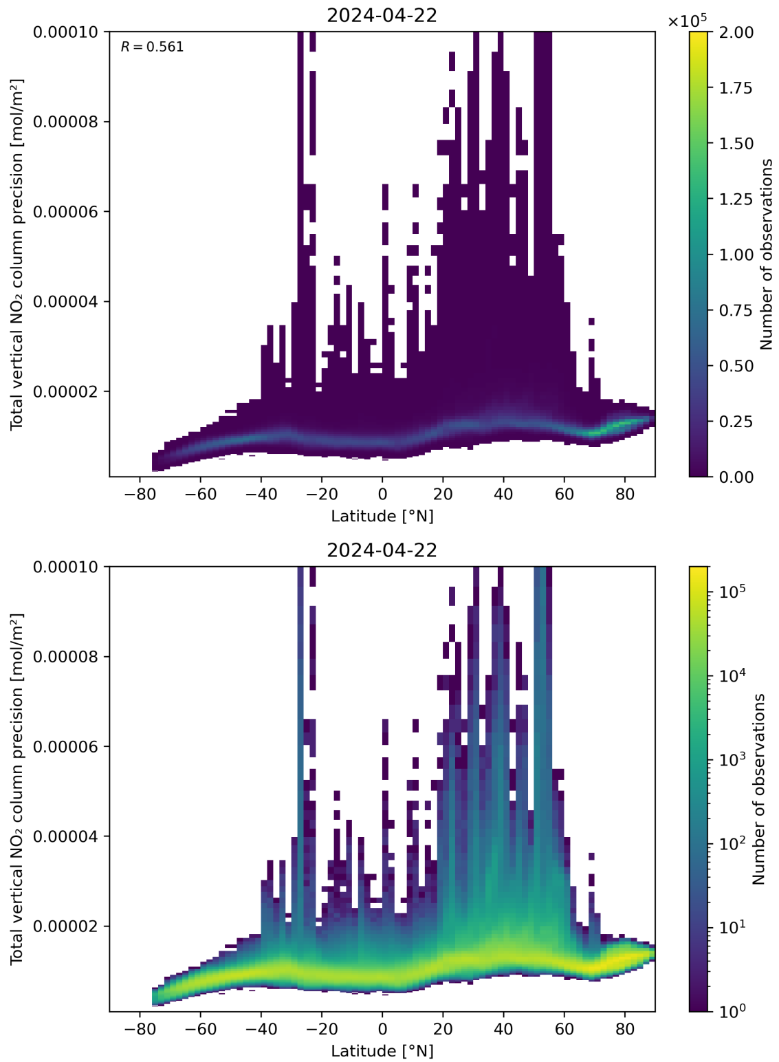
Figure 91: Scatter density plot of “Latitude” against “Total vertical NO 2 column precision” for 2024-04-21 to 2024-04-23.
