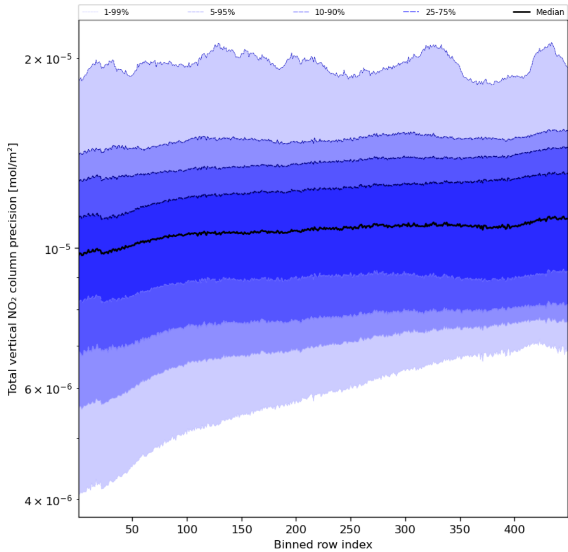
Figure 56: Along track statistics of “Total vertical NO 2 column precision” for 2024-04-21 to 2024-04-23
