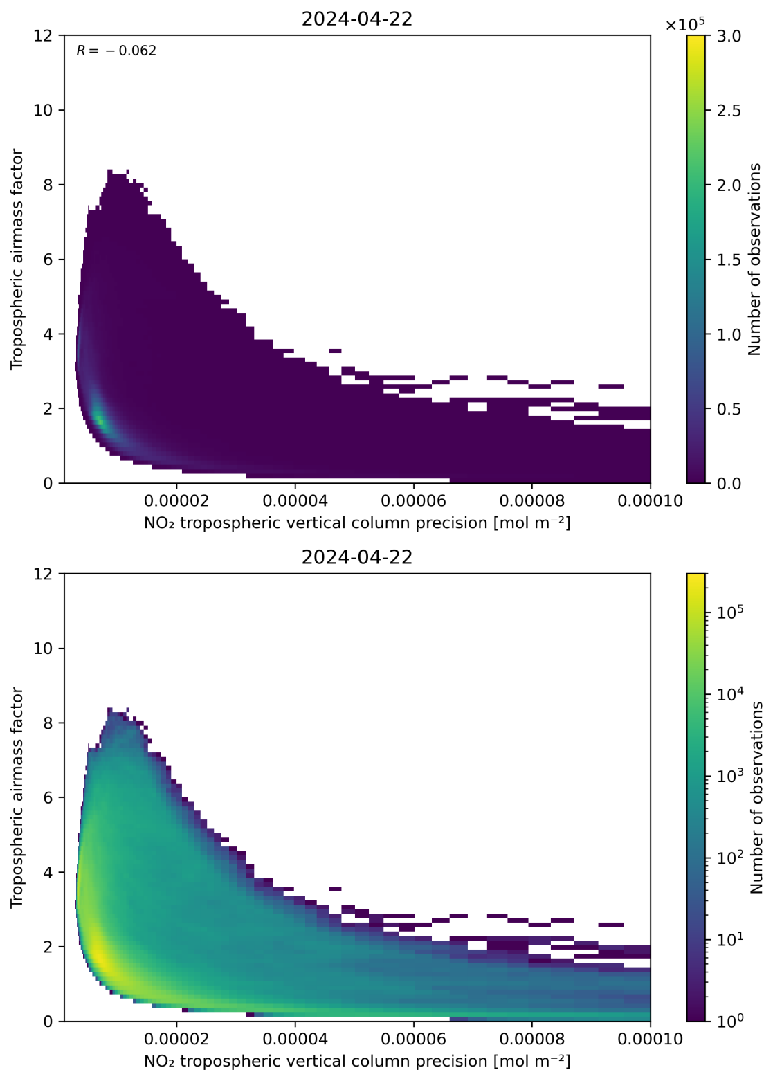
Figure 133: Scatter density plot of “NO 2 tropospheric vertical column precision” against “Tropospheric airmass factor” for 2024-04-21 to 2024-04-23.
