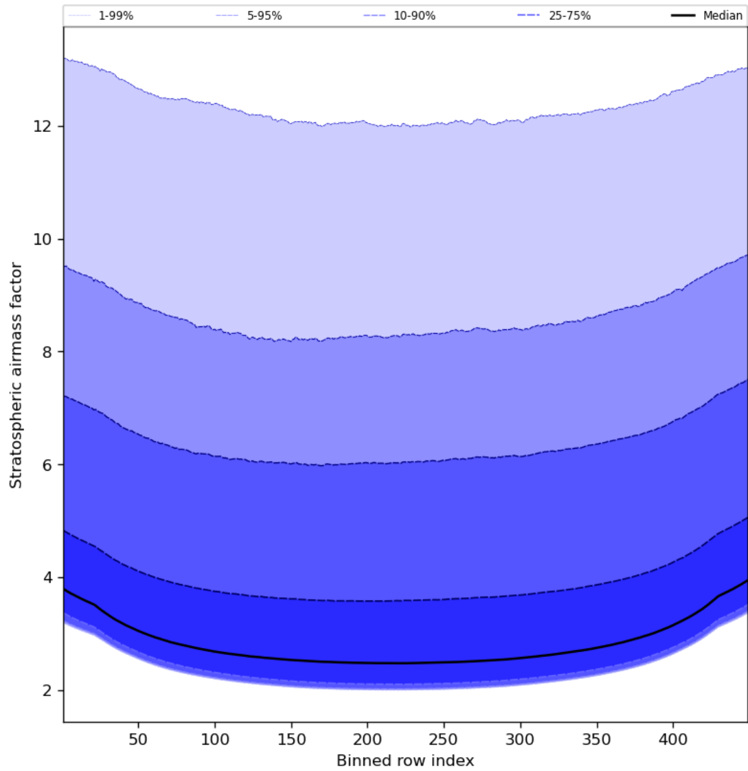
Figure 61: Along track statistics of “Stratospheric airmass factor” for 2024-04-21 to 2024-04-23
