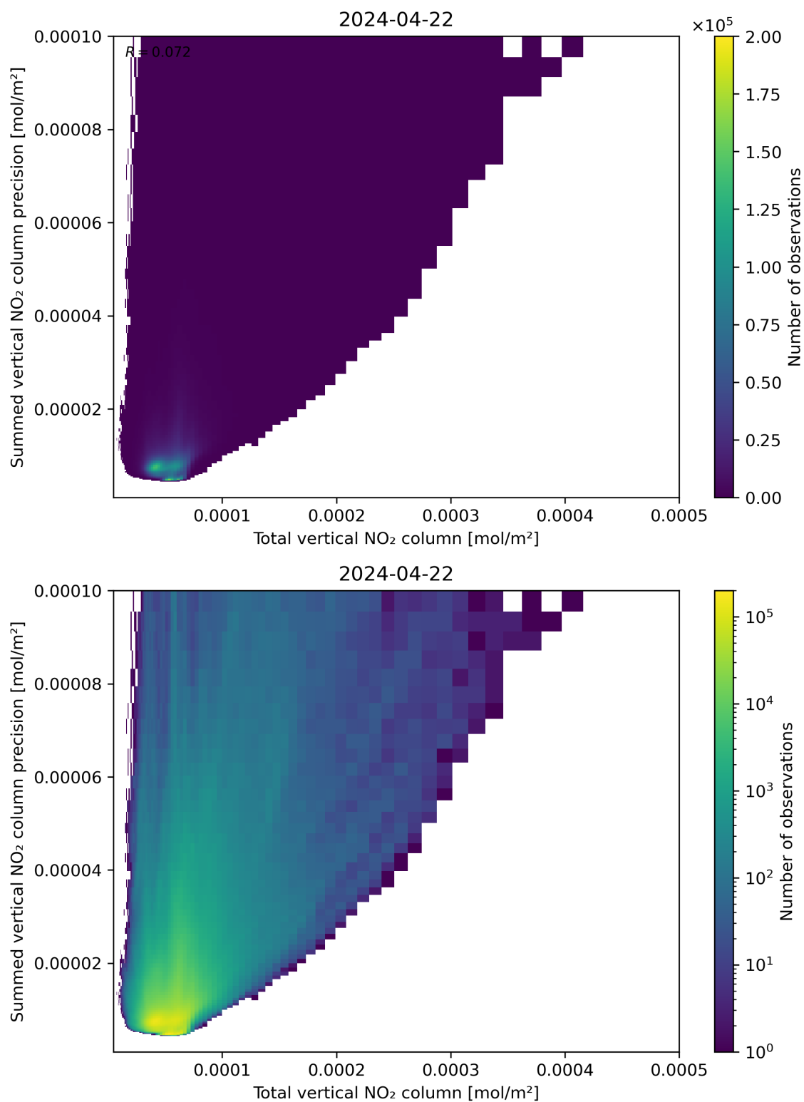
Figure 113: Scatter density plot of “Total vertical NO 2 column” against “Summed vertical NO 2 column precision” for 2024-04-21 to 2024-04-23.
