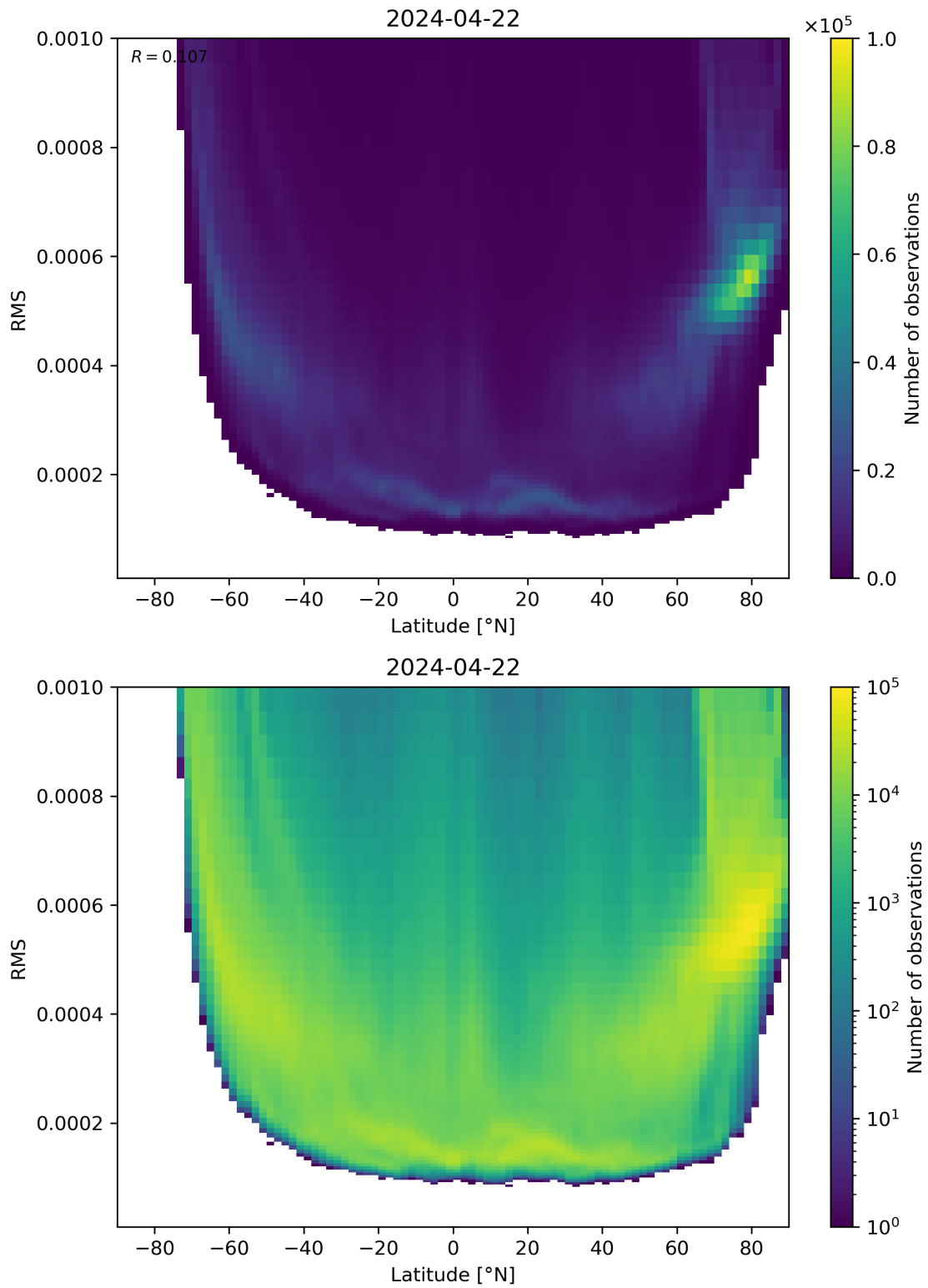
Figure 94: Scatter density plot of “Latitude” against “RMS” for 2024-04-21 to 2024-04-23.
