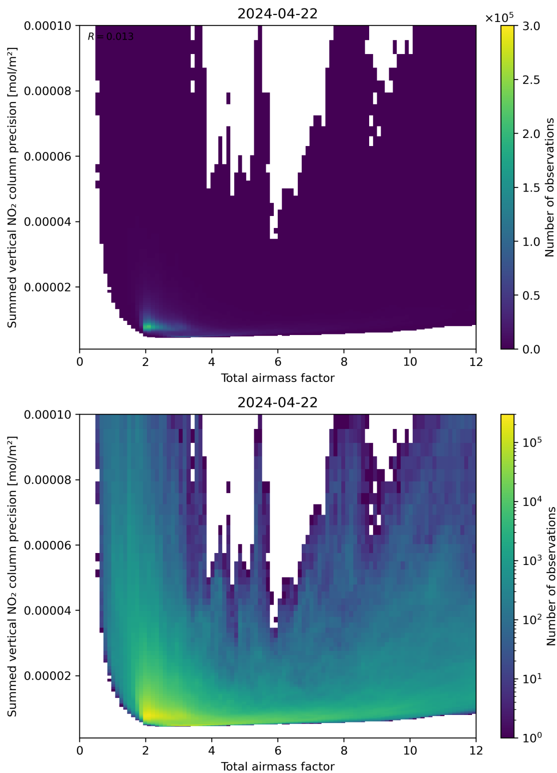
Figure 66: Scatter density plot of “Total airmass factor” against “Summed vertical NO 2 column precision” for 2024-04-21 to 2024-04-23.
