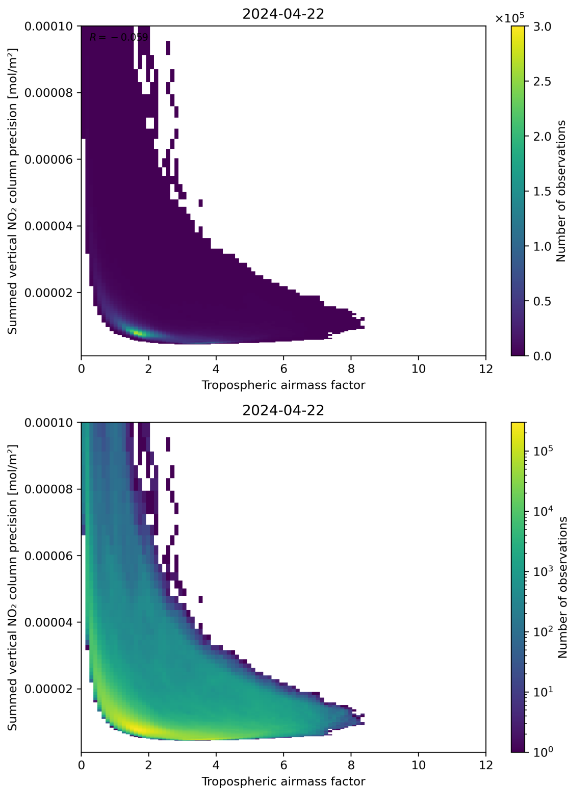
Figure 76: Scatter density plot of “Tropospheric air mass factor” against “Summed vertical NO 2 column precision” for 2024-04-21 to 2024-04-23.
