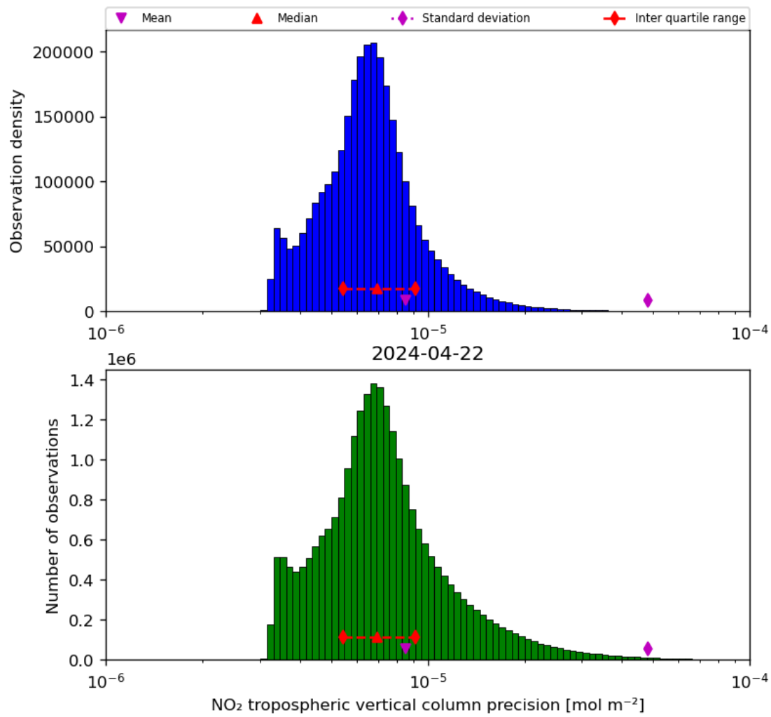
Figure 30: Histogram of “NO 2 tropospheric vertical column precision” for 2024-04-21 to 2024-04-23
