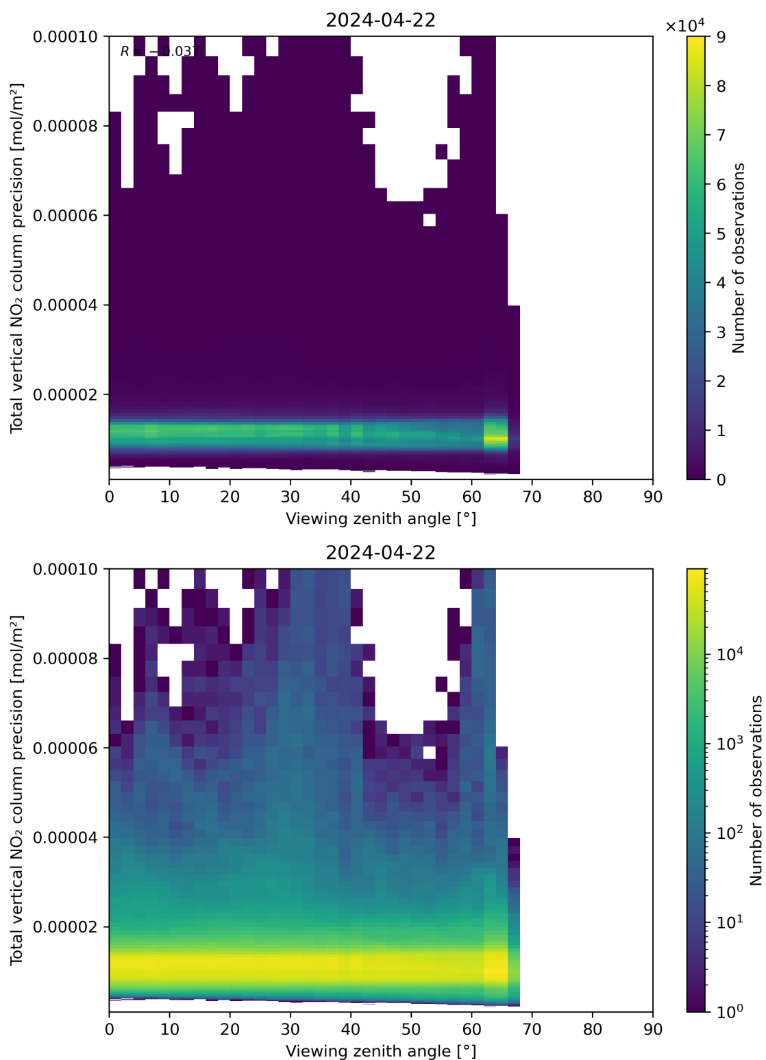
Figure 168: Scatter density plot of “Viewing zenith angle” against “Total vertical NO 2 column precision” for 2024-04-21 to 2024-04-23.
