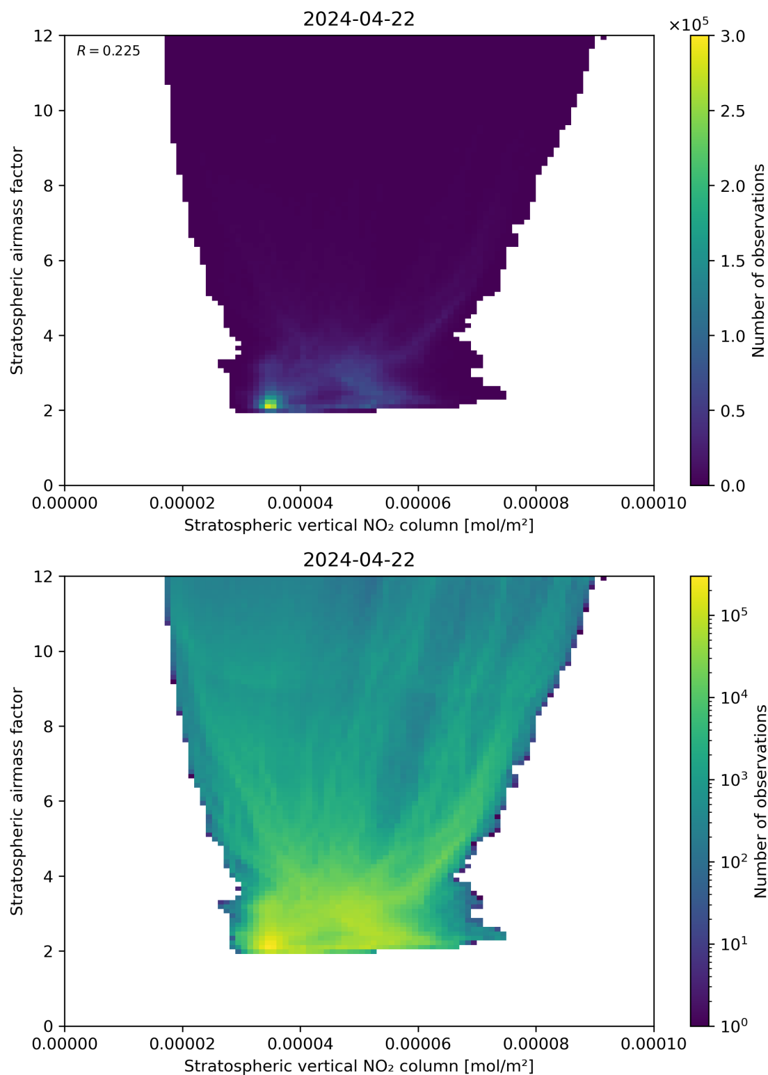
Figure 96: Scatter density plot of “Stratospheric vertical NO 2 column” against “Stratospheric airmass factor” for 2024-04-21 to 2024-04-23.
