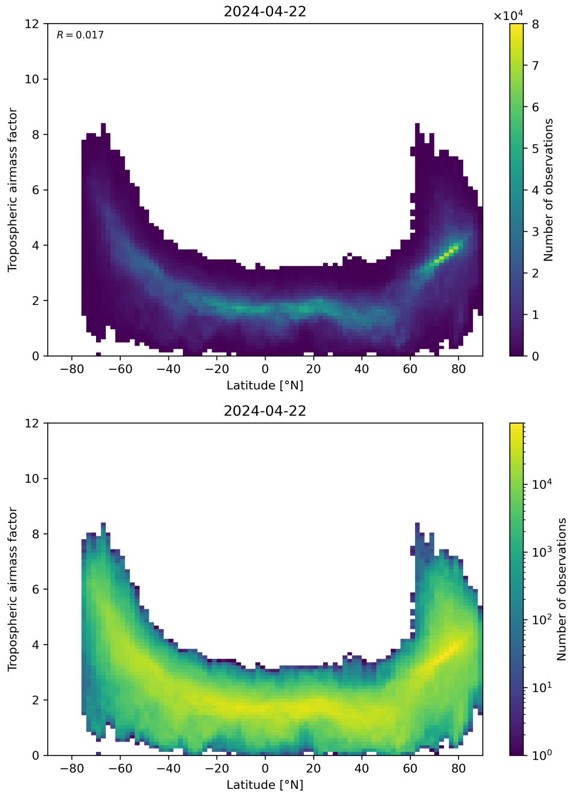
Figure 85: Scatter density plot of “Latitude” against “Tropospheric air mass factor” for 2024-04-21 to 2024-04-23.
