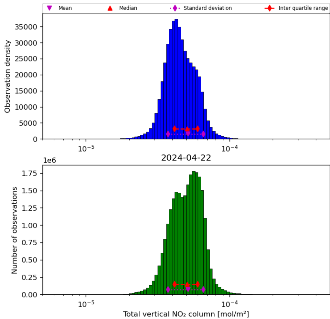
Figure 38: Histogram of “Total vertical NO 2 column” for 2024-04-21 to 2024-04-23
