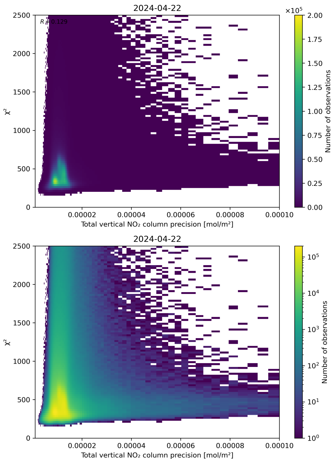
Figure 116: Scatter density plot of “Total vertical NO 2 column precision” against “ \chi^2 ” for 2024-04-21 to 2024-04-23.
