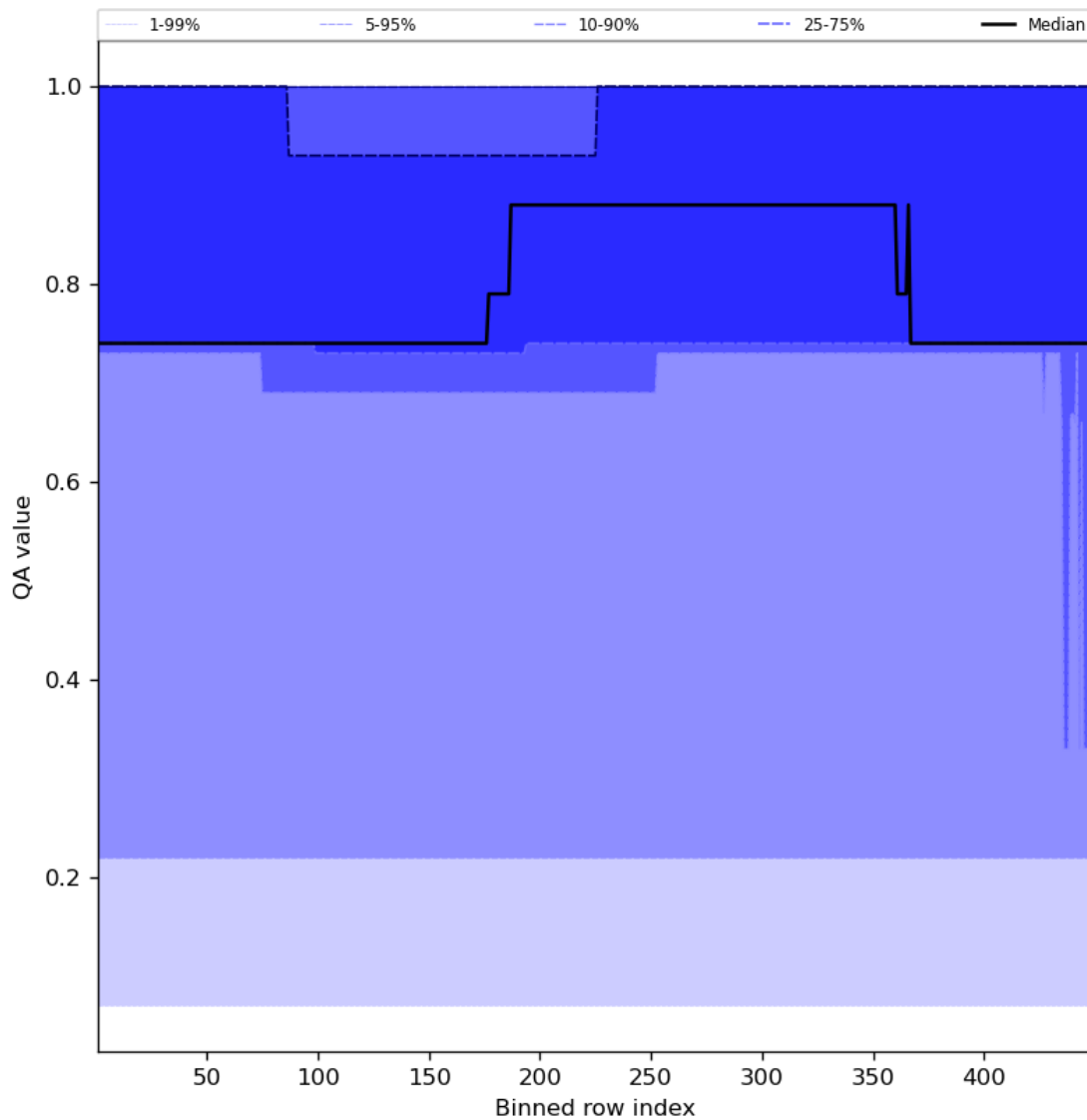
Figure 45: Along track statistics of “QA value” for 2024-04-21 to 2024-04-23
