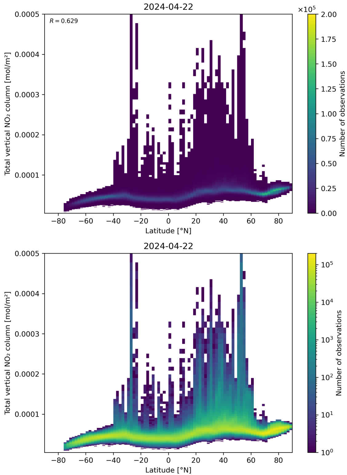
Figure 90: Scatter density plot of “Latitude” against “Total vertical \text{NO}_2 column” for 2024-04-21 to 2024-04-23.
