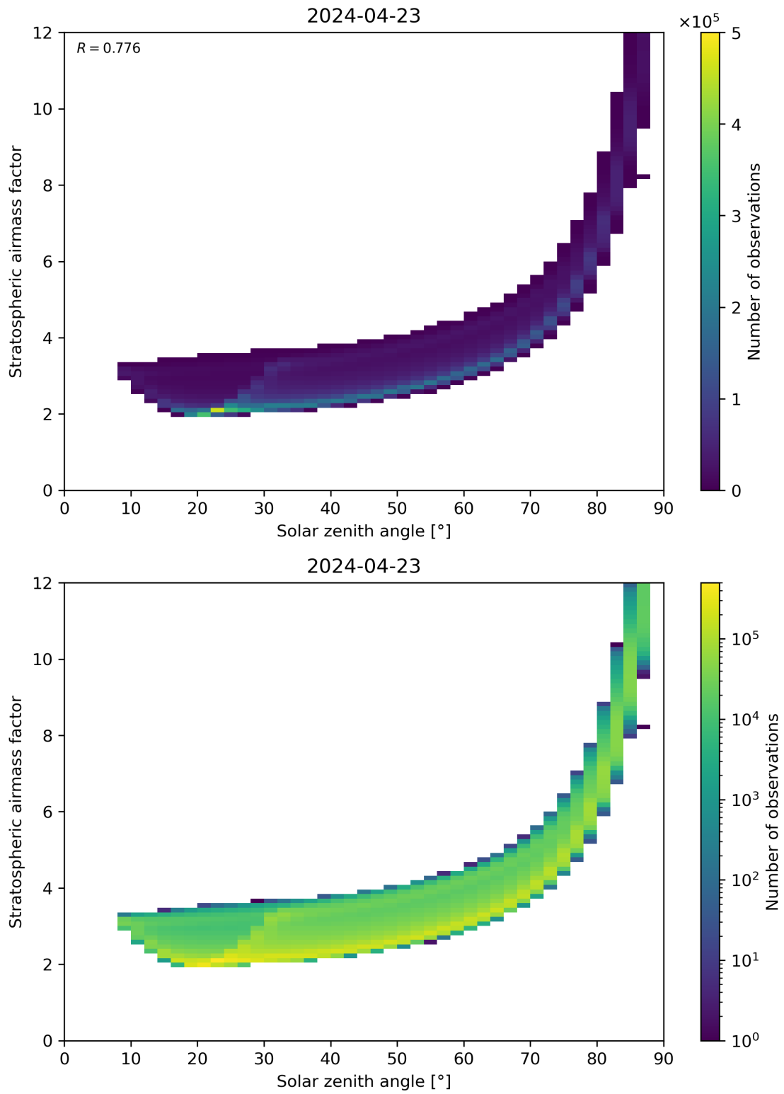
Figure 145: Scatter density plot of “Solar zenith angle” against “Stratospheric airmass factor” for 2024-04-22 to 2024-04-24.
