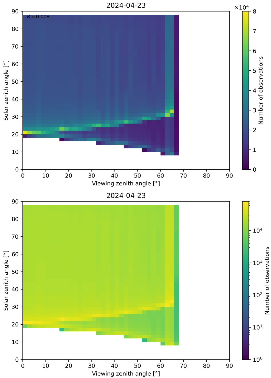
Figure 172: Scatter density plot of “Viewing zenith angle” against “Solar zenith angle” for 2024-04-22 to 2024-04-24.
