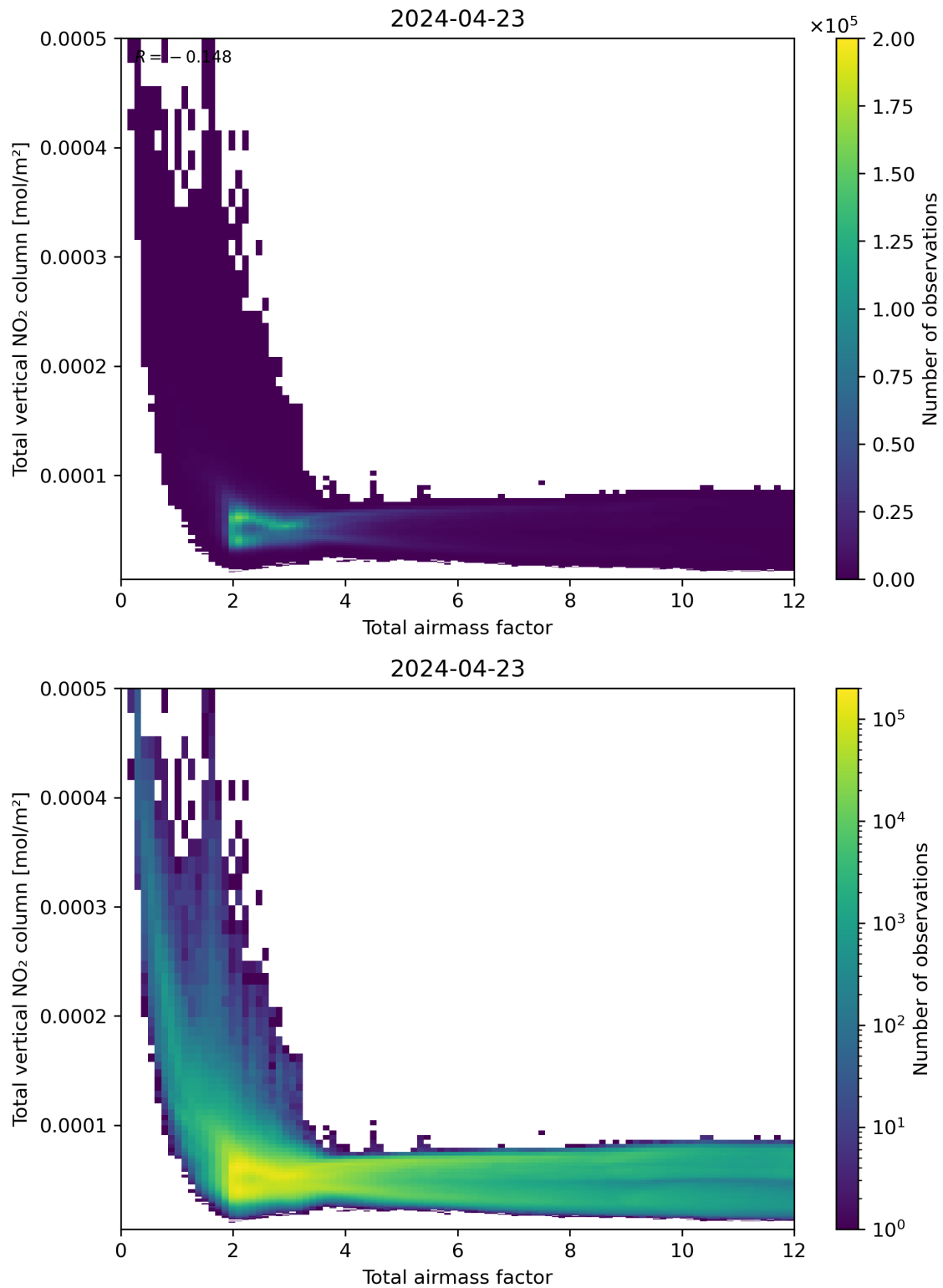
Figure 67: Scatter density plot of “Total airmass factor” against “Total vertical NO 2 column” for 2024-04-22 to 2024-04-24.
