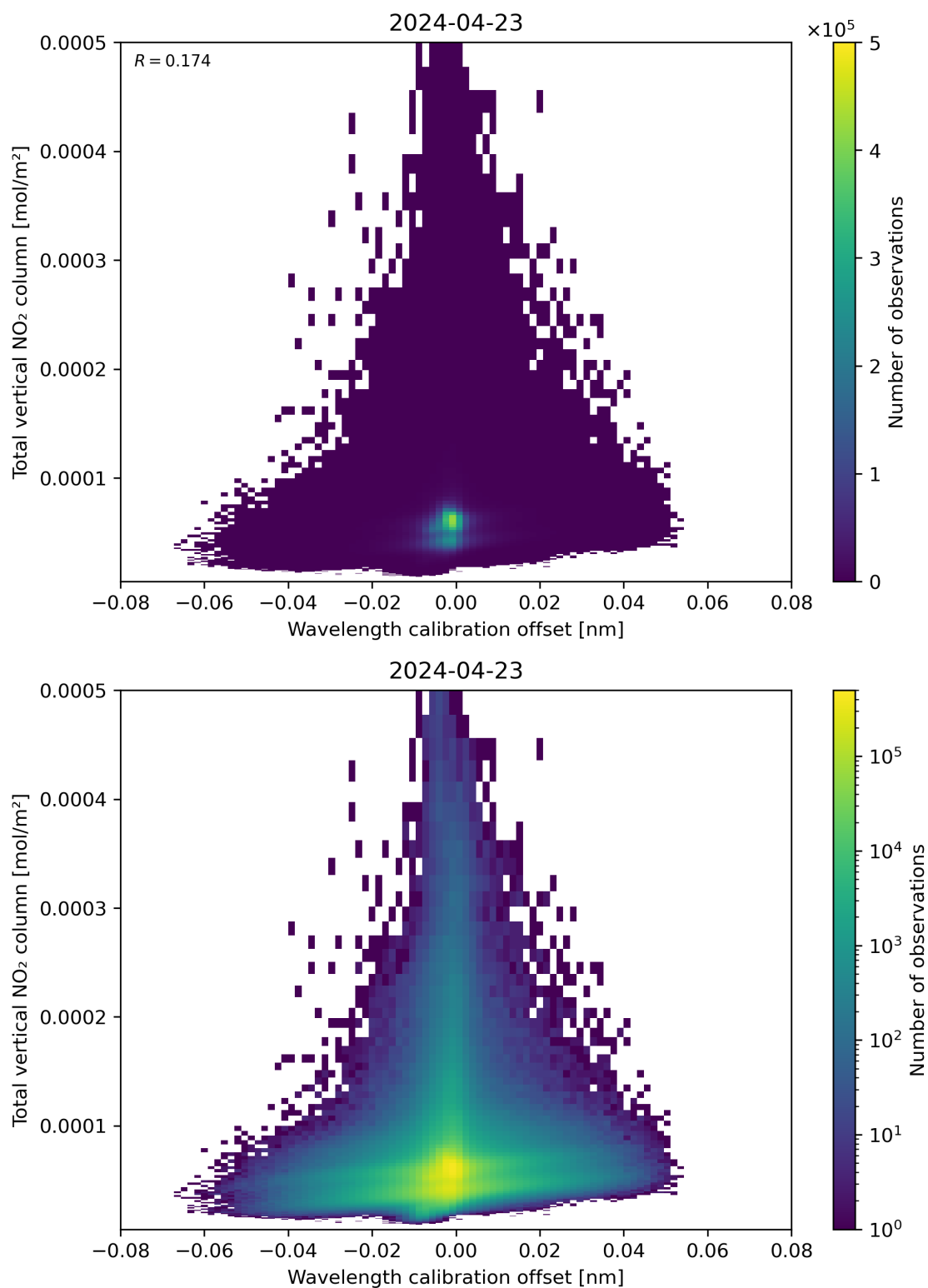
Figure 179: Scatter density plot of “Wavelength calibration offset” against “Total vertical NO 2 column” for 2024-04-22 to 2024-04-24.
