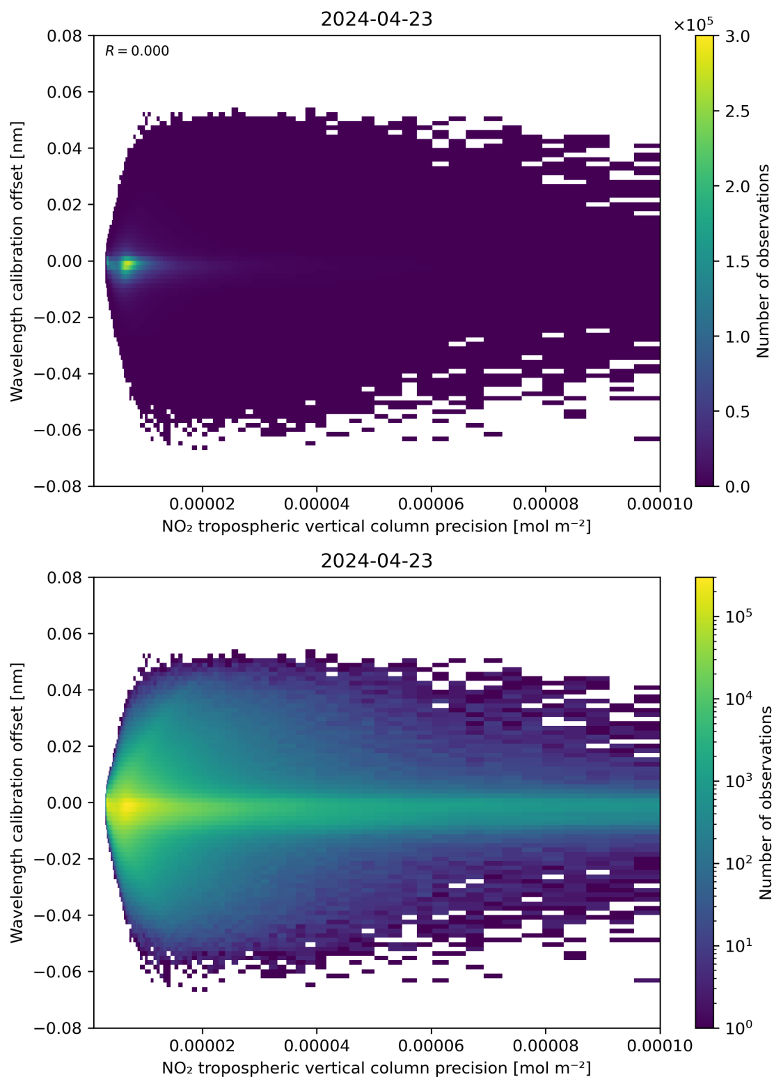
Figure 141: Scatter density plot of “NO 2 tropospheric vertical column precision” against “Wavelength calibration offset” for 2024-04-22 to 2024-04-24.
