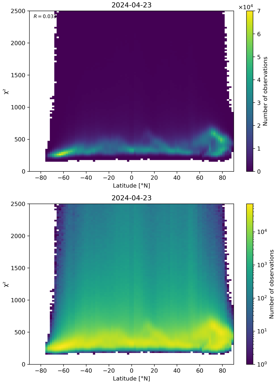
Figure 86: Scatter density plot of “Latitude” against “ \chi^2 ” for 2024-04-22 to 2024-04-24.
