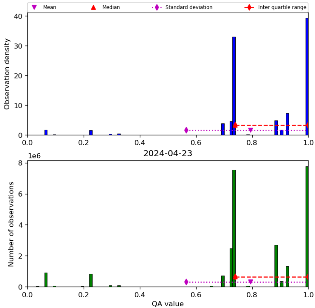
Figure 28: Histogram of “QA value” for 2024-04-22 to 2024-04-24
