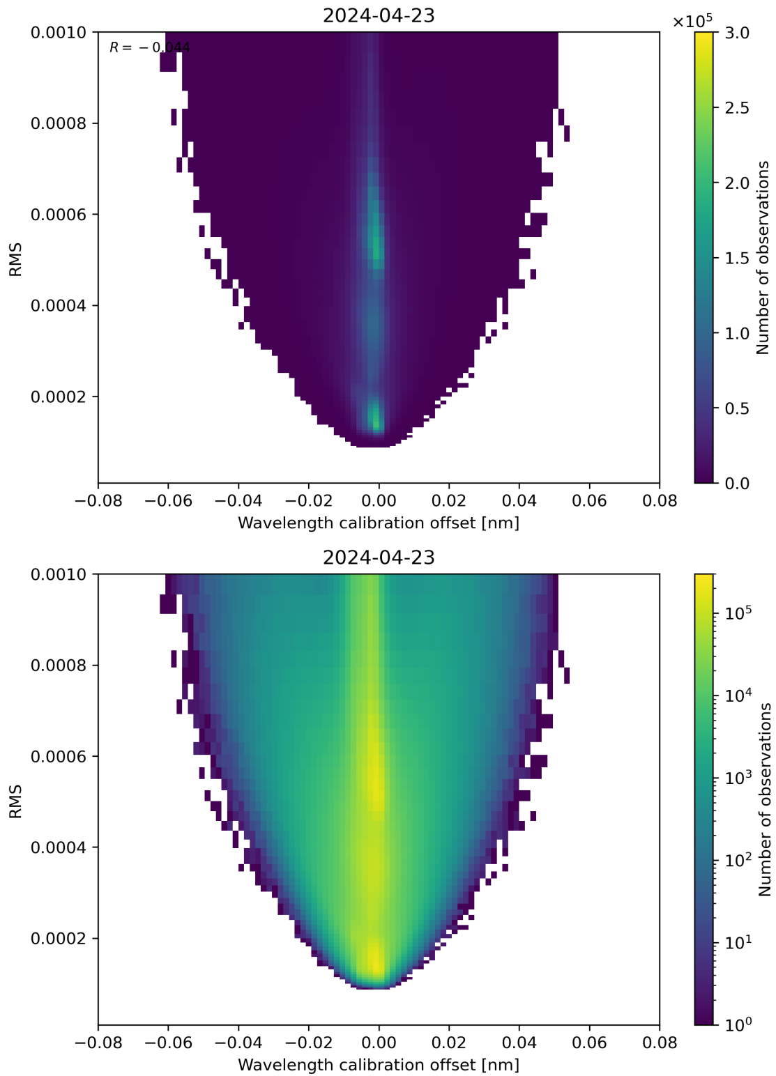
Figure 181: Scatter density plot of “Wavelength calibration offset” against “RMS” for 2024-04-22 to 2024-04-24.
