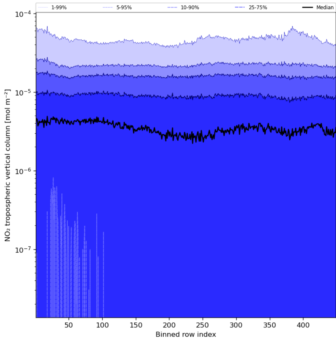
Figure 46: Along track statistics of “NO 2 tropospheric vertical column” for 2024-04-22 to 2024-04-24
