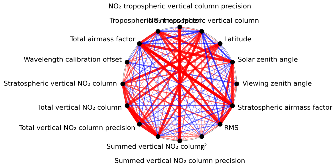
Figure 1: Map of correlation graph for 2024-04-22 to 2024-04-24.
