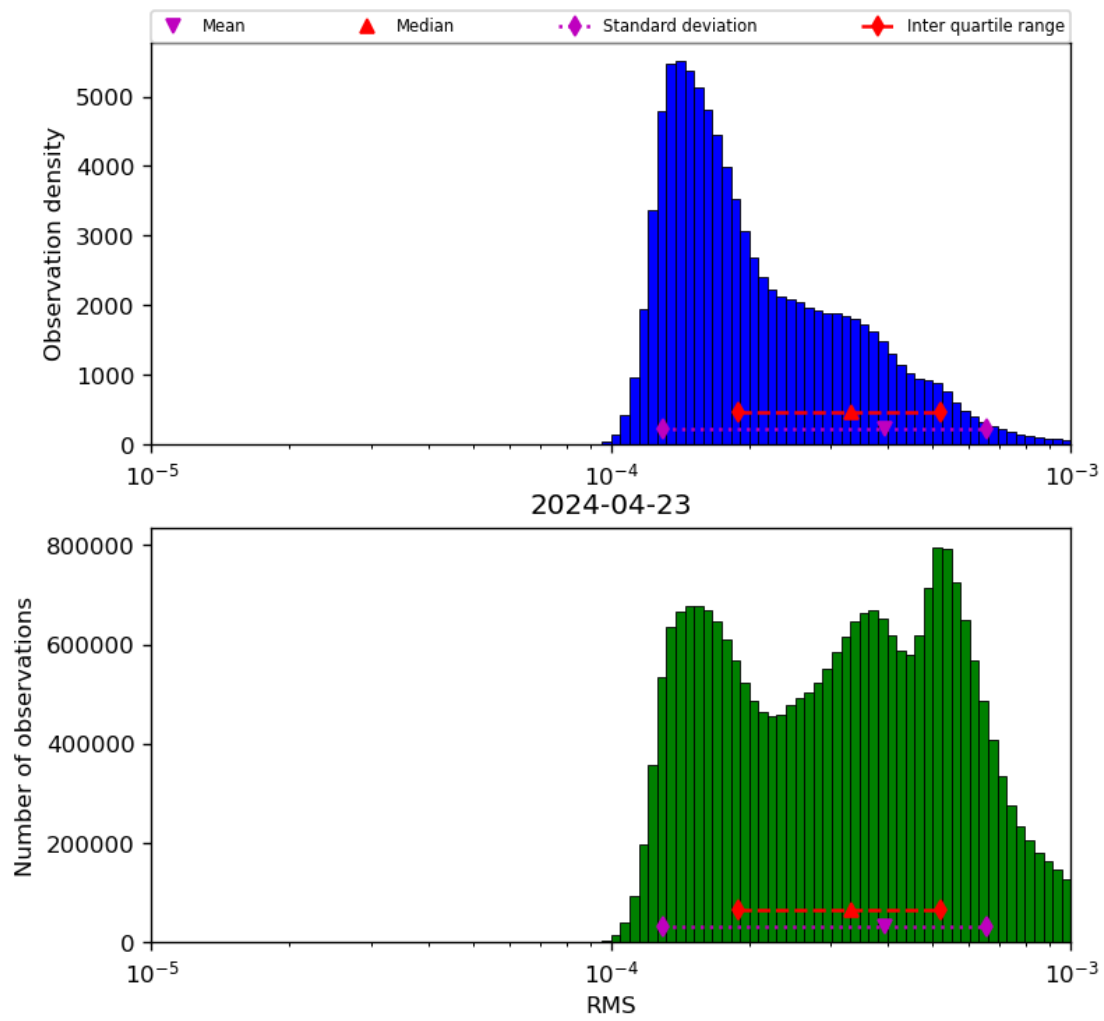
Figure 43: Histogram of “RMS” for 2024-04-22 to 2024-04-24
