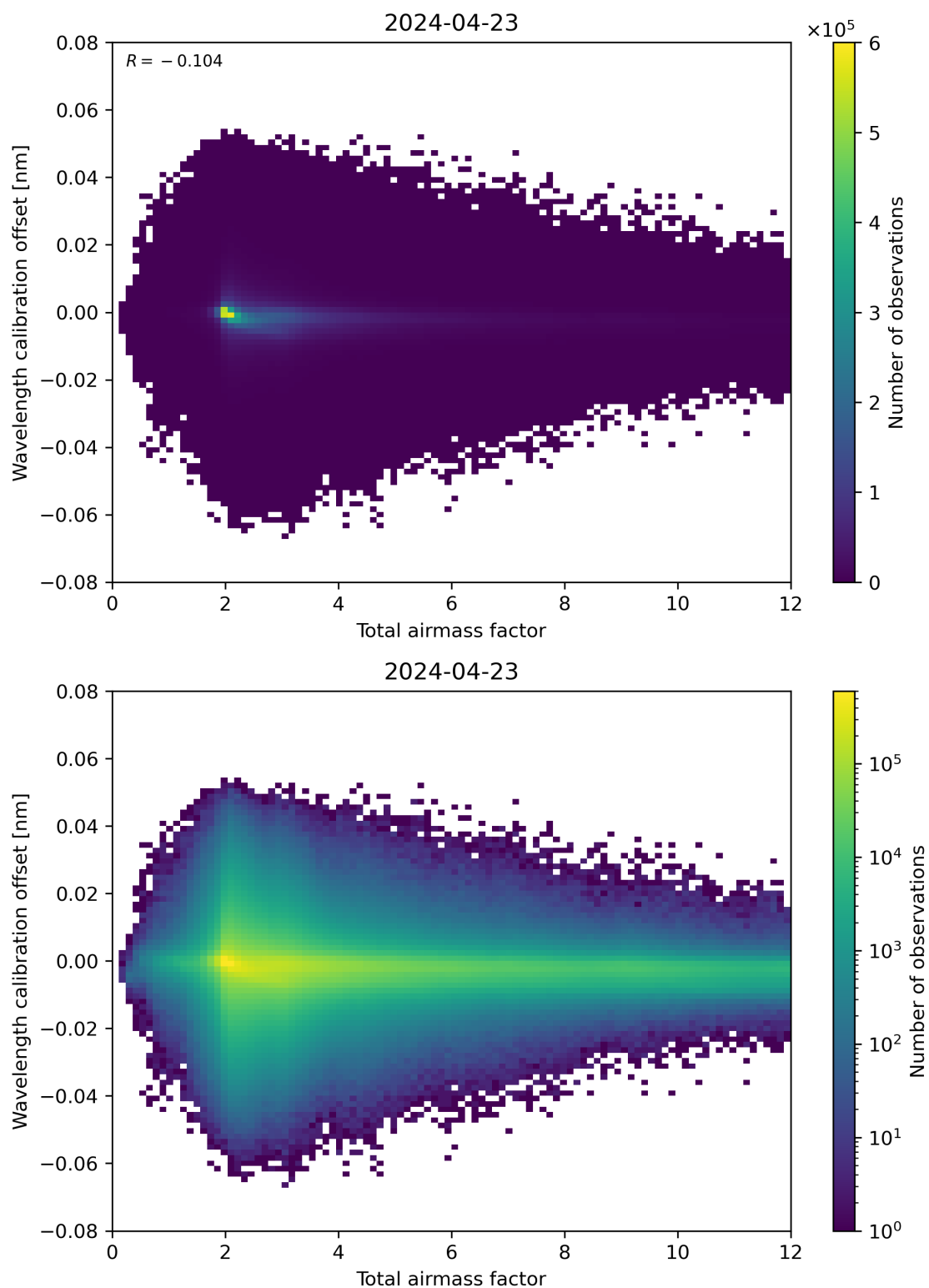
Figure 70: Scatter density plot of “Total airmass factor” against “Wavelength calibration offset” for 2024-04-22 to 2024-04-24.
