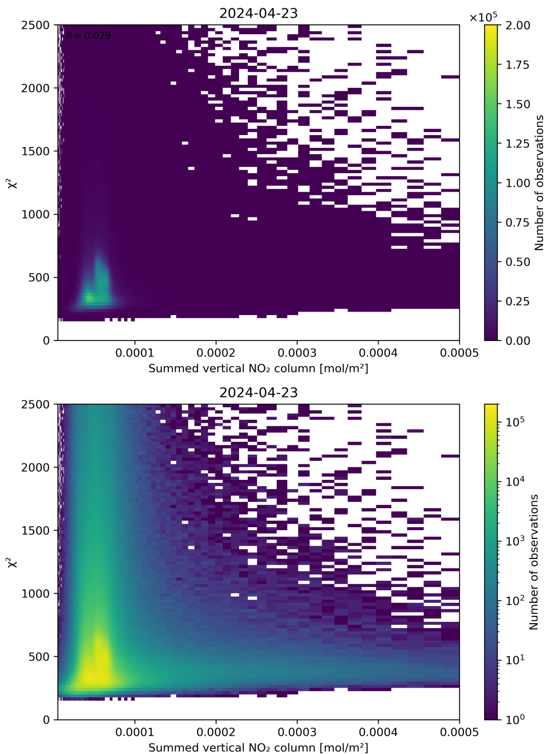
Figure 104: Scatter density plot of “Summed vertical NO 2 column” against “ \chi^2 ” for 2024-04-22 to 2024-04-24.
