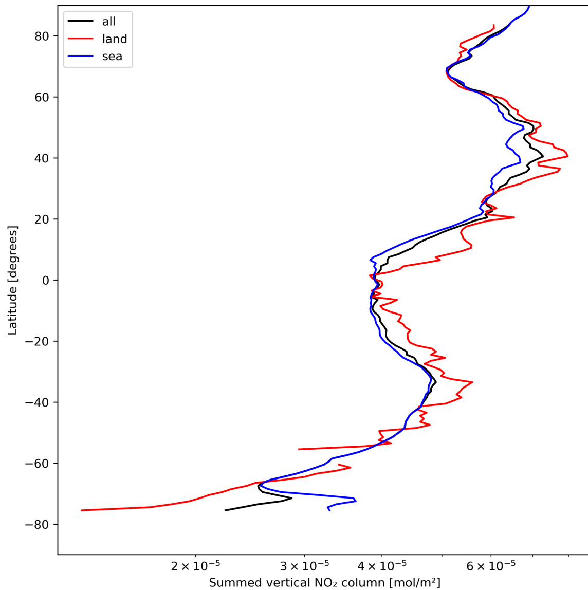
Figure 23: Zonal average of “Summed vertical NO 2 column” for 2024-04-22 to 2024-04-24.
