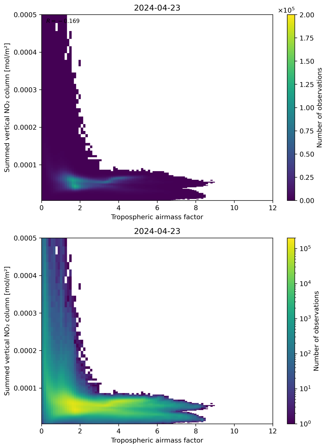
Figure 75: Scatter density plot of “Tropospheric airmass factor” against “Summed vertical NO 2 column” for 2024-04-22 to 2024-04-24.
