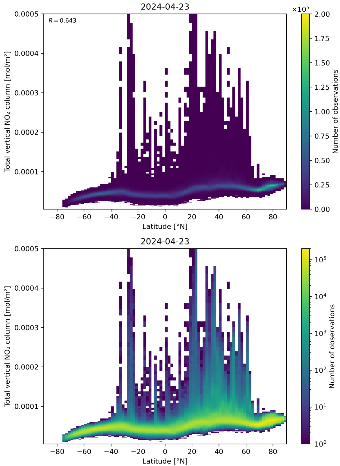
Figure 90: Scatter density plot of “Latitude” against “Total vertical NO 2 column” for 2024-04-22 to 2024-04-24.
