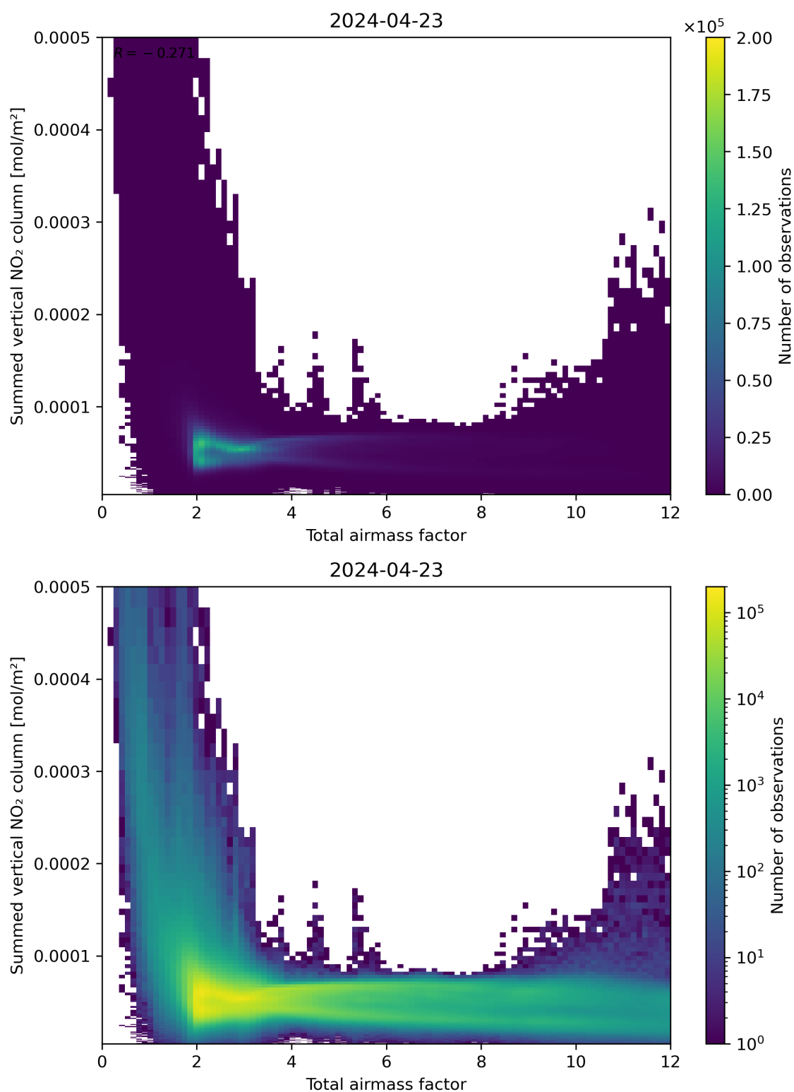
Figure 65: Scatter density plot of “Total airmass factor” against “Summed vertical NO 2 column” for 2024-04-22 to 2024-04-24.
