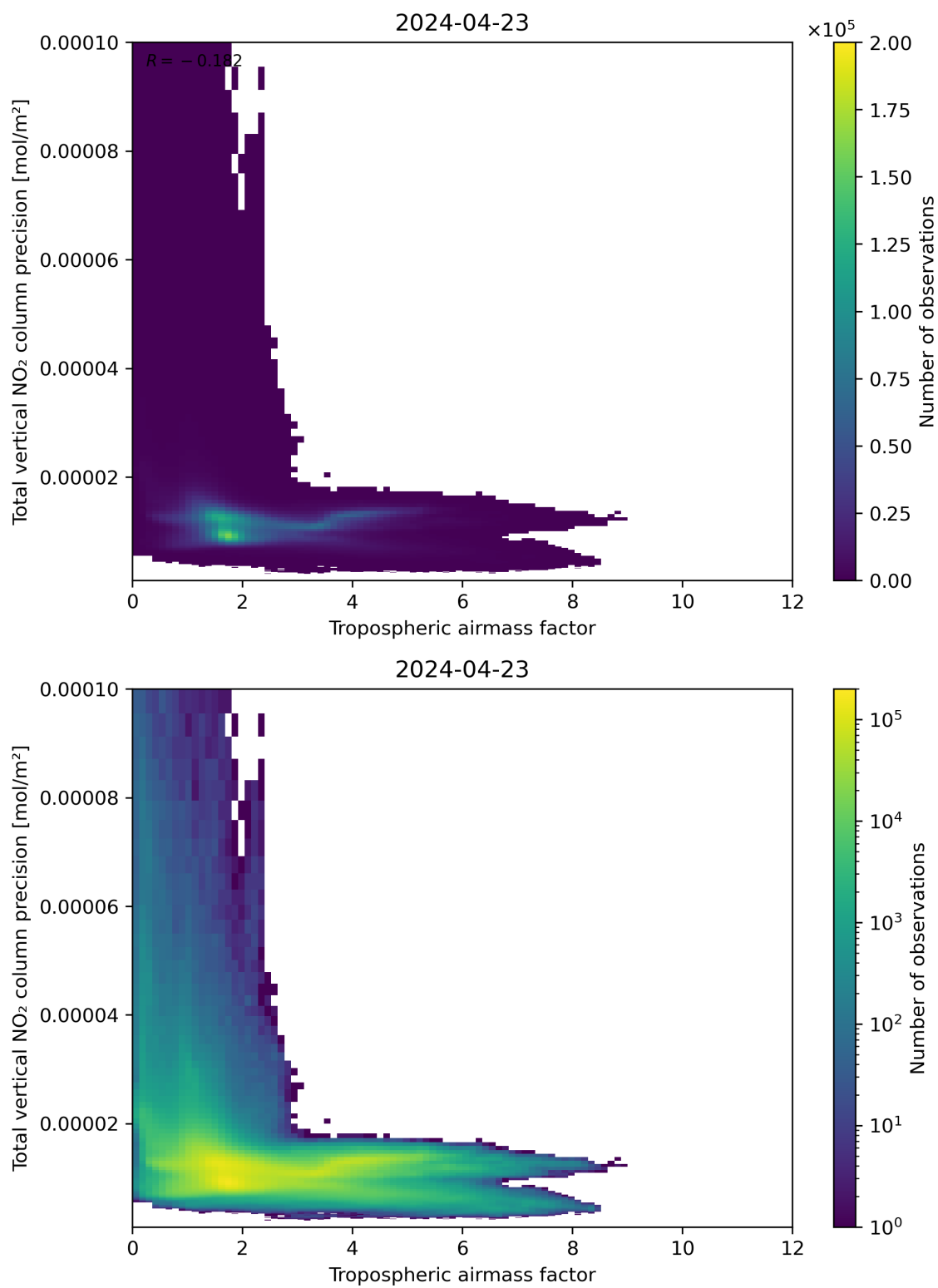
Figure 78: Scatter density plot of “Tropospheric air mass factor” against “Total vertical NO 2 column precision” for 2024-04-22 to 2024-04-24.
