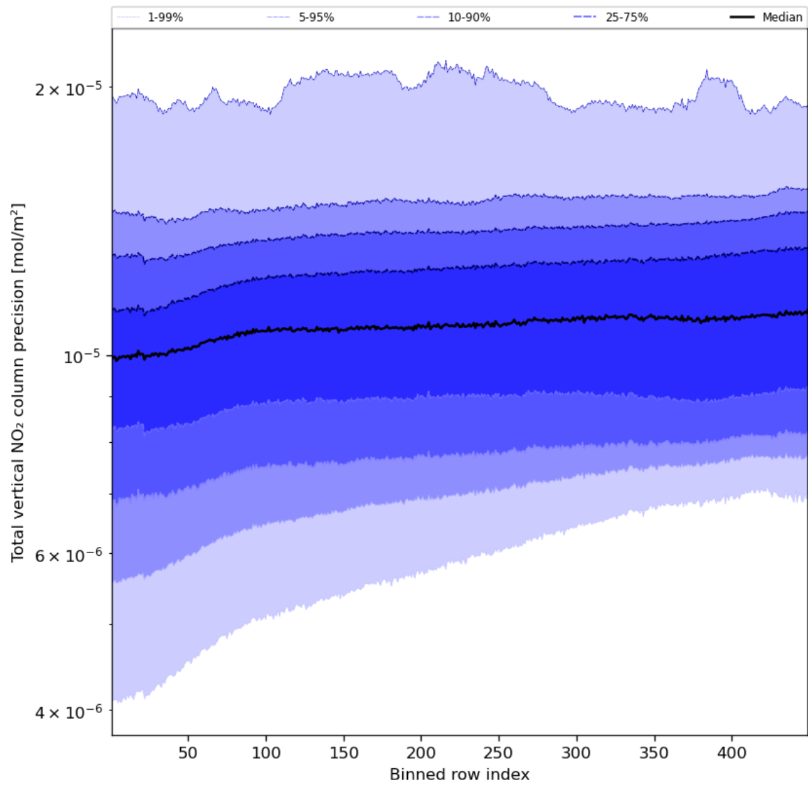
Figure 56: Along track statistics of “Total vertical NO 2 column precision” for 2024-04-22 to 2024-04-24
