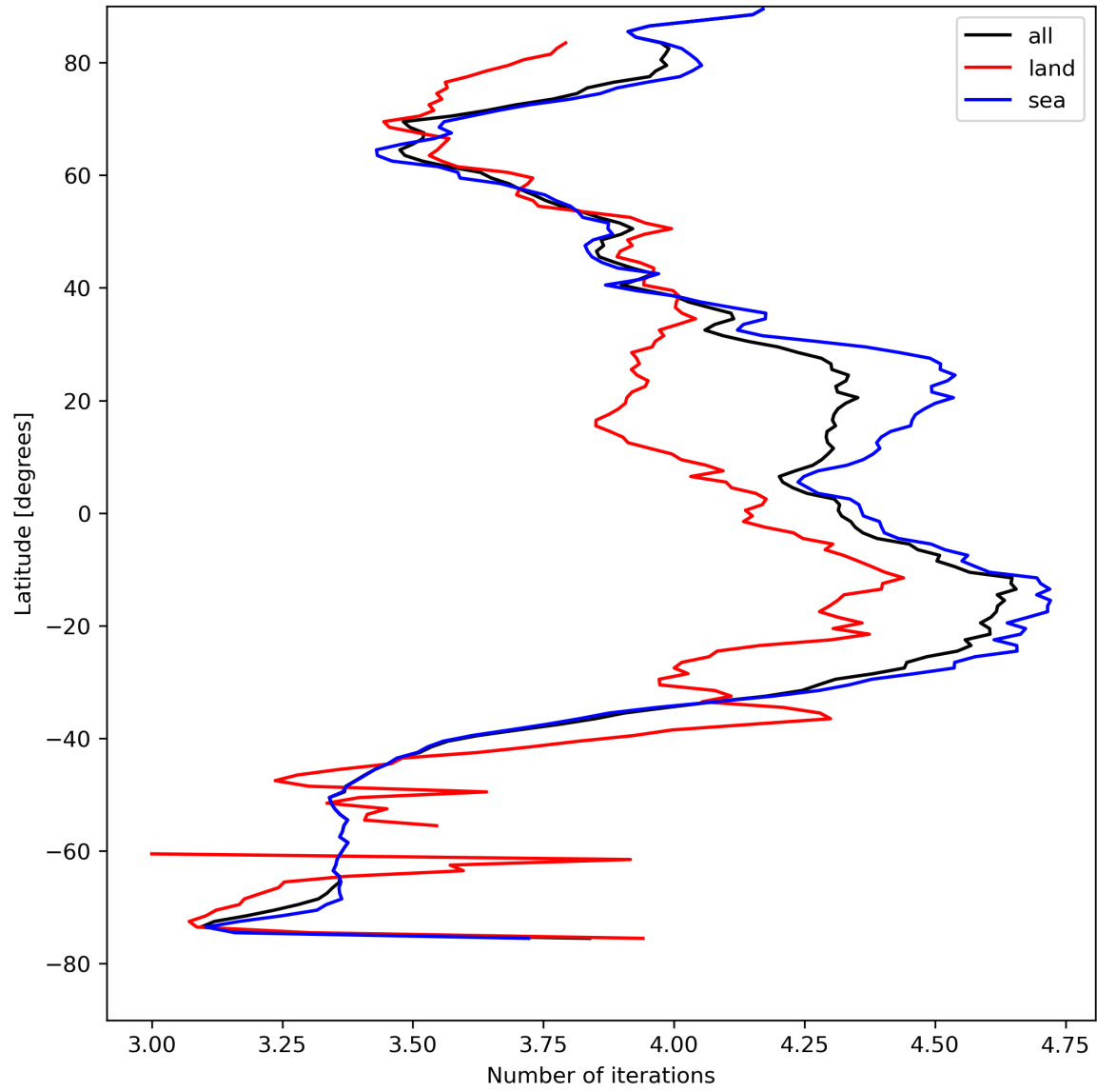
Figure 17: Zonal average of “Number of iterations” for 2024-04-22 to 2024-04-24.
