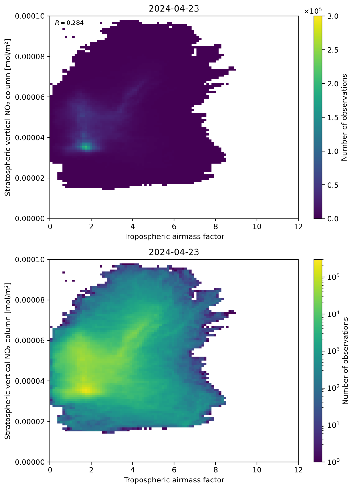
Figure 74: Scatter density plot of “Tropospheric air mass factor” against “Stratospheric vertical NO 2 column” for 2024-04-22 to 2024-04-24.
