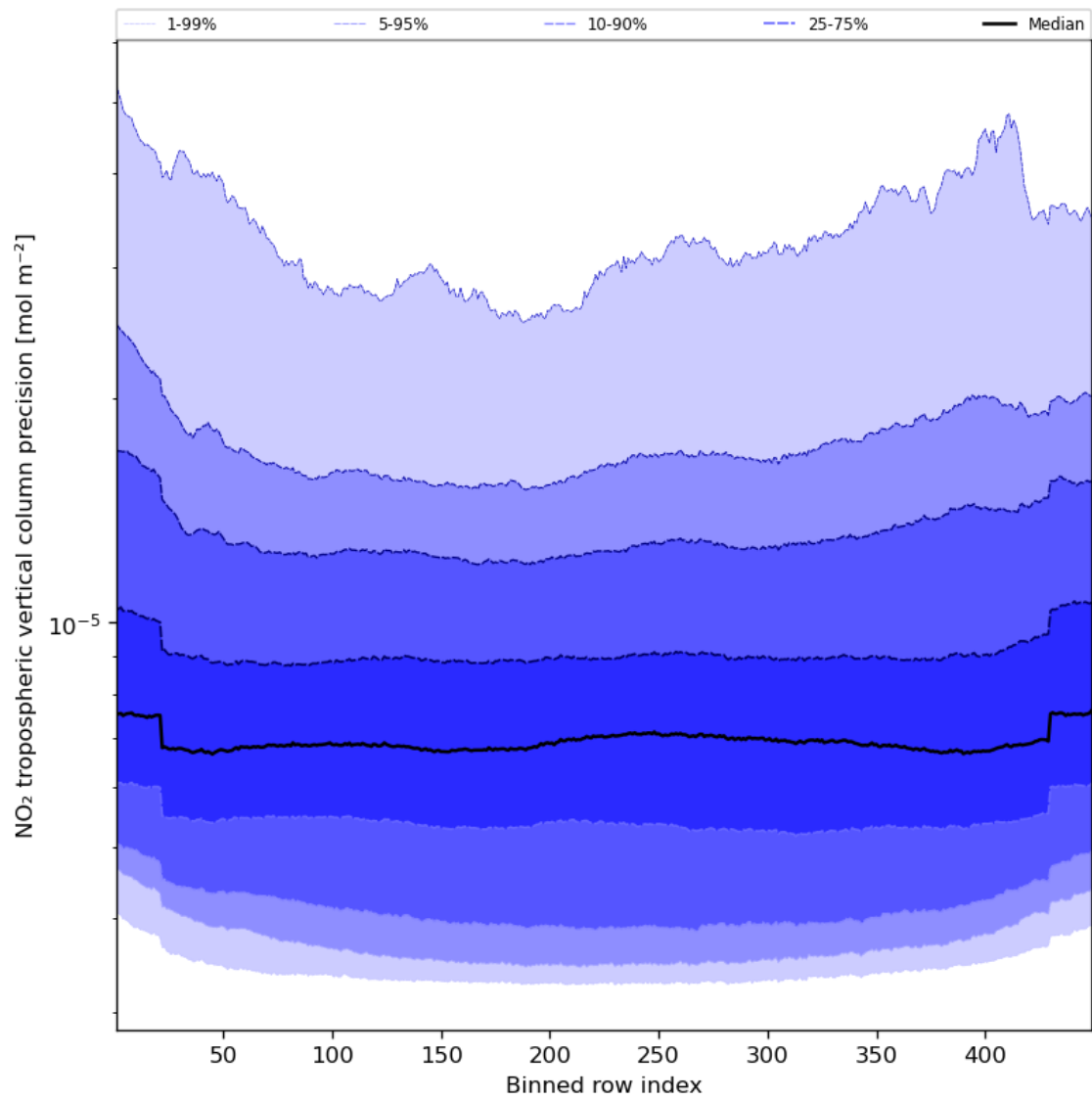
Figure 47: Along track statistics of “NO 2 tropospheric vertical column precision” for 2024-04-22 to 2024-04-24
