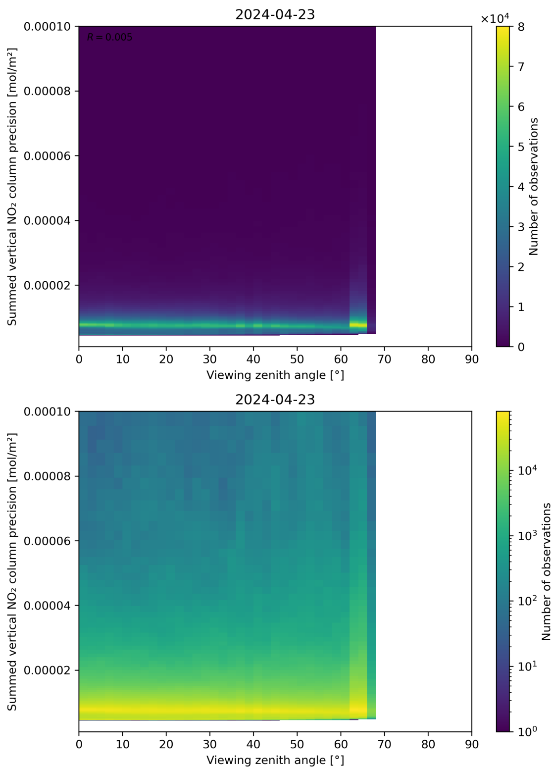
Figure 166: Scatter density plot of “Viewing zenith angle” against “Summed vertical NO 2 column precision” for 2024-04-22 to 2024-04-24.
