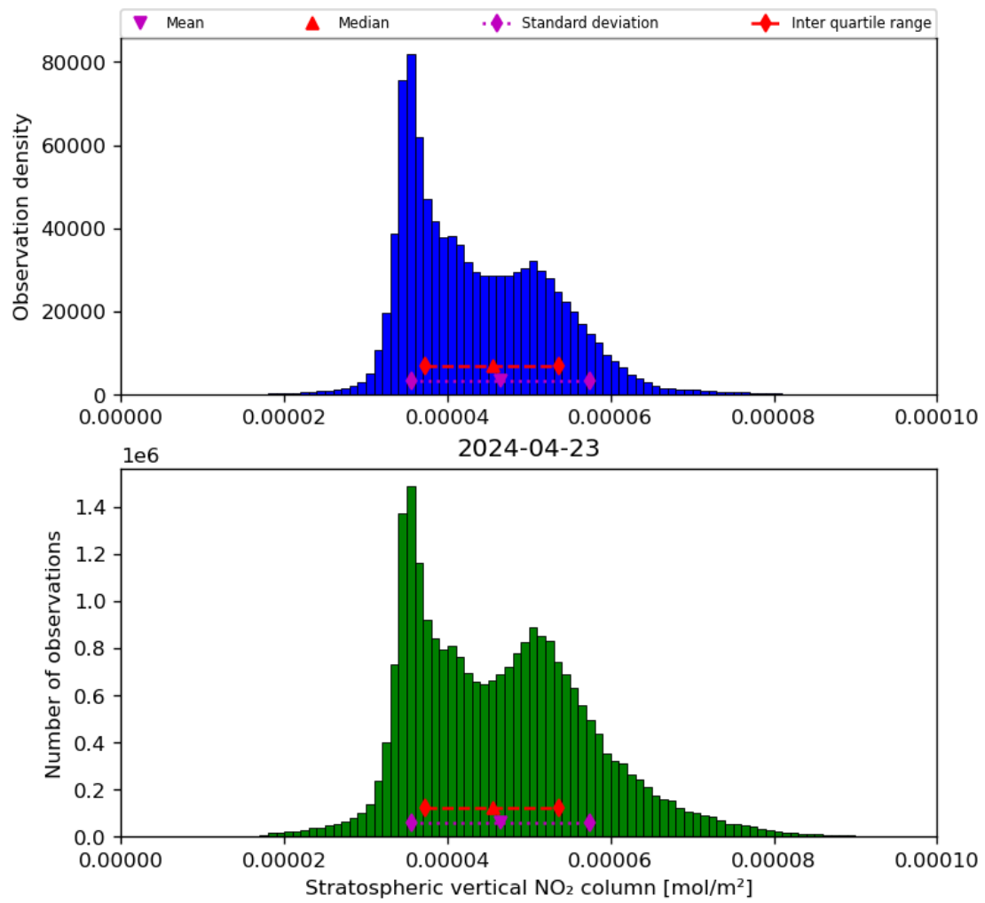
Figure 36: Histogram of “Stratospheric vertical NO 2 column” for 2024-04-22 to 2024-04-24
