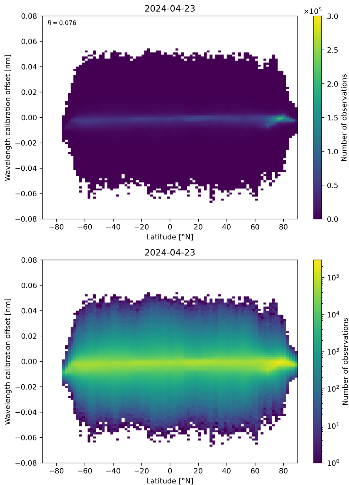
Figure 95: Scatter density plot of “Latitude” against “Wavelength calibration offset” for 2024-04-22 to 2024-04-24.
