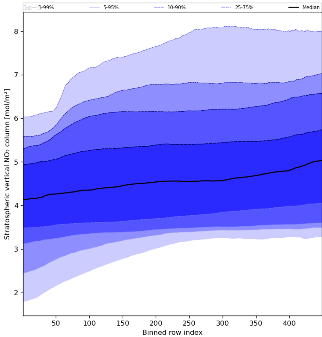
Figure 53: Along track statistics of “Stratospheric vertical NO 2 column” for 2024-04-22 to 2024-04-24
