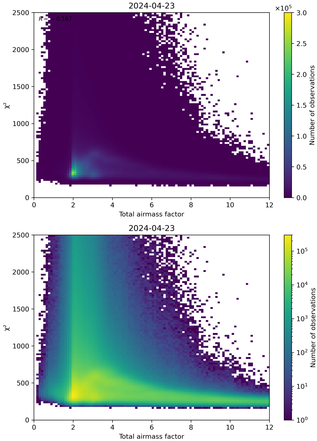
Figure 63: Scatter density plot of “Total airmass factor” against “ \chi^2 ” for 2024-04-22 to 2024-04-24.
