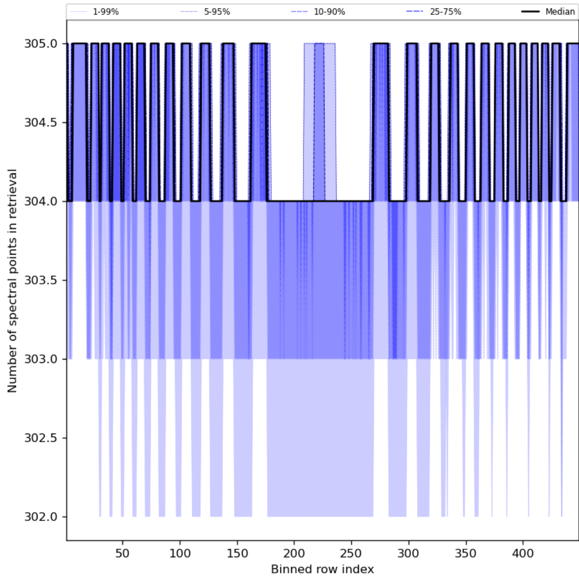
Figure 50: Along track statistics of “Number of spectral points in retrieval” for 2024-04-22 to 2024-04-24
