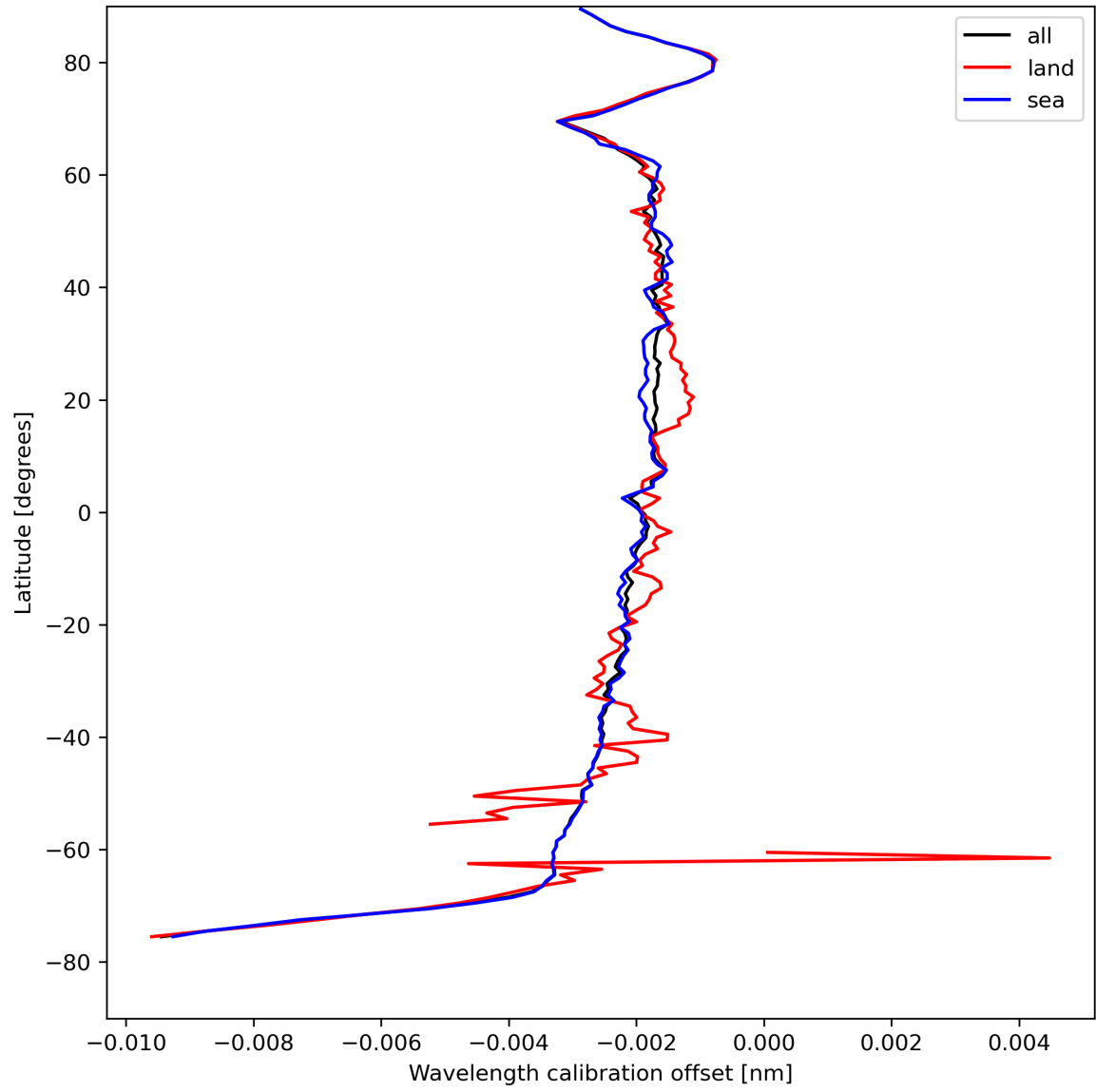
Figure 18: Zonal average of “Wavelength calibration offset” for 2024-04-22 to 2024-04-24.
