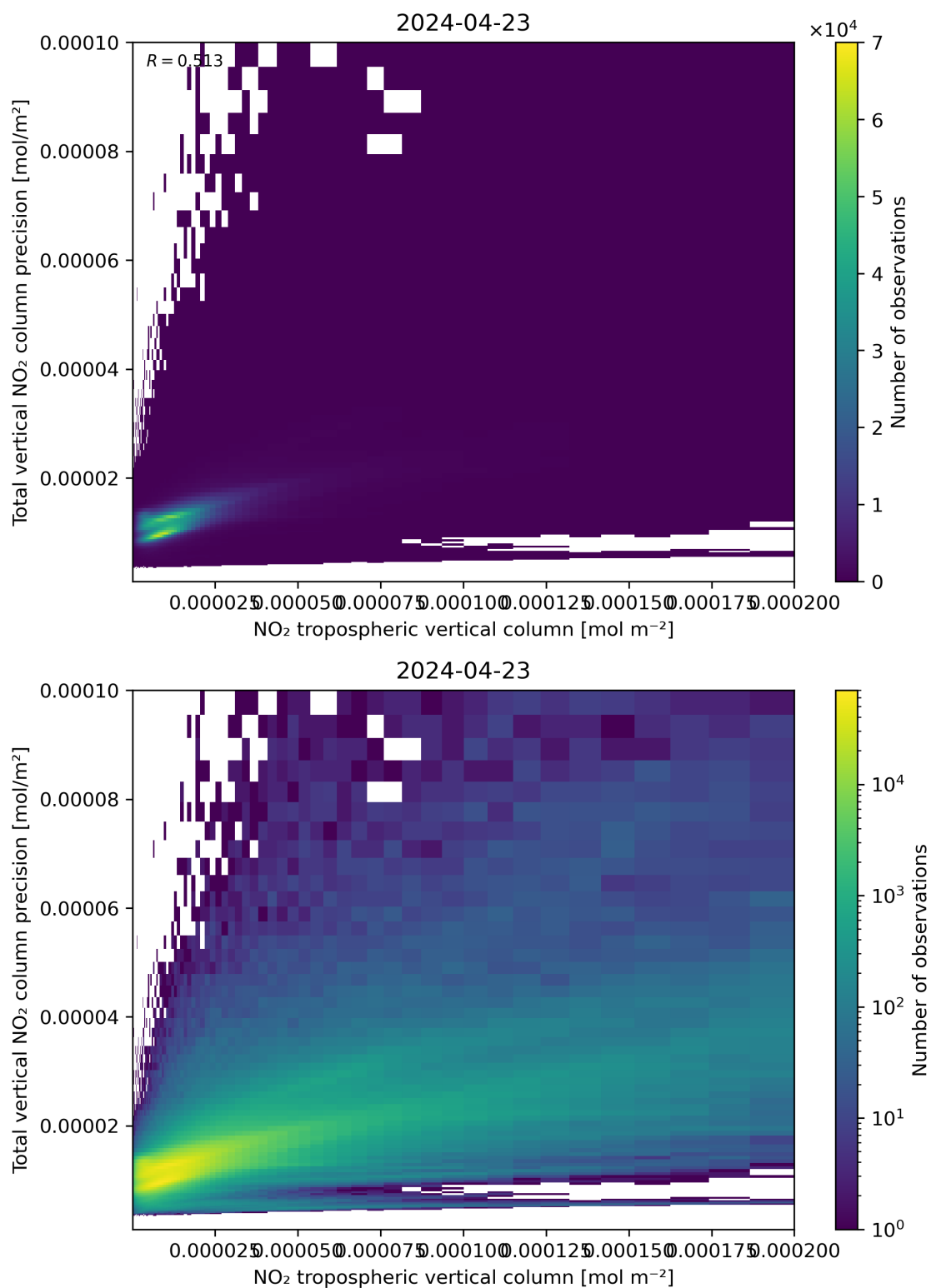
Figure 129: Scatter density plot of “NO 2 tropospheric vertical column” against “Total vertical NO 2 column precision” for 2024-04-22 to 2024-04-24.
