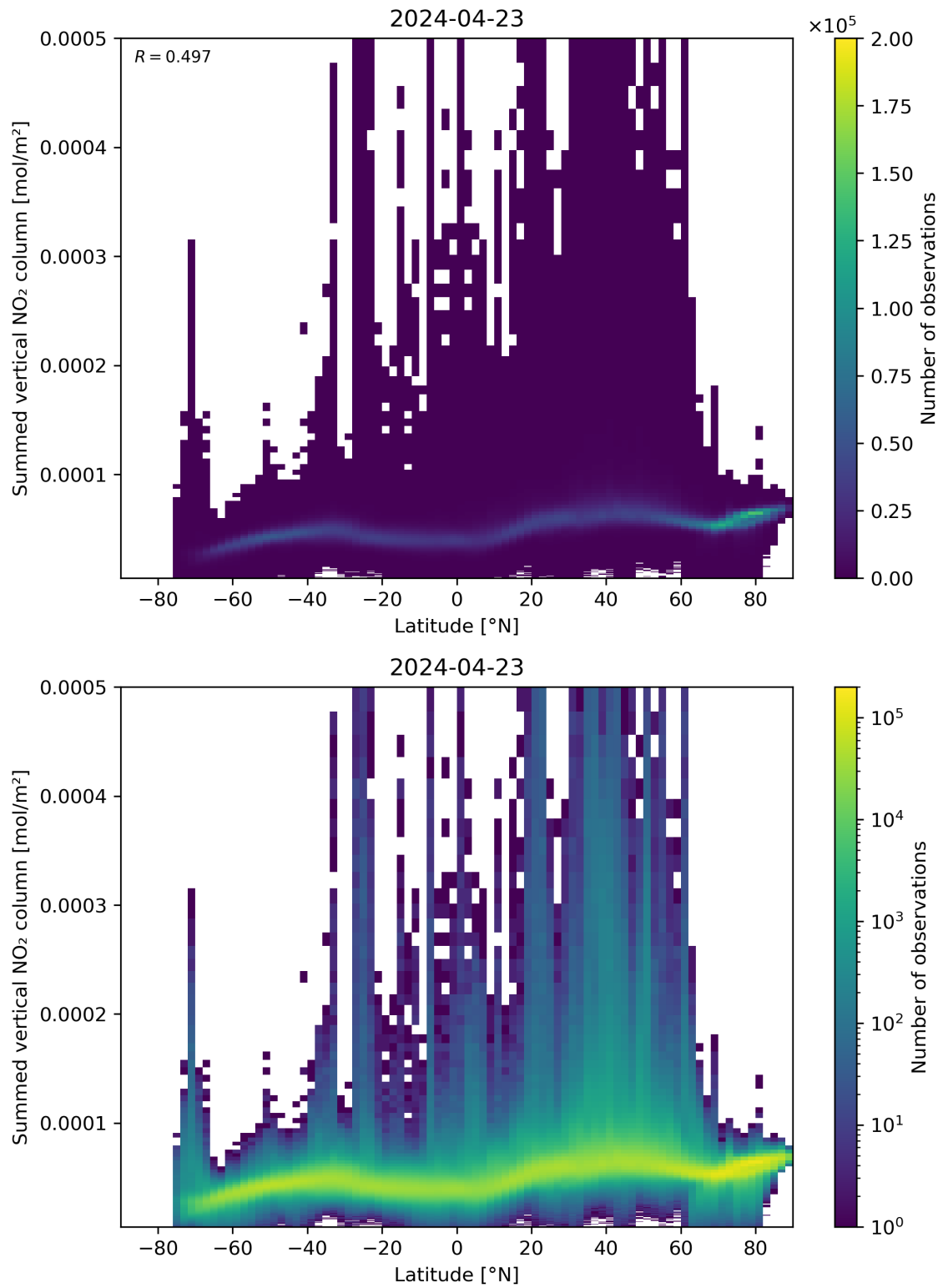
Figure 88: Scatter density plot of “Latitude” against “Summed vertical NO 2 column” for 2024-04-22 to 2024-04-24.
