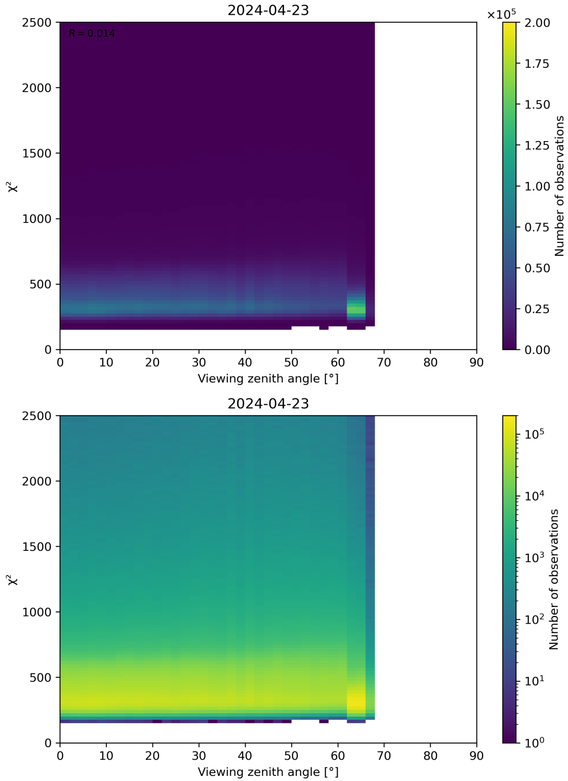
Figure 162: Scatter density plot of “Viewing zenith angle” against “ \chi^2 ” for 2024-04-22 to 2024-04-24.
