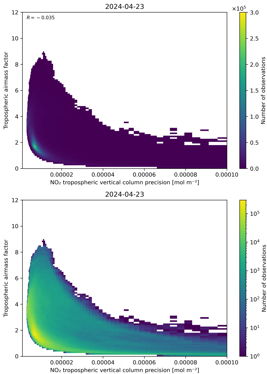
Figure 133: Scatter density plot of “NO 2 tropospheric vertical column precision” against “Tropospheric airmass factor” for 2024-04-22 to 2024-04-24.
