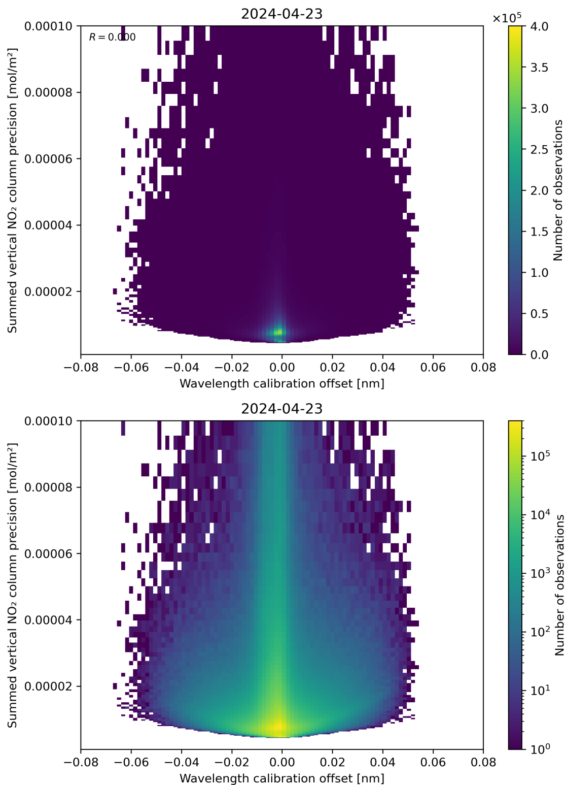
Figure 178: Scatter density plot of “Wavelength calibration offset” against “Summed vertical NO 2 column precision” for 2024-04-22 to 2024-04-24.
