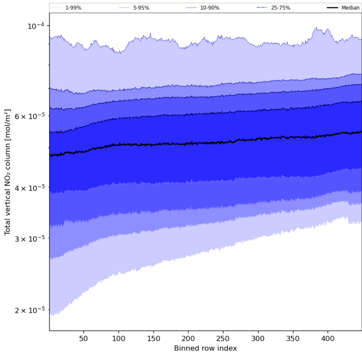
Figure 55: Along track statistics of “Total vertical NO 2 column” for 2024-04-22 to 2024-04-24
