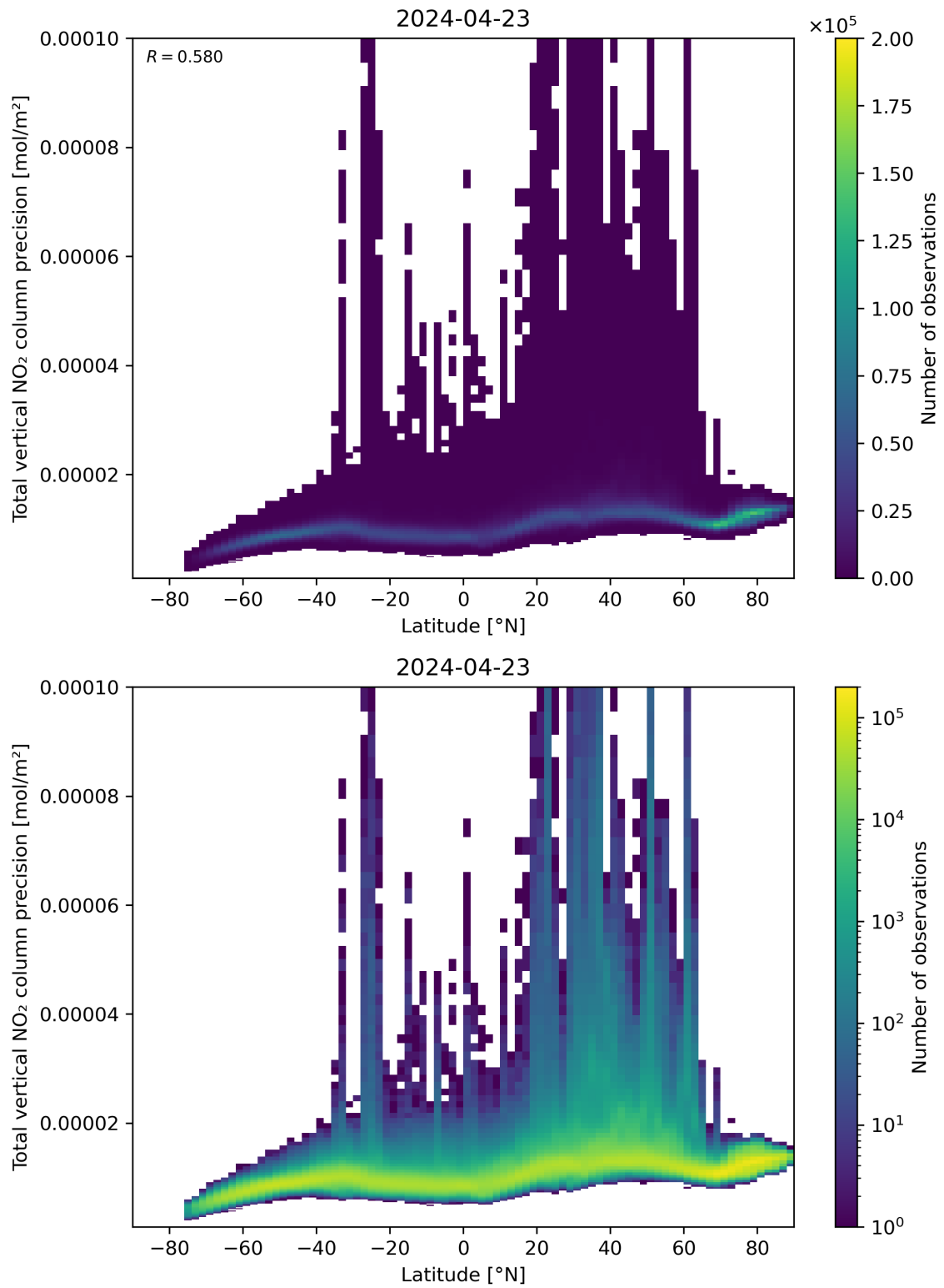
Figure 91: Scatter density plot of “Latitude” against “Total vertical NO 2 column precision” for 2024-04-22 to 2024-04-24.
