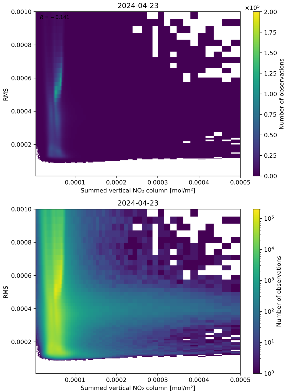
Figure 109: Scatter density plot of “Summed vertical NO 2 column” against “RMS” for 2024-04-22 to 2024-04-24.
