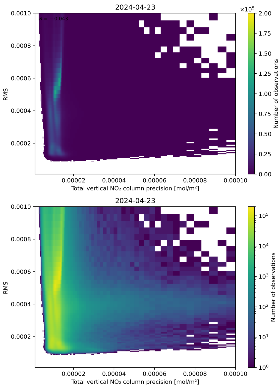
Figure 119: Scatter density plot of “Total vertical NO 2 column precision” against “RMS” for 2024-04-22 to 2024-04-24.
