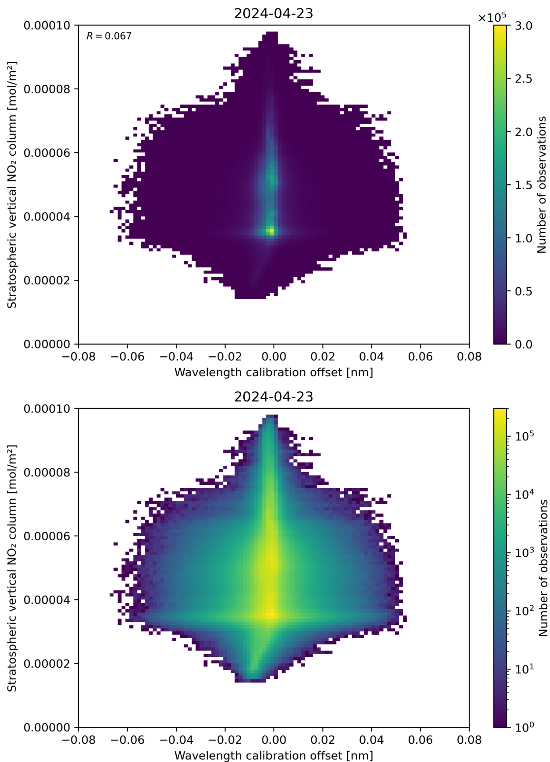
Figure 176: Scatter density plot of “Wavelength calibration offset” against “Stratospheric vertical NO 2 column” for 2024-04-22 to 2024-04-24.
