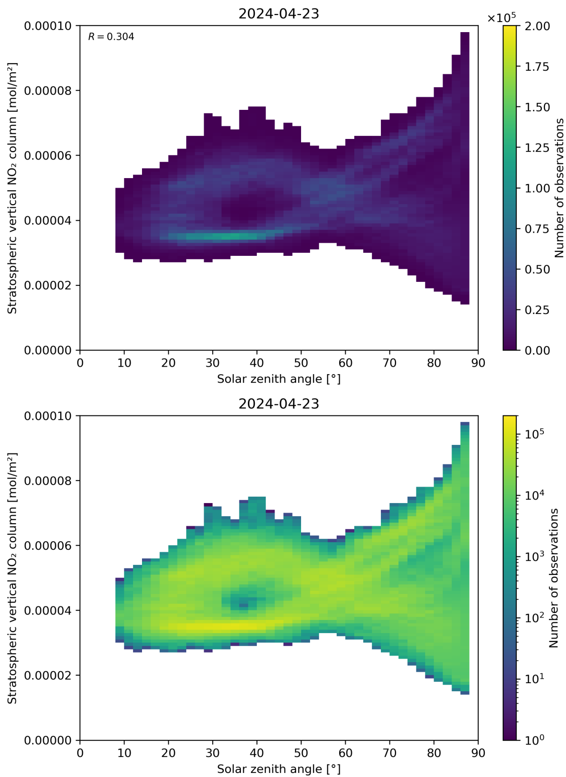
Figure 150: Scatter density plot of “Solar zenith angle” against “Stratospheric vertical NO 2 column” for 2024-04-22 to 2024-04-24.
