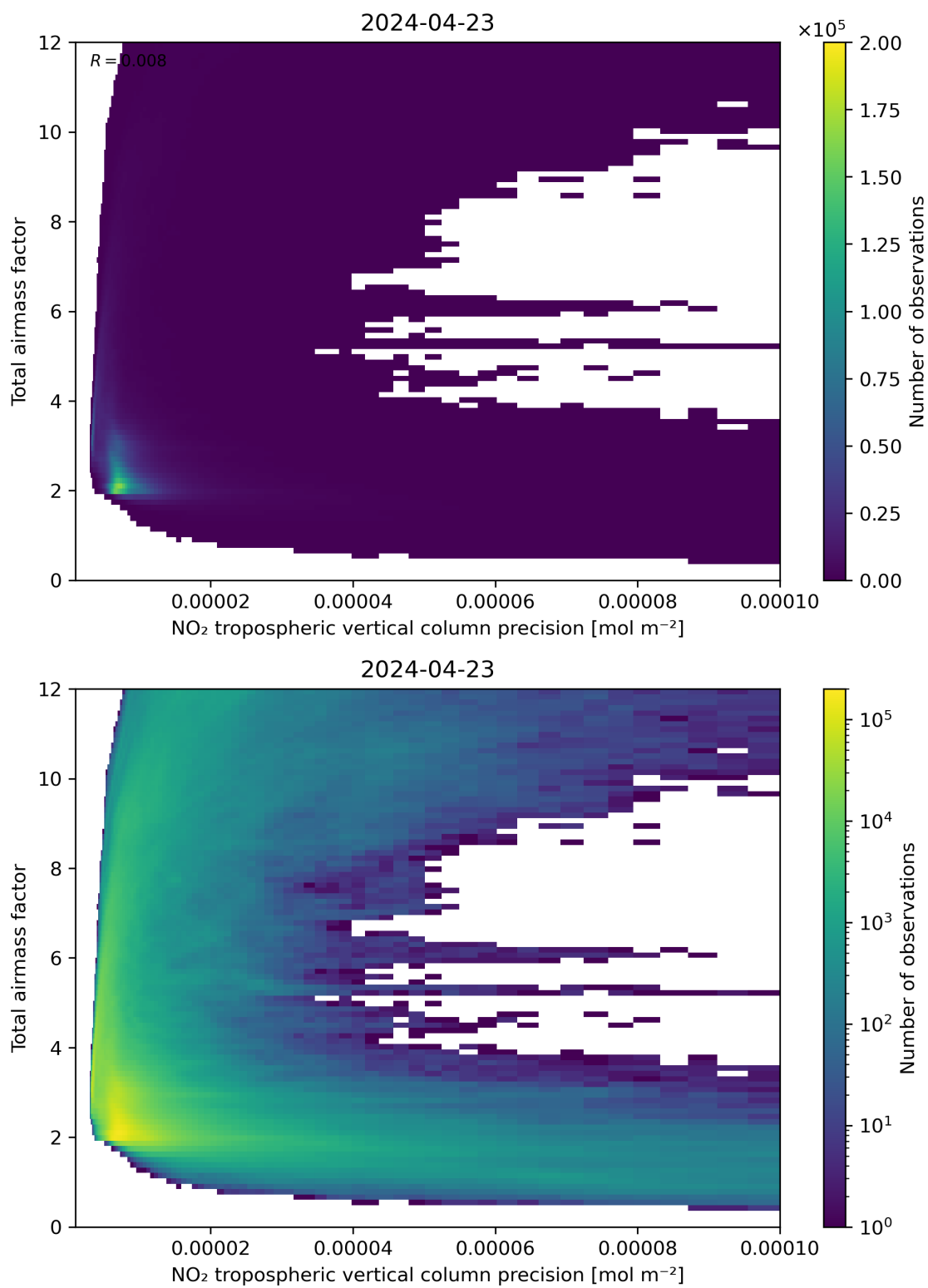
Figure 132: Scatter density plot of “NO 2 tropospheric vertical column precision” against “Total air mass factor” for 2024-04-22 to 2024-04-24.
