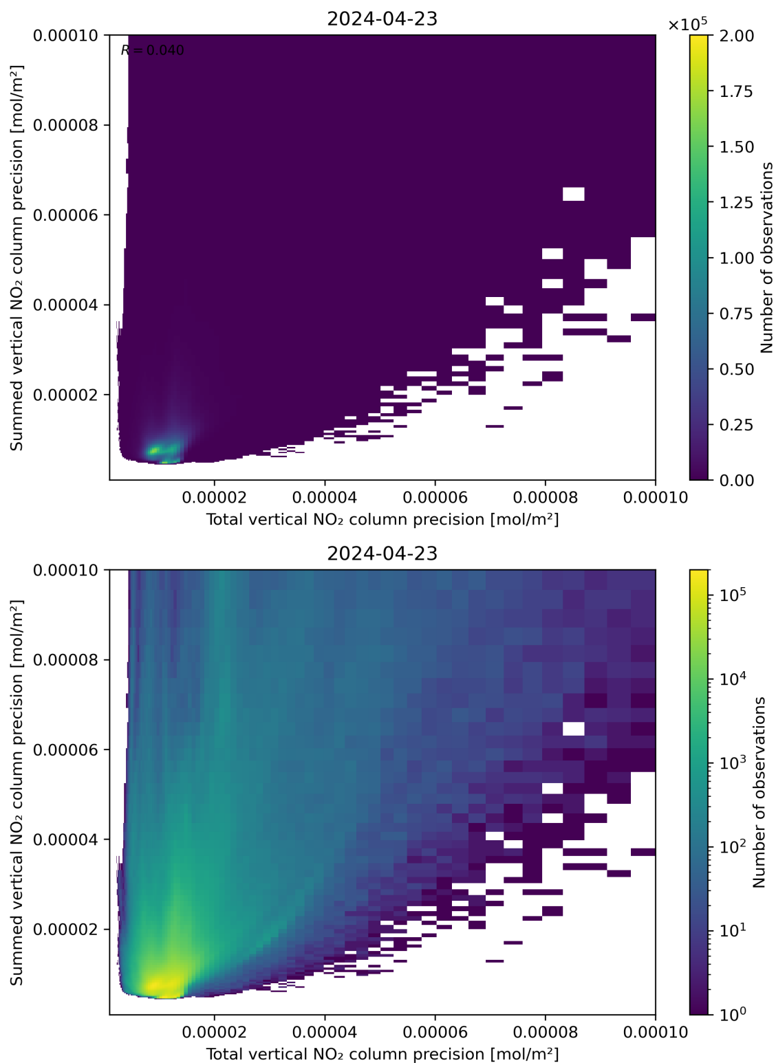
Figure 118: Scatter density plot of “Total vertical NO 2 column precision” against “Summed vertical NO 2 column precision” for 2024-04-22 to 2024-04-24.
