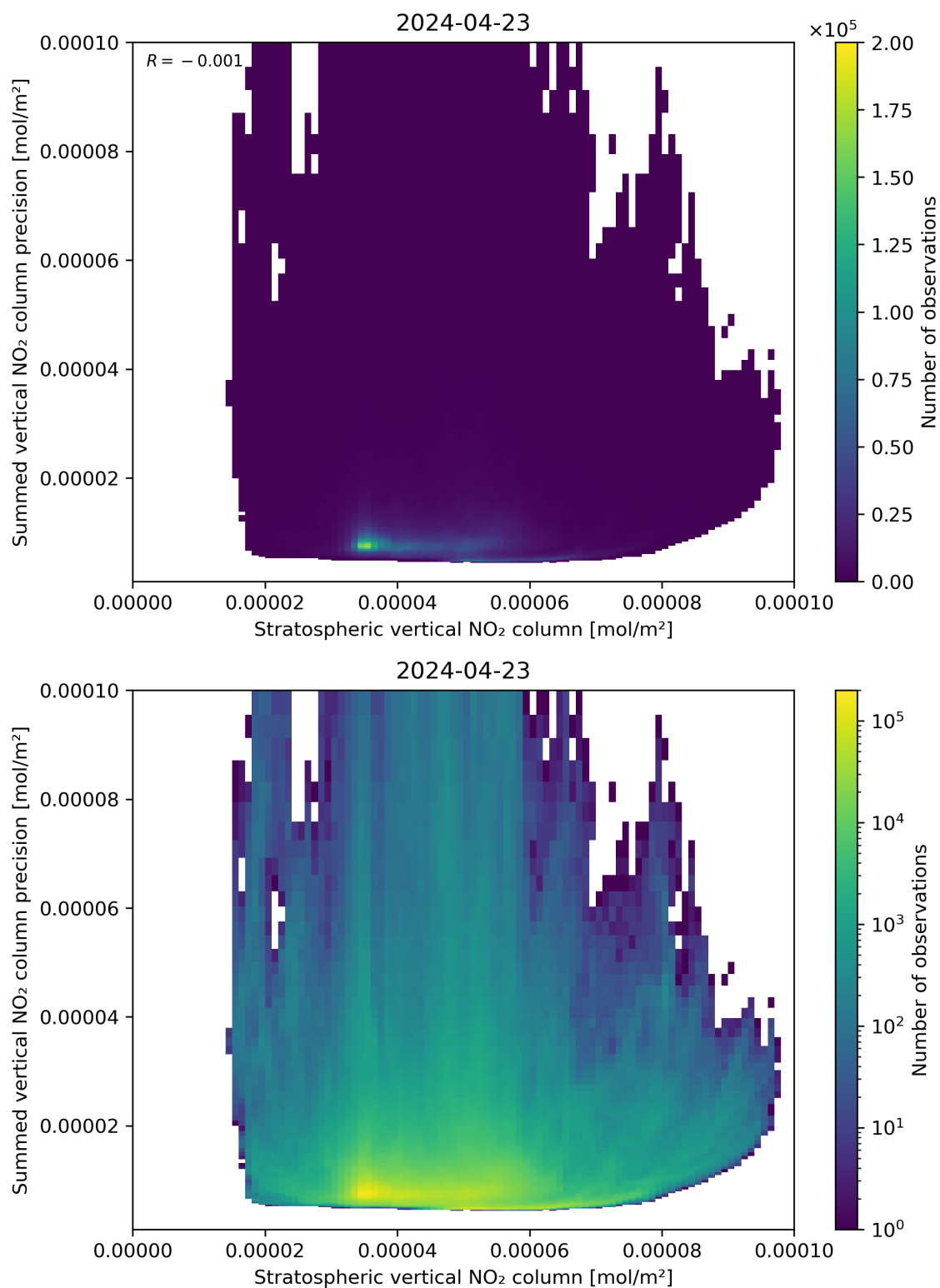
Figure 99: Scatter density plot of “Stratospheric vertical NO 2 column” against “Summed vertical NO 2 column precision” for 2024-04-22 to 2024-04-24.
