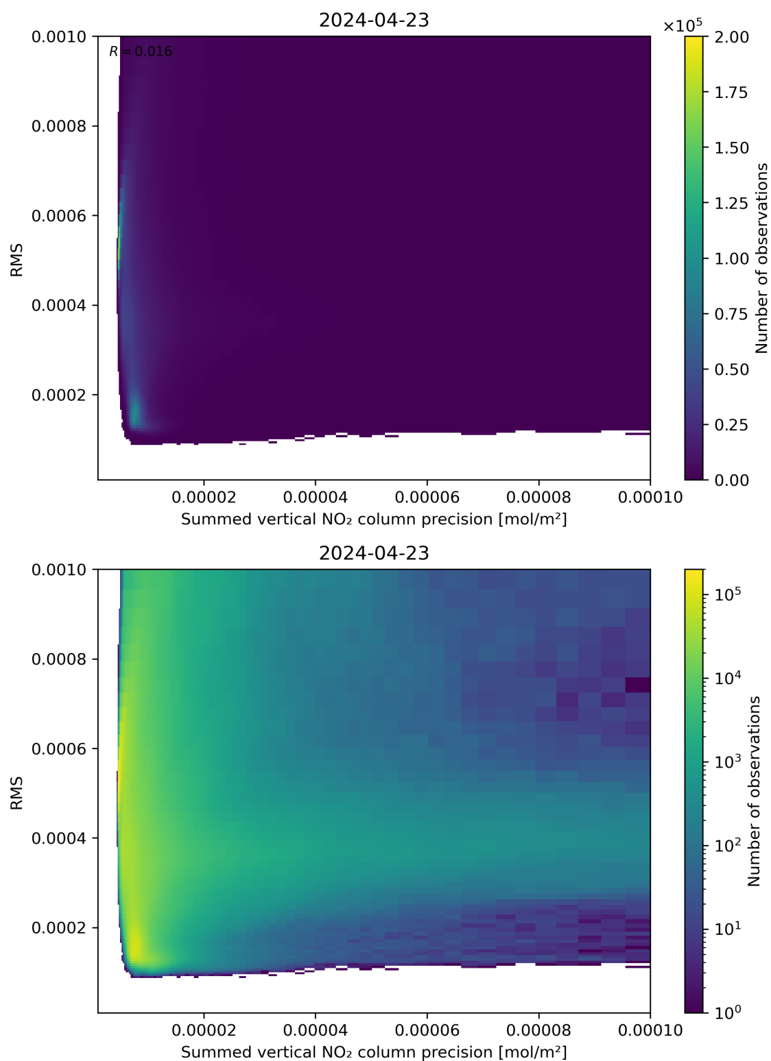
Figure 108: Scatter density plot of “Summed vertical NO 2 column precision” against “RMS” for 2024-04-22 to 2024-04-24.
