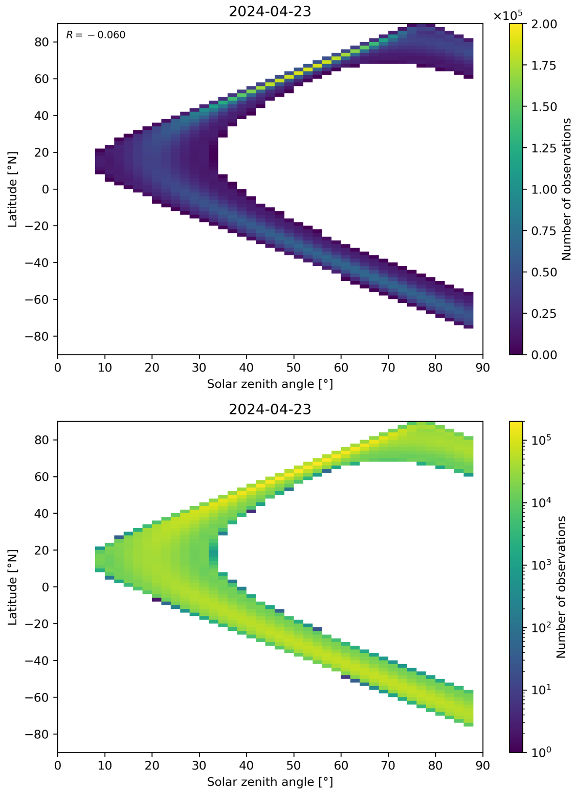
Figure 149: Scatter density plot of “Solar zenith angle” against “Latitude” for 2024-04-22 to 2024-04-24.
