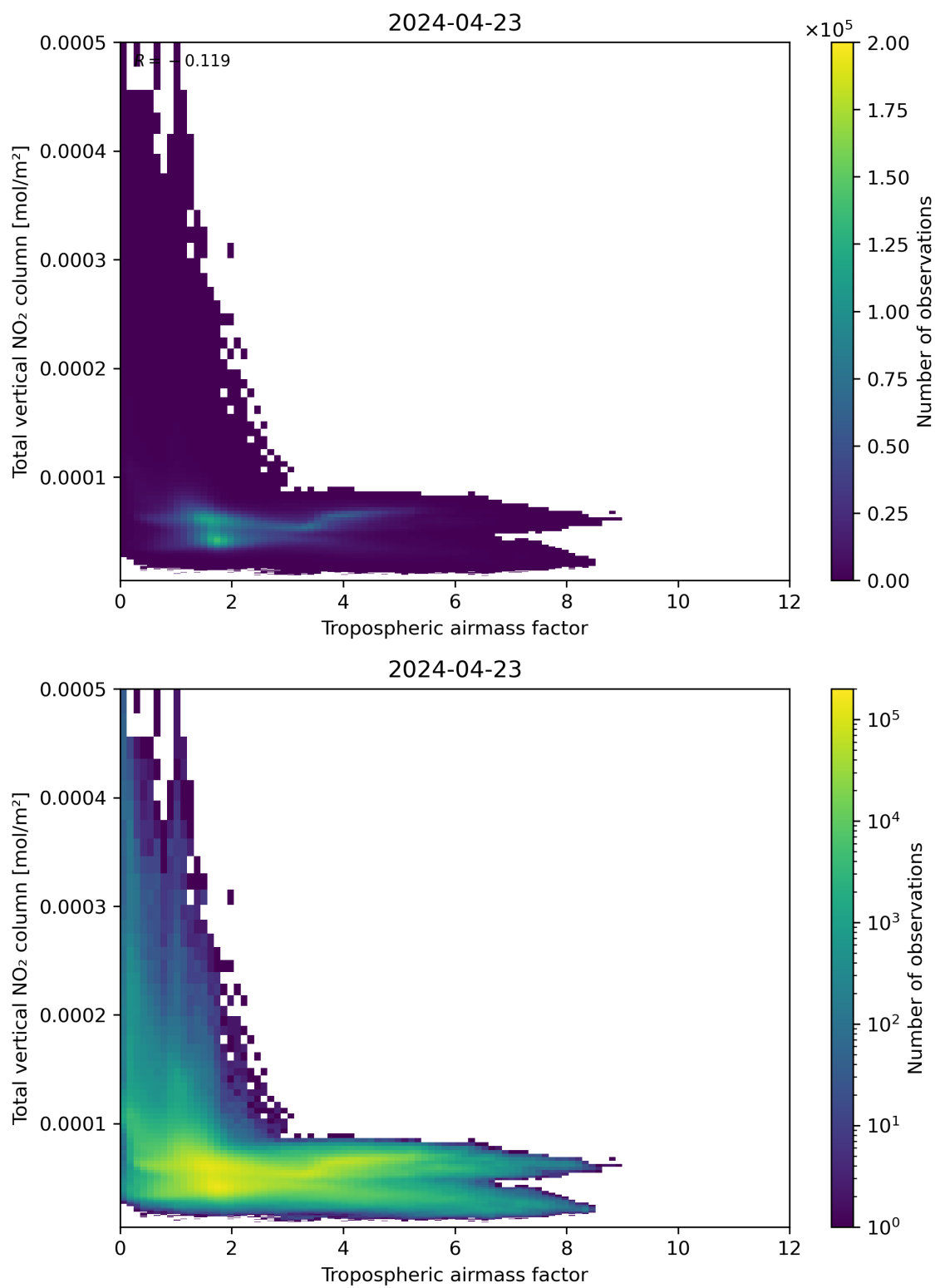
Figure 77: Scatter density plot of “Tropospheric airmass factor” against “Total vertical NO 2 column” for 2024-04-22 to 2024-04-24.
