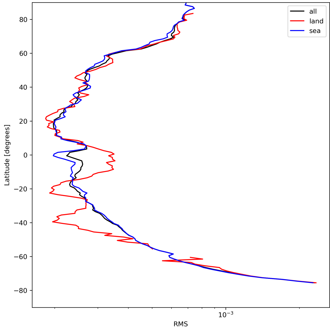
Figure 26: Zonal average of “RMS” for 2024-04-22 to 2024-04-24.
