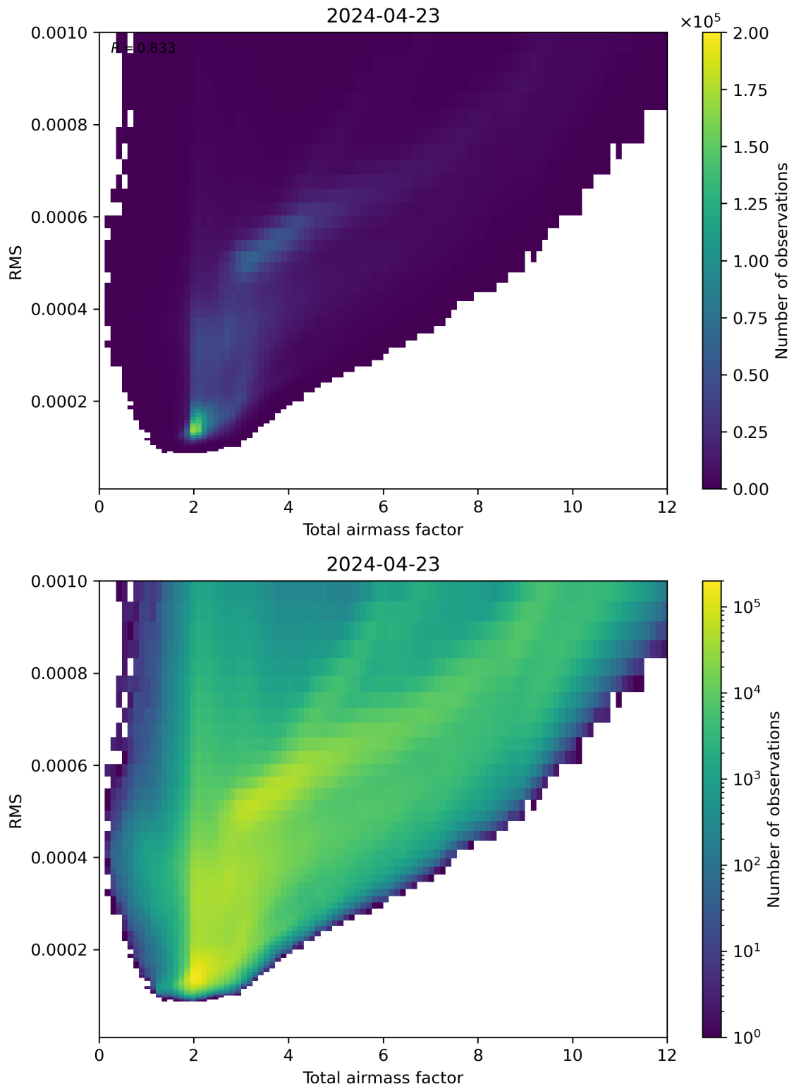
Figure 69: Scatter density plot of “Total airmass factor” against “RMS” for 2024-04-22 to 2024-04-24.
