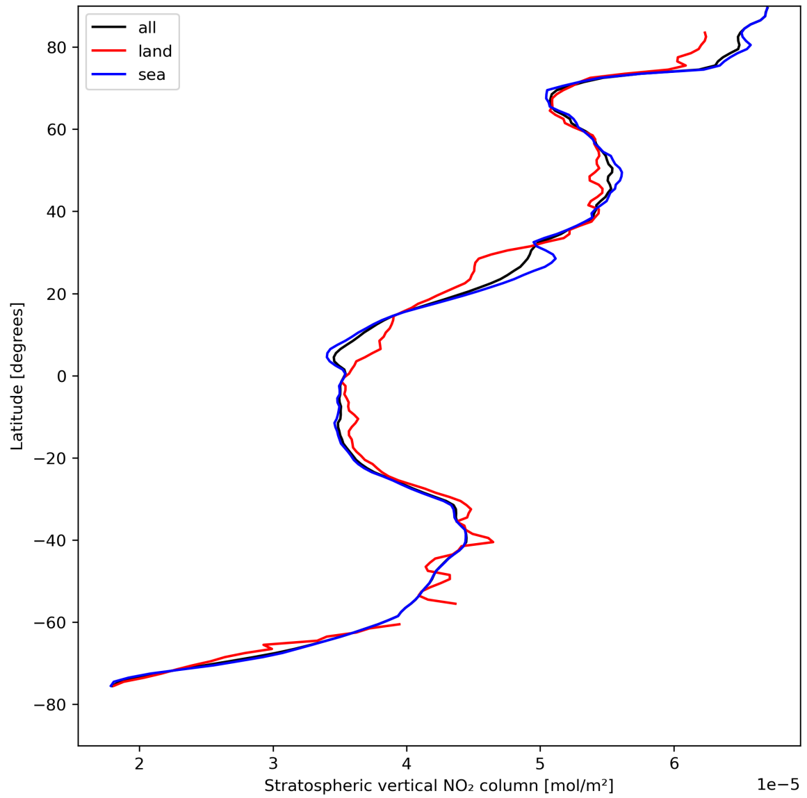
Figure 19: Zonal average of “Stratospheric vertical NO 2 column” for 2024-04-22 to 2024-04-24.
