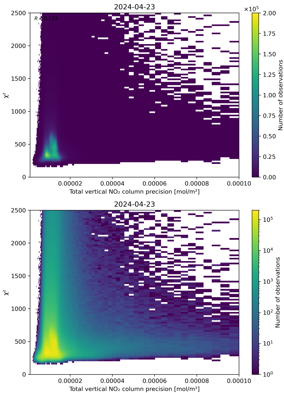
Figure 116: Scatter density plot of “Total vertical NO 2 column precision” against “ \chi^2 ” for 2024-04-22 to 2024-04-24.
