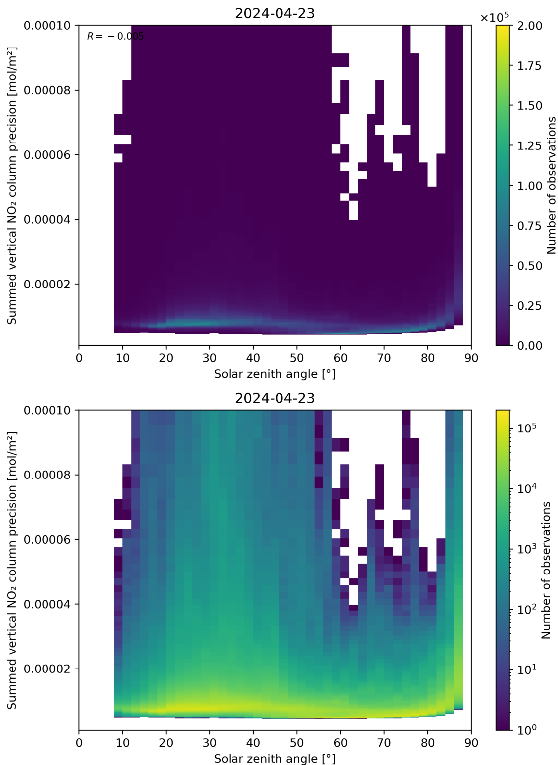
Figure 152: Scatter density plot of “Solar zenith angle” against “Summed vertical NO 2 column precision” for 2024-04-22 to 2024-04-24.
