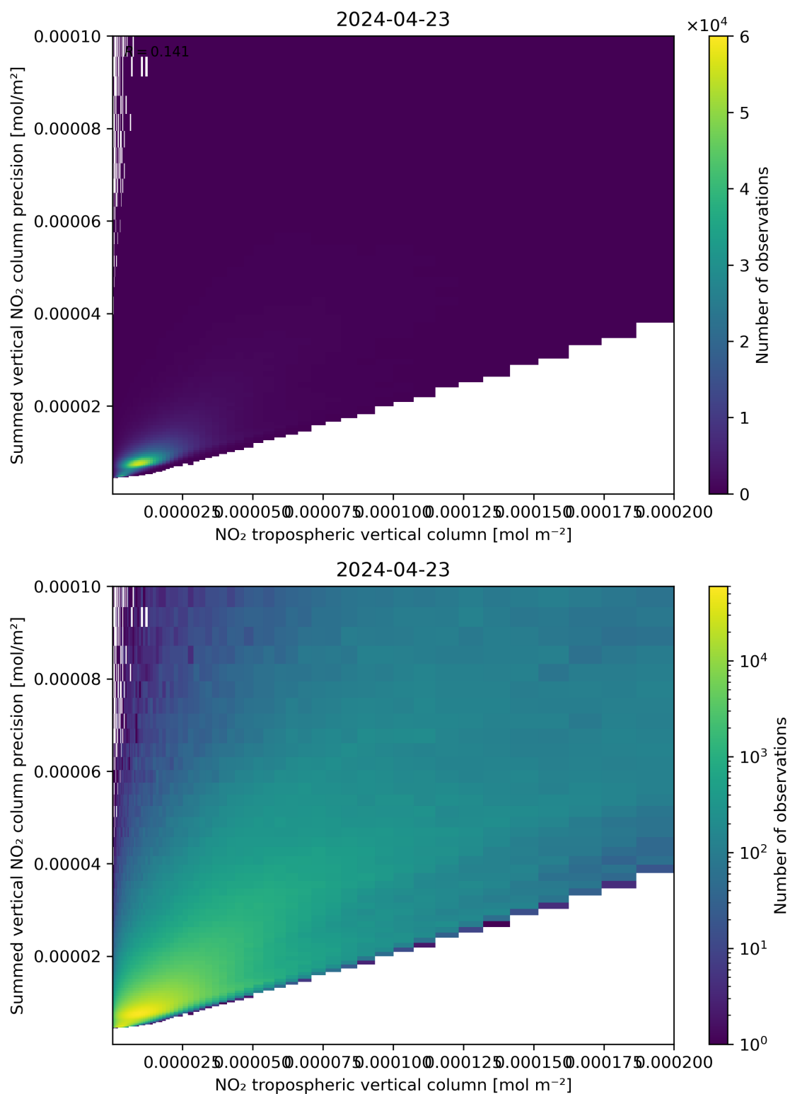
Figure 127: Scatter density plot of “NO 2 tropospheric vertical column” against “Summed vertical NO 2 column precision” for 2024-04-22 to 2024-04-24.
