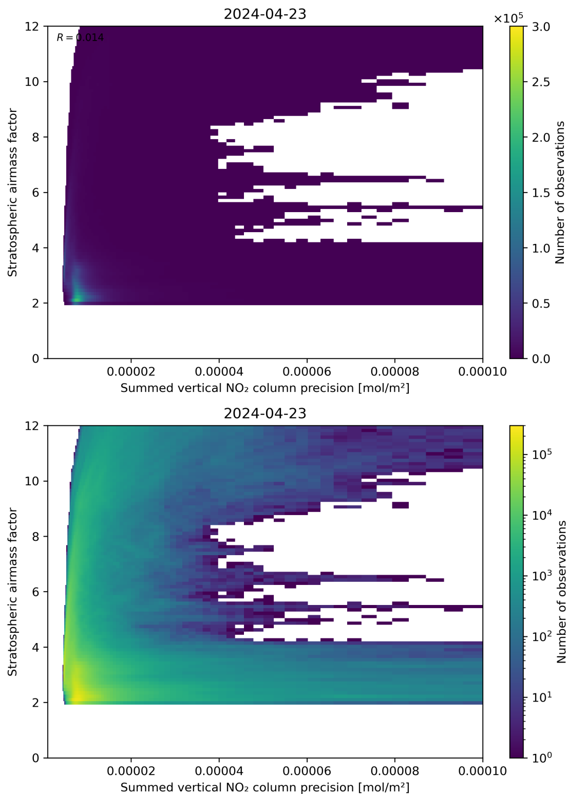
Figure 106: Scatter density plot of “Summed vertical NO 2 column precision” against “Stratospheric airmass factor” for 2024-04-22 to 2024-04-24.
