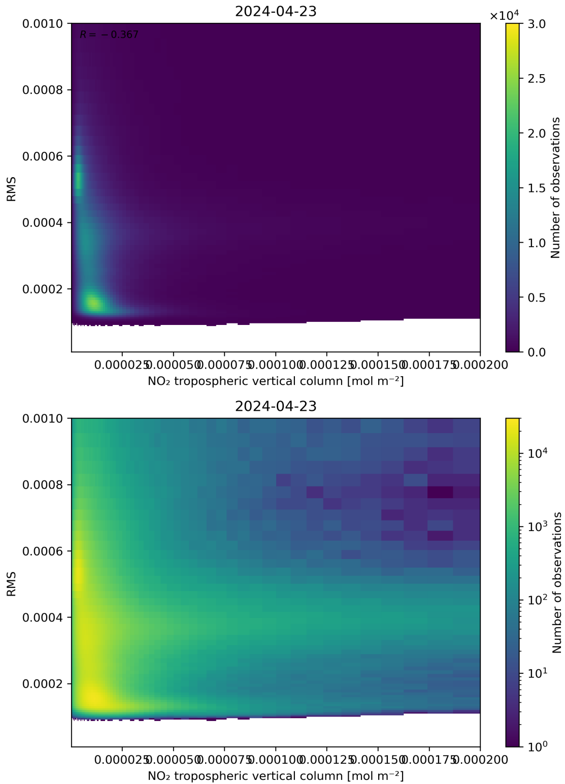
Figure 142: Scatter density plot of “NO 2 tropospheric vertical column” against “RMS” for 2024-04-22 to 2024-04-24.
