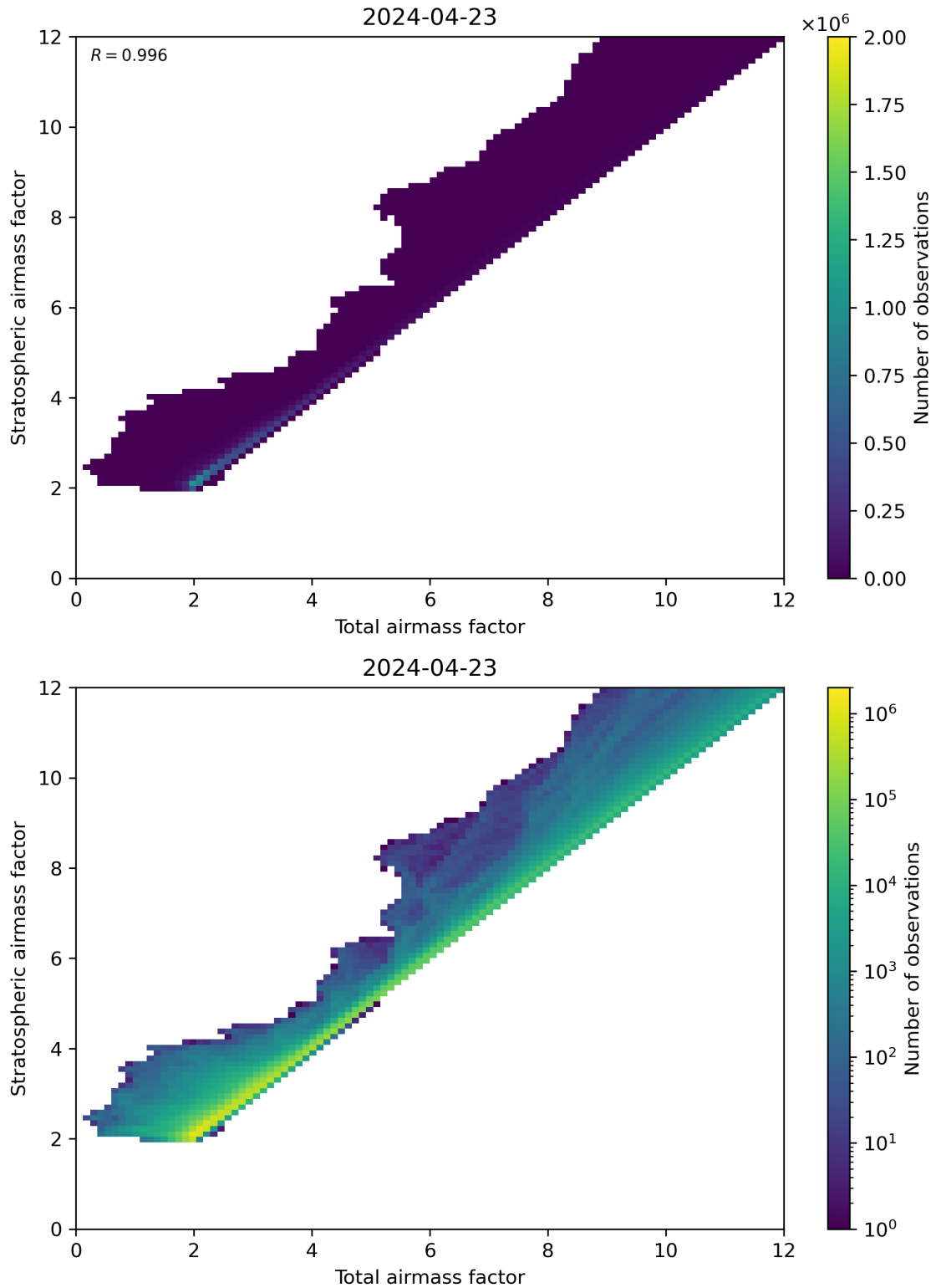
Figure 62: Scatter density plot of “Total airmass factor” against “Stratospheric airmass factor” for 2024-04-22 to 2024-04-24.
