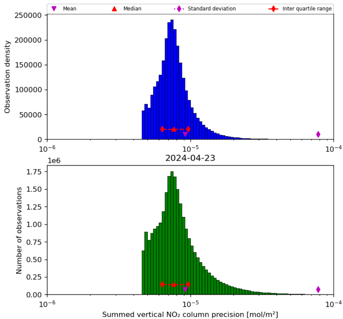
Figure 41: Histogram of “Summed vertical NO 2 column precision” for 2024-04-22 to 2024-04-24
