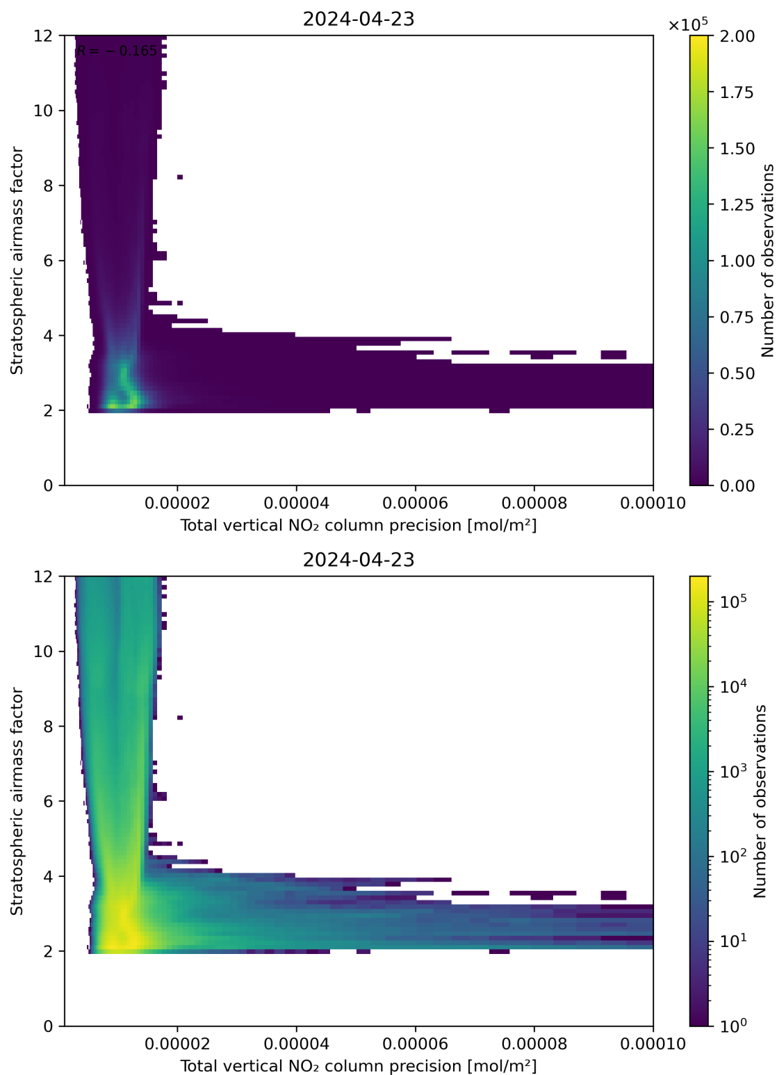
Figure 115: Scatter density plot of “Total vertical NO 2 column precision” against “Stratospheric air mass factor” for 2024-04-22 to 2024-04-24.
