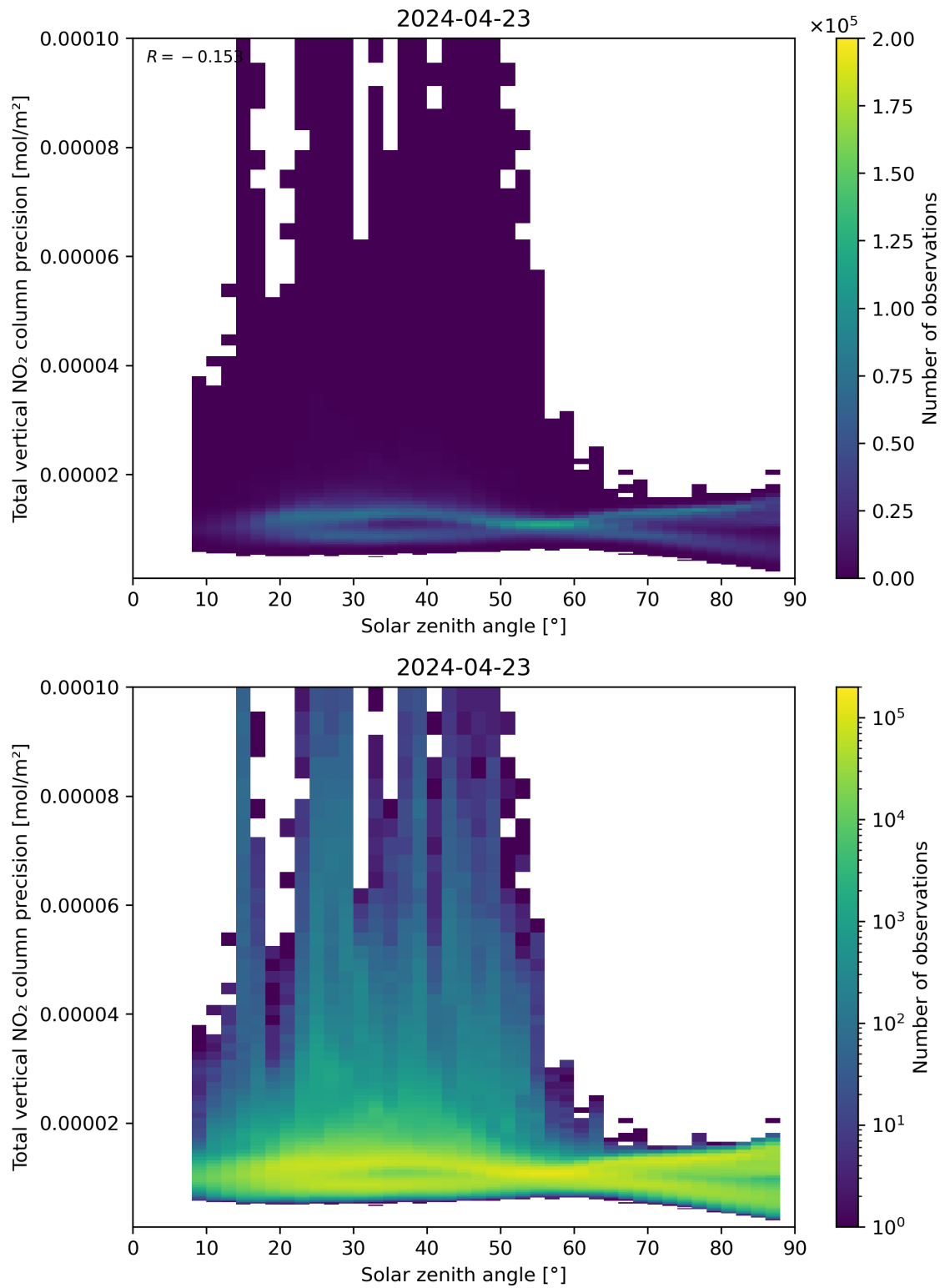
Figure 154: Scatter density plot of “Solar zenith angle” against “Total vertical NO 2 column precision” for 2024-04-22 to 2024-04-24.
