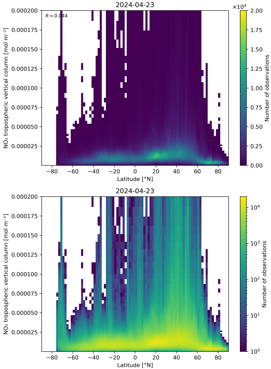
Figure 92: Scatter density plot of “Latitude” against “NO 2 tropospheric vertical column” for 2024-04-22 to 2024-04-24.
