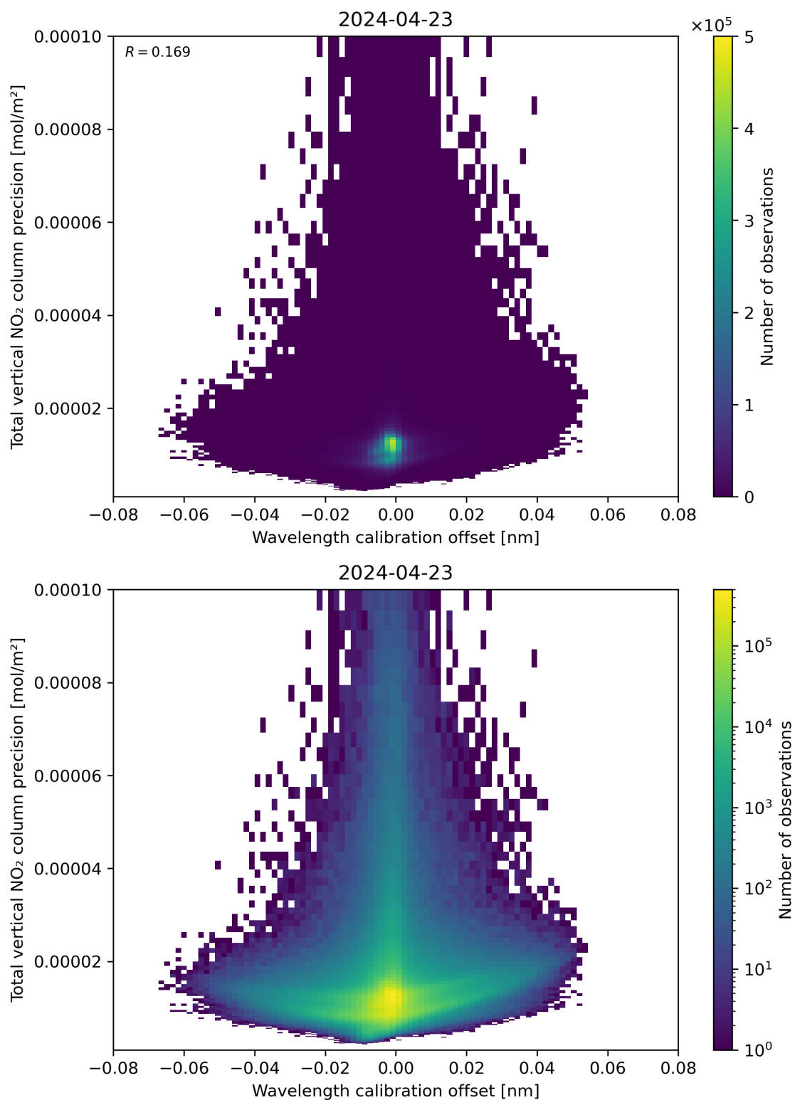
Figure 180: Scatter density plot of “Wavelength calibration offset” against “Total vertical NO 2 column precision” for 2024-04-22 to 2024-04-24.
