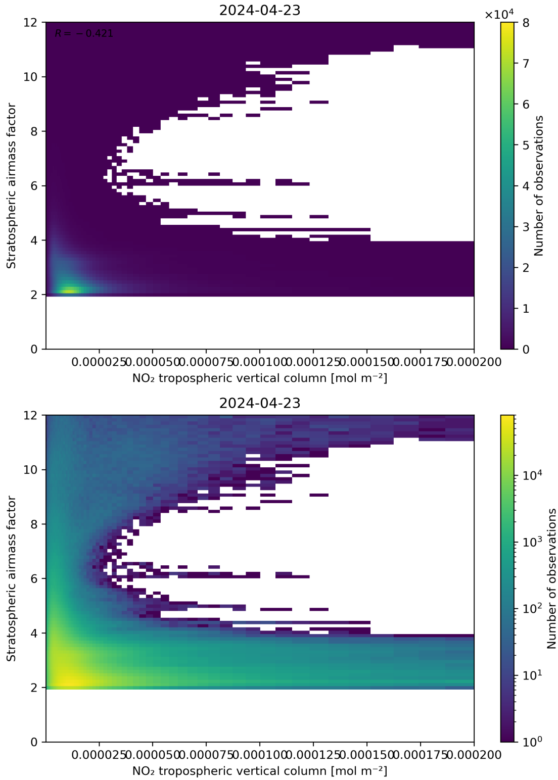
Figure 121: Scatter density plot of “NO 2 tropospheric vertical column” against “Stratospheric air mass factor” for 2024-04-22 to 2024-04-24.
