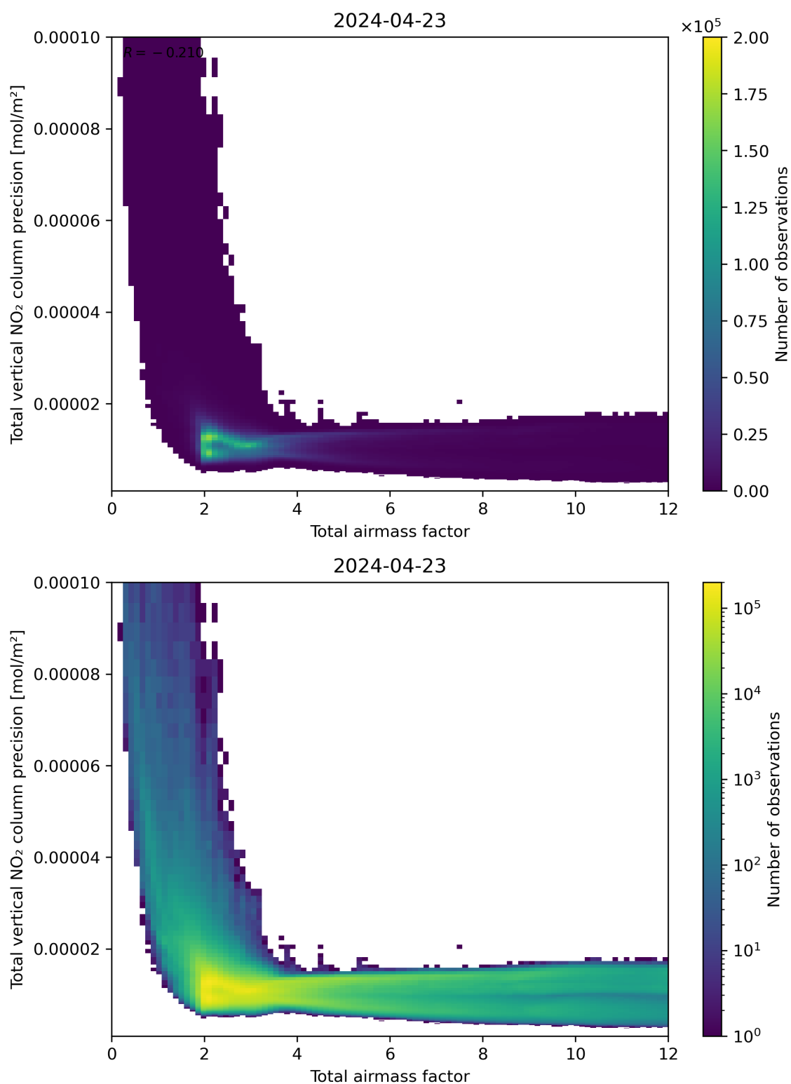
Figure 68: Scatter density plot of “Total airmass factor” against “Total vertical NO 2 column precision” for 2024-04-22 to 2024-04-24.
