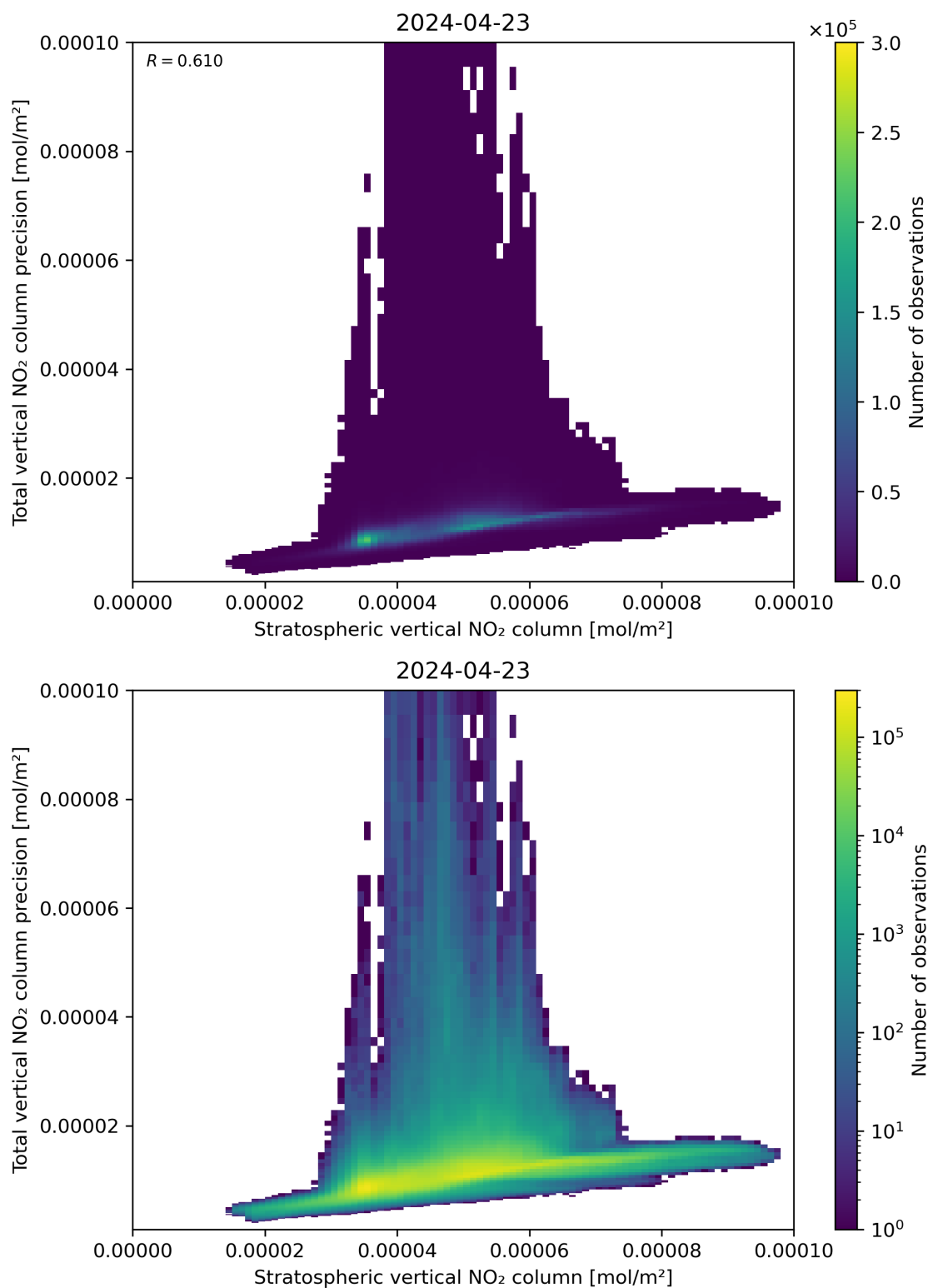
Figure 101: Scatter density plot of “Stratospheric vertical NO 2 column” against “Total vertical NO 2 column precision” for 2024-04-22 to 2024-04-24.
