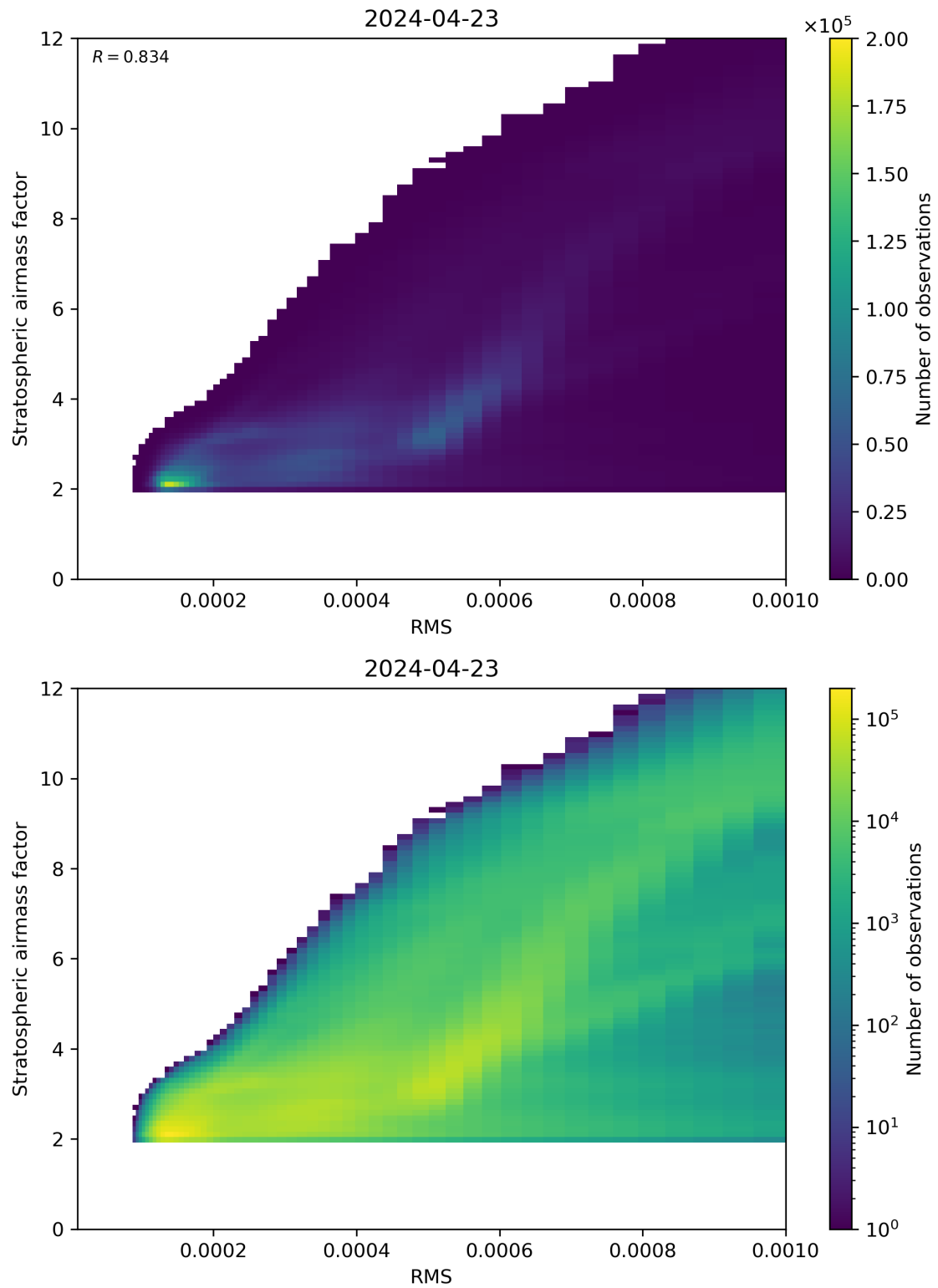
Figure 144: Scatter density plot of “RMS” against “Stratospheric airmass factor” for 2024-04-22 to 2024-04-24.
