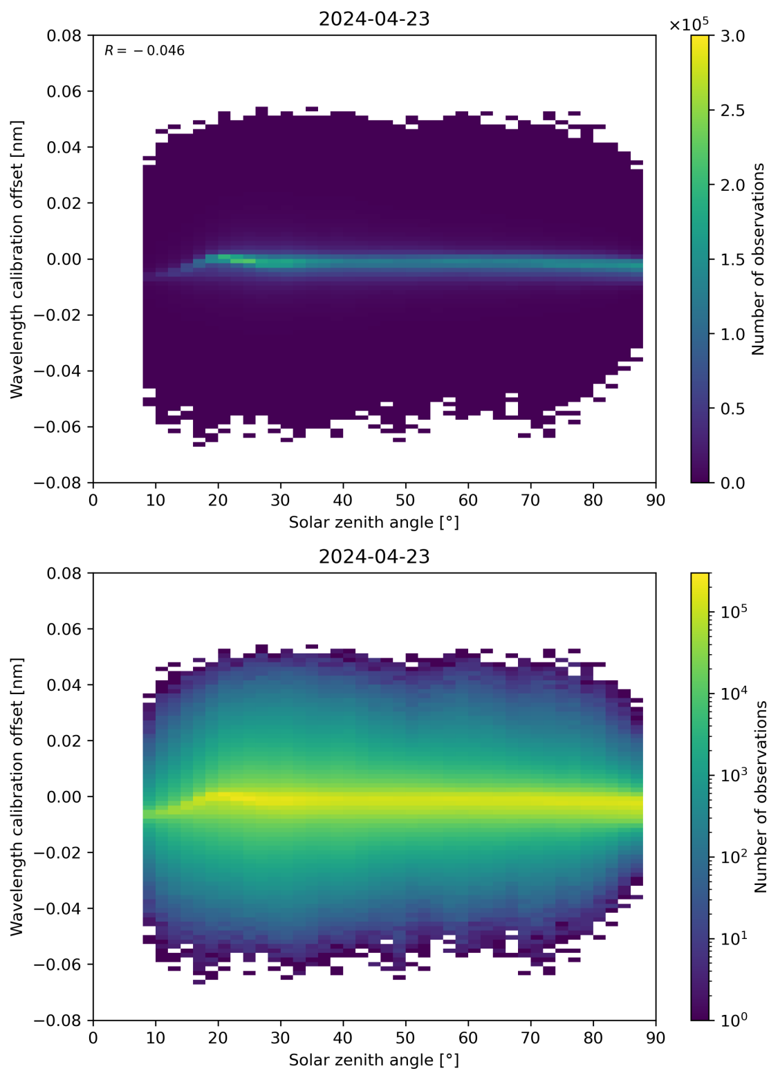
Figure 158: Scatter density plot of “Solar zenith angle” against “Wavelength calibration offset” for 2024-04-22 to 2024-04-24.
