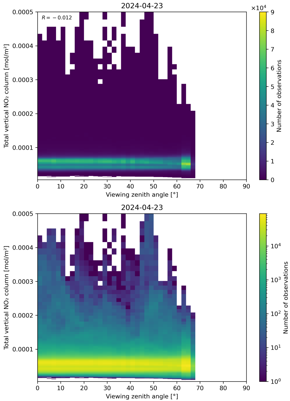
Figure 167: Scatter density plot of “Viewing zenith angle” against “Total vertical NO 2 column” for 2024-04-22 to 2024-04-24.
