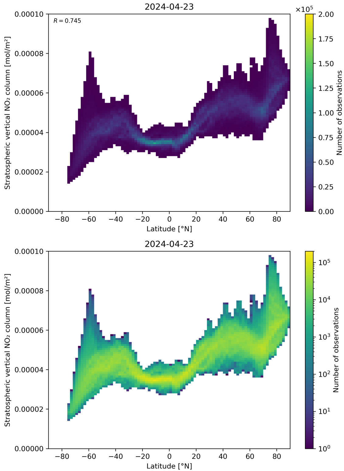
Figure 87: Scatter density plot of “Latitude” against “Stratospheric vertical \text{NO}_2 column” for 2024-04-22 to 2024-04-24.
