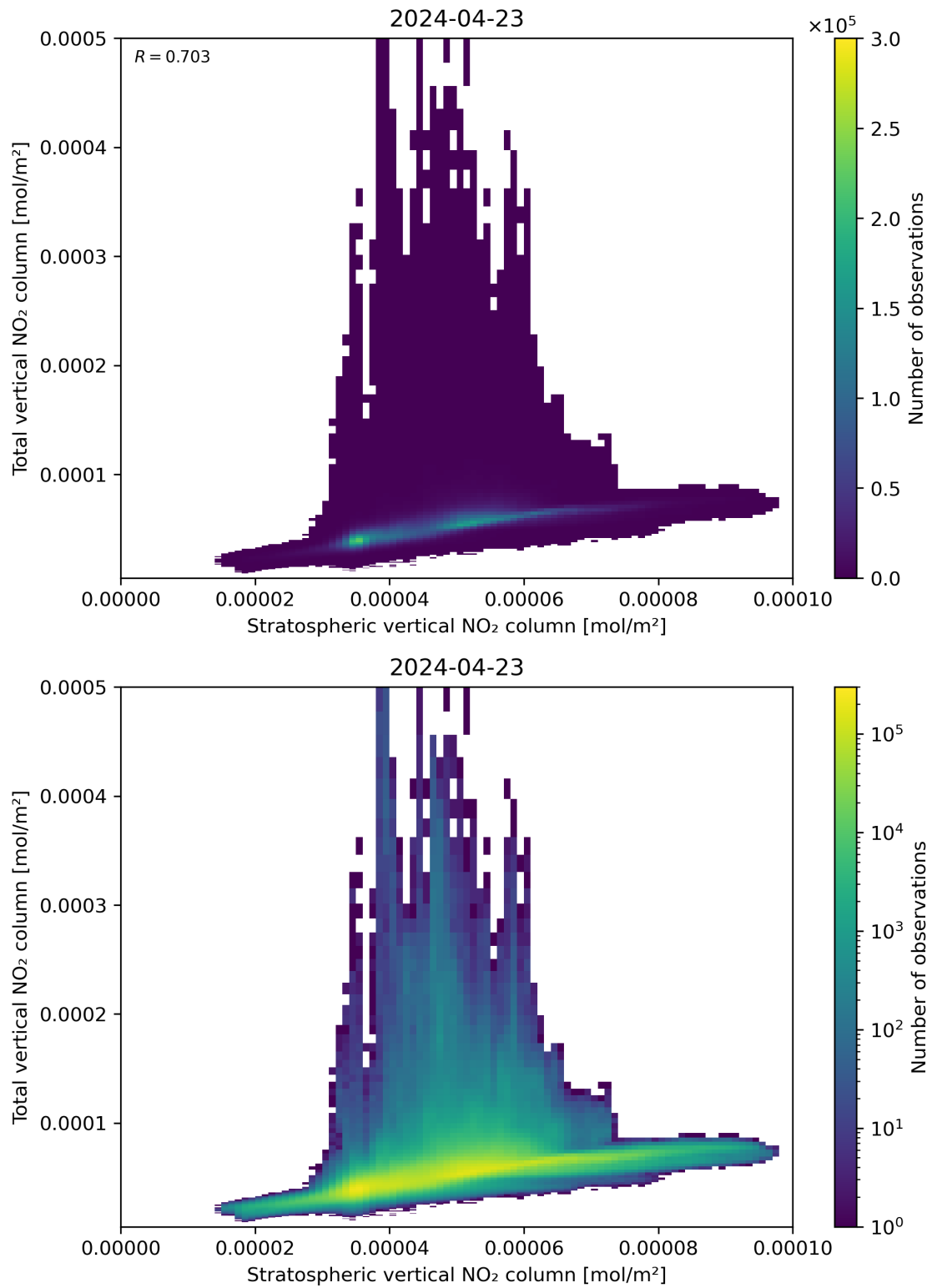
Figure 100: Scatter density plot of “Stratospheric vertical NO 2 column” against “Total vertical NO 2 column” for 2024-04-22 to 2024-04-24.
