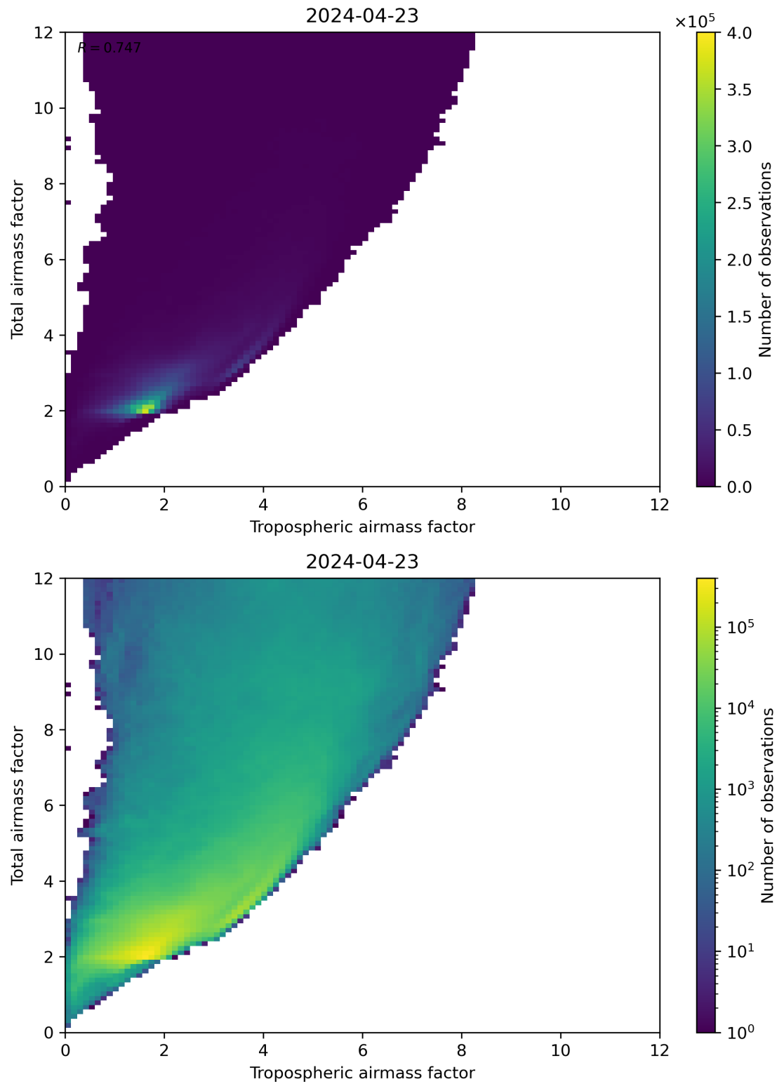
Figure 72: Scatter density plot of “Tropospheric airmass factor” against “Total airmass factor” for 2024-04-22 to 2024-04-24.
