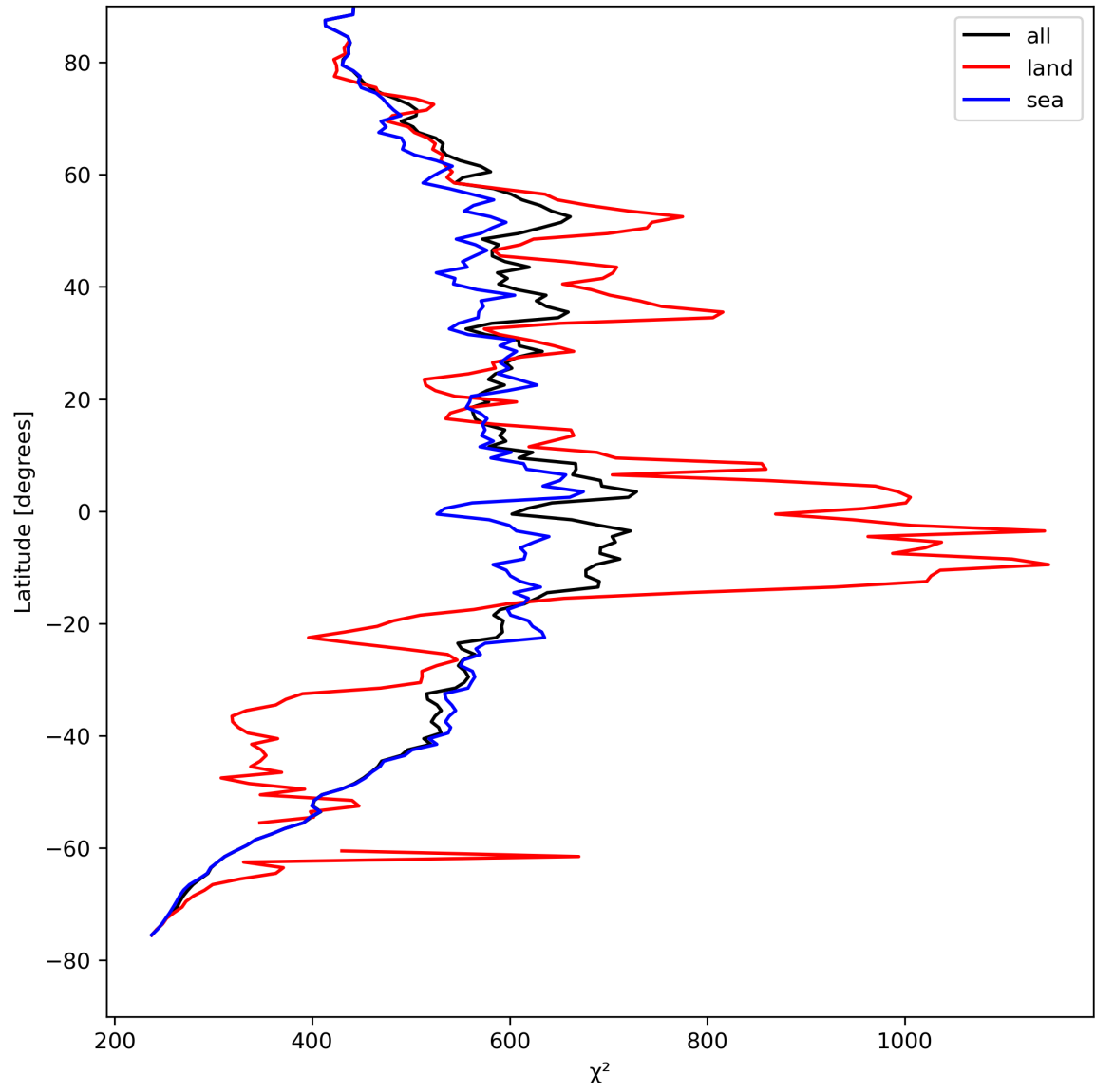
Figure 25: Zonal average of “ \chi^2 ” for 2024-04-22 to 2024-04-24.
