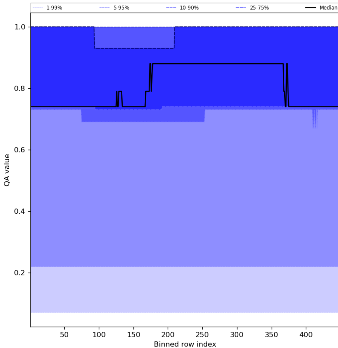
Figure 45: Along track statistics of “QA value” for 2024-04-22 to 2024-04-24
