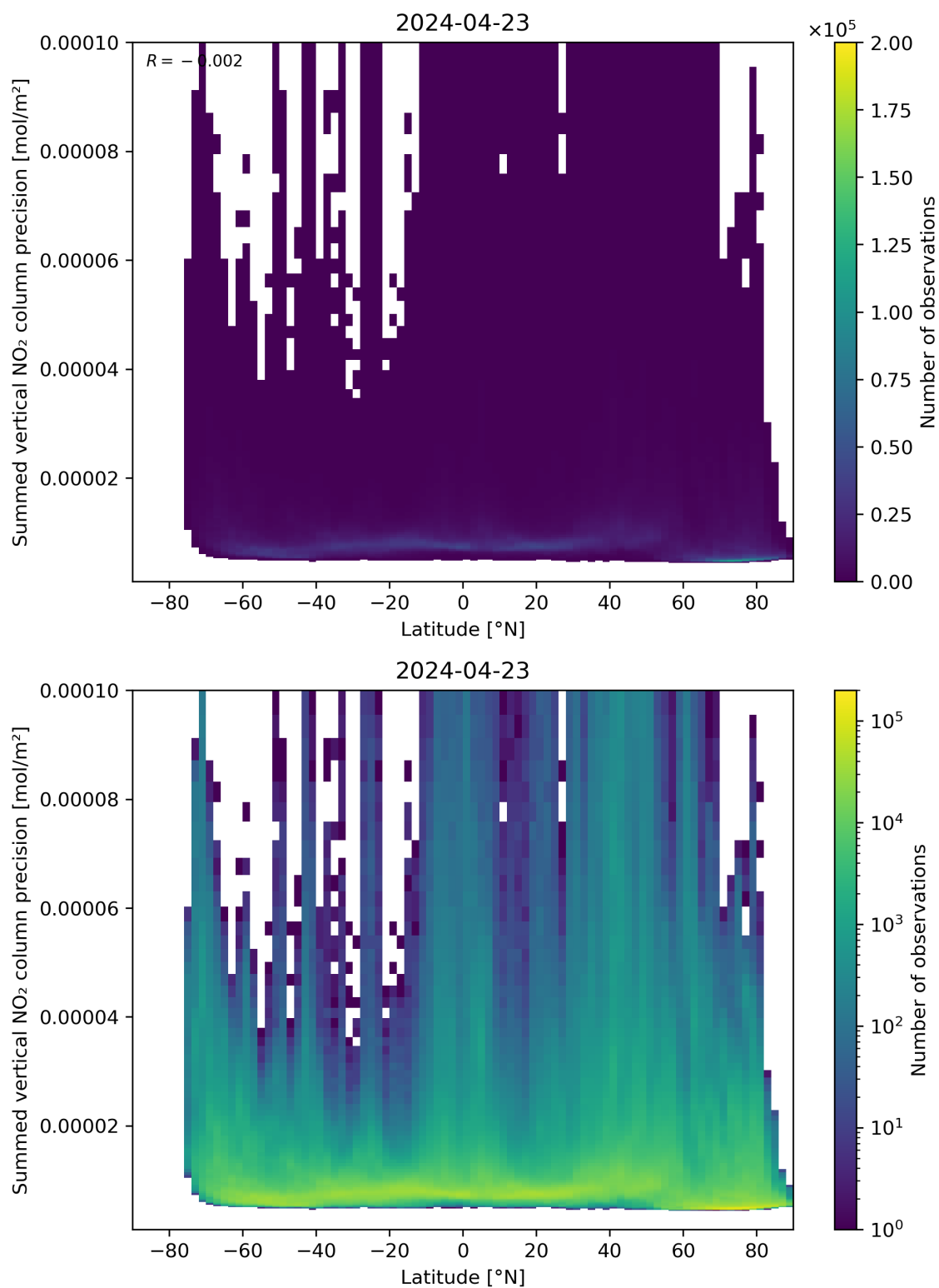
Figure 89: Scatter density plot of “Latitude” against “Summed vertical NO 2 column precision” for 2024-04-22 to 2024-04-24.
