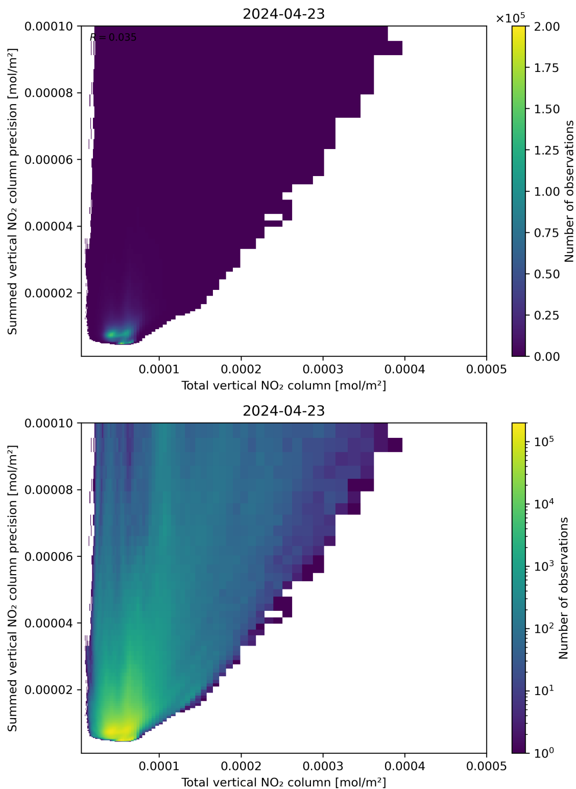
Figure 113: Scatter density plot of “Total vertical NO 2 column” against “Summed vertical NO 2 column precision” for 2024-04-22 to 2024-04-24.
