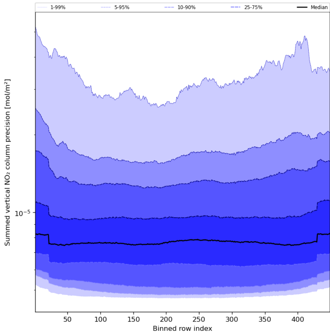
Figure 58: Along track statistics of “Summed vertical NO 2 column precision” for 2024-04-22 to 2024-04-24
