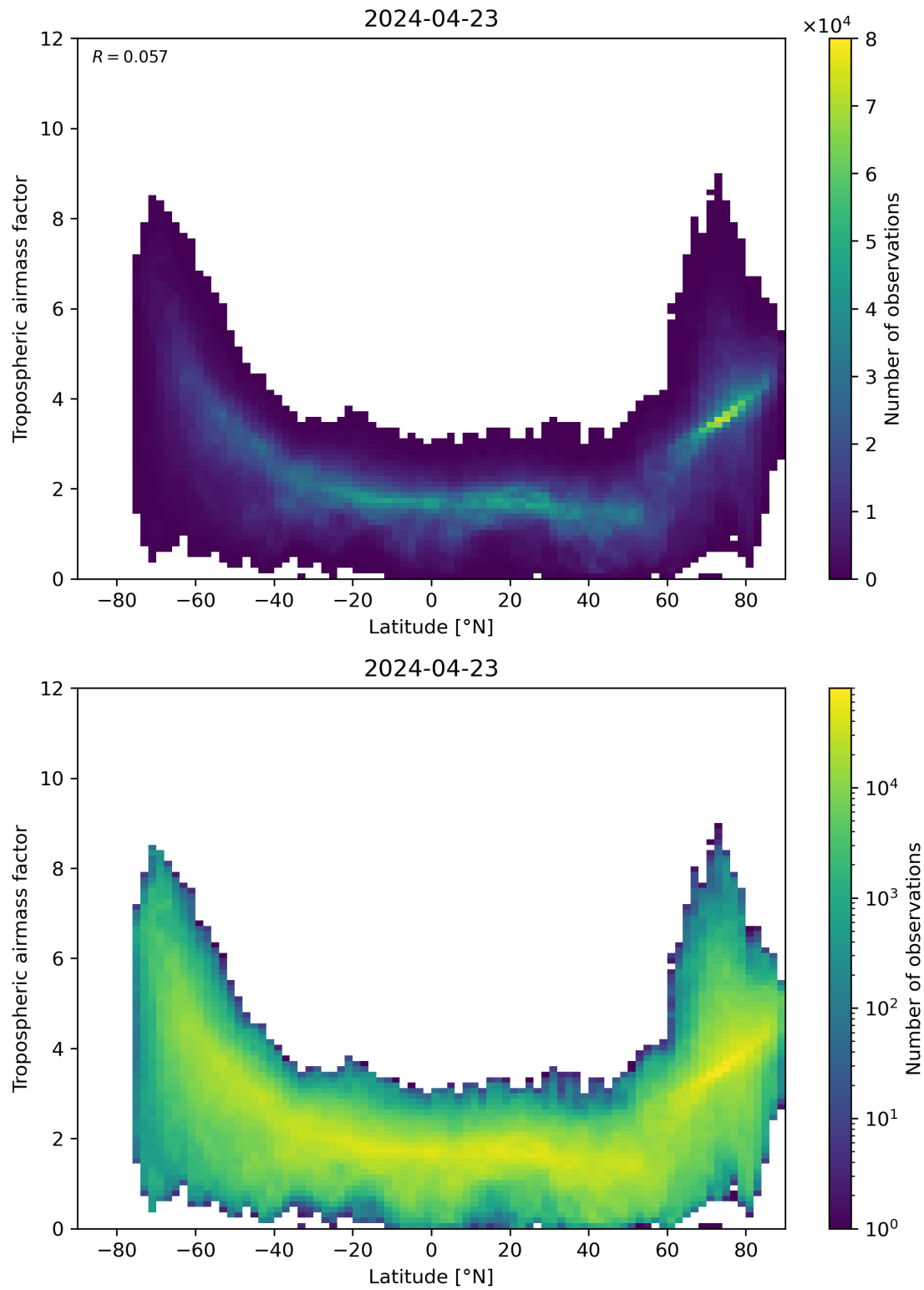
Figure 85: Scatter density plot of “Latitude” against “Tropospheric airmass factor” for 2024-04-22 to 2024-04-24.
