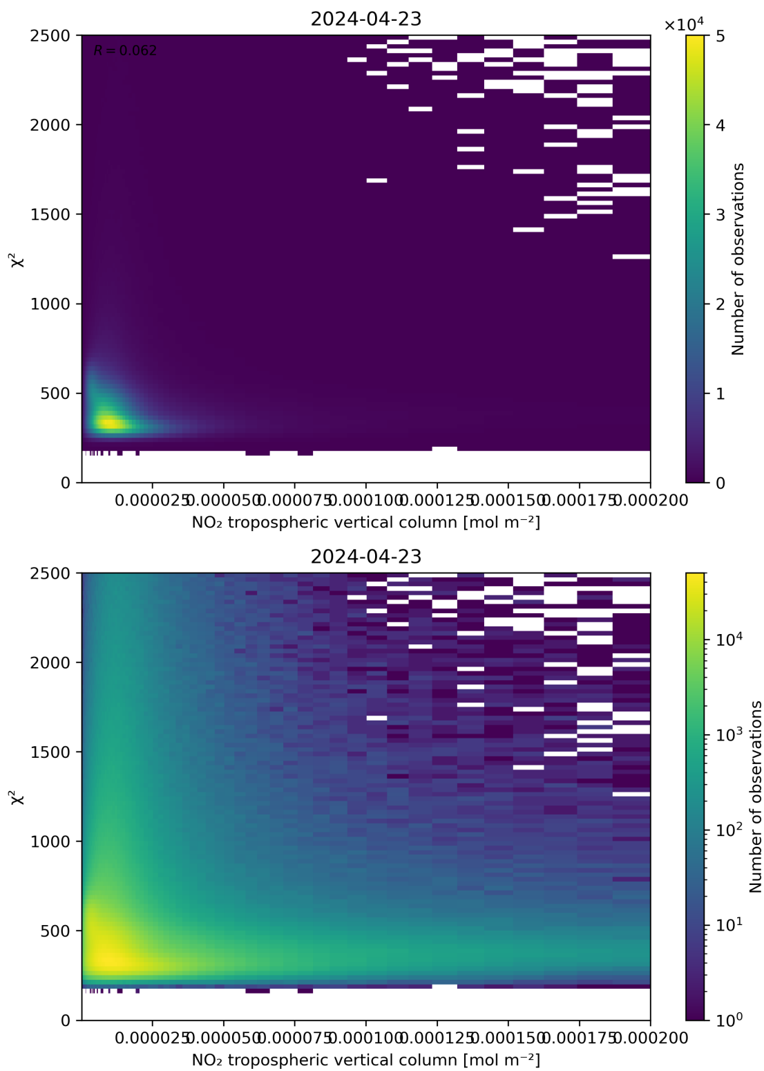
Figure 124: Scatter density plot of “NO 2 tropospheric vertical column” against “ \chi^2 ” for 2024-04-22 to 2024-04-24.
