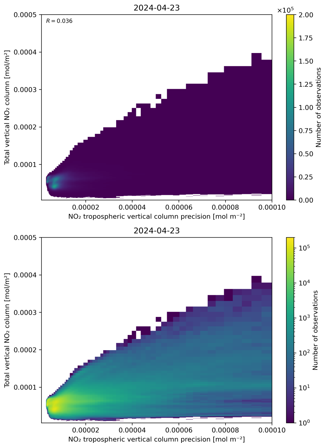
Figure 138: Scatter density plot of “NO 2 tropospheric vertical column precision” against “Total vertical NO 2 column” for 2024-04-22 to 2024-04-24.
