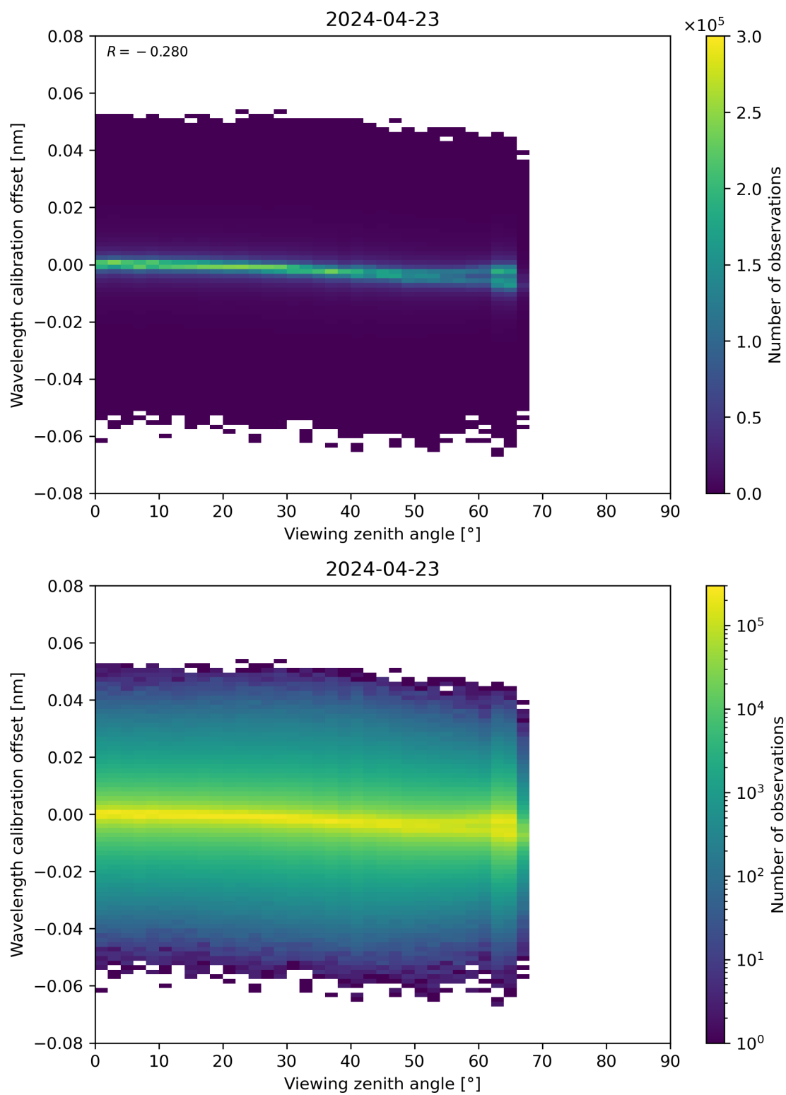
Figure 173: Scatter density plot of “Viewing zenith angle” against “Wavelength calibration offset” for 2024-04-22 to 2024-04-24.
