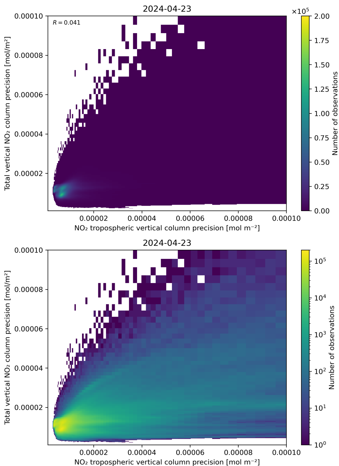
Figure 139: Scatter density plot of “NO 2 tropospheric vertical column precision” against “Total vertical NO 2 column precision” for 2024-04-22 to 2024-04-24.
