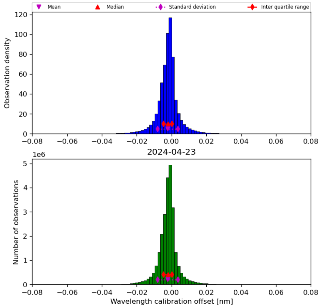
Figure 35: Histogram of “Wavelength calibration offset” for 2024-04-22 to 2024-04-24
