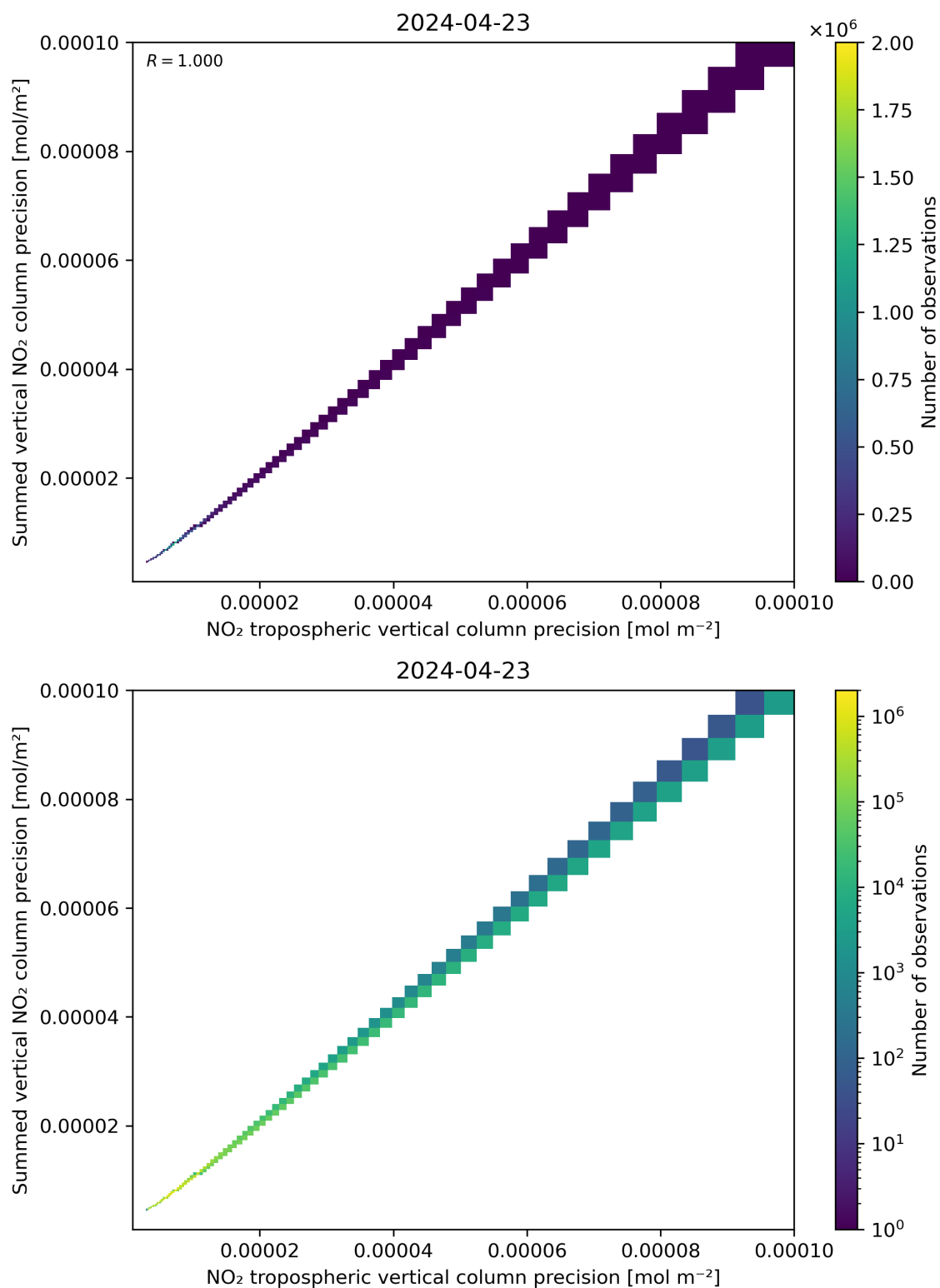
Figure 137: Scatter density plot of “NO 2 tropospheric vertical column precision” against “Summed vertical NO 2 column precision” for 2024-04-22 to 2024-04-24.
