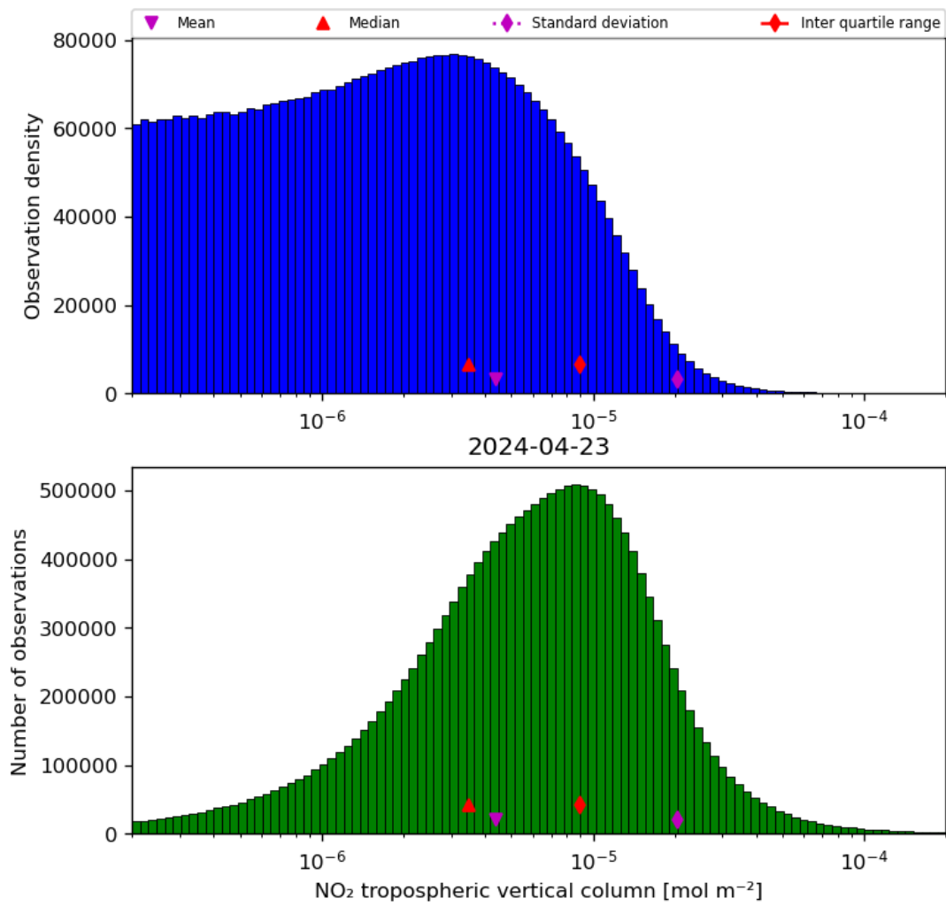
Figure 29: Histogram of “NO 2 tropospheric vertical column” for 2024-04-22 to 2024-04-24
