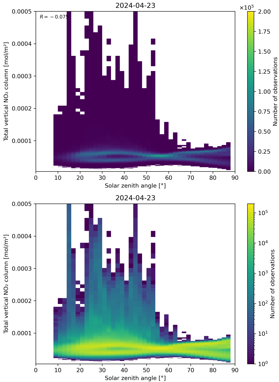
Figure 153: Scatter density plot of “Solar zenith angle” against “Total vertical NO 2 column” for 2024-04-22 to 2024-04-24.
