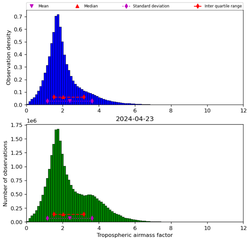
Figure 31: Histogram of “Tropospheric airmass factor” for 2024-04-22 to 2024-04-24
