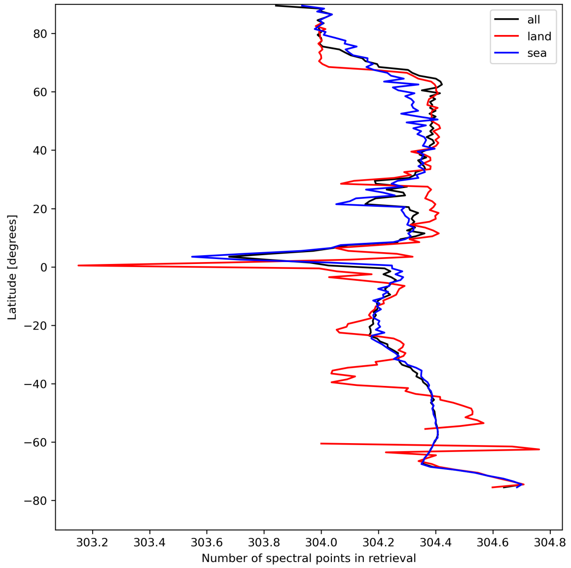
Figure 16: Zonal average of “Number of spectral points in retrieval” for 2024-04-22 to 2024-04-24.
