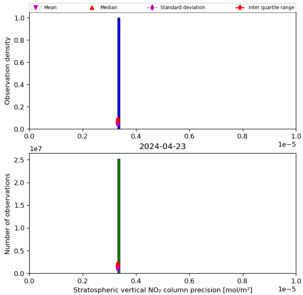
Figure 37: Histogram of “Stratospheric vertical NO 2 column precision” for 2024-04-22 to 2024-04-24
