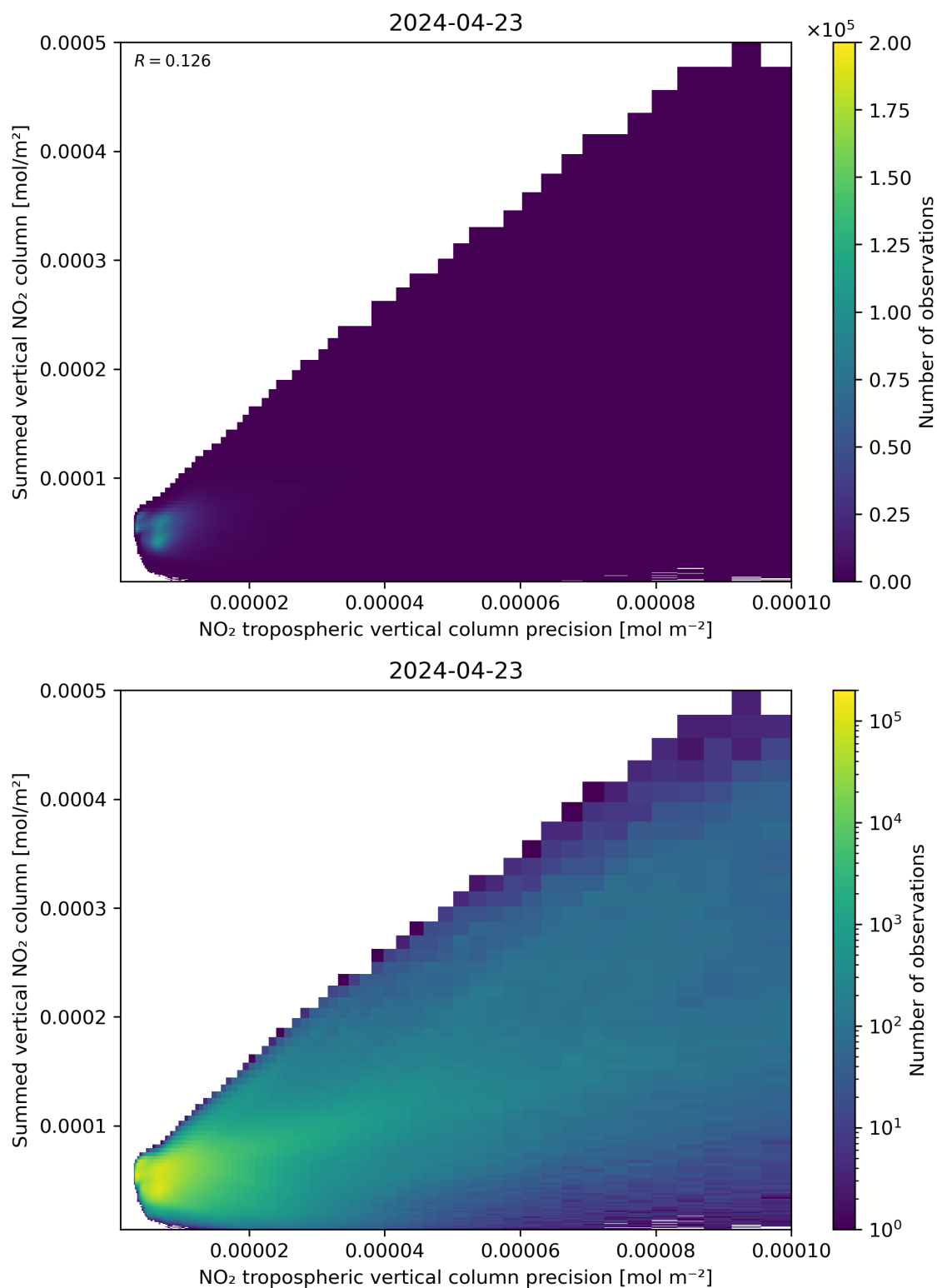
Figure 136: Scatter density plot of “NO 2 tropospheric vertical column precision” against “Summed vertical NO 2 column” for 2024-04-22 to 2024-04-24.
