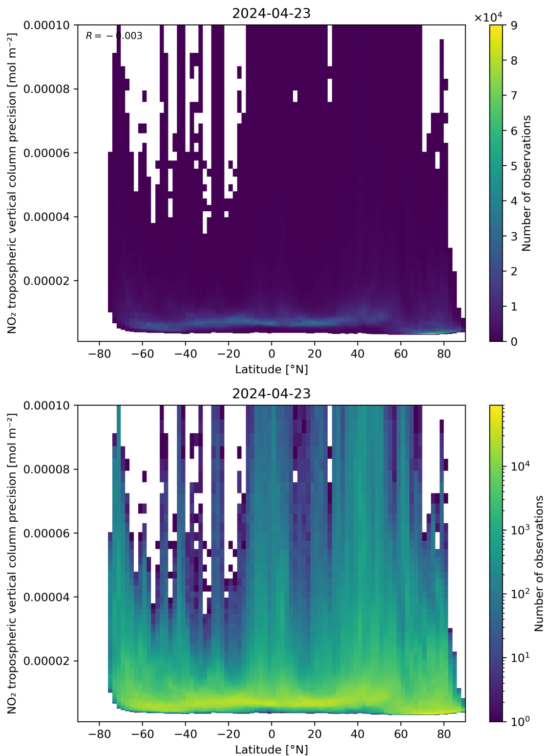
Figure 93: Scatter density plot of “Latitude” against “NO 2 tropospheric vertical column precision” for 2024-04-22 to 2024-04-24.
