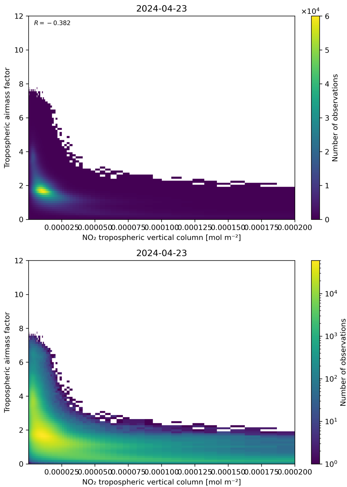
Figure 123: Scatter density plot of “NO 2 tropospheric vertical column” against “Tropospheric airmass factor” for 2024-04-22 to 2024-04-24.
