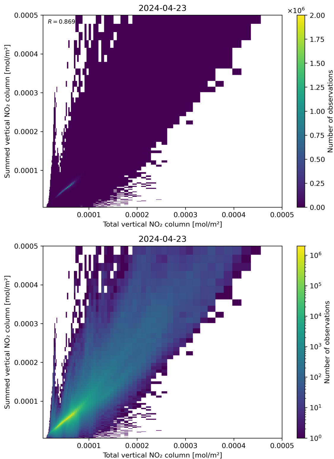
Figure 112: Scatter density plot of “Total vertical NO 2 column” against “Summed vertical NO 2 column” for 2024-04-22 to 2024-04-24.
