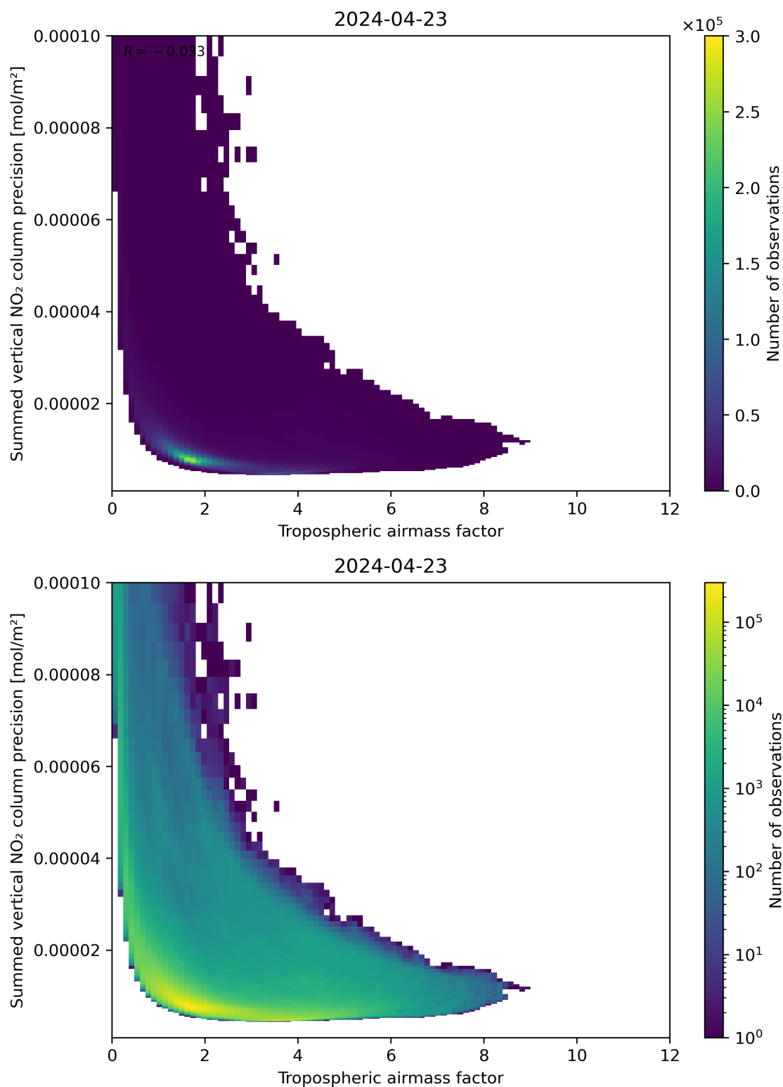
Figure 76: Scatter density plot of “Tropospheric air mass factor” against “Summed vertical NO 2 column precision” for 2024-04-22 to 2024-04-24.
