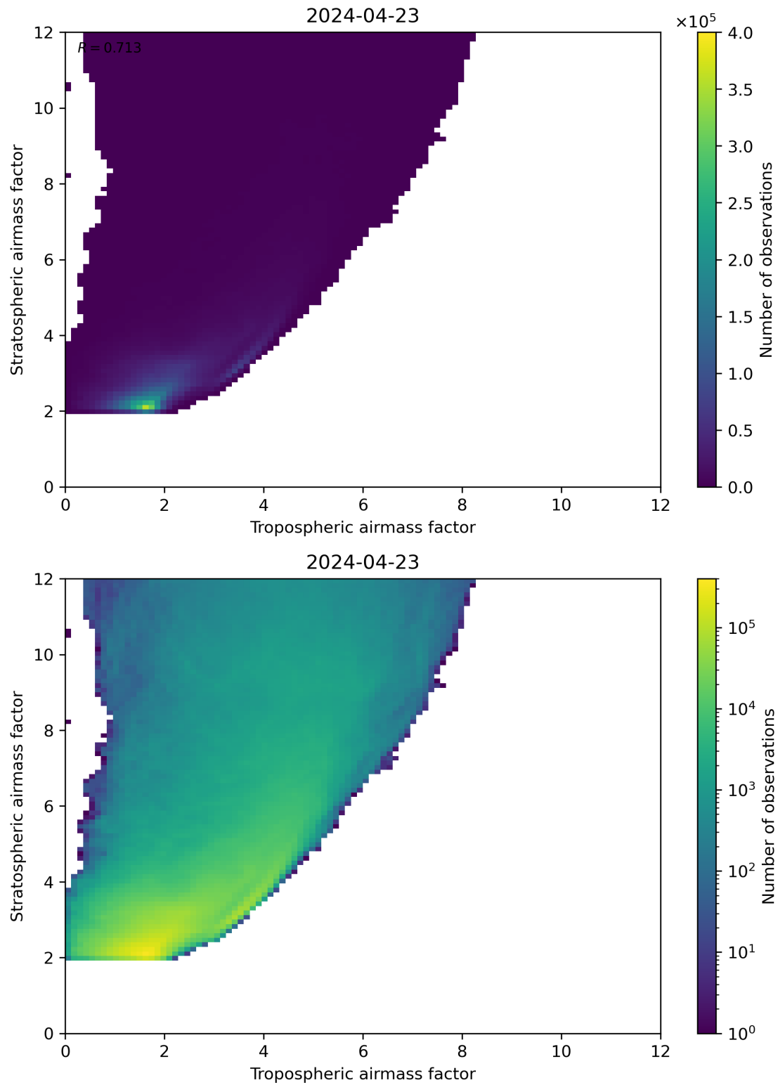
Figure 71: Scatter density plot of “Tropospheric airmass factor” against “Stratospheric airmass factor” for 2024-04-22 to 2024-04-24.
