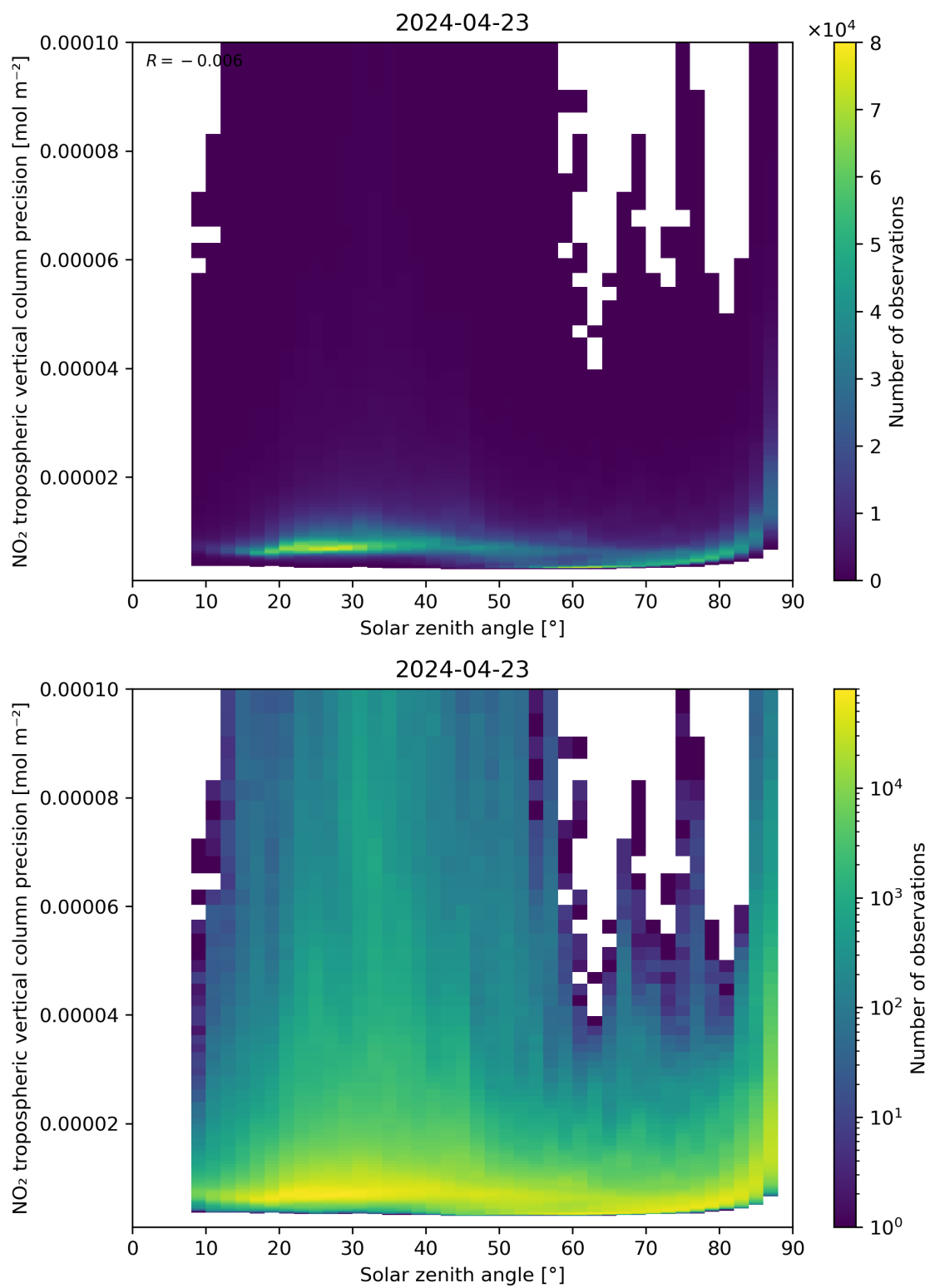
Figure 156: Scatter density plot of “Solar zenith angle” against “NO 2 tropospheric vertical column precision” for 2024-04-22 to 2024-04-24.
