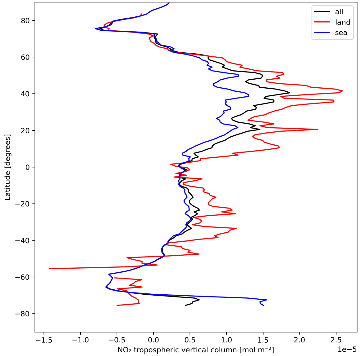
Figure 12: Zonal average of “NO 2 tropospheric vertical column” for 2024-04-22 to 2024-04-24.
