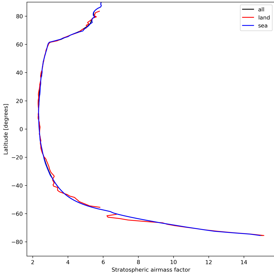
Figure 27: Zonal average of “Stratospheric air mass factor” for 2024-04-22 to 2024-04-24.
