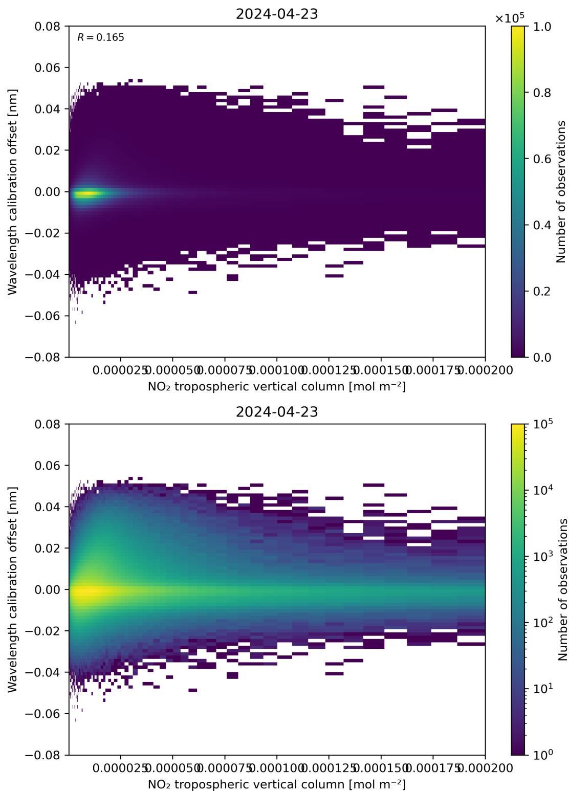
Figure 143: Scatter density plot of “NO 2 tropospheric vertical column” against “Wavelength calibration offset” for 2024-04-22 to 2024-04-24.
