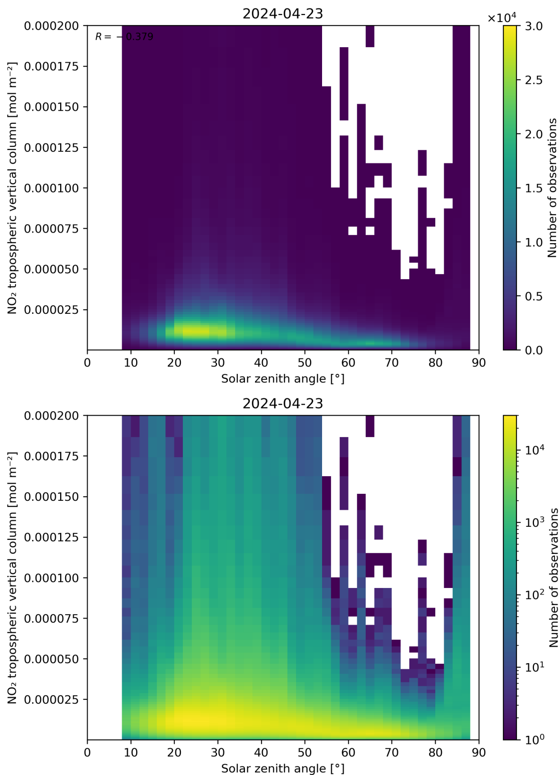
Figure 155: Scatter density plot of “Solar zenith angle” against “NO 2 tropospheric vertical column” for 2024-04-22 to 2024-04-24.
