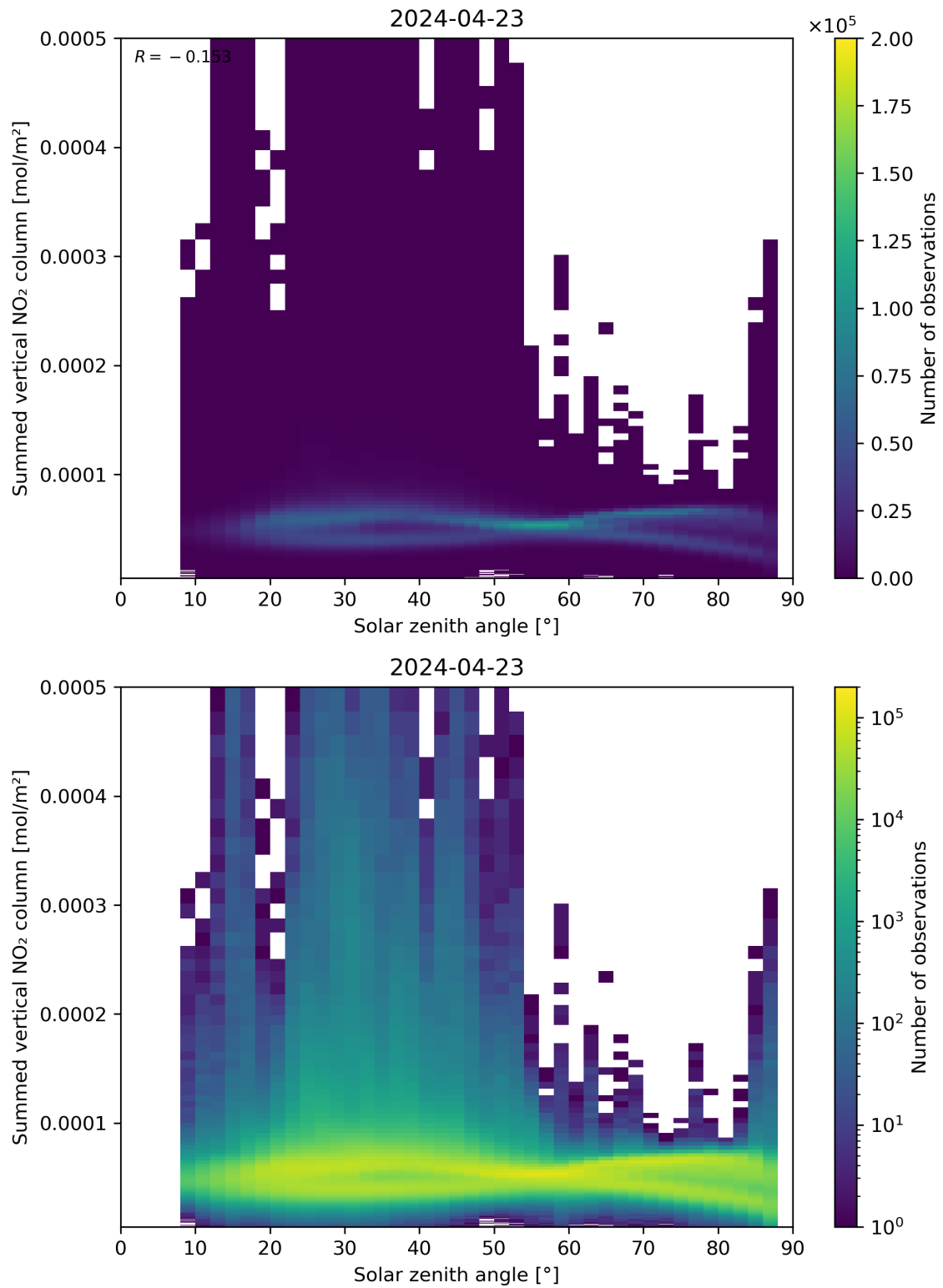
Figure 151: Scatter density plot of “Solar zenith angle” against “Summed vertical NO 2 column” for 2024-04-22 to 2024-04-24.
