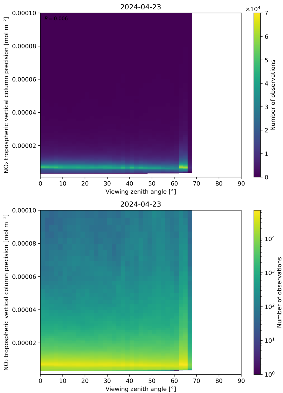
Figure 170: Scatter density plot of “Viewing zenith angle” against “NO 2 tropospheric vertical column precision” for 2024-04-22 to 2024-04-24.
