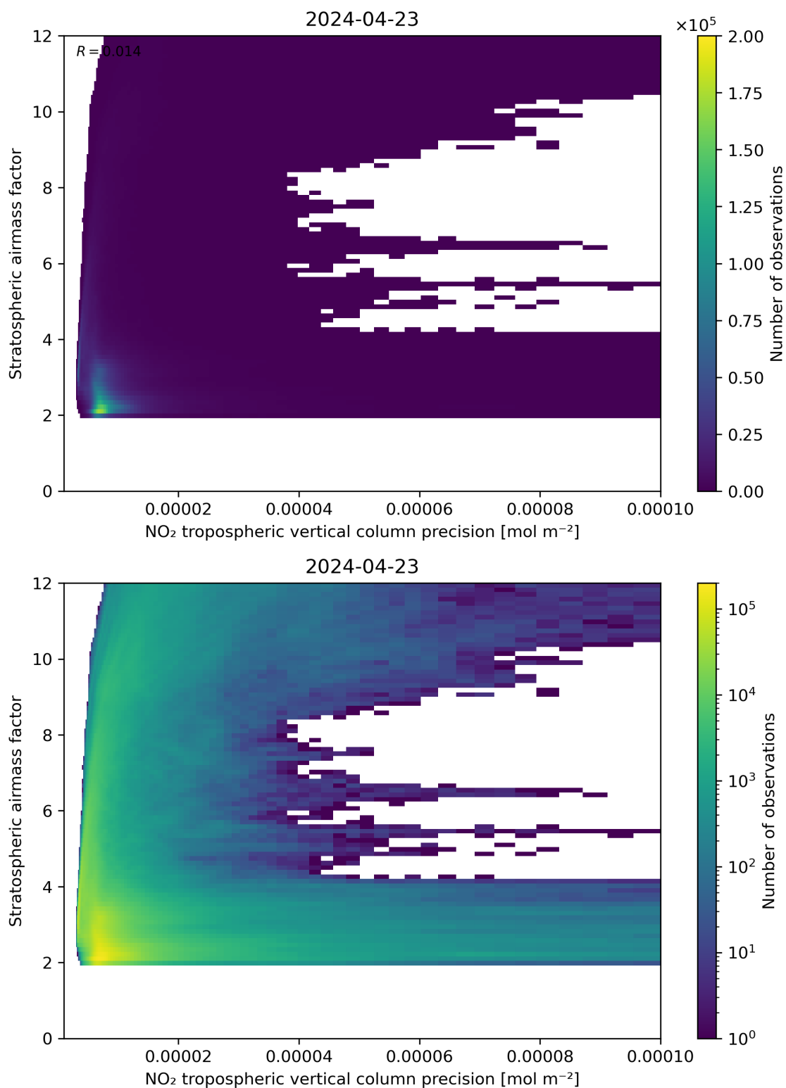
Figure 131: Scatter density plot of “NO 2 tropospheric vertical column precision” against “Stratospheric airmass factor” for 2024-04-22 to 2024-04-24.
