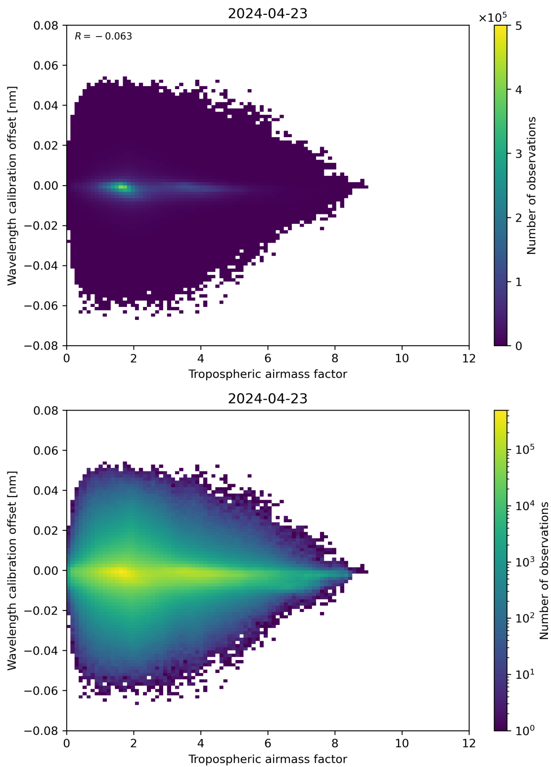
Figure 80: Scatter density plot of “Tropospheric airmass factor” against “Wavelength calibration offset” for 2024-04-22 to 2024-04-24.
