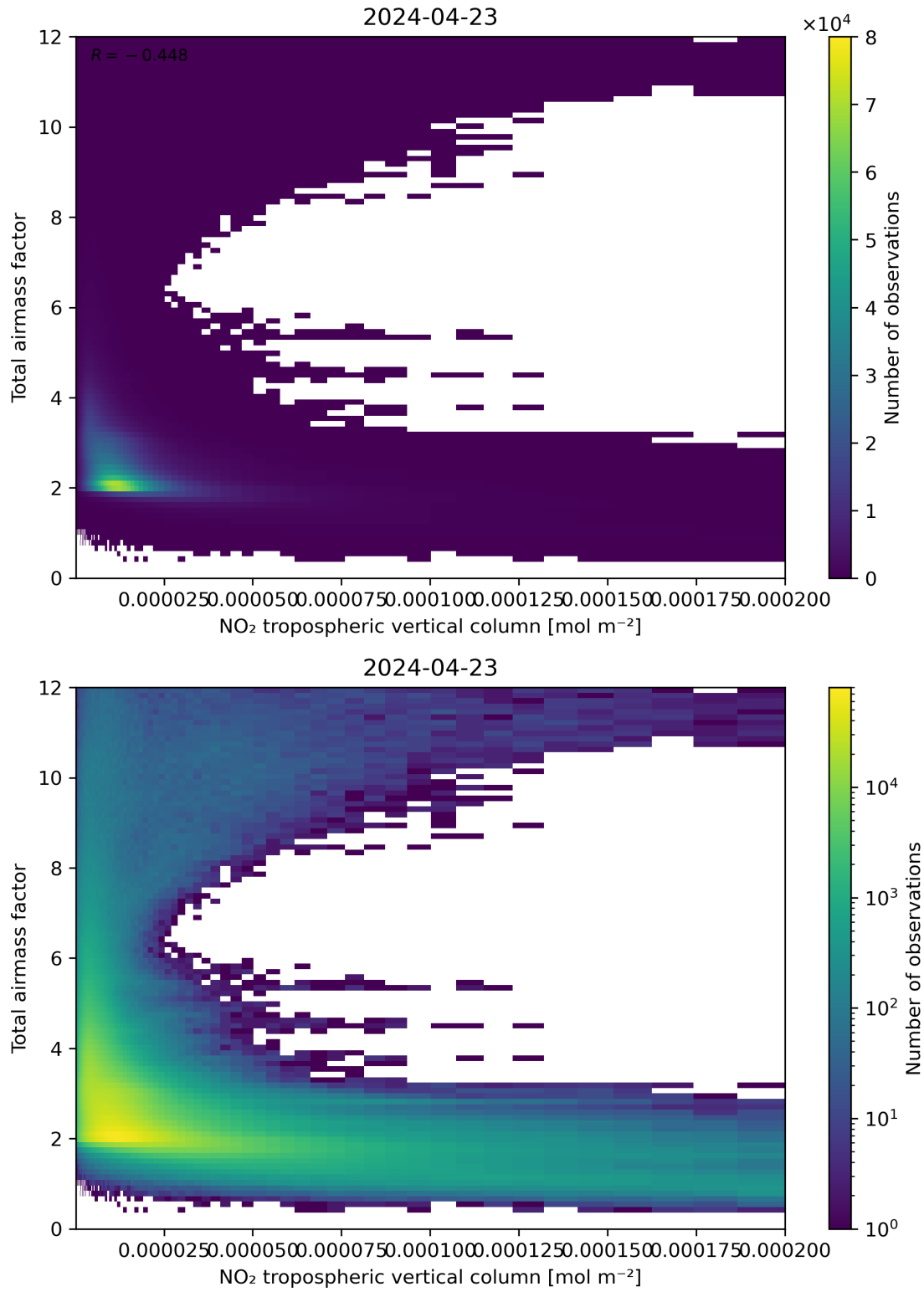
Figure 122: Scatter density plot of “NO 2 tropospheric vertical column” against “Total air mass factor” for 2024-04-22 to 2024-04-24.
