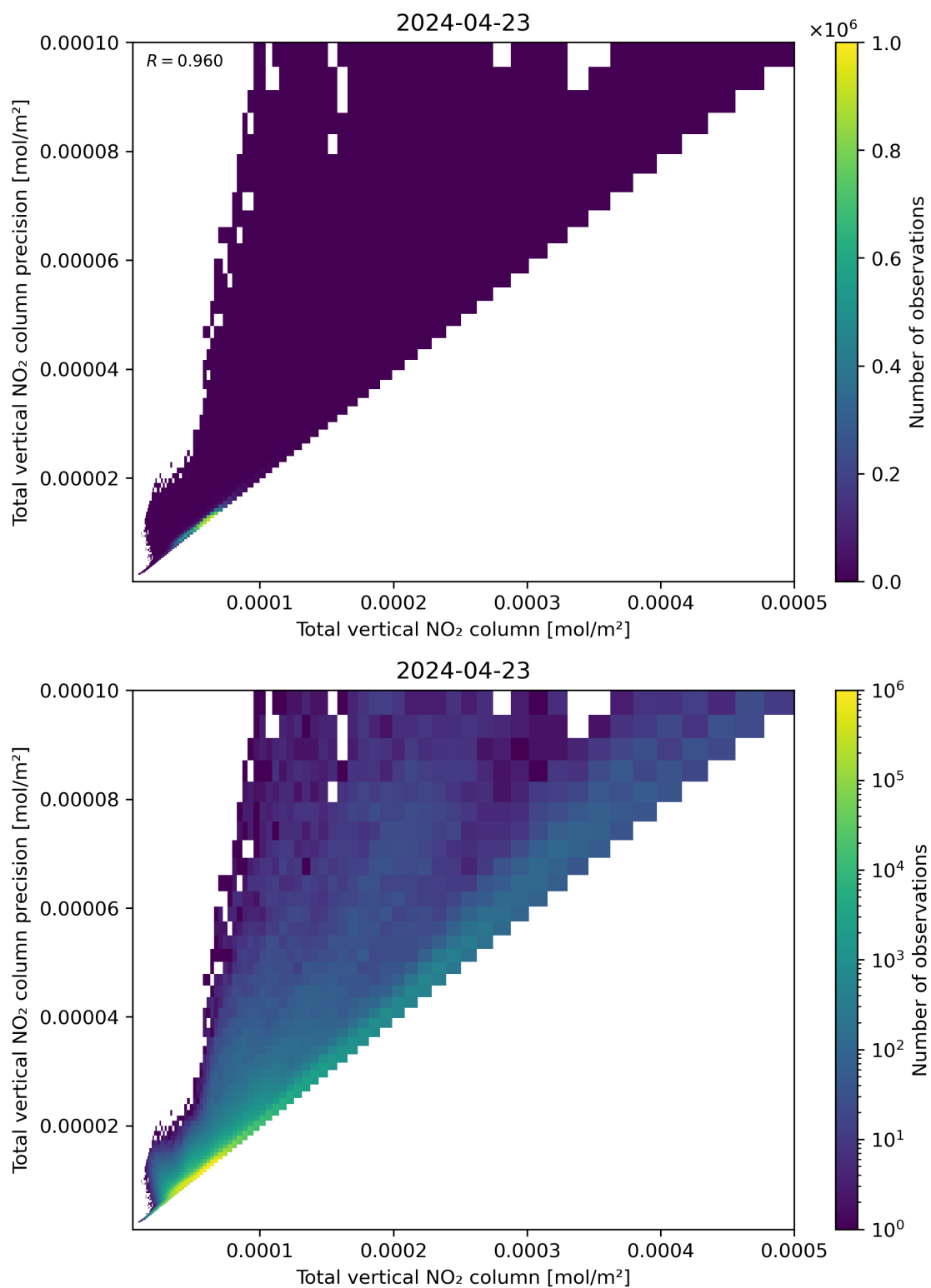
Figure 114: Scatter density plot of “Total vertical NO 2 column” against “Total vertical NO 2 column precision” for 2024-04-22 to 2024-04-24.
