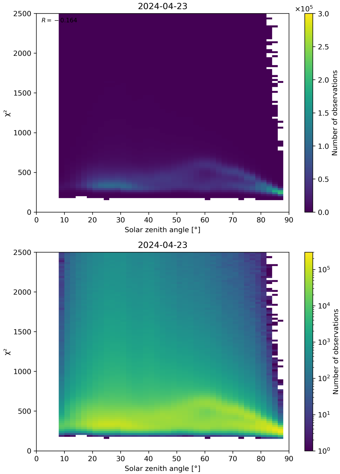
Figure 148: Scatter density plot of “Solar zenith angle” against “ \chi^2 ” for 2024-04-22 to 2024-04-24.
