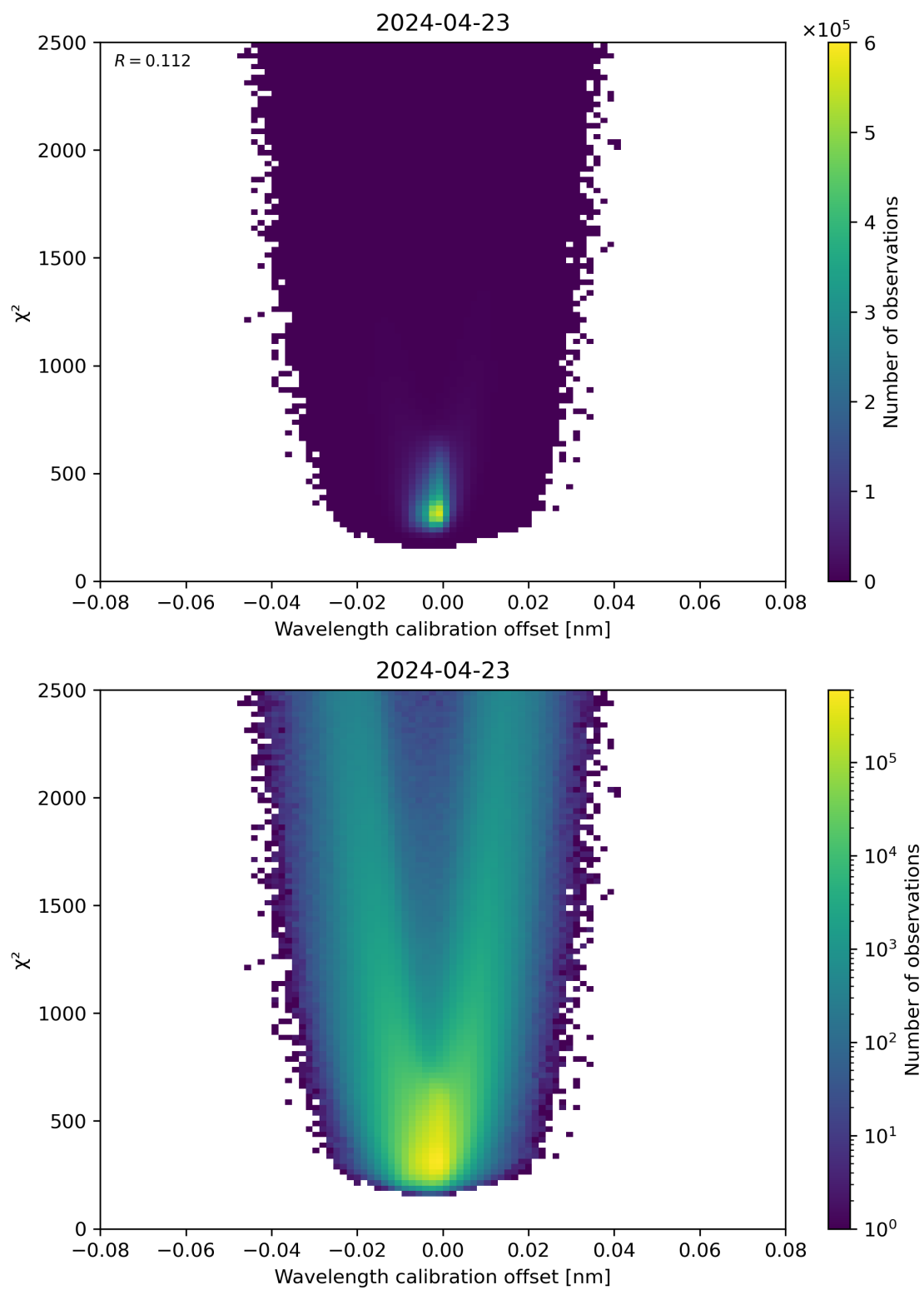
Figure 175: Scatter density plot of “Wavelength calibration offset” against “ \chi^2 ” for 2024-04-22 to 2024-04-24.
