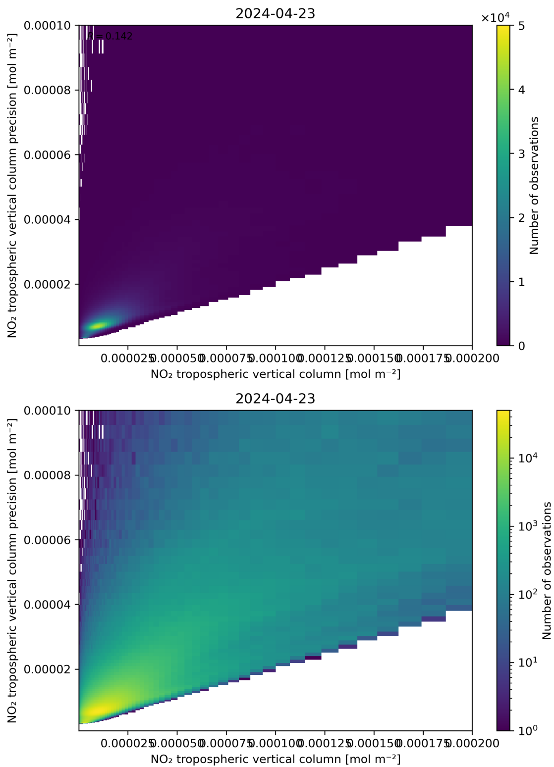
Figure 130: Scatter density plot of “NO 2 tropospheric vertical column” against “NO 2 tropospheric vertical column precision” for 2024-04-22 to 2024-04-24.
