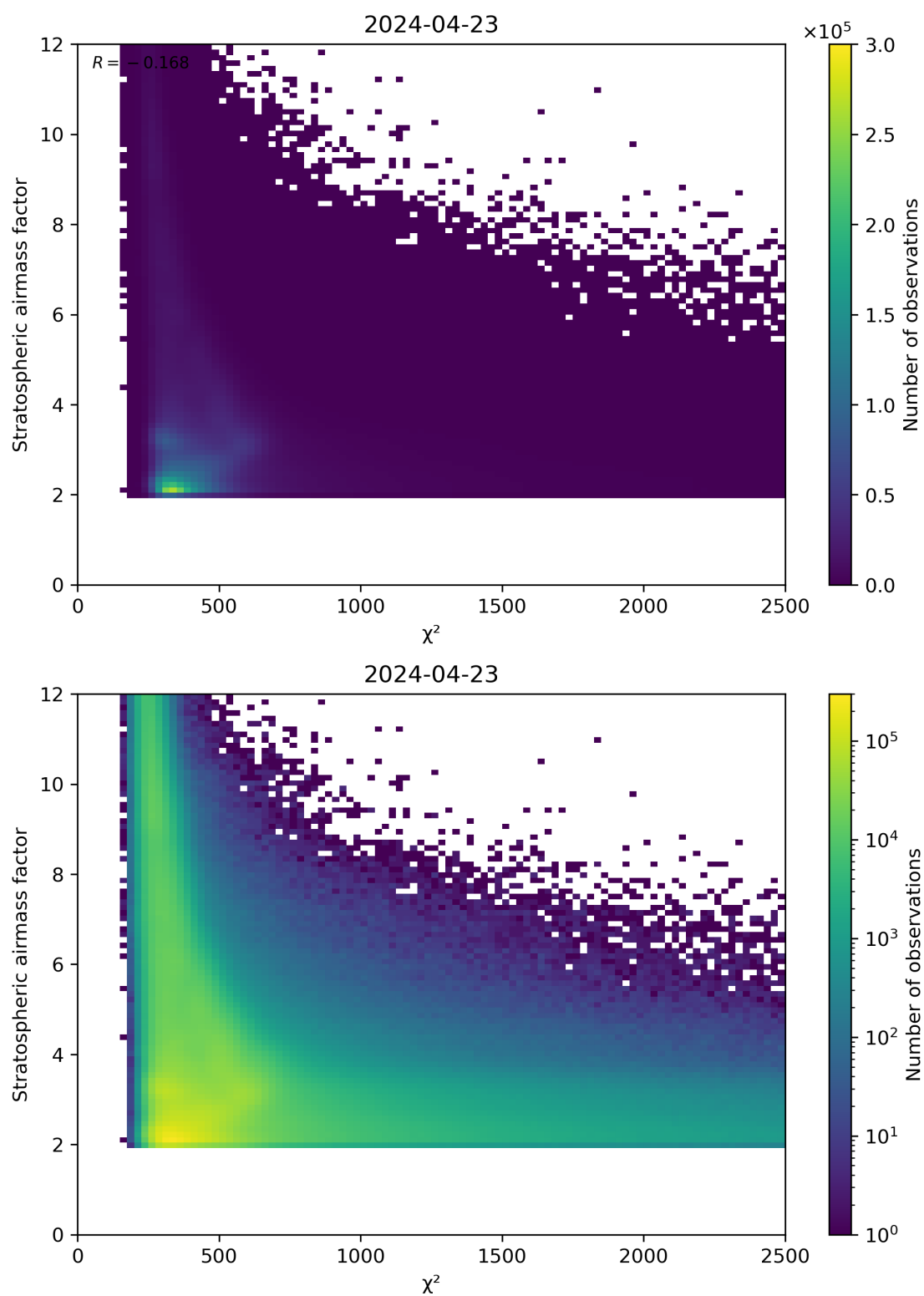
Figure 81: Scatter density plot of “ \chi^2 ” against “Stratospheric airmass factor” for 2024-04-22 to 2024-04-24.
