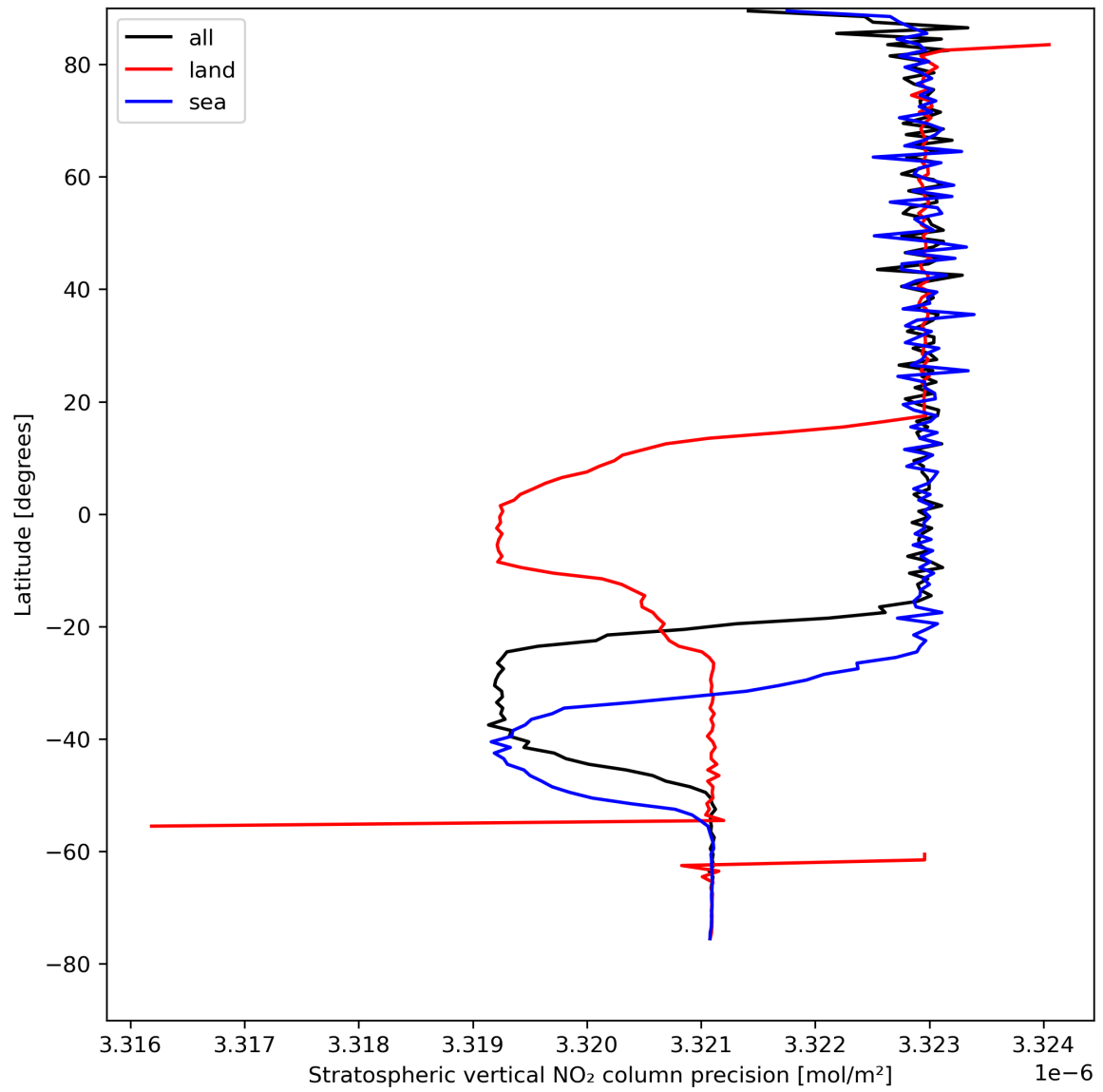
Figure 20: Zonal average of “Stratospheric vertical NO 2 column precision” for 2024-04-22 to 2024-04-24.
