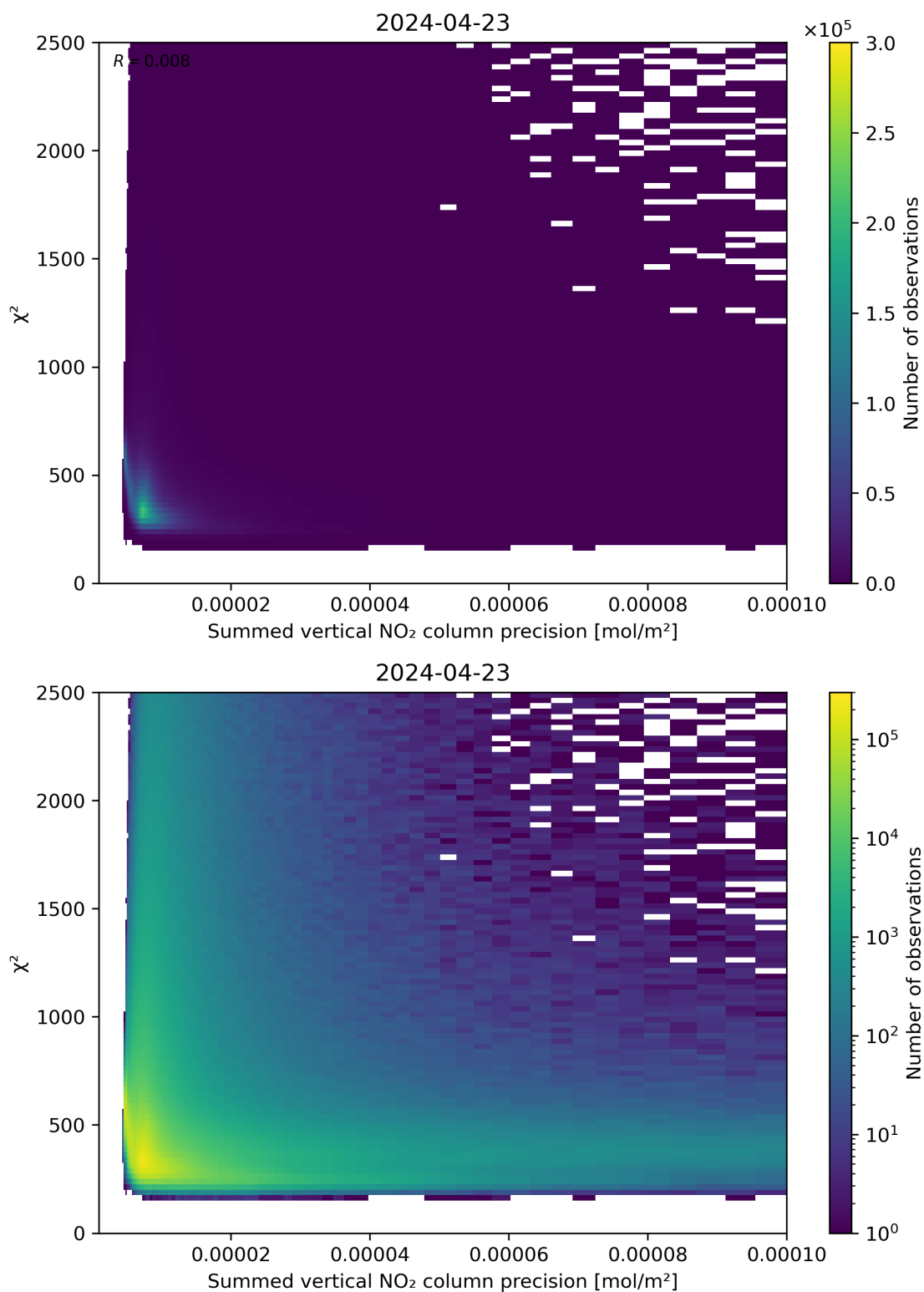
Figure 107: Scatter density plot of “Summed vertical NO 2 column precision” against “ \chi^2 ” for 2024-04-22 to 2024-04-24.
