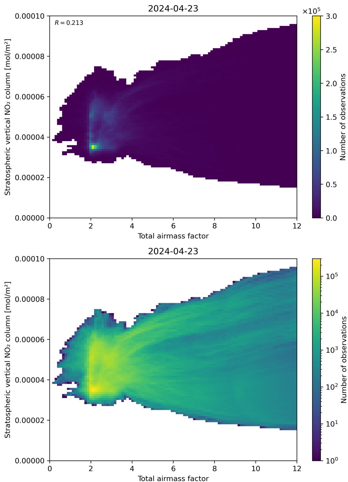
Figure 64: Scatter density plot of “Total airmass factor” against “Stratospheric vertical NO 2 column” for 2024-04-22 to 2024-04-24.
