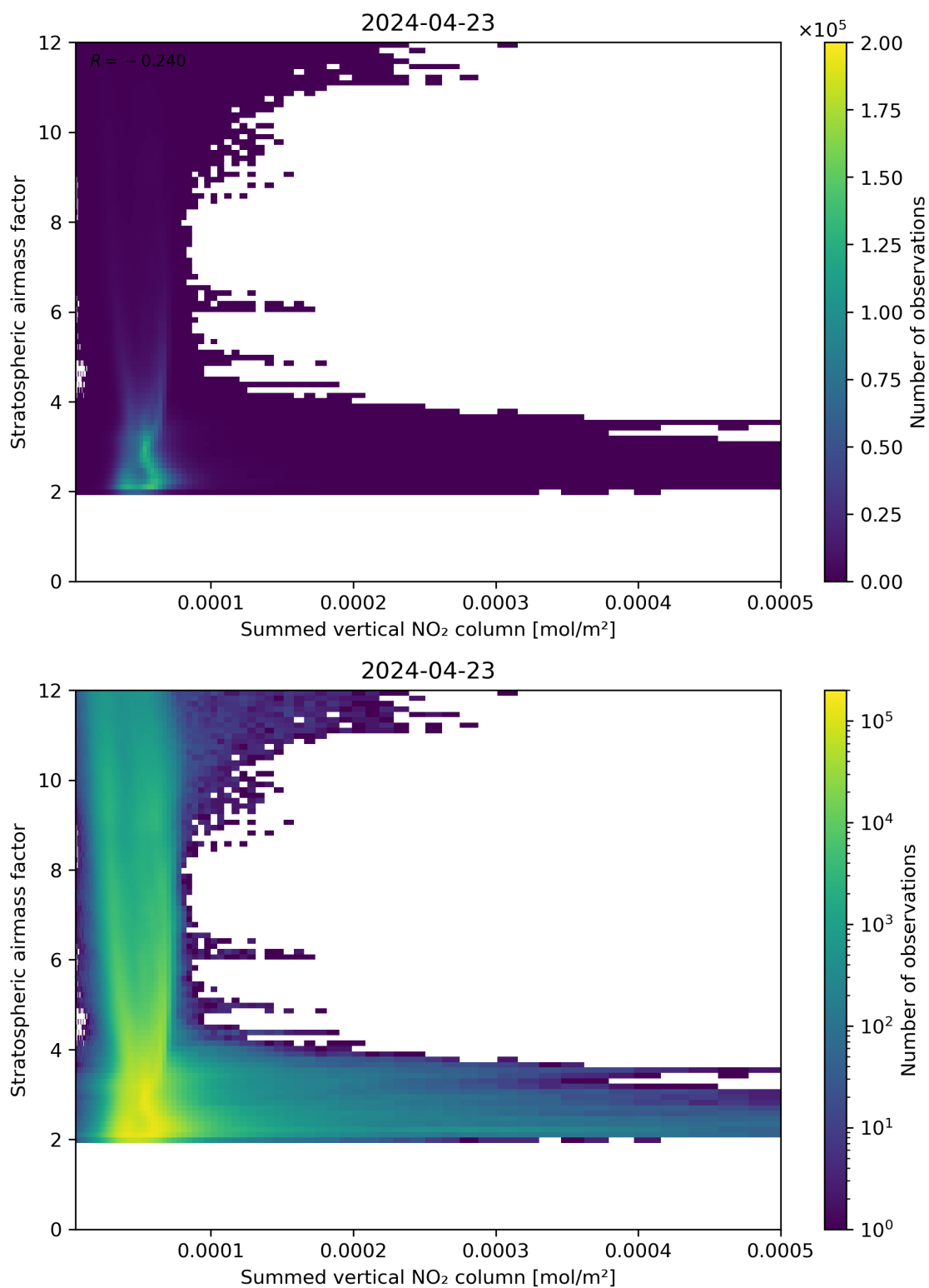
Figure 103: Scatter density plot of “Summed vertical NO 2 column” against “Stratospheric air mass factor” for 2024-04-22 to 2024-04-24.
