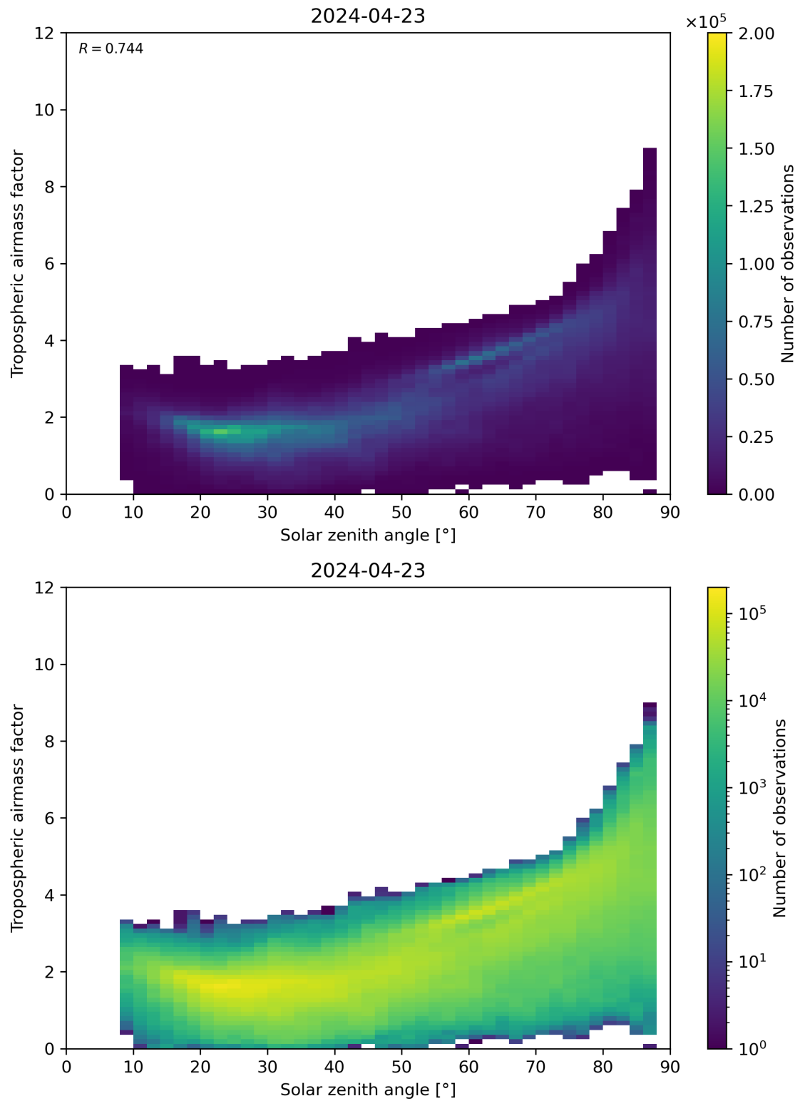
Figure 147: Scatter density plot of “Solar zenith angle” against “Tropospheric airmass factor” for 2024-04-22 to 2024-04-24.
