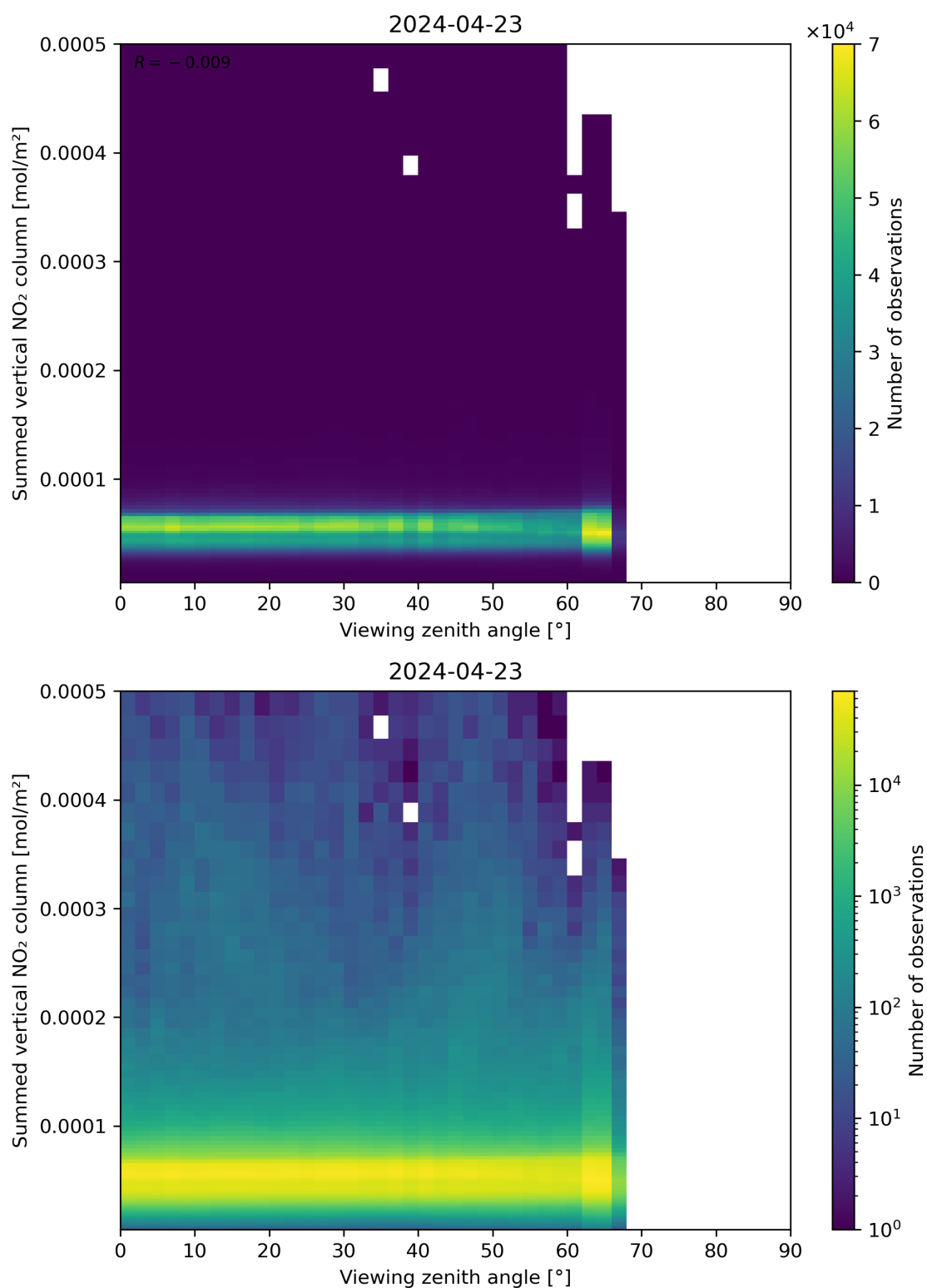
Figure 165: Scatter density plot of “Viewing zenith angle” against “Summed vertical NO 2 column” for 2024-04-22 to 2024-04-24.
