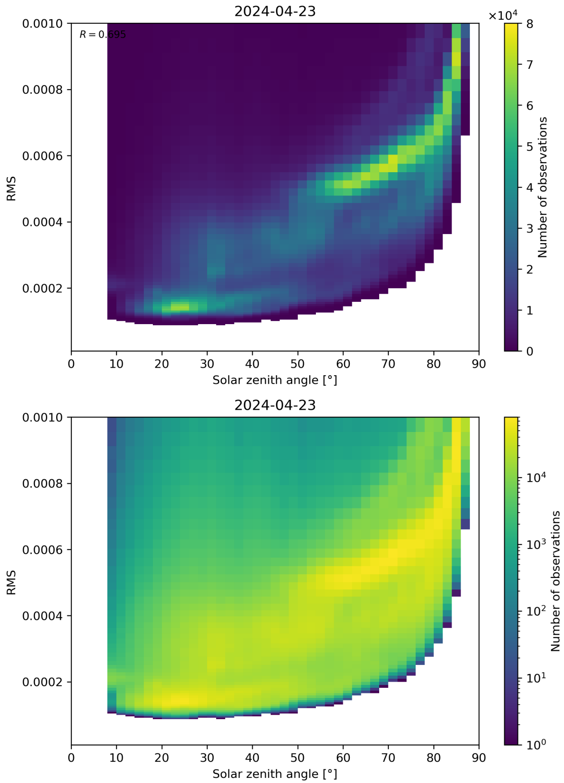
Figure 157: Scatter density plot of “Solar zenith angle” against “RMS” for 2024-04-22 to 2024-04-24.
