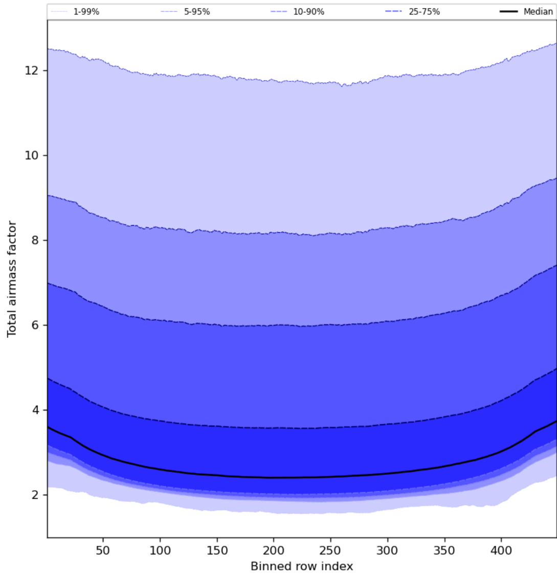
Figure 49: Along track statistics of “Total airmass factor” for 2024-04-22 to 2024-04-24
