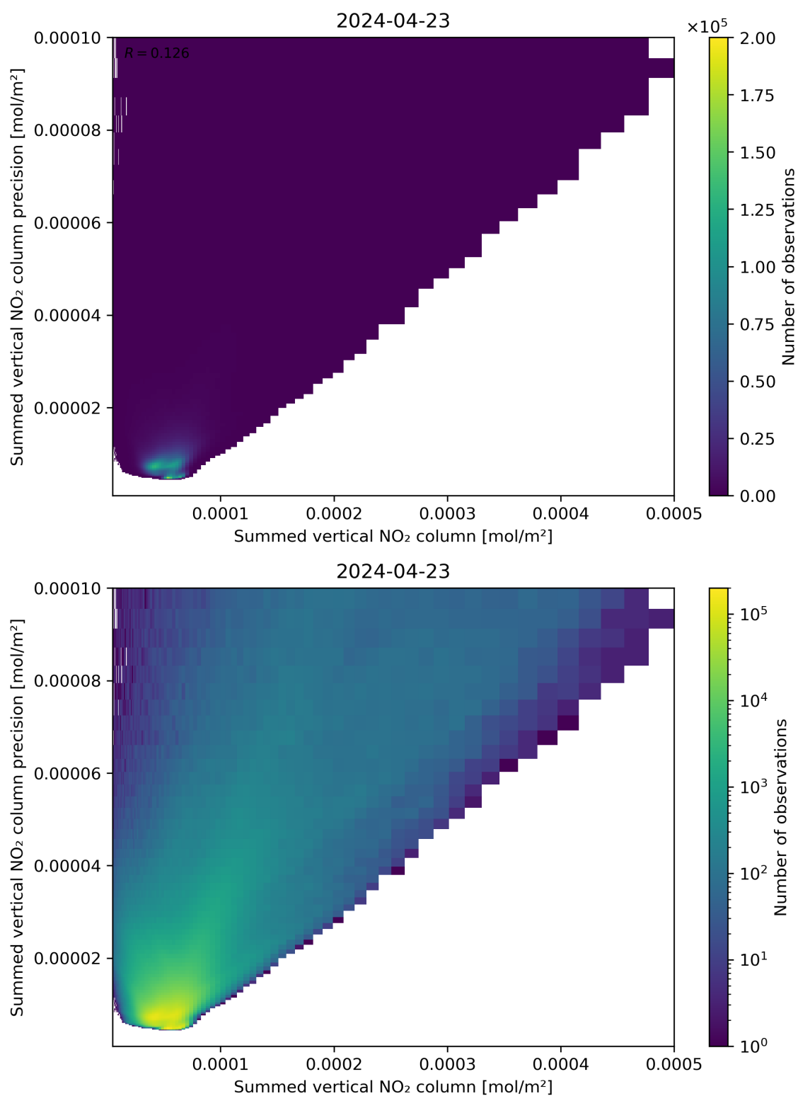
Figure 105: Scatter density plot of “Summed vertical NO 2 column” against “Summed vertical NO 2 column precision” for 2024-04-22 to 2024-04-24.
