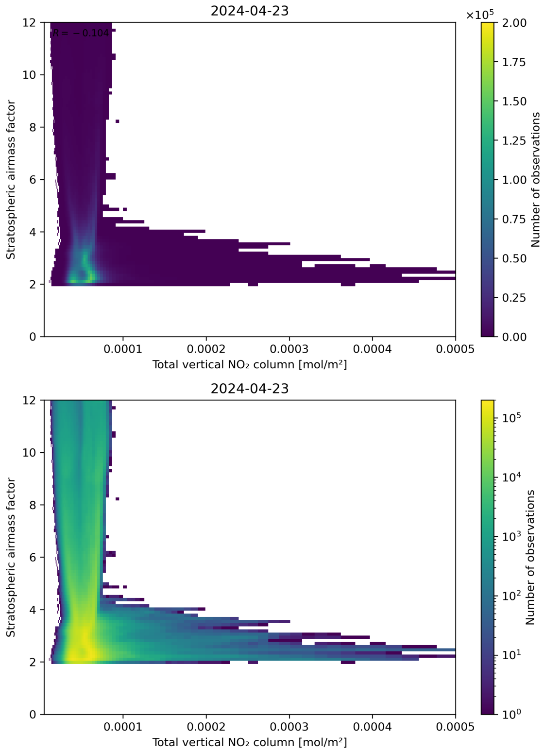
Figure 110: Scatter density plot of “Total vertical NO 2 column” against “Stratospheric airmass factor” for 2024-04-22 to 2024-04-24.
