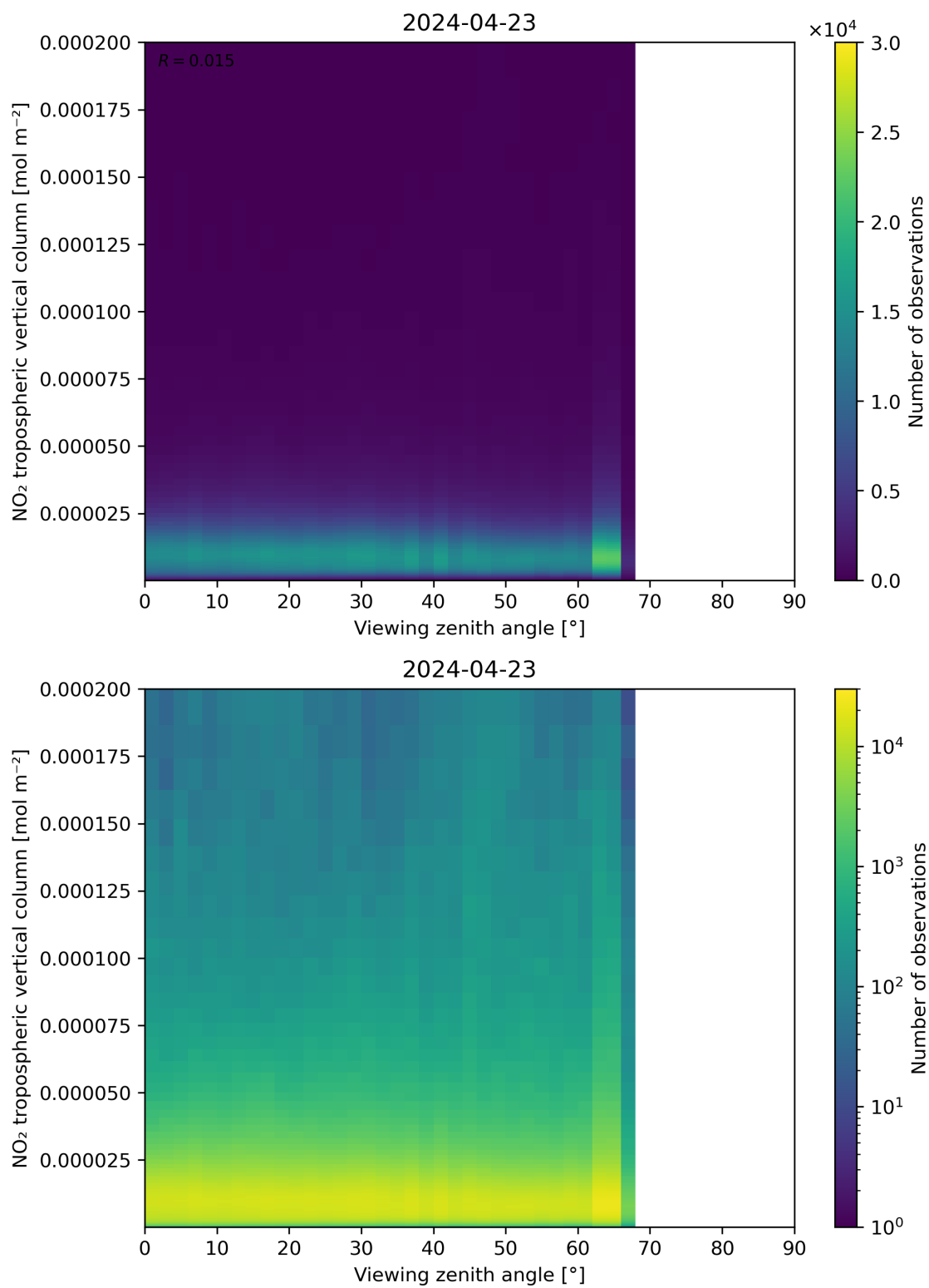
Figure 169: Scatter density plot of “Viewing zenith angle” against “NO 2 tropospheric vertical column” for 2024-04-22 to 2024-04-24.
