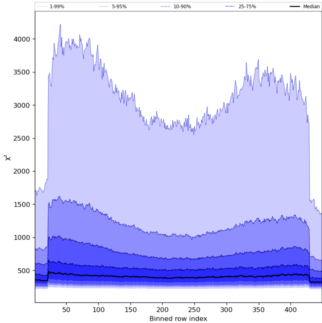
Figure 59: Along track statistics of “ \chi^2 ” for 2024-04-22 to 2024-04-24
