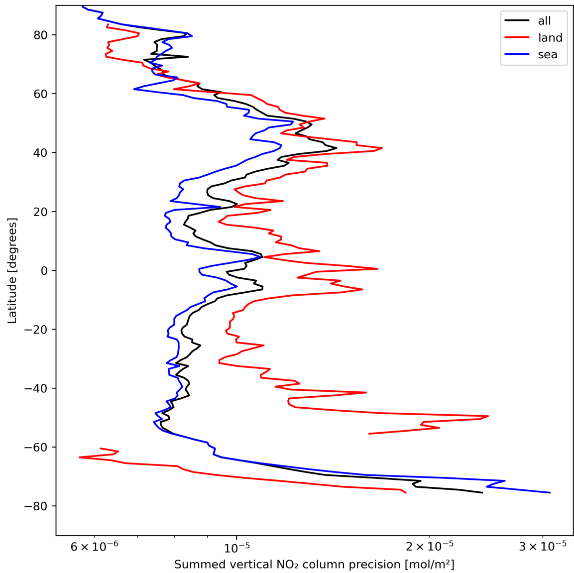
Figure 24: Zonal average of “Summed vertical NO 2 column precision” for 2024-04-22 to 2024-04-24.
