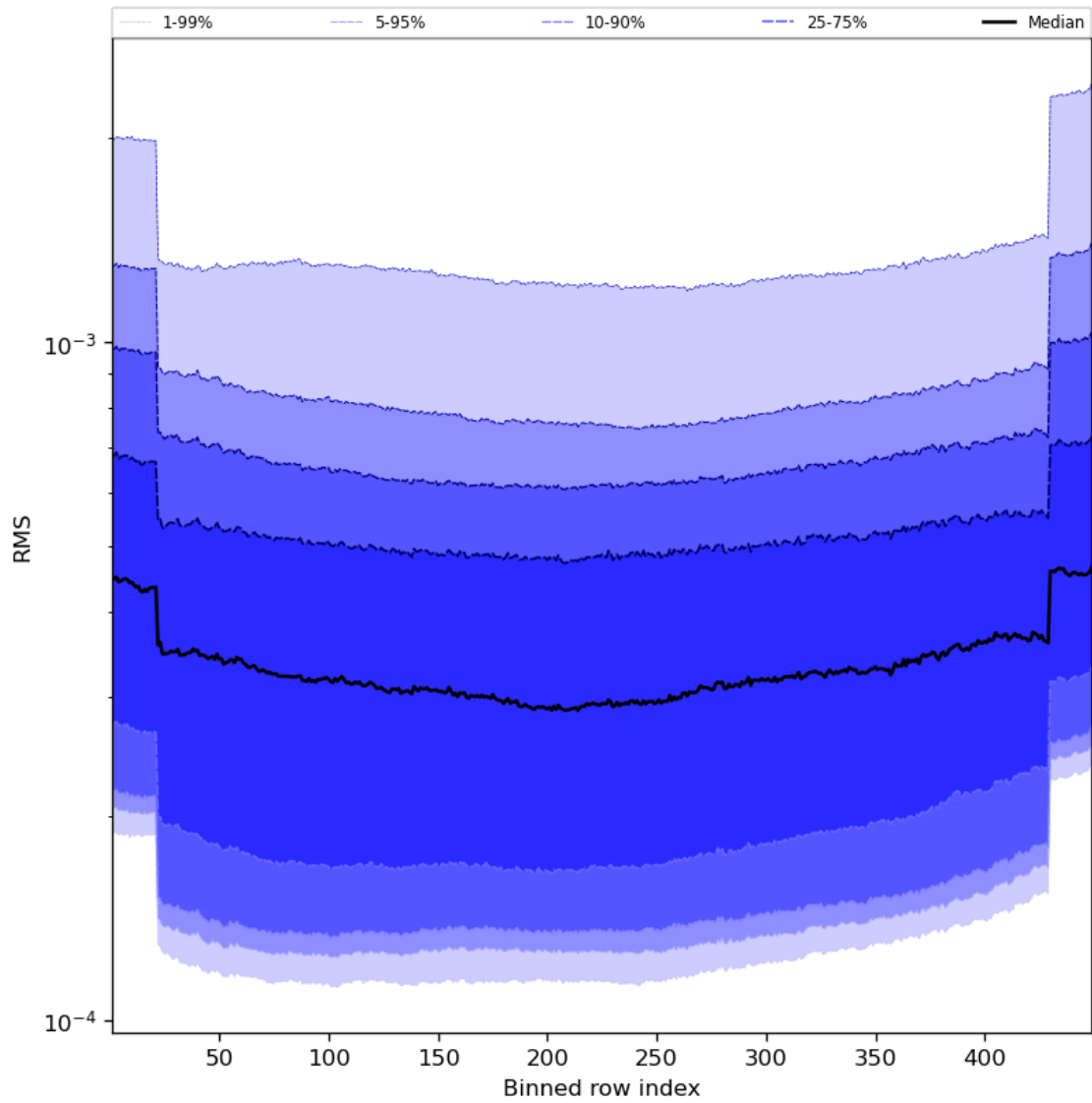
Figure 60: Along track statistics of “RMS” for 2024-04-22 to 2024-04-24
