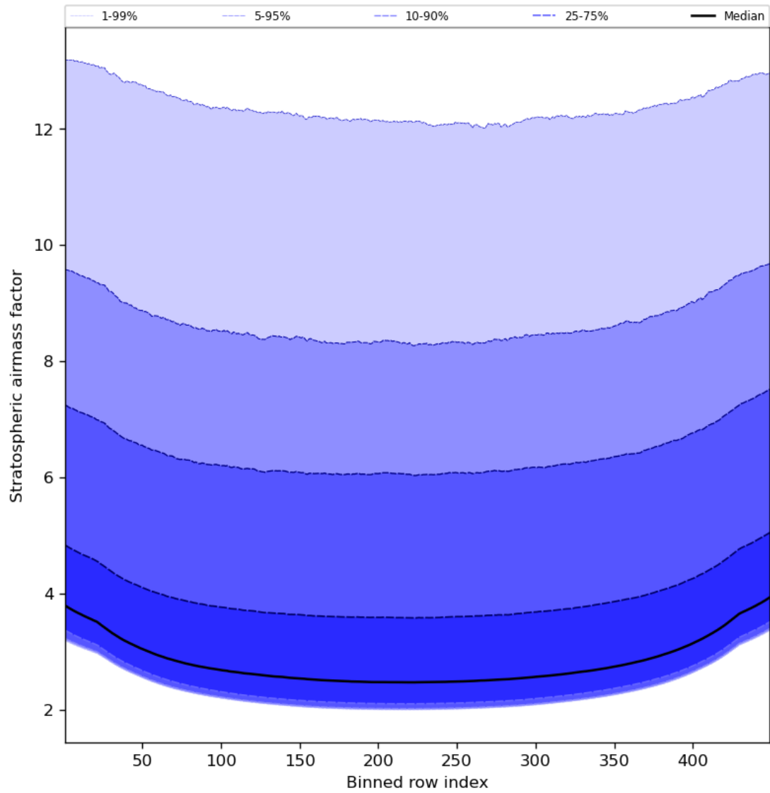
Figure 61: Along track statistics of “Stratospheric airmass factor” for 2024-04-22 to 2024-04-24
