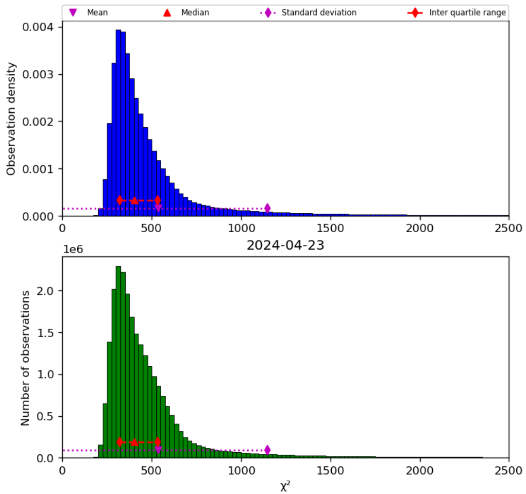
Figure 42: Histogram of “ \chi^2 ” for 2024-04-22 to 2024-04-24
