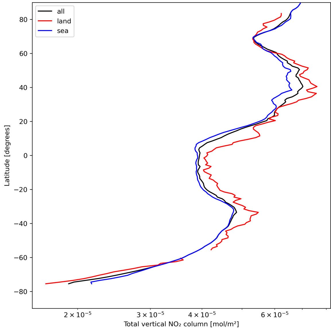
Figure 21: Zonal average of “Total vertical NO 2 column” for 2024-04-22 to 2024-04-24.
