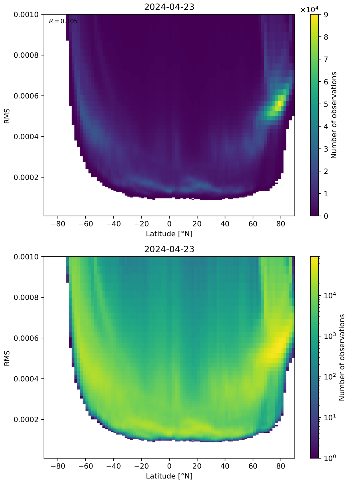
Figure 94: Scatter density plot of “Latitude” against “RMS” for 2024-04-22 to 2024-04-24.
