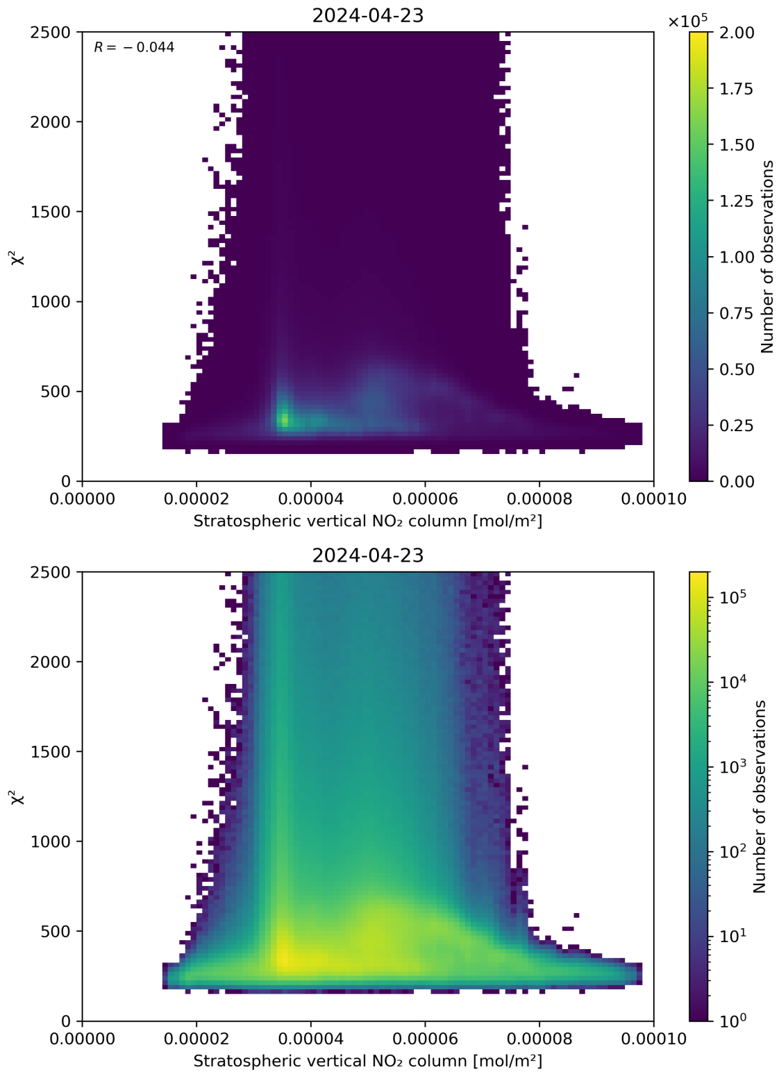
Figure 97: Scatter density plot of “Stratospheric vertical NO 2 column” against “ \chi^2 ” for 2024-04-22 to 2024-04-24.
