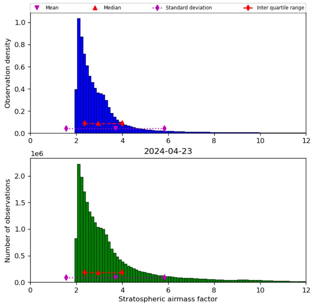
Figure 44: Histogram of “Stratospheric airmass factor” for 2024-04-22 to 2024-04-24
