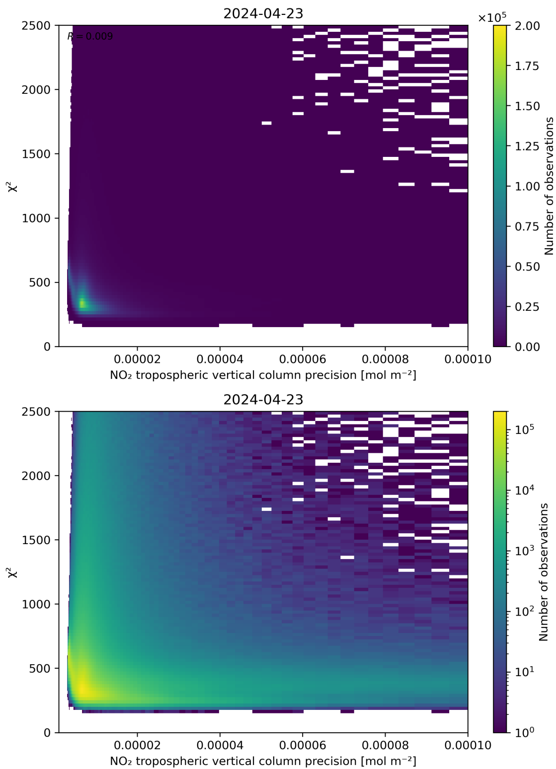
Figure 134: Scatter density plot of “NO 2 tropospheric vertical column precision” against “ \chi^2 ” for 2024-04-22 to 2024-04-24.
