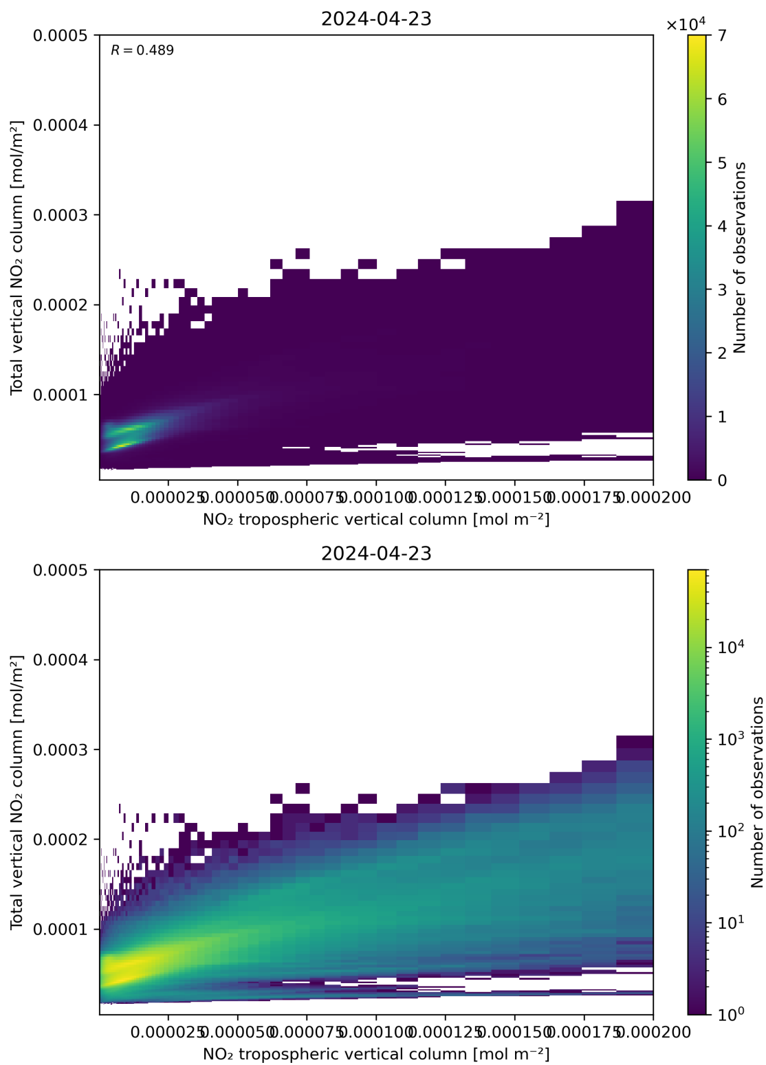
Figure 128: Scatter density plot of “NO 2 tropospheric vertical column” against “Total vertical NO 2 column” for 2024-04-22 to 2024-04-24.
