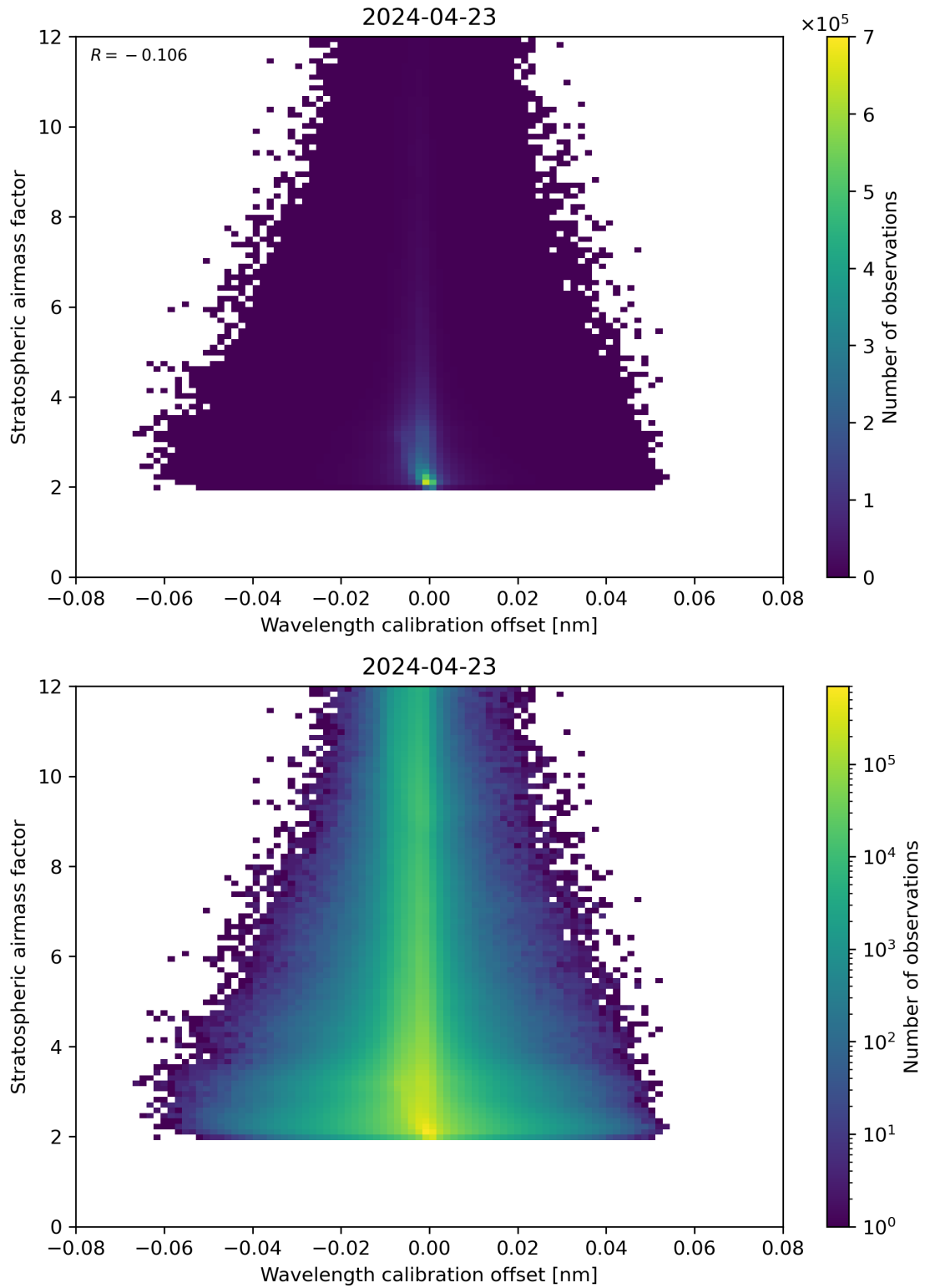
Figure 174: Scatter density plot of “Wavelength calibration offset” against “Stratospheric airmass factor” for 2024-04-22 to 2024-04-24.
