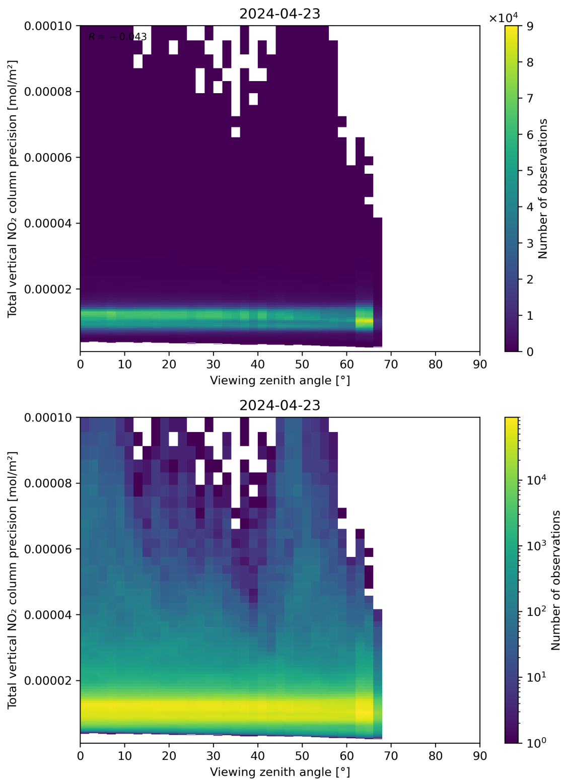
Figure 168: Scatter density plot of “Viewing zenith angle” against “Total vertical NO 2 column precision” for 2024-04-22 to 2024-04-24.
