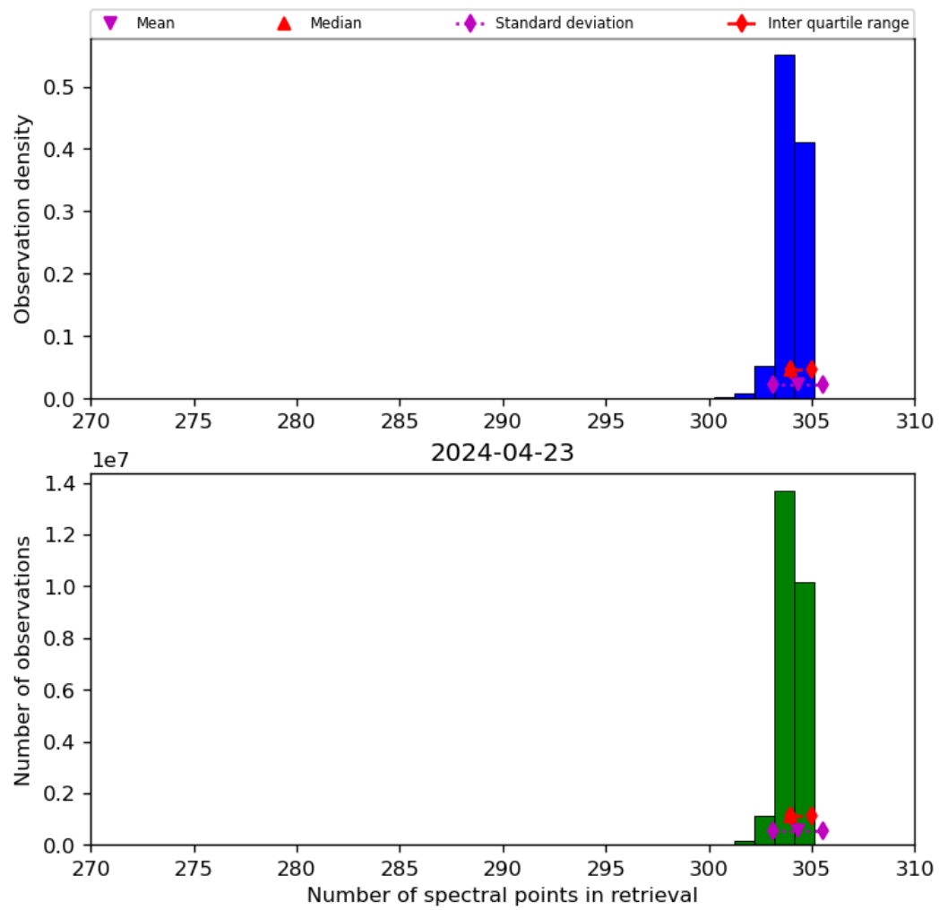
Figure 33: Histogram of “Number of spectral points in retrieval” for 2024-04-22 to 2024-04-24
