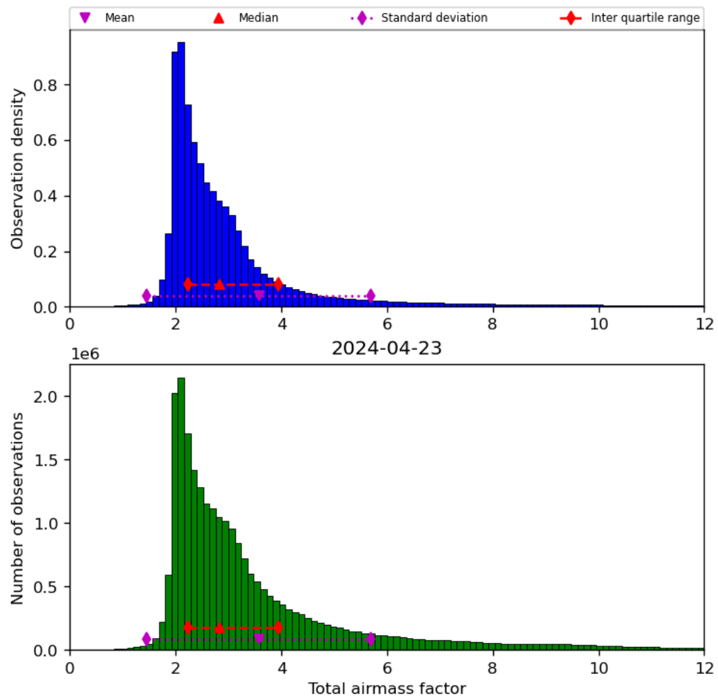
Figure 32: Histogram of “Total airmass factor” for 2024-04-22 to 2024-04-24
