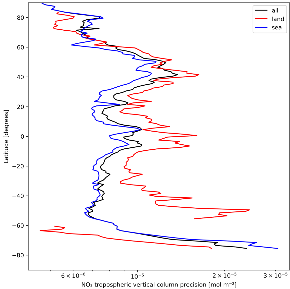
Figure 13: Zonal average of “NO 2 tropospheric vertical column precision” for 2024-04-22 to 2024-04-24.
