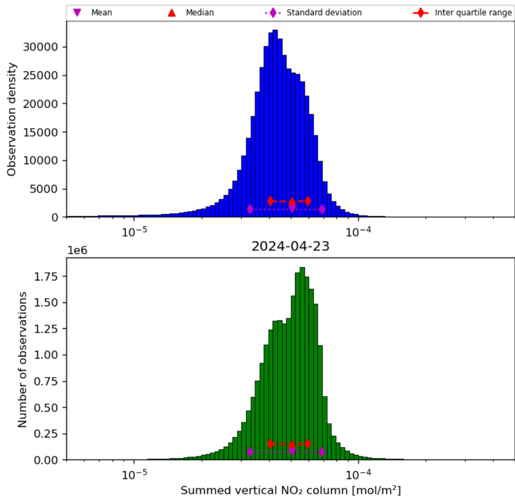
Figure 40: Histogram of “Summed vertical NO 2 column” for 2024-04-22 to 2024-04-24
