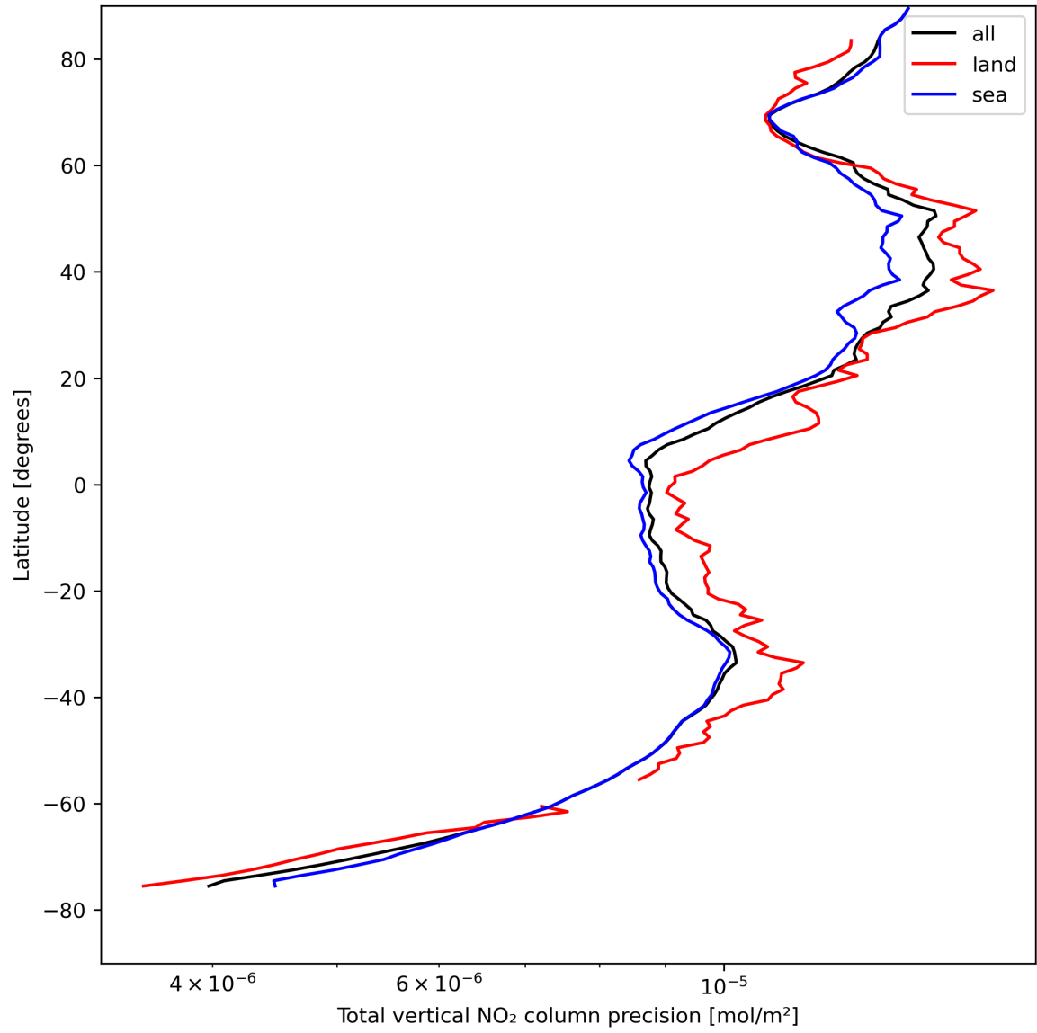
Figure 22: Zonal average of “Total vertical NO 2 column precision” for 2024-04-22 to 2024-04-24.
