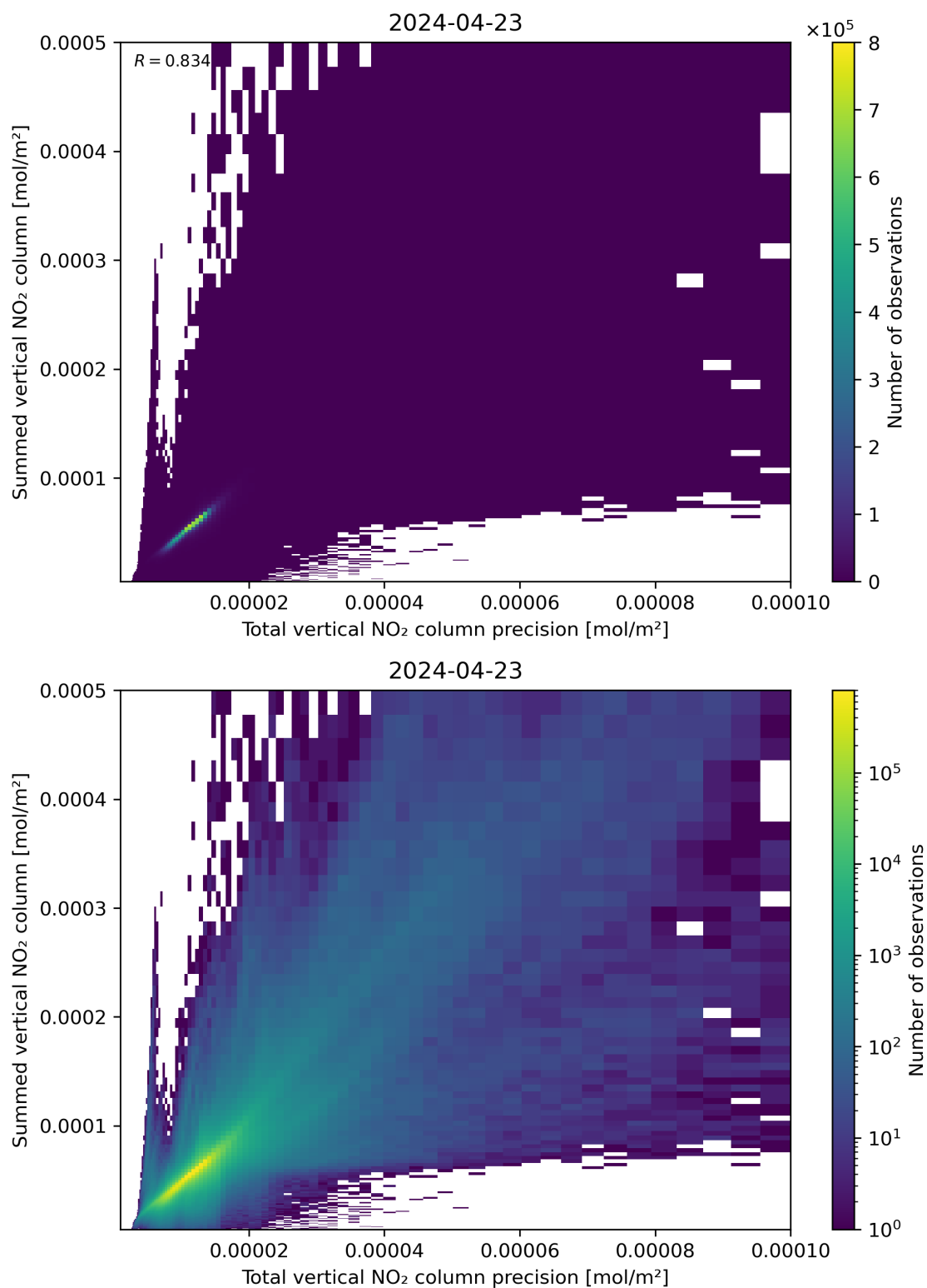
Figure 117: Scatter density plot of “Total vertical NO 2 column precision” against “Summed vertical NO 2 column” for 2024-04-22 to 2024-04-24.
