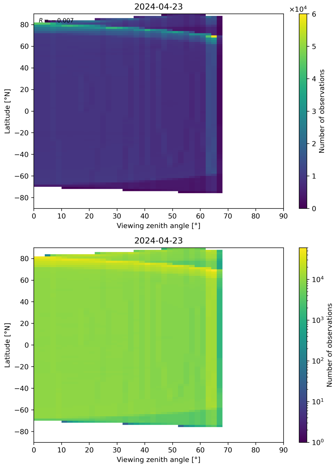
Figure 163: Scatter density plot of “Viewing zenith angle” against “Latitude” for 2024-04-22 to 2024-04-24.
