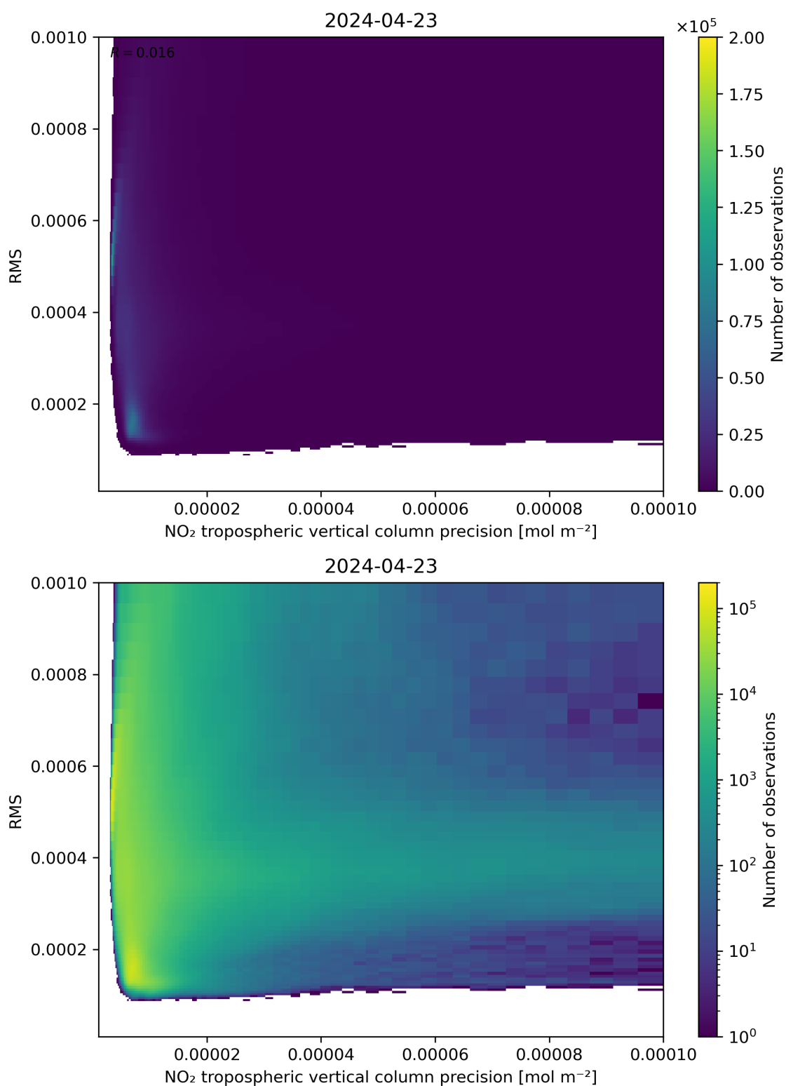
Figure 140: Scatter density plot of “NO 2 tropospheric vertical column precision” against “RMS” for 2024-04-22 to 2024-04-24.
