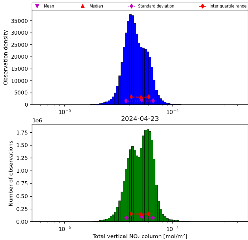
Figure 38: Histogram of “Total vertical NO 2 column” for 2024-04-22 to 2024-04-24
