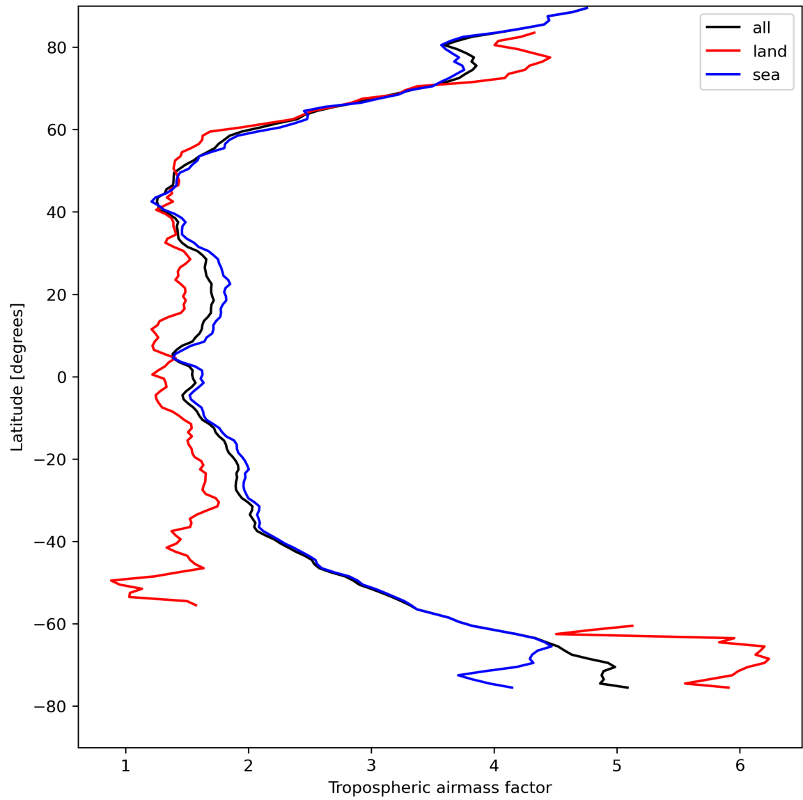
Figure 14: Zonal average of “Tropospheric airmass factor” for 2024-04-22 to 2024-04-24.
