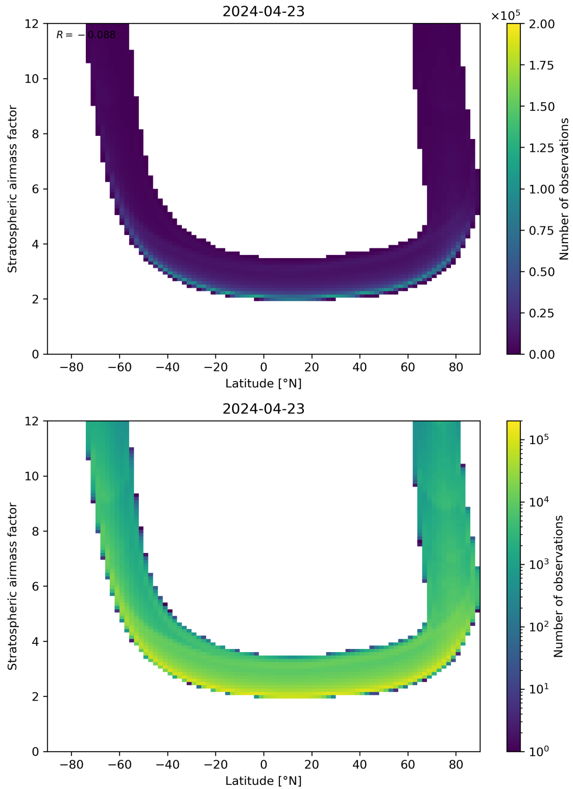
Figure 83: Scatter density plot of “Latitude” against “Stratospheric air mass factor” for 2024-04-22 to 2024-04-24.
