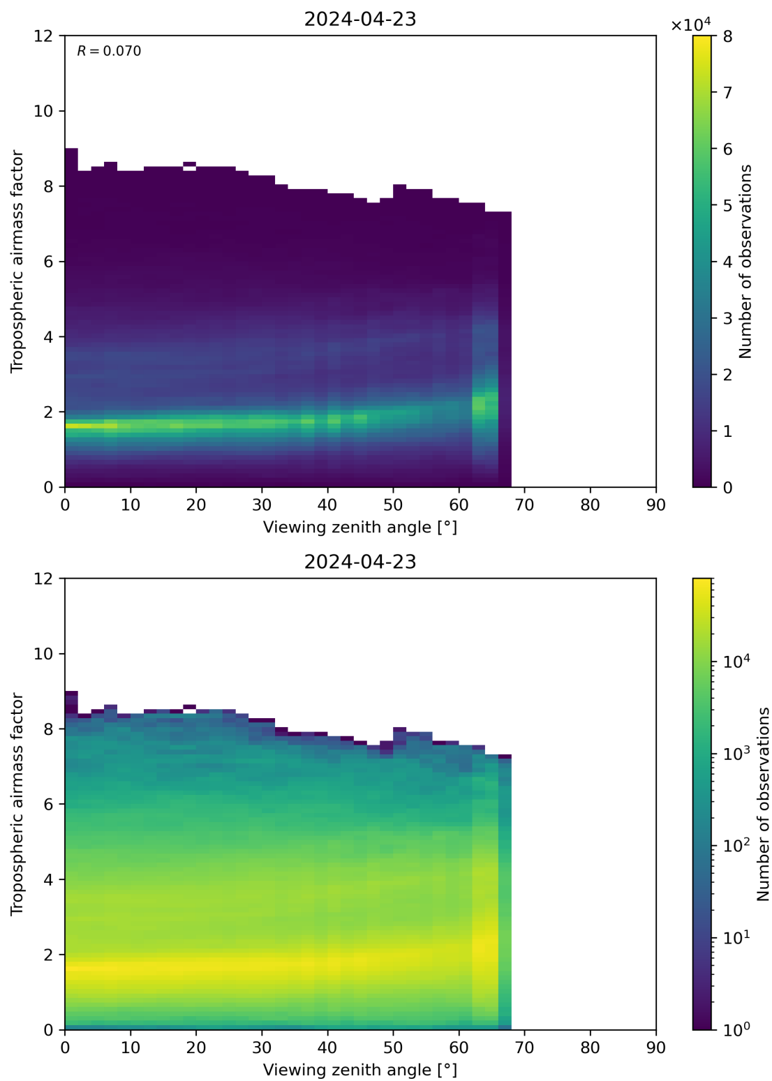
Figure 161: Scatter density plot of “Viewing zenith angle” against “Tropospheric airmass factor” for 2024-04-22 to 2024-04-24.
