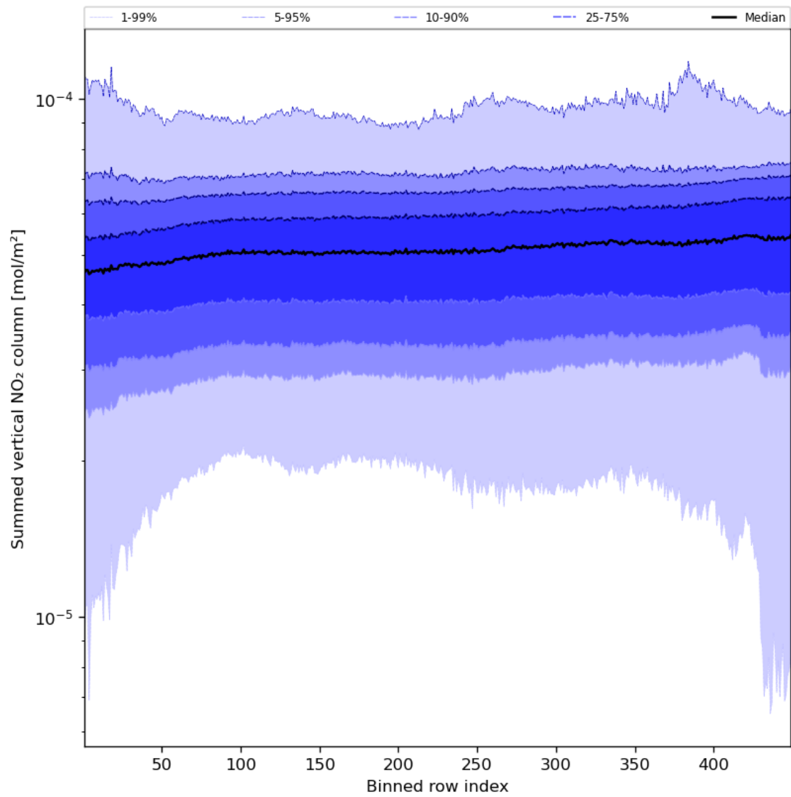
Figure 57: Along track statistics of “Summed vertical NO 2 column” for 2024-04-22 to 2024-04-24
