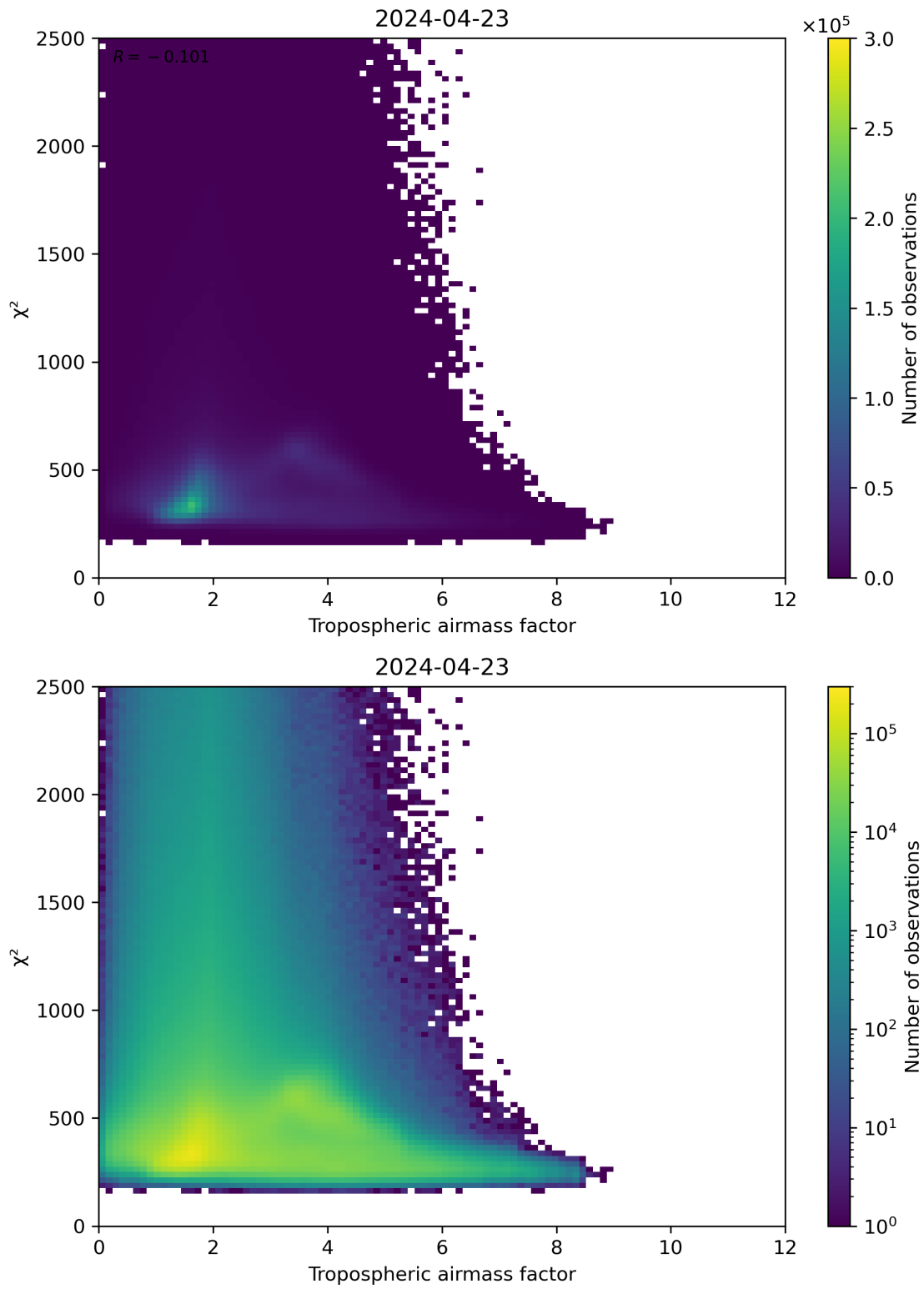
Figure 73: Scatter density plot of “Tropospheric airmass factor” against “ \chi^2 ” for 2024-04-22 to 2024-04-24.
