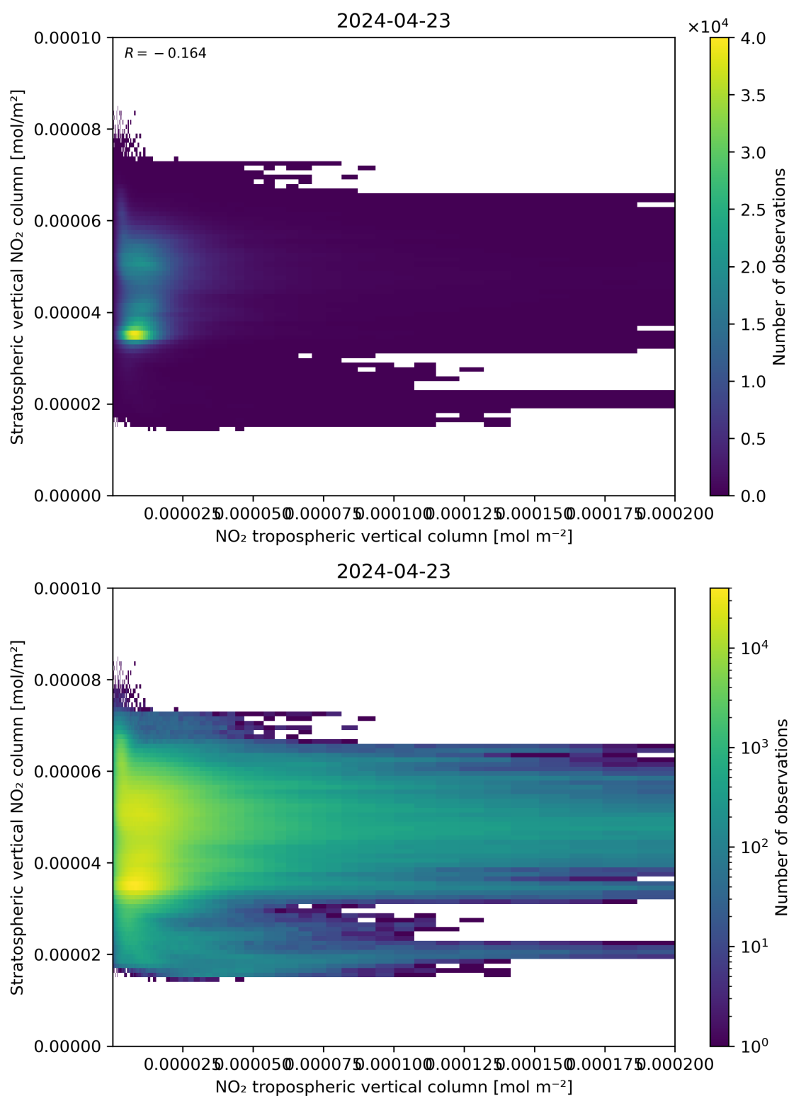
Figure 125: Scatter density plot of “NO 2 tropospheric vertical column” against “Stratospheric vertical NO 2 column” for 2024-04-22 to 2024-04-24.
