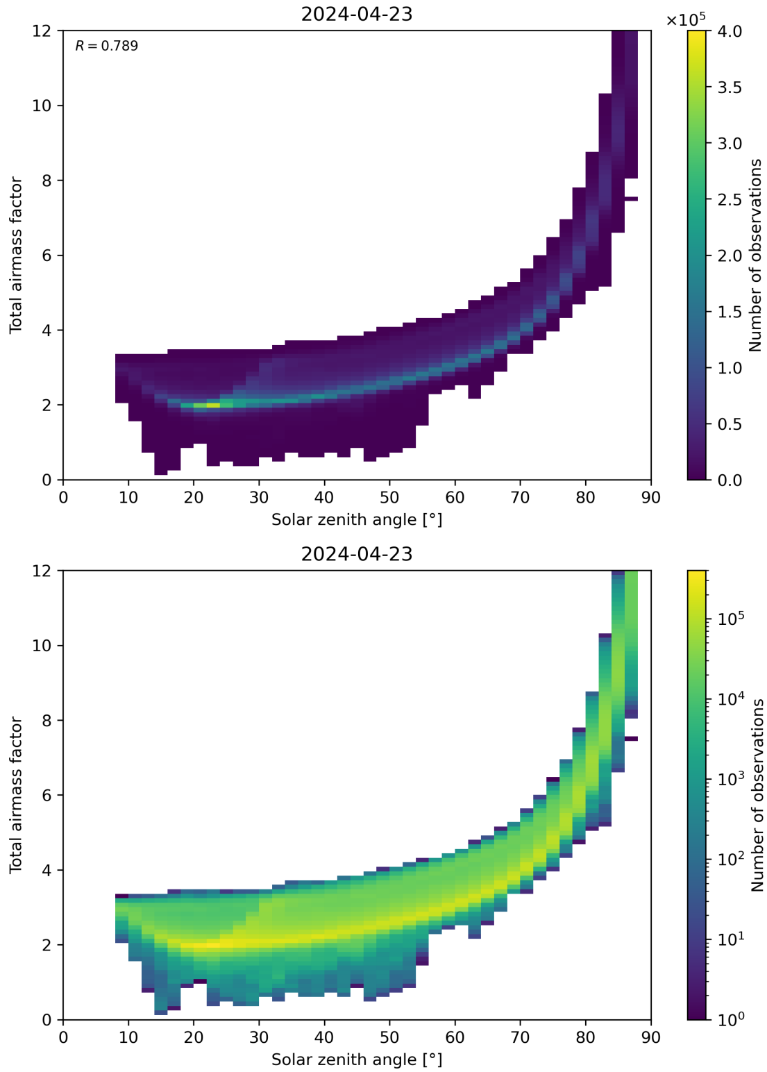
Figure 146: Scatter density plot of “Solar zenith angle” against “Total air mass factor” for 2024-04-22 to 2024-04-24.
