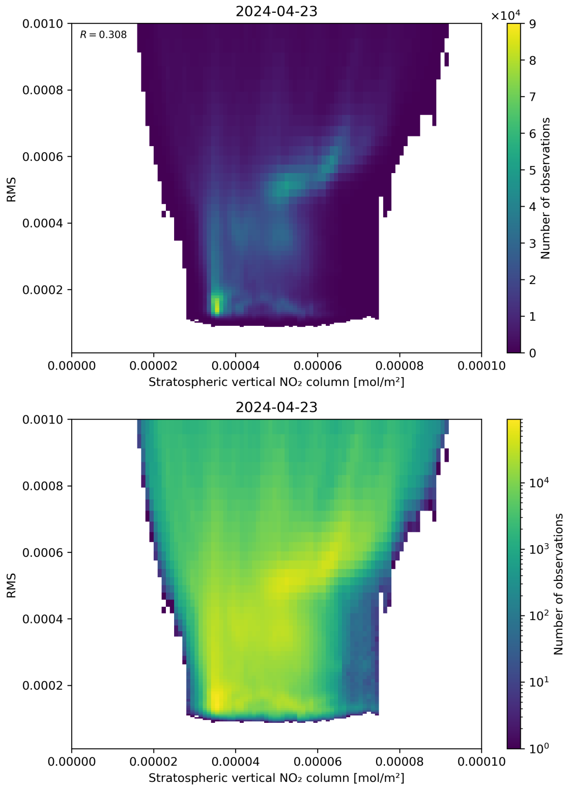
Figure 102: Scatter density plot of “Stratospheric vertical NO 2 column” against “RMS” for 2024-04-22 to 2024-04-24.
