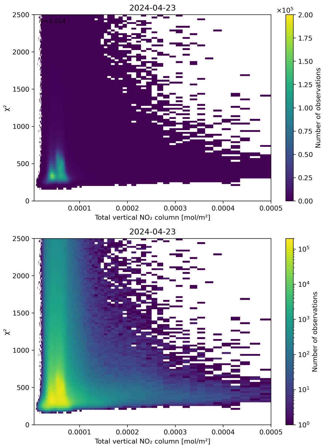
Figure 111: Scatter density plot of “Total vertical NO 2 column” against “ \chi^2 ” for 2024-04-22 to 2024-04-24.
