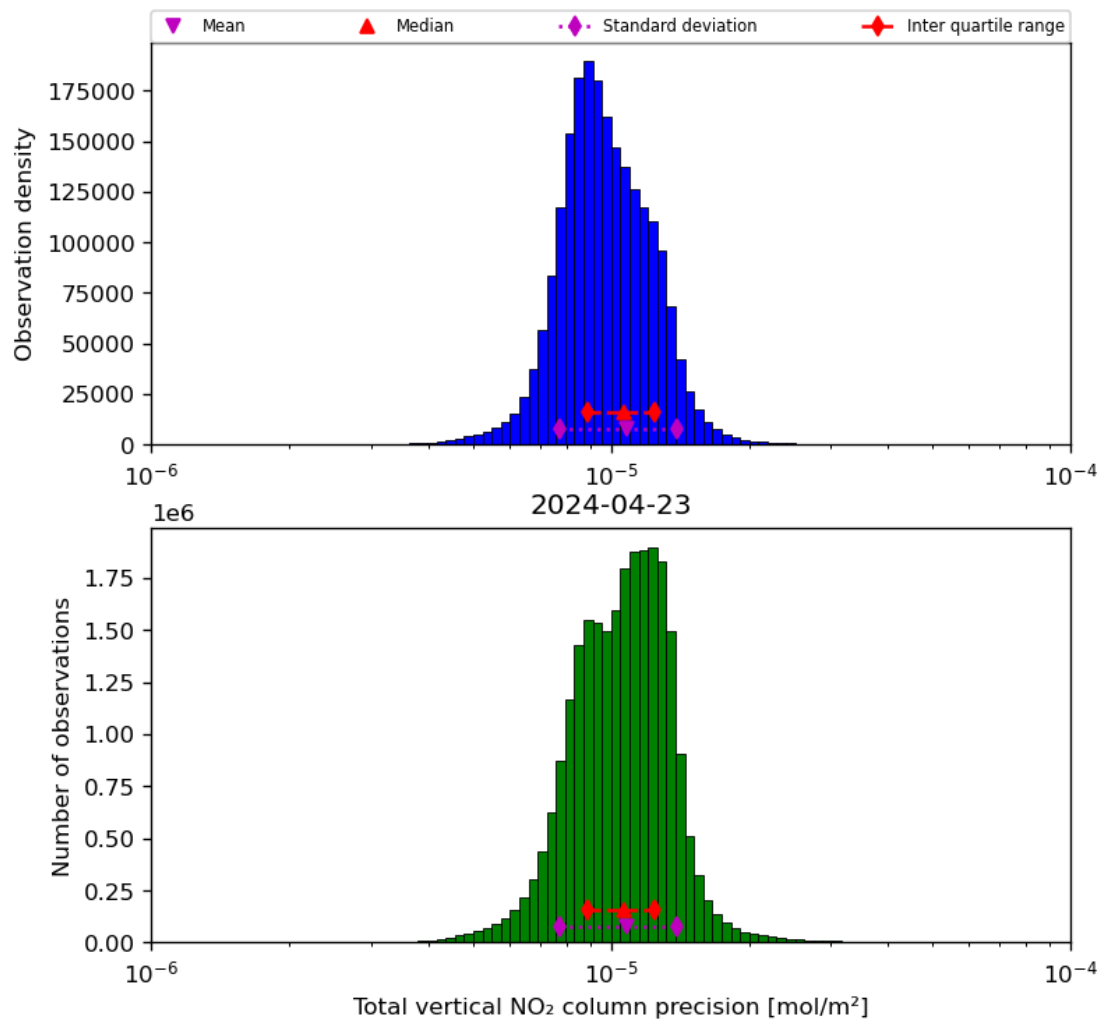
Figure 39: Histogram of “Total vertical NO 2 column precision” for 2024-04-22 to 2024-04-24
