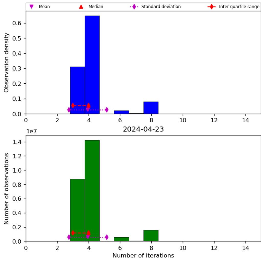
Figure 34: Histogram of “Number of iterations” for 2024-04-22 to 2024-04-24
