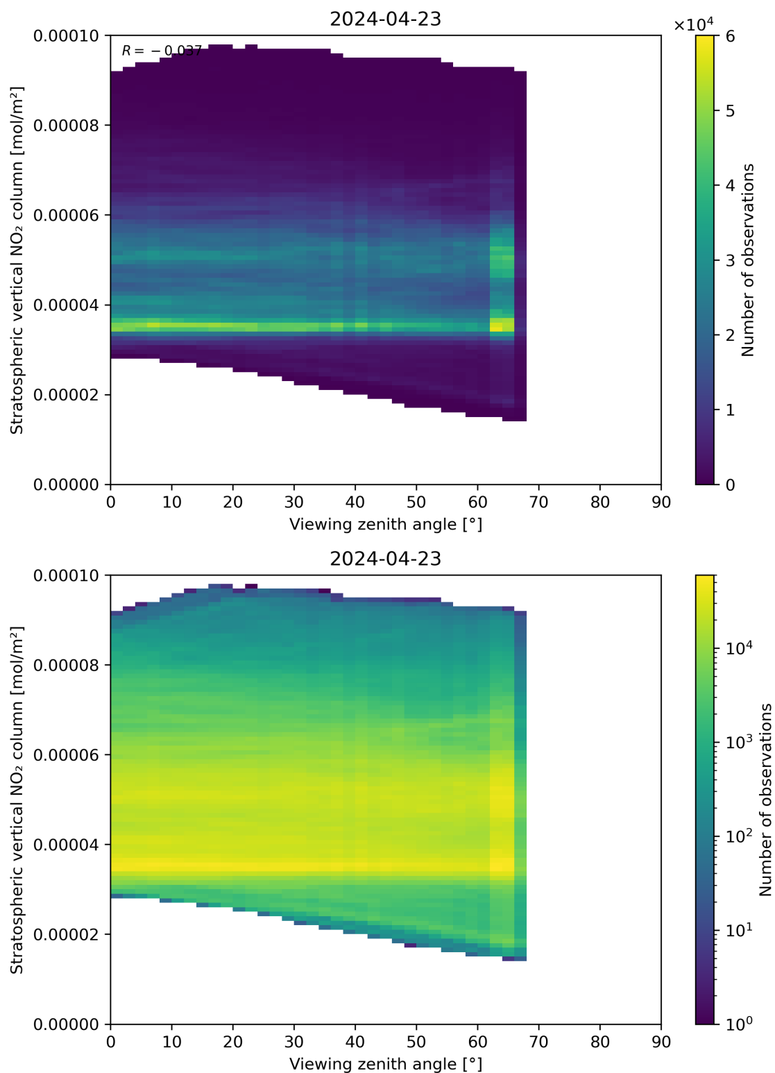
Figure 164: Scatter density plot of “Viewing zenith angle” against “Stratospheric vertical NO 2 column” for 2024-04-22 to 2024-04-24.
