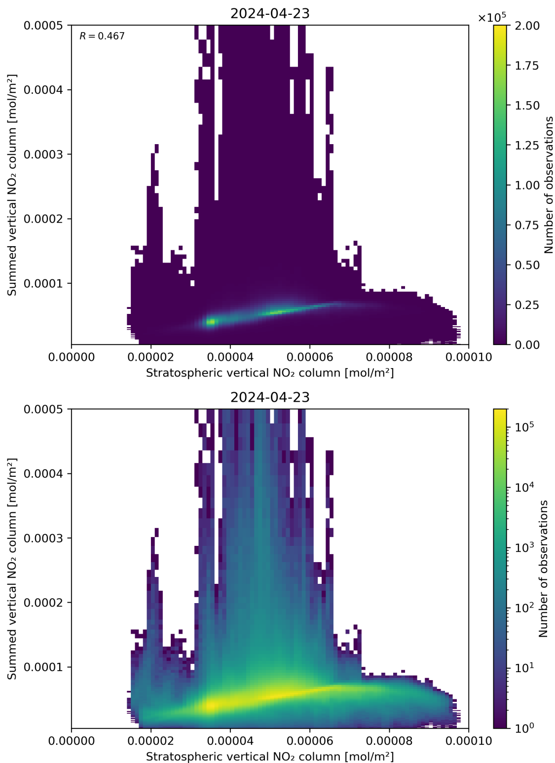
Figure 98: Scatter density plot of “Stratospheric vertical NO 2 column” against “Summed vertical NO 2 column” for 2024-04-22 to 2024-04-24.
