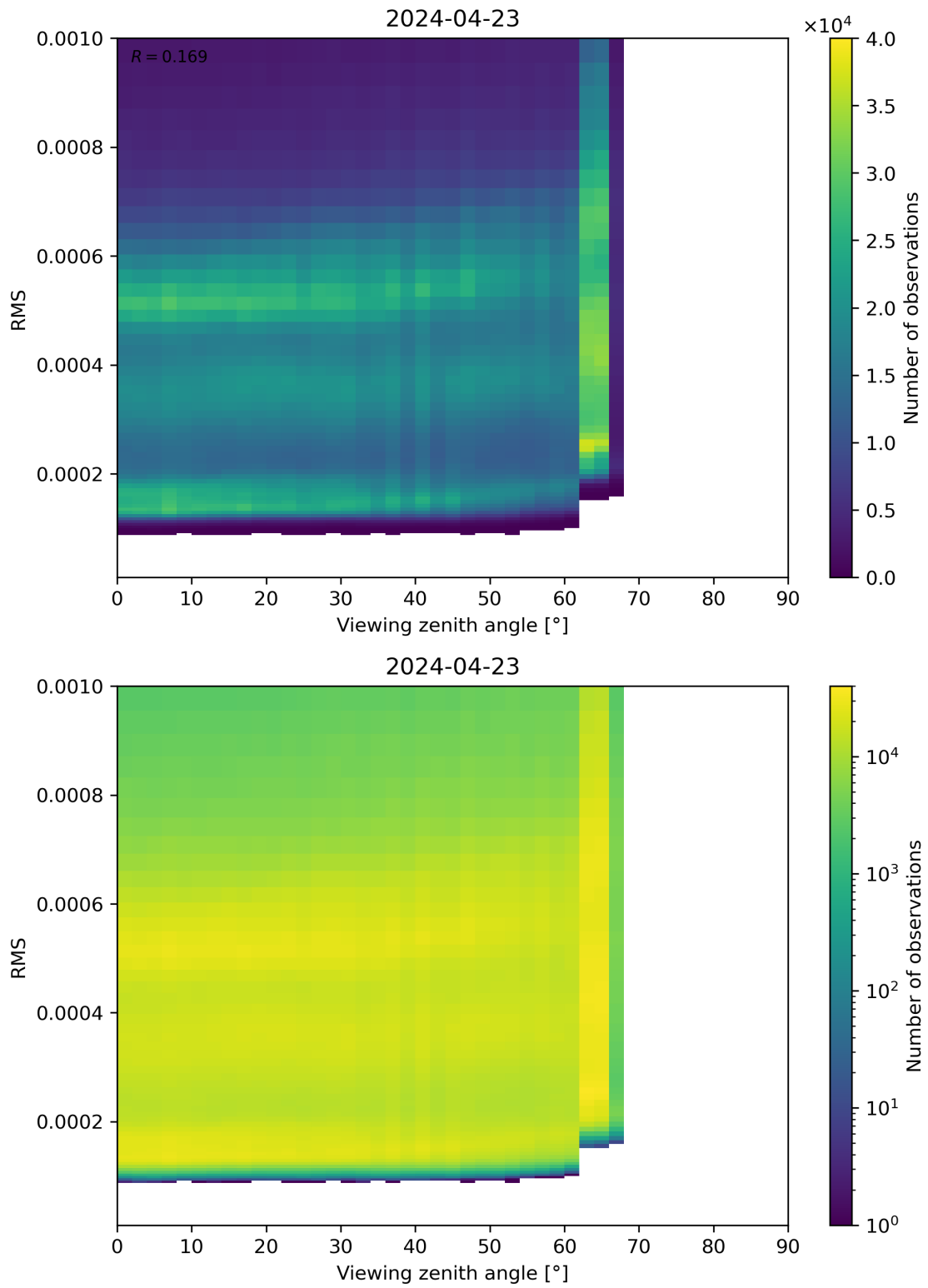
Figure 171: Scatter density plot of “Viewing zenith angle” against “RMS” for 2024-04-22 to 2024-04-24.
