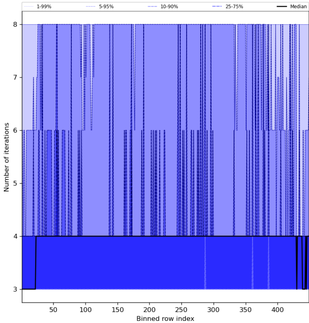
Figure 51: Along track statistics of “Number of iterations” for 2024-04-22 to 2024-04-24
