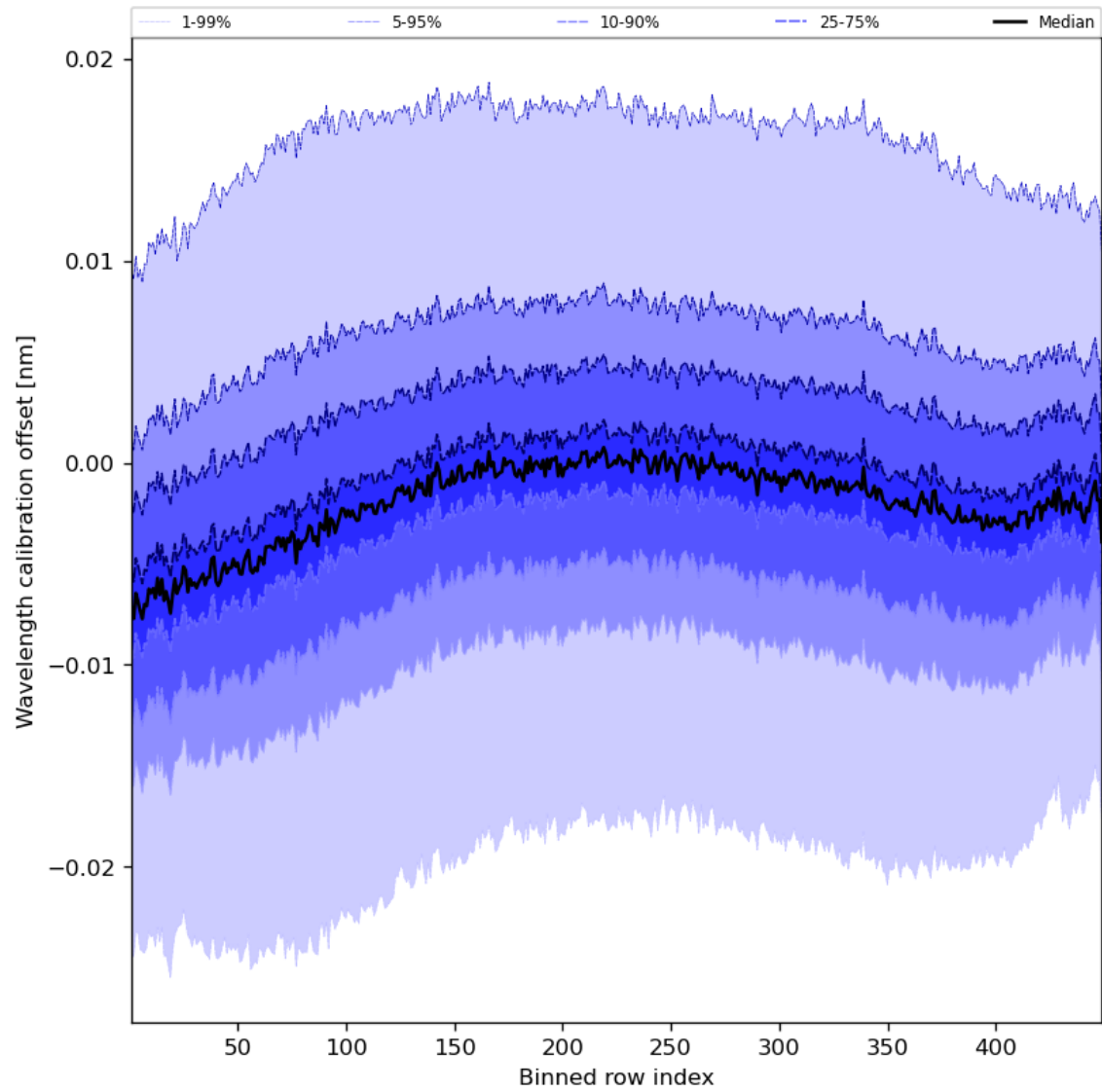
Figure 52: Along track statistics of “Wavelength calibration offset” for 2024-04-22 to 2024-04-24
