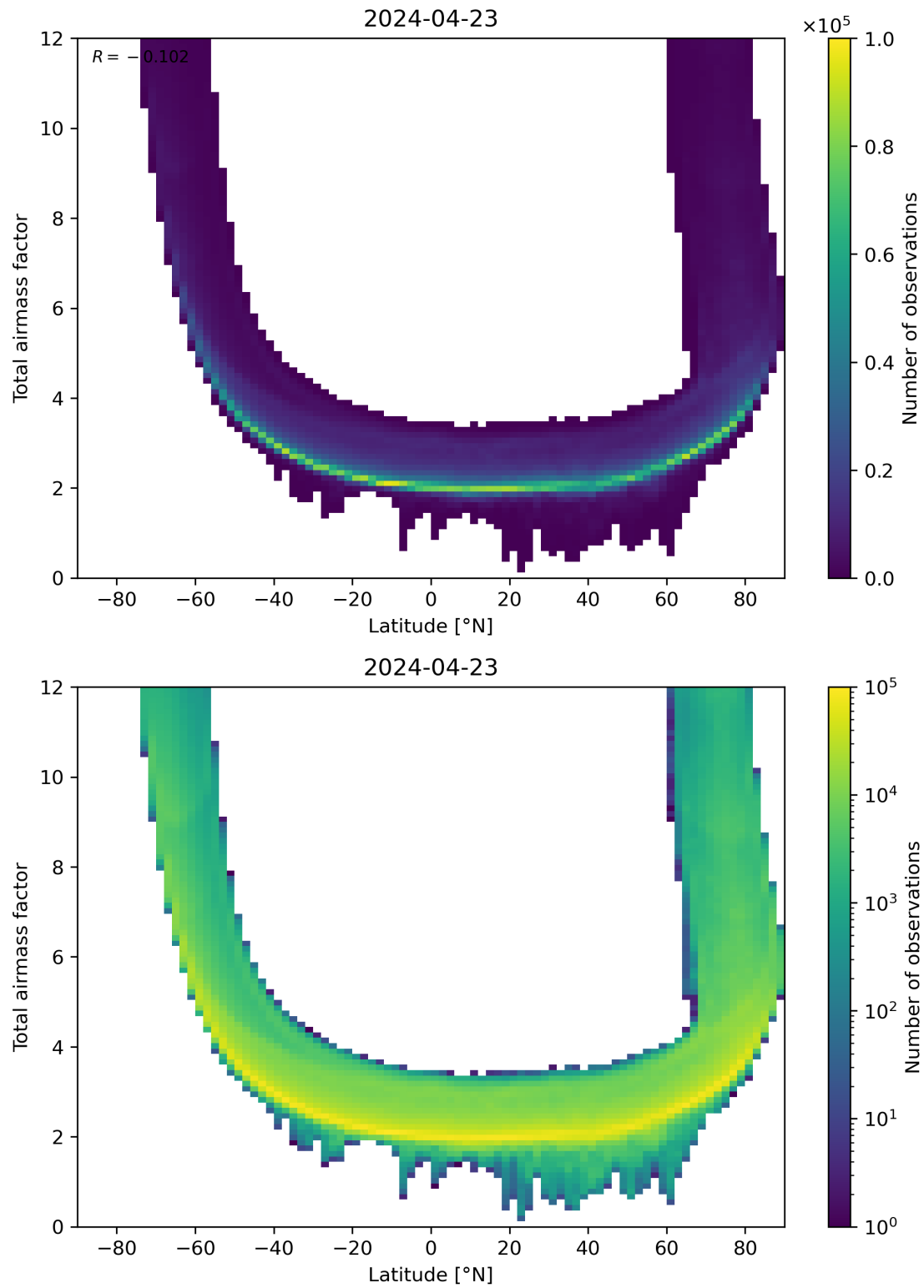
Figure 84: Scatter density plot of “Latitude” against “Total airmass factor” for 2024-04-22 to 2024-04-24.
