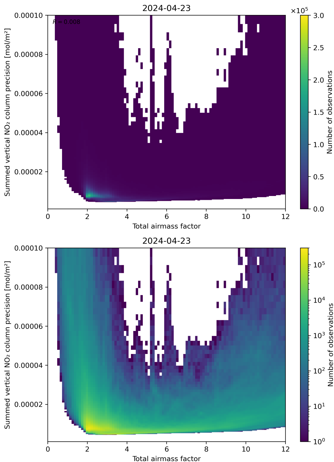
Figure 66: Scatter density plot of “Total airmass factor” against “Summed vertical NO 2 column precision” for 2024-04-22 to 2024-04-24.
