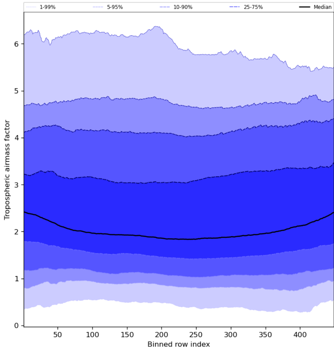
Figure 48: Along track statistics of “Tropospheric airmass factor” for 2024-04-22 to 2024-04-24
