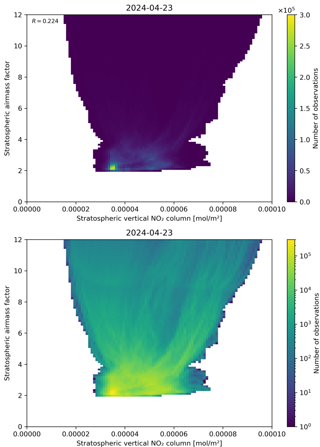
Figure 96: Scatter density plot of “Stratospheric vertical NO 2 column” against “Stratospheric airmass factor” for 2024-04-22 to 2024-04-24.
