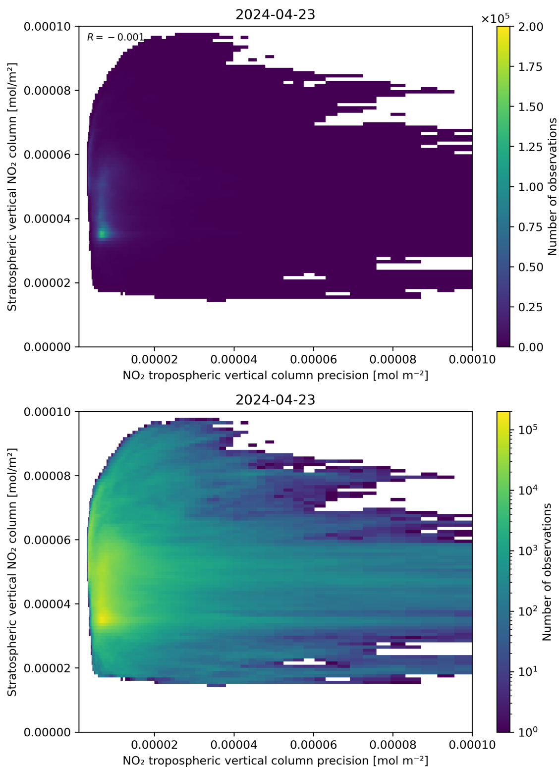
Figure 135: Scatter density plot of “NO 2 tropospheric vertical column precision” against “Stratospheric vertical NO 2 column” for 2024-04-22 to 2024-04-24.
