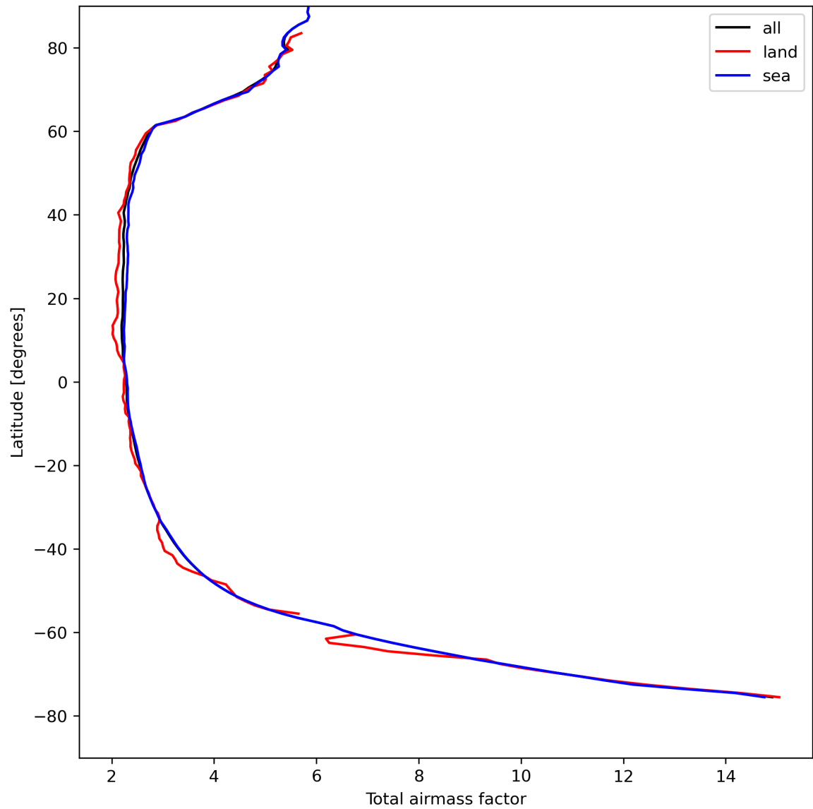
Figure 15: Zonal average of “Total airmass factor” for 2024-04-22 to 2024-04-24.
