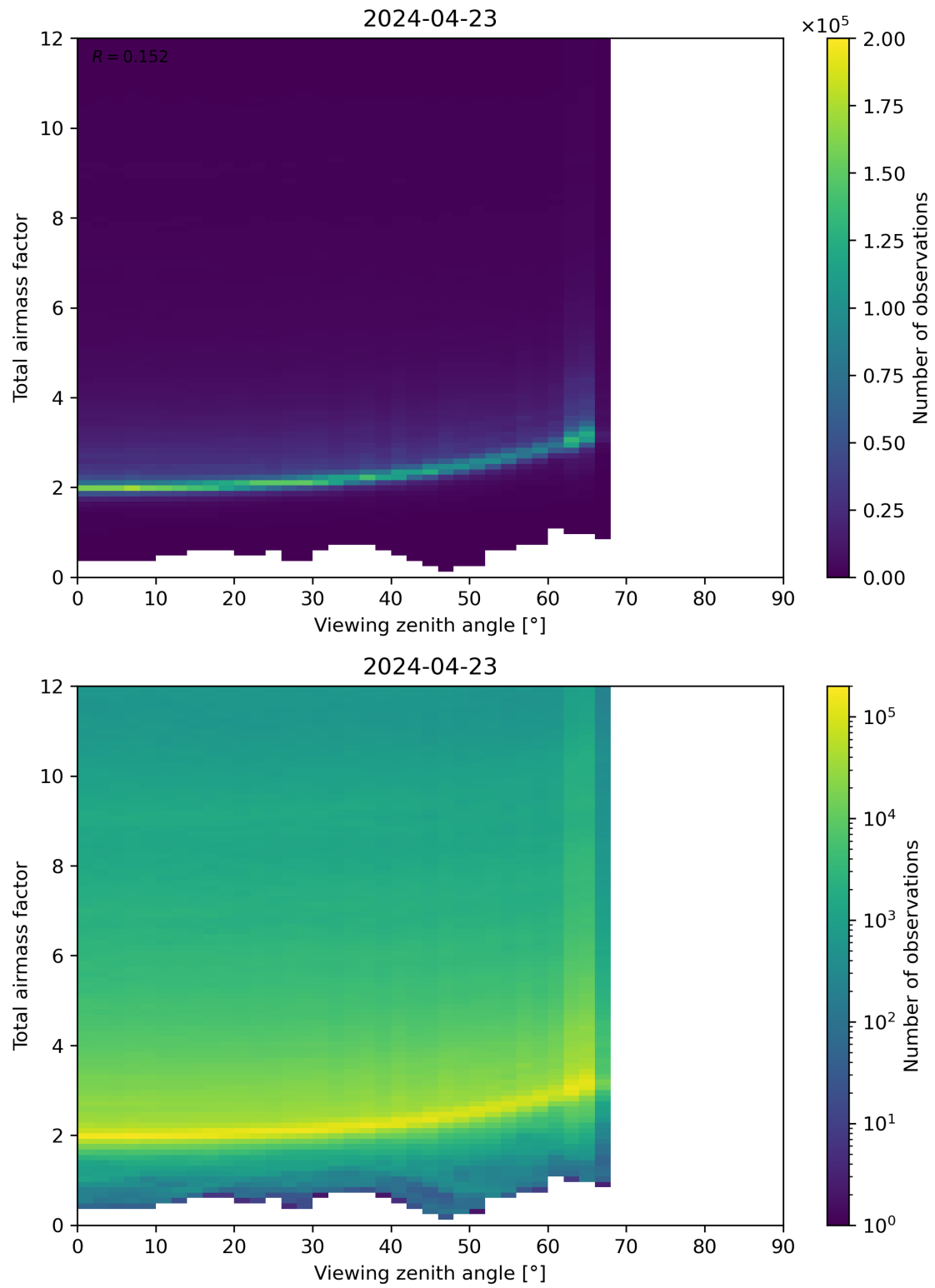
Figure 160: Scatter density plot of “Viewing zenith angle” against “Total airmass factor” for 2024-04-22 to 2024-04-24.
