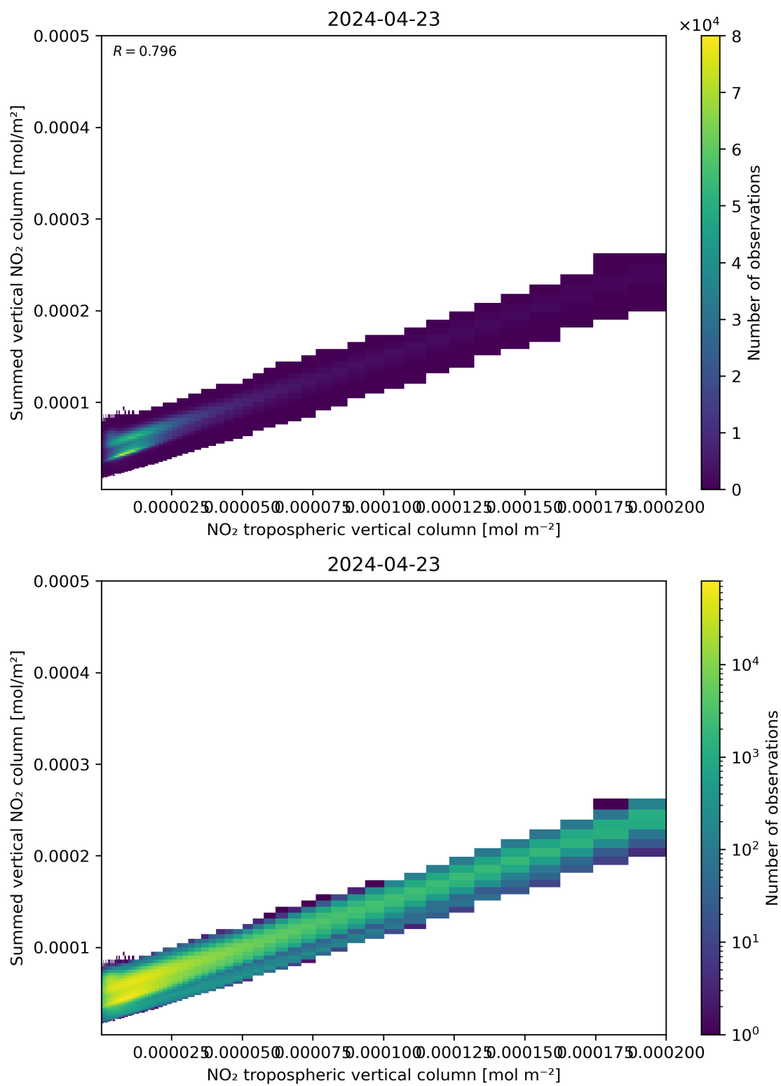
Figure 126: Scatter density plot of “NO 2 tropospheric vertical column” against “Summed vertical NO 2 column” for 2024-04-22 to 2024-04-24.
