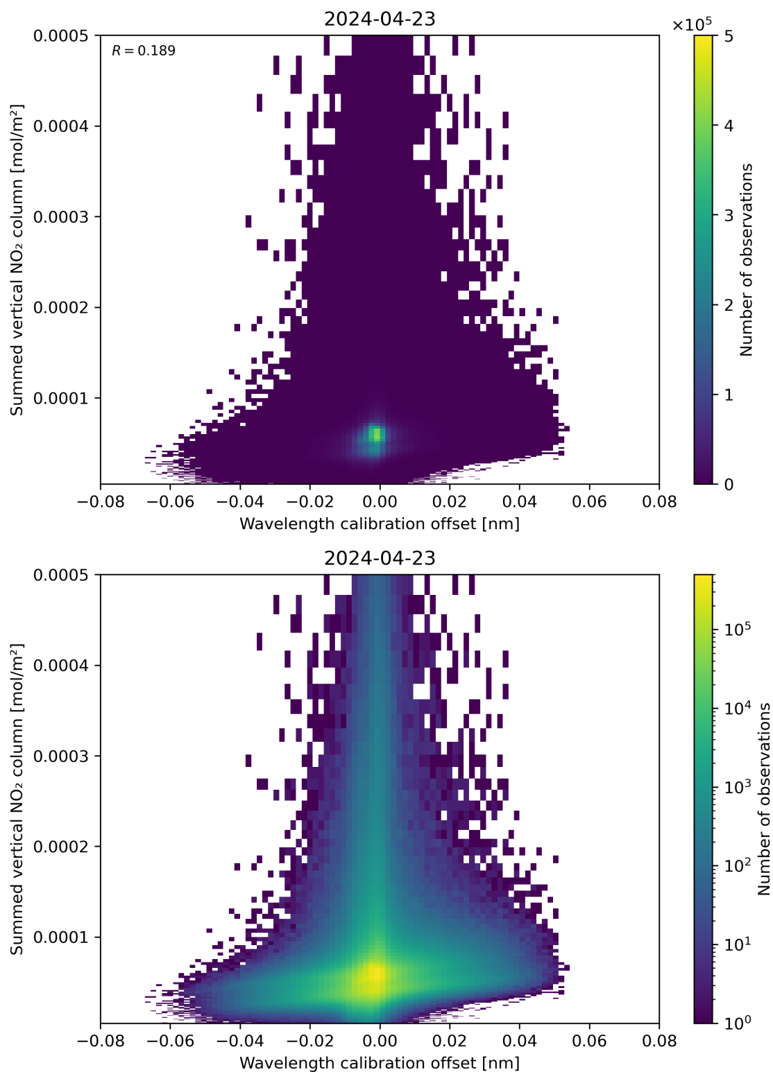
Figure 177: Scatter density plot of “Wavelength calibration offset” against “Summed vertical NO 2 column” for 2024-04-22 to 2024-04-24.
