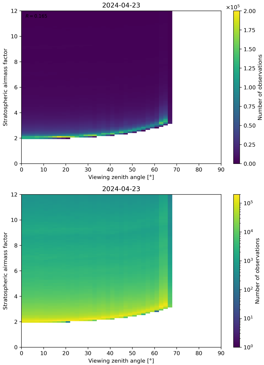
Figure 159: Scatter density plot of “Viewing zenith angle” against “Stratospheric airmass factor” for 2024-04-22 to 2024-04-24.
