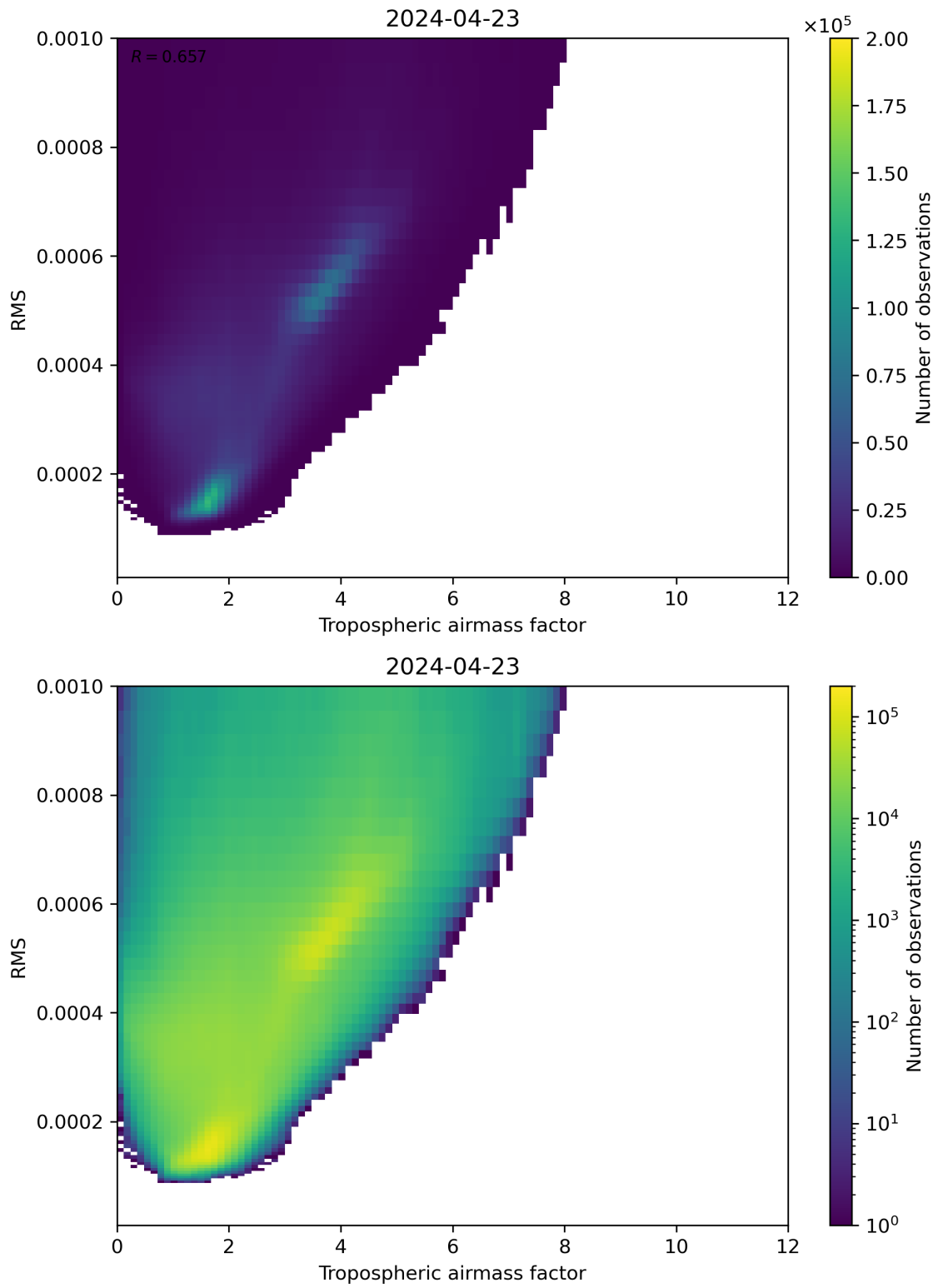
Figure 79: Scatter density plot of “Tropospheric airmass factor” against “RMS” for 2024-04-22 to 2024-04-24.
