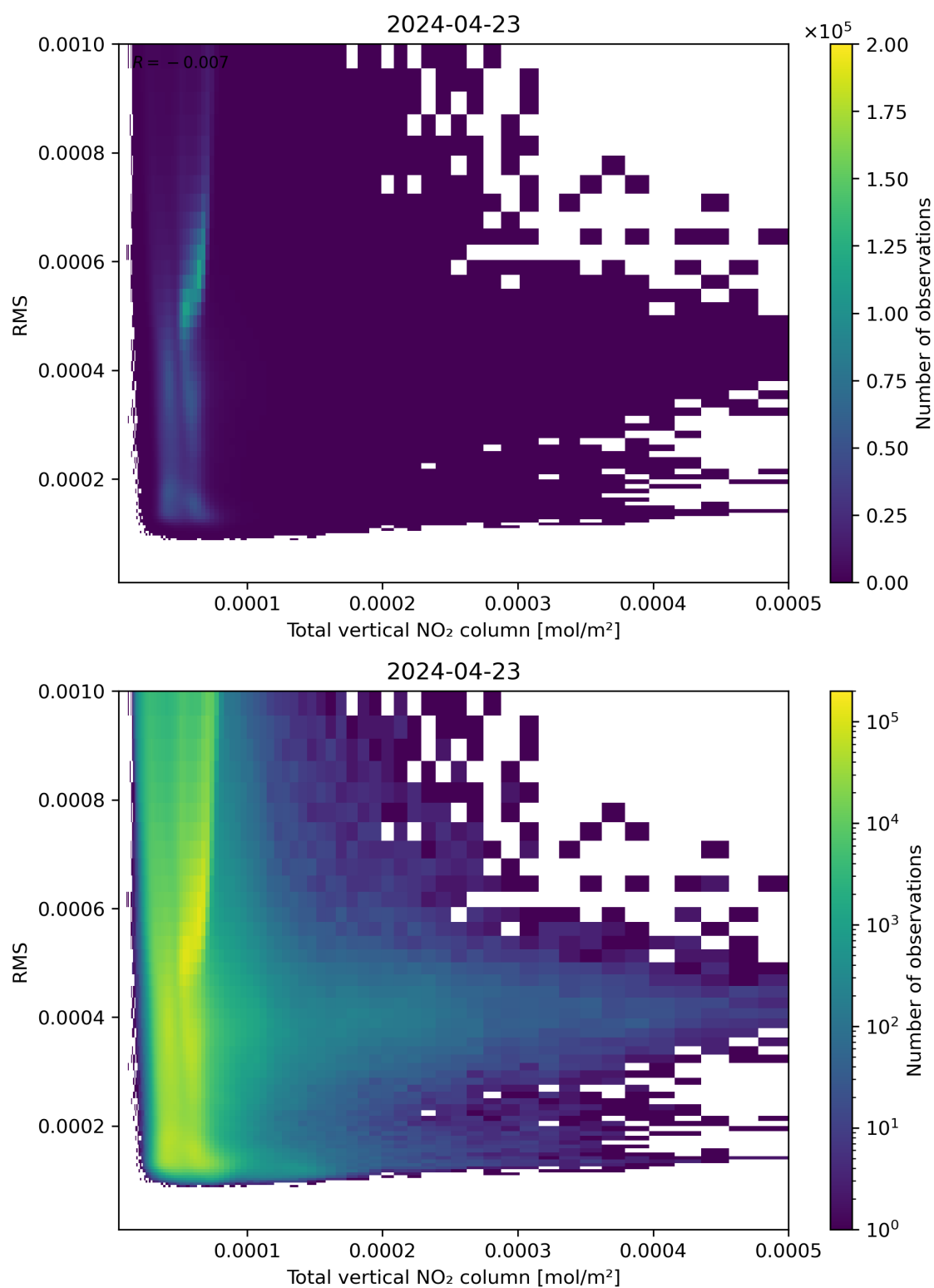
Figure 120: Scatter density plot of “Total vertical NO 2 column” against “RMS” for 2024-04-22 to 2024-04-24.
