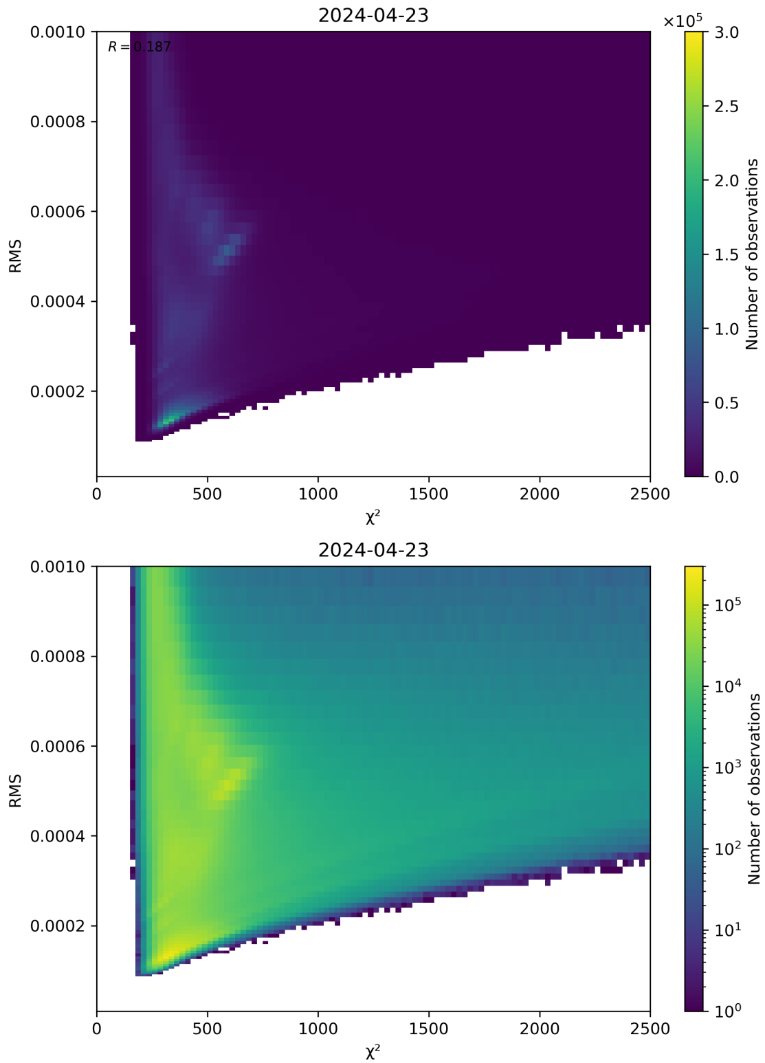
Figure 82: Scatter density plot of “ \chi^2 ” against “RMS” for 2024-04-22 to 2024-04-24.
