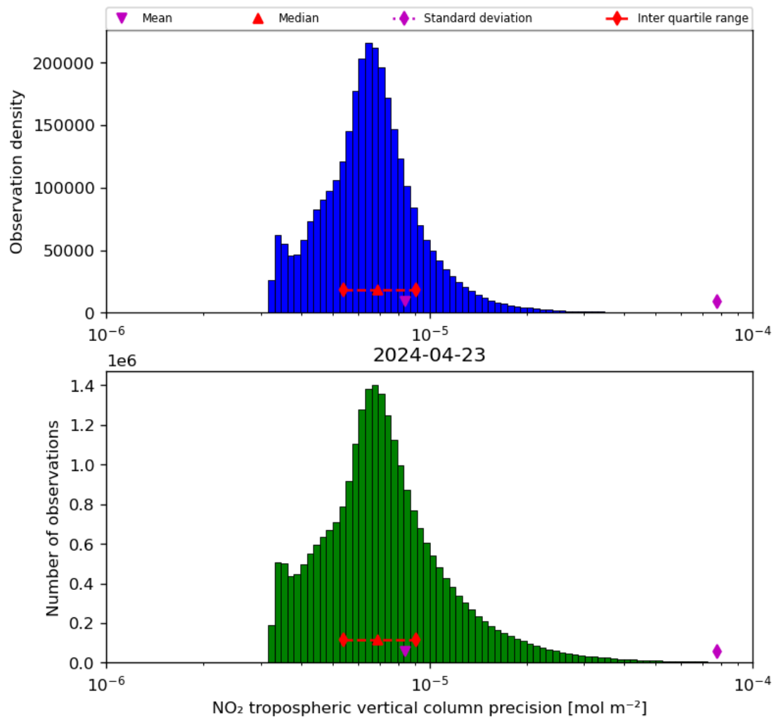
Figure 30: Histogram of “NO 2 tropospheric vertical column precision” for 2024-04-22 to 2024-04-24
