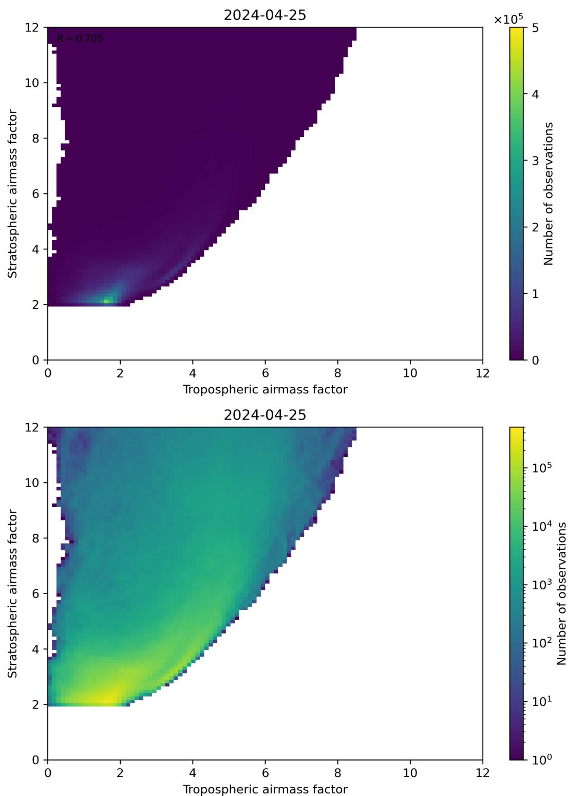
Figure 71: Scatter density plot of “Tropospheric airmass factor” against “Stratospheric airmass factor” for 2024-04-24 to 2024-04-26.
