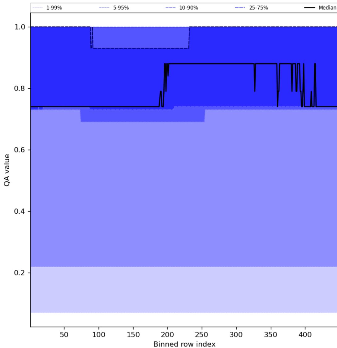
Figure 45: Along track statistics of “QA value” for 2024-04-24 to 2024-04-26
