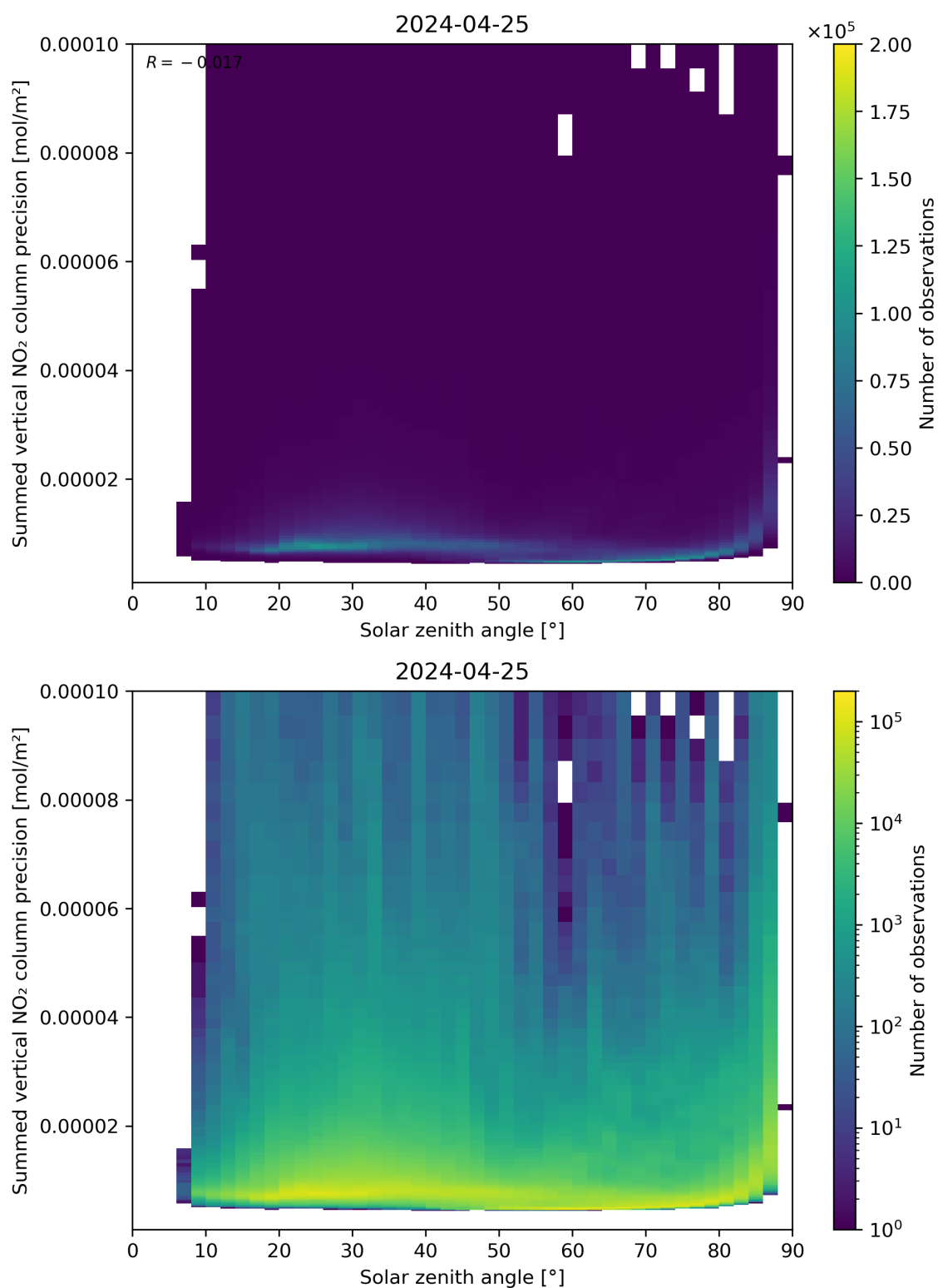
Figure 152: Scatter density plot of “Solar zenith angle” against “Summed vertical NO 2 column precision” for 2024-04-24 to 2024-04-26.
