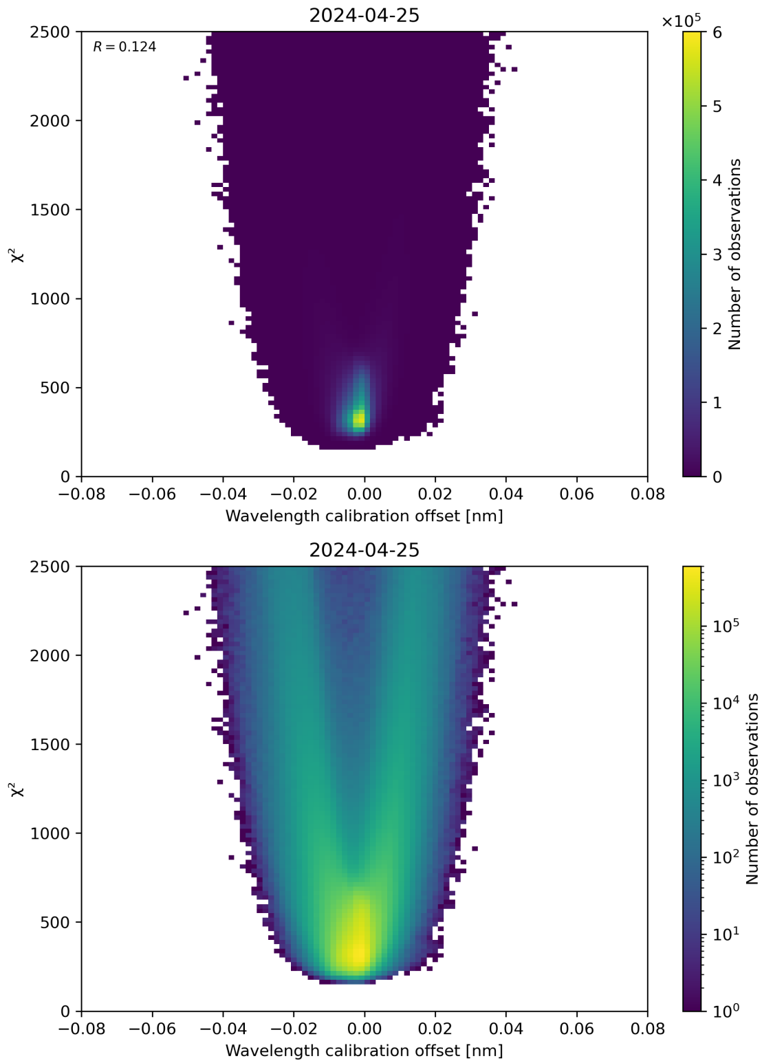
Figure 175: Scatter density plot of “Wavelength calibration offset” against “ \chi^2 ” for 2024-04-24 to 2024-04-26.
