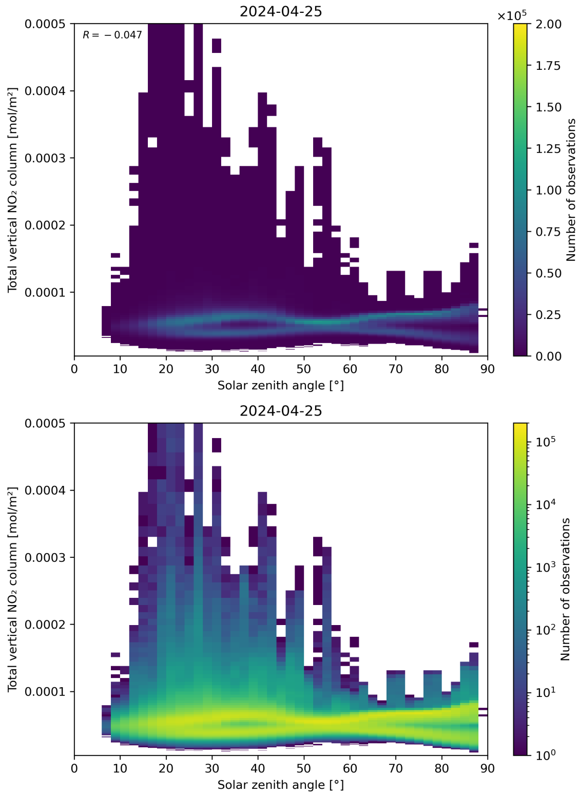
Figure 153: Scatter density plot of “Solar zenith angle” against “Total vertical NO 2 column” for 2024-04-24 to 2024-04-26.
