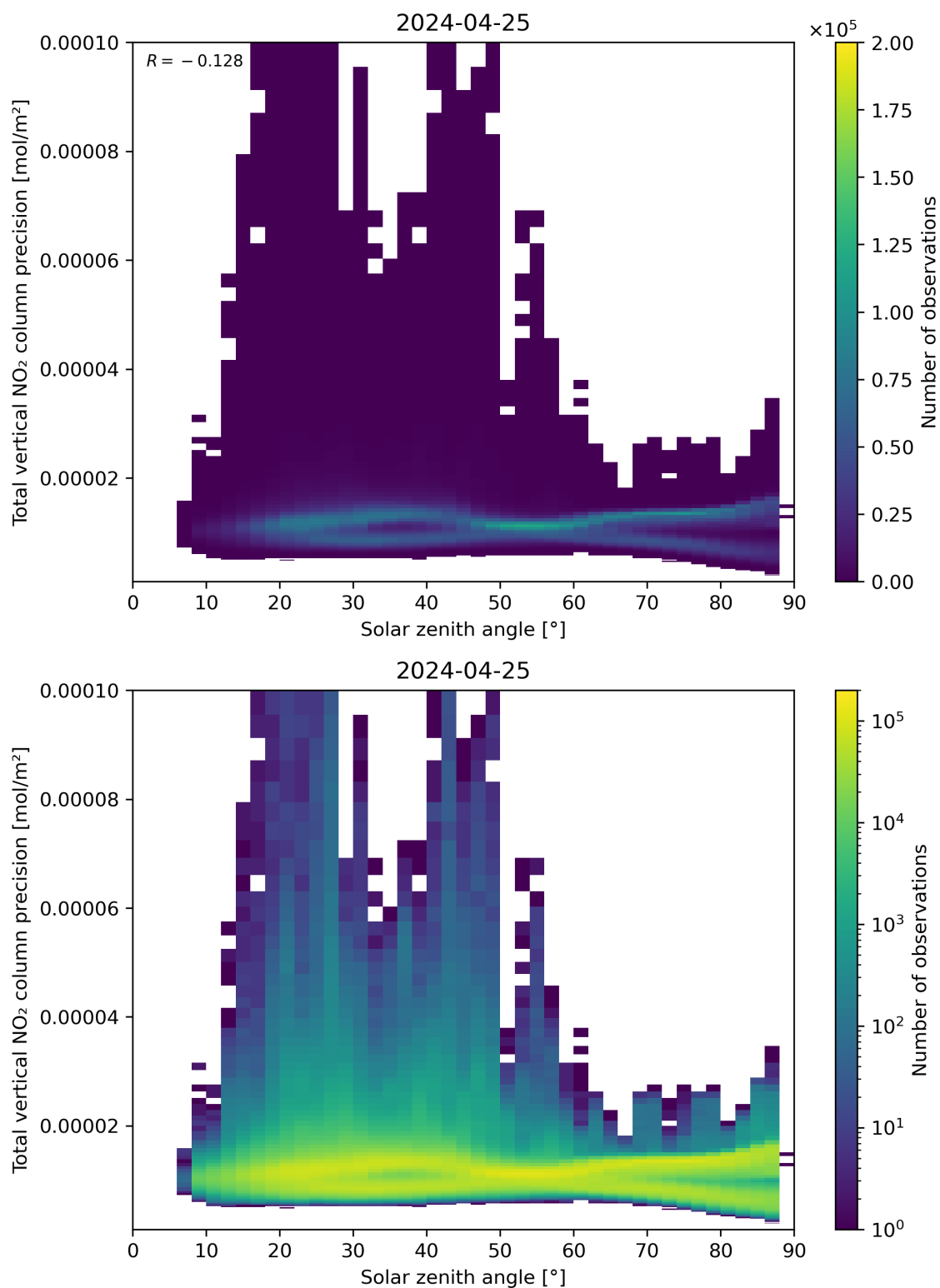
Figure 154: Scatter density plot of “Solar zenith angle” against “Total vertical NO 2 column precision” for 2024-04-24 to 2024-04-26.
