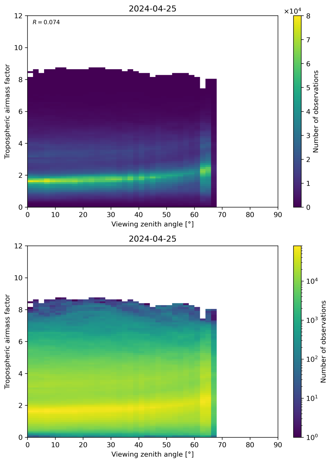
Figure 161: Scatter density plot of “Viewing zenith angle” against “Tropospheric airmass factor” for 2024-04-24 to 2024-04-26.
