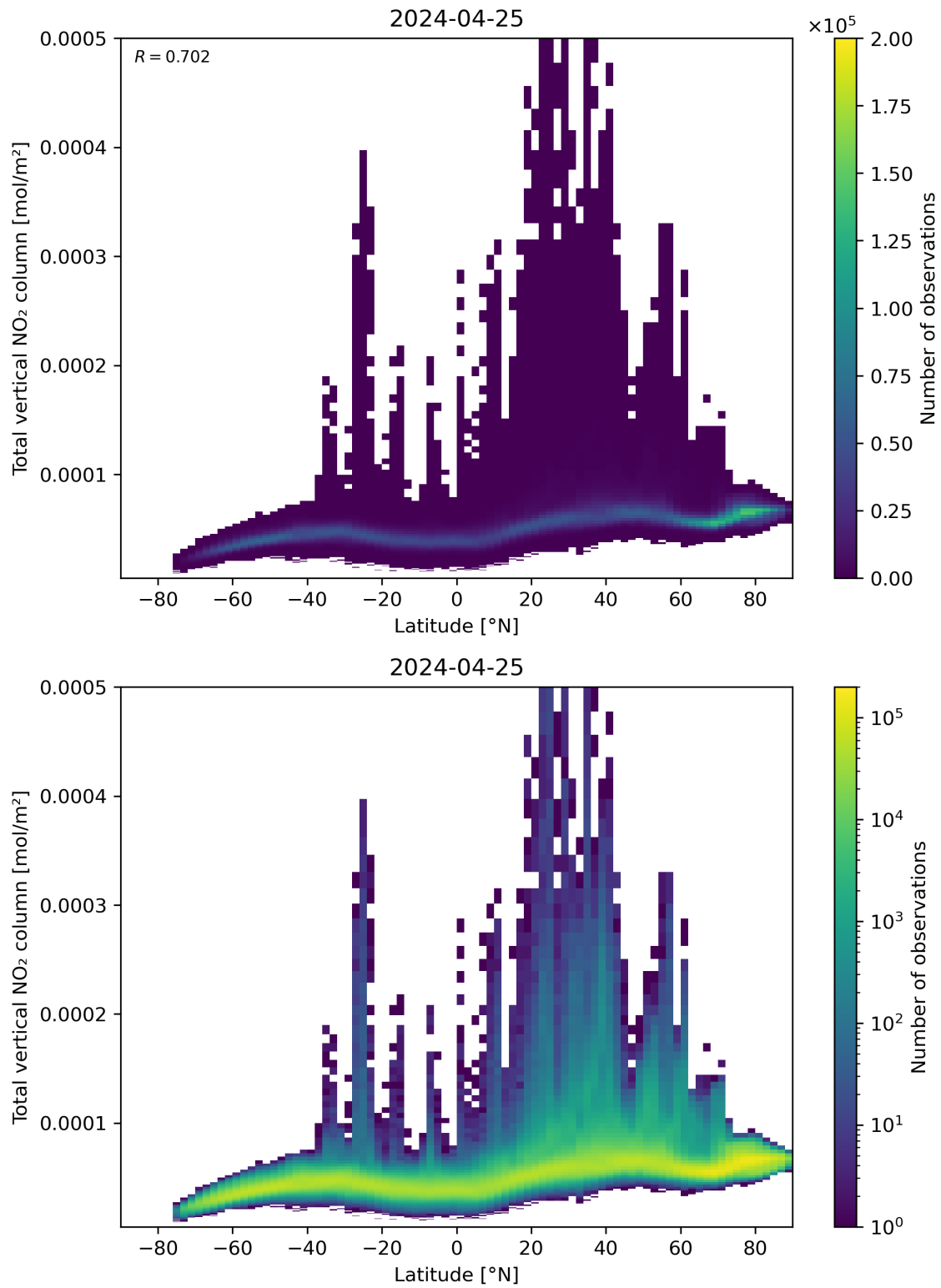
Figure 90: Scatter density plot of “Latitude” against “Total vertical NO 2 column” for 2024-04-24 to 2024-04-26.
