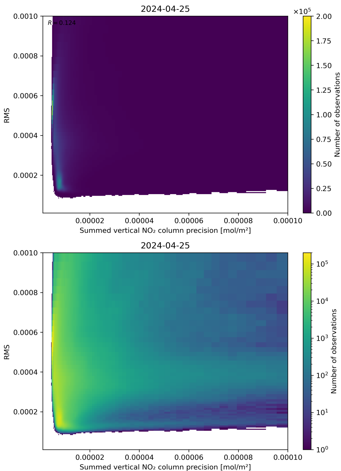
Figure 108: Scatter density plot of “Summed vertical NO 2 column precision” against “RMS” for 2024-04-24 to 2024-04-26.
