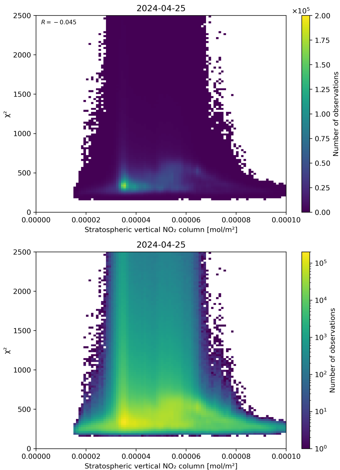
Figure 97: Scatter density plot of “Stratospheric vertical NO 2 column” against “ \chi^2 ” for 2024-04-24 to 2024-04-26.
