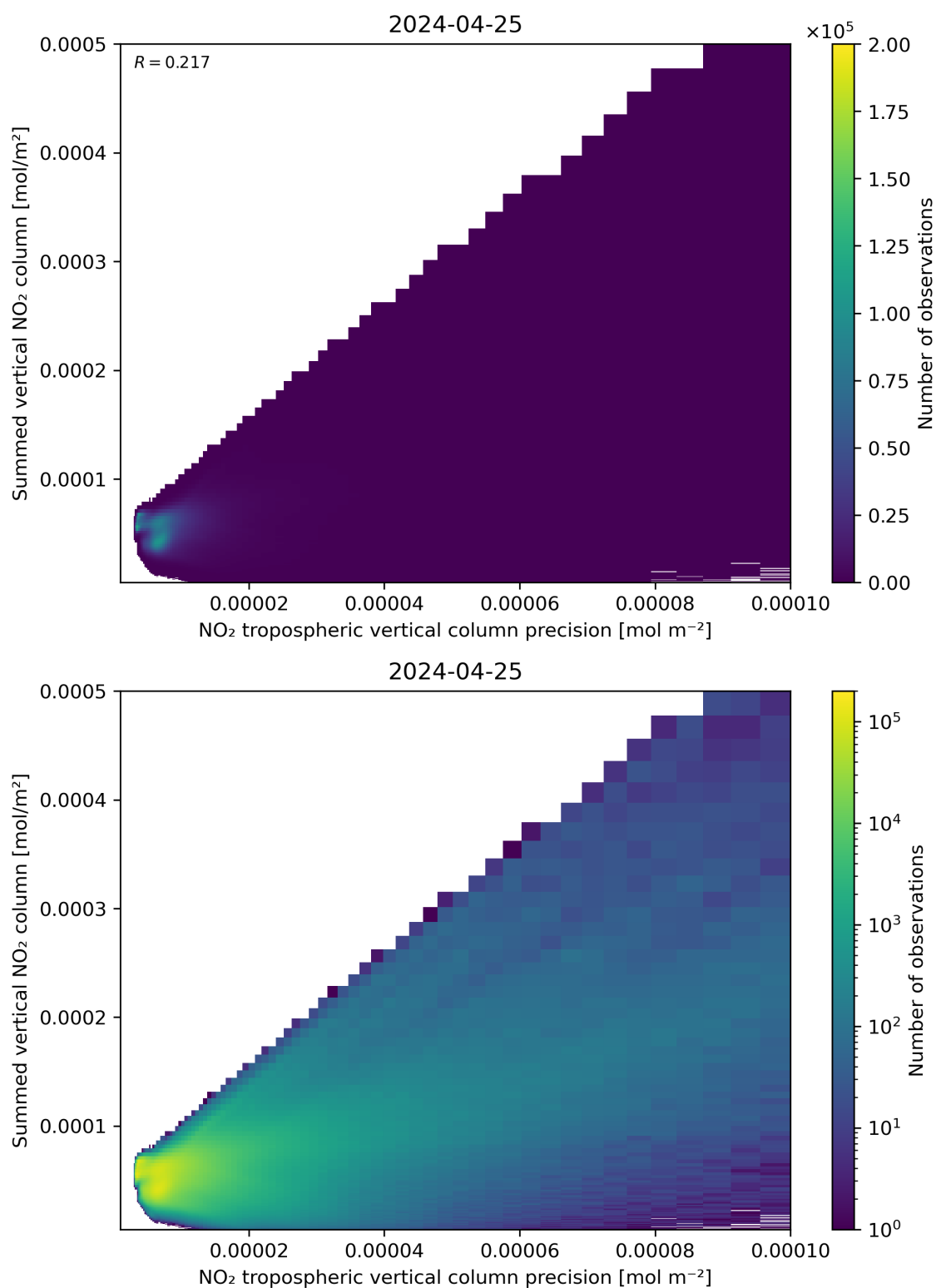
Figure 136: Scatter density plot of “NO 2 tropospheric vertical column precision” against “Summed vertical NO 2 column” for 2024-04-24 to 2024-04-26.
