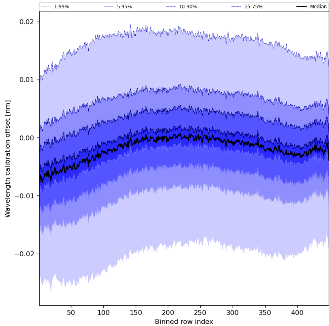
Figure 52: Along track statistics of “Wavelength calibration offset” for 2024-04-24 to 2024-04-26
