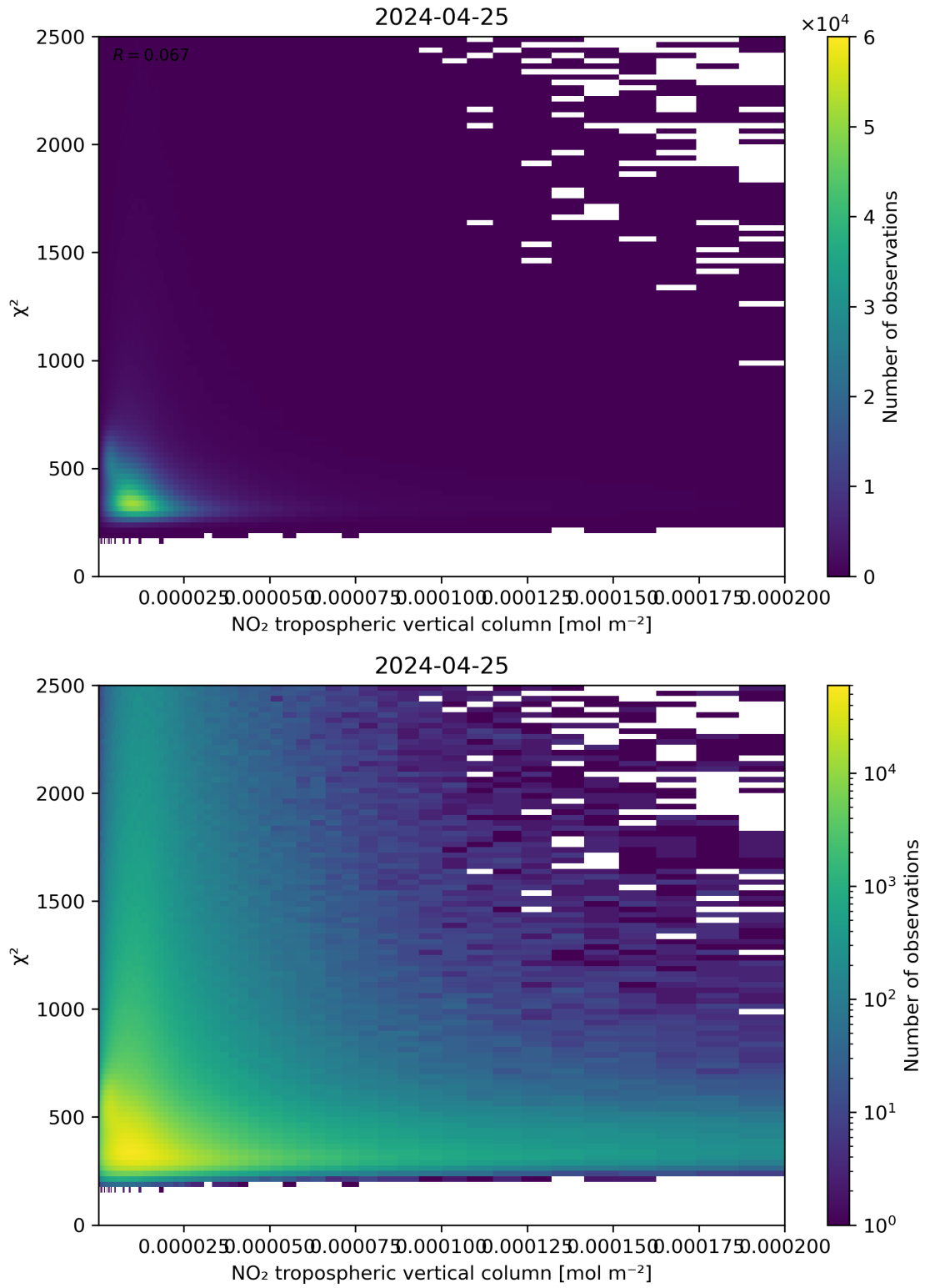
Figure 124: Scatter density plot of “NO 2 tropospheric vertical column” against “ \chi^2 ” for 2024-04-24 to 2024-04-26.
