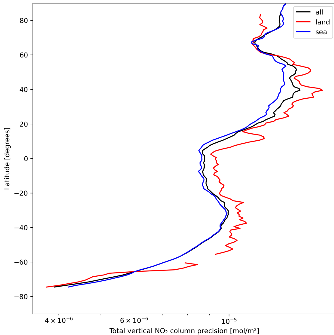
Figure 22: Zonal average of “Total vertical NO 2 column precision” for 2024-04-24 to 2024-04-26.
