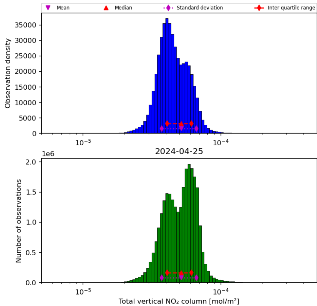
Figure 38: Histogram of “Total vertical NO 2 column” for 2024-04-24 to 2024-04-26
