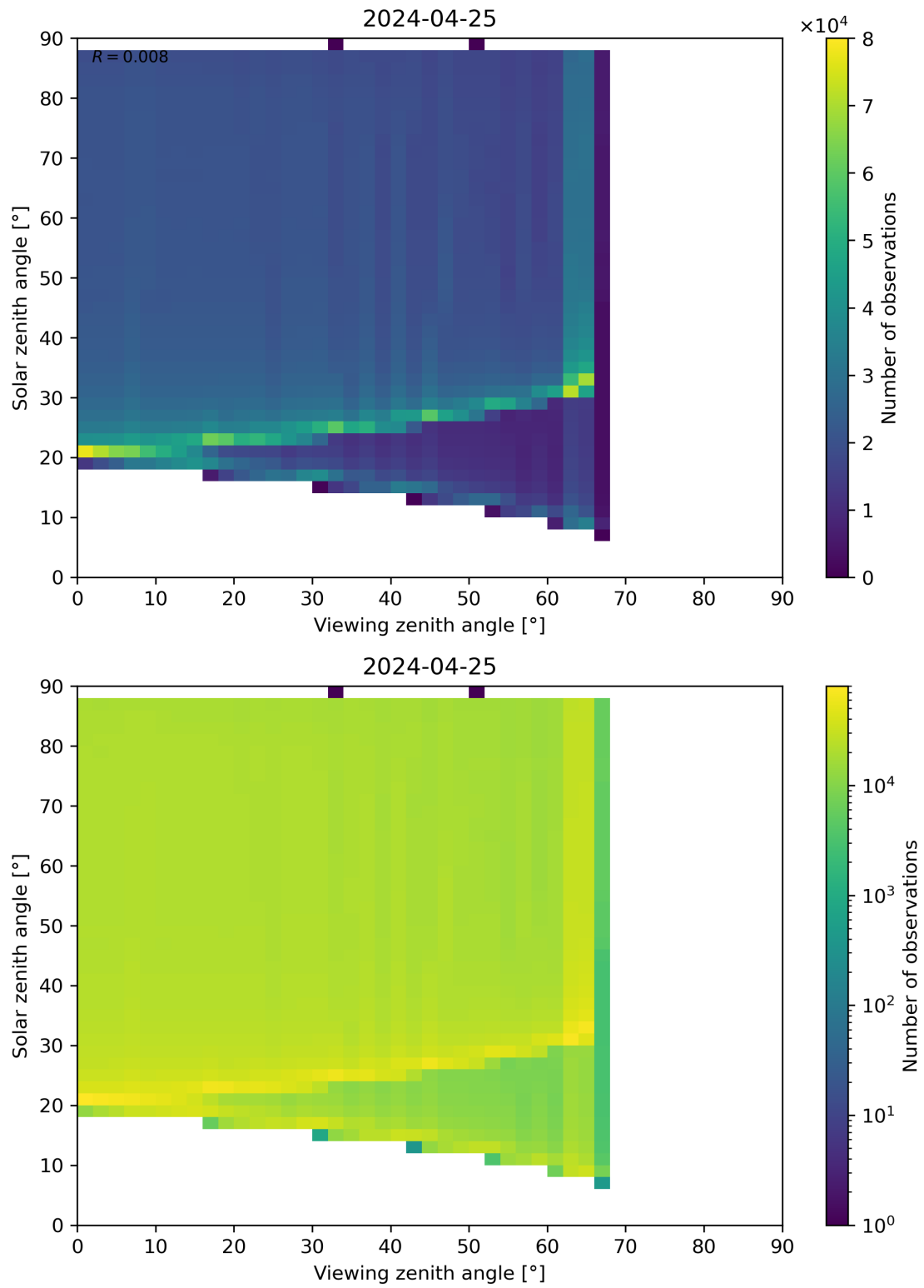
Figure 172: Scatter density plot of “Viewing zenith angle” against “Solar zenith angle” for 2024-04-24 to 2024-04-26.
