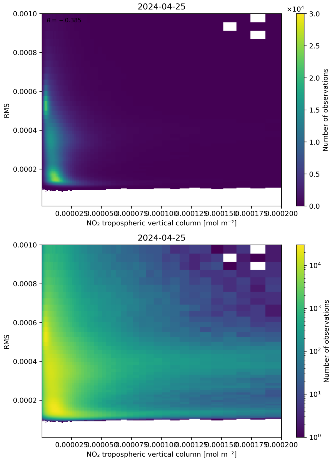
Figure 142: Scatter density plot of “NO 2 tropospheric vertical column” against “RMS” for 2024-04-24 to 2024-04-26.
