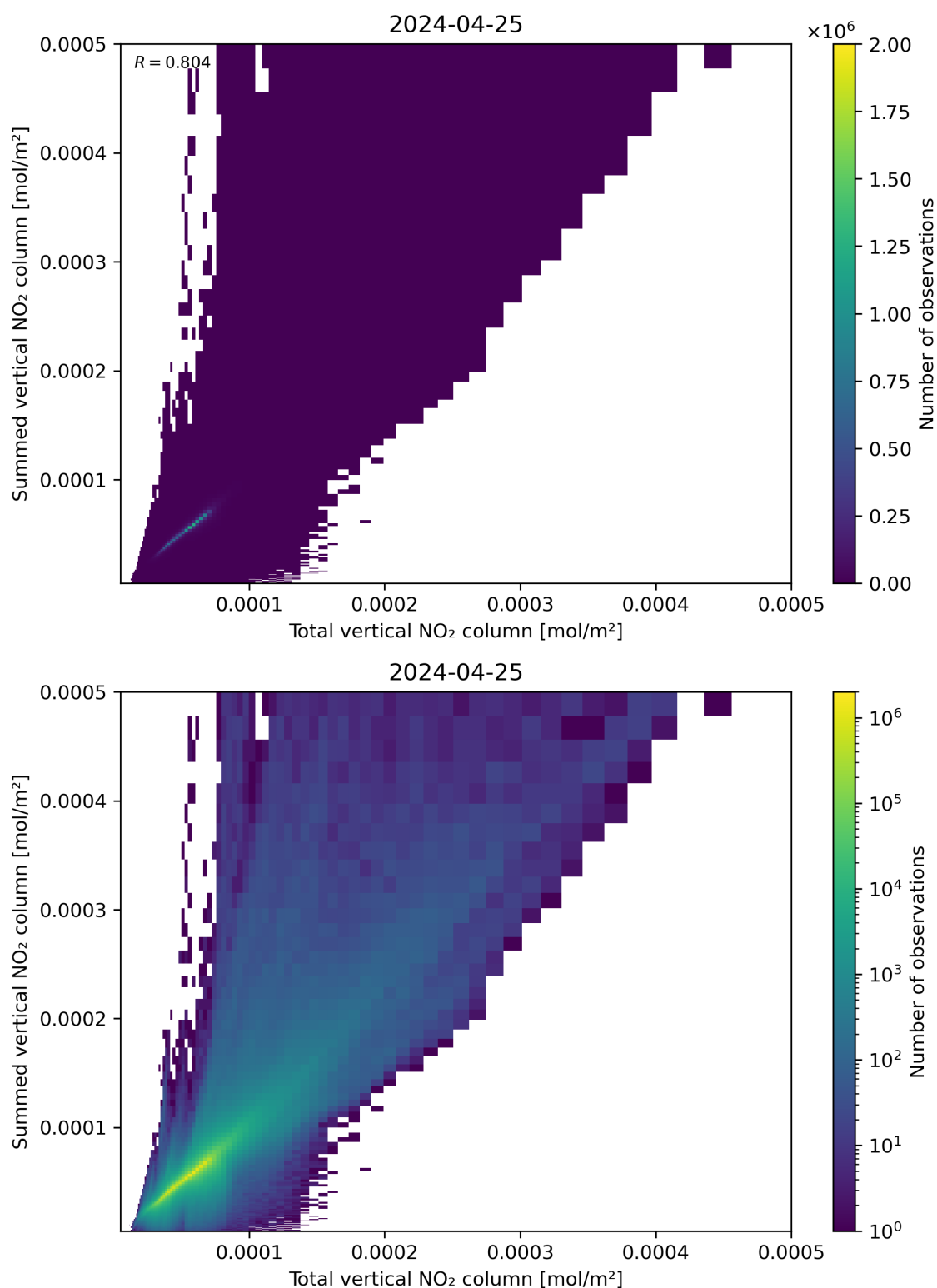
Figure 112: Scatter density plot of “Total vertical NO 2 column” against “Summed vertical NO 2 column” for 2024-04-24 to 2024-04-26.
