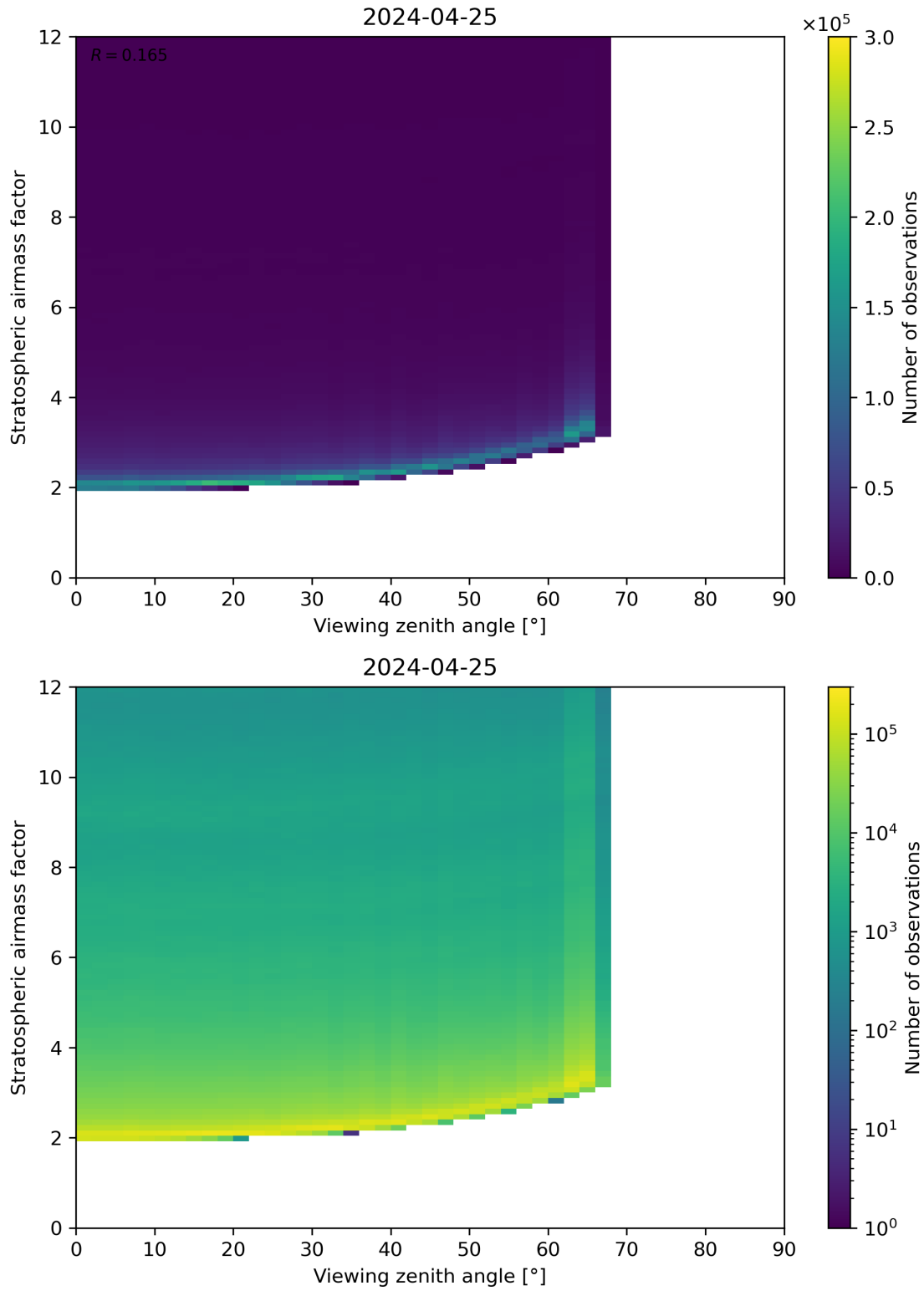
Figure 159: Scatter density plot of “Viewing zenith angle” against “Stratospheric airmass factor” for 2024-04-24 to 2024-04-26.
