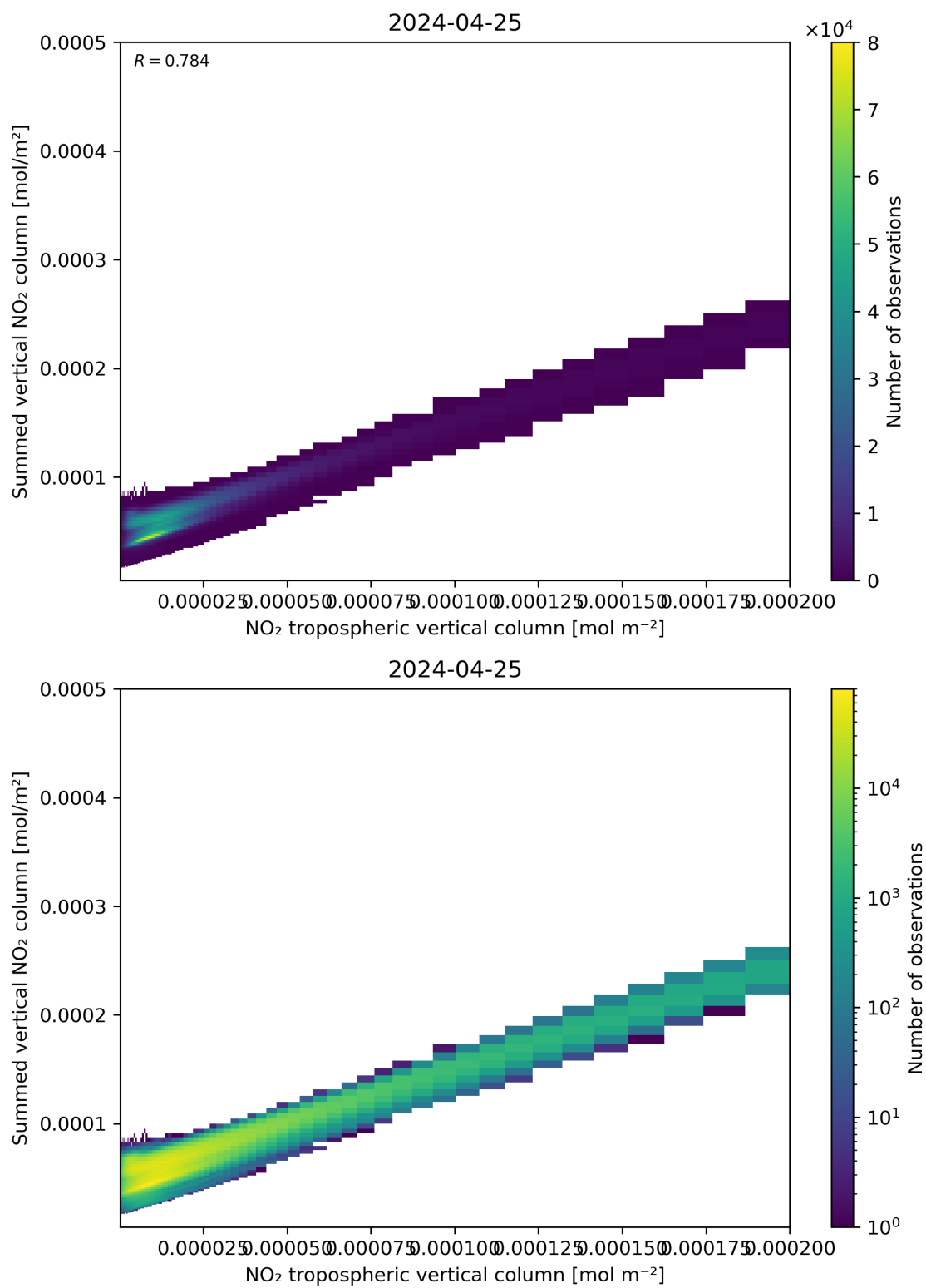
Figure 126: Scatter density plot of “NO 2 tropospheric vertical column” against “Summed vertical NO 2 column” for 2024-04-24 to 2024-04-26.
