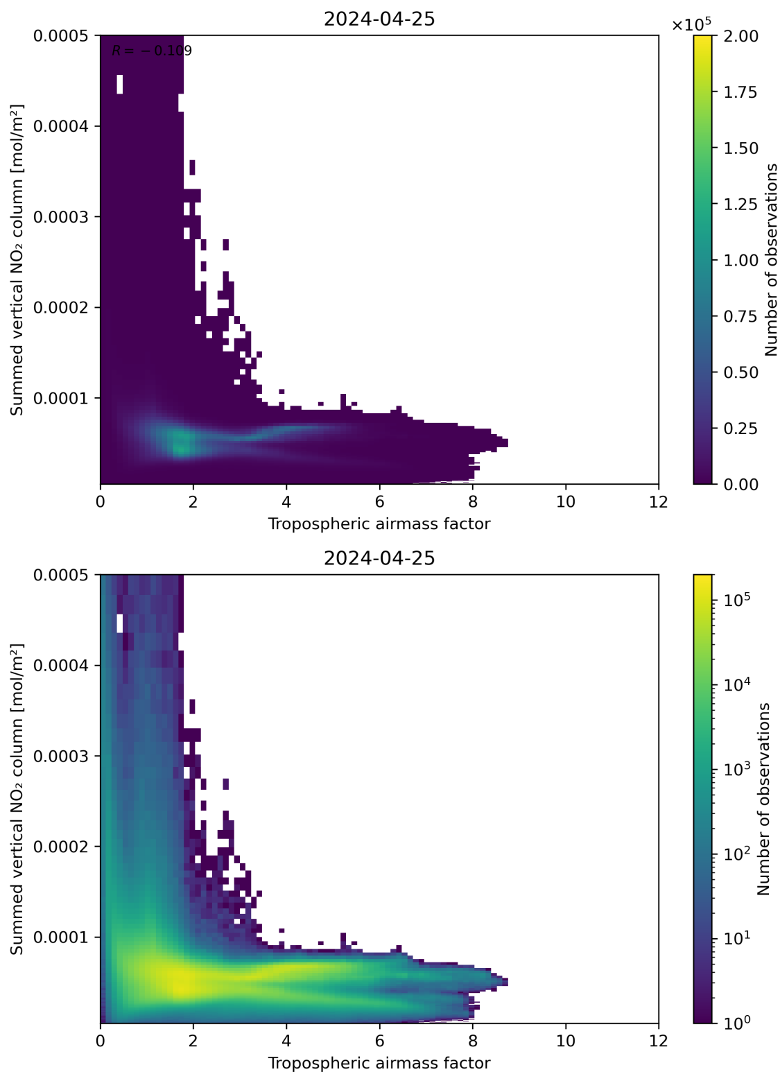
Figure 75: Scatter density plot of “Tropospheric airmass factor” against “Summed vertical NO 2 column” for 2024-04-24 to 2024-04-26.
