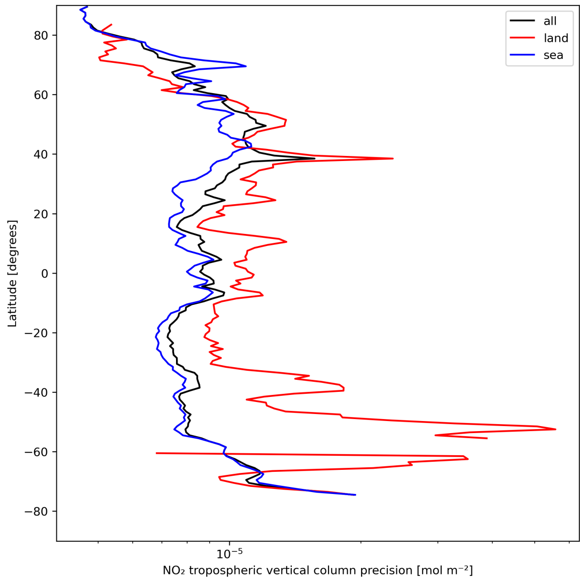
Figure 13: Zonal average of “NO 2 tropospheric vertical column precision” for 2024-04-24 to 2024-04-26.
