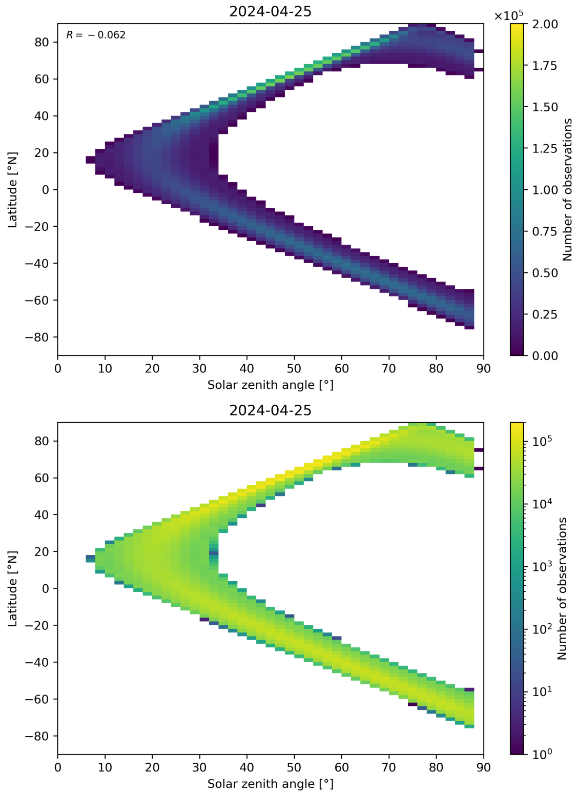
Figure 149: Scatter density plot of “Solar zenith angle” against “Latitude” for 2024-04-24 to 2024-04-26.
