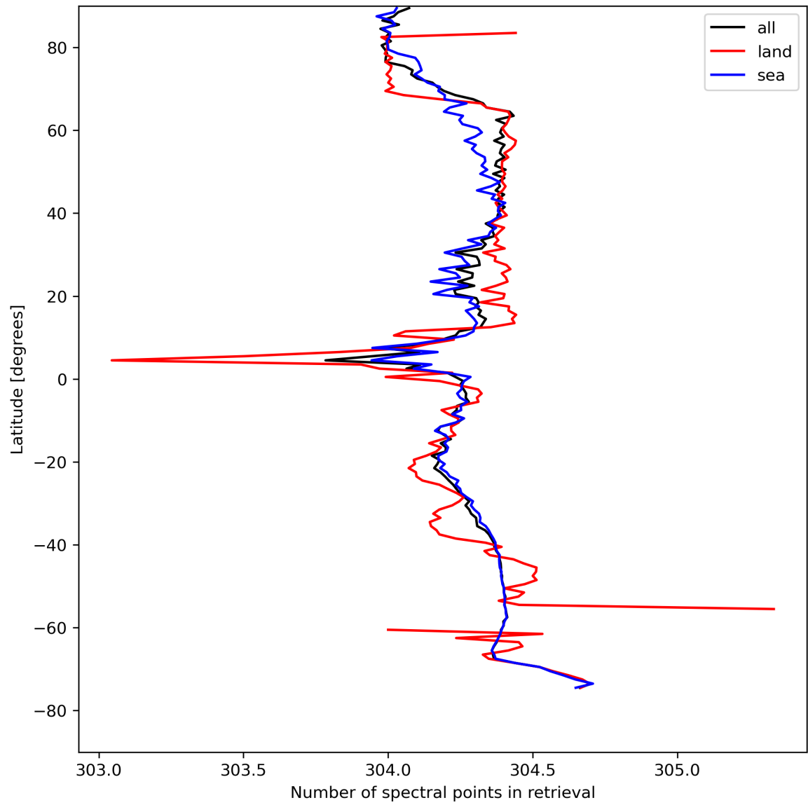
Figure 16: Zonal average of “Number of spectral points in retrieval” for 2024-04-24 to 2024-04-26.
