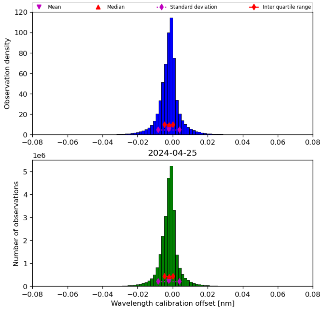
Figure 35: Histogram of “Wavelength calibration offset” for 2024-04-24 to 2024-04-26
