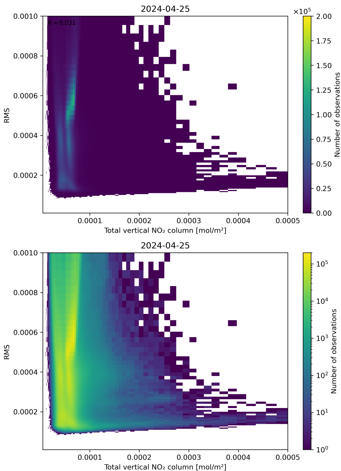
Figure 120: Scatter density plot of “Total vertical NO 2 column” against “RMS” for 2024-04-24 to 2024-04-26.
