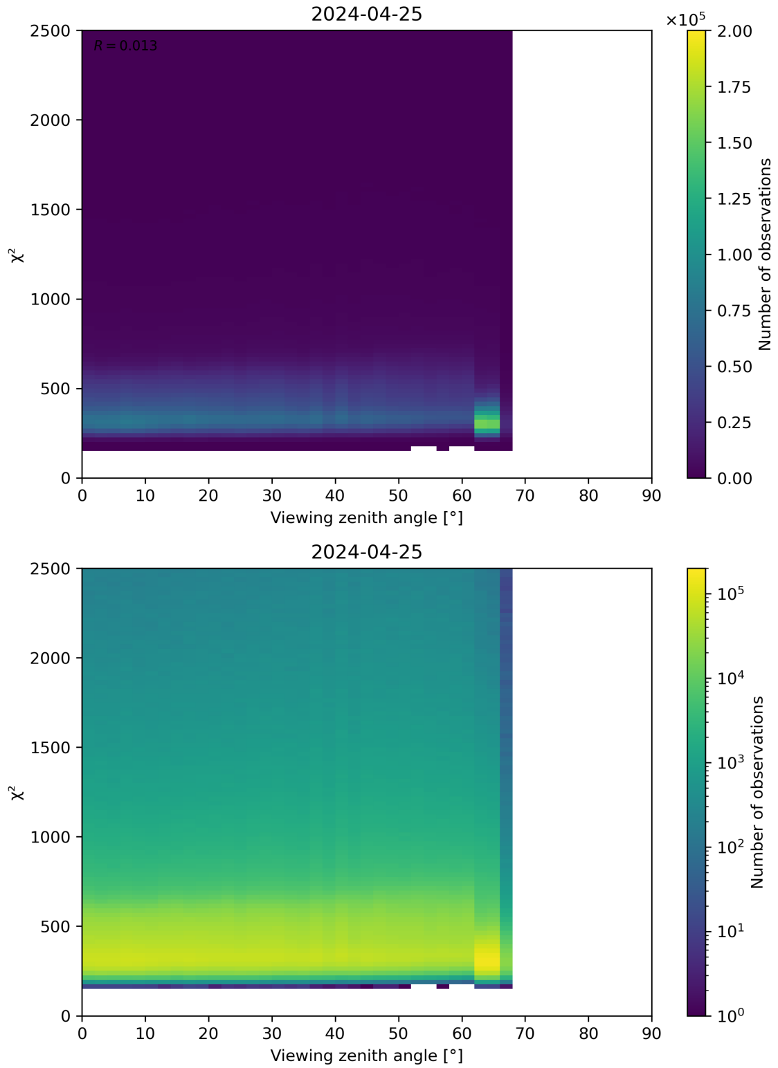
Figure 162: Scatter density plot of “Viewing zenith angle” against “ \chi^2 ” for 2024-04-24 to 2024-04-26.
