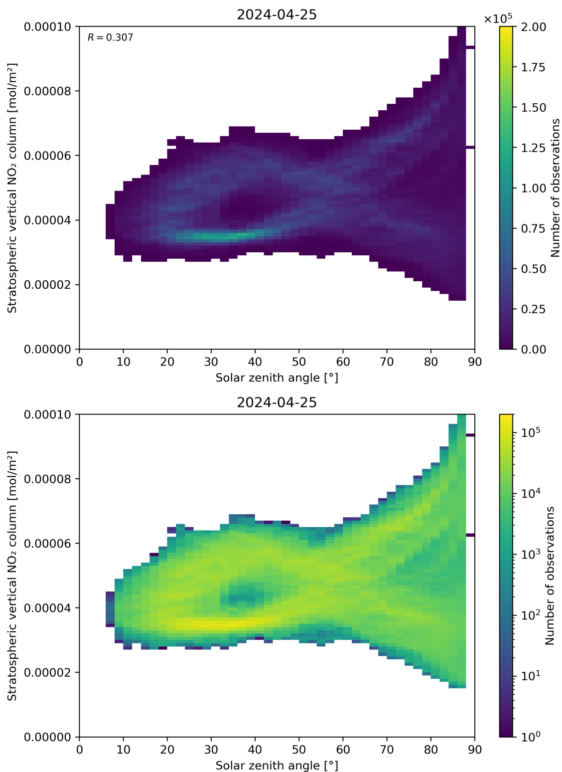
Figure 150: Scatter density plot of “Solar zenith angle” against “Stratospheric vertical NO 2 column” for 2024-04-24 to 2024-04-26.
