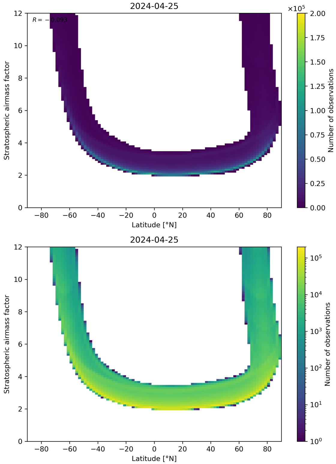
Figure 83: Scatter density plot of “Latitude” against “Stratospheric air mass factor” for 2024-04-24 to 2024-04-26.
