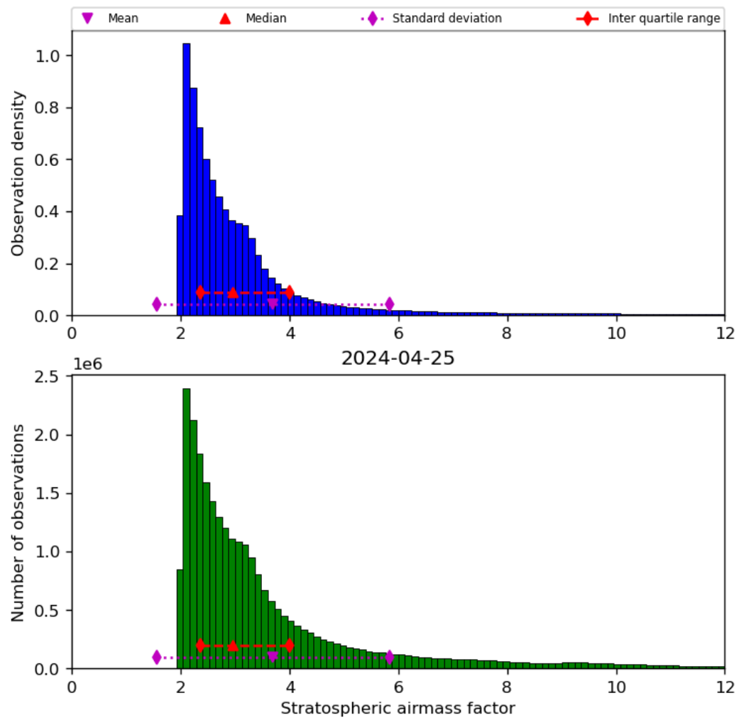
Figure 44: Histogram of “Stratospheric airmass factor” for 2024-04-24 to 2024-04-26
