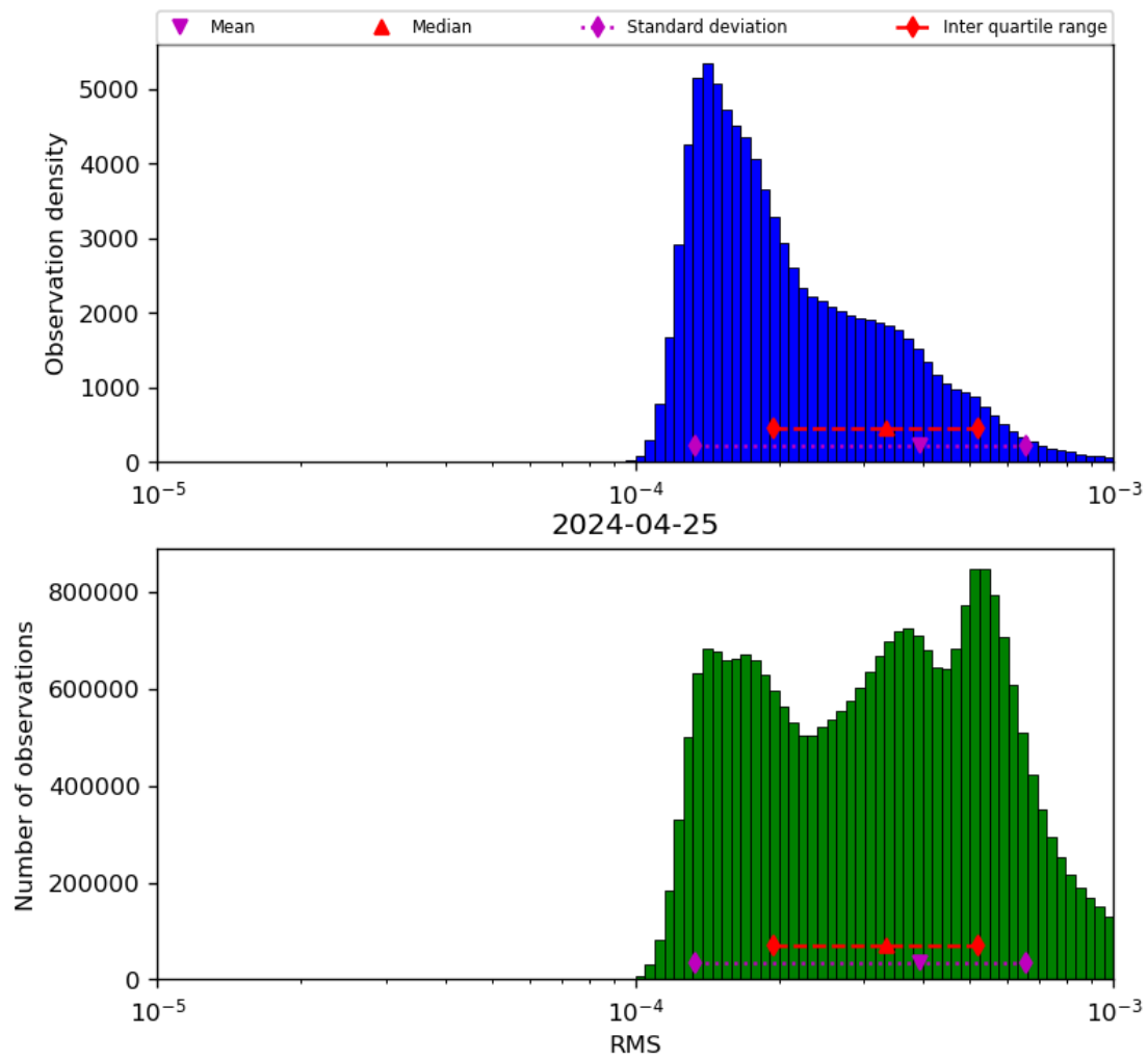
Figure 43: Histogram of “RMS” for 2024-04-24 to 2024-04-26
