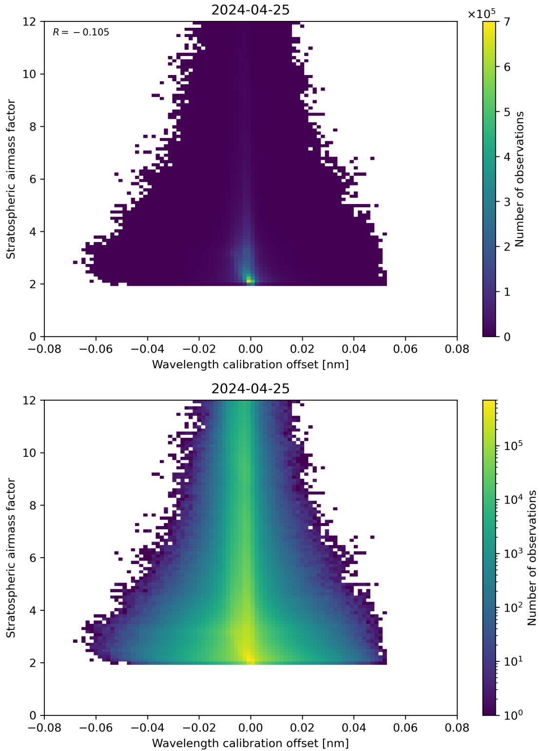
Figure 174: Scatter density plot of “Wavelength calibration offset” against “Stratospheric air mass factor” for 2024-04-24 to 2024-04-26.
