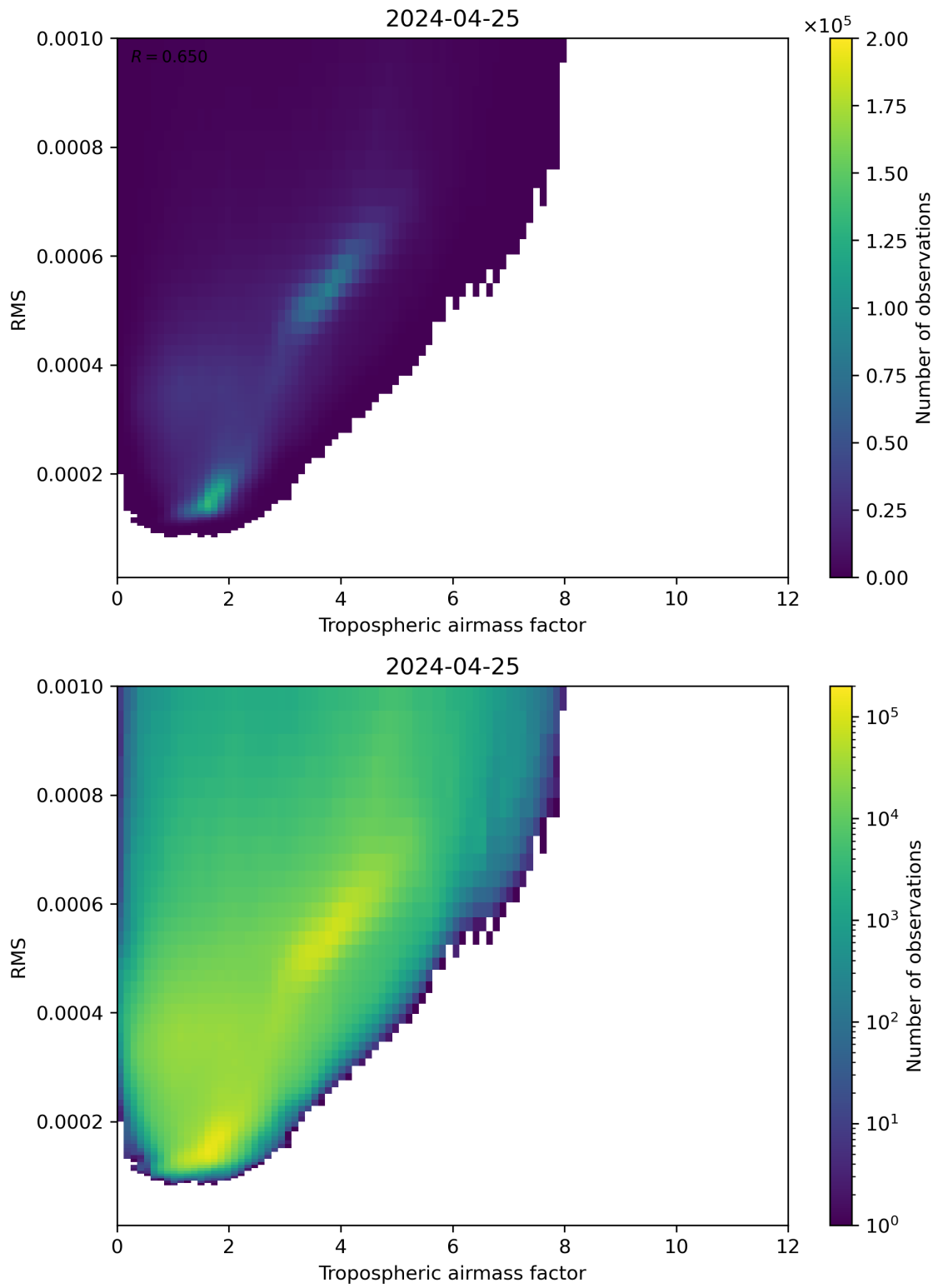
Figure 79: Scatter density plot of “Tropospheric airmass factor” against “RMS” for 2024-04-24 to 2024-04-26.
