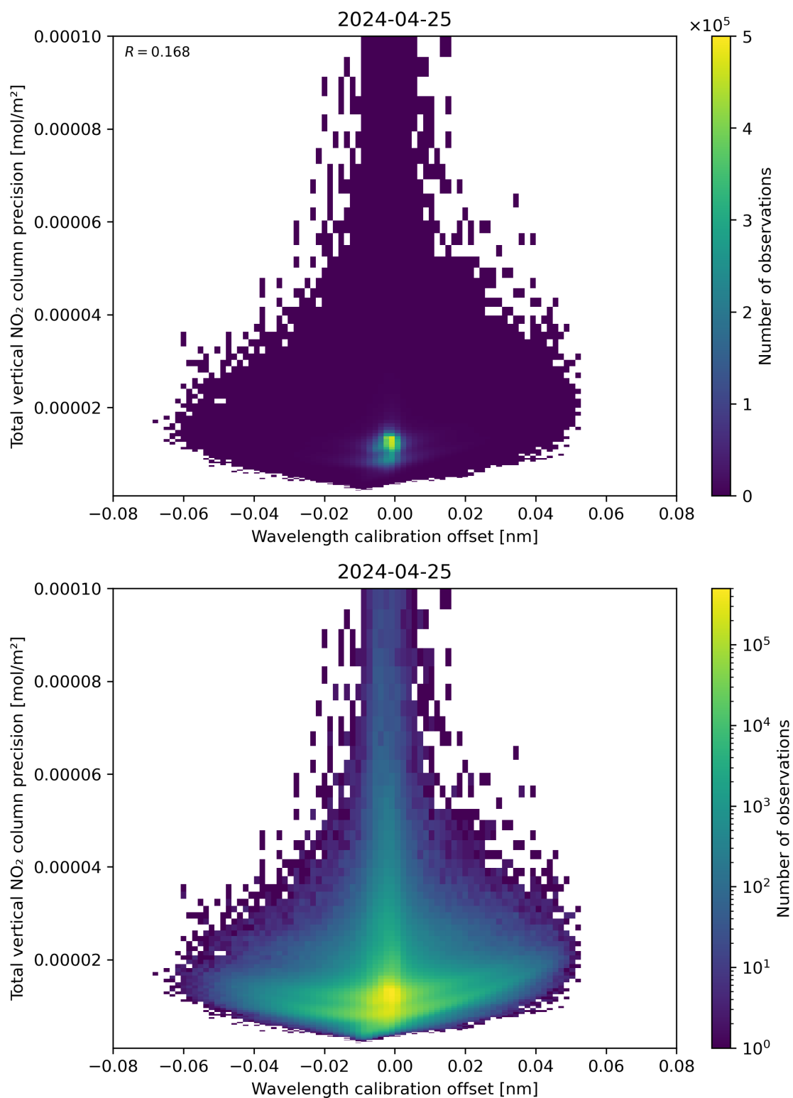
Figure 180: Scatter density plot of “Wavelength calibration offset” against “Total vertical NO 2 column precision” for 2024-04-24 to 2024-04-26.
