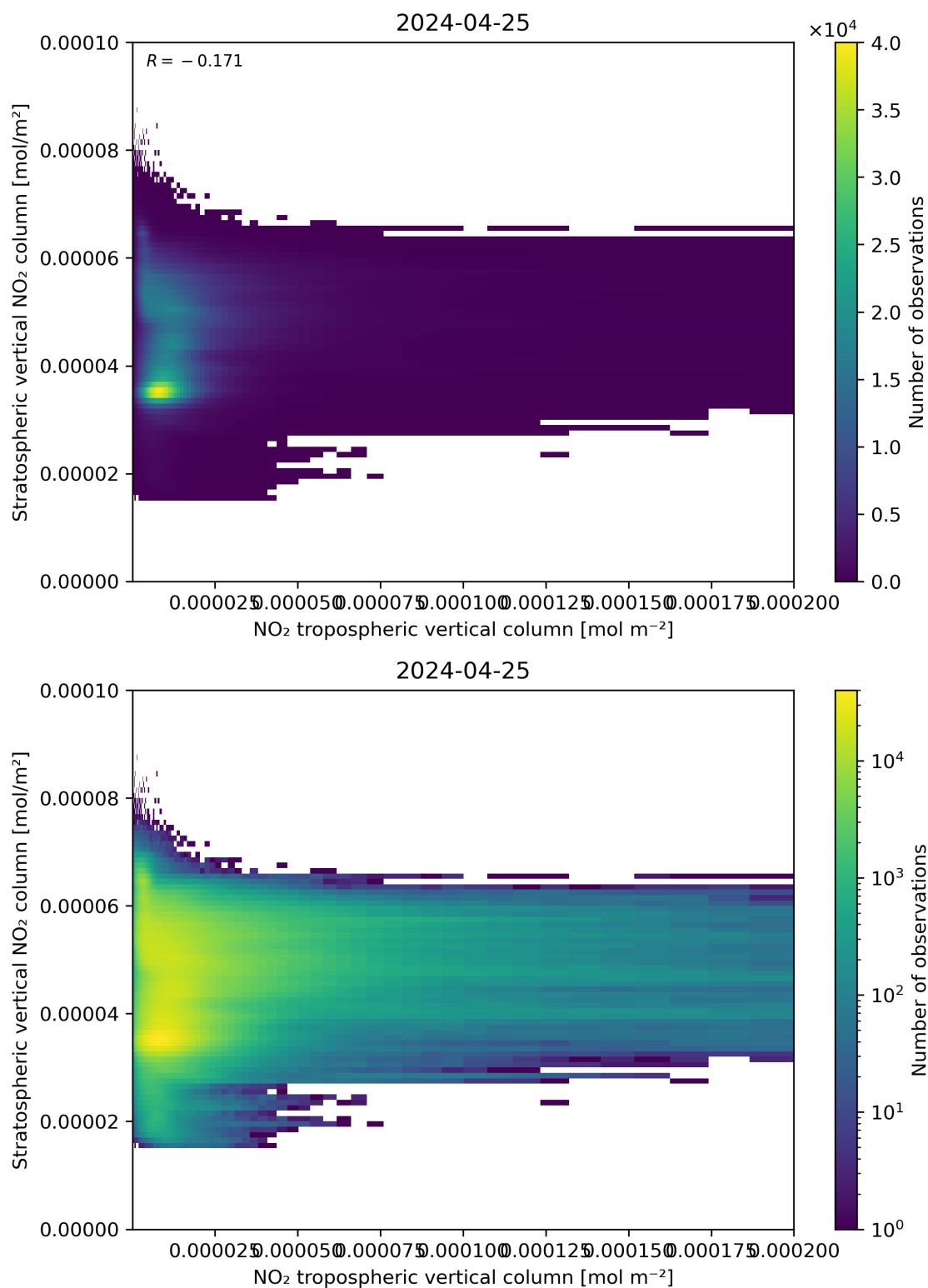
Figure 125: Scatter density plot of “NO 2 tropospheric vertical column” against “Stratospheric vertical NO 2 column” for 2024-04-24 to 2024-04-26.
