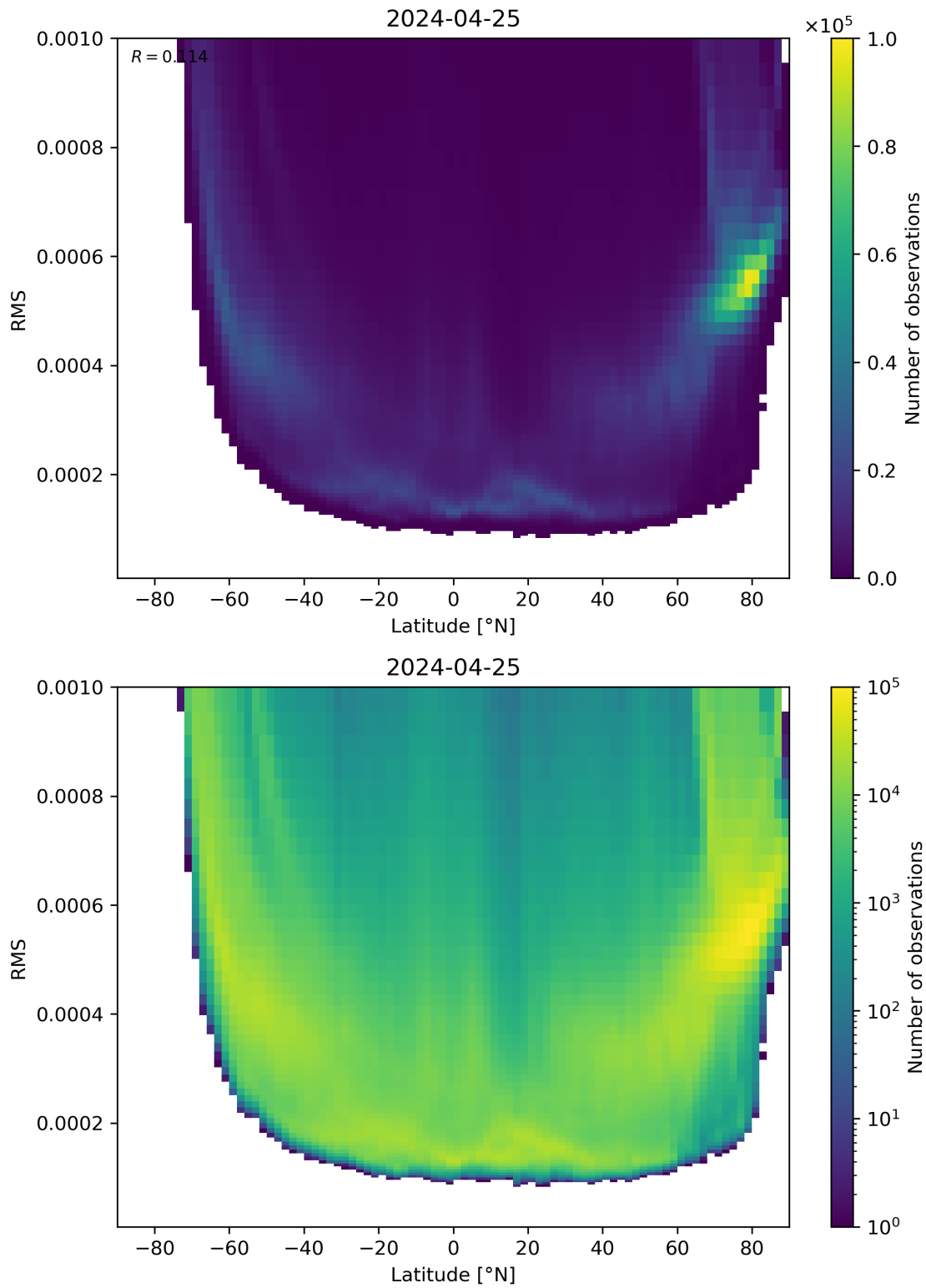
Figure 94: Scatter density plot of “Latitude” against “RMS” for 2024-04-24 to 2024-04-26.
