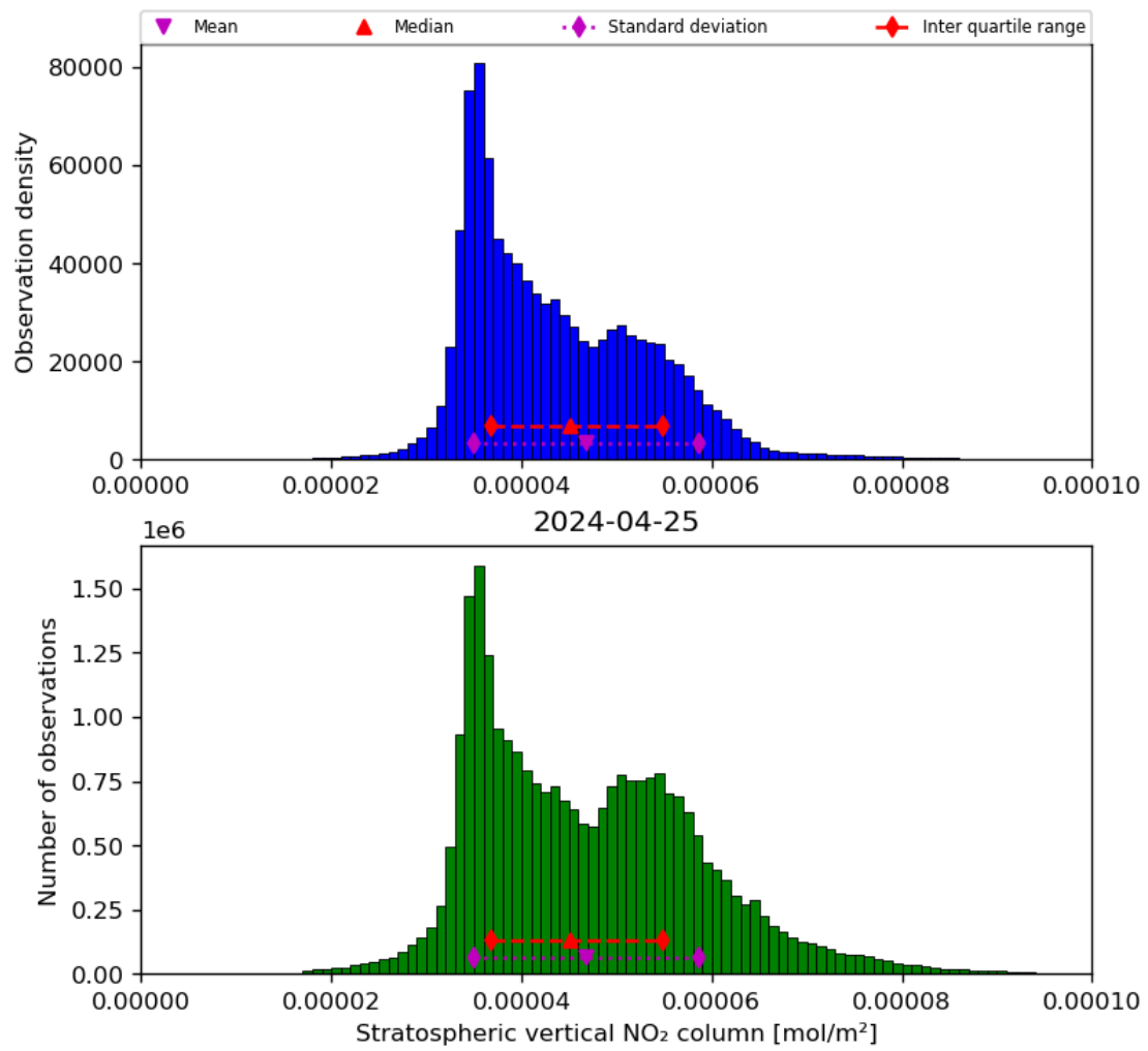
Figure 36: Histogram of “Stratospheric vertical NO 2 column” for 2024-04-24 to 2024-04-26
