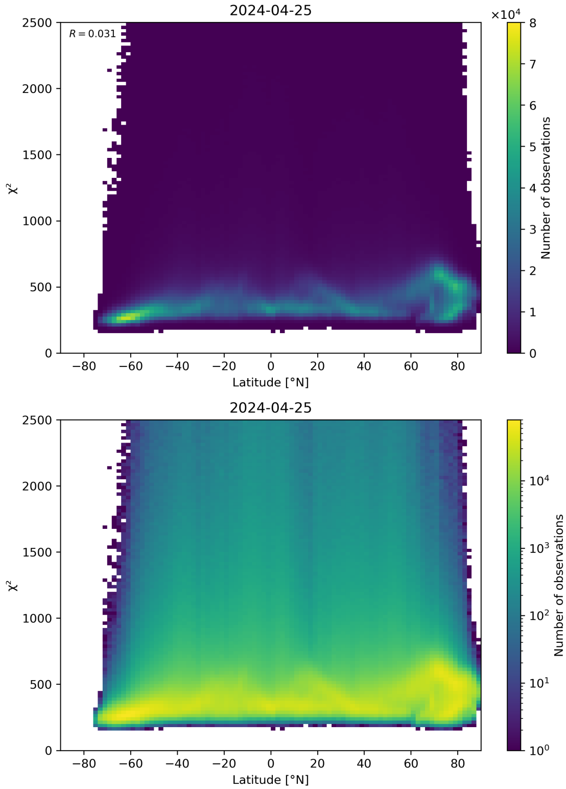
Figure 86: Scatter density plot of “Latitude” against “ \chi^2 ” for 2024-04-24 to 2024-04-26.
