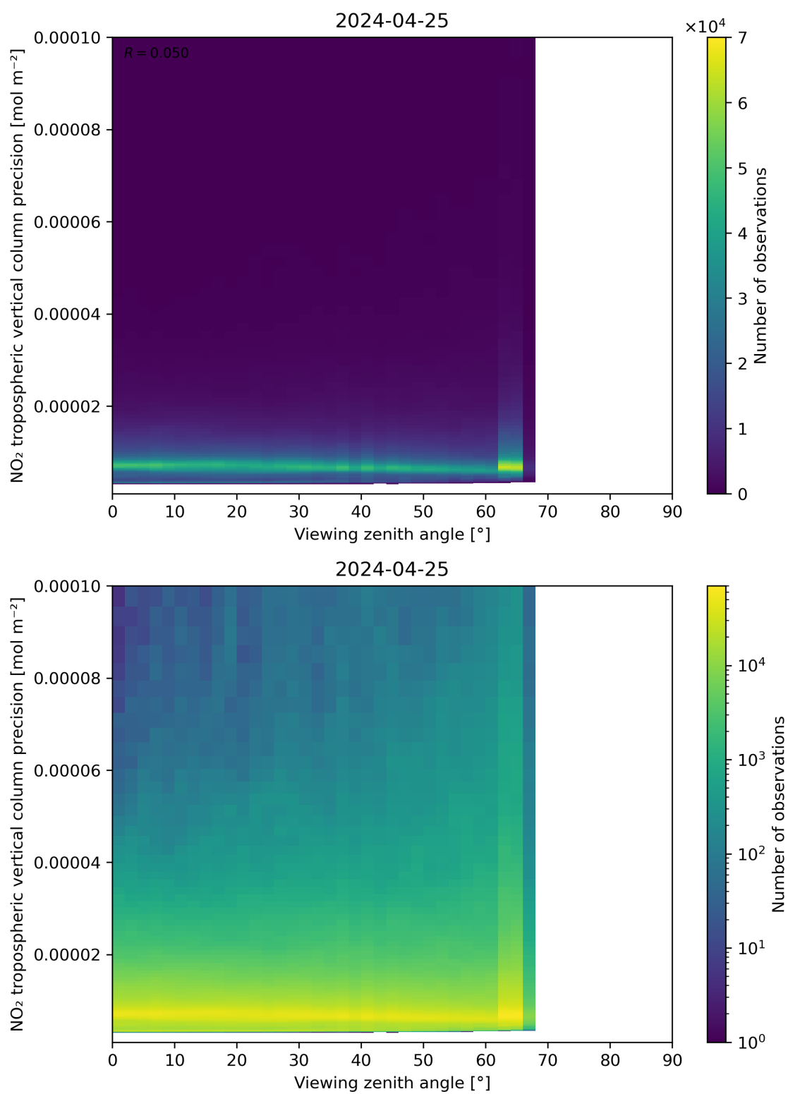
Figure 170: Scatter density plot of “Viewing zenith angle” against “NO 2 tropospheric vertical column precision” for 2024-04-24 to 2024-04-26.
