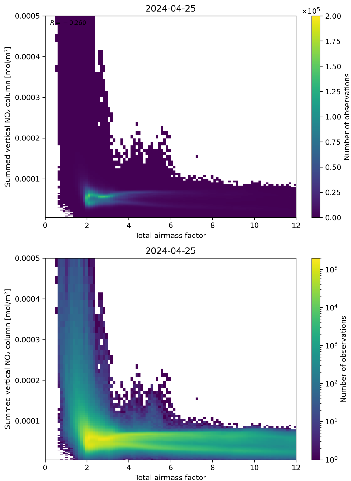
Figure 65: Scatter density plot of “Total airmass factor” against “Summed vertical NO 2 column” for 2024-04-24 to 2024-04-26.
