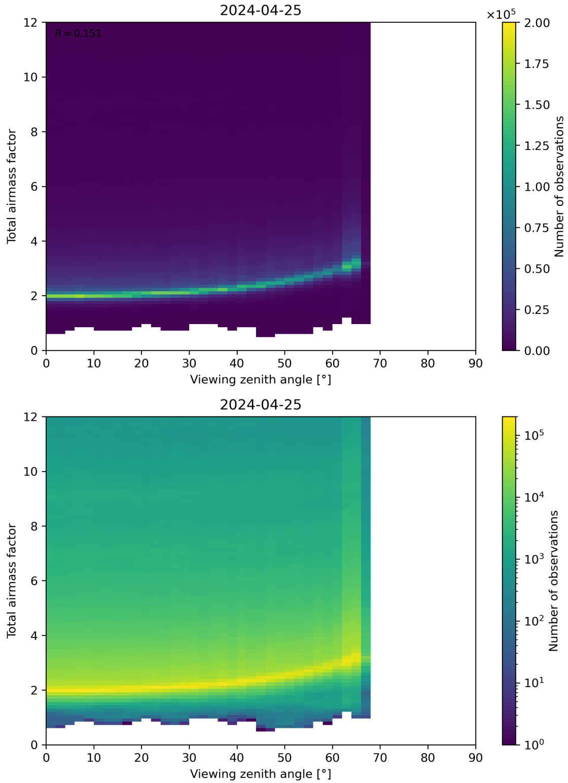
Figure 160: Scatter density plot of “Viewing zenith angle” against “Total airmass factor” for 2024-04-24 to 2024-04-26.
