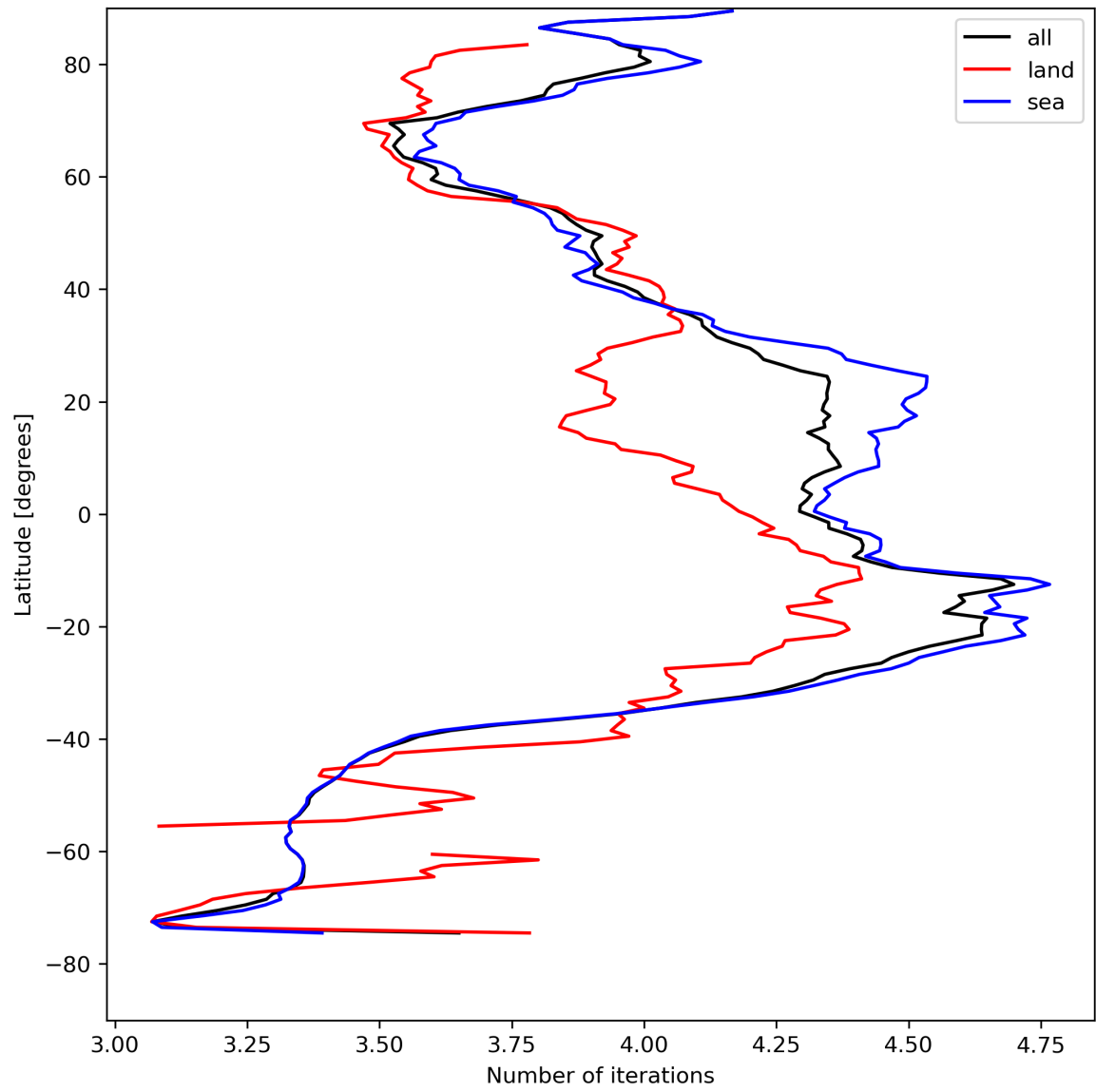
Figure 17: Zonal average of “Number of iterations” for 2024-04-24 to 2024-04-26.
