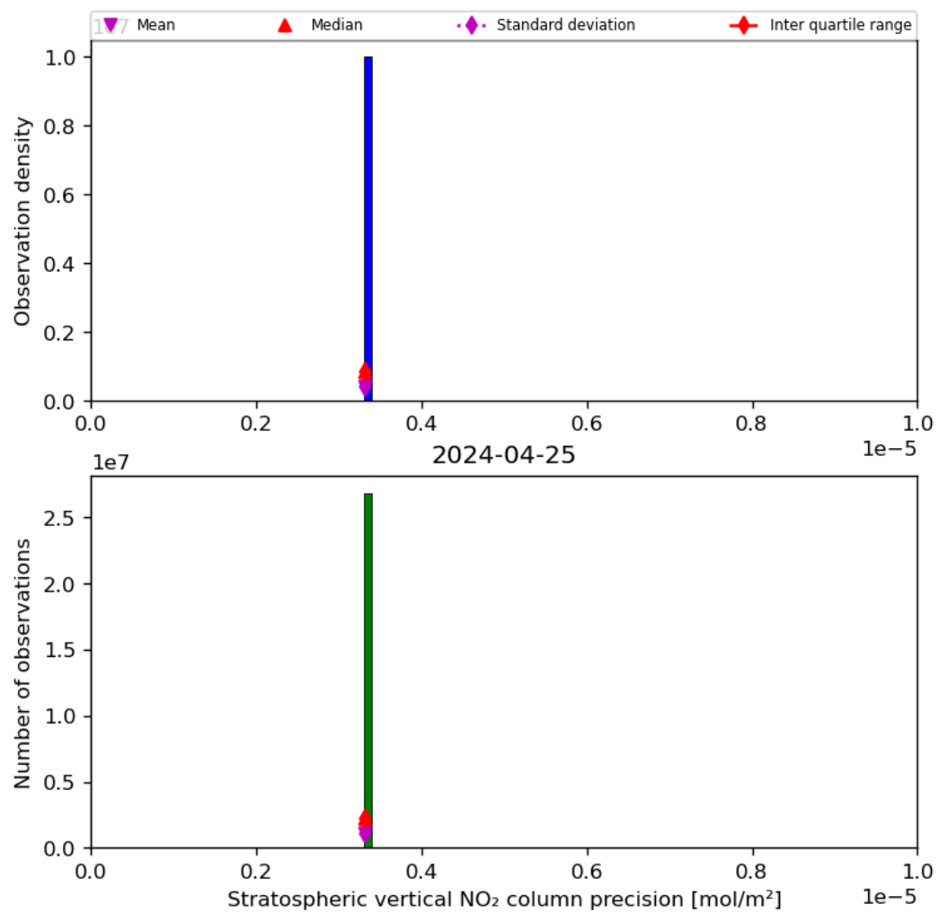
Figure 37: Histogram of “Stratospheric vertical NO 2 column precision” for 2024-04-24 to 2024-04-26
