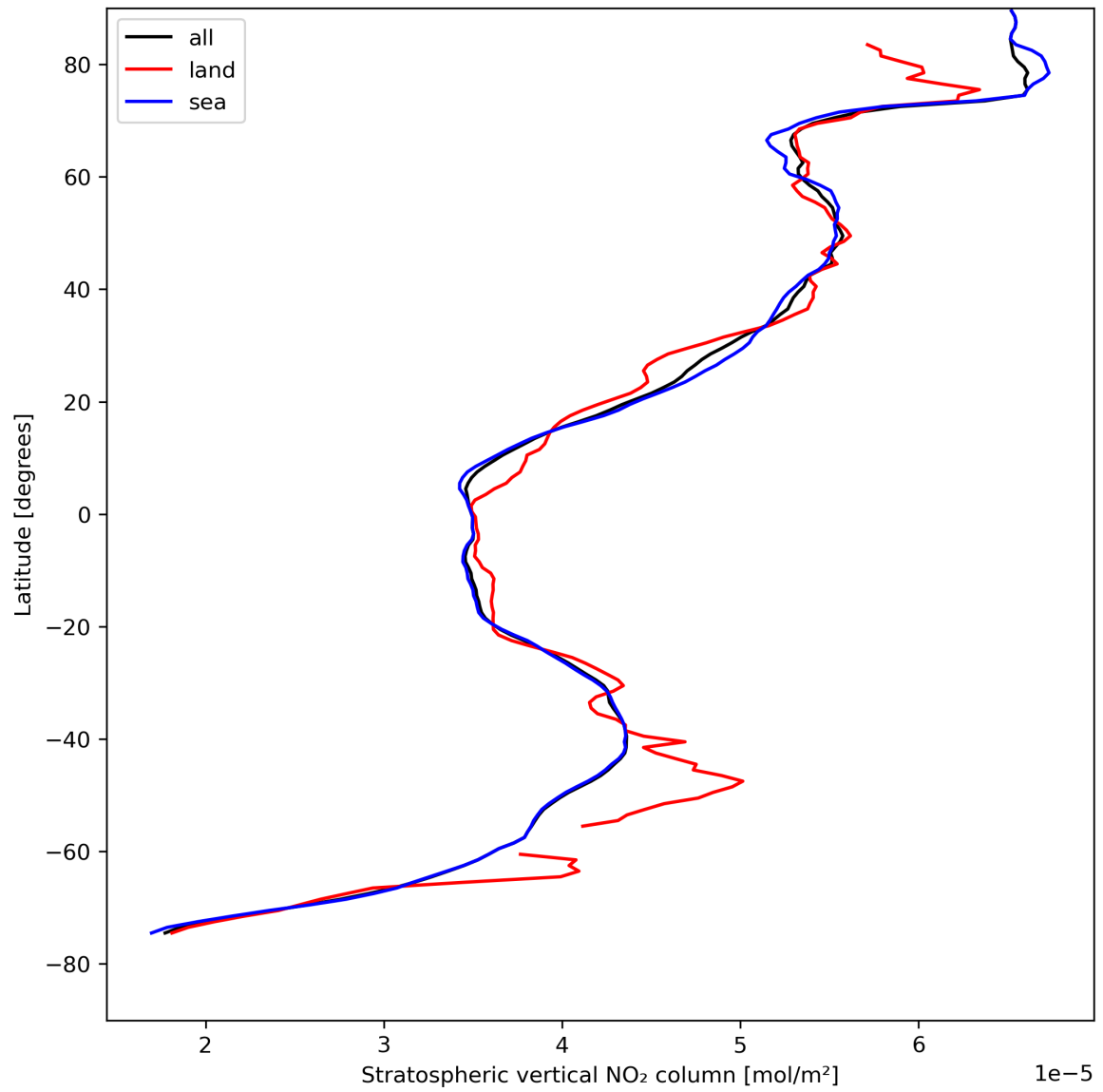
Figure 19: Zonal average of “Stratospheric vertical NO 2 column” for 2024-04-24 to 2024-04-26.
