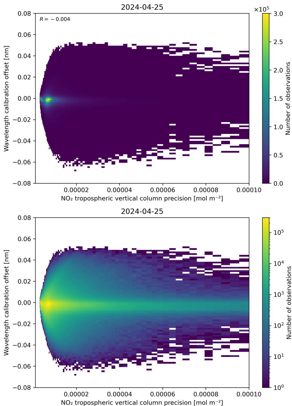
Figure 141: Scatter density plot of “NO 2 tropospheric vertical column precision” against “Wavelength calibration offset” for 2024-04-24 to 2024-04-26.
