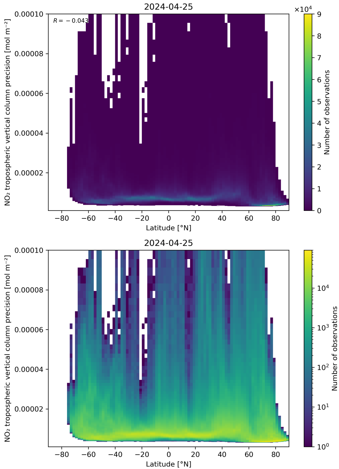
Figure 93: Scatter density plot of “Latitude” against “NO 2 tropospheric vertical column precision” for 2024-04-24 to 2024-04-26.
