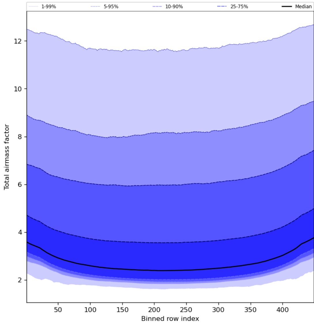
Figure 49: Along track statistics of “Total airmass factor” for 2024-04-24 to 2024-04-26
