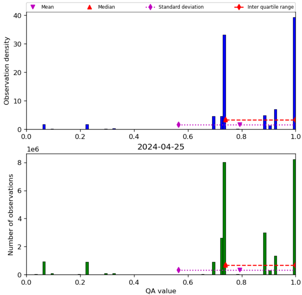
Figure 28: Histogram of “QA value” for 2024-04-24 to 2024-04-26
