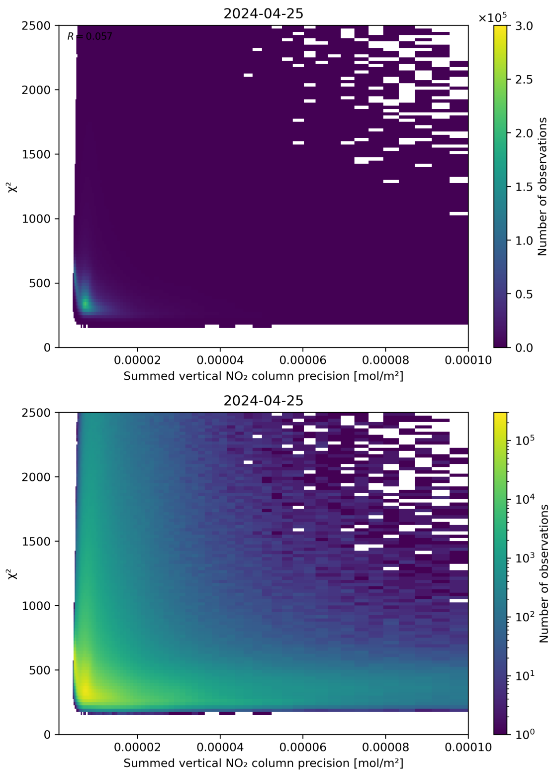
Figure 107: Scatter density plot of “Summed vertical NO 2 column precision” against “ \chi^2 ” for 2024-04-24 to 2024-04-26.
