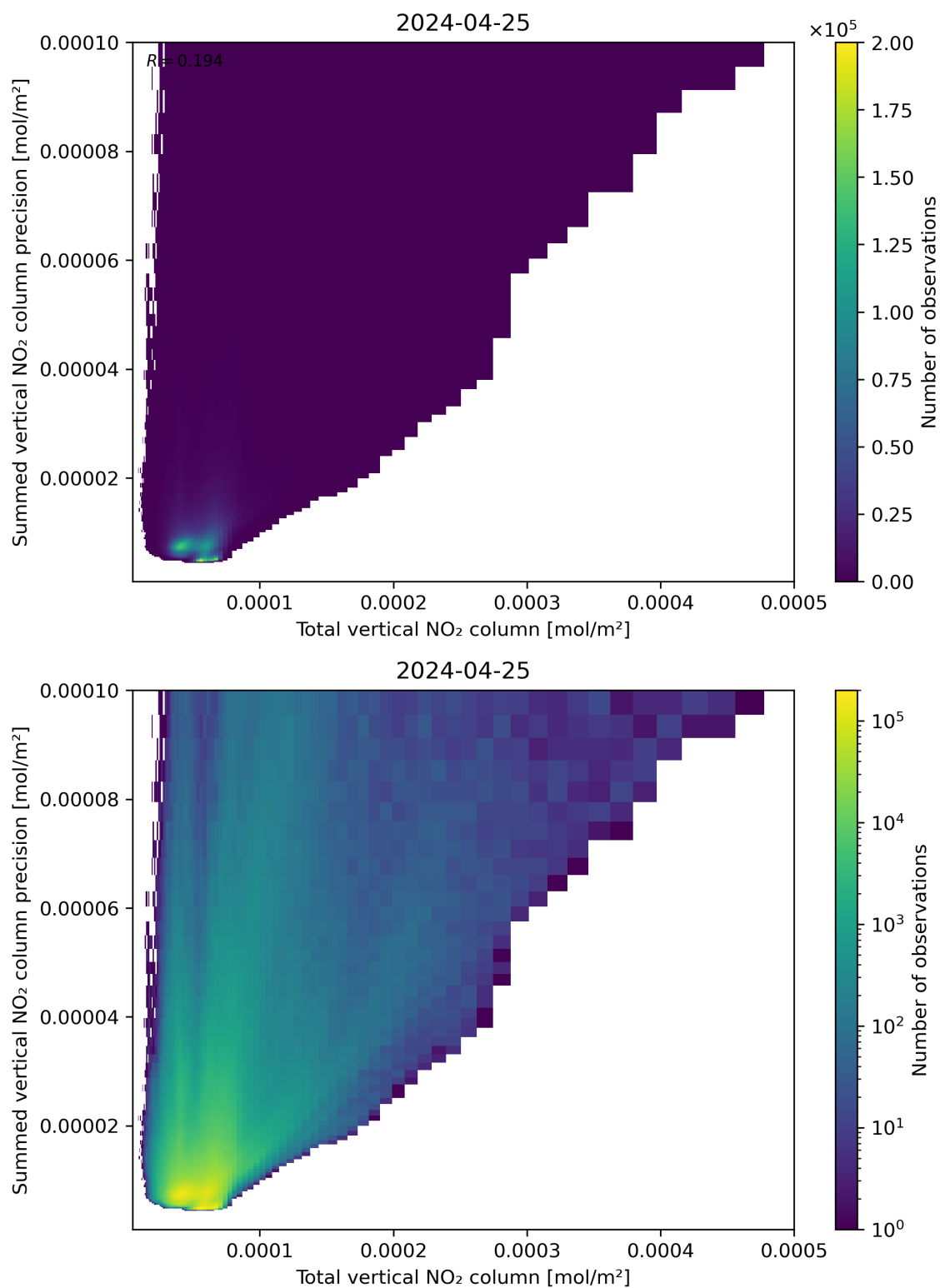
Figure 113: Scatter density plot of “Total vertical NO 2 column” against “Summed vertical NO 2 column precision” for 2024-04-24 to 2024-04-26.
