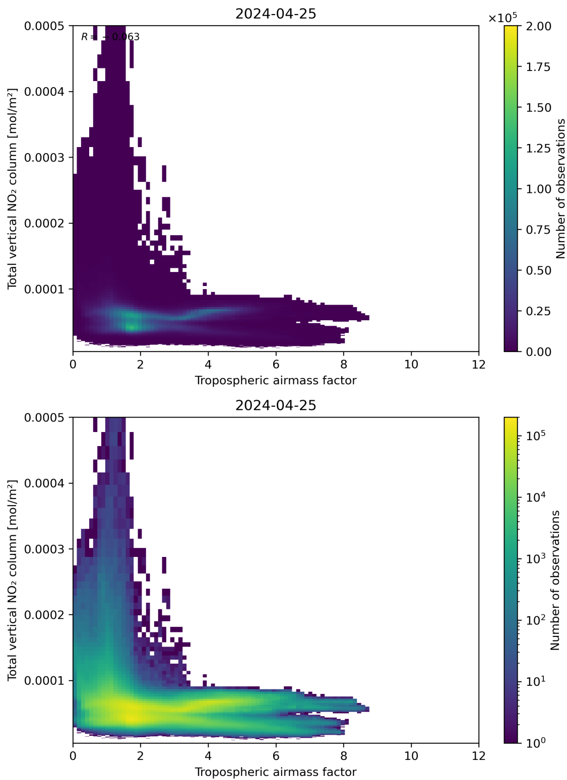
Figure 77: Scatter density plot of “Tropospheric airmass factor” against “Total vertical NO 2 column” for 2024-04-24 to 2024-04-26.
