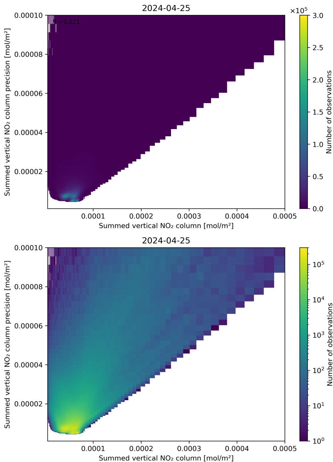
Figure 105: Scatter density plot of “Summed vertical NO 2 column” against “Summed vertical NO 2 column precision” for 2024-04-24 to 2024-04-26.
