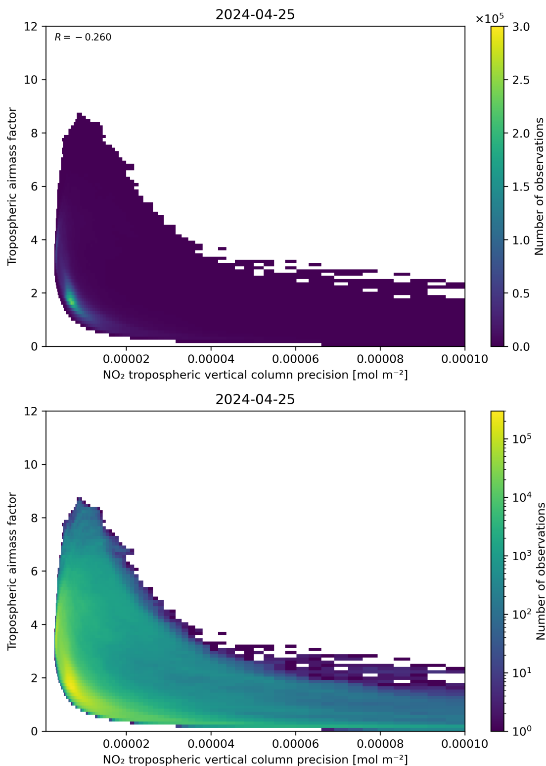
Figure 133: Scatter density plot of “NO 2 tropospheric vertical column precision” against “Tropospheric airmass factor” for 2024-04-24 to 2024-04-26.
