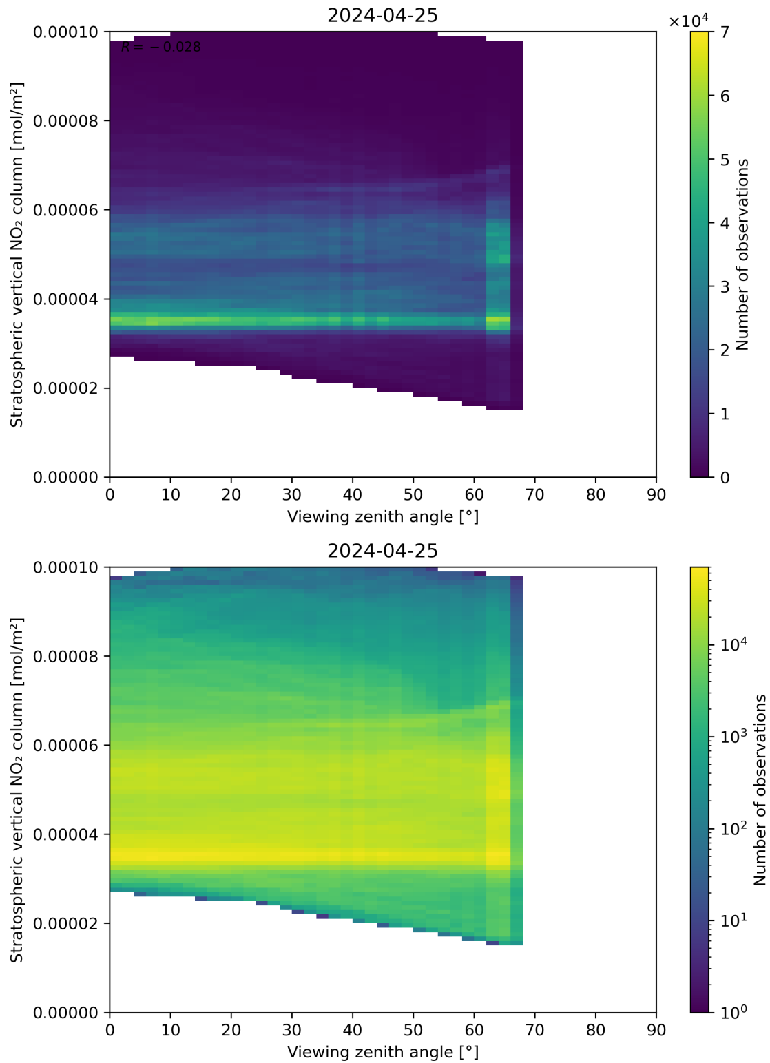
Figure 164: Scatter density plot of “Viewing zenith angle” against “Stratospheric vertical NO 2 column” for 2024-04-24 to 2024-04-26.
