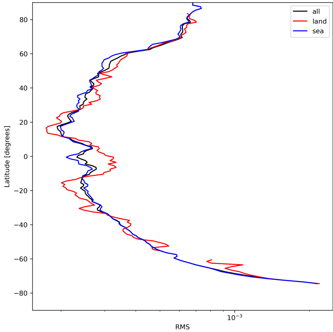
Figure 26: Zonal average of “RMS” for 2024-04-24 to 2024-04-26.
