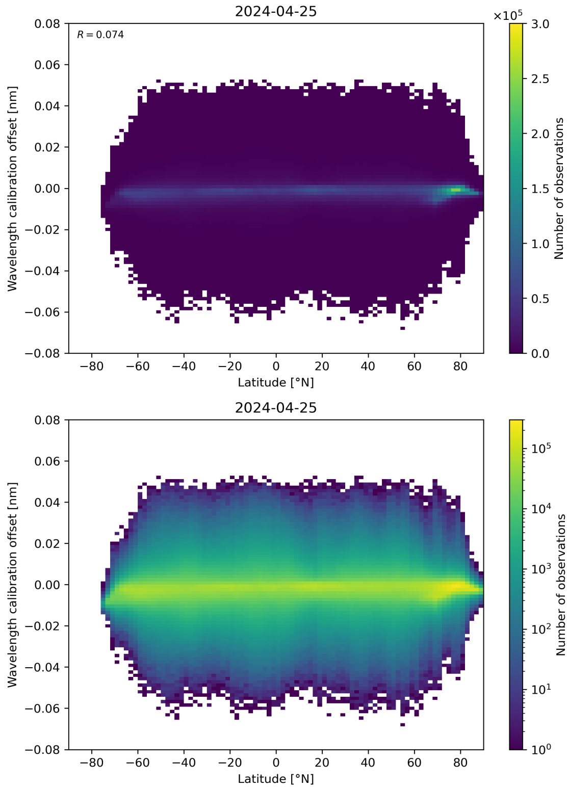
Figure 95: Scatter density plot of “Latitude” against “Wavelength calibration offset” for 2024-04-24 to 2024-04-26.
