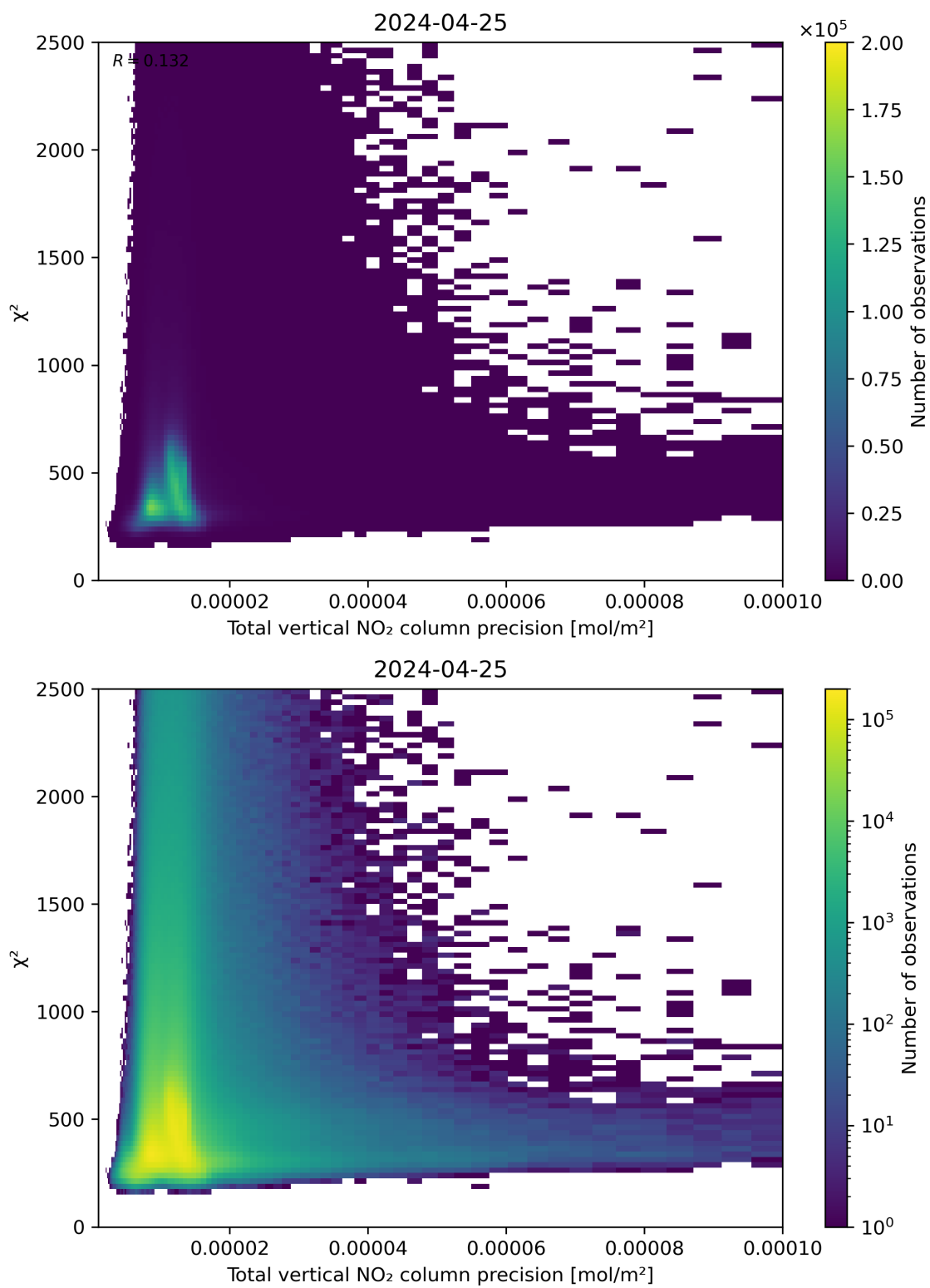
Figure 116: Scatter density plot of “Total vertical NO 2 column precision” against “ \chi^2 ” for 2024-04-24 to 2024-04-26.
