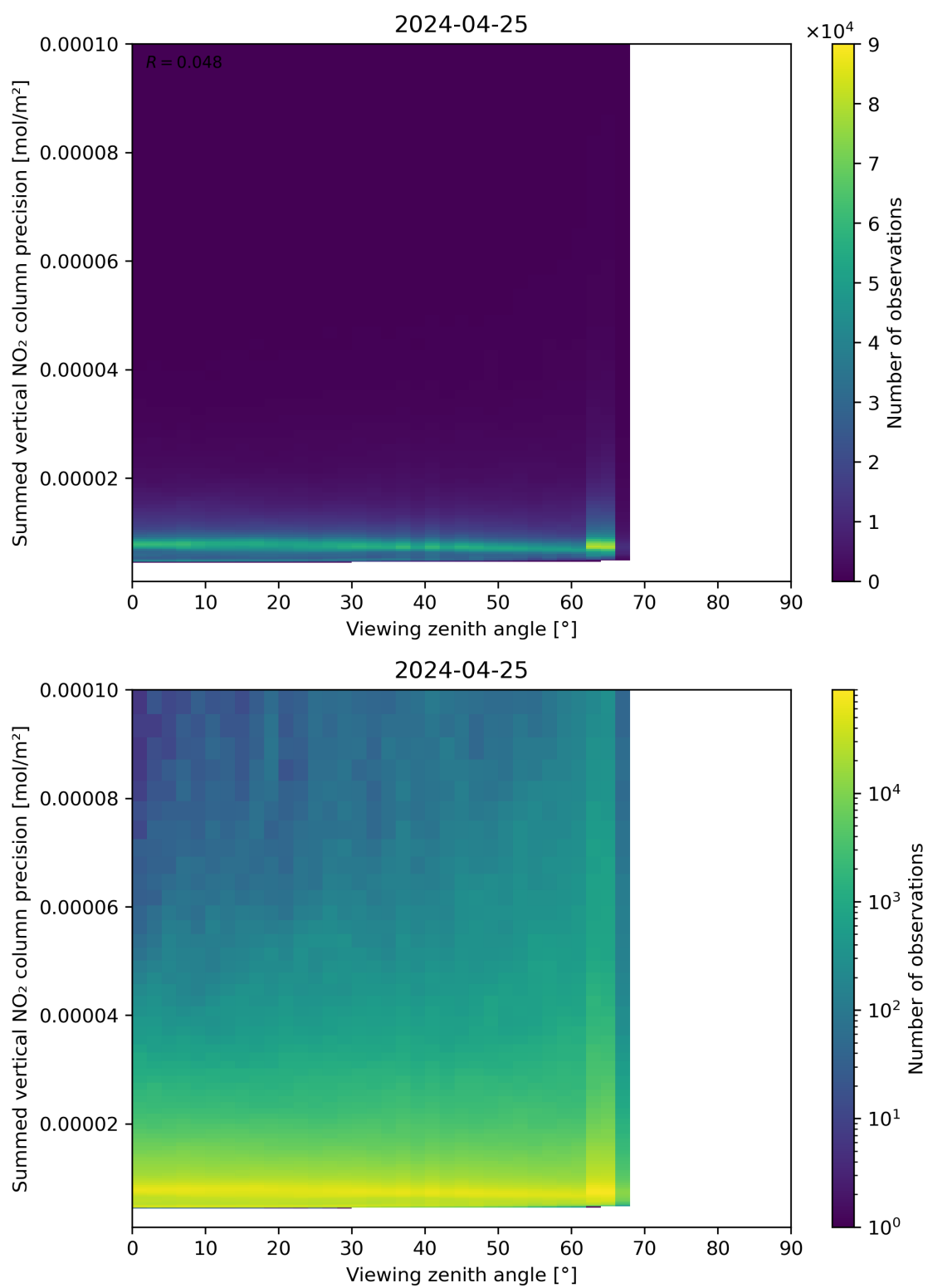
Figure 166: Scatter density plot of “Viewing zenith angle” against “Summed vertical NO 2 column precision” for 2024-04-24 to 2024-04-26.
