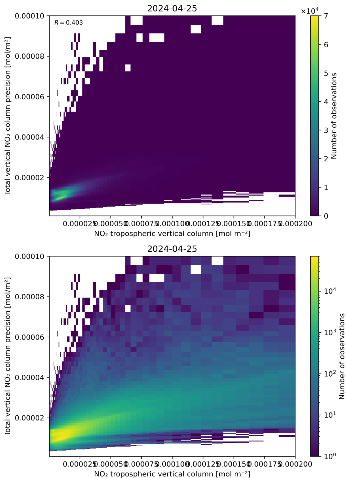
Figure 129: Scatter density plot of “NO 2 tropospheric vertical column” against “Total vertical NO 2 column precision” for 2024-04-24 to 2024-04-26.
