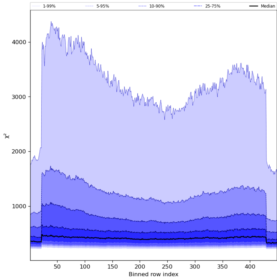
Figure 59: Along track statistics of “ \chi^2 ” for 2024-04-24 to 2024-04-26
