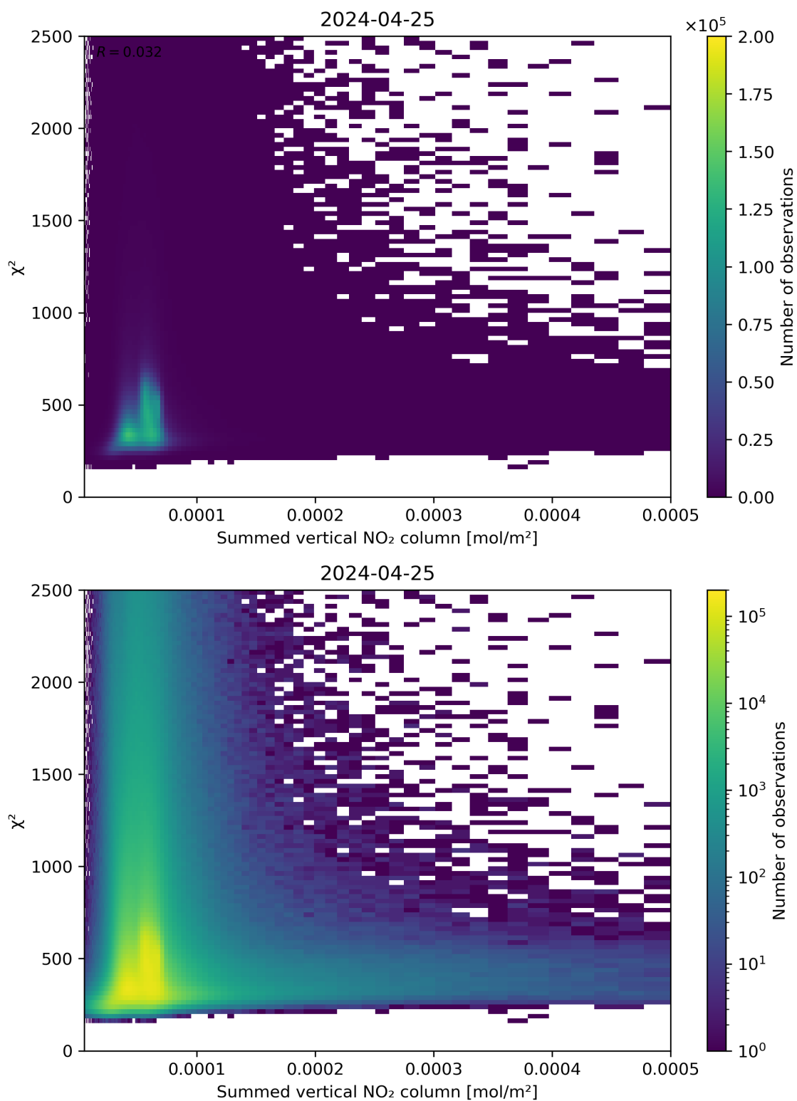
Figure 104: Scatter density plot of “Summed vertical NO 2 column” against “ \chi^2 ” for 2024-04-24 to 2024-04-26.
