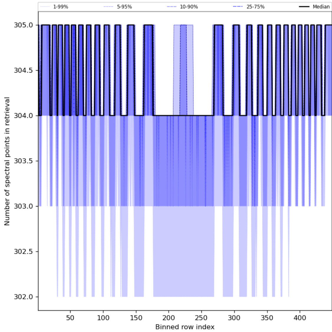
Figure 50: Along track statistics of “Number of spectral points in retrieval” for 2024-04-24 to 2024-04-26
