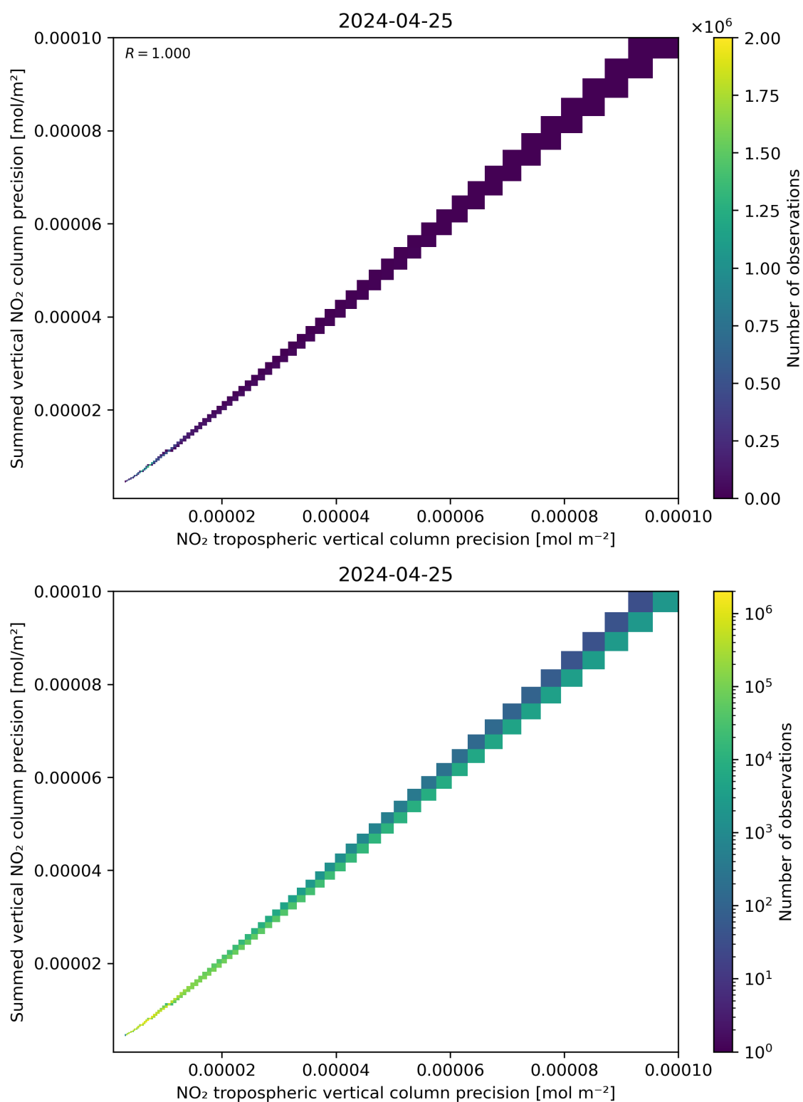
Figure 137: Scatter density plot of “NO 2 tropospheric vertical column precision” against “Summed vertical NO 2 column precision” for 2024-04-24 to 2024-04-26.
