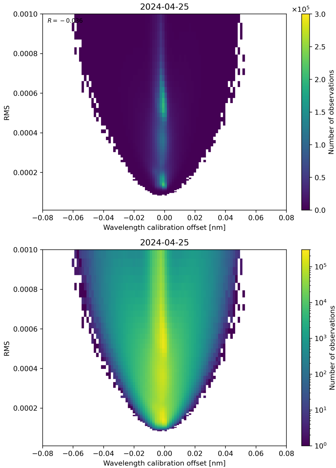
Figure 181: Scatter density plot of “Wavelength calibration offset” against “RMS” for 2024-04-24 to 2024-04-26.
