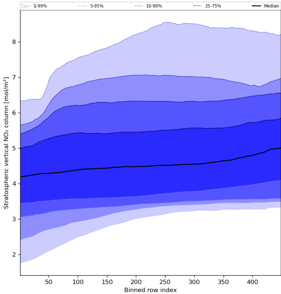
Figure 53: Along track statistics of “Stratospheric vertical NO 2 column” for 2024-04-24 to 2024-04-26
