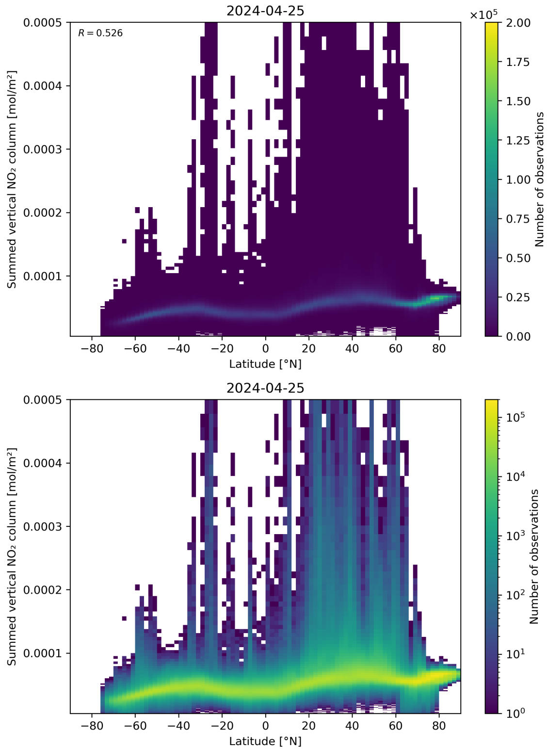
Figure 88: Scatter density plot of “Latitude” against “Summed vertical NO 2 column” for 2024-04-24 to 2024-04-26.
