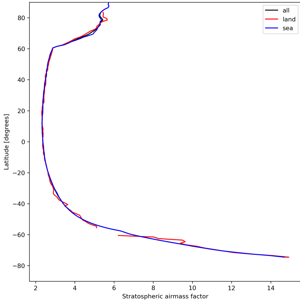
Figure 27: Zonal average of “Stratospheric airmass factor” for 2024-04-24 to 2024-04-26.
