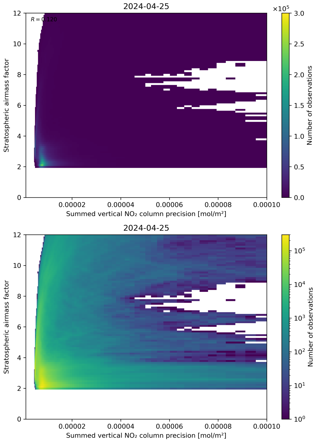
Figure 106: Scatter density plot of “Summed vertical NO 2 column precision” against “Stratospheric airmass factor” for 2024-04-24 to 2024-04-26.
