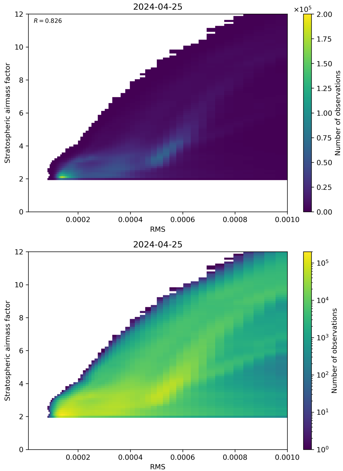
Figure 144: Scatter density plot of “RMS” against “Stratospheric airmass factor” for 2024-04-24 to 2024-04-26.
