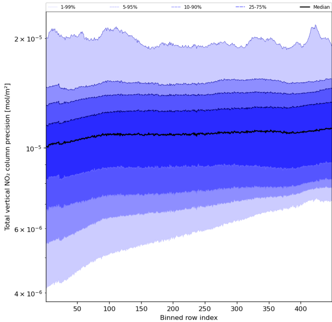
Figure 56: Along track statistics of “Total vertical NO 2 column precision” for 2024-04-24 to 2024-04-26
