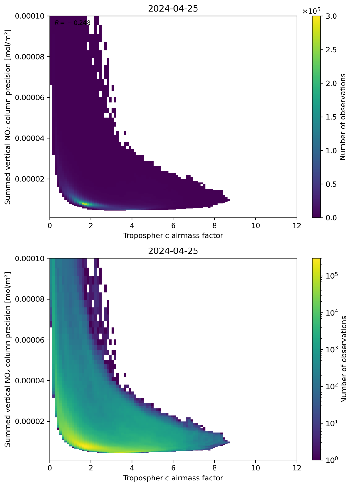
Figure 76: Scatter density plot of “Tropospheric air mass factor” against “Summed vertical NO 2 column precision” for 2024-04-24 to 2024-04-26.
