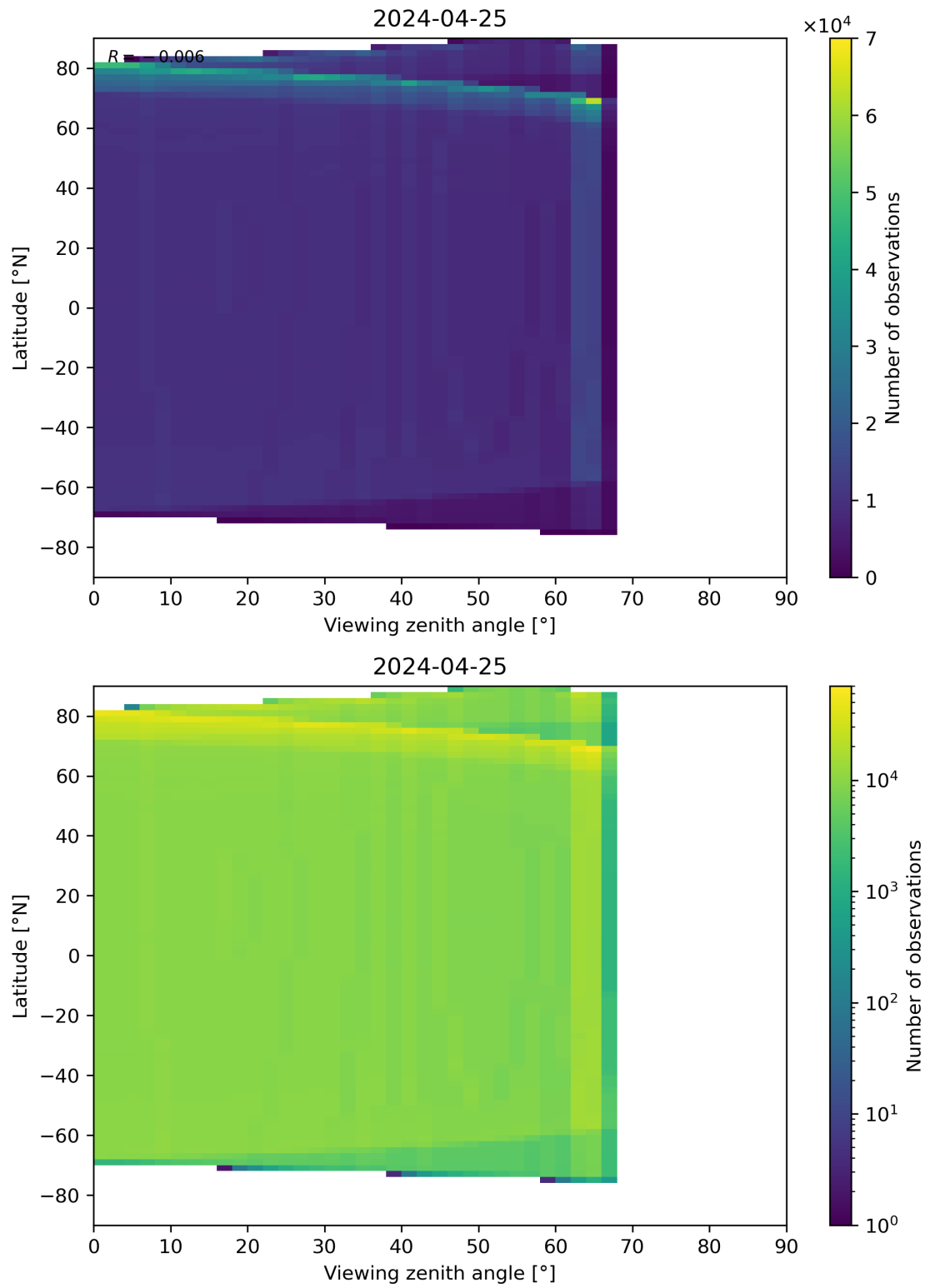
Figure 163: Scatter density plot of “Viewing zenith angle” against “Latitude” for 2024-04-24 to 2024-04-26.
