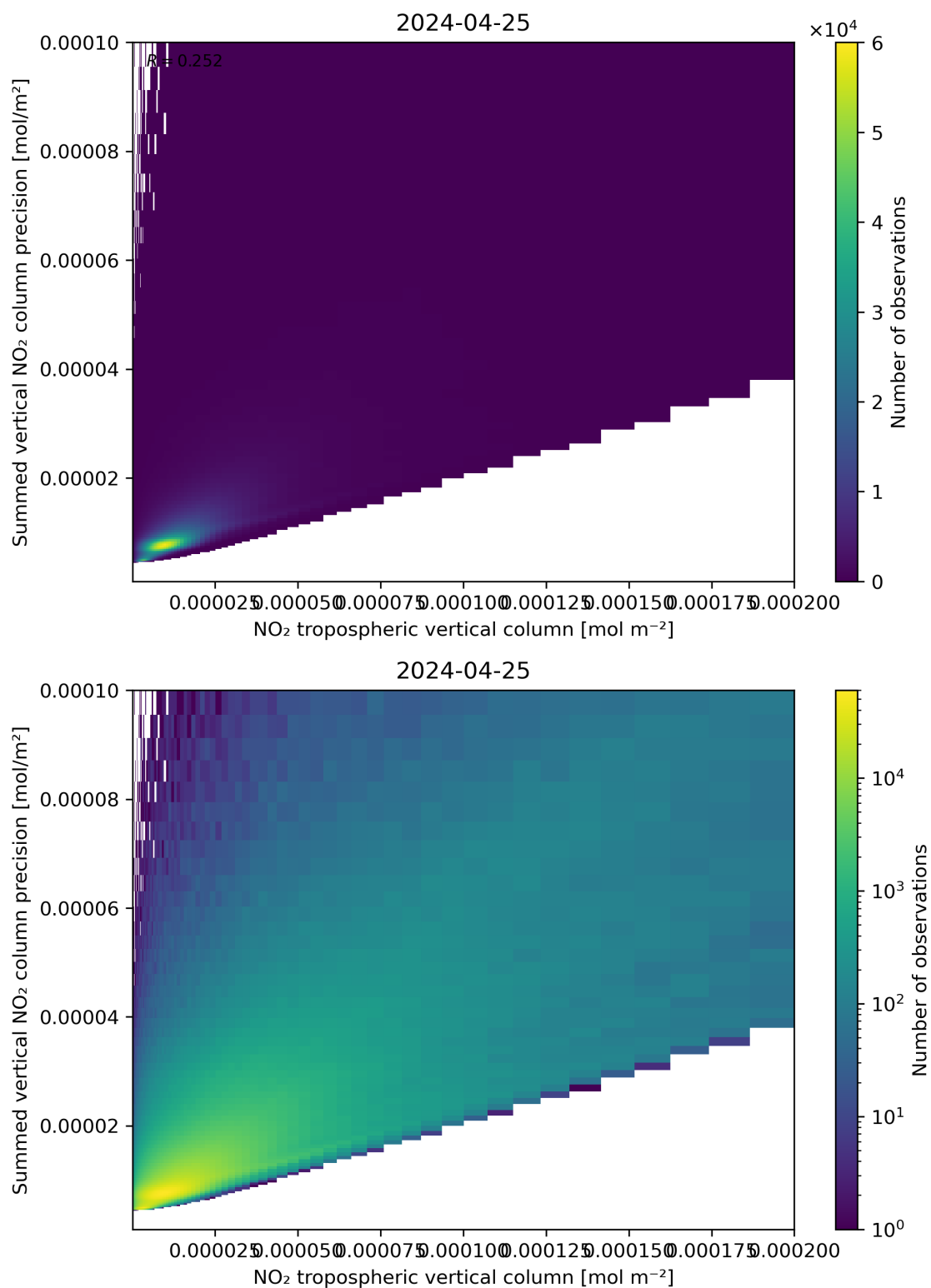
Figure 127: Scatter density plot of “NO 2 tropospheric vertical column” against “Summed vertical NO 2 column precision” for 2024-04-24 to 2024-04-26.
