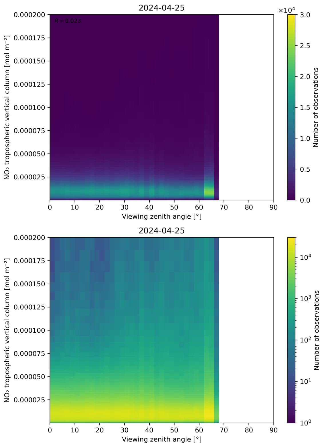
Figure 169: Scatter density plot of “Viewing zenith angle” against “NO 2 tropospheric vertical column” for 2024-04-24 to 2024-04-26.
