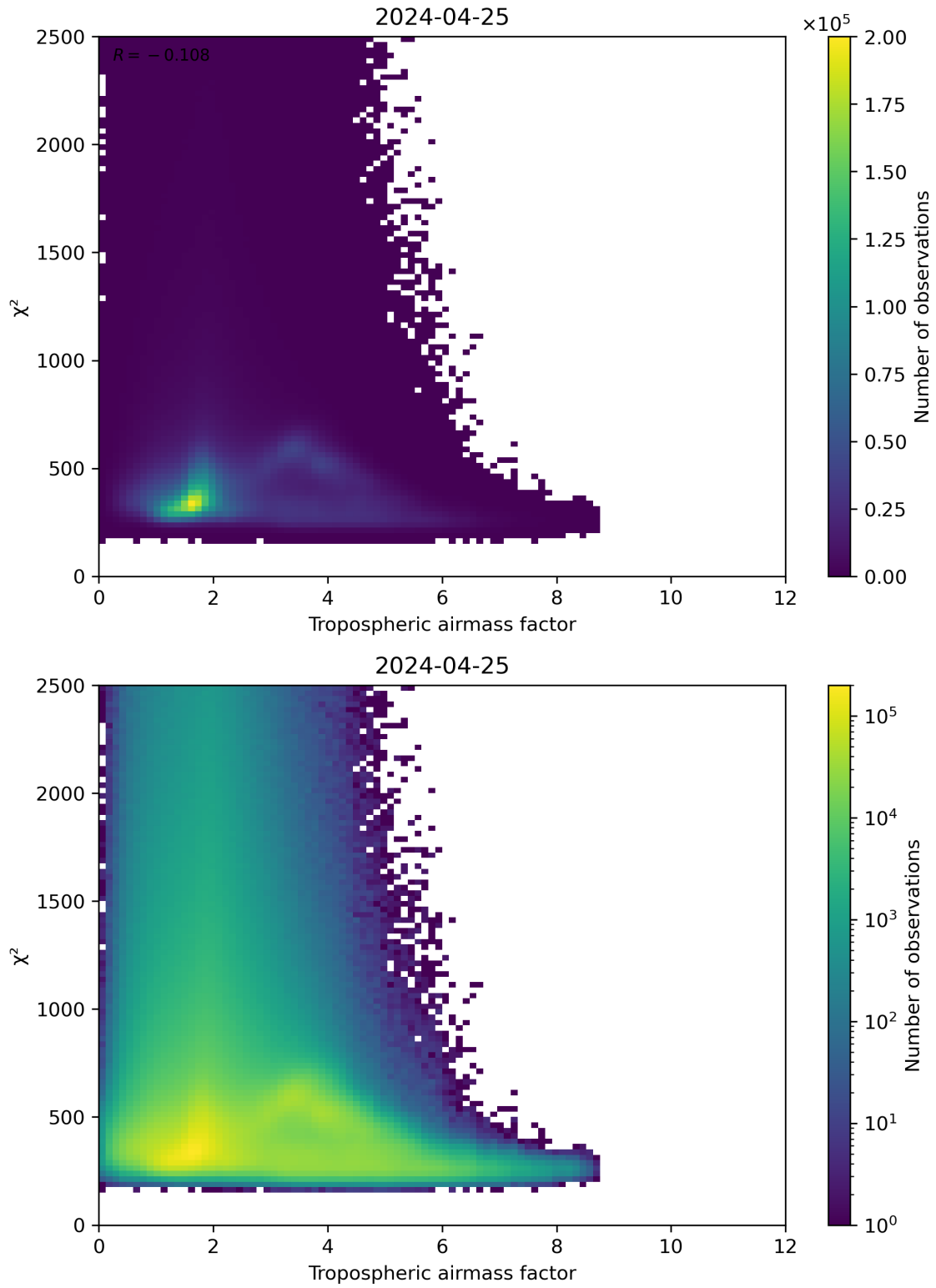
Figure 73: Scatter density plot of “Tropospheric airmass factor” against “ \chi^2 ” for 2024-04-24 to 2024-04-26.
