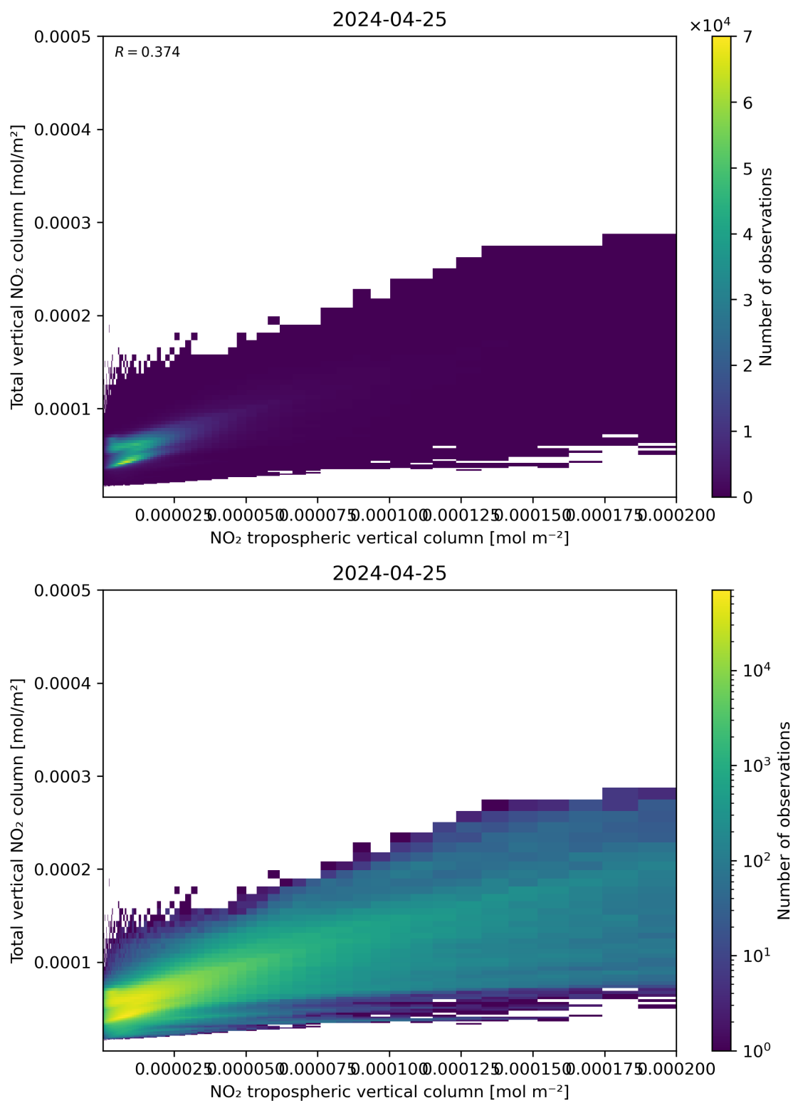
Figure 128: Scatter density plot of “NO 2 tropospheric vertical column” against “Total vertical NO 2 column” for 2024-04-24 to 2024-04-26.
