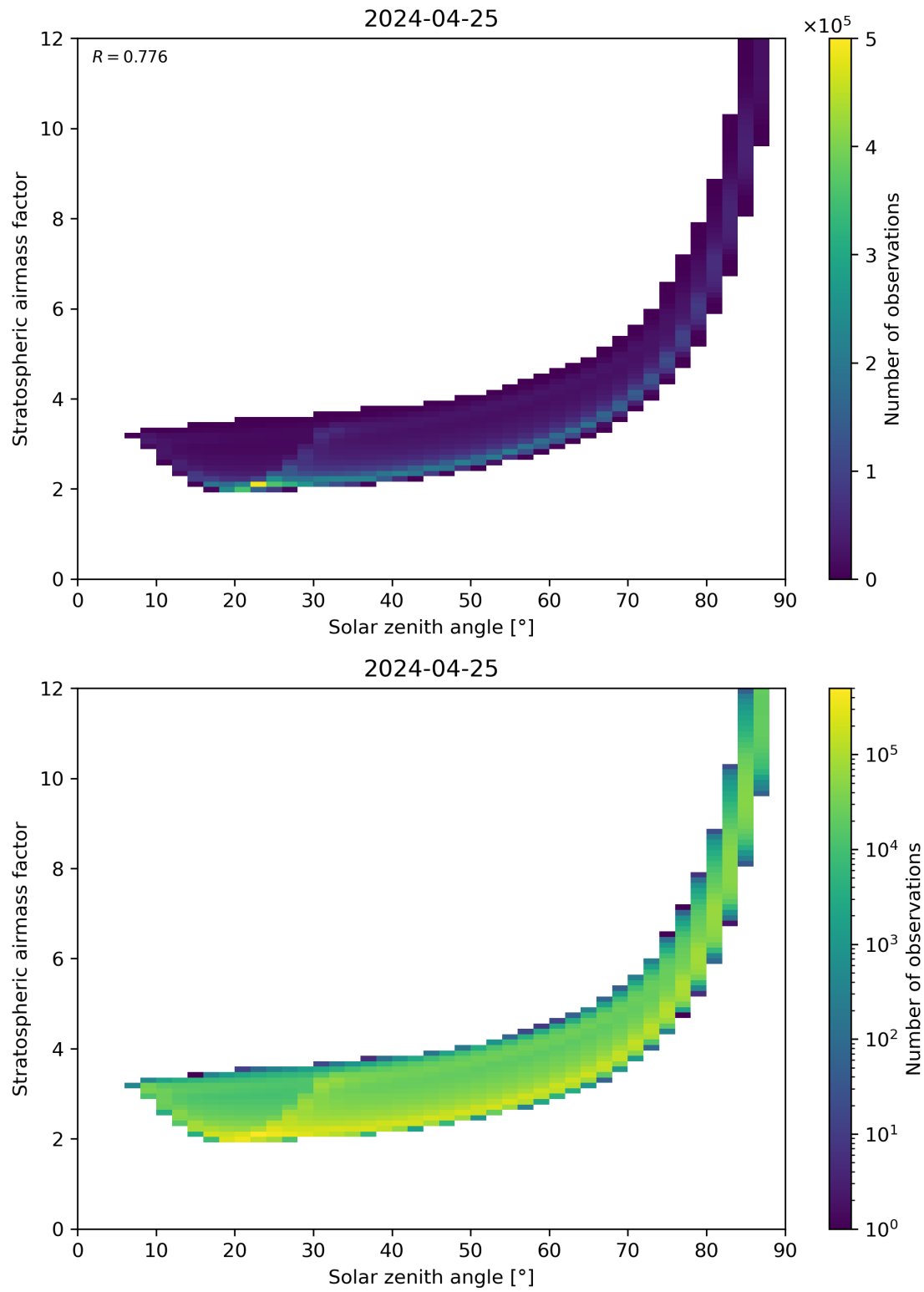
Figure 145: Scatter density plot of “Solar zenith angle” against “Stratospheric airmass factor” for 2024-04-24 to 2024-04-26.
