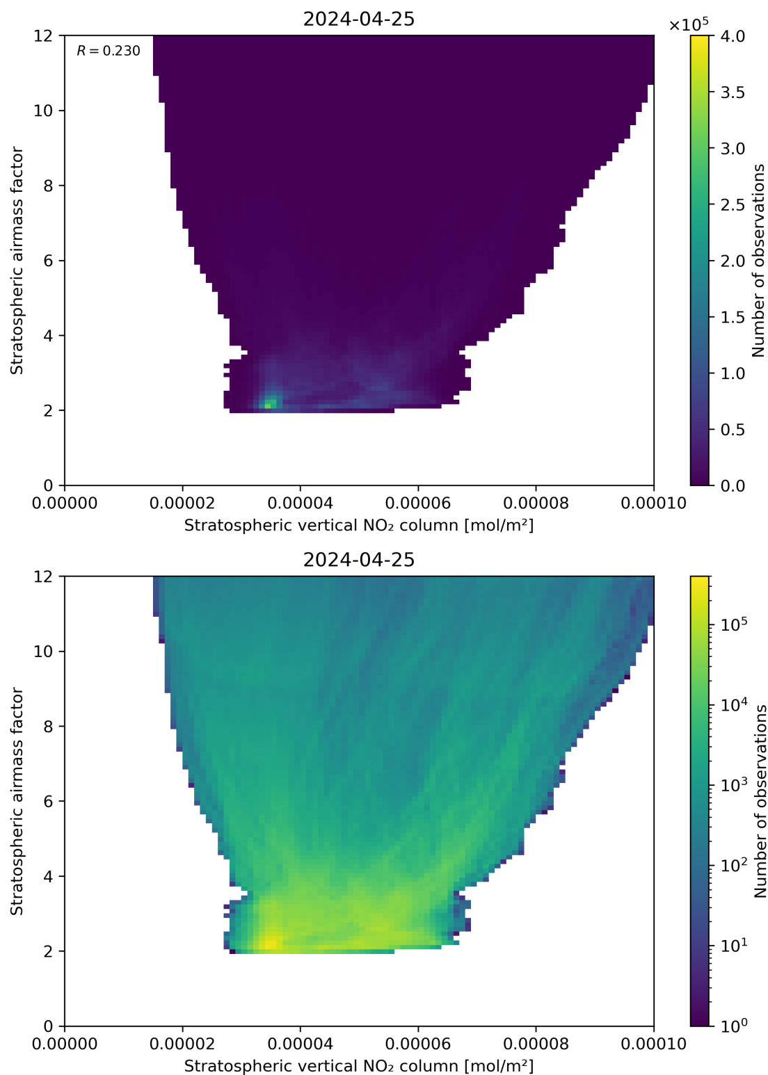
Figure 96: Scatter density plot of “Stratospheric vertical NO 2 column” against “Stratospheric airmass factor” for 2024-04-24 to 2024-04-26.
