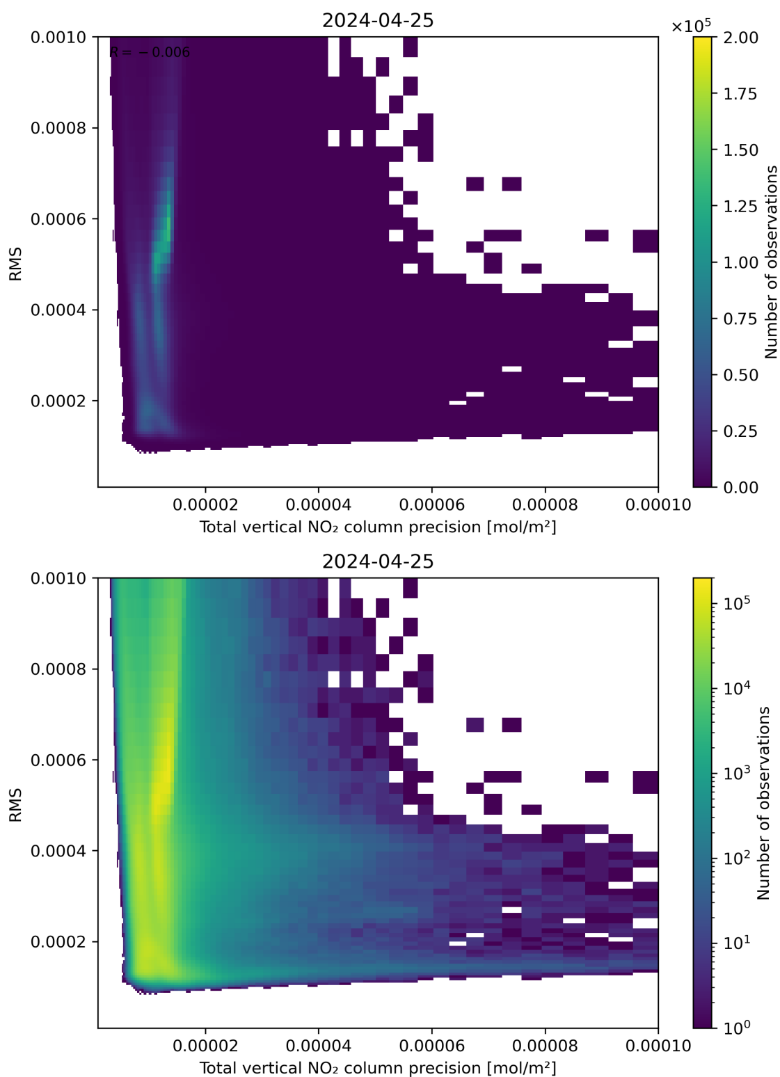
Figure 119: Scatter density plot of “Total vertical NO 2 column precision” against “RMS” for 2024-04-24 to 2024-04-26.
