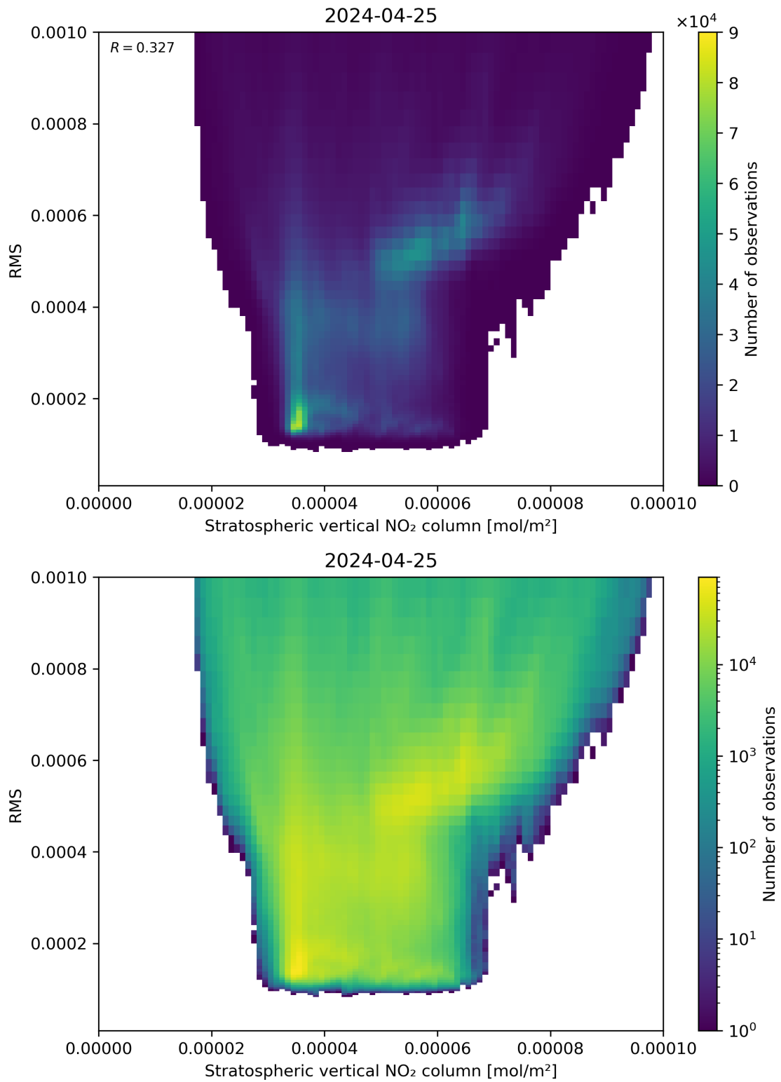
Figure 102: Scatter density plot of “Stratospheric vertical NO 2 column” against “RMS” for 2024-04-24 to 2024-04-26.
