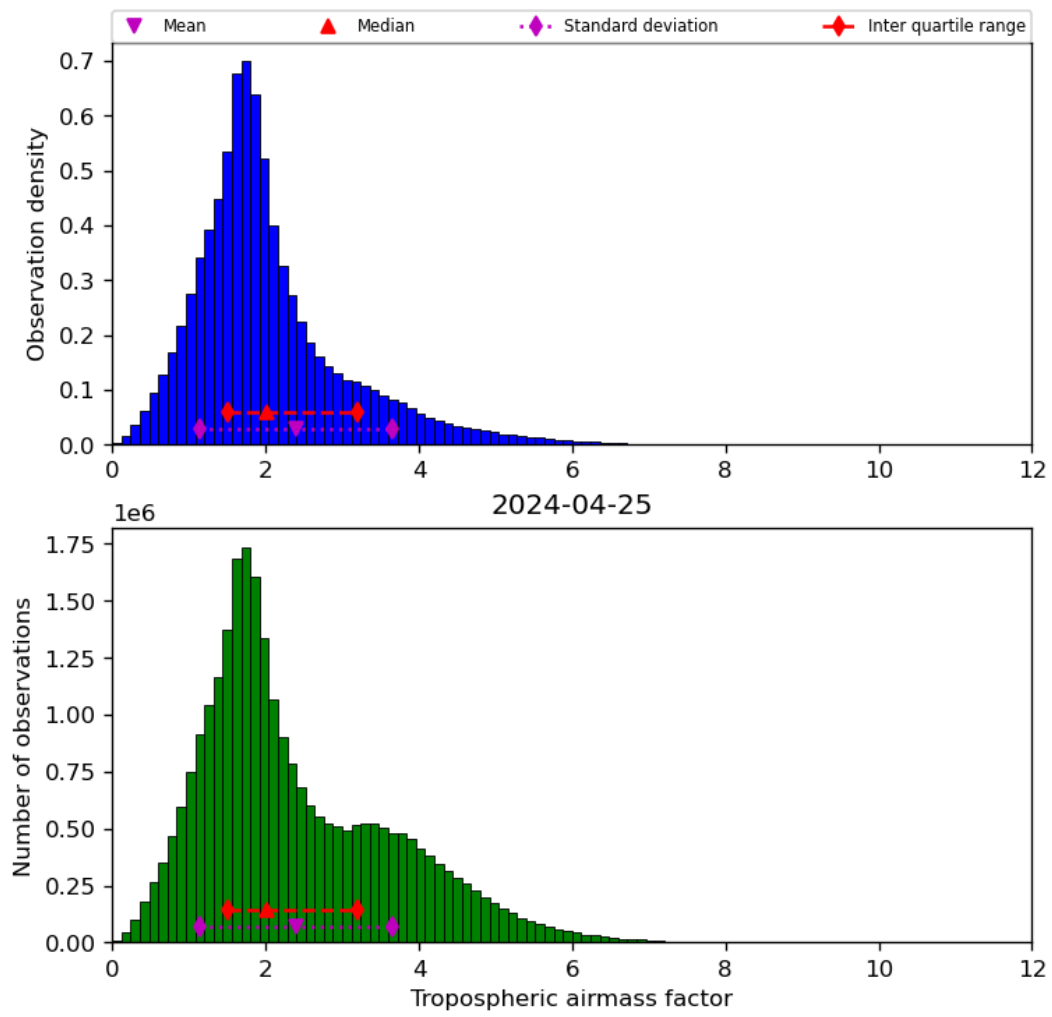
Figure 31: Histogram of “Tropospheric airmass factor” for 2024-04-24 to 2024-04-26
