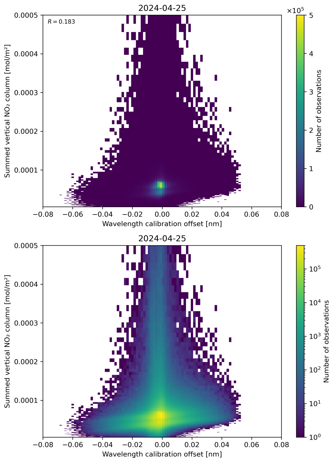
Figure 177: Scatter density plot of “Wavelength calibration offset” against “Summed vertical NO 2 column” for 2024-04-24 to 2024-04-26.
