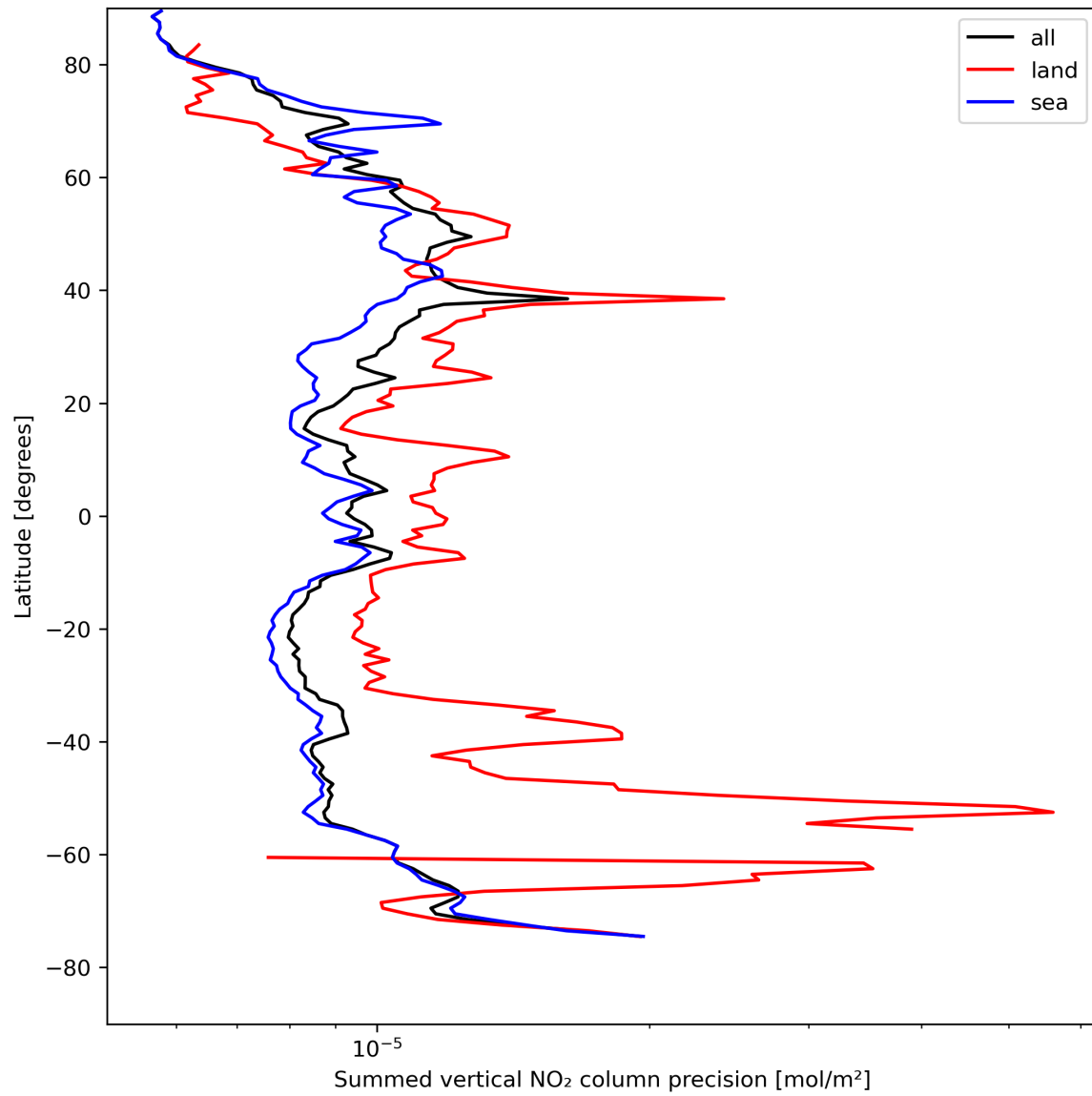
Figure 24: Zonal average of “Summed vertical NO 2 column precision” for 2024-04-24 to 2024-04-26.
