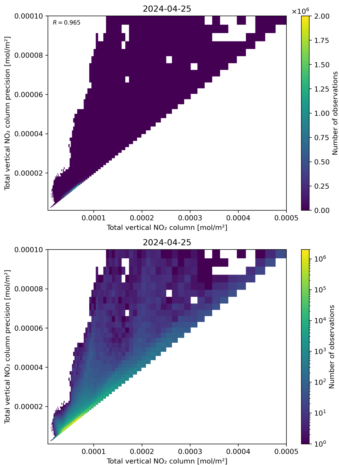
Figure 114: Scatter density plot of “Total vertical NO 2 column” against “Total vertical NO 2 column precision” for 2024-04-24 to 2024-04-26.
