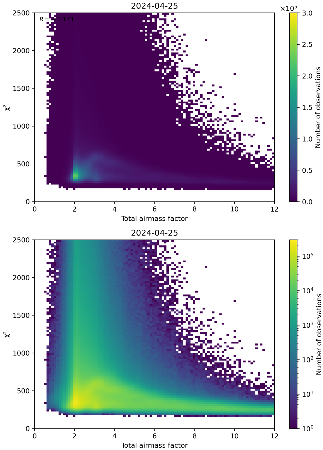
Figure 63: Scatter density plot of “Total airmass factor” against “ \chi^2 ” for 2024-04-24 to 2024-04-26.
