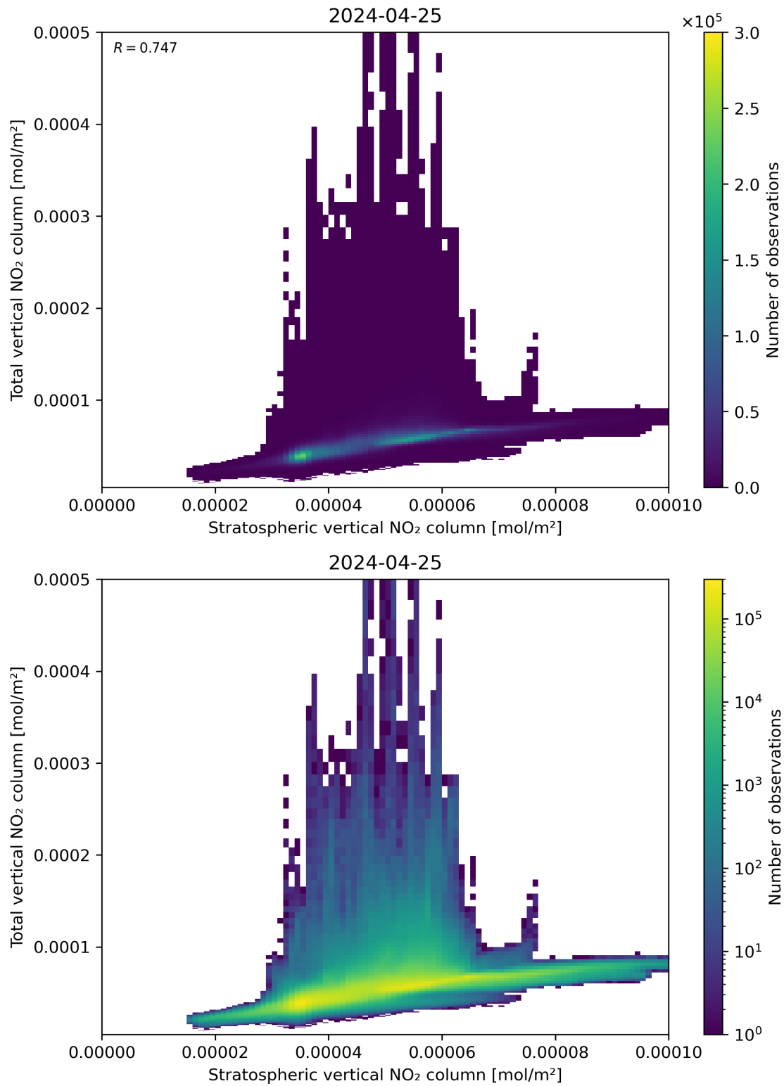
Figure 100: Scatter density plot of “Stratospheric vertical NO 2 column” against “Total vertical NO 2 column” for 2024-04-24 to 2024-04-26.
