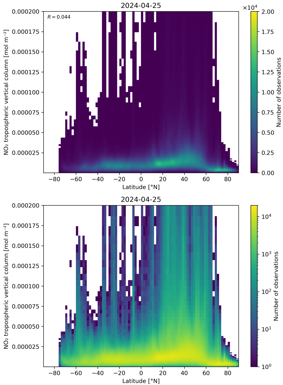
Figure 92: Scatter density plot of “Latitude” against “NO 2 tropospheric vertical column” for 2024-04-24 to 2024-04-26.
