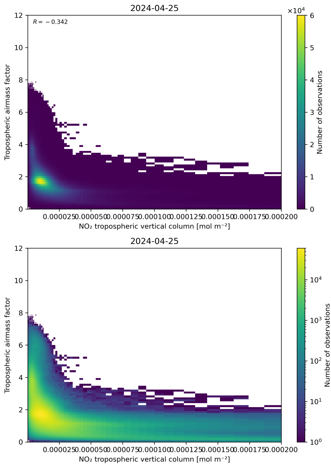
Figure 123: Scatter density plot of “NO 2 tropospheric vertical column” against “Tropospheric air mass factor” for 2024-04-24 to 2024-04-26.
