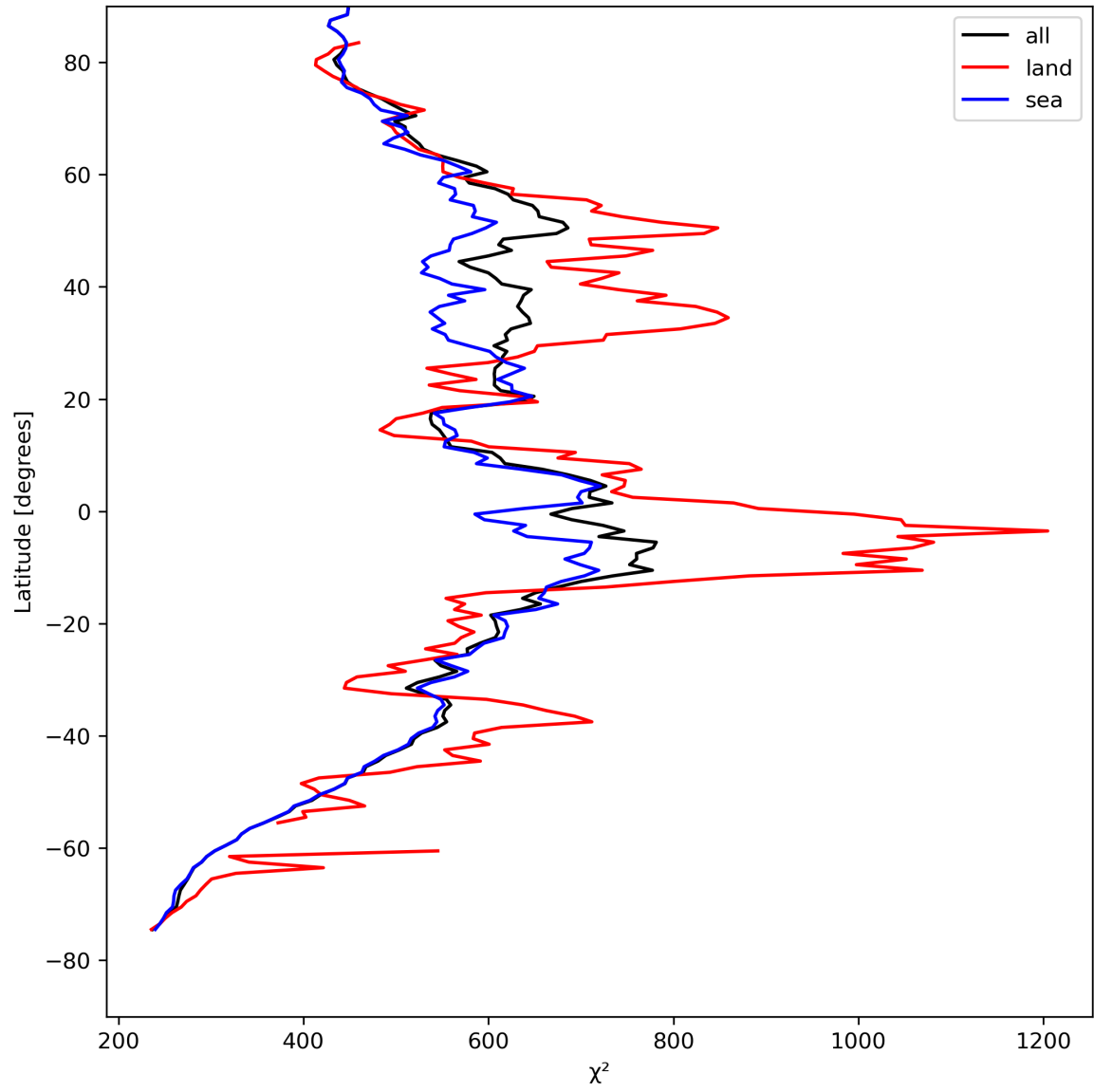
Figure 25: Zonal average of “ \chi^2 ” for 2024-04-24 to 2024-04-26.
