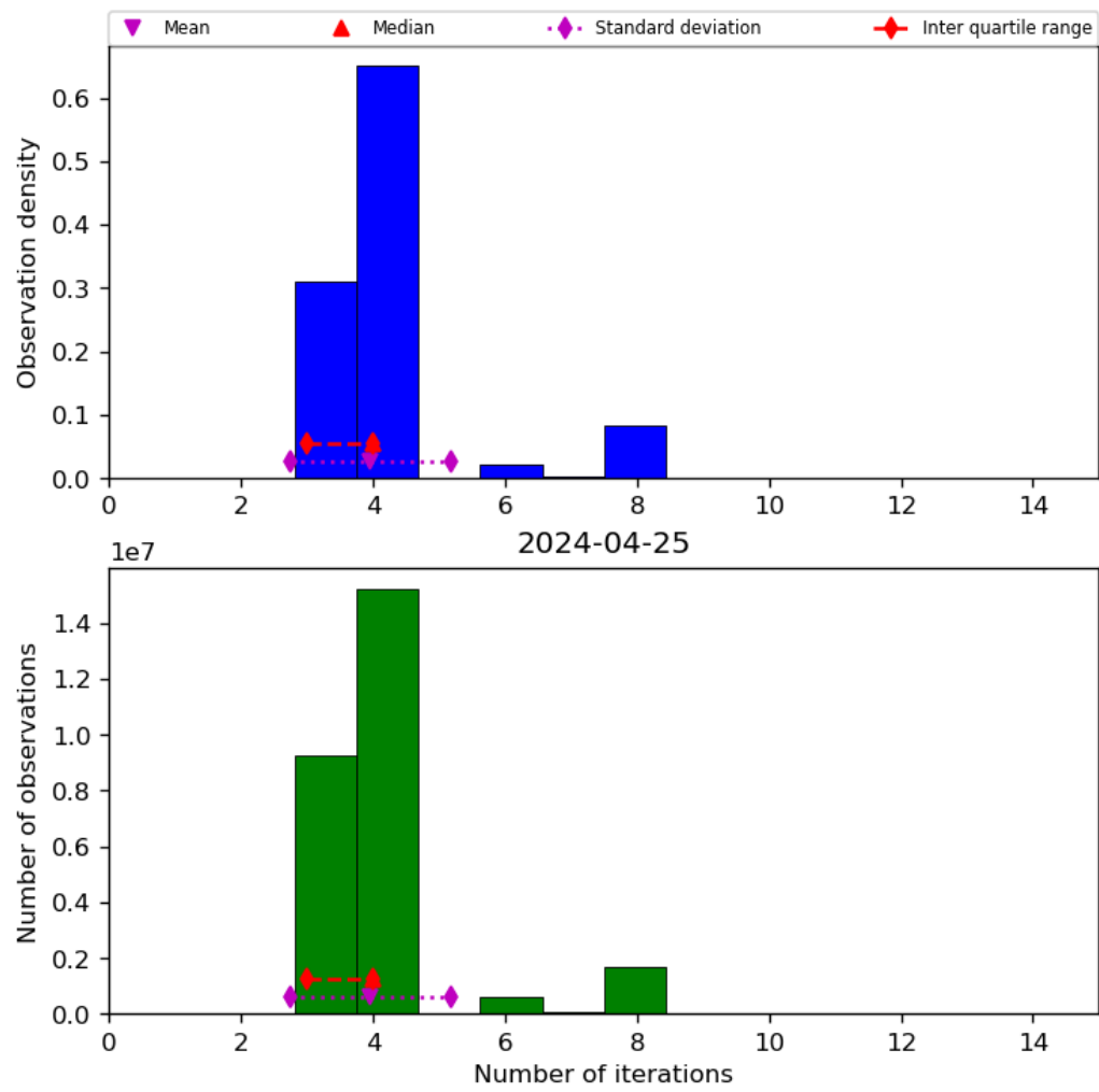
Figure 34: Histogram of “Number of iterations” for 2024-04-24 to 2024-04-26
