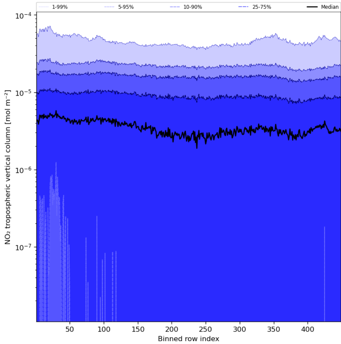
Figure 46: Along track statistics of “NO 2 tropospheric vertical column” for 2024-04-24 to 2024-04-26
