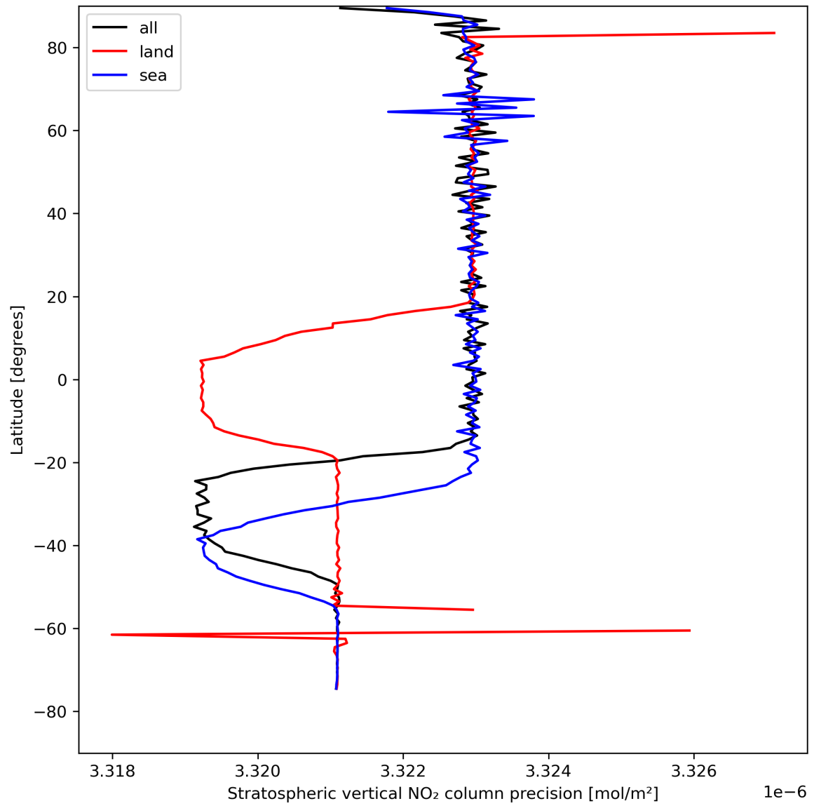
Figure 20: Zonal average of “Stratospheric vertical NO 2 column precision” for 2024-04-24 to 2024-04-26.
