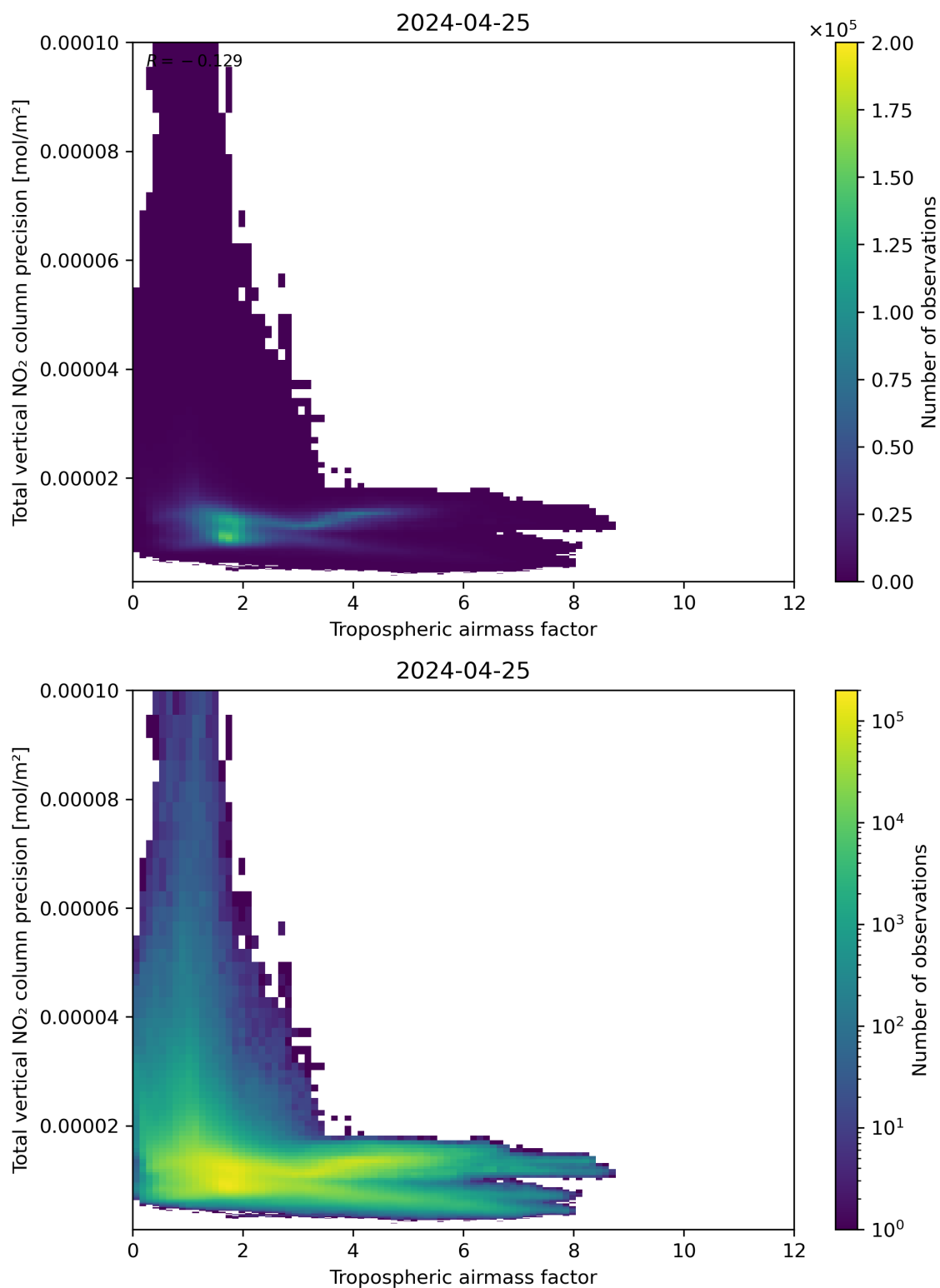
Figure 78: Scatter density plot of “Tropospheric air mass factor” against “Total vertical NO 2 column precision” for 2024-04-24 to 2024-04-26.
