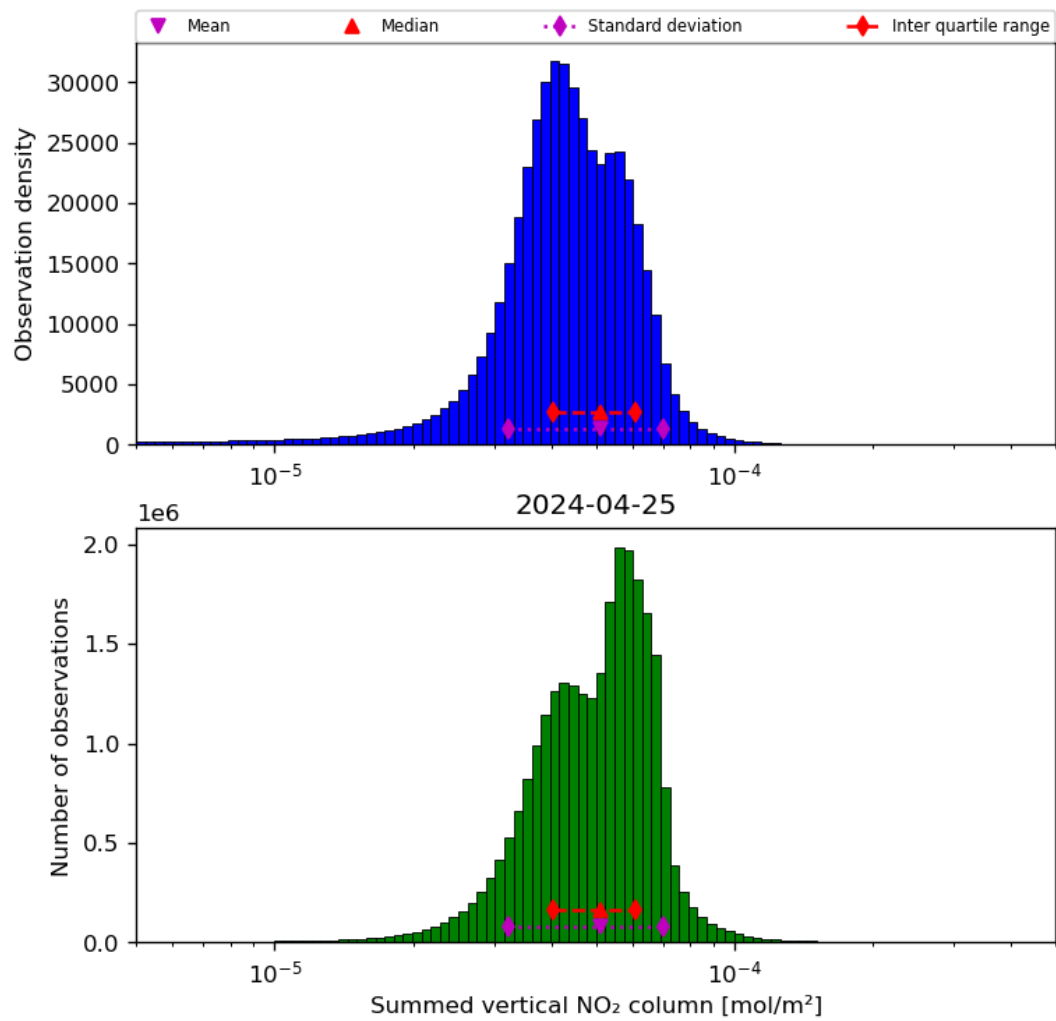
Figure 40: Histogram of "Summed vertical NO 2 column" for 2024-04-24 to 2024-04-26
