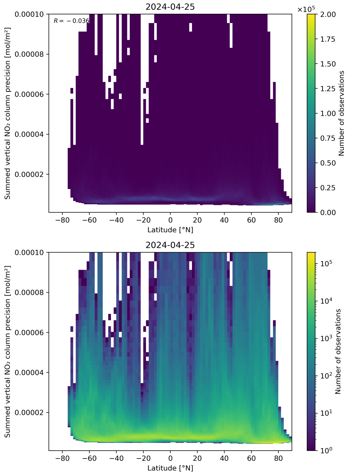
Figure 89: Scatter density plot of “Latitude” against “Summed vertical NO 2 column precision” for 2024-04-24 to 2024-04-26.
