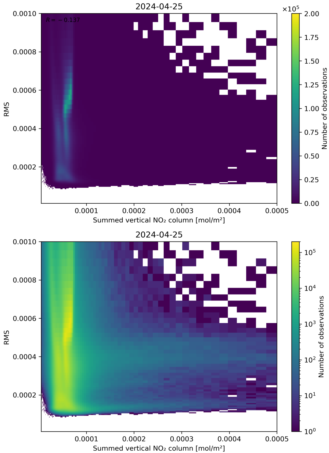
Figure 109: Scatter density plot of “Summed vertical NO 2 column” against “RMS” for 2024-04-24 to 2024-04-26.
