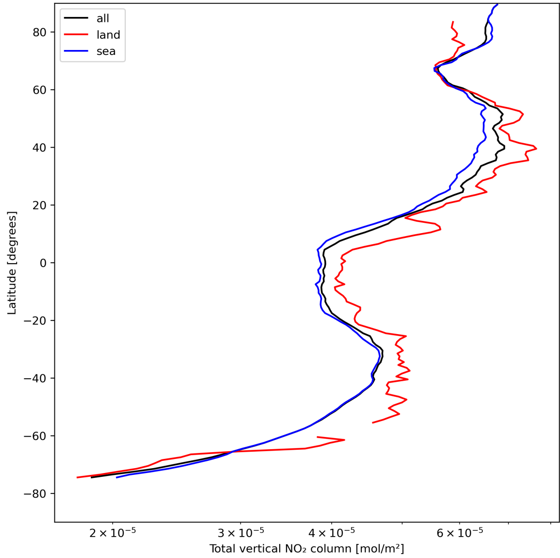
Figure 21: Zonal average of “Total vertical NO 2 column” for 2024-04-24 to 2024-04-26.
