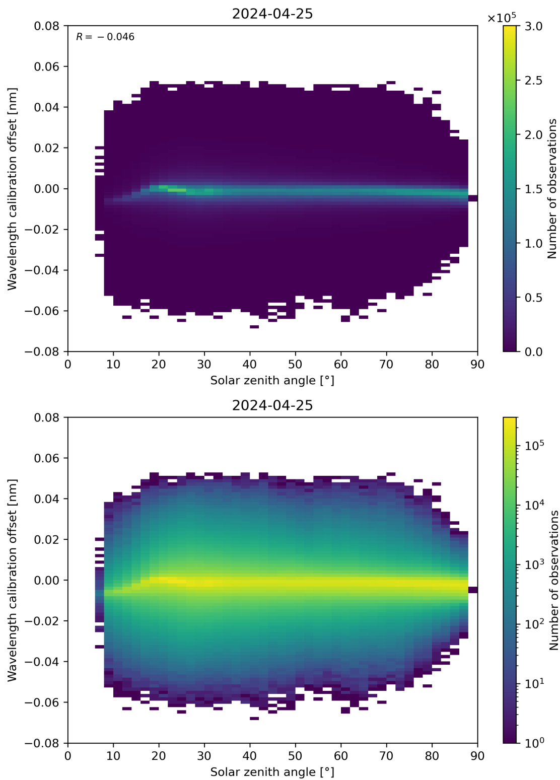
Figure 158: Scatter density plot of “Solar zenith angle” against “Wavelength calibration offset” for 2024-04-24 to 2024-04-26.
