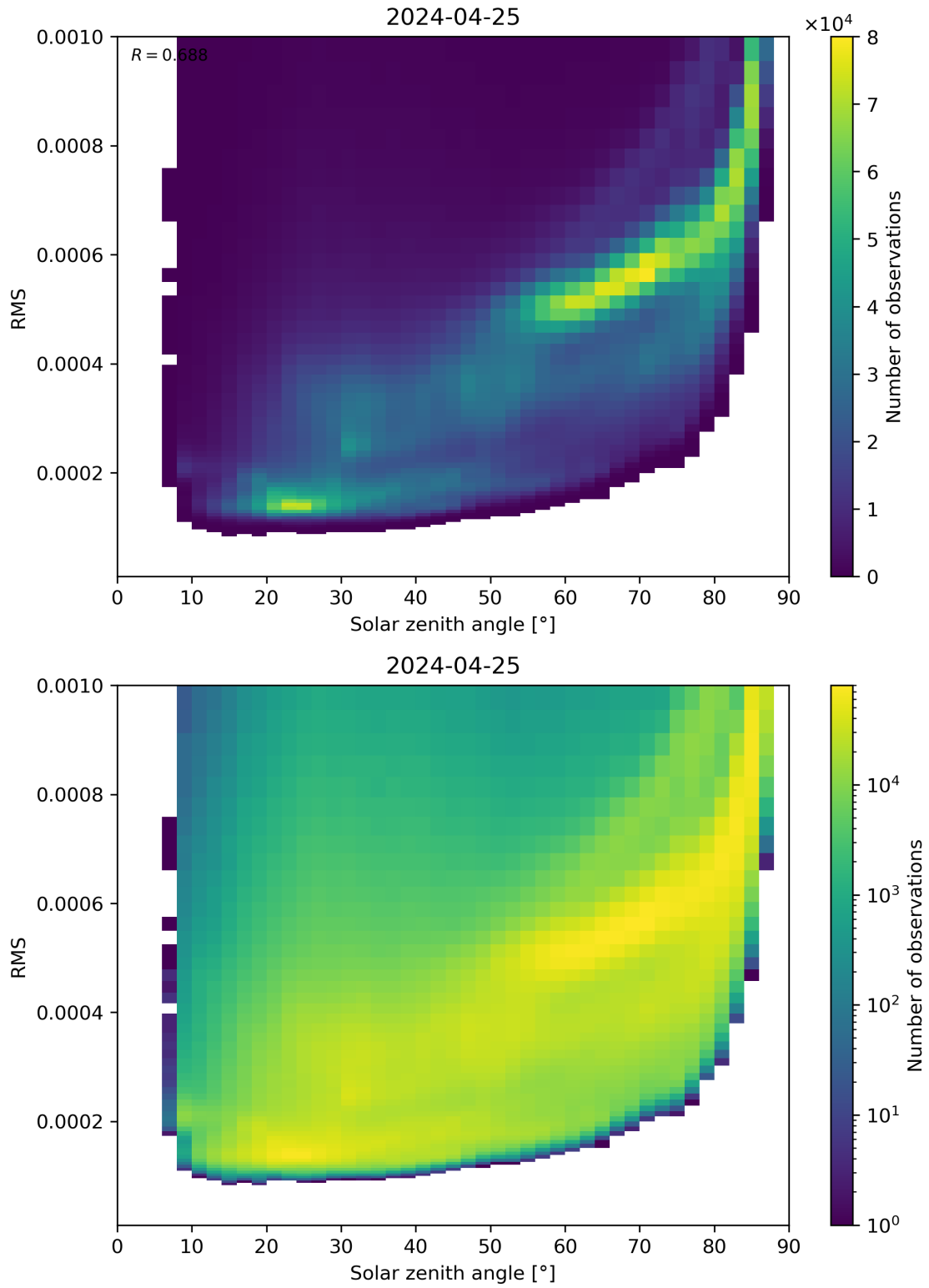
Figure 157: Scatter density plot of “Solar zenith angle” against “RMS” for 2024-04-24 to 2024-04-26.
