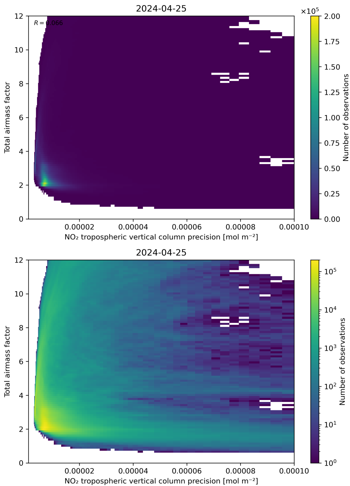
Figure 132: Scatter density plot of “NO 2 tropospheric vertical column precision” against “Total air mass factor” for 2024-04-24 to 2024-04-26.
