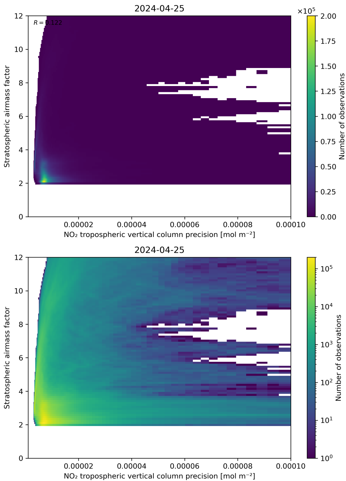
Figure 131: Scatter density plot of “NO 2 tropospheric vertical column precision” against “Stratospheric airmass factor” for 2024-04-24 to 2024-04-26.
