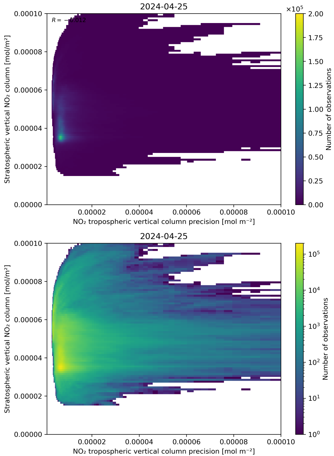
Figure 135: Scatter density plot of “NO 2 tropospheric vertical column precision” against “Stratospheric vertical NO 2 column” for 2024-04-24 to 2024-04-26.
