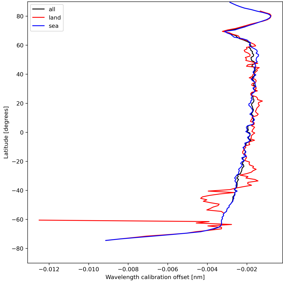
Figure 18: Zonal average of “Wavelength calibration offset” for 2024-04-24 to 2024-04-26.
