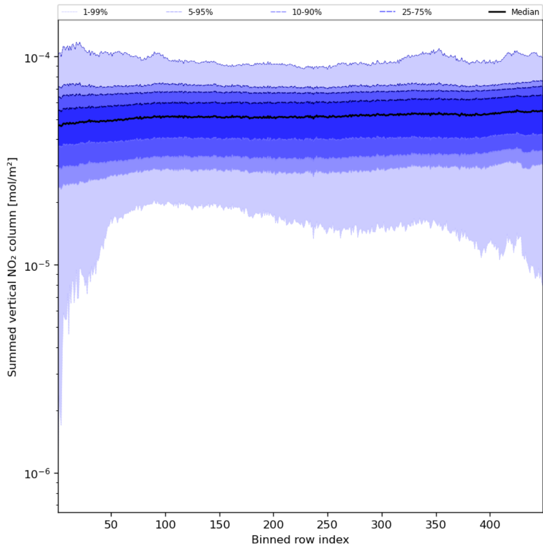
Figure 57: Along track statistics of “Summed vertical NO 2 column” for 2024-04-24 to 2024-04-26
