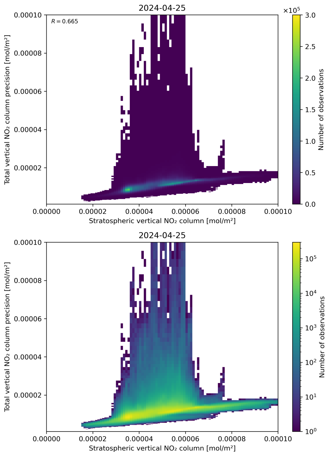
Figure 101: Scatter density plot of “Stratospheric vertical NO 2 column” against “Total vertical NO 2 column precision” for 2024-04-24 to 2024-04-26.
