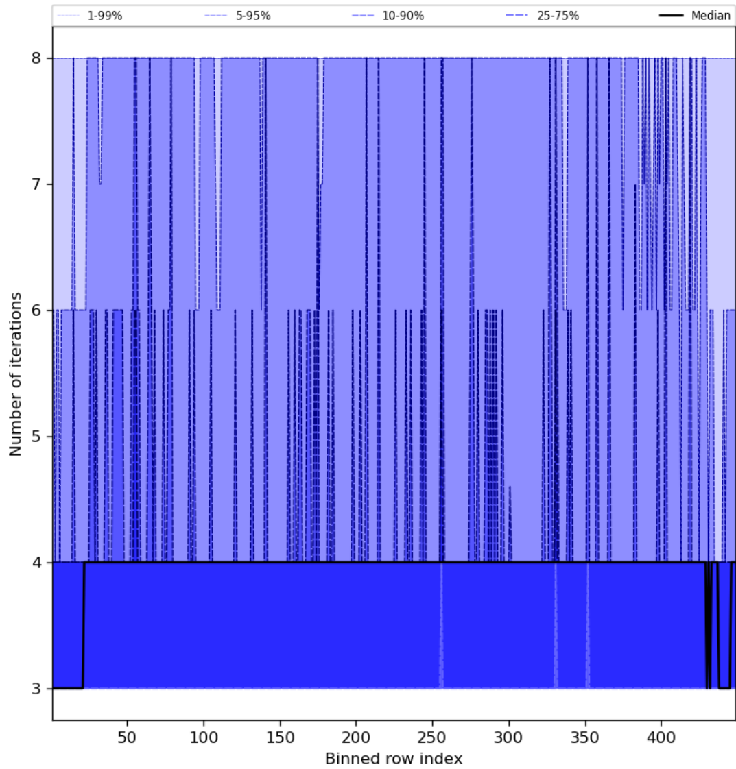
Figure 51: Along track statistics of “Number of iterations” for 2024-04-24 to 2024-04-26
