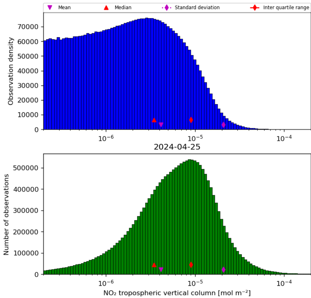
Figure 29: Histogram of “NO 2 tropospheric vertical column” for 2024-04-24 to 2024-04-26
