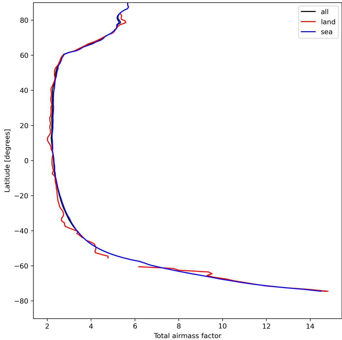
Figure 15: Zonal average of “Total airmass factor” for 2024-04-24 to 2024-04-26.
