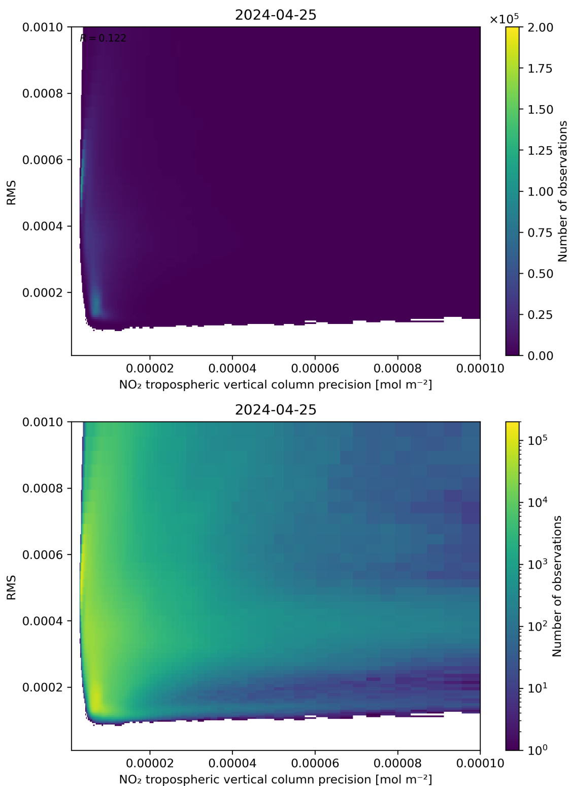
Figure 140: Scatter density plot of “NO 2 tropospheric vertical column precision” against “RMS” for 2024-04-24 to 2024-04-26.
