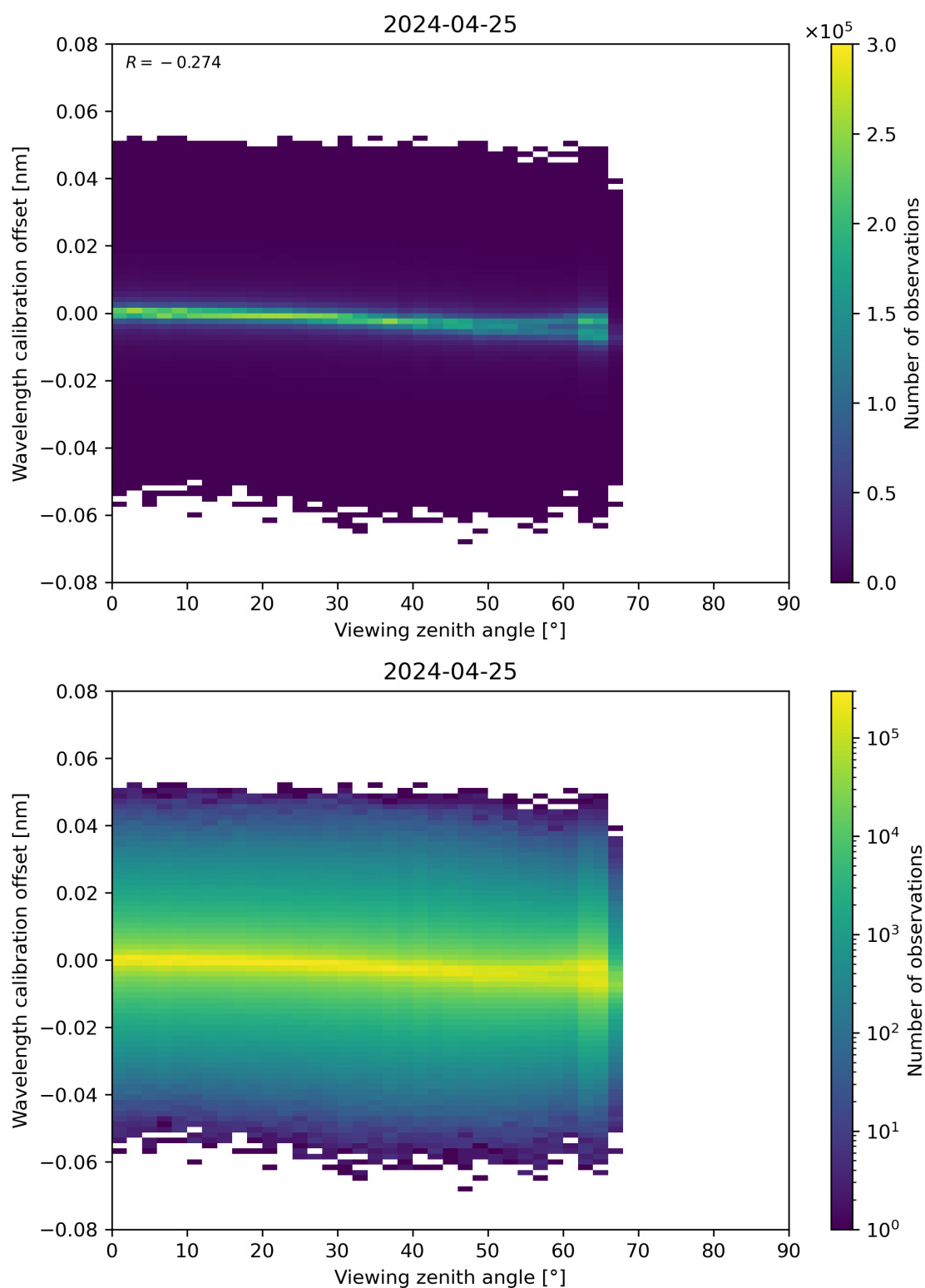
Figure 173: Scatter density plot of “Viewing zenith angle” against “Wavelength calibration offset” for 2024-04-24 to 2024-04-26.
