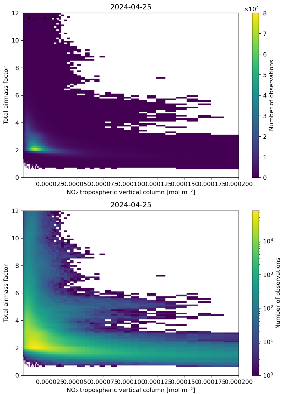
Figure 122: Scatter density plot of “NO 2 tropospheric vertical column” against “Total air mass factor” for 2024-04-24 to 2024-04-26.
