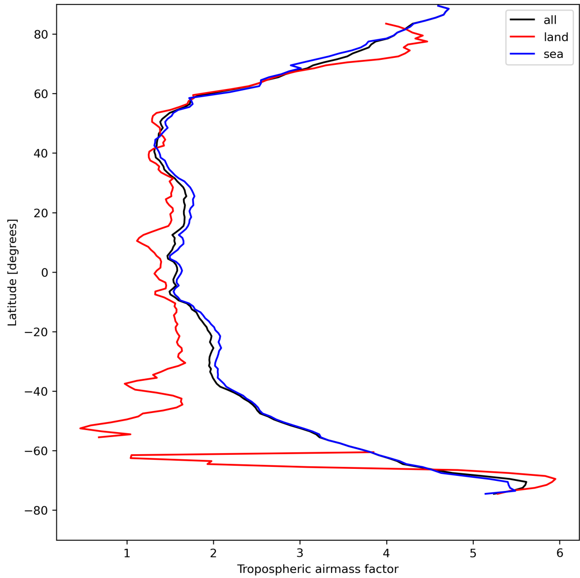
Figure 14: Zonal average of “Tropospheric airmass factor” for 2024-04-24 to 2024-04-26.
