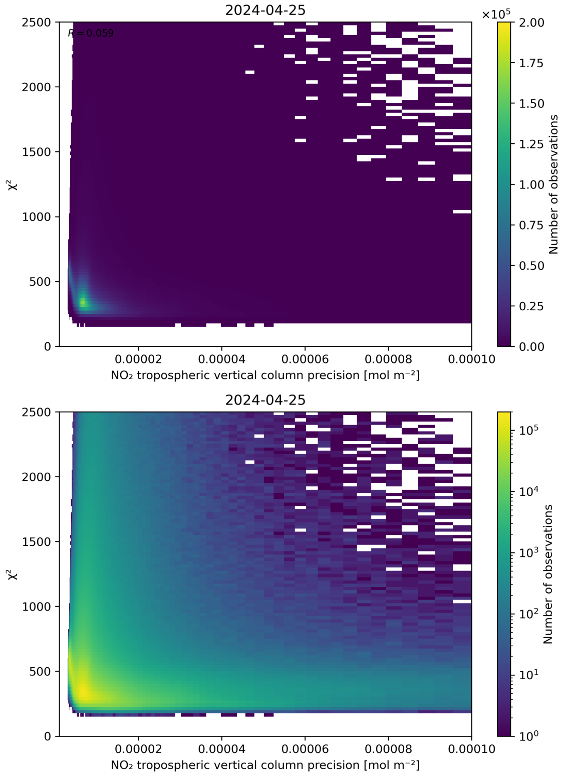
Figure 134: Scatter density plot of “NO 2 tropospheric vertical column precision” against “ \chi^2 ” for 2024-04-24 to 2024-04-26.
