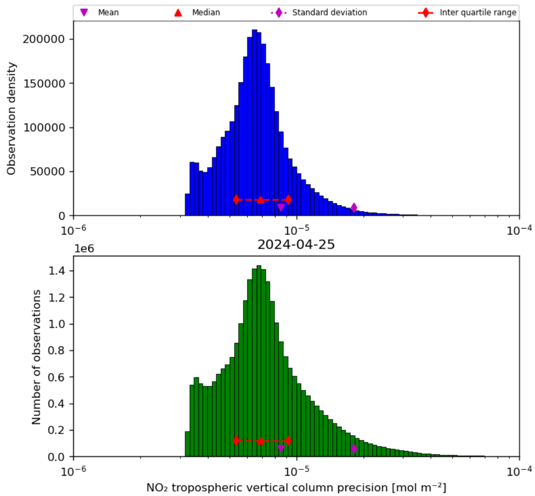
Figure 30: Histogram of “NO 2 tropospheric vertical column precision” for 2024-04-24 to 2024-04-26
