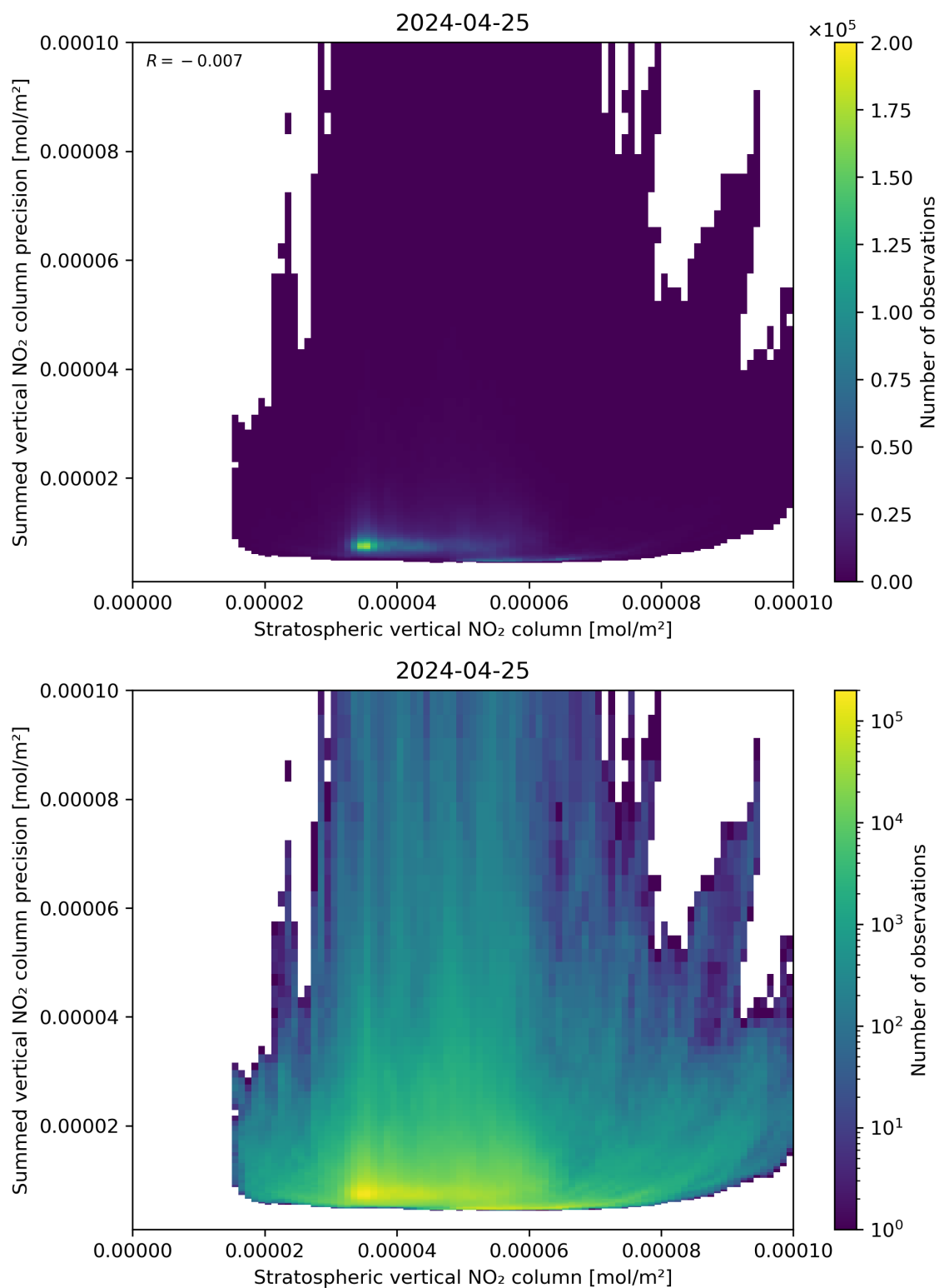
Figure 99: Scatter density plot of “Stratospheric vertical NO 2 column” against “Summed vertical NO 2 column precision” for 2024-04-24 to 2024-04-26.
