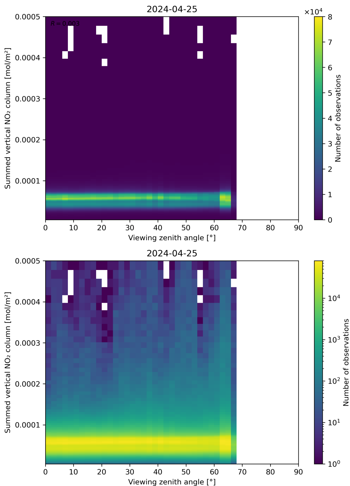
Figure 165: Scatter density plot of “Viewing zenith angle” against “Summed vertical NO 2 column” for 2024-04-24 to 2024-04-26.
