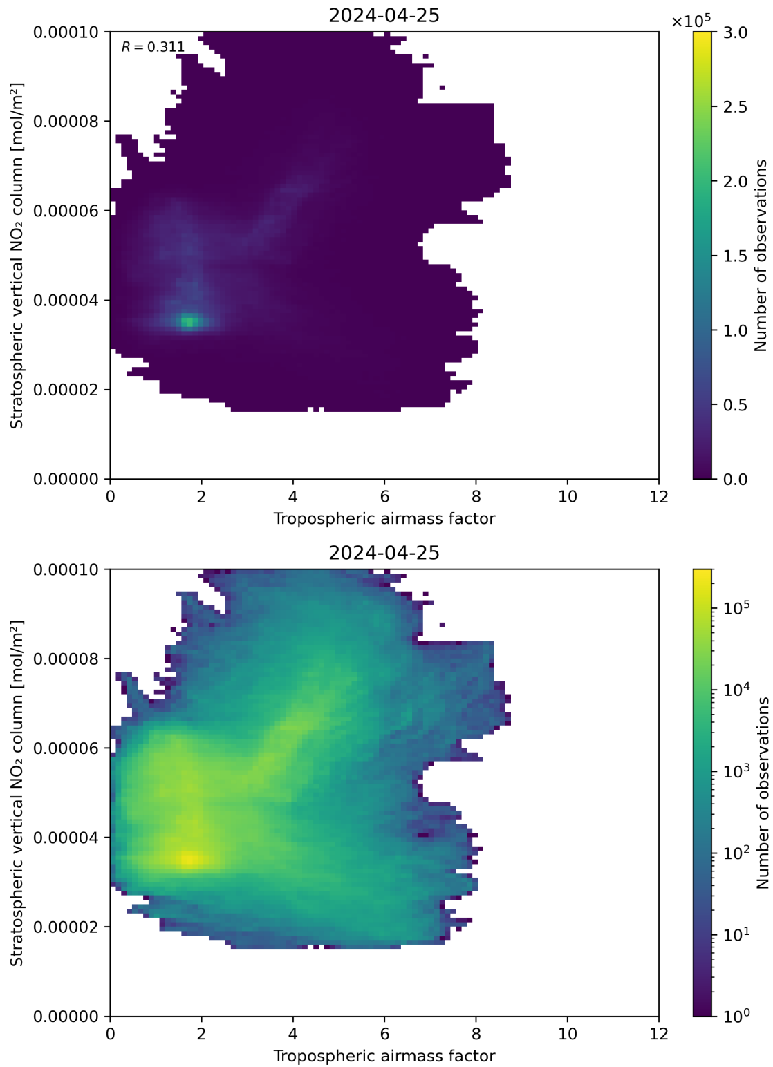
Figure 74: Scatter density plot of “Tropospheric air mass factor” against “Stratospheric vertical NO 2 column” for 2024-04-24 to 2024-04-26.
