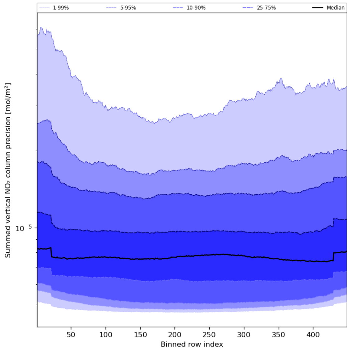
Figure 58: Along track statistics of “Summed vertical NO 2 column precision” for 2024-04-24 to 2024-04-26
