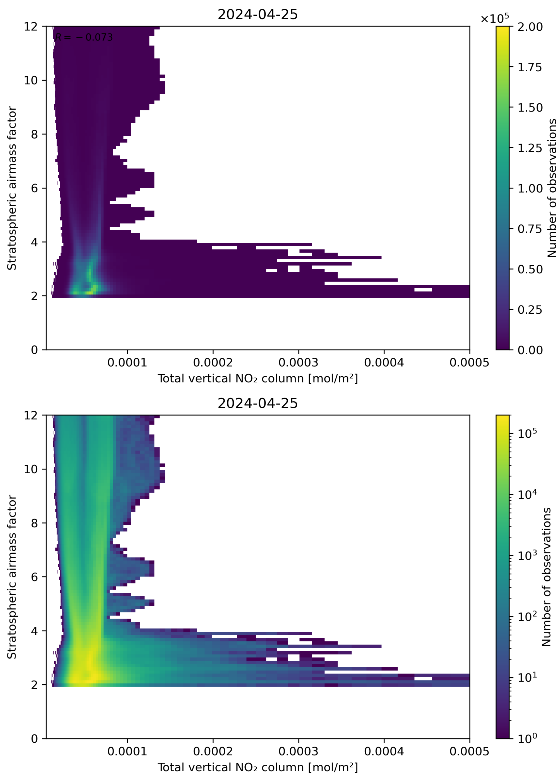
Figure 110: Scatter density plot of “Total vertical NO 2 column” against “Stratospheric air mass factor” for 2024-04-24 to 2024-04-26.
