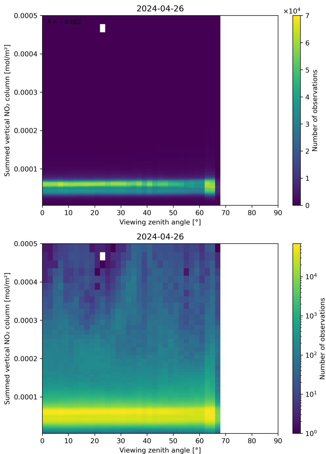
Figure 165: Scatter density plot of “Viewing zenith angle” against “Summed vertical NO 2 column” for 2024-04-26 to 2024-04-27.
