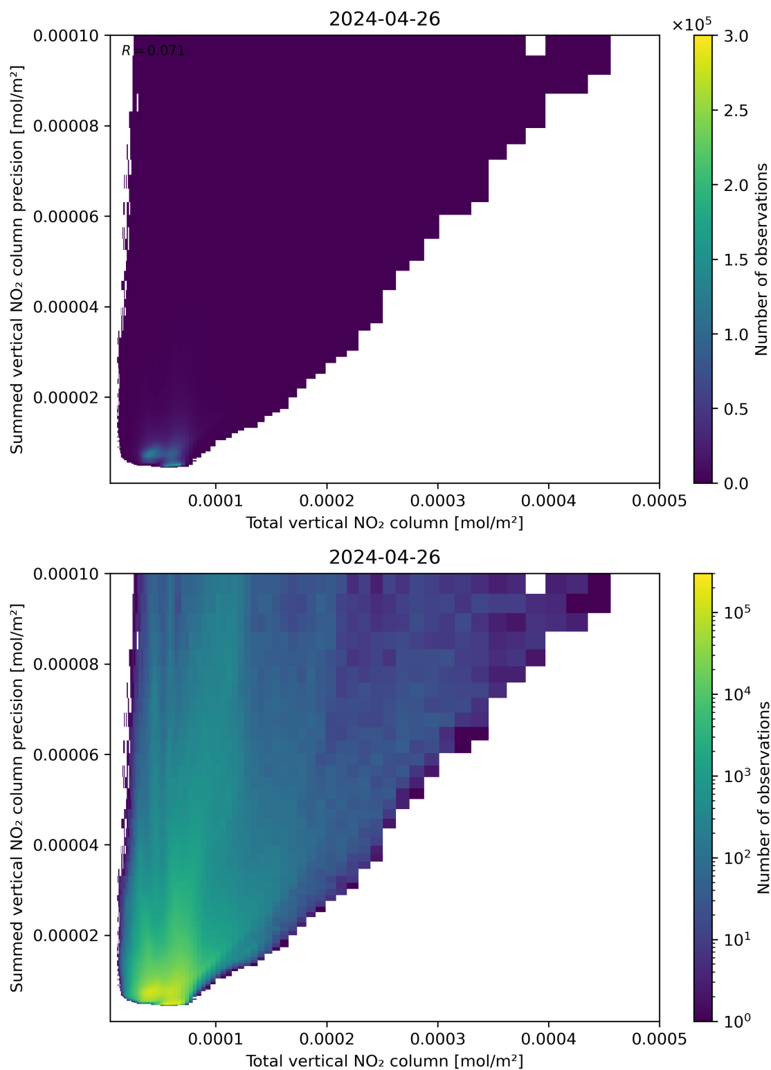
Figure 113: Scatter density plot of “Total vertical NO 2 column” against “Summed vertical NO 2 column precision” for 2024-04-26 to 2024-04-27.
