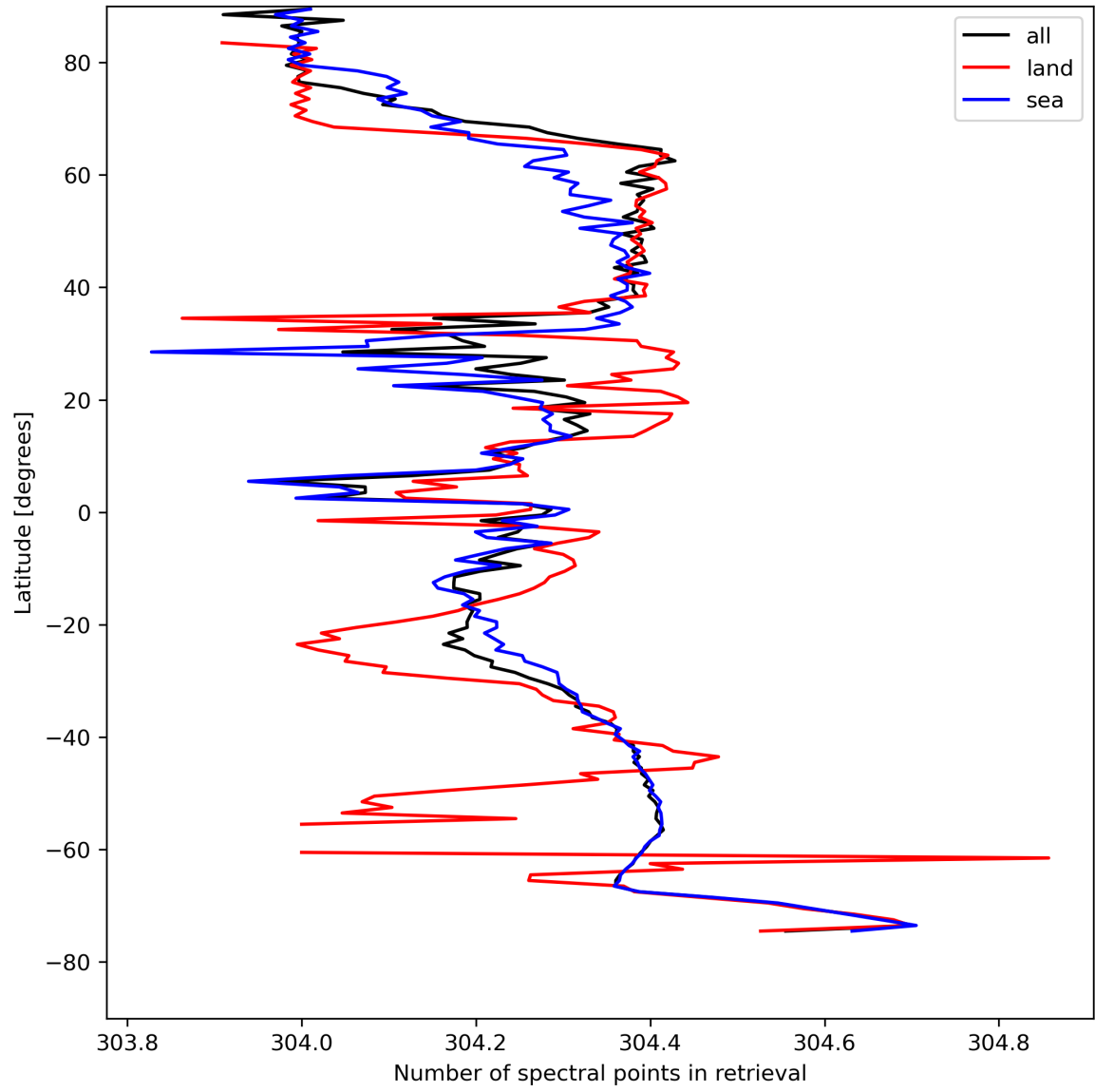
Figure 16: Zonal average of “Number of spectral points in retrieval” for 2024-04-26 to 2024-04-27.
