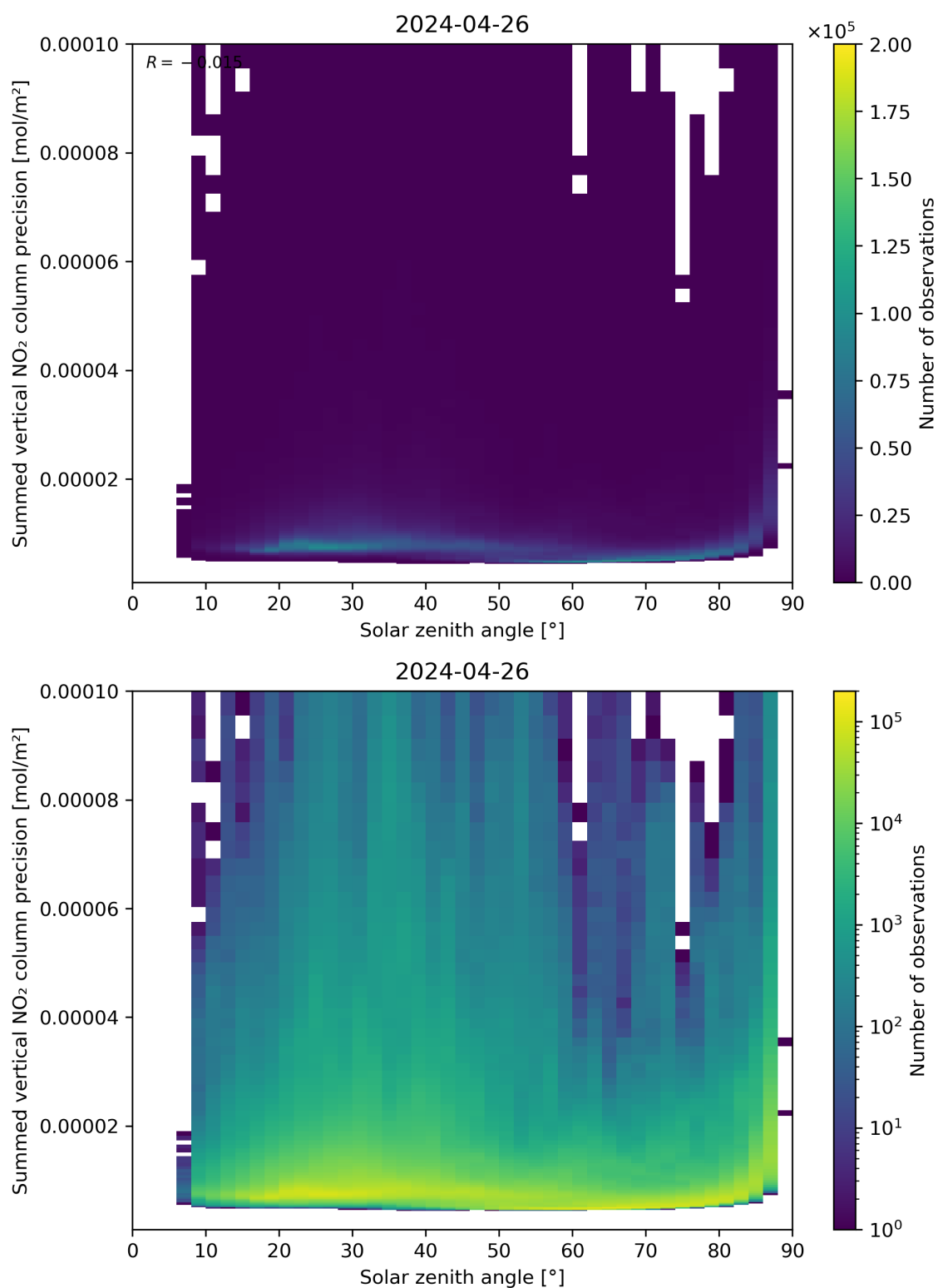
Figure 152: Scatter density plot of “Solar zenith angle” against “Summed vertical NO 2 column precision” for 2024-04-26 to 2024-04-27.
