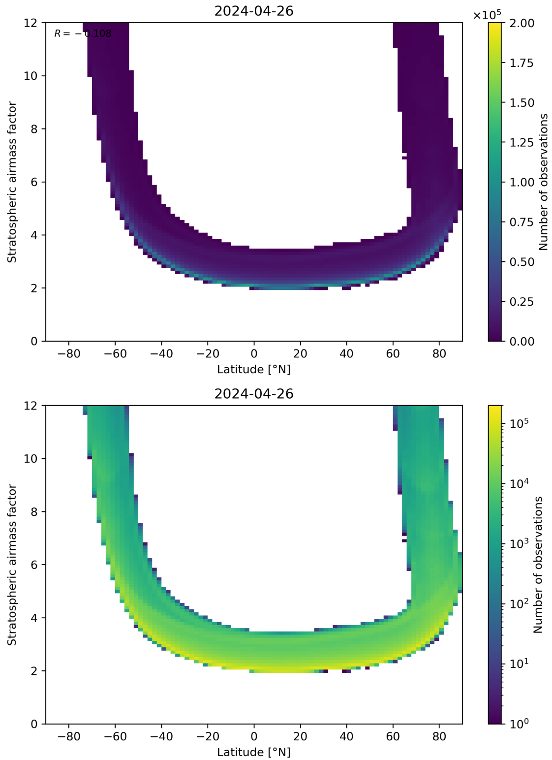
Figure 83: Scatter density plot of “Latitude” against “Stratospheric airmass factor” for 2024-04-26 to 2024-04-27.
