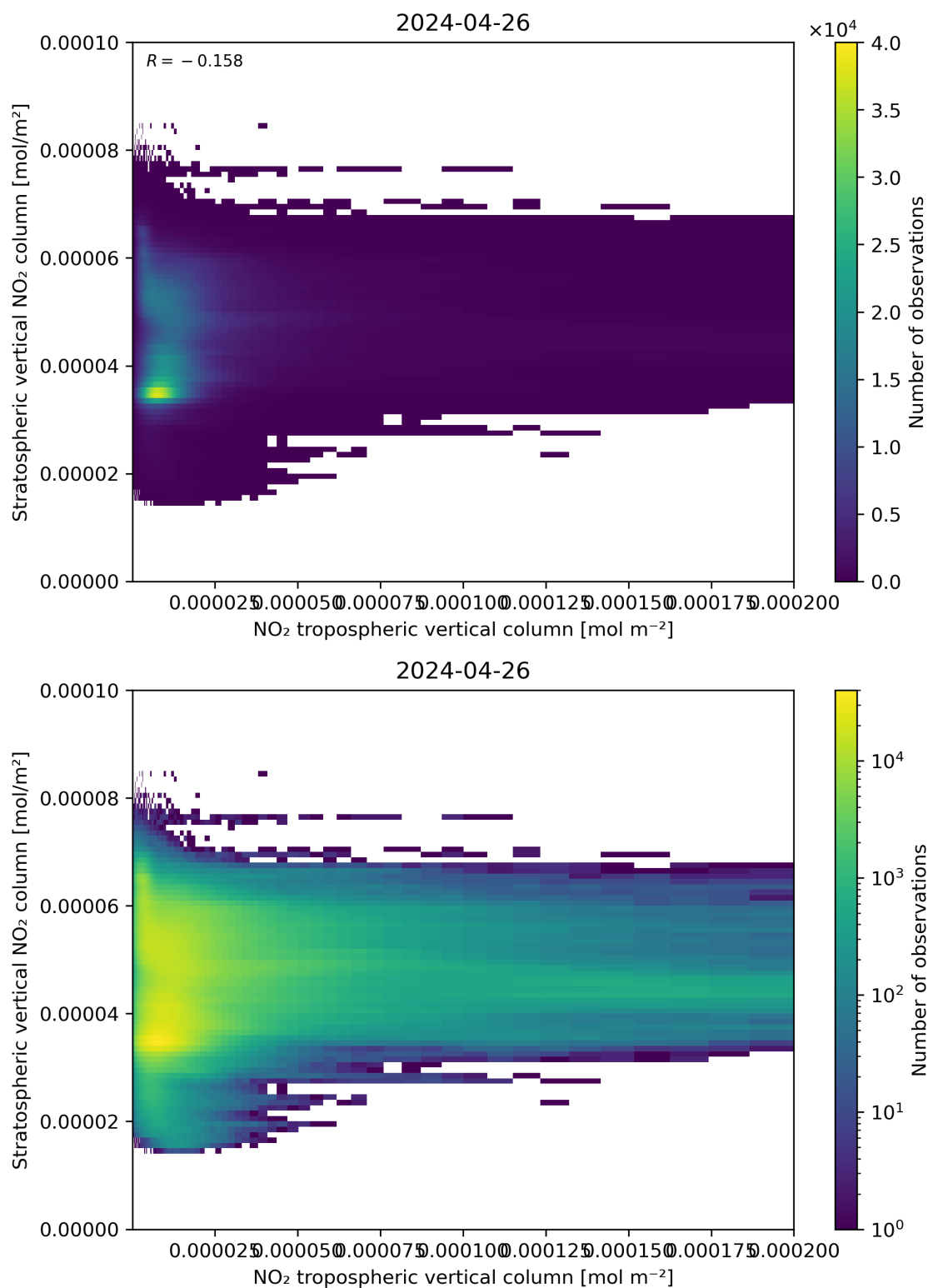
Figure 125: Scatter density plot of “NO 2 tropospheric vertical column” against “Stratospheric vertical NO 2 column” for 2024-04-26 to 2024-04-27.
