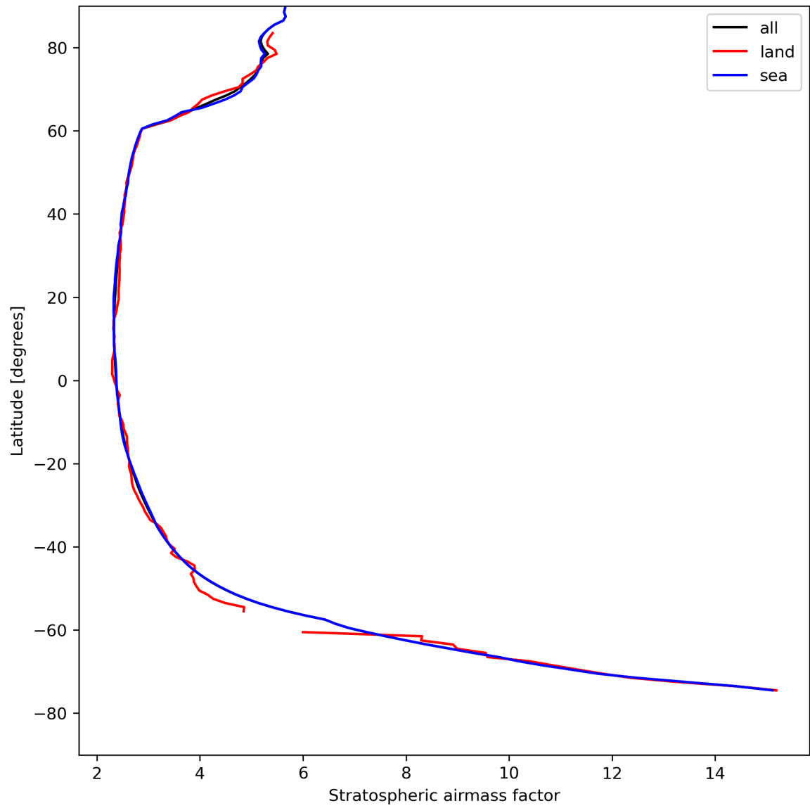
Figure 27: Zonal average of “Stratospheric air mass factor” for 2024-04-26 to 2024-04-27.
