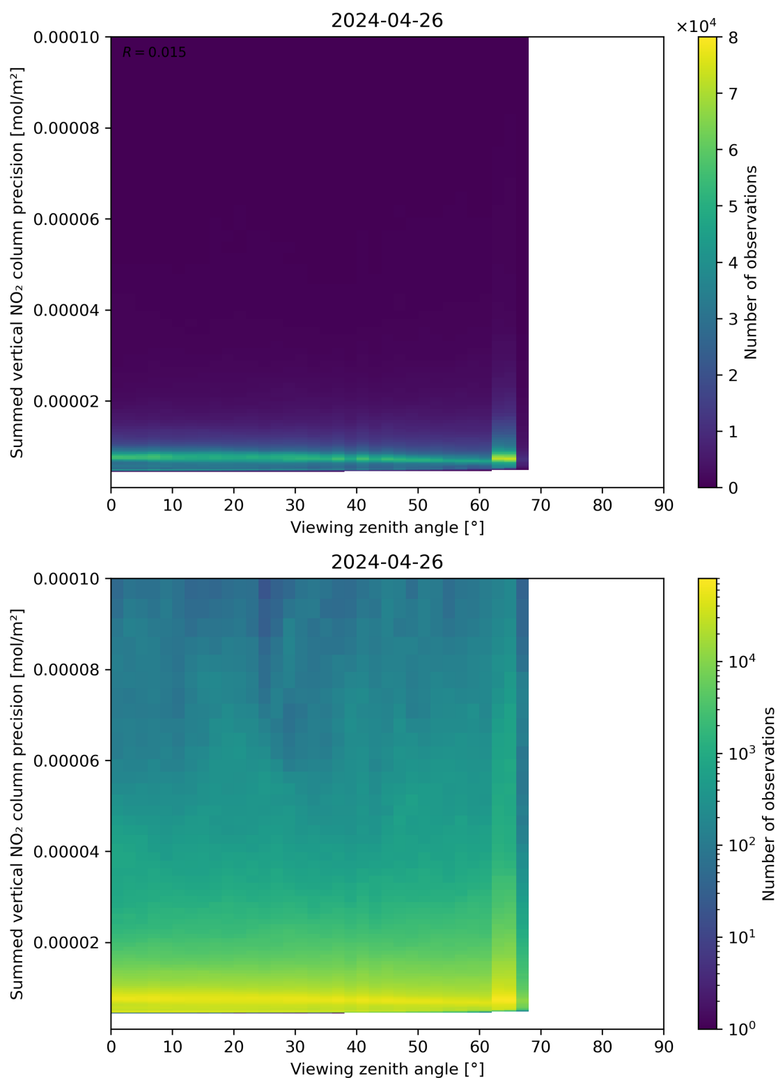
Figure 166: Scatter density plot of “Viewing zenith angle” against “Summed vertical NO 2 column precision” for 2024-04-26 to 2024-04-27.
