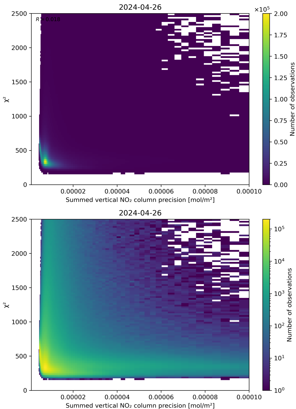
Figure 107: Scatter density plot of “Summed vertical NO 2 column precision” against “ \chi^2 ” for 2024-04-26 to 2024-04-27.
