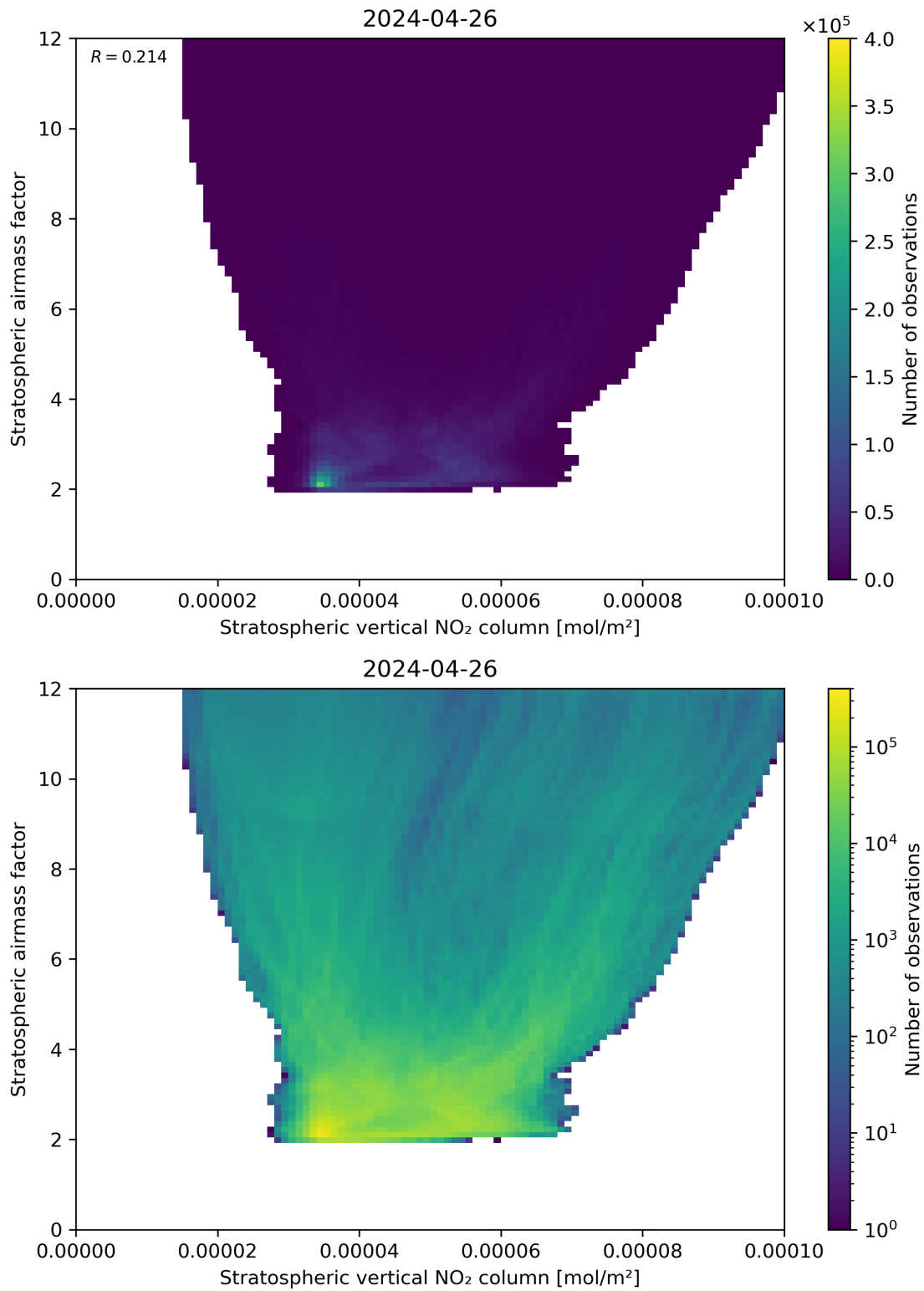
Figure 96: Scatter density plot of “Stratospheric vertical NO 2 column” against “Stratospheric airmass factor” for 2024-04-26 to 2024-04-27.
