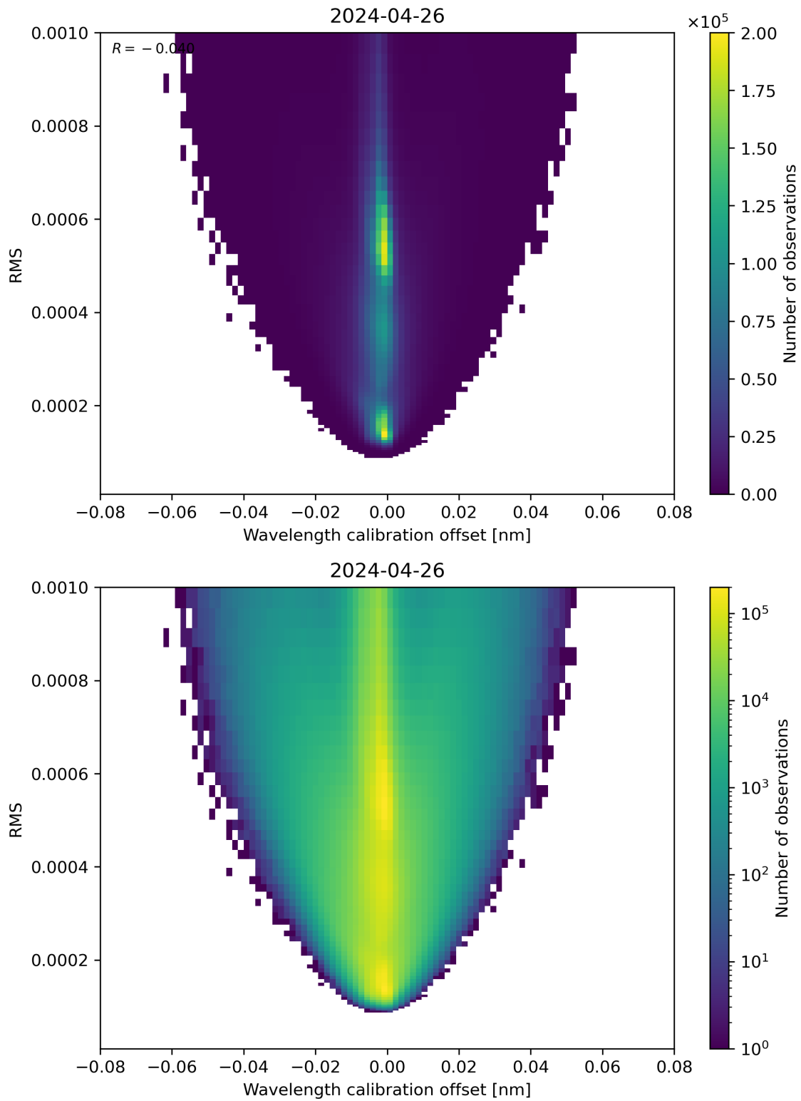
Figure 181: Scatter density plot of “Wavelength calibration offset” against “RMS” for 2024-04-26 to 2024-04-27.
