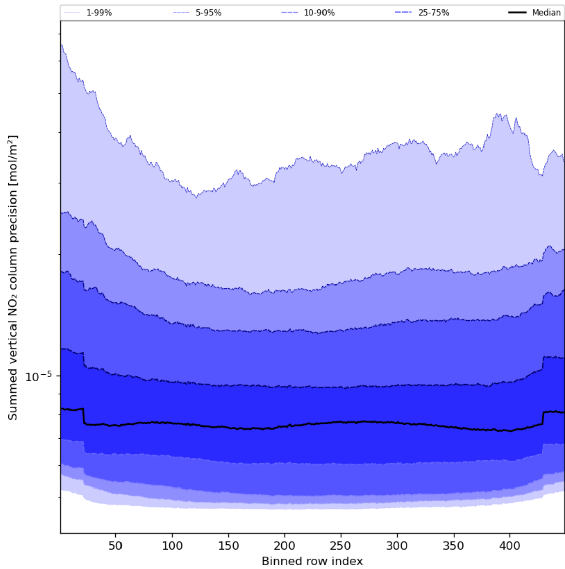
Figure 58: Along track statistics of “Summed vertical NO 2 column precision” for 2024-04-26 to 2024-04-27
