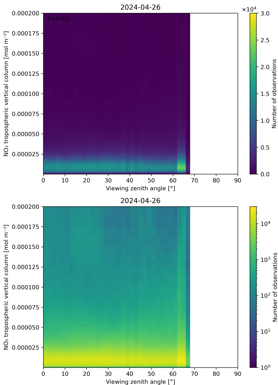
Figure 169: Scatter density plot of “Viewing zenith angle” against “NO 2 tropospheric vertical column” for 2024-04-26 to 2024-04-27.
