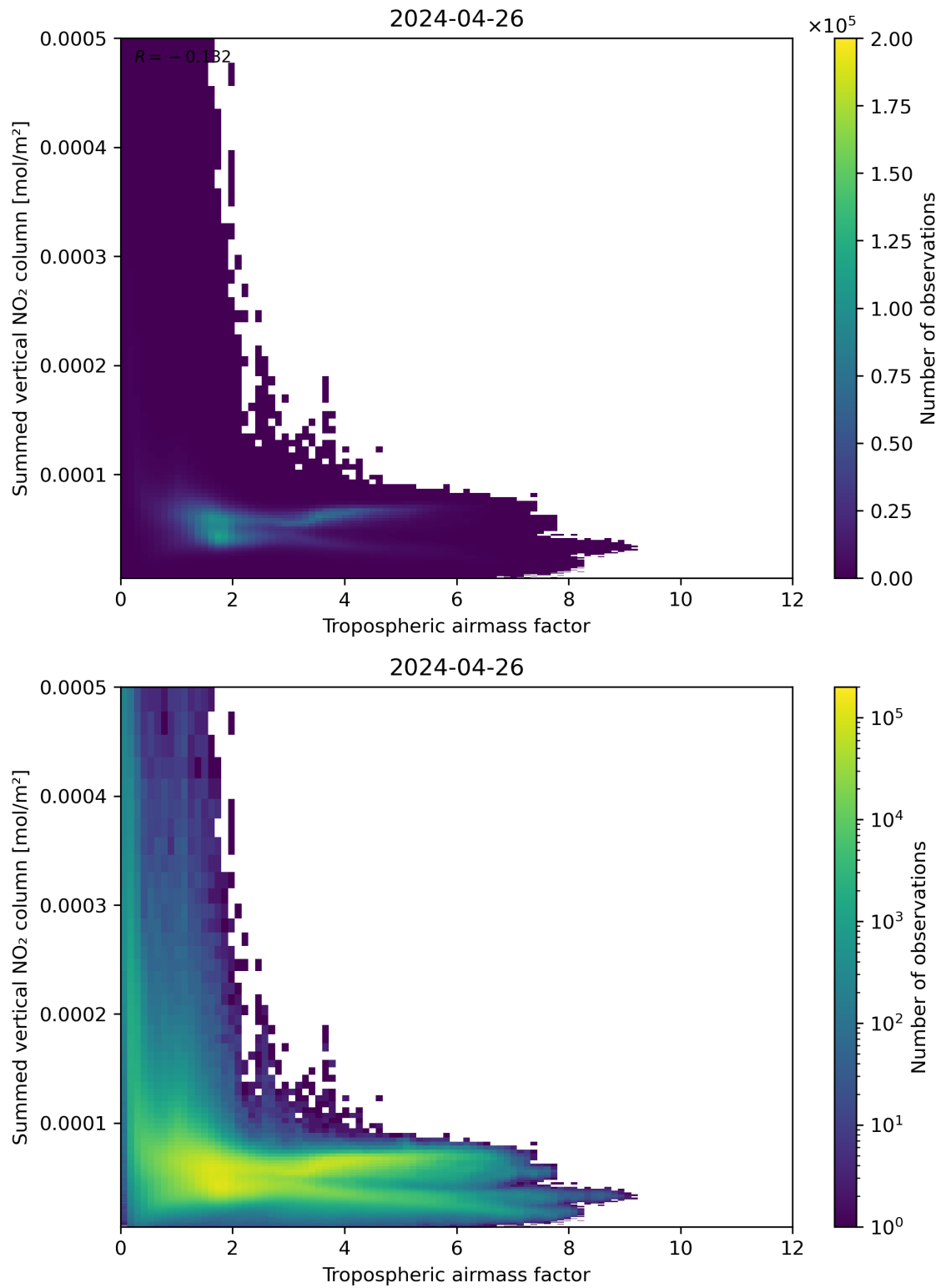
Figure 75: Scatter density plot of “Tropospheric airmass factor” against “Summed vertical NO 2 column” for 2024-04-26 to 2024-04-27.
