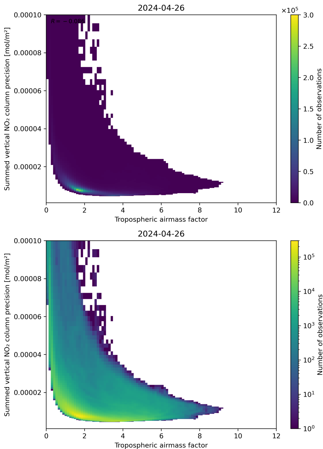
Figure 76: Scatter density plot of “Tropospheric air mass factor” against “Summed vertical NO 2 column precision” for 2024-04-26 to 2024-04-27.
