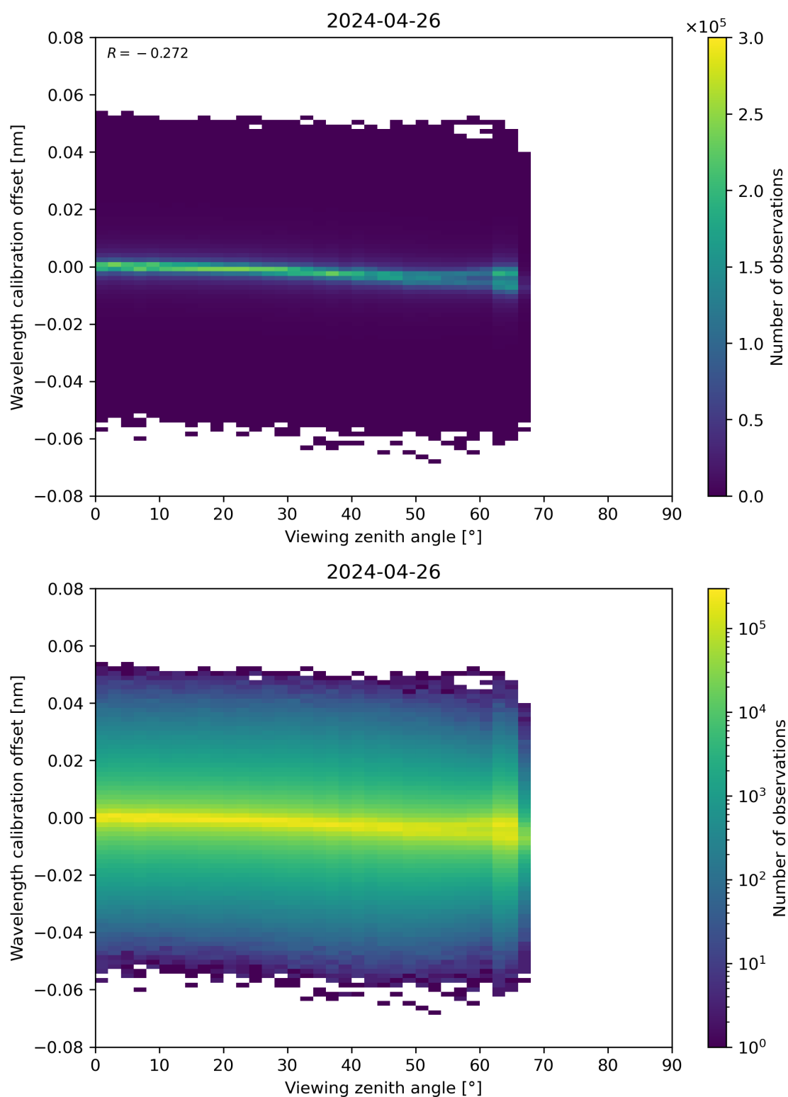
Figure 173: Scatter density plot of “Viewing zenith angle” against “Wavelength calibration offset” for 2024-04-26 to 2024-04-27.
