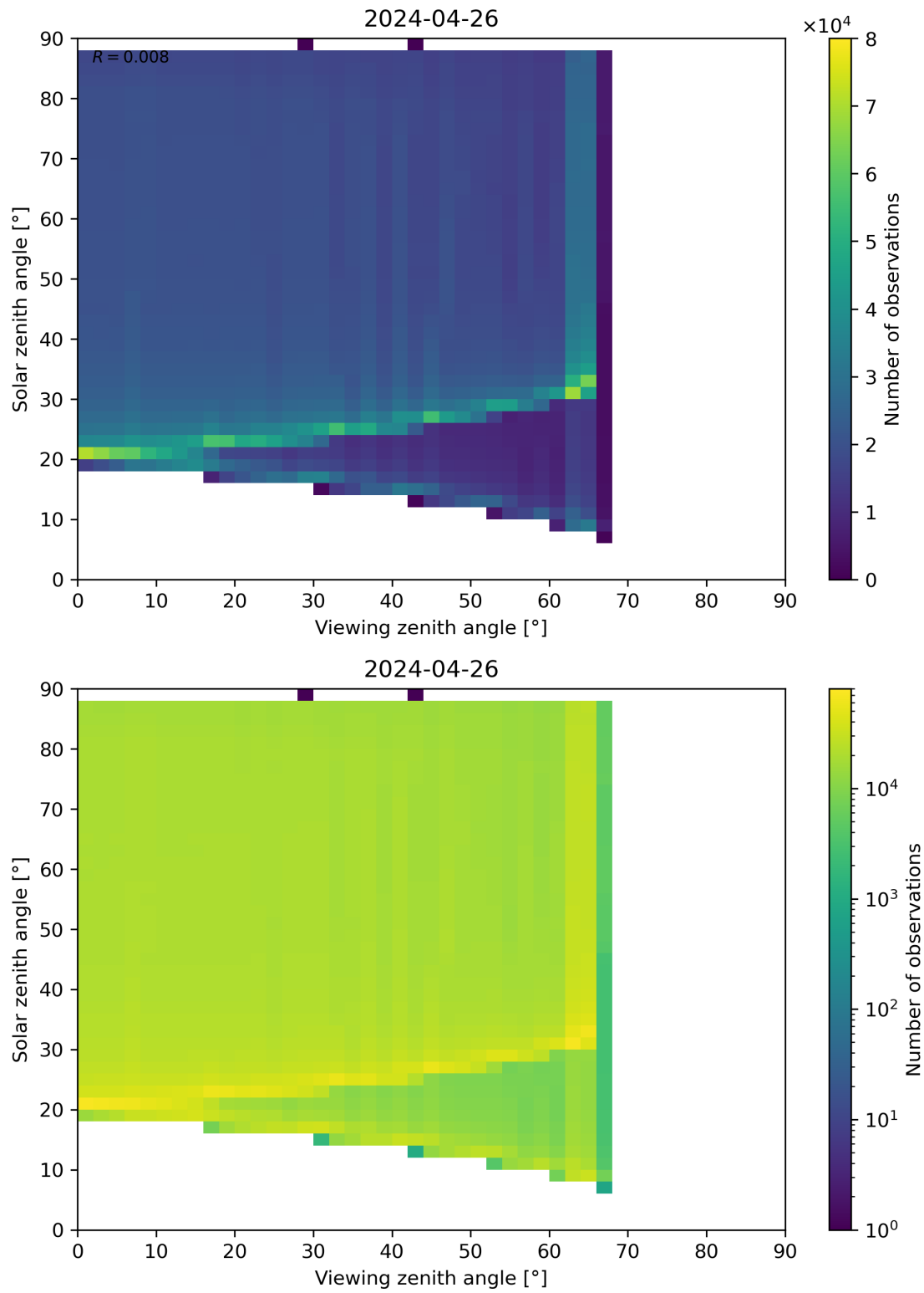
Figure 172: Scatter density plot of “Viewing zenith angle” against “Solar zenith angle” for 2024-04-26 to 2024-04-27.
