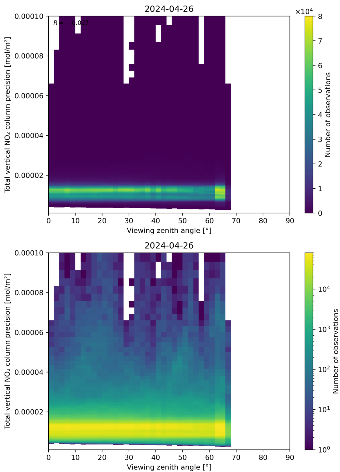
Figure 168: Scatter density plot of “Viewing zenith angle” against “Total vertical NO 2 column precision” for 2024-04-26 to 2024-04-27.
