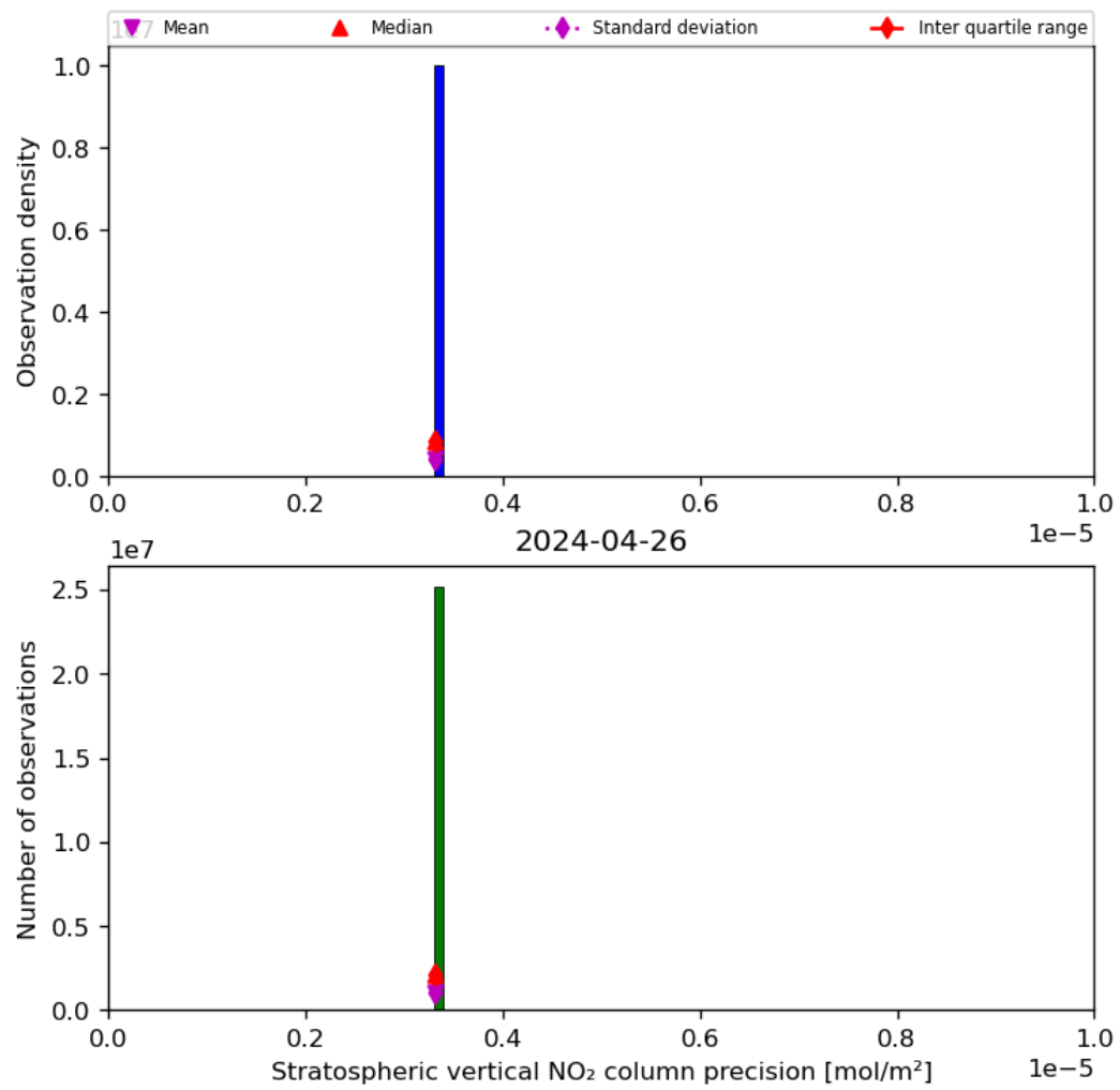
Figure 37: Histogram of “Stratospheric vertical NO 2 column precision” for 2024-04-26 to 2024-04-27
