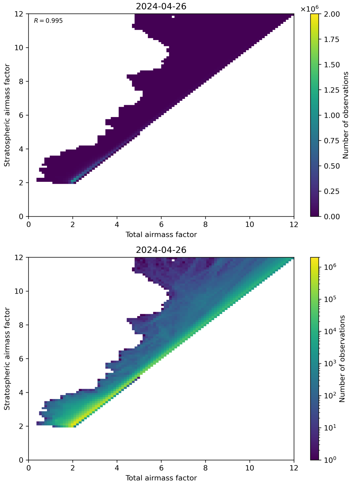
Figure 62: Scatter density plot of “Total airmass factor” against “Stratospheric airmass factor” for 2024-04-26 to 2024-04-27.
