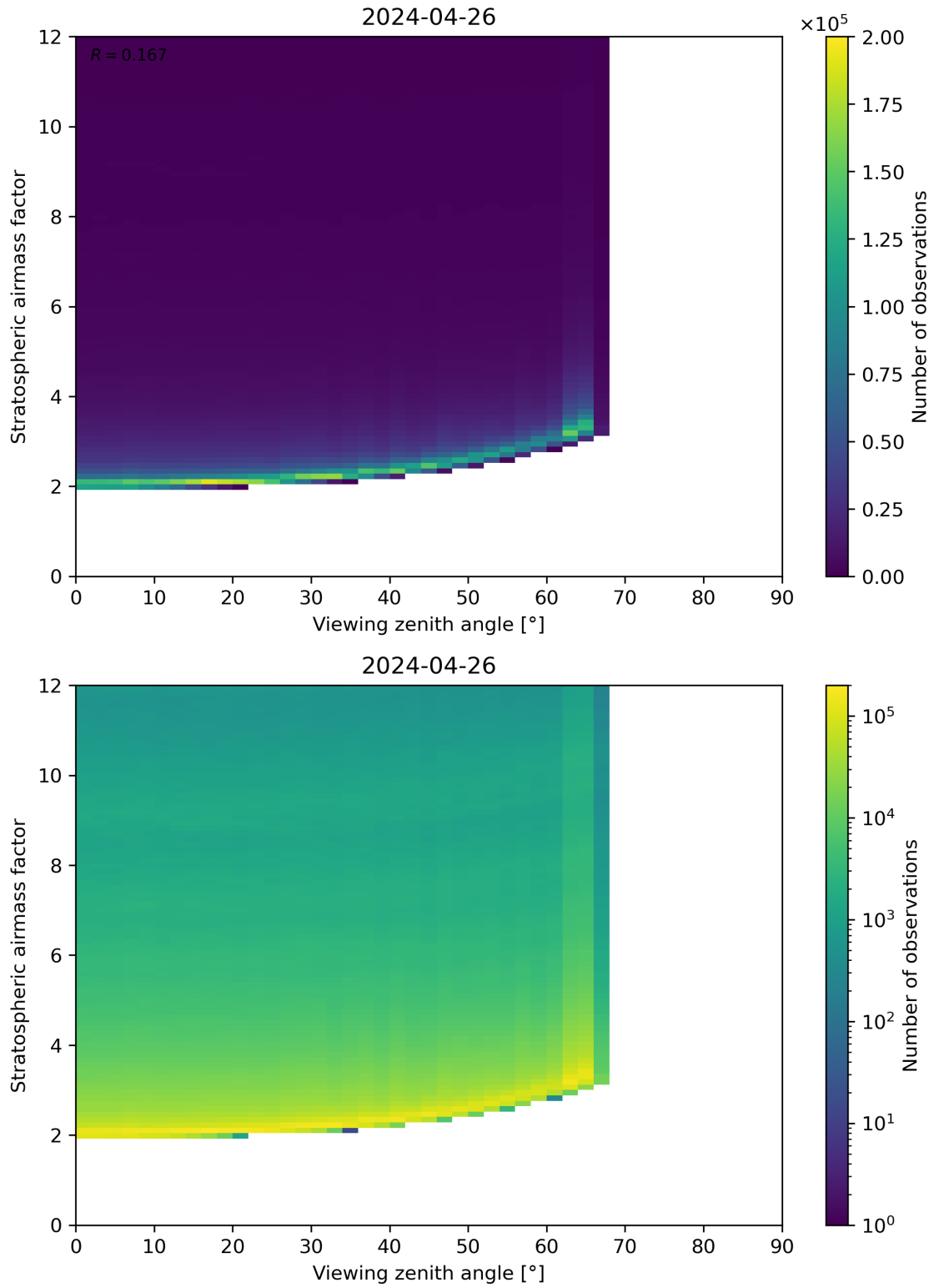
Figure 159: Scatter density plot of “Viewing zenith angle” against “Stratospheric airmass factor” for 2024-04-26 to 2024-04-27.
