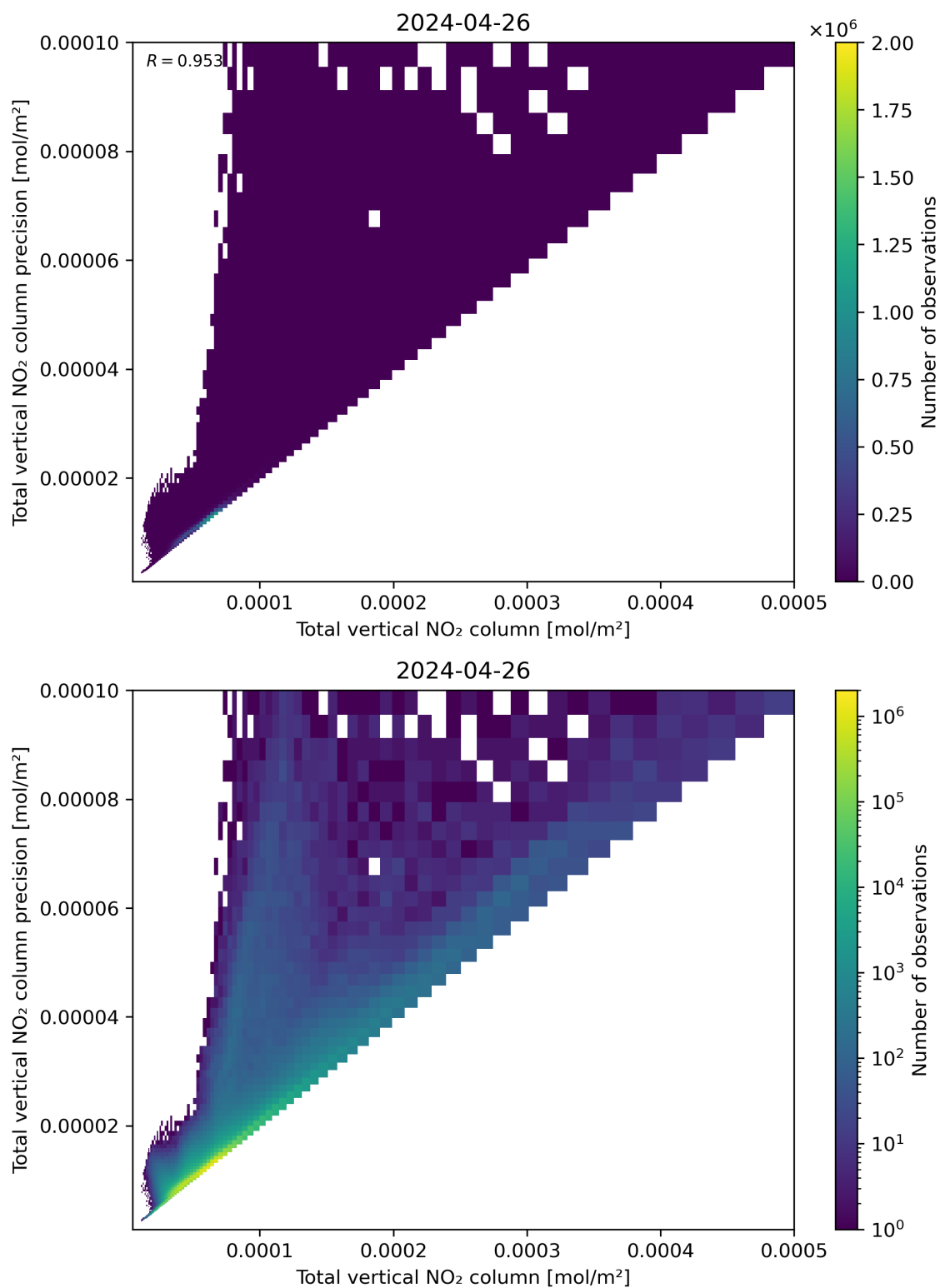
Figure 114: Scatter density plot of “Total vertical NO 2 column” against “Total vertical NO 2 column precision” for 2024-04-26 to 2024-04-27.
