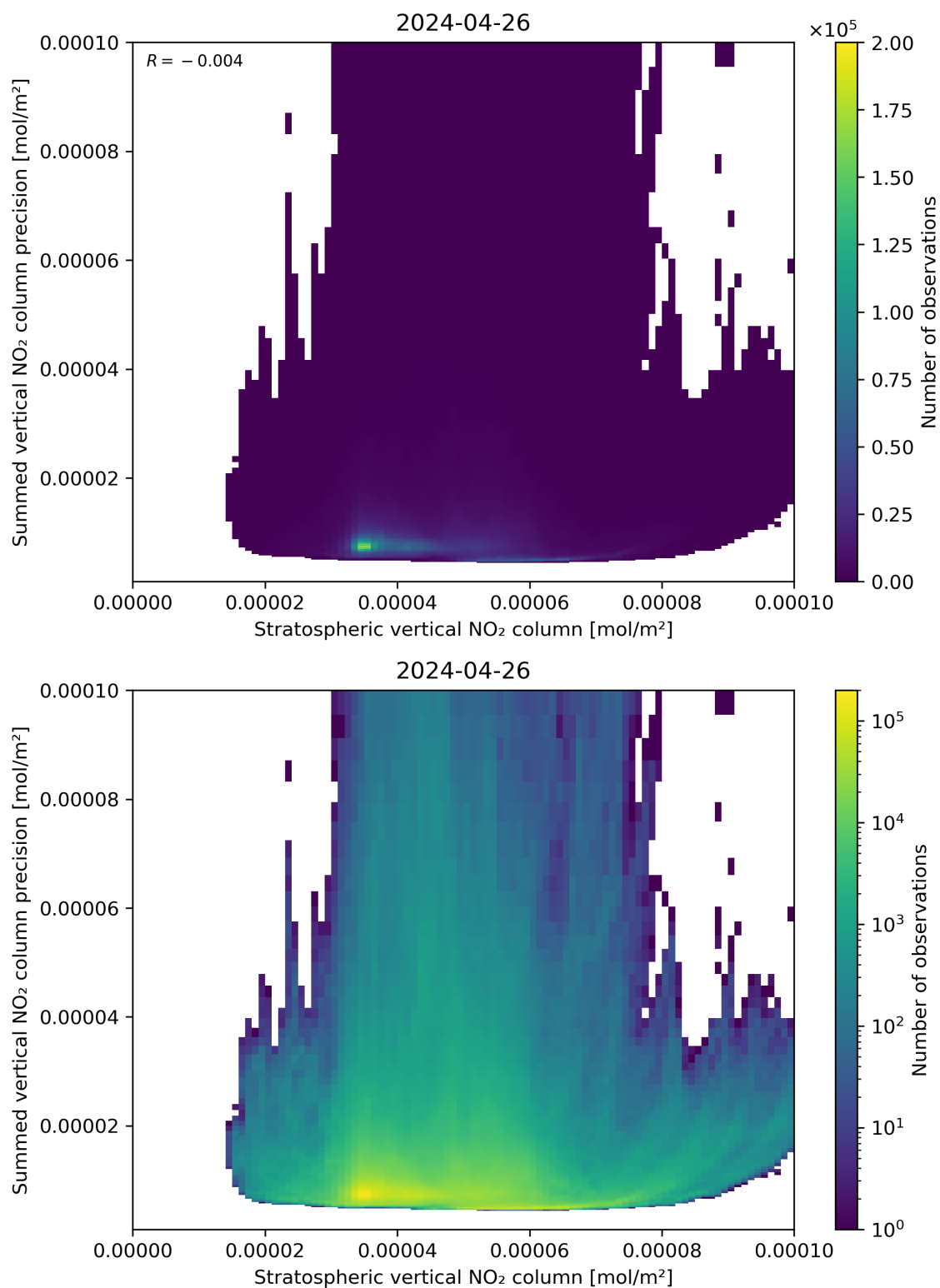
Figure 99: Scatter density plot of “Stratospheric vertical NO 2 column” against “Summed vertical NO 2 column precision” for 2024-04-26 to 2024-04-27.
