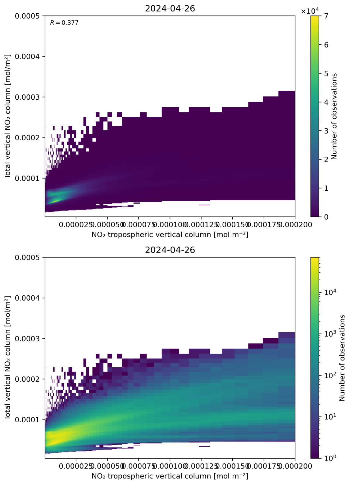
Figure 128: Scatter density plot of “NO 2 tropospheric vertical column” against “Total vertical NO 2 column” for 2024-04-26 to 2024-04-27.
