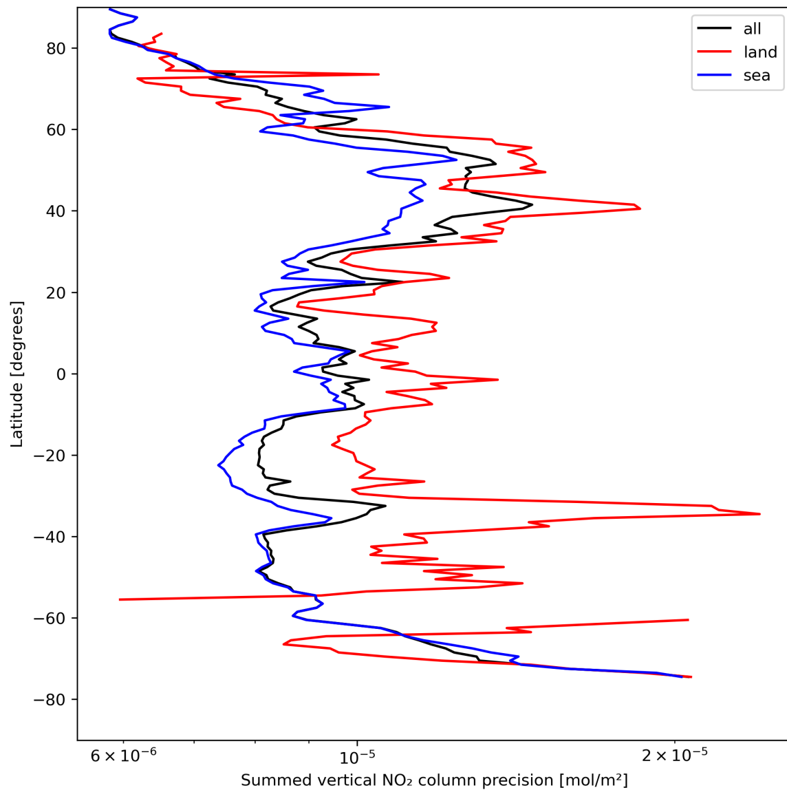
Figure 24: Zonal average of “Summed vertical NO 2 column precision” for 2024-04-26 to 2024-04-27.
