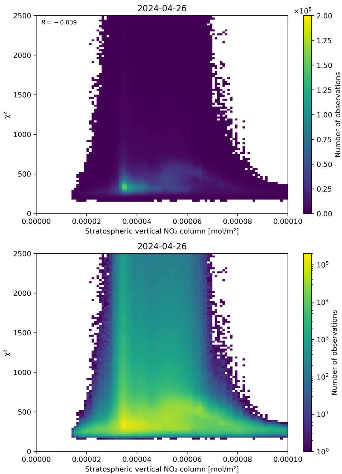
Figure 97: Scatter density plot of “Stratospheric vertical NO 2 column” against “ \chi^2 ” for 2024-04-26 to 2024-04-27.
