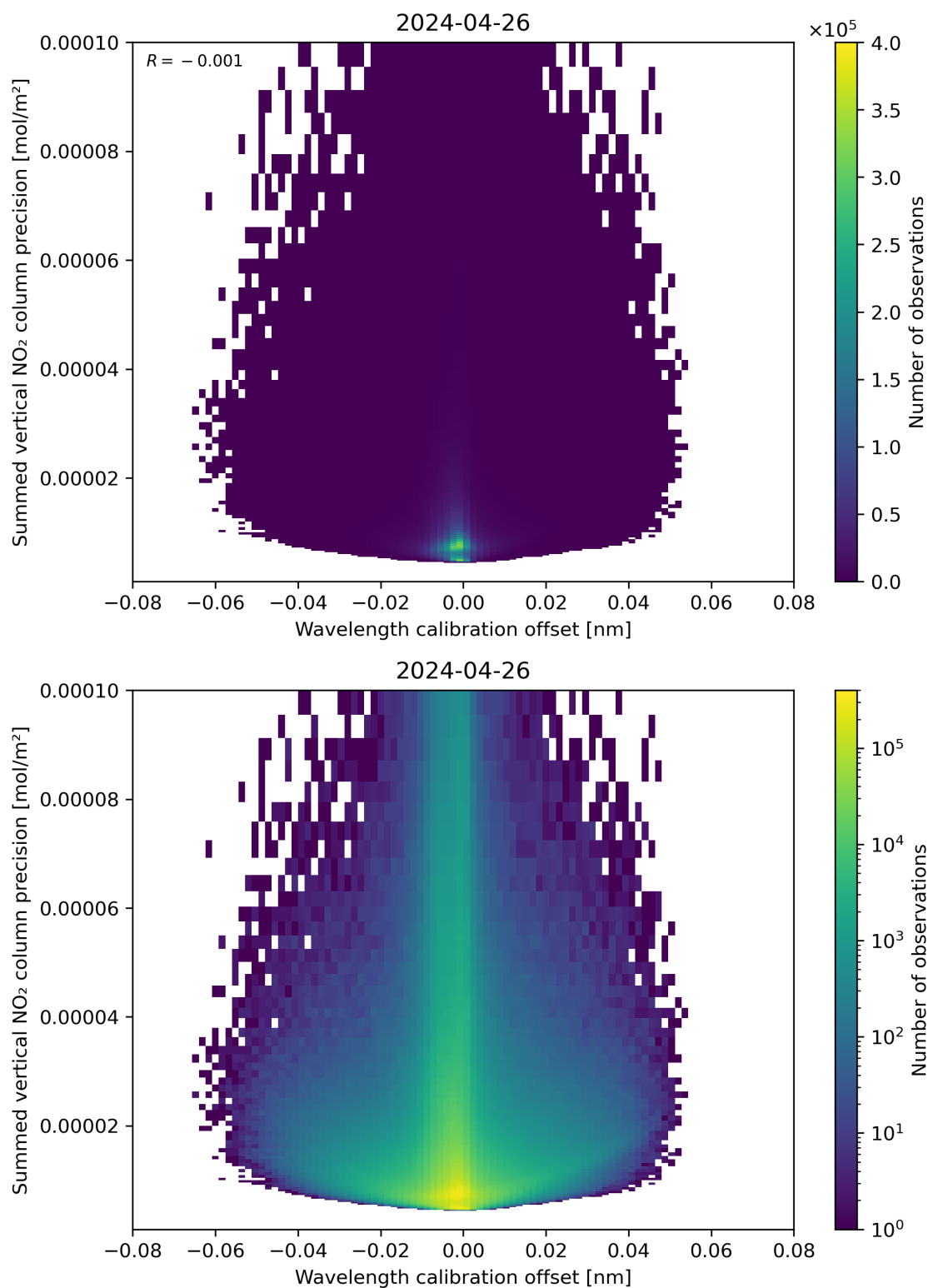
Figure 178: Scatter density plot of “Wavelength calibration offset” against “Summed vertical NO 2 column precision” for 2024-04-26 to 2024-04-27.
