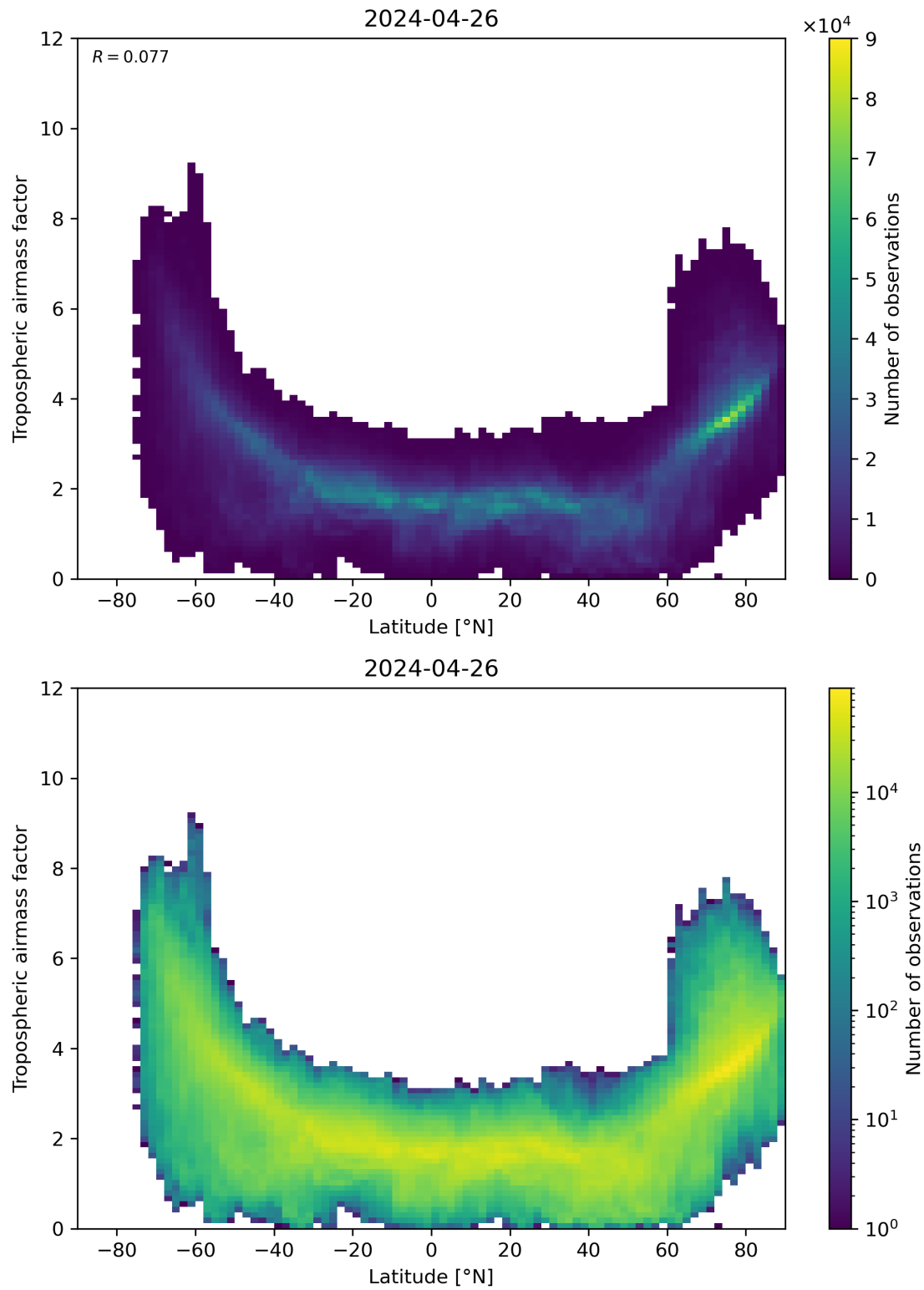
Figure 85: Scatter density plot of “Latitude” against “Tropospheric airmass factor” for 2024-04-26 to 2024-04-27.
