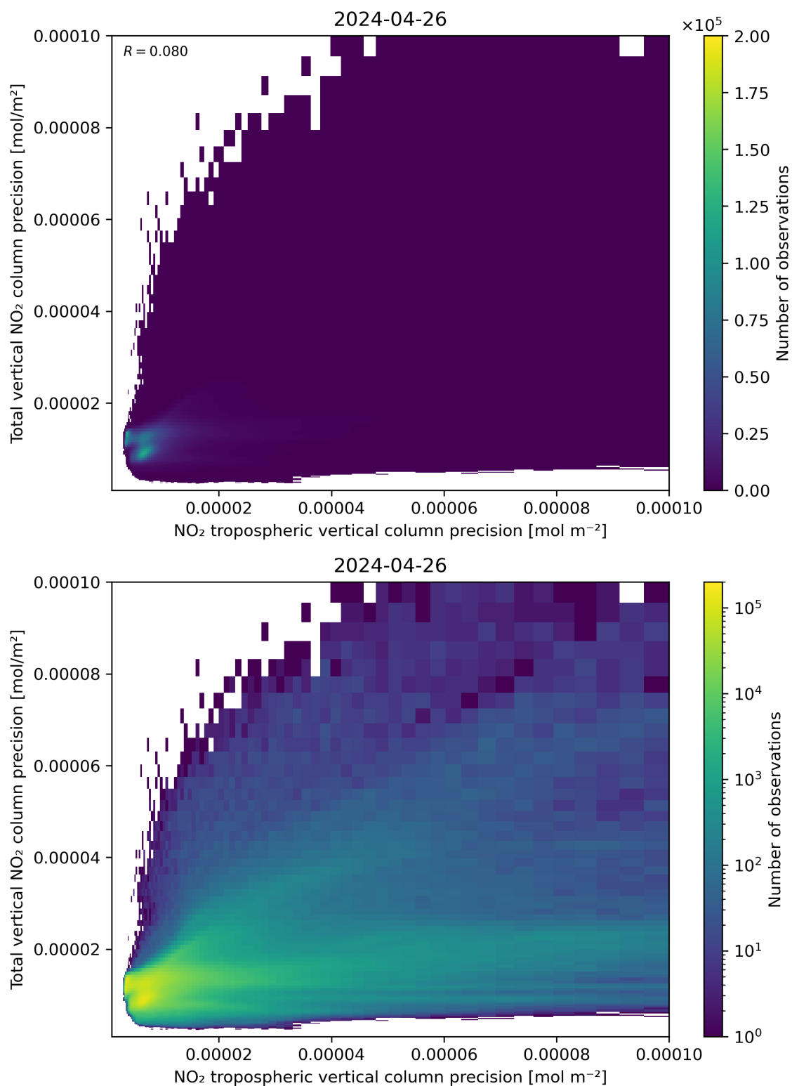
Figure 139: Scatter density plot of “NO 2 tropospheric vertical column precision” against “Total vertical NO 2 column precision” for 2024-04-26 to 2024-04-27.
