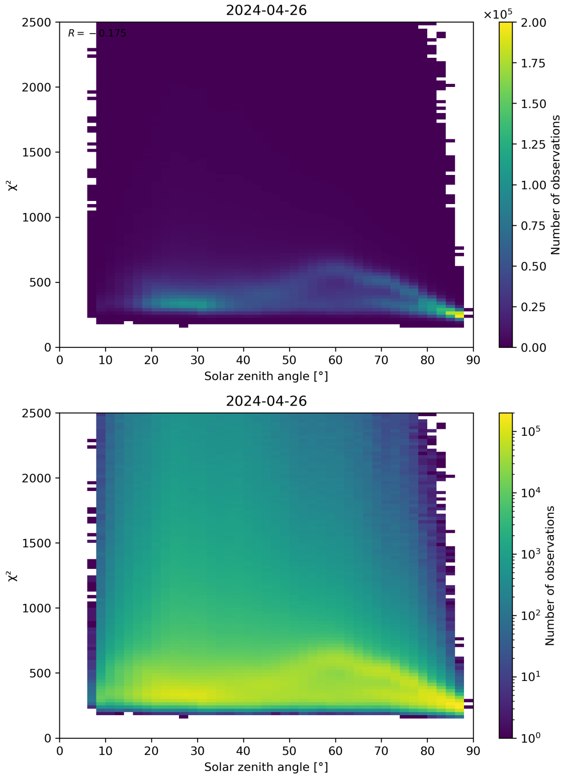
Figure 148: Scatter density plot of “Solar zenith angle” against “ \chi^2 ” for 2024-04-26 to 2024-04-27.
