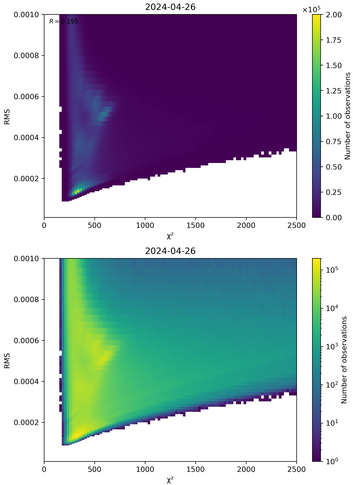
Figure 82: Scatter density plot of “ \chi^2 ” against “RMS” for 2024-04-26 to 2024-04-27.
