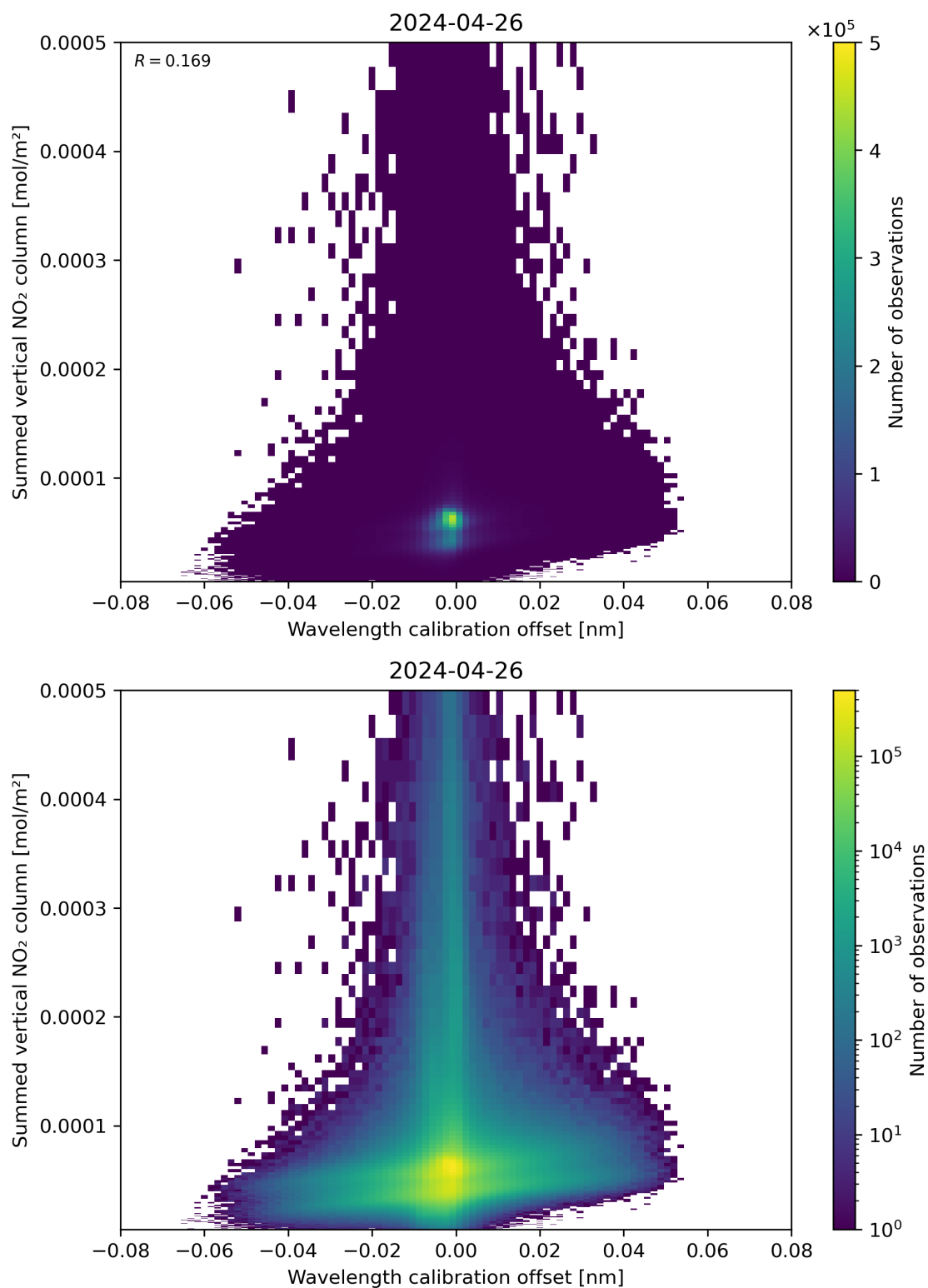
Figure 177: Scatter density plot of “Wavelength calibration offset” against “Summed vertical NO 2 column” for 2024-04-26 to 2024-04-27.
