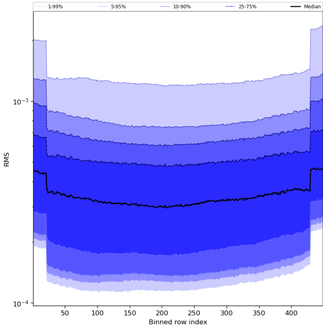
Figure 60: Along track statistics of “RMS” for 2024-04-26 to 2024-04-27
