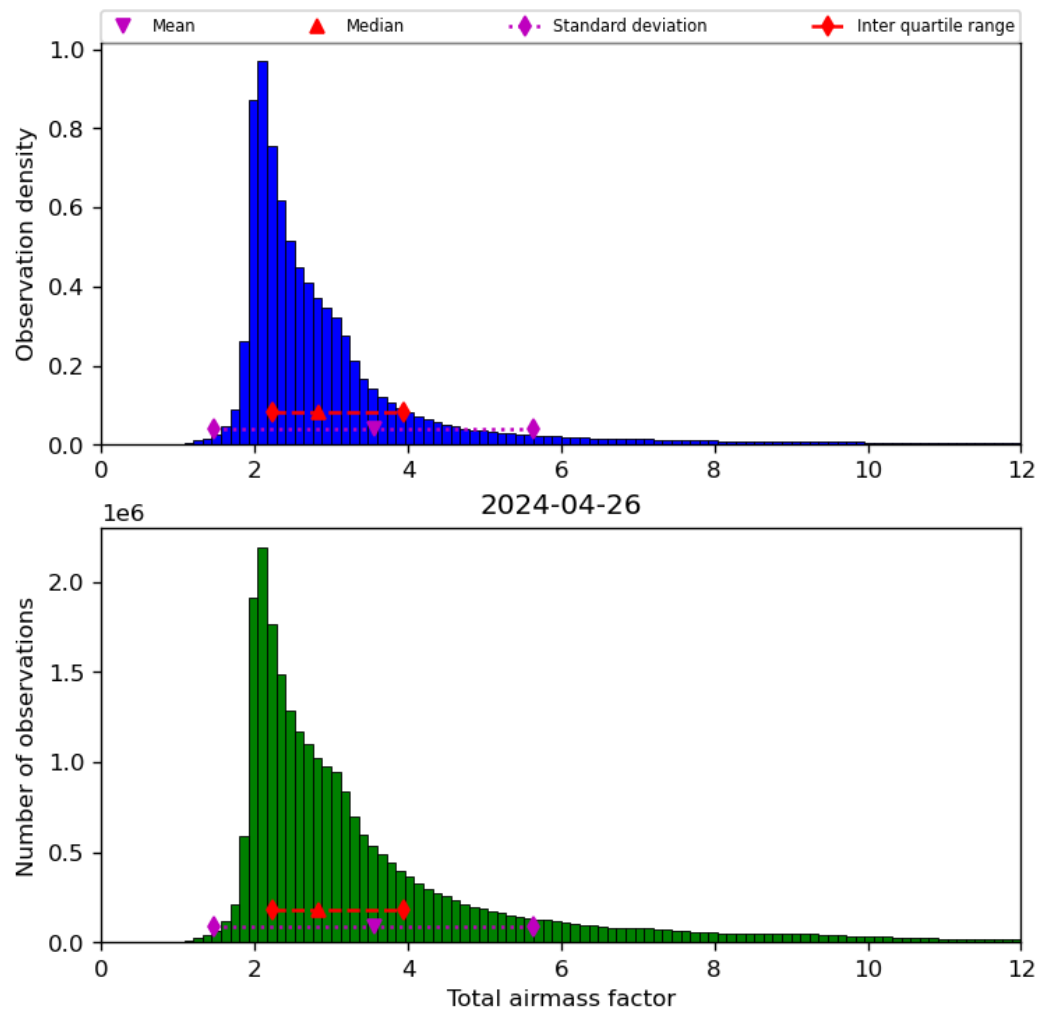
Figure 32: Histogram of “Total airmass factor” for 2024-04-26 to 2024-04-27
