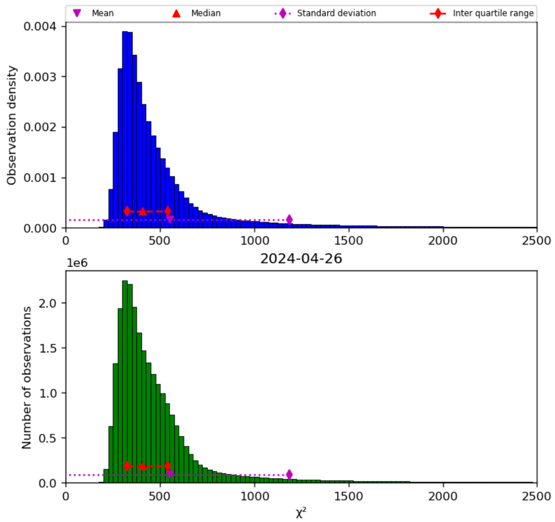
Figure 42: Histogram of " \chi^2 " for 2024-04-26 to 2024-04-27
