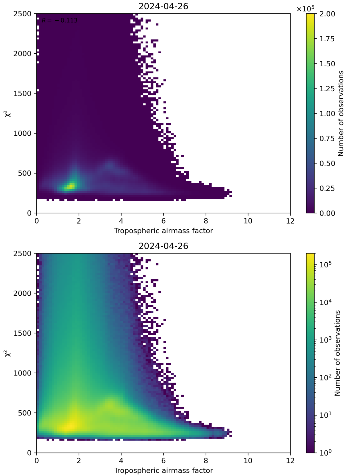
Figure 73: Scatter density plot of “Tropospheric airmass factor” against “ \chi^2 ” for 2024-04-26 to 2024-04-27.
