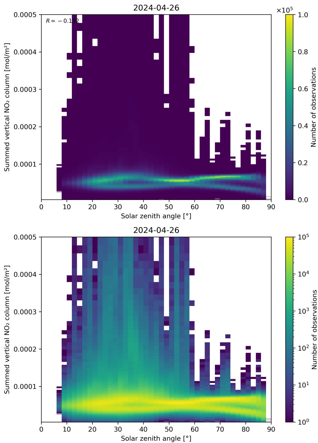
Figure 151: Scatter density plot of “Solar zenith angle” against “Summed vertical NO 2 column” for 2024-04-26 to 2024-04-27.
