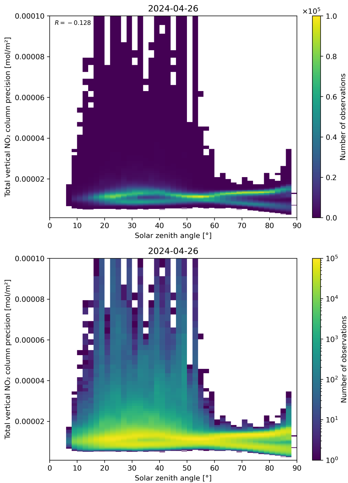
Figure 154: Scatter density plot of “Solar zenith angle” against “Total vertical NO 2 column precision” for 2024-04-26 to 2024-04-27.
