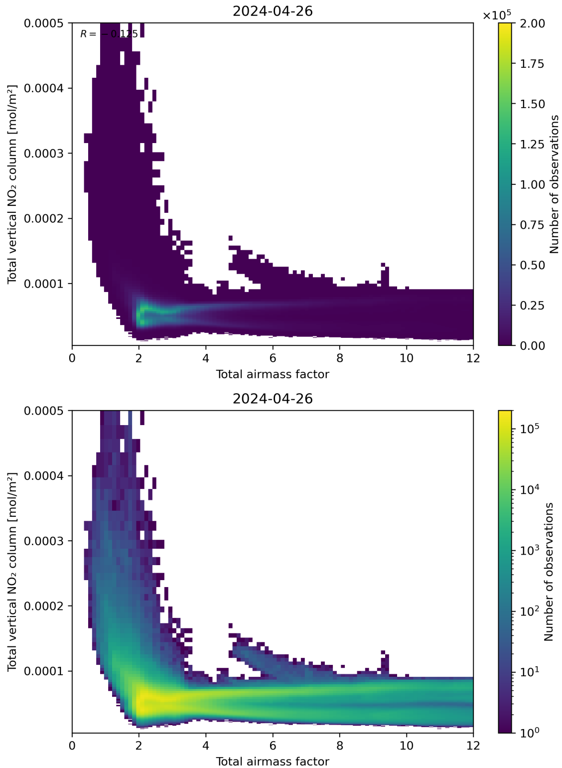
Figure 67: Scatter density plot of “Total airmass factor” against “Total vertical NO 2 column” for 2024-04-26 to 2024-04-27.
