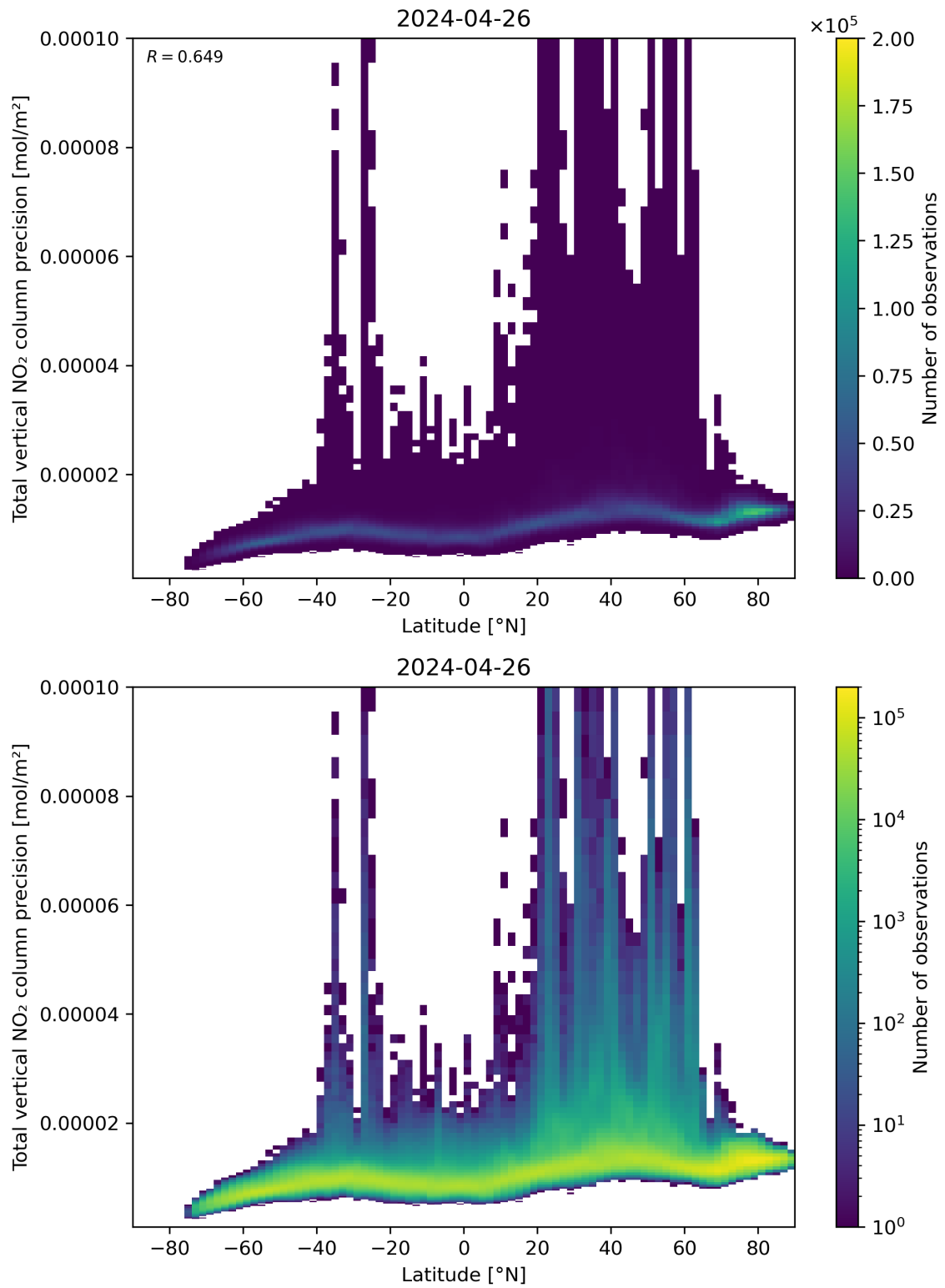
Figure 91: Scatter density plot of “Latitude” against “Total vertical NO 2 column precision” for 2024-04-26 to 2024-04-27.
