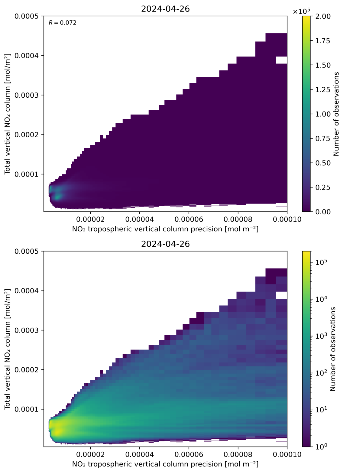
Figure 138: Scatter density plot of “NO 2 tropospheric vertical column precision” against “Total vertical NO 2 column” for 2024-04-26 to 2024-04-27.
