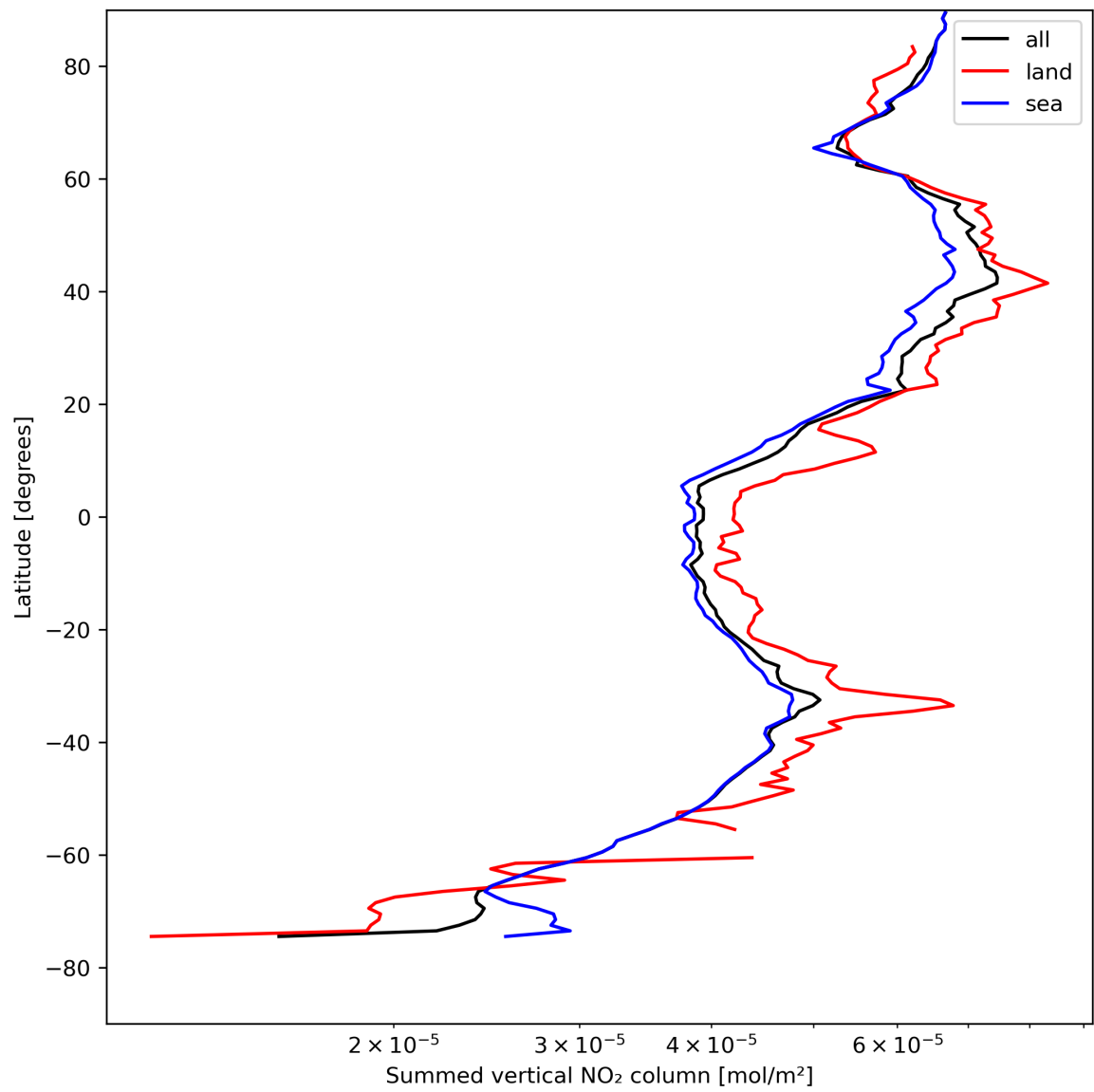
Figure 23: Zonal average of “Summed vertical NO 2 column” for 2024-04-26 to 2024-04-27.
