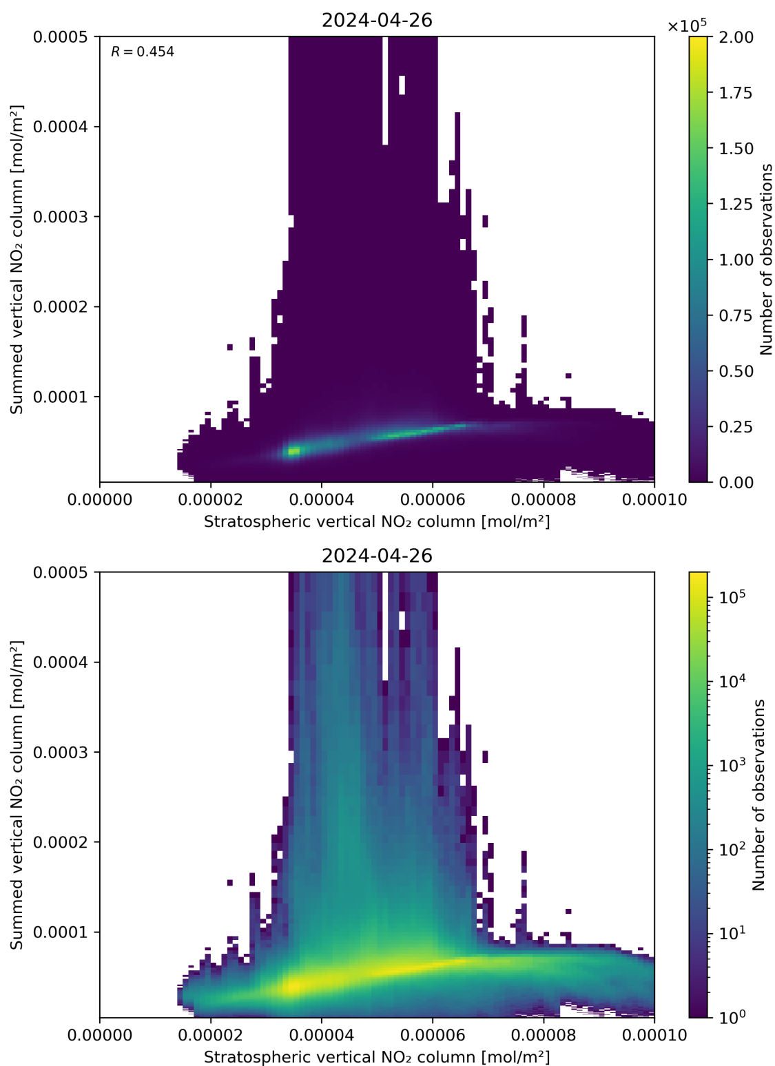
Figure 98: Scatter density plot of “Stratospheric vertical NO 2 column” against “Summed vertical NO 2 column” for 2024-04-26 to 2024-04-27.
