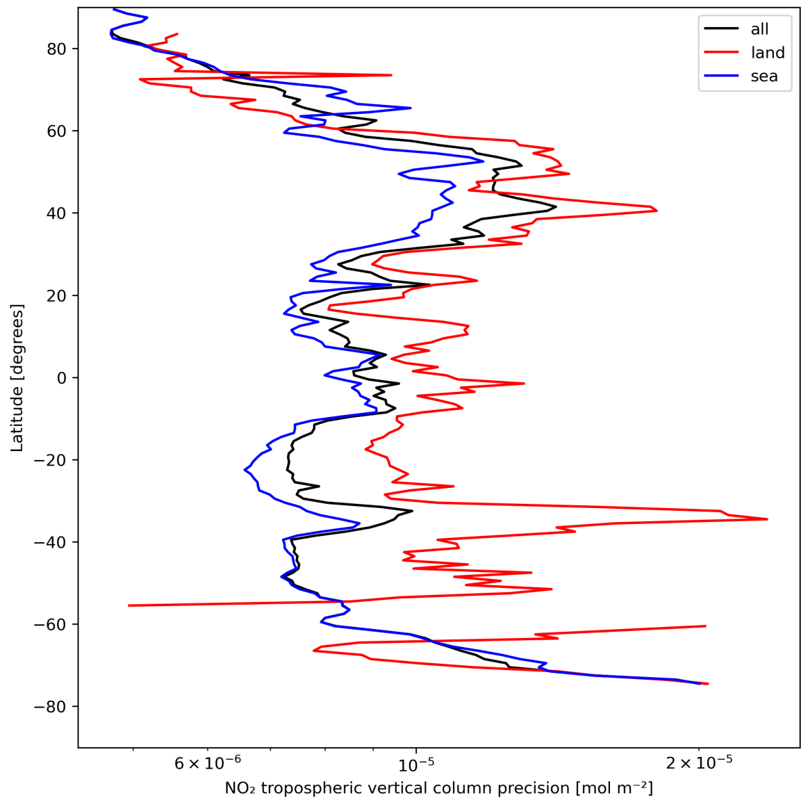
Figure 13: Zonal average of “NO 2 tropospheric vertical column precision” for 2024-04-26 to 2024-04-27.
