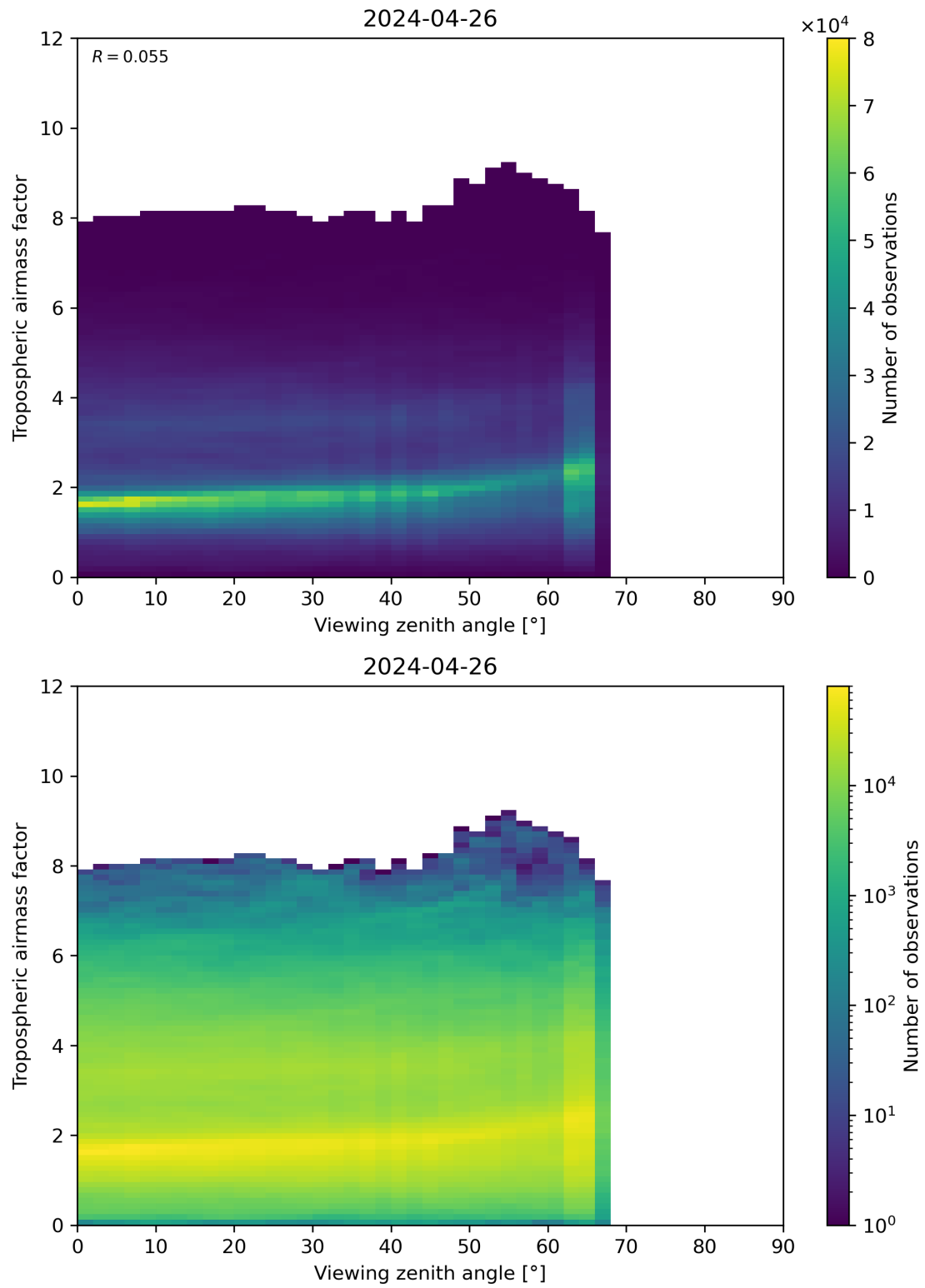
Figure 161: Scatter density plot of “Viewing zenith angle” against “Tropospheric airmass factor” for 2024-04-26 to 2024-04-27.
