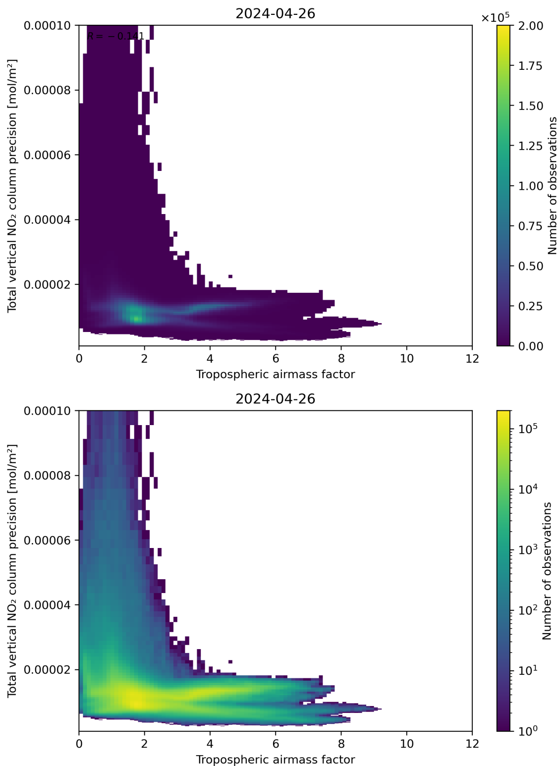
Figure 78: Scatter density plot of “Tropospheric air mass factor” against “Total vertical NO 2 column precision” for 2024-04-26 to 2024-04-27.
