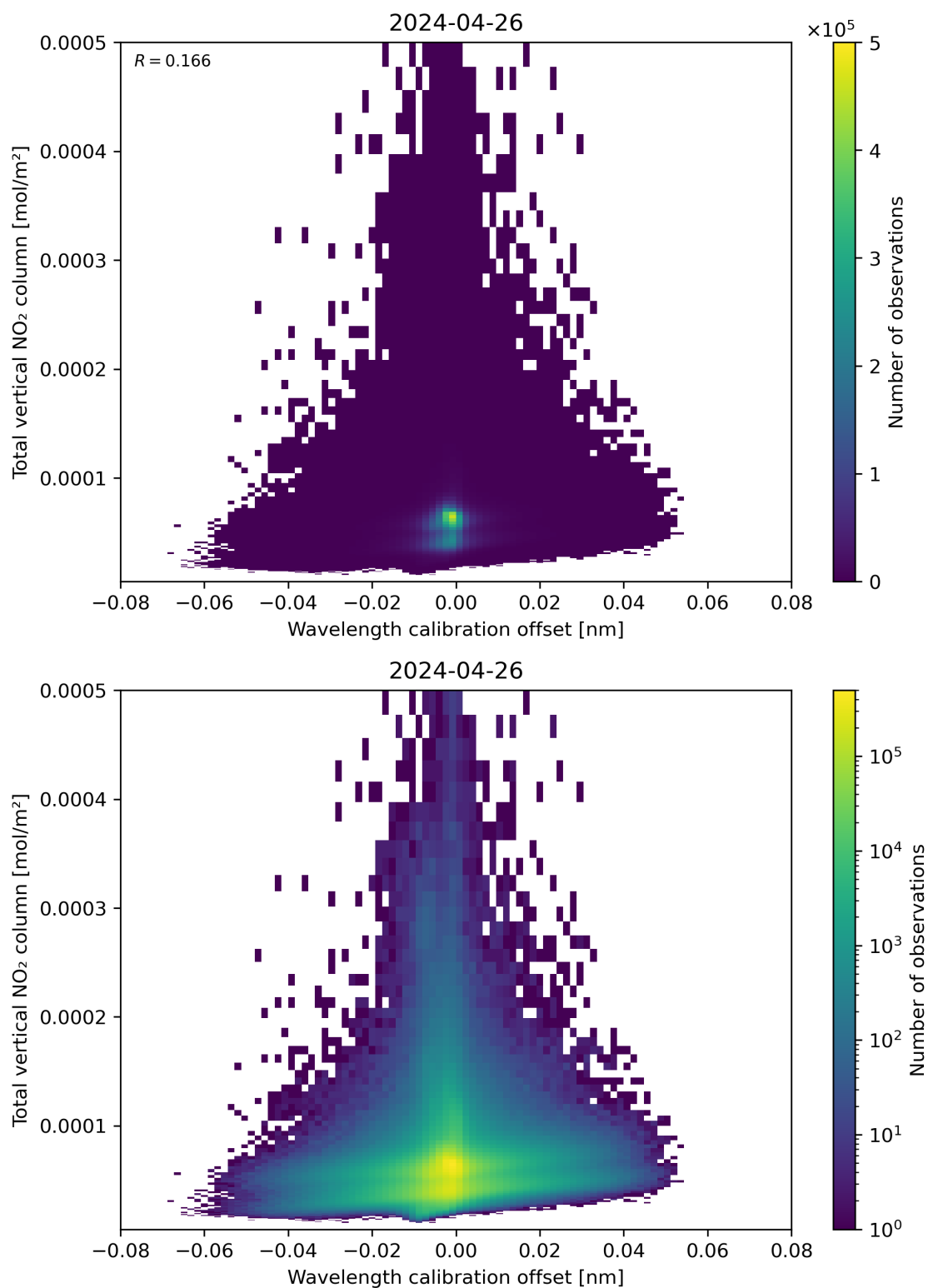
Figure 179: Scatter density plot of “Wavelength calibration offset” against “Total vertical NO 2 column” for 2024-04-26 to 2024-04-27.
