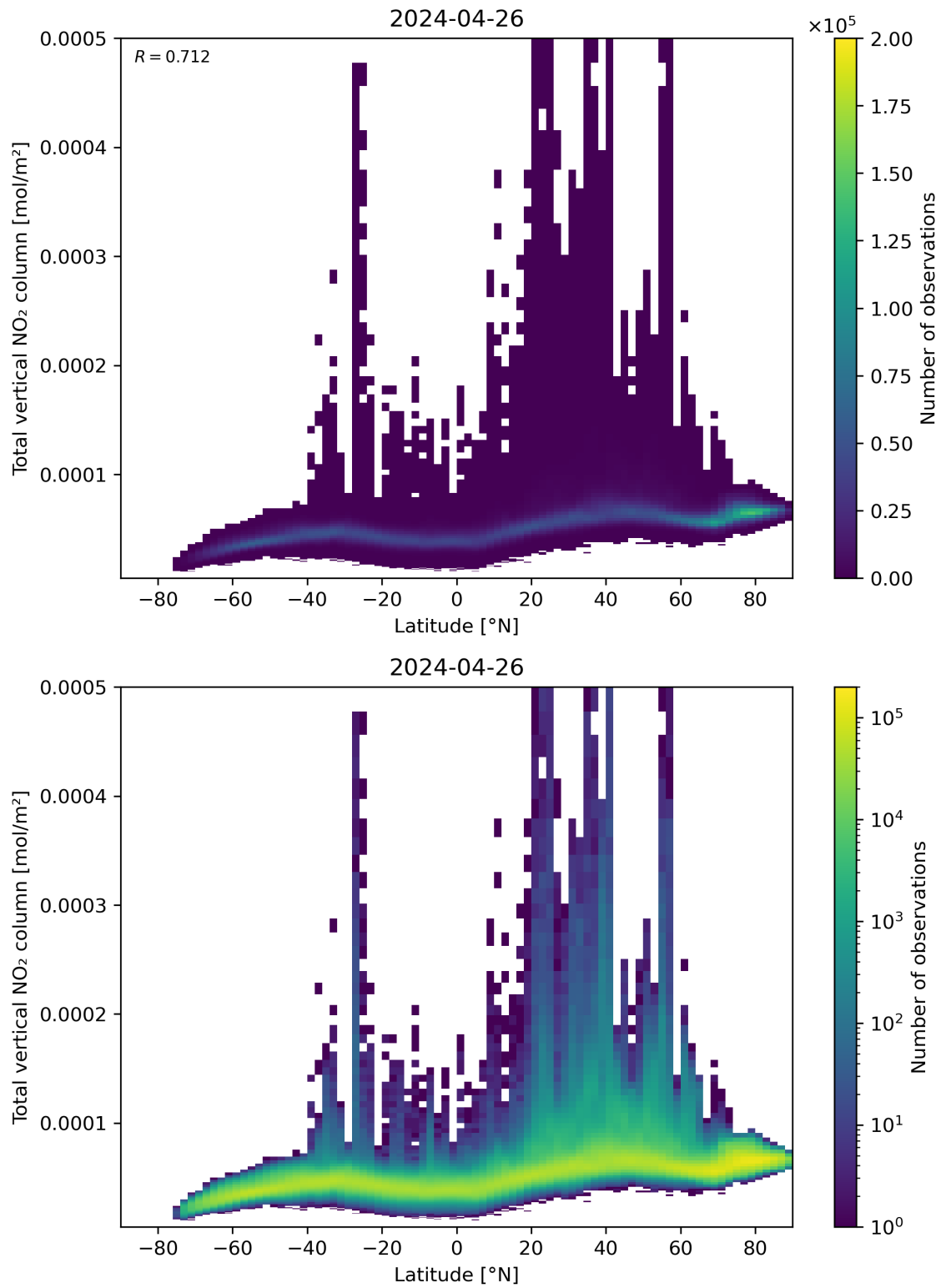
Figure 90: Scatter density plot of “Latitude” against “Total vertical NO 2 column” for 2024-04-26 to 2024-04-27.
