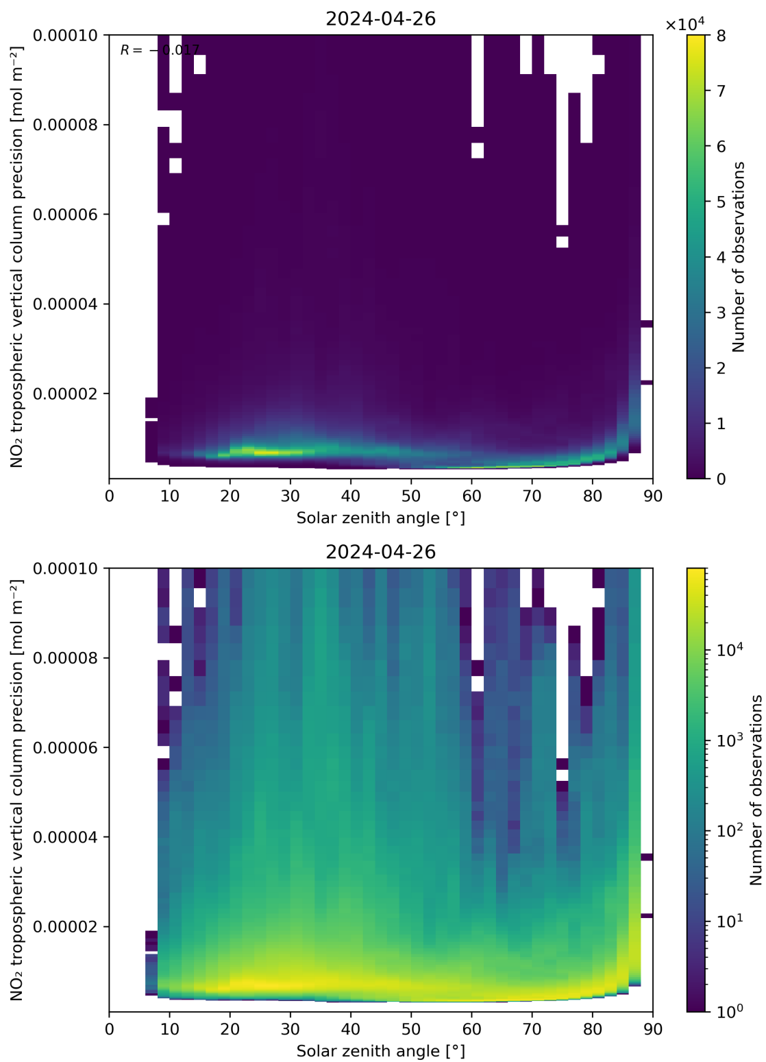
Figure 156: Scatter density plot of “Solar zenith angle” against “NO 2 tropospheric vertical column precision” for 2024-04-26 to 2024-04-27.
