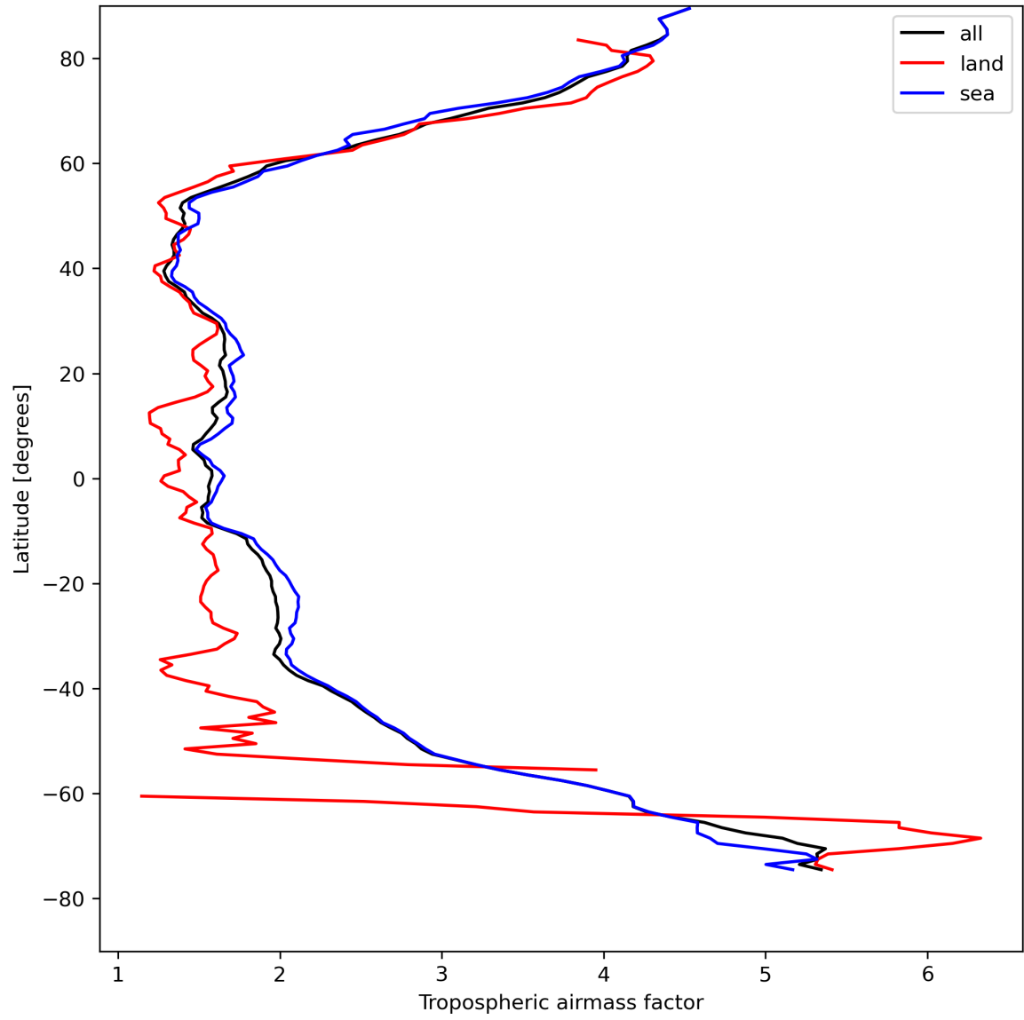
Figure 14: Zonal average of “Tropospheric airmass factor” for 2024-04-26 to 2024-04-27.
