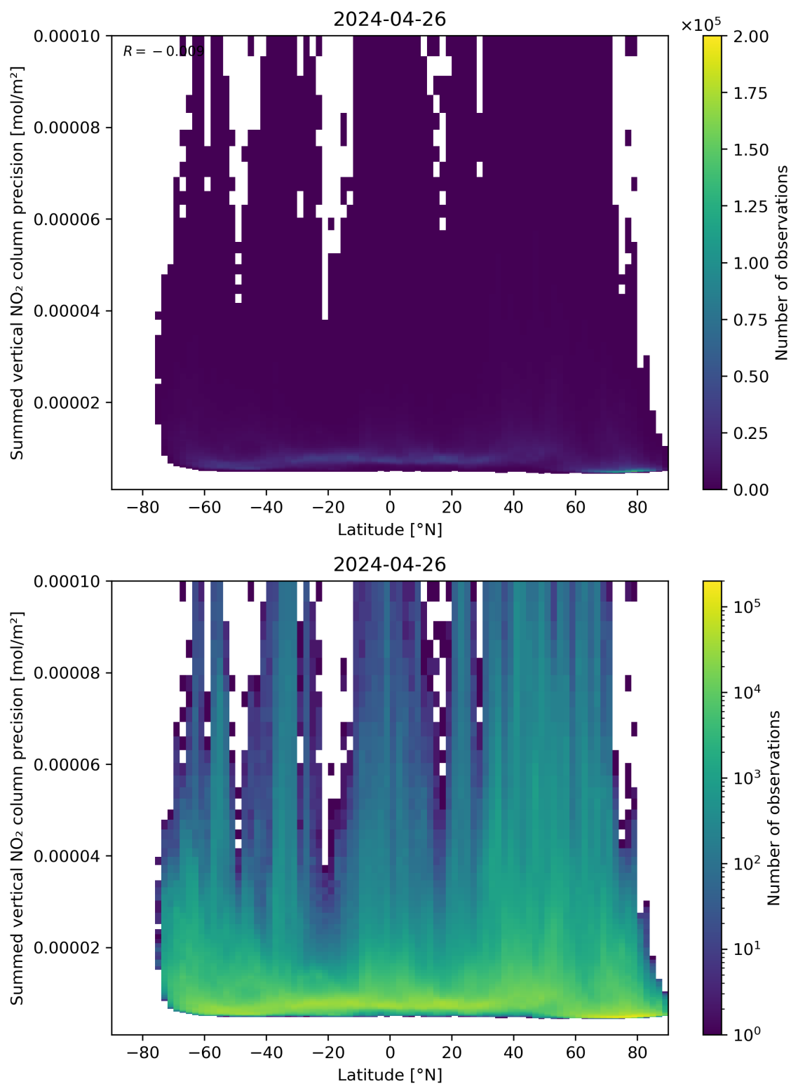
Figure 89: Scatter density plot of “Latitude” against “Summed vertical NO 2 column precision” for 2024-04-26 to 2024-04-27.
