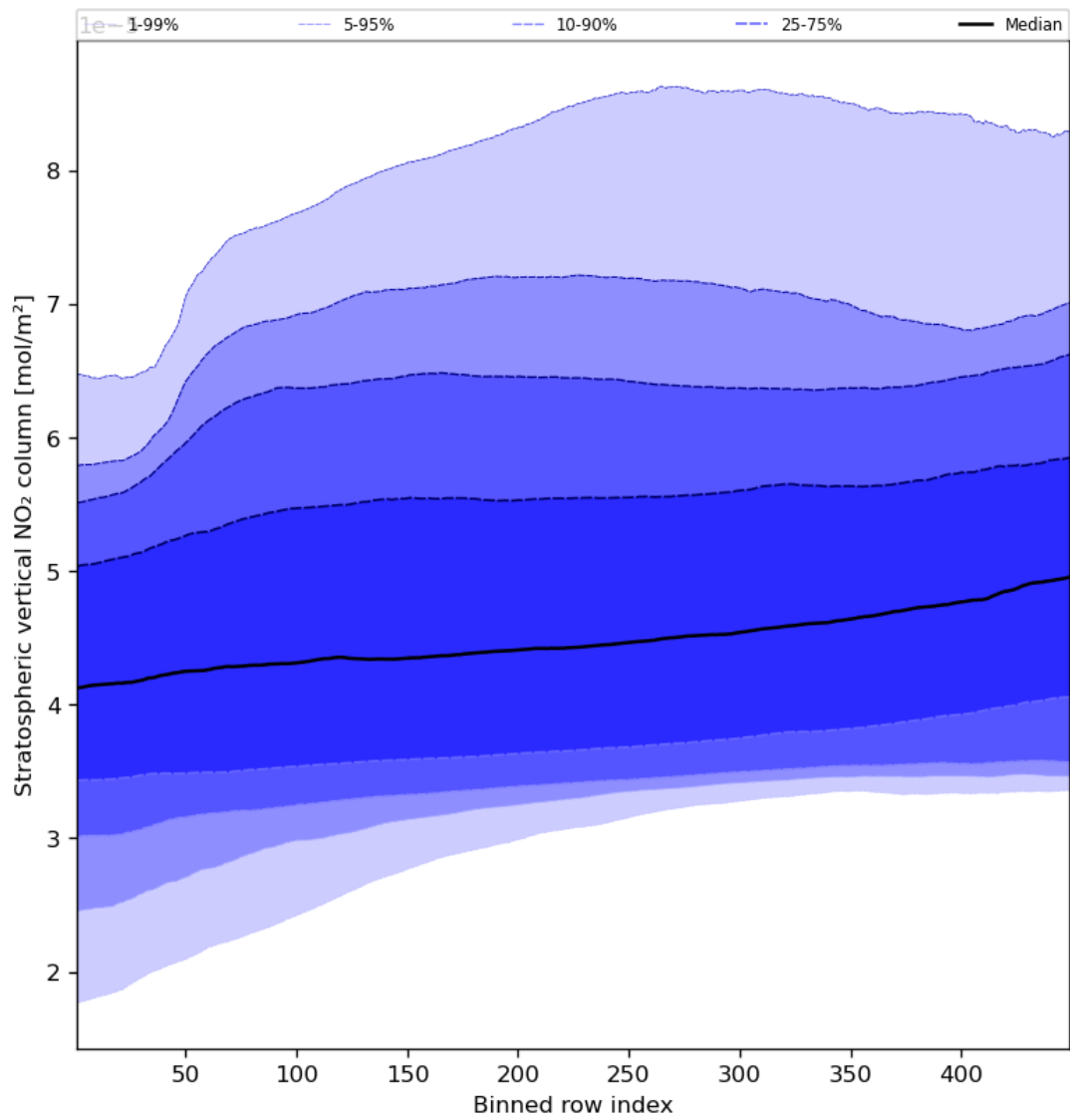
Figure 53: Along track statistics of “Stratospheric vertical NO 2 column” for 2024-04-26 to 2024-04-27
