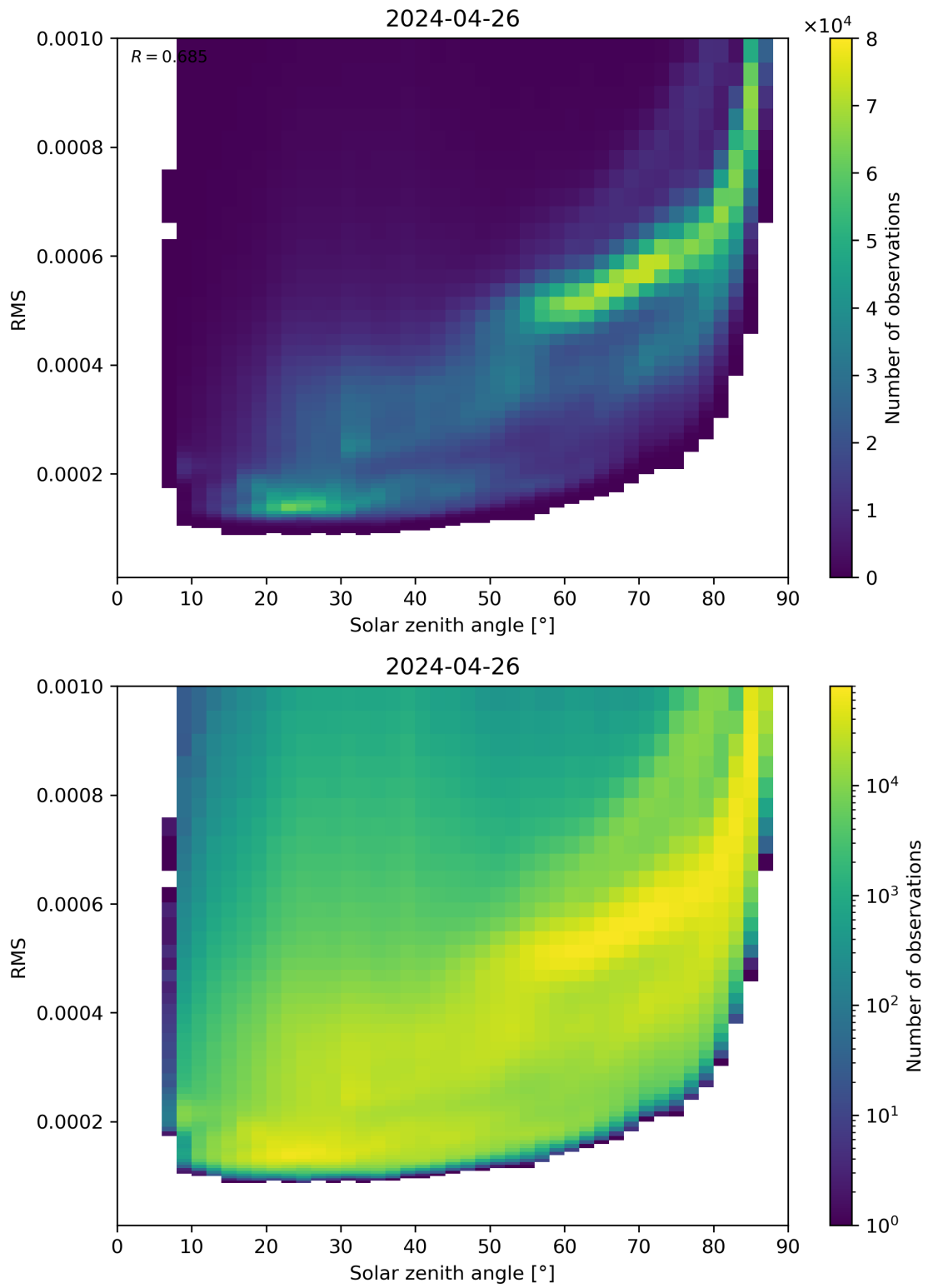
Figure 157: Scatter density plot of “Solar zenith angle” against “RMS” for 2024-04-26 to 2024-04-27.
