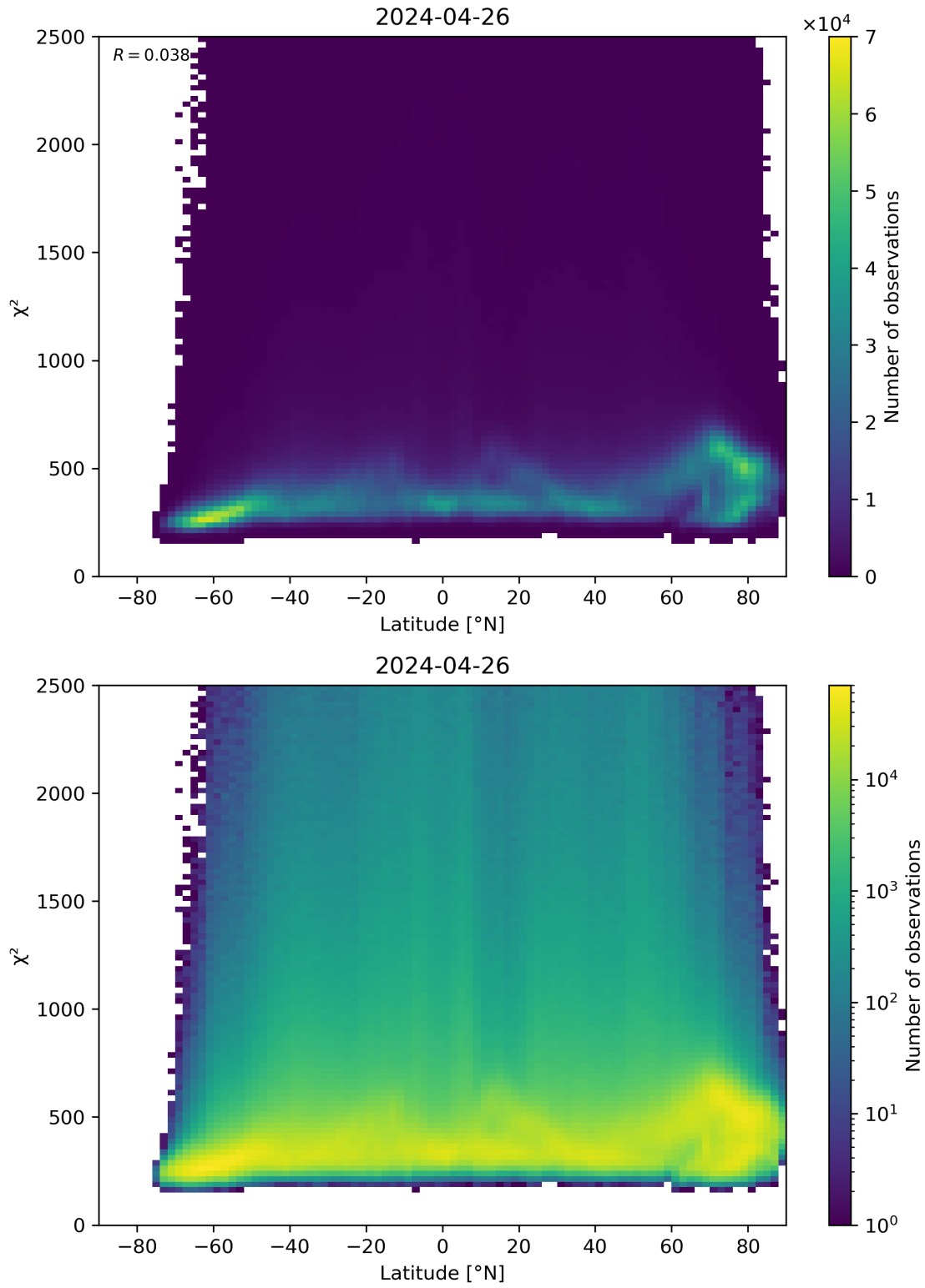
Figure 86: Scatter density plot of “Latitude” against “ \chi^2 ” for 2024-04-26 to 2024-04-27.
