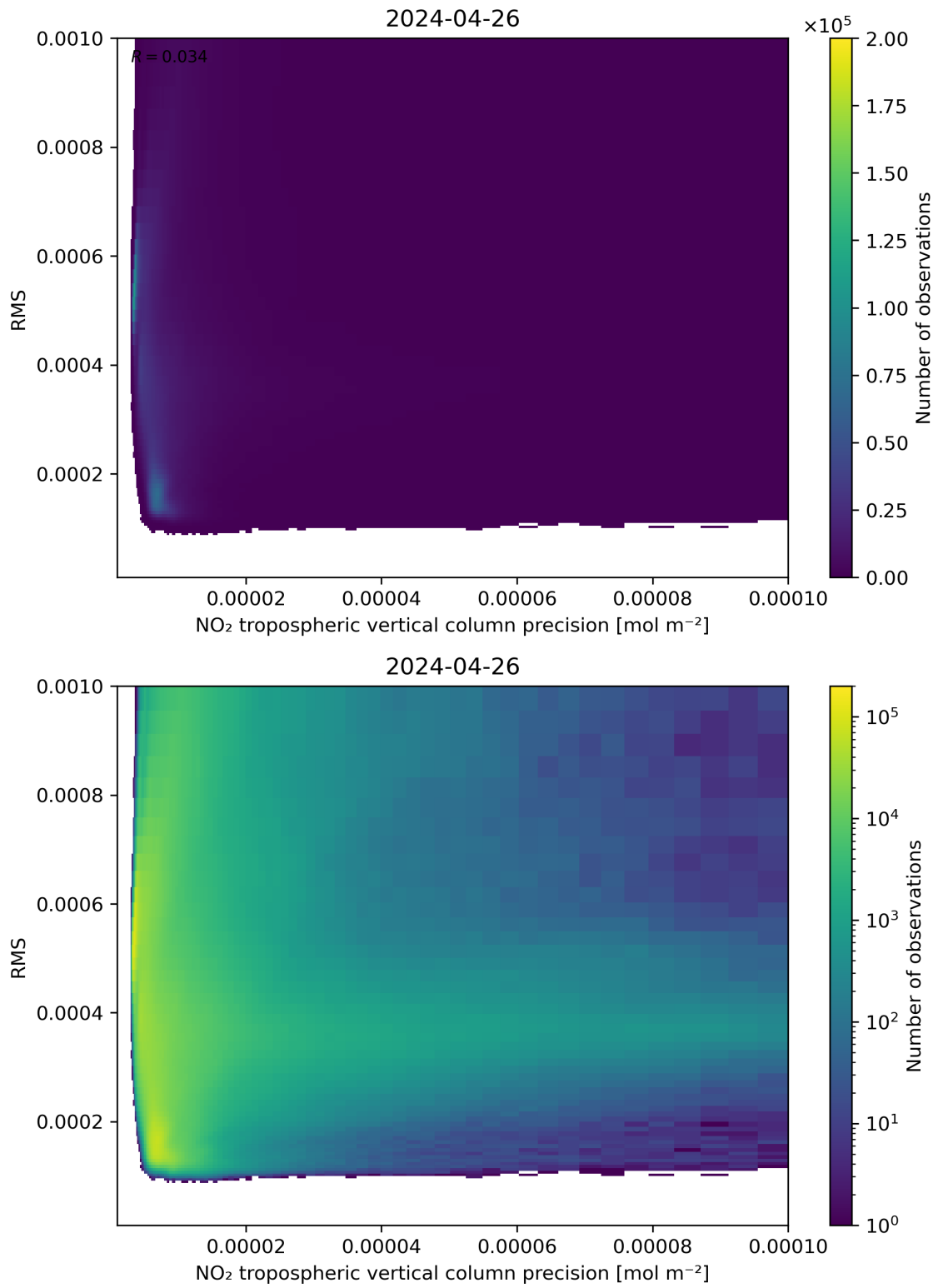
Figure 140: Scatter density plot of “NO 2 tropospheric vertical column precision” against “RMS” for 2024-04-26 to 2024-04-27.
