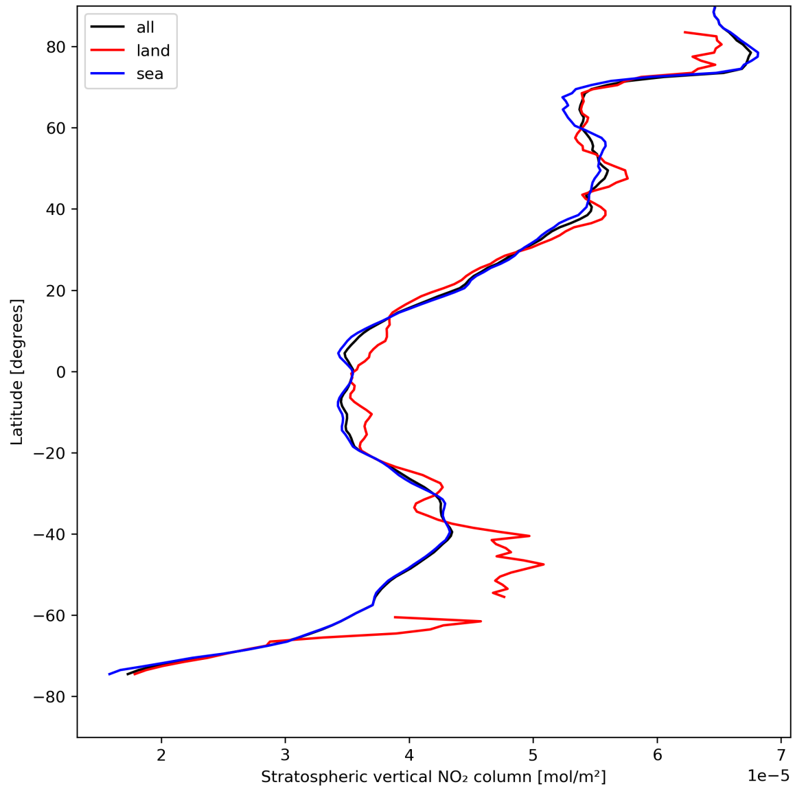
Figure 19: Zonal average of “Stratospheric vertical NO 2 column” for 2024-04-26 to 2024-04-27.
