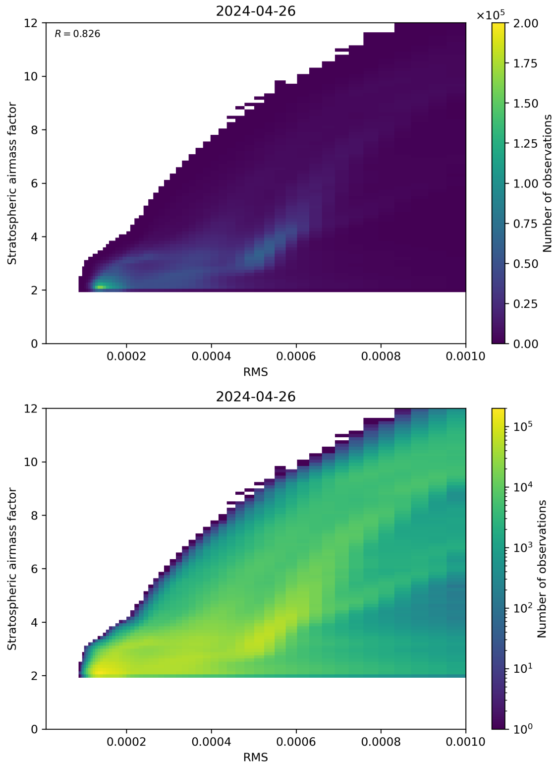
Figure 144: Scatter density plot of “RMS” against “Stratospheric airmass factor” for 2024-04-26 to 2024-04-27.
