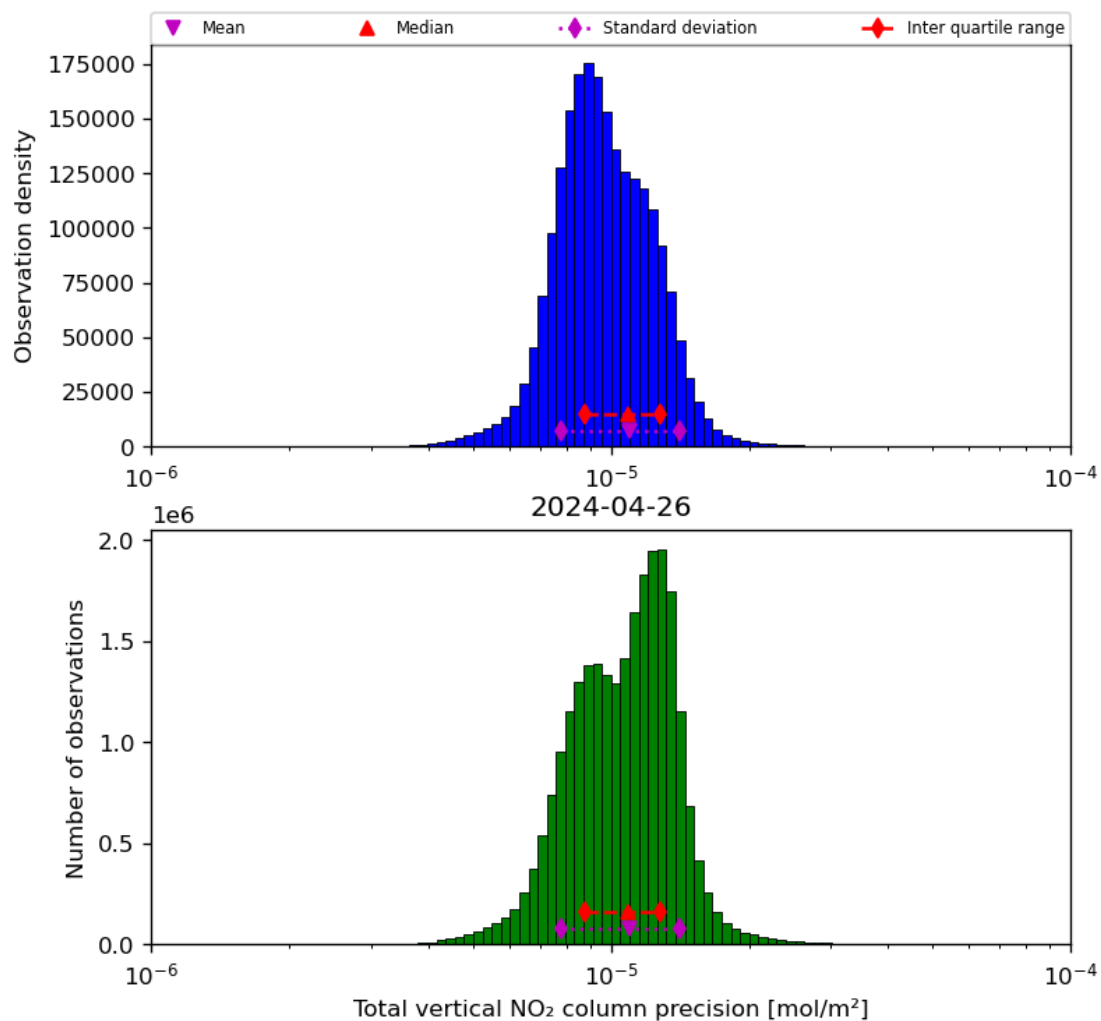
Figure 39: Histogram of “Total vertical NO 2 column precision” for 2024-04-26 to 2024-04-27
