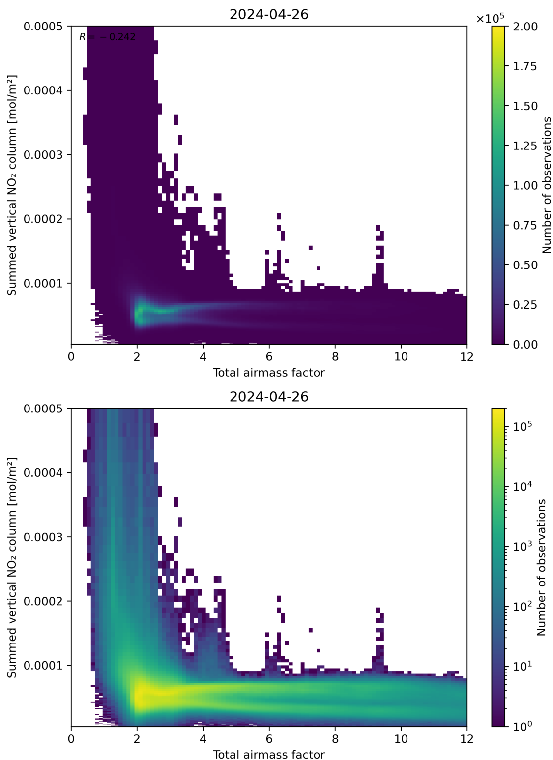
Figure 65: Scatter density plot of “Total airmass factor” against “Summed vertical NO 2 column” for 2024-04-26 to 2024-04-27.
