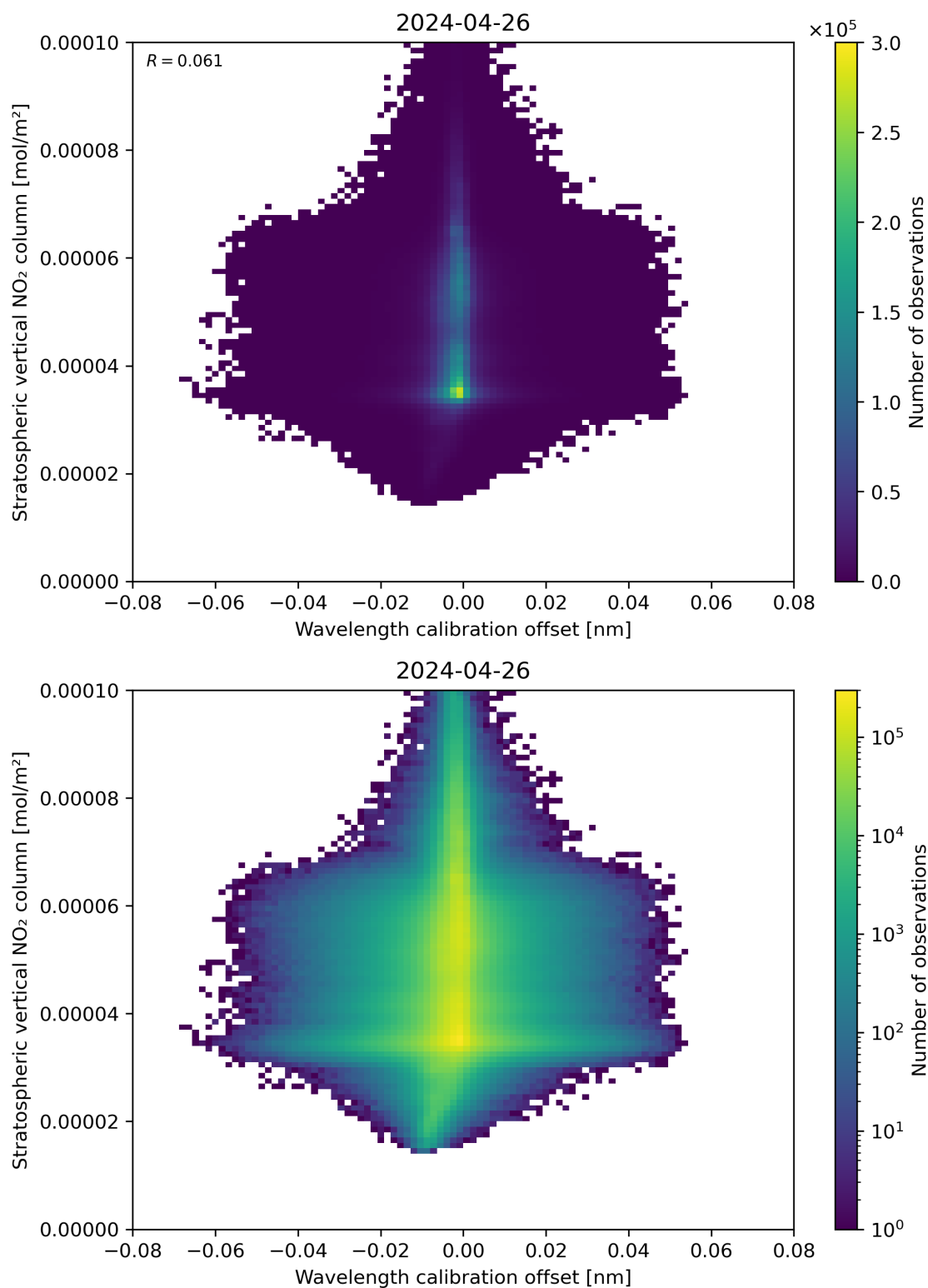
Figure 176: Scatter density plot of “Wavelength calibration offset” against “Stratospheric vertical NO 2 column” for 2024-04-26 to 2024-04-27.
