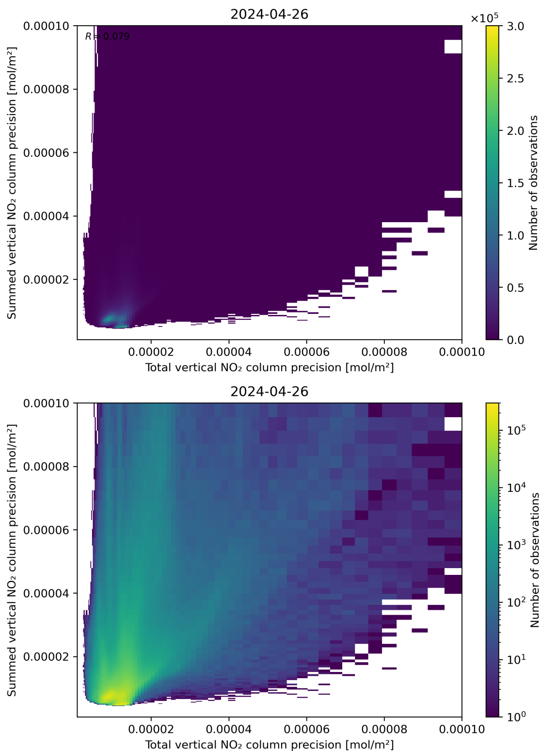
Figure 118: Scatter density plot of “Total vertical NO 2 column precision” against “Summed vertical NO 2 column precision” for 2024-04-26 to 2024-04-27.
