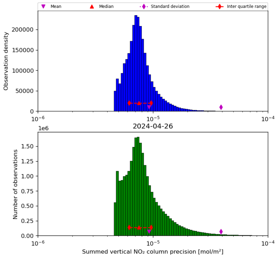
Figure 41: Histogram of “Summed vertical NO 2 column precision” for 2024-04-26 to 2024-04-27
