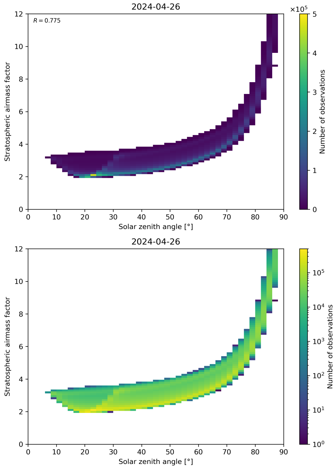
Figure 145: Scatter density plot of “Solar zenith angle” against “Stratospheric airmass factor” for 2024-04-26 to 2024-04-27.
