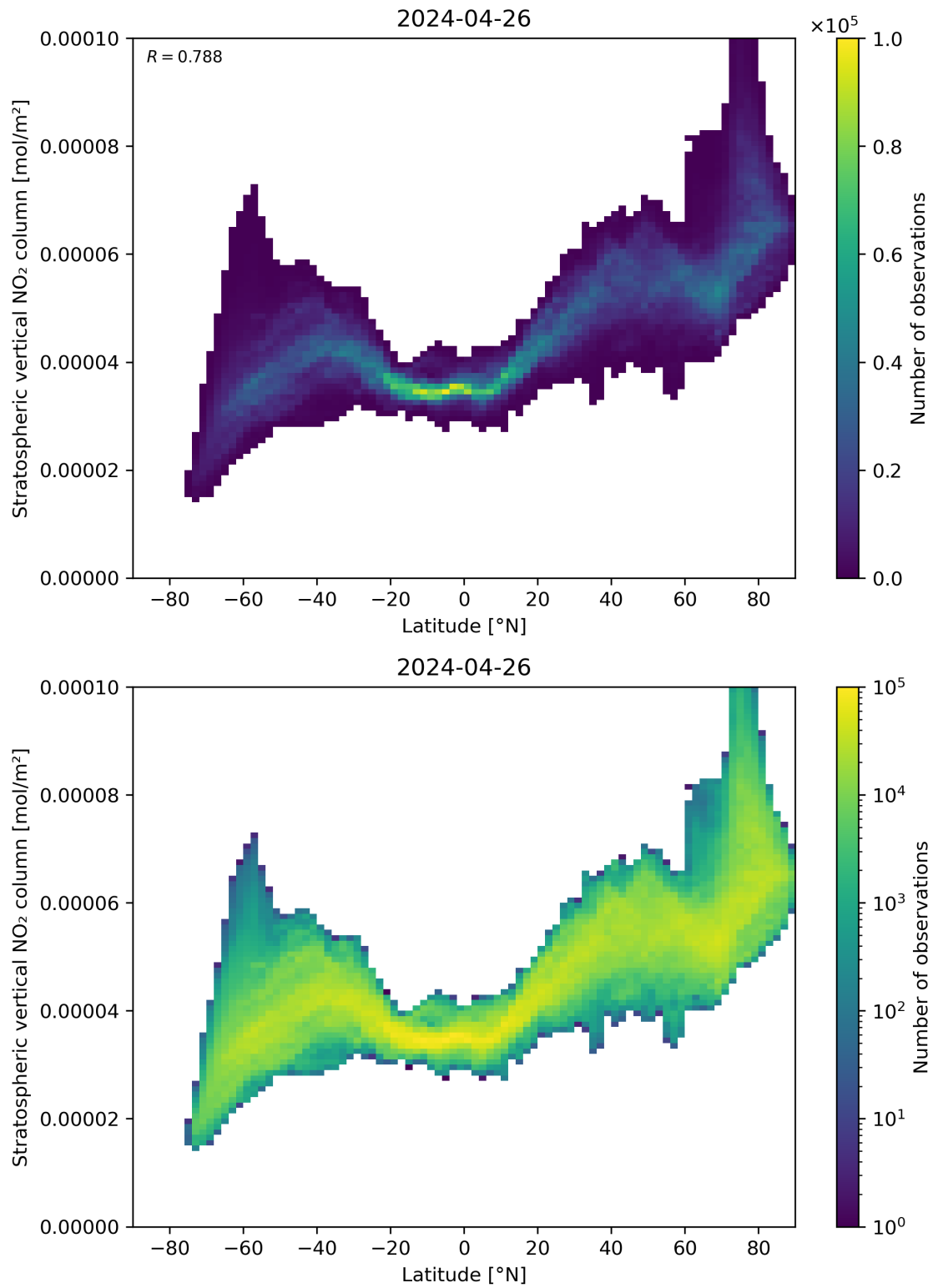
Figure 87: Scatter density plot of “Latitude” against “Stratospheric vertical NO 2 column” for 2024-04-26 to 2024-04-27.
