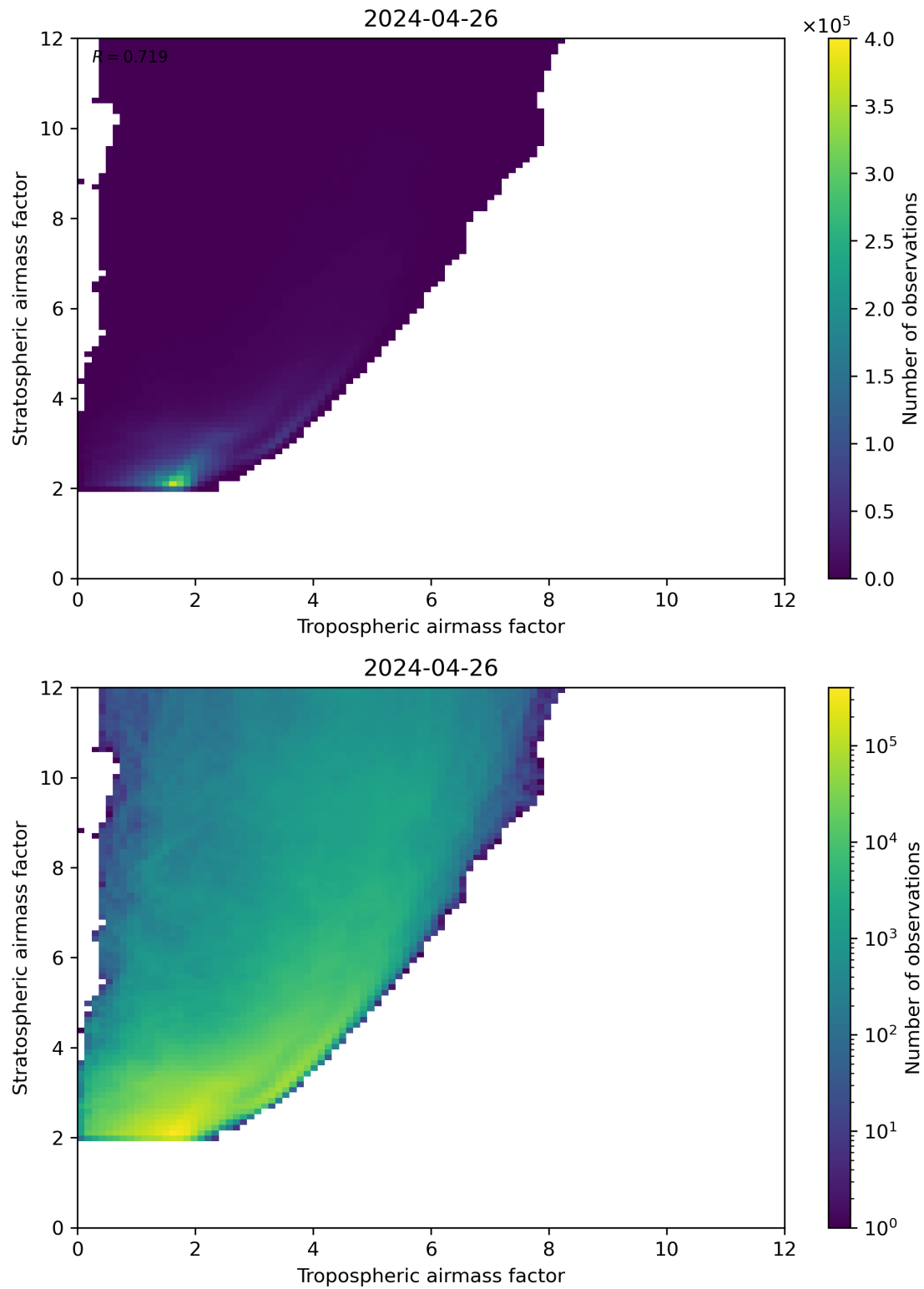
Figure 71: Scatter density plot of “Tropospheric airmass factor” against “Stratospheric airmass factor” for 2024-04-26 to 2024-04-27.
