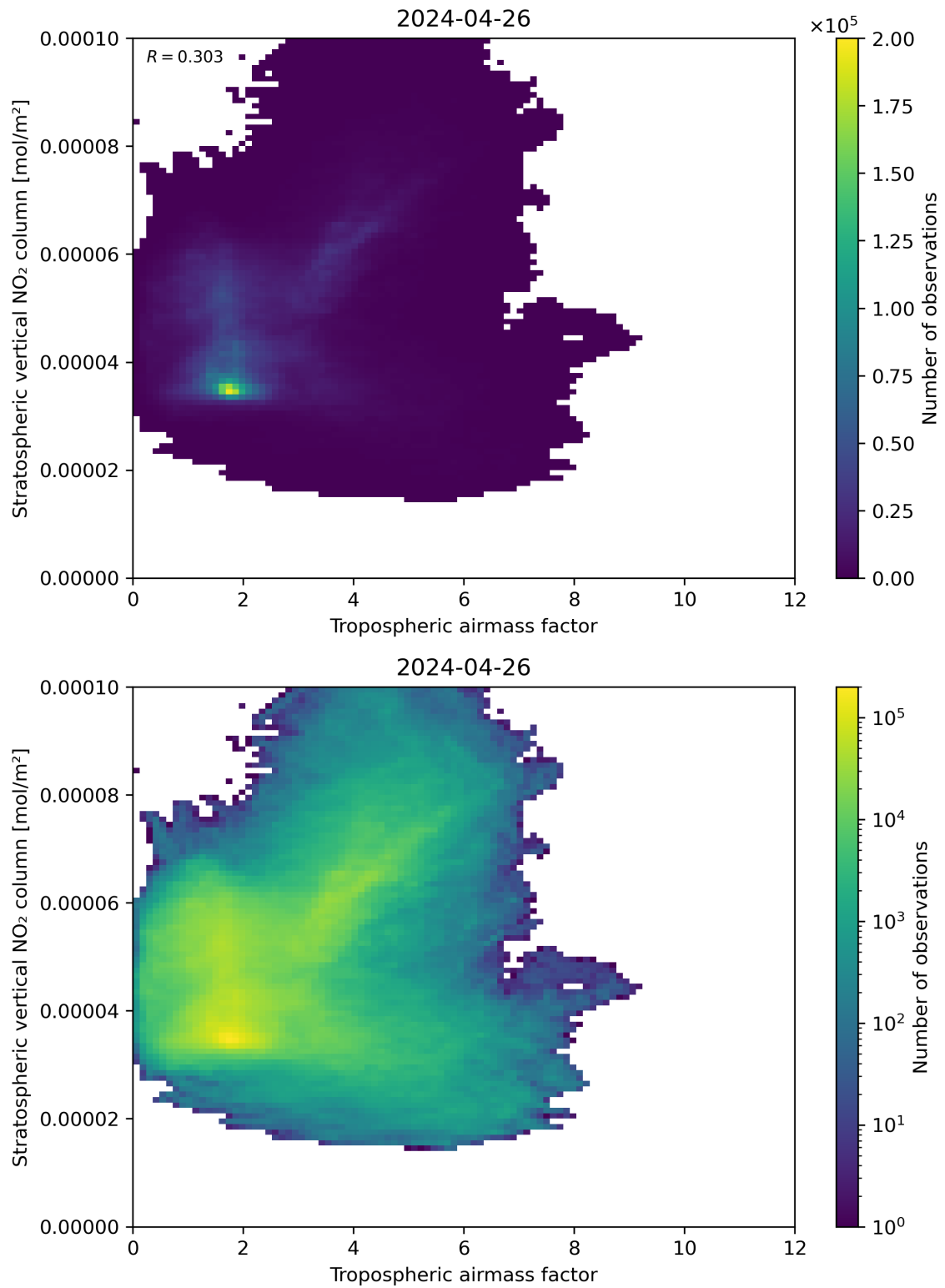
Figure 74: Scatter density plot of “Tropospheric air mass factor” against “Stratospheric vertical NO 2 column” for 2024-04-26 to 2024-04-27.
