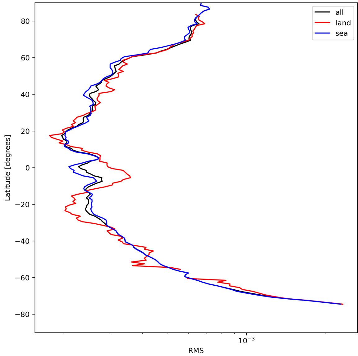
Figure 26: Zonal average of “RMS” for 2024-04-26 to 2024-04-27.
