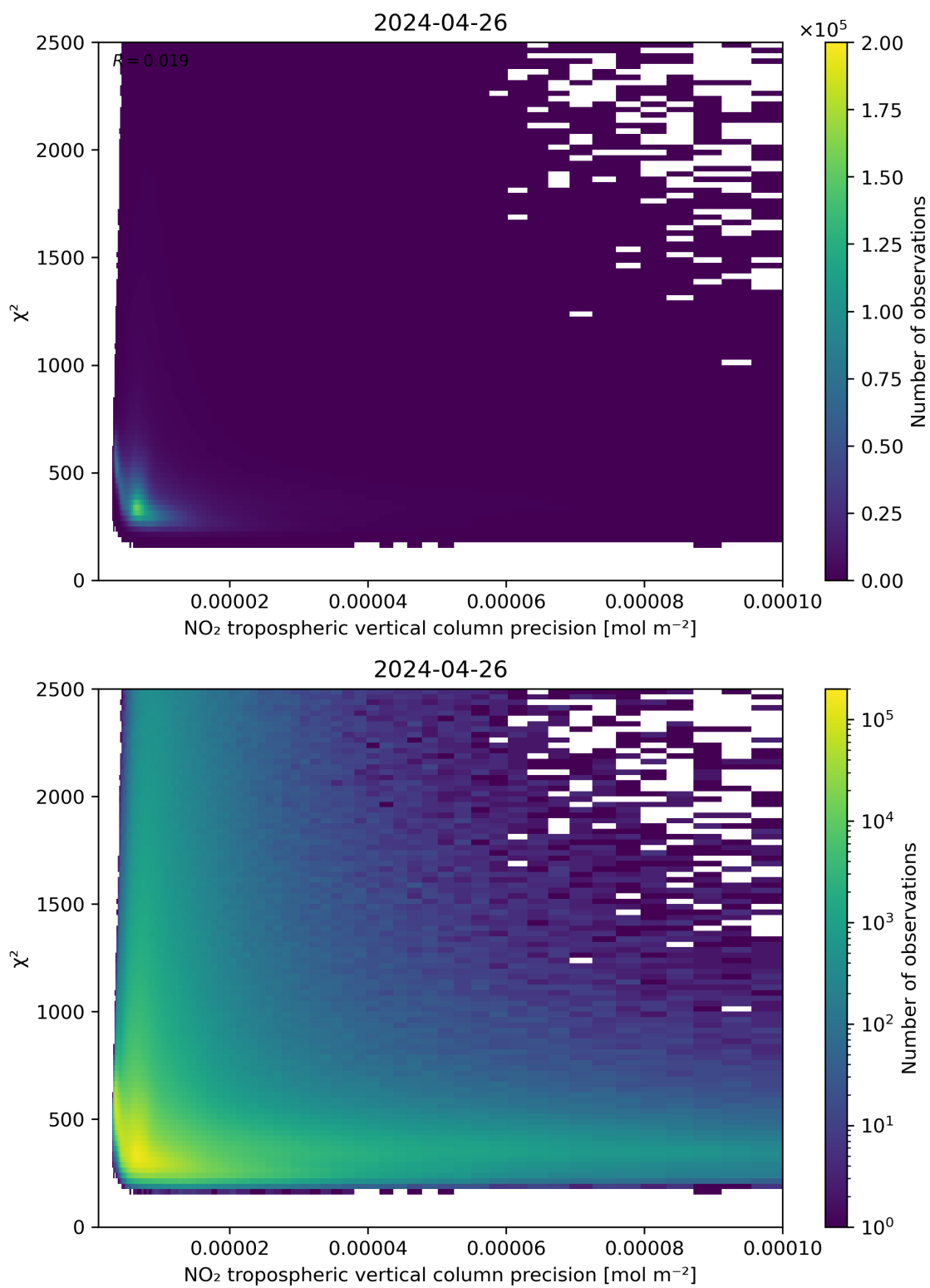
Figure 134: Scatter density plot of “NO 2 tropospheric vertical column precision” against “ \chi^2 ” for 2024-04-26 to 2024-04-27.
