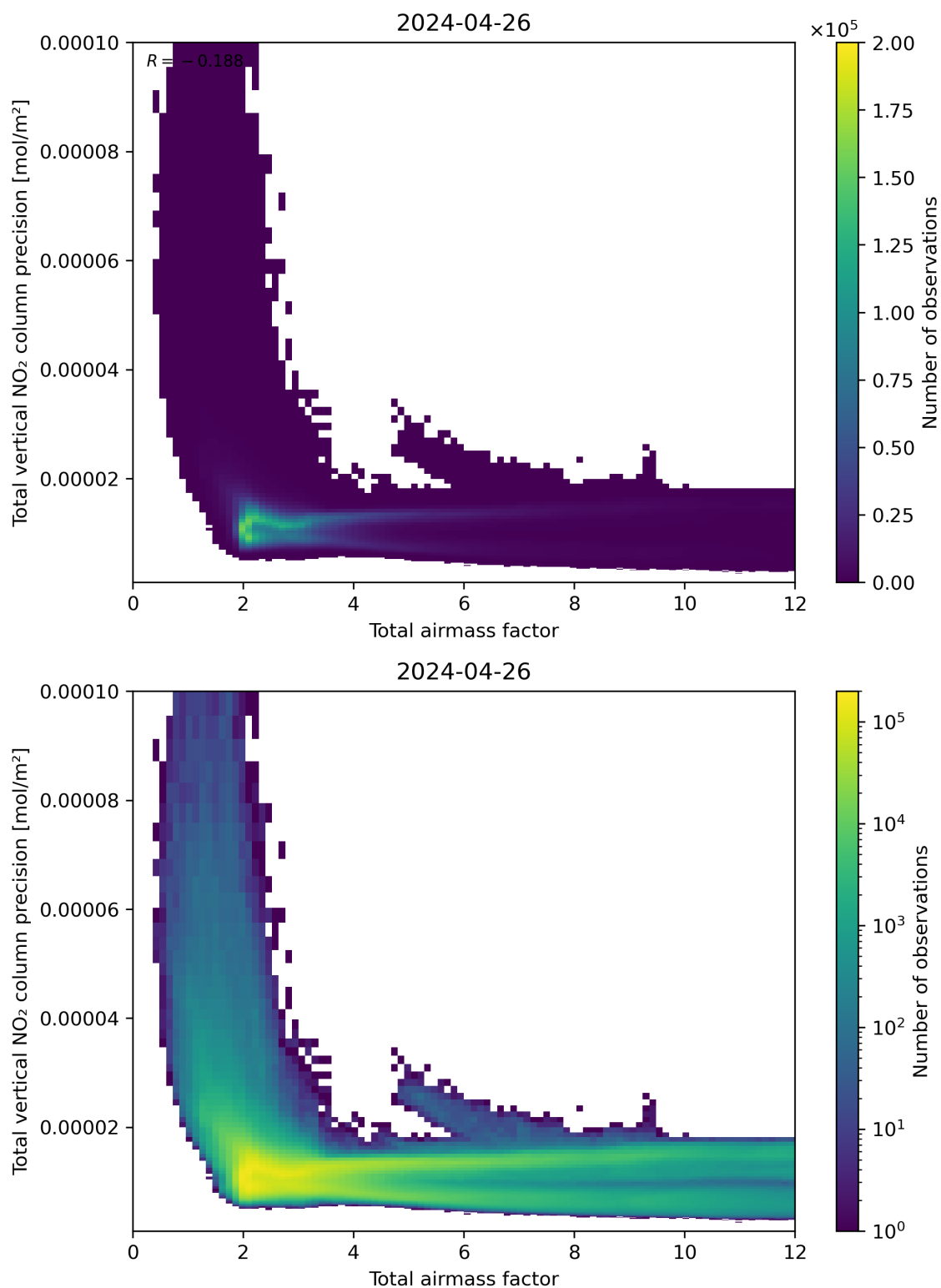
Figure 68: Scatter density plot of “Total airmass factor” against “Total vertical NO 2 column precision” for 2024-04-26 to 2024-04-27.
