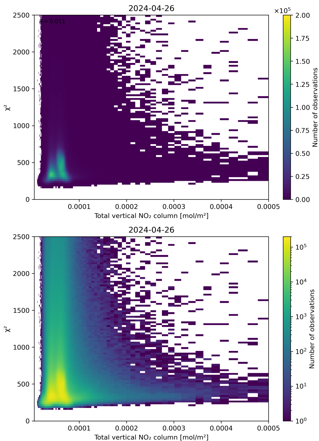
Figure 111: Scatter density plot of “Total vertical NO 2 column” against “ \chi^2 ” for 2024-04-26 to 2024-04-27.
