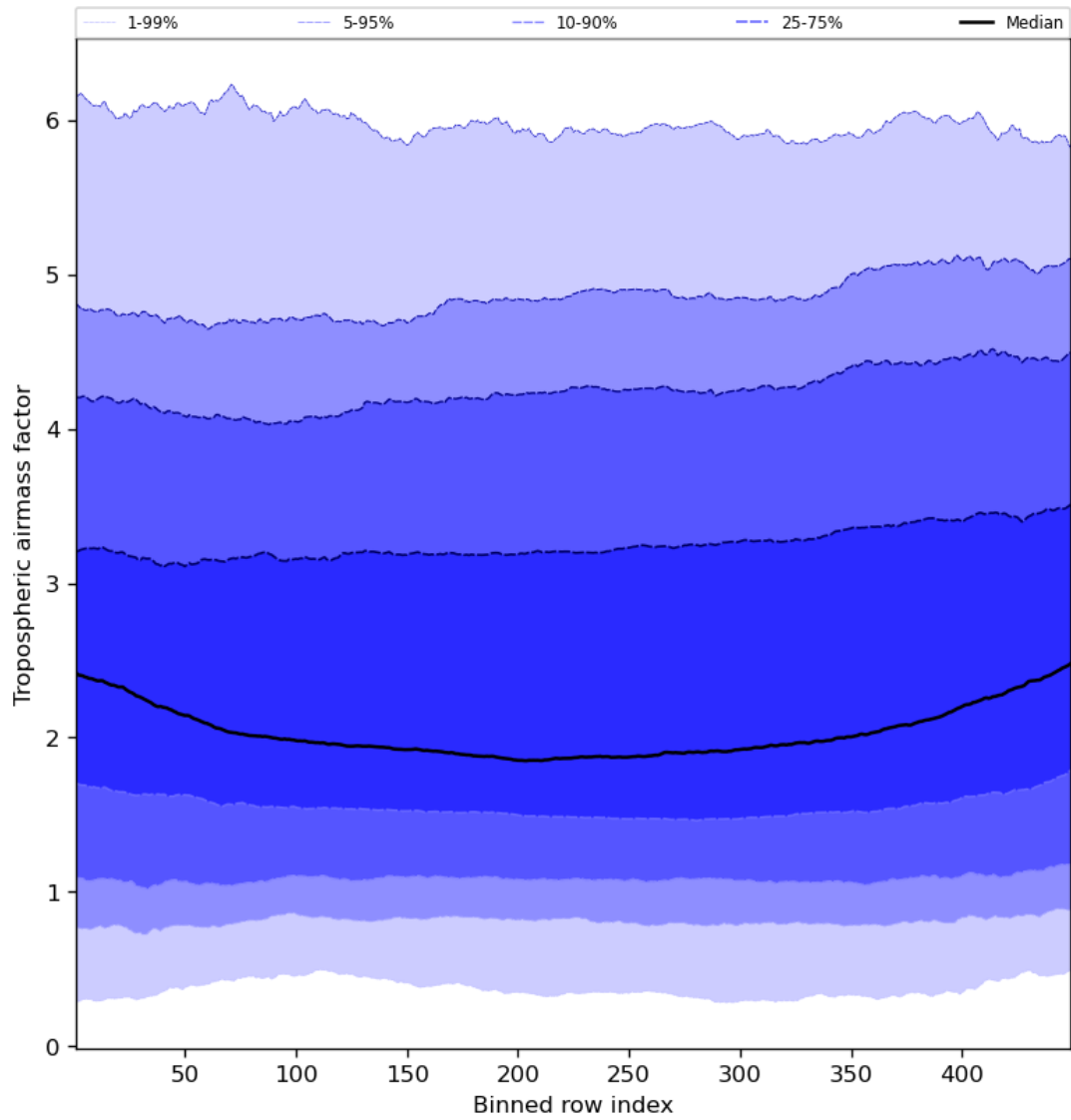
Figure 48: Along track statistics of “Tropospheric airmass factor” for 2024-04-26 to 2024-04-27
