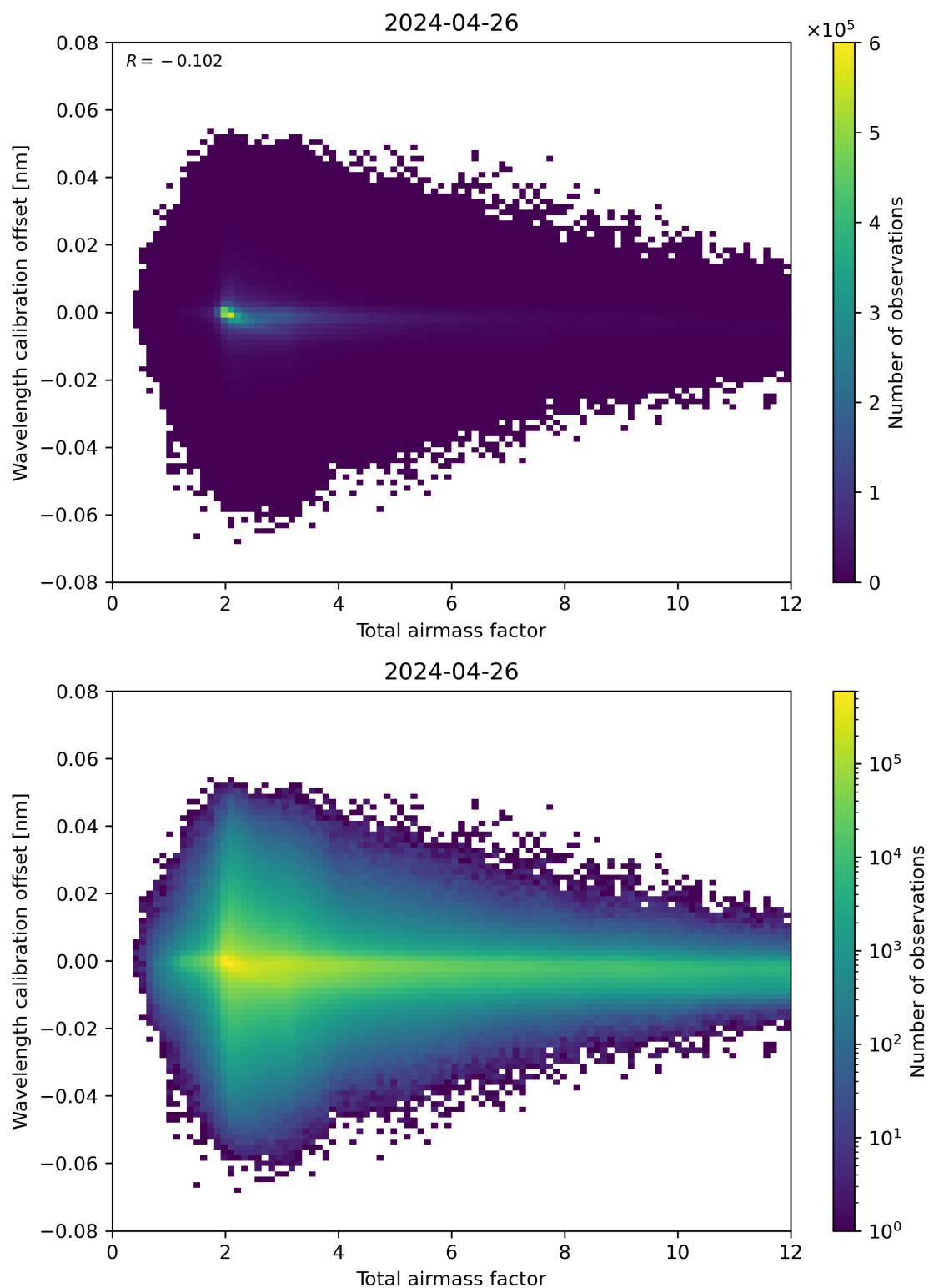
Figure 70: Scatter density plot of “Total airmass factor” against “Wavelength calibration offset” for 2024-04-26 to 2024-04-27.
