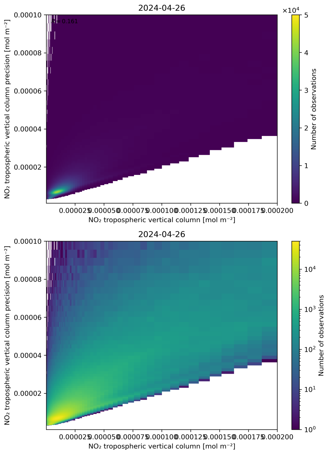
Figure 130: Scatter density plot of “NO 2 tropospheric vertical column” against “NO 2 tropospheric vertical column precision” for 2024-04-26 to 2024-04-27.
