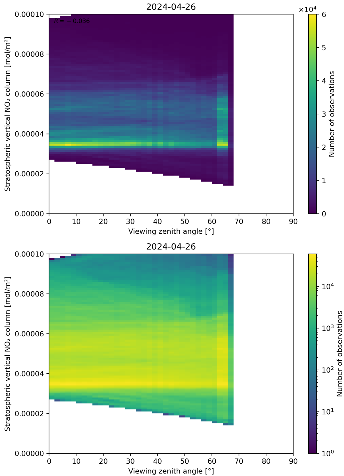
Figure 164: Scatter density plot of “Viewing zenith angle” against “Stratospheric vertical NO 2 column” for 2024-04-26 to 2024-04-27.
