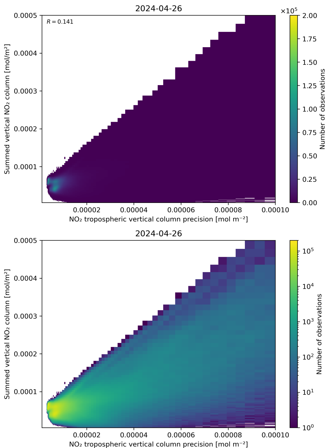
Figure 136: Scatter density plot of “NO 2 tropospheric vertical column precision” against “Summed vertical NO 2 column” for 2024-04-26 to 2024-04-27.
