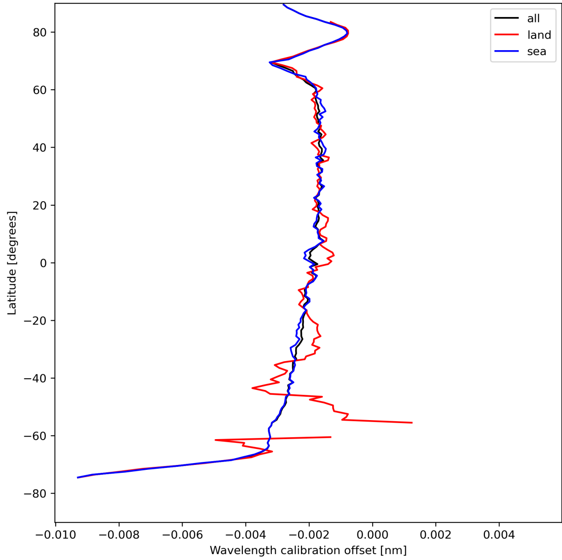
Figure 18: Zonal average of “Wavelength calibration offset” for 2024-04-26 to 2024-04-27.
