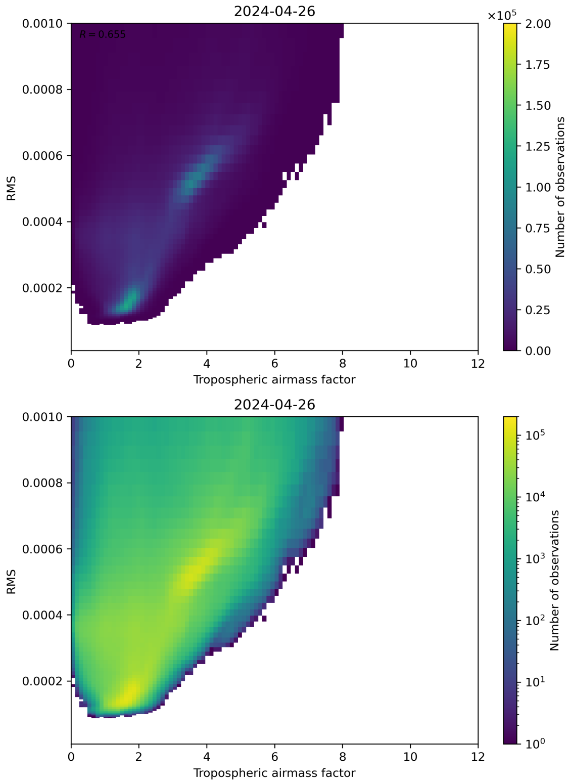
Figure 79: Scatter density plot of “Tropospheric airmass factor” against “RMS” for 2024-04-26 to 2024-04-27.
