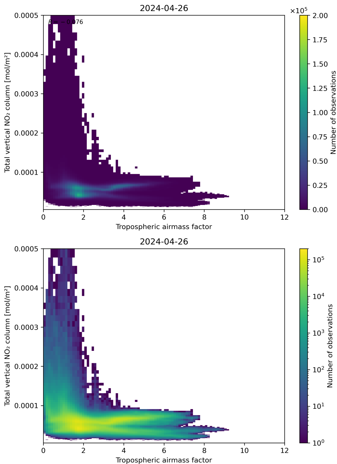
Figure 77: Scatter density plot of “Tropospheric airmass factor” against “Total vertical NO 2 column” for 2024-04-26 to 2024-04-27.
