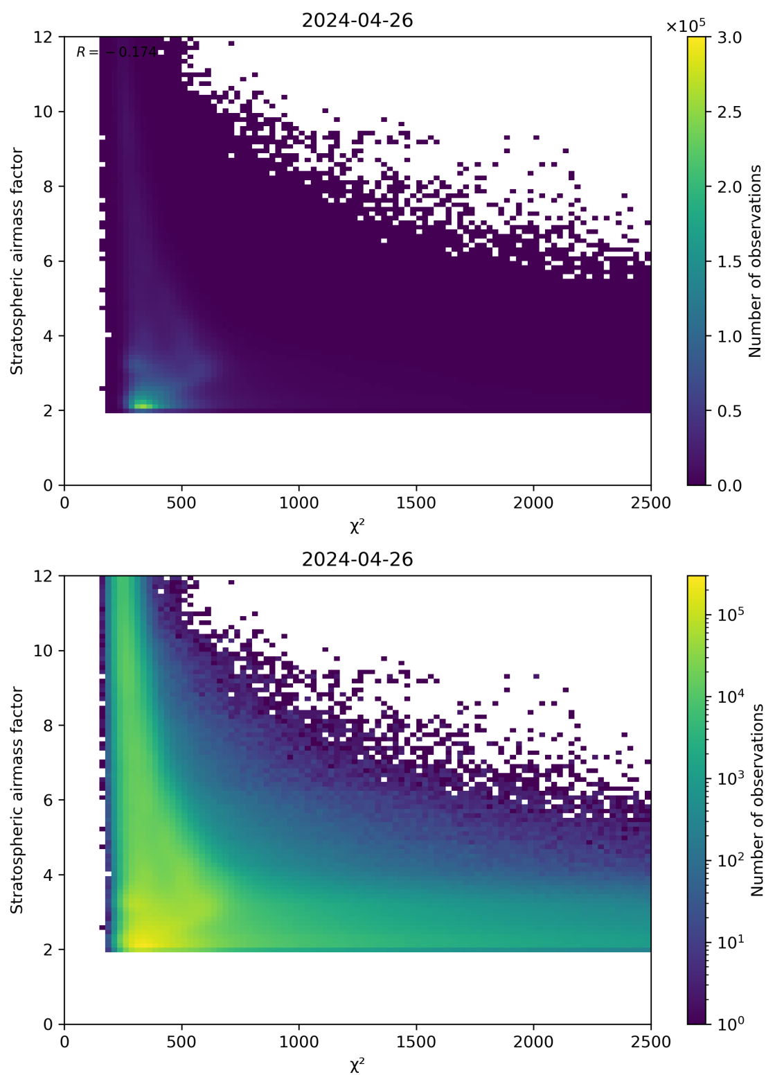
Figure 81: Scatter density plot of “ \chi^2 ” against “Stratospheric airmass factor” for 2024-04-26 to 2024-04-27.
