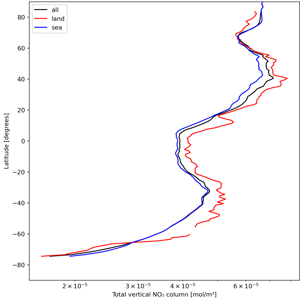
Figure 21: Zonal average of “Total vertical NO 2 column” for 2024-04-26 to 2024-04-27.
