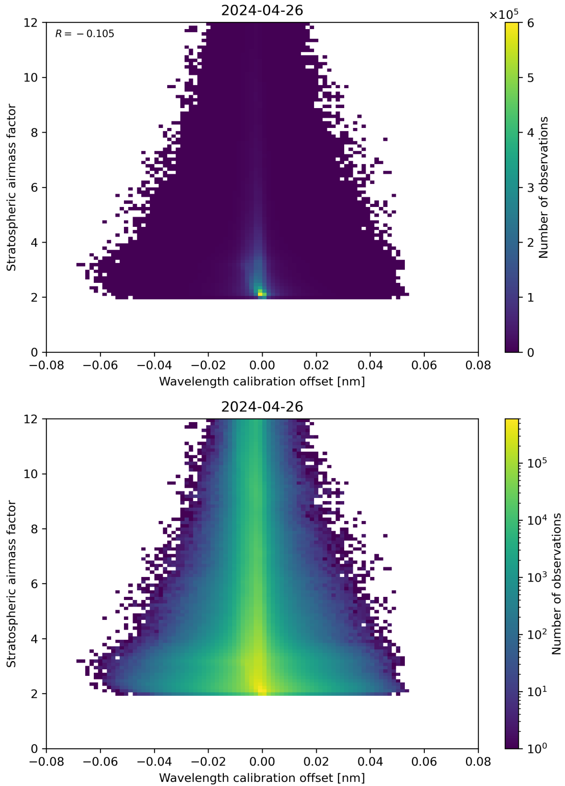
Figure 174: Scatter density plot of “Wavelength calibration offset” against “Stratospheric air mass factor” for 2024-04-26 to 2024-04-27.
