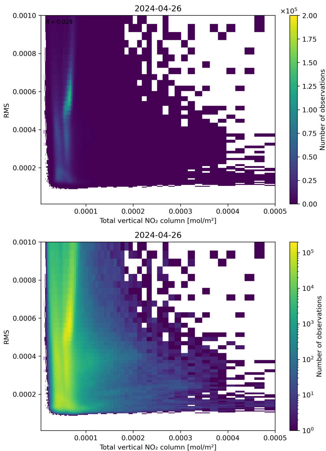
Figure 120: Scatter density plot of “Total vertical NO 2 column” against “RMS” for 2024-04-26 to 2024-04-27.
