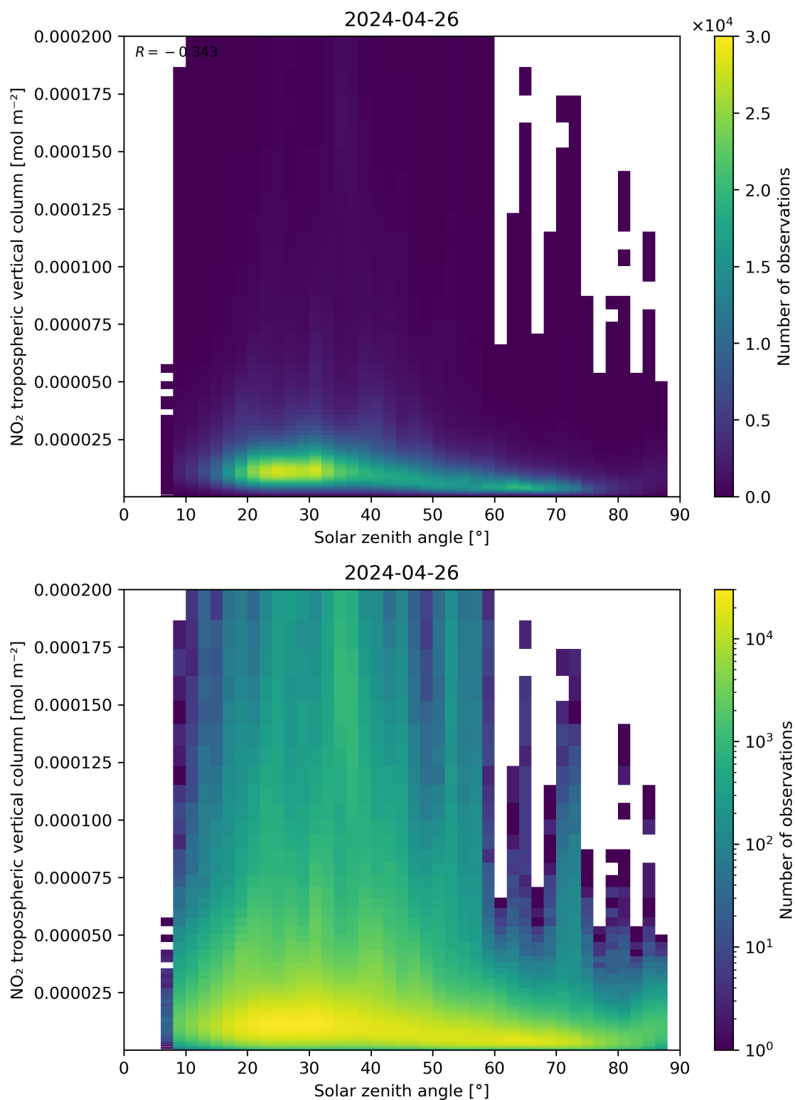
Figure 155: Scatter density plot of “Solar zenith angle” against “NO 2 tropospheric vertical column” for 2024-04-26 to 2024-04-27.
