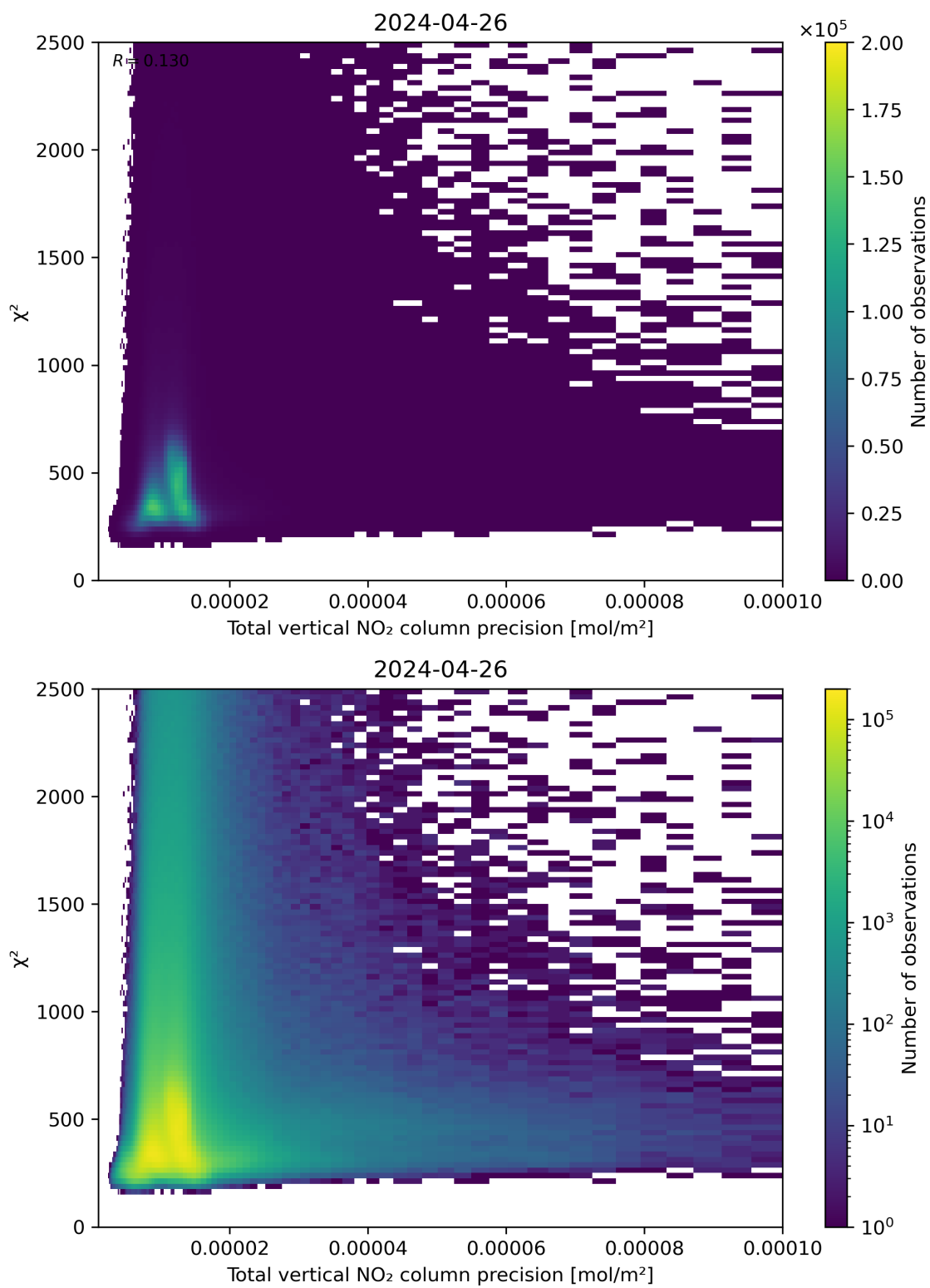
Figure 116: Scatter density plot of “Total vertical NO 2 column precision” against “ \chi^2 ” for 2024-04-26 to 2024-04-27.
