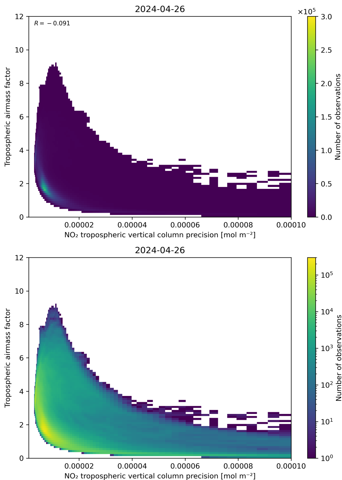
Figure 133: Scatter density plot of “NO 2 tropospheric vertical column precision” against “Tropospheric airmass factor” for 2024-04-26 to 2024-04-27.
