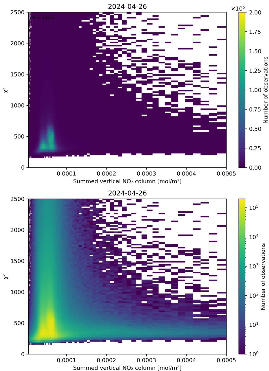
Figure 104: Scatter density plot of “Summed vertical NO 2 column” against “ \chi^2 ” for 2024-04-26 to 2024-04-27.
