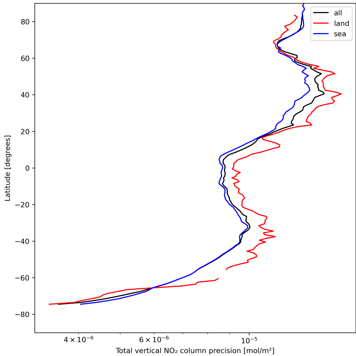
Figure 22: Zonal average of "Total vertical NO 2 column precision" for 2024-04-26 to 2024-04-27.
