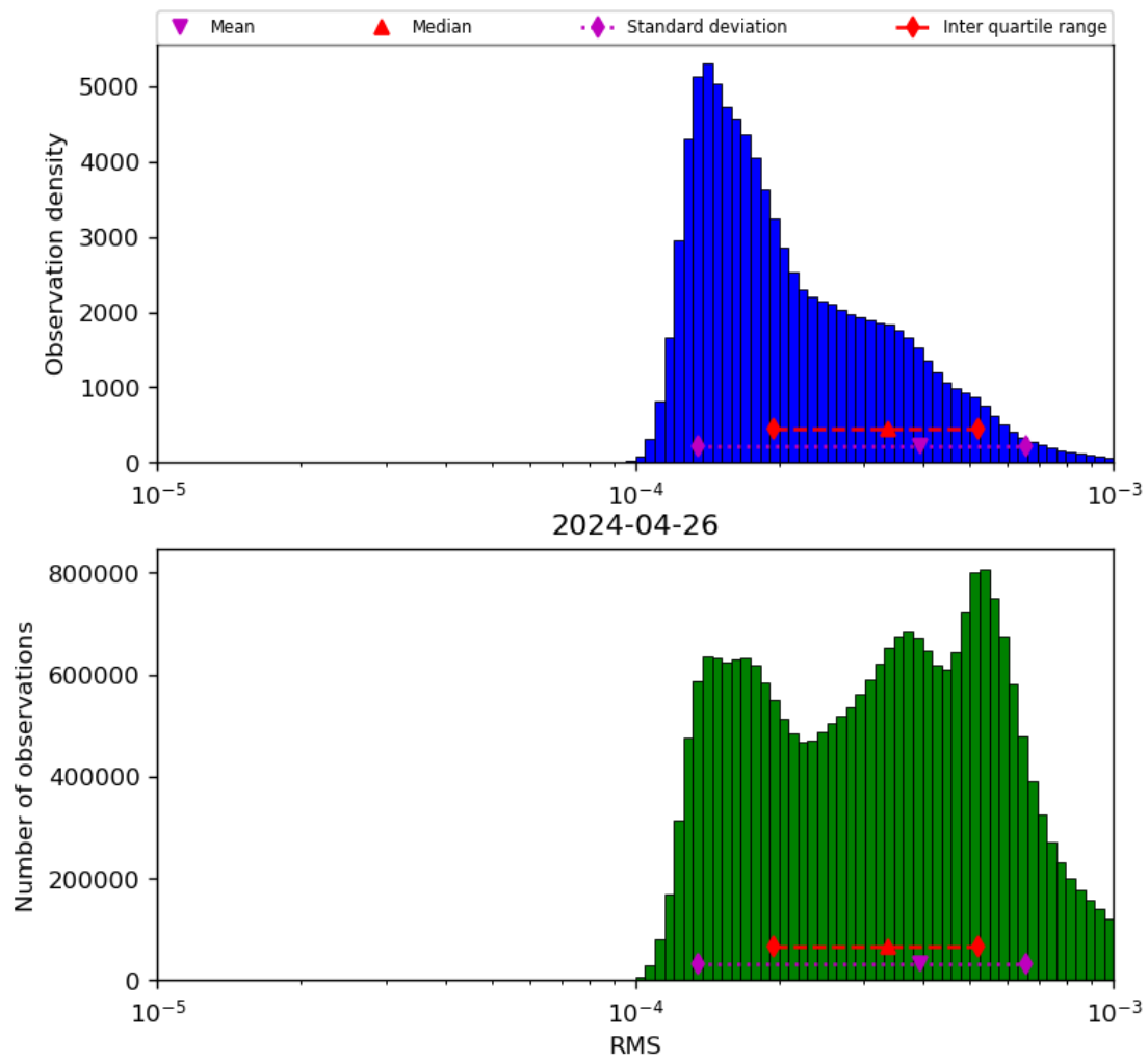
Figure 43: Histogram of “RMS” for 2024-04-26 to 2024-04-27
