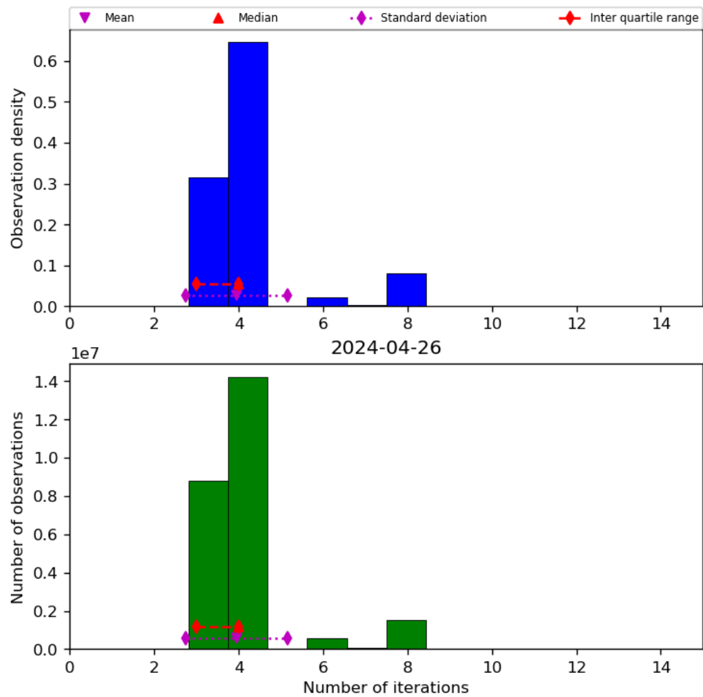
Figure 34: Histogram of “Number of iterations” for 2024-04-26 to 2024-04-27
