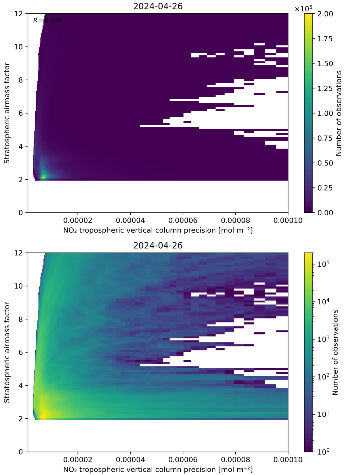
Figure 131: Scatter density plot of “NO 2 tropospheric vertical column precision” against “Stratospheric airmass factor” for 2024-04-26 to 2024-04-27.
