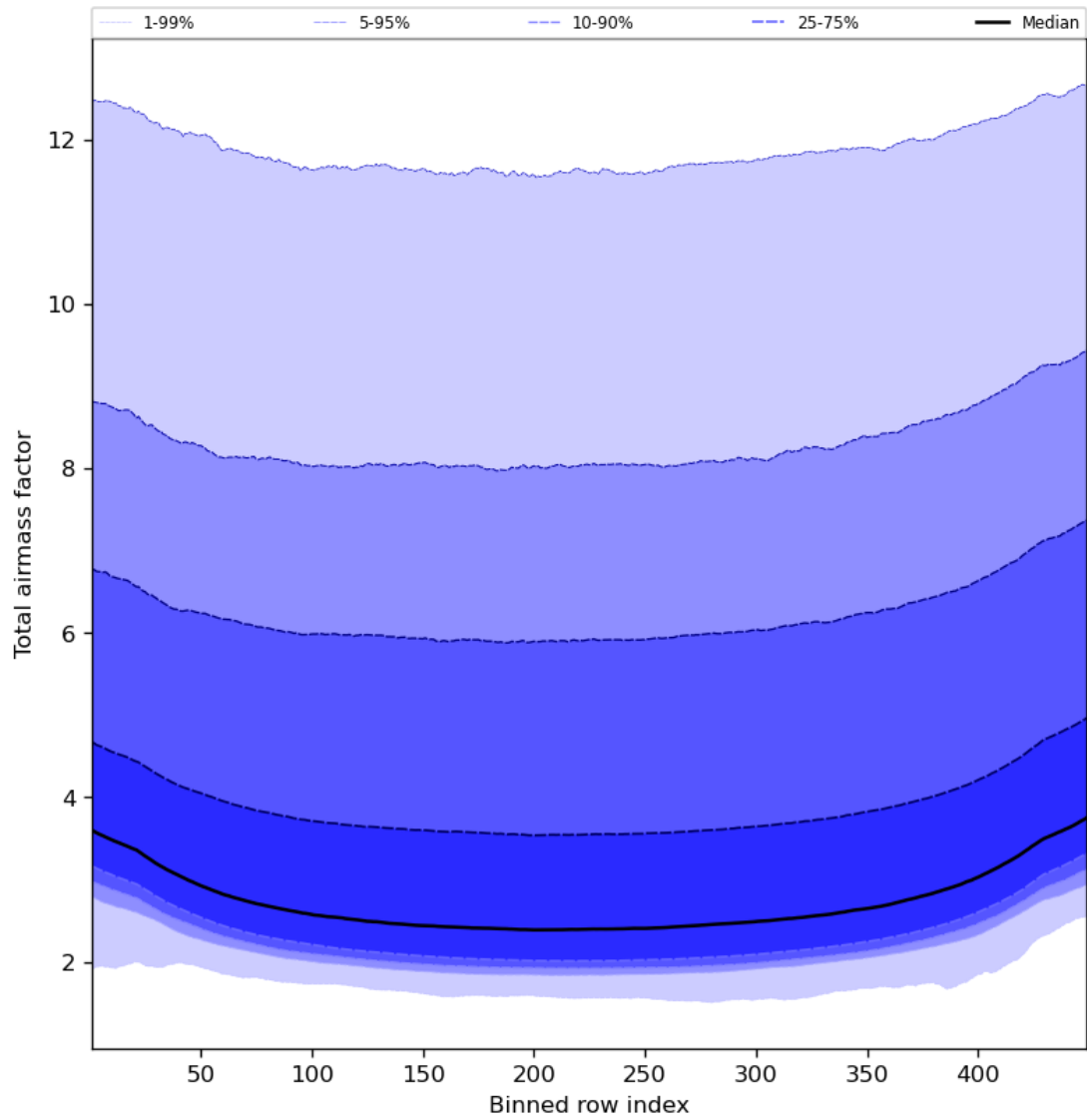
Figure 49: Along track statistics of “Total airmass factor” for 2024-04-26 to 2024-04-27
