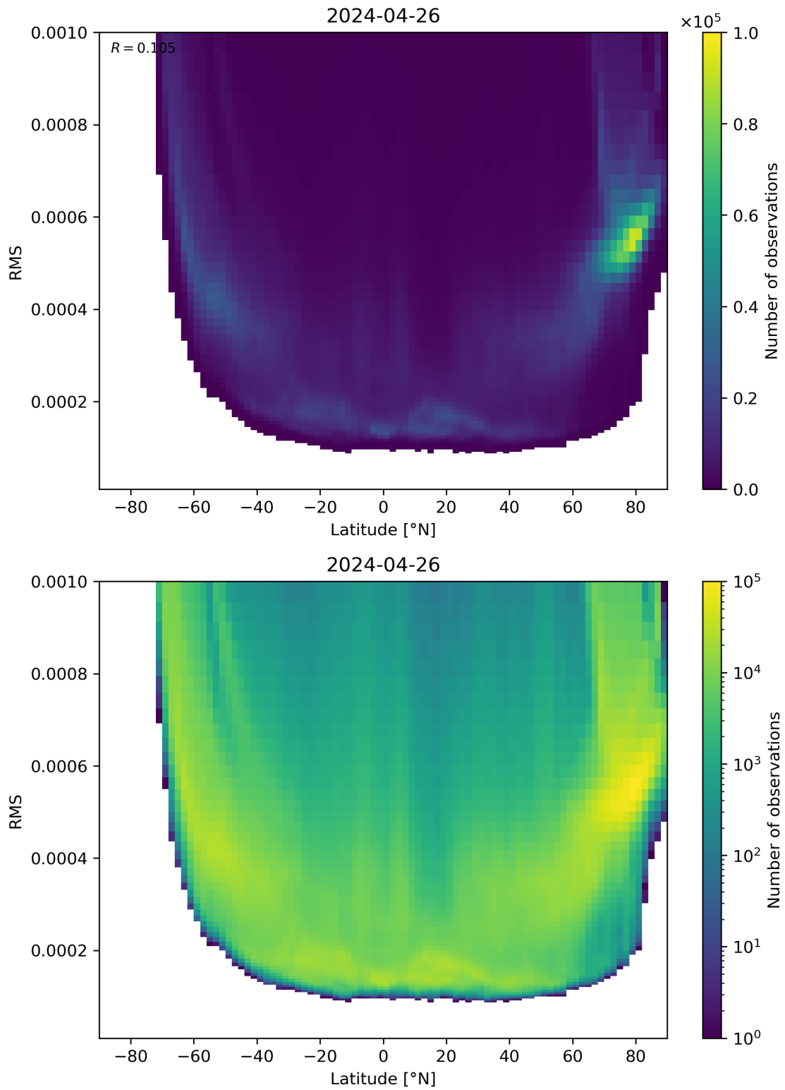
Figure 94: Scatter density plot of “Latitude” against “RMS” for 2024-04-26 to 2024-04-27.
