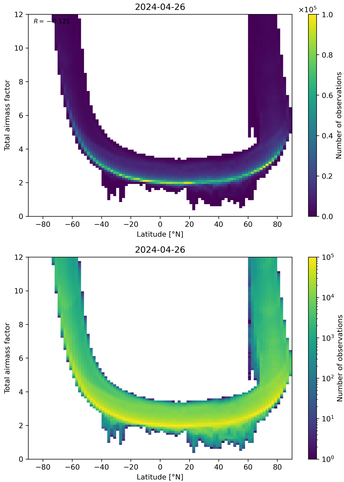
Figure 84: Scatter density plot of “Latitude” against “Total airmass factor” for 2024-04-26 to 2024-04-27.
