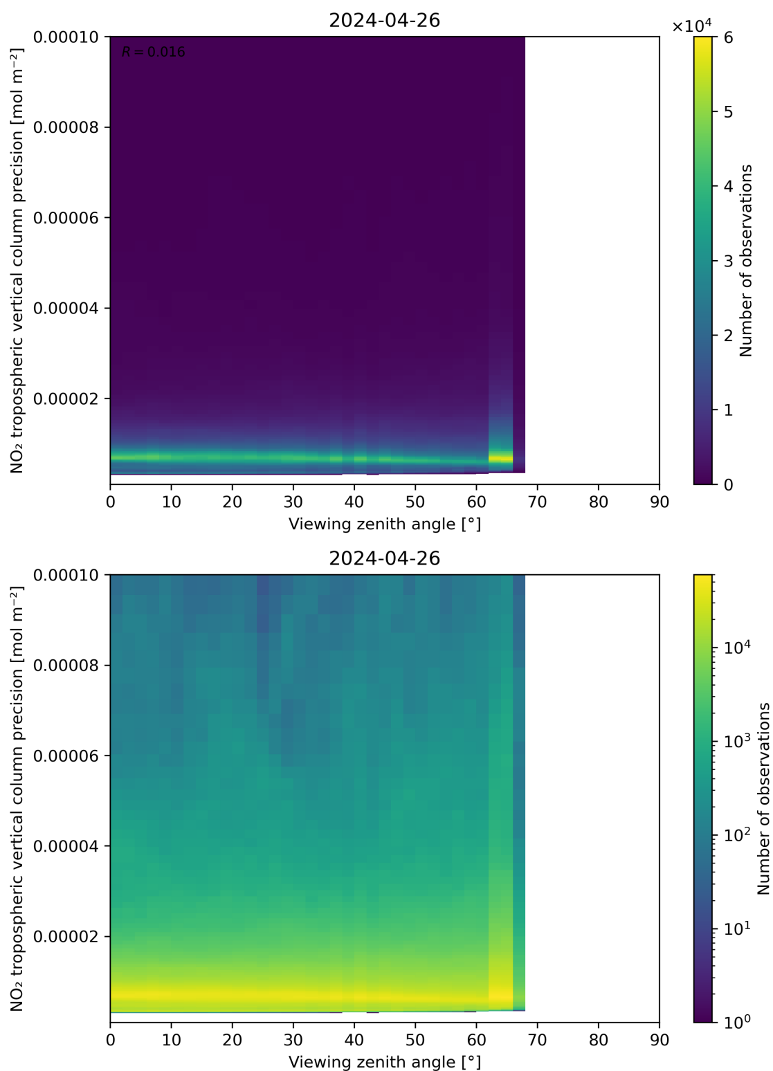
Figure 170: Scatter density plot of “Viewing zenith angle” against “NO 2 tropospheric vertical column precision” for 2024-04-26 to 2024-04-27.
