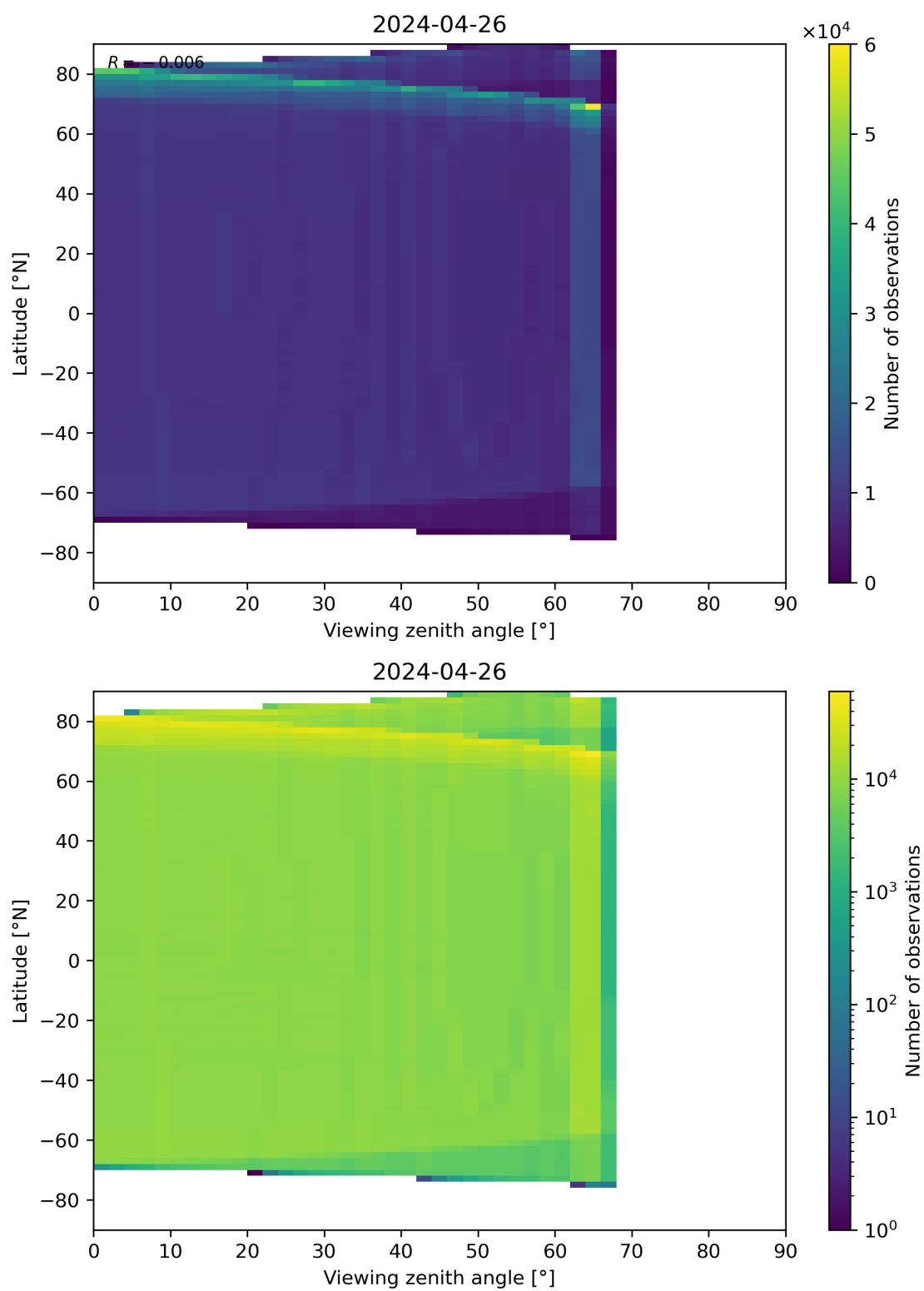
Figure 163: Scatter density plot of “Viewing zenith angle” against “Latitude” for 2024-04-26 to 2024-04-27.
