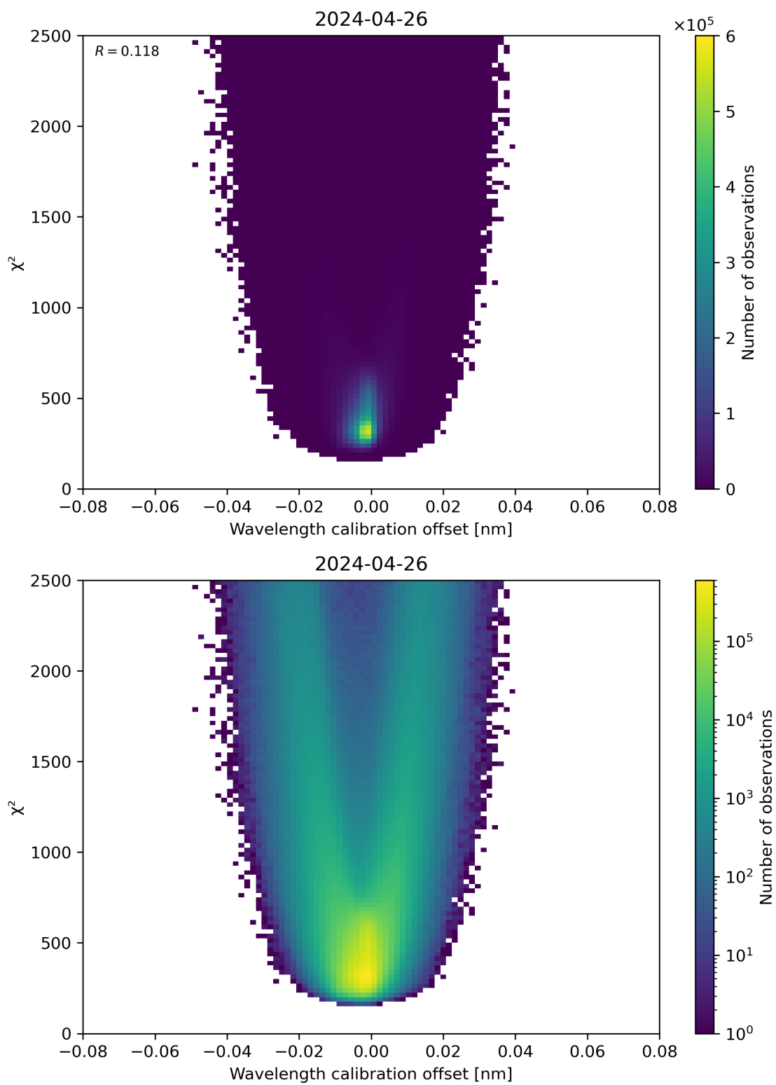
Figure 175: Scatter density plot of “Wavelength calibration offset” against “ \chi^2 ” for 2024-04-26 to 2024-04-27.
