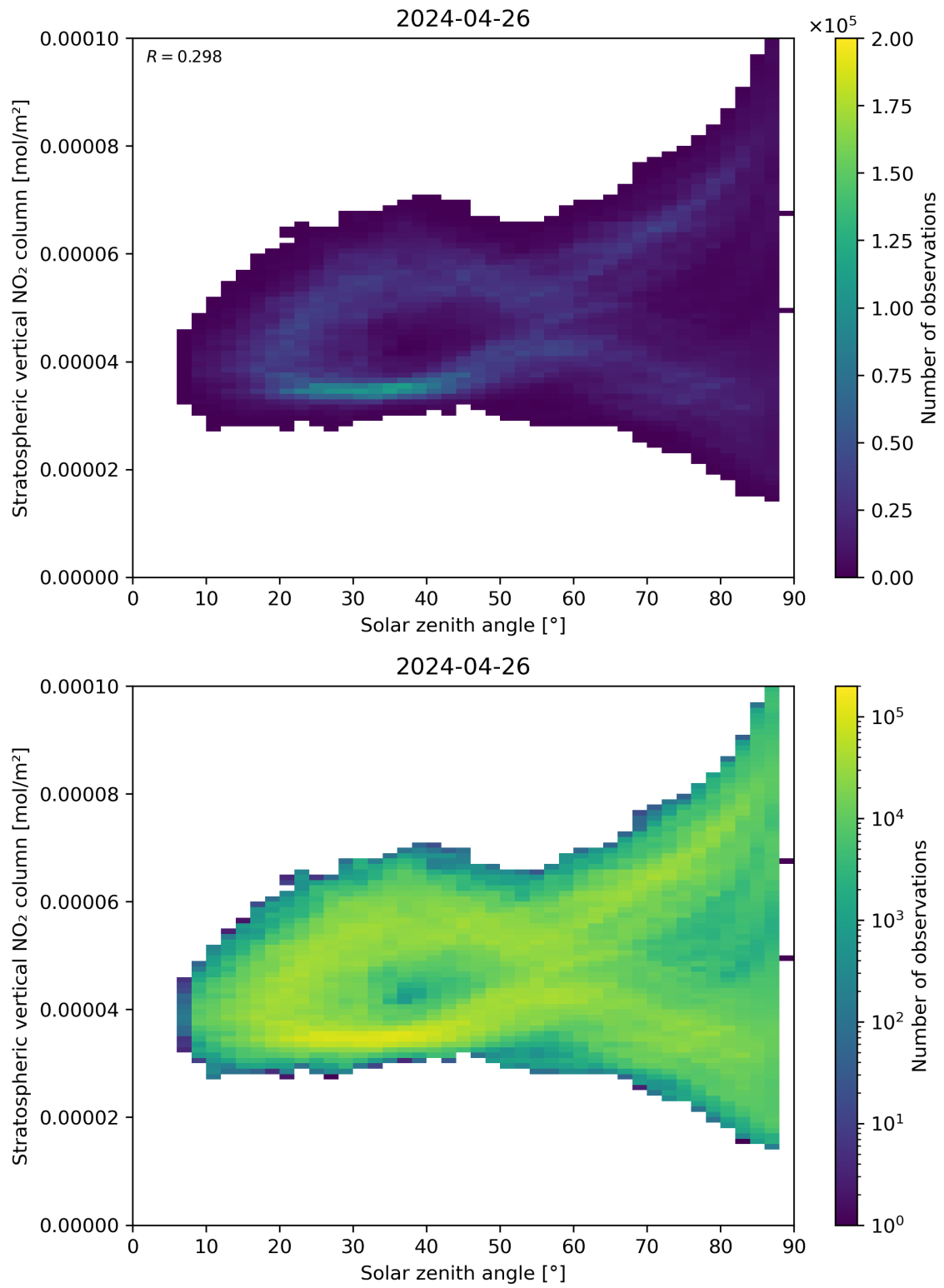
Figure 150: Scatter density plot of “Solar zenith angle” against “Stratospheric vertical NO 2 column” for 2024-04-26 to 2024-04-27.
