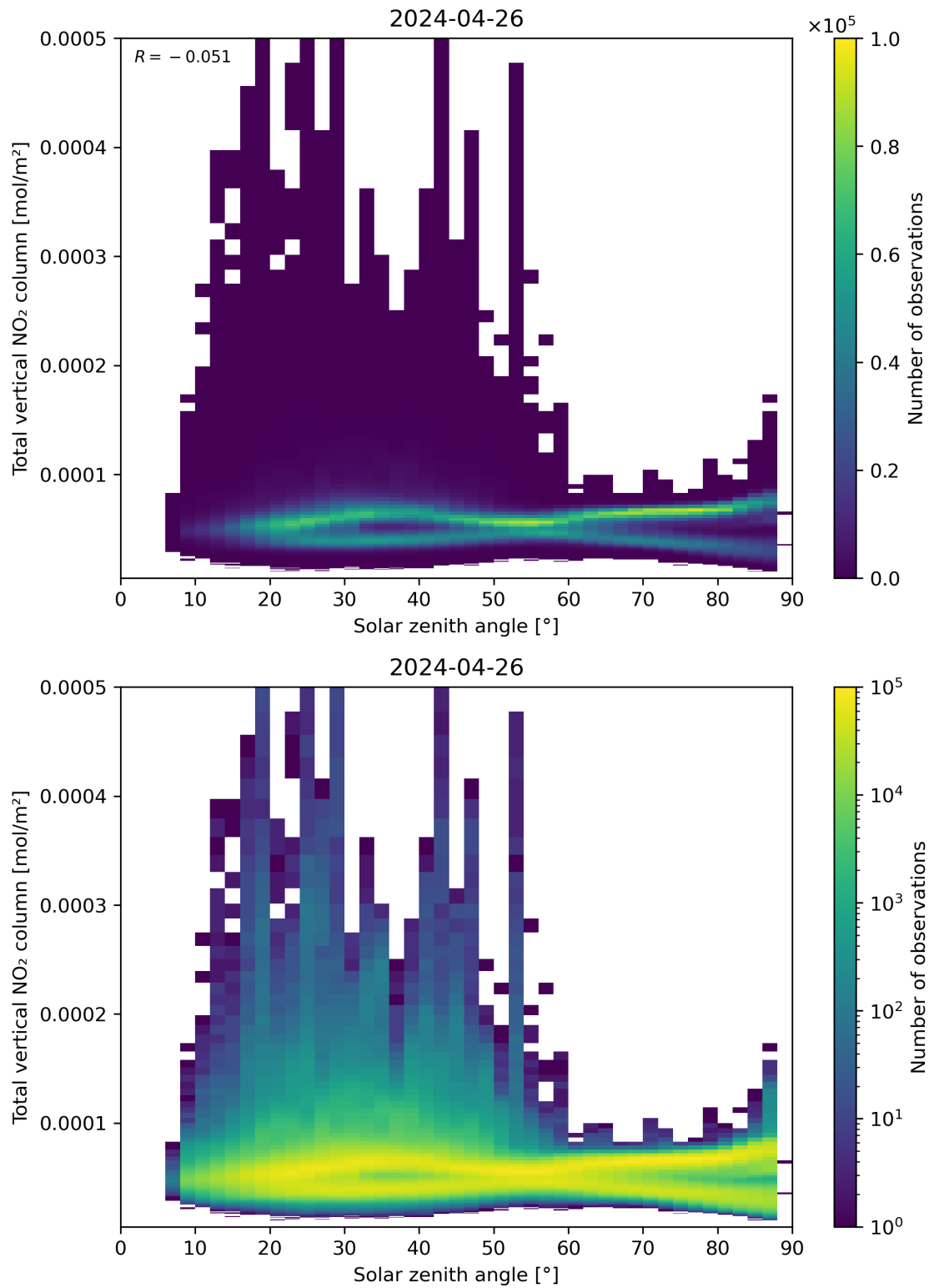
Figure 153: Scatter density plot of “Solar zenith angle” against “Total vertical NO 2 column” for 2024-04-26 to 2024-04-27.
