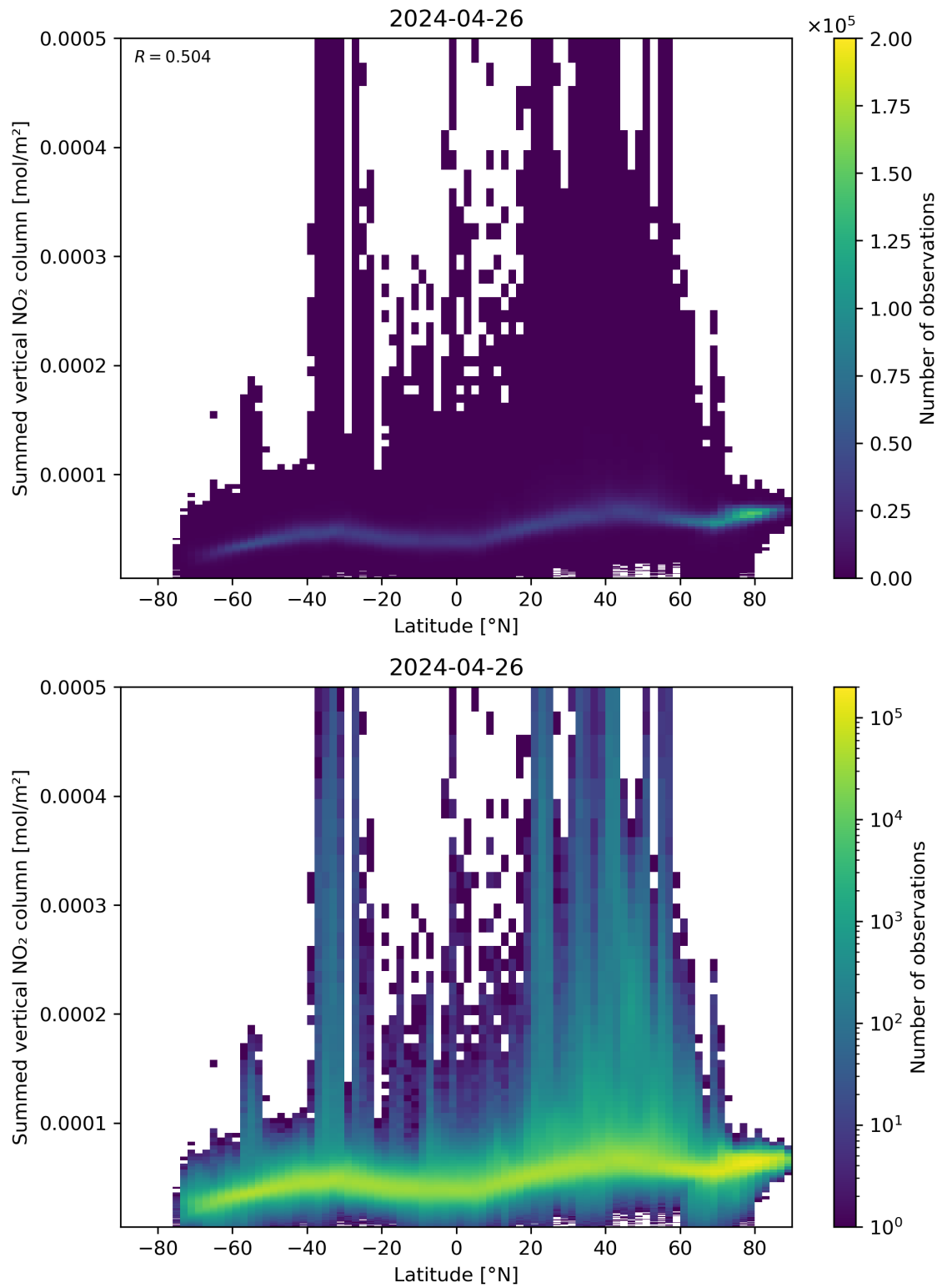
Figure 88: Scatter density plot of “Latitude” against “Summed vertical NO 2 column” for 2024-04-26 to 2024-04-27.
