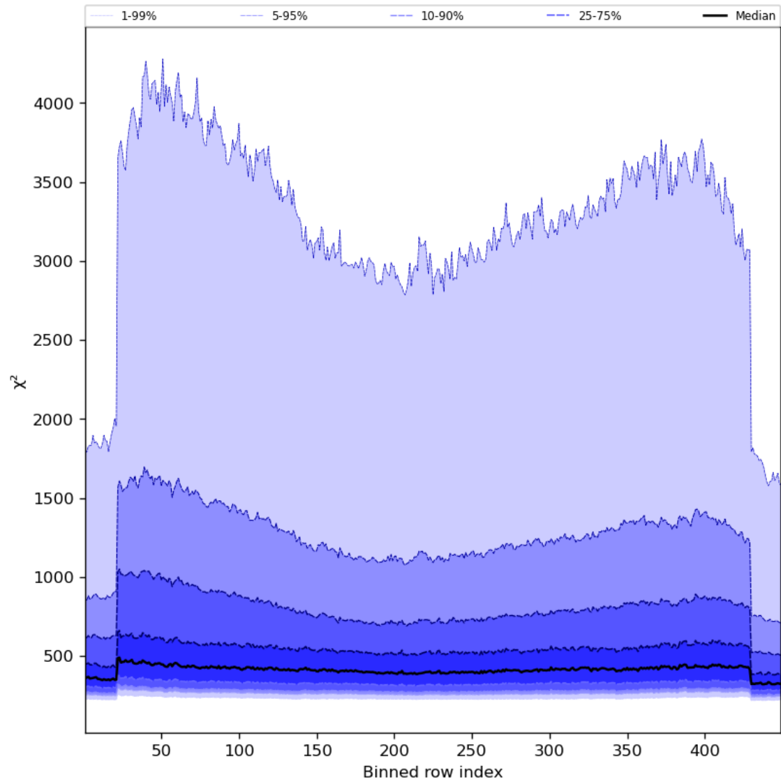
Figure 59: Along track statistics of “ \chi^2 ” for 2024-04-26 to 2024-04-27
