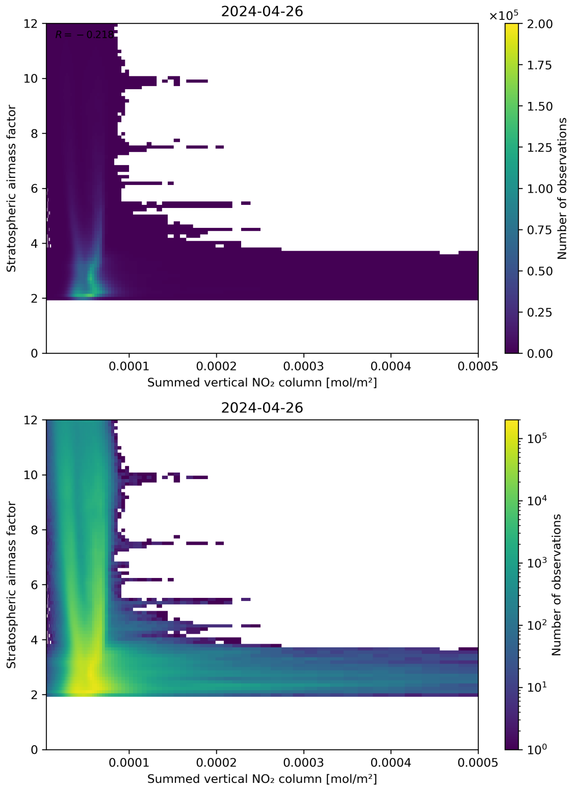
Figure 103: Scatter density plot of “Summed vertical NO 2 column” against “Stratospheric airmass factor” for 2024-04-26 to 2024-04-27.
