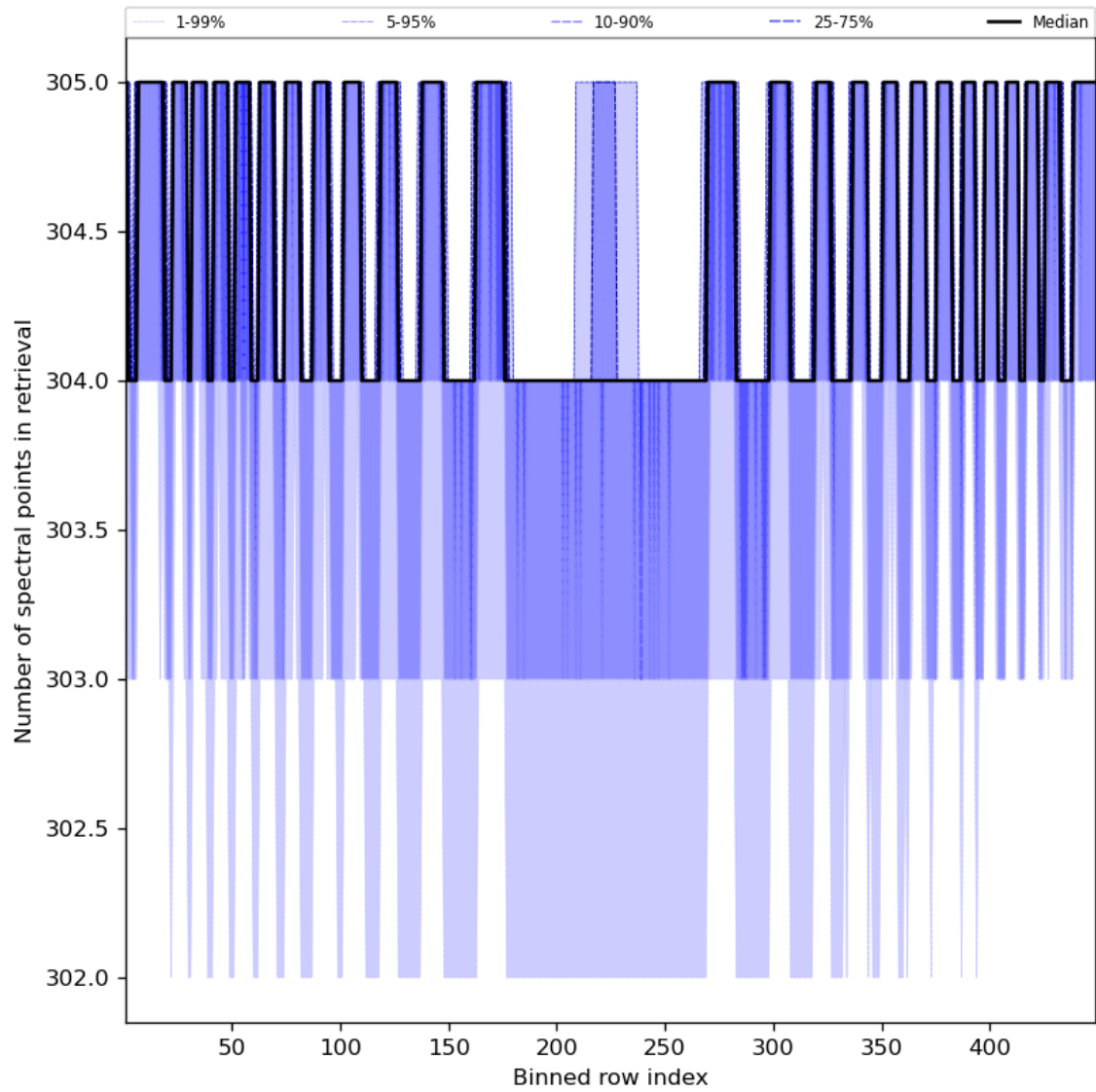
Figure 50: Along track statistics of “Number of spectral points in retrieval” for 2024-04-26 to 2024-04-27
