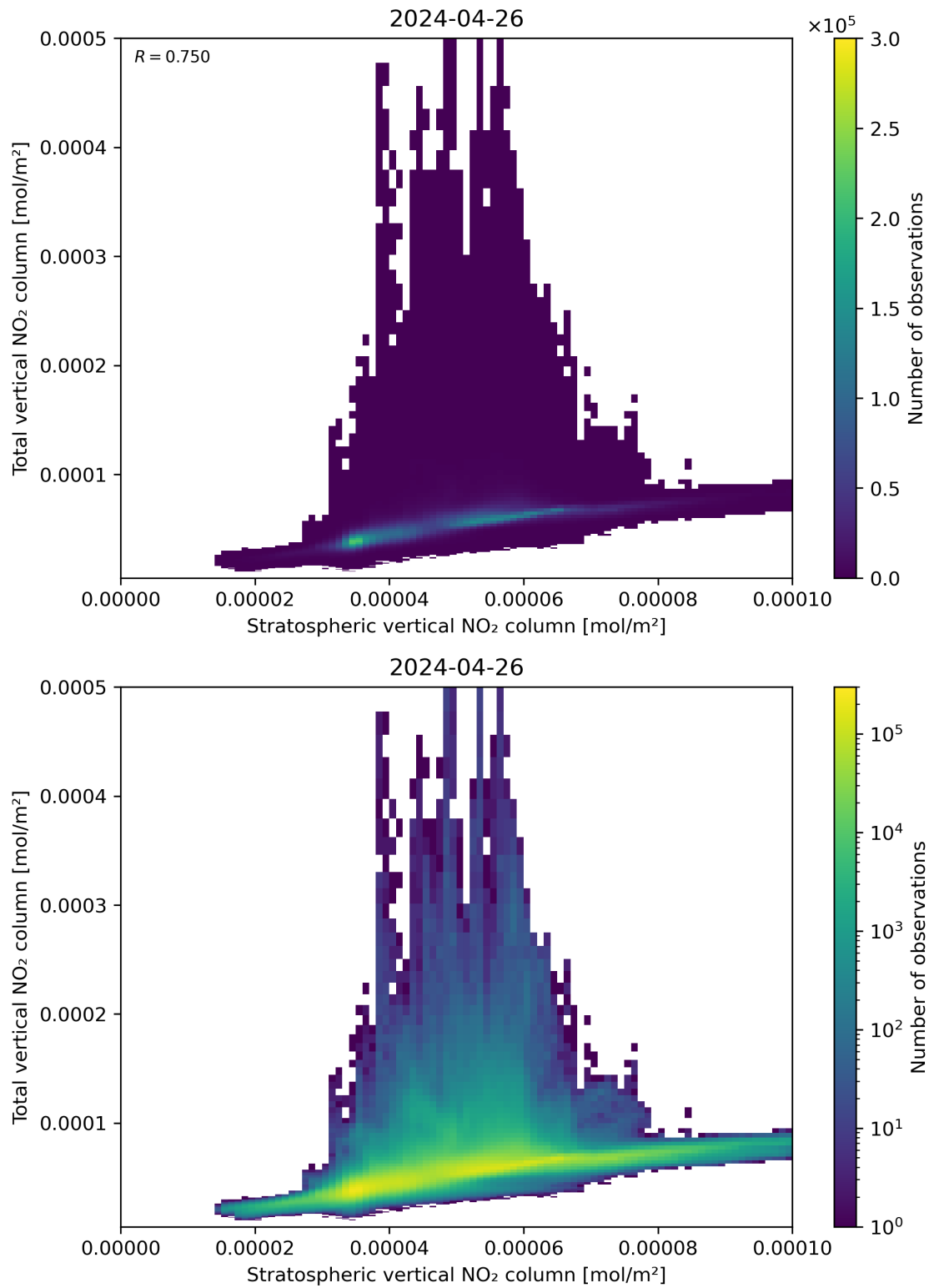
Figure 100: Scatter density plot of “Stratospheric vertical NO 2 column” against “Total vertical NO 2 column” for 2024-04-26 to 2024-04-27.
