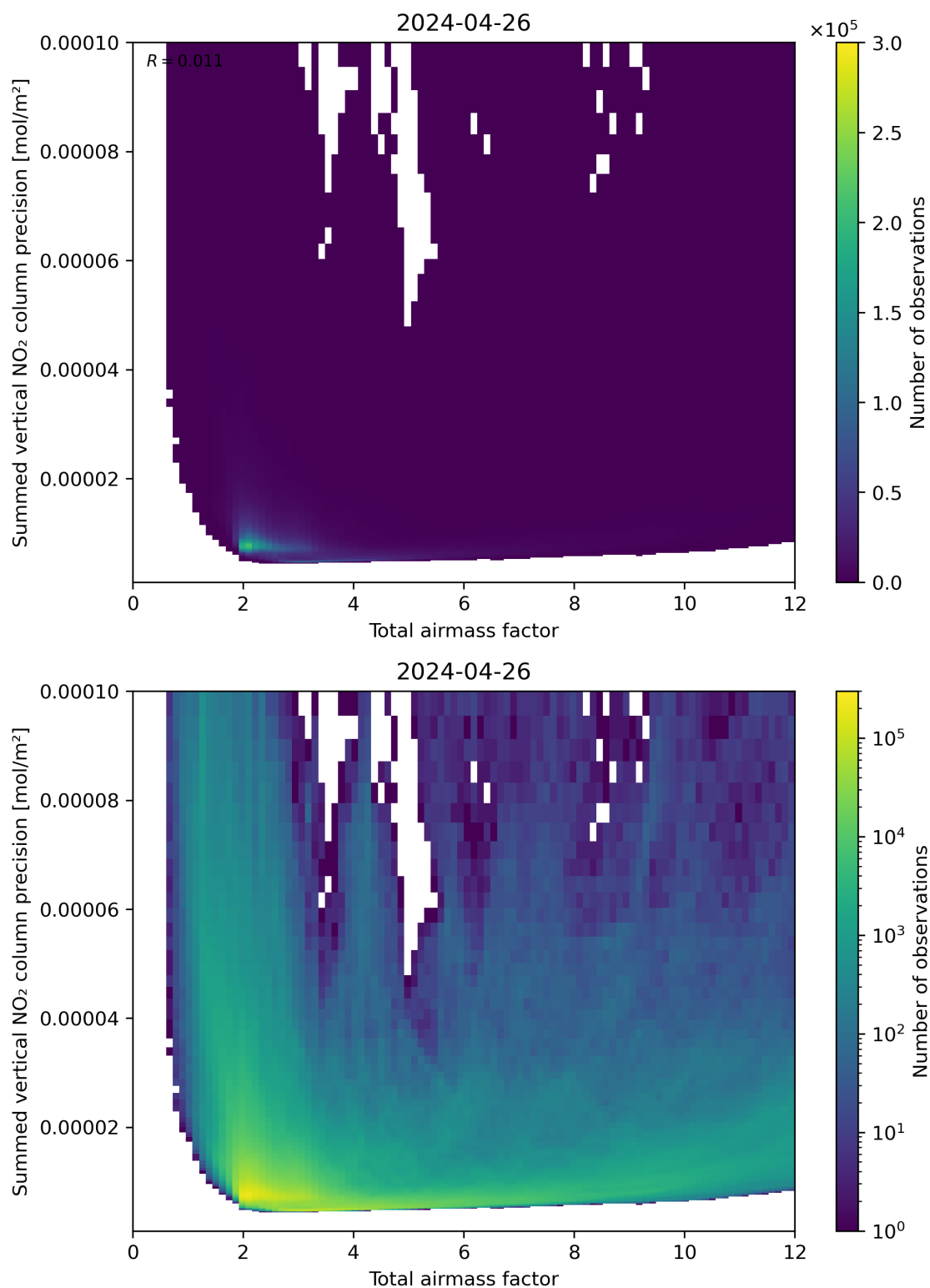
Figure 66: Scatter density plot of “Total airmass factor” against “Summed vertical NO 2 column precision” for 2024-04-26 to 2024-04-27.
