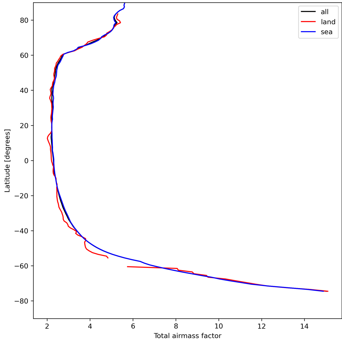
Figure 15: Zonal average of “Total airmass factor” for 2024-04-26 to 2024-04-27.
