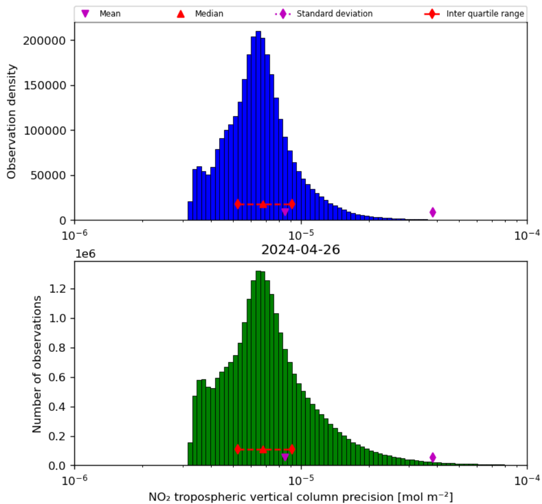
Figure 30: Histogram of “NO 2 tropospheric vertical column precision” for 2024-04-26 to 2024-04-27
