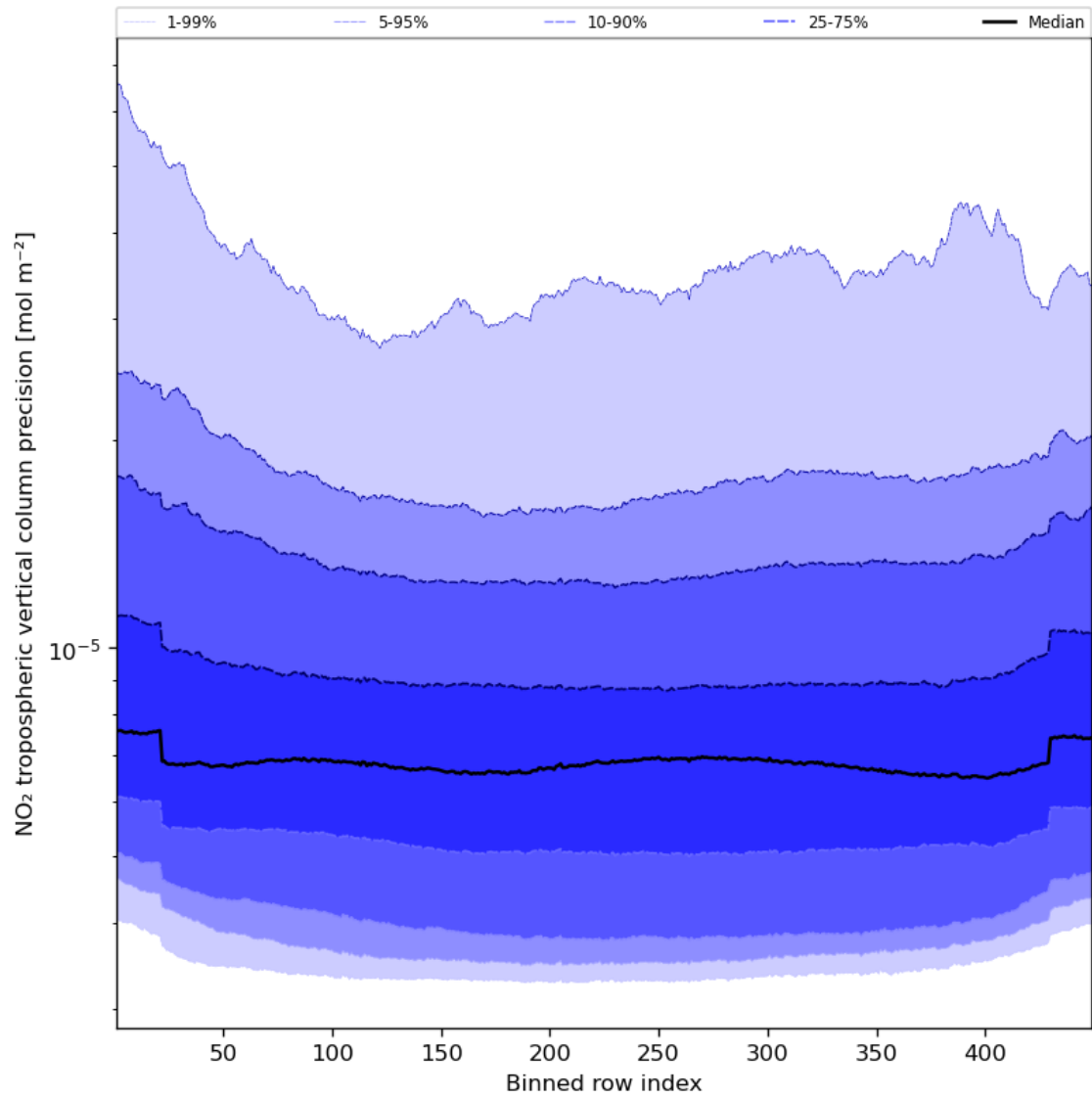
Figure 47: Along track statistics of “NO 2 tropospheric vertical column precision” for 2024-04-26 to 2024-04-27
