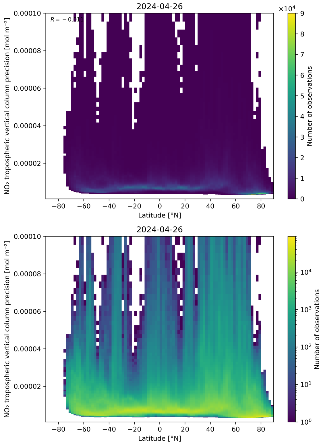
Figure 93: Scatter density plot of “Latitude” against “NO 2 tropospheric vertical column precision” for 2024-04-26 to 2024-04-27.
