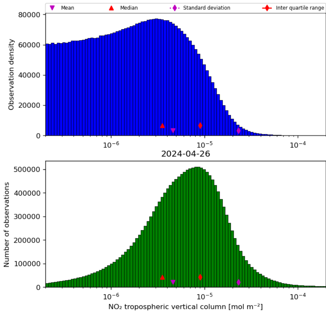
Figure 29: Histogram of “NO 2 tropospheric vertical column” for 2024-04-26 to 2024-04-27
