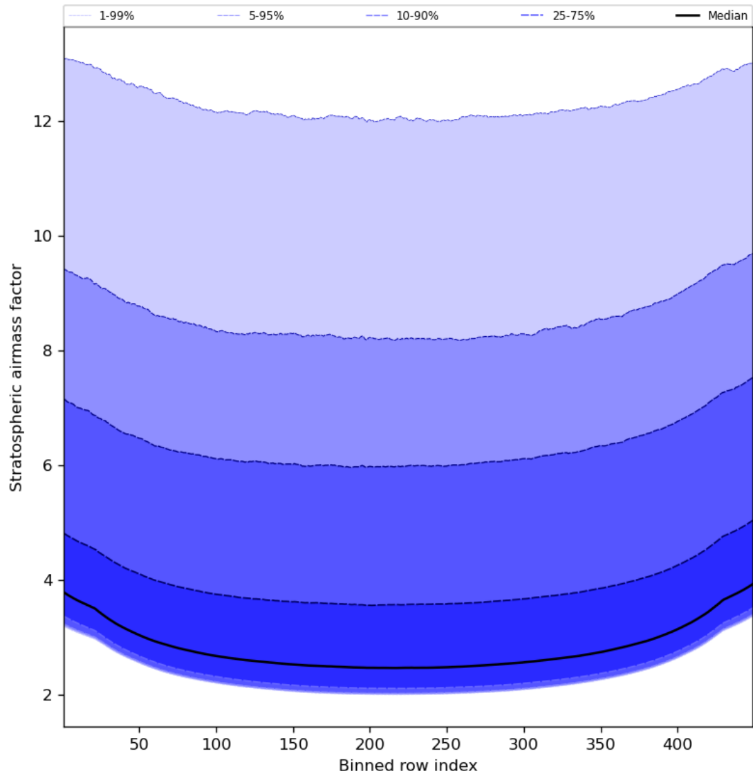
Figure 61: Along track statistics of “Stratospheric airmass factor” for 2024-04-26 to 2024-04-27
