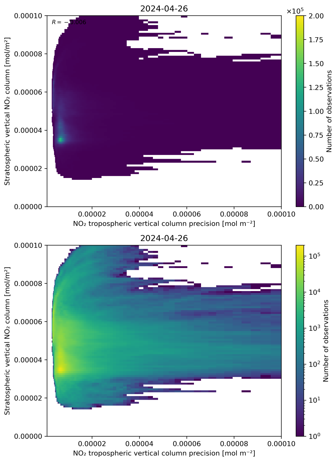
Figure 135: Scatter density plot of “NO 2 tropospheric vertical column precision” against “Stratospheric vertical NO 2 column” for 2024-04-26 to 2024-04-27.
