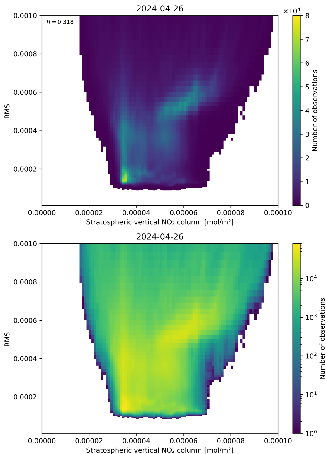
Figure 102: Scatter density plot of “Stratospheric vertical NO 2 column” against “RMS” for 2024-04-26 to 2024-04-27.
