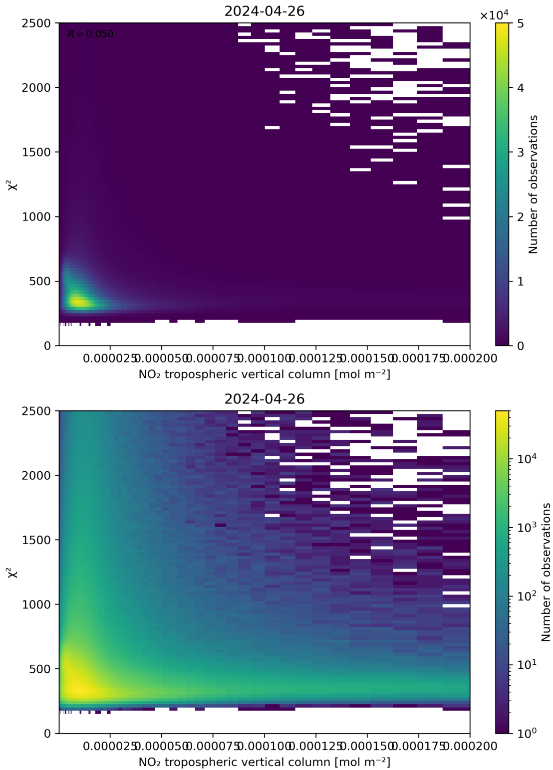
Figure 124: Scatter density plot of “NO 2 tropospheric vertical column” against “ \chi^2 ” for 2024-04-26 to 2024-04-27.
