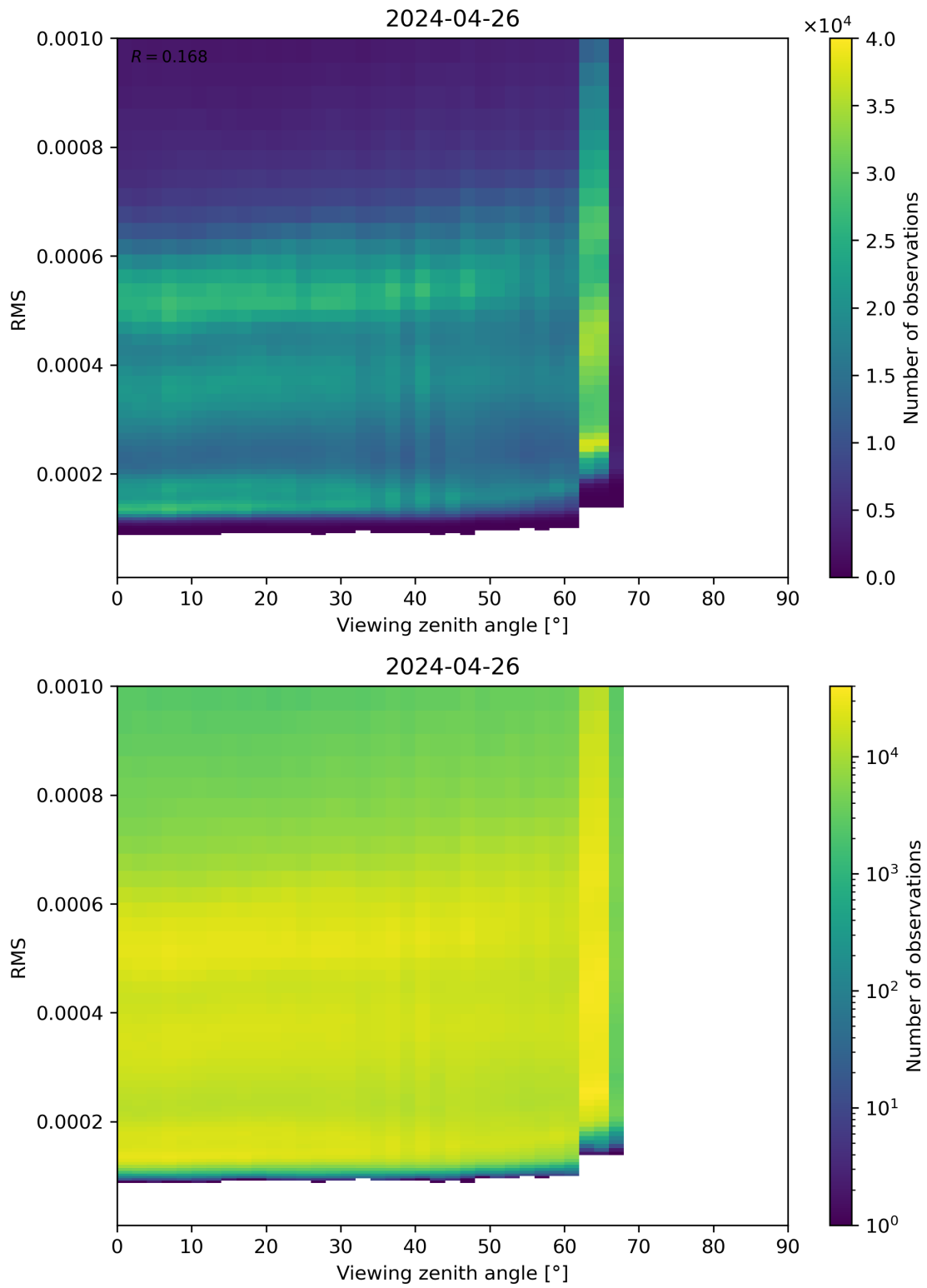
Figure 171: Scatter density plot of “Viewing zenith angle” against “RMS” for 2024-04-26 to 2024-04-27.
