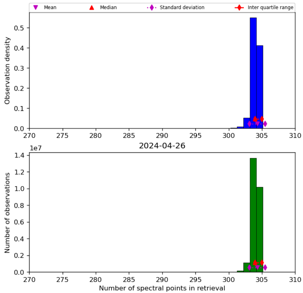
Figure 33: Histogram of “Number of spectral points in retrieval” for 2024-04-26 to 2024-04-27
