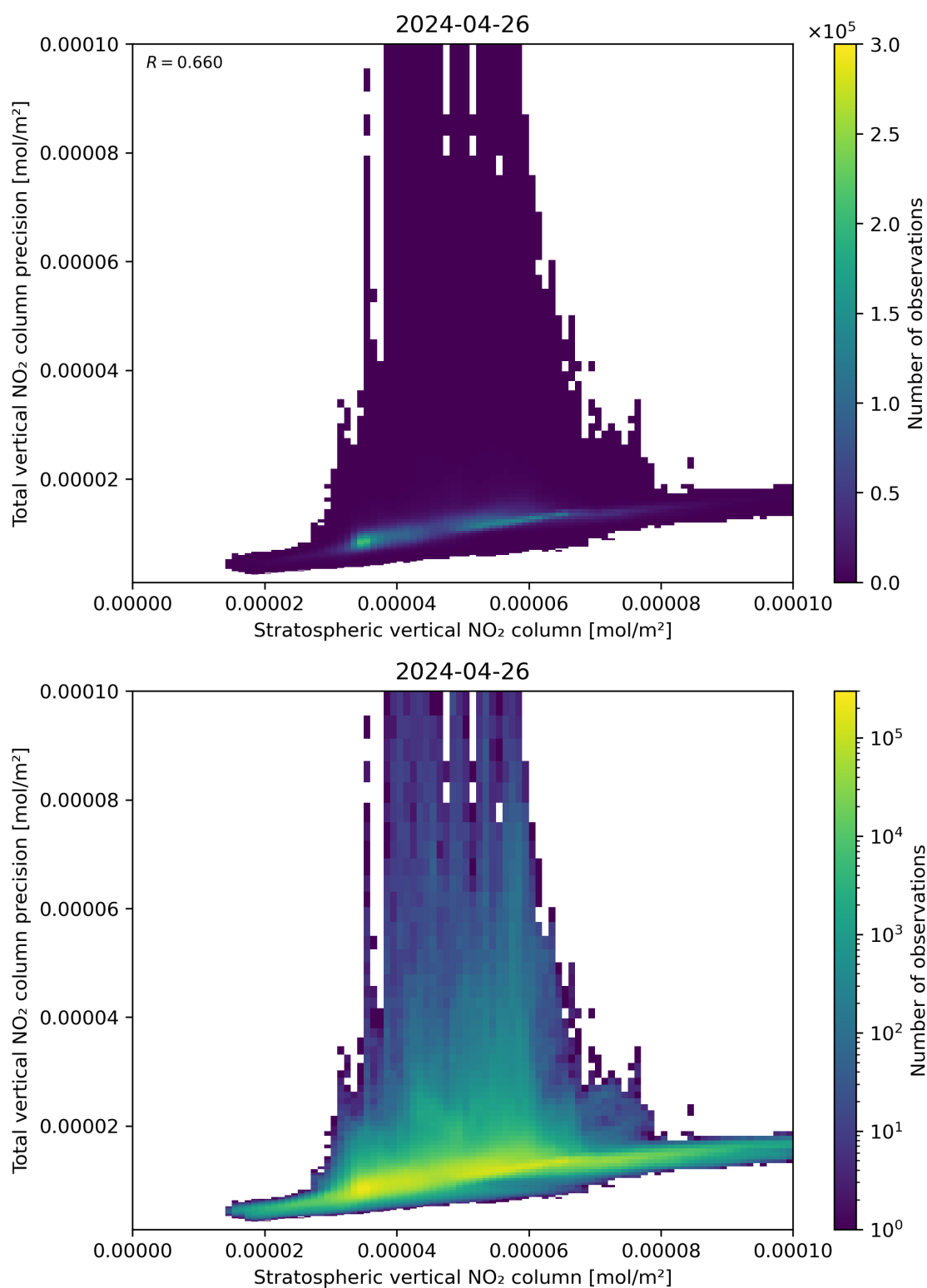
Figure 101: Scatter density plot of “Stratospheric vertical NO 2 column” against “Total vertical NO 2 column precision” for 2024-04-26 to 2024-04-27.
