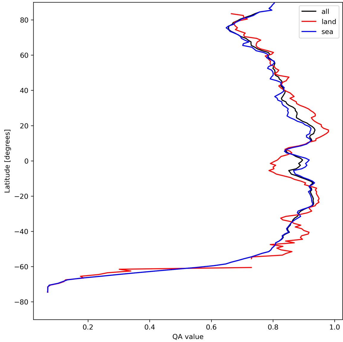
Figure 11: Zonal average of “QA value” for 2024-04-26 to 2024-04-27.
