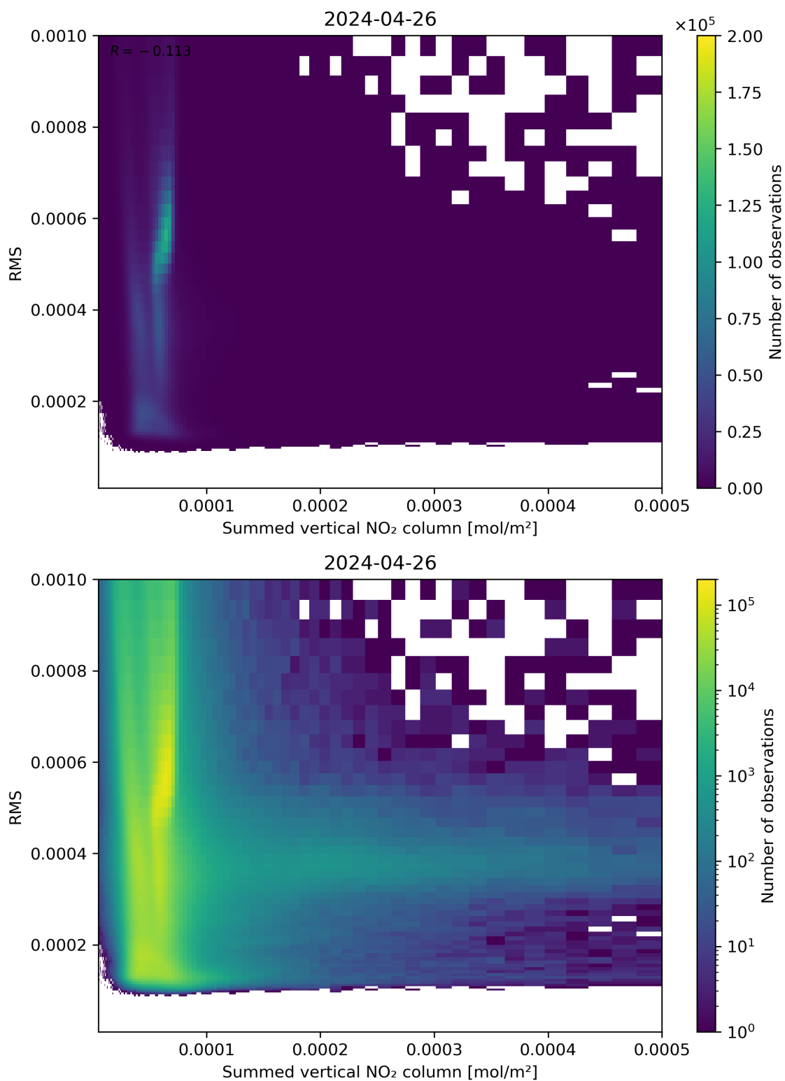
Figure 109: Scatter density plot of “Summed vertical NO 2 column” against “RMS” for 2024-04-26 to 2024-04-27.
