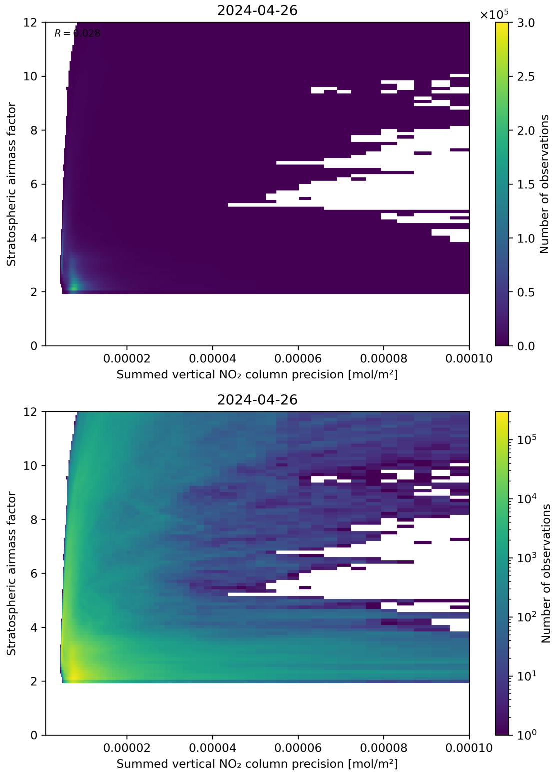
Figure 106: Scatter density plot of “Summed vertical NO 2 column precision” against “Stratospheric airmass factor” for 2024-04-26 to 2024-04-27.
