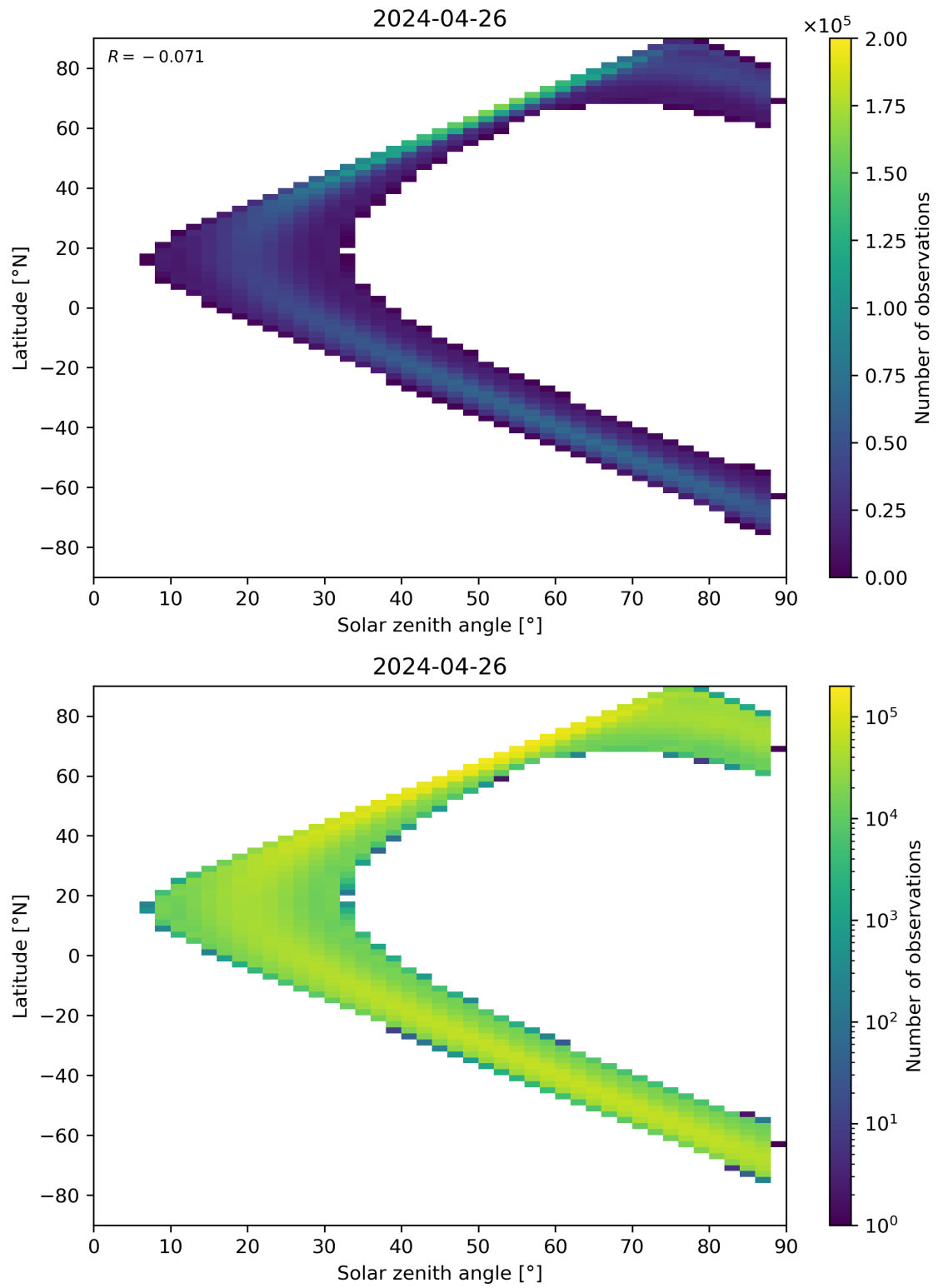
Figure 149: Scatter density plot of “Solar zenith angle” against “Latitude” for 2024-04-26 to 2024-04-27.
