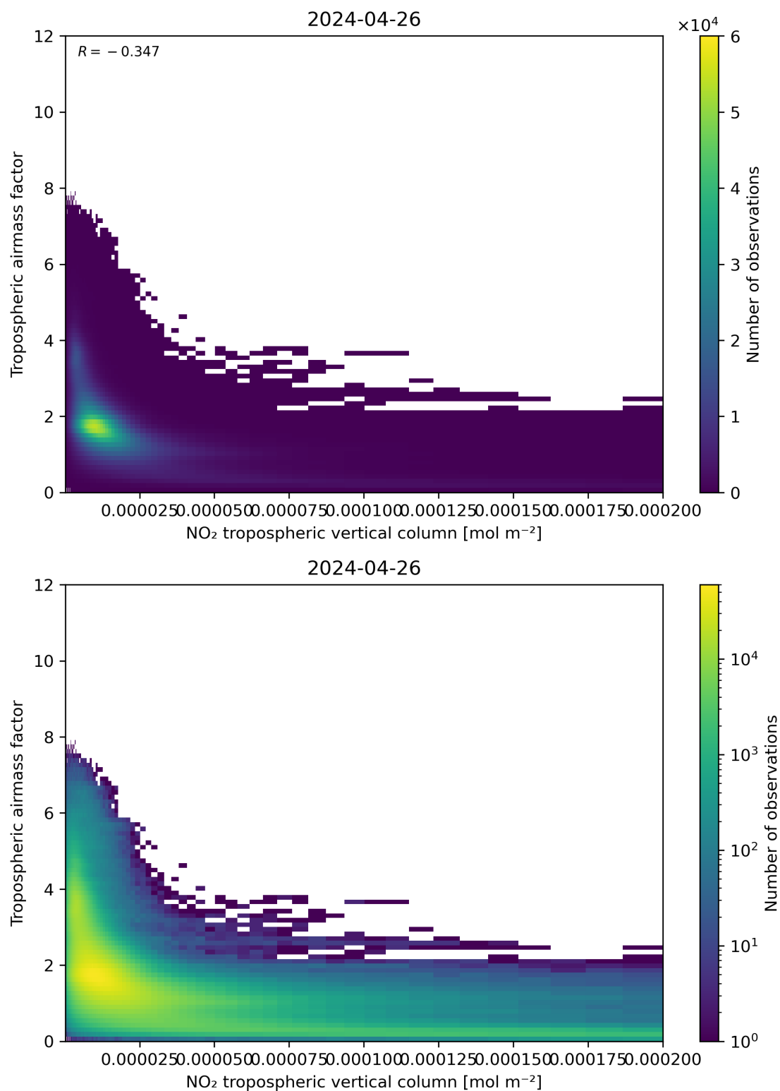
Figure 123: Scatter density plot of “NO 2 tropospheric vertical column” against “Tropospheric air mass factor” for 2024-04-26 to 2024-04-27.
