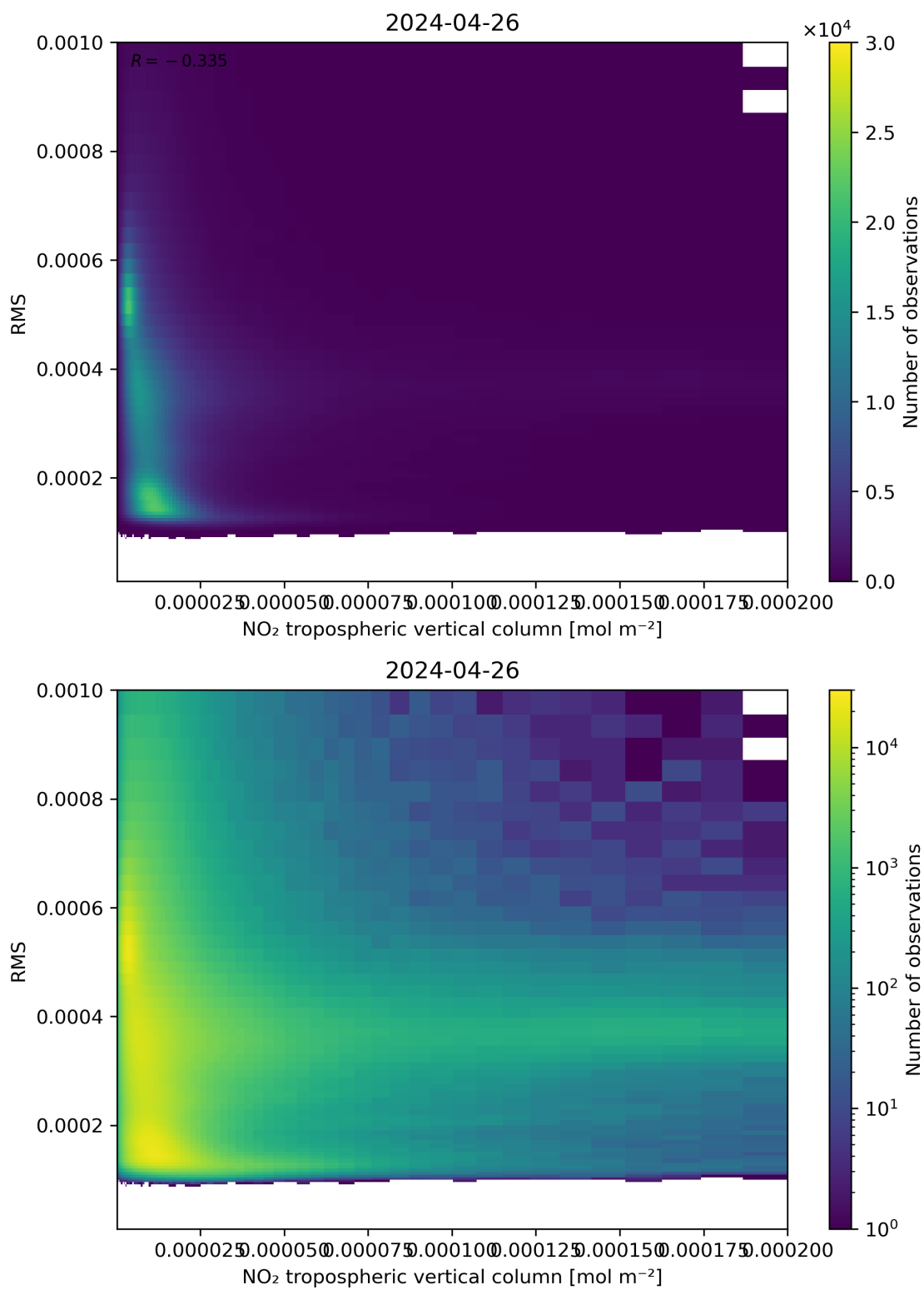
Figure 142: Scatter density plot of “NO 2 tropospheric vertical column” against “RMS” for 2024-04-26 to 2024-04-27.
