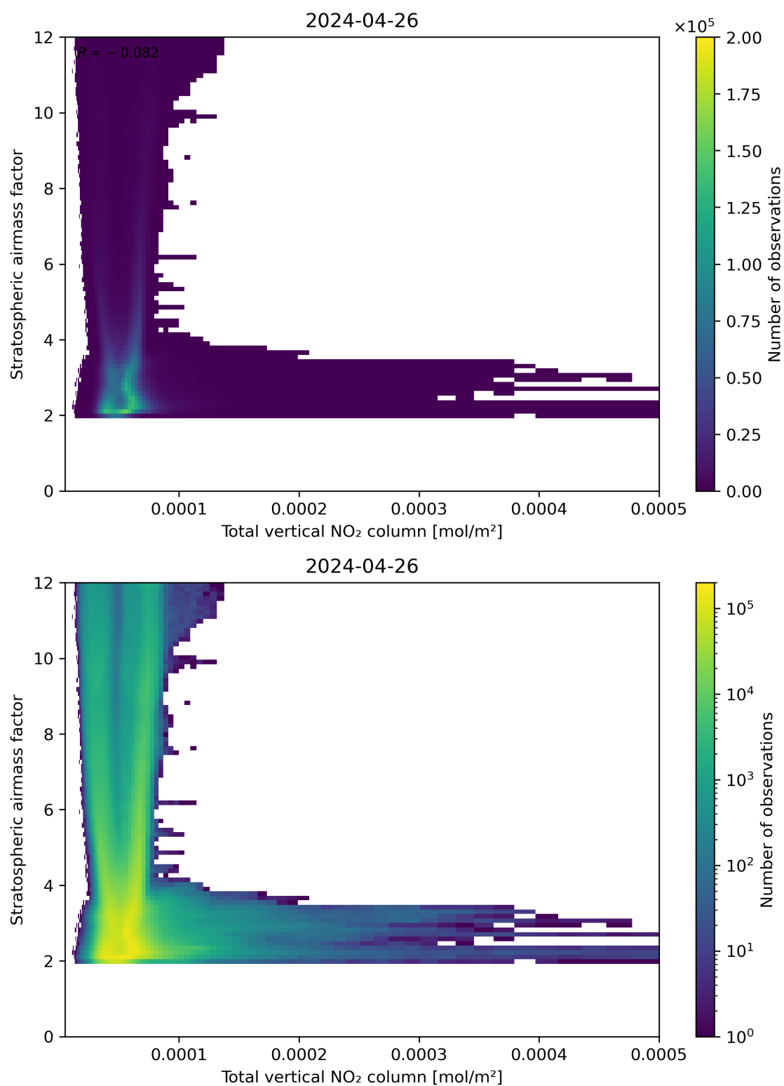
Figure 110: Scatter density plot of “Total vertical NO 2 column” against “Stratospheric airmass factor” for 2024-04-26 to 2024-04-27.
