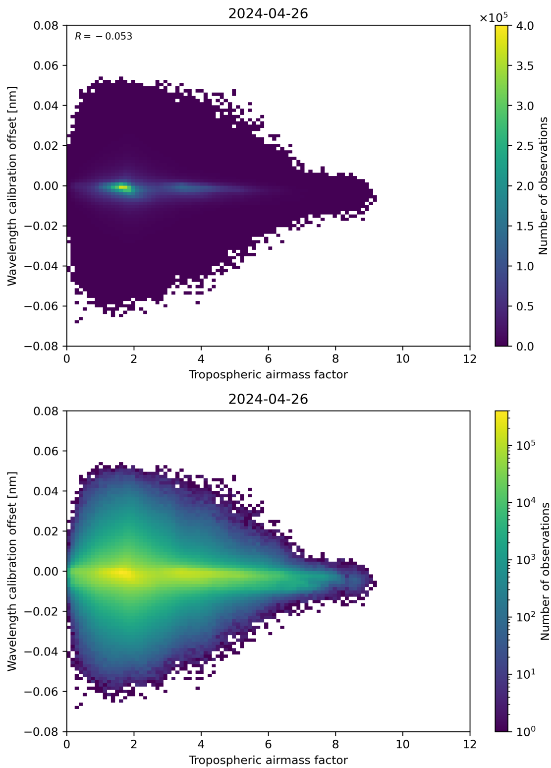
Figure 80: Scatter density plot of “Tropospheric airmass factor” against “Wavelength calibration offset” for 2024-04-26 to 2024-04-27.
