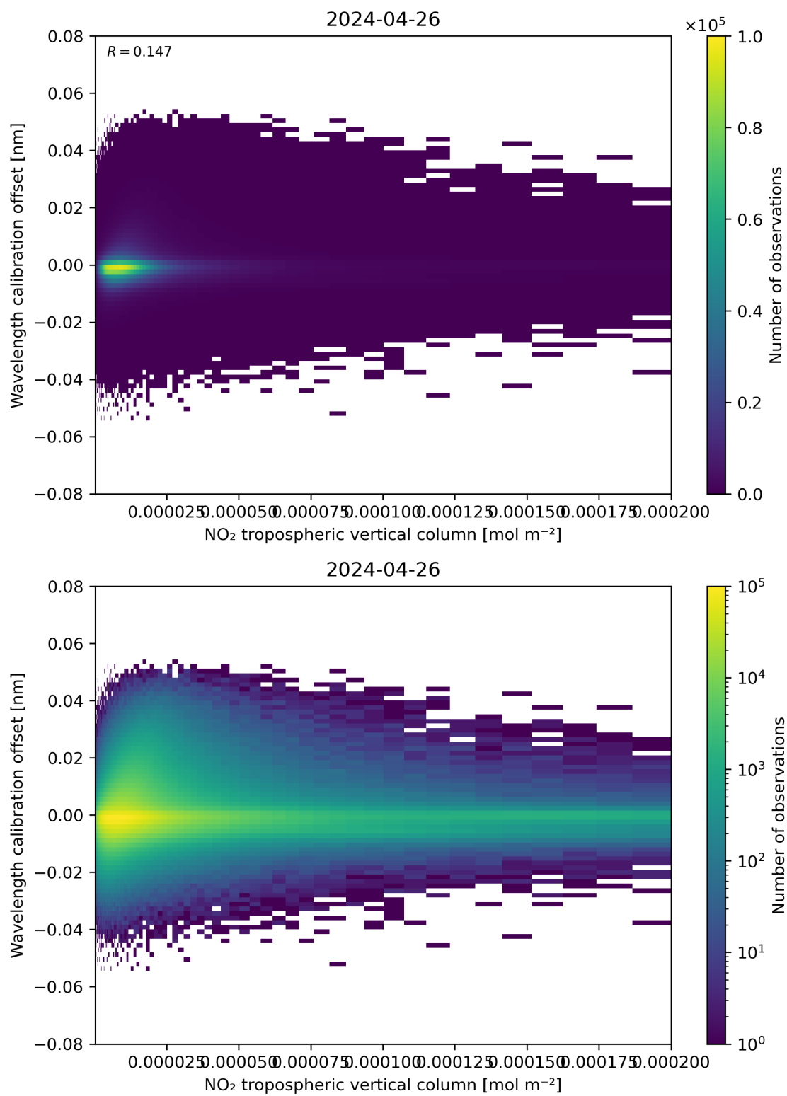
Figure 143: Scatter density plot of “NO 2 tropospheric vertical column” against “Wavelength calibration offset” for 2024-04-26 to 2024-04-27.
