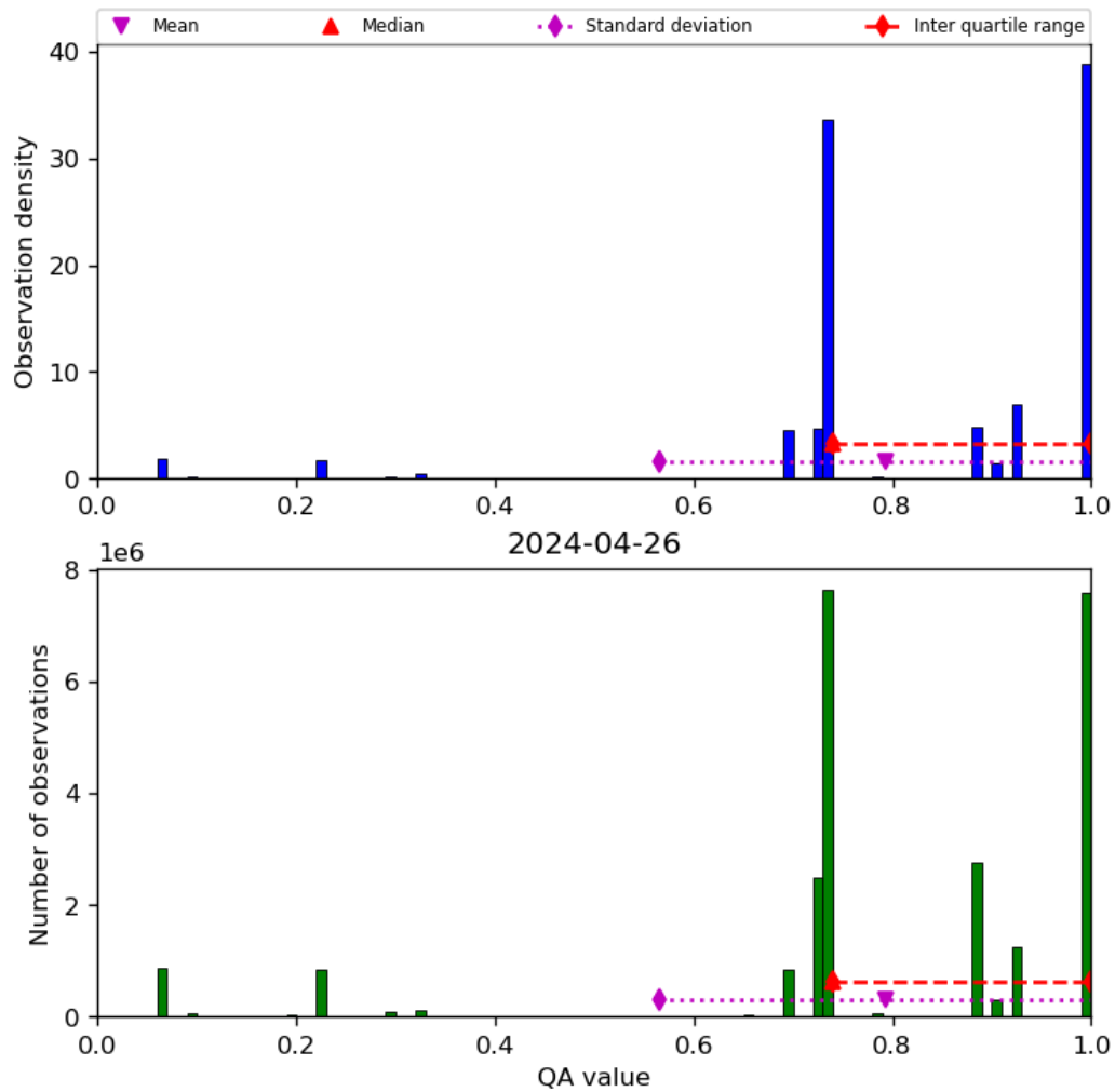
Figure 28: Histogram of “QA value” for 2024-04-26 to 2024-04-27
