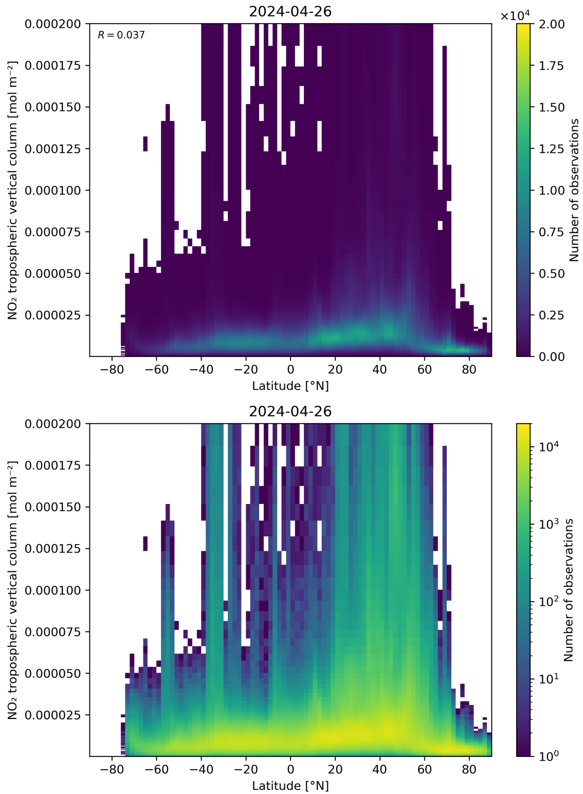
Figure 92: Scatter density plot of “Latitude” against “NO 2 tropospheric vertical column” for 2024-04-26 to 2024-04-27.
