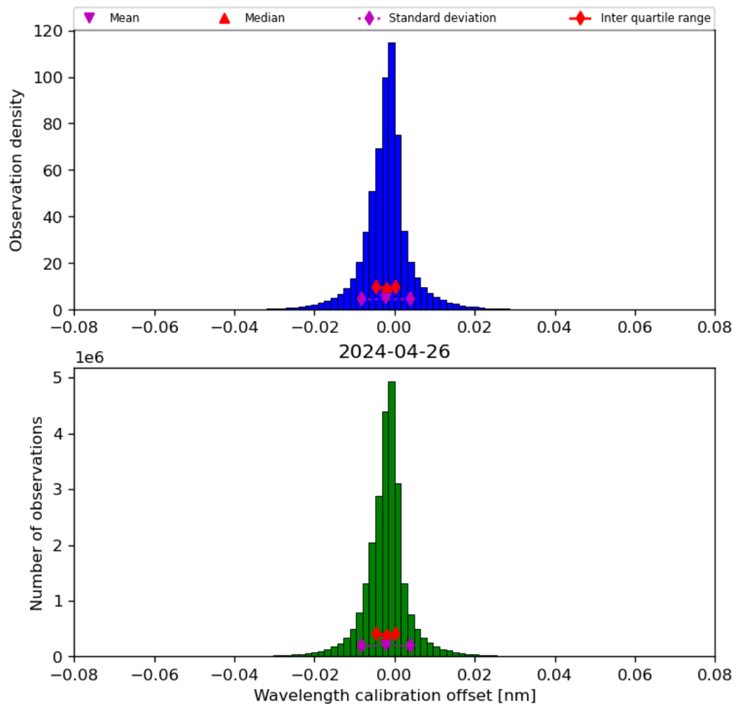
Figure 35: Histogram of “Wavelength calibration offset” for 2024-04-26 to 2024-04-27
