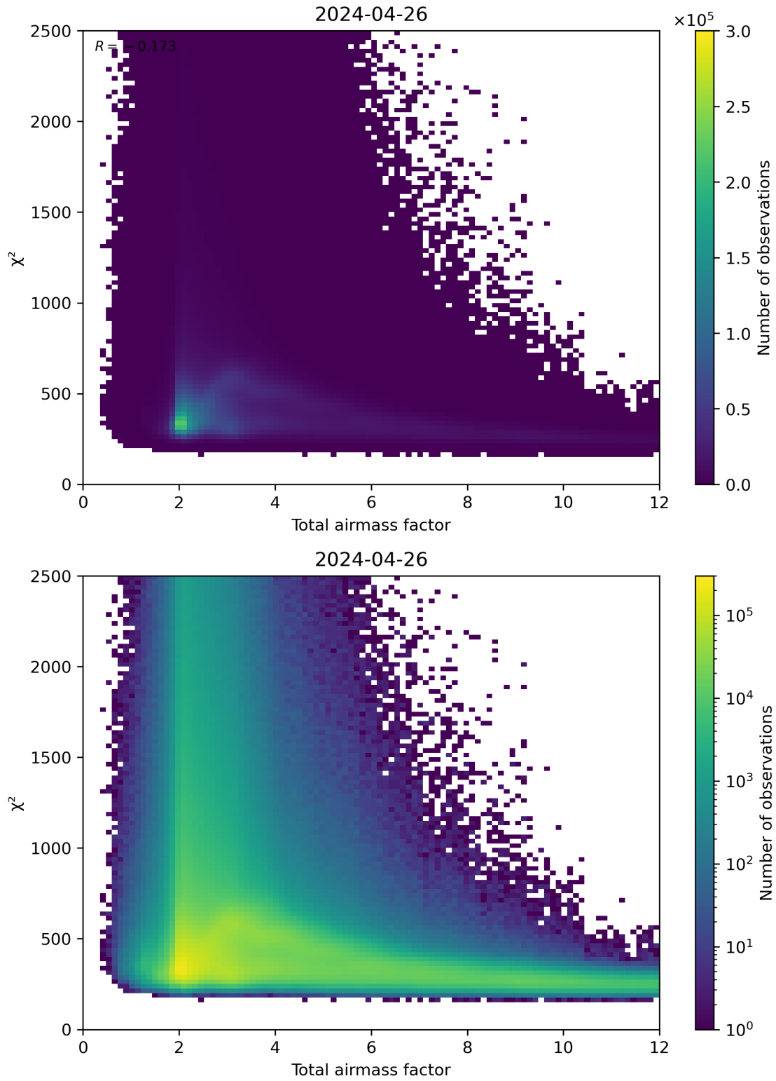
Figure 63: Scatter density plot of “Total airmass factor” against “ \chi^2 ” for 2024-04-26 to 2024-04-27.
