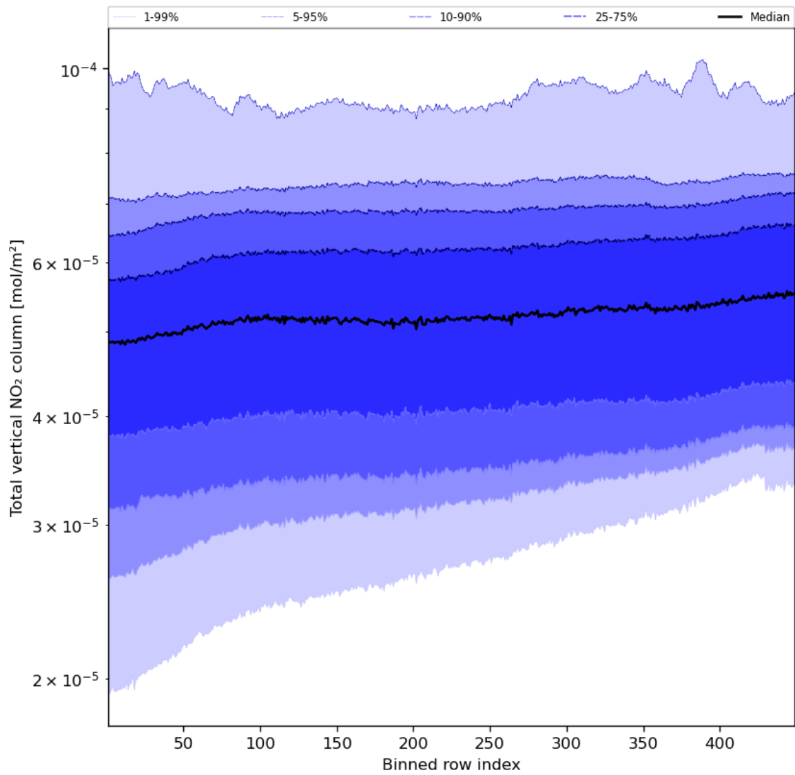
Figure 55: Along track statistics of “Total vertical NO 2 column” for 2024-04-26 to 2024-04-27
