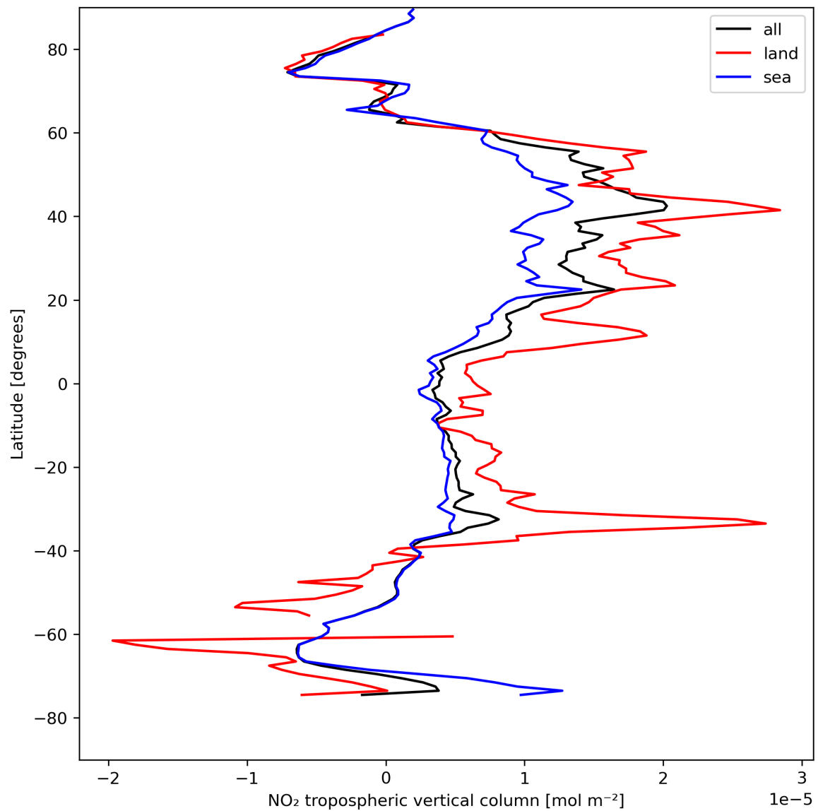
Figure 12: Zonal average of “NO 2 tropospheric vertical column” for 2024-04-26 to 2024-04-27.
