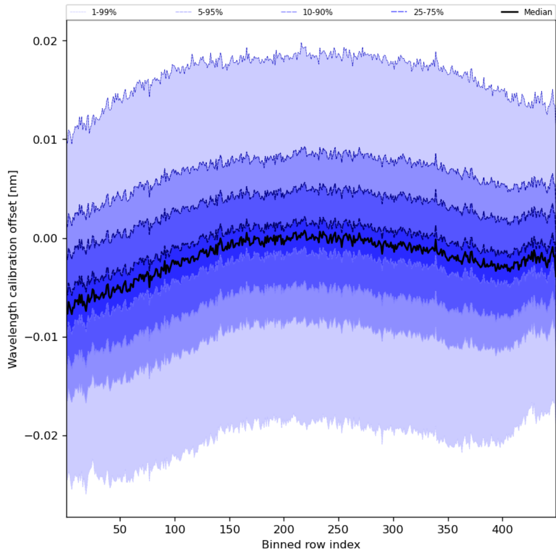
Figure 52: Along track statistics of “Wavelength calibration offset” for 2024-04-26 to 2024-04-27
