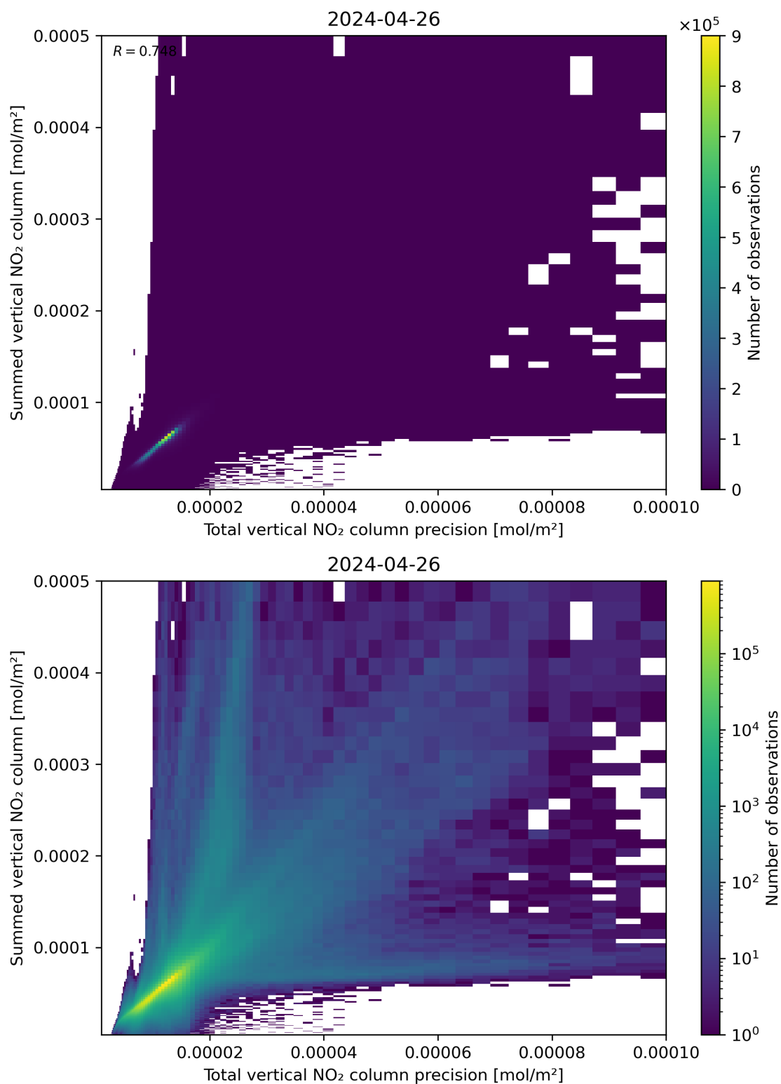
Figure 117: Scatter density plot of “Total vertical NO 2 column precision” against “Summed vertical NO 2 column” for 2024-04-26 to 2024-04-27.
