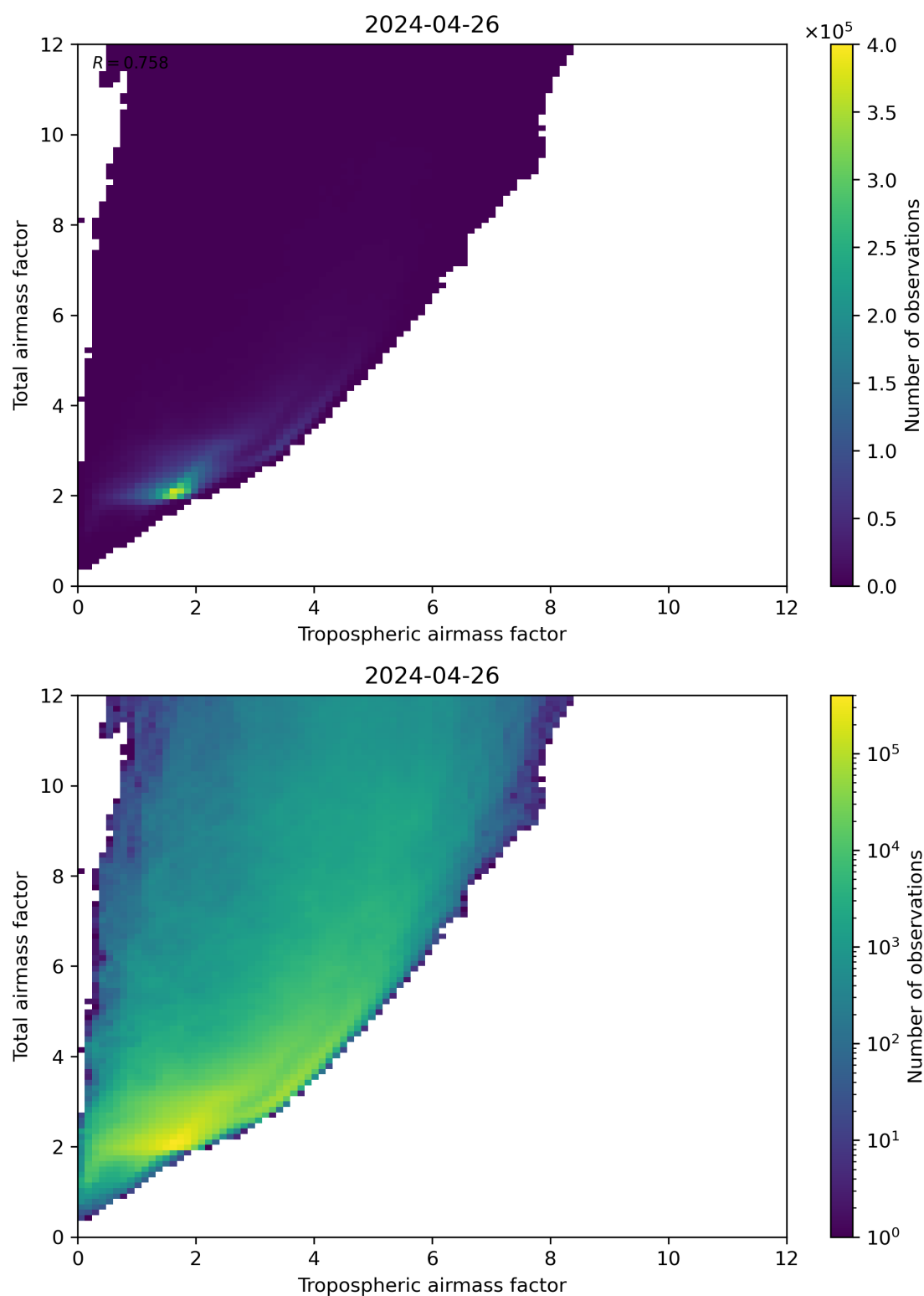
Figure 72: Scatter density plot of “Tropospheric airmass factor” against “Total airmass factor” for 2024-04-26 to 2024-04-27.
