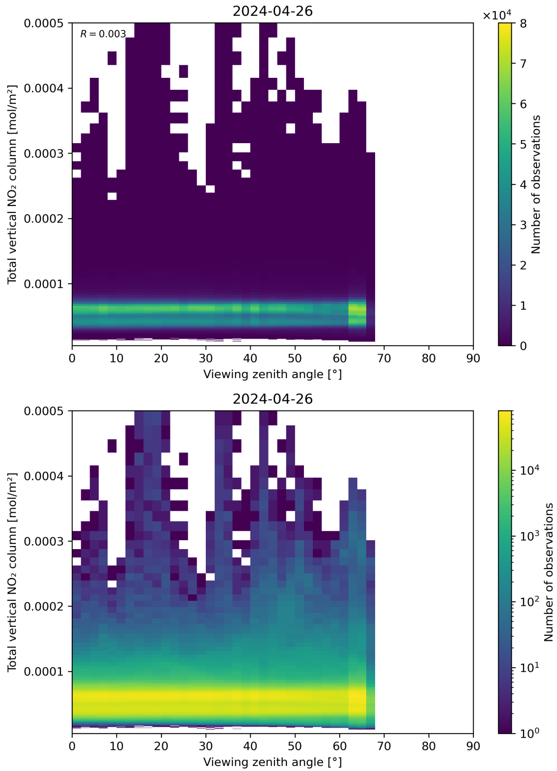
Figure 167: Scatter density plot of “Viewing zenith angle” against “Total vertical NO 2 column” for 2024-04-26 to 2024-04-27.
