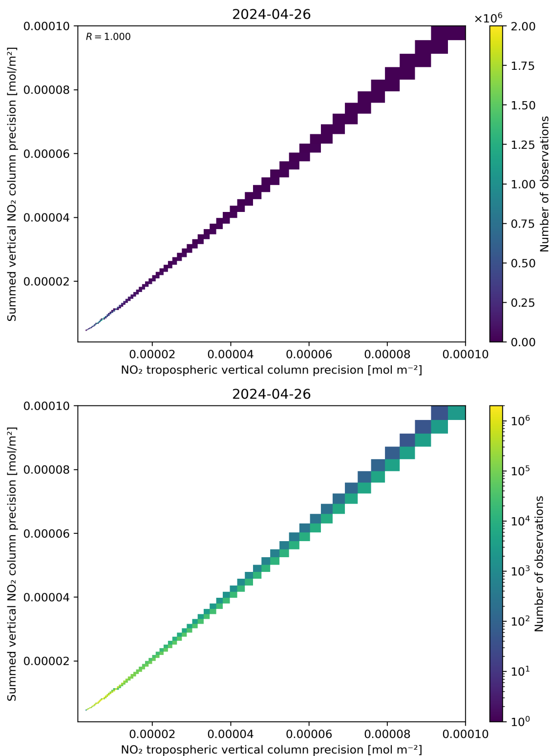
Figure 137: Scatter density plot of “NO 2 tropospheric vertical column precision” against “Summed vertical NO 2 column precision” for 2024-04-26 to 2024-04-27.
