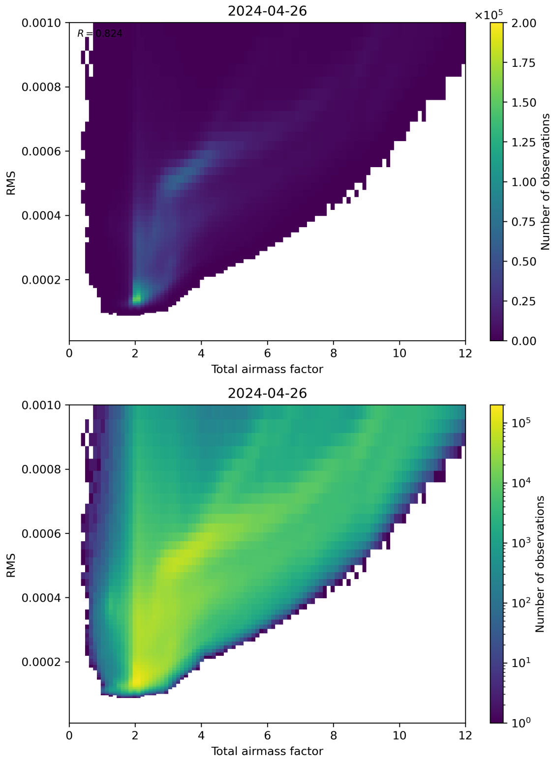
Figure 69: Scatter density plot of “Total airmass factor” against “RMS” for 2024-04-26 to 2024-04-27.
