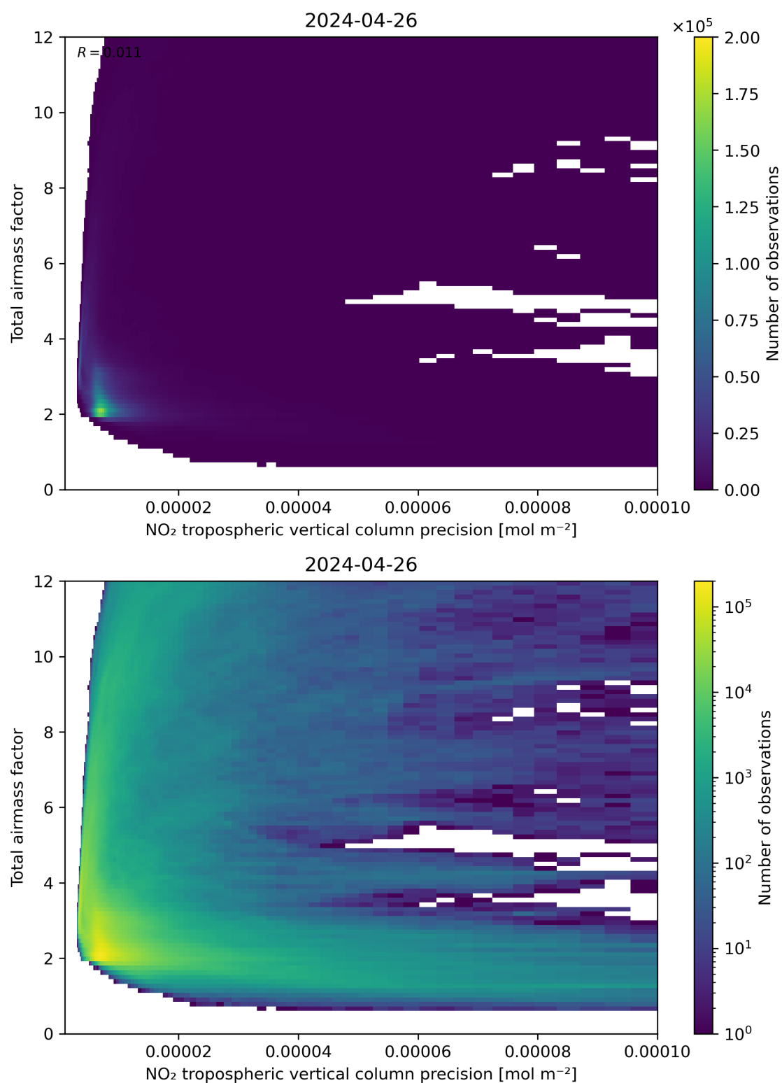
Figure 132: Scatter density plot of “NO 2 tropospheric vertical column precision” against “Total air mass factor” for 2024-04-26 to 2024-04-27.
