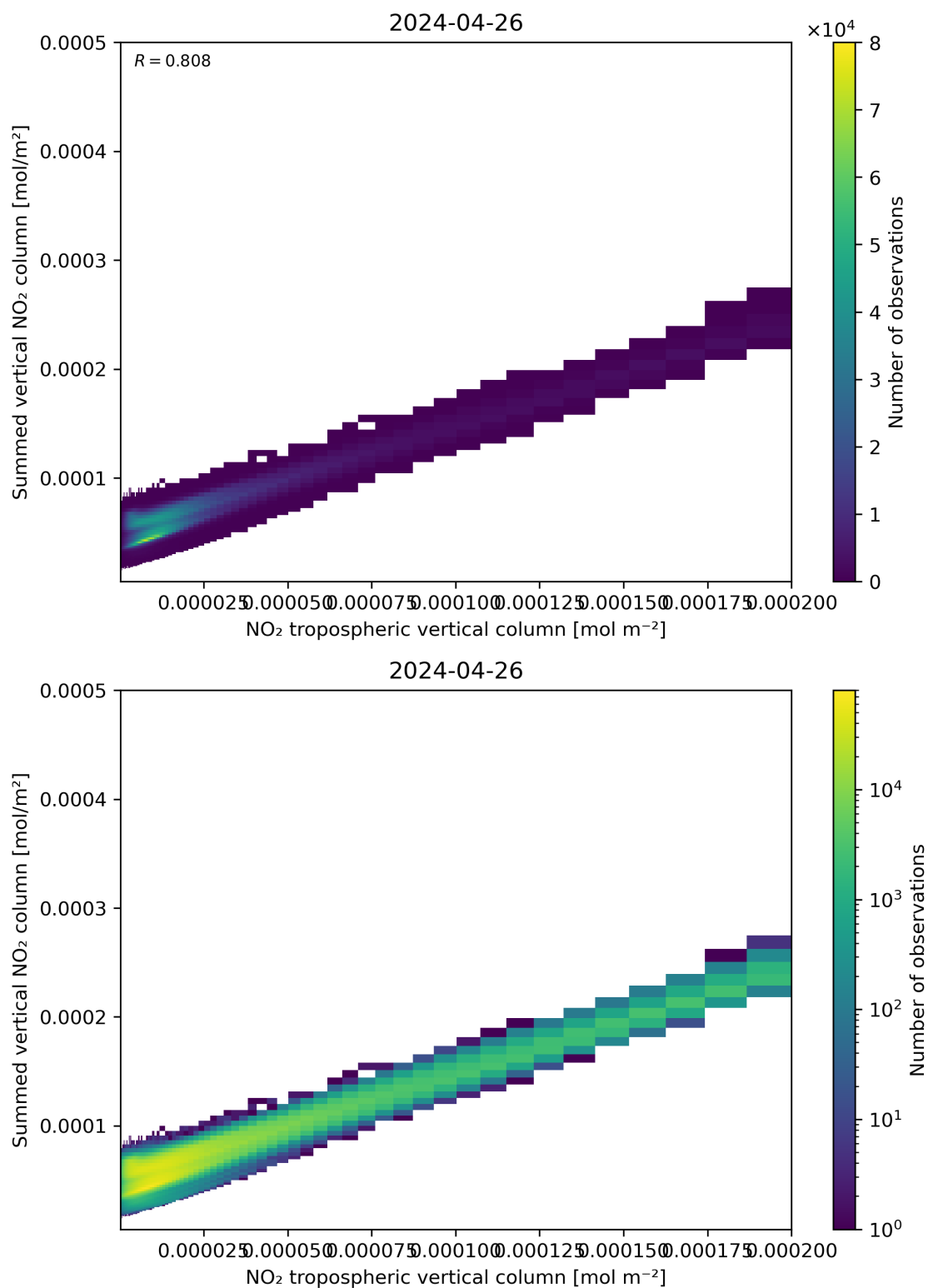
Figure 126: Scatter density plot of “NO 2 tropospheric vertical column” against “Summed vertical NO 2 column” for 2024-04-26 to 2024-04-27.
