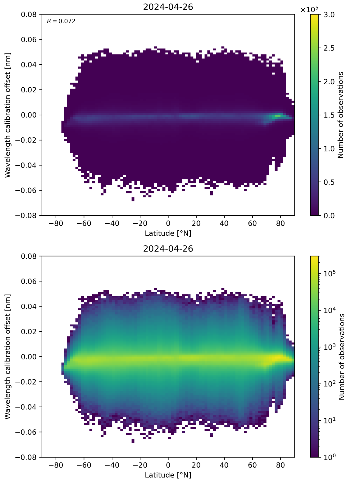
Figure 95: Scatter density plot of “Latitude” against “Wavelength calibration offset” for 2024-04-26 to 2024-04-27.
