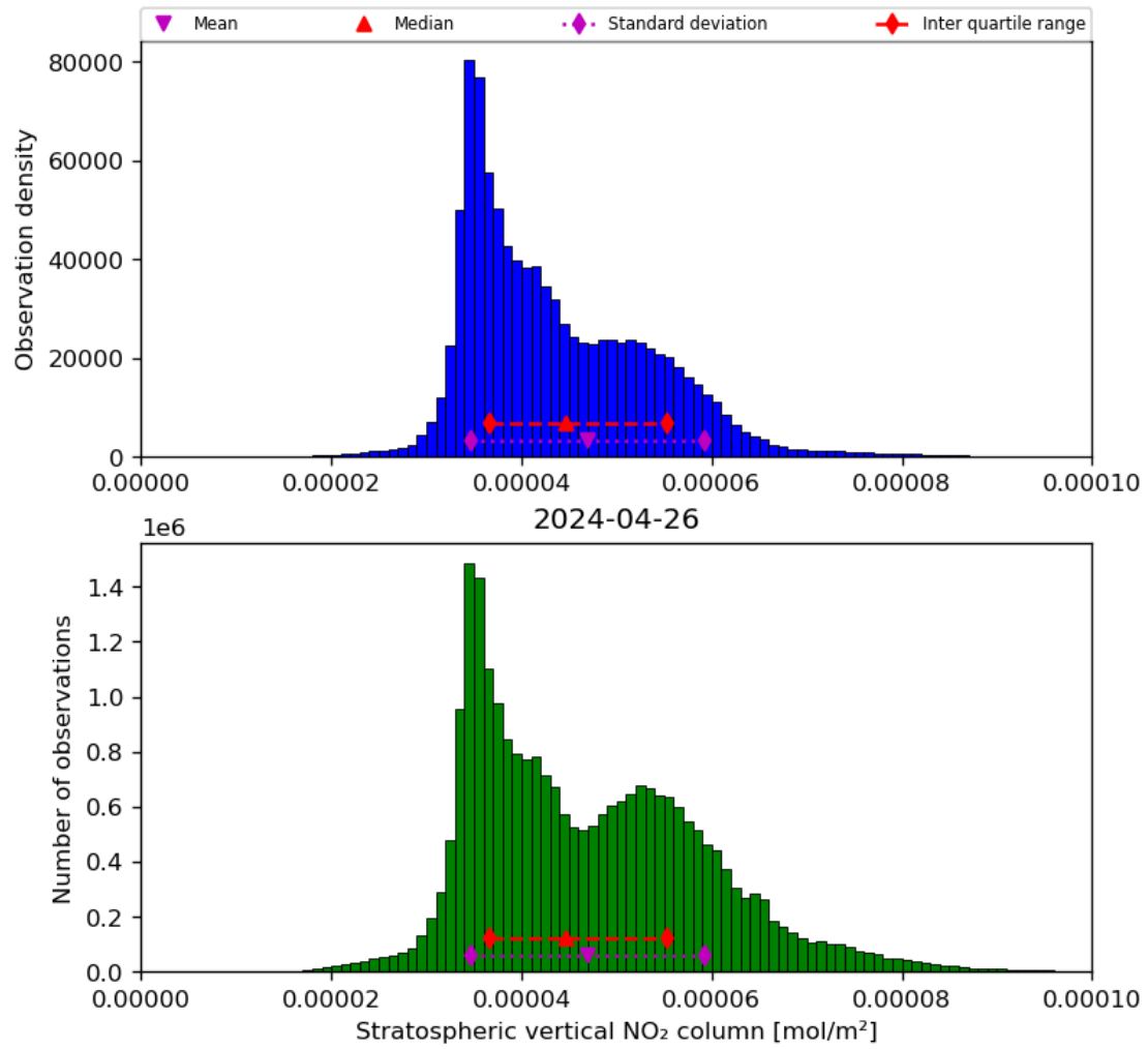
Figure 36: Histogram of “Stratospheric vertical NO 2 column” for 2024-04-26 to 2024-04-27
