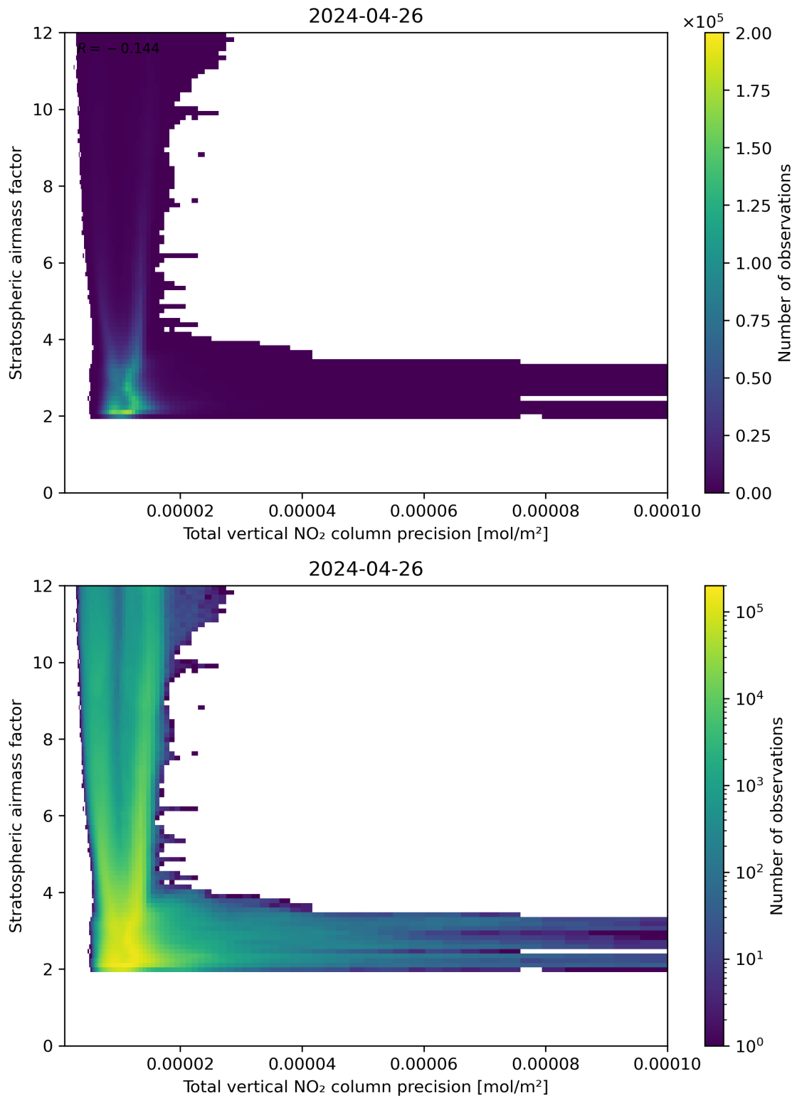
Figure 115: Scatter density plot of “Total vertical NO 2 column precision” against “Stratospheric air mass factor” for 2024-04-26 to 2024-04-27.
