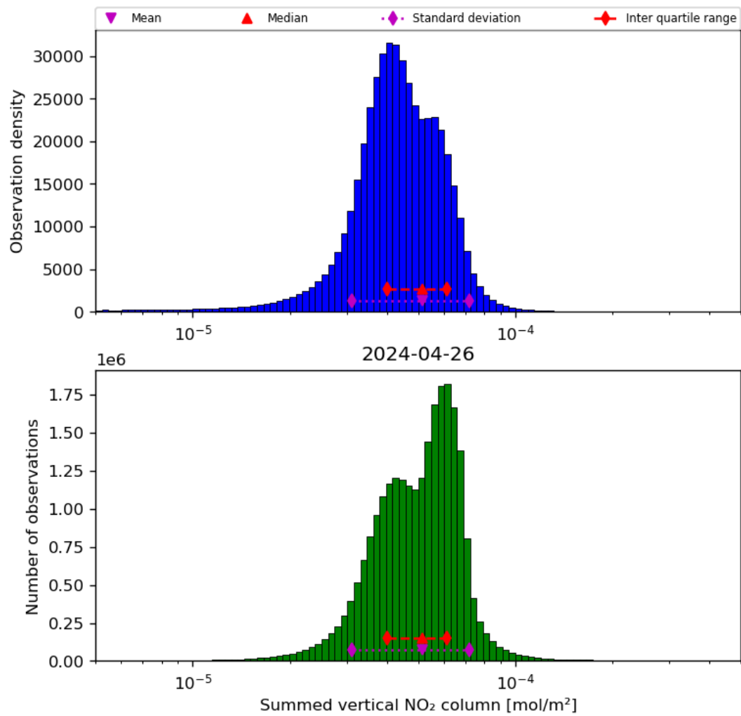
Figure 40: Histogram of “Summed vertical NO 2 column” for 2024-04-26 to 2024-04-27
