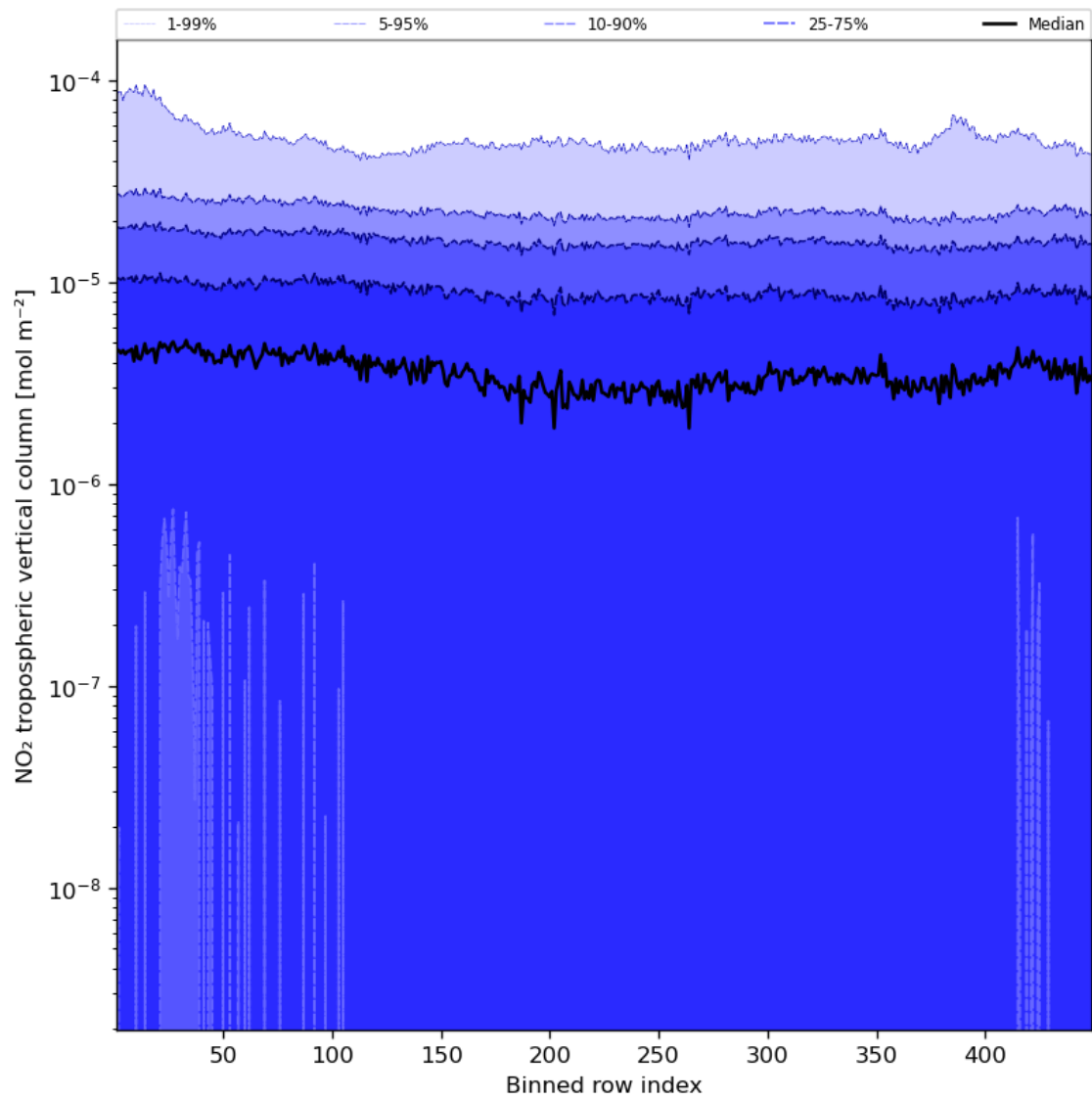
Figure 46: Along track statistics of “NO 2 tropospheric vertical column” for 2024-04-26 to 2024-04-27
