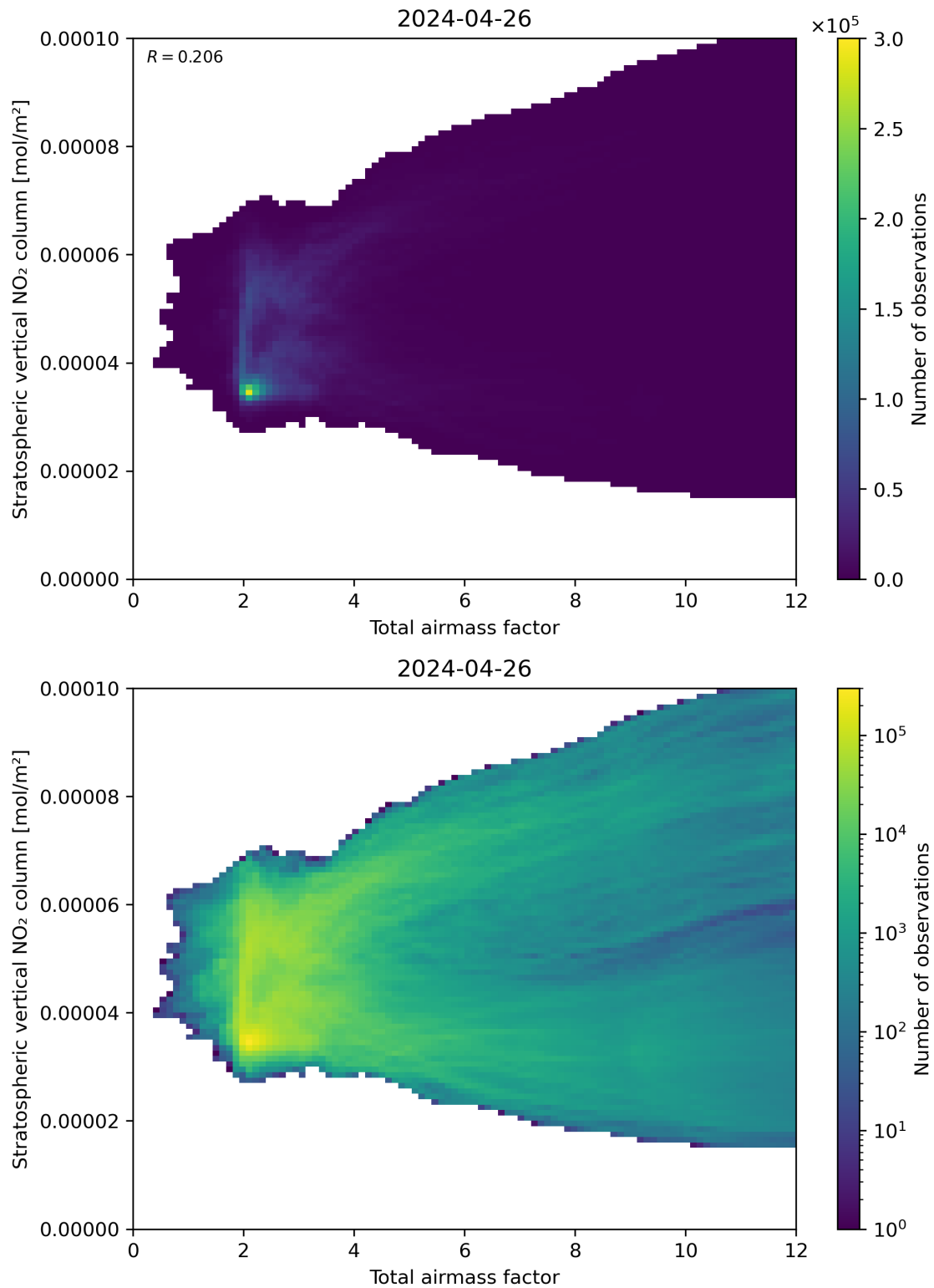
Figure 64: Scatter density plot of “Total airmass factor” against “Stratospheric vertical NO 2 column” for 2024-04-26 to 2024-04-27.
