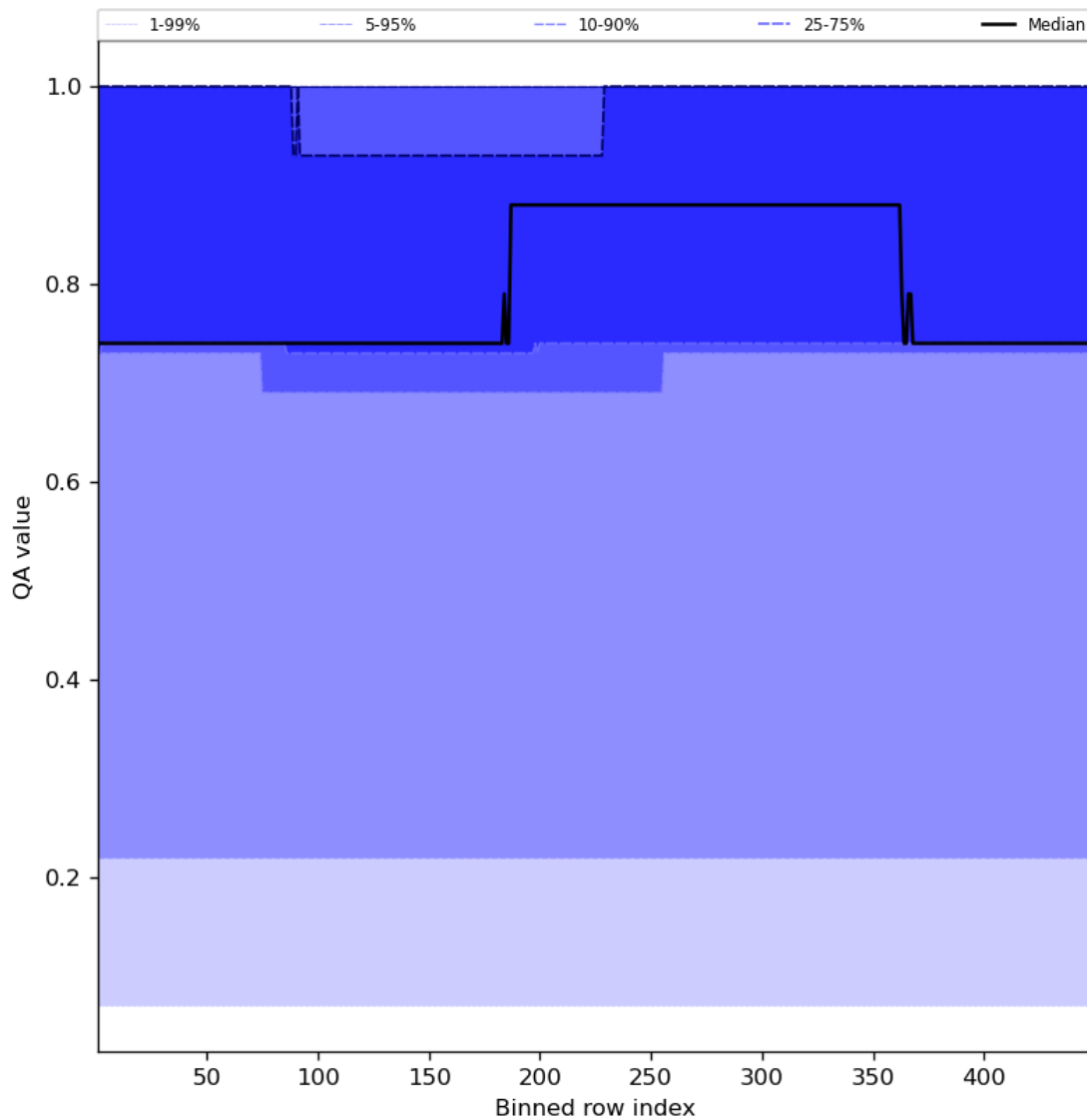
Figure 45: Along track statistics of “QA value” for 2024-04-26 to 2024-04-27
