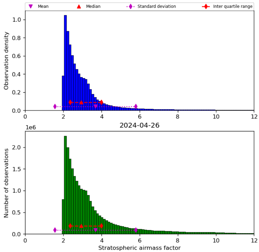
Figure 44: Histogram of “Stratospheric airmass factor” for 2024-04-26 to 2024-04-27
