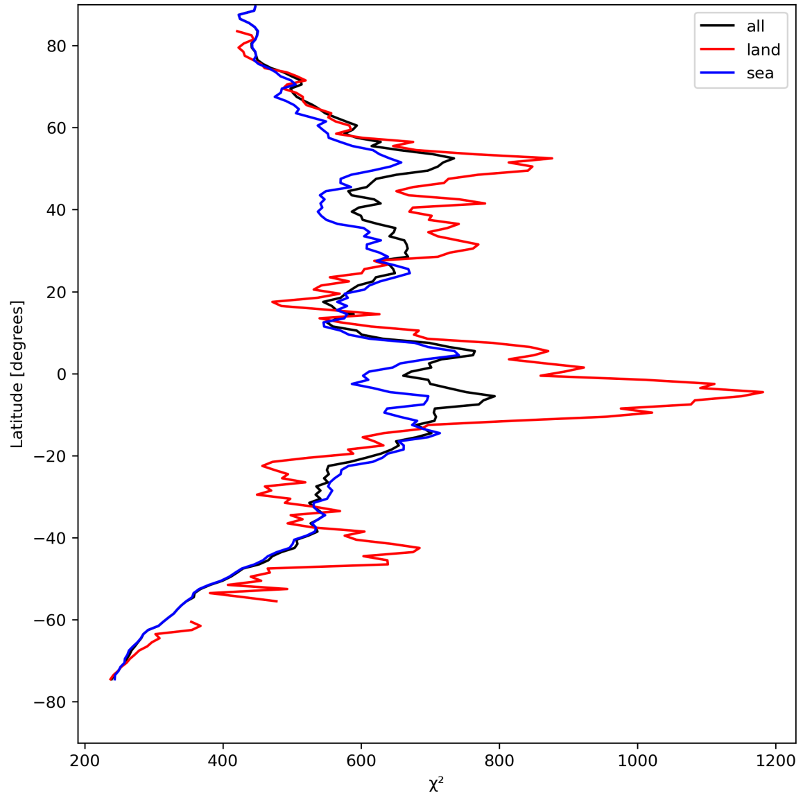
Figure 25: Zonal average of “ \chi^2 ” for 2024-04-26 to 2024-04-27.
