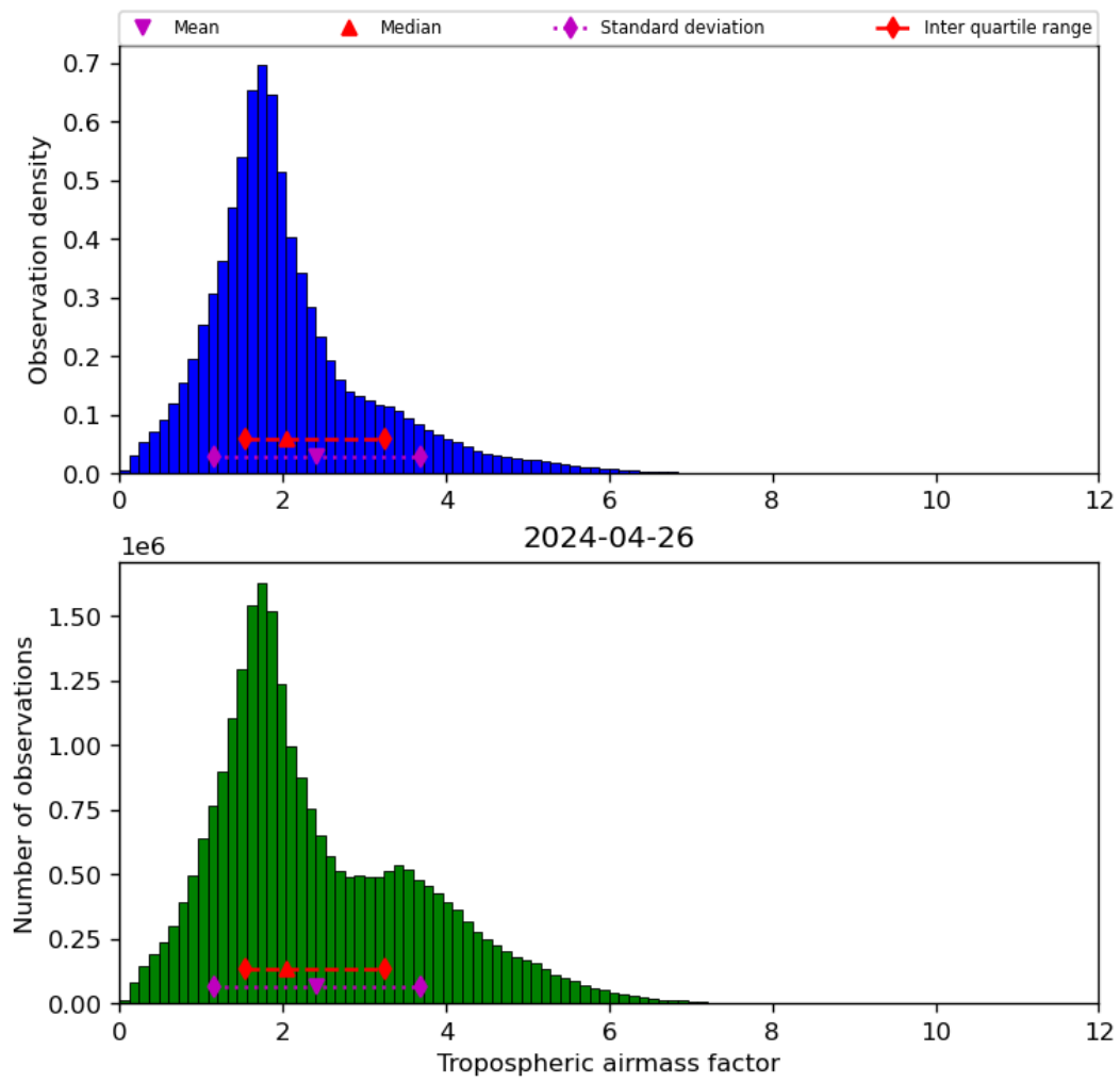
Figure 31: Histogram of “Tropospheric airmass factor” for 2024-04-26 to 2024-04-27
