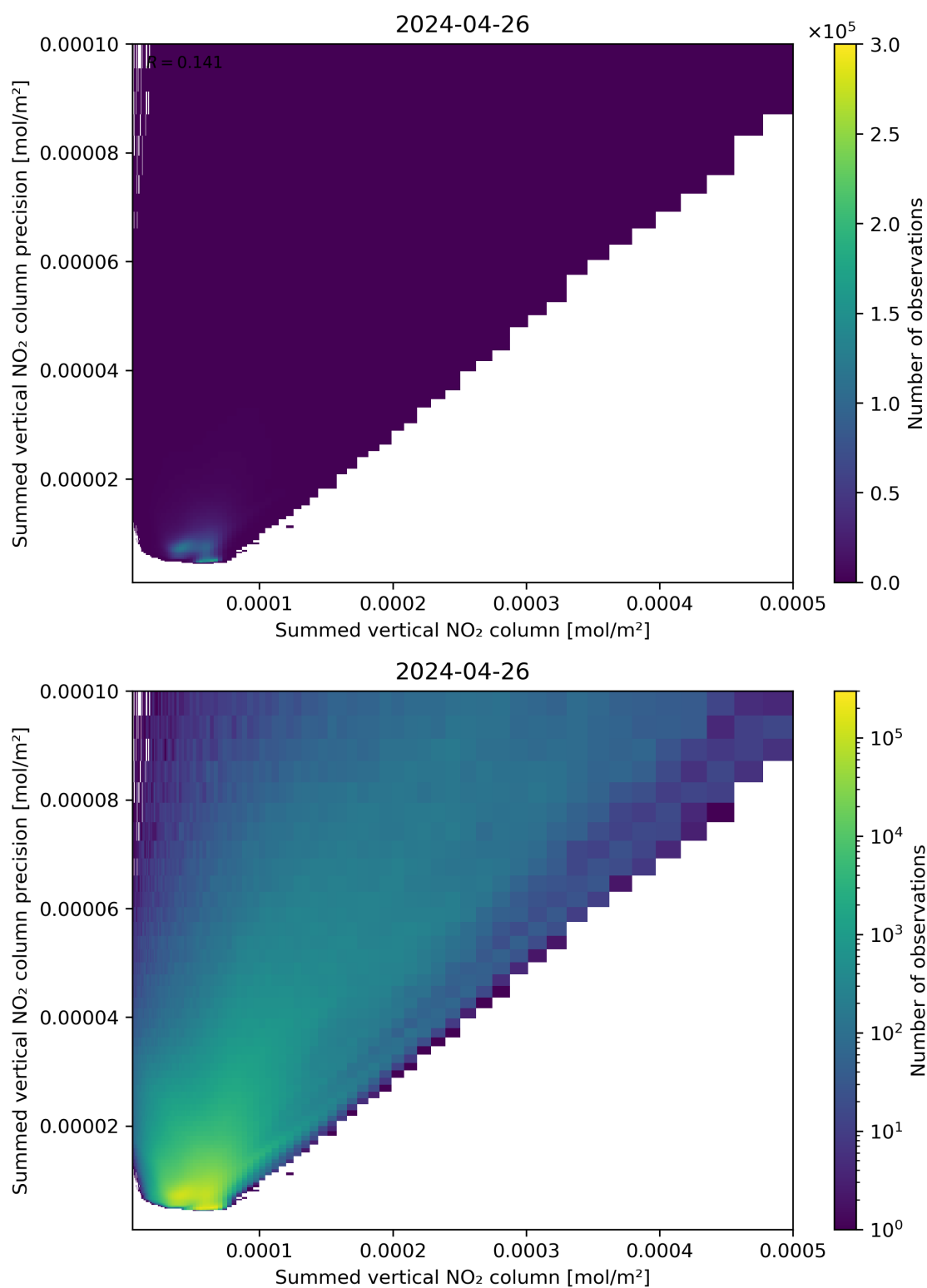
Figure 105: Scatter density plot of “Summed vertical NO 2 column” against “Summed vertical NO 2 column precision” for 2024-04-26 to 2024-04-27.
