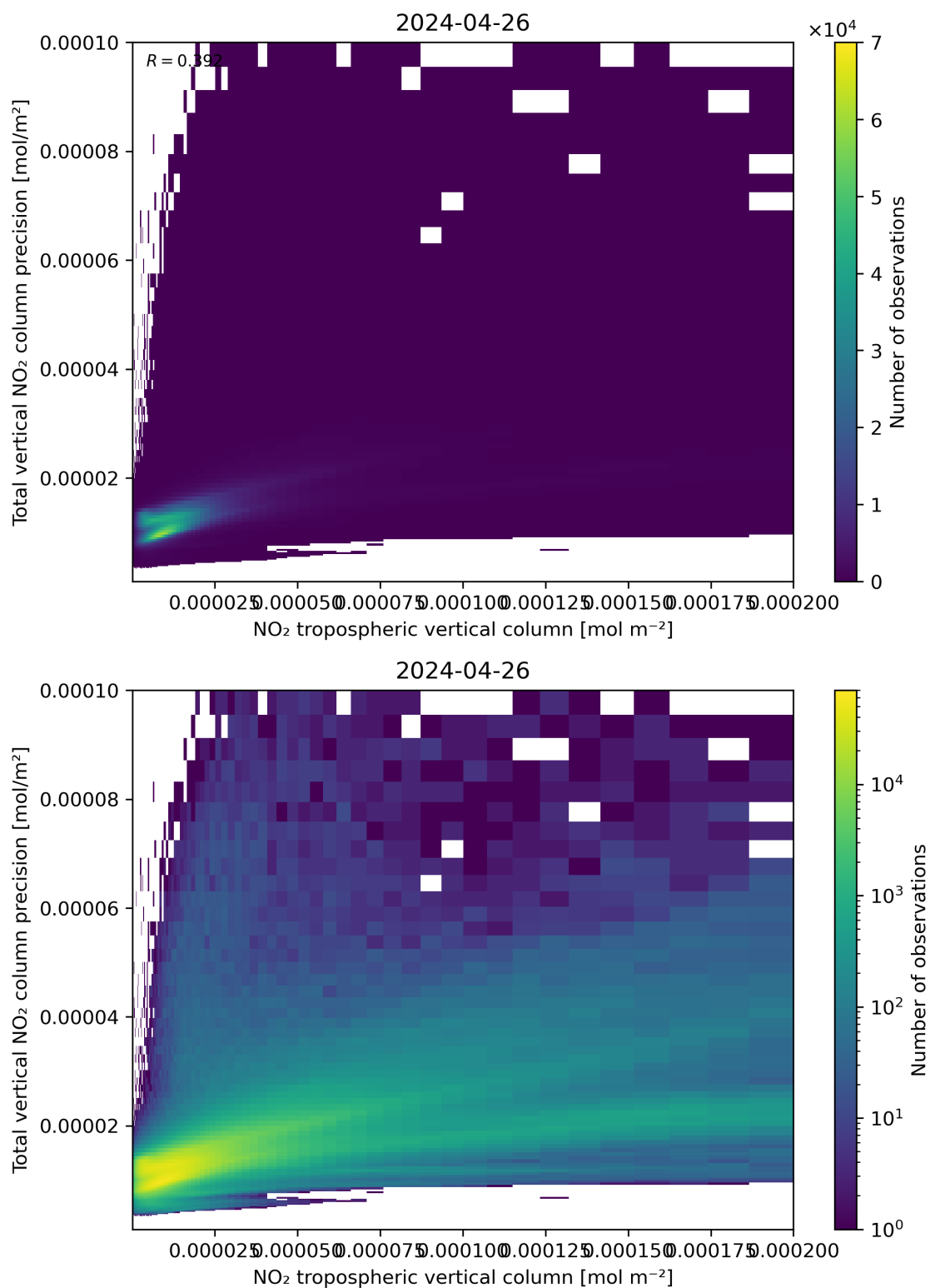
Figure 129: Scatter density plot of “NO 2 tropospheric vertical column” against “Total vertical NO 2 column precision” for 2024-04-26 to 2024-04-27.
