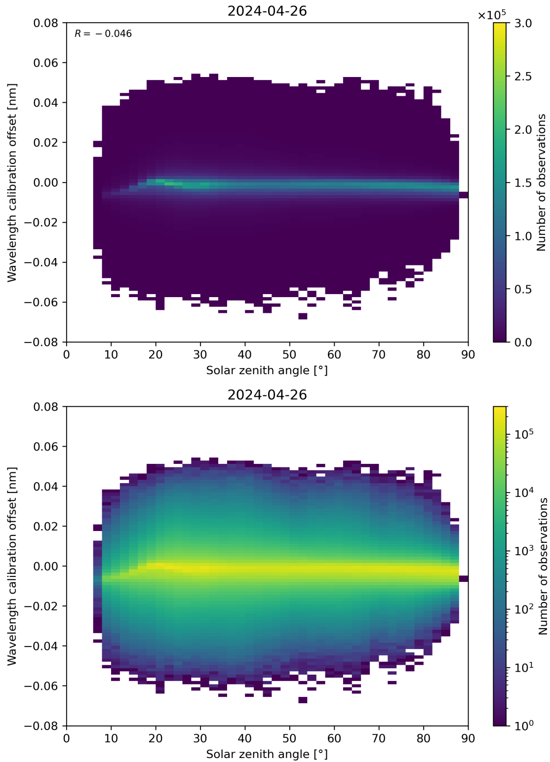
Figure 158: Scatter density plot of “Solar zenith angle” against “Wavelength calibration offset” for 2024-04-26 to 2024-04-27.
