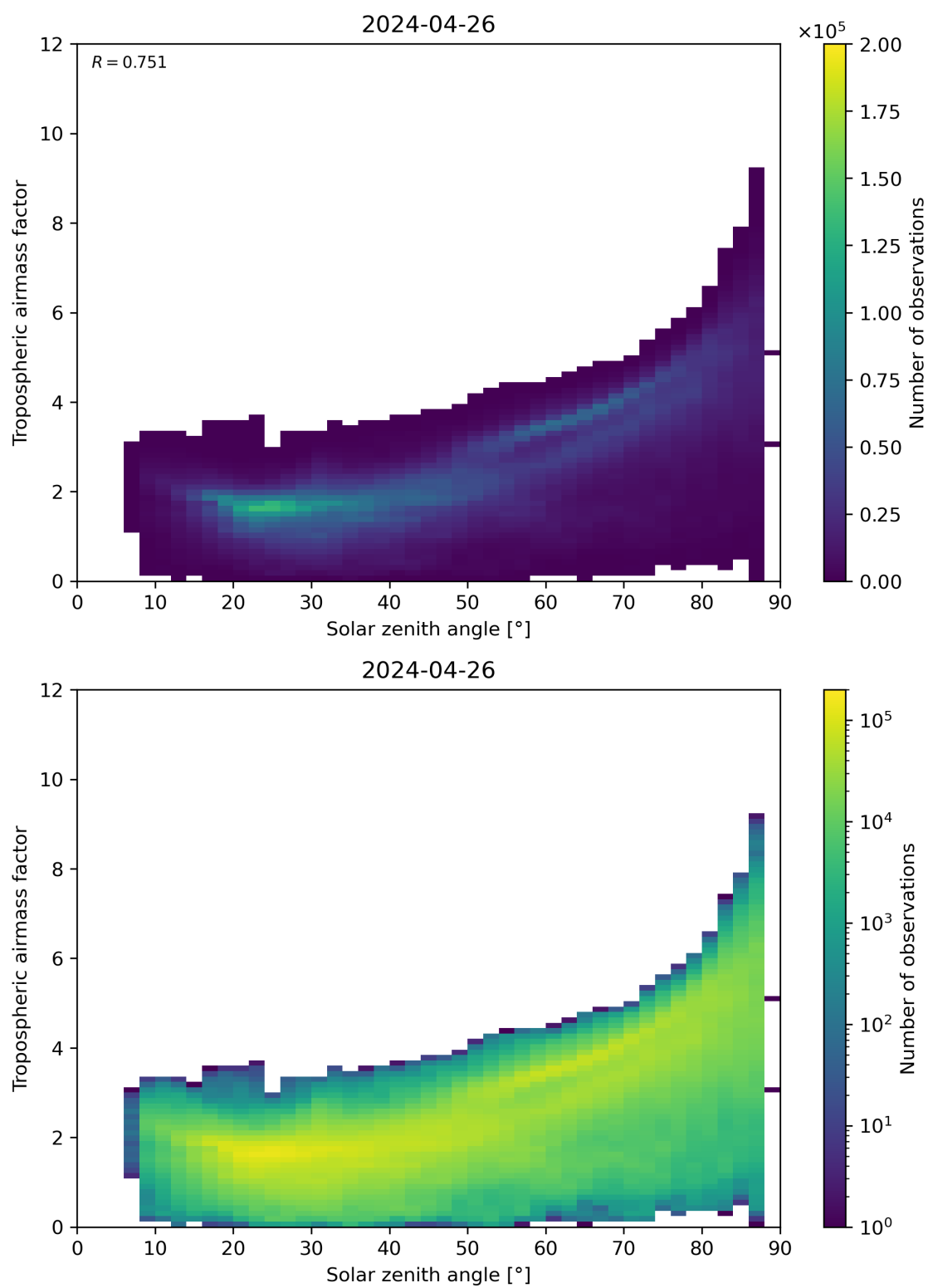
Figure 147: Scatter density plot of “Solar zenith angle” against “Tropospheric airmass factor” for 2024-04-26 to 2024-04-27.
