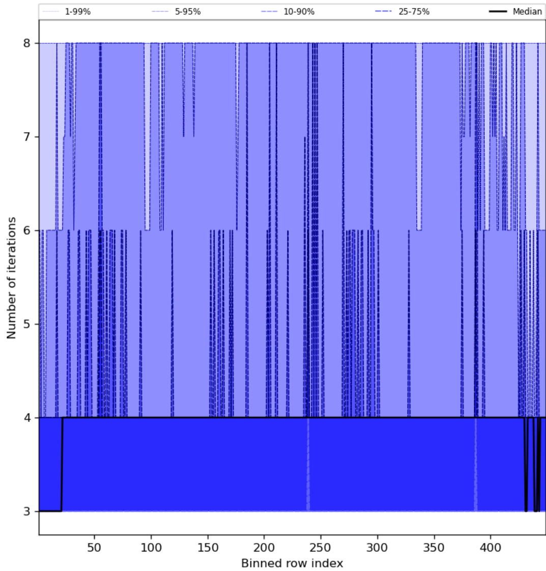
Figure 51: Along track statistics of “Number of iterations” for 2024-04-26 to 2024-04-27
