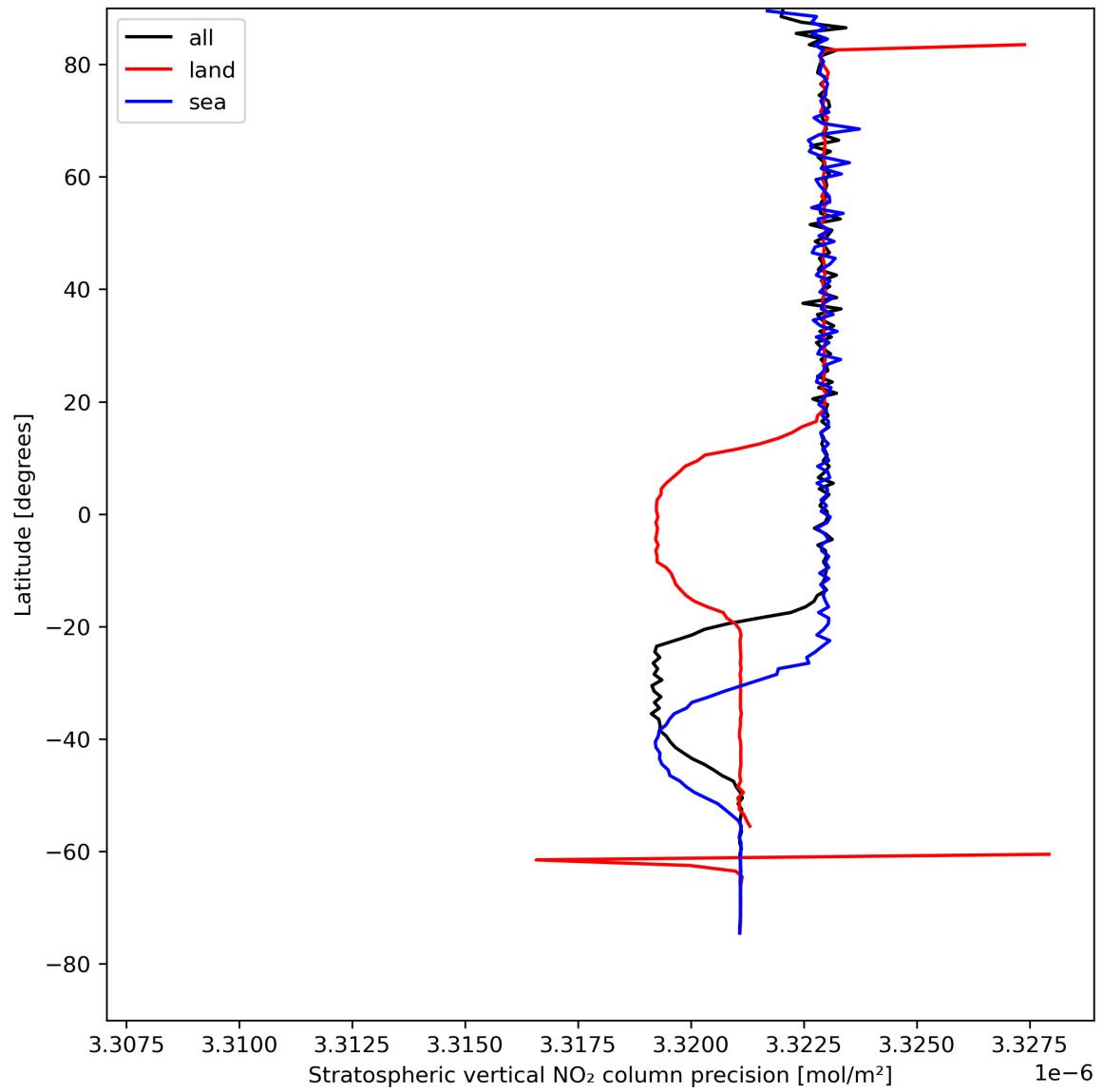
Figure 20: Zonal average of “Stratospheric vertical NO 2 column precision” for 2024-04-26 to 2024-04-27.
