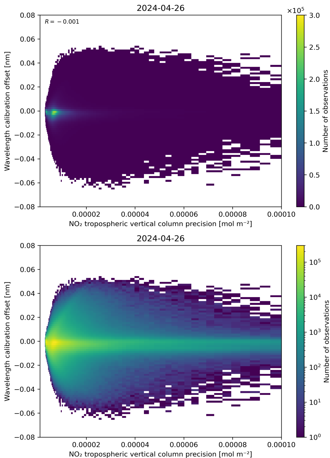
Figure 141: Scatter density plot of “NO 2 tropospheric vertical column precision” against “Wavelength calibration offset” for 2024-04-26 to 2024-04-27.
