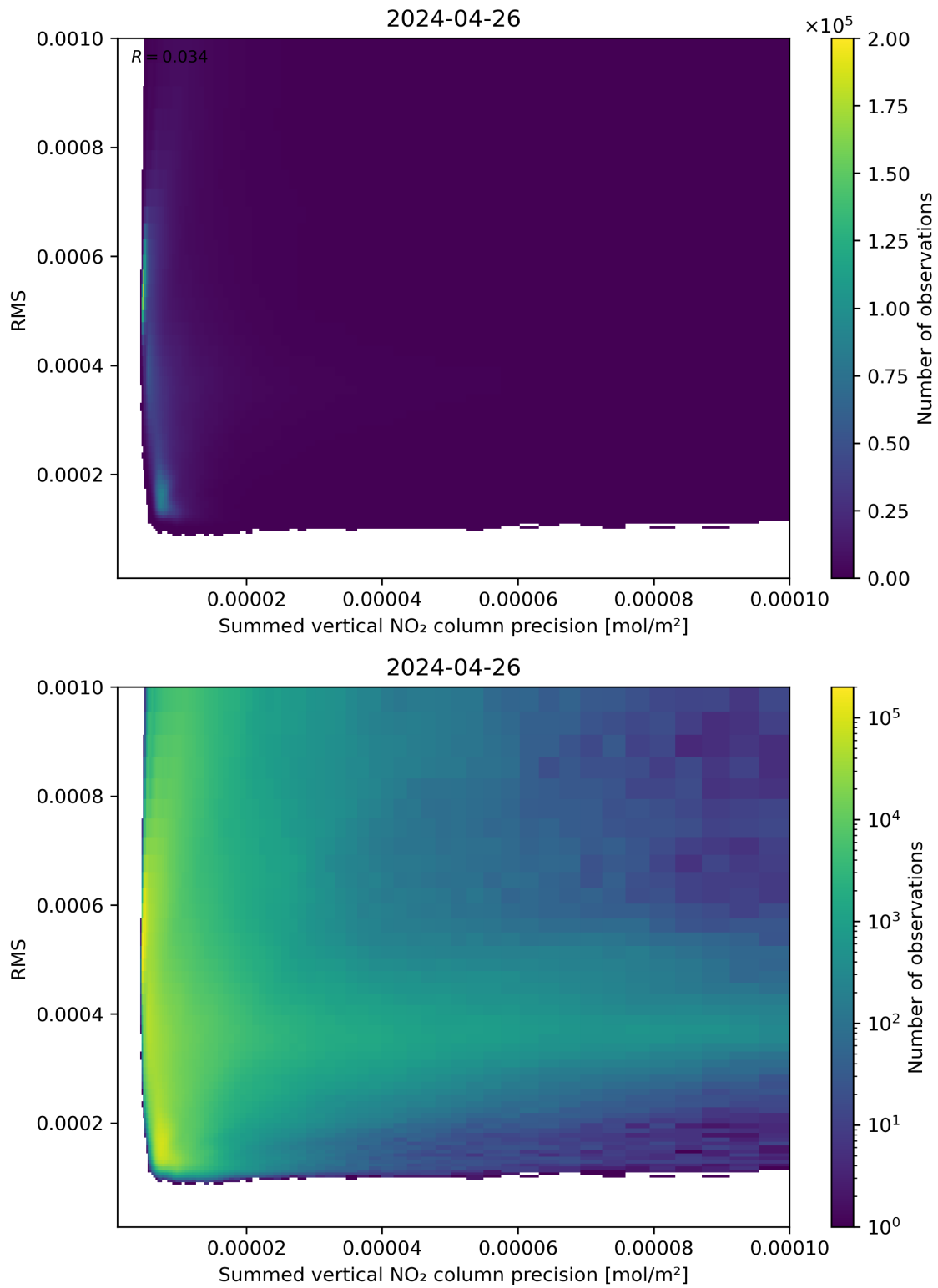
Figure 108: Scatter density plot of “Summed vertical NO 2 column precision” against “RMS” for 2024-04-26 to 2024-04-27.
