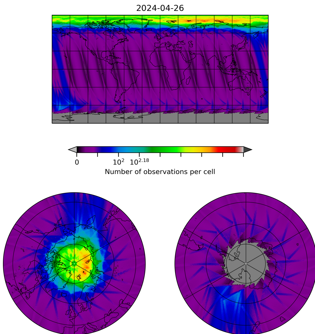
Figure 10: Map of the number of observations for 2024-04-26 to 2024-04-27
