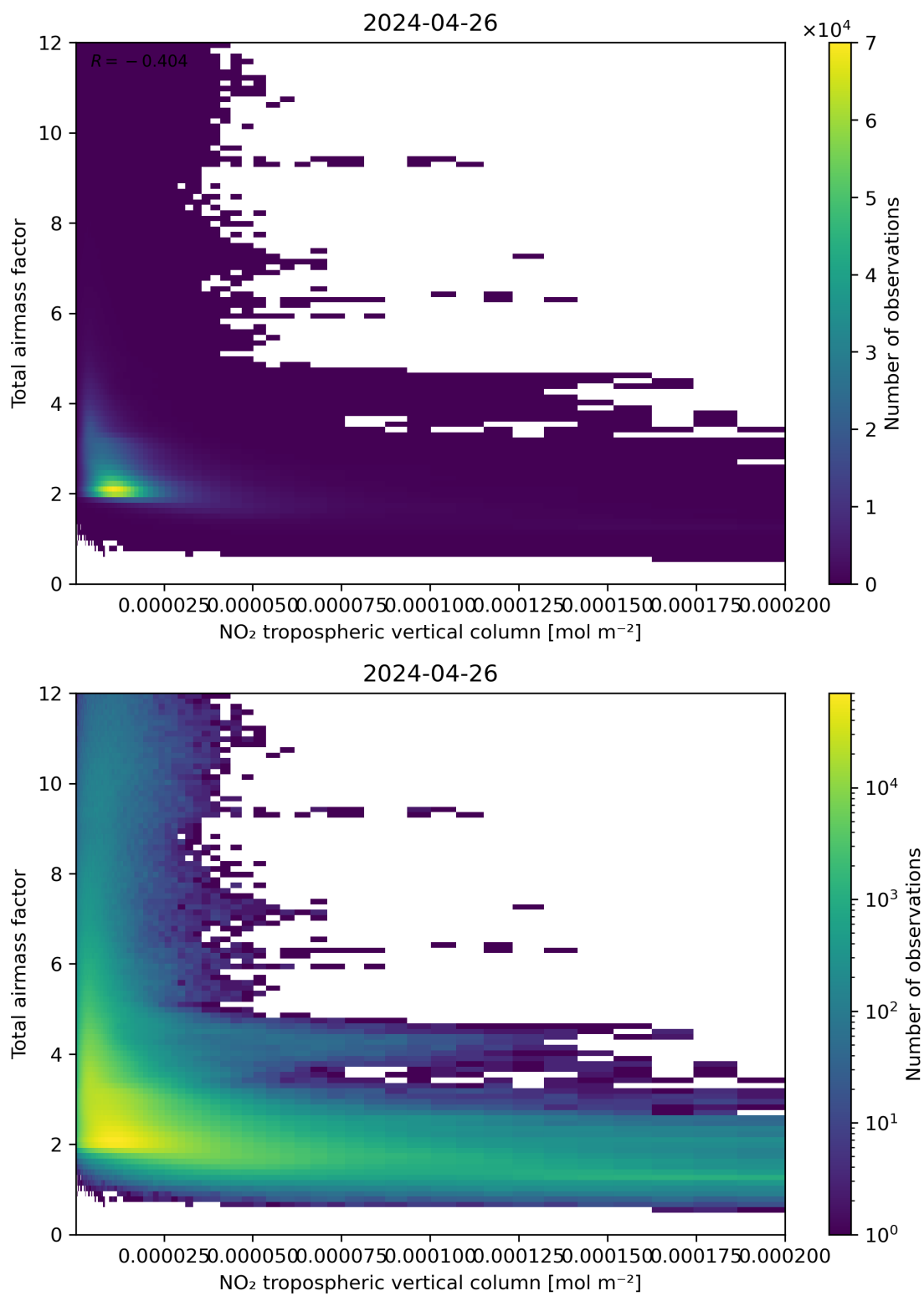
Figure 122: Scatter density plot of “NO 2 tropospheric vertical column” against “Total air mass factor” for 2024-04-26 to 2024-04-27.
