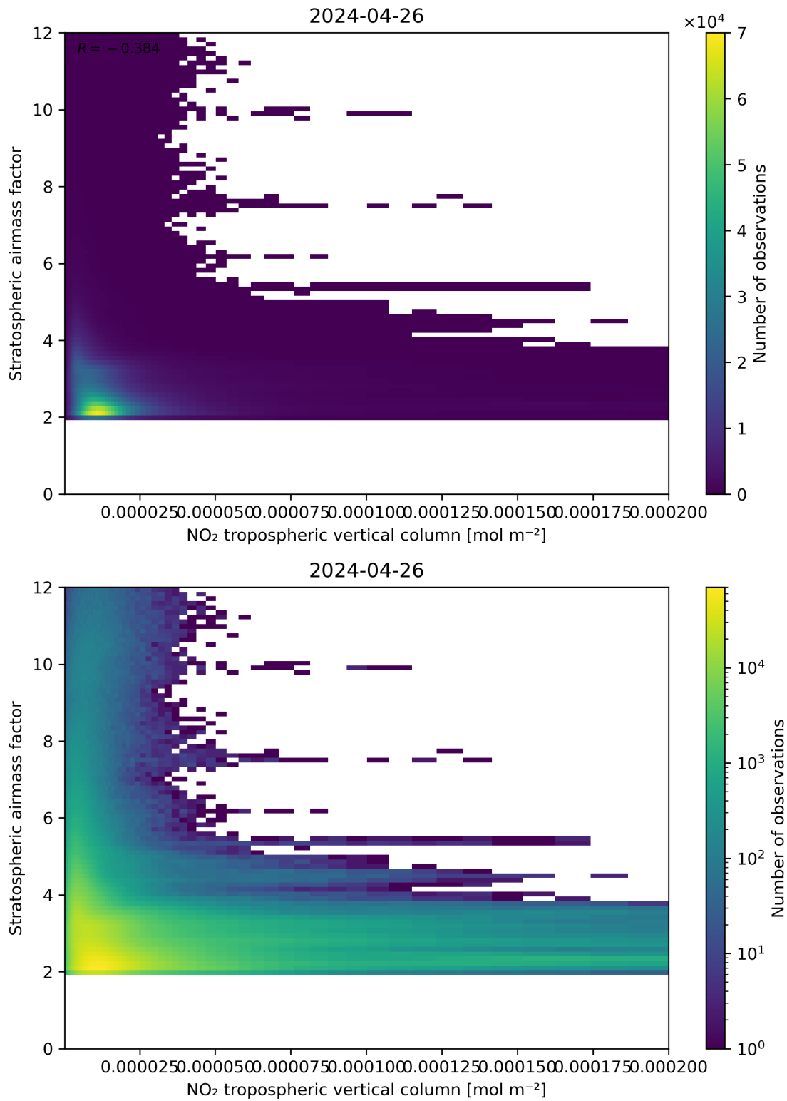
Figure 121: Scatter density plot of “NO 2 tropospheric vertical column” against “Stratospheric air mass factor” for 2024-04-26 to 2024-04-27.
