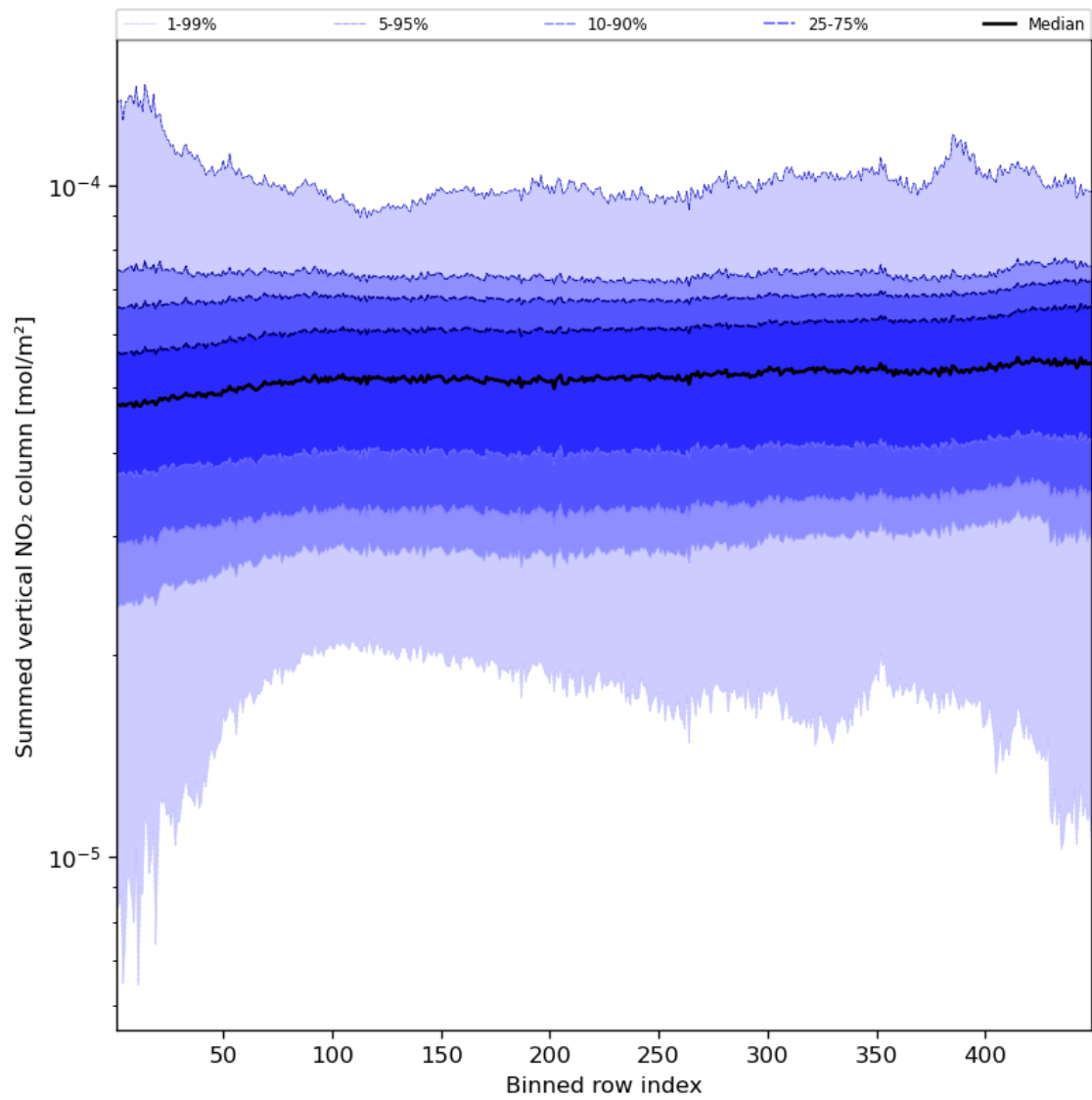
Figure 57: Along track statistics of “Summed vertical NO 2 column” for 2024-04-26 to 2024-04-27
