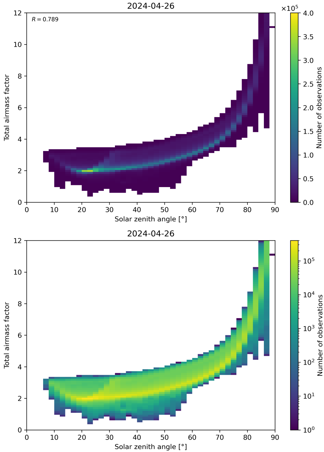
Figure 146: Scatter density plot of “Solar zenith angle” against “Total airmass factor” for 2024-04-26 to 2024-04-27.
