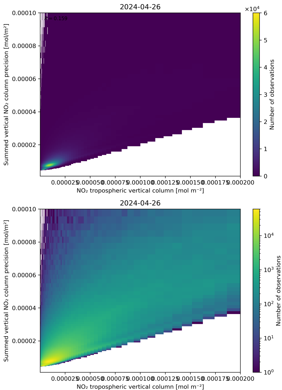
Figure 127: Scatter density plot of “NO 2 tropospheric vertical column” against “Summed vertical NO 2 column precision” for 2024-04-26 to 2024-04-27.
