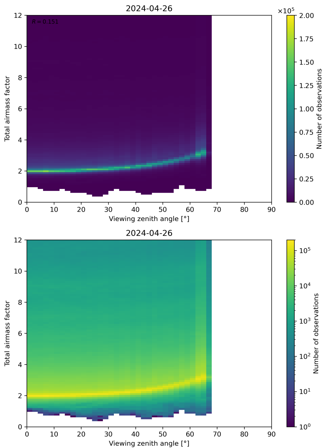
Figure 160: Scatter density plot of “Viewing zenith angle” against “Total airmass factor” for 2024-04-26 to 2024-04-27.
