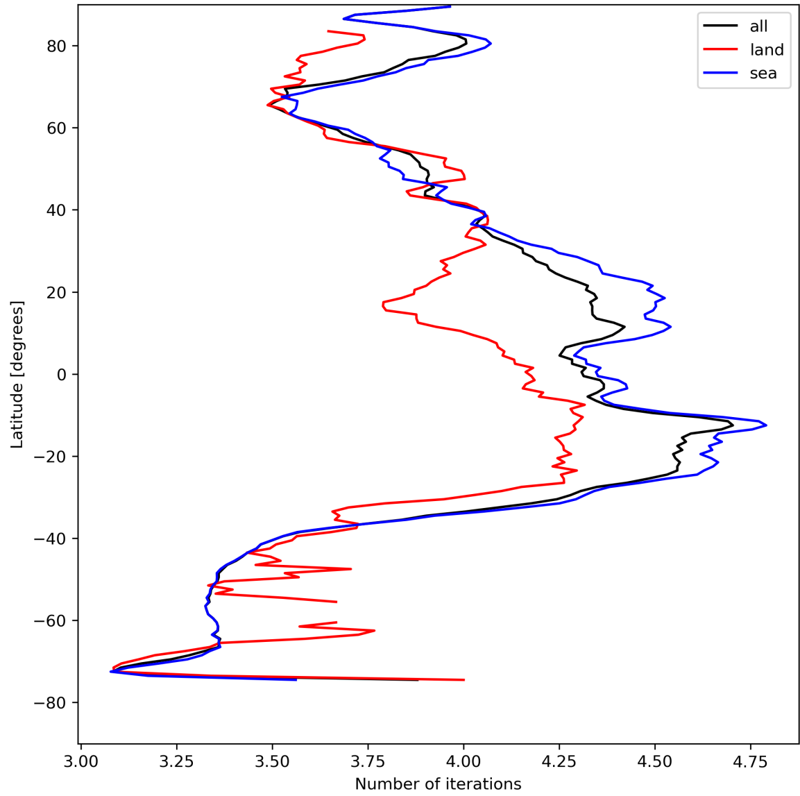
Figure 17: Zonal average of “Number of iterations” for 2024-04-26 to 2024-04-27.
