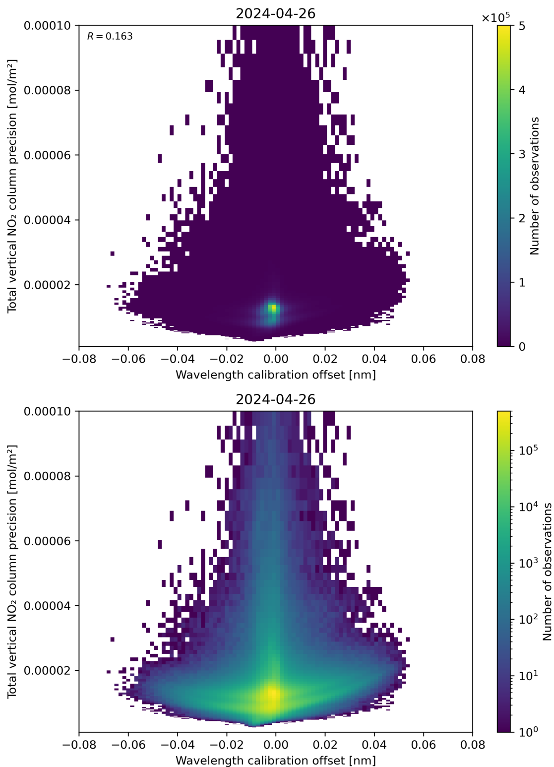
Figure 180: Scatter density plot of “Wavelength calibration offset” against “Total vertical NO 2 column precision” for 2024-04-26 to 2024-04-27.
