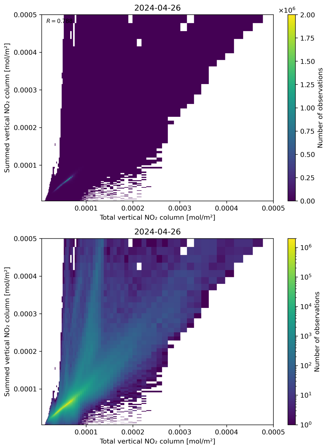
Figure 112: Scatter density plot of “Total vertical NO 2 column” against “Summed vertical NO 2 column” for 2024-04-26 to 2024-04-27.
