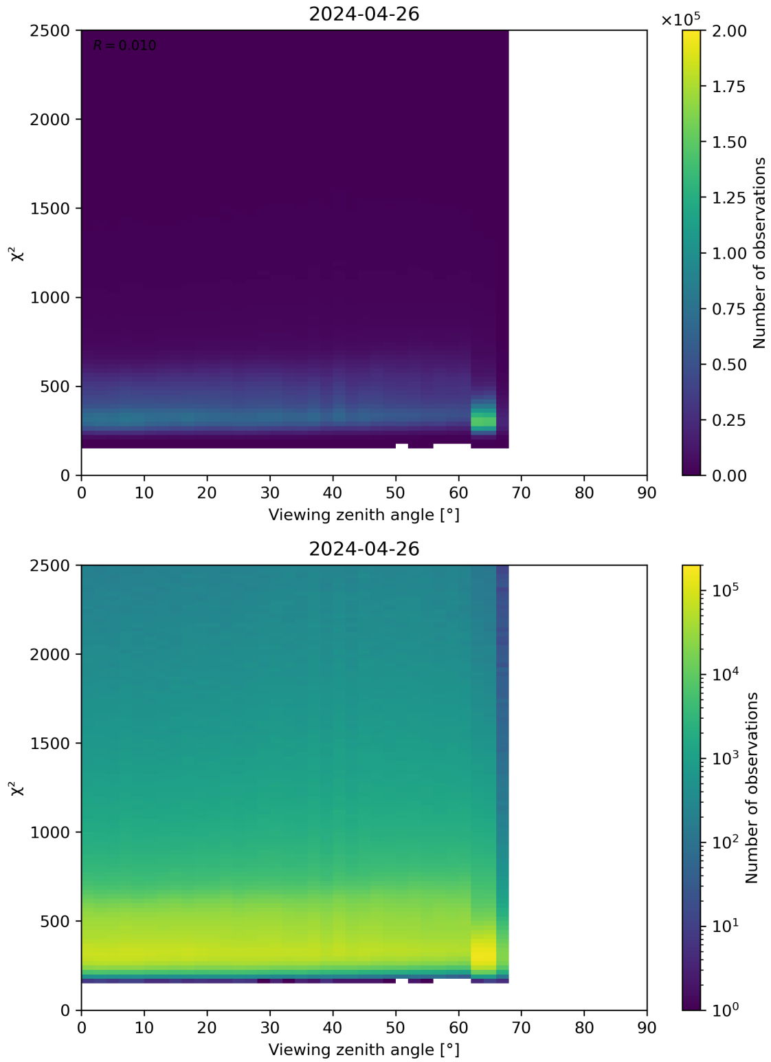
Figure 162: Scatter density plot of “Viewing zenith angle” against “ \chi^2 ” for 2024-04-26 to 2024-04-27.
