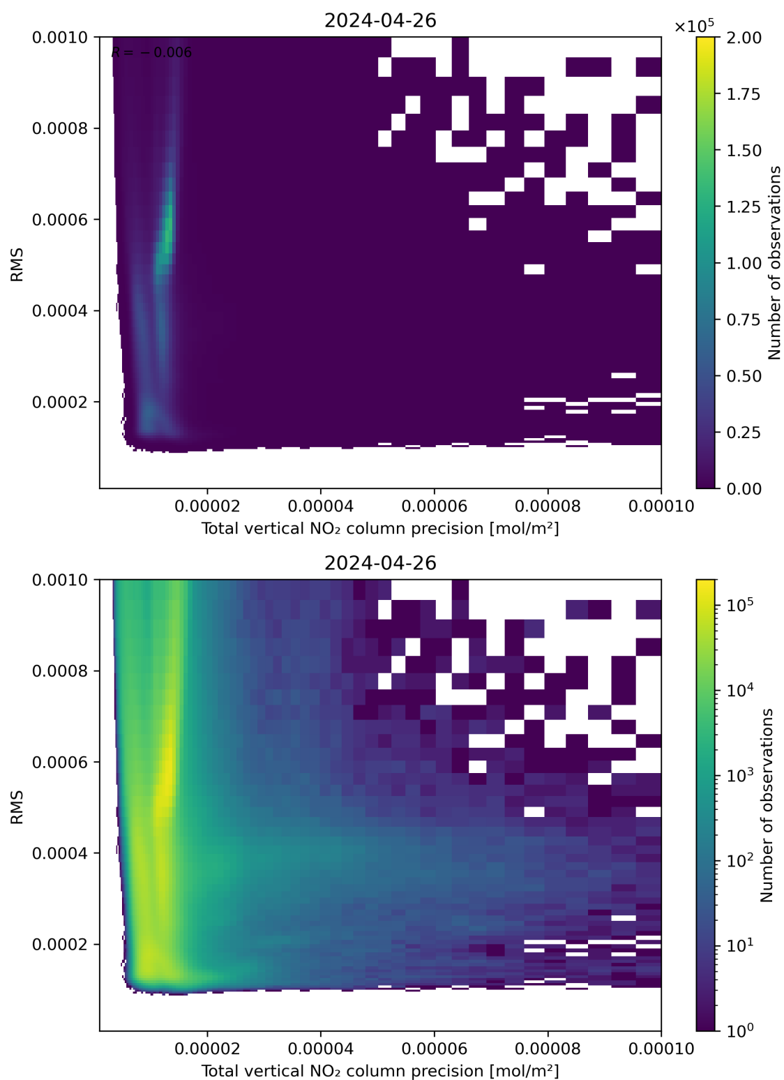
Figure 119: Scatter density plot of “Total vertical NO 2 column precision” against “RMS” for 2024-04-26 to 2024-04-27.
