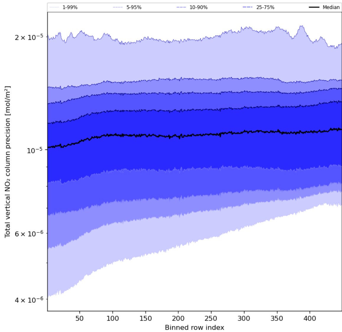
Figure 56: Along track statistics of “Total vertical NO 2 column precision” for 2024-04-26 to 2024-04-27
