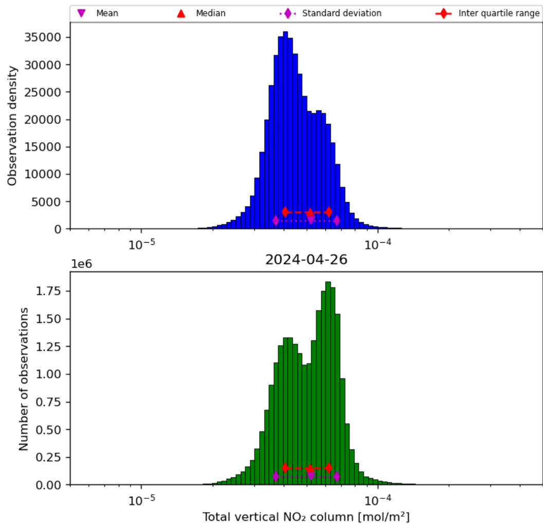
Figure 38: Histogram of "Total vertical NO 2 column" for 2024-04-26 to 2024-04-27
