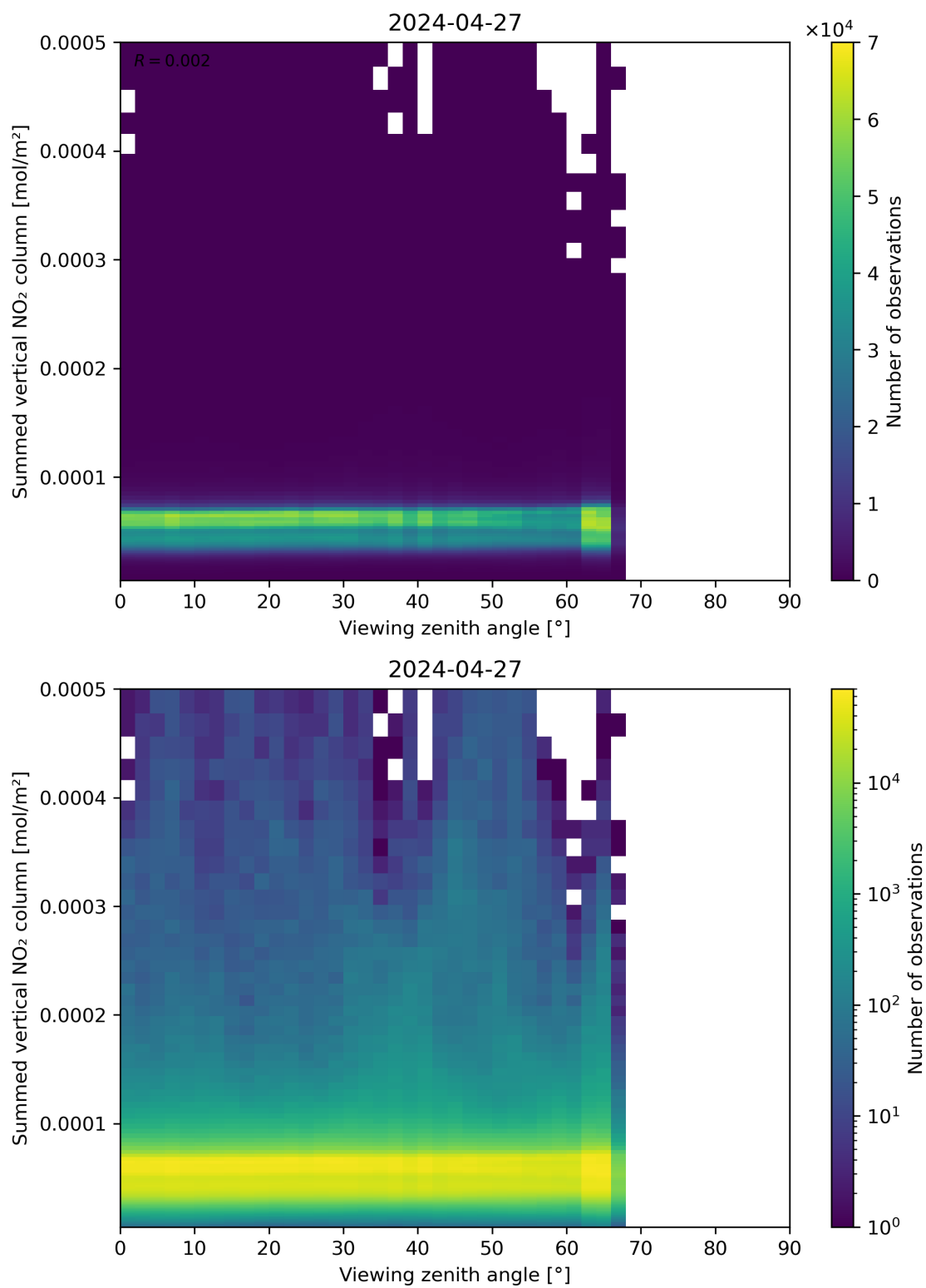
Figure 165: Scatter density plot of “Viewing zenith angle” against “Summed vertical NO 2 column” for 2024-04-26 to 2024-04-28.
