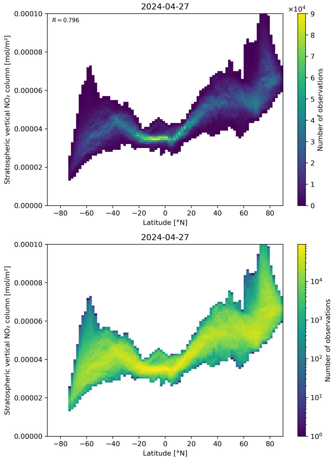
Figure 87: Scatter density plot of “Latitude” against “Stratospheric vertical NO 2 column” for 2024-04-26 to 2024-04-28.
