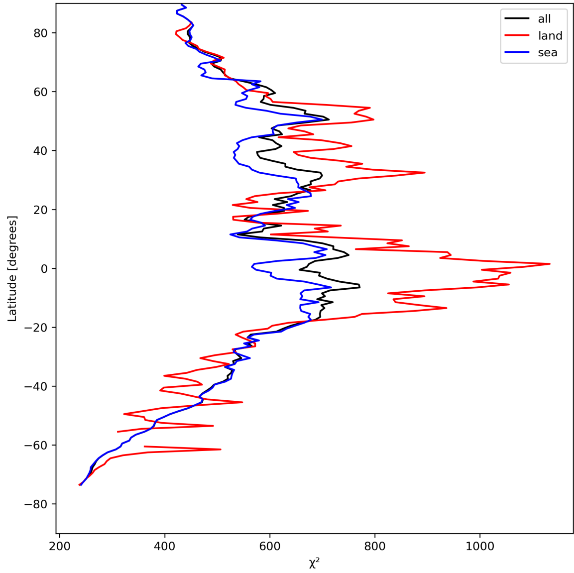
Figure 25: Zonal average of “ \chi^2 ” for 2024-04-26 to 2024-04-28.
