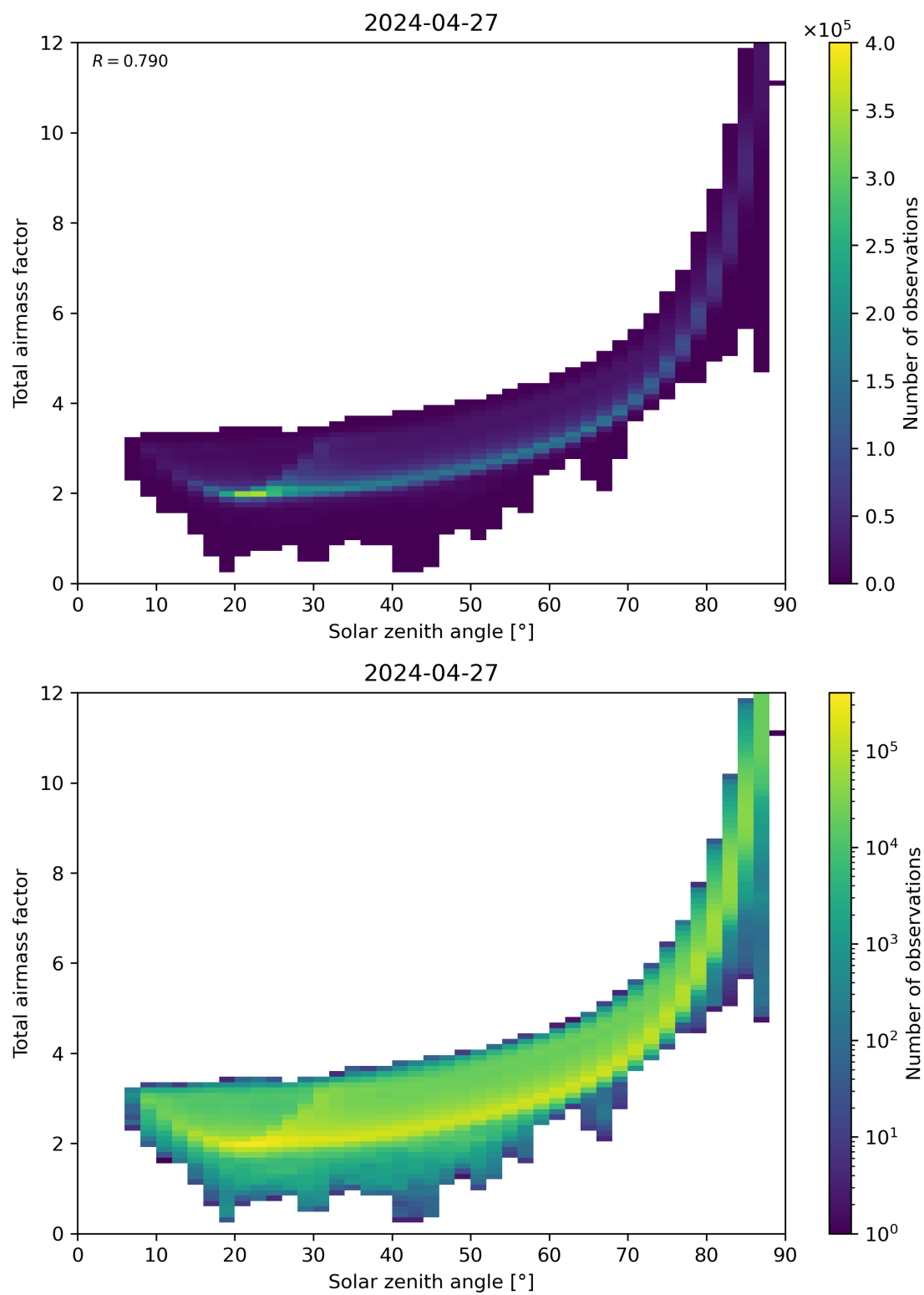
Figure 146: Scatter density plot of “Solar zenith angle” against “Total air mass factor” for 2024-04-26 to 2024-04-28.
