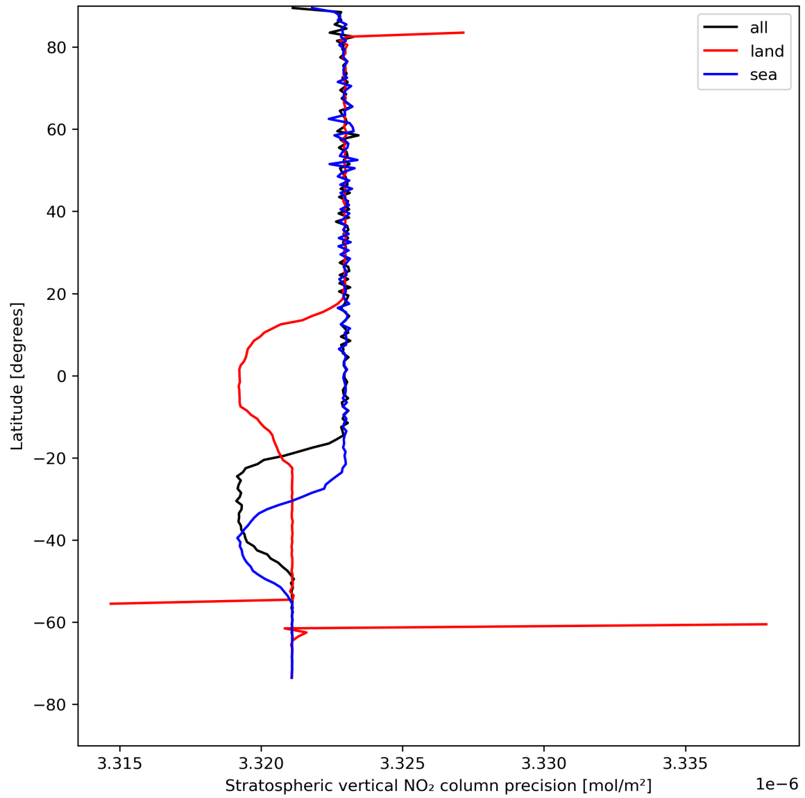
Figure 20: Zonal average of “Stratospheric vertical NO 2 column precision” for 2024-04-26 to 2024-04-28.
