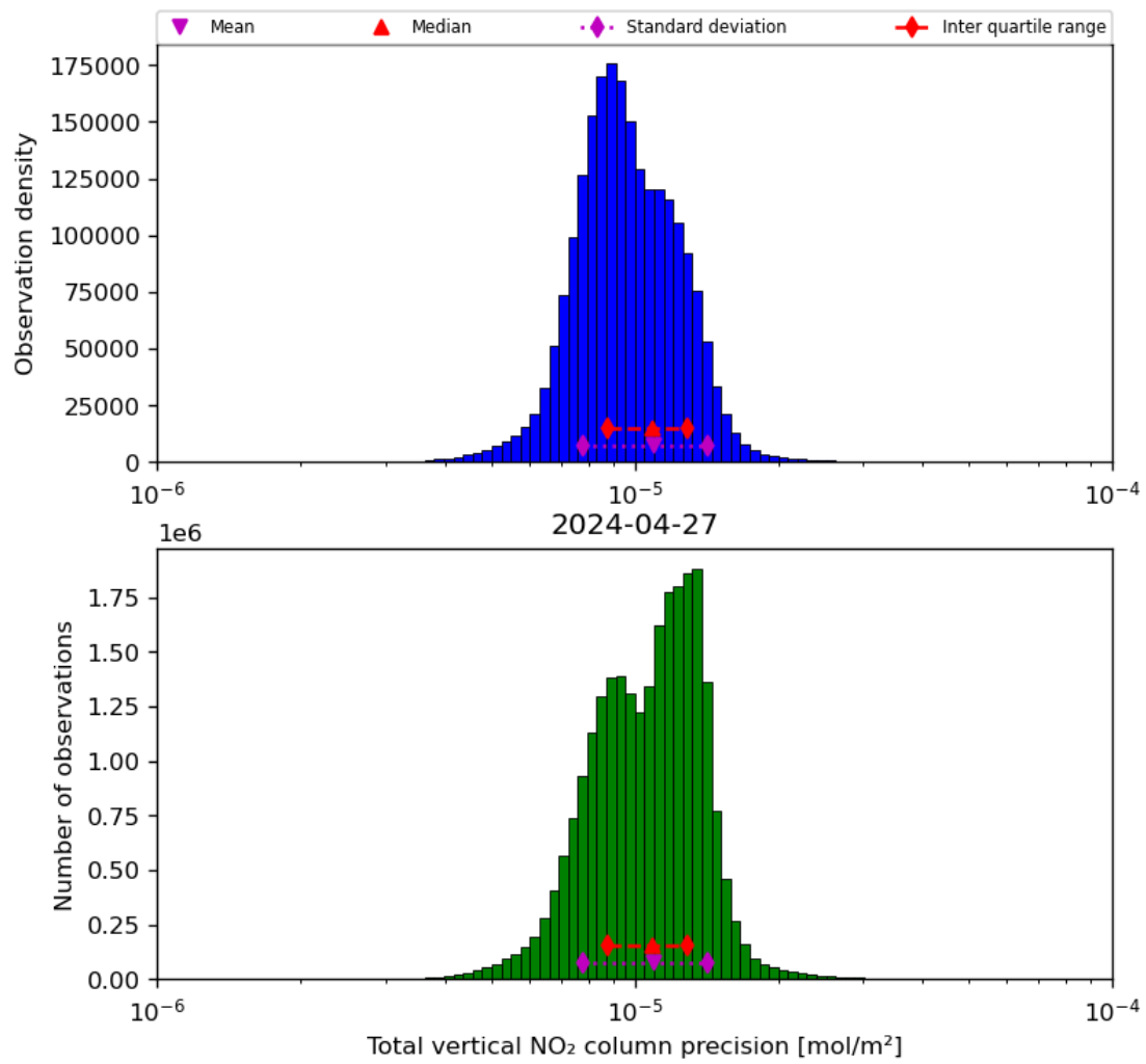
Figure 39: Histogram of “Total vertical NO 2 column precision” for 2024-04-26 to 2024-04-28
