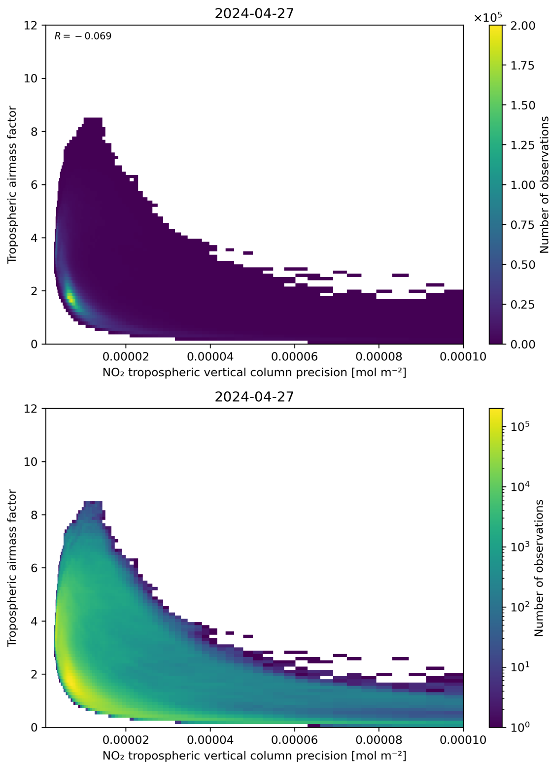
Figure 133: Scatter density plot of “NO 2 tropospheric vertical column precision” against “Tropospheric airmass factor” for 2024-04-26 to 2024-04-28.
