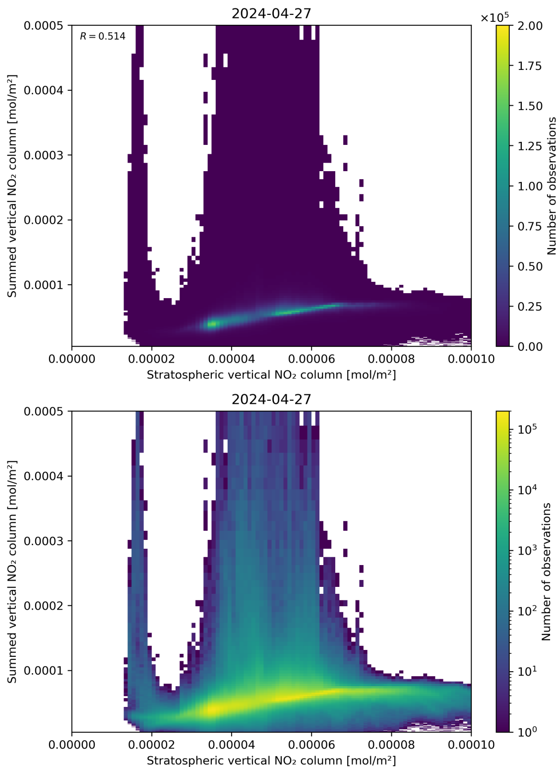
Figure 98: Scatter density plot of “Stratospheric vertical NO 2 column” against “Summed vertical NO 2 column” for 2024-04-26 to 2024-04-28.
