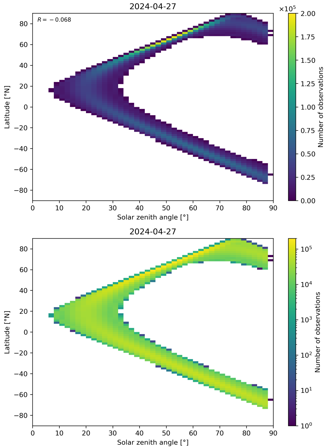
Figure 149: Scatter density plot of “Solar zenith angle” against “Latitude” for 2024-04-26 to 2024-04-28.
