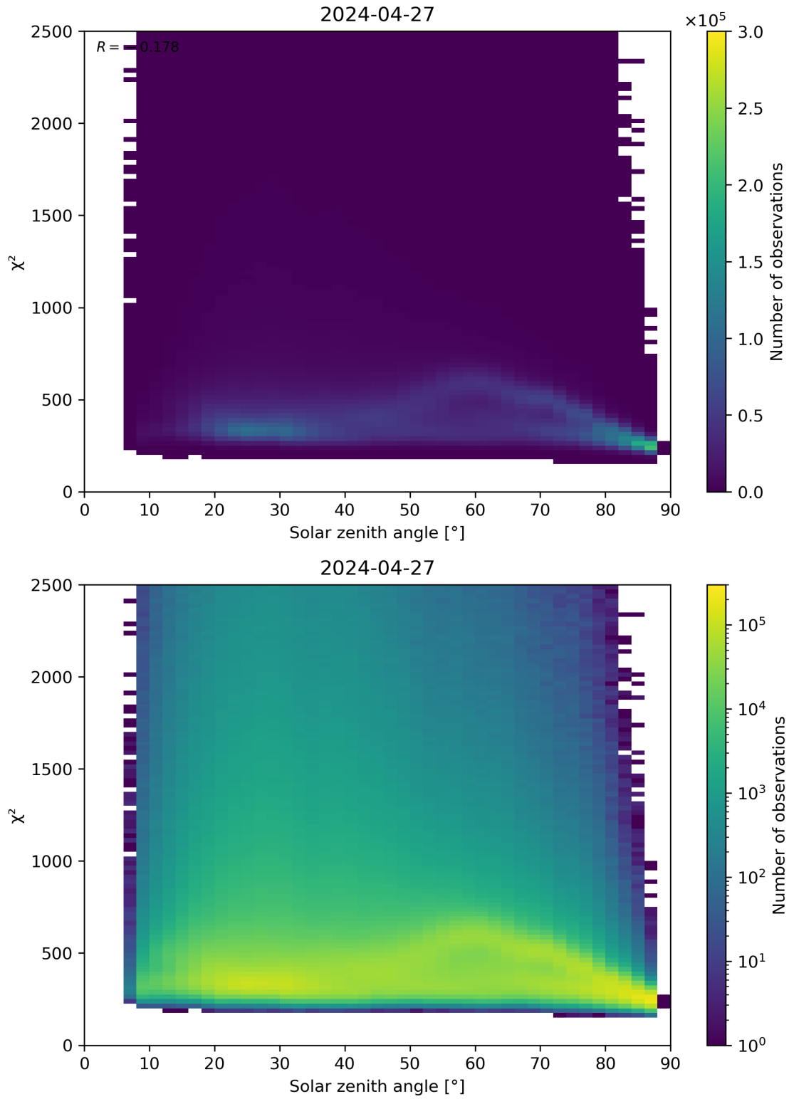
Figure 148: Scatter density plot of “Solar zenith angle” against “ \chi^2 ” for 2024-04-26 to 2024-04-28.
