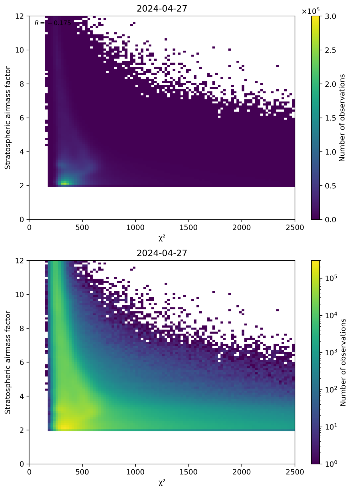
Figure 81: Scatter density plot of “ \chi^2 ” against “Stratospheric airmass factor” for 2024-04-26 to 2024-04-28.
