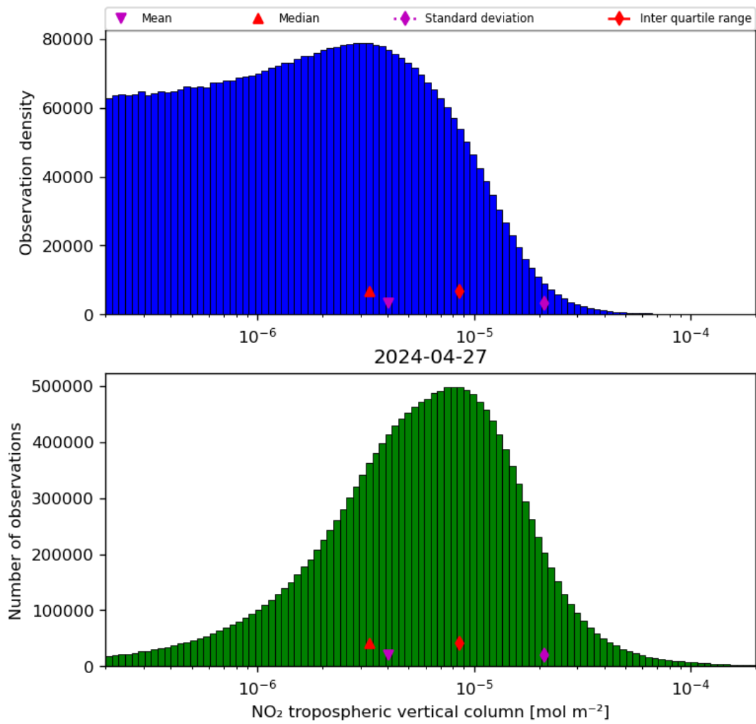
Figure 29: Histogram of “NO 2 tropospheric vertical column” for 2024-04-26 to 2024-04-28
