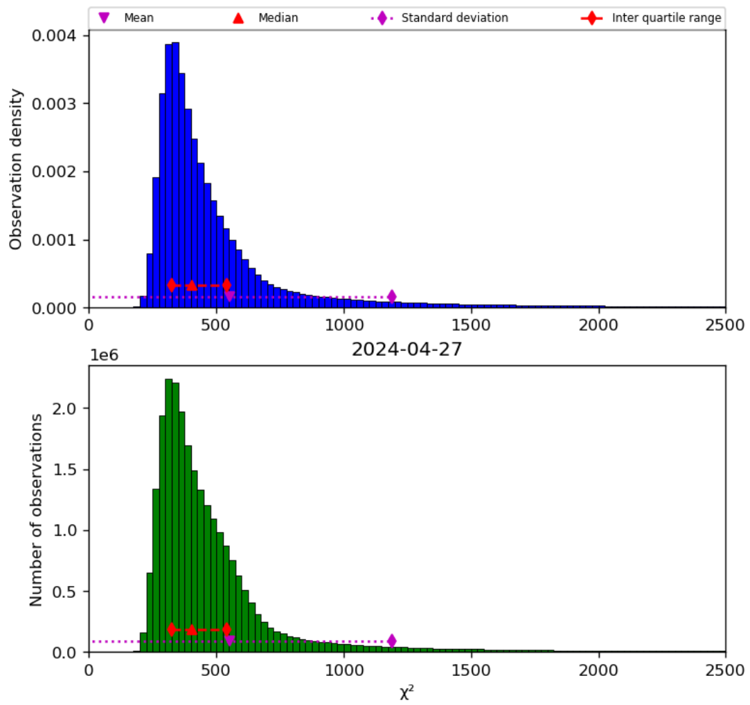
Figure 42: Histogram of “ \chi^2 ” for 2024-04-26 to 2024-04-28
