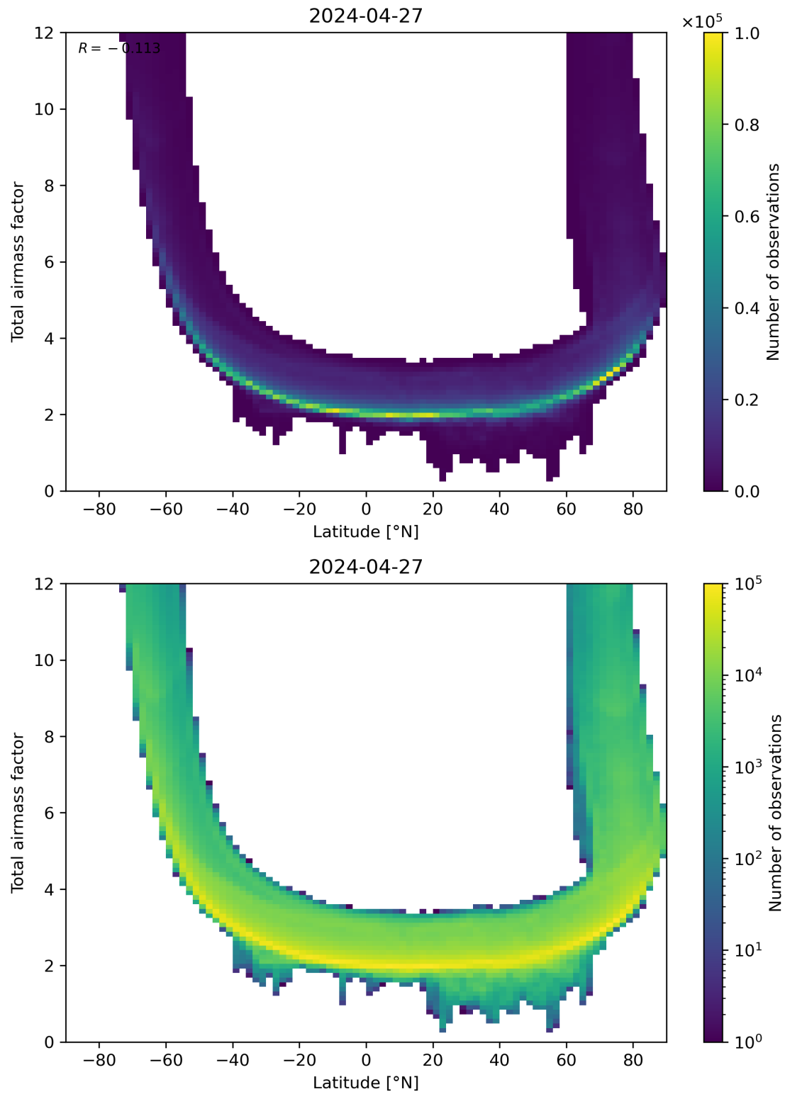
Figure 84: Scatter density plot of “Latitude” against “Total airmass factor” for 2024-04-26 to 2024-04-28.
