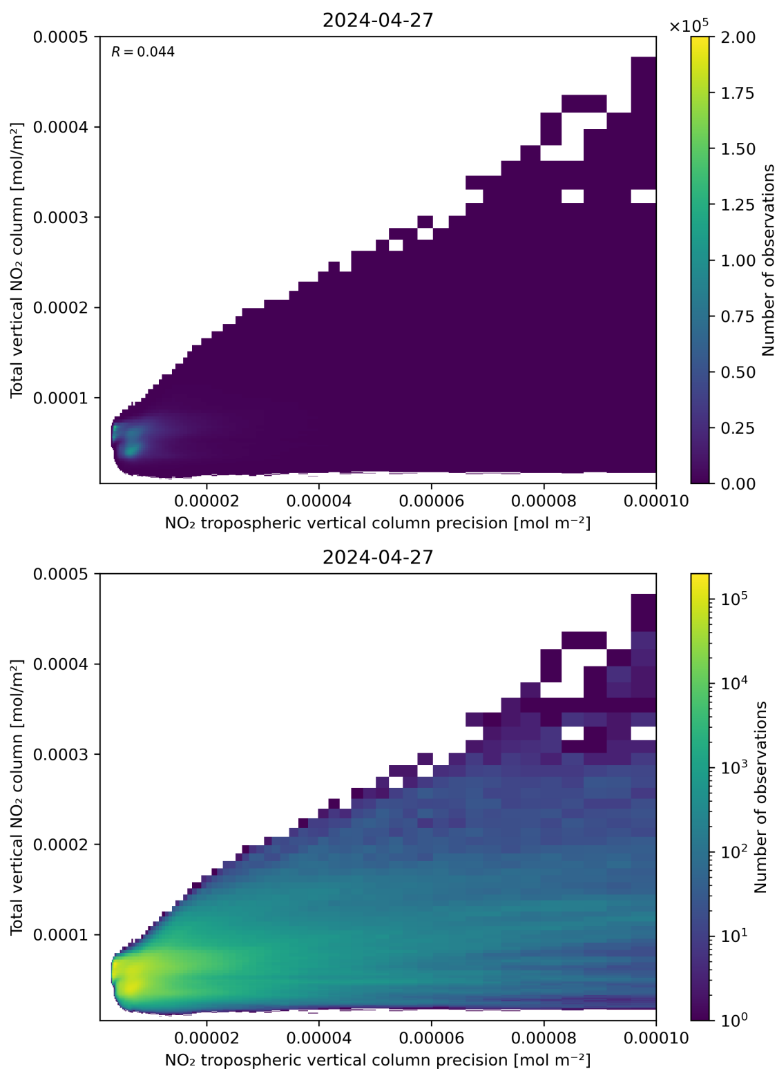
Figure 138: Scatter density plot of “NO 2 tropospheric vertical column precision” against “Total vertical NO 2 column” for 2024-04-26 to 2024-04-28.
