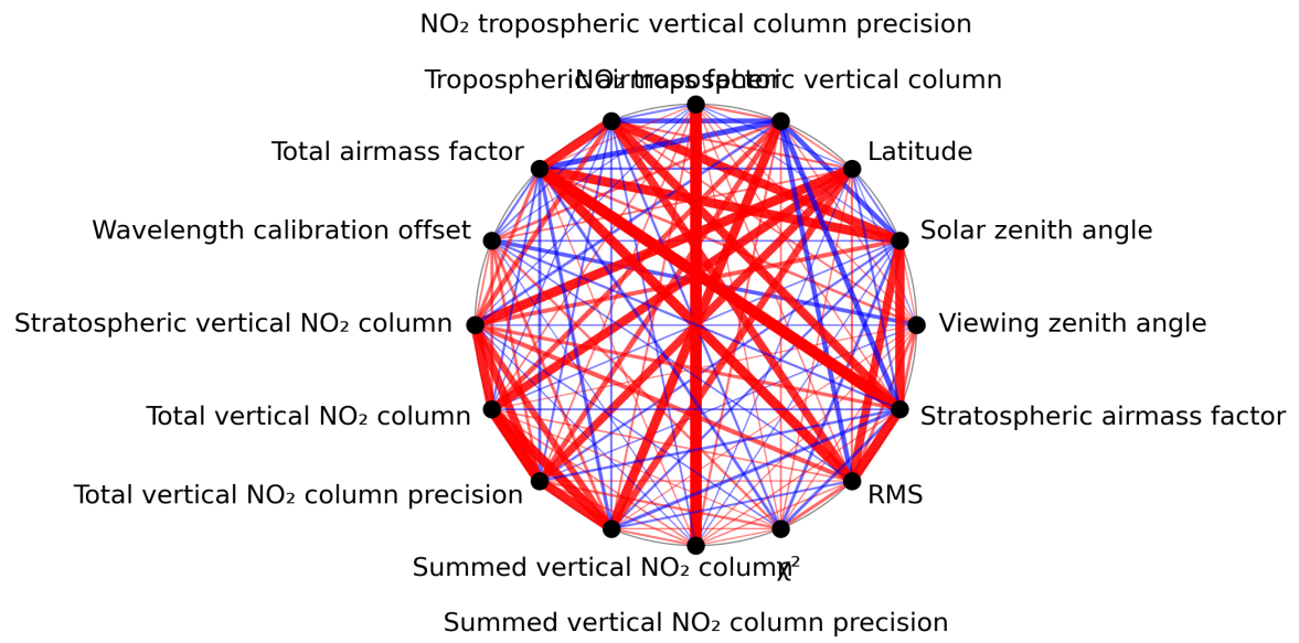
Figure 1: Map of correlation graph for 2024-04-26 to 2024-04-28.
