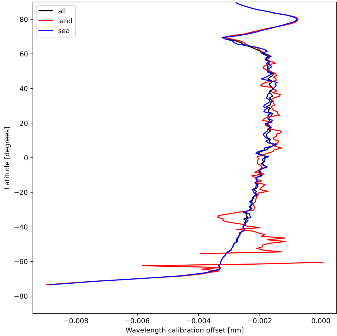
Figure 18: Zonal average of “Wavelength calibration offset” for 2024-04-26 to 2024-04-28.
