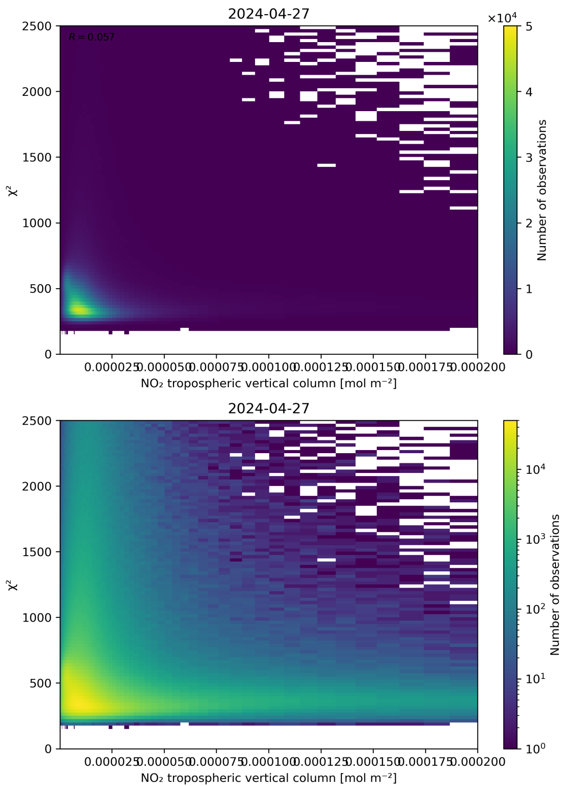
Figure 124: Scatter density plot of “NO 2 tropospheric vertical column” against “ \chi^2 ” for 2024-04-26 to 2024-04-28.
