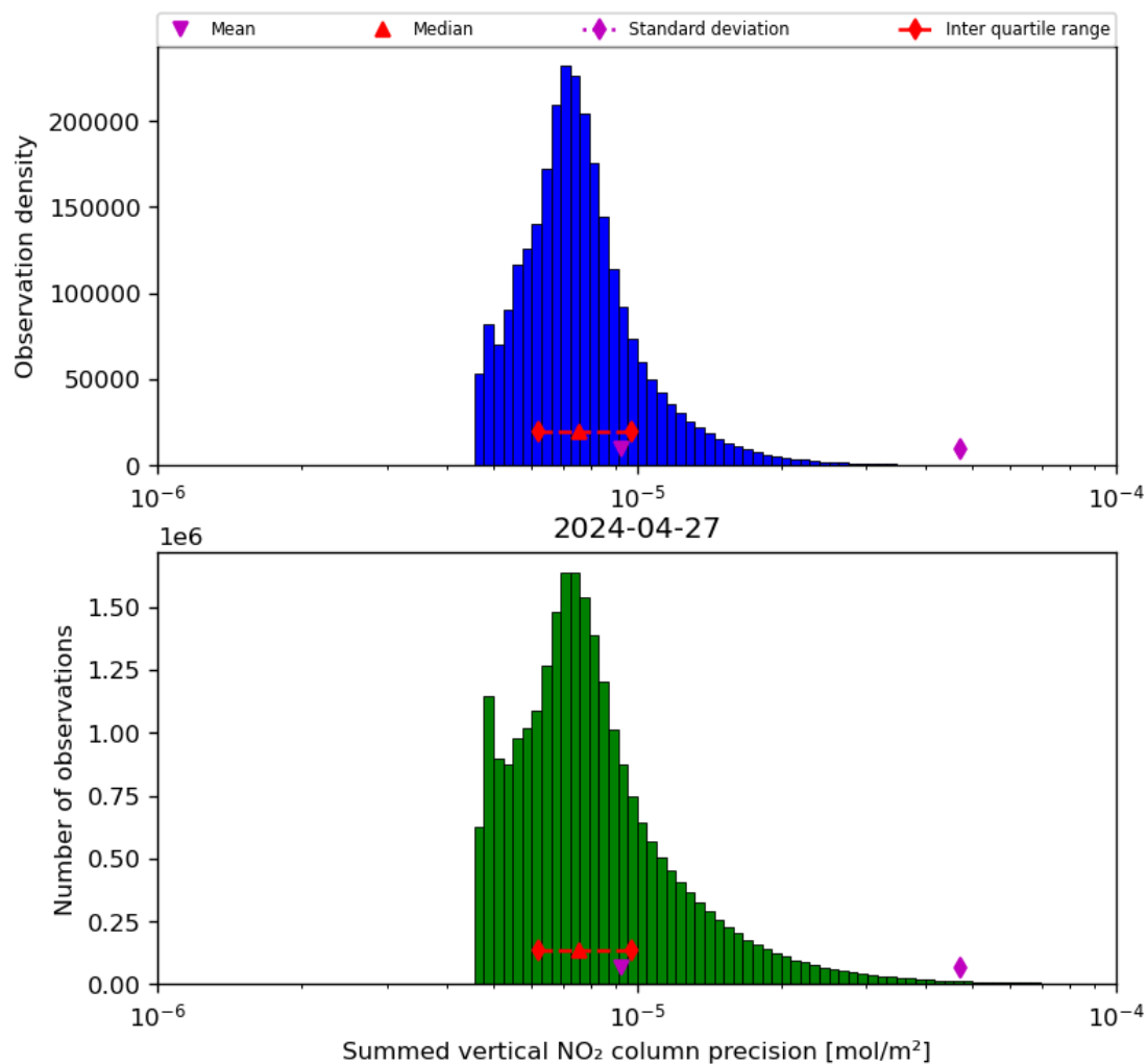
Figure 41: Histogram of “Summed vertical NO 2 column precision” for 2024-04-26 to 2024-04-28
