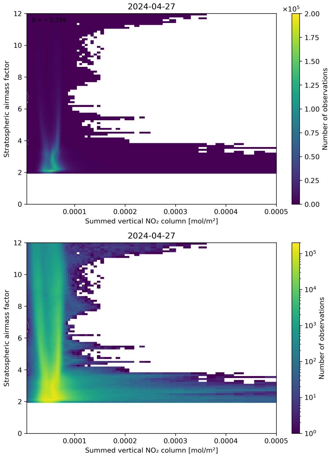
Figure 103: Scatter density plot of “Summed vertical NO 2 column” against “Stratospheric air mass factor” for 2024-04-26 to 2024-04-28.
