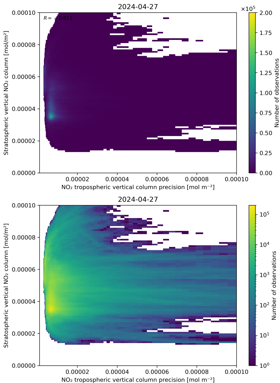
Figure 135: Scatter density plot of “NO 2 tropospheric vertical column precision” against “Stratospheric vertical NO 2 column” for 2024-04-26 to 2024-04-28.
