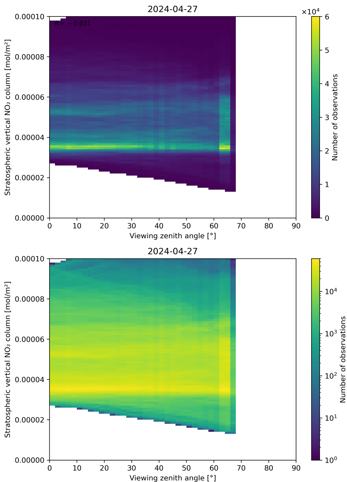
Figure 164: Scatter density plot of “Viewing zenith angle” against “Stratospheric vertical NO 2 column” for 2024-04-26 to 2024-04-28.
