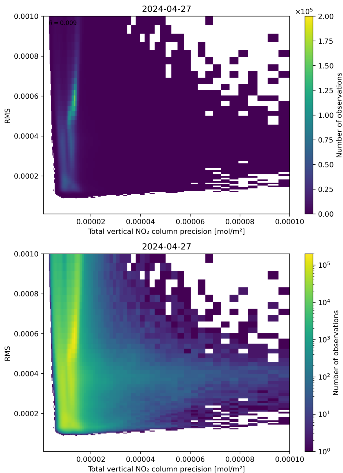
Figure 119: Scatter density plot of “Total vertical NO 2 column precision” against “RMS” for 2024-04-26 to 2024-04-28.
