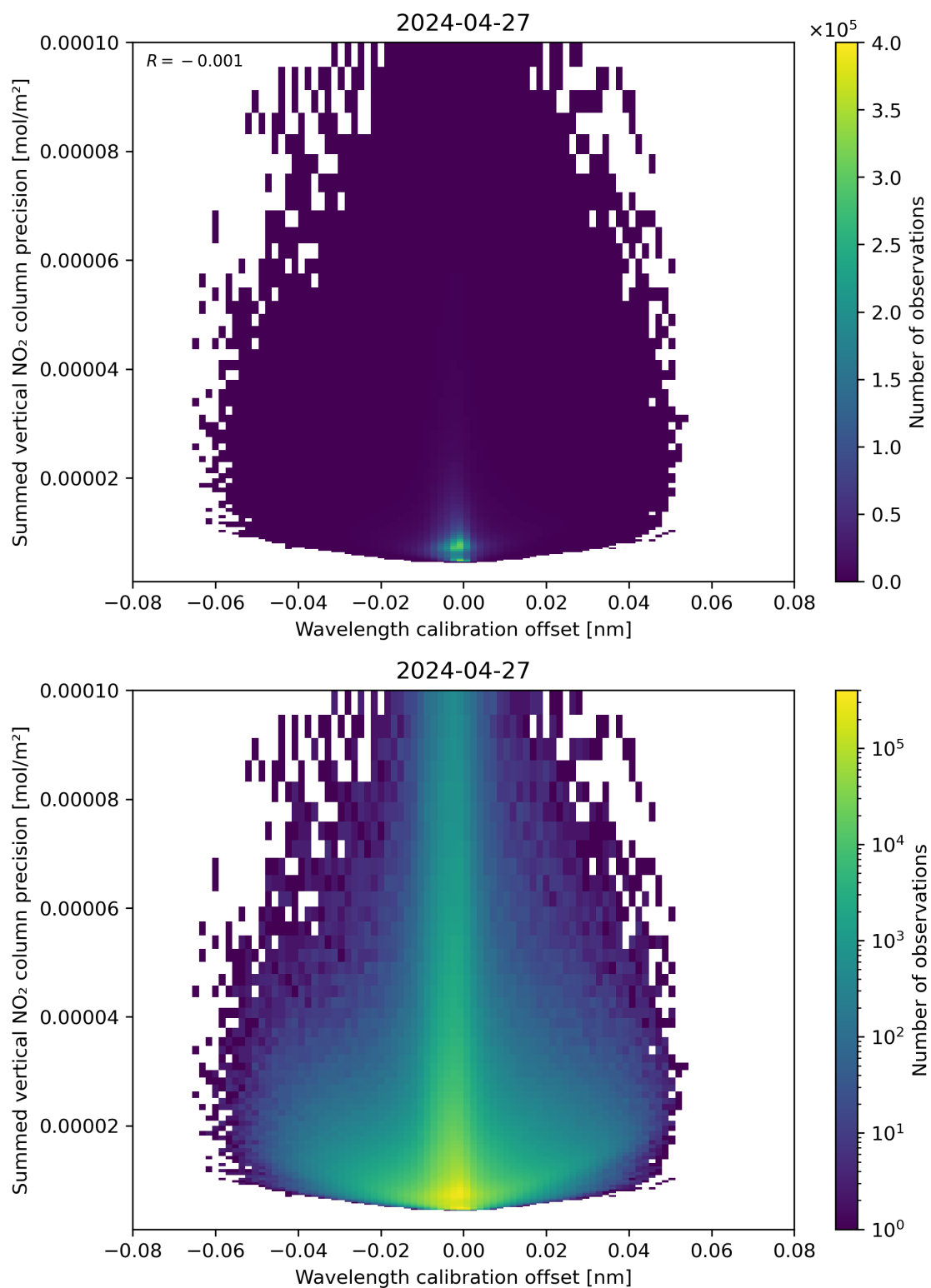
Figure 178: Scatter density plot of “Wavelength calibration offset” against “Summed vertical NO 2 column precision” for 2024-04-26 to 2024-04-28.
