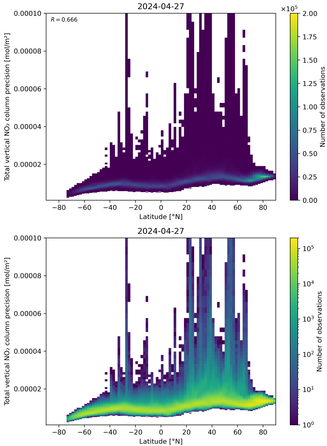
Figure 91: Scatter density plot of “Latitude” against “Total vertical NO 2 column precision” for 2024-04-26 to 2024-04-28.
