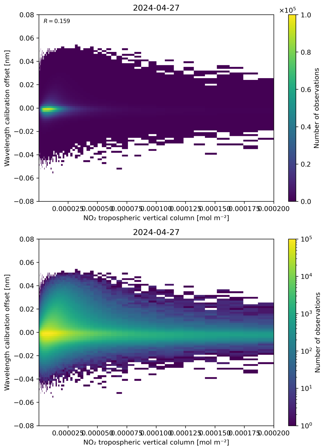
Figure 143: Scatter density plot of “NO 2 tropospheric vertical column” against “Wavelength calibration offset” for 2024-04-26 to 2024-04-28.
