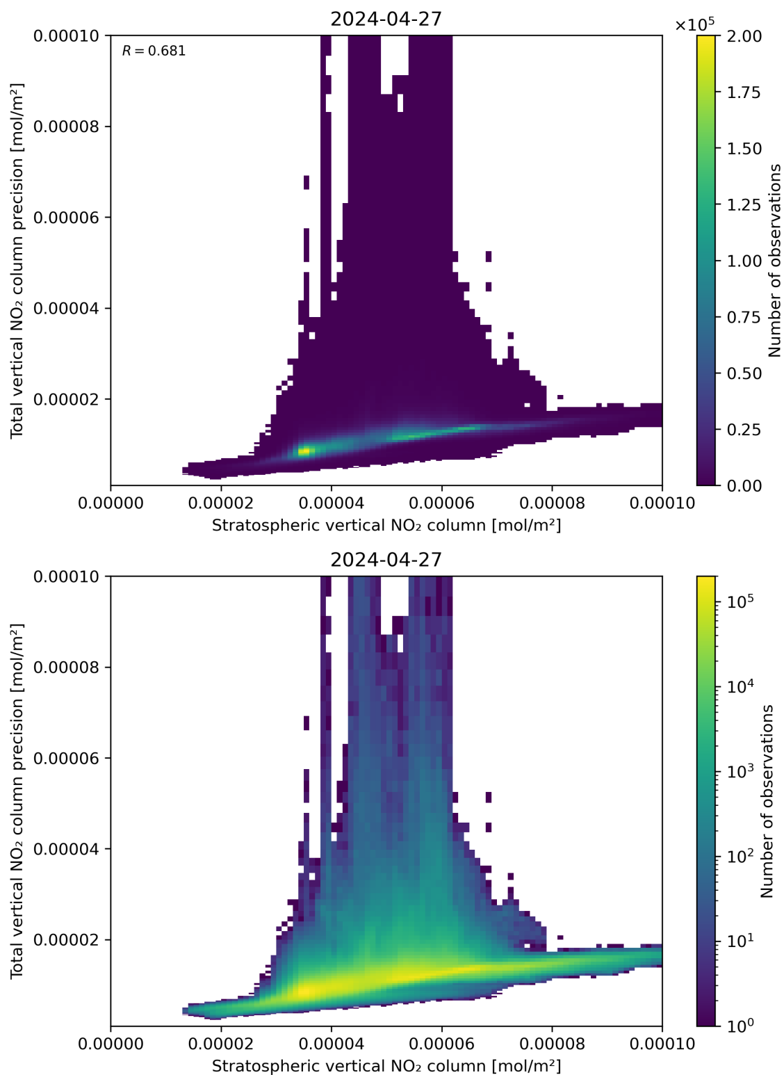
Figure 101: Scatter density plot of “Stratospheric vertical NO 2 column” against “Total vertical NO 2 column precision” for 2024-04-26 to 2024-04-28.
