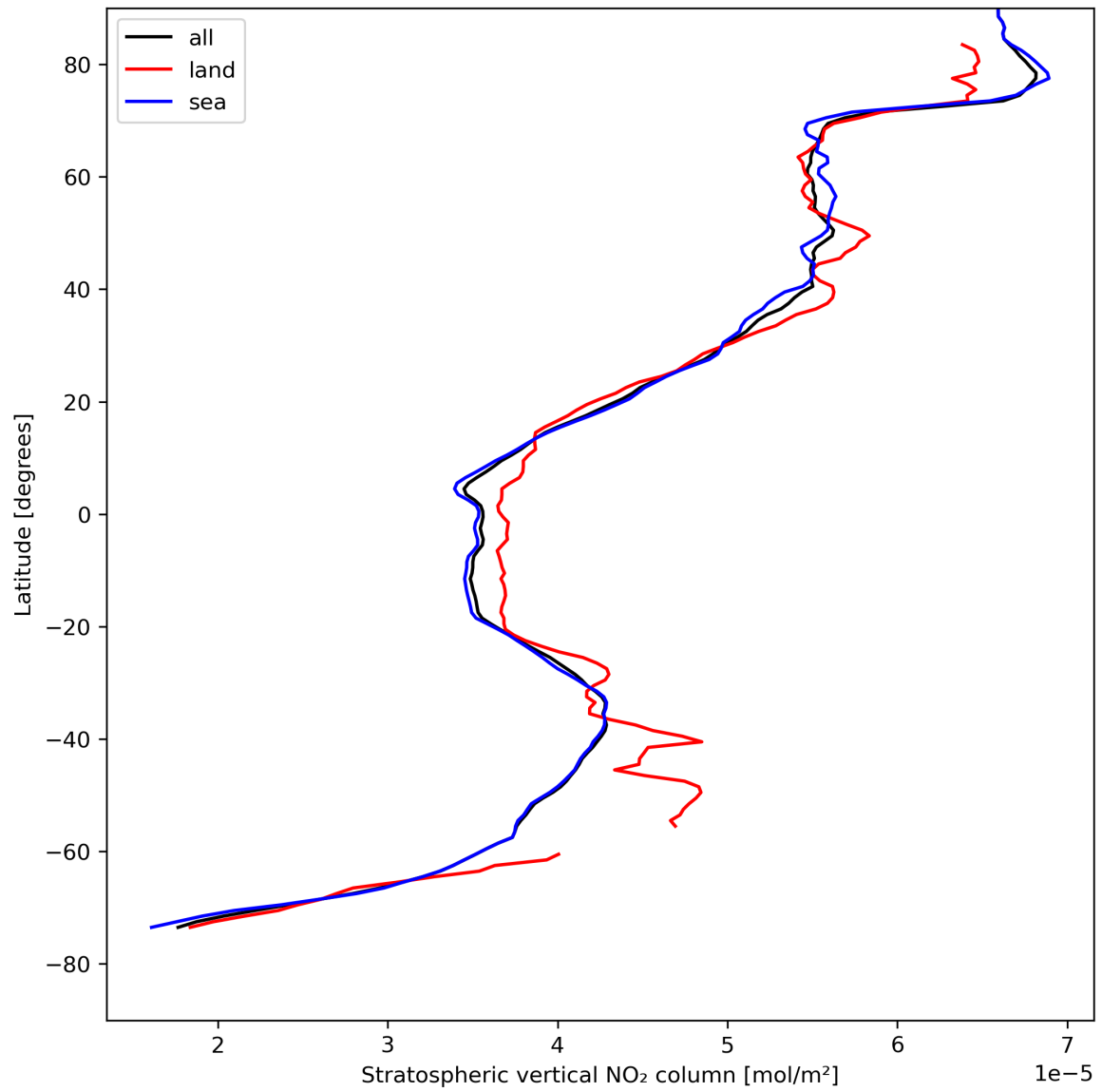
Figure 19: Zonal average of “Stratospheric vertical NO 2 column” for 2024-04-26 to 2024-04-28.
