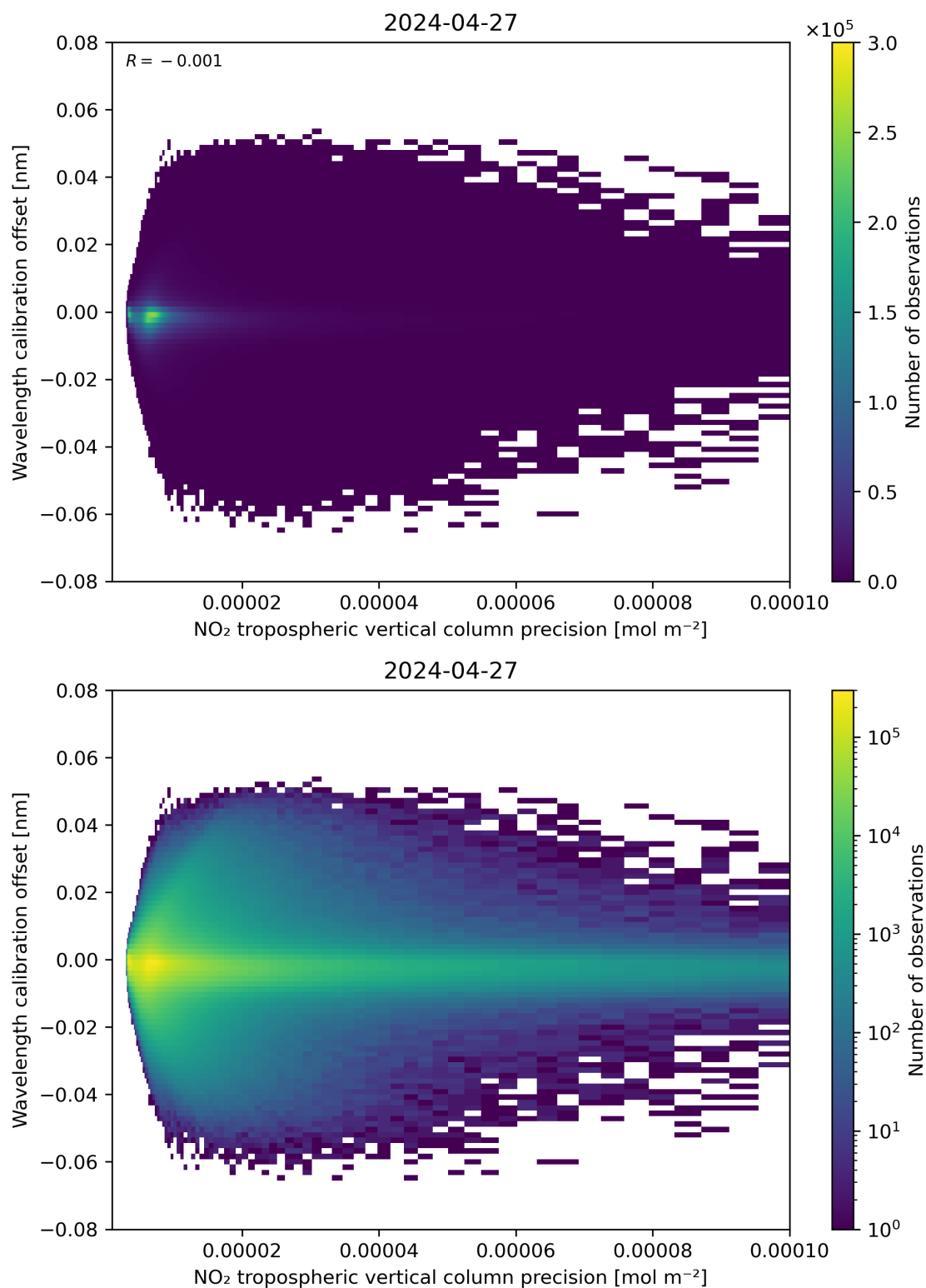
Figure 141: Scatter density plot of “NO 2 tropospheric vertical column precision” against “Wavelength calibration offset” for 2024-04-26 to 2024-04-28.
