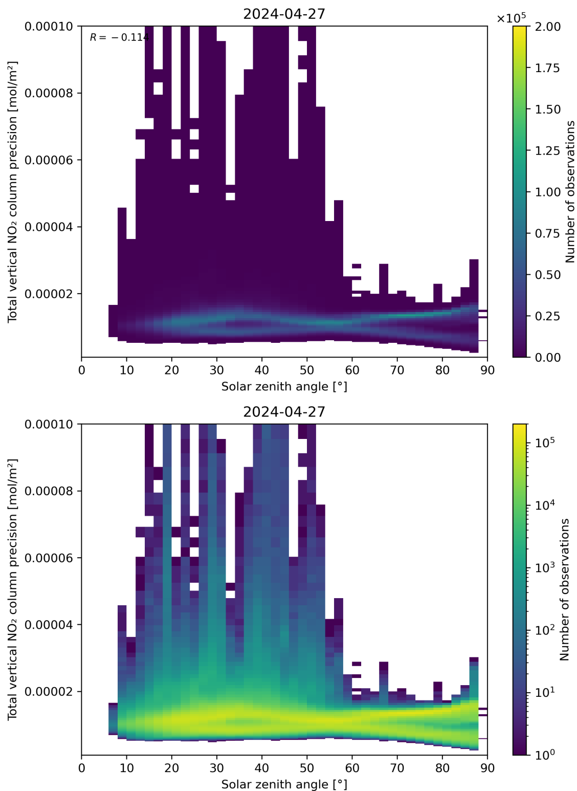
Figure 154: Scatter density plot of “Solar zenith angle” against “Total vertical NO 2 column precision” for 2024-04-26 to 2024-04-28.
