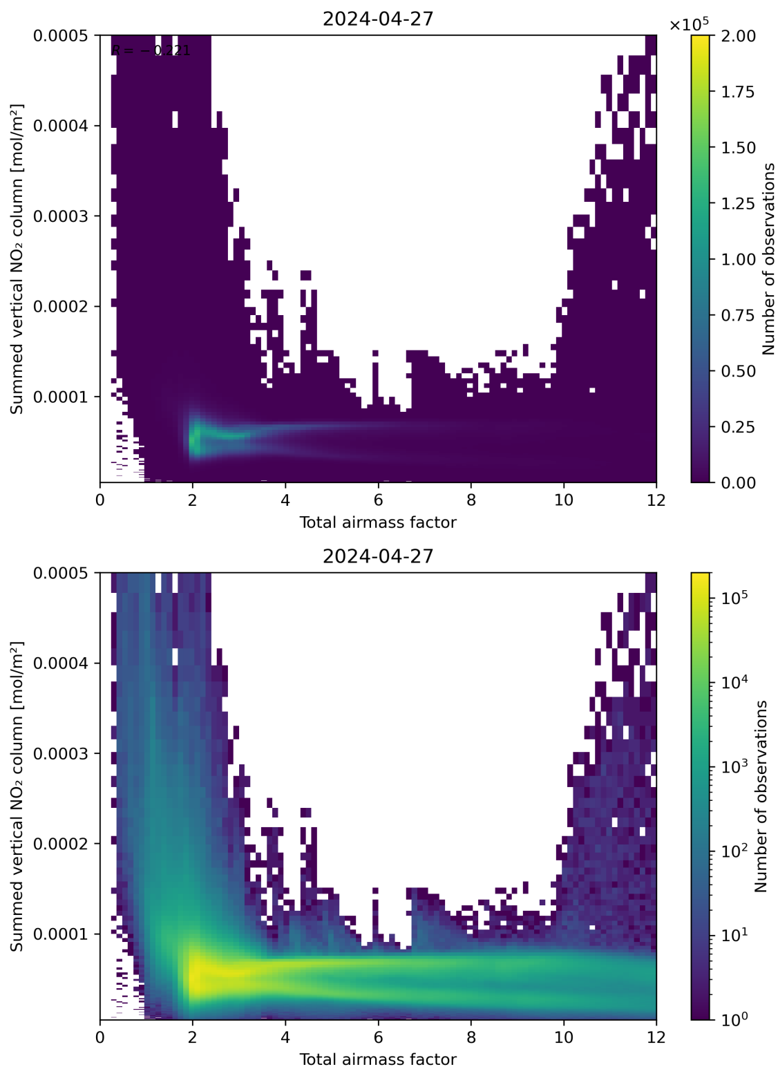
Figure 65: Scatter density plot of “Total airmass factor” against “Summed vertical NO 2 column” for 2024-04-26 to 2024-04-28.
