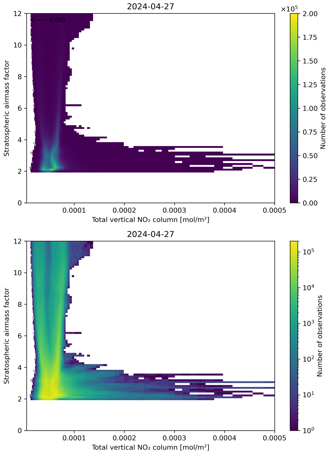
Figure 110: Scatter density plot of “Total vertical NO 2 column” against “Stratospheric airmass factor” for 2024-04-26 to 2024-04-28.
