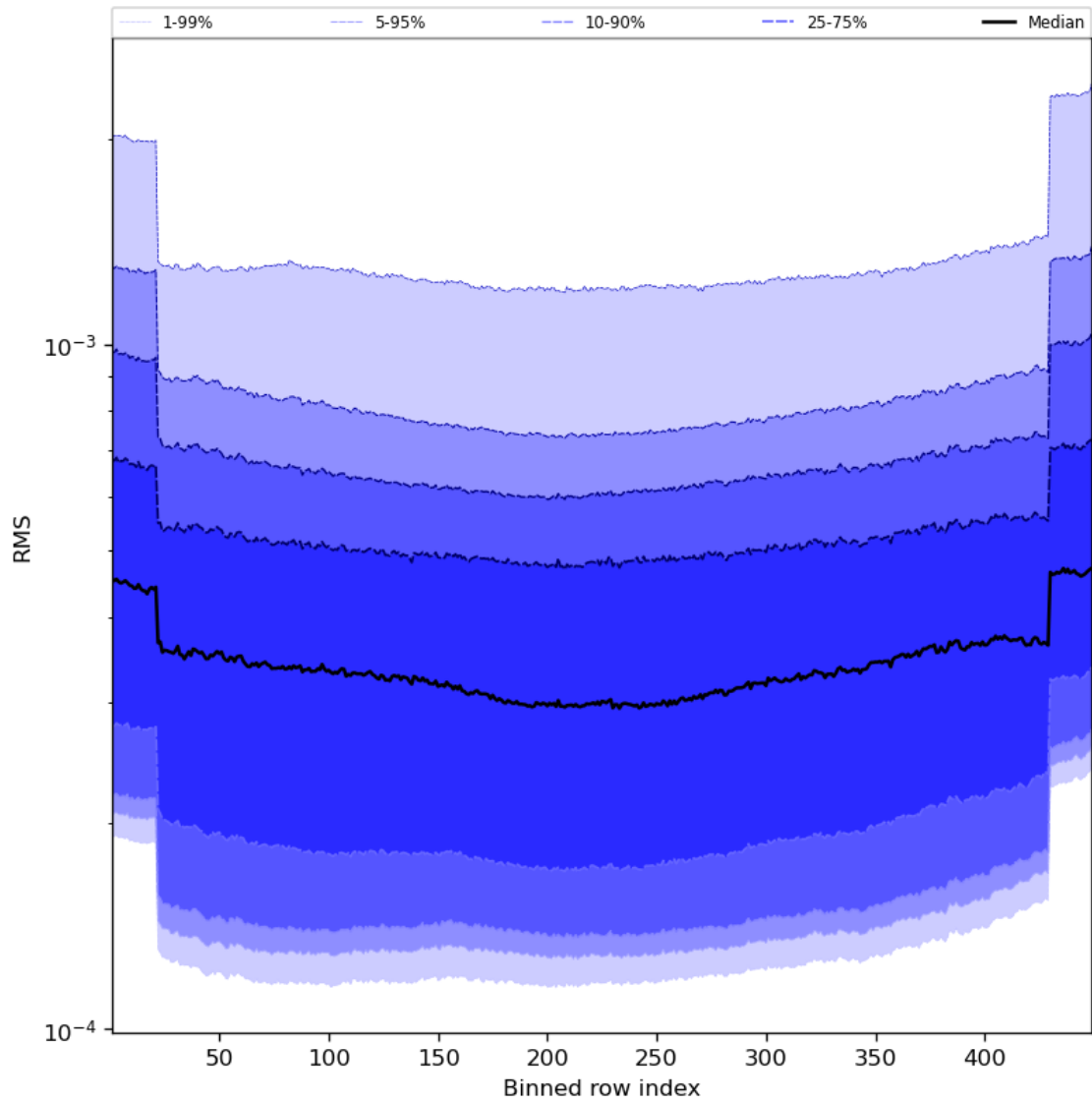
Figure 60: Along track statistics of “RMS” for 2024-04-26 to 2024-04-28
