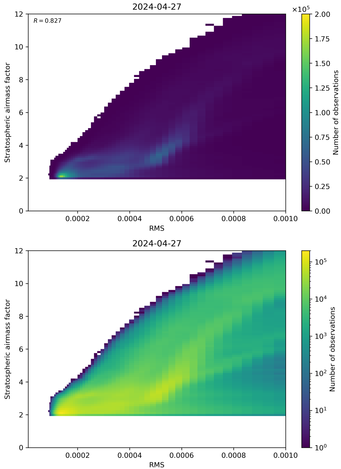
Figure 144: Scatter density plot of “RMS” against “Stratospheric airmass factor” for 2024-04-26 to 2024-04-28.
