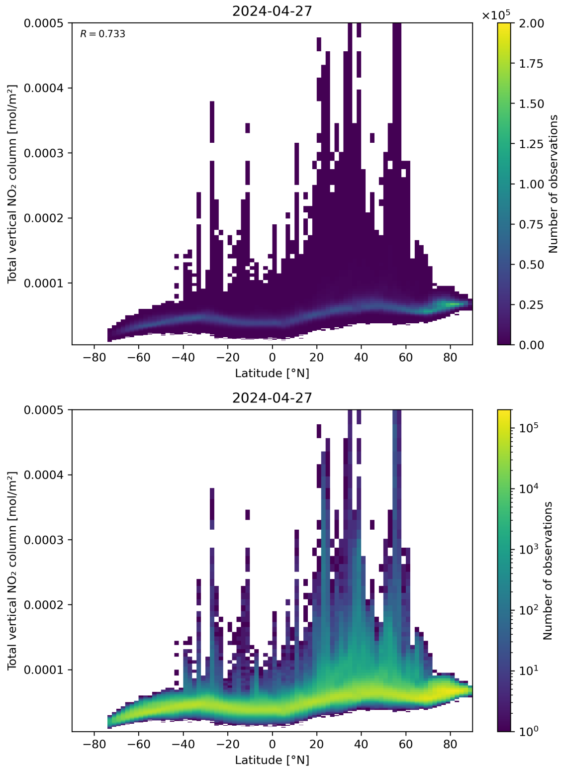
Figure 90: Scatter density plot of “Latitude” against “Total vertical NO 2 column” for 2024-04-26 to 2024-04-28.
