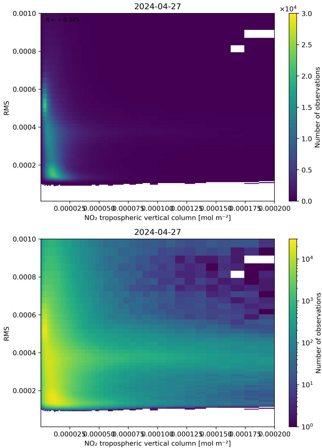
Figure 142: Scatter density plot of “NO 2 tropospheric vertical column” against “RMS” for 2024-04-26 to 2024-04-28.
