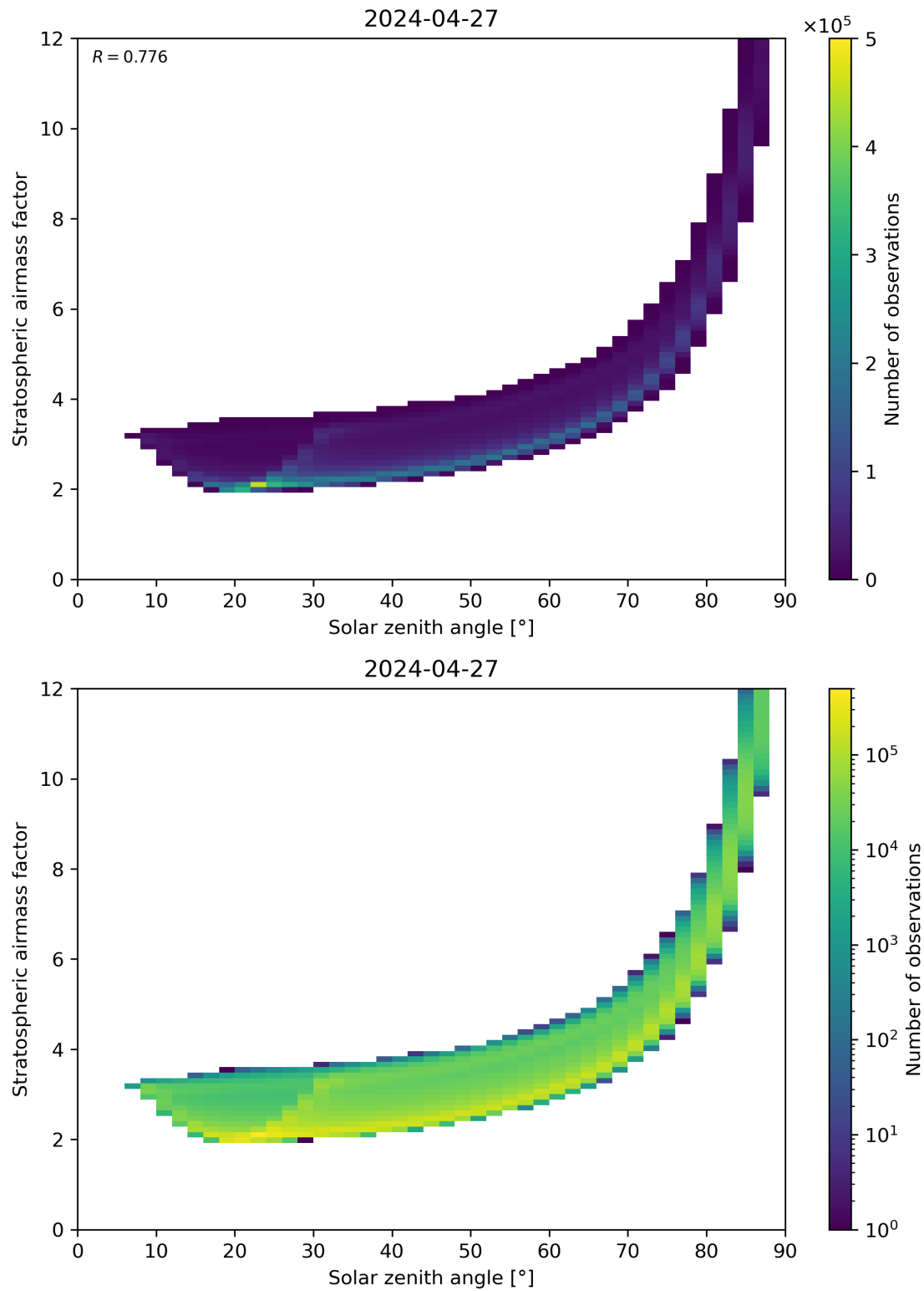
Figure 145: Scatter density plot of “Solar zenith angle” against “Stratospheric airmass factor” for 2024-04-26 to 2024-04-28.
