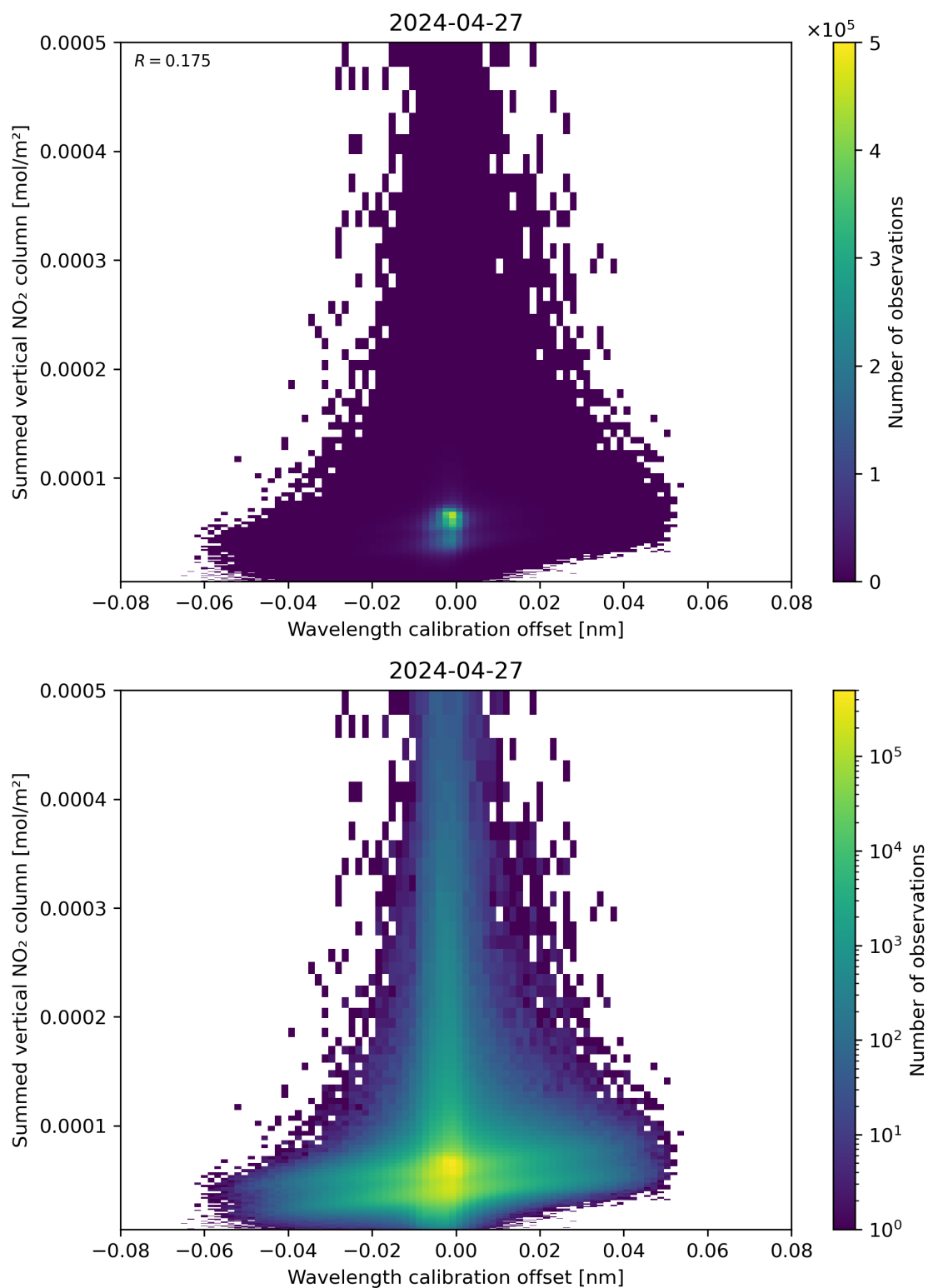
Figure 177: Scatter density plot of “Wavelength calibration offset” against “Summed vertical NO 2 column” for 2024-04-26 to 2024-04-28.
