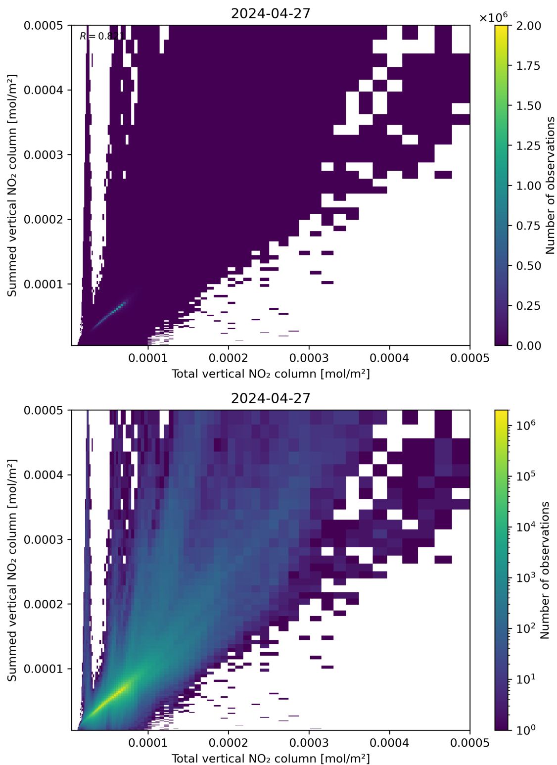
Figure 112: Scatter density plot of “Total vertical NO 2 column” against “Summed vertical NO 2 column” for 2024-04-26 to 2024-04-28.
