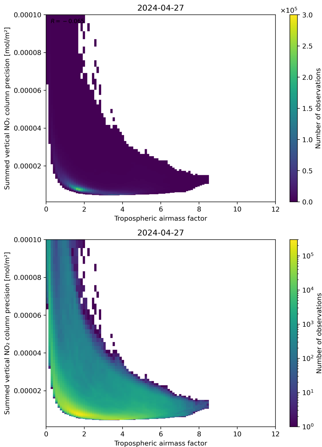
Figure 76: Scatter density plot of “Tropospheric air mass factor” against “Summed vertical NO 2 column precision” for 2024-04-26 to 2024-04-28.
