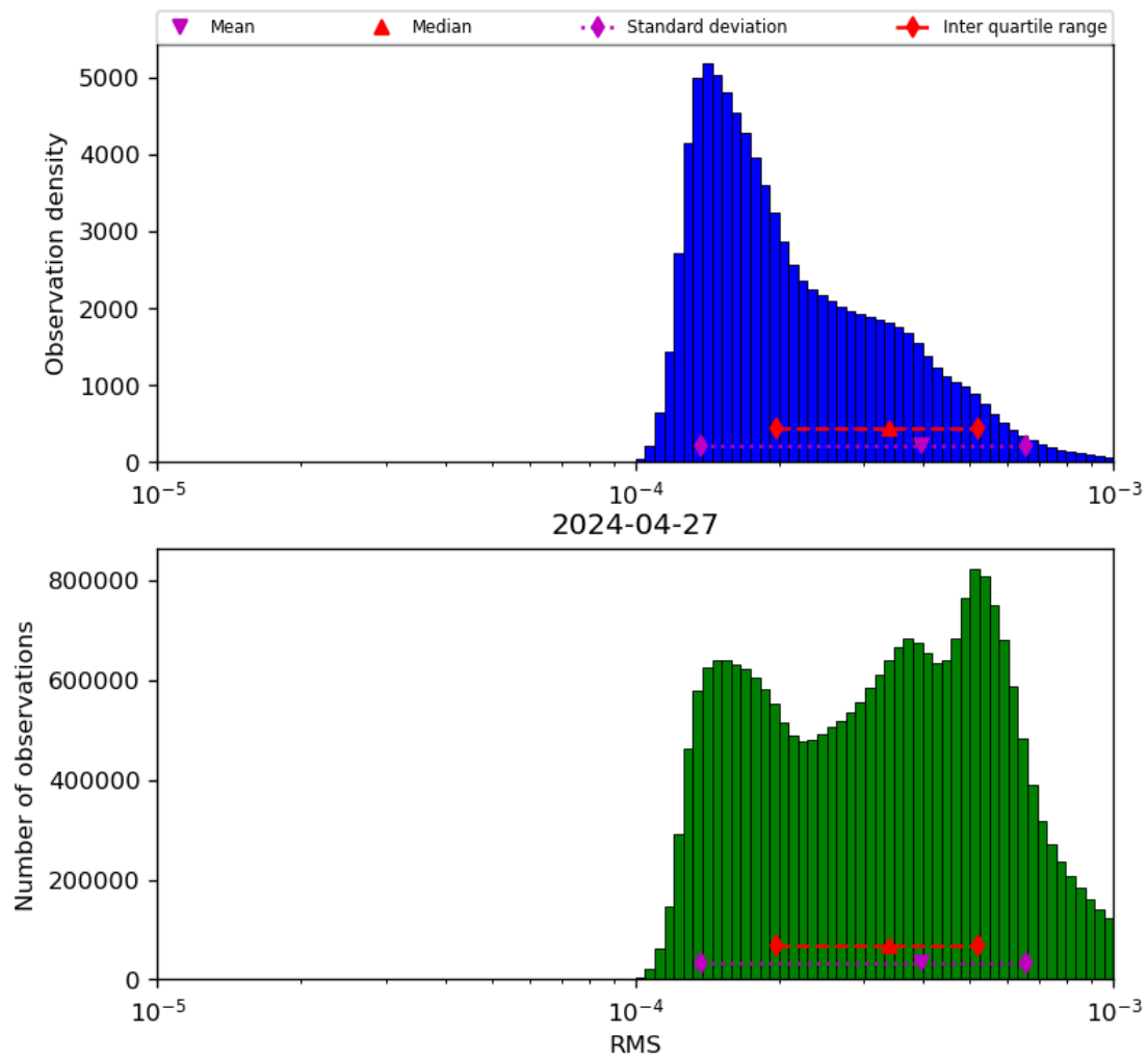
Figure 43: Histogram of “RMS” for 2024-04-26 to 2024-04-28
