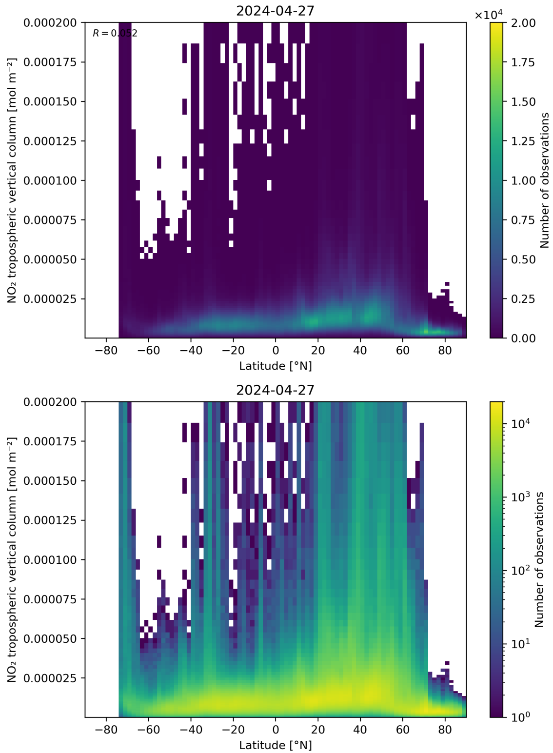
Figure 92: Scatter density plot of “Latitude” against “NO 2 tropospheric vertical column” for 2024-04-26 to 2024-04-28.
