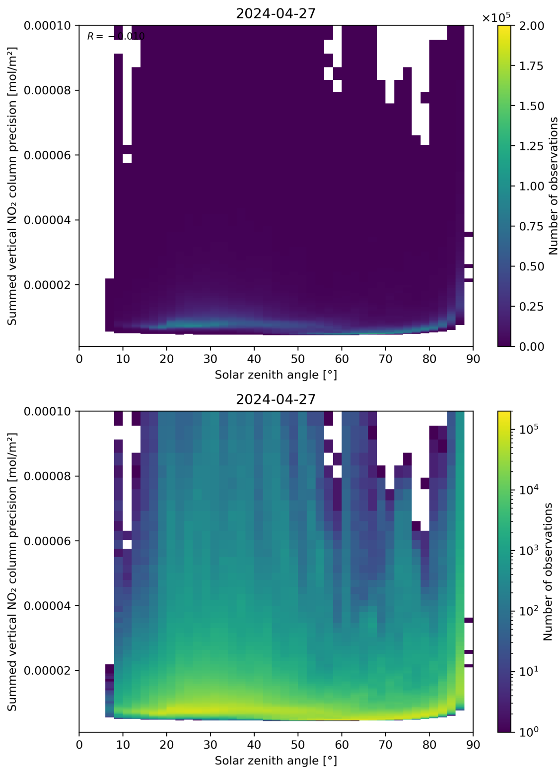
Figure 152: Scatter density plot of “Solar zenith angle” against “Summed vertical NO 2 column precision” for 2024-04-26 to 2024-04-28.
