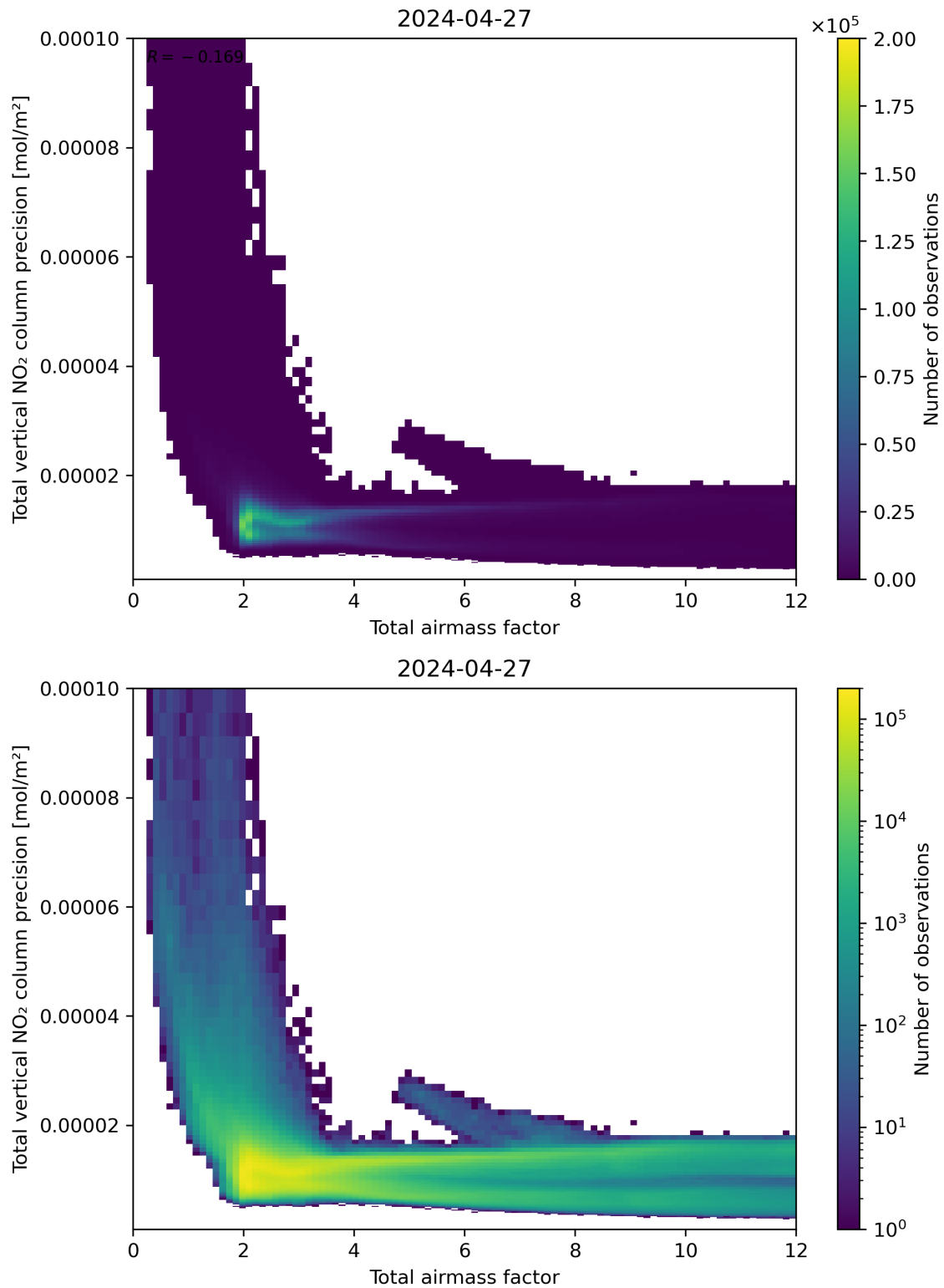
Figure 68: Scatter density plot of “Total airmass factor” against “Total vertical NO 2 column precision” for 2024-04-26 to 2024-04-28.
