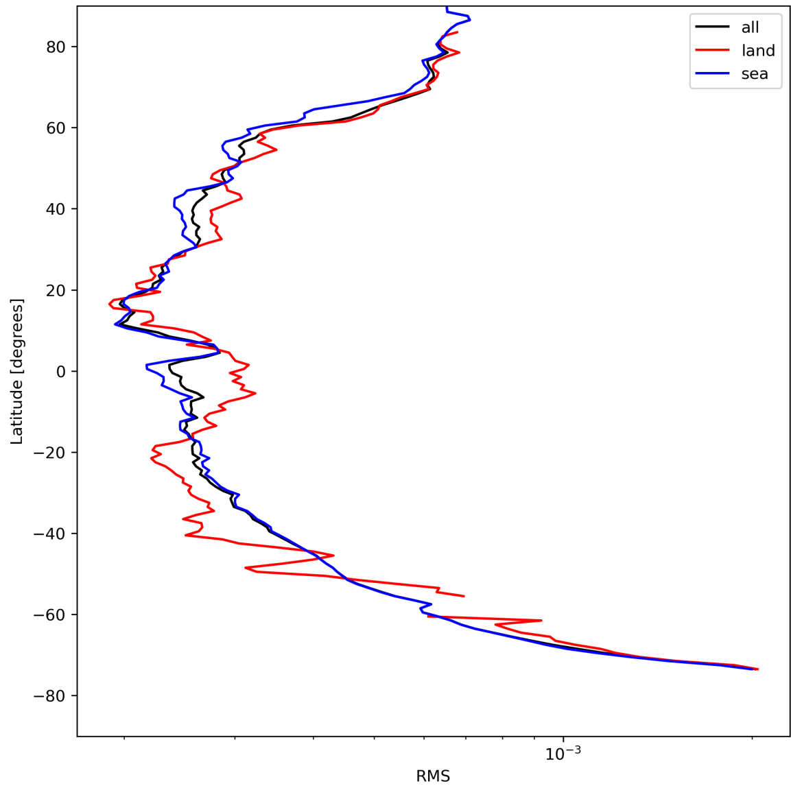
Figure 26: Zonal average of “RMS” for 2024-04-26 to 2024-04-28.
