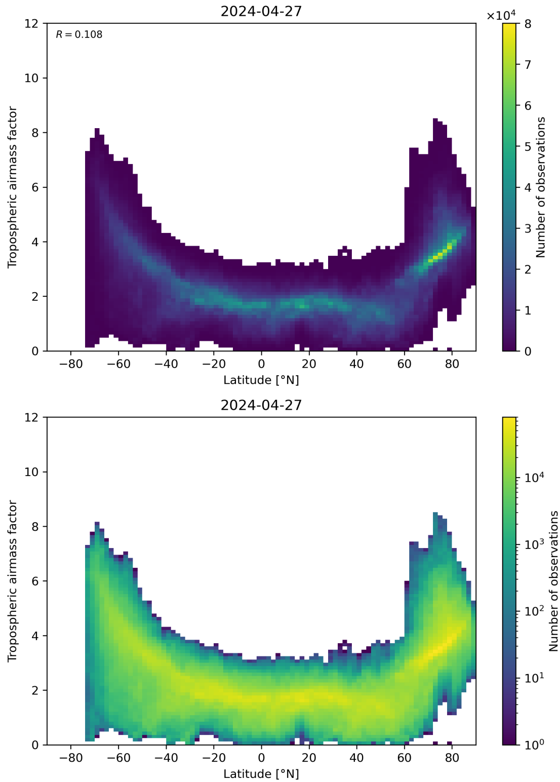
Figure 85: Scatter density plot of “Latitude” against “Tropospheric airmass factor” for 2024-04-26 to 2024-04-28.
