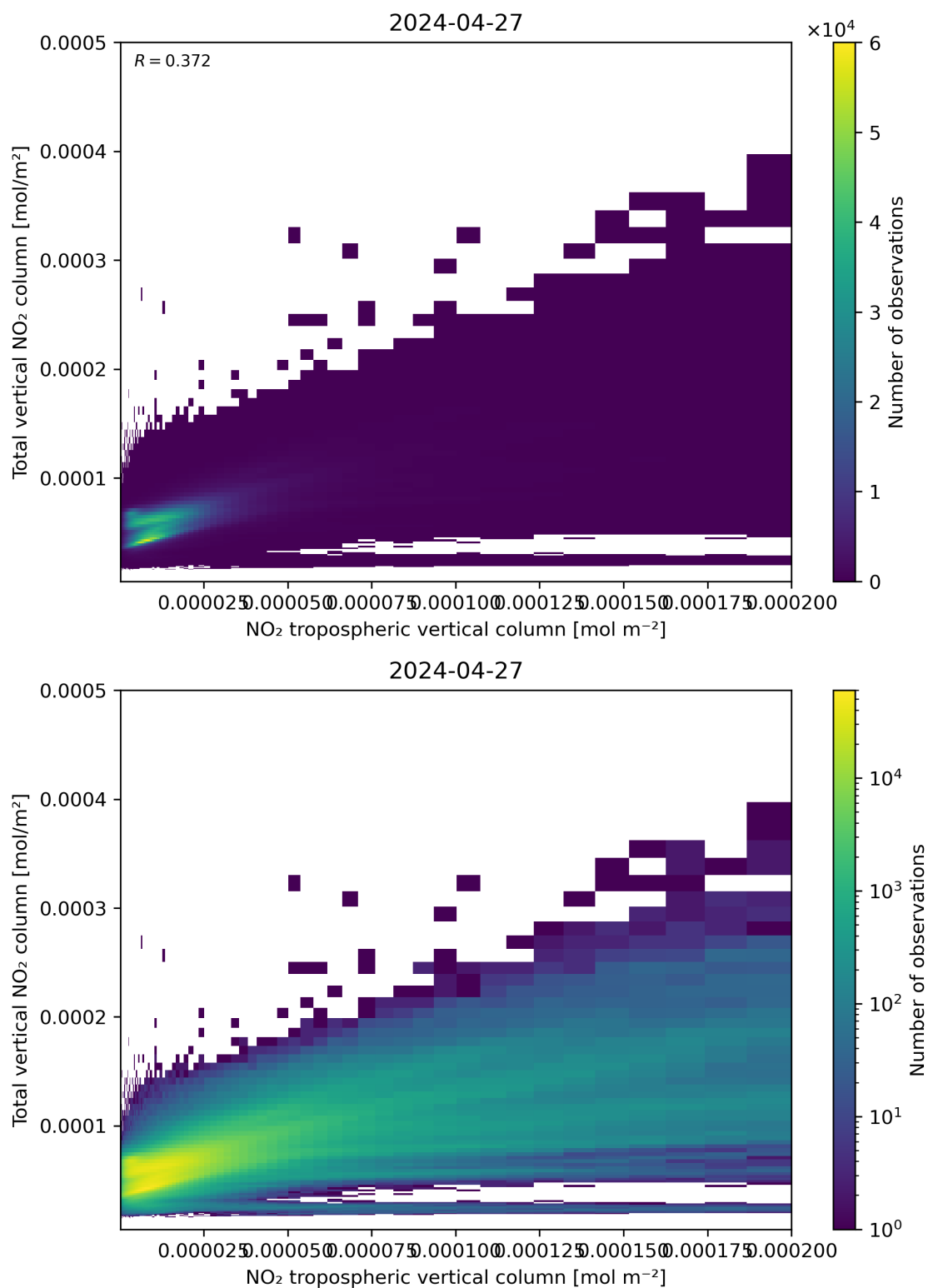
Figure 128: Scatter density plot of “NO 2 tropospheric vertical column” against “Total vertical NO 2 column” for 2024-04-26 to 2024-04-28.
