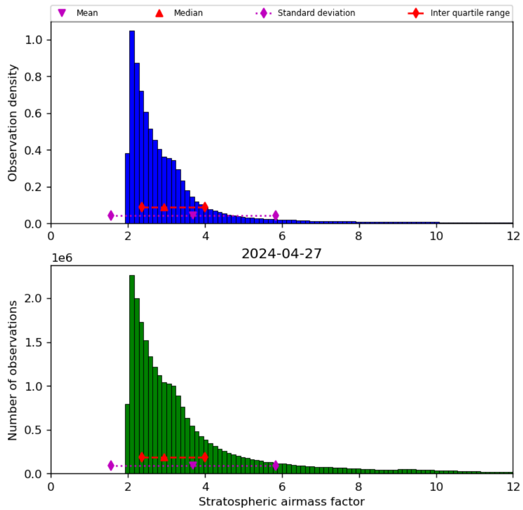
Figure 44: Histogram of “Stratospheric airmass factor” for 2024-04-26 to 2024-04-28
