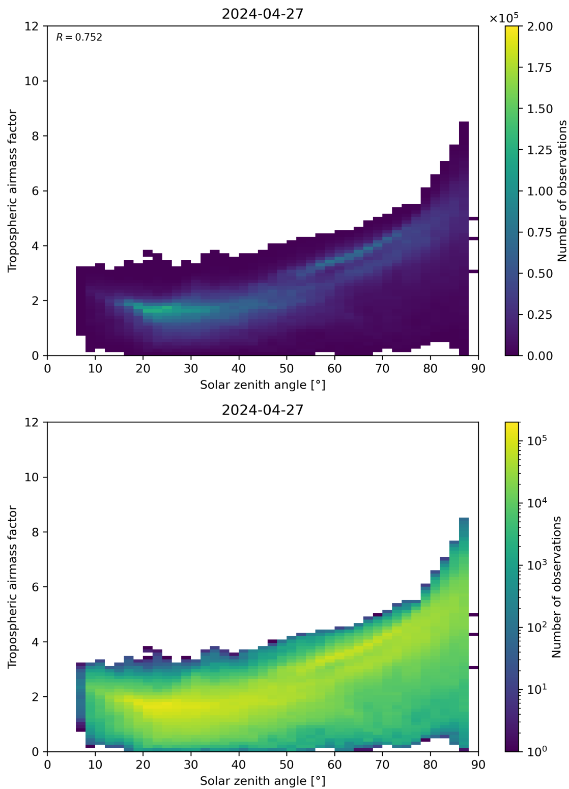
Figure 147: Scatter density plot of “Solar zenith angle” against “Tropospheric airmass factor” for 2024-04-26 to 2024-04-28.
