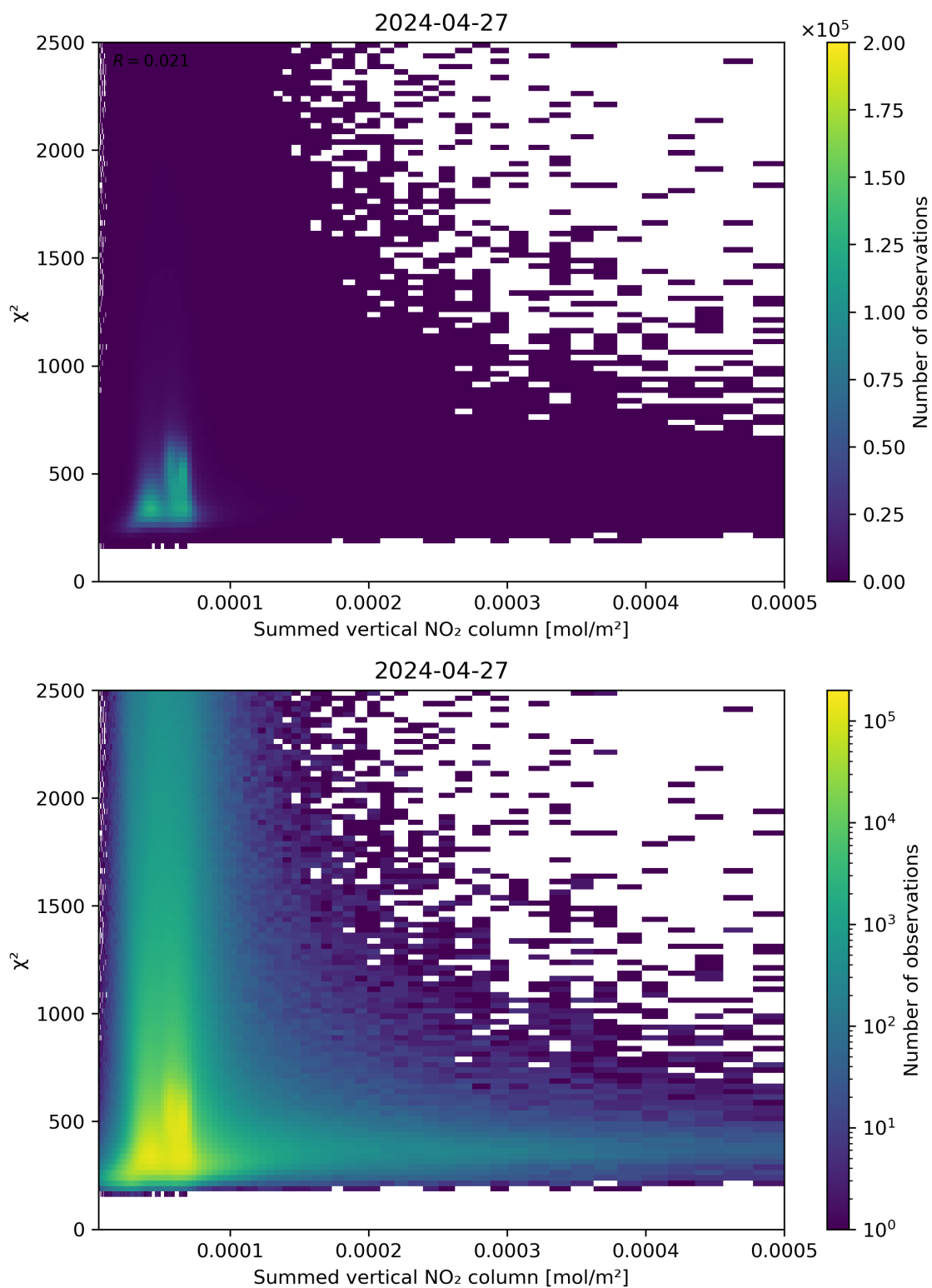
Figure 104: Scatter density plot of “Summed vertical NO 2 column” against “ \chi^2 ” for 2024-04-26 to 2024-04-28.
