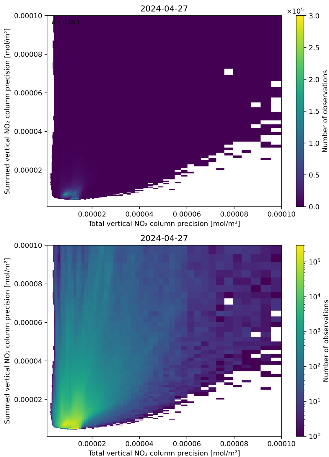
Figure 118: Scatter density plot of “Total vertical NO 2 column precision” against “Summed vertical NO 2 column precision” for 2024-04-26 to 2024-04-28.
