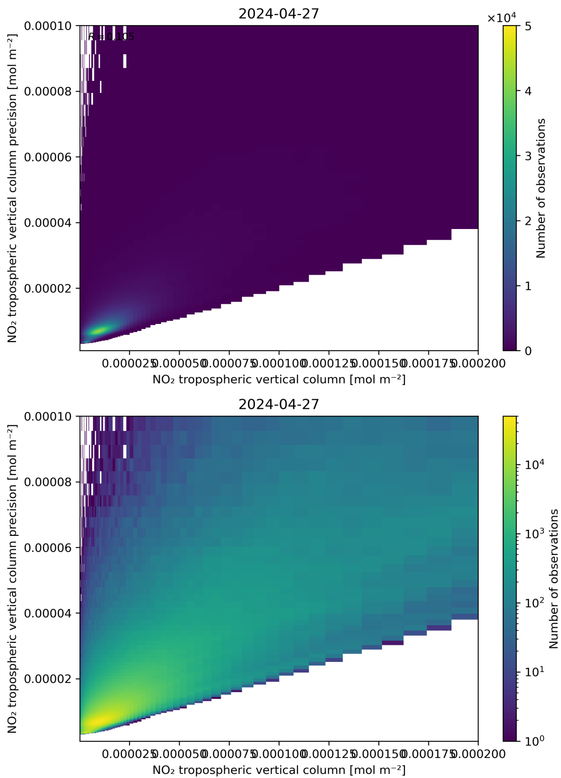
Figure 130: Scatter density plot of “NO 2 tropospheric vertical column” against “NO 2 tropospheric vertical column precision” for 2024-04-26 to 2024-04-28.
