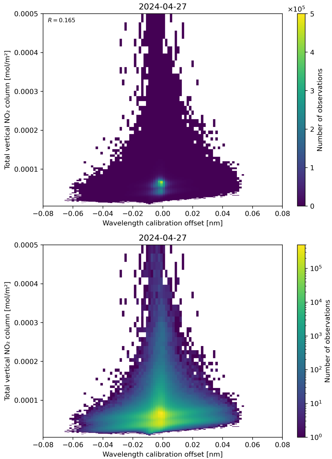
Figure 179: Scatter density plot of “Wavelength calibration offset” against “Total vertical NO 2 column” for 2024-04-26 to 2024-04-28.
