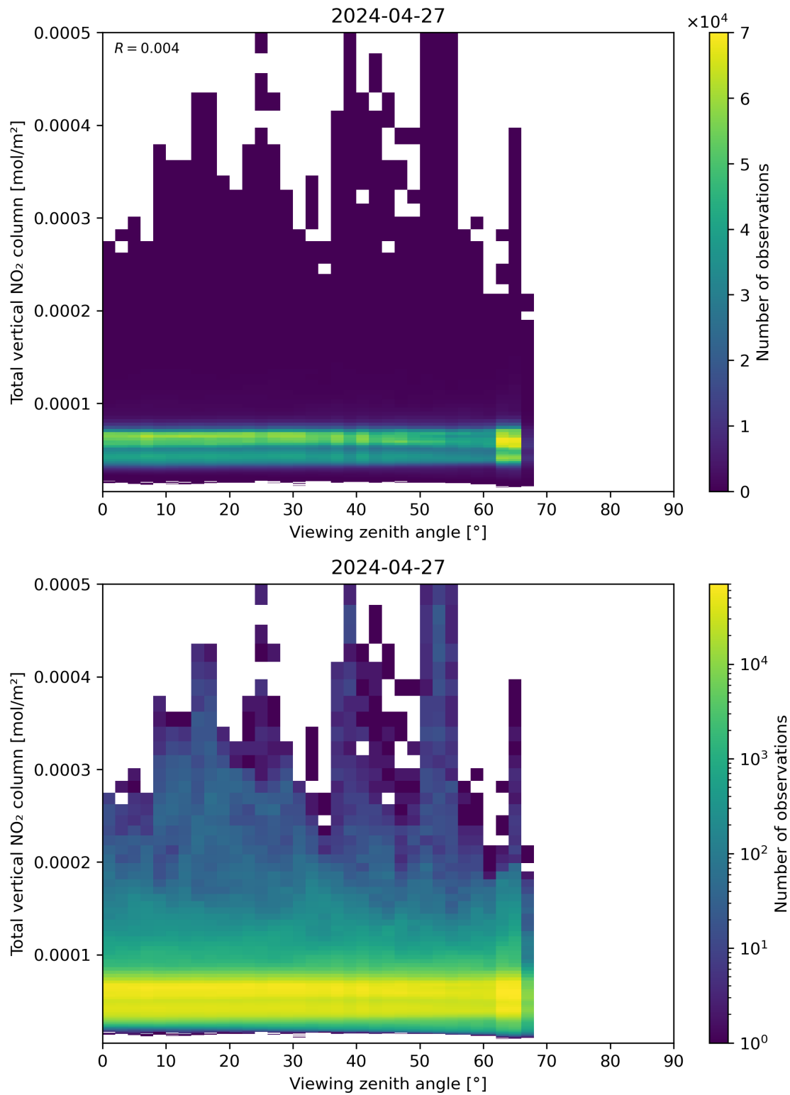
Figure 167: Scatter density plot of “Viewing zenith angle” against “Total vertical NO 2 column” for 2024-04-26 to 2024-04-28.
