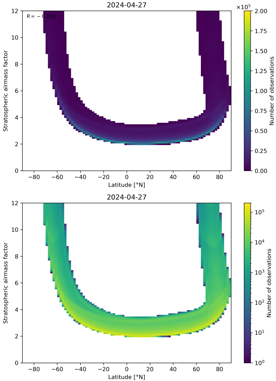
Figure 83: Scatter density plot of “Latitude” against “Stratospheric airmass factor” for 2024-04-26 to 2024-04-28.
