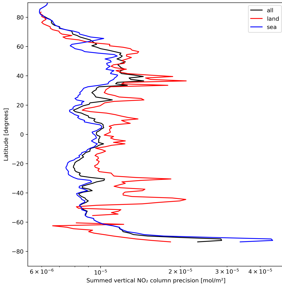
Figure 24: Zonal average of “Summed vertical NO 2 column precision” for 2024-04-26 to 2024-04-28.
