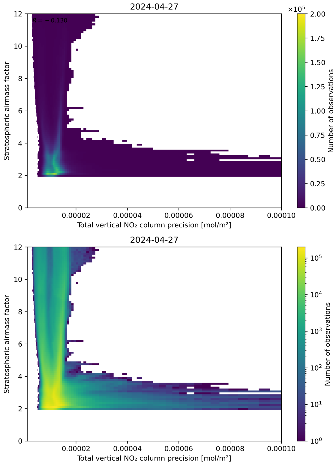
Figure 115: Scatter density plot of “Total vertical NO 2 column precision” against “Stratospheric air mass factor” for 2024-04-26 to 2024-04-28.
