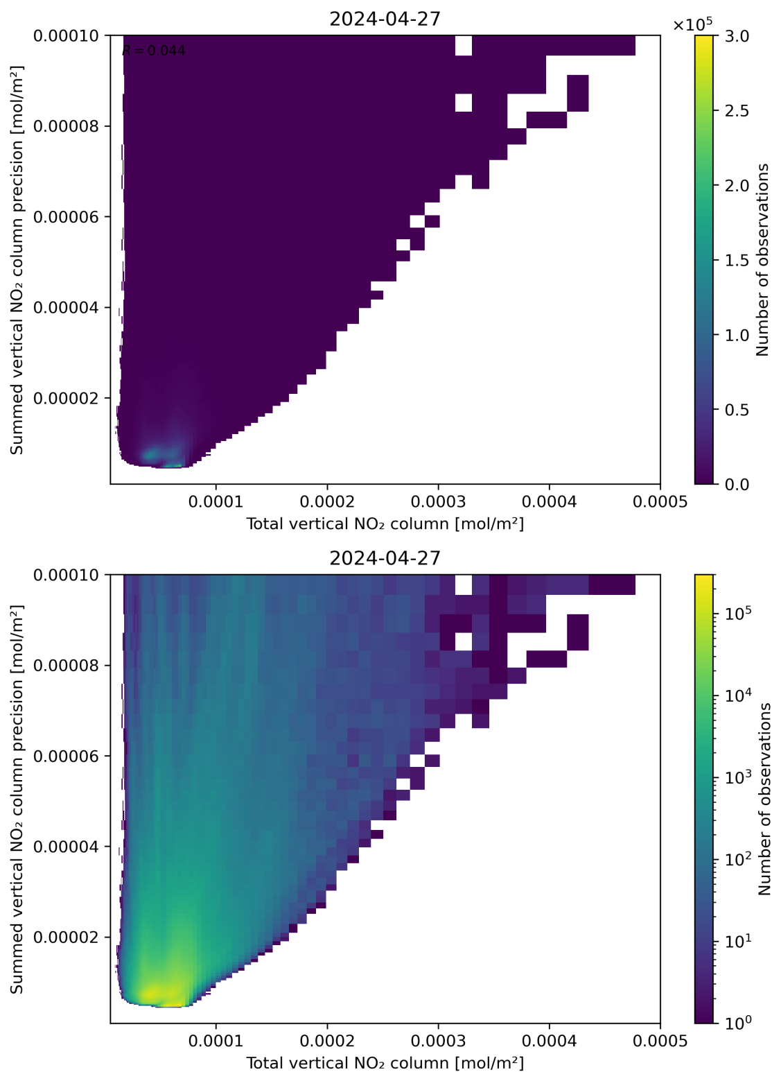
Figure 113: Scatter density plot of “Total vertical NO 2 column” against “Summed vertical NO 2 column precision” for 2024-04-26 to 2024-04-28.
