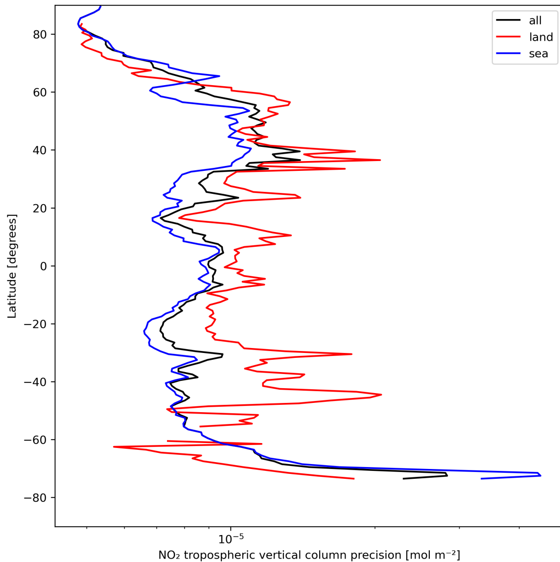
Figure 13: Zonal average of “NO 2 tropospheric vertical column precision” for 2024-04-26 to 2024-04-28.
