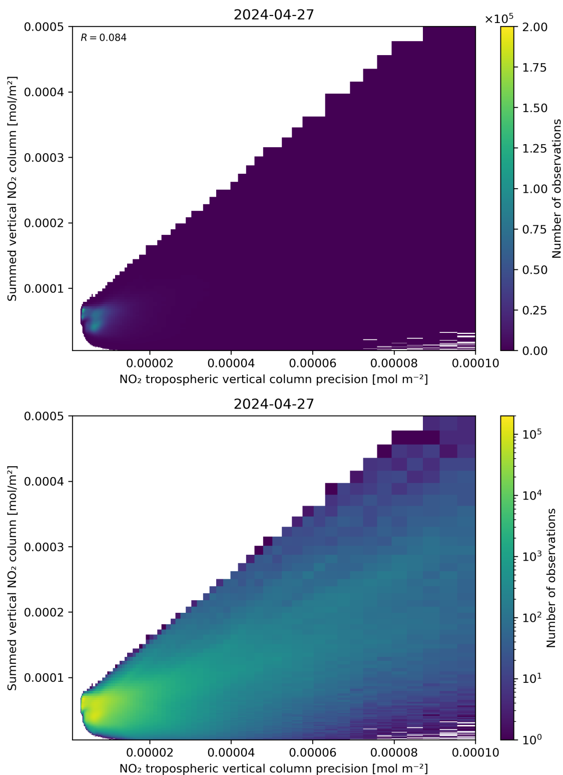
Figure 136: Scatter density plot of “NO 2 tropospheric vertical column precision” against “Summed vertical NO 2 column” for 2024-04-26 to 2024-04-28.
