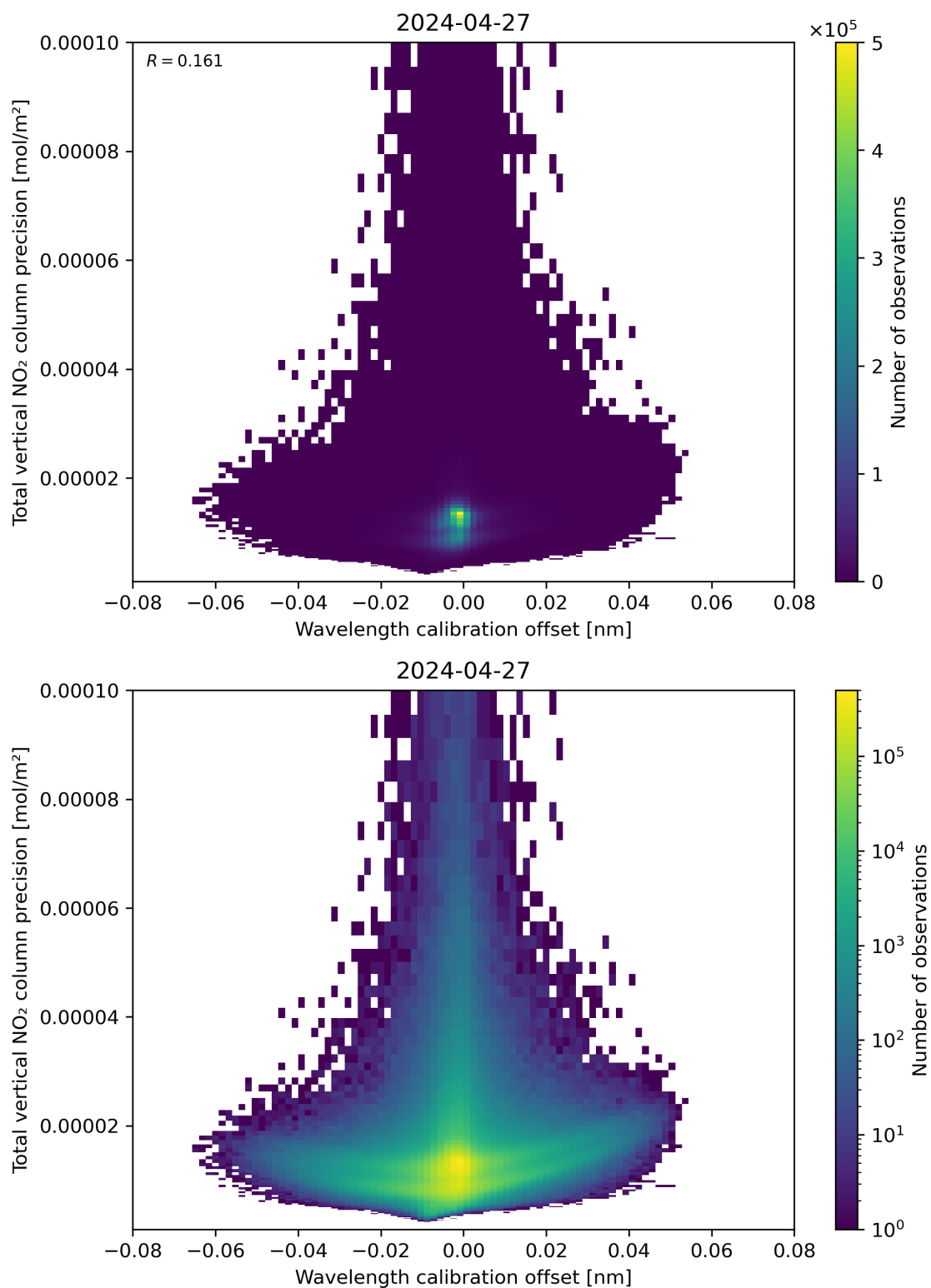
Figure 180: Scatter density plot of “Wavelength calibration offset” against “Total vertical NO 2 column precision” for 2024-04-26 to 2024-04-28.
