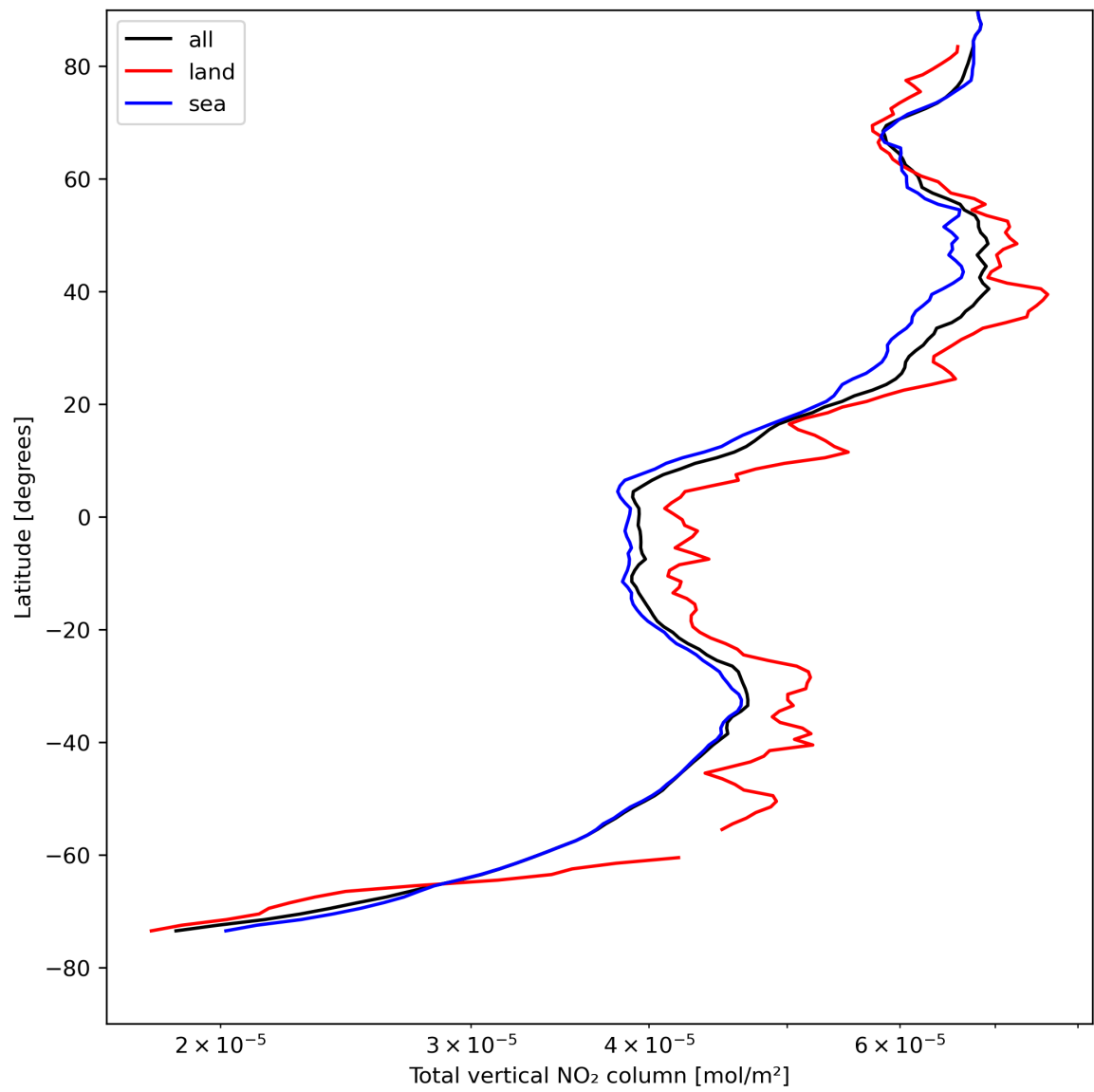
Figure 21: Zonal average of “Total vertical NO 2 column” for 2024-04-26 to 2024-04-28.
