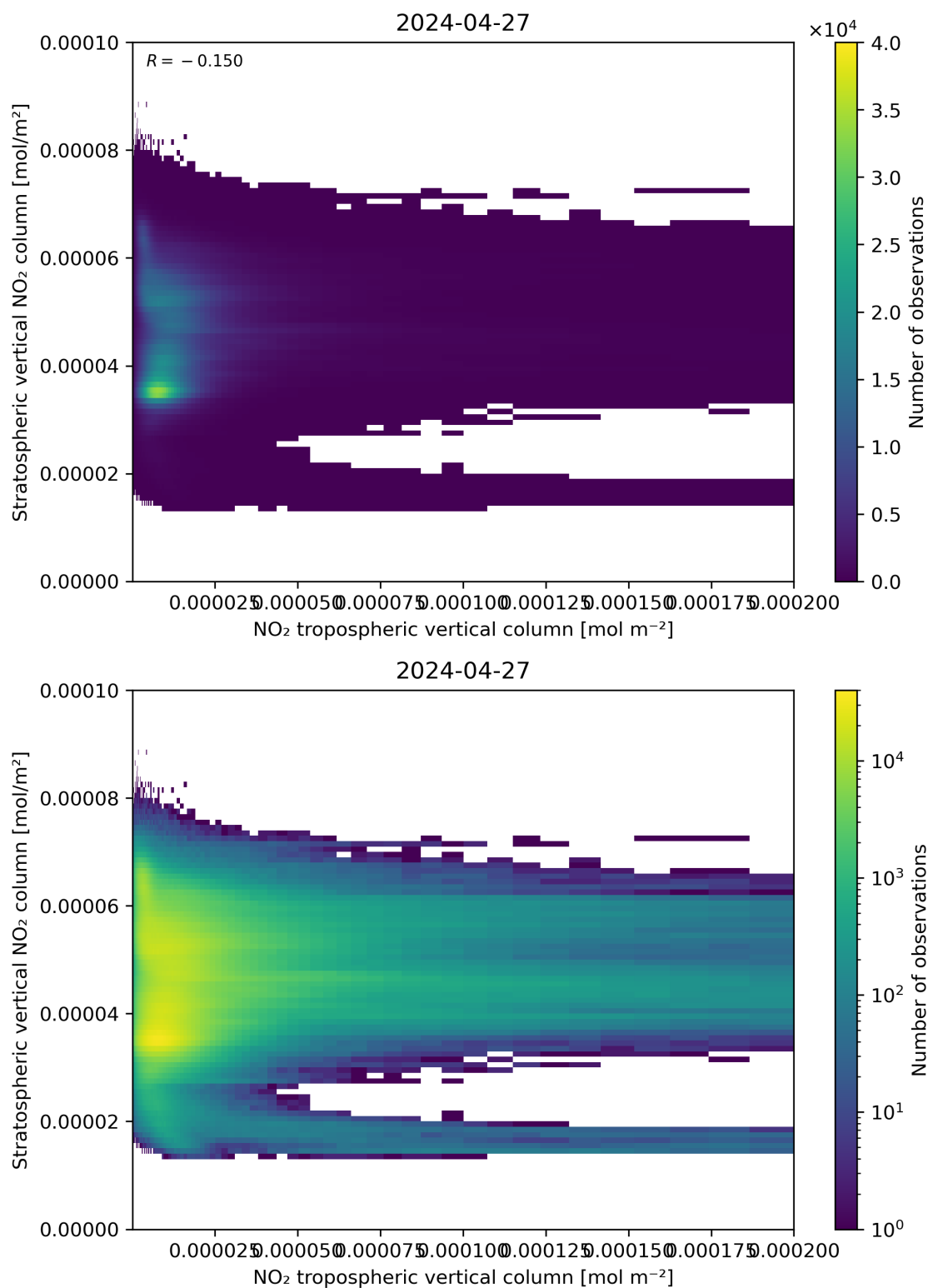
Figure 125: Scatter density plot of “NO 2 tropospheric vertical column” against “Stratospheric vertical NO 2 column” for 2024-04-26 to 2024-04-28.
