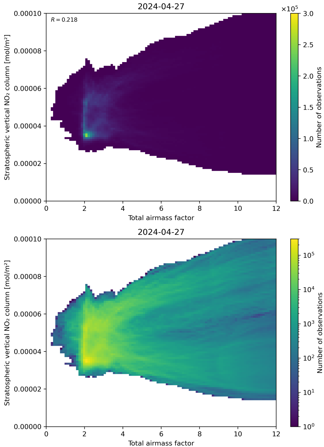
Figure 64: Scatter density plot of “Total airmass factor” against “Stratospheric vertical NO 2 column” for 2024-04-26 to 2024-04-28.
