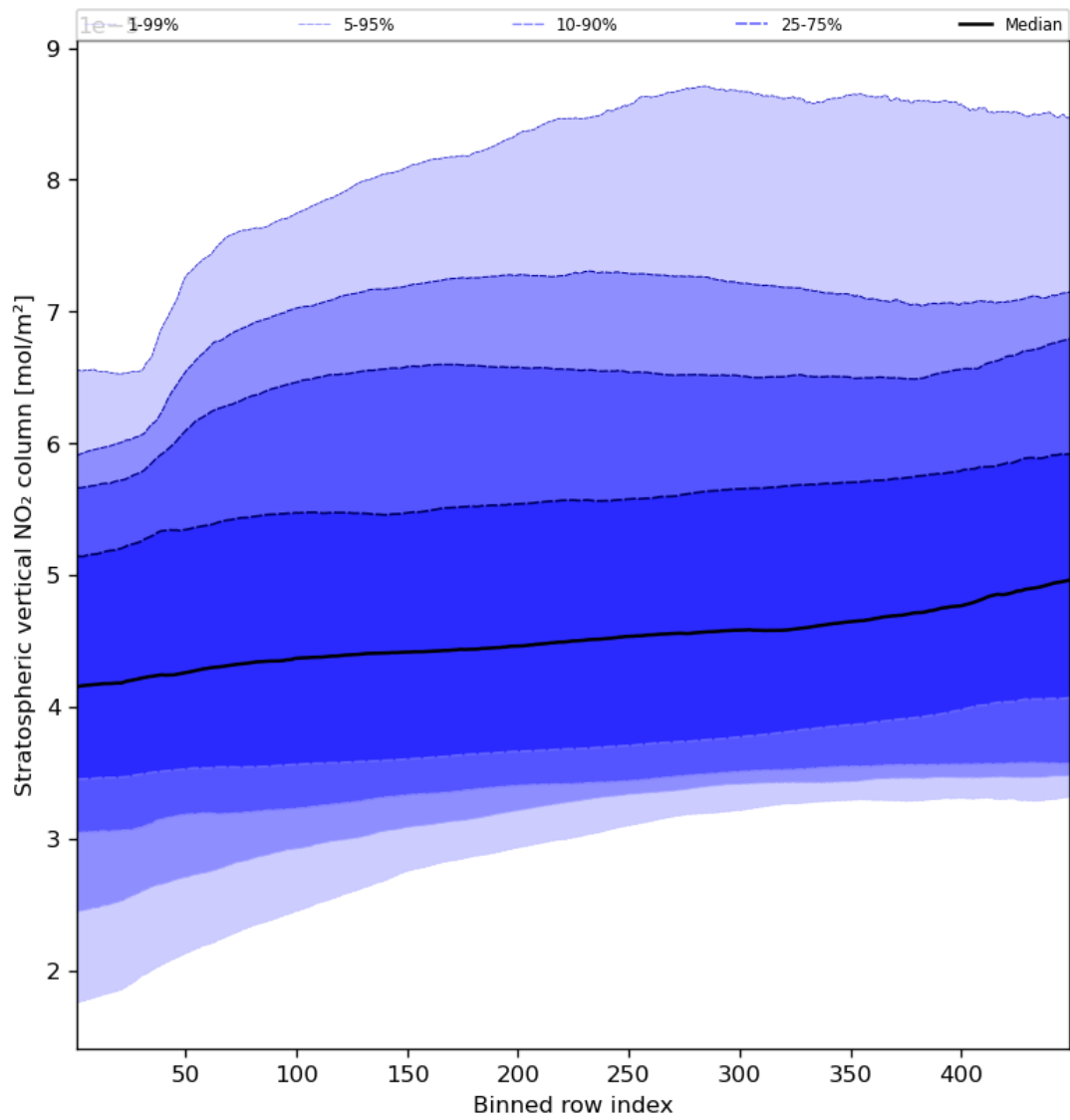
Figure 53: Along track statistics of “Stratospheric vertical NO 2 column” for 2024-04-26 to 2024-04-28
