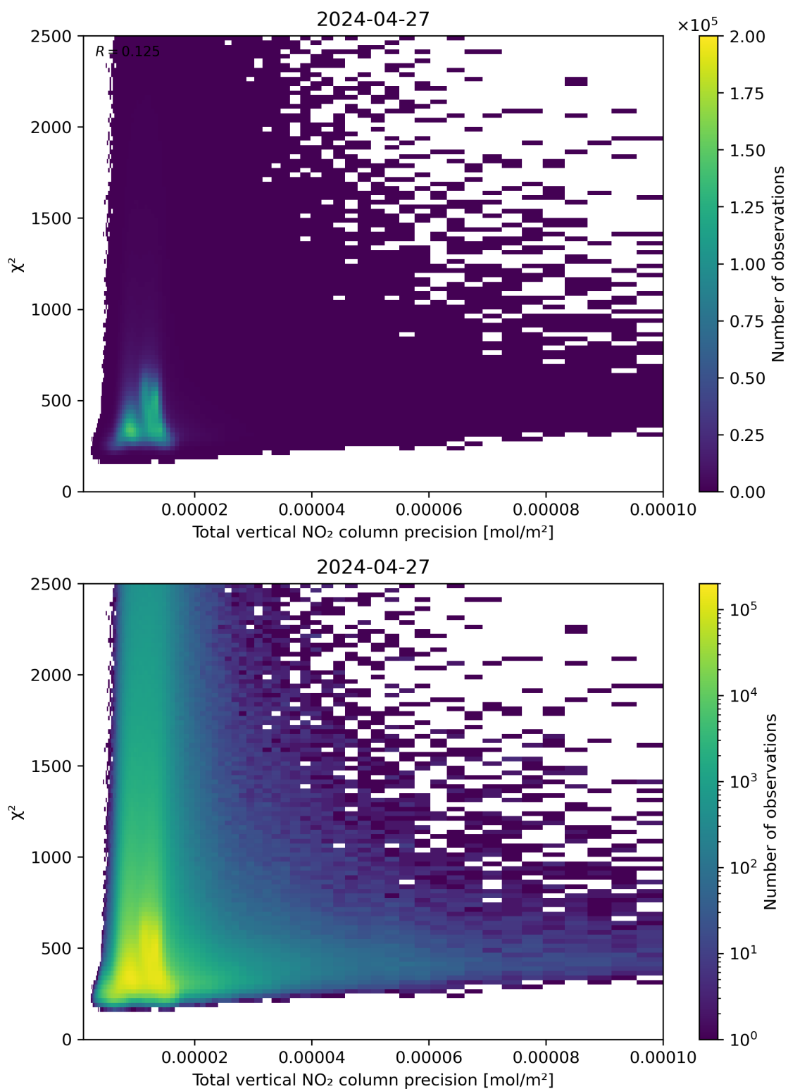
Figure 116: Scatter density plot of “Total vertical NO 2 column precision” against “ \chi^2 ” for 2024-04-26 to 2024-04-28.
