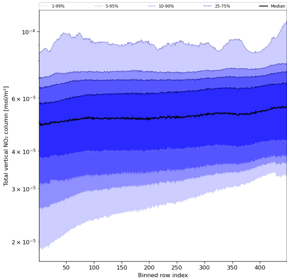
Figure 55: Along track statistics of “Total vertical NO 2 column” for 2024-04-26 to 2024-04-28
