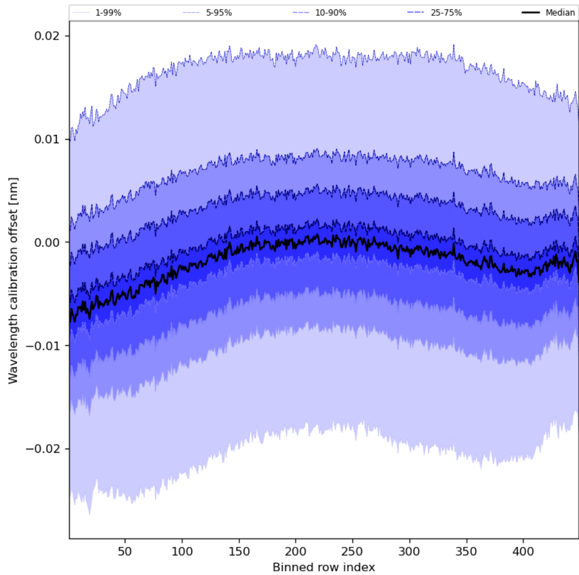
Figure 52: Along track statistics of “Wavelength calibration offset” for 2024-04-26 to 2024-04-28
