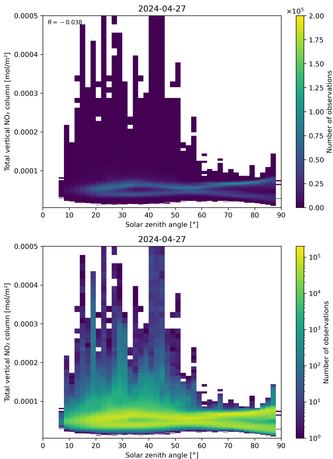
Figure 153: Scatter density plot of “Solar zenith angle” against “Total vertical NO 2 column” for 2024-04-26 to 2024-04-28.
