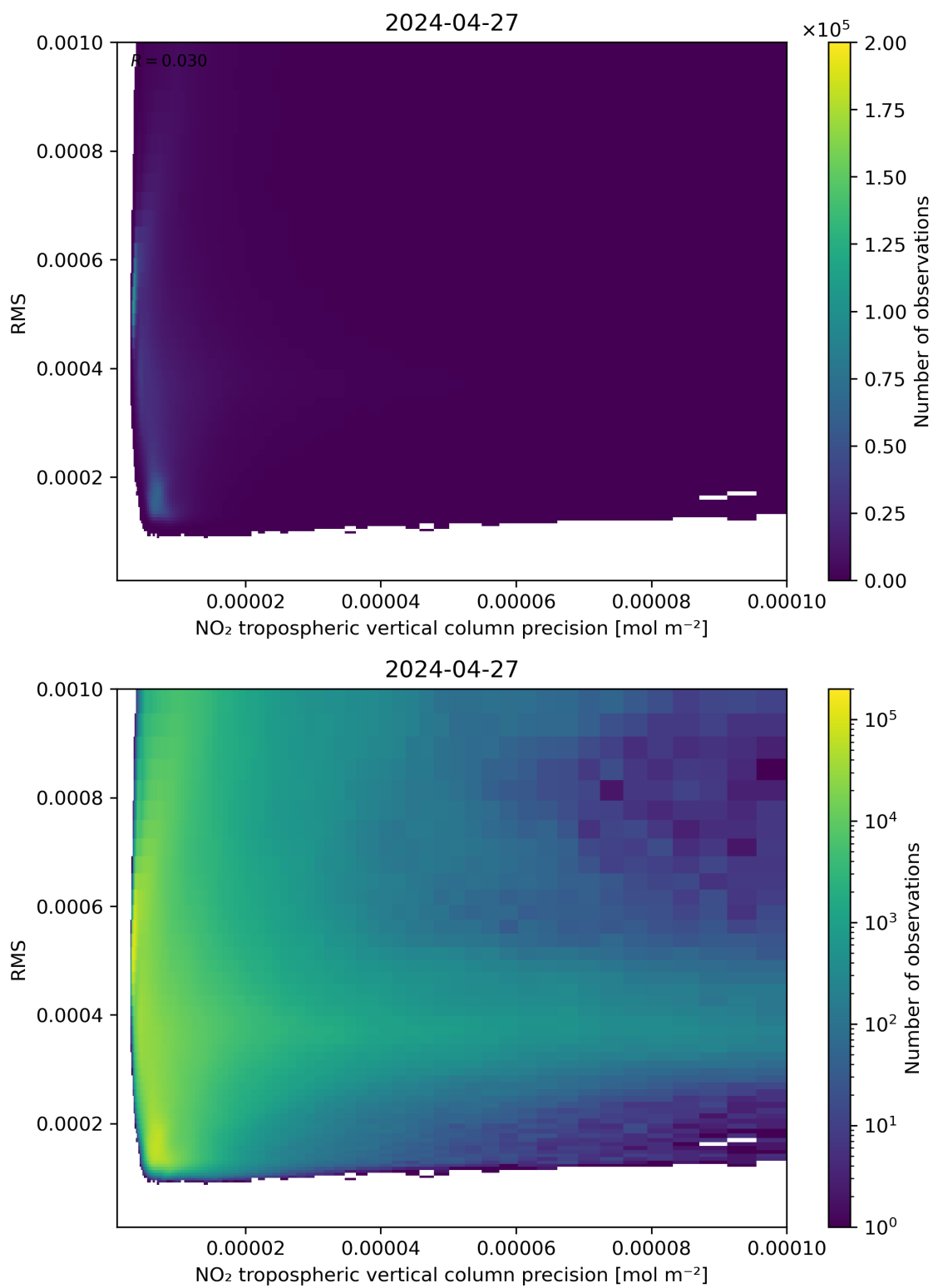
Figure 140: Scatter density plot of “NO 2 tropospheric vertical column precision” against “RMS” for 2024-04-26 to 2024-04-28.
