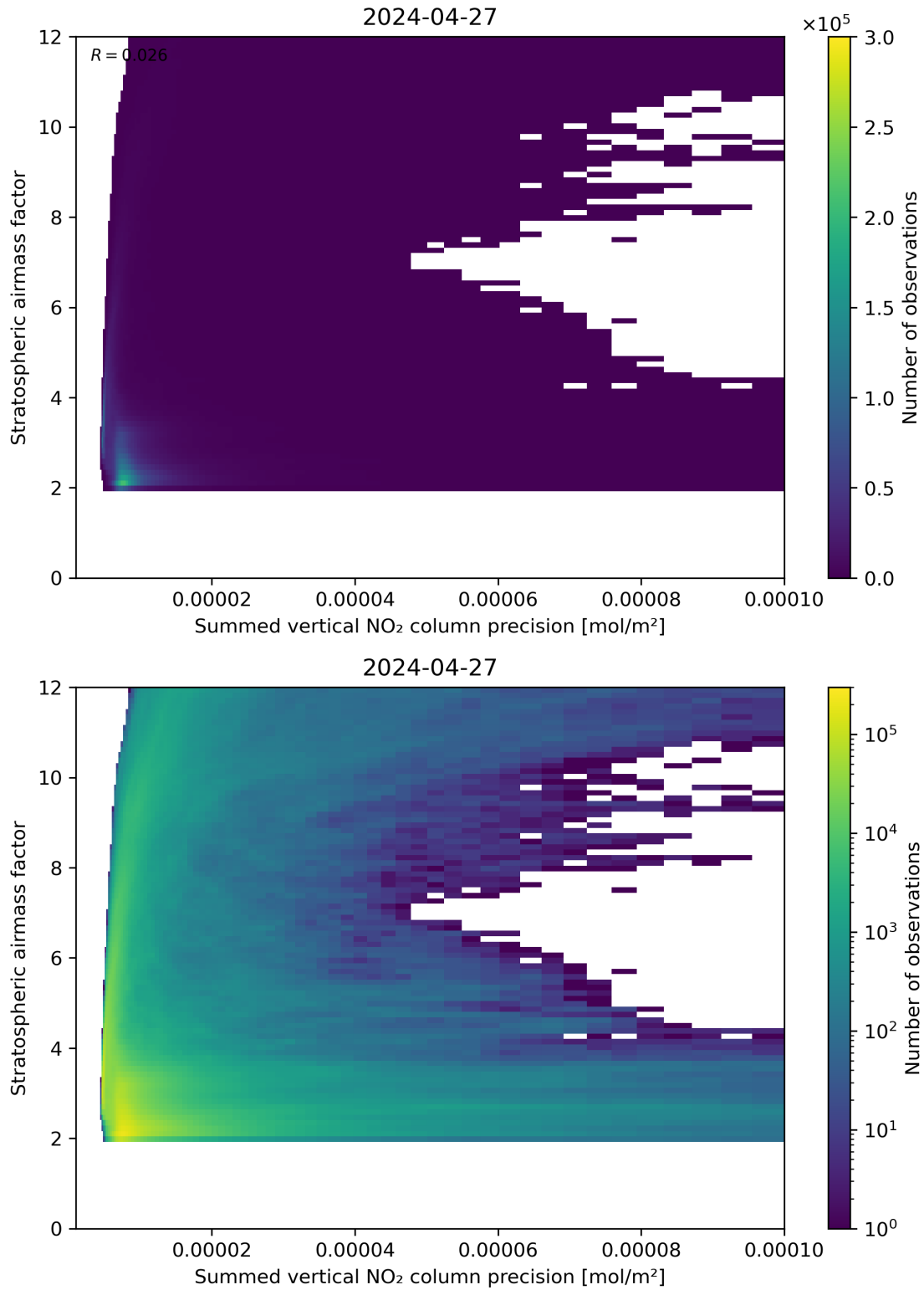
Figure 106: Scatter density plot of “Summed vertical NO 2 column precision” against “Stratospheric airmass factor” for 2024-04-26 to 2024-04-28.
