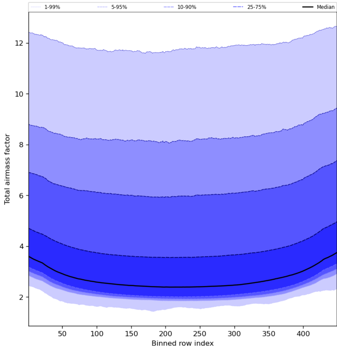
Figure 49: Along track statistics of “Total airmass factor” for 2024-04-26 to 2024-04-28
