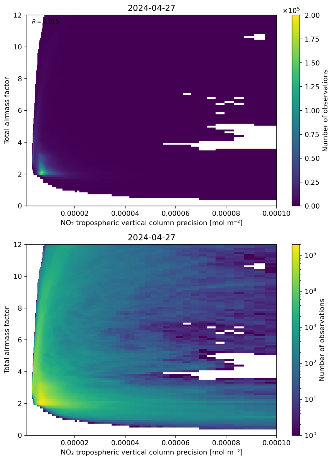
Figure 132: Scatter density plot of “NO 2 tropospheric vertical column precision” against “Total air mass factor” for 2024-04-26 to 2024-04-28.
