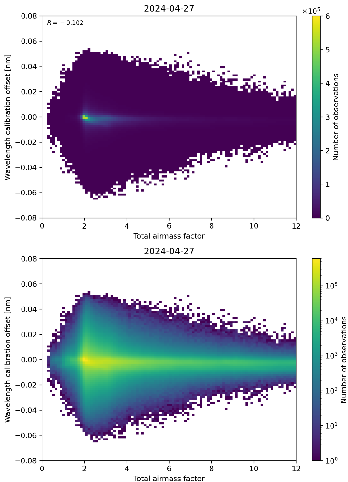
Figure 70: Scatter density plot of “Total airmass factor” against “Wavelength calibration offset” for 2024-04-26 to 2024-04-28.
