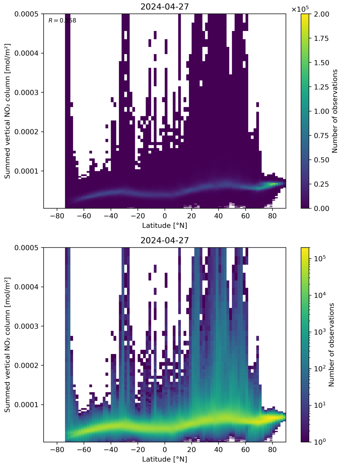
Figure 88: Scatter density plot of “Latitude” against “Summed vertical NO 2 column” for 2024-04-26 to 2024-04-28.
