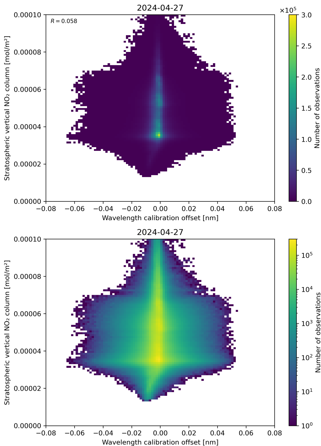
Figure 176: Scatter density plot of “Wavelength calibration offset” against “Stratospheric vertical NO 2 column” for 2024-04-26 to 2024-04-28.
