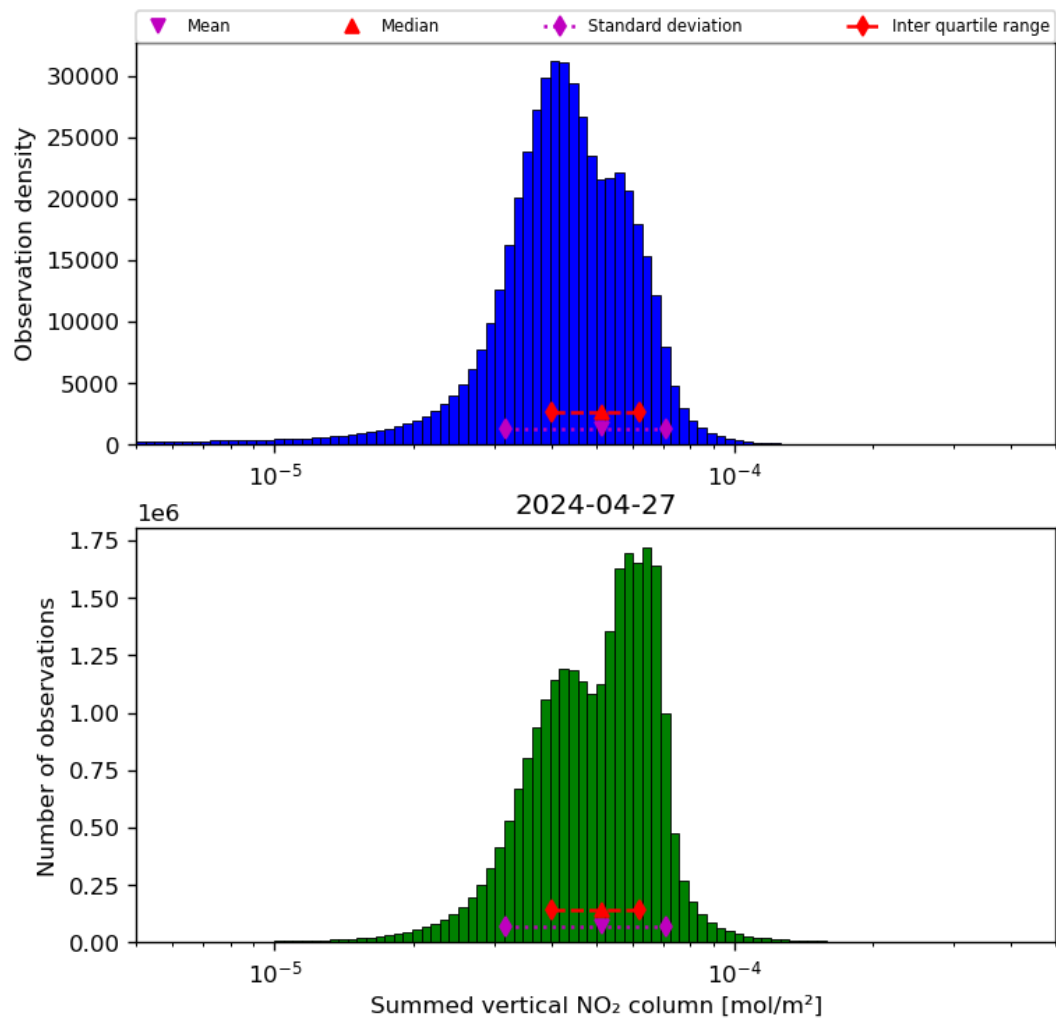
Figure 40: Histogram of “Summed vertical NO 2 column” for 2024-04-26 to 2024-04-28
