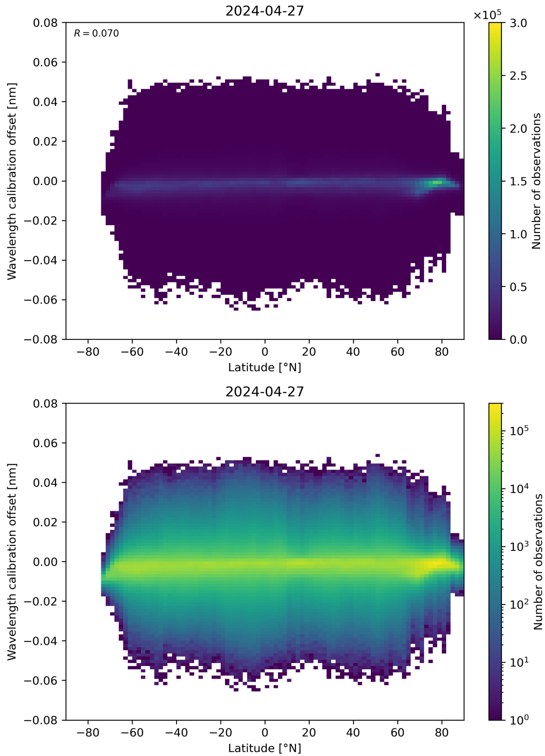
Figure 95: Scatter density plot of “Latitude” against “Wavelength calibration offset” for 2024-04-26 to 2024-04-28.
