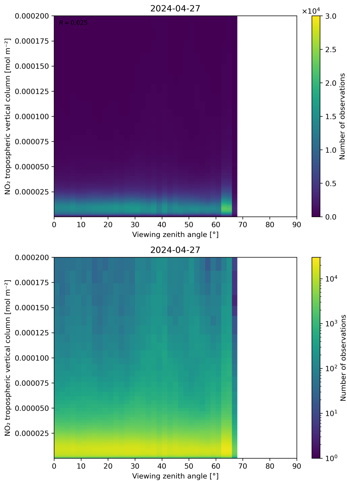
Figure 169: Scatter density plot of “Viewing zenith angle” against “NO 2 tropospheric vertical column” for 2024-04-26 to 2024-04-28.
