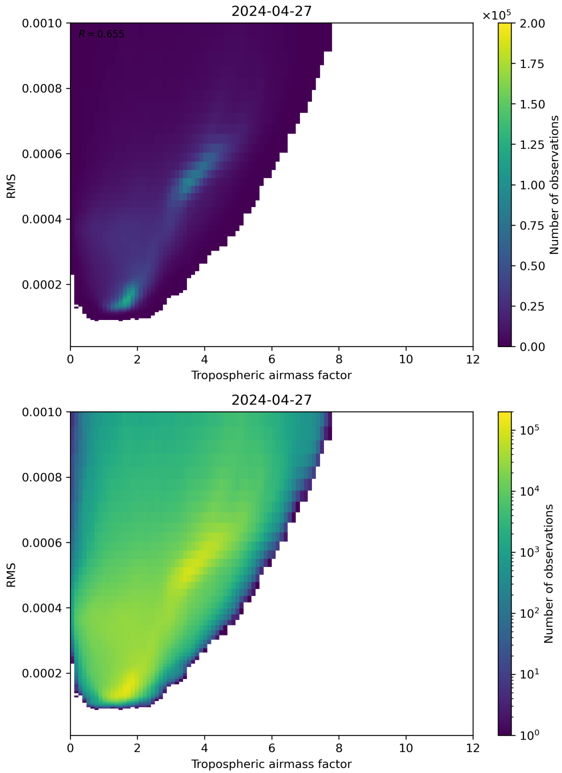
Figure 79: Scatter density plot of “Tropospheric airmass factor” against “RMS” for 2024-04-26 to 2024-04-28.
