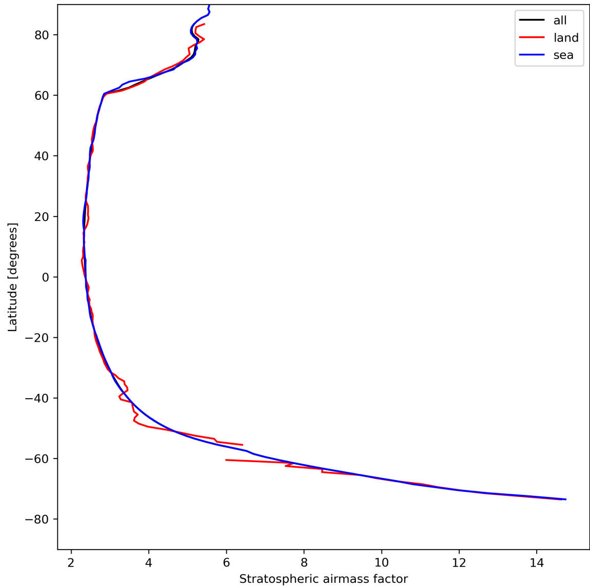
Figure 27: Zonal average of “Stratospheric air mass factor” for 2024-04-26 to 2024-04-28.
