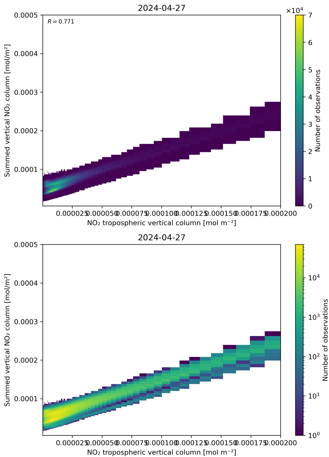
Figure 126: Scatter density plot of “NO 2 tropospheric vertical column” against “Summed vertical NO 2 column” for 2024-04-26 to 2024-04-28.
