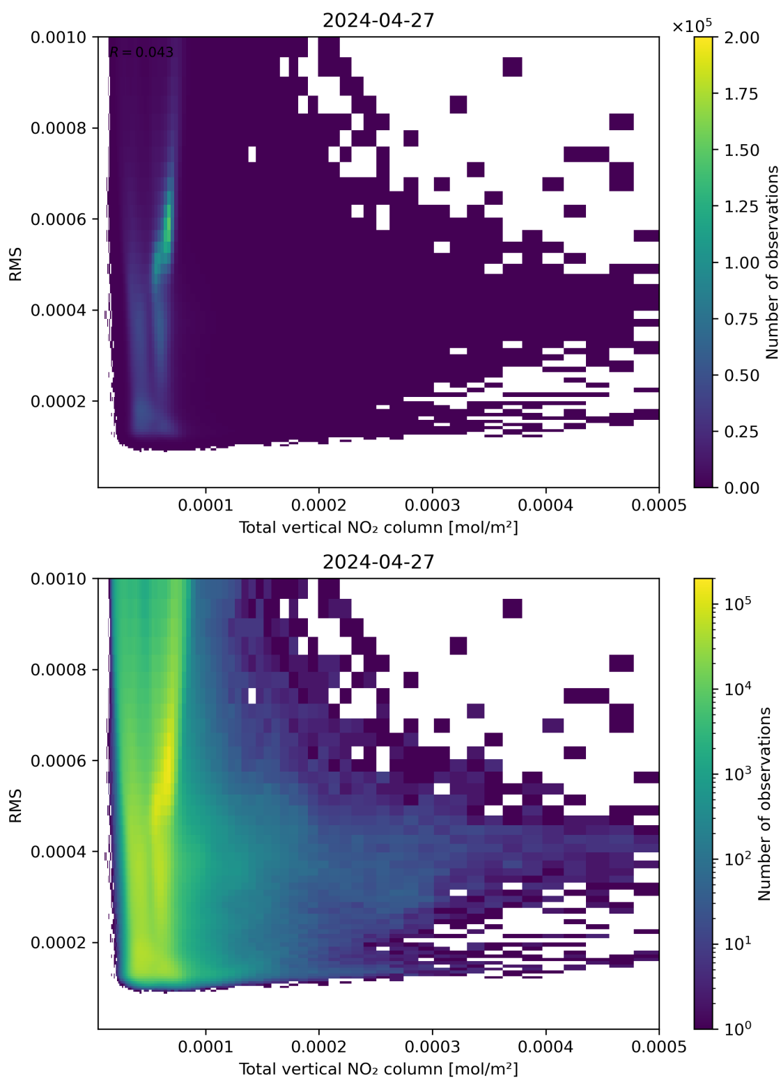
Figure 120: Scatter density plot of “Total vertical NO 2 column” against “RMS” for 2024-04-26 to 2024-04-28.
