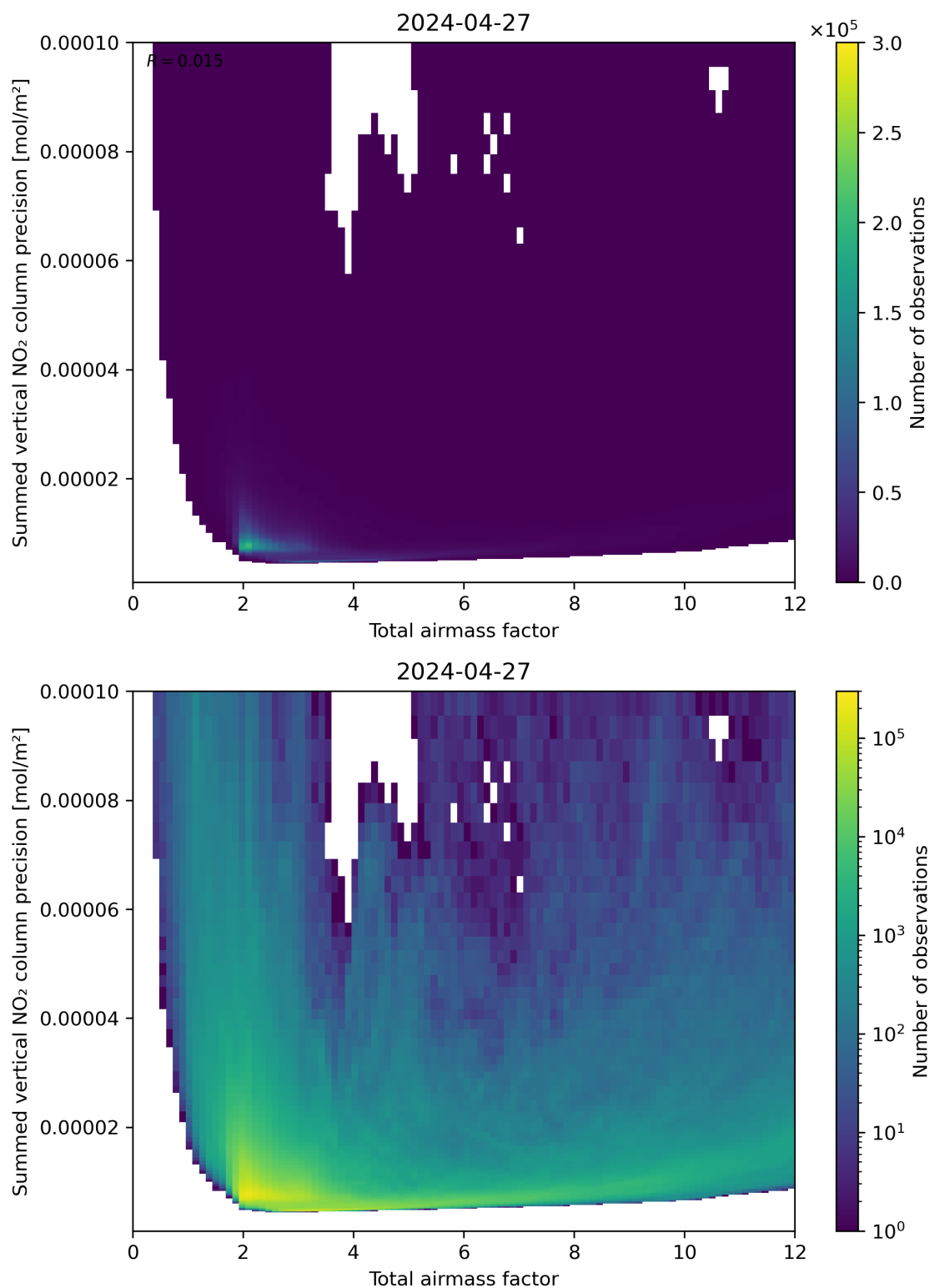
Figure 66: Scatter density plot of “Total airmass factor” against “Summed vertical NO 2 column precision” for 2024-04-26 to 2024-04-28.
