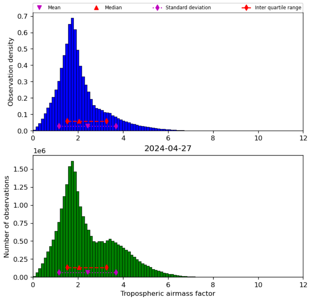
Figure 31: Histogram of “Tropospheric airmass factor” for 2024-04-26 to 2024-04-28
