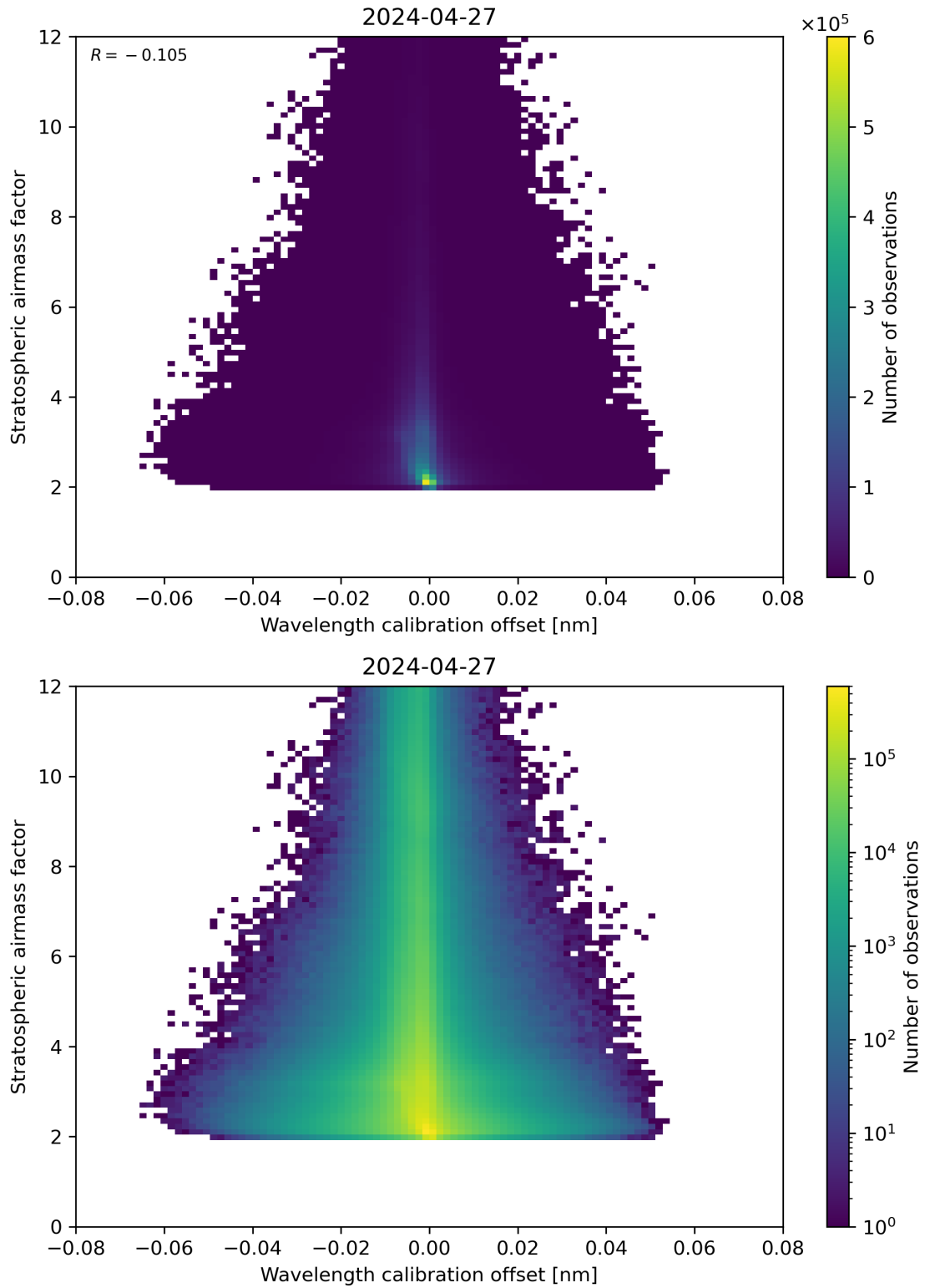
Figure 174: Scatter density plot of “Wavelength calibration offset” against “Stratospheric airmass factor” for 2024-04-26 to 2024-04-28.
