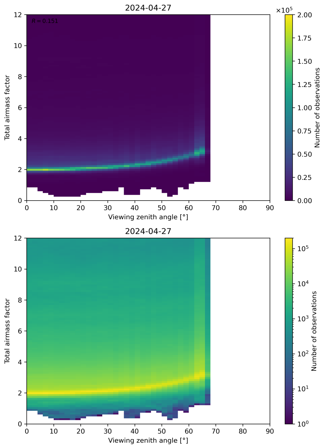
Figure 160: Scatter density plot of “Viewing zenith angle” against “Total airmass factor” for 2024-04-26 to 2024-04-28.
