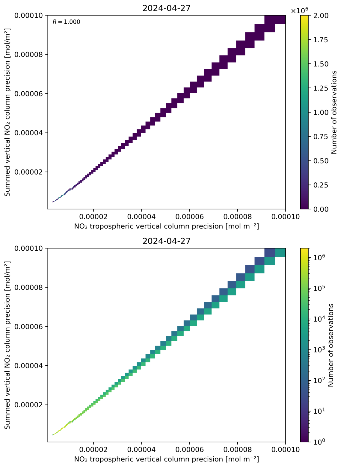
Figure 137: Scatter density plot of “NO 2 tropospheric vertical column precision” against “Summed vertical NO 2 column precision” for 2024-04-26 to 2024-04-28.
