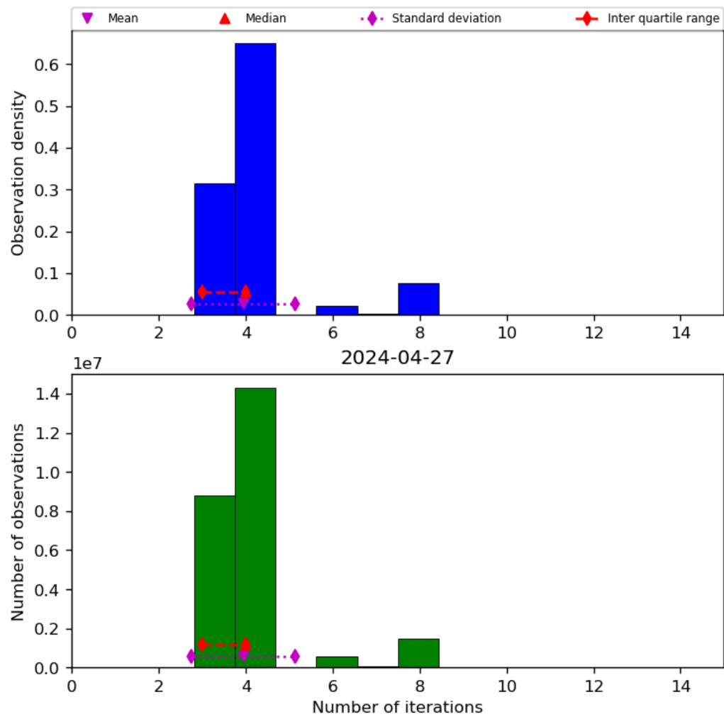
Figure 34: Histogram of “Number of iterations” for 2024-04-26 to 2024-04-28
