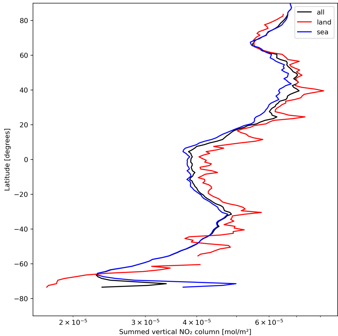
Figure 23: Zonal average of “Summed vertical NO 2 column” for 2024-04-26 to 2024-04-28.
