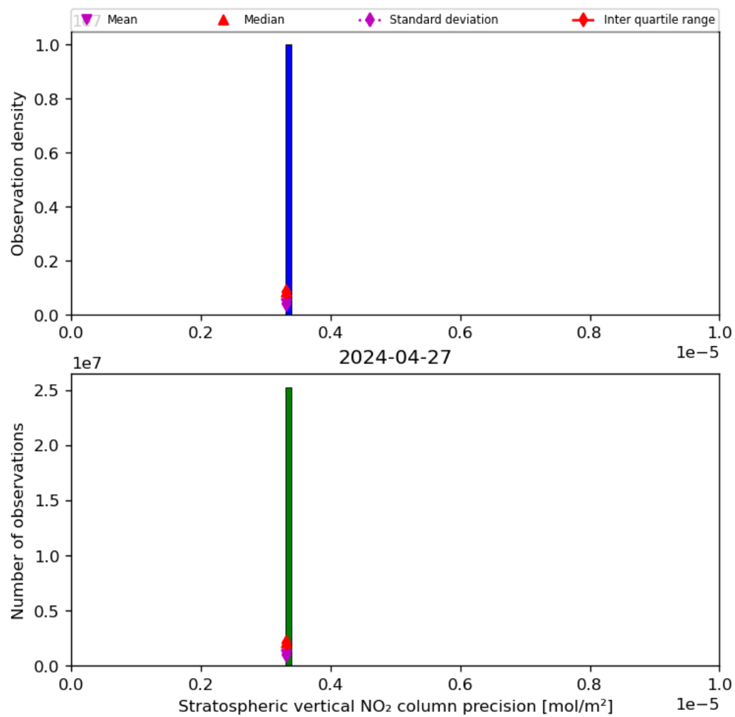
Figure 37: Histogram of “Stratospheric vertical NO 2 column precision” for 2024-04-26 to 2024-04-28
