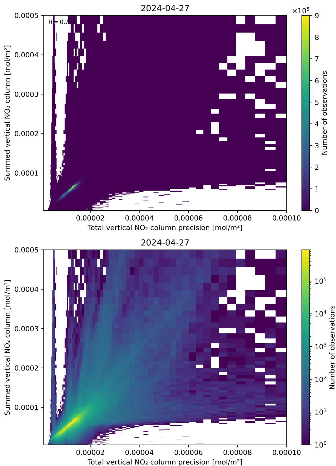
Figure 117: Scatter density plot of “Total vertical NO 2 column precision” against “Summed vertical NO 2 column” for 2024-04-26 to 2024-04-28.
