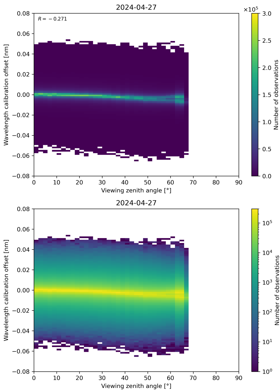
Figure 173: Scatter density plot of “Viewing zenith angle” against “Wavelength calibration offset” for 2024-04-26 to 2024-04-28.
