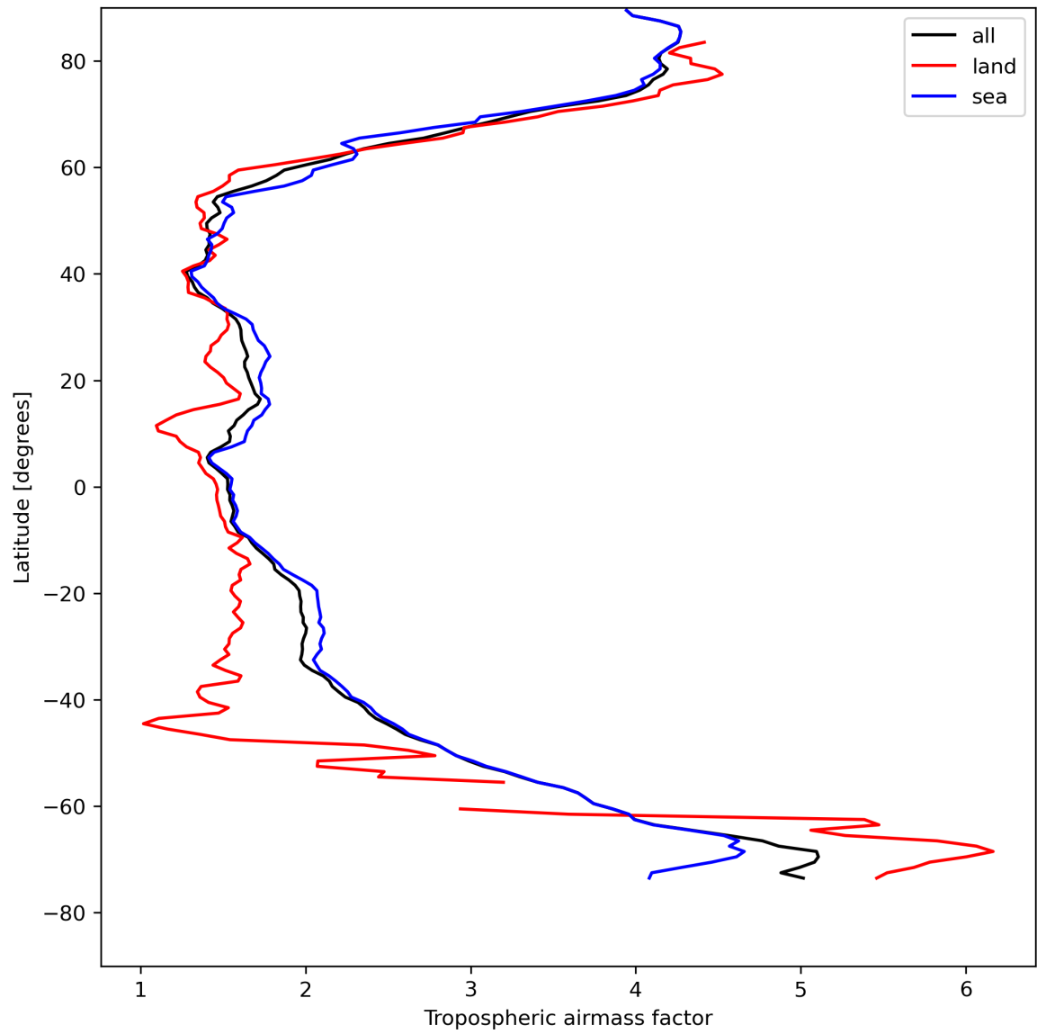
Figure 14: Zonal average of “Tropospheric airmass factor” for 2024-04-26 to 2024-04-28.
