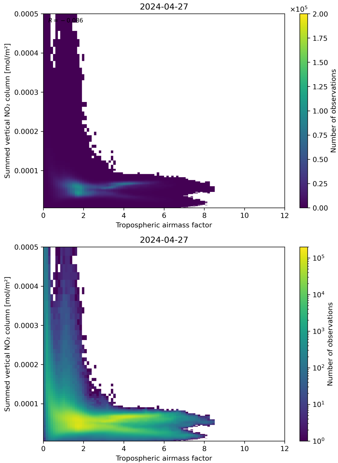
Figure 75: Scatter density plot of “Tropospheric air mass factor” against “Summed vertical NO 2 column” for 2024-04-26 to 2024-04-28.
