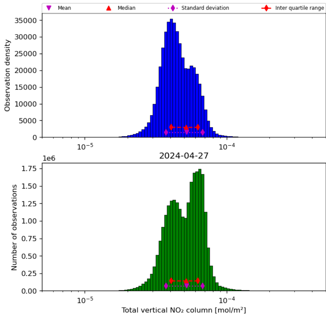
Figure 38: Histogram of “Total vertical NO 2 column” for 2024-04-26 to 2024-04-28
