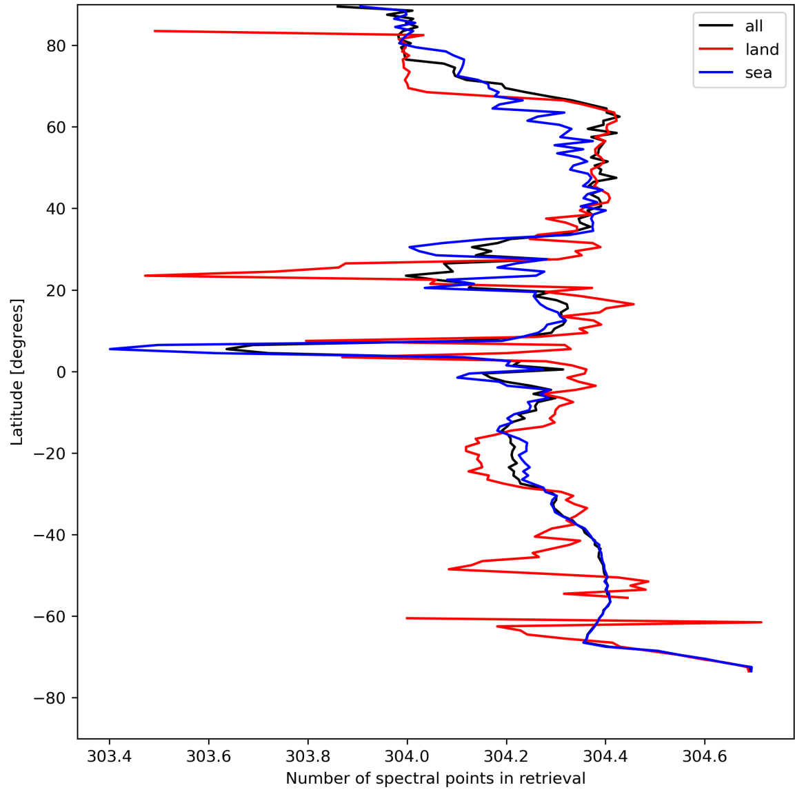
Figure 16: Zonal average of “Number of spectral points in retrieval” for 2024-04-26 to 2024-04-28.
