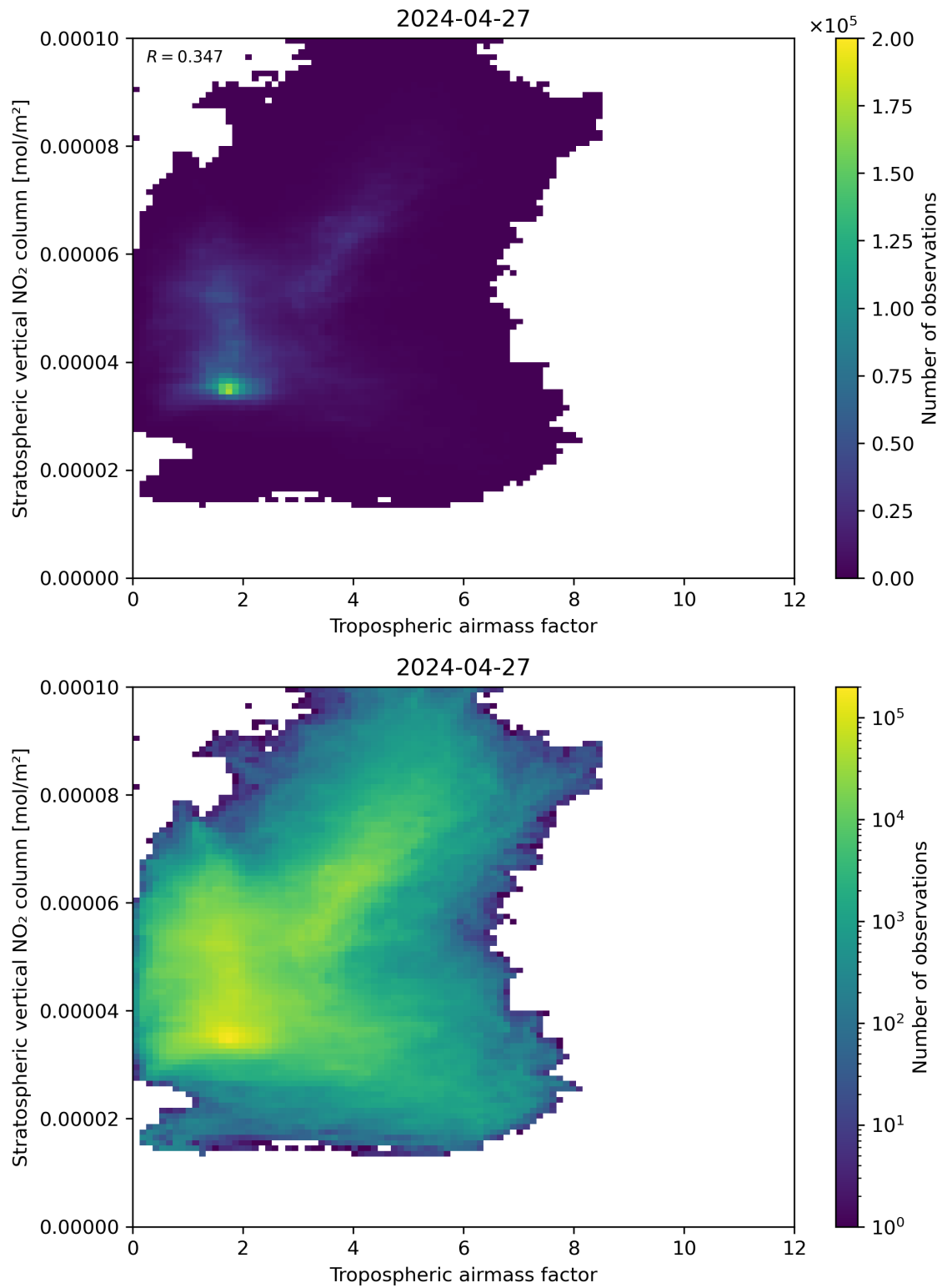
Figure 74: Scatter density plot of “Tropospheric air mass factor” against “Stratospheric vertical \text{NO}_2 column” for 2024-04-26 to 2024-04-28.
