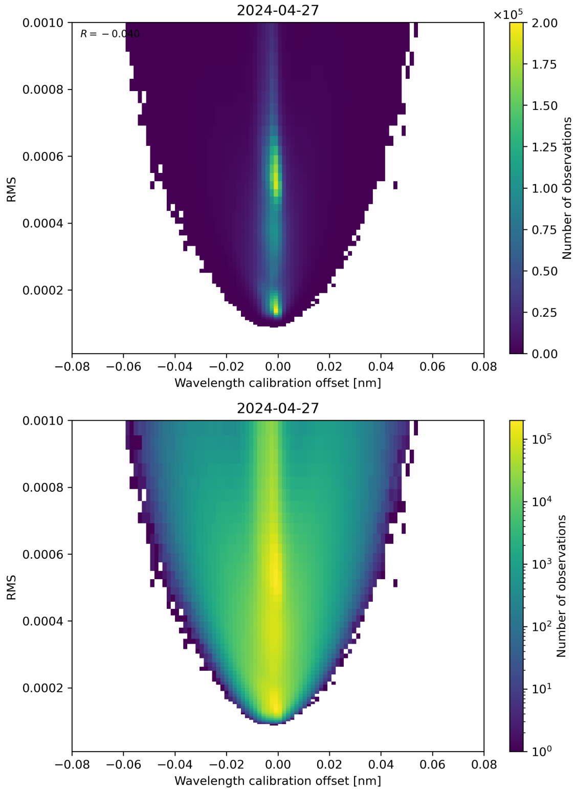
Figure 181: Scatter density plot of “Wavelength calibration offset” against “RMS” for 2024-04-26 to 2024-04-28.
