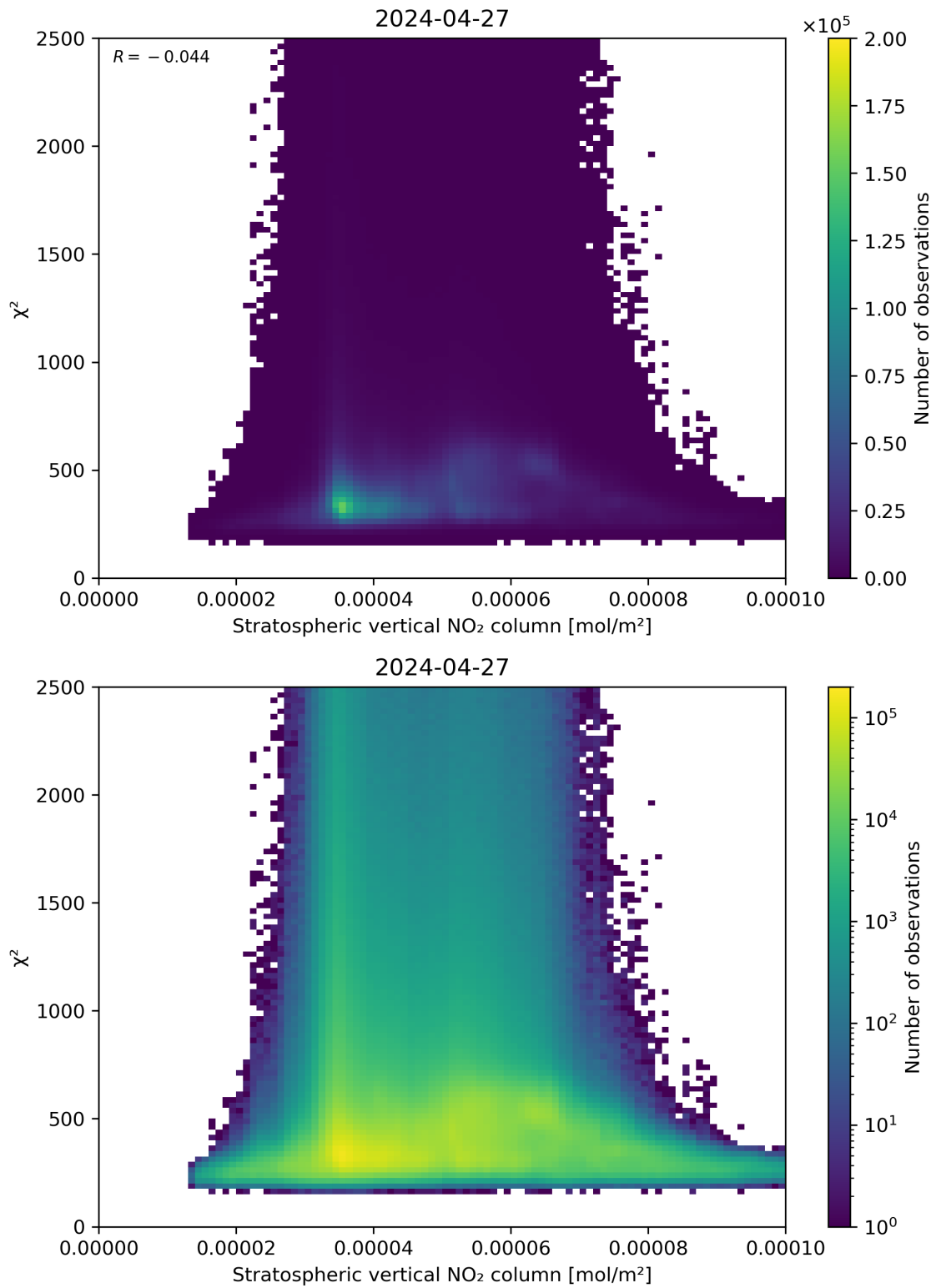
Figure 97: Scatter density plot of “Stratospheric vertical NO 2 column” against “ \chi^2 ” for 2024-04-26 to 2024-04-28.
