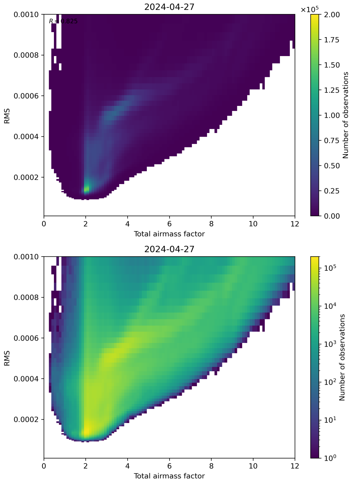
Figure 69: Scatter density plot of “Total airmass factor” against “RMS” for 2024-04-26 to 2024-04-28.
