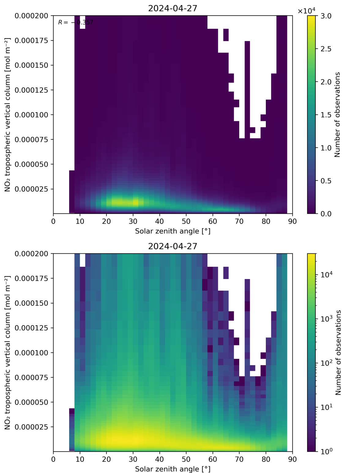
Figure 155: Scatter density plot of “Solar zenith angle” against “NO 2 tropospheric vertical column” for 2024-04-26 to 2024-04-28.
