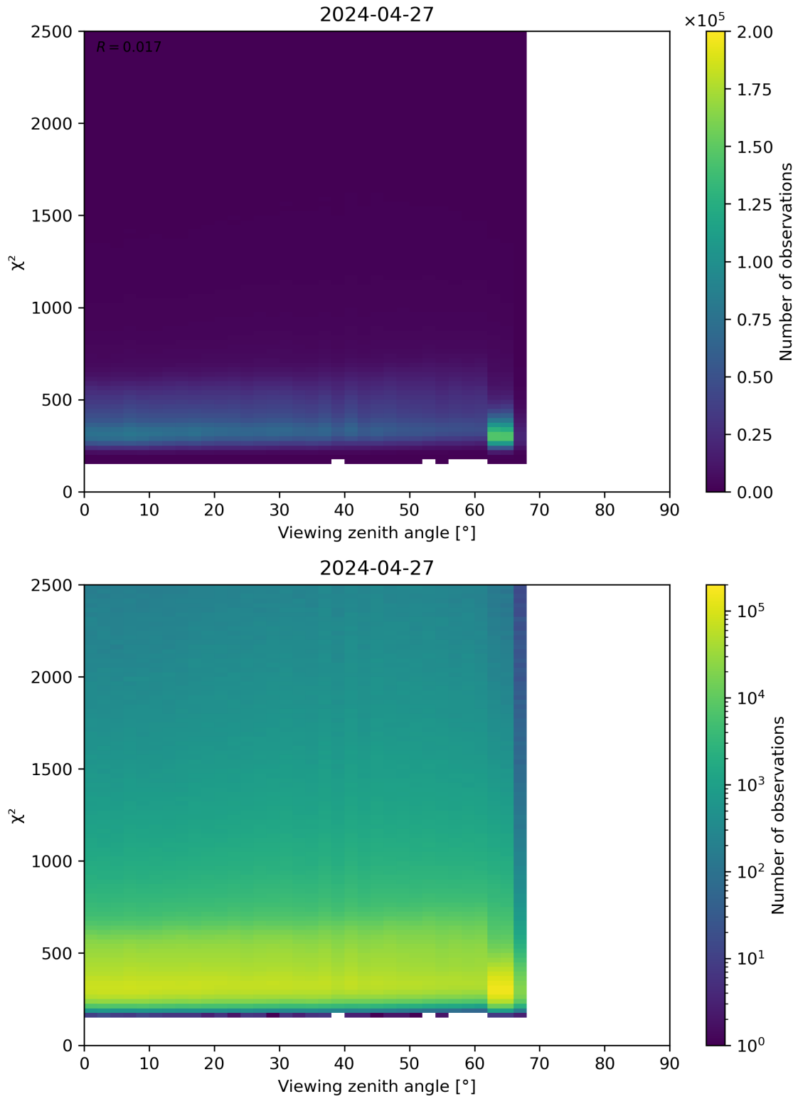
Figure 162: Scatter density plot of “Viewing zenith angle” against “ \chi^2 ” for 2024-04-26 to 2024-04-28.
