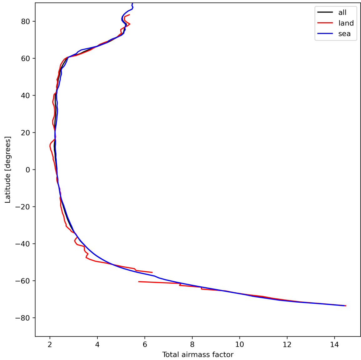
Figure 15: Zonal average of “Total airmass factor” for 2024-04-26 to 2024-04-28.
