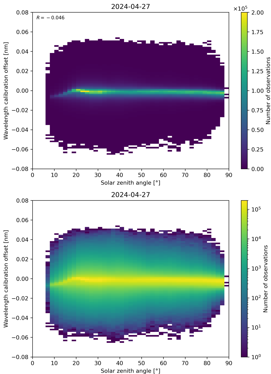
Figure 158: Scatter density plot of “Solar zenith angle” against “Wavelength calibration offset” for 2024-04-26 to 2024-04-28.
