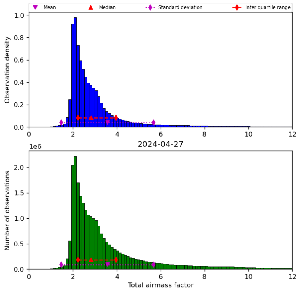
Figure 32: Histogram of “Total airmass factor” for 2024-04-26 to 2024-04-28
