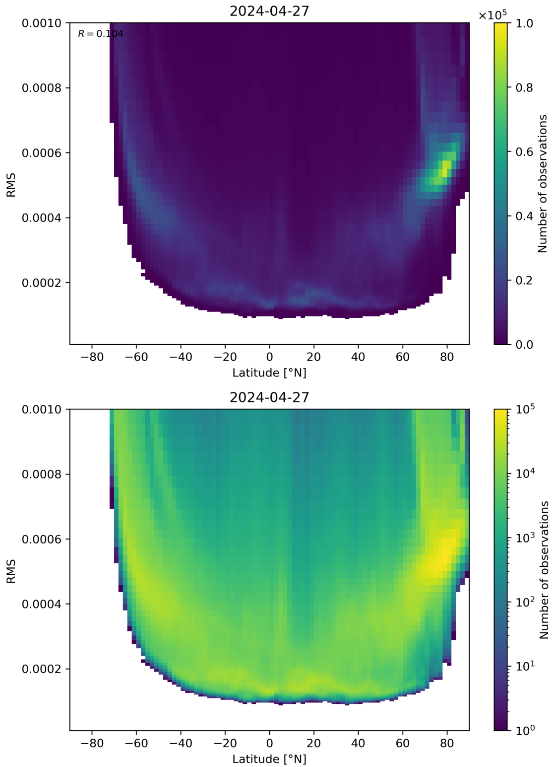
Figure 94: Scatter density plot of “Latitude” against “RMS” for 2024-04-26 to 2024-04-28.
