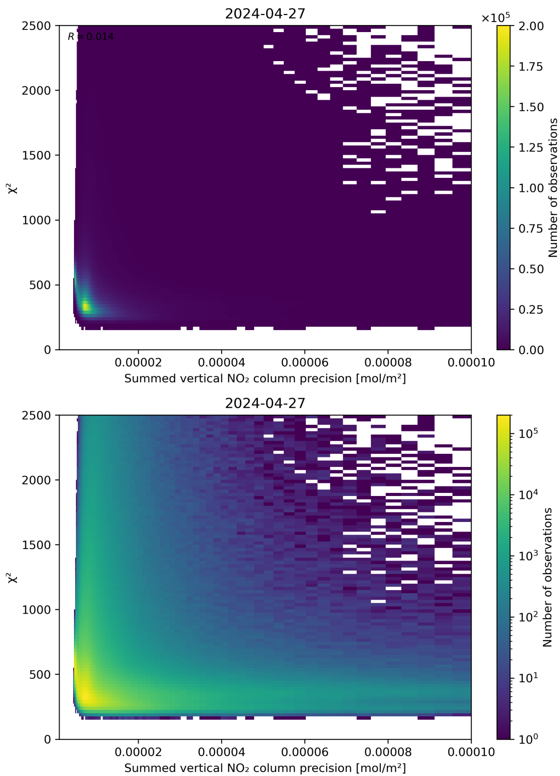
Figure 107: Scatter density plot of “Summed vertical NO 2 column precision” against “ \chi^2 ” for 2024-04-26 to 2024-04-28.
