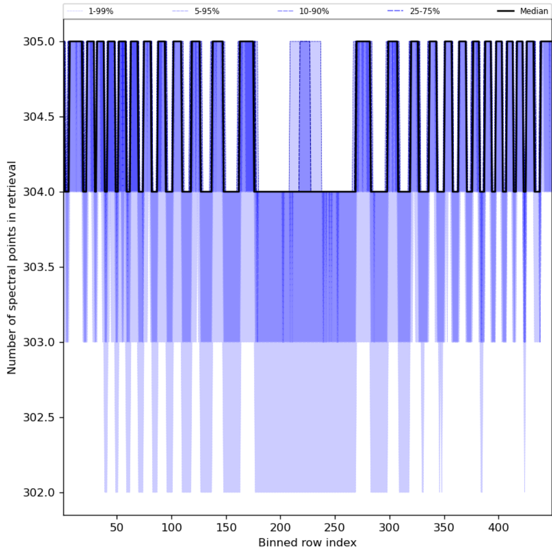
Figure 50: Along track statistics of “Number of spectral points in retrieval” for 2024-04-26 to 2024-04-28
