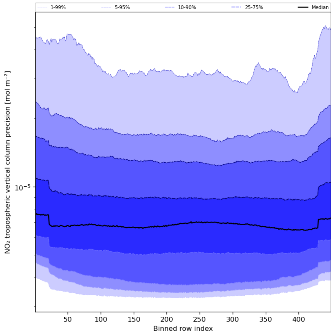
Figure 47: Along track statistics of “NO 2 tropospheric vertical column precision” for 2024-04-26 to 2024-04-28
