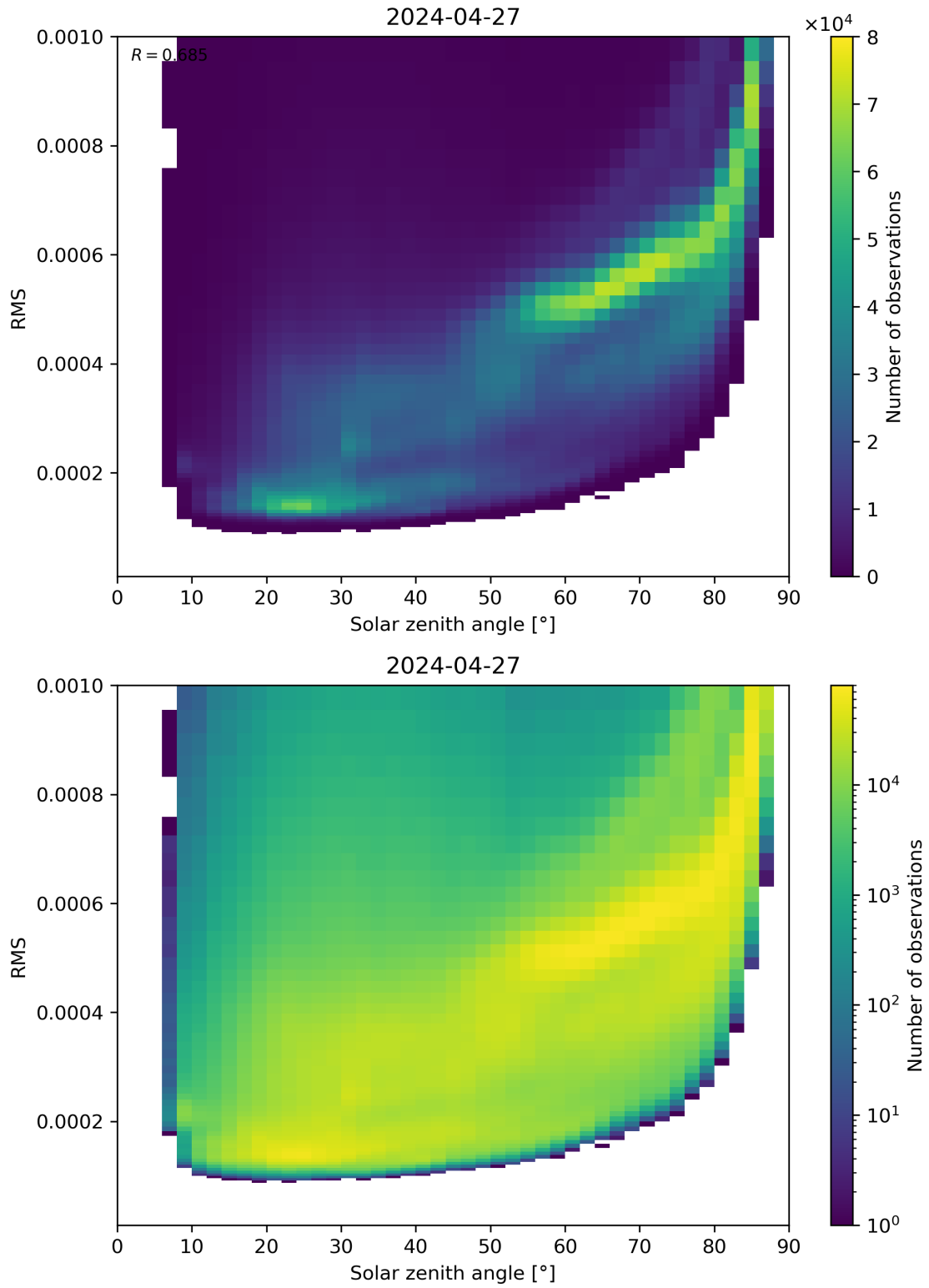
Figure 157: Scatter density plot of “Solar zenith angle” against “RMS” for 2024-04-26 to 2024-04-28.
