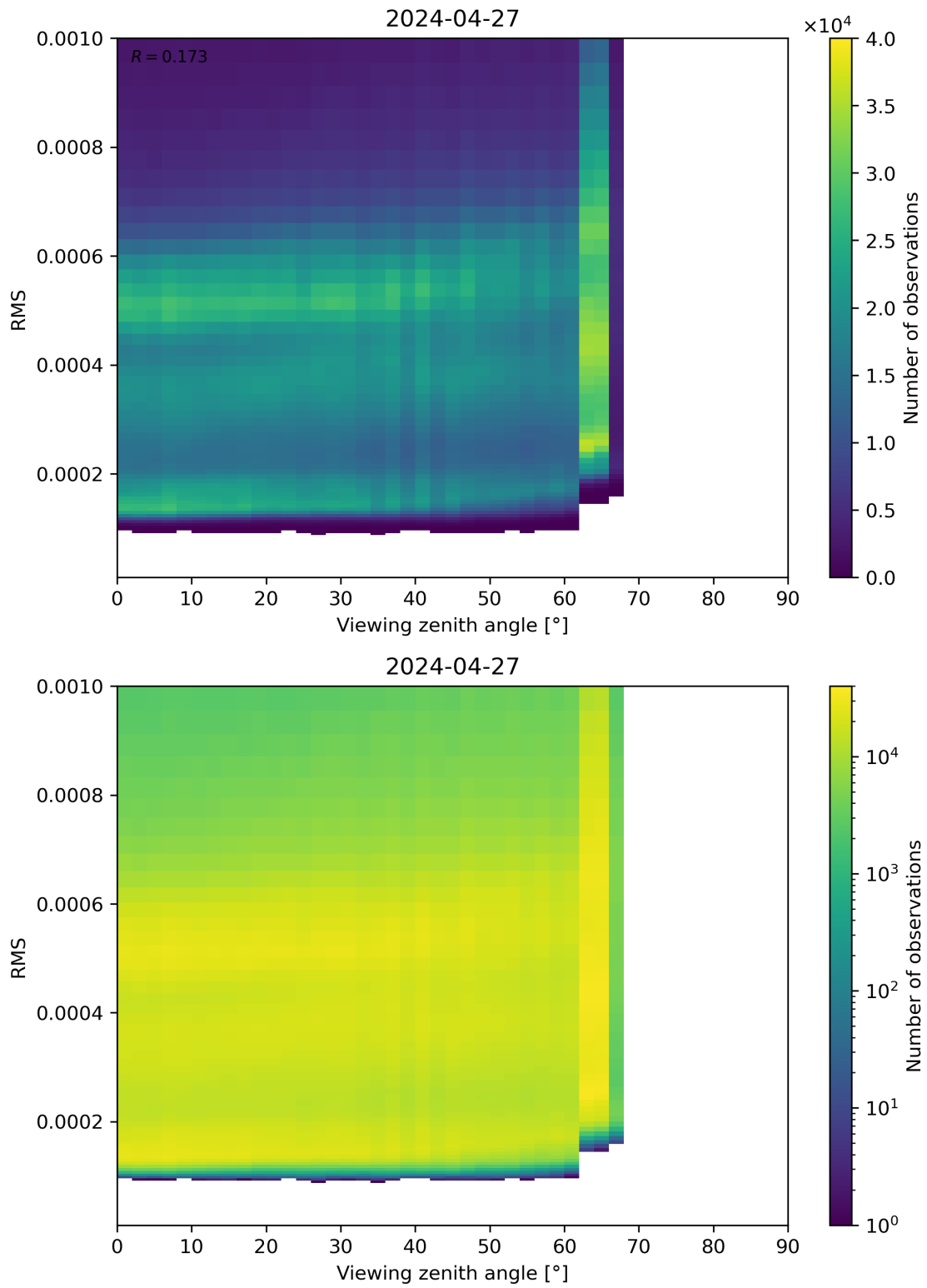
Figure 171: Scatter density plot of “Viewing zenith angle” against “RMS” for 2024-04-26 to 2024-04-28.
