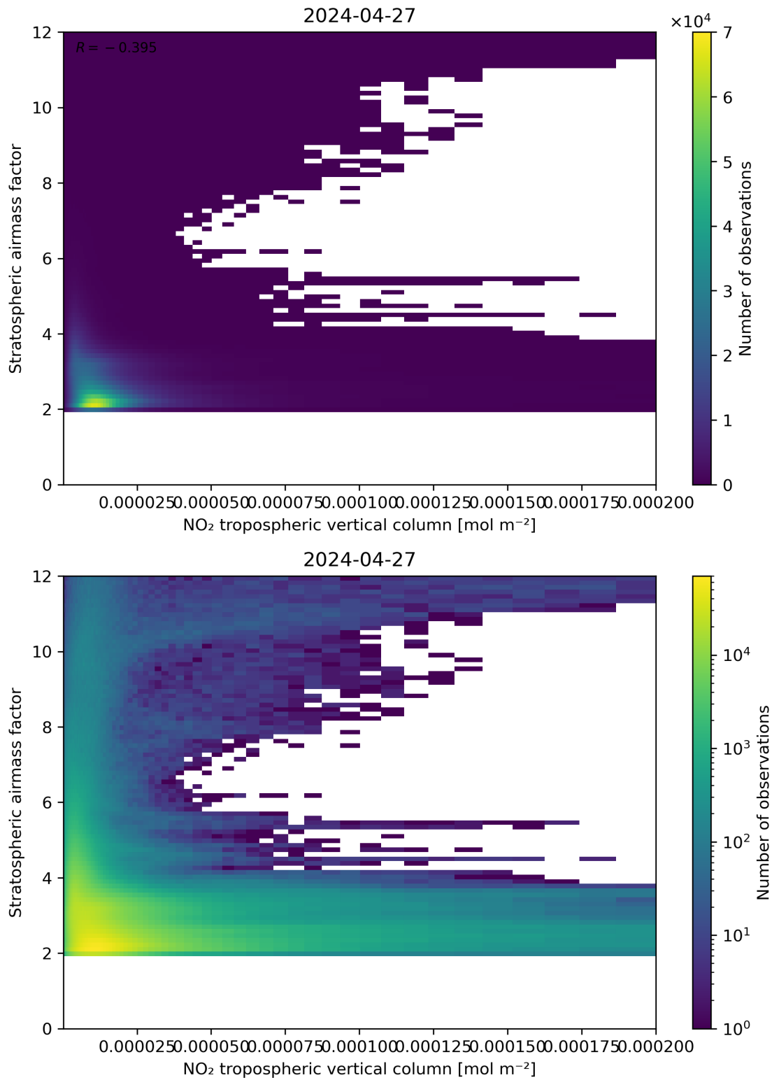
Figure 121: Scatter density plot of “NO 2 tropospheric vertical column” against “Stratospheric air mass factor” for 2024-04-26 to 2024-04-28.
