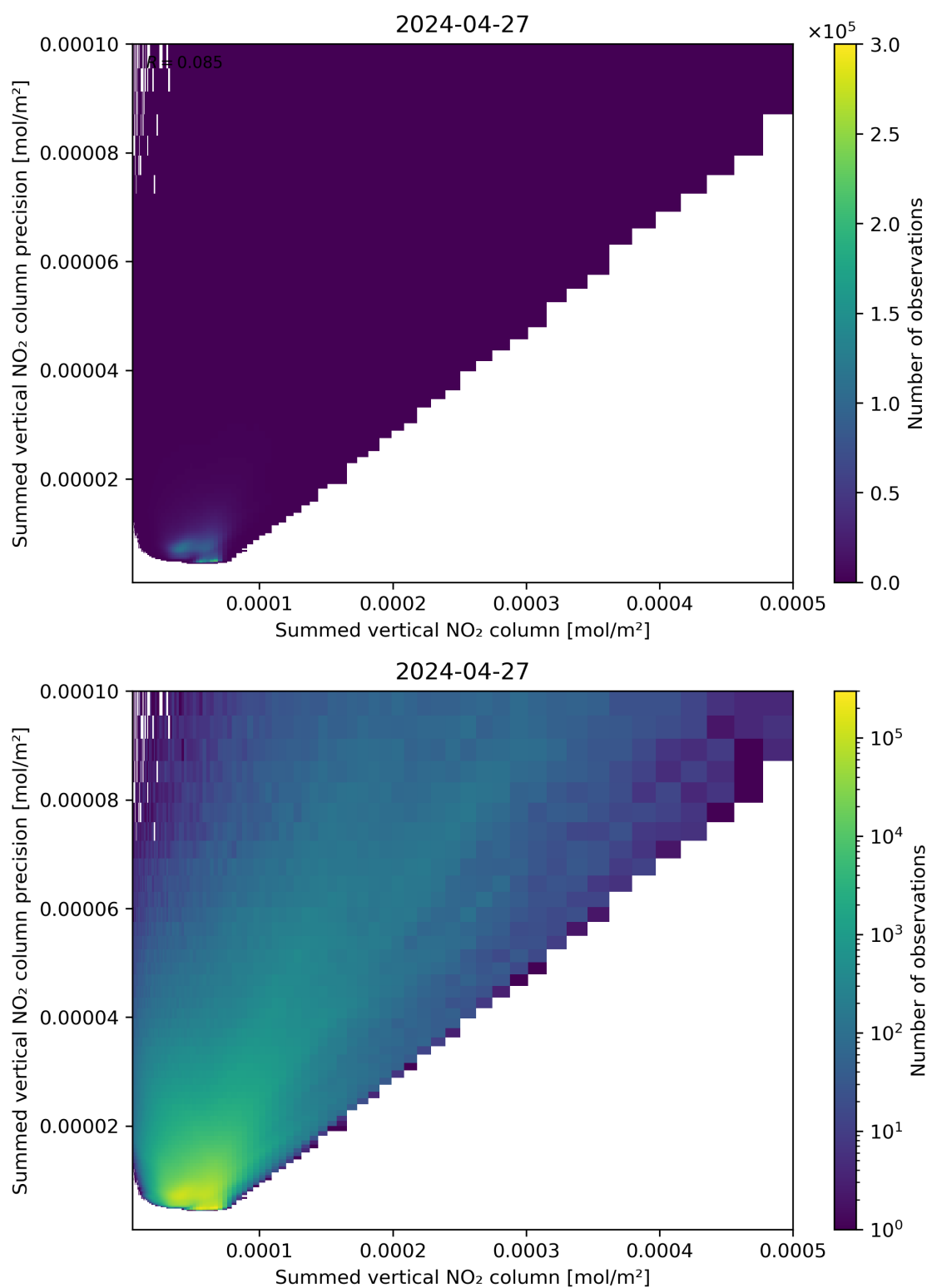
Figure 105: Scatter density plot of “Summed vertical NO 2 column” against “Summed vertical NO 2 column precision” for 2024-04-26 to 2024-04-28.
