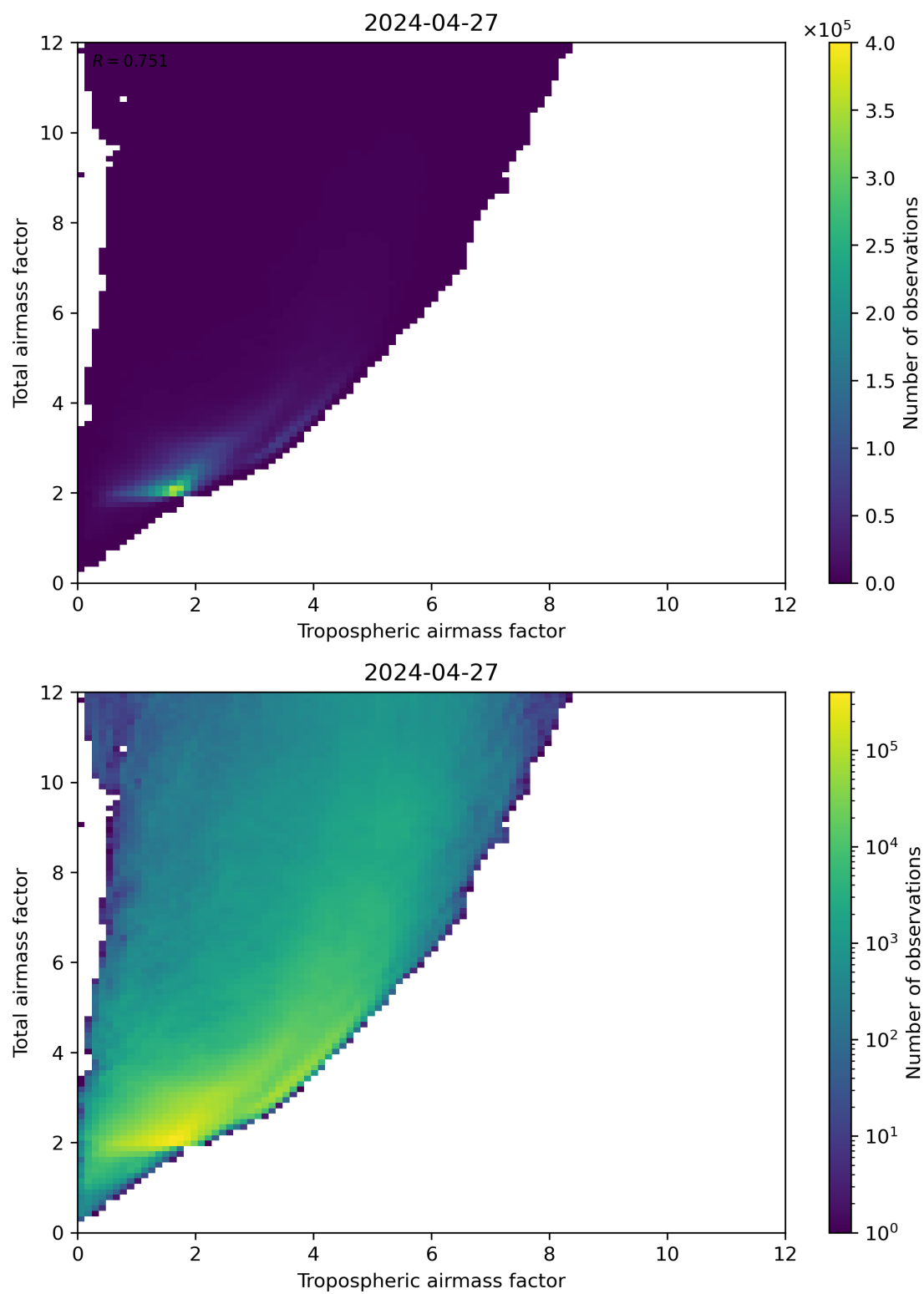
Figure 72: Scatter density plot of “Tropospheric airmass factor” against “Total airmass factor” for 2024-04-26 to 2024-04-28.
