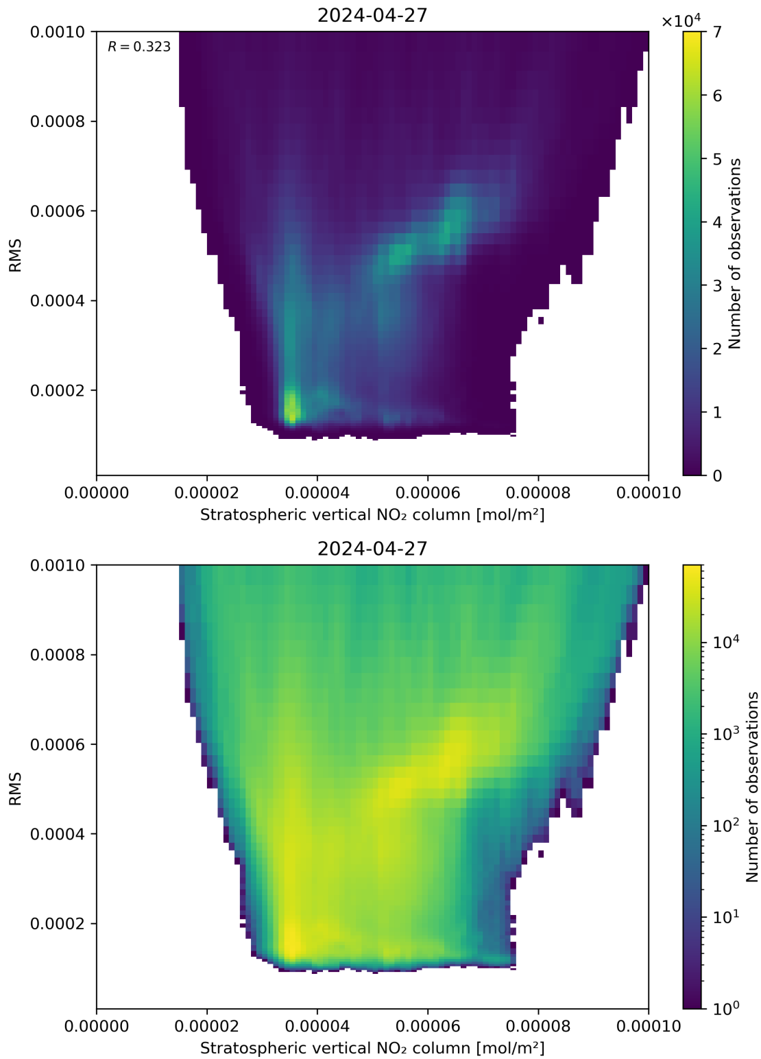
Figure 102: Scatter density plot of “Stratospheric vertical NO 2 column” against “RMS” for 2024-04-26 to 2024-04-28.
