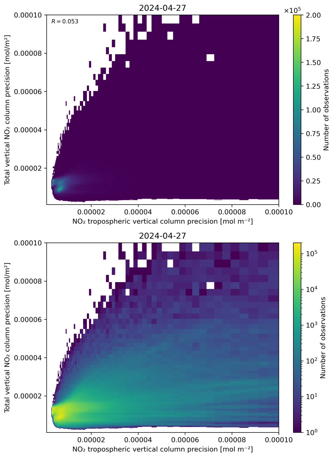
Figure 139: Scatter density plot of “NO 2 tropospheric vertical column precision” against “Total vertical NO 2 column precision” for 2024-04-26 to 2024-04-28.
