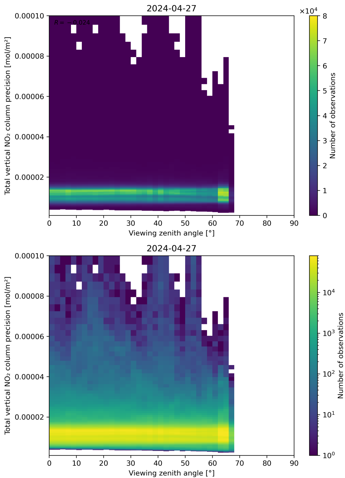
Figure 168: Scatter density plot of “Viewing zenith angle” against “Total vertical NO 2 column precision” for 2024-04-26 to 2024-04-28.
