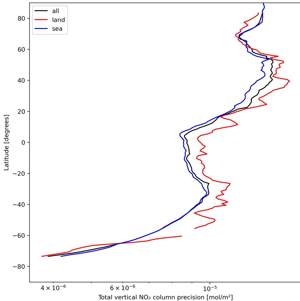
Figure 22: Zonal average of “Total vertical NO 2 column precision” for 2024-04-26 to 2024-04-28.
