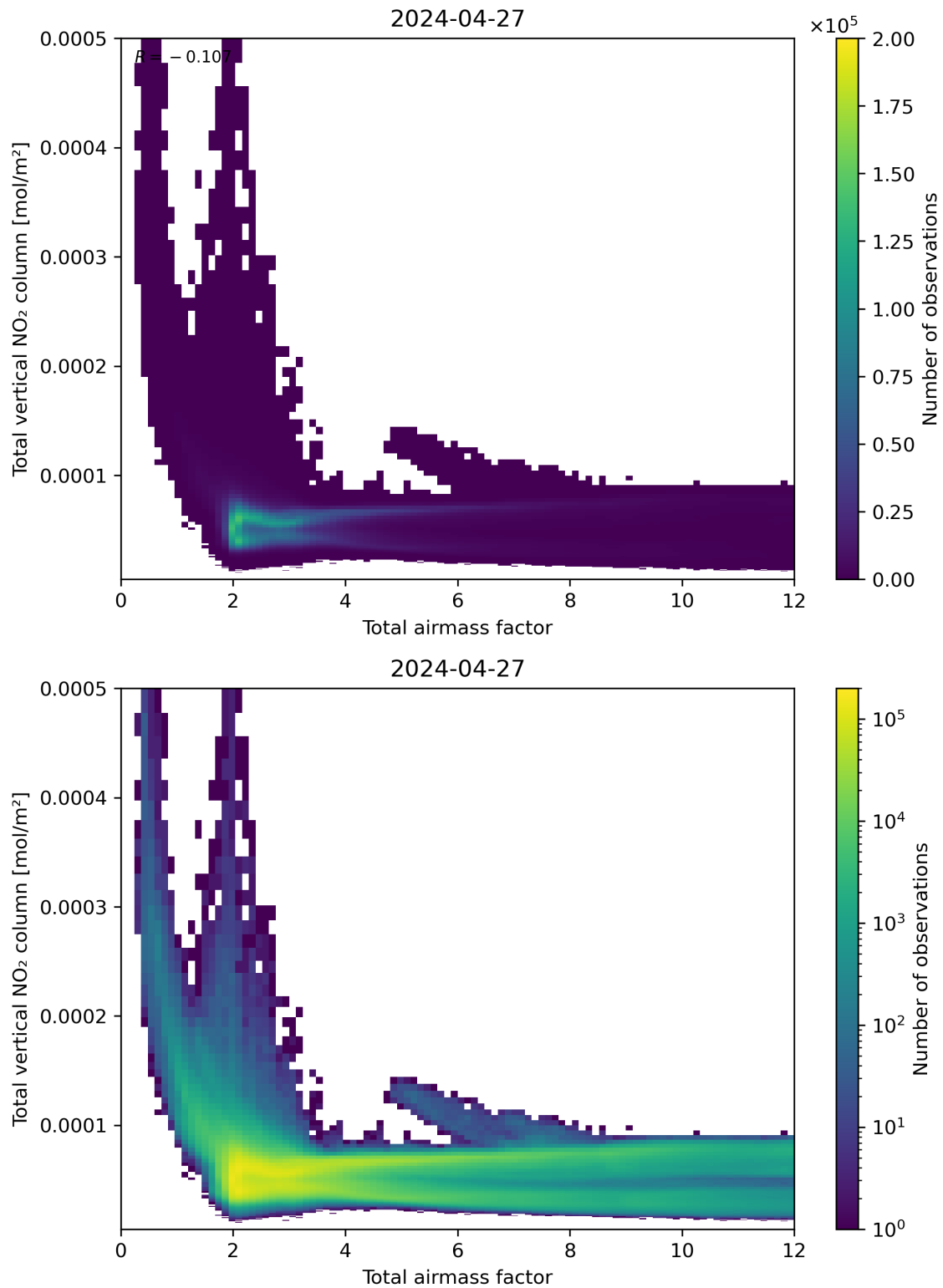
Figure 67: Scatter density plot of “Total airmass factor” against “Total vertical NO 2 column” for 2024-04-26 to 2024-04-28.
