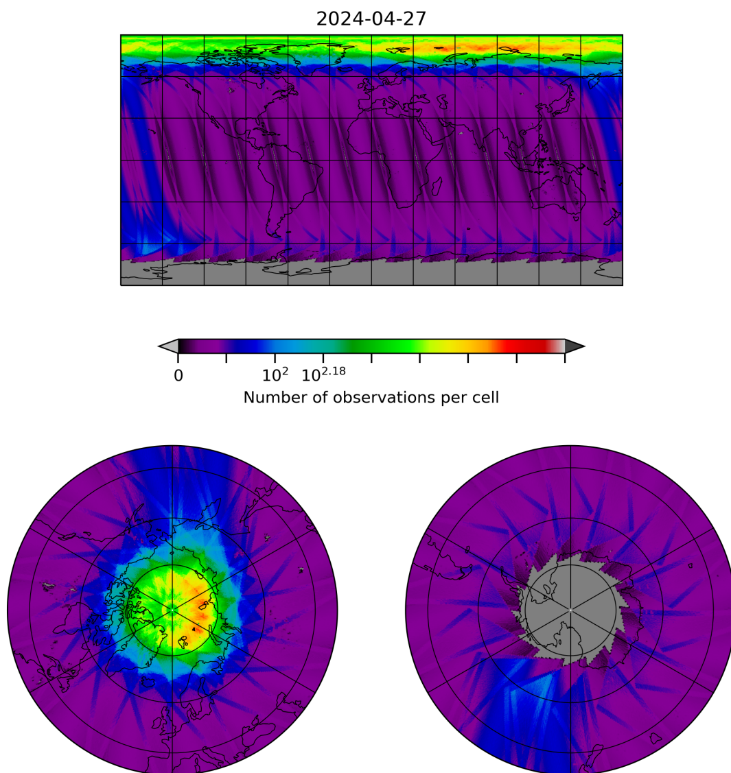
Figure 10: Map of the number of observations for 2024-04-26 to 2024-04-28
