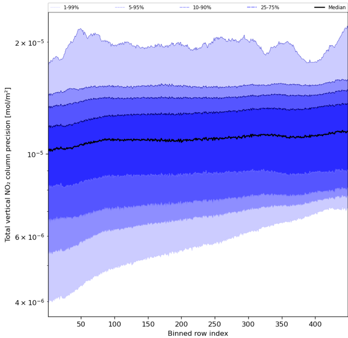
Figure 56: Along track statistics of “Total vertical NO 2 column precision” for 2024-04-26 to 2024-04-28
