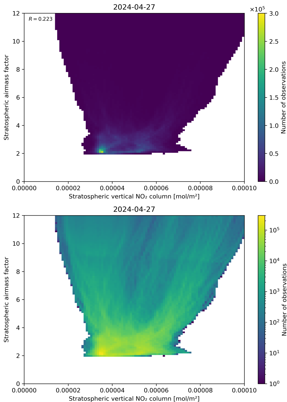
Figure 96: Scatter density plot of “Stratospheric vertical NO 2 column” against “Stratospheric airmass factor” for 2024-04-26 to 2024-04-28.
