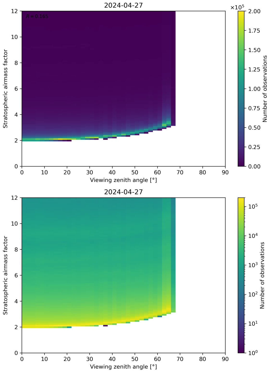
Figure 159: Scatter density plot of “Viewing zenith angle” against “Stratospheric airmass factor” for 2024-04-26 to 2024-04-28.
