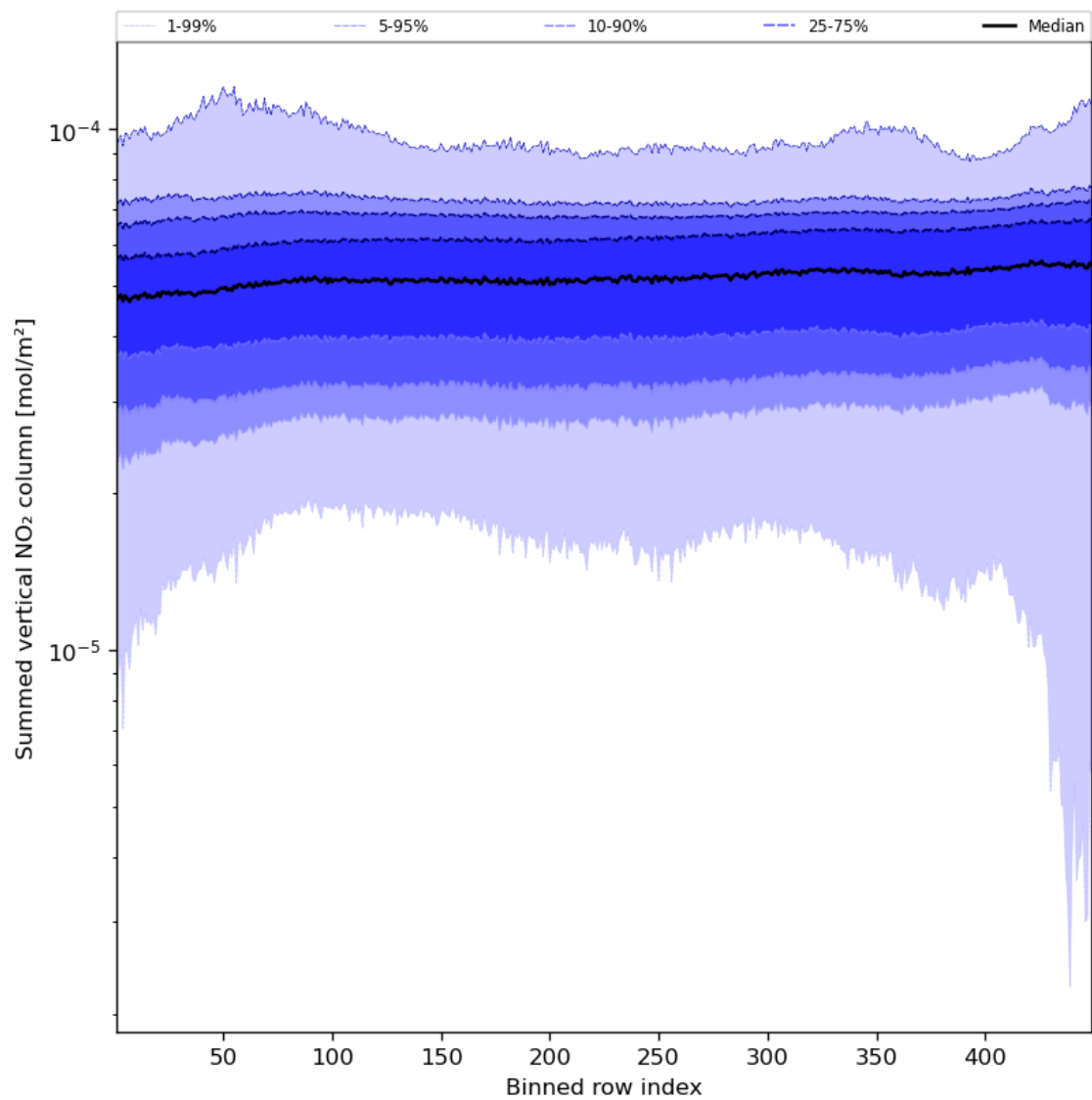
Figure 57: Along track statistics of “Summed vertical NO 2 column” for 2024-04-26 to 2024-04-28
