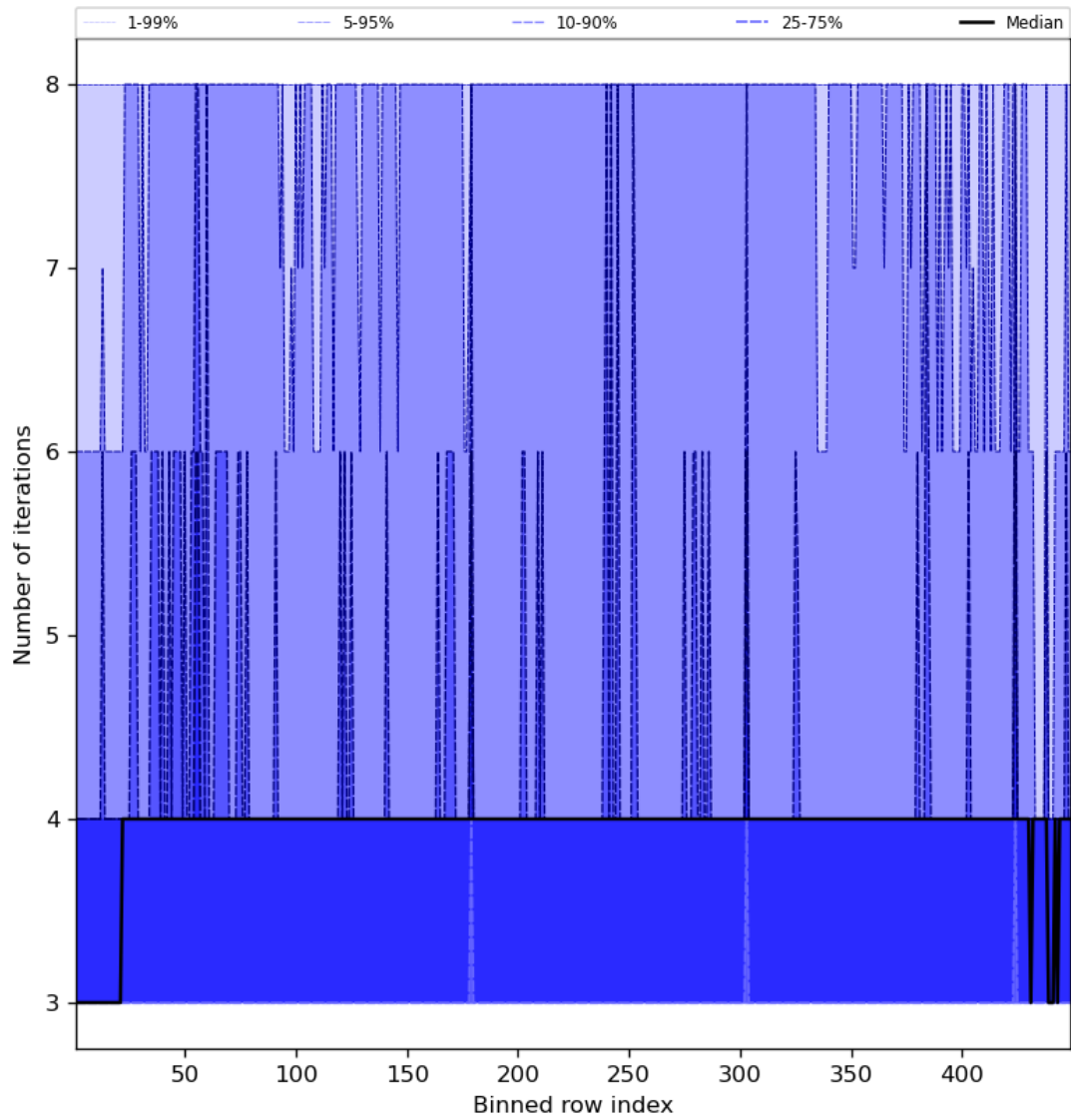
Figure 51: Along track statistics of “Number of iterations” for 2024-04-26 to 2024-04-28
