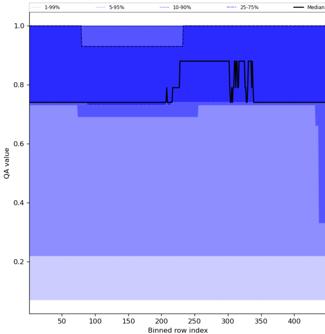
Figure 45: Along track statistics of “QA value” for 2024-04-26 to 2024-04-28
