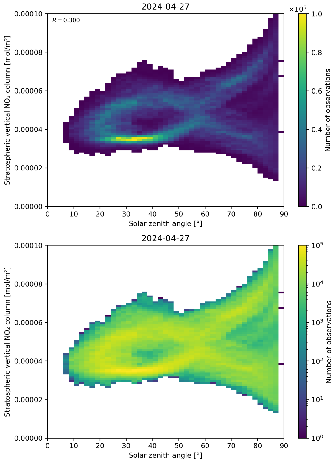
Figure 150: Scatter density plot of “Solar zenith angle” against “Stratospheric vertical NO 2 column” for 2024-04-26 to 2024-04-28.
