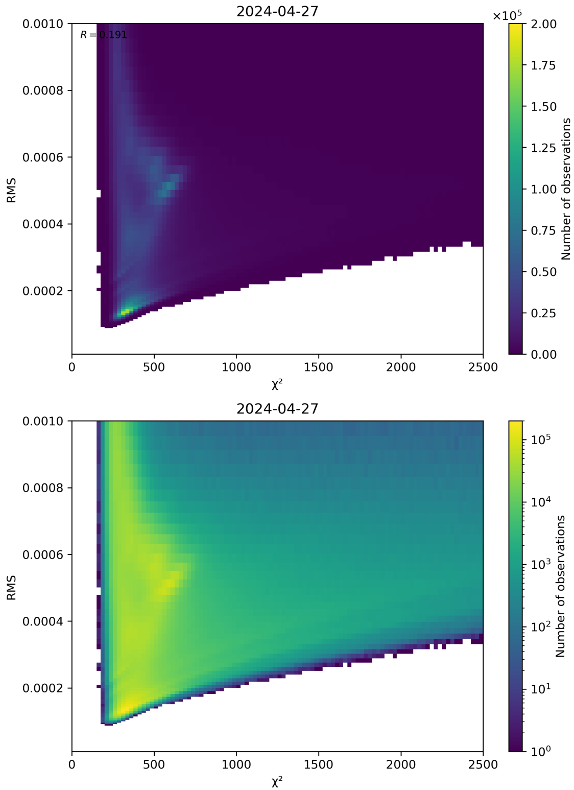
Figure 82: Scatter density plot of “ \chi^2 ” against “RMS” for 2024-04-26 to 2024-04-28.
