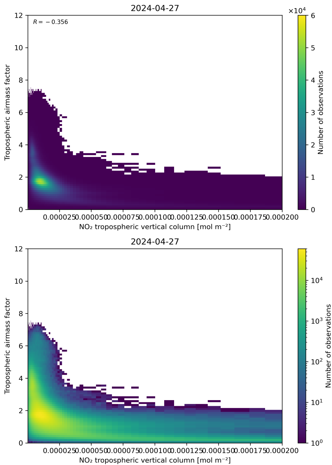
Figure 123: Scatter density plot of “NO 2 tropospheric vertical column” against “Tropospheric airmass factor” for 2024-04-26 to 2024-04-28.
