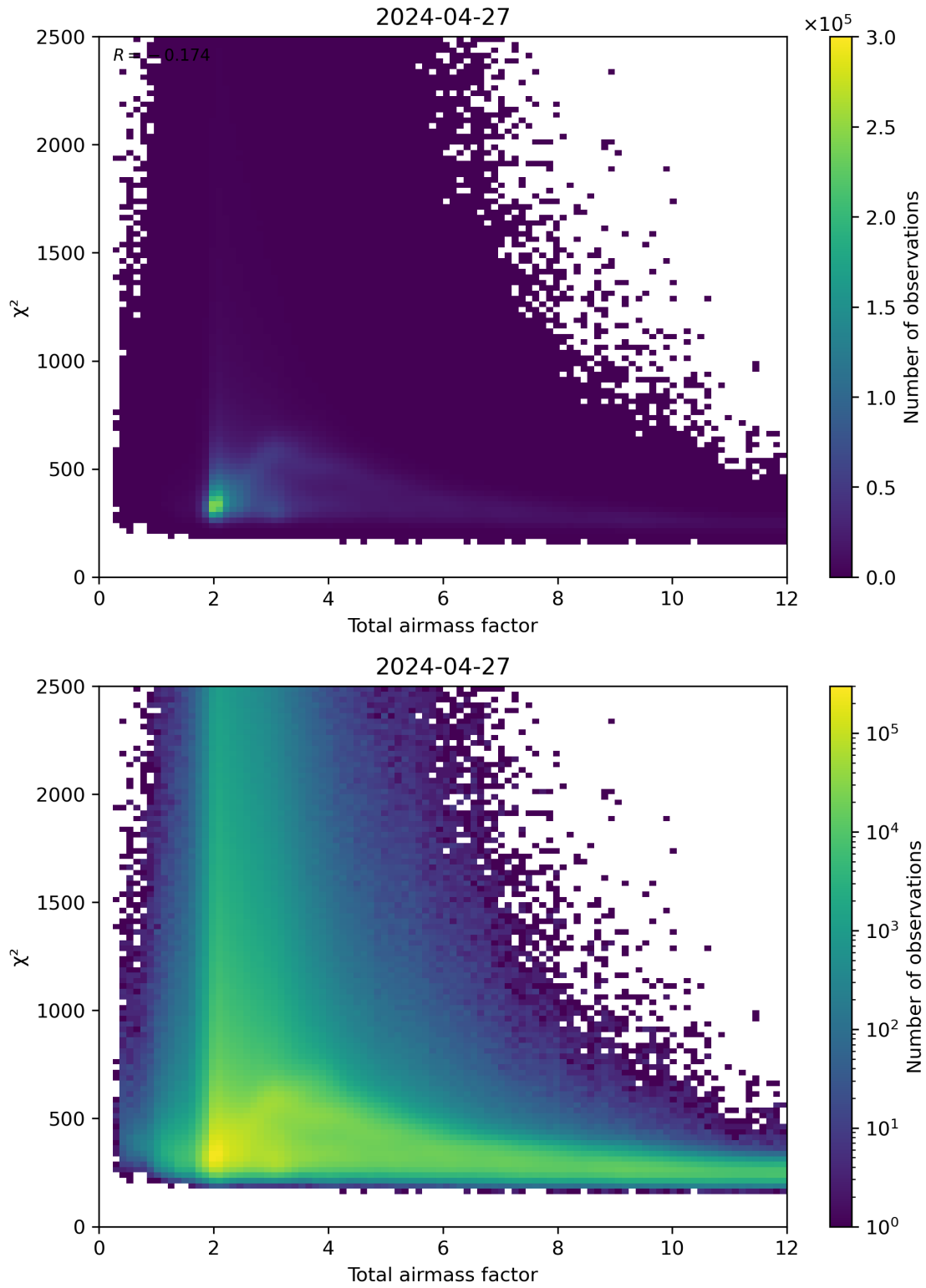
Figure 63: Scatter density plot of “Total airmass factor” against “ \chi^2 ” for 2024-04-26 to 2024-04-28.
