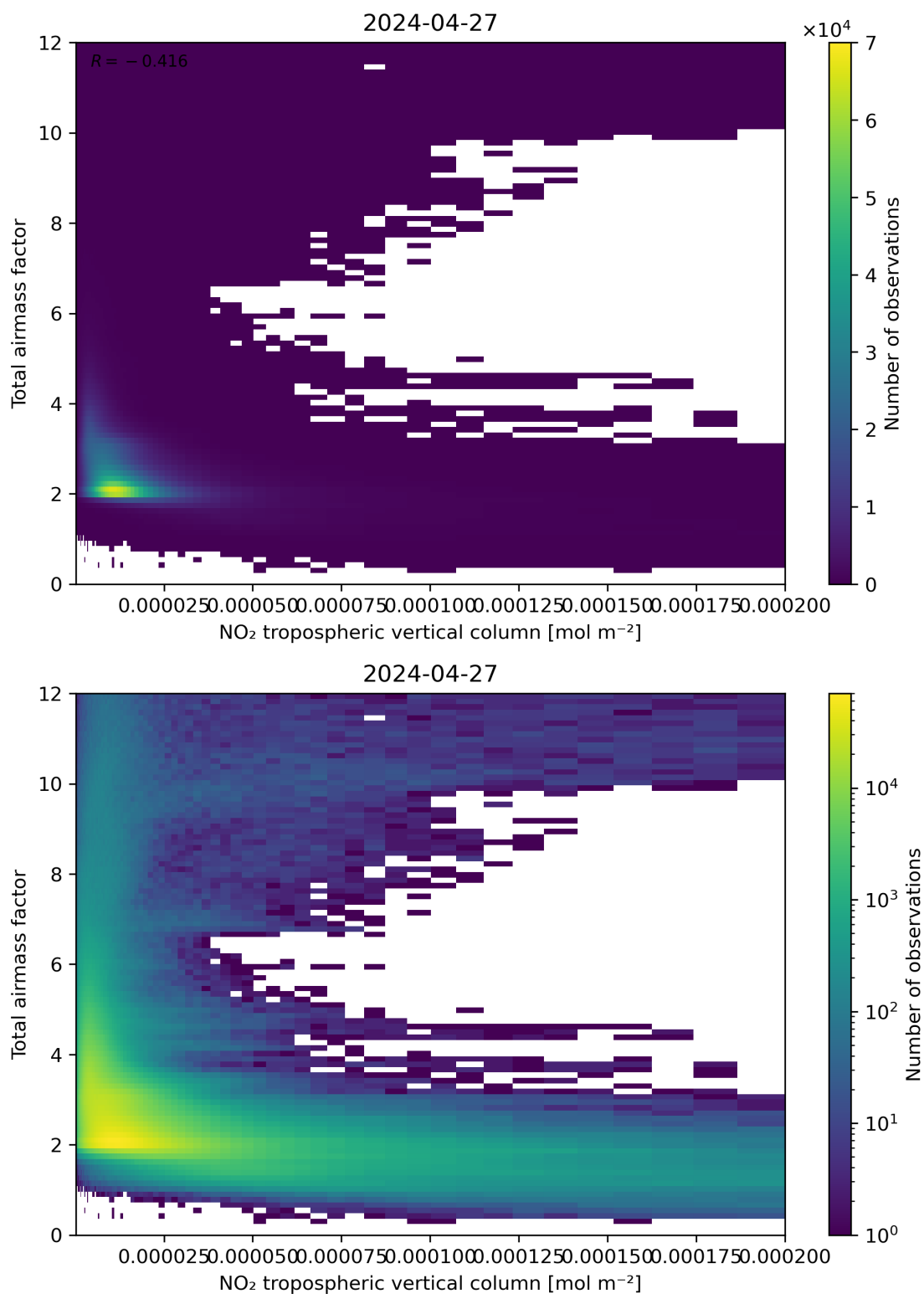
Figure 122: Scatter density plot of “NO 2 tropospheric vertical column” against “Total air mass factor” for 2024-04-26 to 2024-04-28.
