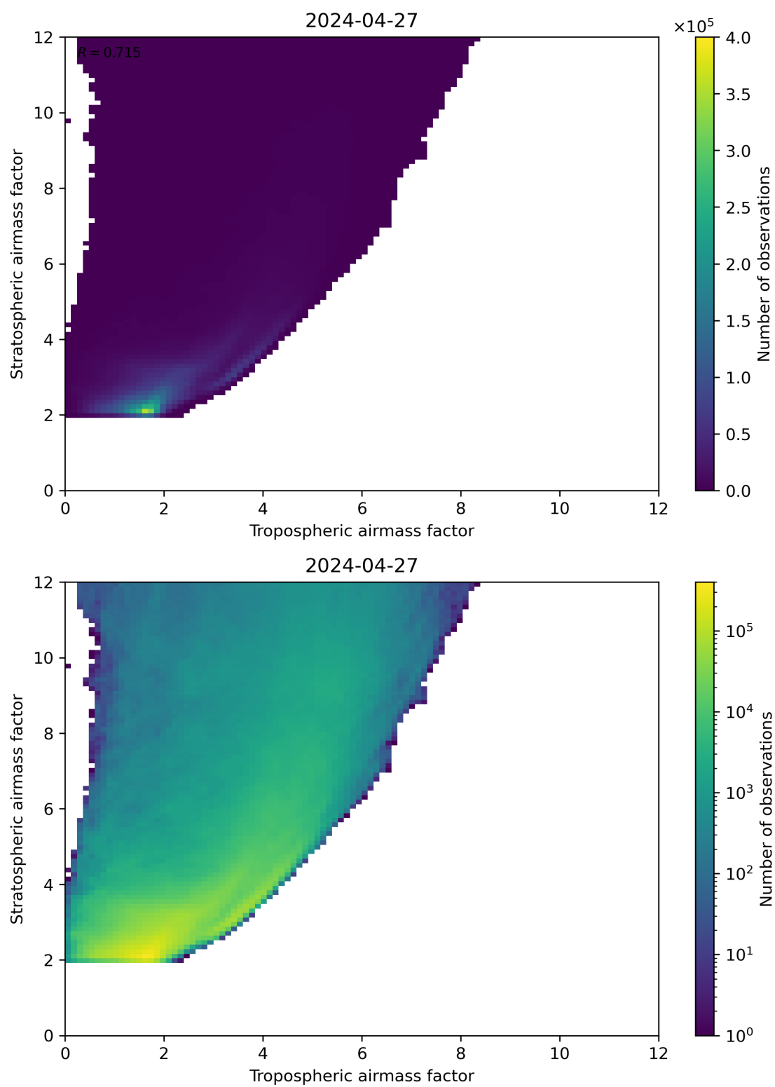
Figure 71: Scatter density plot of “Tropospheric airmass factor” against “Stratospheric airmass factor” for 2024-04-26 to 2024-04-28.
