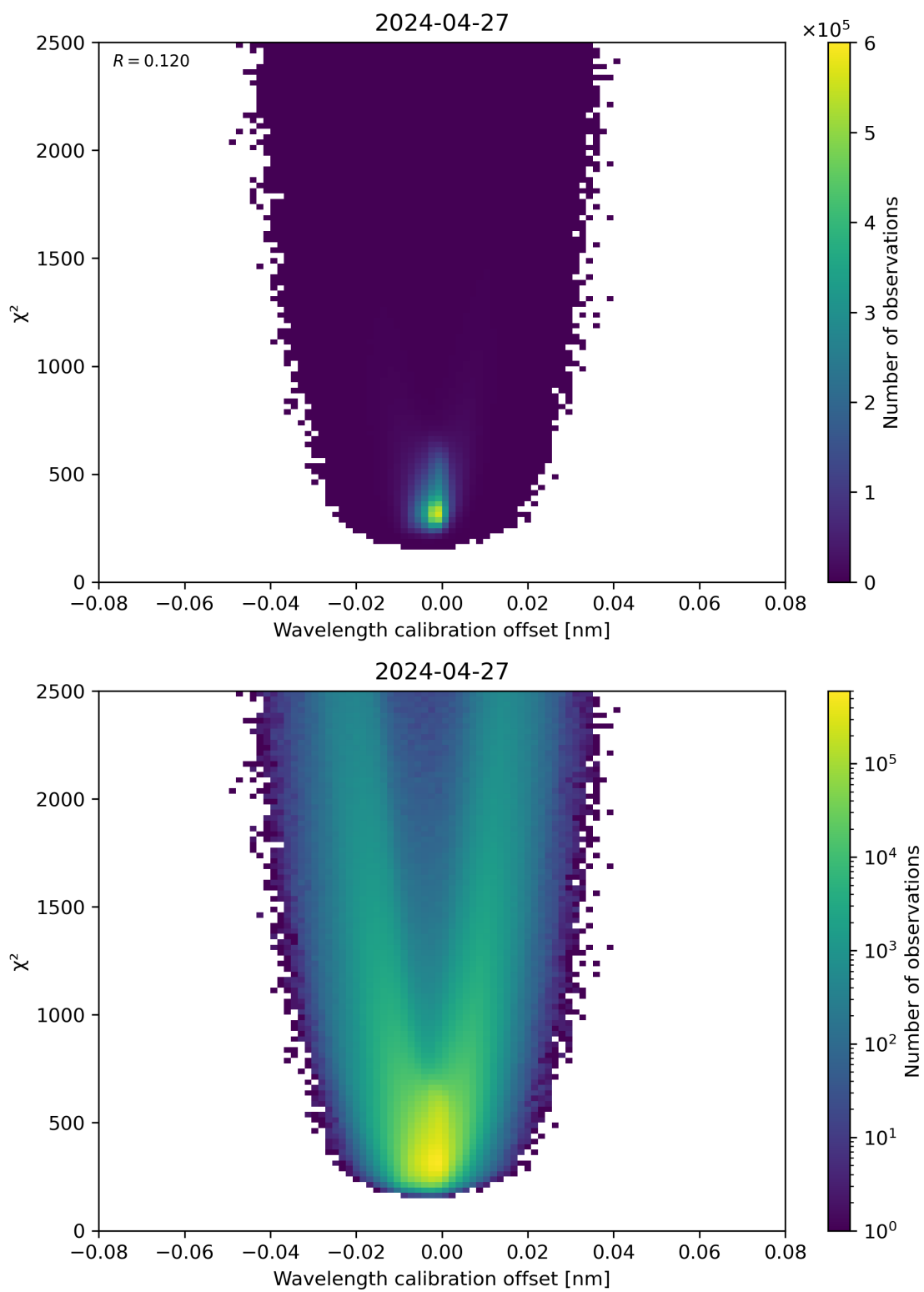
Figure 175: Scatter density plot of “Wavelength calibration offset” against “ \chi^2 ” for 2024-04-26 to 2024-04-28.
