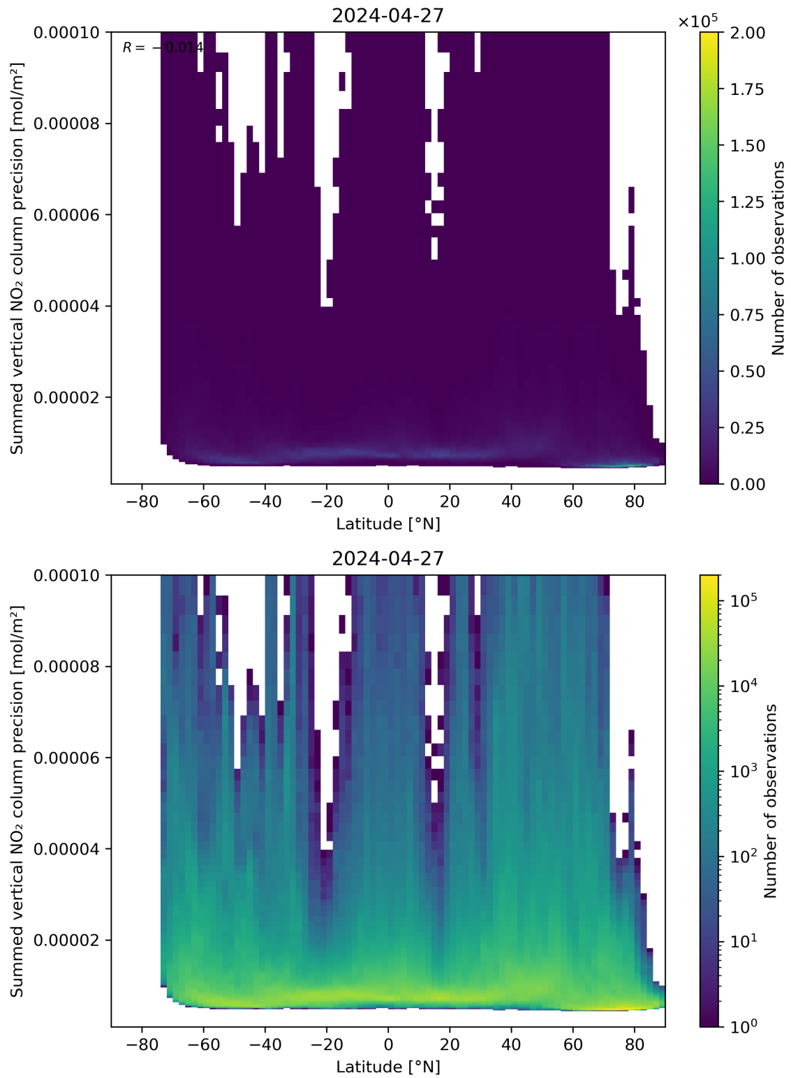
Figure 89: Scatter density plot of “Latitude” against “Summed vertical NO 2 column precision” for 2024-04-26 to 2024-04-28.
