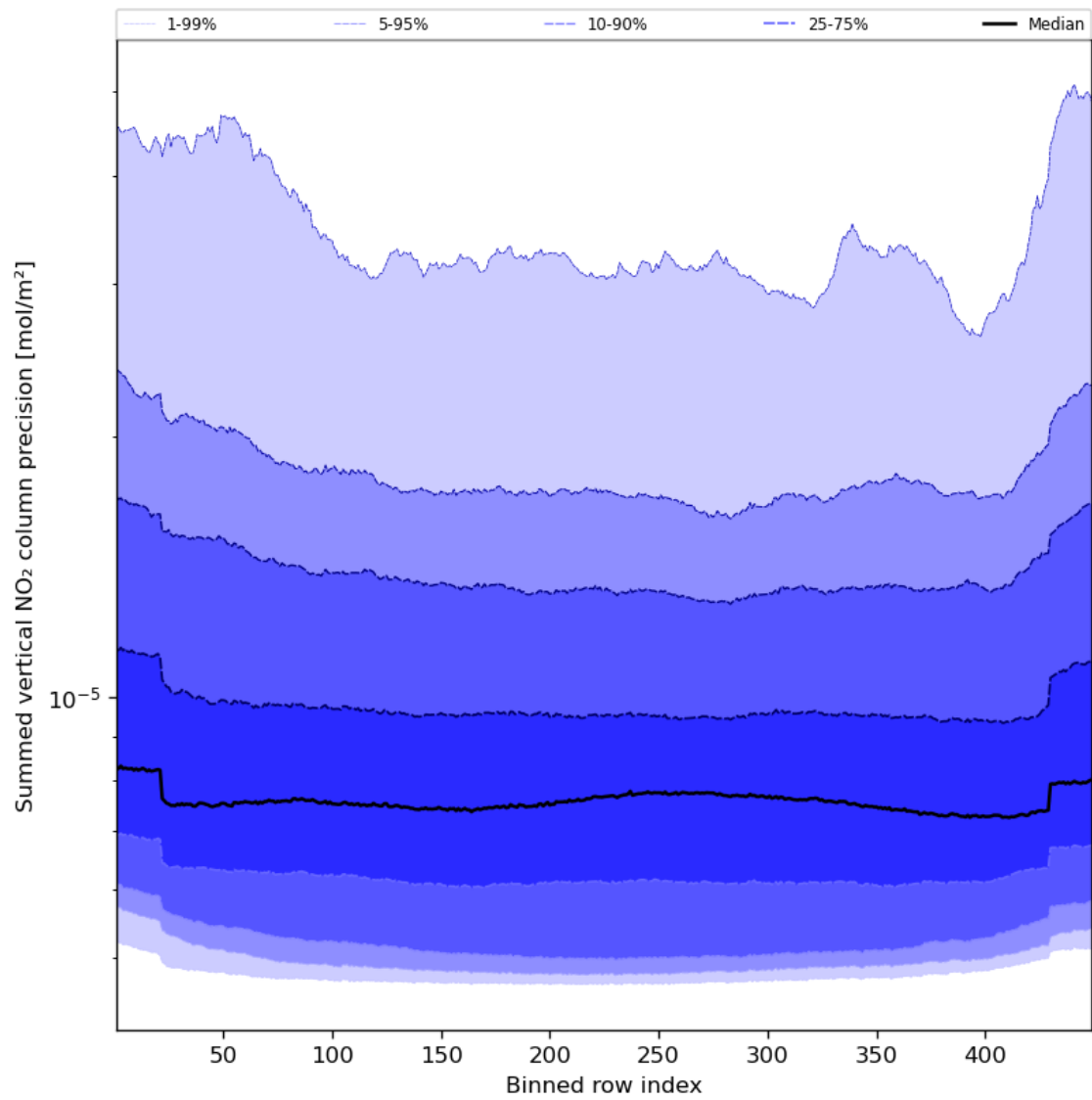
Figure 58: Along track statistics of “Summed vertical NO 2 column precision” for 2024-04-26 to 2024-04-28
