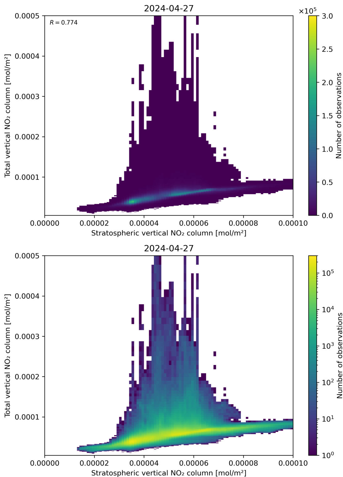
Figure 100: Scatter density plot of “Stratospheric vertical NO 2 column” against “Total vertical NO 2 column” for 2024-04-26 to 2024-04-28.
