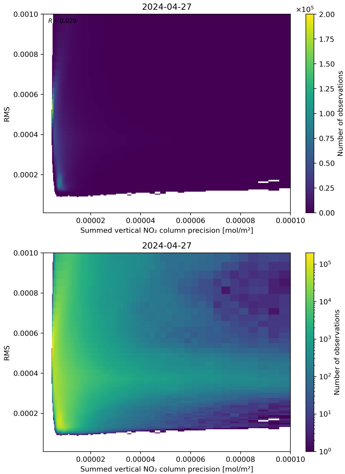
Figure 108: Scatter density plot of “Summed vertical NO 2 column precision” against “RMS” for 2024-04-26 to 2024-04-28.
