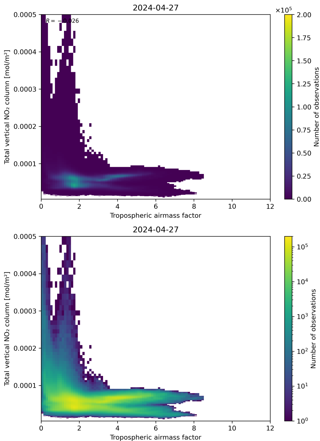
Figure 77: Scatter density plot of “Tropospheric airmass factor” against “Total vertical NO 2 column” for 2024-04-26 to 2024-04-28.
