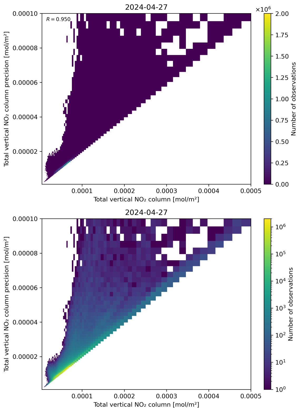
Figure 114: Scatter density plot of “Total vertical NO 2 column” against “Total vertical NO 2 column precision” for 2024-04-26 to 2024-04-28.
