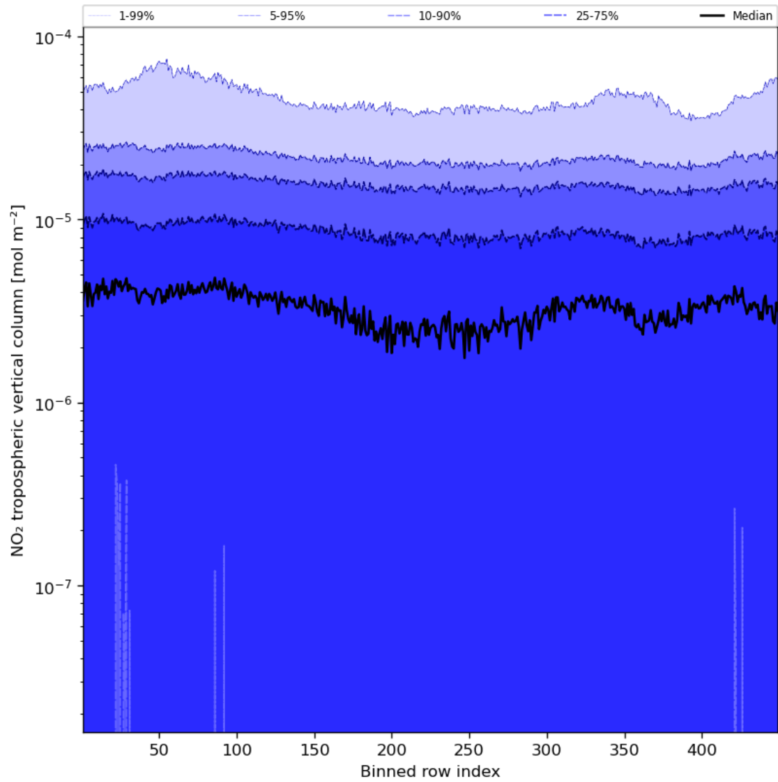
Figure 46: Along track statistics of “NO 2 tropospheric vertical column” for 2024-04-26 to 2024-04-28
