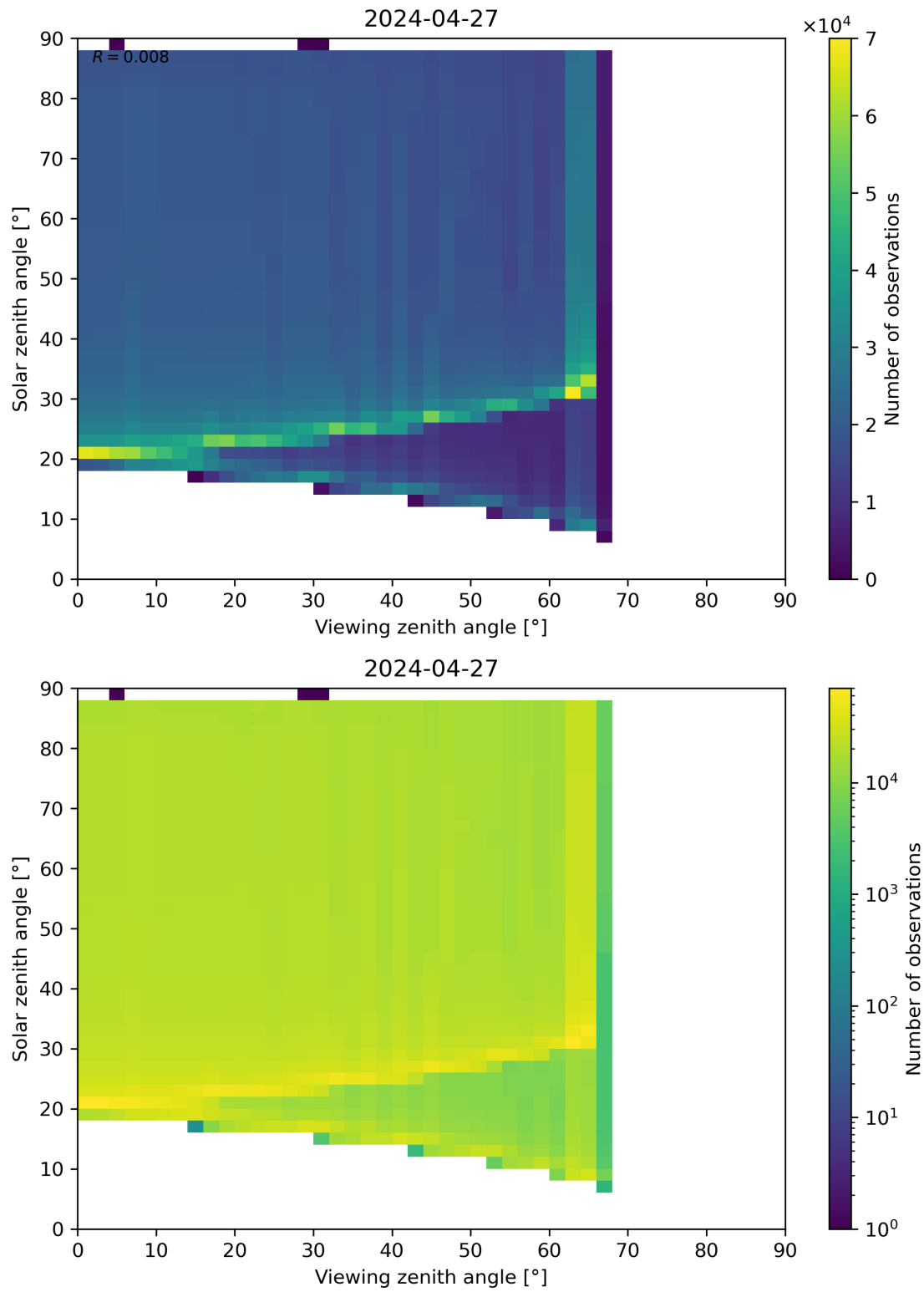
Figure 172: Scatter density plot of “Viewing zenith angle” against “Solar zenith angle” for 2024-04-26 to 2024-04-28.
