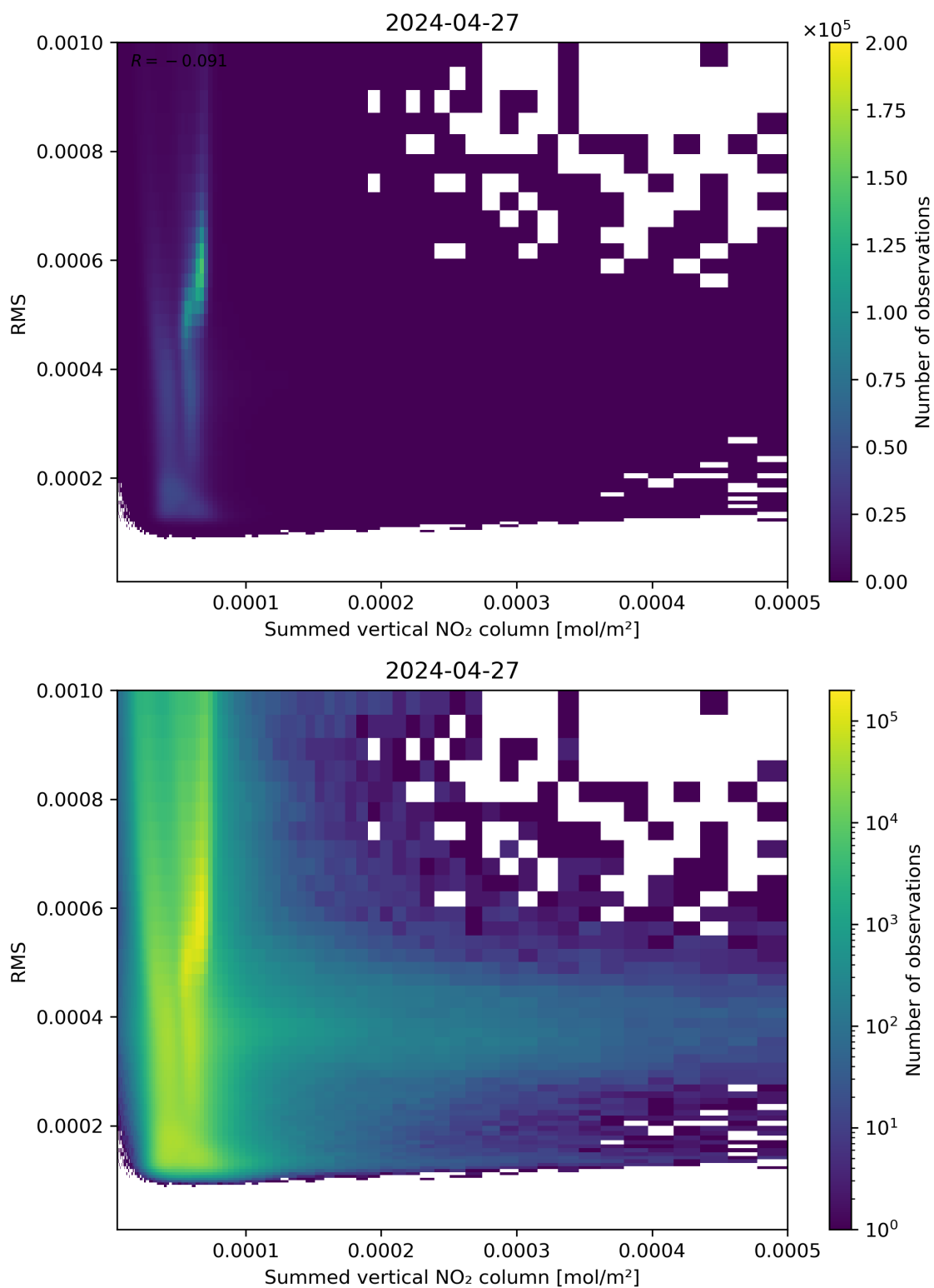
Figure 109: Scatter density plot of “Summed vertical NO 2 column” against “RMS” for 2024-04-26 to 2024-04-28.
