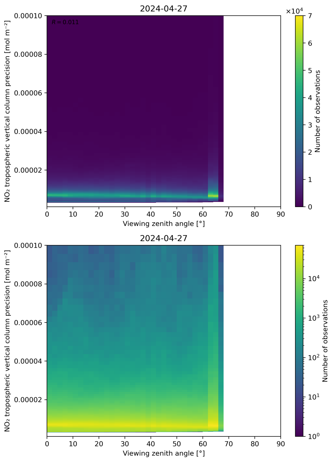
Figure 170: Scatter density plot of “Viewing zenith angle” against “NO 2 tropospheric vertical column precision” for 2024-04-26 to 2024-04-28.
