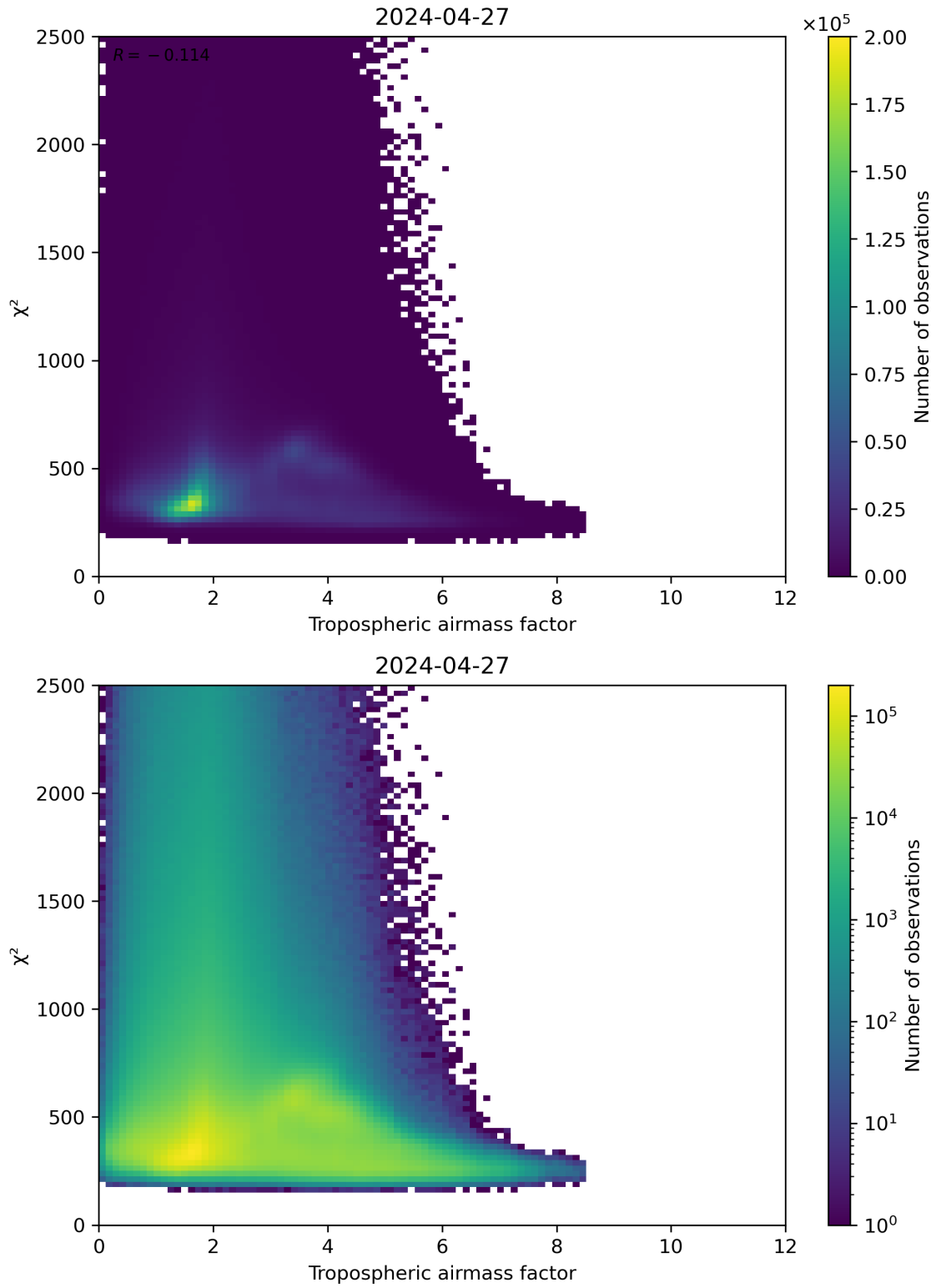
Figure 73: Scatter density plot of “Tropospheric airmass factor” against “ \chi^2 ” for 2024-04-26 to 2024-04-28.
