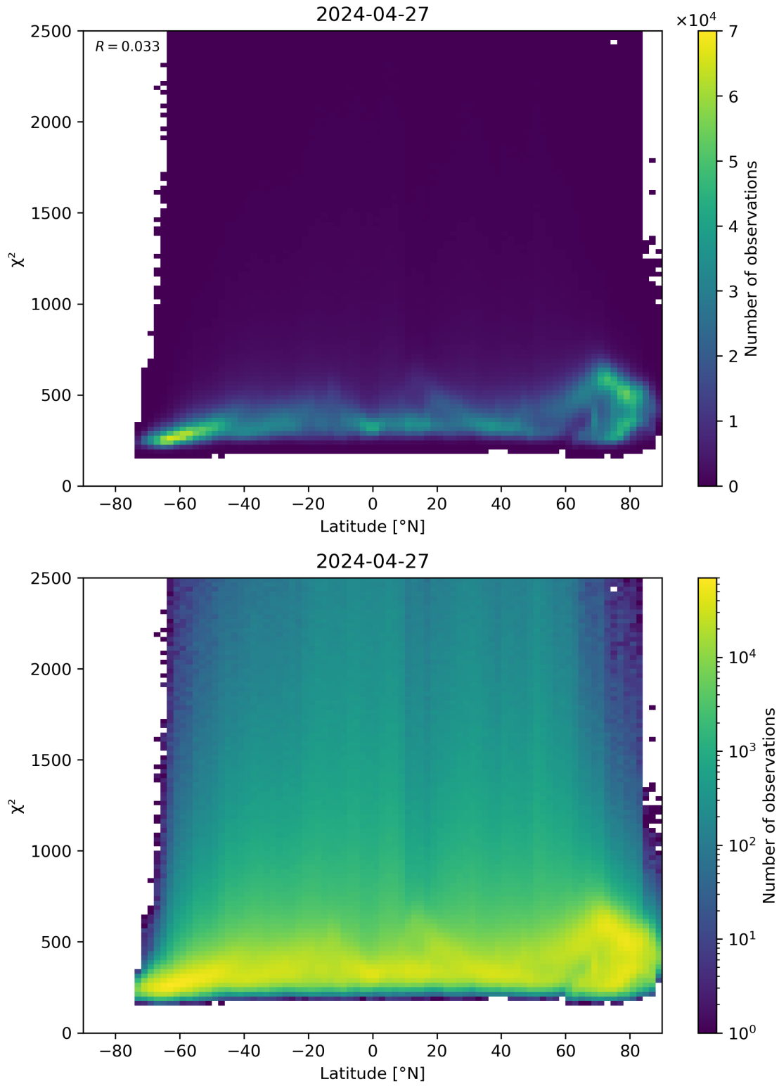
Figure 86: Scatter density plot of “Latitude” against “ \chi^2 ” for 2024-04-26 to 2024-04-28.
