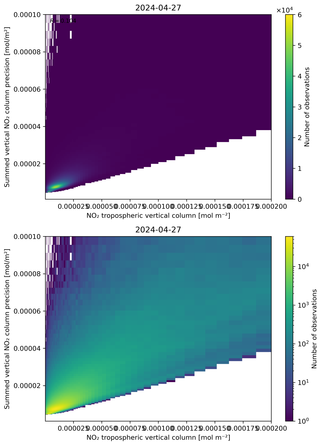
Figure 127: Scatter density plot of “NO 2 tropospheric vertical column” against “Summed vertical NO 2 column precision” for 2024-04-26 to 2024-04-28.
