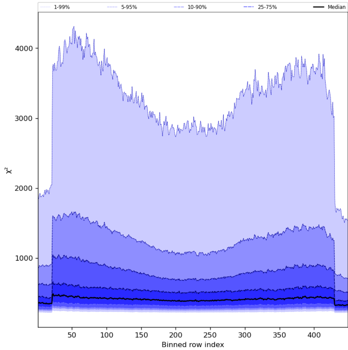
Figure 59: Along track statistics of “ \chi^2 ” for 2024-04-26 to 2024-04-28
