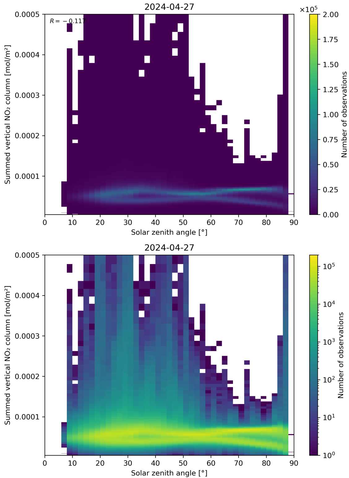
Figure 151: Scatter density plot of “Solar zenith angle” against “Summed vertical NO 2 column” for 2024-04-26 to 2024-04-28.
