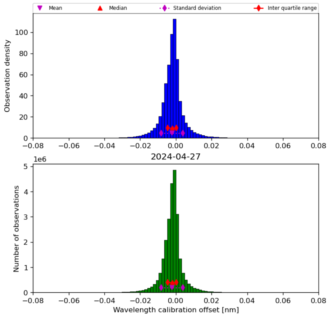
Figure 35: Histogram of “Wavelength calibration offset” for 2024-04-26 to 2024-04-28
