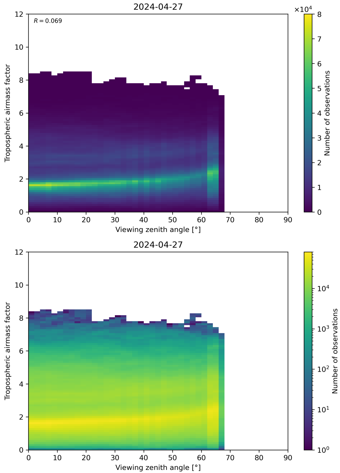
Figure 161: Scatter density plot of “Viewing zenith angle” against “Tropospheric airmass factor” for 2024-04-26 to 2024-04-28.
