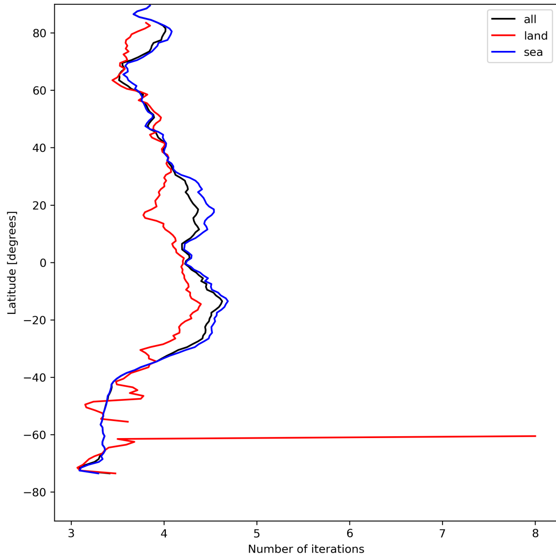
Figure 17: Zonal average of “Number of iterations” for 2024-04-26 to 2024-04-28.
