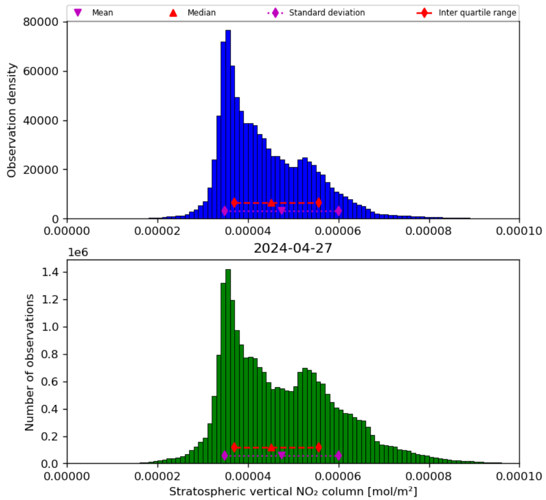
Figure 36: Histogram of “Stratospheric vertical NO 2 column” for 2024-04-26 to 2024-04-28
