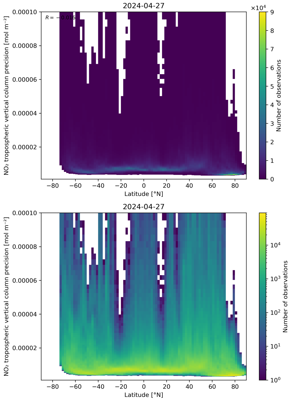
Figure 93: Scatter density plot of “Latitude” against “NO 2 tropospheric vertical column precision” for 2024-04-26 to 2024-04-28.
