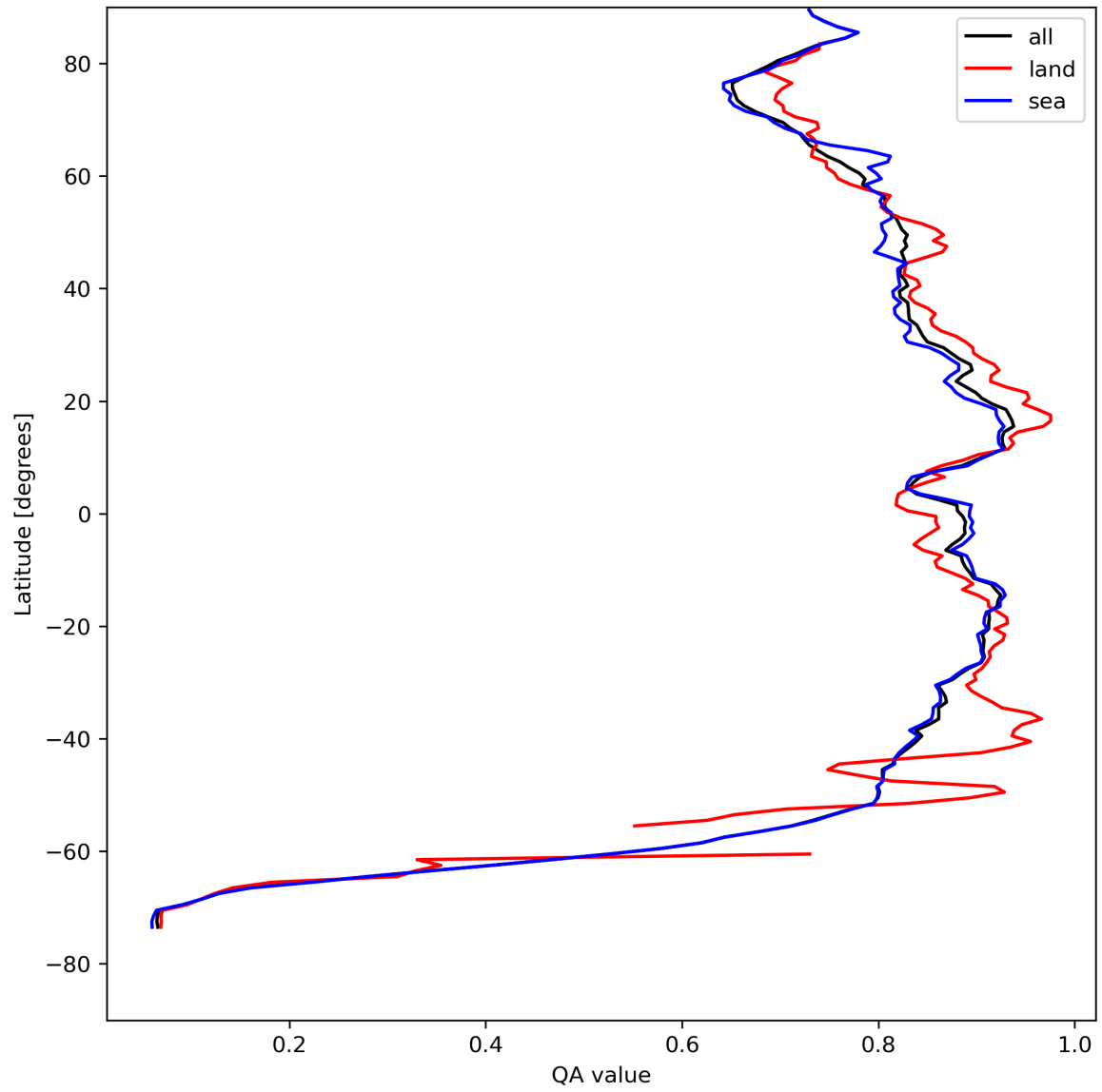
Figure 11: Zonal average of “QA value” for 2024-04-26 to 2024-04-28.
