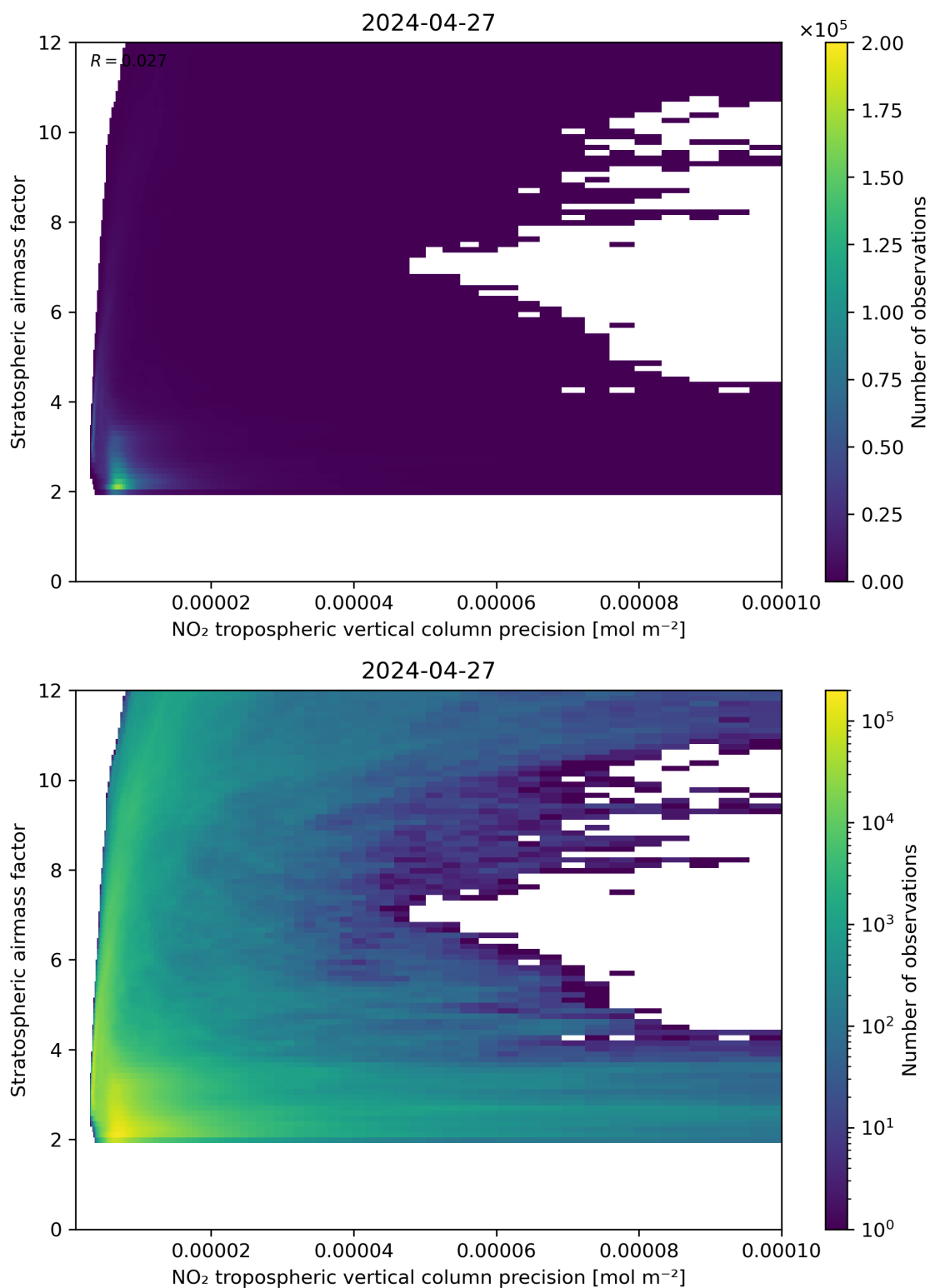
Figure 131: Scatter density plot of “NO 2 tropospheric vertical column precision” against “Stratospheric airmass factor” for 2024-04-26 to 2024-04-28.
