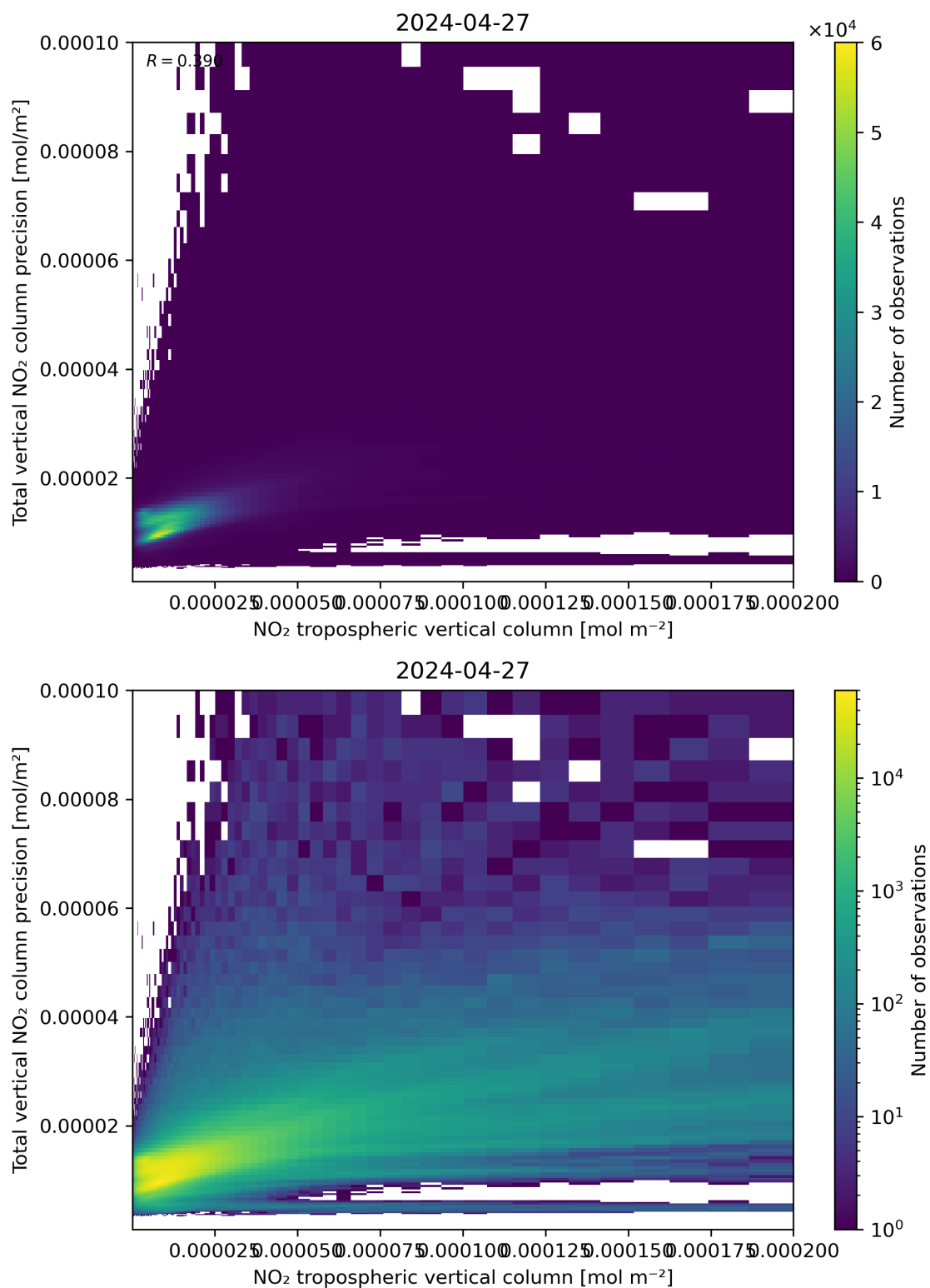
Figure 129: Scatter density plot of “NO 2 tropospheric vertical column” against “Total vertical NO 2 column precision” for 2024-04-26 to 2024-04-28.
