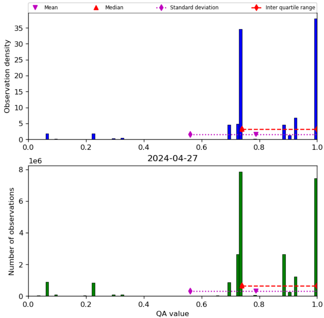
Figure 28: Histogram of “QA value” for 2024-04-26 to 2024-04-28
