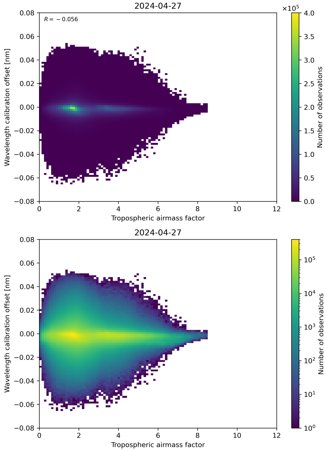
Figure 80: Scatter density plot of “Tropospheric airmass factor” against “Wavelength calibration offset” for 2024-04-26 to 2024-04-28.
