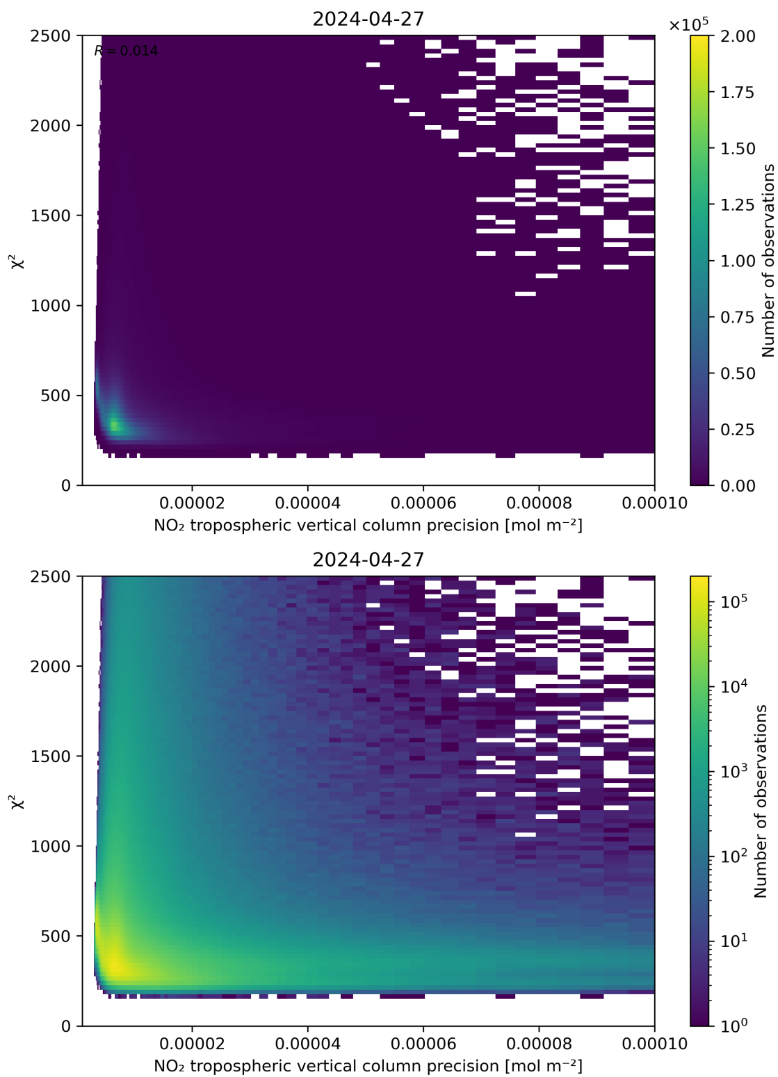
Figure 134: Scatter density plot of “NO 2 tropospheric vertical column precision” against “ \chi^2 ” for 2024-04-26 to 2024-04-28.
