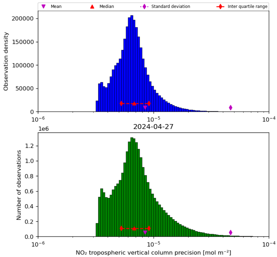
Figure 30: Histogram of “NO 2 tropospheric vertical column precision” for 2024-04-26 to 2024-04-28
