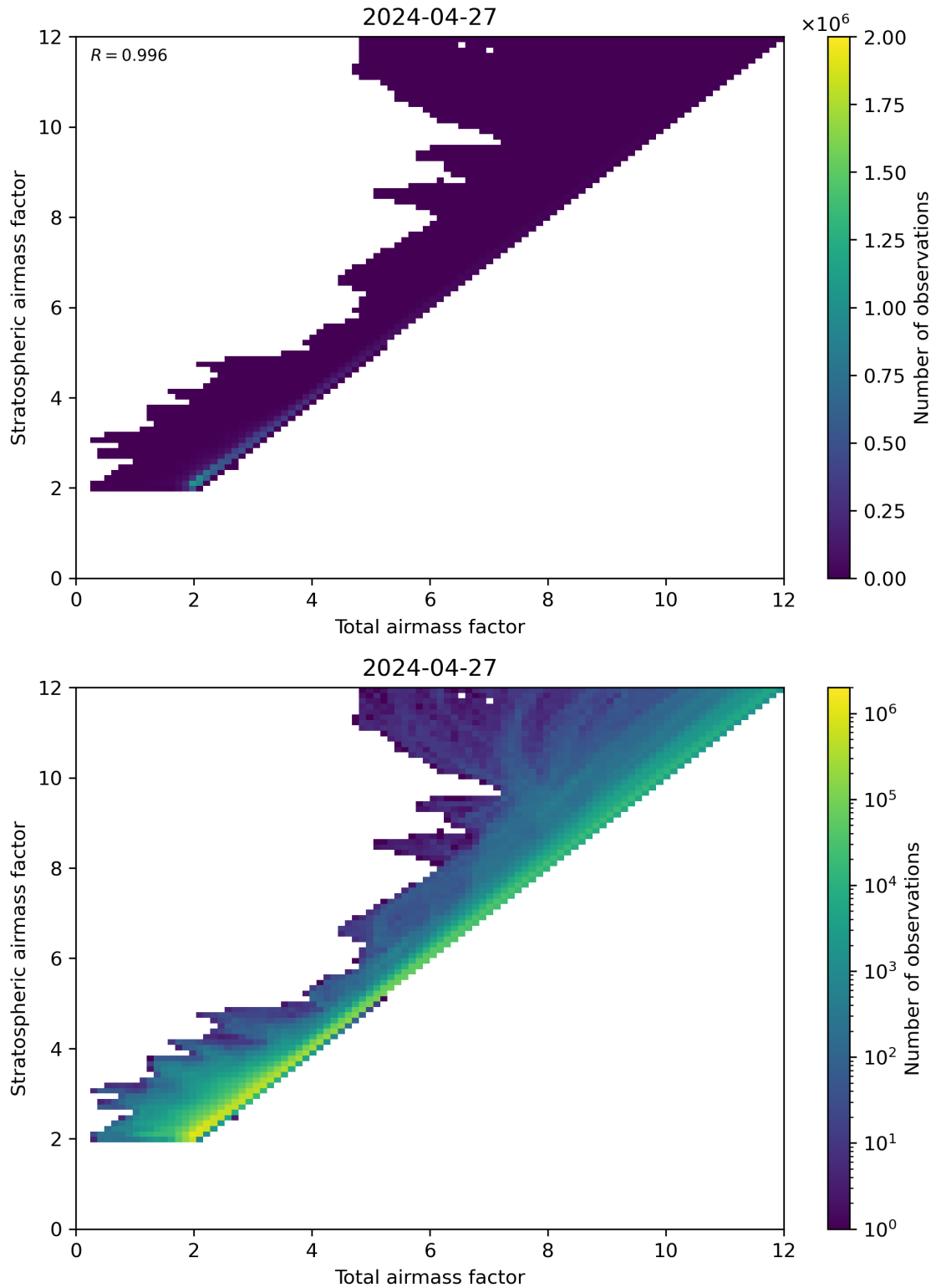
Figure 62: Scatter density plot of “Total airmass factor” against “Stratospheric airmass factor” for 2024-04-26 to 2024-04-28.
