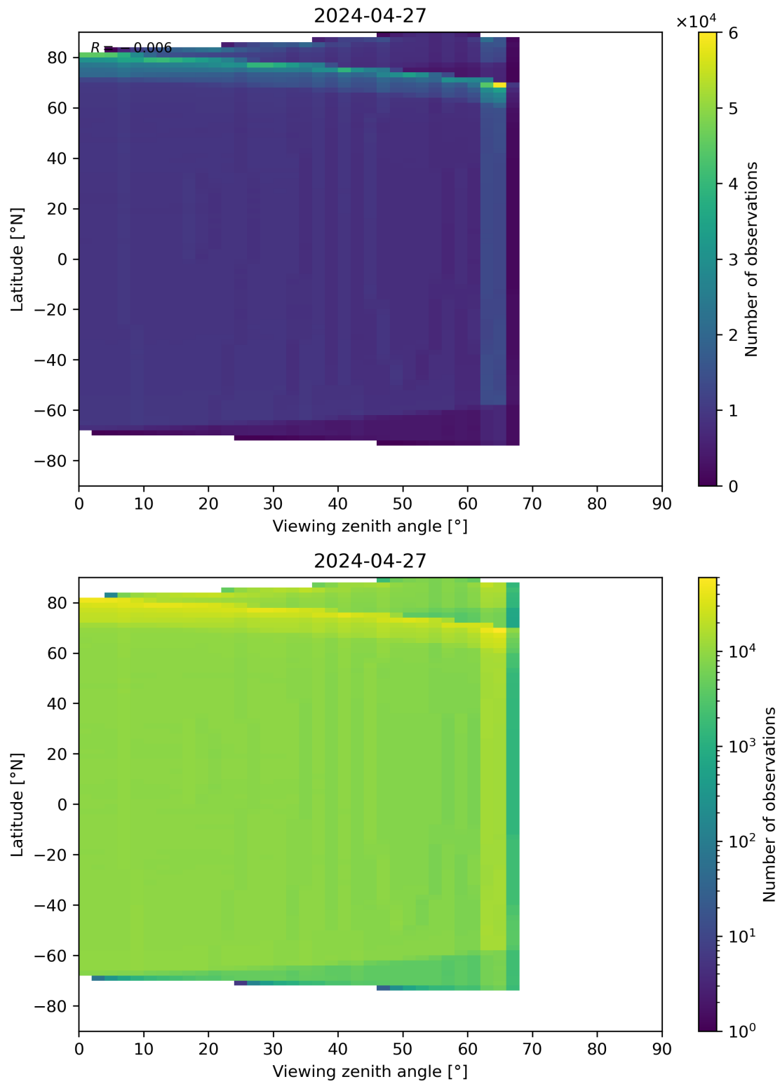
Figure 163: Scatter density plot of “Viewing zenith angle” against “Latitude” for 2024-04-26 to 2024-04-28.
