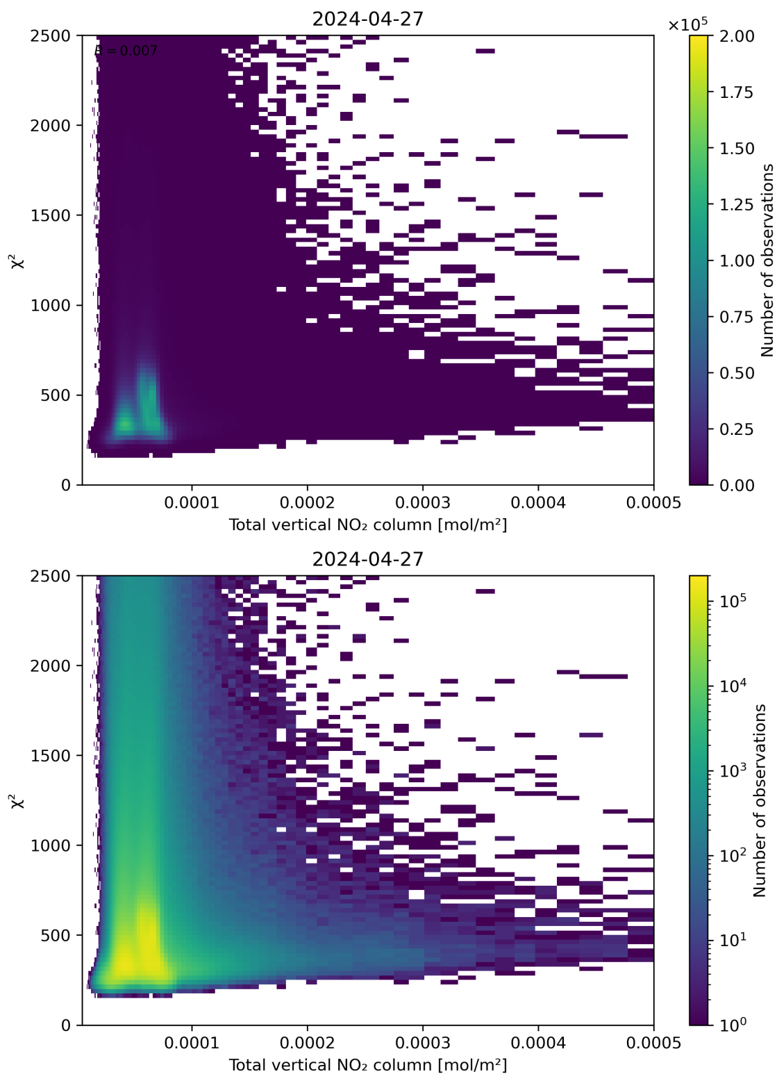
Figure 111: Scatter density plot of “Total vertical NO 2 column” against “ \chi^2 ” for 2024-04-26 to 2024-04-28.
