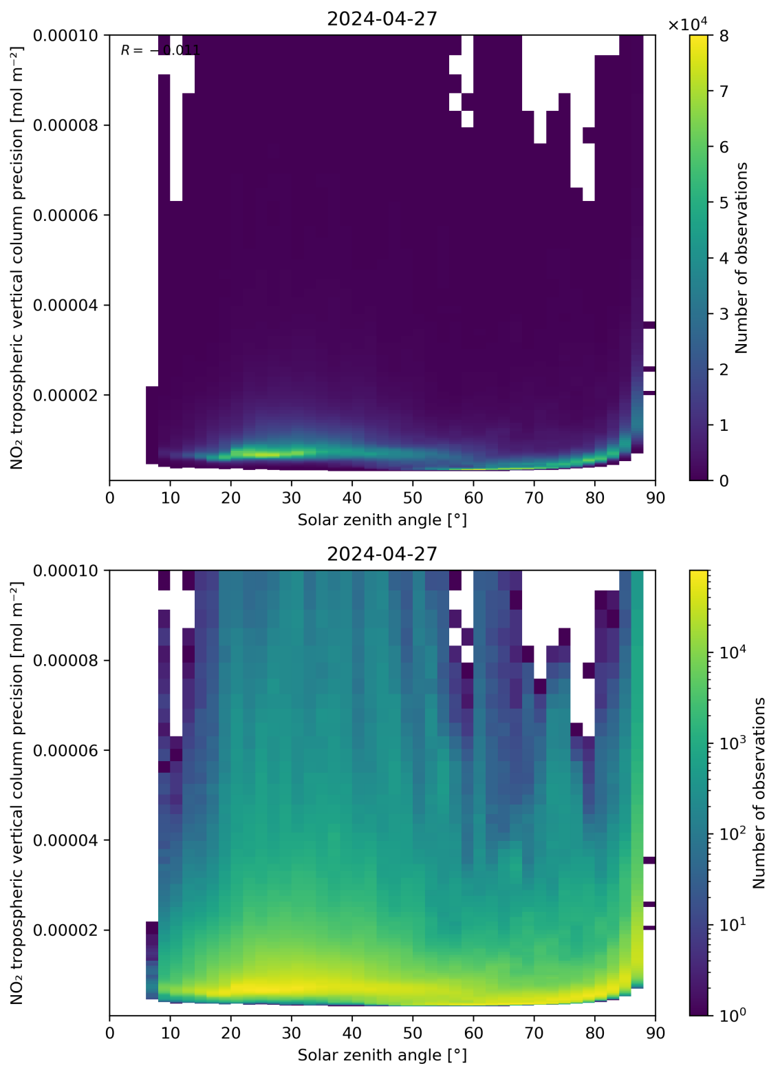
Figure 156: Scatter density plot of “Solar zenith angle” against “NO 2 tropospheric vertical column precision” for 2024-04-26 to 2024-04-28.
