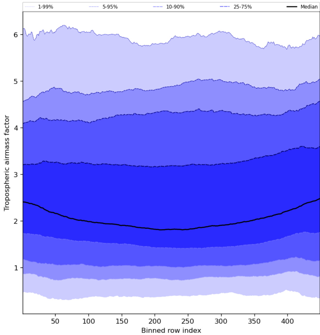
Figure 48: Along track statistics of “Tropospheric airmass factor” for 2024-04-26 to 2024-04-28
