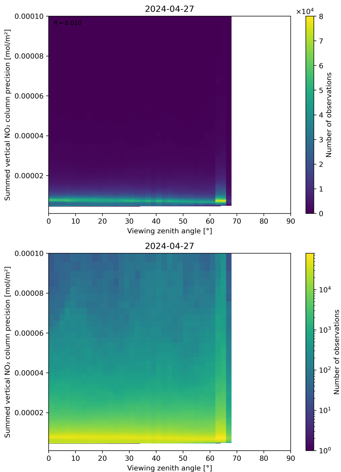
Figure 166: Scatter density plot of “Viewing zenith angle” against “Summed vertical NO 2 column precision” for 2024-04-26 to 2024-04-28.
