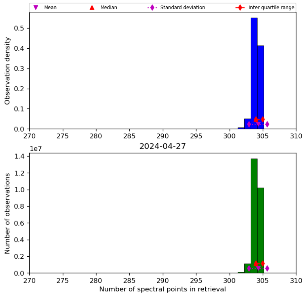
Figure 33: Histogram of “Number of spectral points in retrieval” for 2024-04-26 to 2024-04-28
