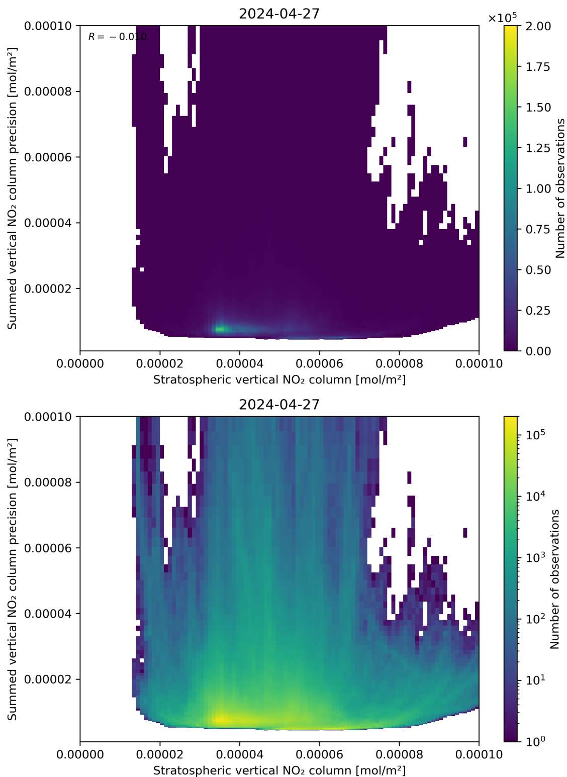
Figure 99: Scatter density plot of “Stratospheric vertical NO 2 column” against “Summed vertical NO 2 column precision” for 2024-04-26 to 2024-04-28.
