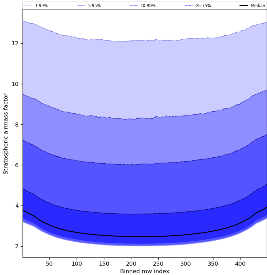
Figure 61: Along track statistics of “Stratospheric airmass factor” for 2024-04-26 to 2024-04-28
