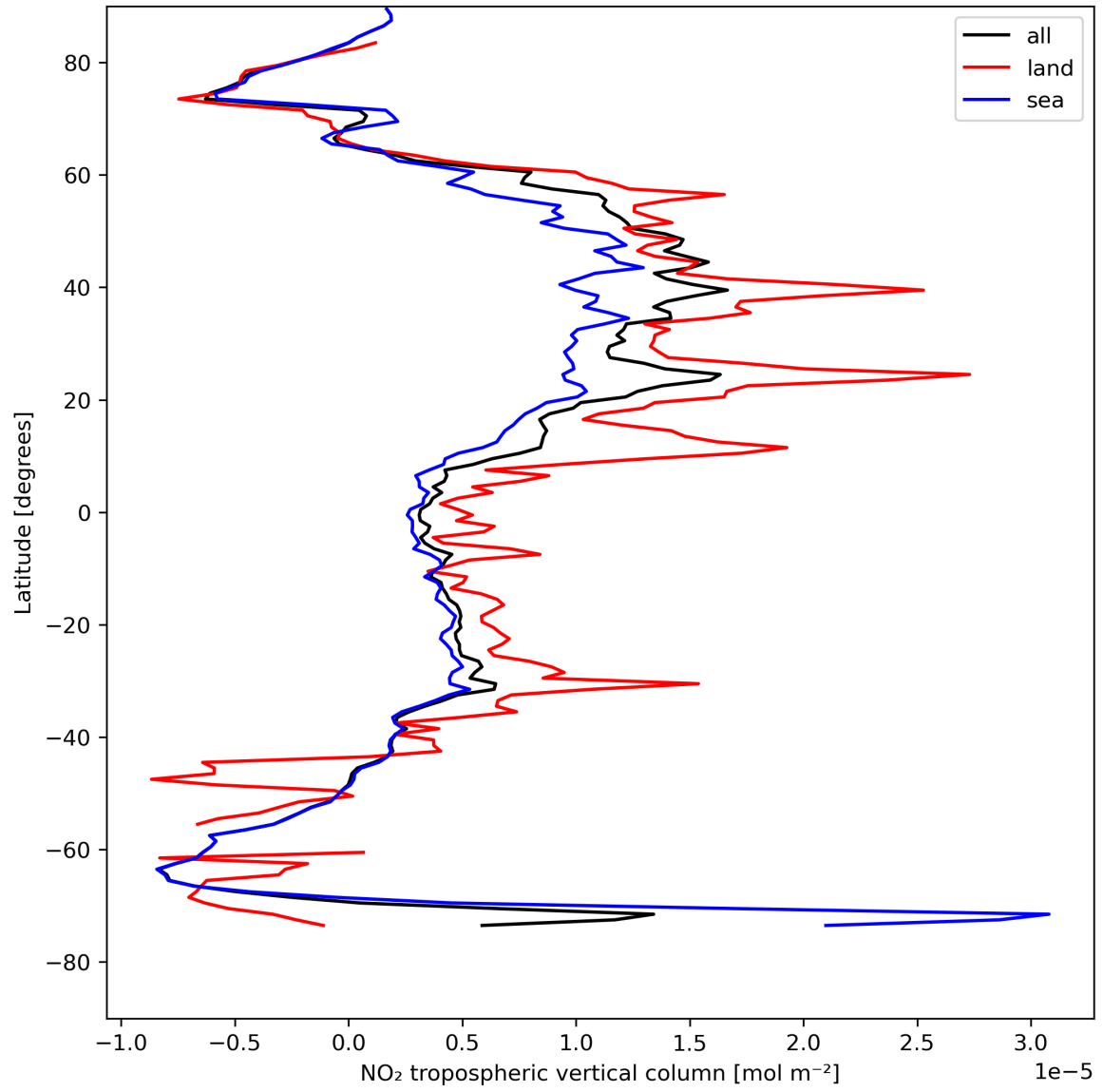
Figure 12: Zonal average of “NO 2 tropospheric vertical column” for 2024-04-26 to 2024-04-28.
