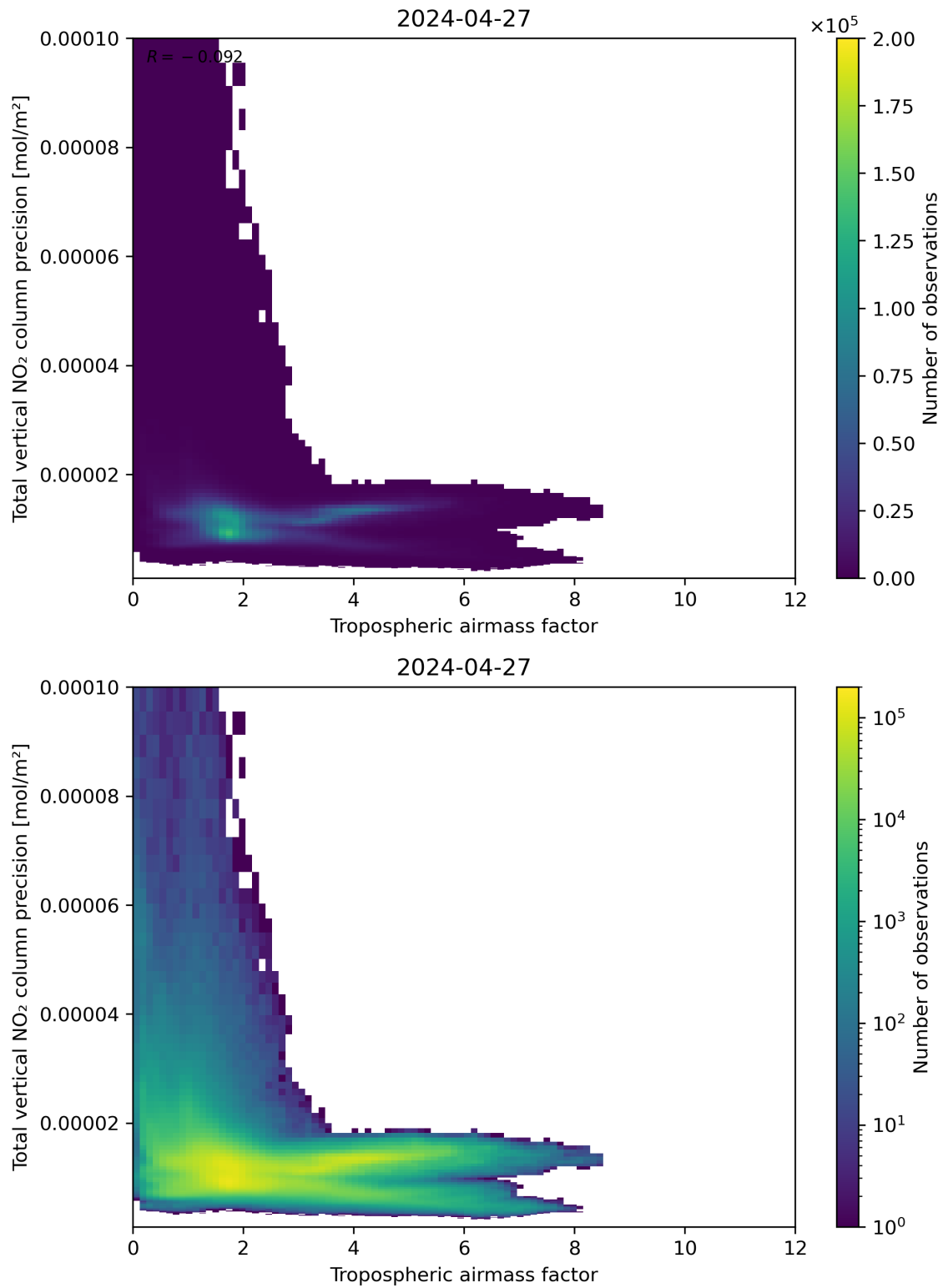
Figure 78: Scatter density plot of “Tropospheric air mass factor” against “Total vertical NO 2 column precision” for 2024-04-26 to 2024-04-28.
