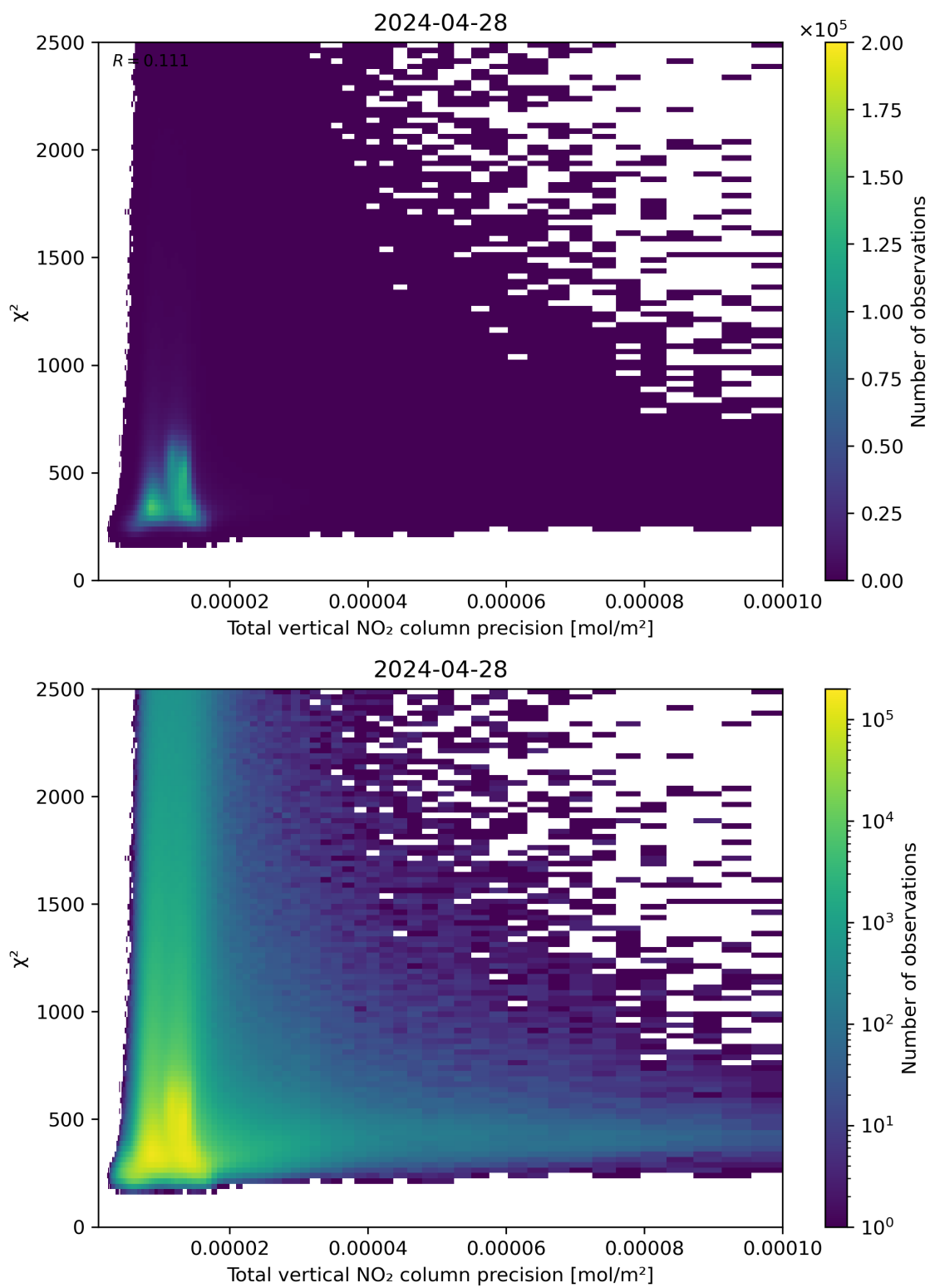
Figure 116: Scatter density plot of “Total vertical NO 2 column precision” against “ \chi^2 ” for 2024-04-27 to 2024-04-29.
