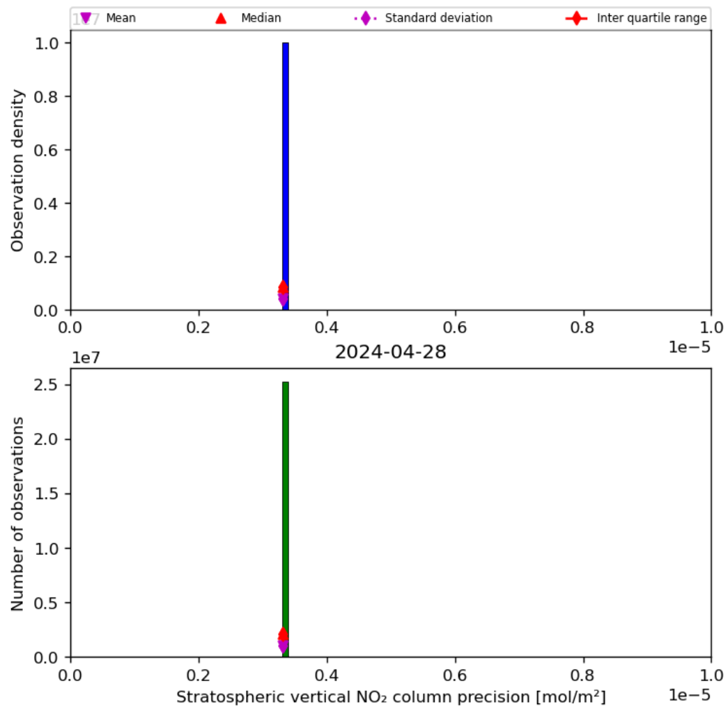
Figure 37: Histogram of “Stratospheric vertical NO 2 column precision” for 2024-04-27 to 2024-04-29
