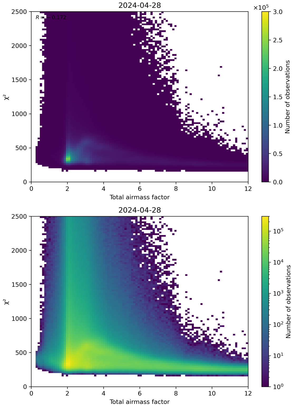
Figure 63: Scatter density plot of “Total airmass factor” against “ \chi^2 ” for 2024-04-27 to 2024-04-29.
