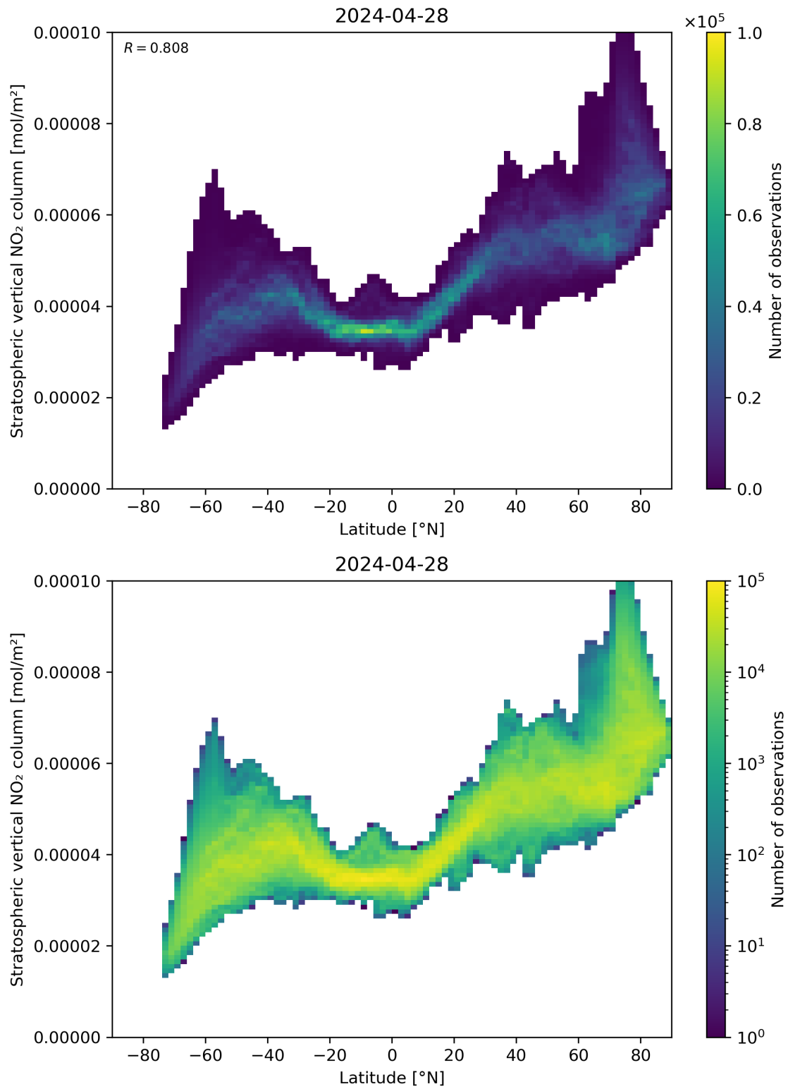
Figure 87: Scatter density plot of “Latitude” against “Stratospheric vertical \text{NO}_2 column” for 2024-04-27 to 2024-04-29.
