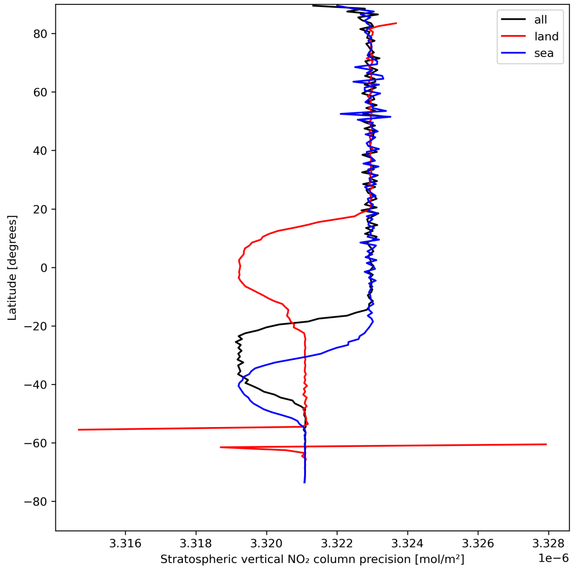
Figure 20: Zonal average of “Stratospheric vertical NO 2 column precision” for 2024-04-27 to 2024-04-29.
