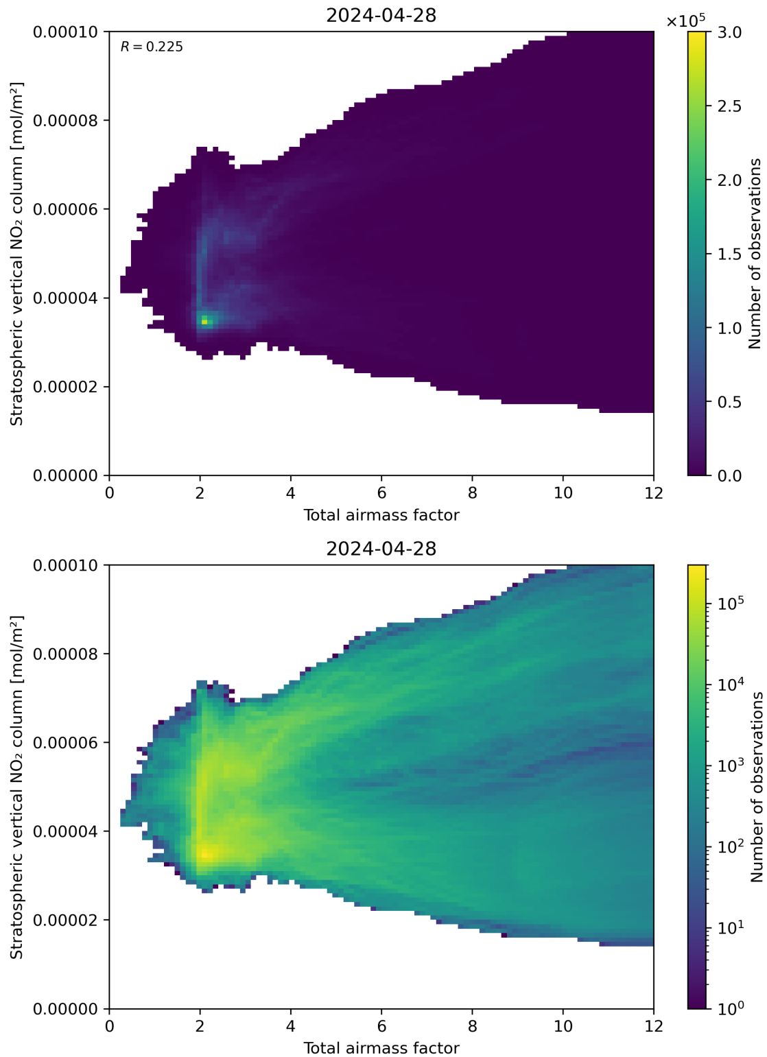
Figure 64: Scatter density plot of “Total airmass factor” against “Stratospheric vertical \text{NO}_2 column” for 2024-04-27 to 2024-04-29.
