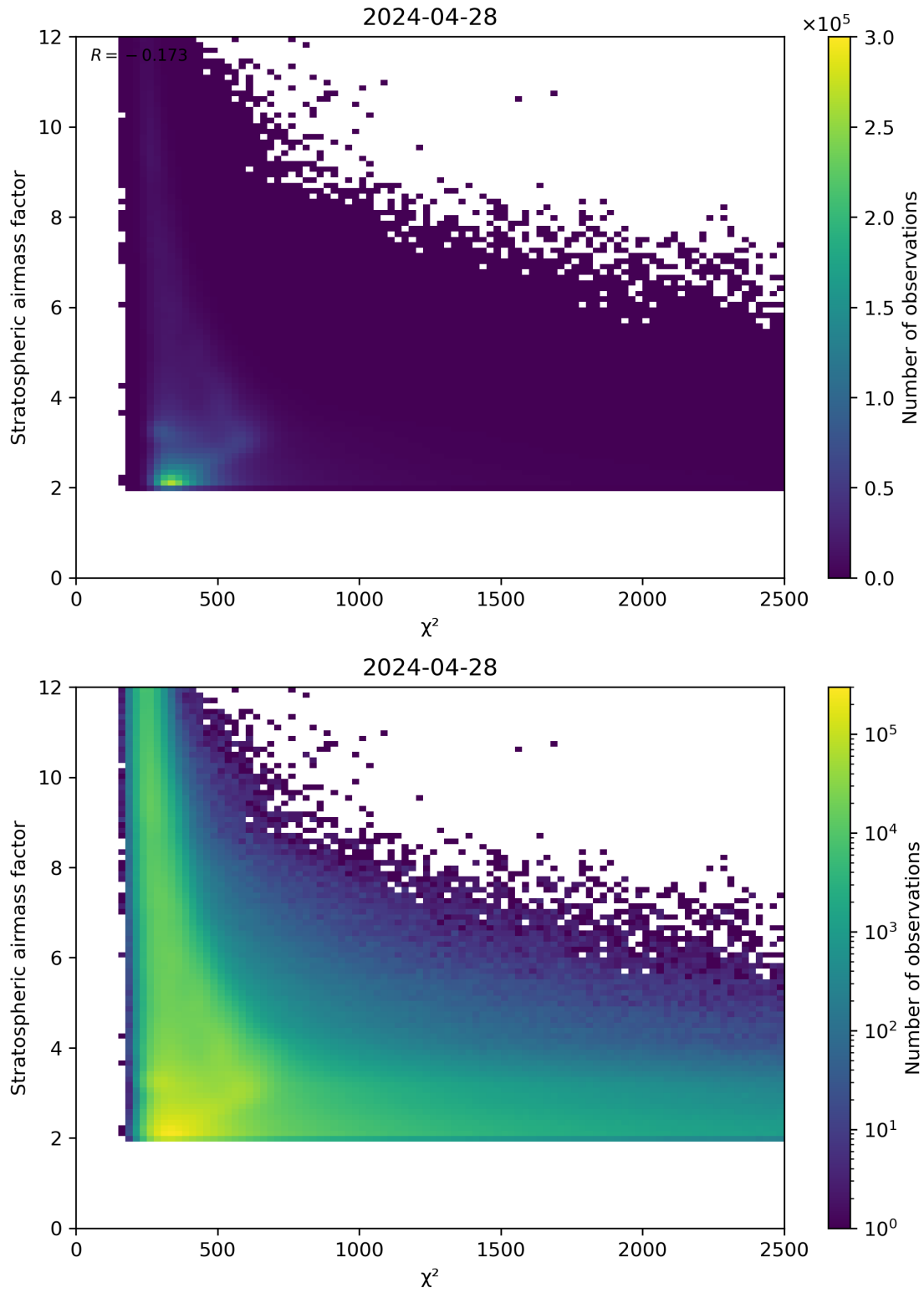
Figure 81: Scatter density plot of “ \chi^2 ” against “Stratospheric airmass factor” for 2024-04-27 to 2024-04-29.
