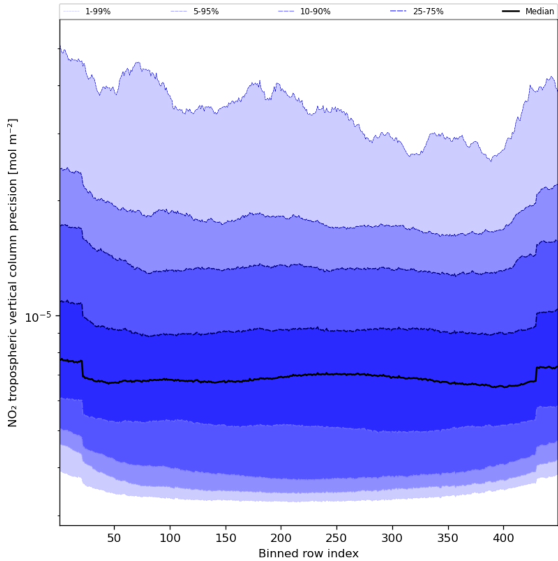
Figure 47: Along track statistics of “NO 2 tropospheric vertical column precision” for 2024-04-27 to 2024-04-29
