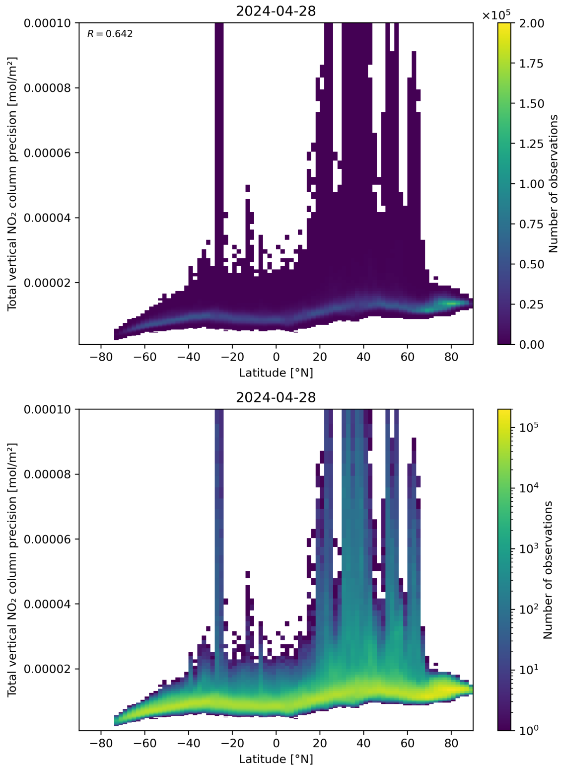
Figure 91: Scatter density plot of “Latitude” against “Total vertical NO 2 column precision” for 2024-04-27 to 2024-04-29.
