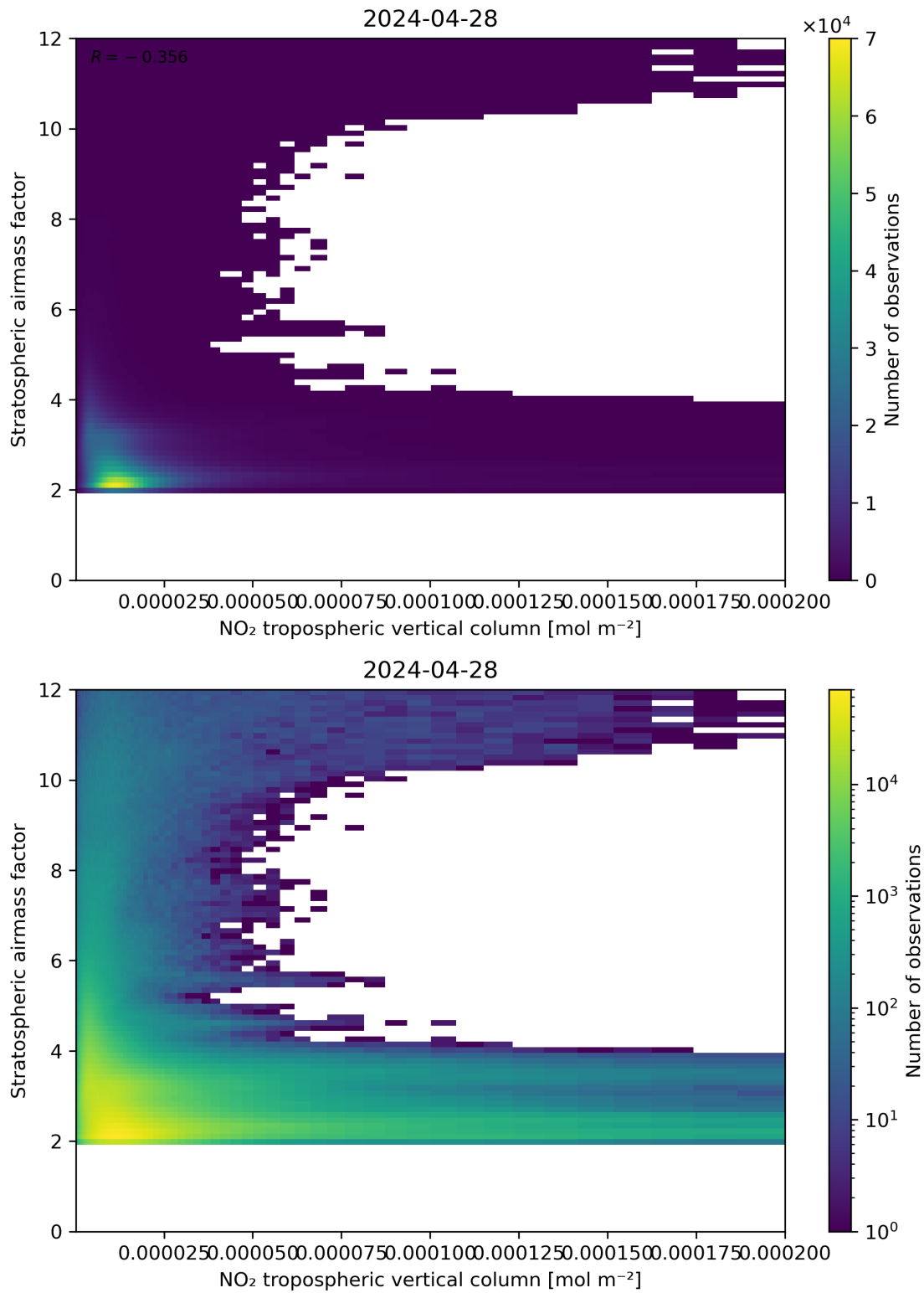
Figure 121: Scatter density plot of “NO 2 tropospheric vertical column” against “Stratospheric air mass factor” for 2024-04-27 to 2024-04-29.
