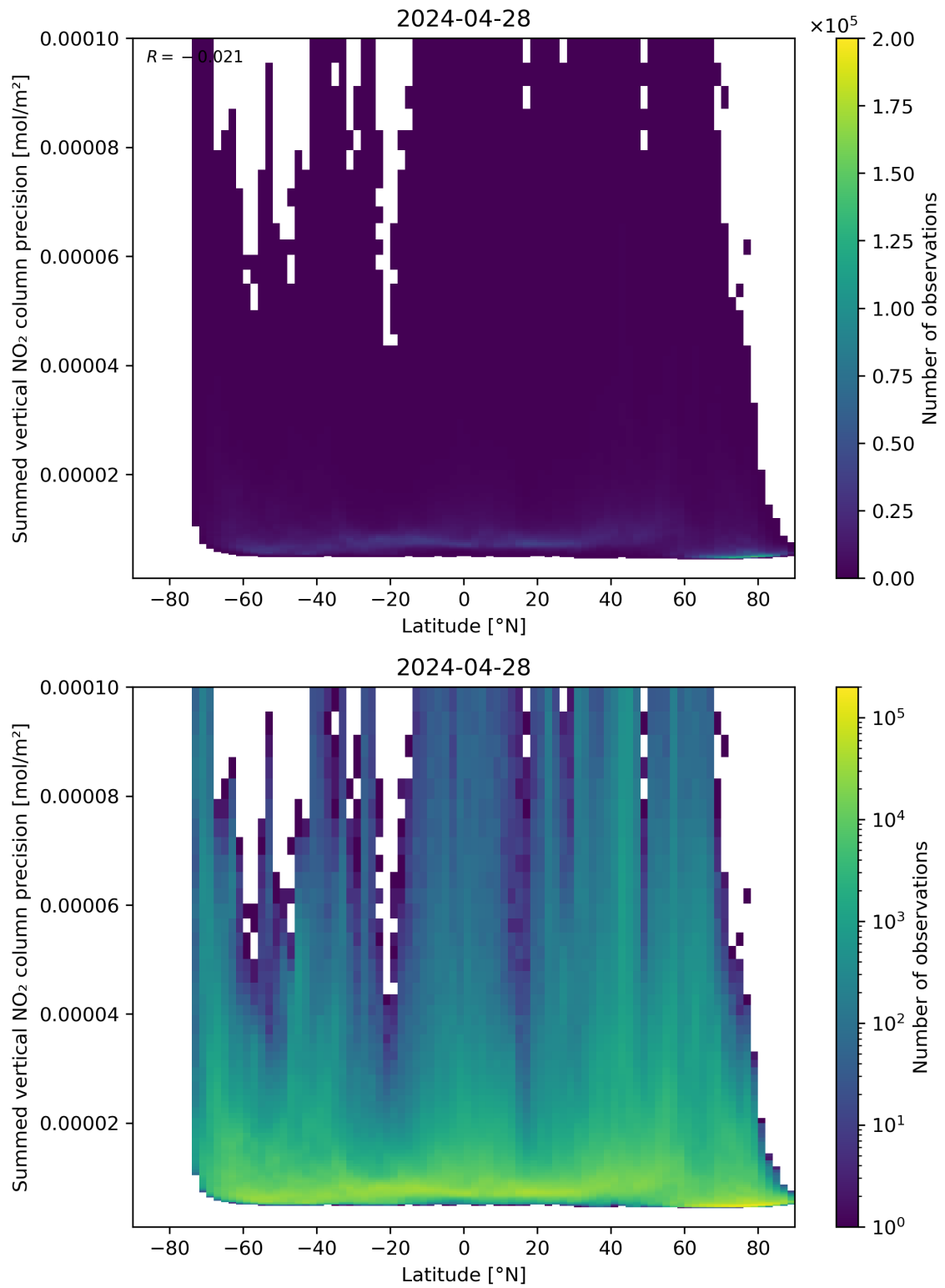
Figure 89: Scatter density plot of “Latitude” against “Summed vertical NO 2 column precision” for 2024-04-27 to 2024-04-29.
