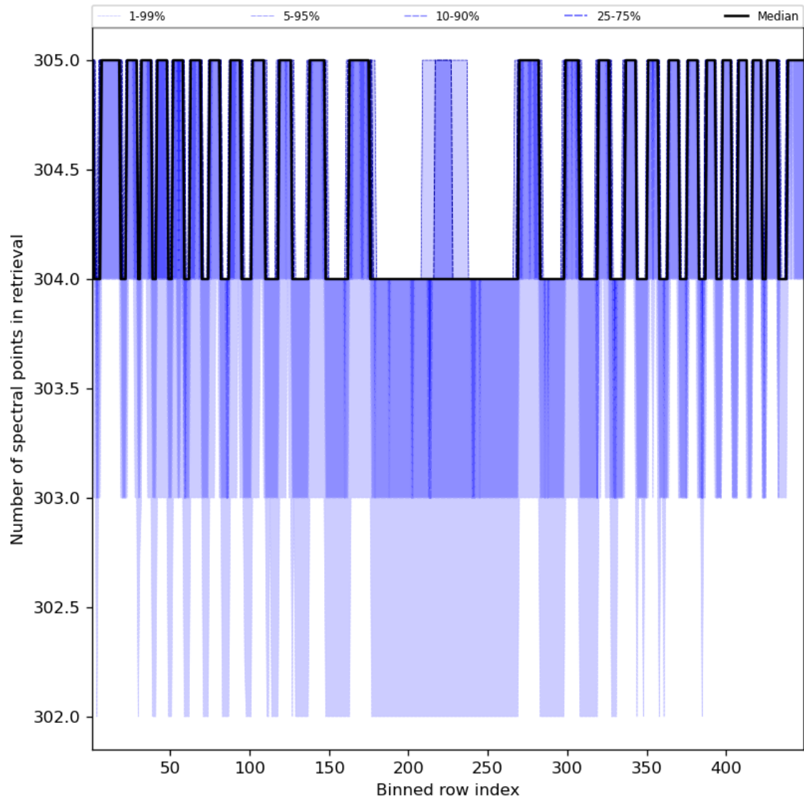
Figure 50: Along track statistics of “Number of spectral points in retrieval” for 2024-04-27 to 2024-04-29
