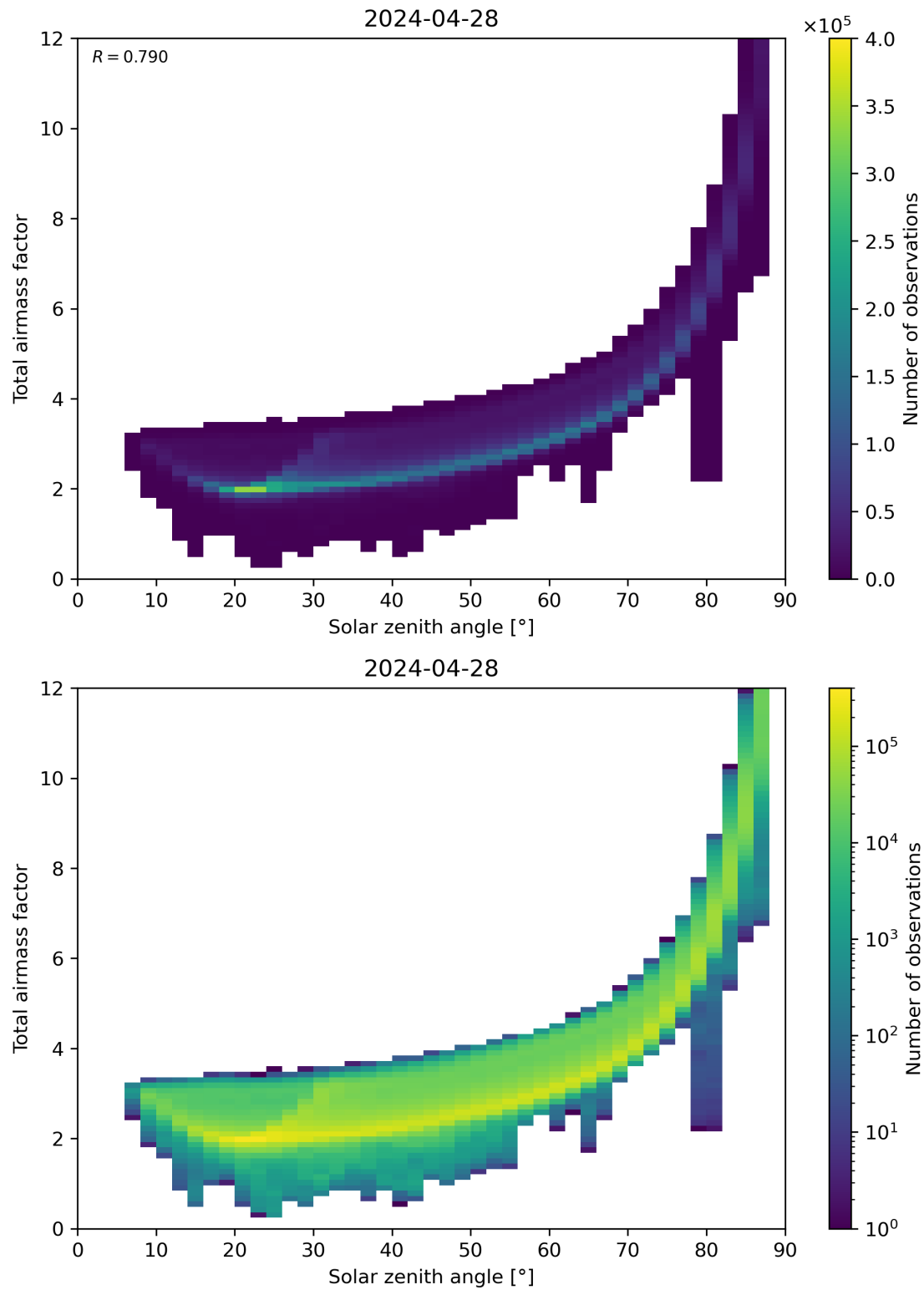
Figure 146: Scatter density plot of “Solar zenith angle” against “Total air mass factor” for 2024-04-27 to 2024-04-29.
