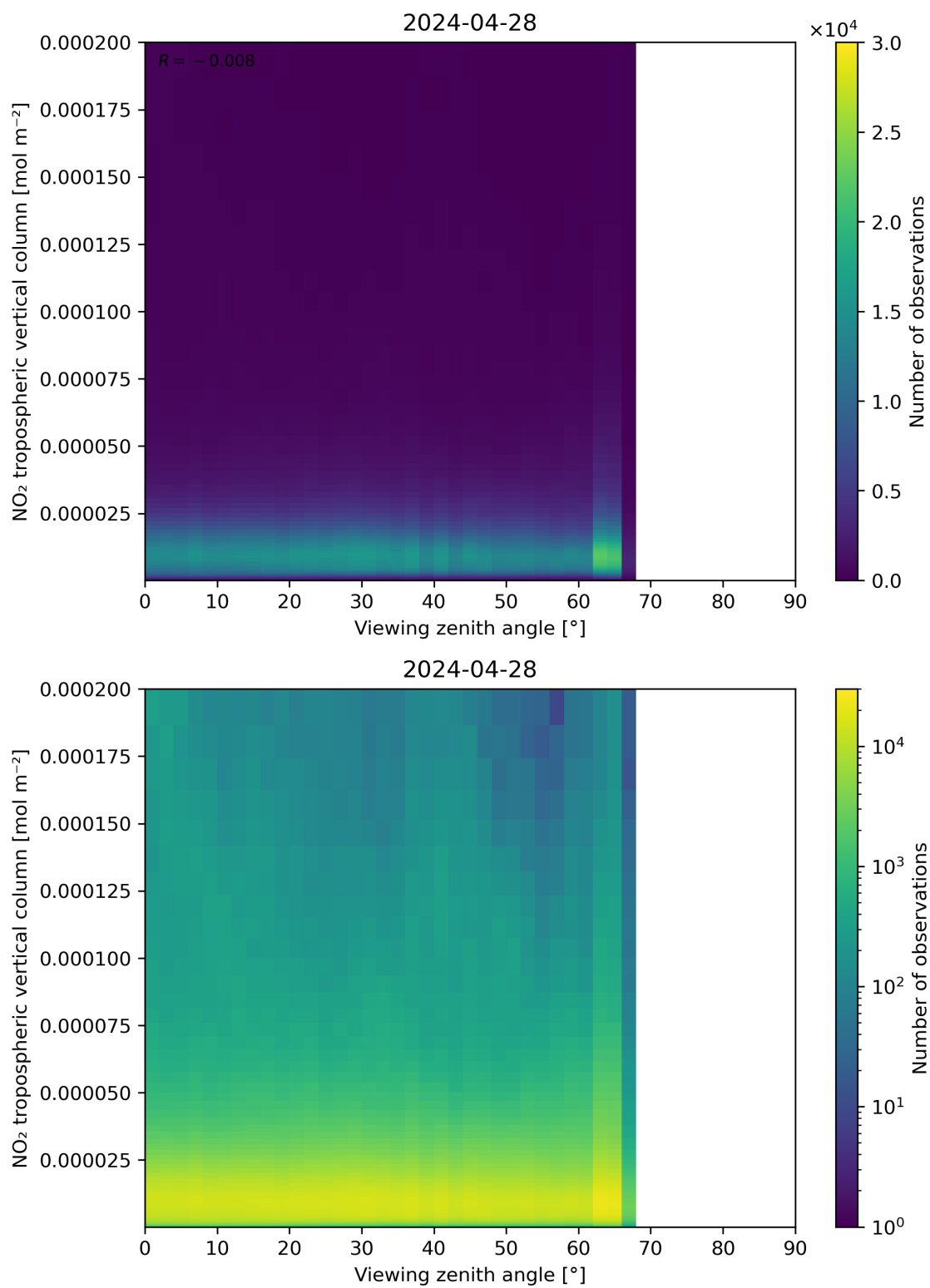
Figure 169: Scatter density plot of “Viewing zenith angle” against “NO 2 tropospheric vertical column” for 2024-04-27 to 2024-04-29.
