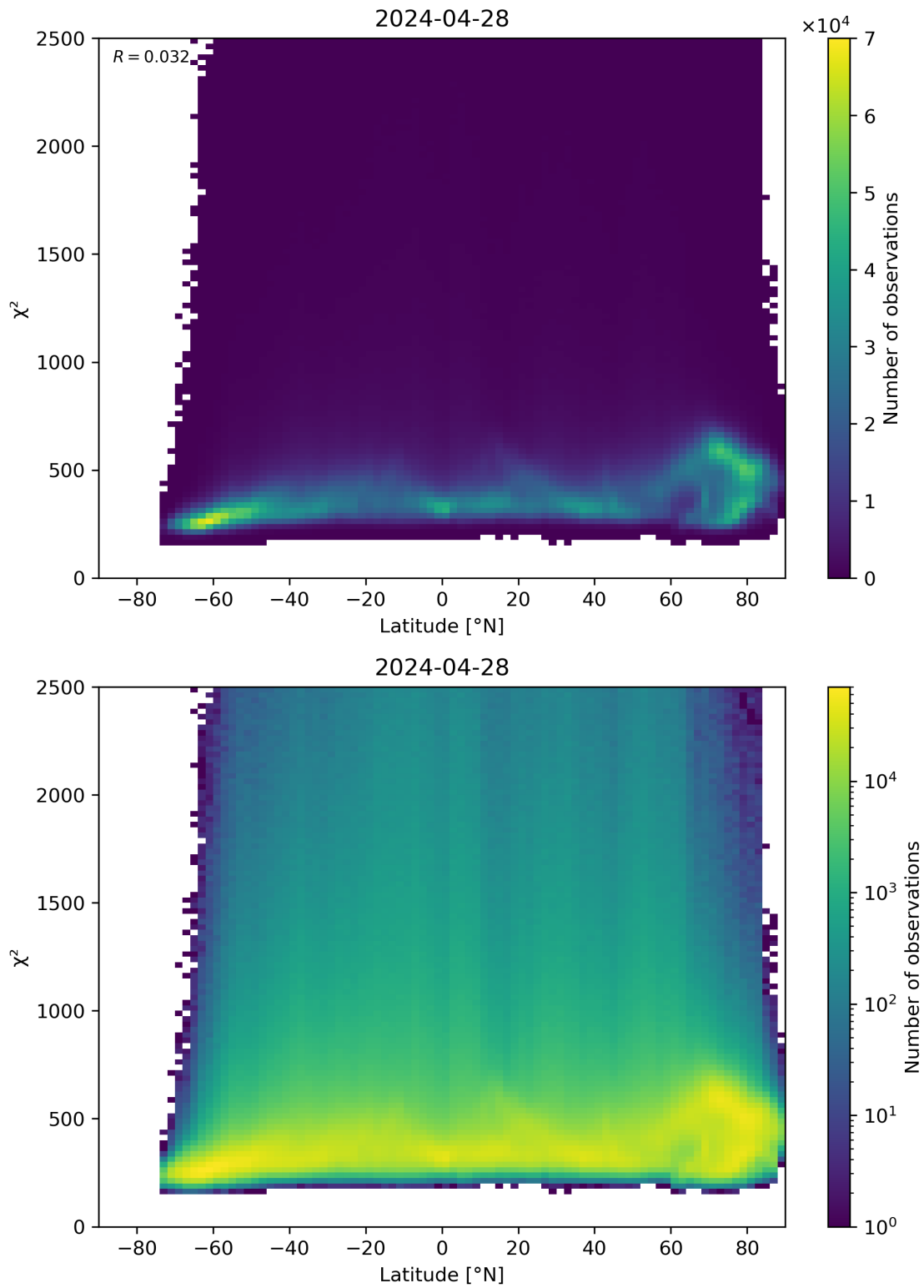
Figure 86: Scatter density plot of “Latitude” against “ \chi^2 ” for 2024-04-27 to 2024-04-29.
