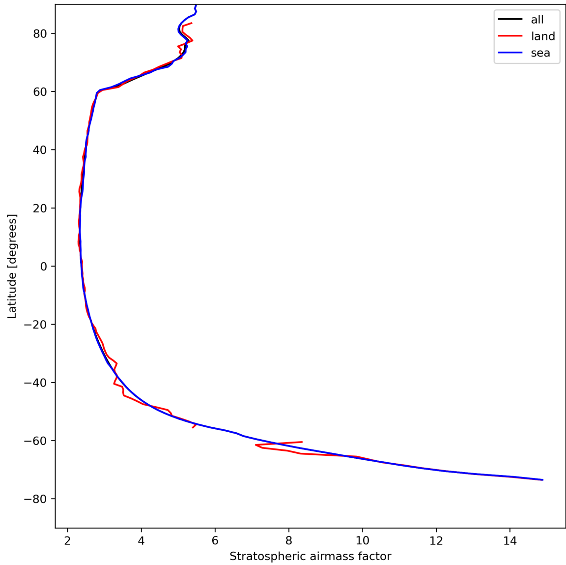
Figure 27: Zonal average of “Stratospheric air mass factor” for 2024-04-27 to 2024-04-29.
