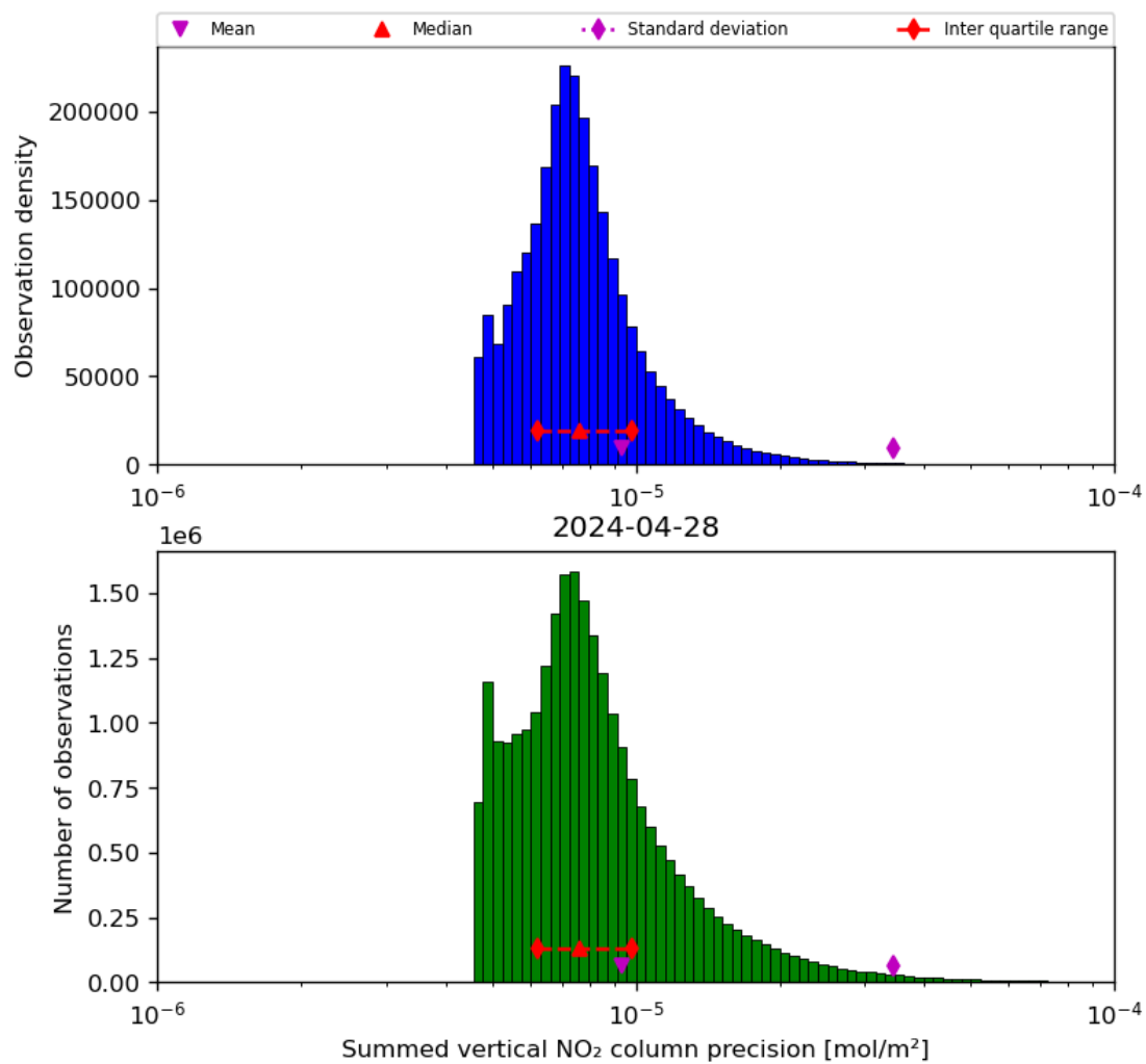
Figure 41: Histogram of “Summed vertical NO 2 column precision” for 2024-04-27 to 2024-04-29
