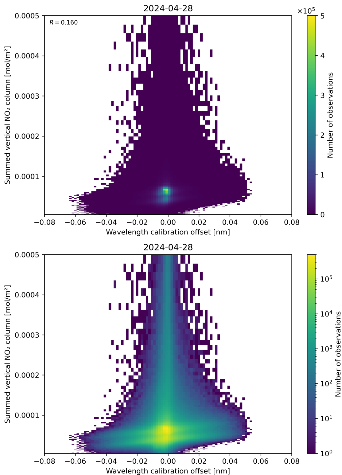
Figure 177: Scatter density plot of “Wavelength calibration offset” against “Summed vertical NO 2 column” for 2024-04-27 to 2024-04-29.
