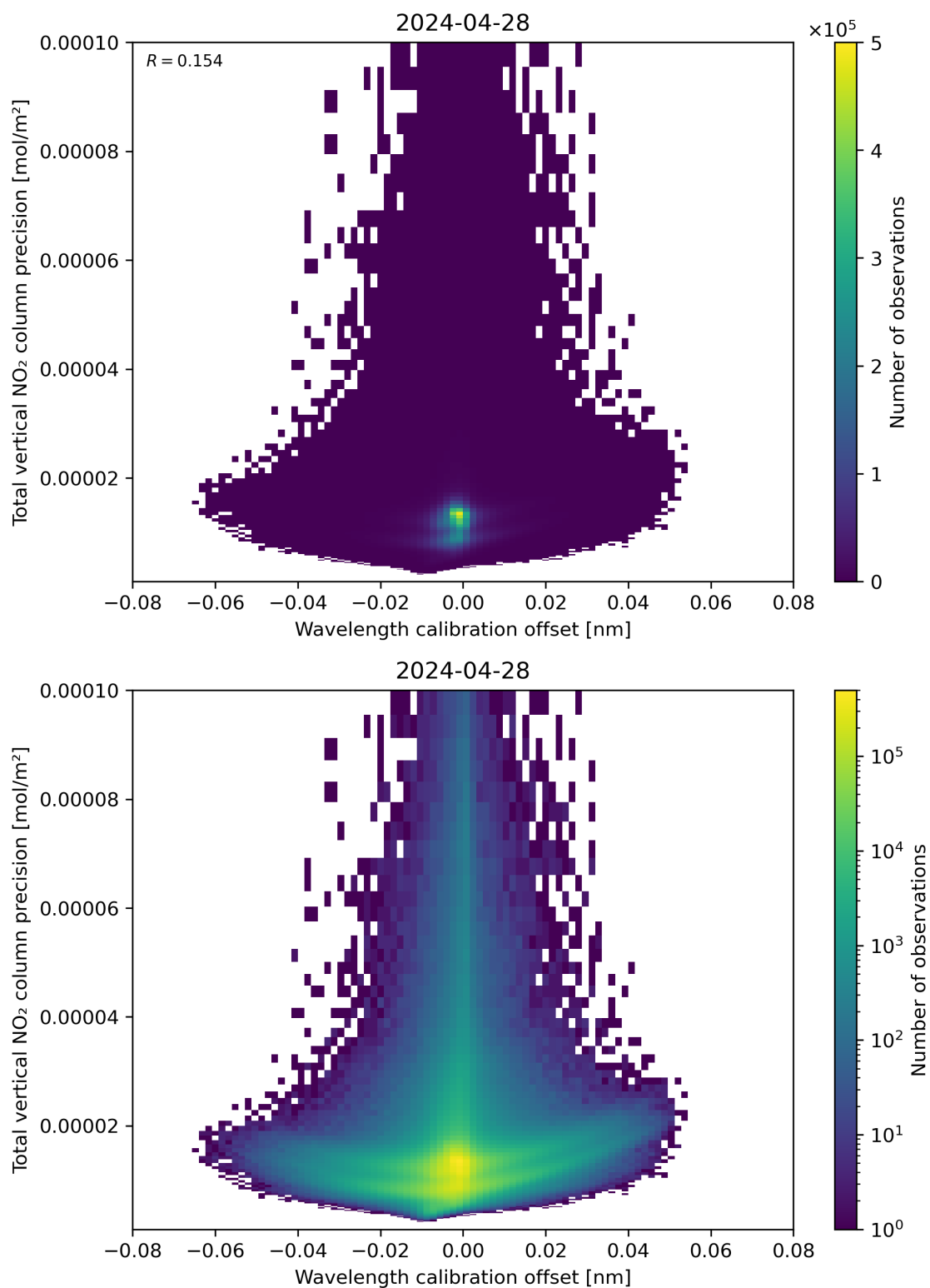
Figure 180: Scatter density plot of “Wavelength calibration offset” against “Total vertical NO 2 column precision” for 2024-04-27 to 2024-04-29.
