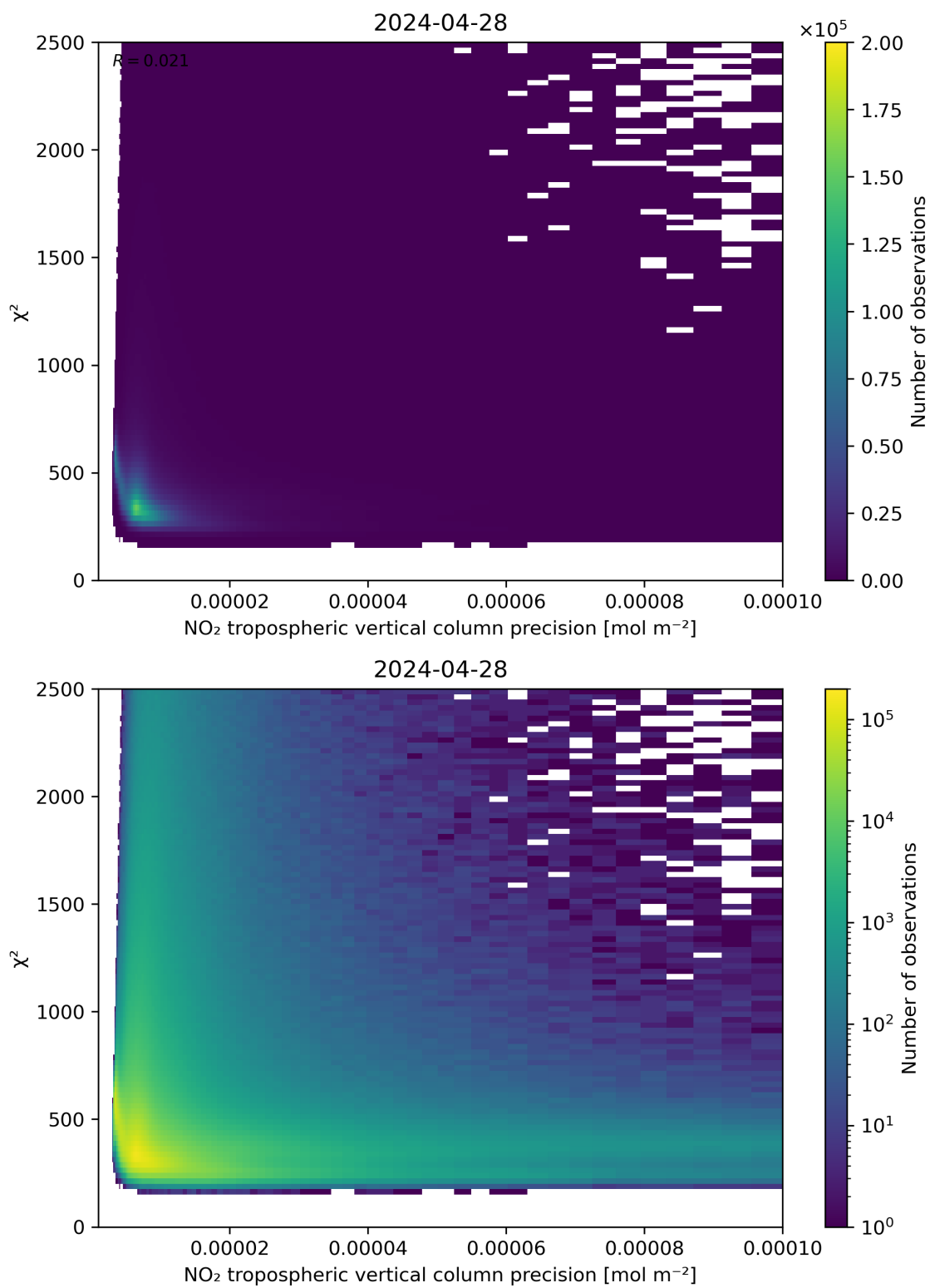
Figure 134: Scatter density plot of “NO 2 tropospheric vertical column precision” against “ \chi^2 ” for 2024-04-27 to 2024-04-29.
