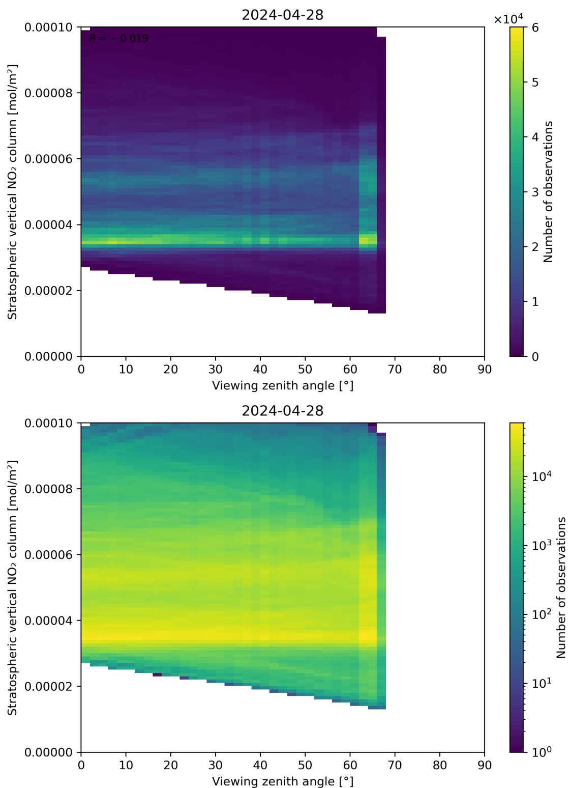
Figure 164: Scatter density plot of “Viewing zenith angle” against “Stratospheric vertical NO 2 column” for 2024-04-27 to 2024-04-29.
