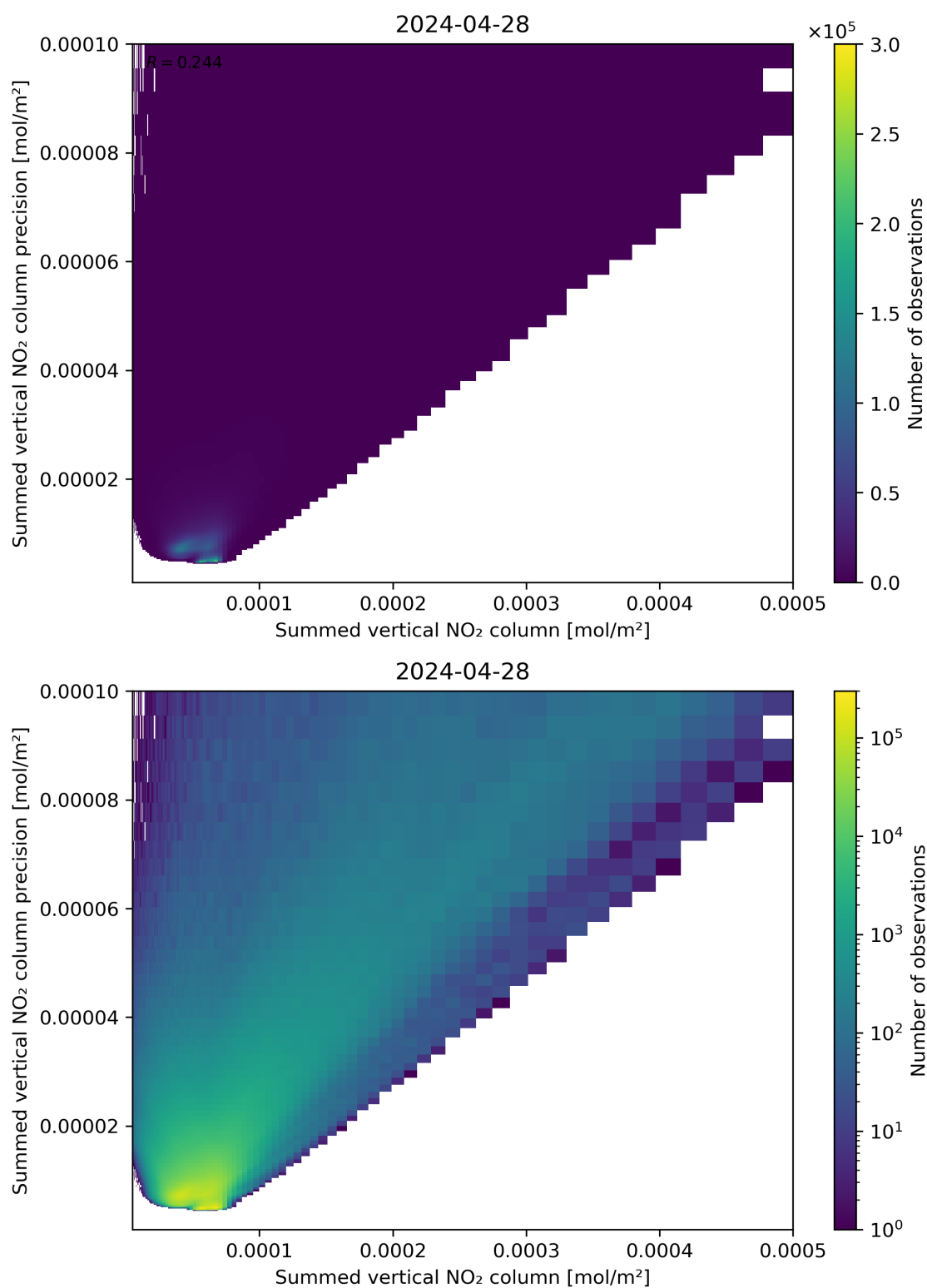
Figure 105: Scatter density plot of “Summed vertical NO 2 column” against “Summed vertical NO 2 column precision” for 2024-04-27 to 2024-04-29.
