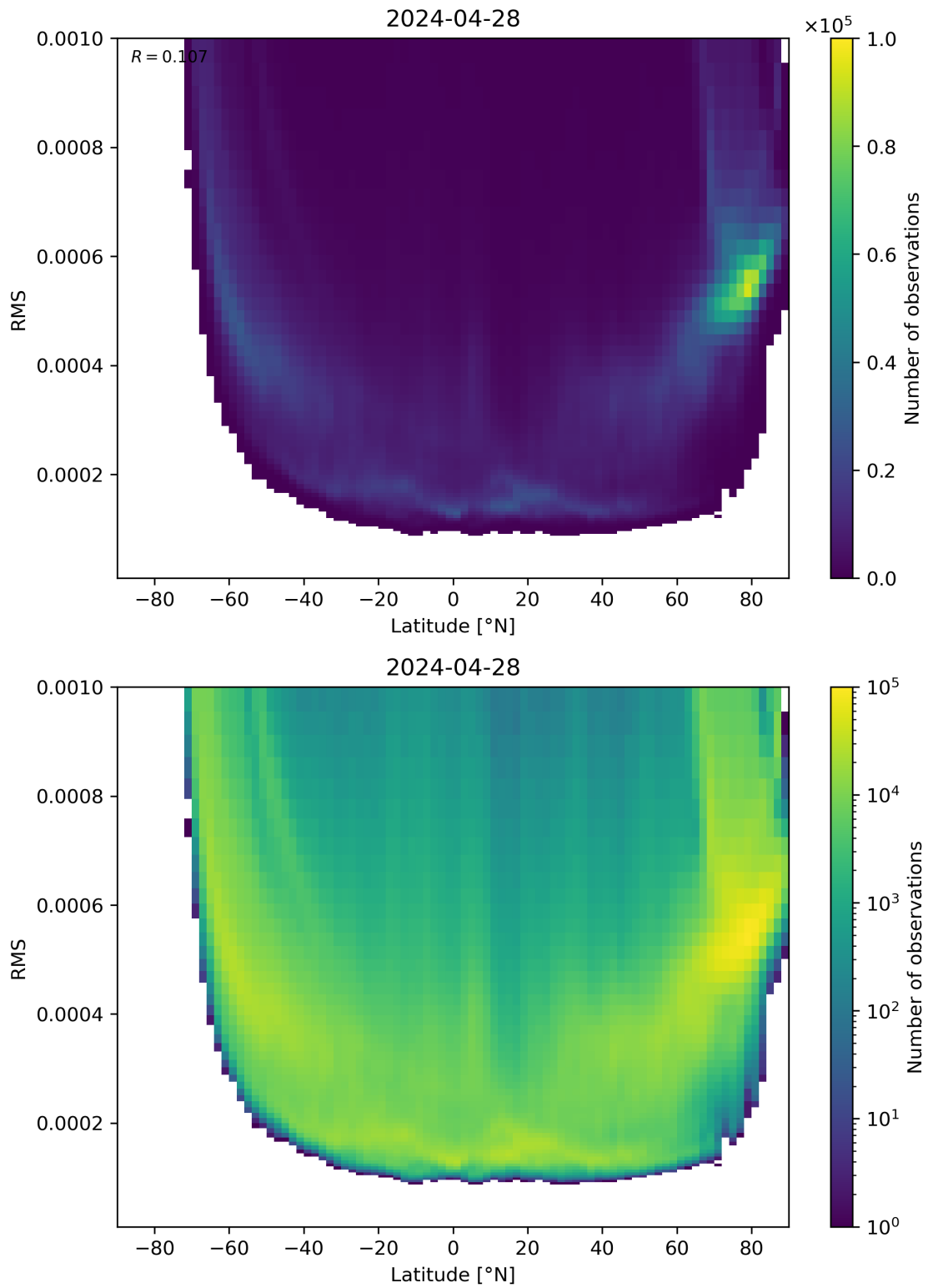
Figure 94: Scatter density plot of “Latitude” against “RMS” for 2024-04-27 to 2024-04-29.
