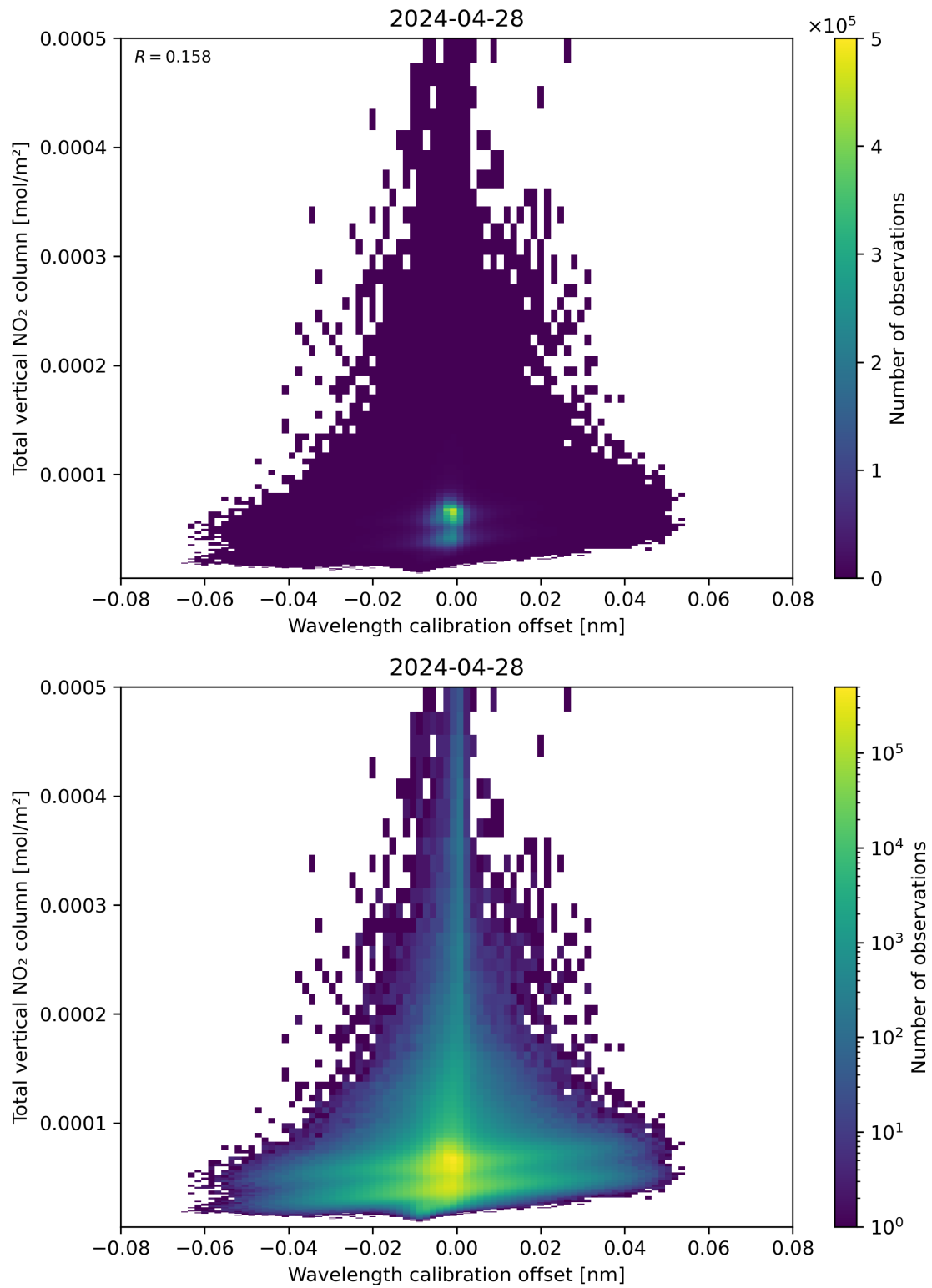
Figure 179: Scatter density plot of “Wavelength calibration offset” against “Total vertical NO 2 column” for 2024-04-27 to 2024-04-29.
