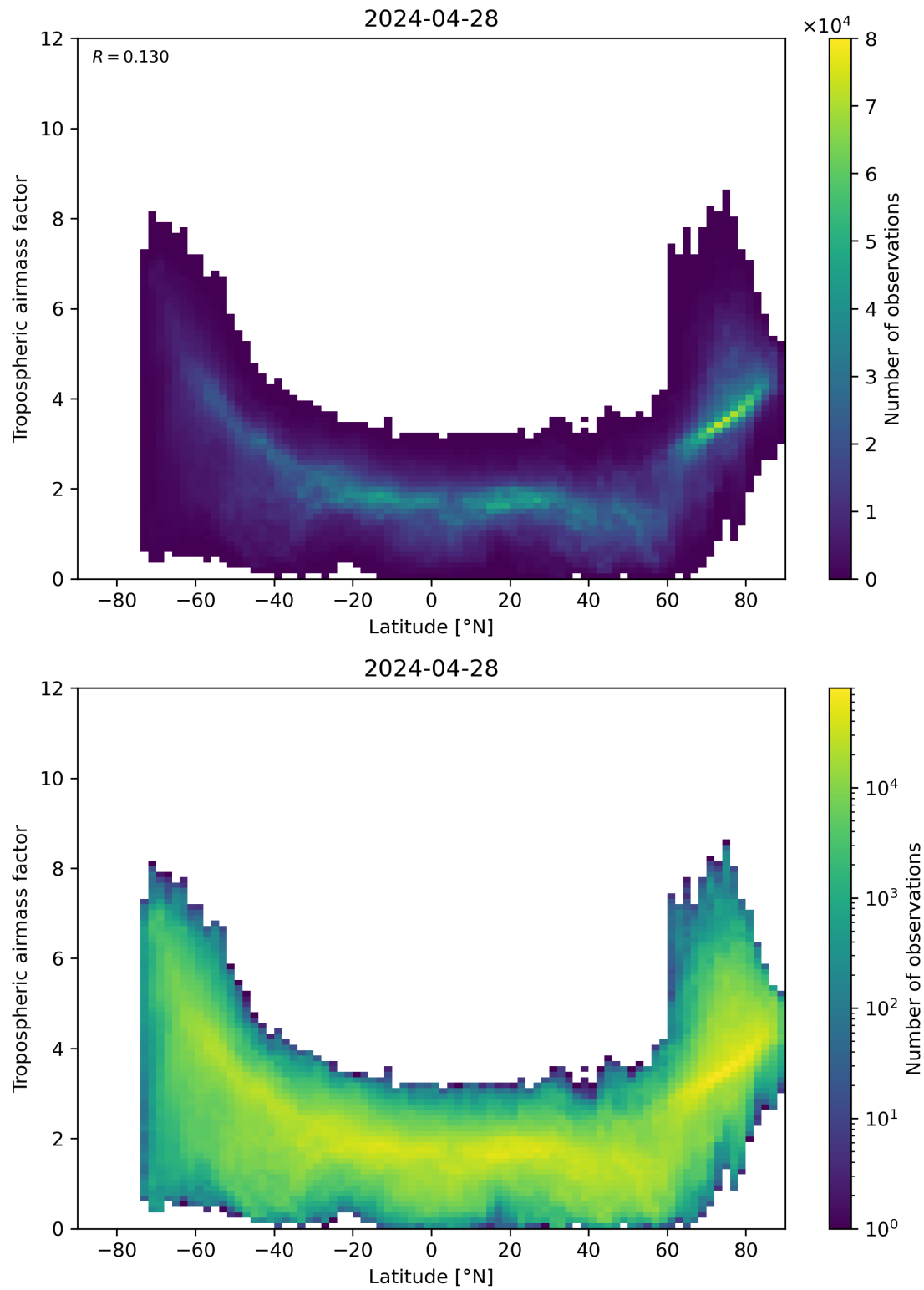
Figure 85: Scatter density plot of “Latitude” against “Tropospheric airmass factor” for 2024-04-27 to 2024-04-29.
