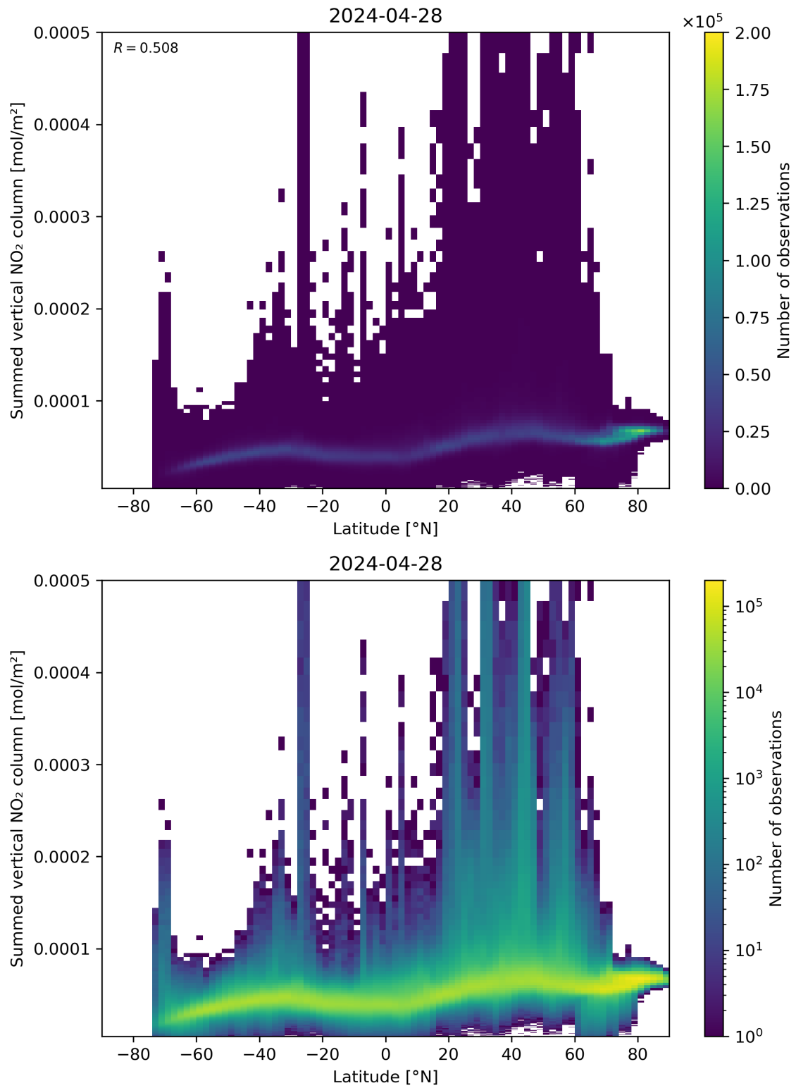
Figure 88: Scatter density plot of “Latitude” against “Summed vertical NO 2 column” for 2024-04-27 to 2024-04-29.
