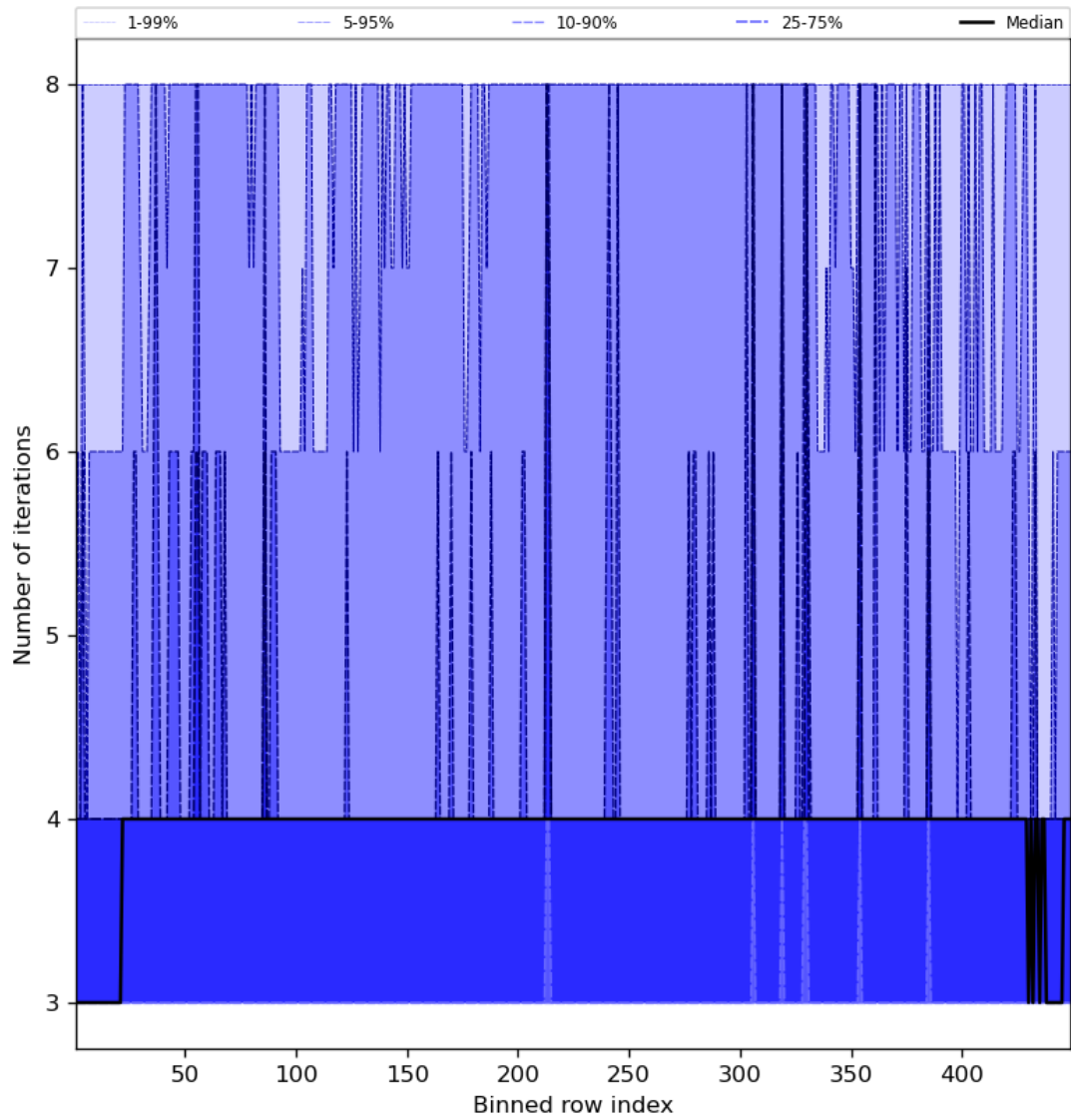
Figure 51: Along track statistics of “Number of iterations” for 2024-04-27 to 2024-04-29
