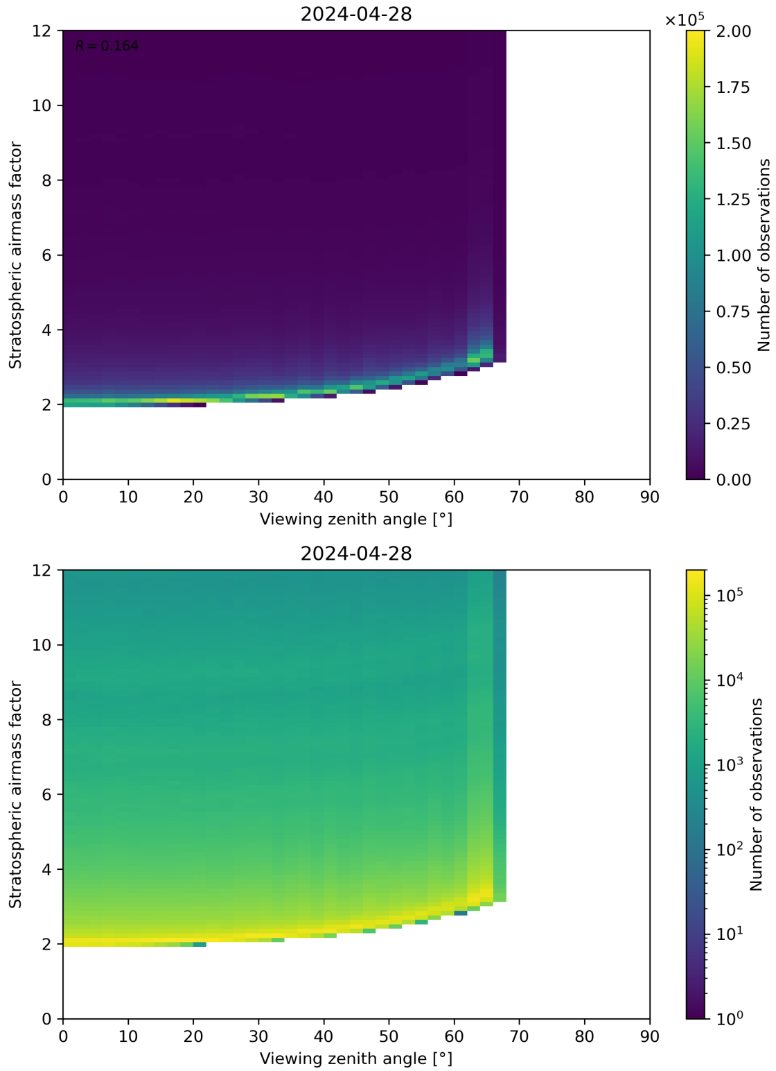
Figure 159: Scatter density plot of “Viewing zenith angle” against “Stratospheric airmass factor” for 2024-04-27 to 2024-04-29.
