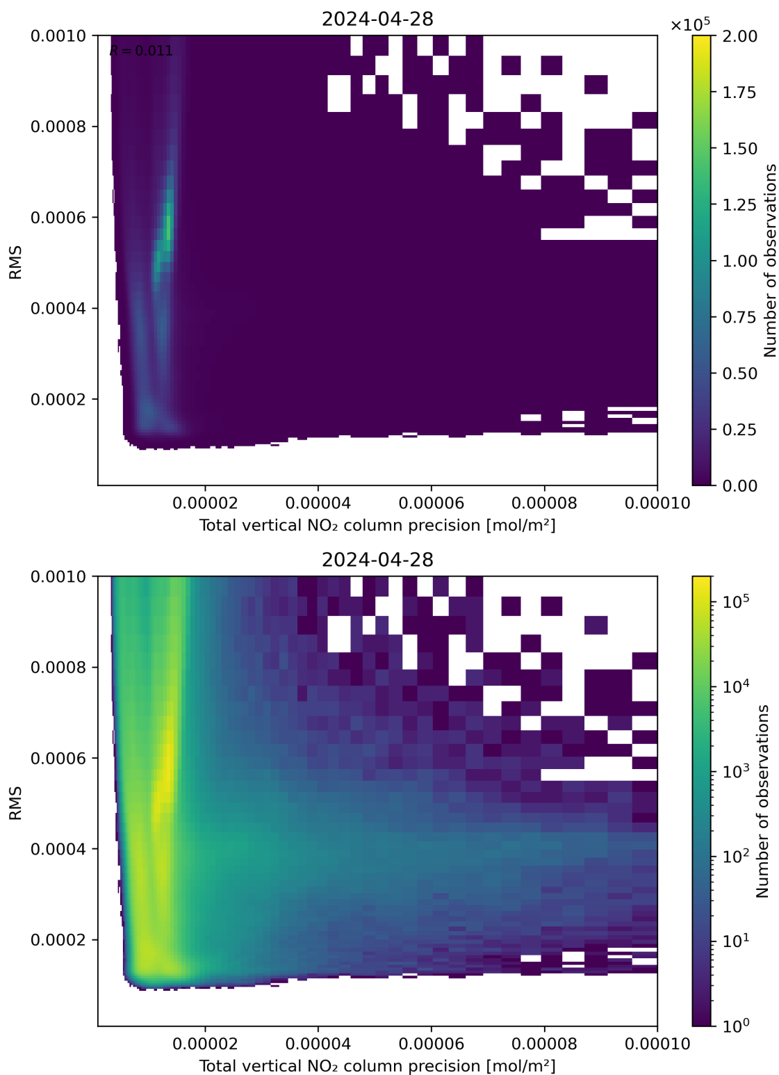
Figure 119: Scatter density plot of “Total vertical NO 2 column precision” against “RMS” for 2024-04-27 to 2024-04-29.
