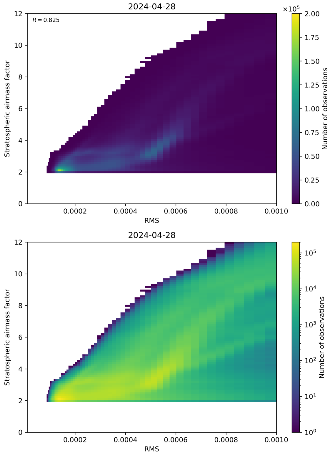
Figure 144: Scatter density plot of “RMS” against “Stratospheric airmass factor” for 2024-04-27 to 2024-04-29.
