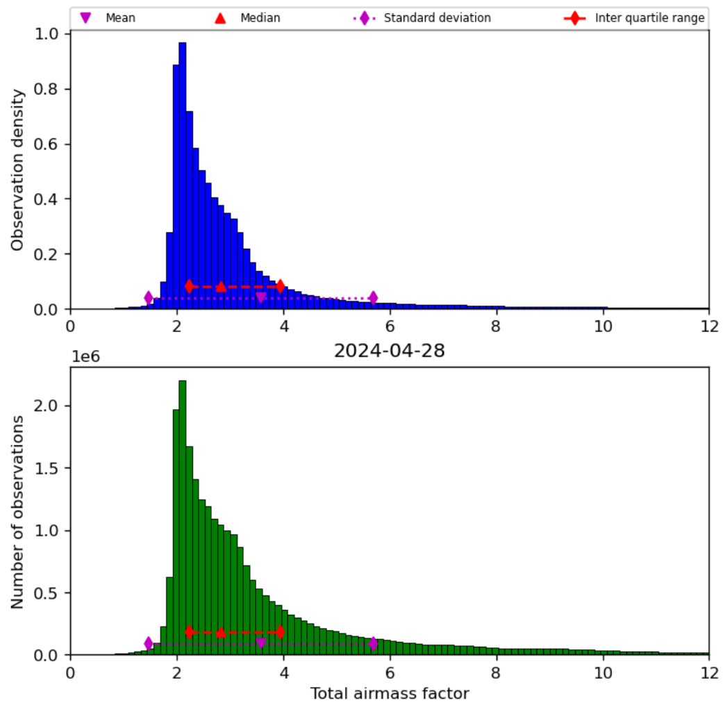
Figure 32: Histogram of “Total airmass factor” for 2024-04-27 to 2024-04-29
