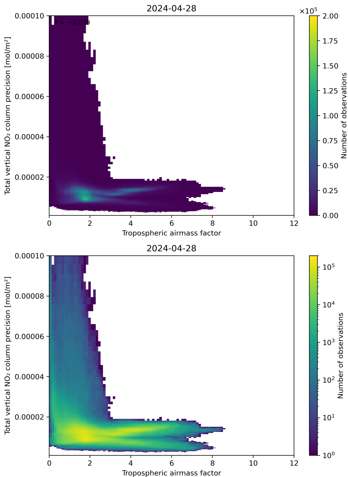
Figure 78: Scatter density plot of “Tropospheric air mass factor” against “Total vertical NO 2 column precision” for 2024-04-27 to 2024-04-29.
