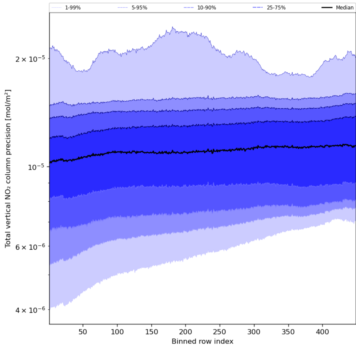
Figure 56: Along track statistics of “Total vertical NO 2 column precision” for 2024-04-27 to 2024-04-29
