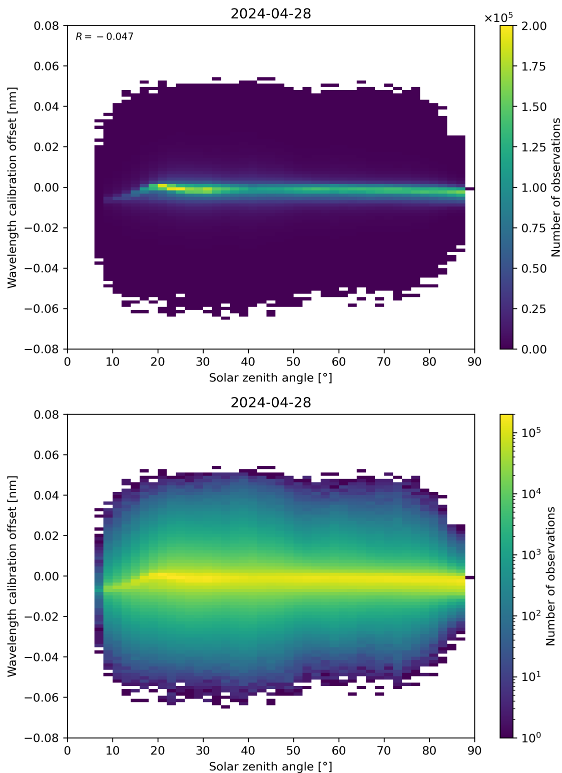
Figure 158: Scatter density plot of “Solar zenith angle” against “Wavelength calibration offset” for 2024-04-27 to 2024-04-29.
