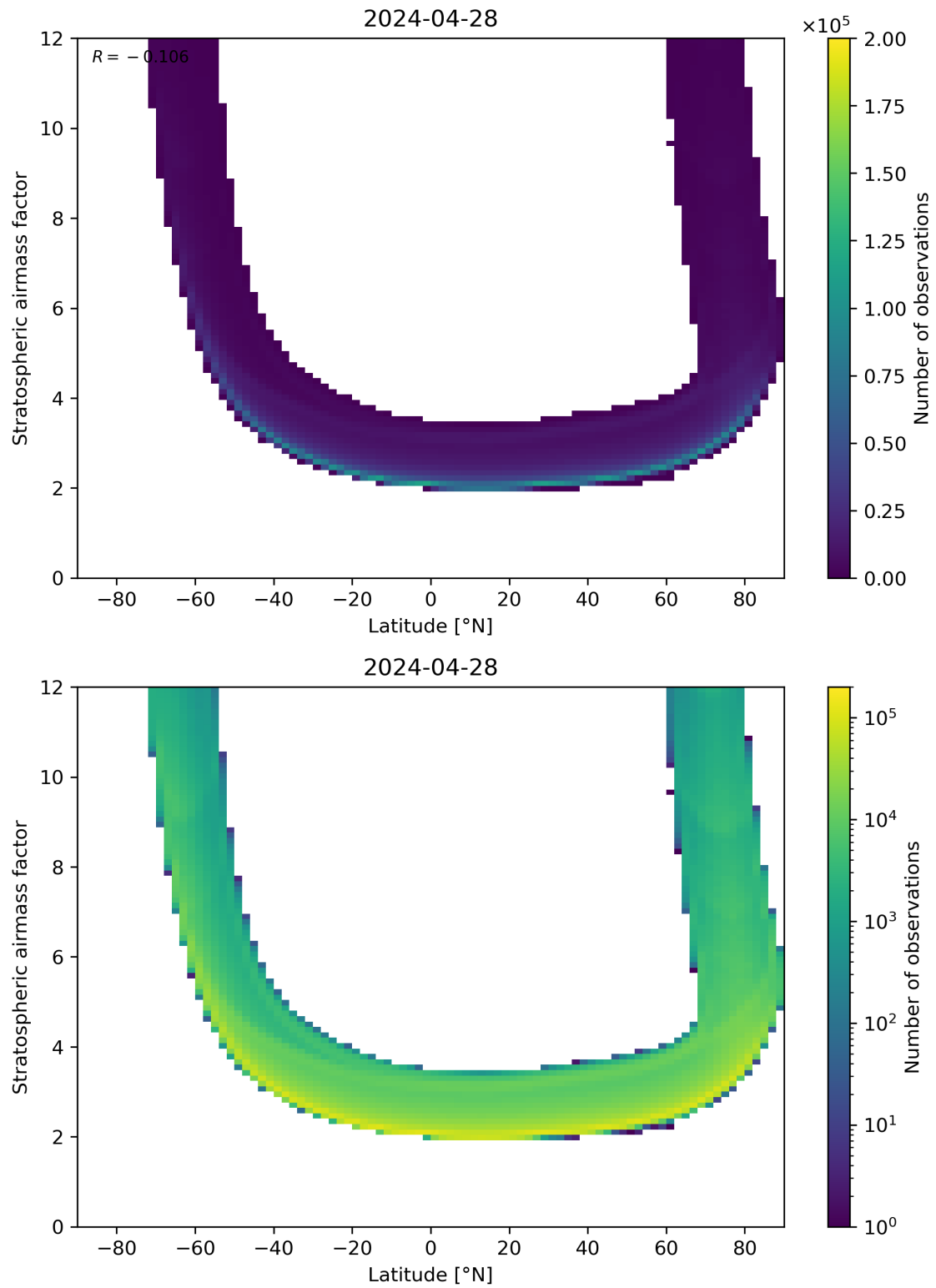
Figure 83: Scatter density plot of “Latitude” against “Stratospheric air mass factor” for 2024-04-27 to 2024-04-29.
