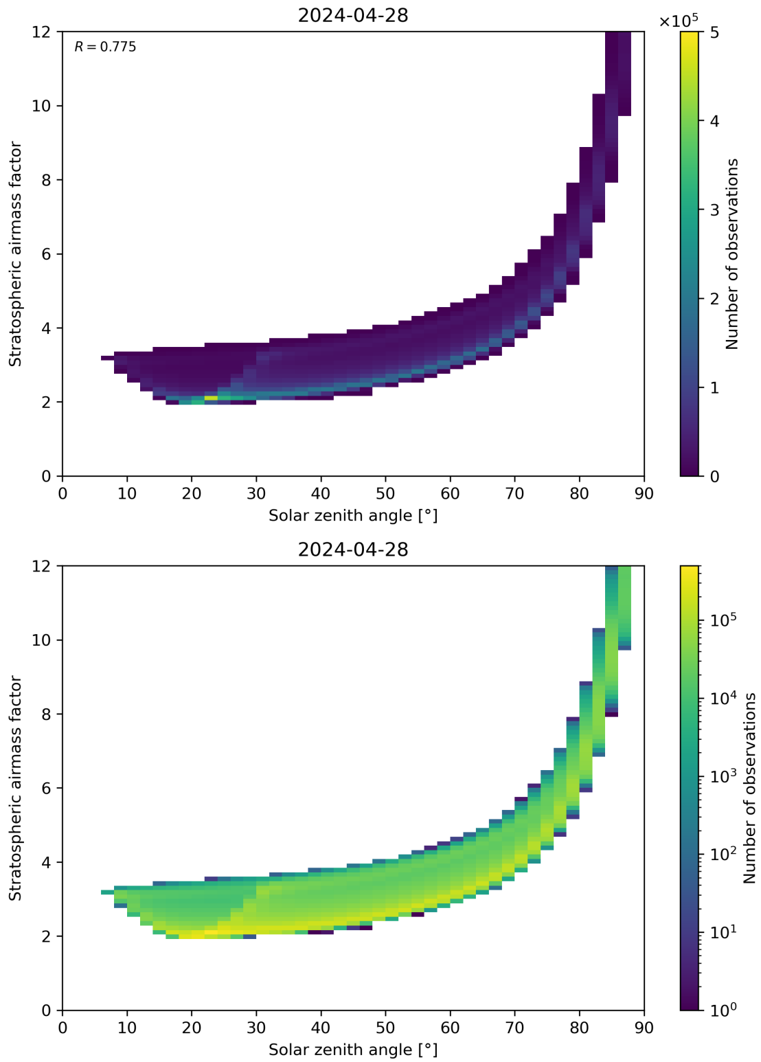
Figure 145: Scatter density plot of “Solar zenith angle” against “Stratospheric airmass factor” for 2024-04-27 to 2024-04-29.
