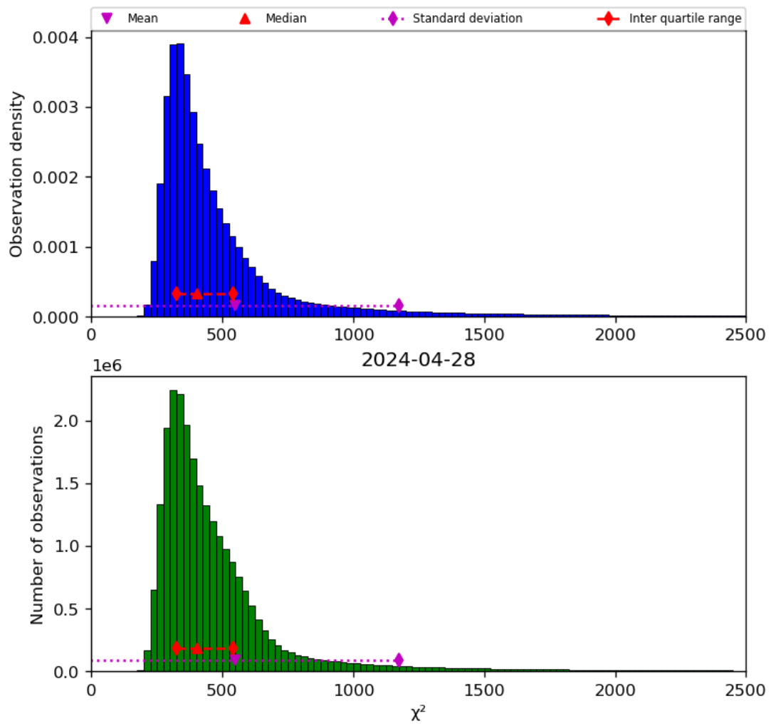
Figure 42: Histogram of “ \chi^2 ” for 2024-04-27 to 2024-04-29
