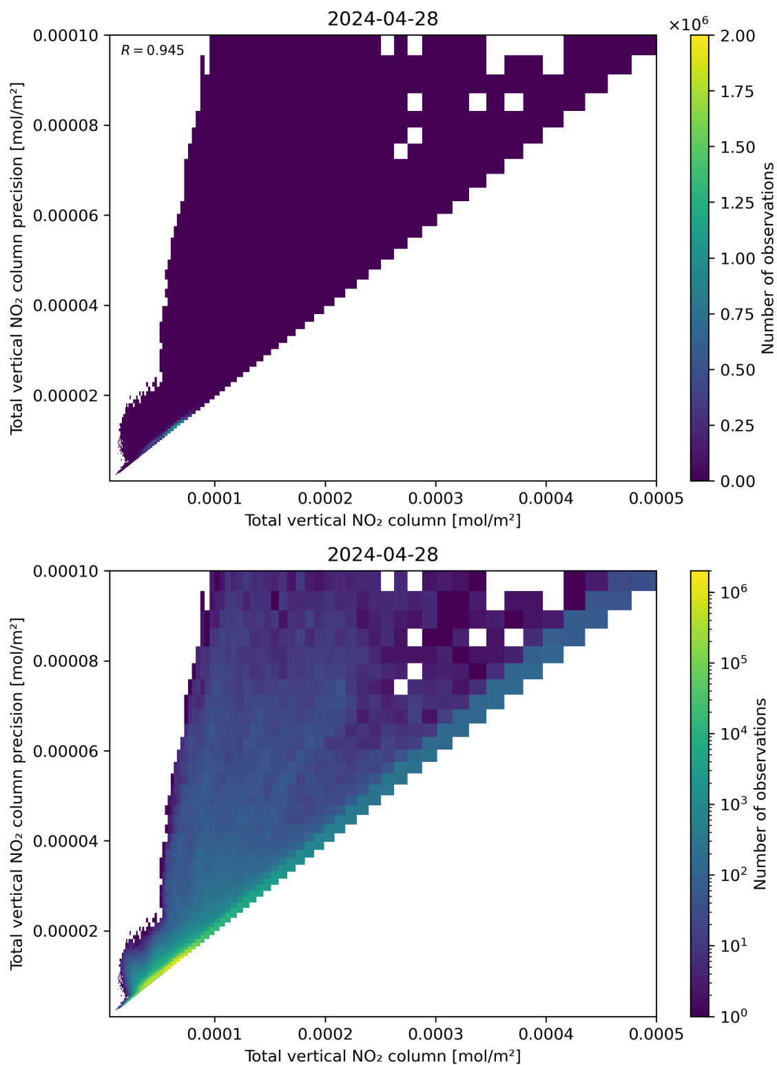
Figure 114: Scatter density plot of “Total vertical NO 2 column” against “Total vertical NO 2 column precision” for 2024-04-27 to 2024-04-29.
