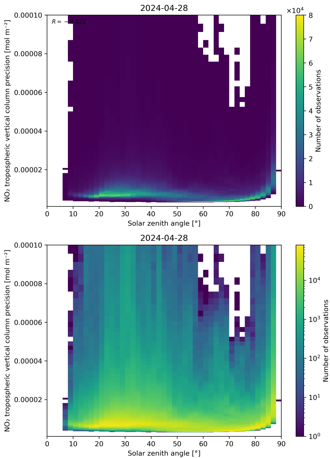
Figure 156: Scatter density plot of “Solar zenith angle” against “NO 2 tropospheric vertical column precision” for 2024-04-27 to 2024-04-29.
