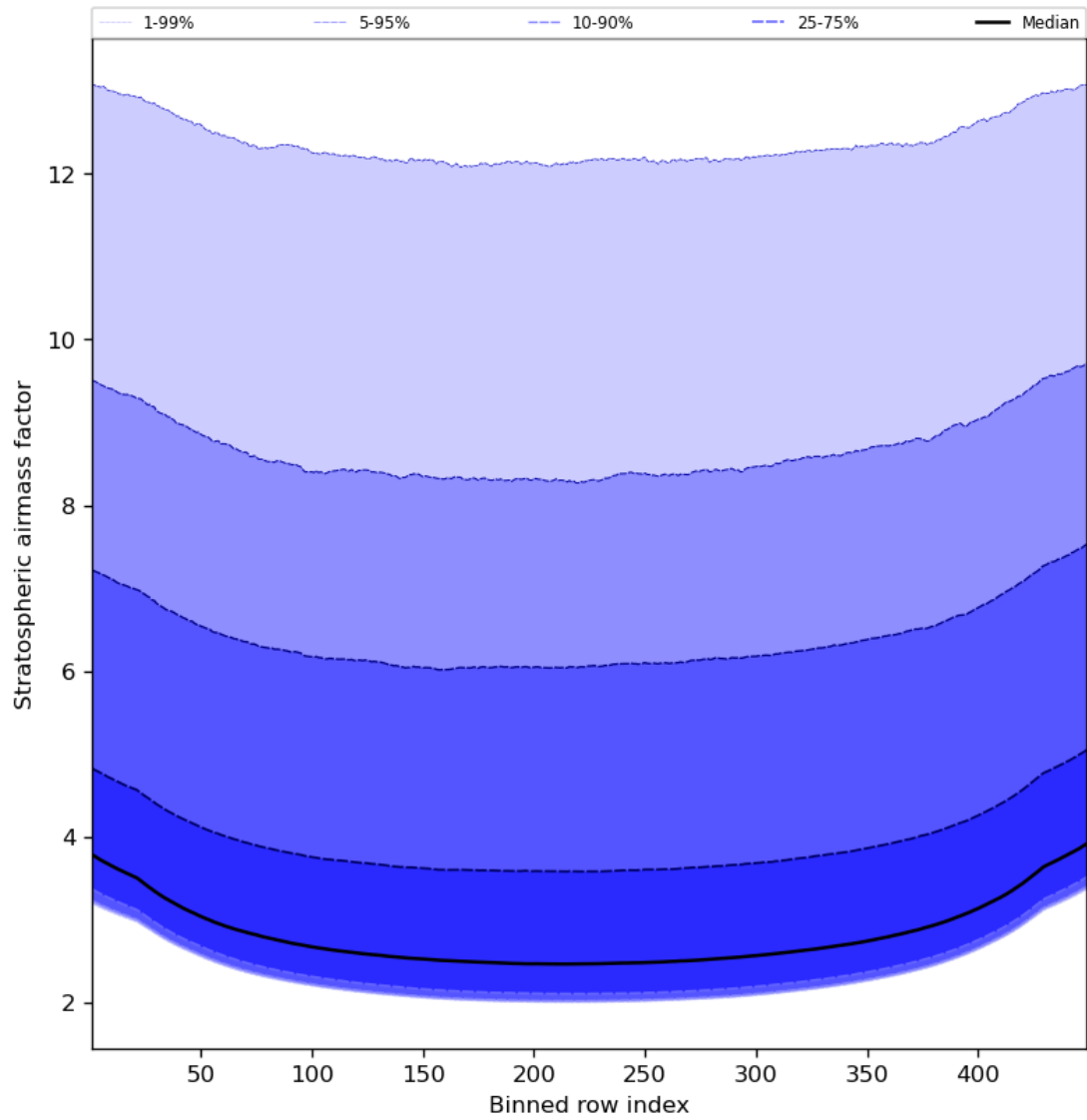
Figure 61: Along track statistics of “Stratospheric airmass factor” for 2024-04-27 to 2024-04-29
