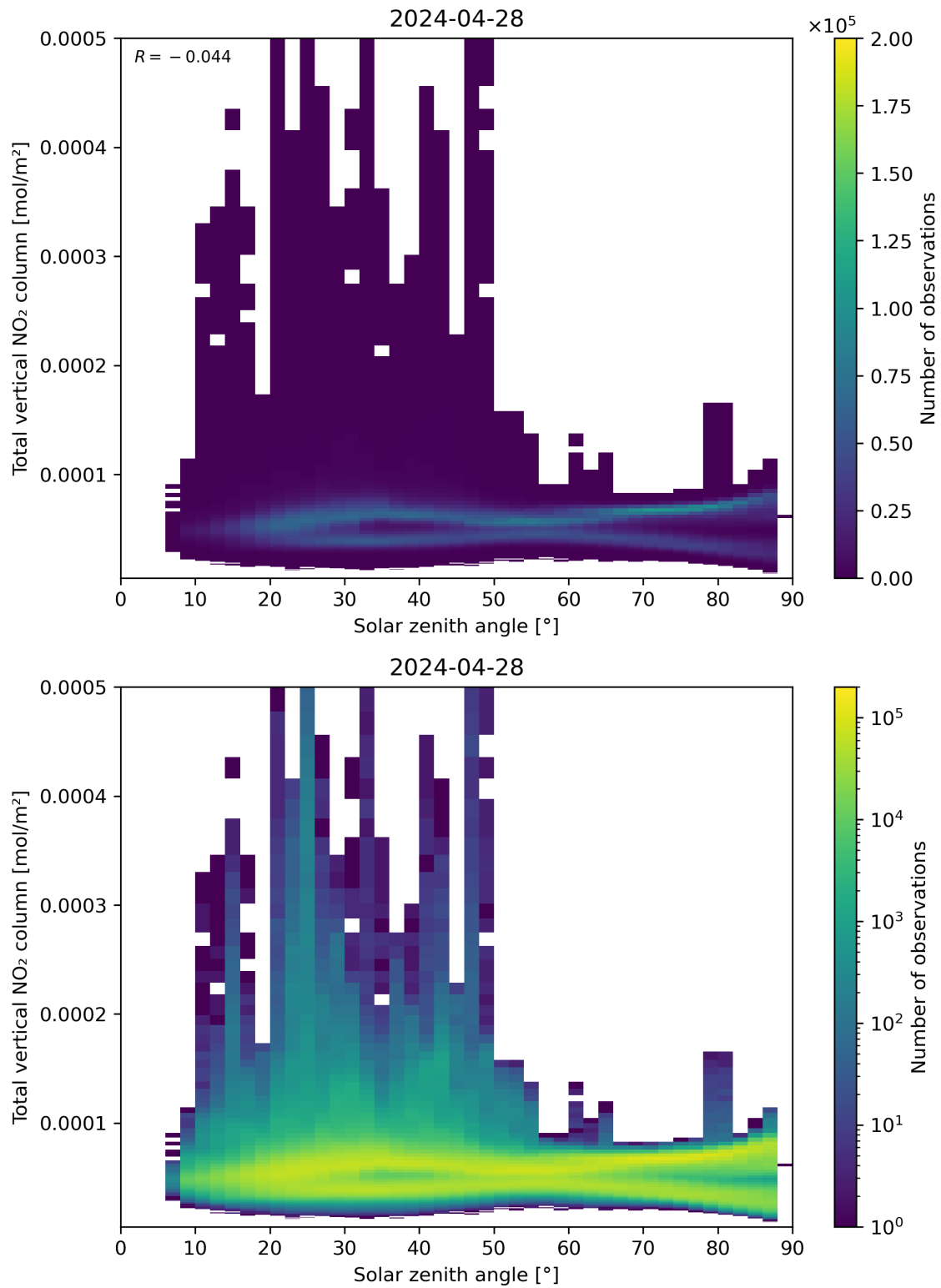
Figure 153: Scatter density plot of “Solar zenith angle” against “Total vertical NO 2 column” for 2024-04-27 to 2024-04-29.
