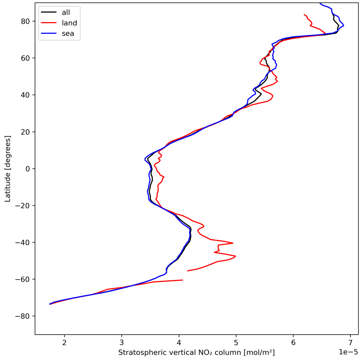
Figure 19: Zonal average of “Stratospheric vertical NO 2 column” for 2024-04-27 to 2024-04-29.
