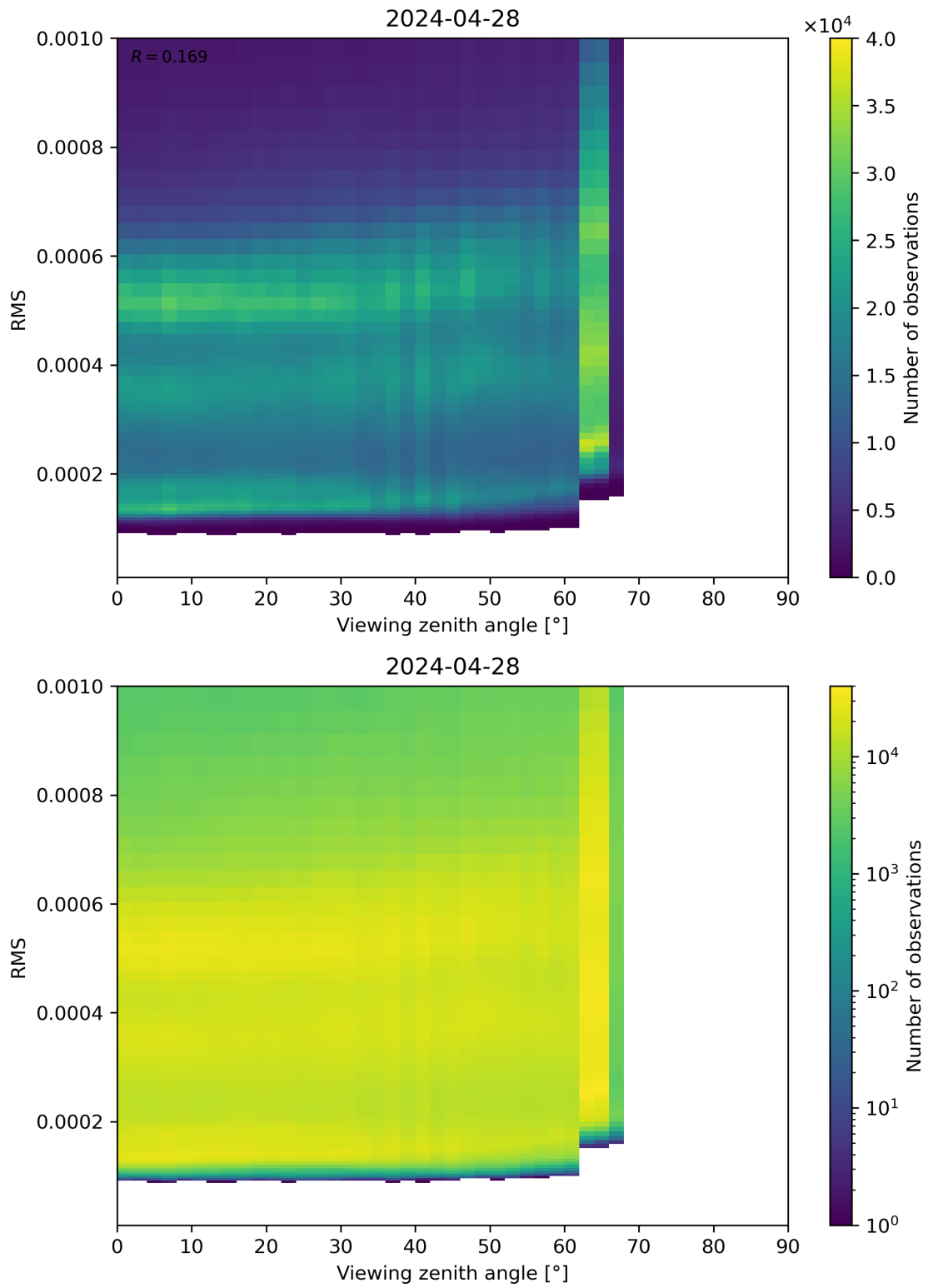
Figure 171: Scatter density plot of “Viewing zenith angle” against “RMS” for 2024-04-27 to 2024-04-29.
