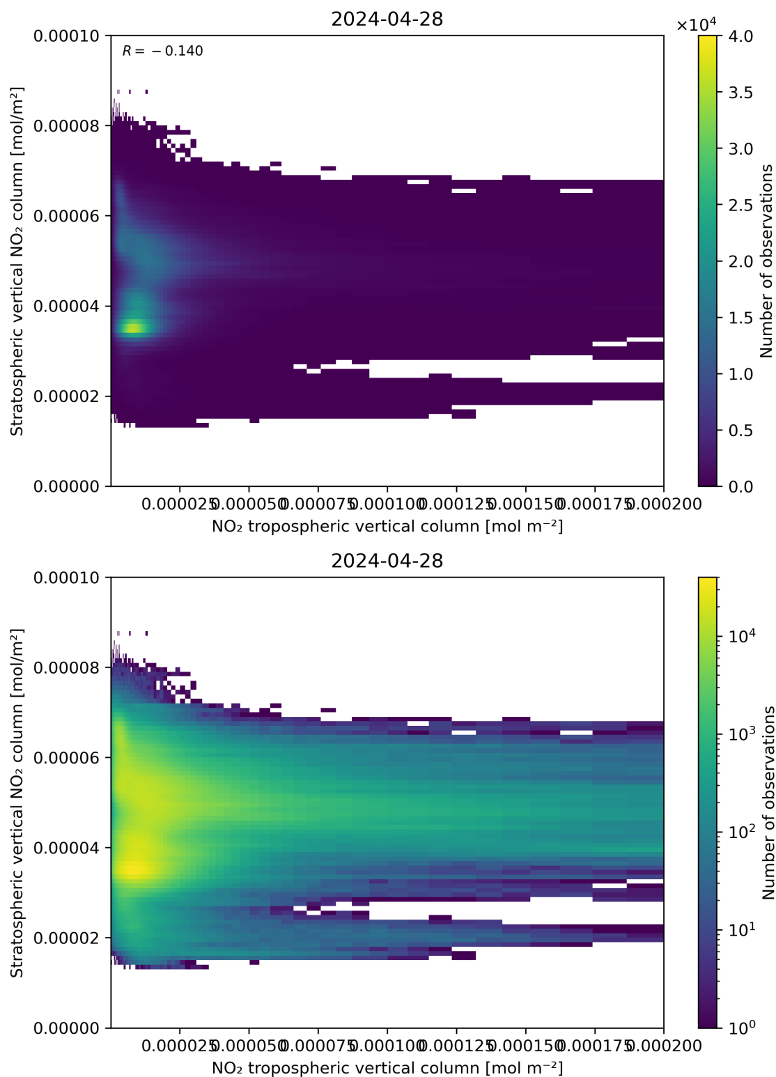
Figure 125: Scatter density plot of “NO 2 tropospheric vertical column” against “Stratospheric vertical NO 2 column” for 2024-04-27 to 2024-04-29.
