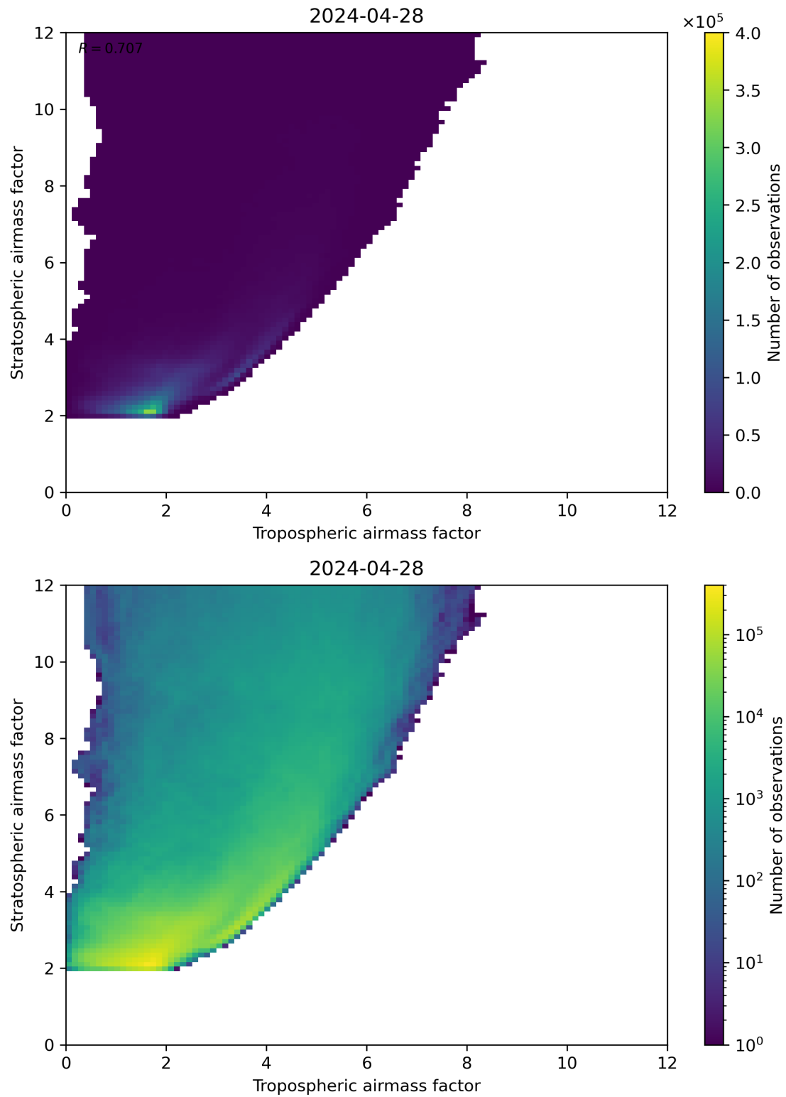
Figure 71: Scatter density plot of “Tropospheric airmass factor” against “Stratospheric airmass factor” for 2024-04-27 to 2024-04-29.
