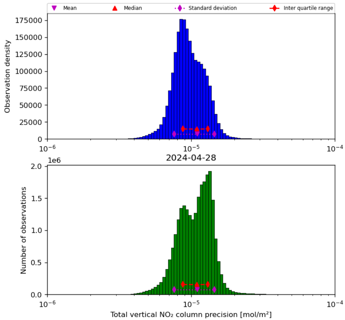
Figure 39: Histogram of "Total vertical NO 2 column precision" for 2024-04-27 to 2024-04-29
