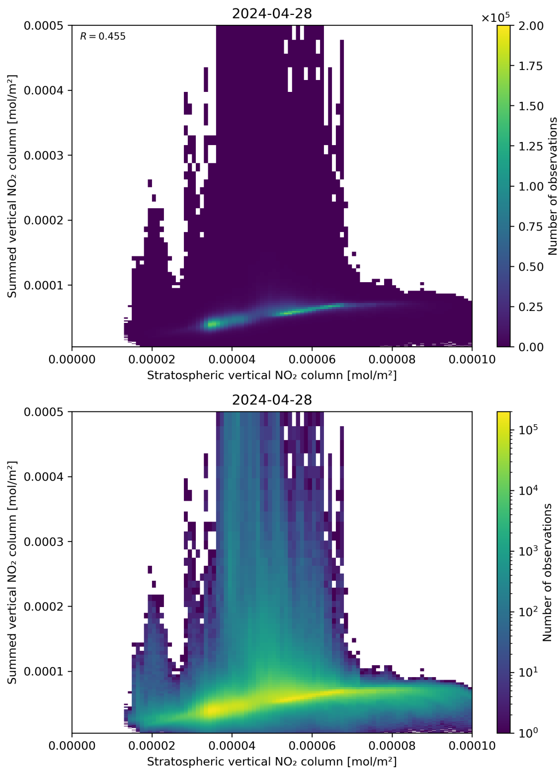
Figure 98: Scatter density plot of “Stratospheric vertical NO 2 column” against “Summed vertical NO 2 column” for 2024-04-27 to 2024-04-29.
