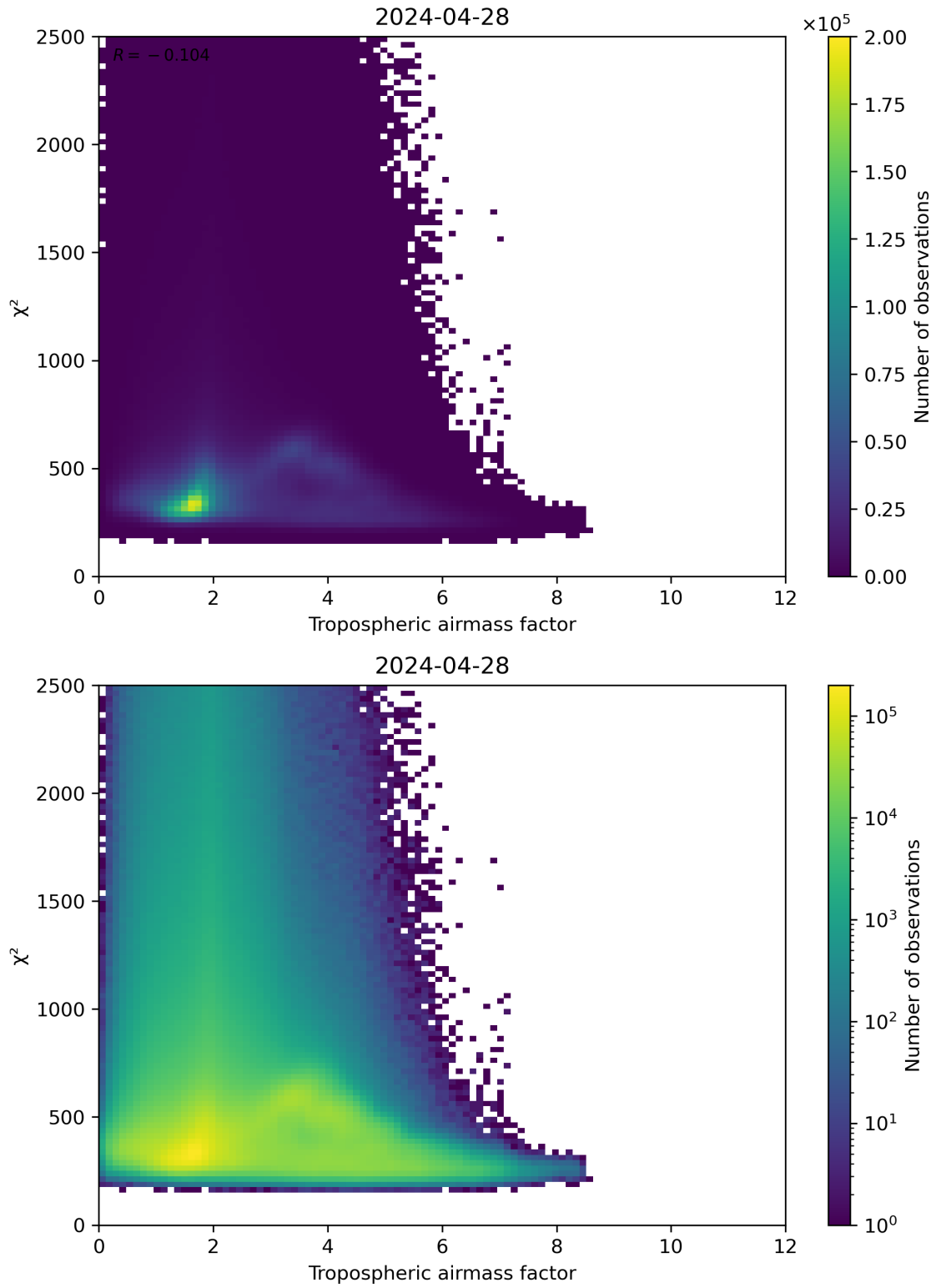
Figure 73: Scatter density plot of “Tropospheric airmass factor” against “ \chi^2 ” for 2024-04-27 to 2024-04-29.
