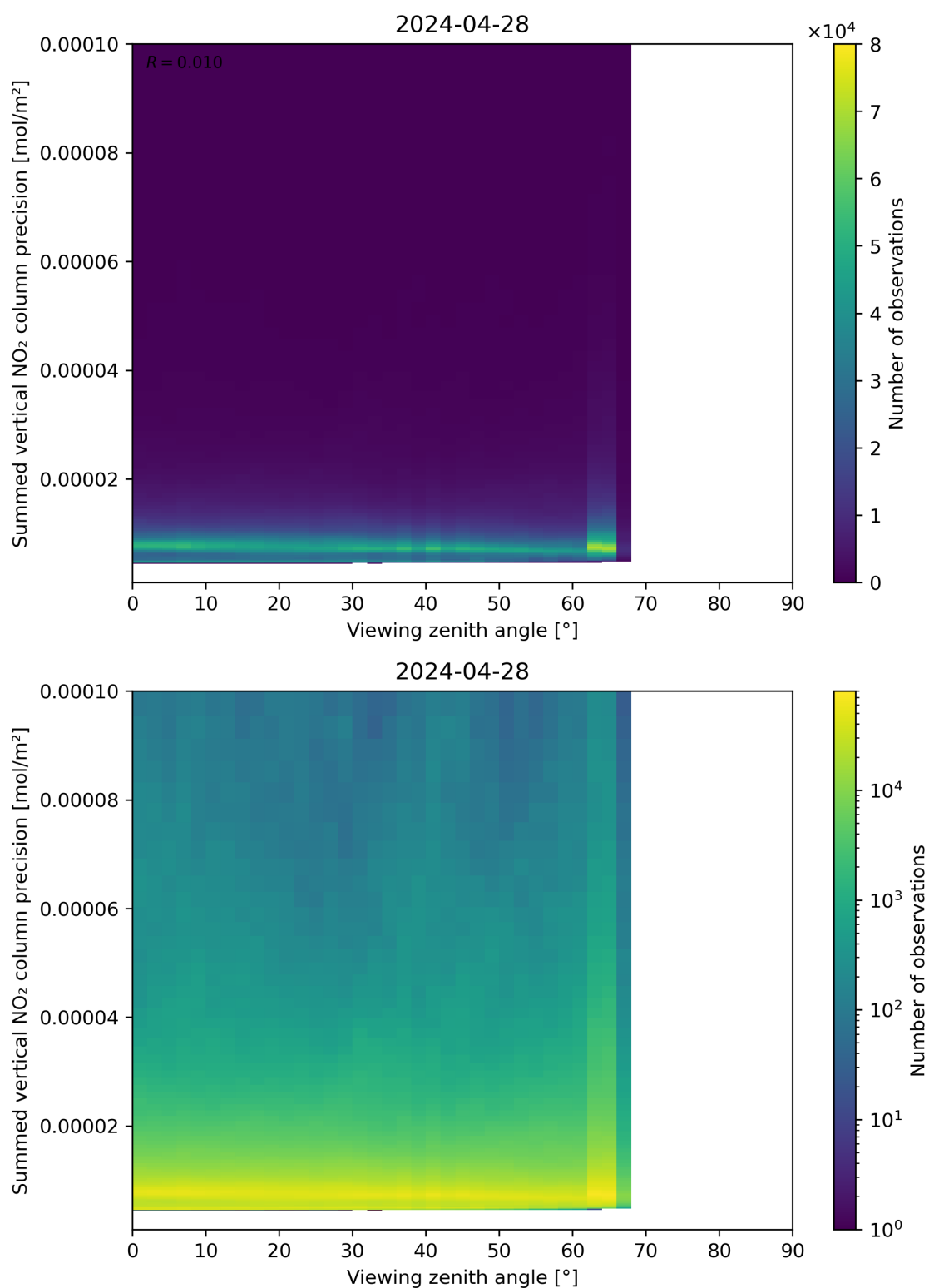
Figure 166: Scatter density plot of “Viewing zenith angle” against “Summed vertical NO 2 column precision” for 2024-04-27 to 2024-04-29.
