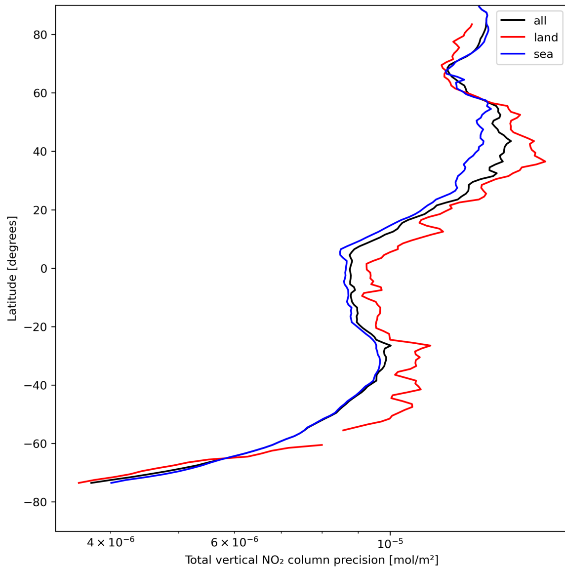
Figure 22: Zonal average of “Total vertical NO 2 column precision” for 2024-04-27 to 2024-04-29.
