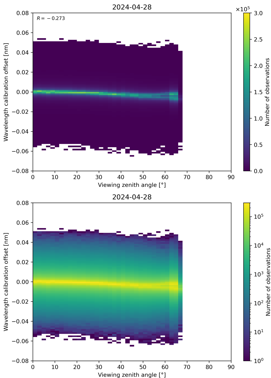
Figure 173: Scatter density plot of “Viewing zenith angle” against “Wavelength calibration offset” for 2024-04-27 to 2024-04-29.
