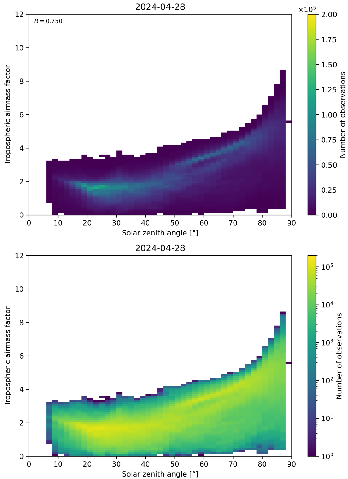
Figure 147: Scatter density plot of “Solar zenith angle” against “Tropospheric airmass factor” for 2024-04-27 to 2024-04-29.
