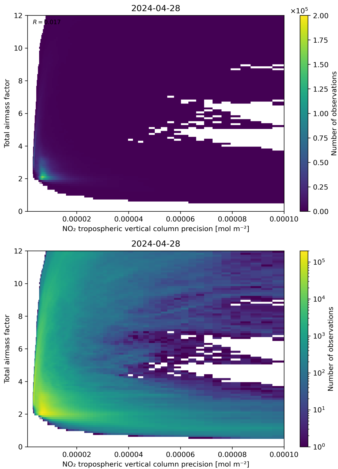
Figure 132: Scatter density plot of “NO 2 tropospheric vertical column precision” against “Total air mass factor” for 2024-04-27 to 2024-04-29.
