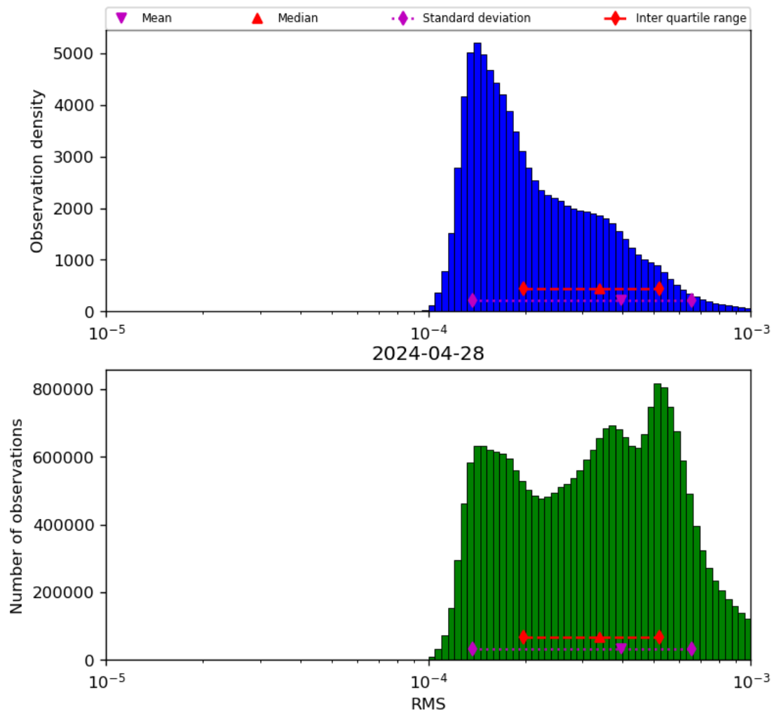
Figure 43: Histogram of “RMS” for 2024-04-27 to 2024-04-29
