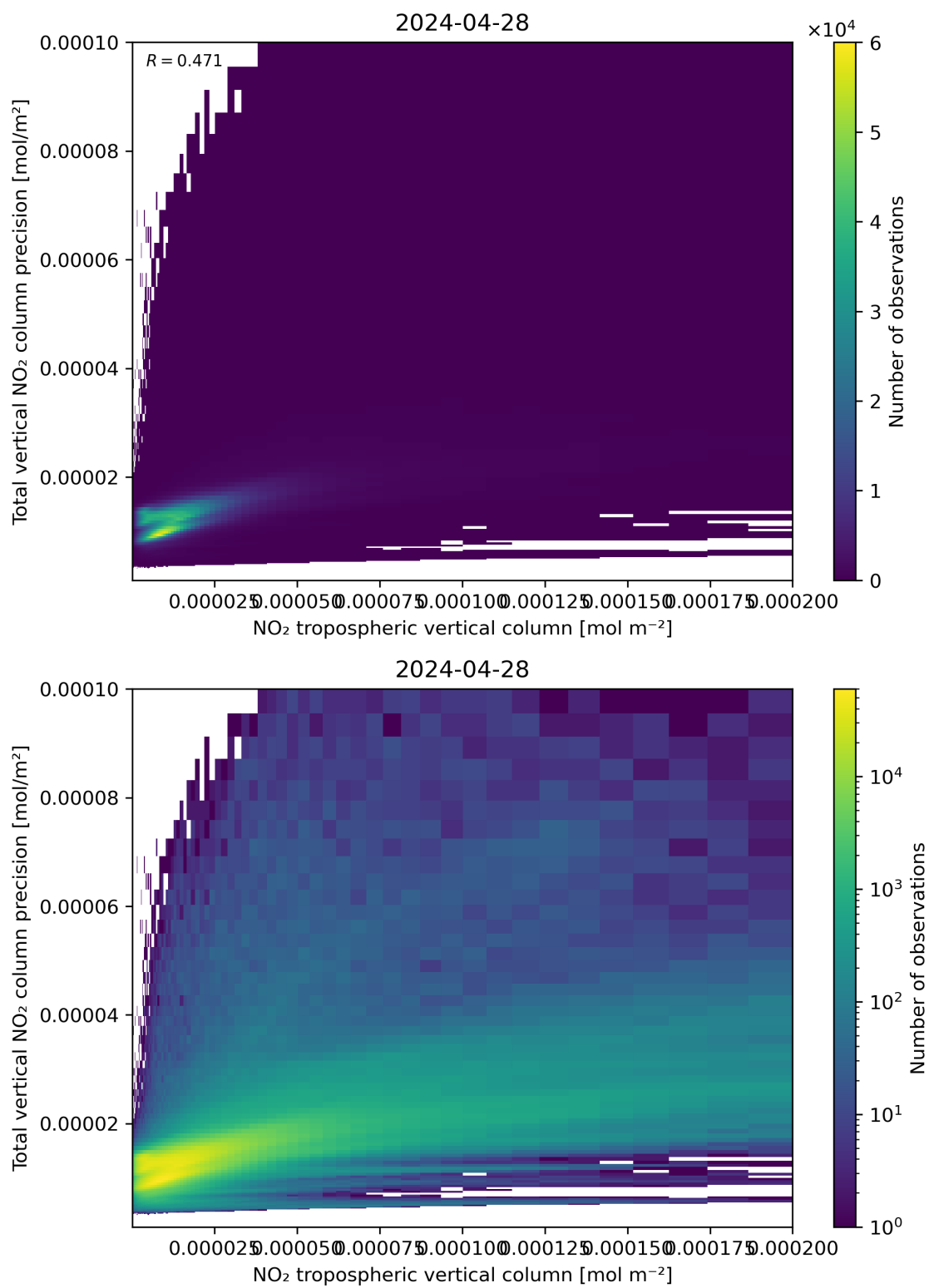
Figure 129: Scatter density plot of “NO 2 tropospheric vertical column” against “Total vertical NO 2 column precision” for 2024-04-27 to 2024-04-29.
