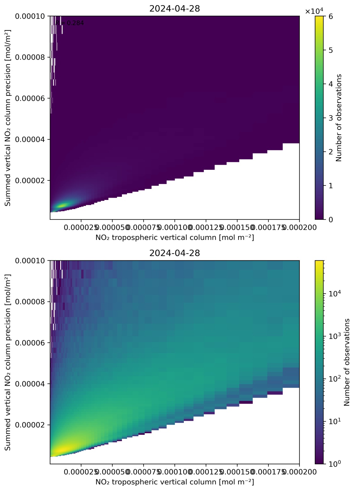
Figure 127: Scatter density plot of “NO 2 tropospheric vertical column” against “Summed vertical NO 2 column precision” for 2024-04-27 to 2024-04-29.
