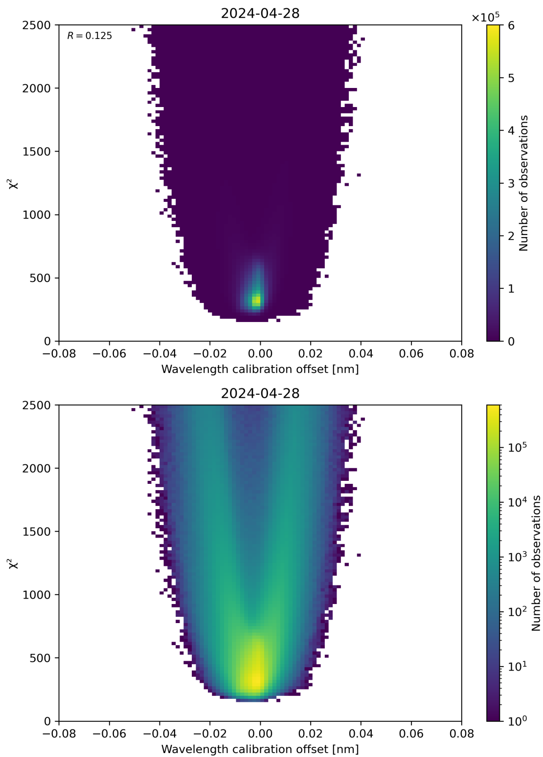
Figure 175: Scatter density plot of “Wavelength calibration offset” against “ \chi^2 ” for 2024-04-27 to 2024-04-29.
