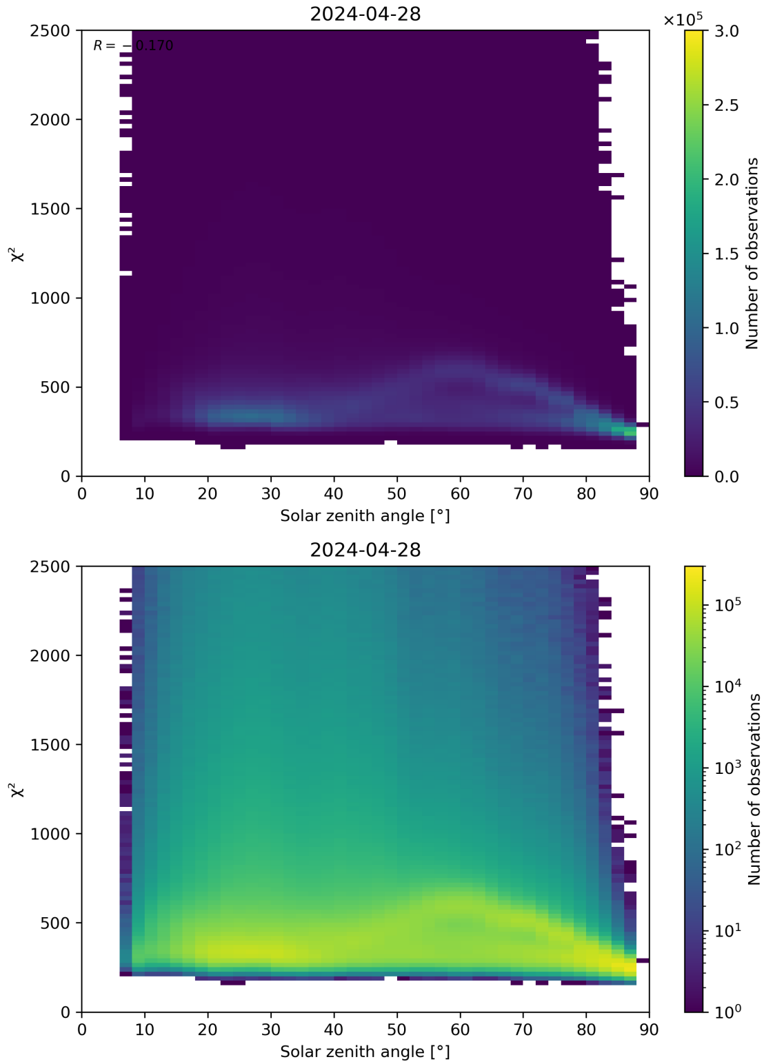
Figure 148: Scatter density plot of “Solar zenith angle” against “ \chi^2 ” for 2024-04-27 to 2024-04-29.
