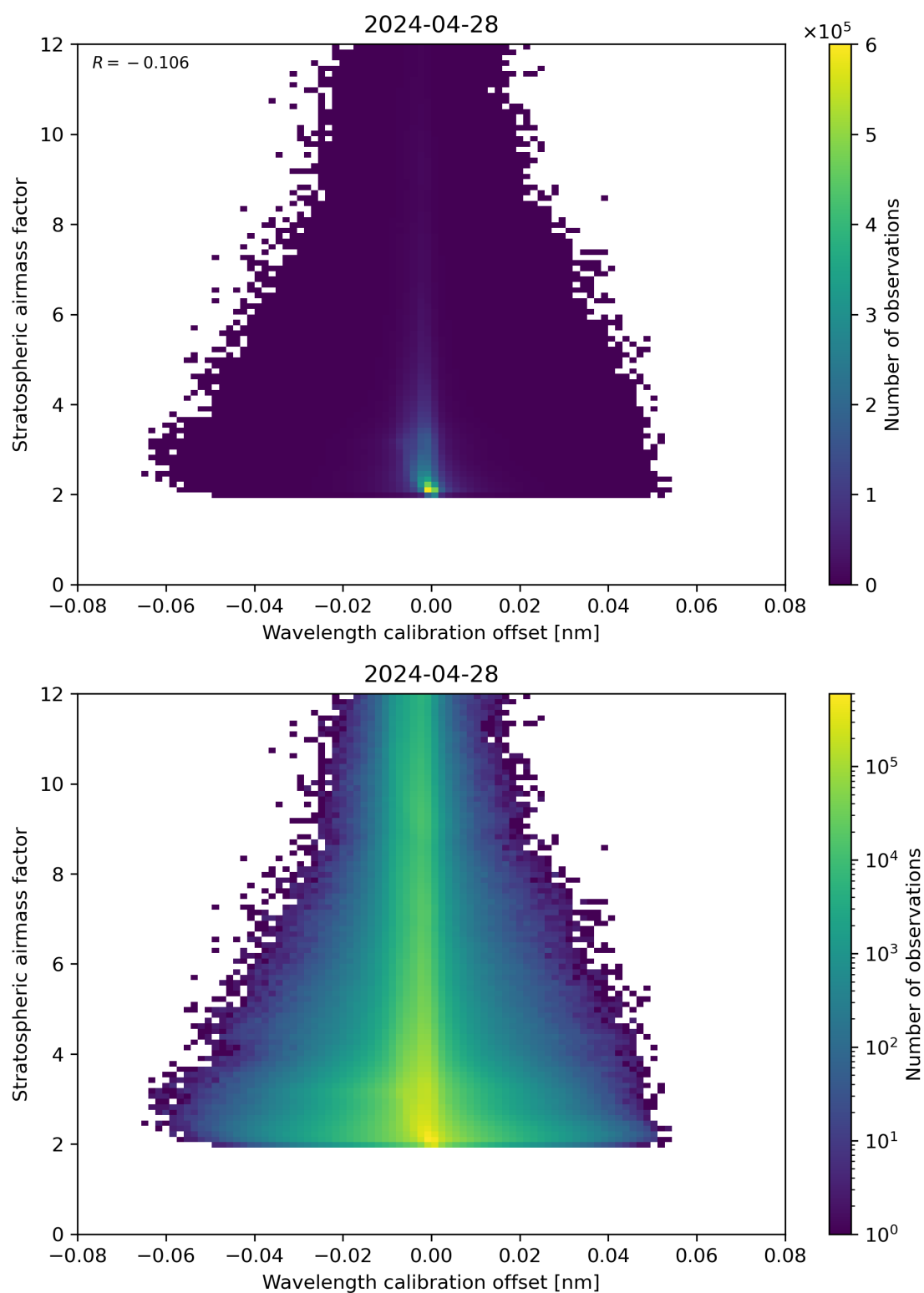
Figure 174: Scatter density plot of “Wavelength calibration offset” against “Stratospheric air mass factor” for 2024-04-27 to 2024-04-29.
