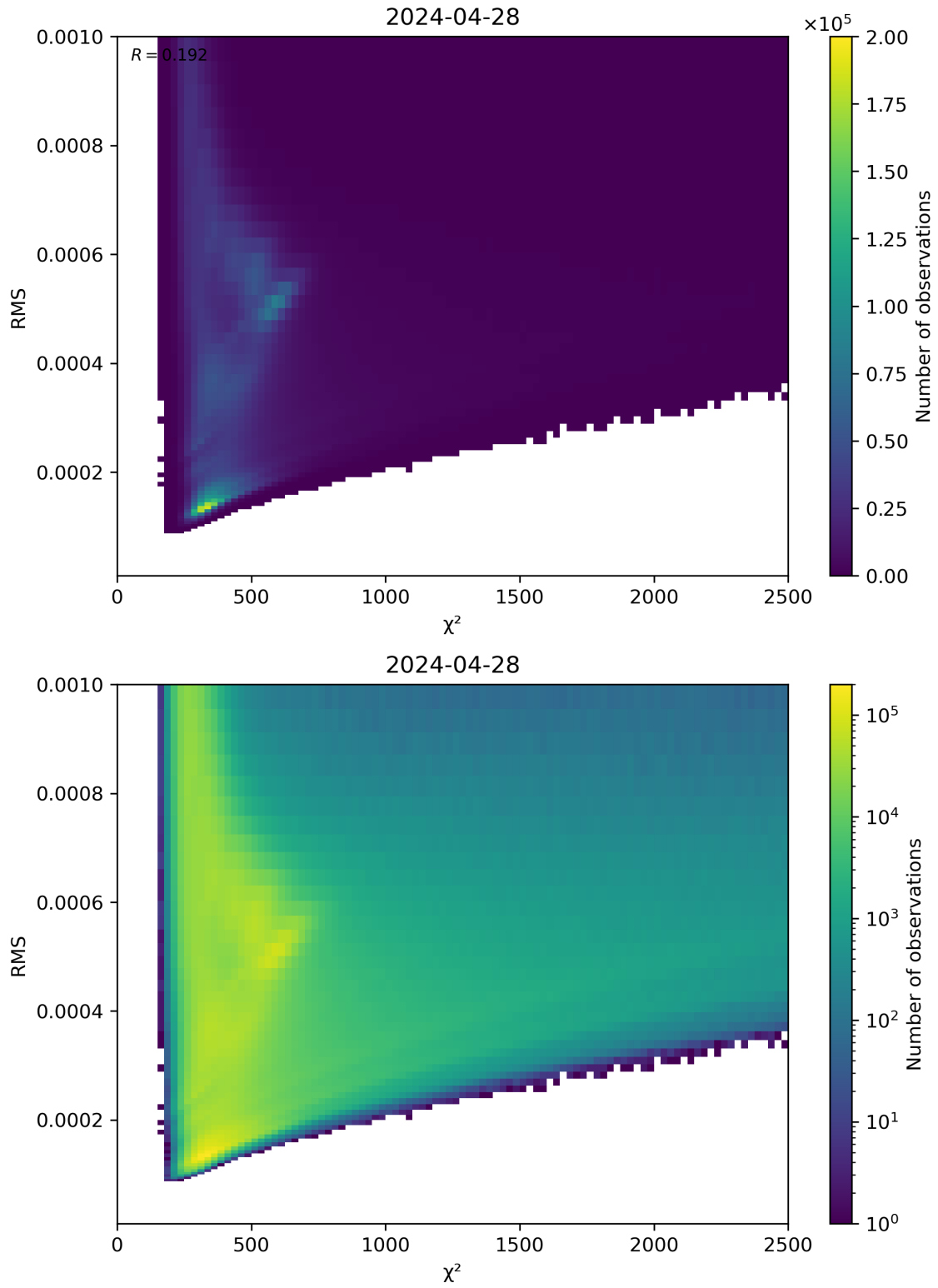
Figure 82: Scatter density plot of “ \chi^2 ” against “RMS” for 2024-04-27 to 2024-04-29.
