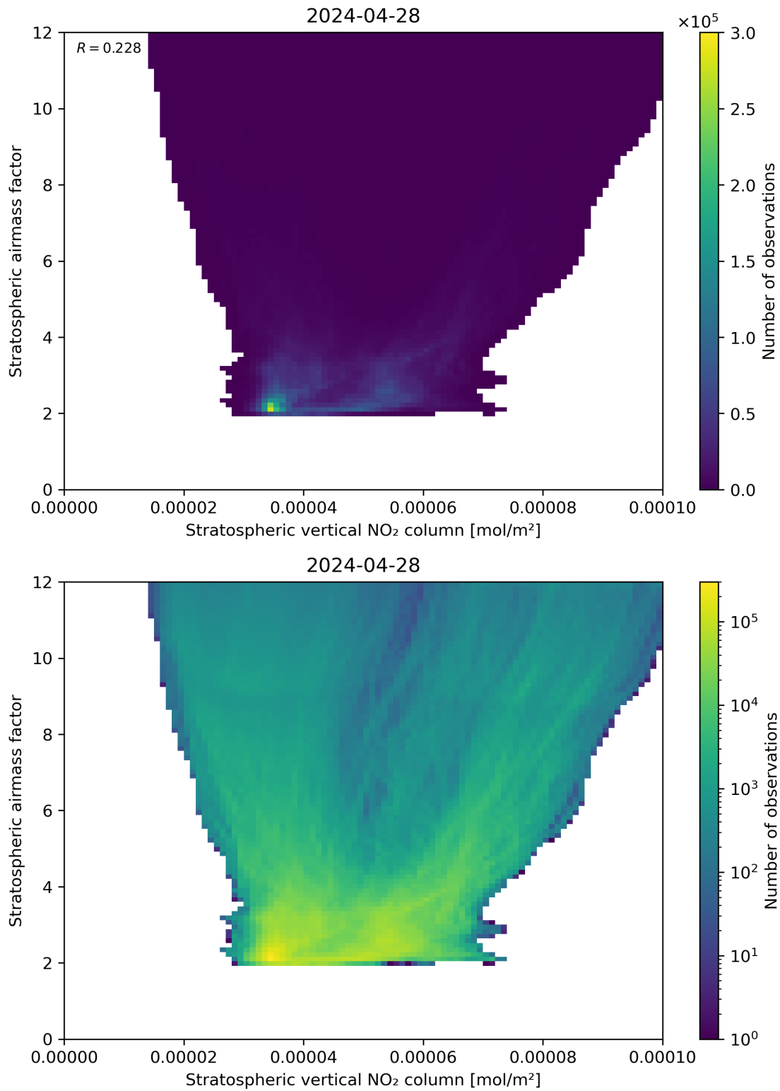
Figure 96: Scatter density plot of “Stratospheric vertical NO 2 column” against “Stratospheric airmass factor” for 2024-04-27 to 2024-04-29.
