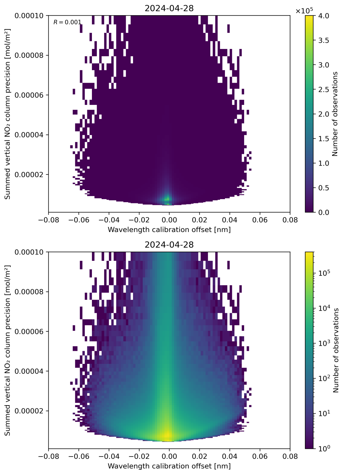
Figure 178: Scatter density plot of “Wavelength calibration offset” against “Summed vertical NO 2 column precision” for 2024-04-27 to 2024-04-29.
