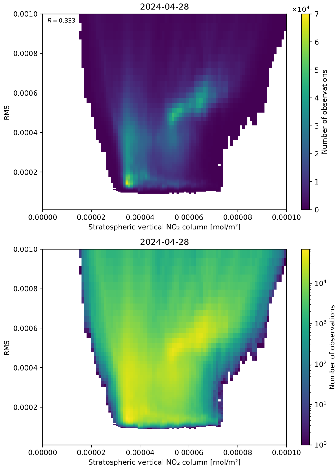
Figure 102: Scatter density plot of “Stratospheric vertical NO 2 column” against “RMS” for 2024-04-27 to 2024-04-29.
