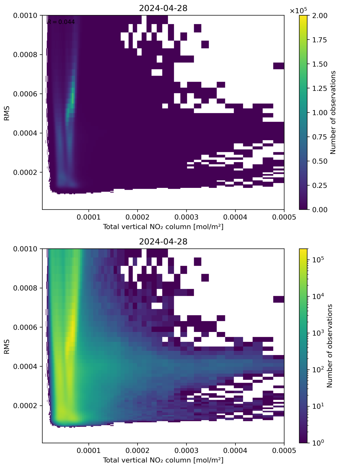
Figure 120: Scatter density plot of “Total vertical NO 2 column” against “RMS” for 2024-04-27 to 2024-04-29.
