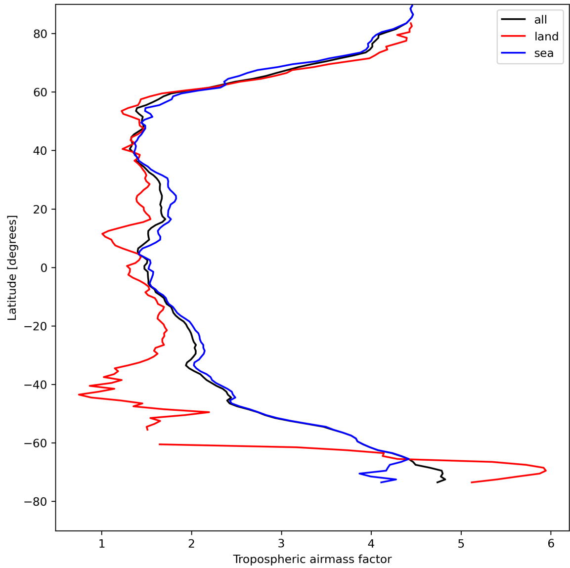
Figure 14: Zonal average of “Tropospheric airmass factor” for 2024-04-27 to 2024-04-29.
