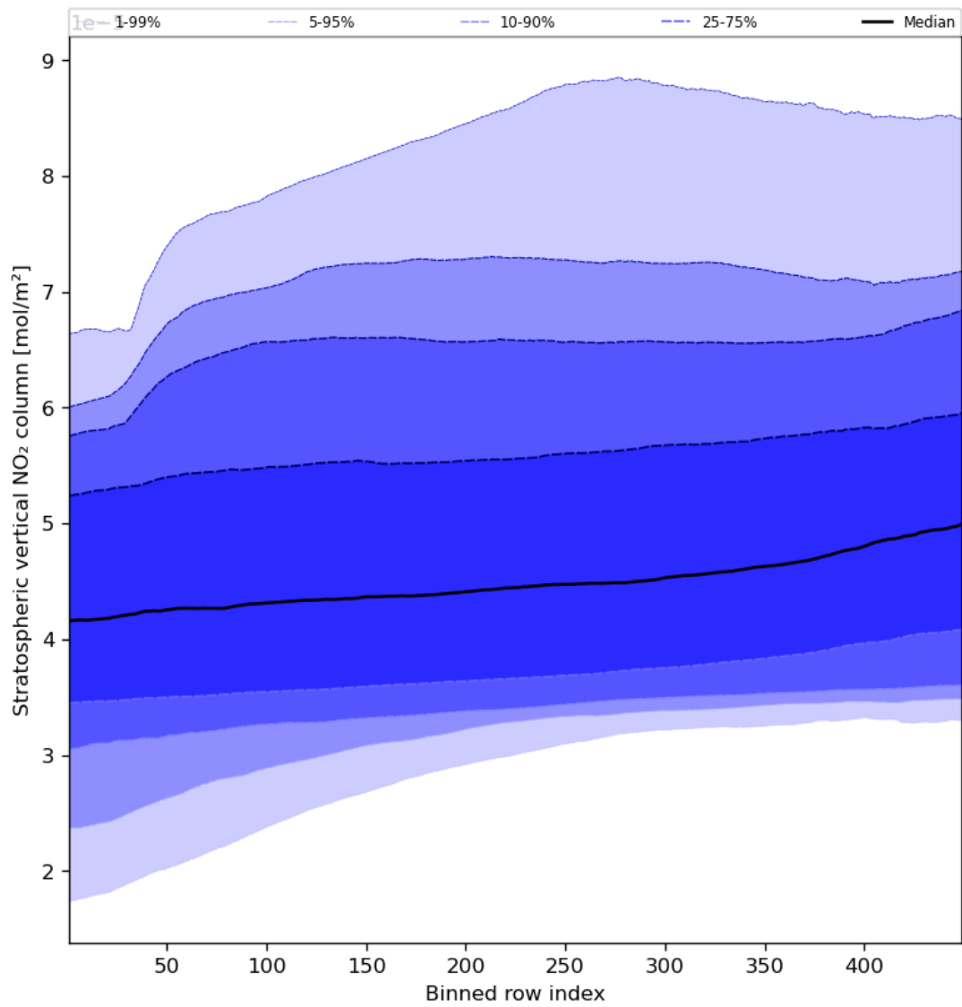
Figure 53: Along track statistics of “Stratospheric vertical NO 2 column” for 2024-04-27 to 2024-04-29
