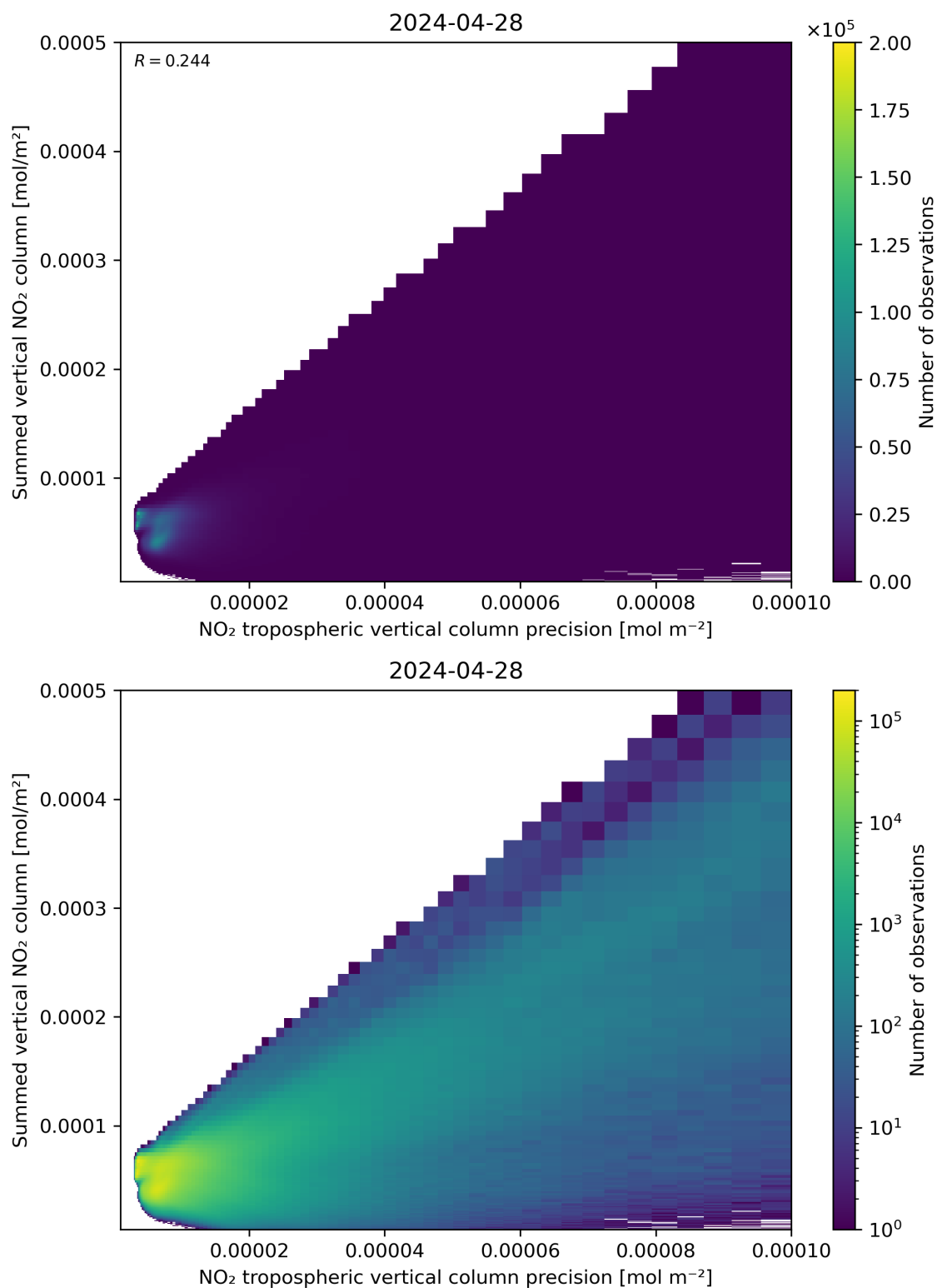
Figure 136: Scatter density plot of “NO 2 tropospheric vertical column precision” against “Summed vertical NO 2 column” for 2024-04-27 to 2024-04-29.
