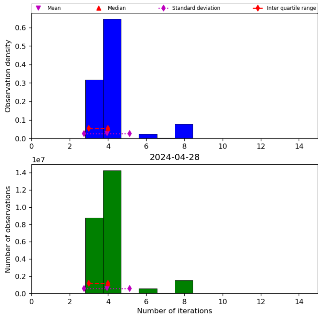
Figure 34: Histogram of “Number of iterations” for 2024-04-27 to 2024-04-29
