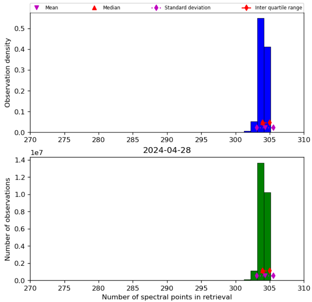
Figure 33: Histogram of “Number of spectral points in retrieval” for 2024-04-27 to 2024-04-29
