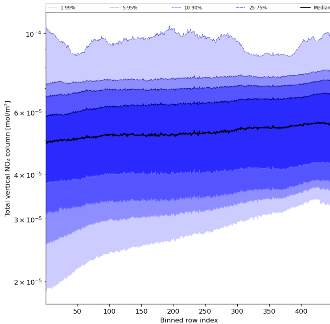
Figure 55: Along track statistics of “Total vertical NO 2 column” for 2024-04-27 to 2024-04-29
