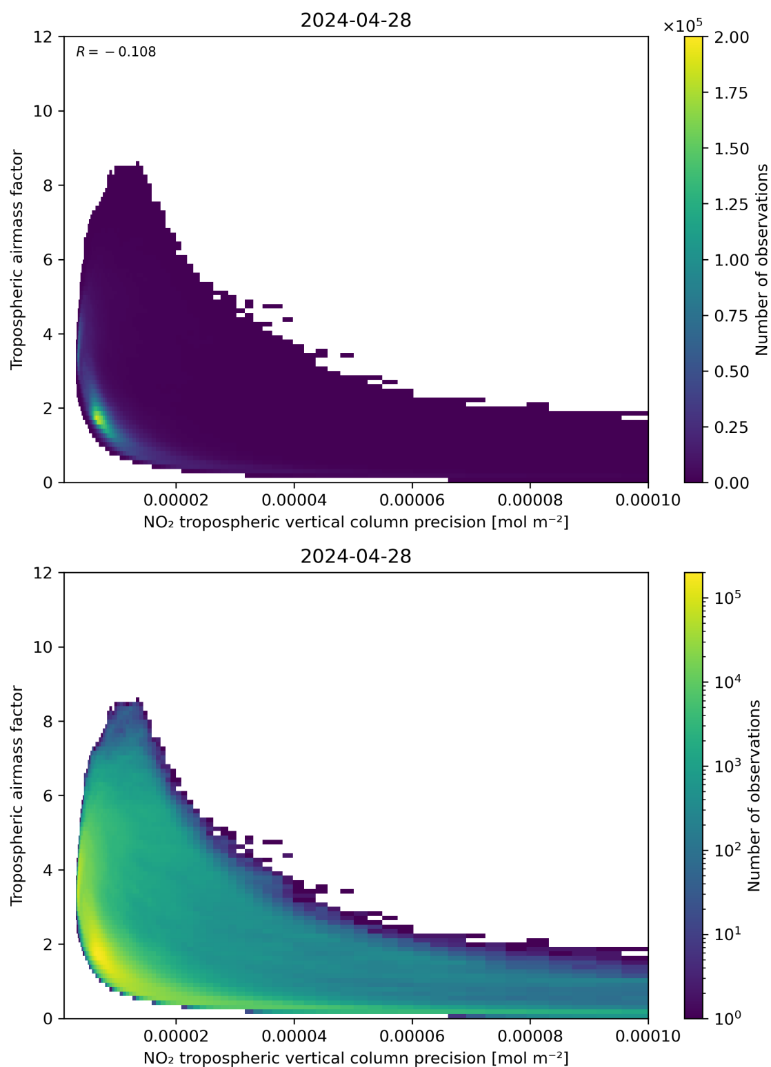
Figure 133: Scatter density plot of “NO 2 tropospheric vertical column precision” against “Tropospheric airmass factor” for 2024-04-27 to 2024-04-29.
