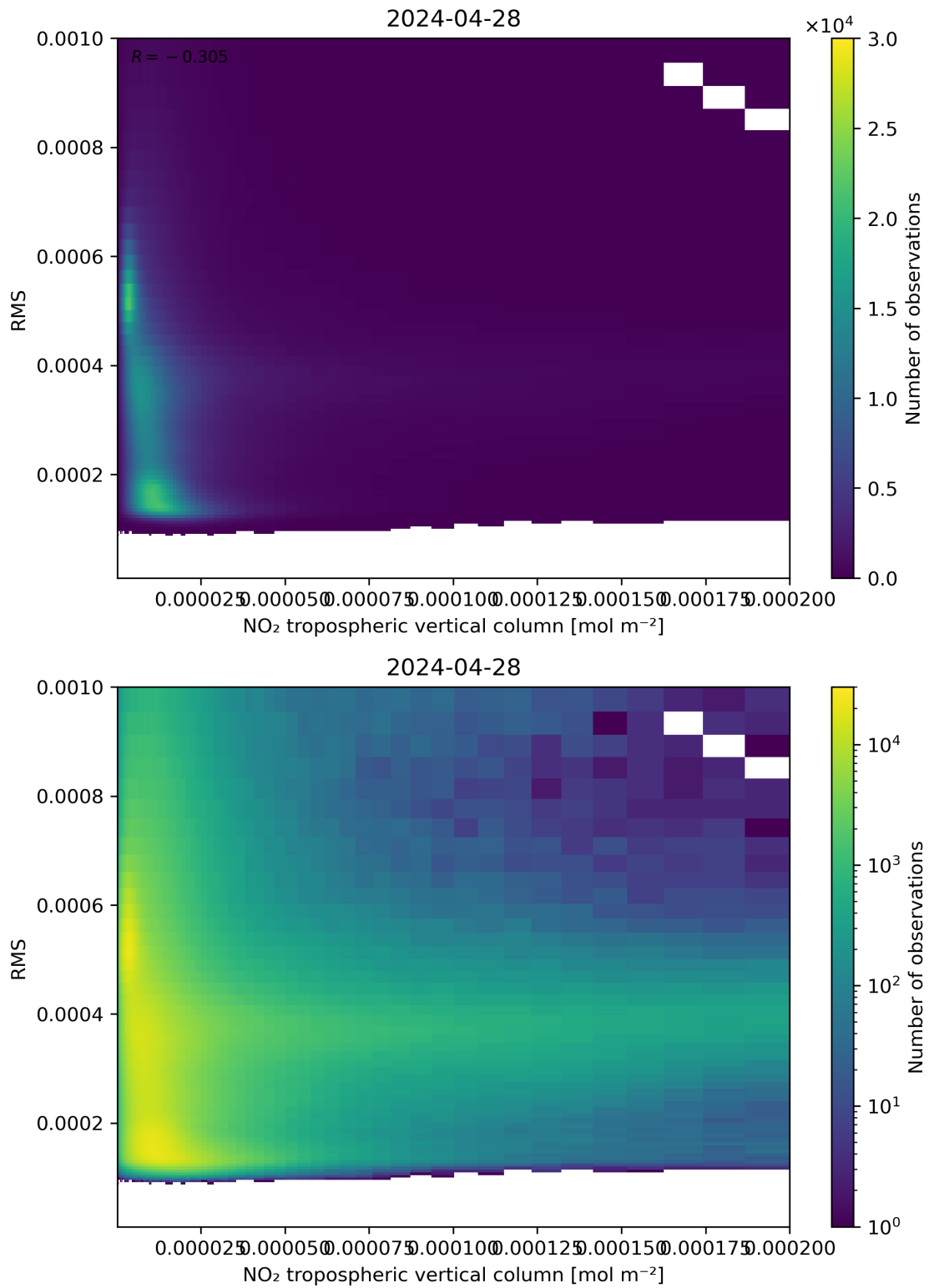
Figure 142: Scatter density plot of “NO 2 tropospheric vertical column” against “RMS” for 2024-04-27 to 2024-04-29.
