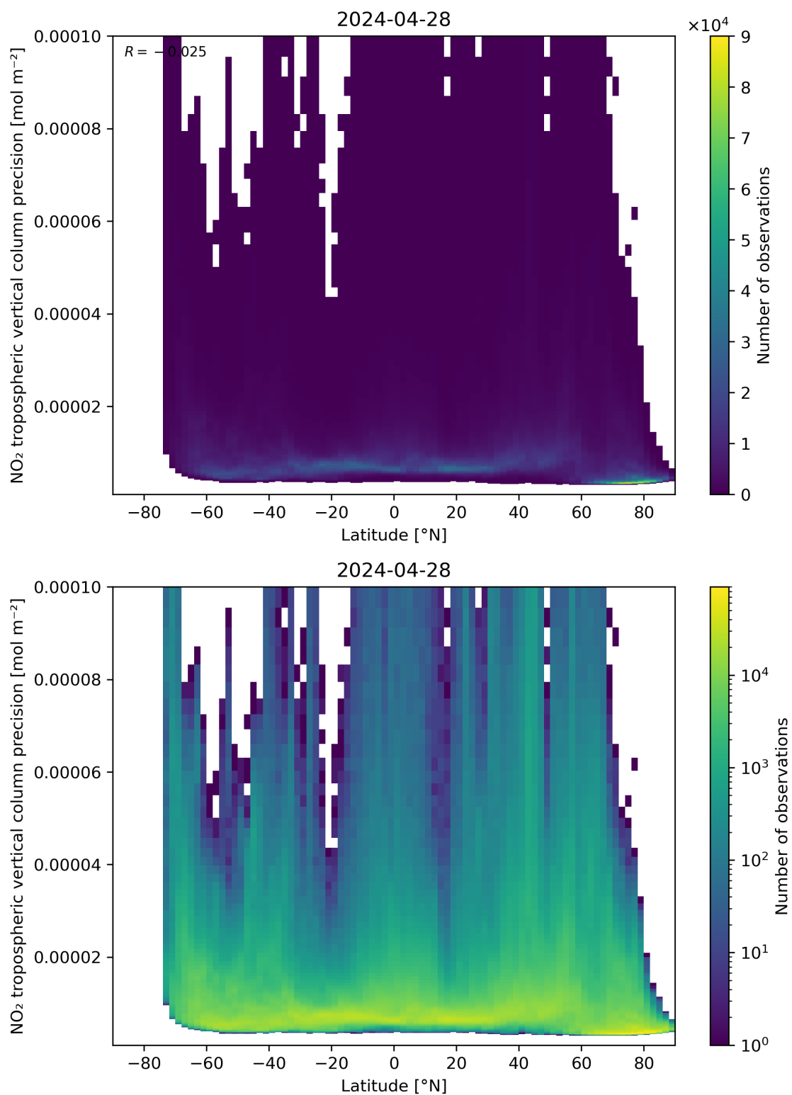
Figure 93: Scatter density plot of “Latitude” against “NO 2 tropospheric vertical column precision” for 2024-04-27 to 2024-04-29.
