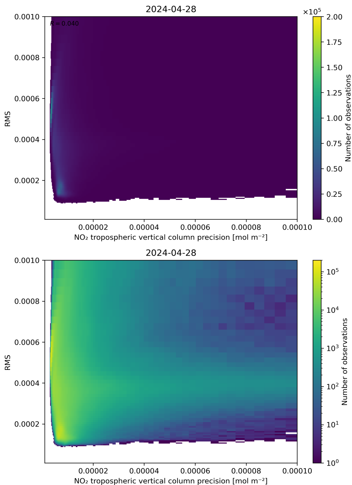
Figure 140: Scatter density plot of “NO 2 tropospheric vertical column precision” against “RMS” for 2024-04-27 to 2024-04-29.
