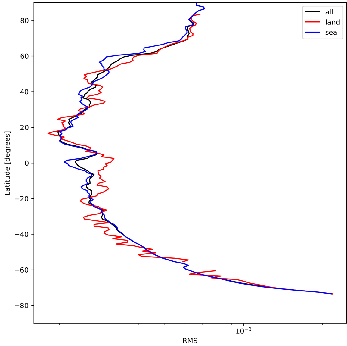
Figure 26: Zonal average of “RMS” for 2024-04-27 to 2024-04-29.
