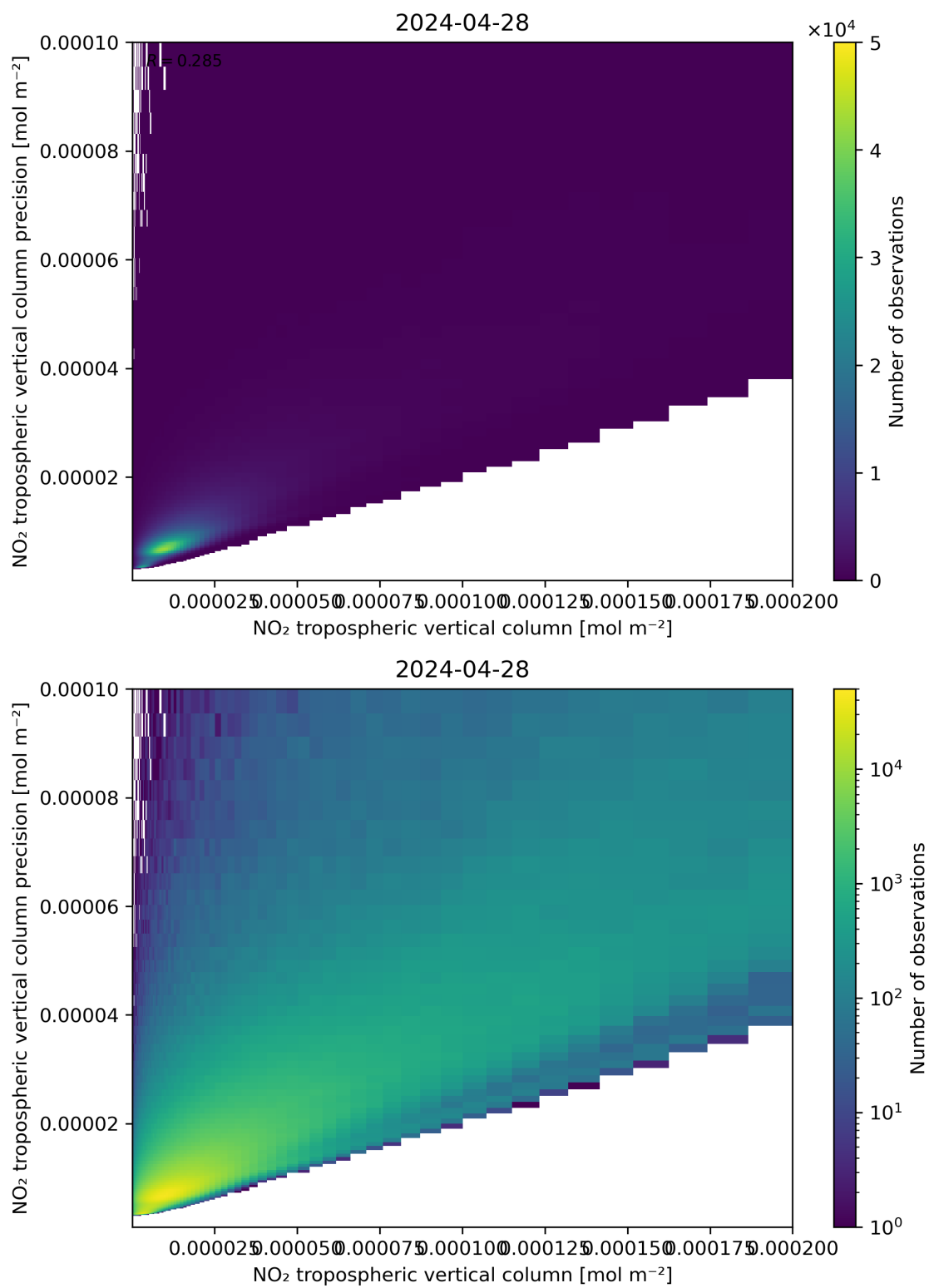
Figure 130: Scatter density plot of “NO 2 tropospheric vertical column” against “NO 2 tropospheric vertical column precision” for 2024-04-27 to 2024-04-29.
