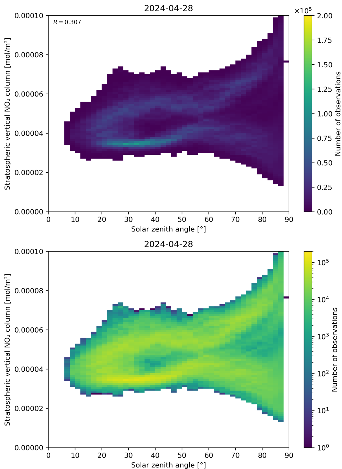
Figure 150: Scatter density plot of “Solar zenith angle” against “Stratospheric vertical NO 2 column” for 2024-04-27 to 2024-04-29.
