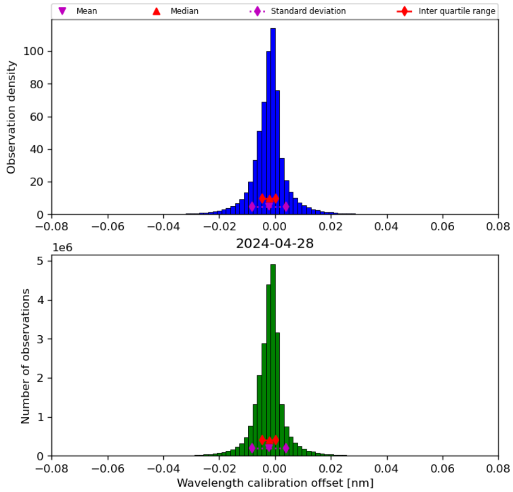
Figure 35: Histogram of “Wavelength calibration offset” for 2024-04-27 to 2024-04-29
