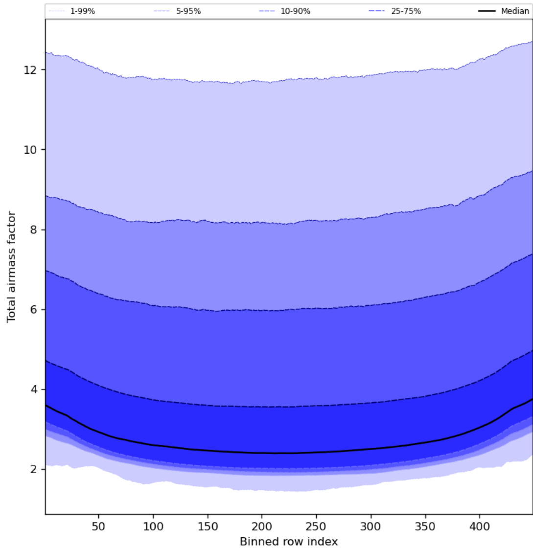
Figure 49: Along track statistics of “Total airmass factor” for 2024-04-27 to 2024-04-29
