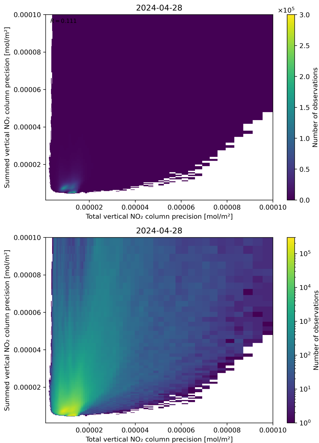
Figure 118: Scatter density plot of “Total vertical NO 2 column precision” against “Summed vertical NO 2 column precision” for 2024-04-27 to 2024-04-29.
