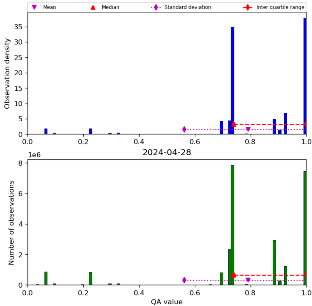
Figure 28: Histogram of “QA value” for 2024-04-27 to 2024-04-29
