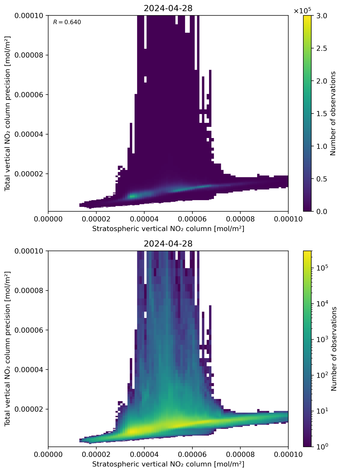
Figure 101: Scatter density plot of “Stratospheric vertical NO 2 column” against “Total vertical NO 2 column precision” for 2024-04-27 to 2024-04-29.
