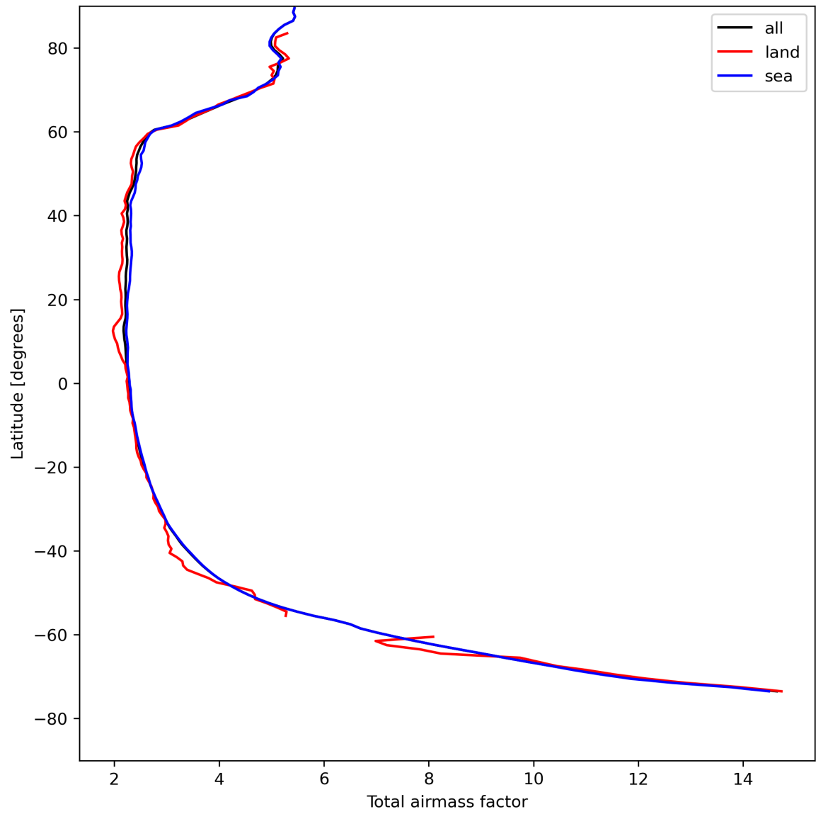
Figure 15: Zonal average of “Total airmass factor” for 2024-04-27 to 2024-04-29.
