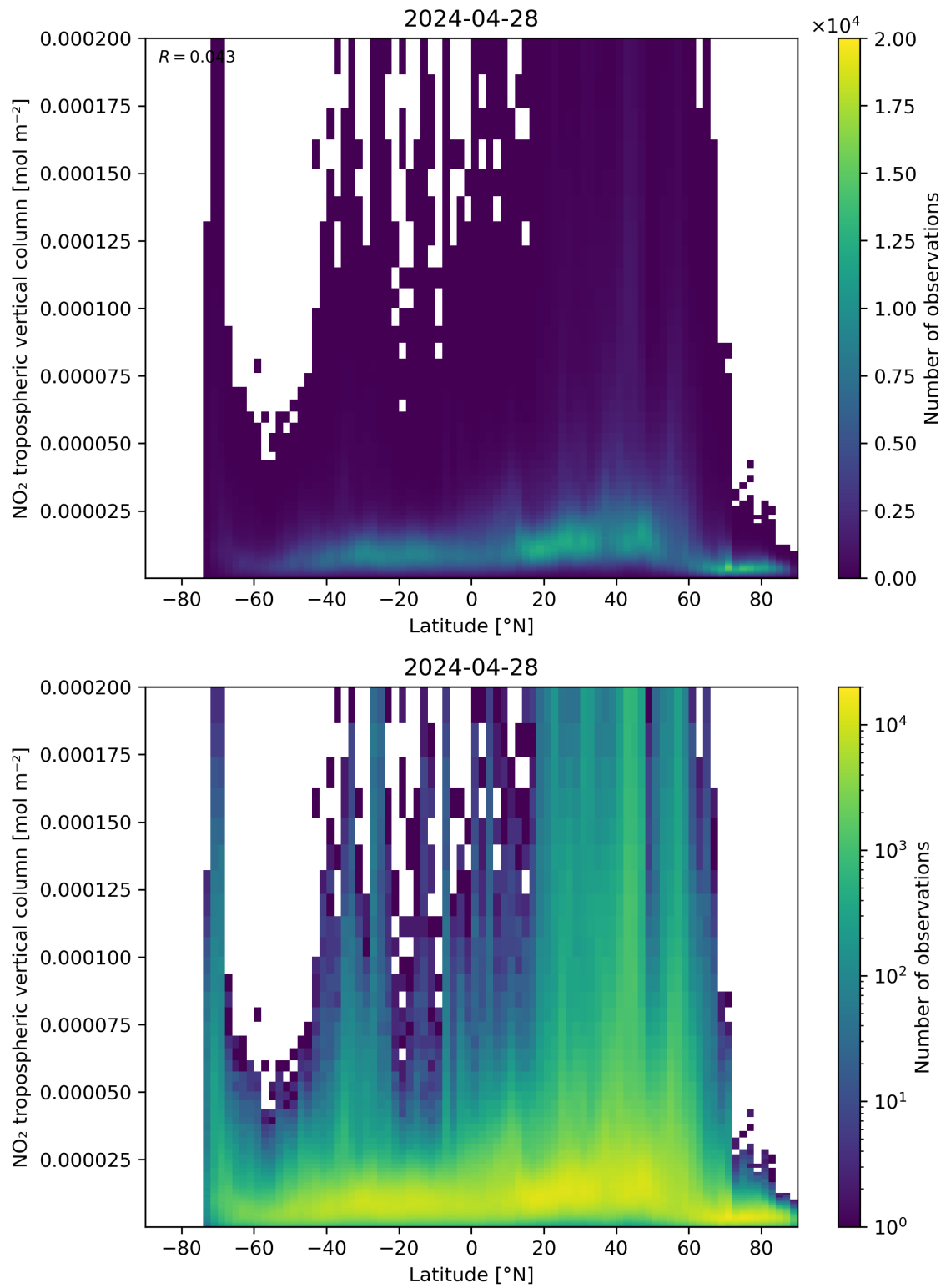
Figure 92: Scatter density plot of “Latitude” against “NO 2 tropospheric vertical column” for 2024-04-27 to 2024-04-29.
