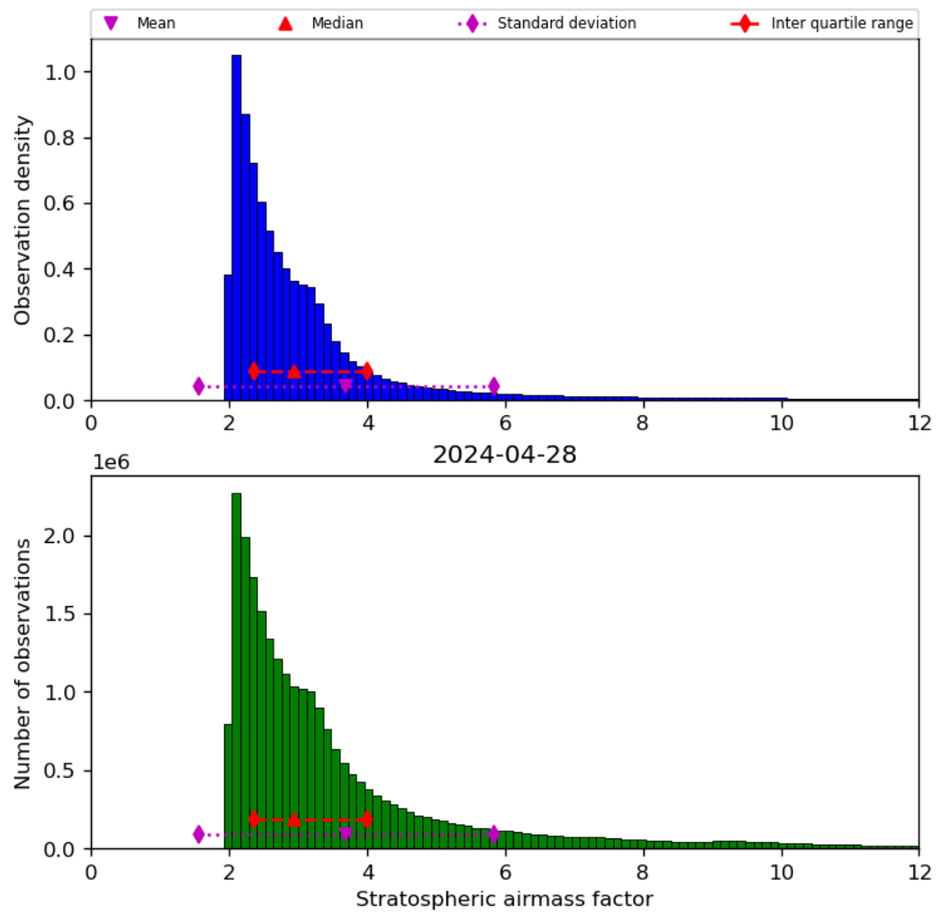
Figure 44: Histogram of “Stratospheric airmass factor” for 2024-04-27 to 2024-04-29
