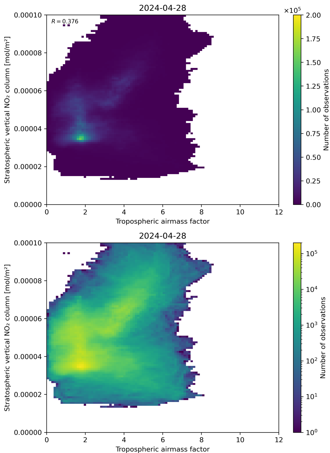
Figure 74: Scatter density plot of “Tropospheric air mass factor” against “Stratospheric vertical NO 2 column” for 2024-04-27 to 2024-04-29.
