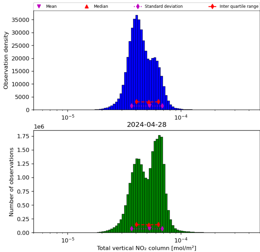
Figure 38: Histogram of “Total vertical NO 2 column” for 2024-04-27 to 2024-04-29
