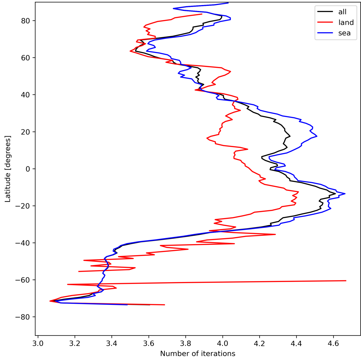
Figure 17: Zonal average of “Number of iterations” for 2024-04-27 to 2024-04-29.
