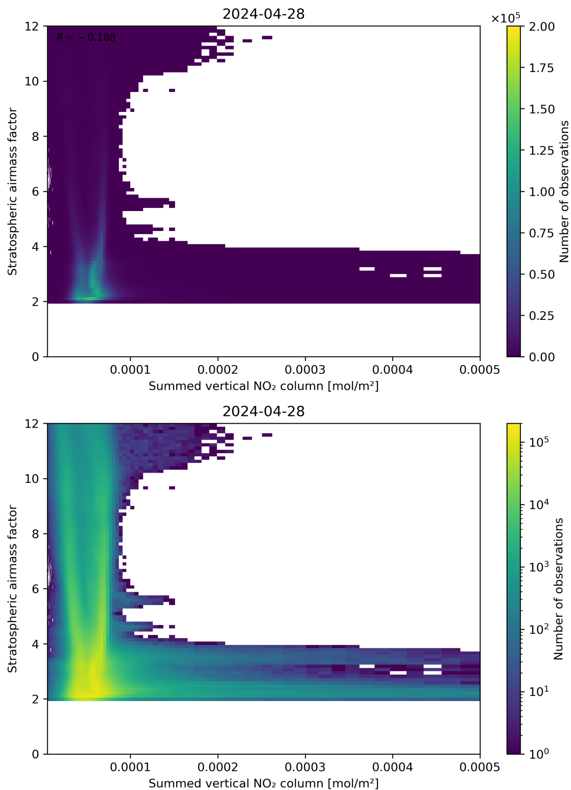
Figure 103: Scatter density plot of “Summed vertical NO 2 column” against “Stratospheric air mass factor” for 2024-04-27 to 2024-04-29.
