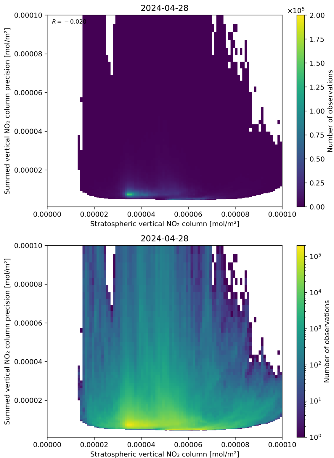
Figure 99: Scatter density plot of “Stratospheric vertical NO 2 column” against “Summed vertical NO 2 column precision” for 2024-04-27 to 2024-04-29.
