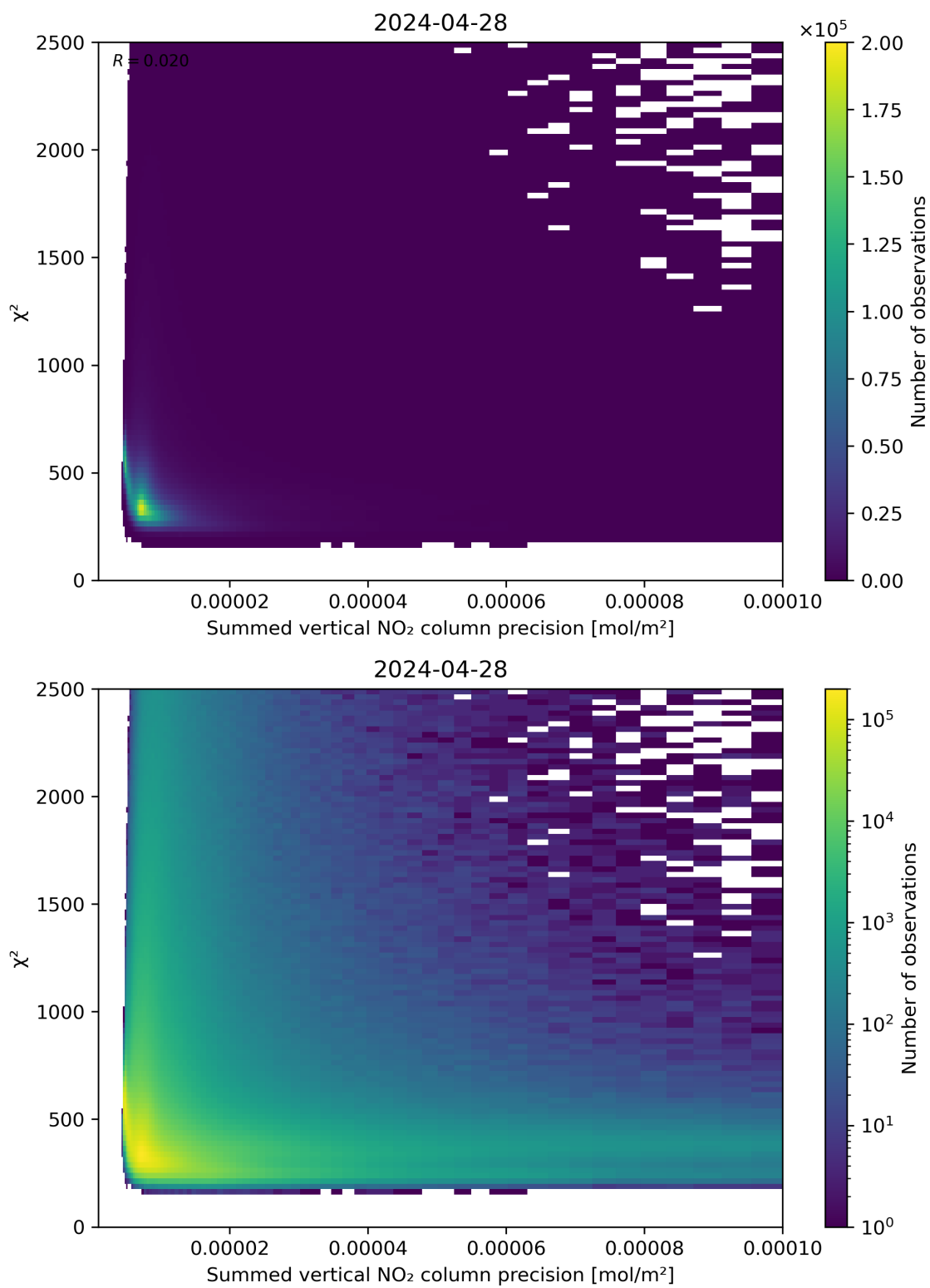
Figure 107: Scatter density plot of “Summed vertical NO 2 column precision” against “ \chi^2 ” for 2024-04-27 to 2024-04-29.
