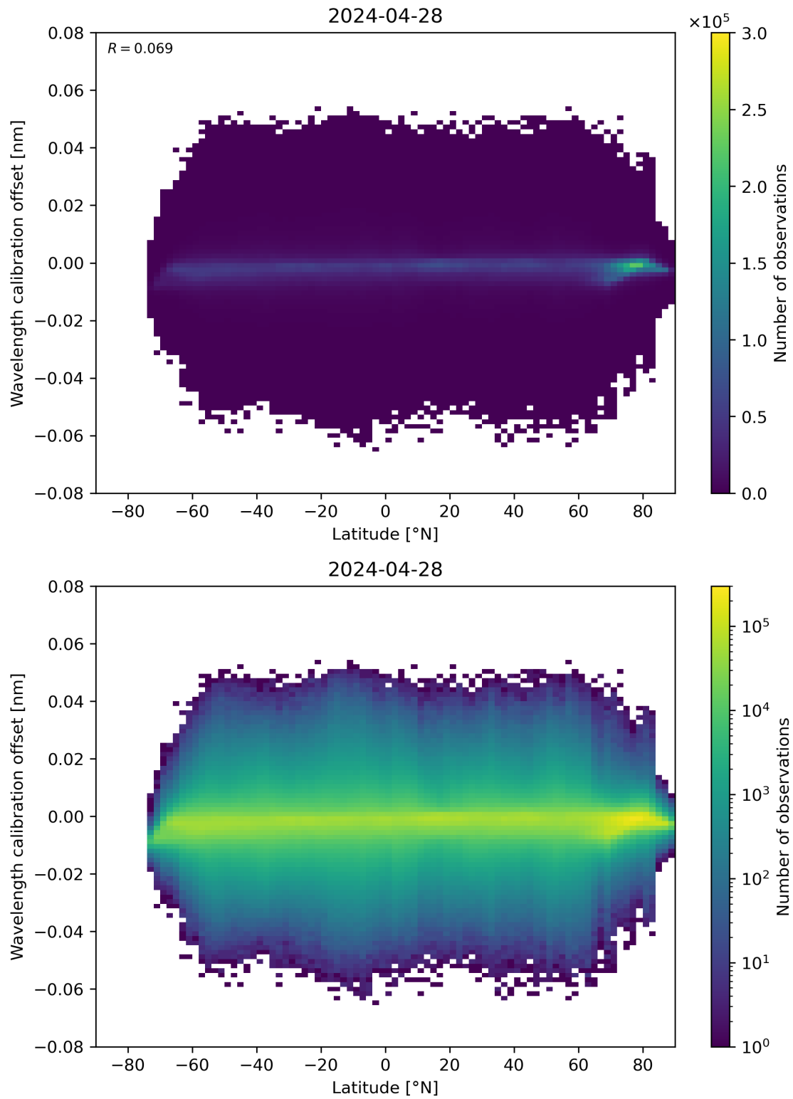
Figure 95: Scatter density plot of “Latitude” against “Wavelength calibration offset” for 2024-04-27 to 2024-04-29.
