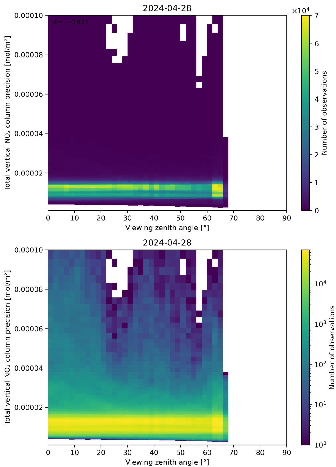
Figure 168: Scatter density plot of “Viewing zenith angle” against “Total vertical NO 2 column precision” for 2024-04-27 to 2024-04-29.
