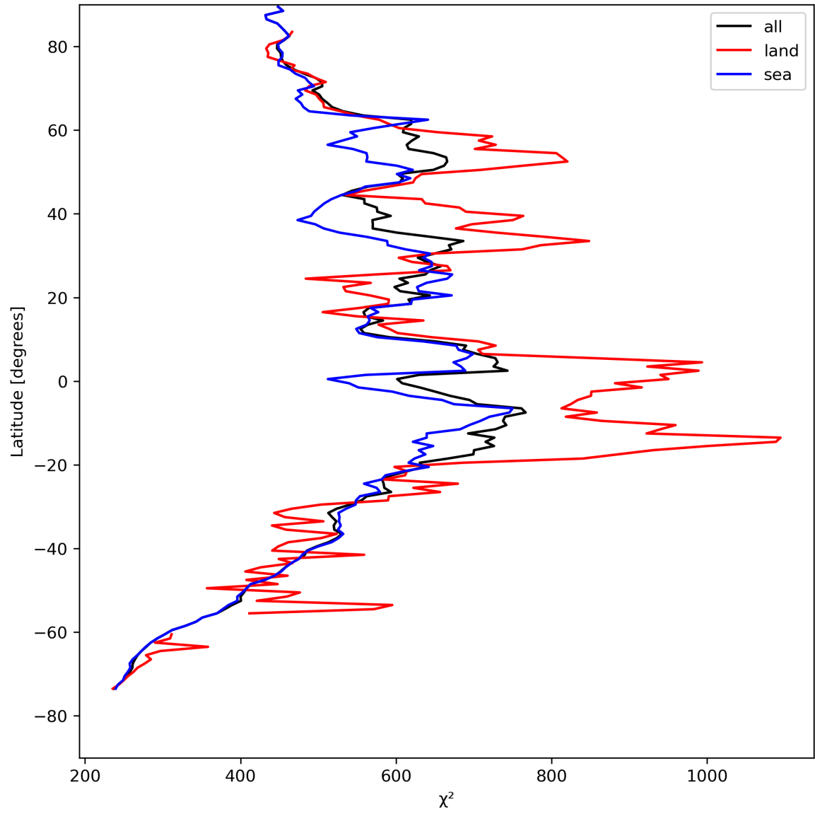
Figure 25: Zonal average of “ \chi^2 ” for 2024-04-27 to 2024-04-29.
