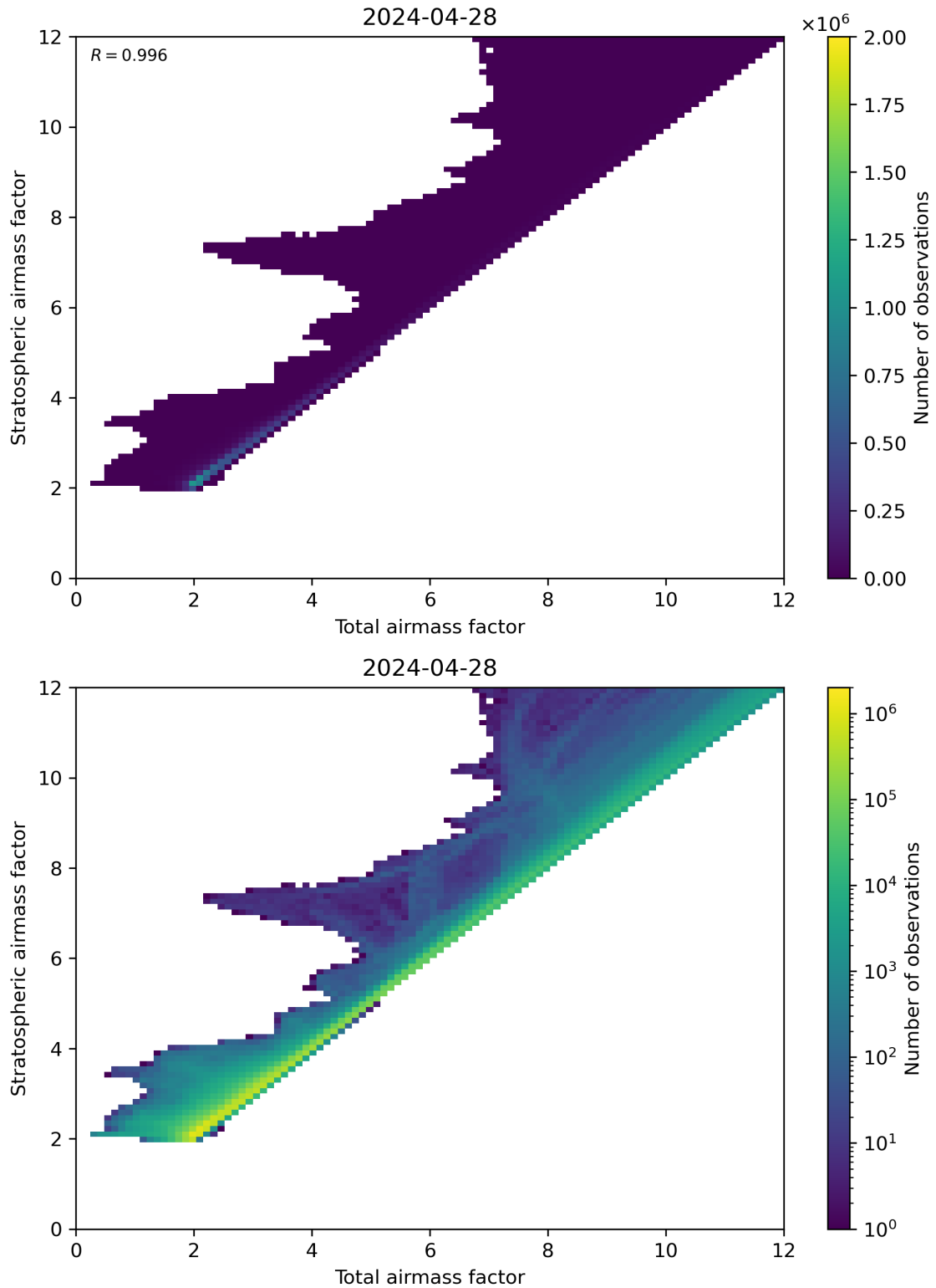
Figure 62: Scatter density plot of “Total airmass factor” against “Stratospheric airmass factor” for 2024-04-27 to 2024-04-29.
