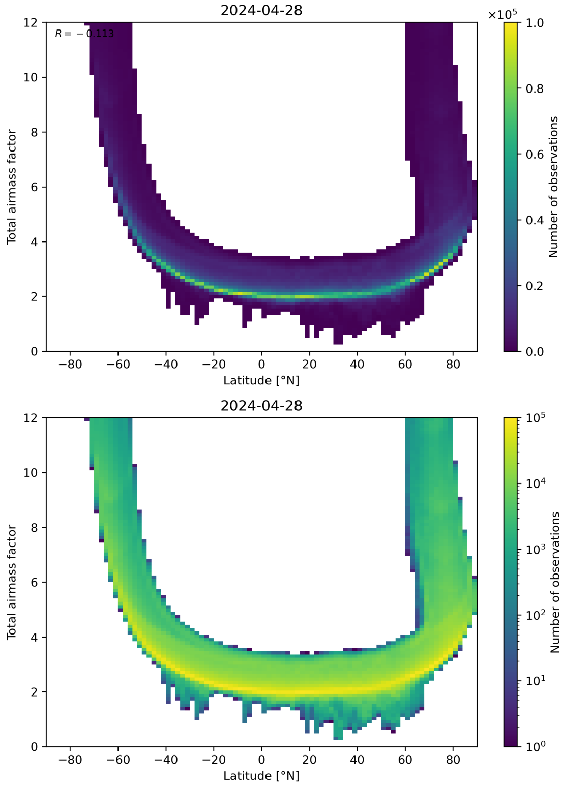
Figure 84: Scatter density plot of “Latitude” against “Total airmass factor” for 2024-04-27 to 2024-04-29.
