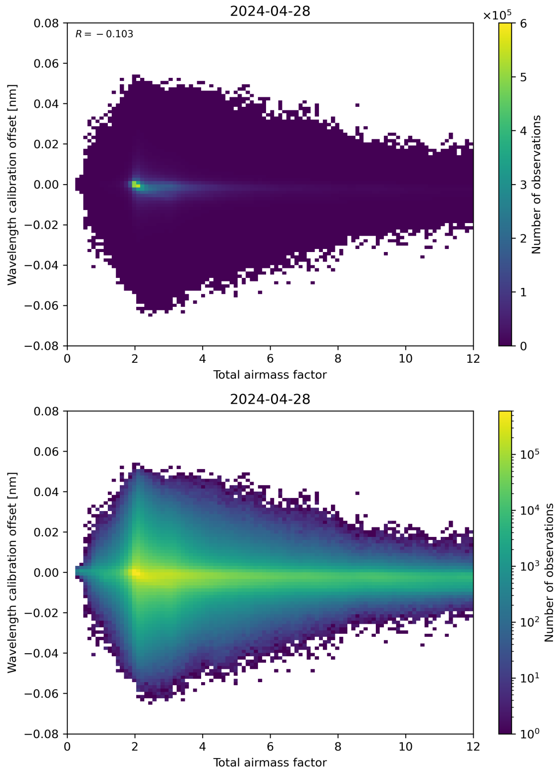
Figure 70: Scatter density plot of “Total airmass factor” against “Wavelength calibration offset” for 2024-04-27 to 2024-04-29.
