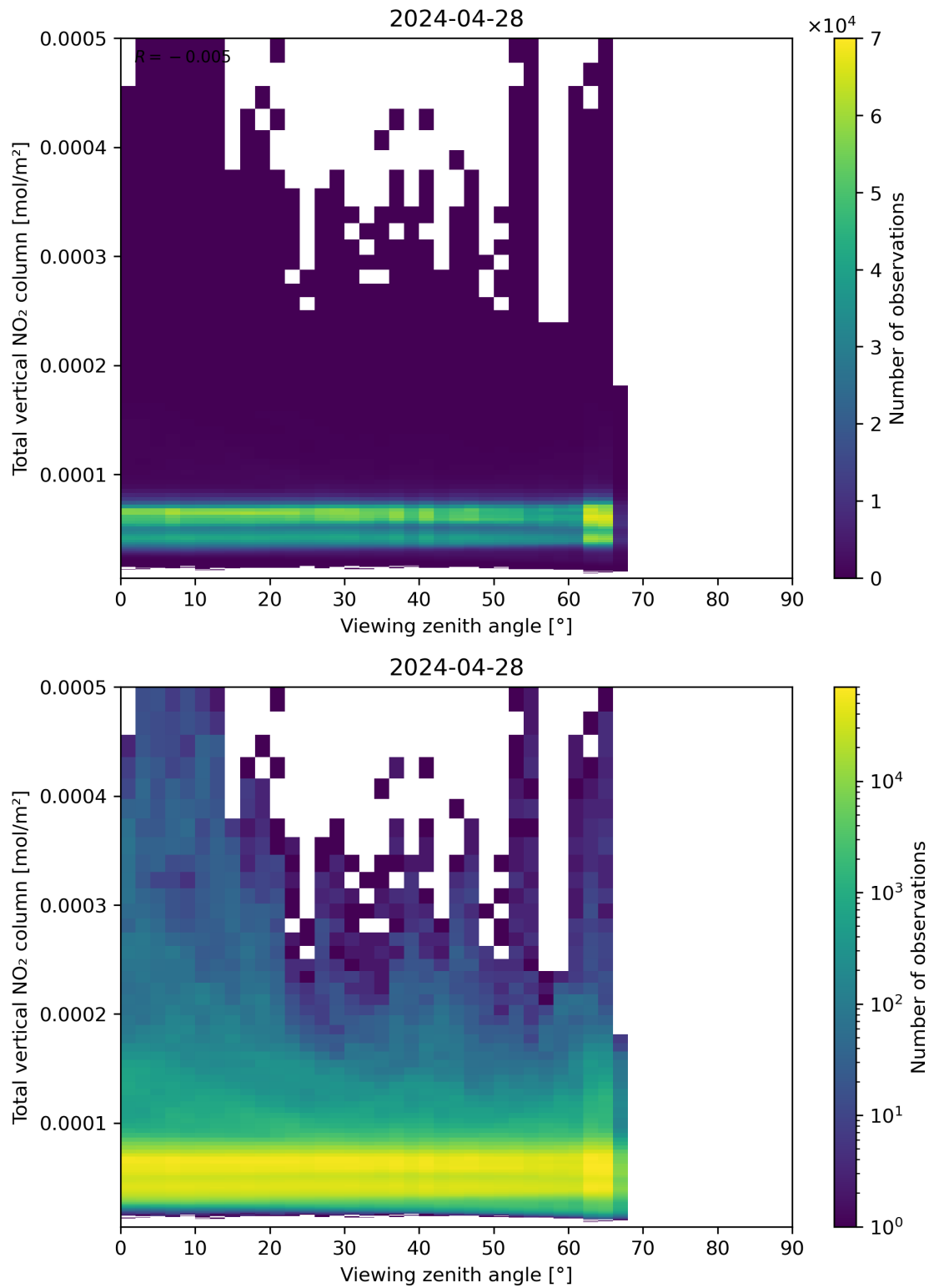
Figure 167: Scatter density plot of “Viewing zenith angle” against “Total vertical NO 2 column” for 2024-04-27 to 2024-04-29.
