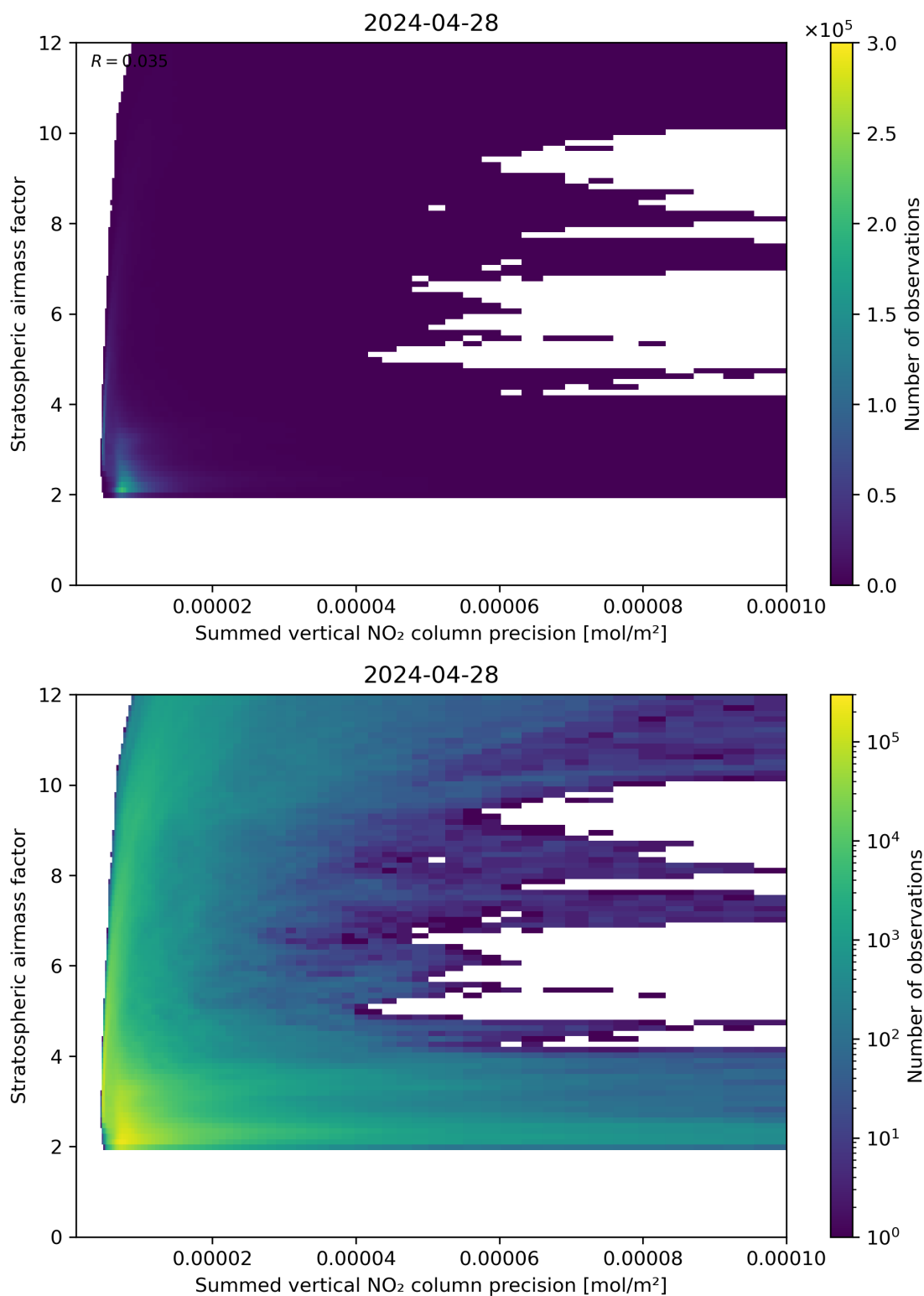
Figure 106: Scatter density plot of “Summed vertical NO 2 column precision” against “Stratospheric airmass factor” for 2024-04-27 to 2024-04-29.
