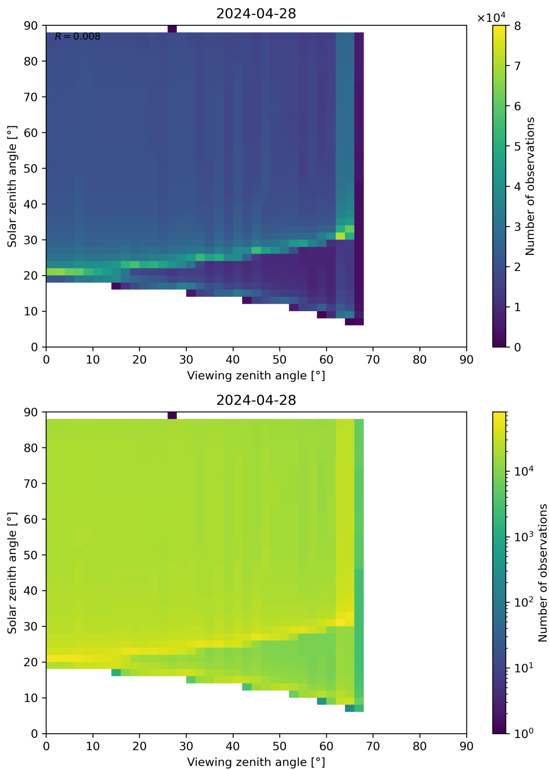
Figure 172: Scatter density plot of “Viewing zenith angle” against “Solar zenith angle” for 2024-04-27 to 2024-04-29.
