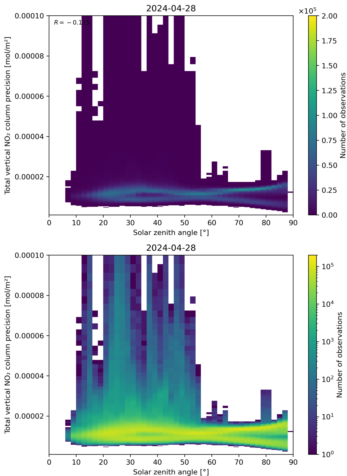
Figure 154: Scatter density plot of “Solar zenith angle” against “Total vertical NO 2 column precision” for 2024-04-27 to 2024-04-29.
