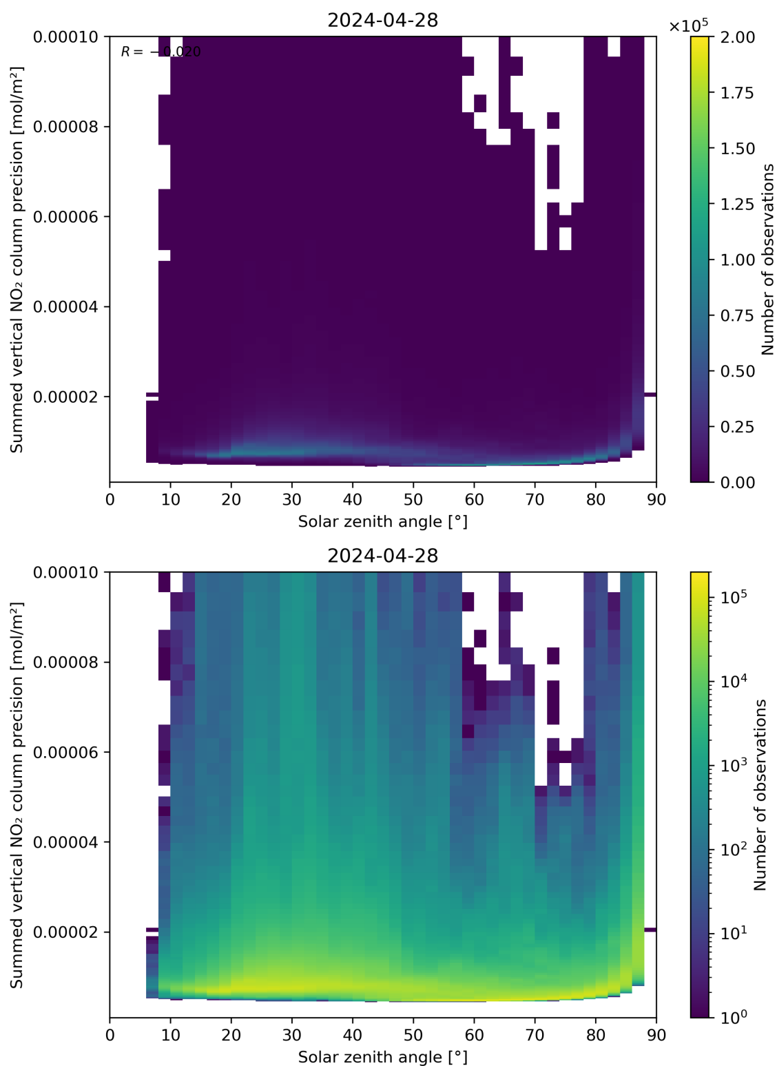
Figure 152: Scatter density plot of “Solar zenith angle” against “Summed vertical NO 2 column precision” for 2024-04-27 to 2024-04-29.
