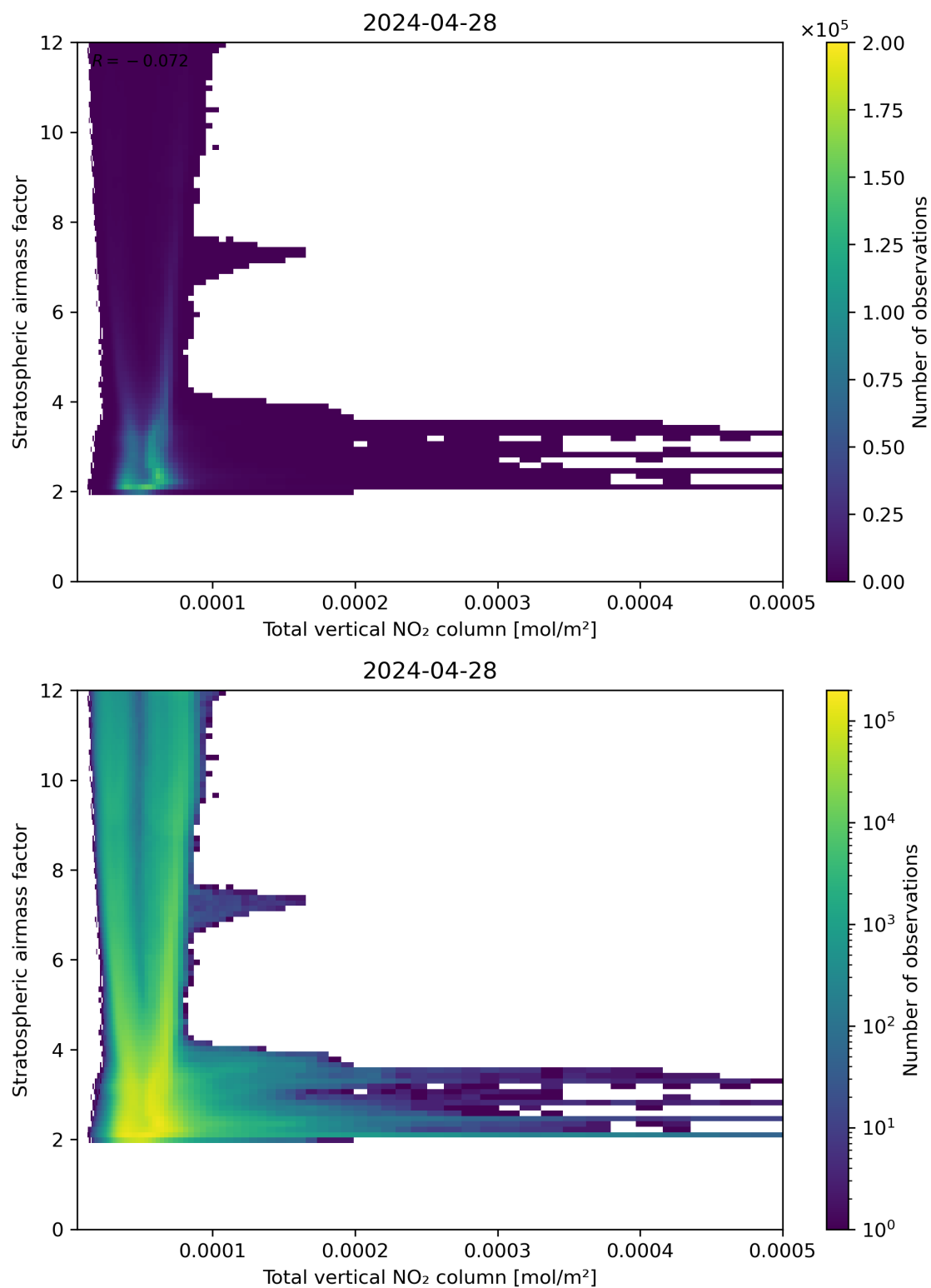
Figure 110: Scatter density plot of “Total vertical NO 2 column” against “Stratospheric airmass factor” for 2024-04-27 to 2024-04-29.
