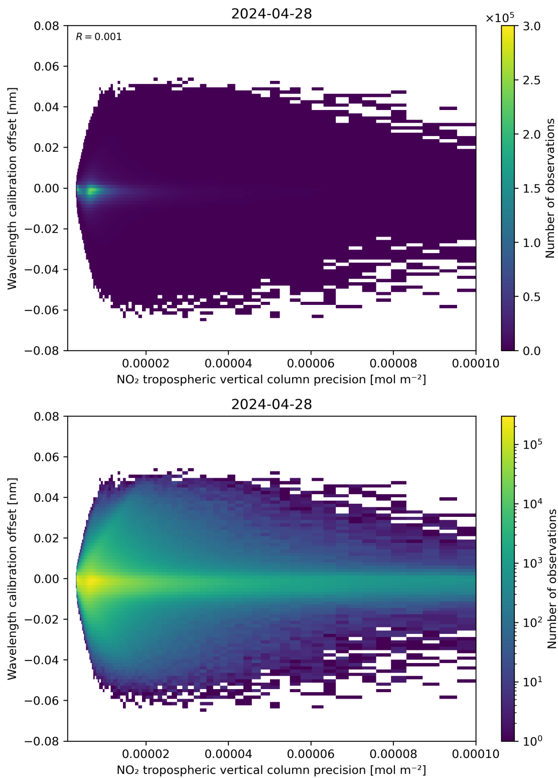
Figure 141: Scatter density plot of “NO 2 tropospheric vertical column precision” against “Wavelength calibration offset” for 2024-04-27 to 2024-04-29.
