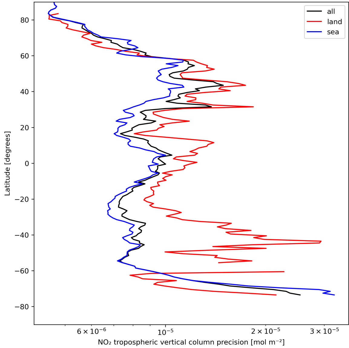
Figure 13: Zonal average of “NO 2 tropospheric vertical column precision” for 2024-04-27 to 2024-04-29.
