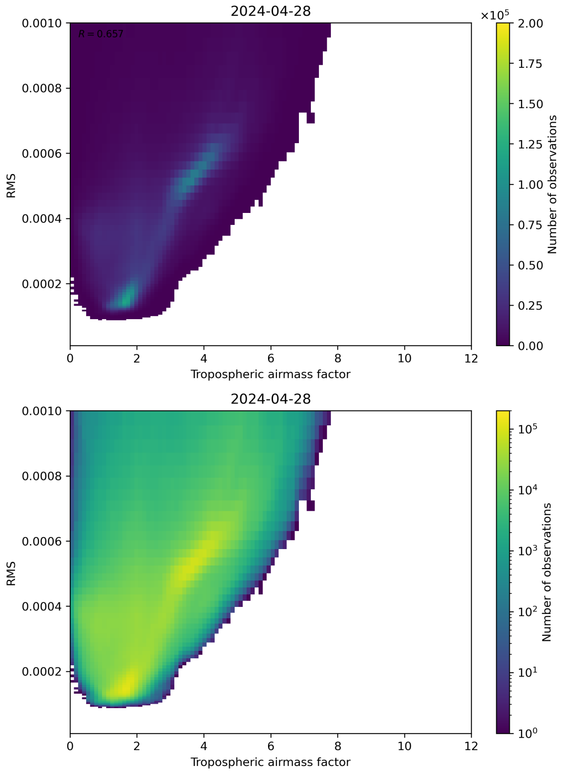
Figure 79: Scatter density plot of “Tropospheric airmass factor” against “RMS” for 2024-04-27 to 2024-04-29.
