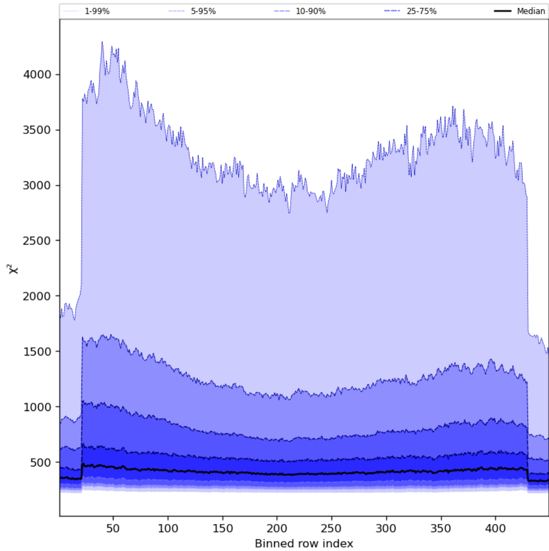
Figure 59: Along track statistics of “ \chi^2 ” for 2024-04-27 to 2024-04-29
