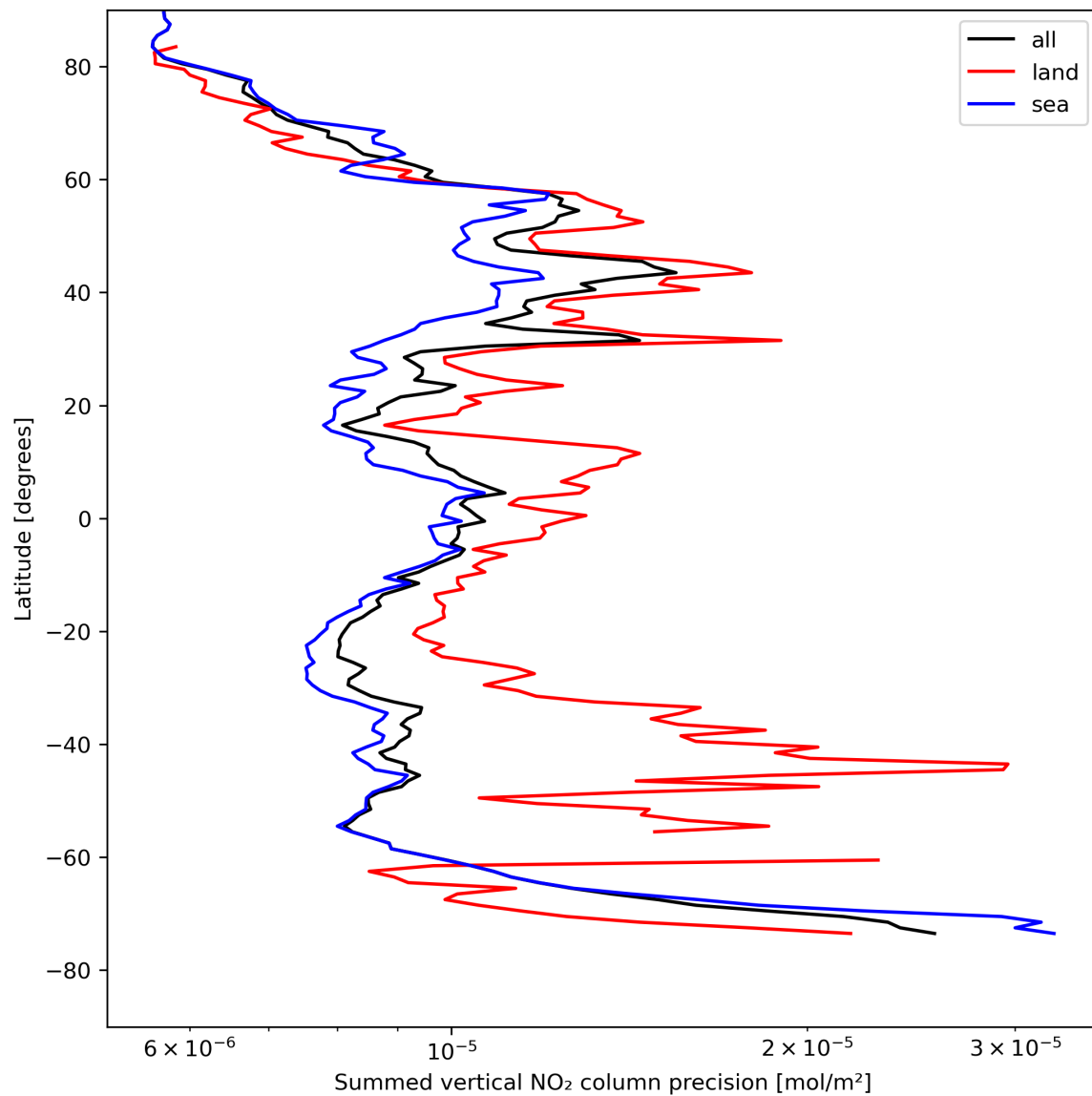
Figure 24: Zonal average of “Summed vertical NO 2 column precision” for 2024-04-27 to 2024-04-29.
