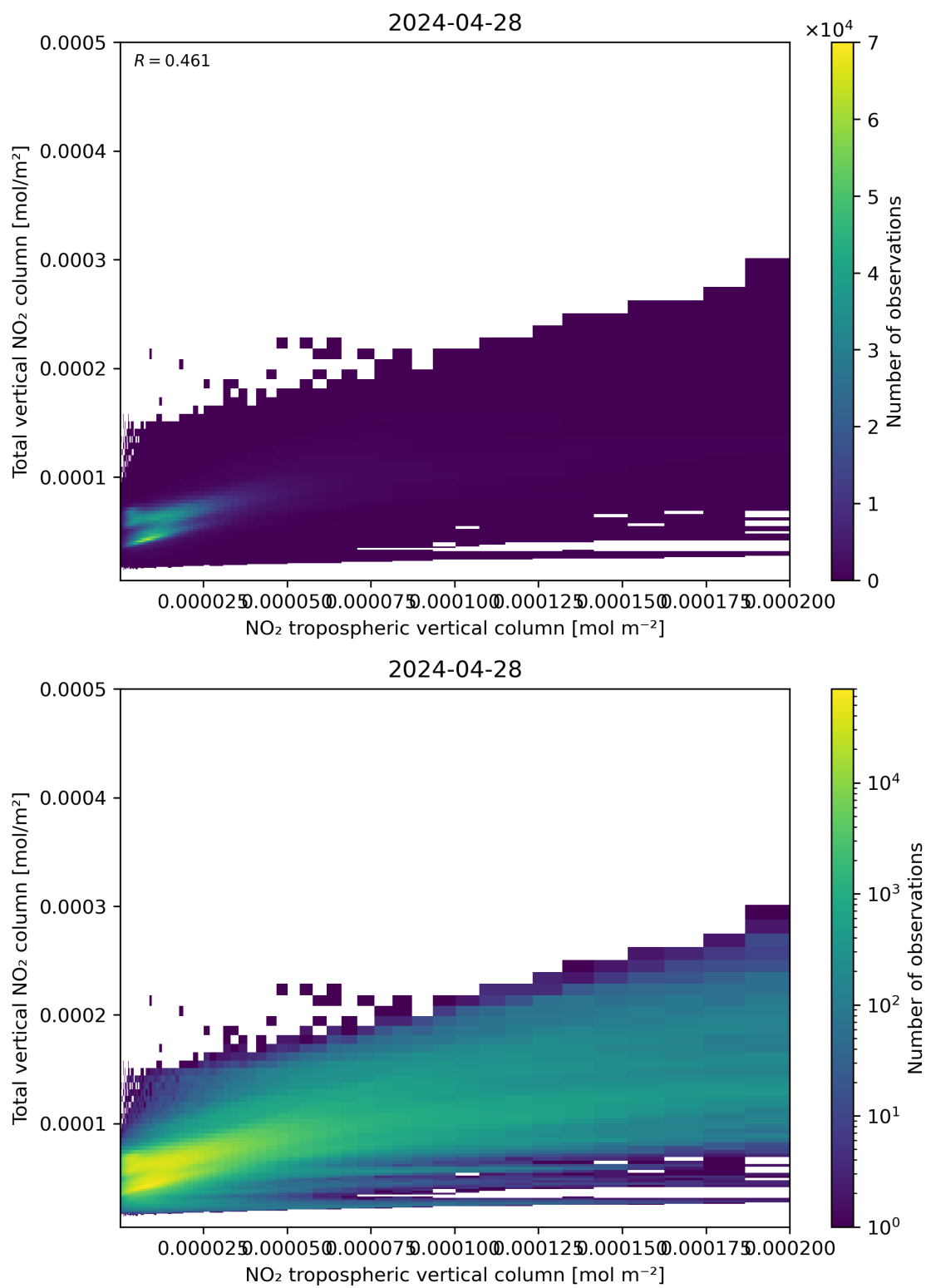
Figure 128: Scatter density plot of “NO 2 tropospheric vertical column” against “Total vertical NO 2 column” for 2024-04-27 to 2024-04-29.
