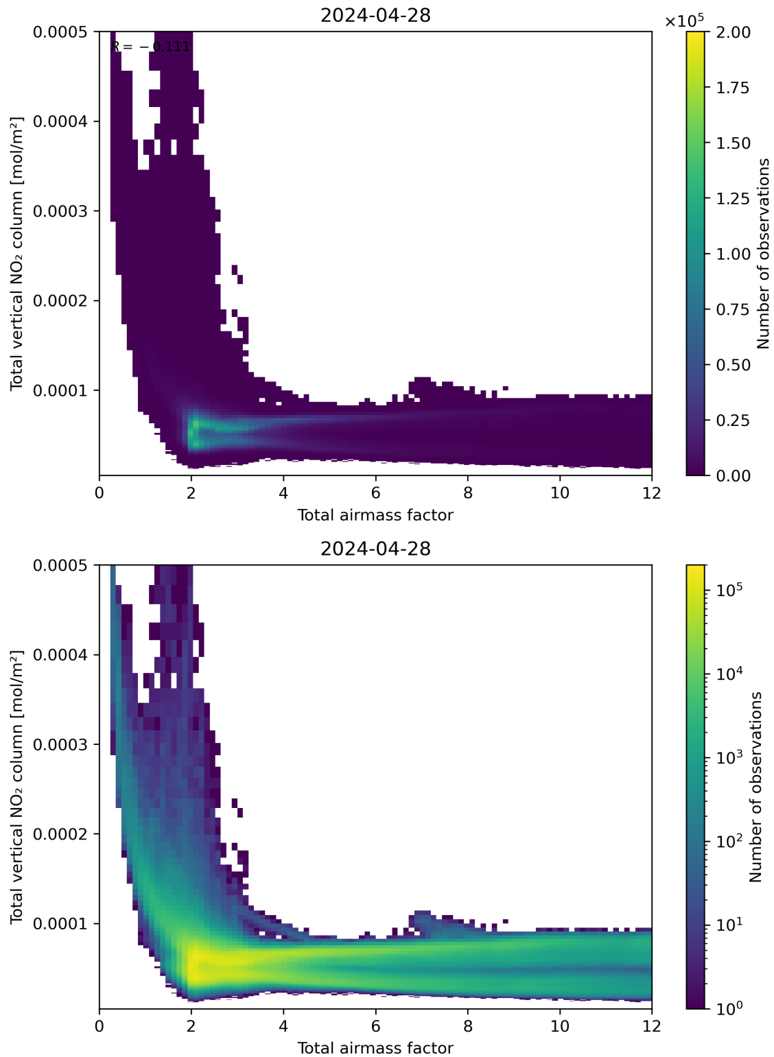
Figure 67: Scatter density plot of “Total airmass factor” against “Total vertical NO 2 column” for 2024-04-27 to 2024-04-29.
