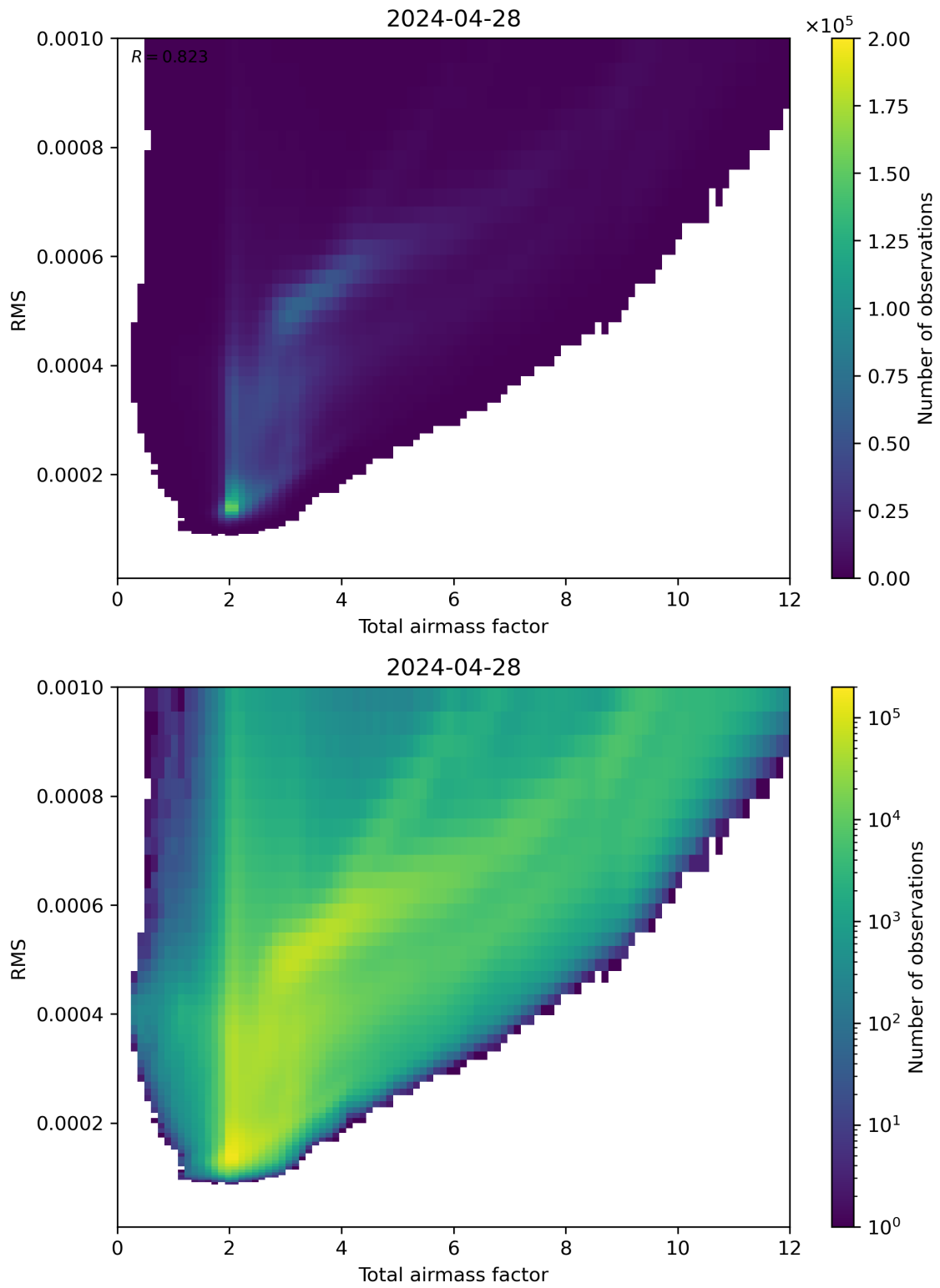
Figure 69: Scatter density plot of “Total airmass factor” against “RMS” for 2024-04-27 to 2024-04-29.
