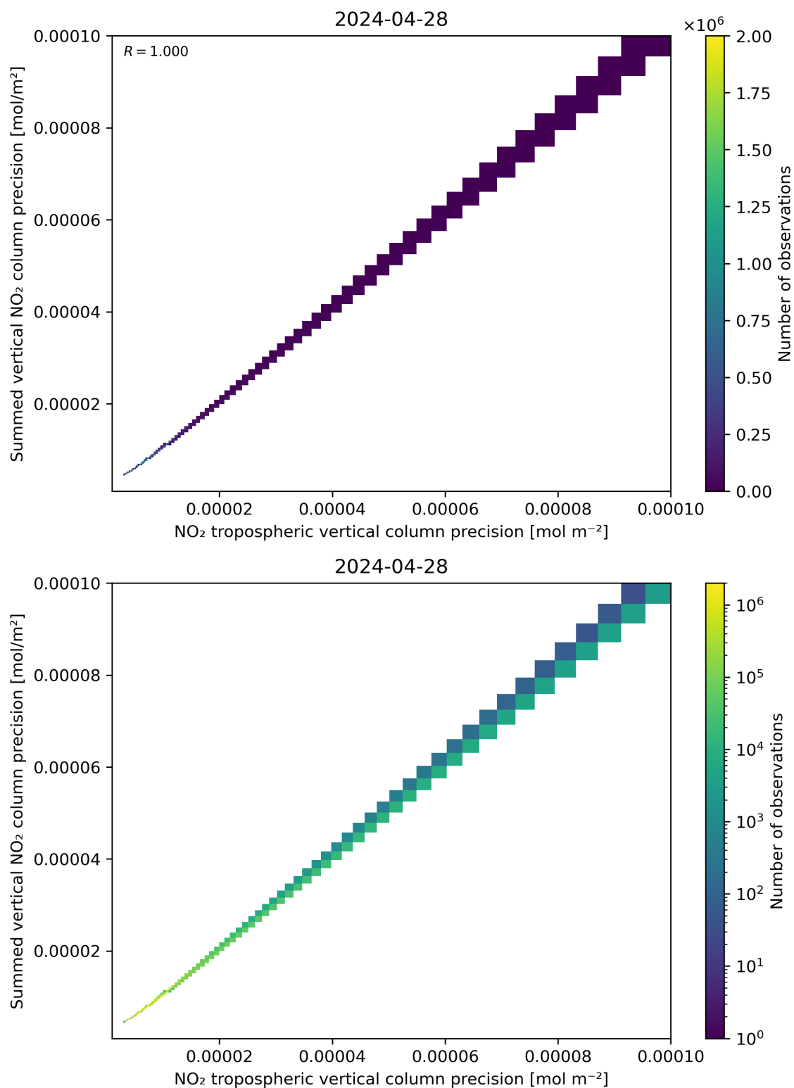
Figure 137: Scatter density plot of “NO 2 tropospheric vertical column precision” against “Summed vertical NO 2 column precision” for 2024-04-27 to 2024-04-29.
