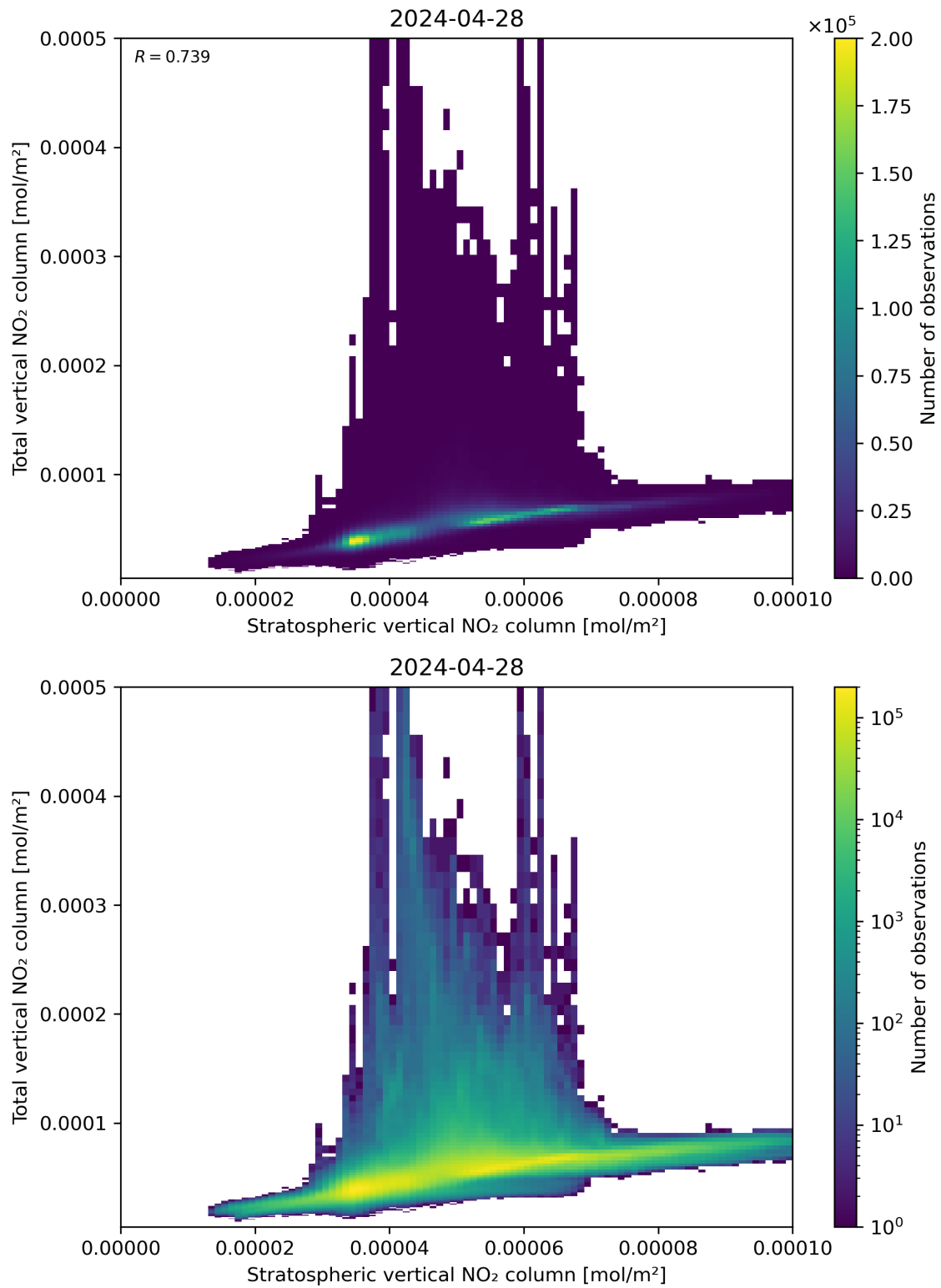
Figure 100: Scatter density plot of “Stratospheric vertical NO 2 column” against “Total vertical NO 2 column” for 2024-04-27 to 2024-04-29.
