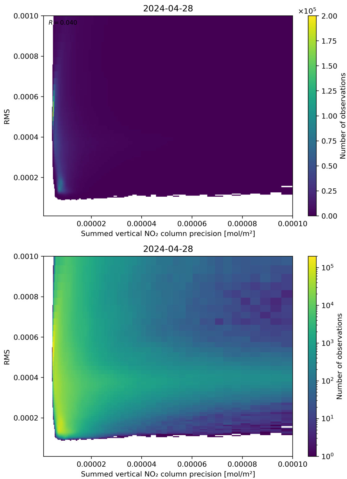
Figure 108: Scatter density plot of “Summed vertical NO 2 column precision” against “RMS” for 2024-04-27 to 2024-04-29.
