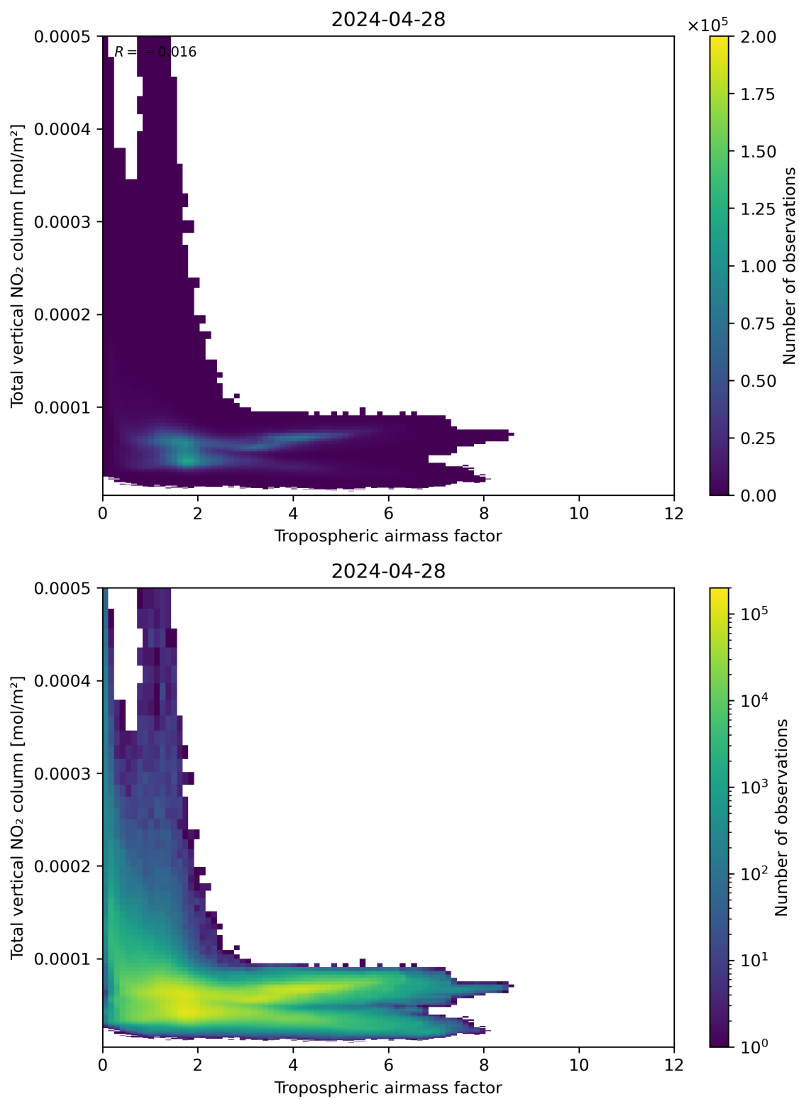
Figure 77: Scatter density plot of “Tropospheric airmass factor” against “Total vertical NO 2 column” for 2024-04-27 to 2024-04-29.
