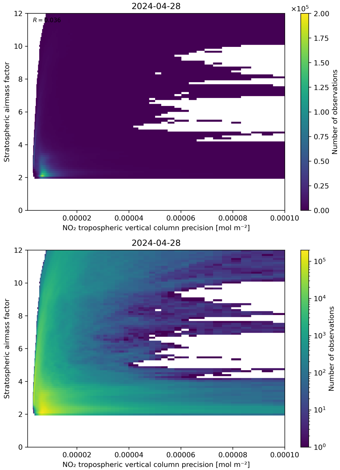
Figure 131: Scatter density plot of “NO 2 tropospheric vertical column precision” against “Stratospheric airmass factor” for 2024-04-27 to 2024-04-29.
