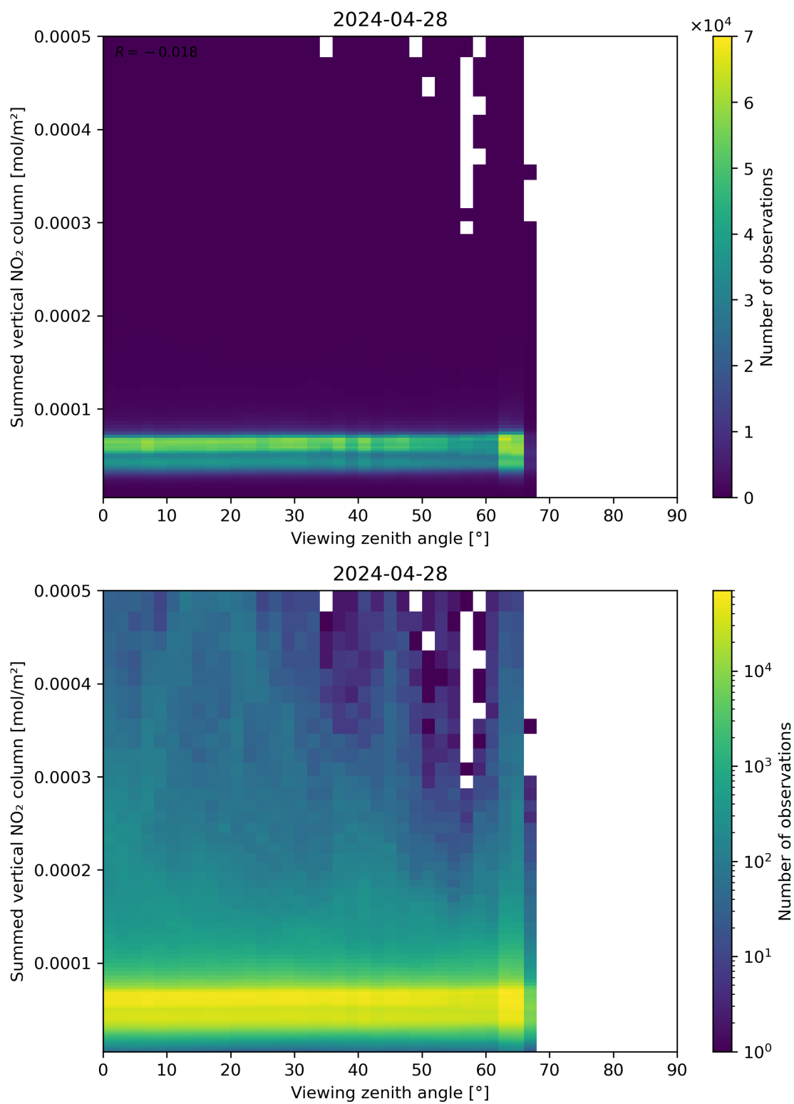
Figure 165: Scatter density plot of “Viewing zenith angle” against “Summed vertical NO 2 column” for 2024-04-27 to 2024-04-29.
