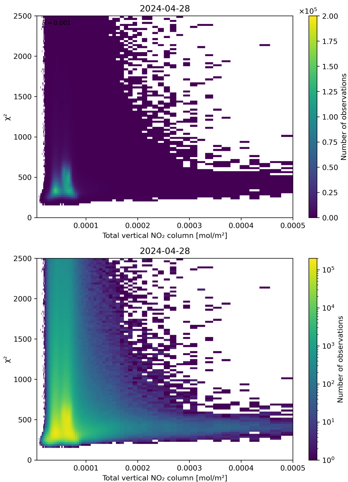
Figure 111: Scatter density plot of “Total vertical NO 2 column” against “ \chi^2 ” for 2024-04-27 to 2024-04-29.
