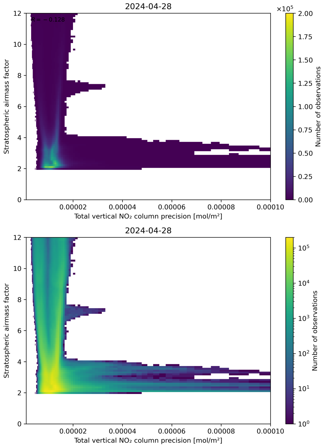
Figure 115: Scatter density plot of “Total vertical NO 2 column precision” against “Stratospheric air mass factor” for 2024-04-27 to 2024-04-29.
