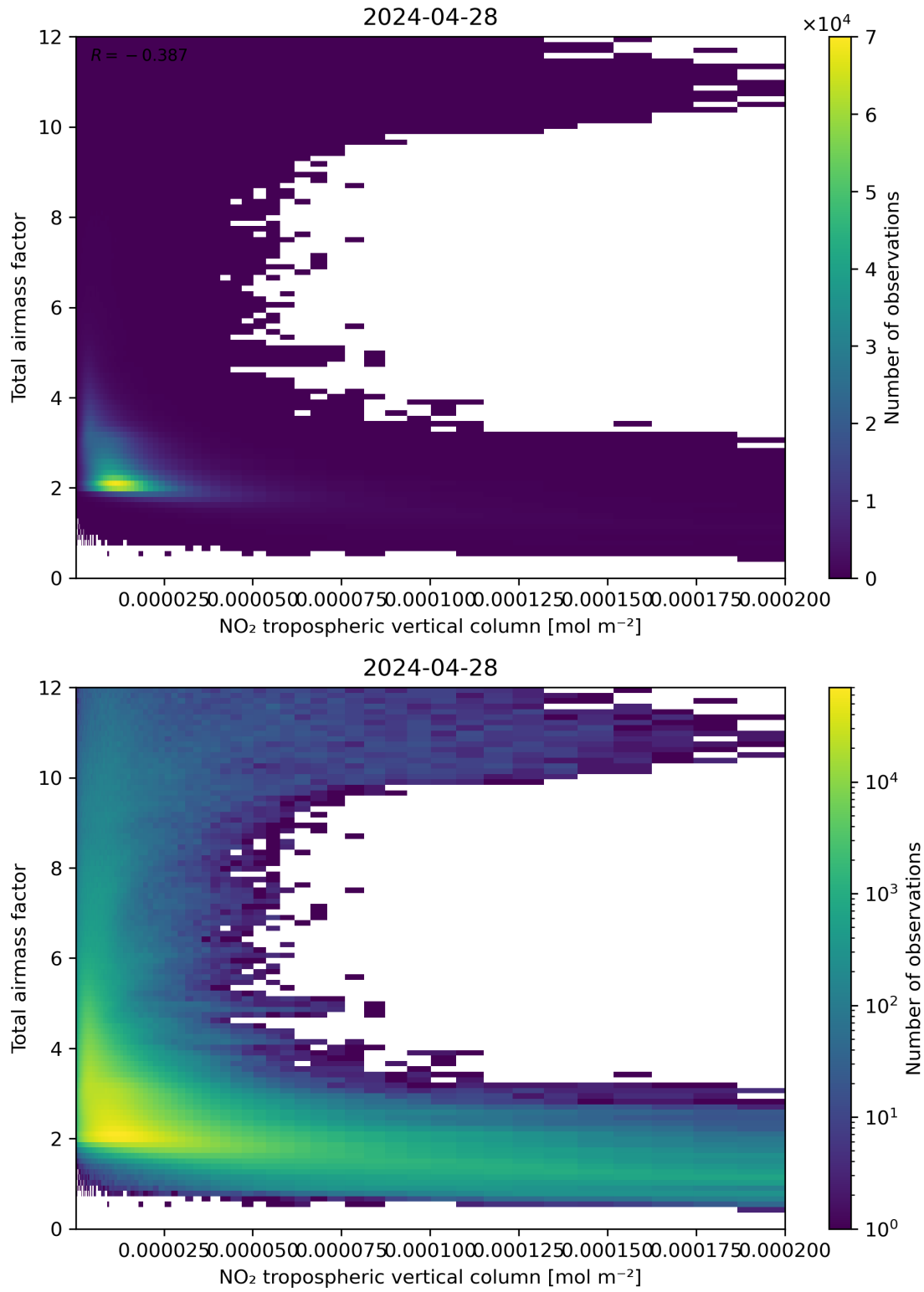
Figure 122: Scatter density plot of “NO 2 tropospheric vertical column” against “Total air mass factor” for 2024-04-27 to 2024-04-29.
