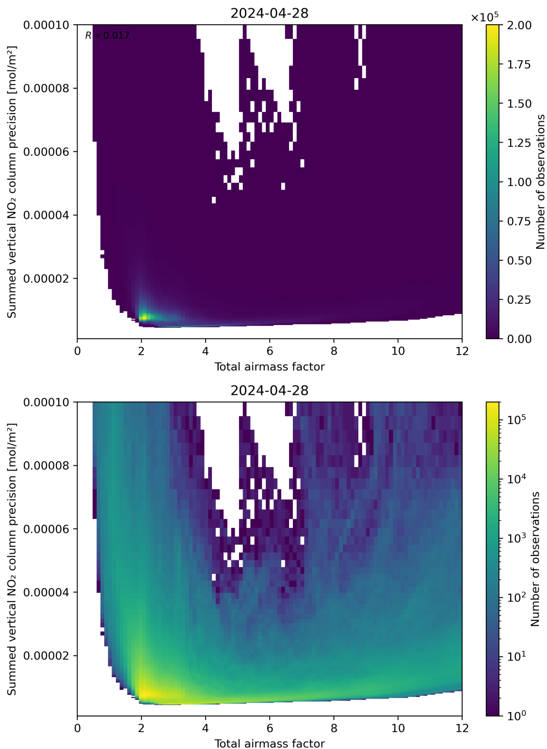
Figure 66: Scatter density plot of “Total airmass factor” against “Summed vertical NO 2 column precision” for 2024-04-27 to 2024-04-29.
