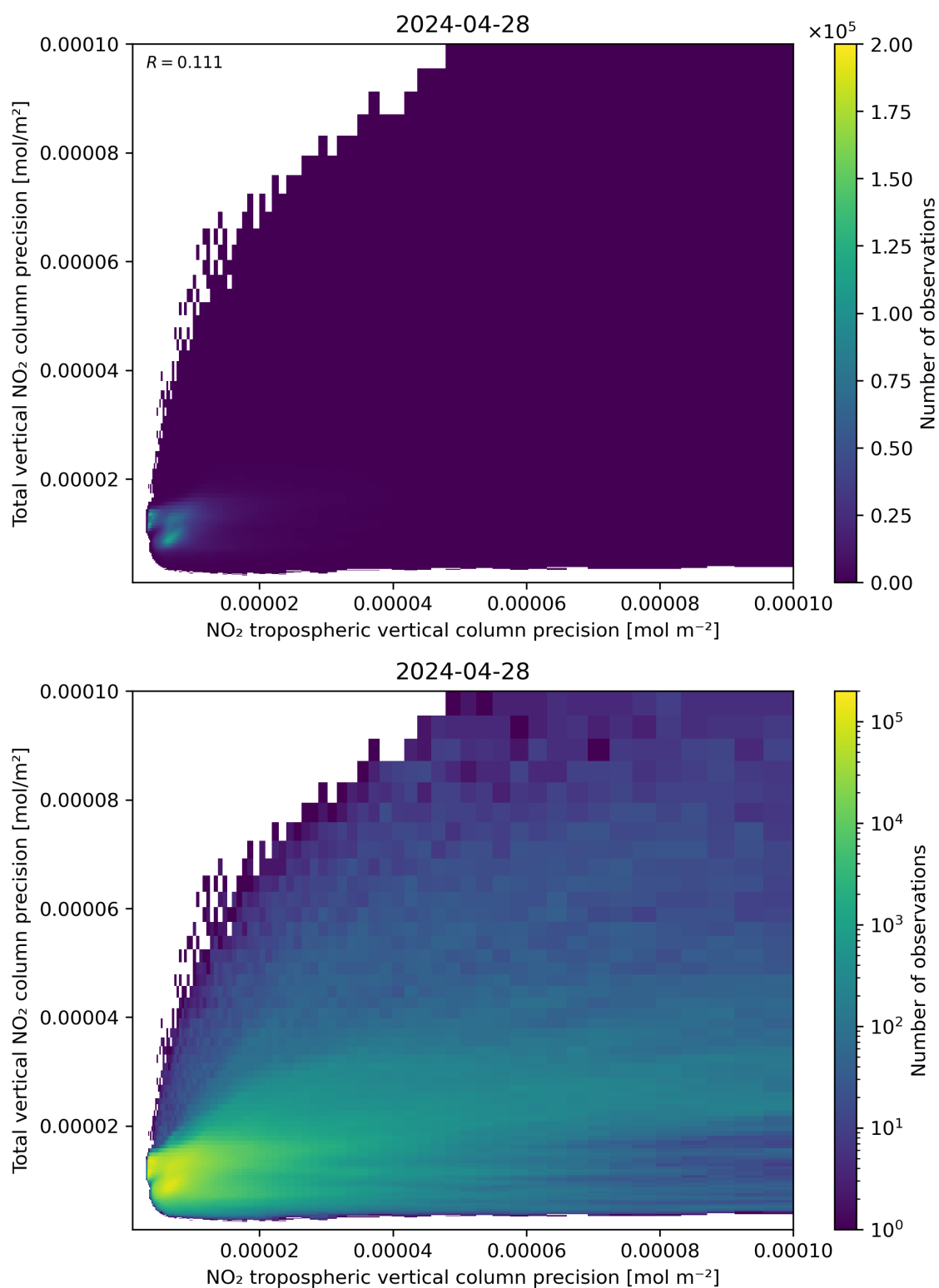
Figure 139: Scatter density plot of “NO 2 tropospheric vertical column precision” against “Total vertical NO 2 column precision” for 2024-04-27 to 2024-04-29.
