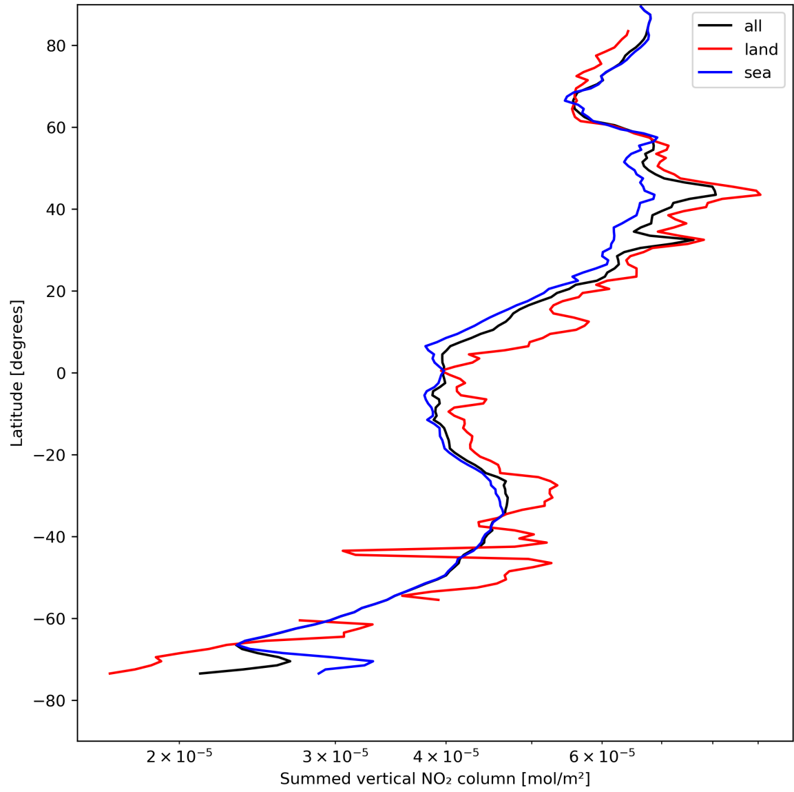
Figure 23: Zonal average of “Summed vertical NO 2 column” for 2024-04-27 to 2024-04-29.
