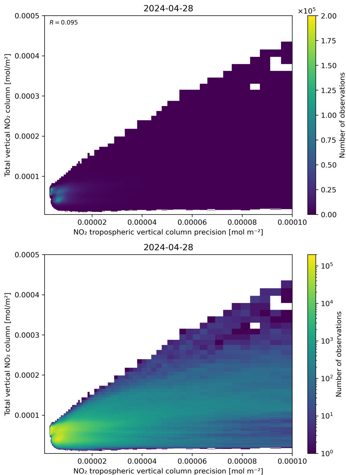
Figure 138: Scatter density plot of “NO 2 tropospheric vertical column precision” against “Total vertical NO 2 column” for 2024-04-27 to 2024-04-29.
