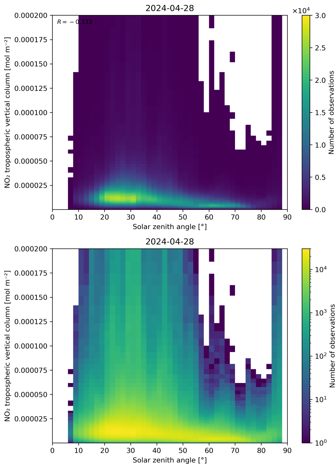
Figure 155: Scatter density plot of “Solar zenith angle” against “NO 2 tropospheric vertical column” for 2024-04-27 to 2024-04-29.
