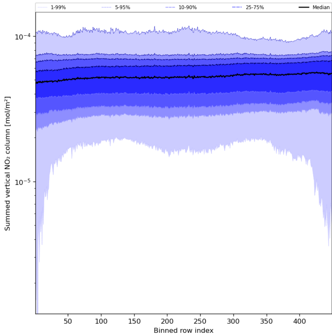
Figure 57: Along track statistics of “Summed vertical NO 2 column” for 2024-04-27 to 2024-04-29
