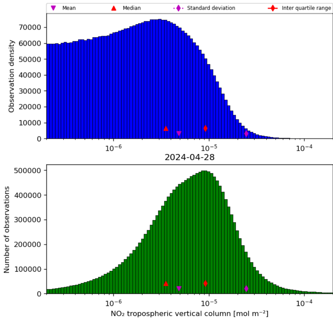
Figure 29: Histogram of “NO 2 tropospheric vertical column” for 2024-04-27 to 2024-04-29
