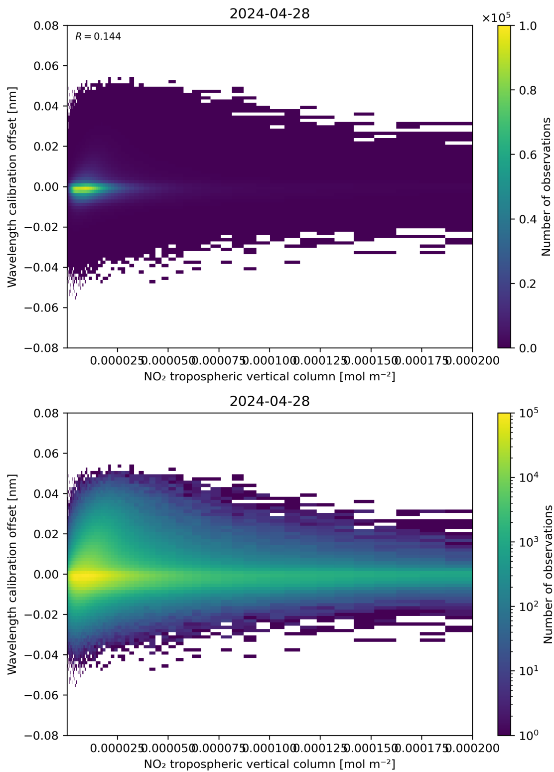
Figure 143: Scatter density plot of “NO 2 tropospheric vertical column” against “Wavelength calibration offset” for 2024-04-27 to 2024-04-29.
