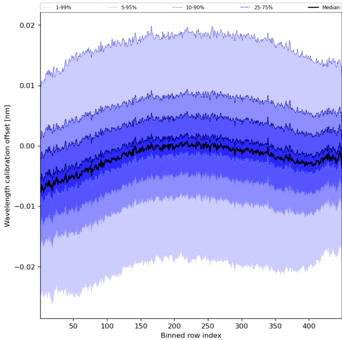
Figure 52: Along track statistics of “Wavelength calibration offset” for 2024-04-27 to 2024-04-29
