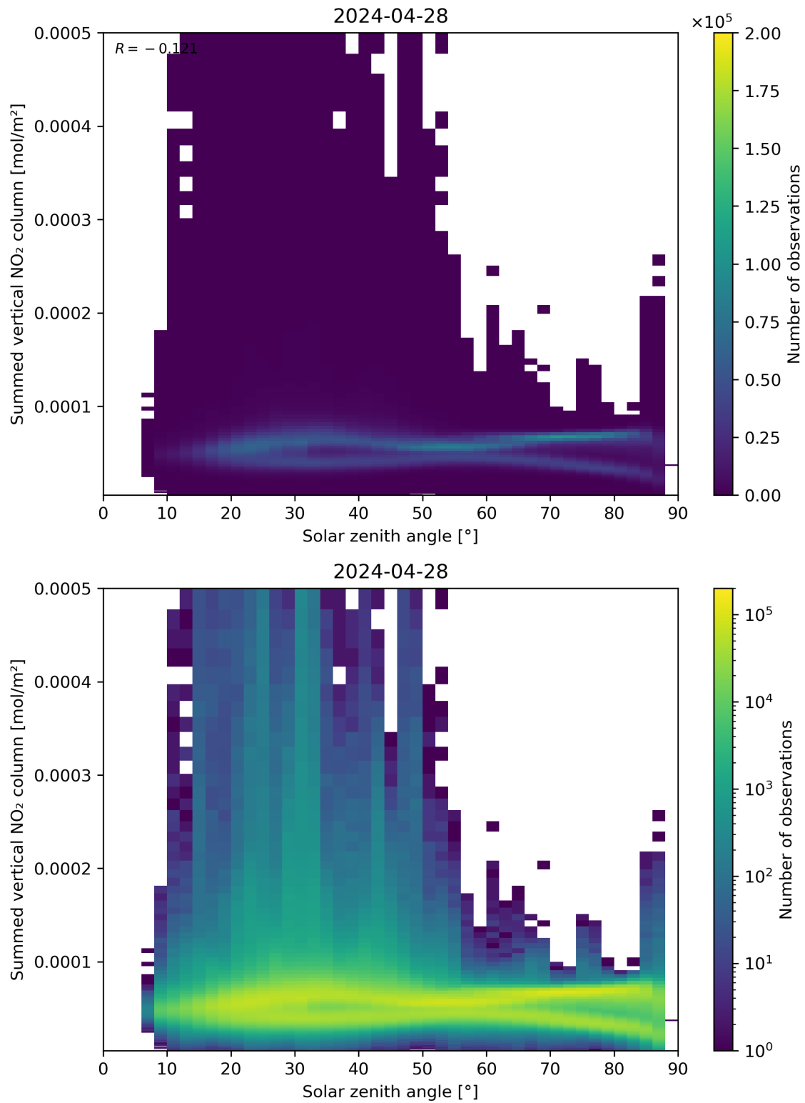
Figure 151: Scatter density plot of “Solar zenith angle” against “Summed vertical NO 2 column” for 2024-04-27 to 2024-04-29.
