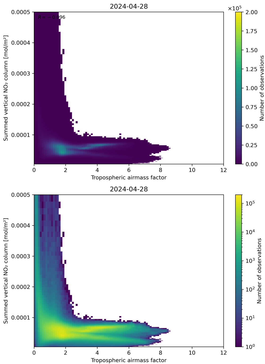
Figure 75: Scatter density plot of “Tropospheric air mass factor” against “Summed vertical NO 2 column” for 2024-04-27 to 2024-04-29.
