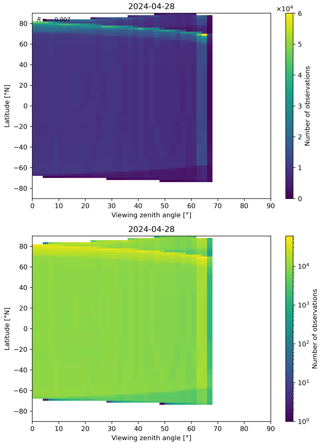
Figure 163: Scatter density plot of “Viewing zenith angle” against “Latitude” for 2024-04-27 to 2024-04-29.
