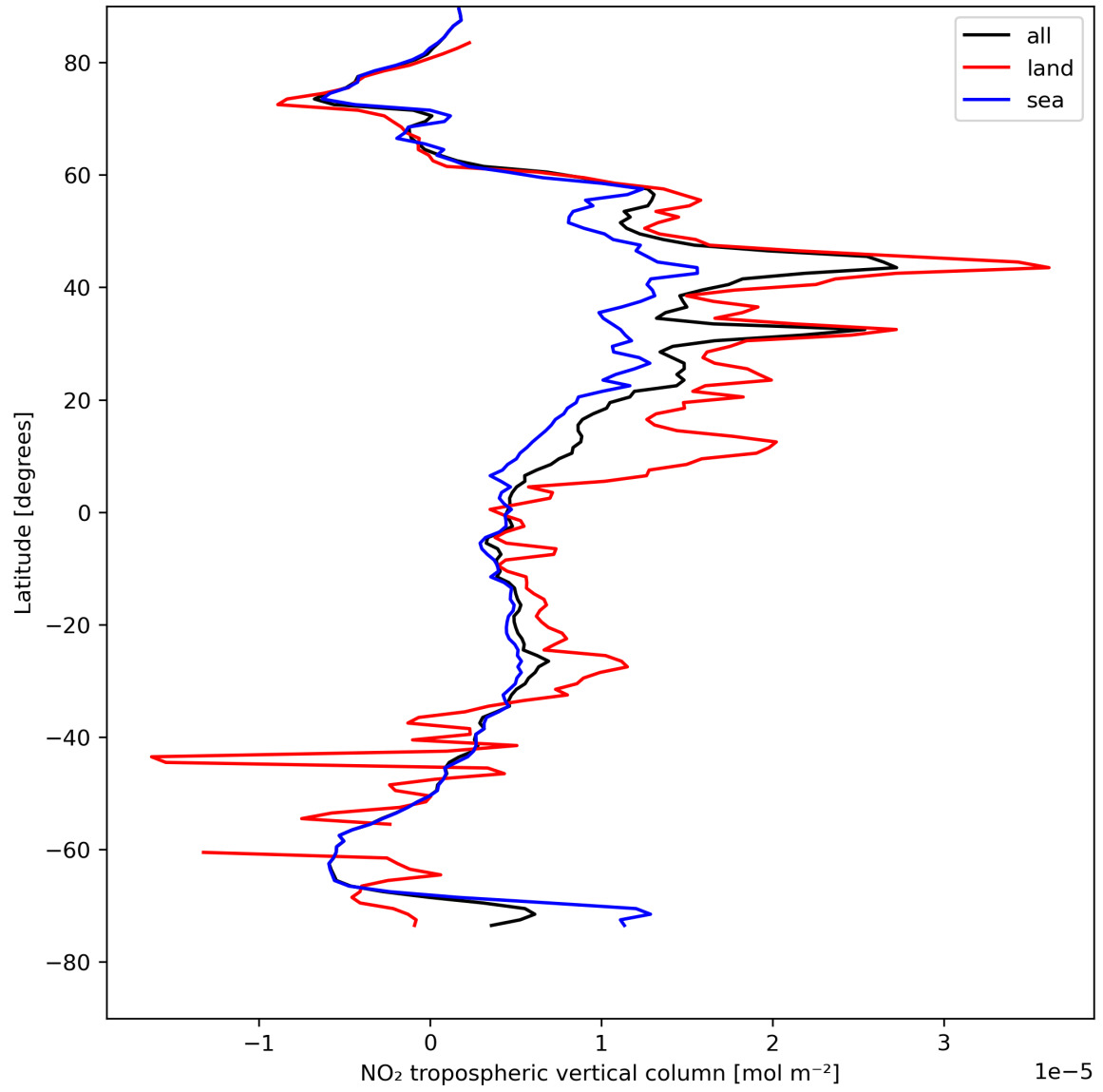
Figure 12: Zonal average of “NO 2 tropospheric vertical column” for 2024-04-27 to 2024-04-29.
