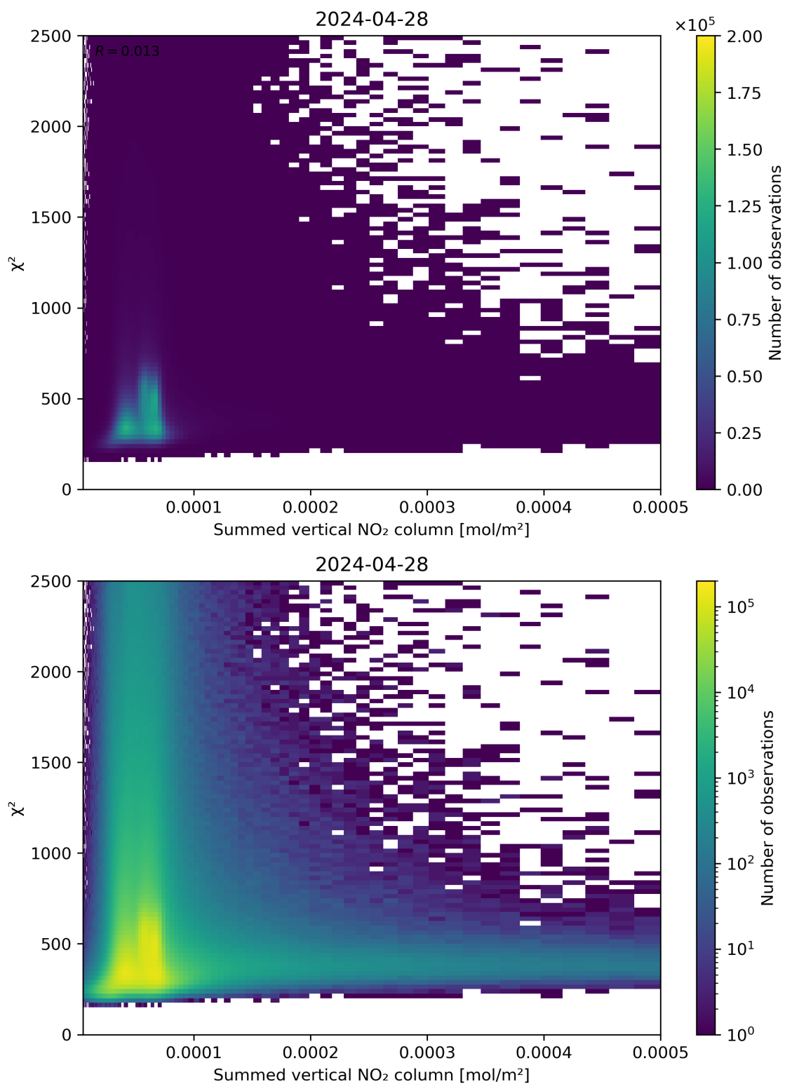
Figure 104: Scatter density plot of “Summed vertical NO 2 column” against “ \chi^2 ” for 2024-04-27 to 2024-04-29.
