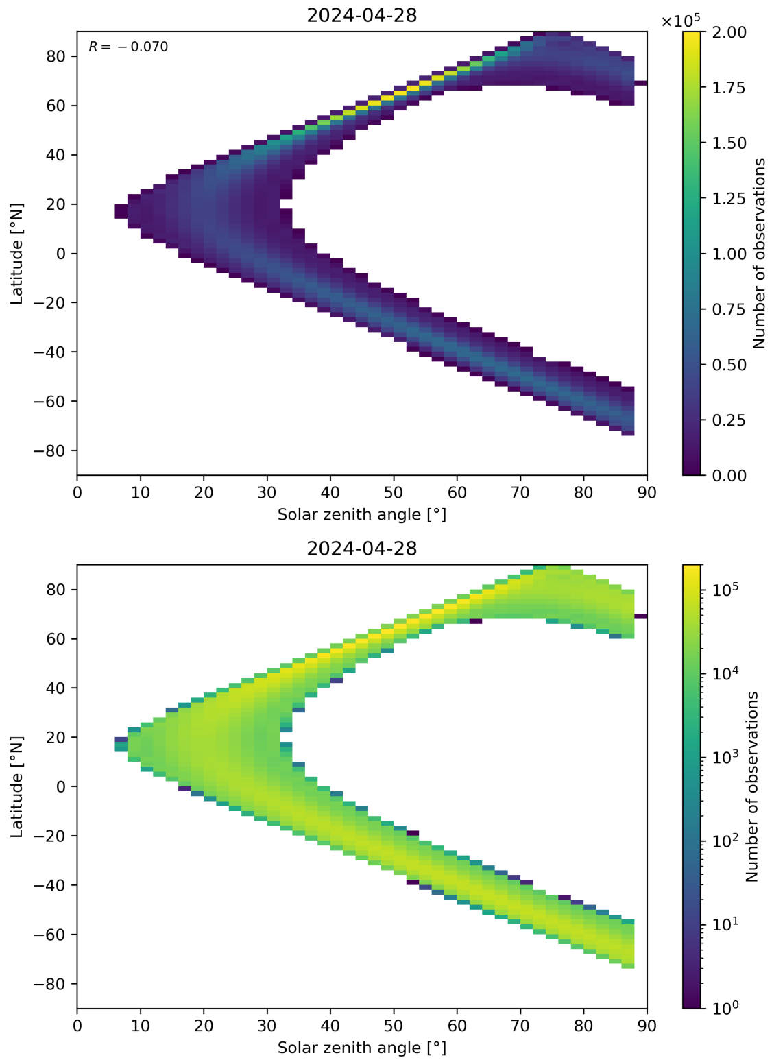
Figure 149: Scatter density plot of “Solar zenith angle” against “Latitude” for 2024-04-27 to 2024-04-29.
