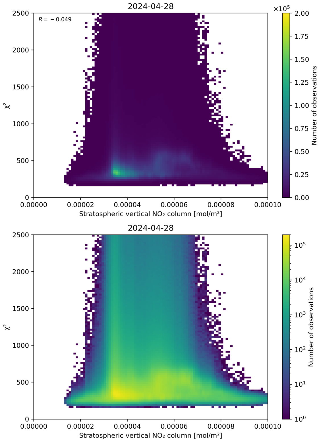
Figure 97: Scatter density plot of “Stratospheric vertical NO 2 column” against “ \chi^2 ” for 2024-04-27 to 2024-04-29.
