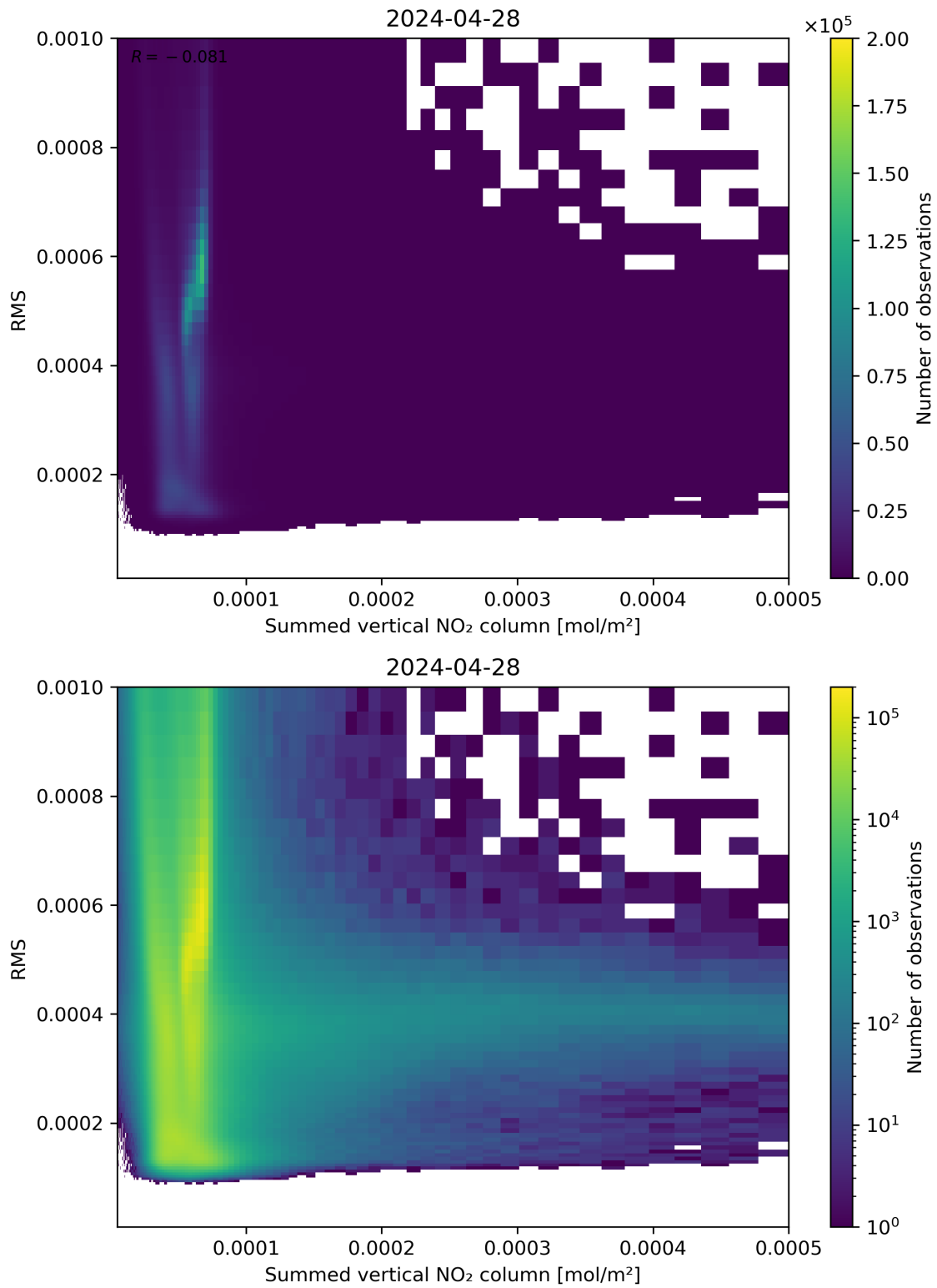
Figure 109: Scatter density plot of “Summed vertical NO 2 column” against “RMS” for 2024-04-27 to 2024-04-29.
