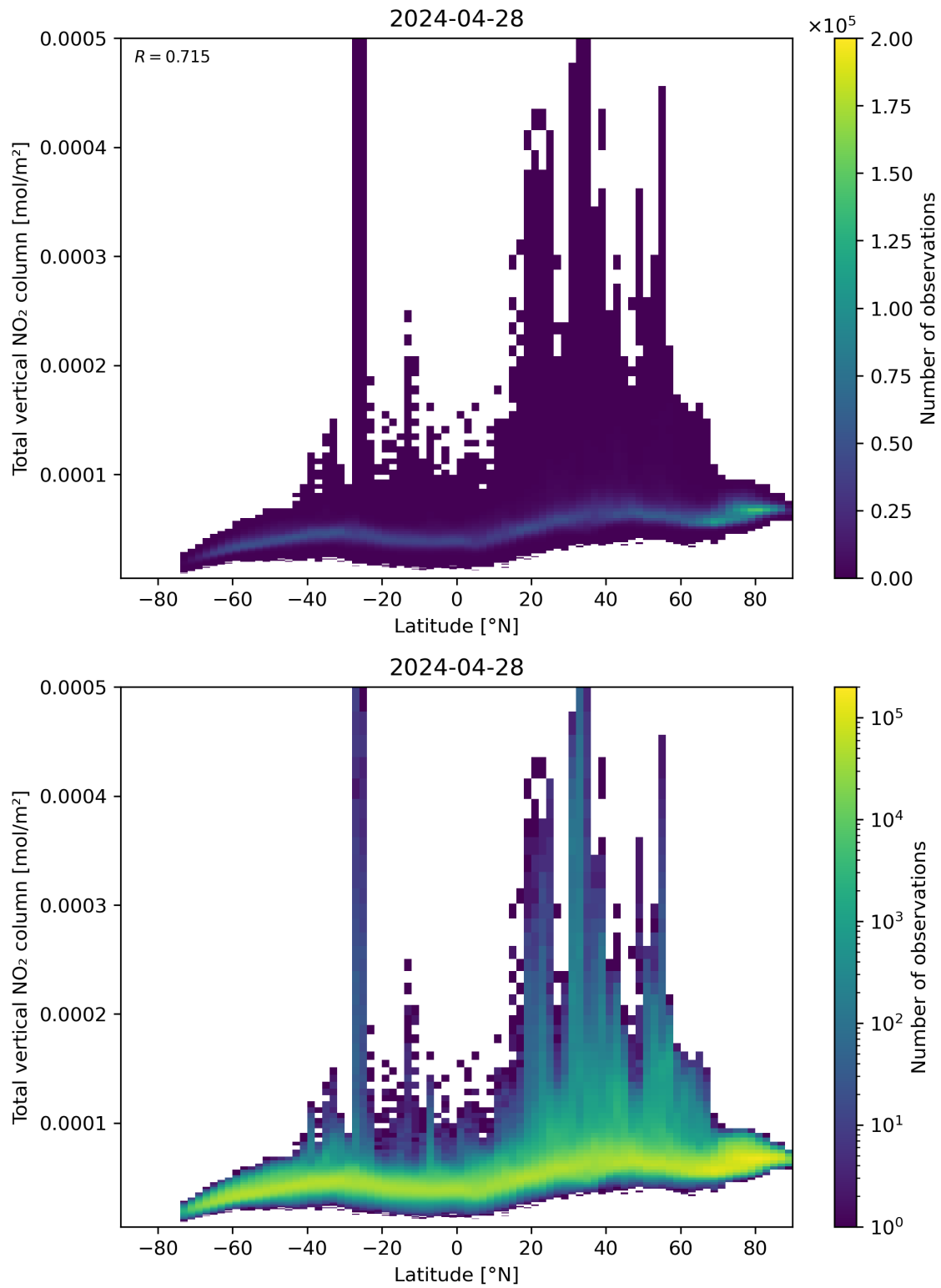
Figure 90: Scatter density plot of “Latitude” against “Total vertical NO 2 column” for 2024-04-27 to 2024-04-29.
