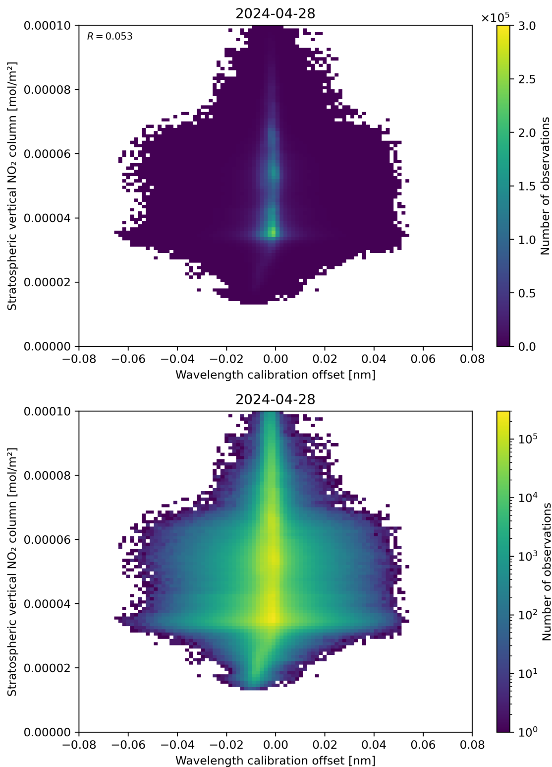
Figure 176: Scatter density plot of “Wavelength calibration offset” against “Stratospheric vertical NO 2 column” for 2024-04-27 to 2024-04-29.
