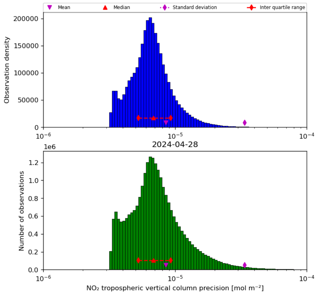
Figure 30: Histogram of “NO 2 tropospheric vertical column precision” for 2024-04-27 to 2024-04-29
