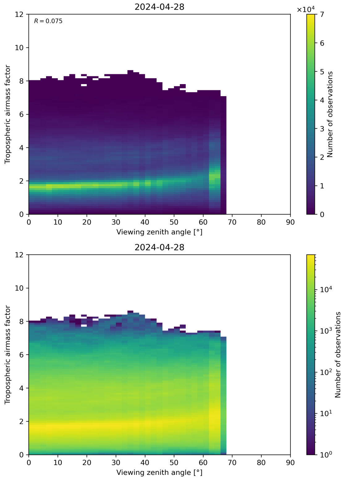
Figure 161: Scatter density plot of “Viewing zenith angle” against “Tropospheric airmass factor” for 2024-04-27 to 2024-04-29.
