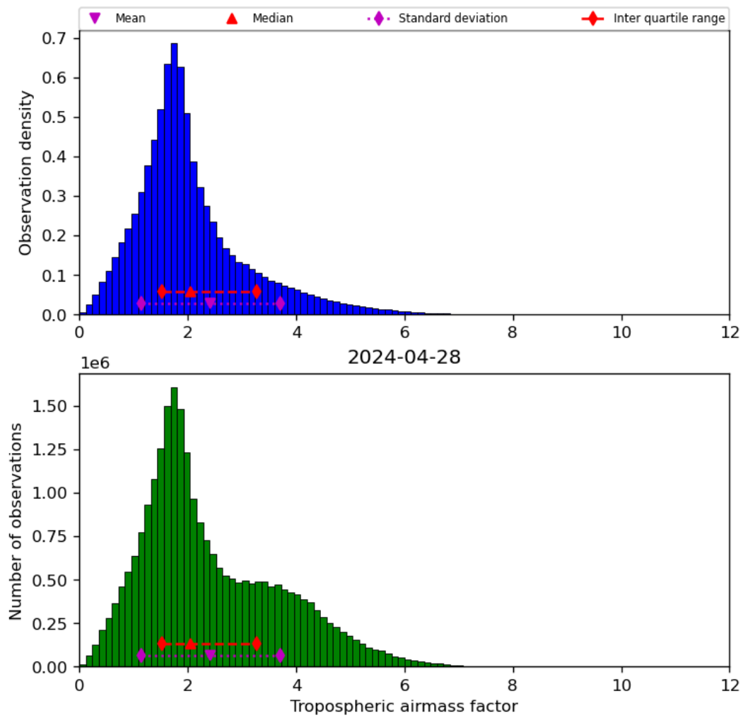
Figure 31: Histogram of “Tropospheric airmass factor” for 2024-04-27 to 2024-04-29
