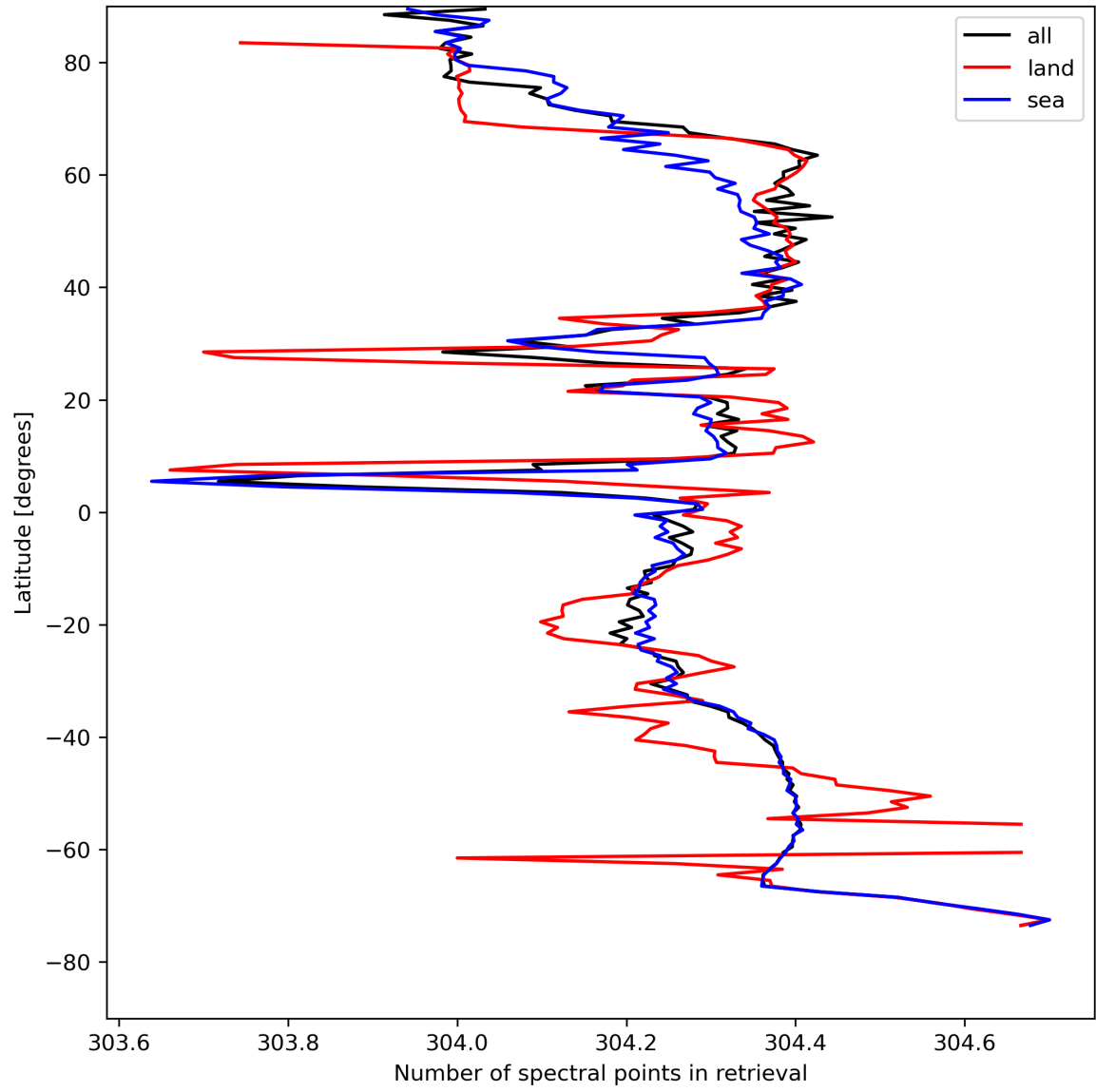
Figure 16: Zonal average of “Number of spectral points in retrieval” for 2024-04-27 to 2024-04-29.
