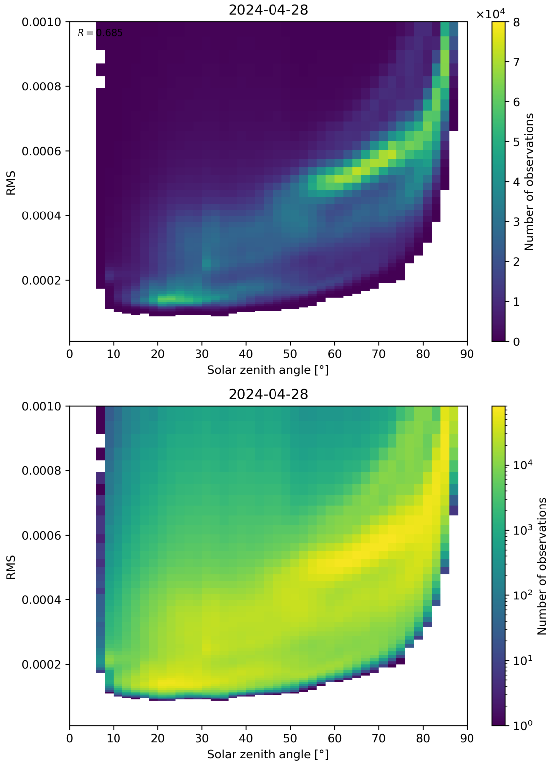
Figure 157: Scatter density plot of “Solar zenith angle” against “RMS” for 2024-04-27 to 2024-04-29.
