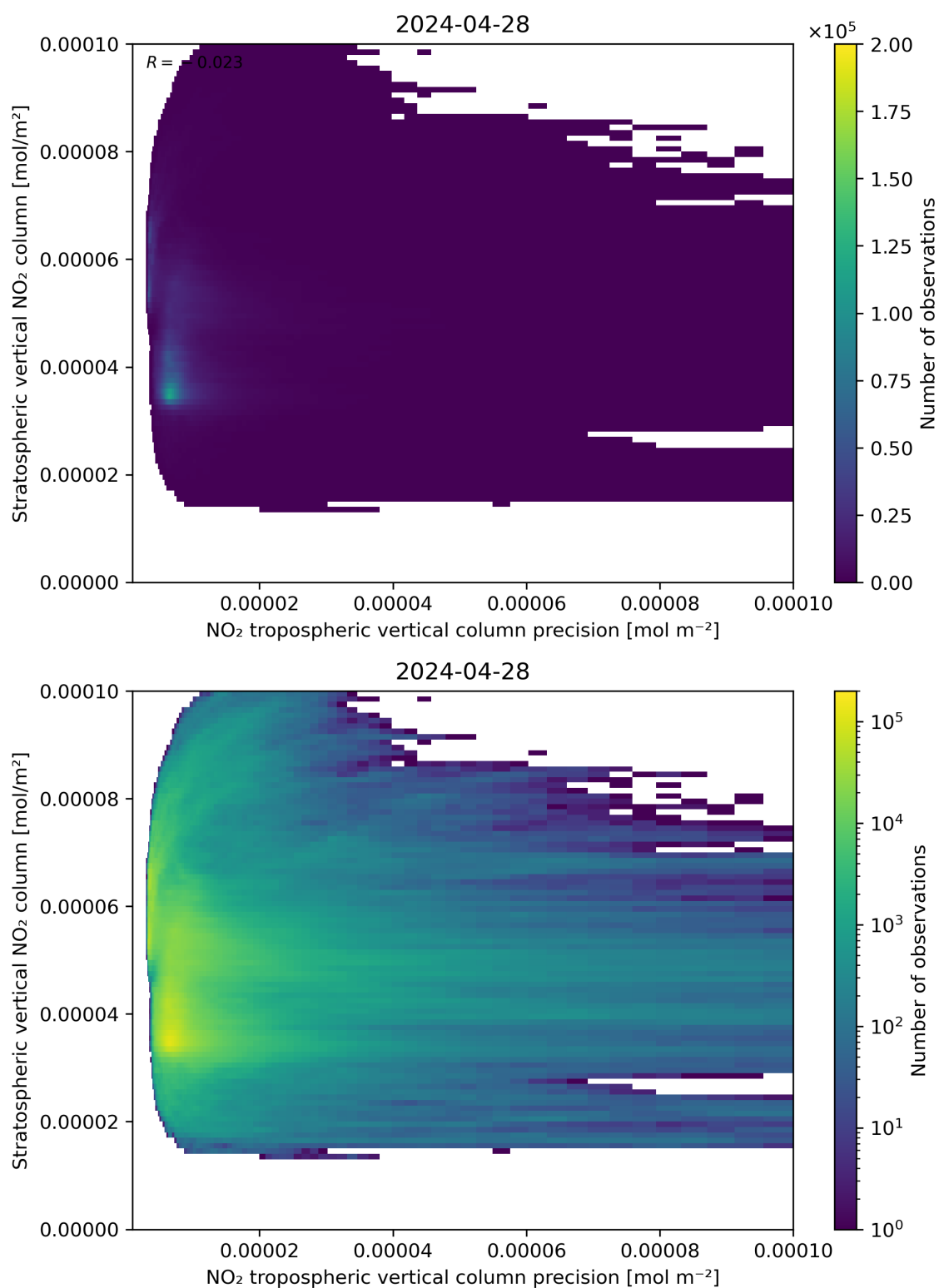
Figure 135: Scatter density plot of “NO 2 tropospheric vertical column precision” against “Stratospheric vertical NO 2 column” for 2024-04-27 to 2024-04-29.
