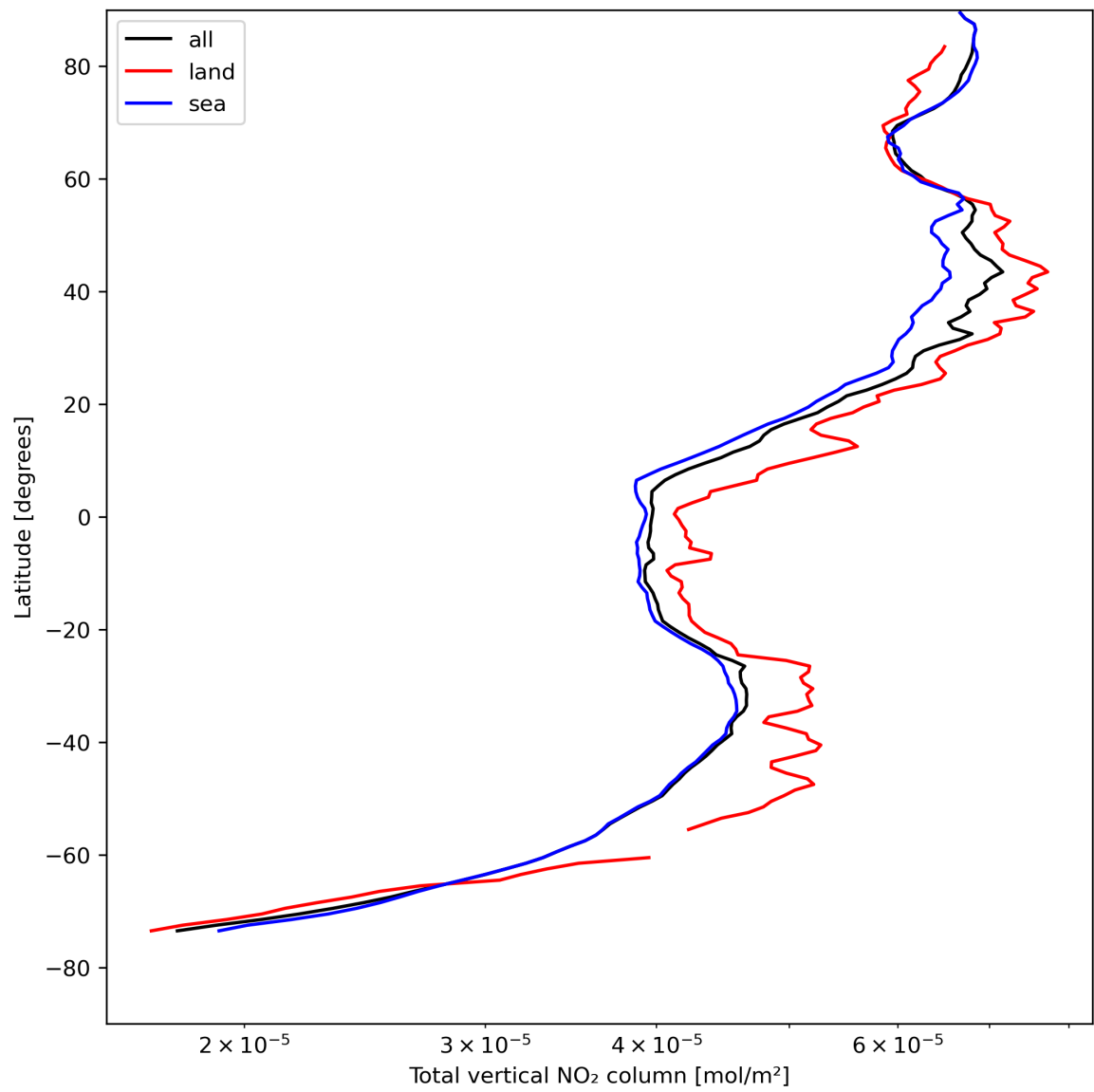
Figure 21: Zonal average of “Total vertical NO 2 column” for 2024-04-27 to 2024-04-29.
