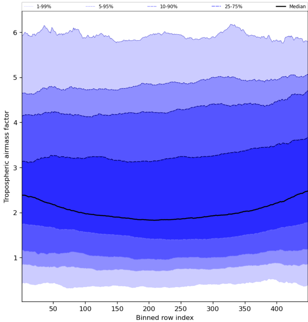
Figure 48: Along track statistics of “Tropospheric airmass factor” for 2024-04-27 to 2024-04-29
