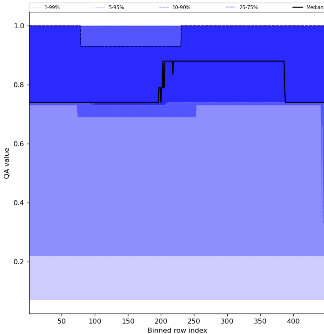
Figure 45: Along track statistics of “QA value” for 2024-04-27 to 2024-04-29
