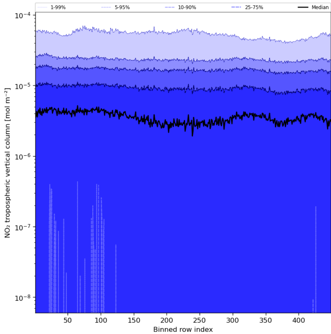
Figure 46: Along track statistics of “NO 2 tropospheric vertical column” for 2024-04-27 to 2024-04-29
