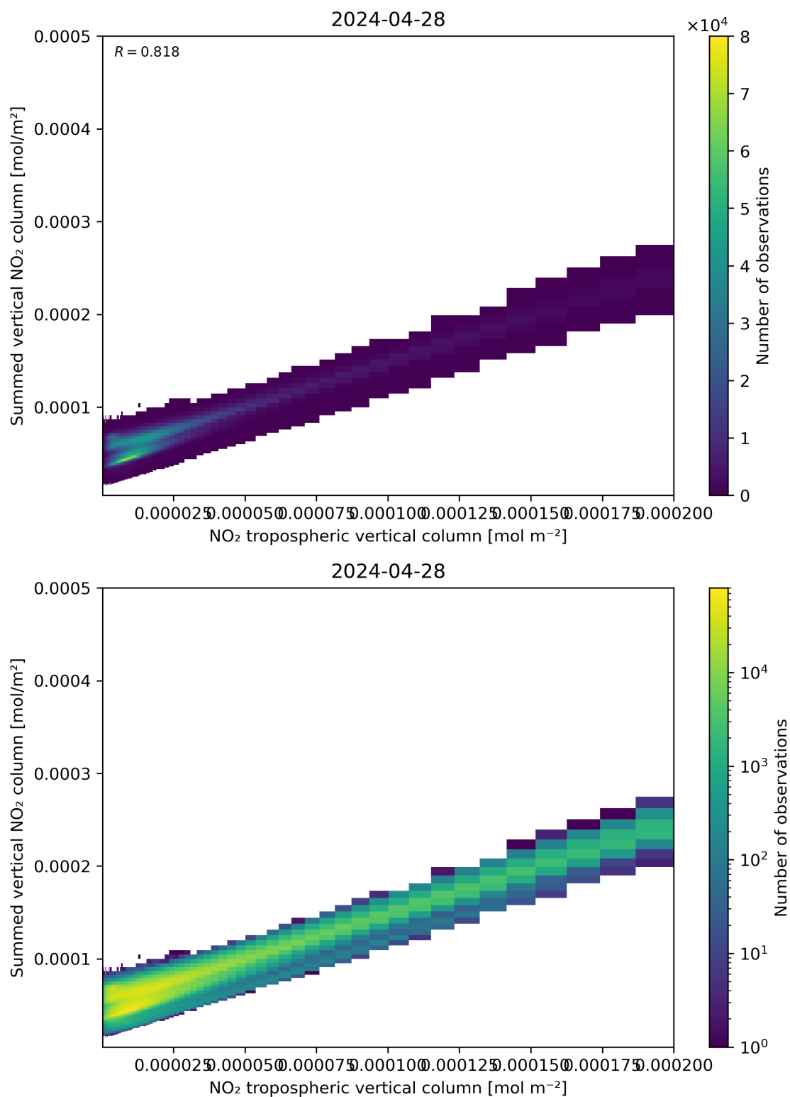
Figure 126: Scatter density plot of “NO 2 tropospheric vertical column” against “Summed vertical NO 2 column” for 2024-04-27 to 2024-04-29.
