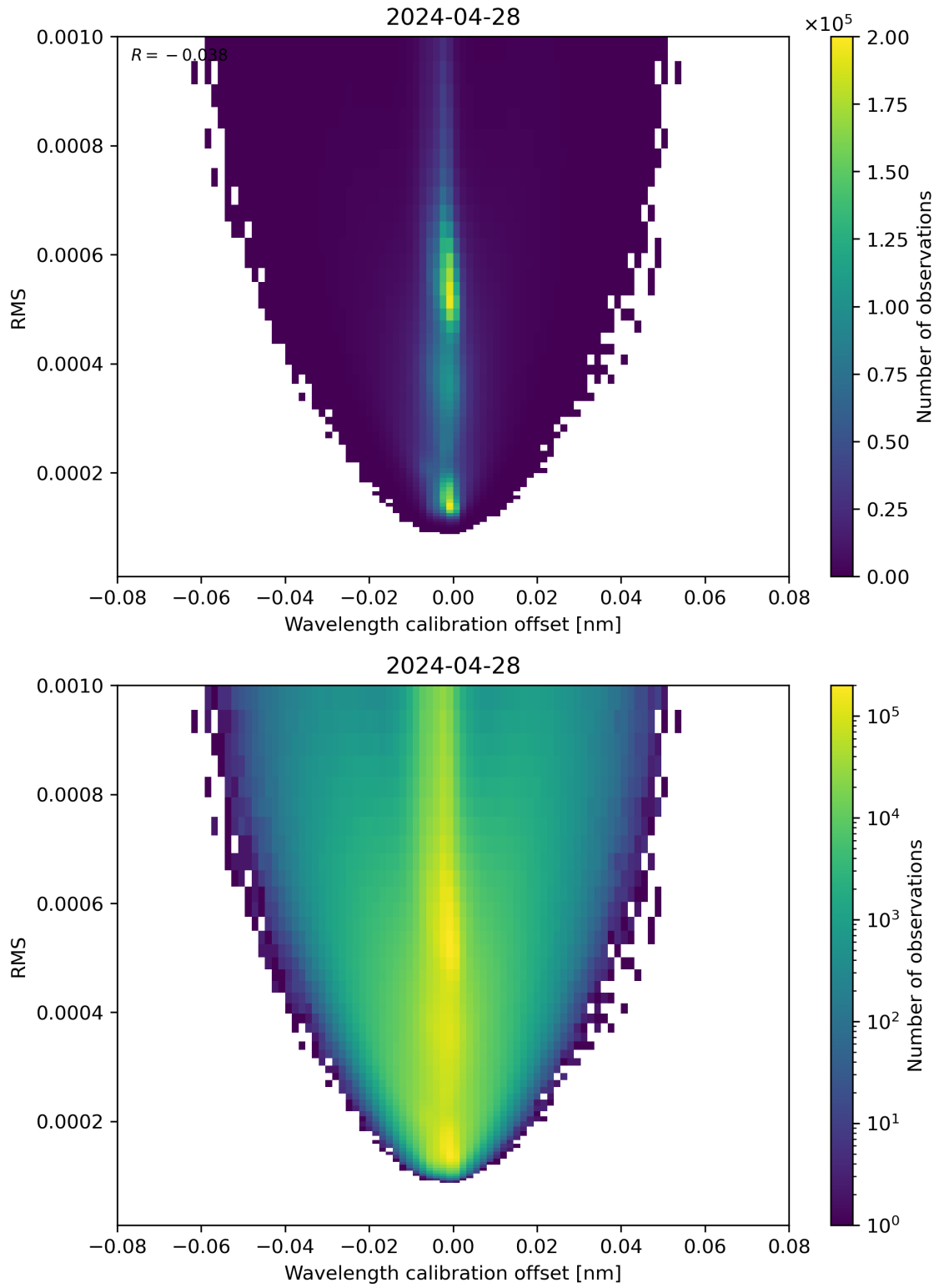
Figure 181: Scatter density plot of “Wavelength calibration offset” against “RMS” for 2024-04-27 to 2024-04-29.
