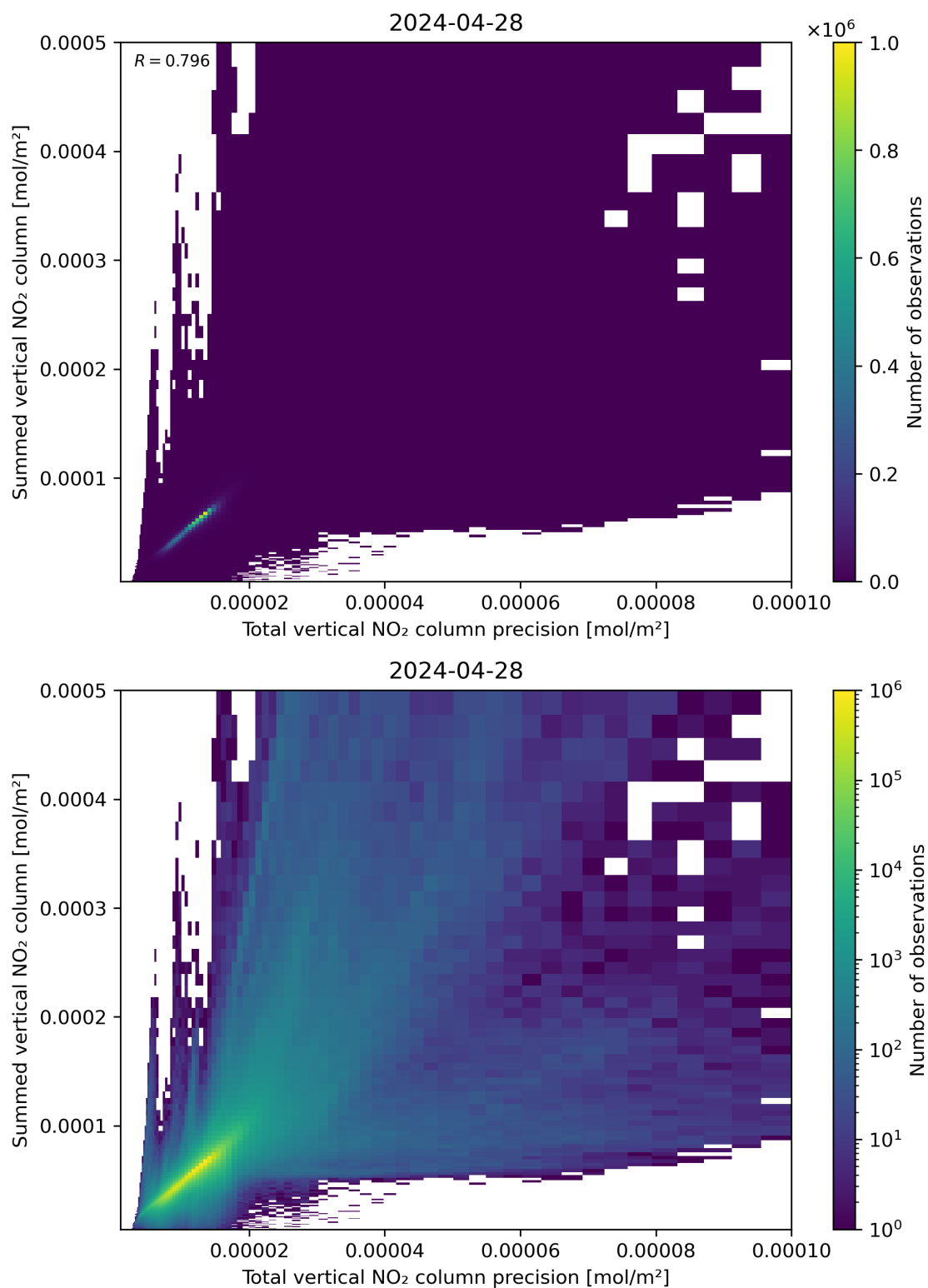
Figure 117: Scatter density plot of “Total vertical NO 2 column precision” against “Summed vertical NO 2 column” for 2024-04-27 to 2024-04-29.
