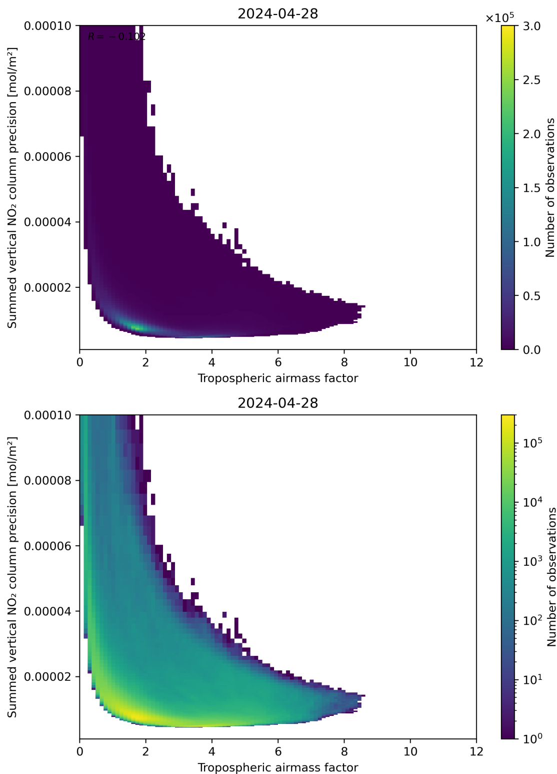
Figure 76: Scatter density plot of “Tropospheric air mass factor” against “Summed vertical NO 2 column precision” for 2024-04-27 to 2024-04-29.
