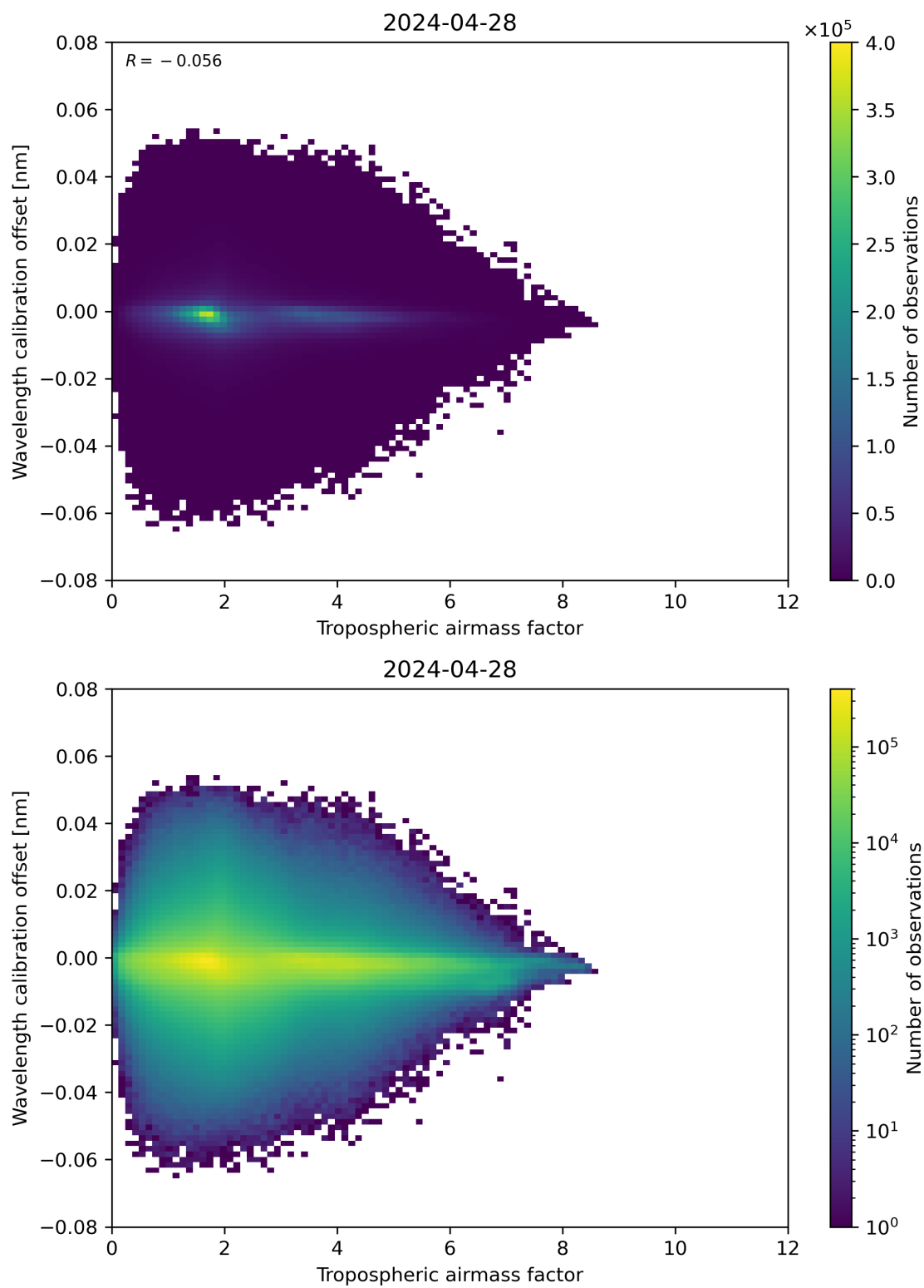
Figure 80: Scatter density plot of “Tropospheric airmass factor” against “Wavelength calibration offset” for 2024-04-27 to 2024-04-29.
