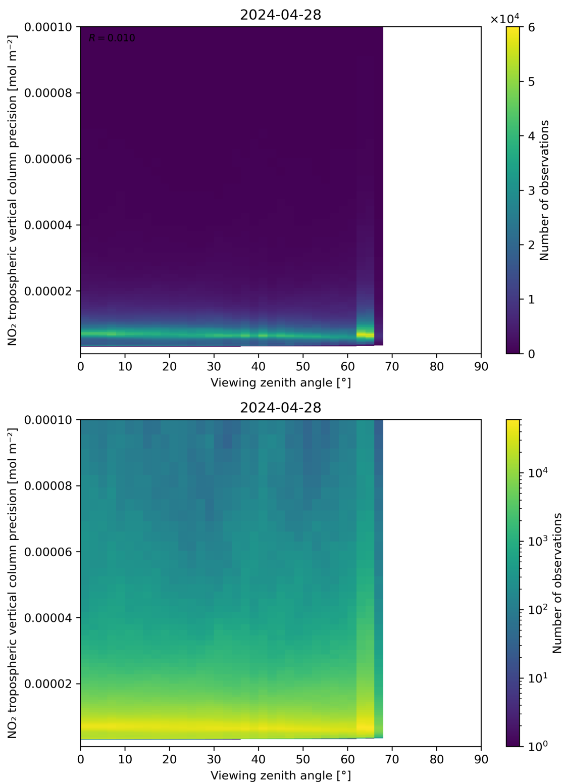
Figure 170: Scatter density plot of “Viewing zenith angle” against “NO 2 tropospheric vertical column precision” for 2024-04-27 to 2024-04-29.
