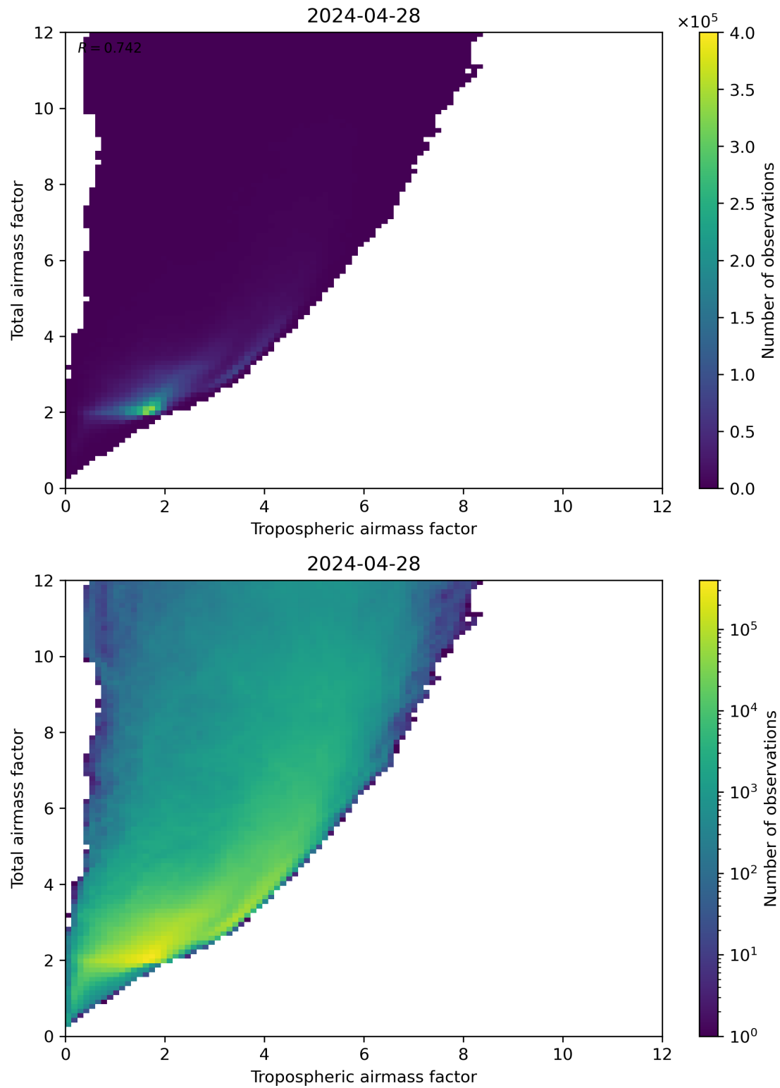
Figure 72: Scatter density plot of “Tropospheric airmass factor” against “Total airmass factor” for 2024-04-27 to 2024-04-29.
