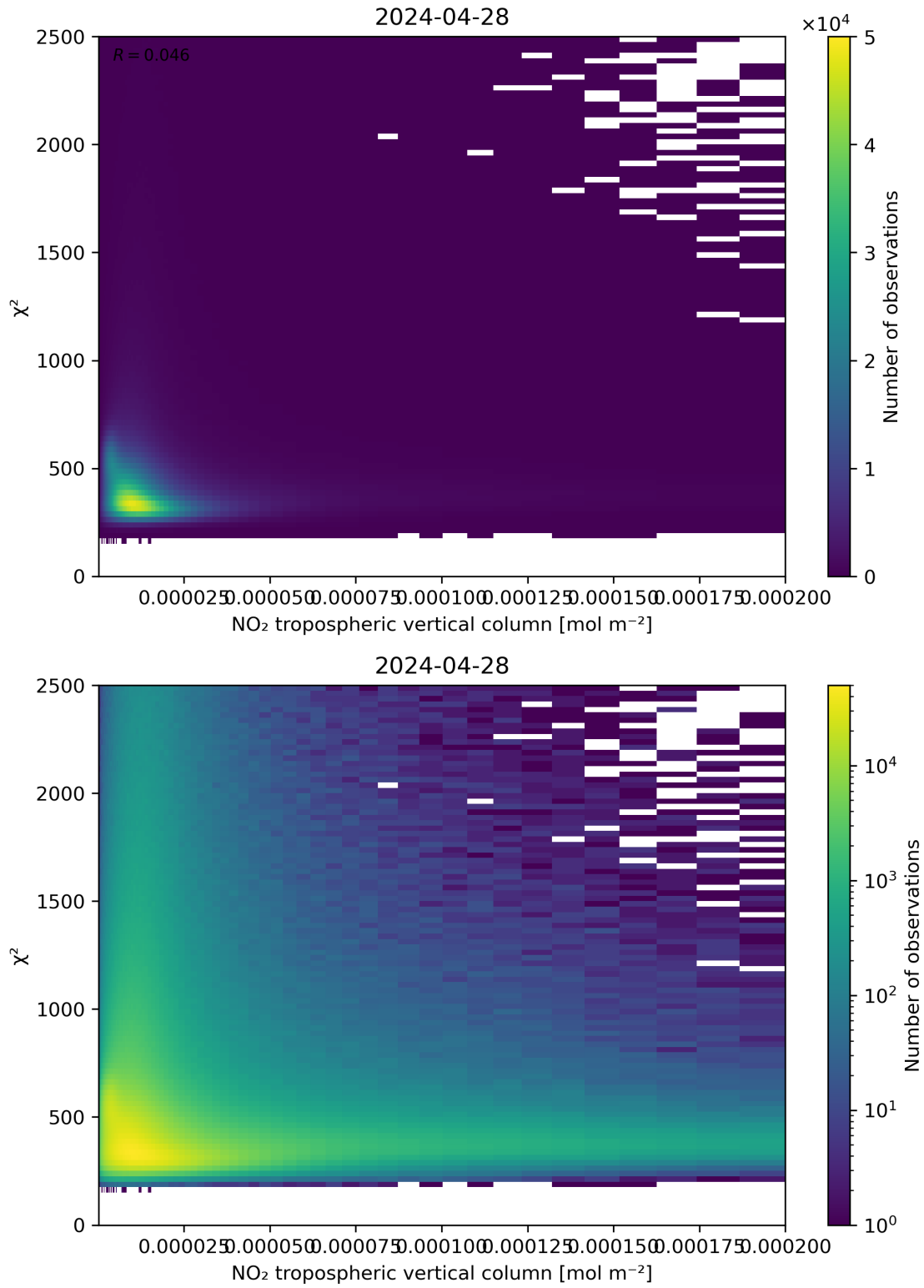
Figure 124: Scatter density plot of “NO 2 tropospheric vertical column” against “ \chi^2 ” for 2024-04-27 to 2024-04-29.
