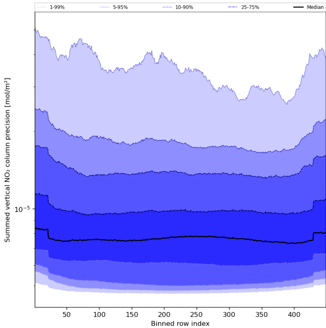
Figure 58: Along track statistics of “Summed vertical NO 2 column precision” for 2024-04-27 to 2024-04-29
