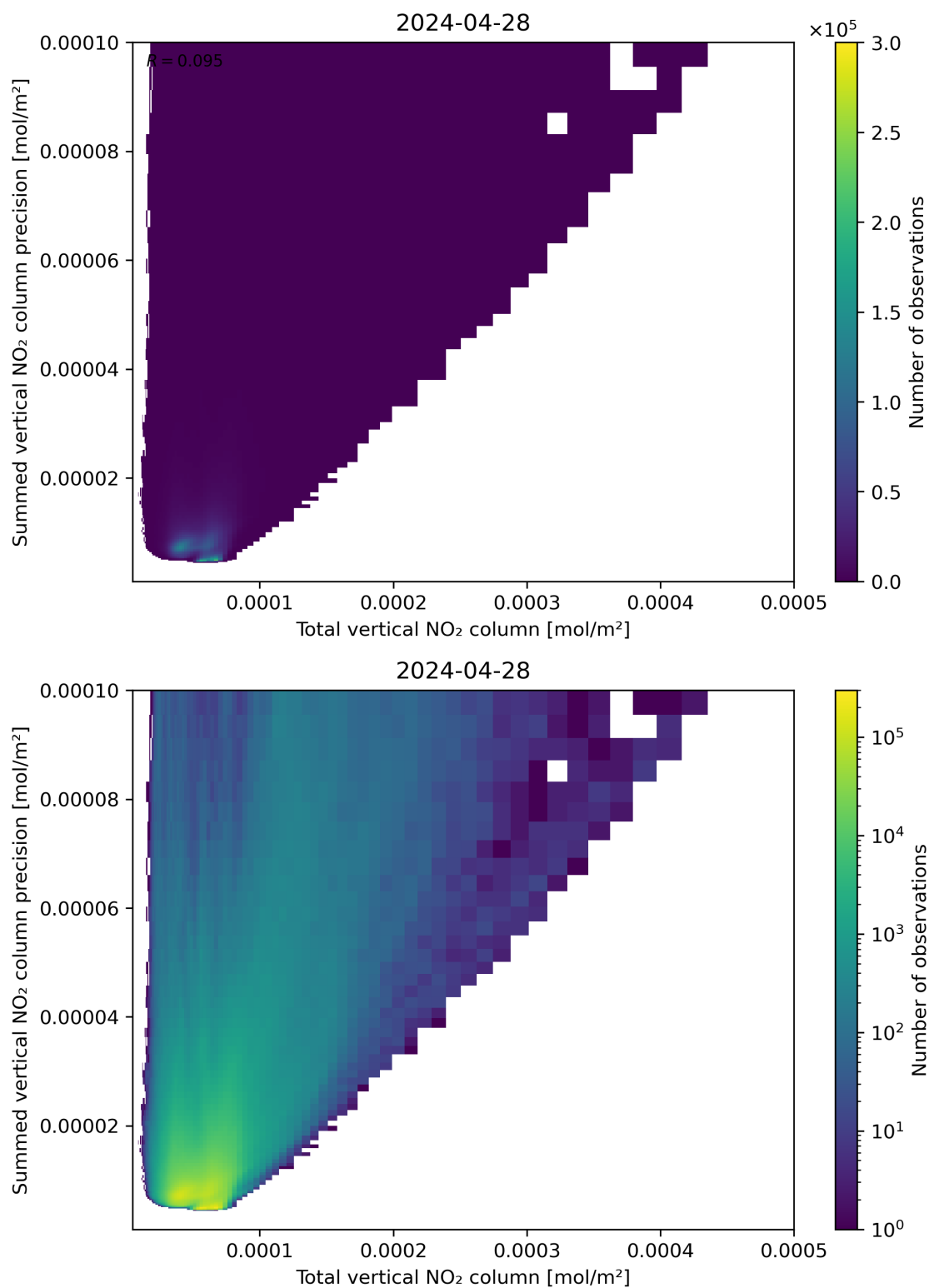
Figure 113: Scatter density plot of “Total vertical NO 2 column” against “Summed vertical NO 2 column precision” for 2024-04-27 to 2024-04-29.
