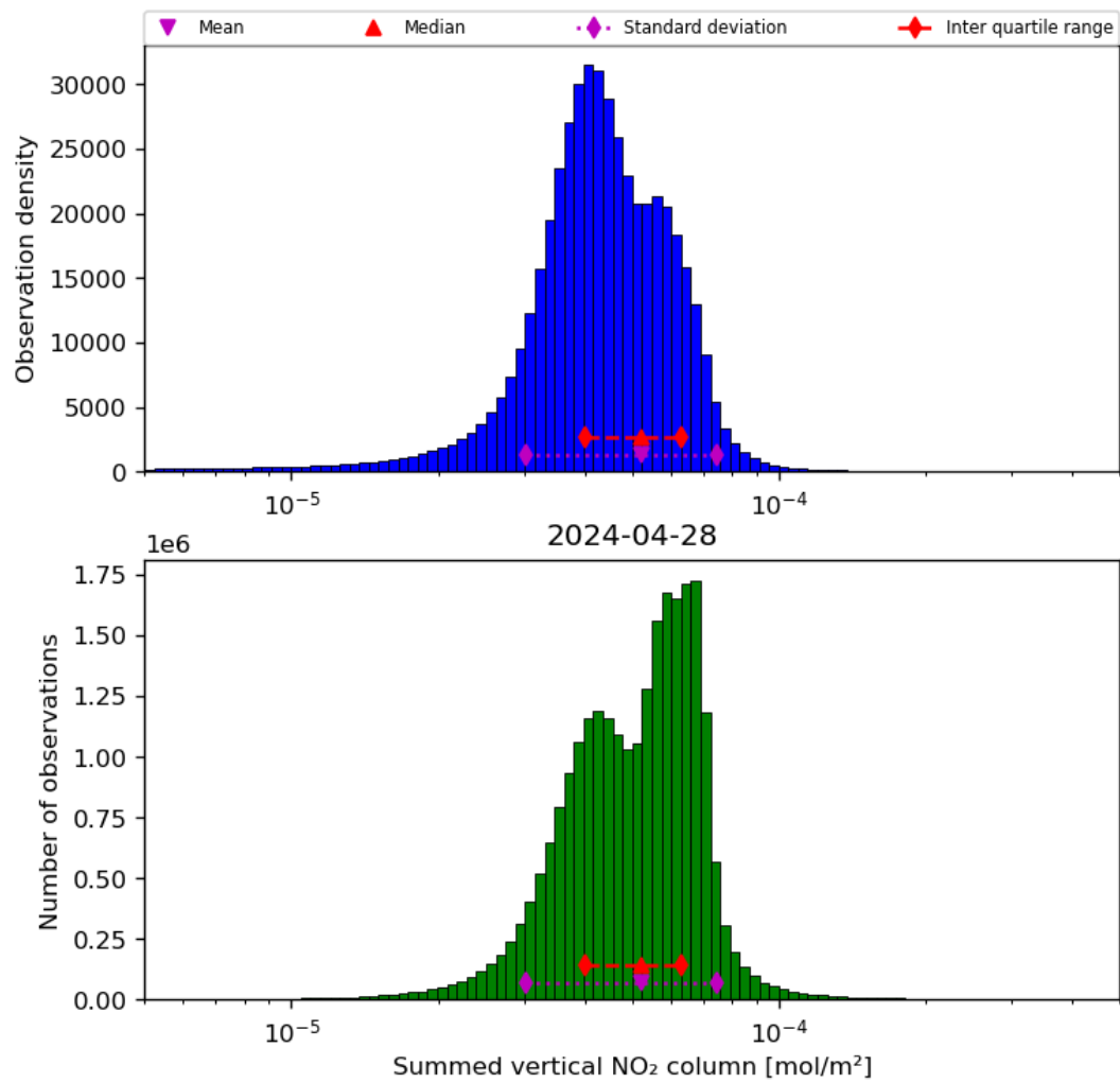
Figure 40: Histogram of “Summed vertical NO 2 column” for 2024-04-27 to 2024-04-29
