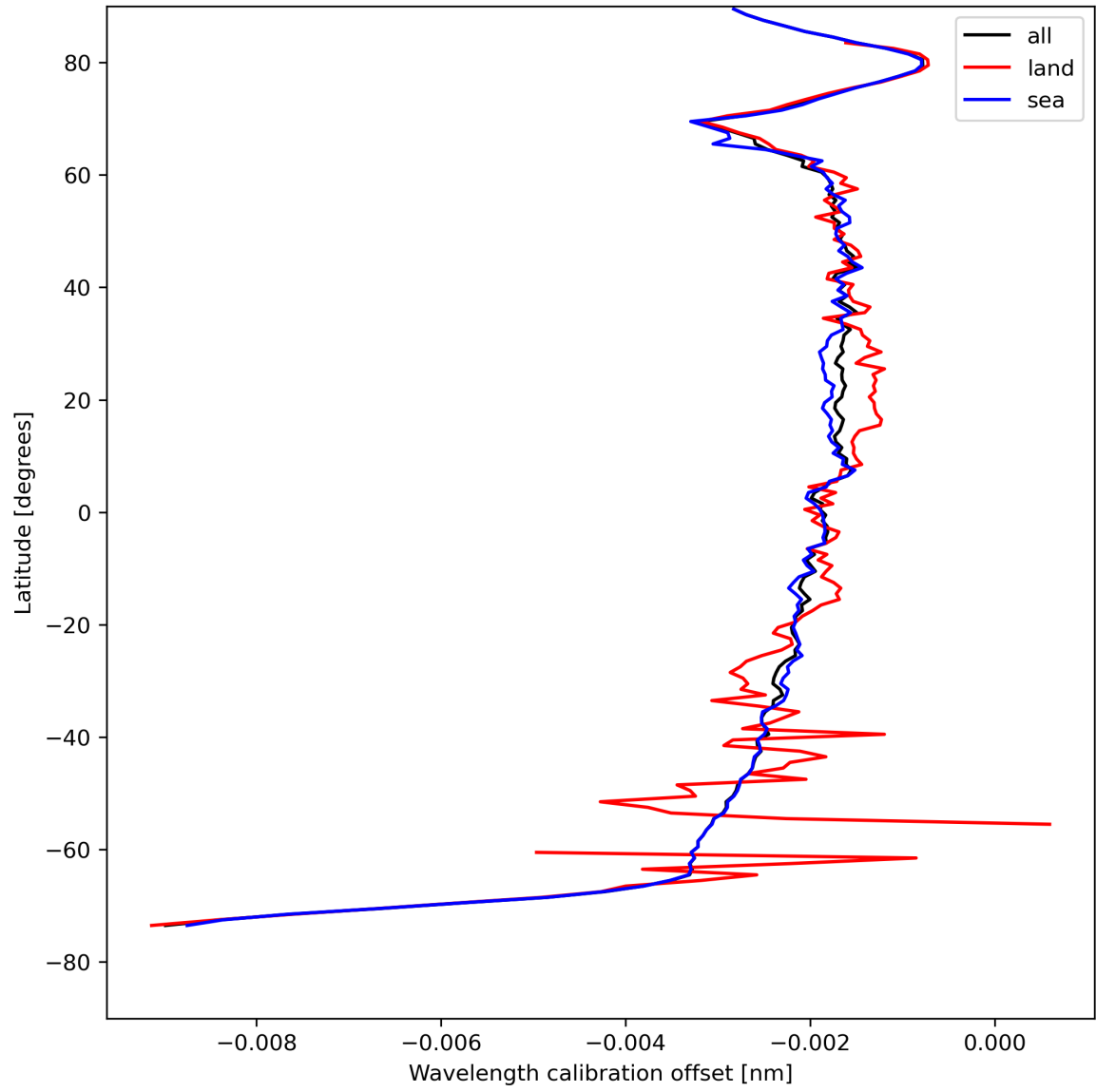
Figure 18: Zonal average of “Wavelength calibration offset” for 2024-04-27 to 2024-04-29.
