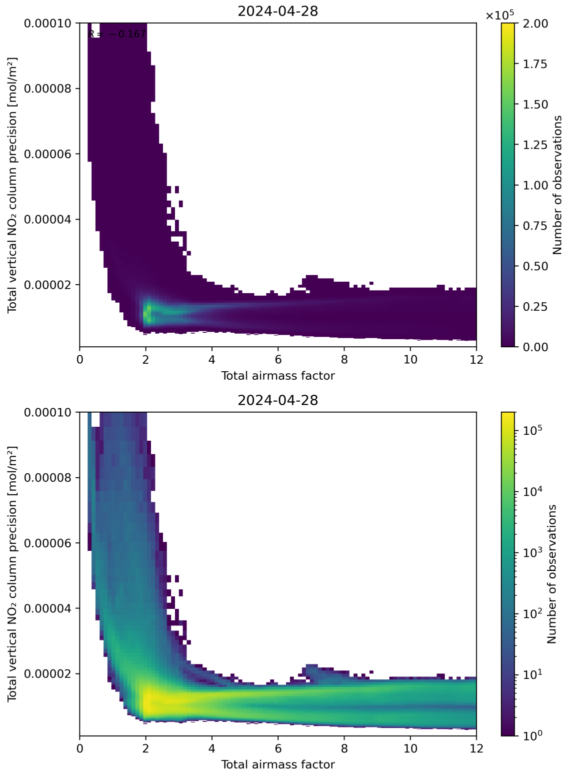
Figure 68: Scatter density plot of “Total airmass factor” against “Total vertical NO 2 column precision” for 2024-04-27 to 2024-04-29.
