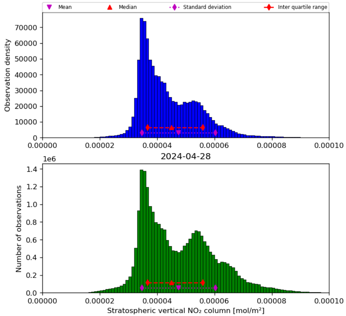
Figure 36: Histogram of “Stratospheric vertical NO 2 column” for 2024-04-27 to 2024-04-29
