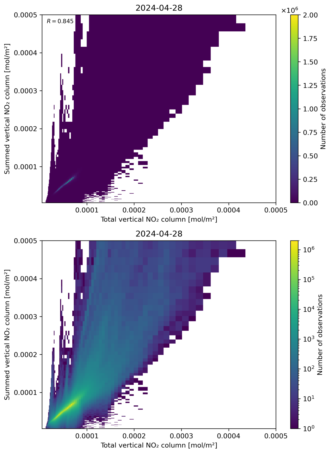
Figure 112: Scatter density plot of “Total vertical NO 2 column” against “Summed vertical NO 2 column” for 2024-04-27 to 2024-04-29.
