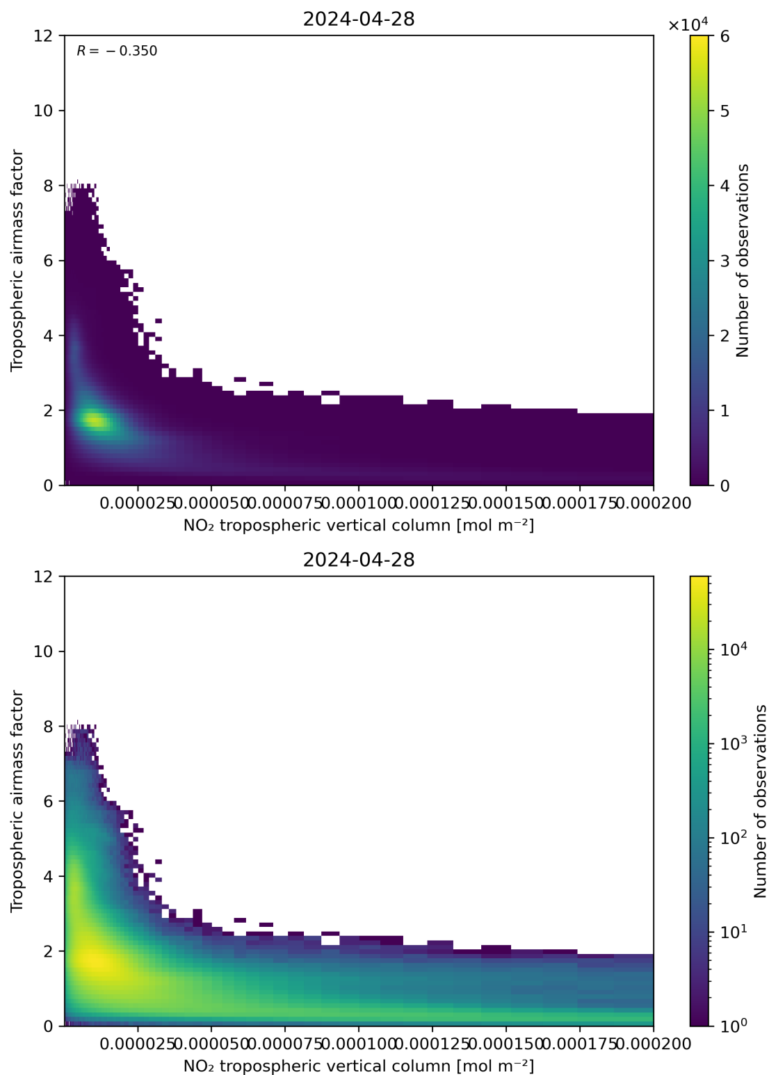
Figure 123: Scatter density plot of “NO 2 tropospheric vertical column” against “Tropospheric airmass factor” for 2024-04-27 to 2024-04-29.
