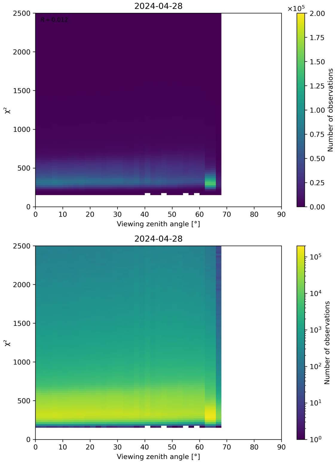
Figure 162: Scatter density plot of “Viewing zenith angle” against “ \chi^2 ” for 2024-04-27 to 2024-04-29.
