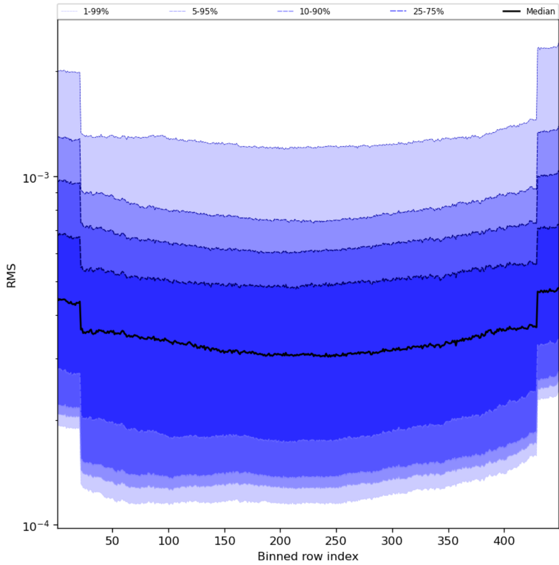
Figure 60: Along track statistics of “RMS” for 2024-04-27 to 2024-04-29
