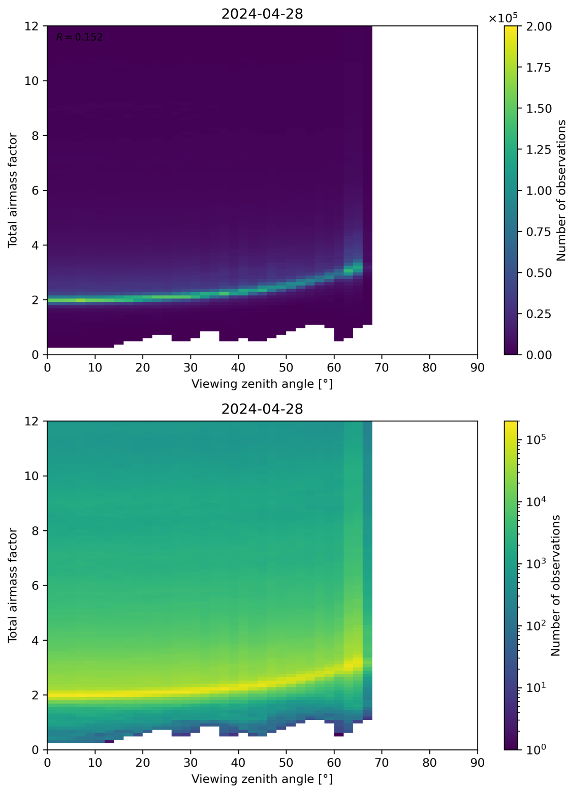
Figure 160: Scatter density plot of “Viewing zenith angle” against “Total airmass factor” for 2024-04-27 to 2024-04-29.
