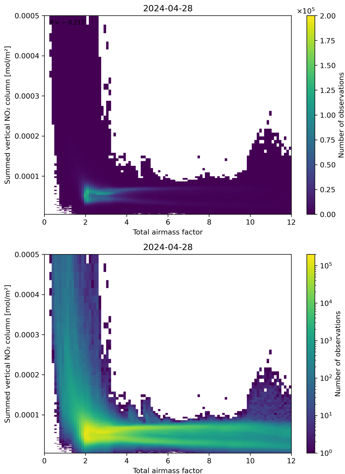
Figure 65: Scatter density plot of “Total air mass factor” against “Summed vertical NO 2 column” for 2024-04-27 to 2024-04-29.
