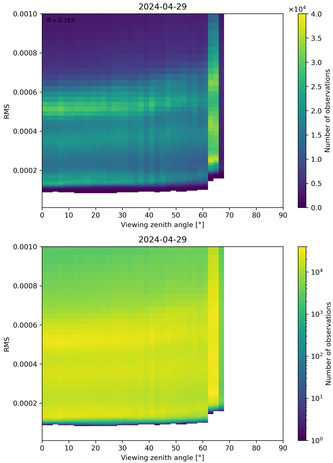
Figure 171: Scatter density plot of “Viewing zenith angle” against “RMS” for 2024-04-28 to 2024-04-30.
