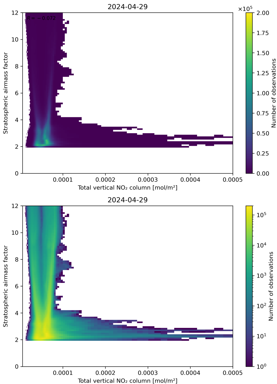
Figure 110: Scatter density plot of “Total vertical NO 2 column” against “Stratospheric airmass factor” for 2024-04-28 to 2024-04-30.
