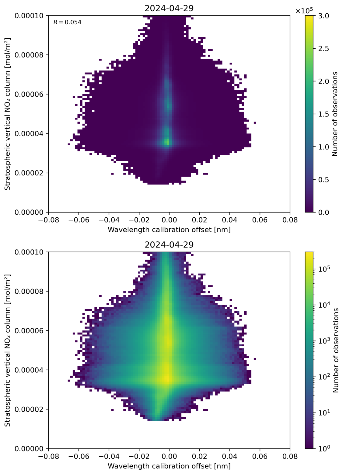
Figure 176: Scatter density plot of “Wavelength calibration offset” against “Stratospheric vertical NO 2 column” for 2024-04-28 to 2024-04-30.
