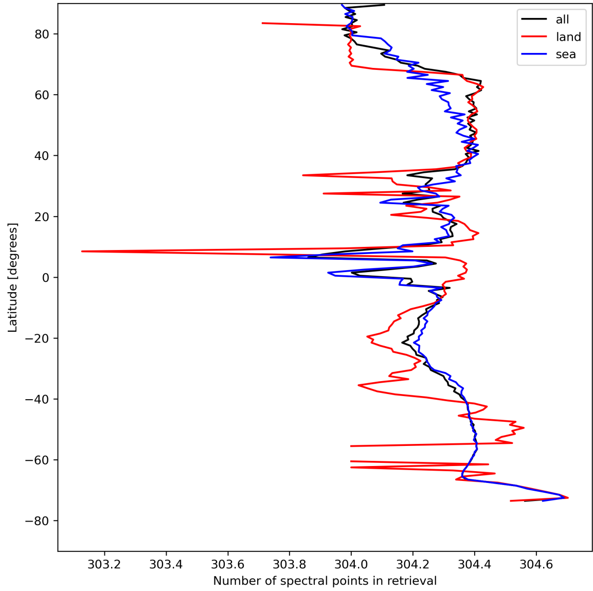
Figure 16: Zonal average of “Number of spectral points in retrieval” for 2024-04-28 to 2024-04-30.
