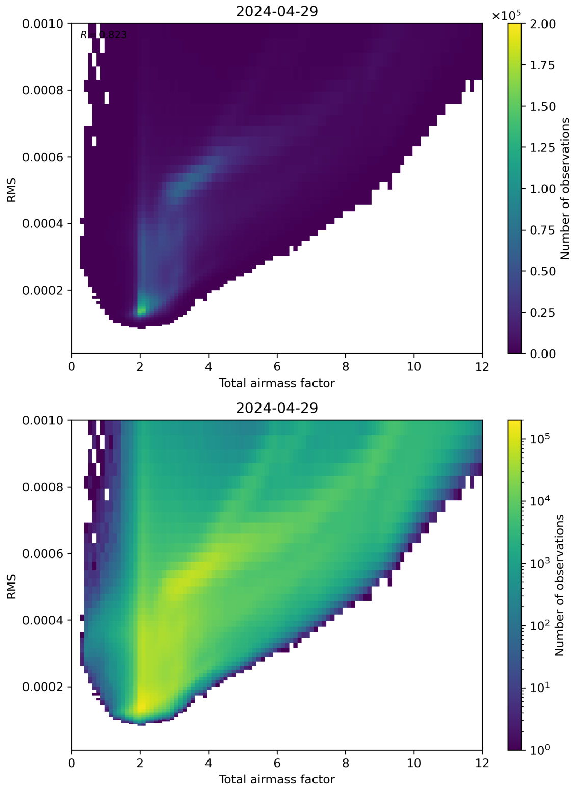
Figure 69: Scatter density plot of “Total airmass factor” against “RMS” for 2024-04-28 to 2024-04-30.
