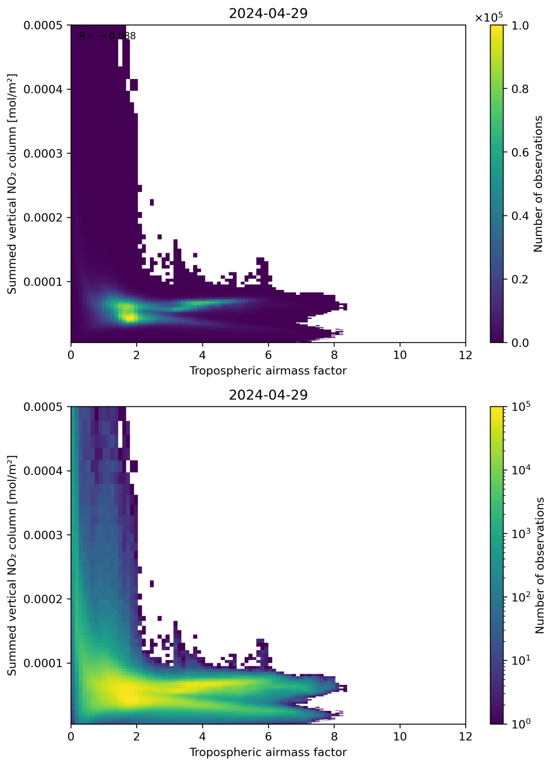
Figure 75: Scatter density plot of “Tropospheric air mass factor” against “Summed vertical NO 2 column” for 2024-04-28 to 2024-04-30.
