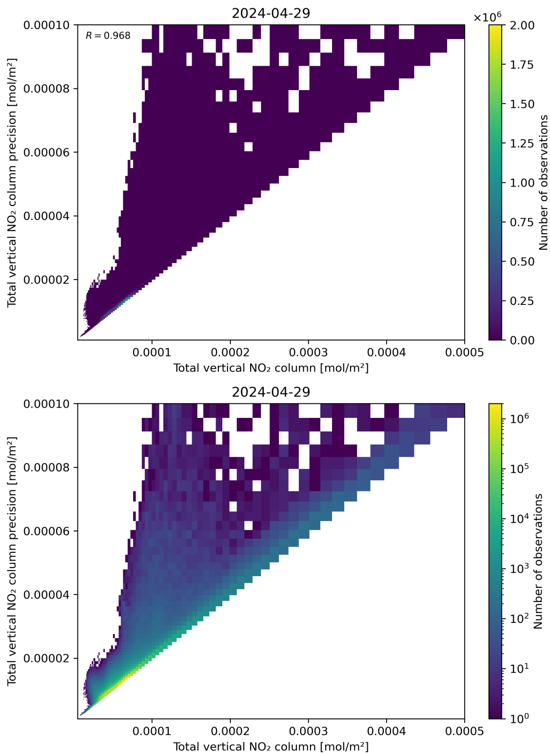
Figure 114: Scatter density plot of “Total vertical NO 2 column” against “Total vertical NO 2 column precision” for 2024-04-28 to 2024-04-30.
