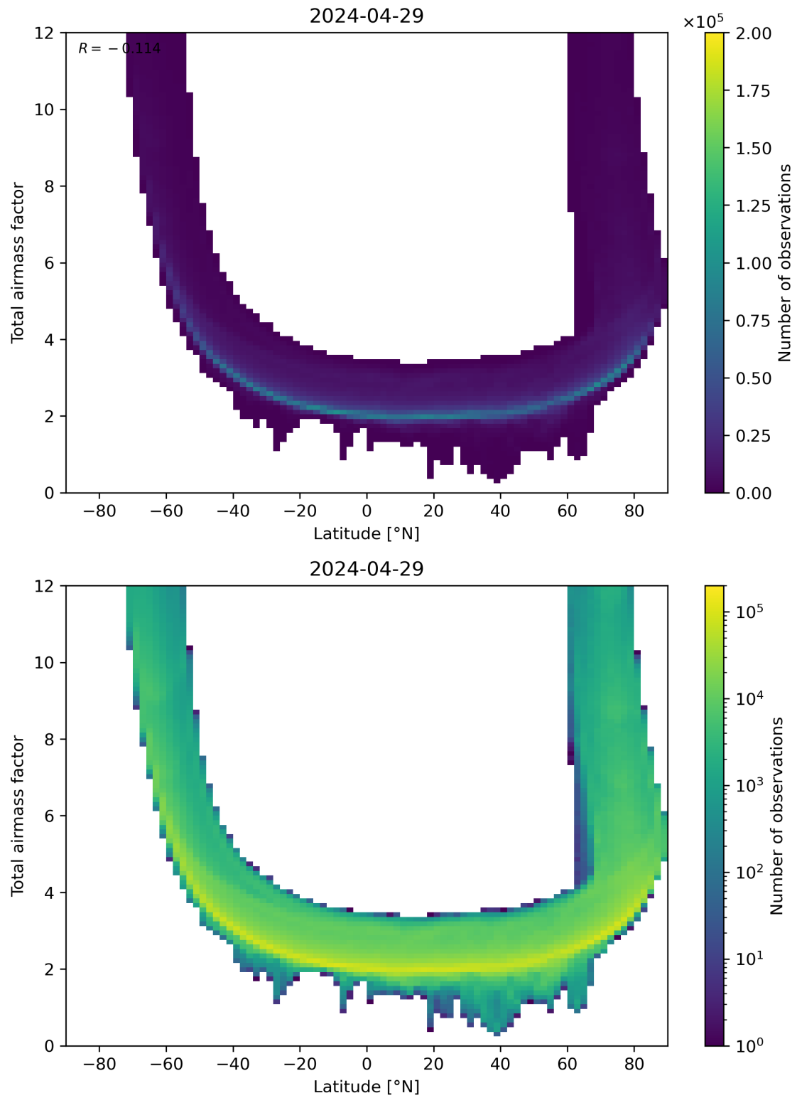
Figure 84: Scatter density plot of “Latitude” against “Total airmass factor” for 2024-04-28 to 2024-04-30.
