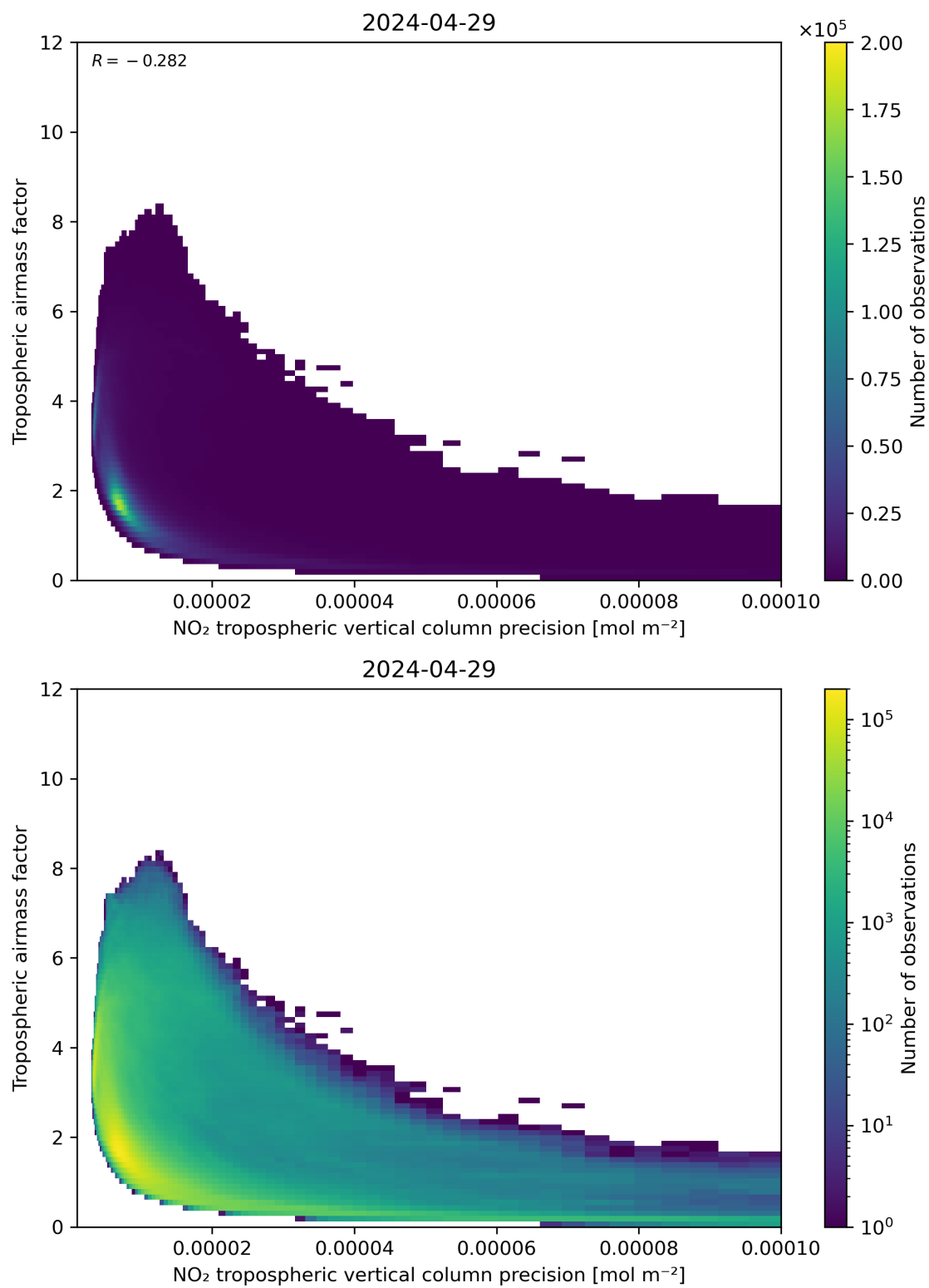
Figure 133: Scatter density plot of “NO 2 tropospheric vertical column precision” against “Tropospheric airmass factor” for 2024-04-28 to 2024-04-30.
