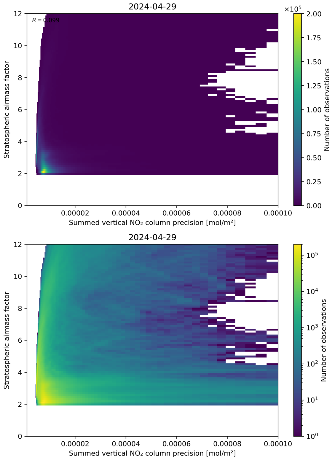
Figure 106: Scatter density plot of “Summed vertical NO 2 column precision” against “Stratospheric airmass factor” for 2024-04-28 to 2024-04-30.
