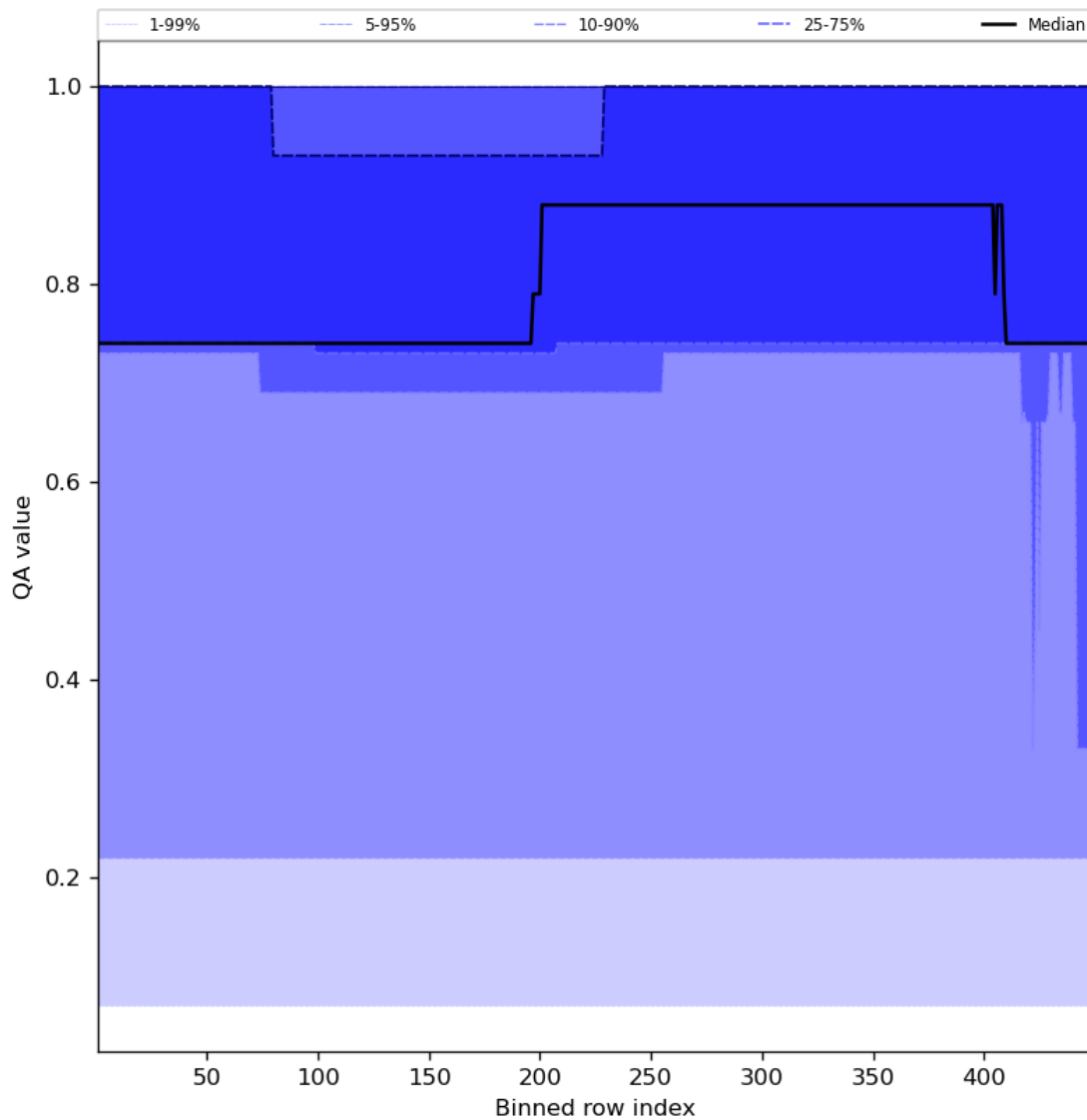
Figure 45: Along track statistics of “QA value” for 2024-04-28 to 2024-04-30
