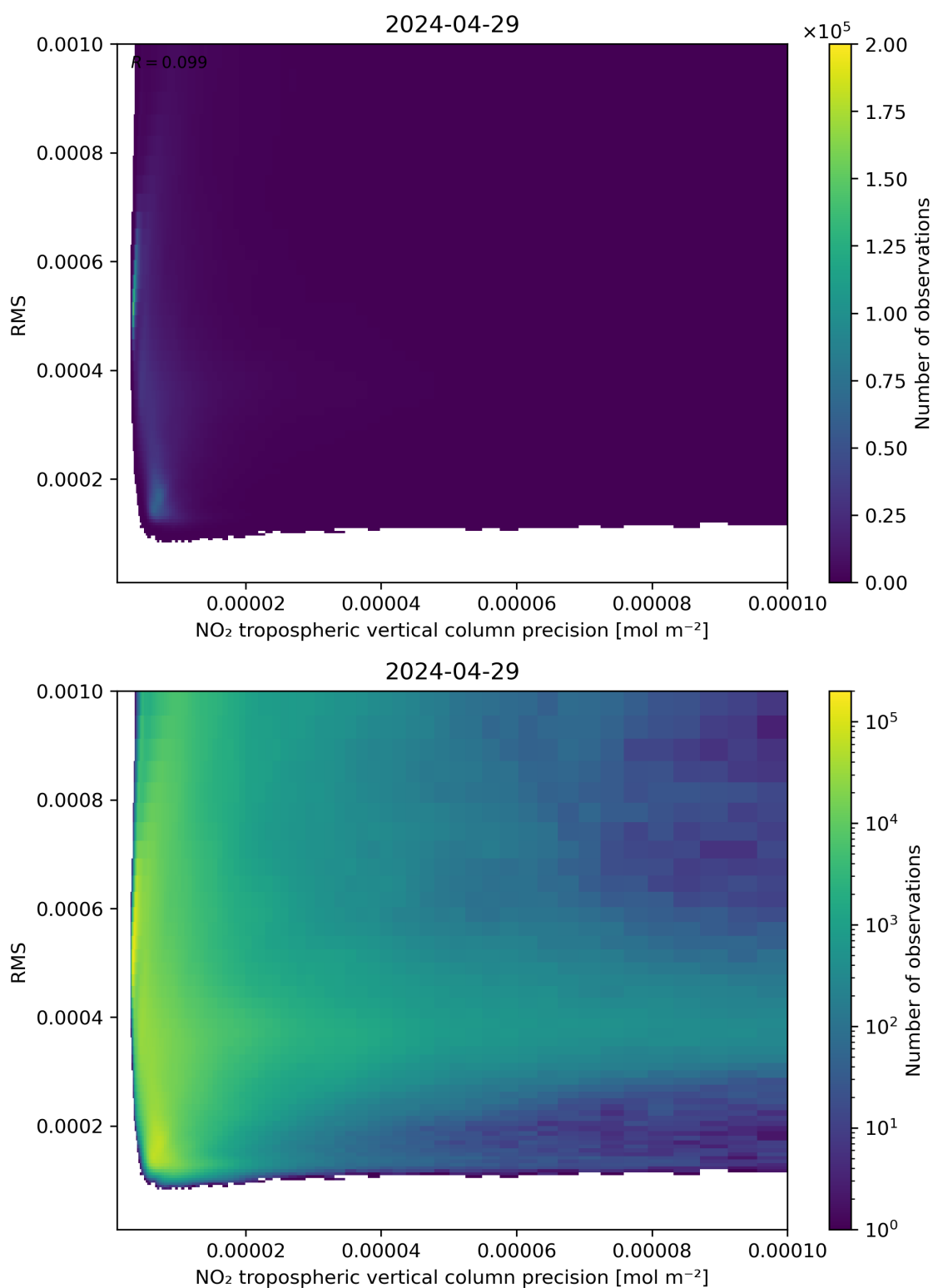
Figure 140: Scatter density plot of “NO 2 tropospheric vertical column precision” against “RMS” for 2024-04-28 to 2024-04-30.
