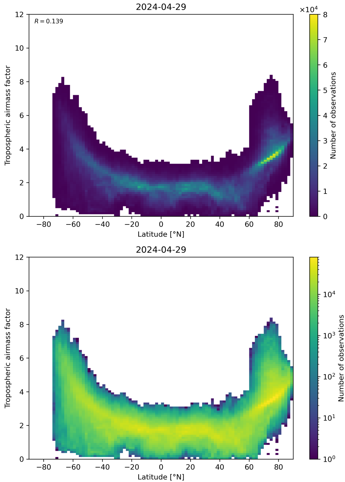
Figure 85: Scatter density plot of “Latitude” against “Tropospheric air mass factor” for 2024-04-28 to 2024-04-30.
