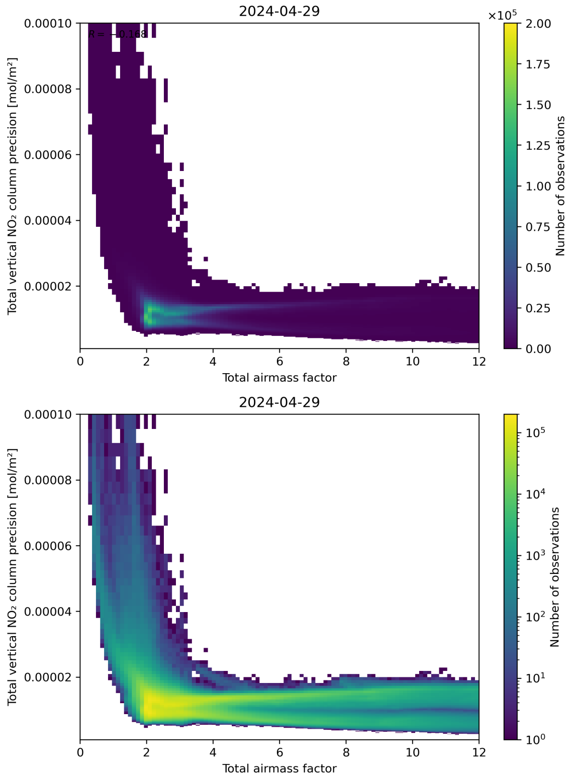
Figure 68: Scatter density plot of “Total airmass factor” against “Total vertical NO 2 column precision” for 2024-04-28 to 2024-04-30.
