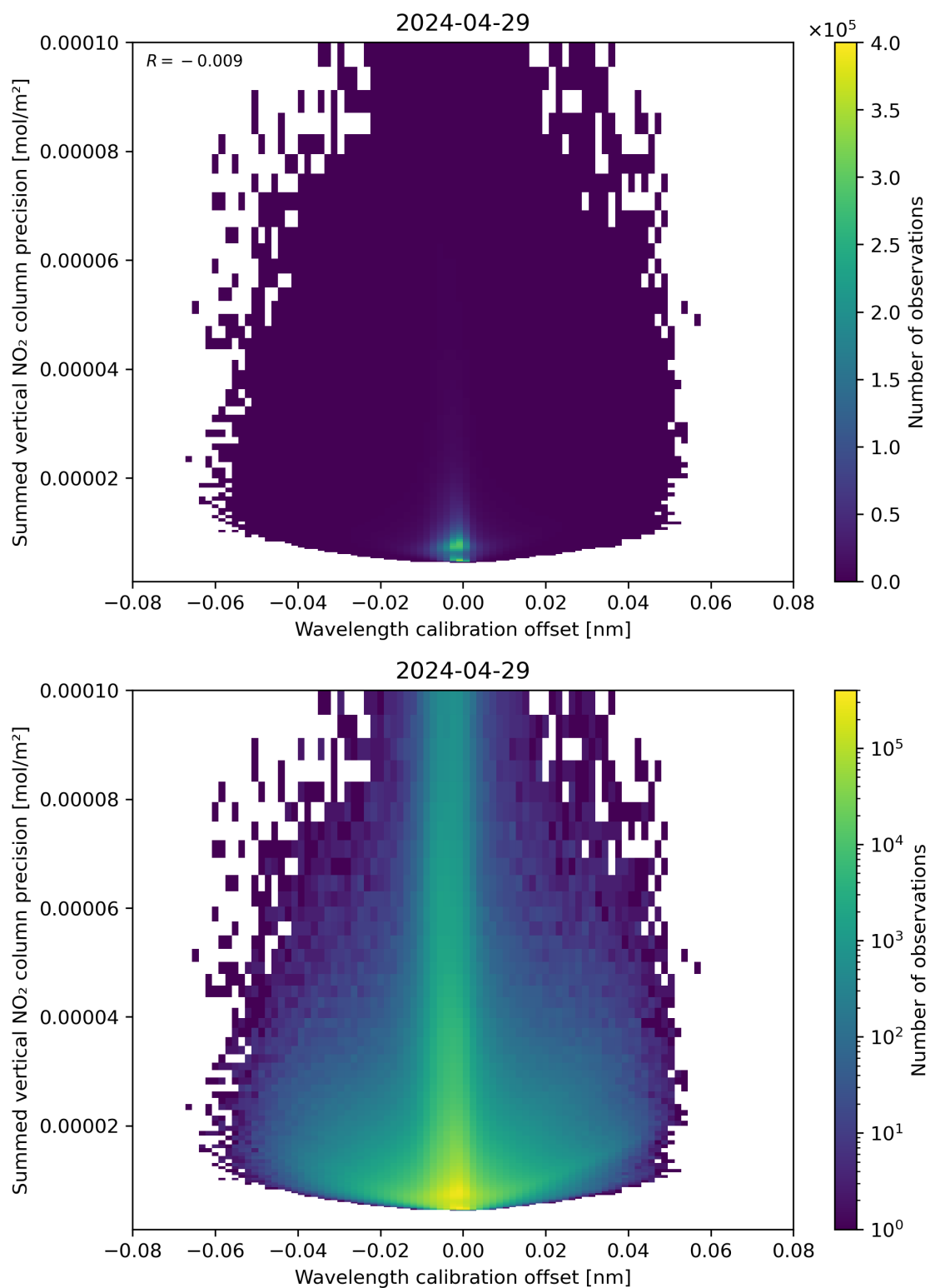
Figure 178: Scatter density plot of “Wavelength calibration offset” against “Summed vertical NO 2 column precision” for 2024-04-28 to 2024-04-30.
