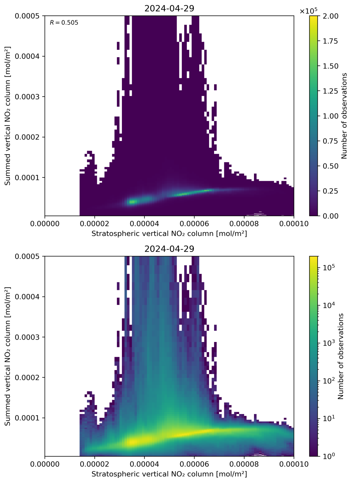
Figure 98: Scatter density plot of “Stratospheric vertical NO 2 column” against “Summed vertical NO 2 column” for 2024-04-28 to 2024-04-30.
