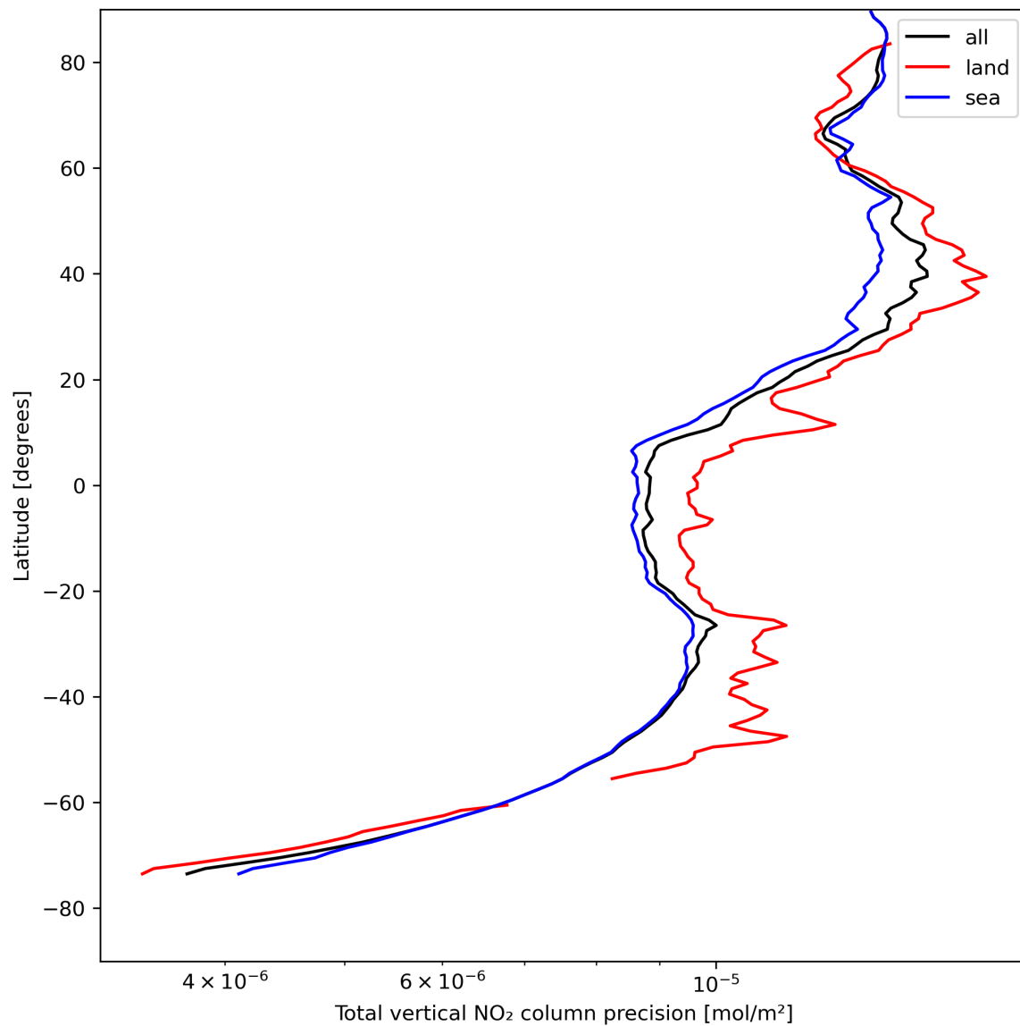
Figure 22: Zonal average of “Total vertical NO 2 column precision” for 2024-04-28 to 2024-04-30.
