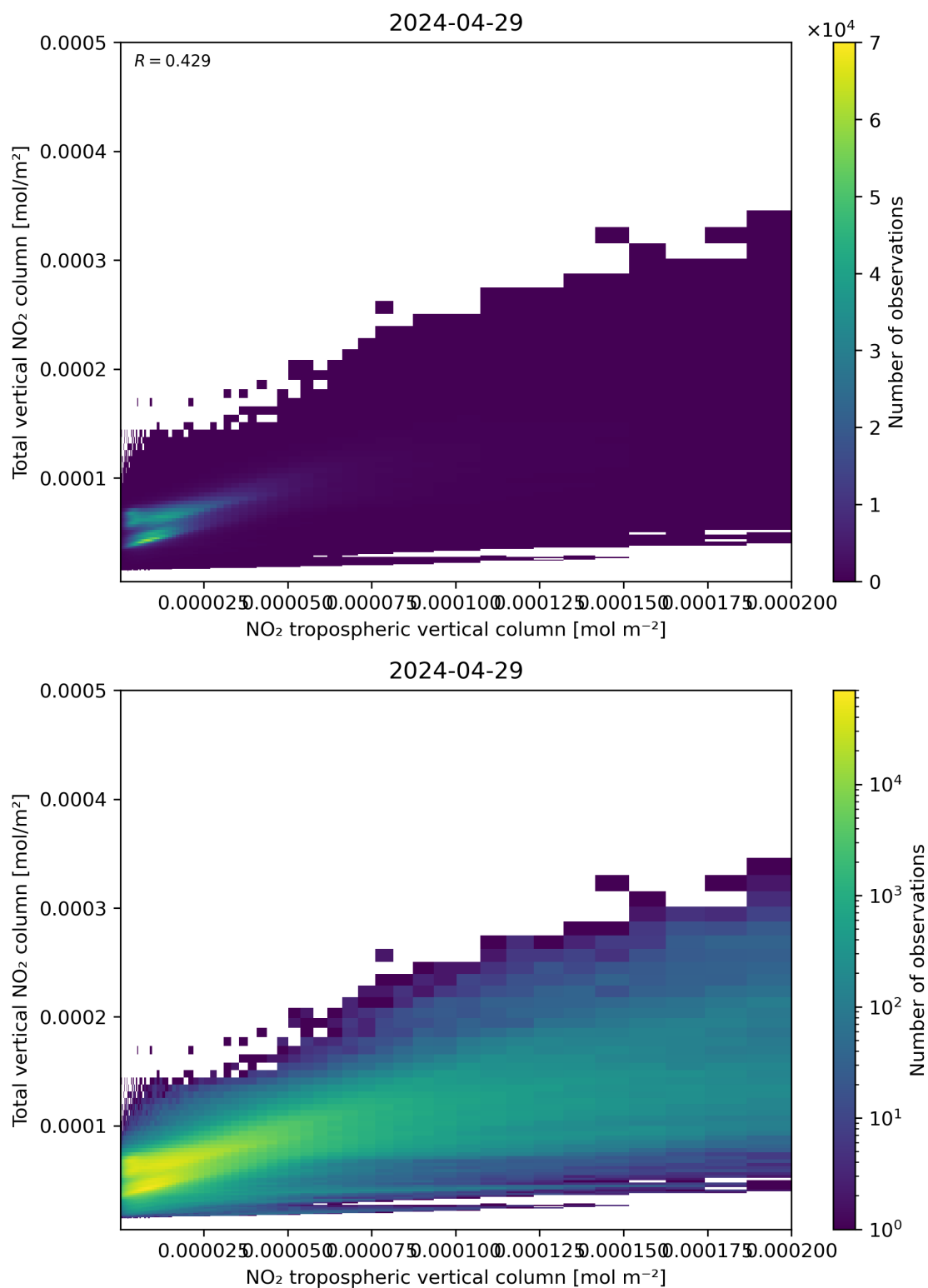
Figure 128: Scatter density plot of “NO 2 tropospheric vertical column” against “Total vertical NO 2 column” for 2024-04-28 to 2024-04-30.
