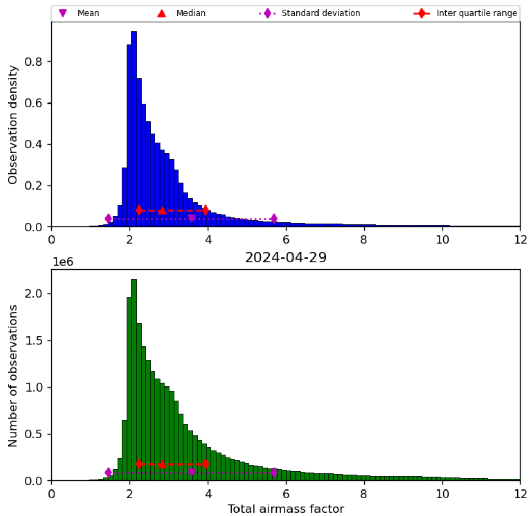
Figure 32: Histogram of “Total airmass factor” for 2024-04-28 to 2024-04-30
