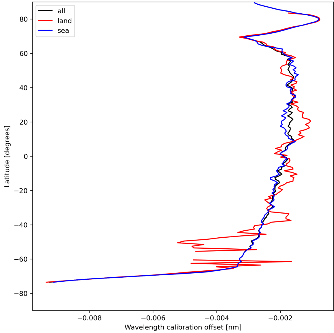
Figure 18: Zonal average of “Wavelength calibration offset” for 2024-04-28 to 2024-04-30.
