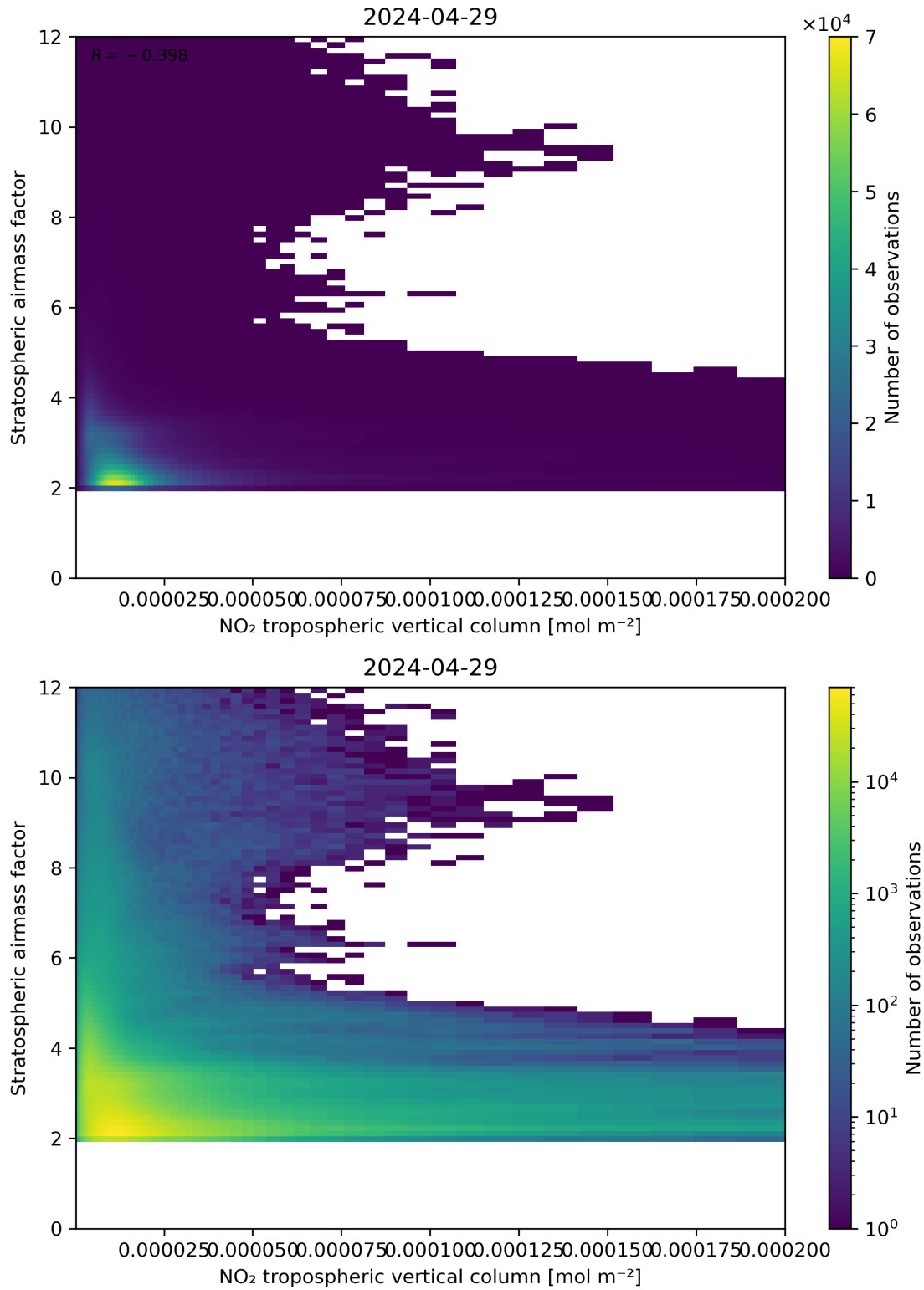
Figure 121: Scatter density plot of “NO 2 tropospheric vertical column” against “Stratospheric air mass factor” for 2024-04-28 to 2024-04-30.
