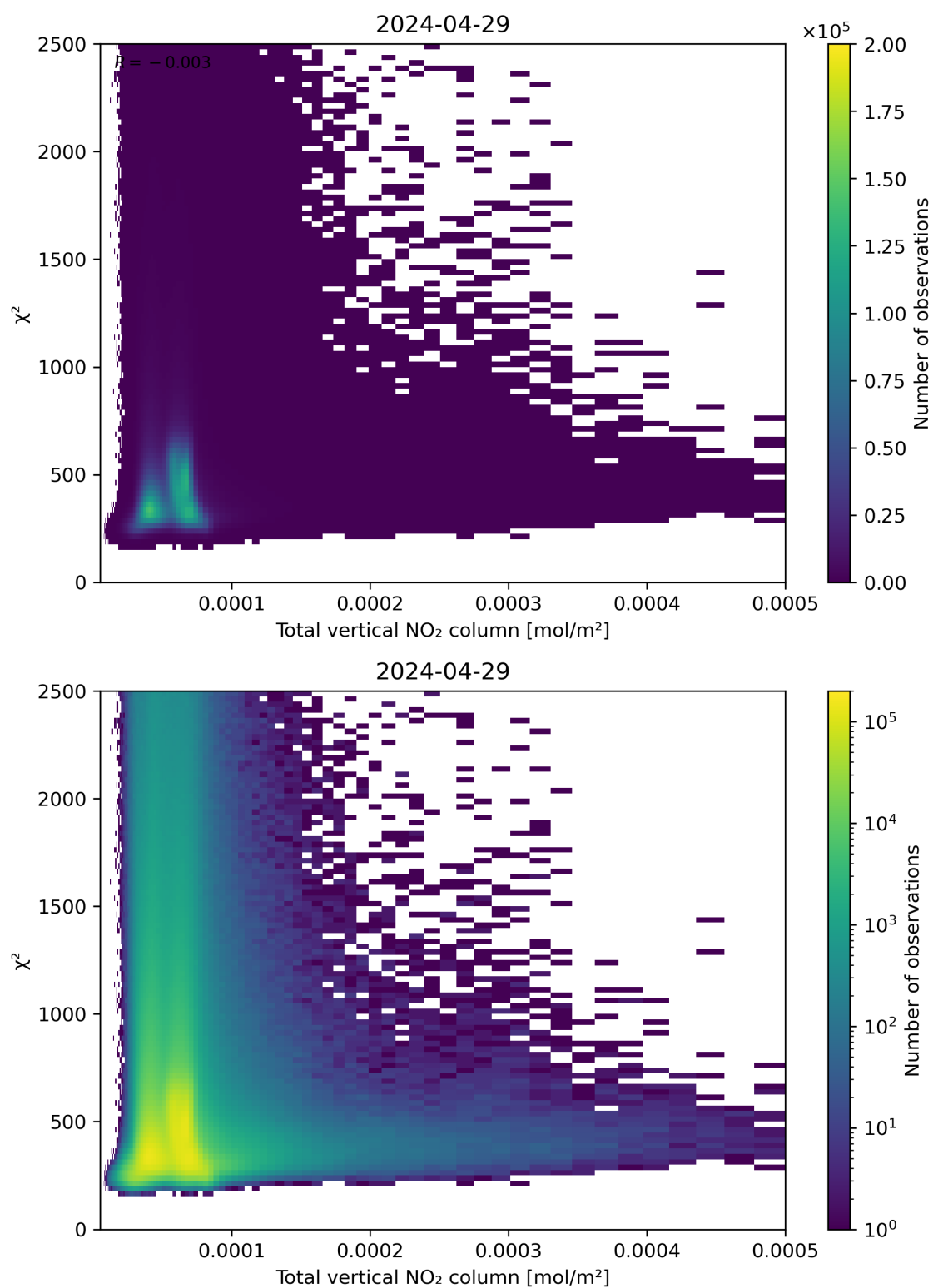
Figure 111: Scatter density plot of “Total vertical NO 2 column” against “ \chi^2 ” for 2024-04-28 to 2024-04-30.
