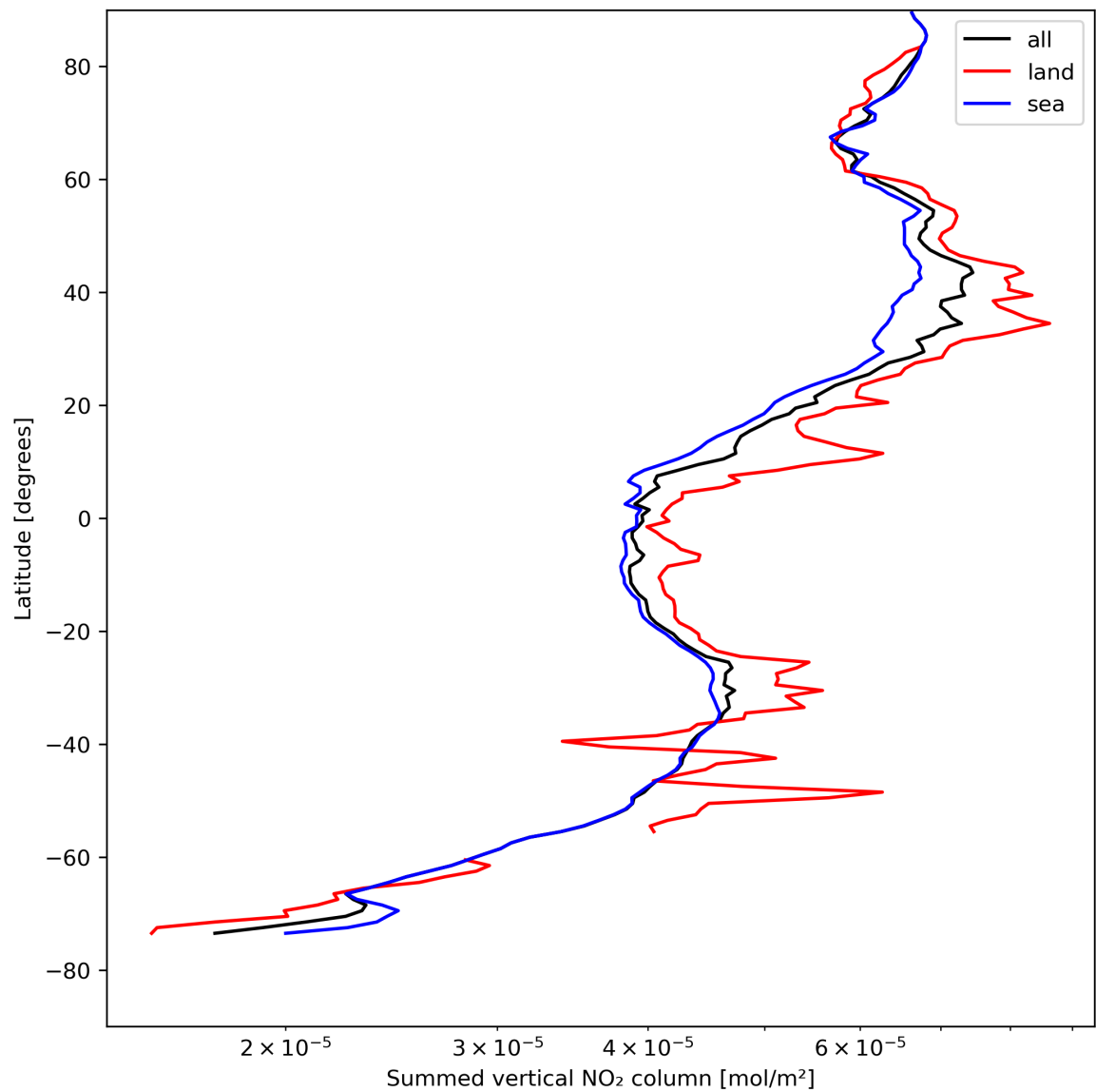
Figure 23: Zonal average of “Summed vertical NO 2 column” for 2024-04-28 to 2024-04-30.
