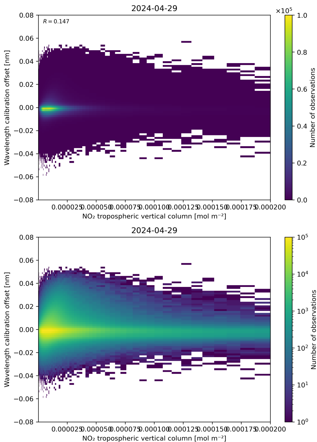
Figure 143: Scatter density plot of “NO 2 tropospheric vertical column” against “Wavelength calibration offset” for 2024-04-28 to 2024-04-30.
