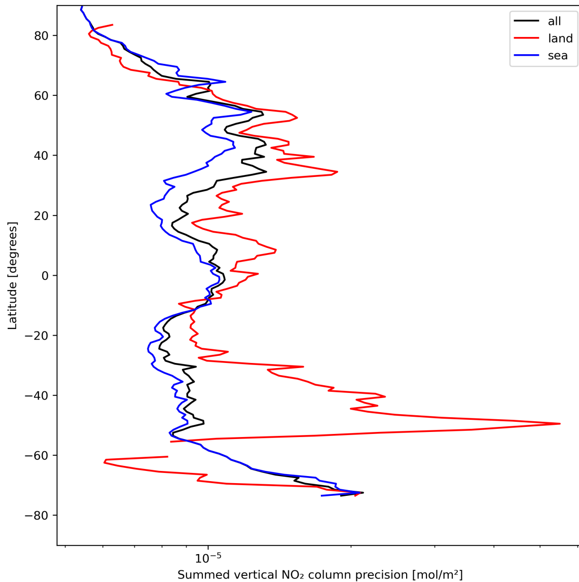
Figure 24: Zonal average of “Summed vertical NO 2 column precision” for 2024-04-28 to 2024-04-30.
