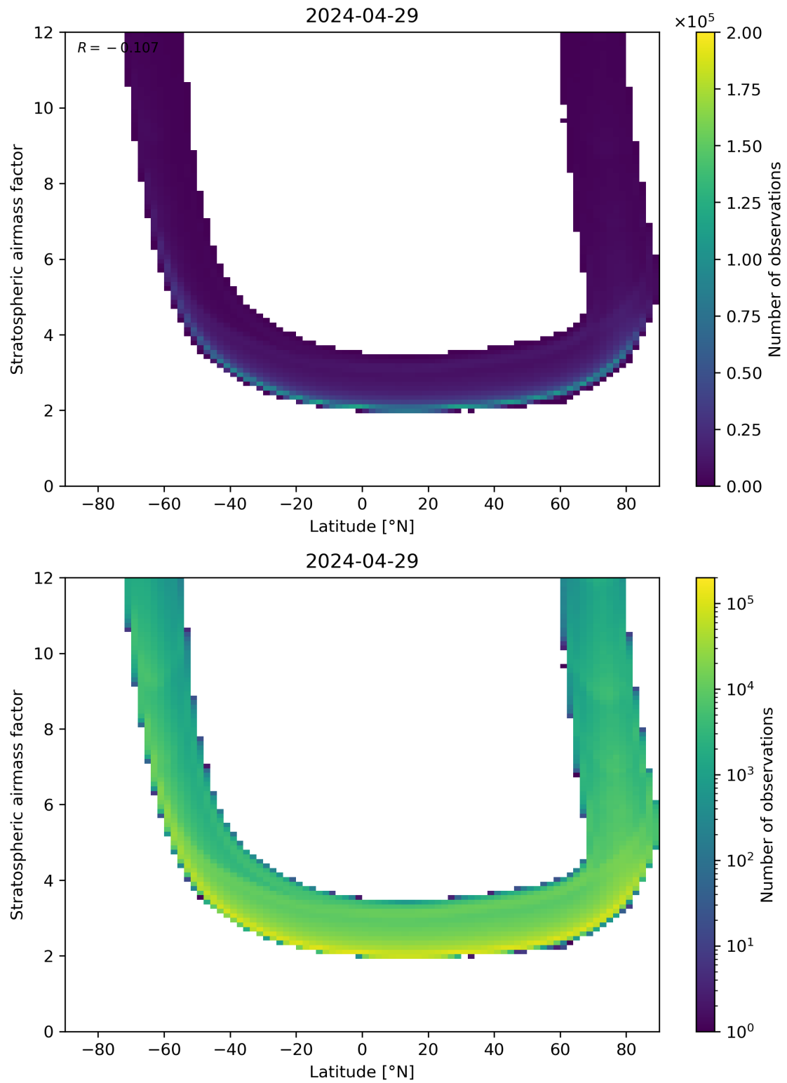
Figure 83: Scatter density plot of “Latitude” against “Stratospheric air mass factor” for 2024-04-28 to 2024-04-30.
