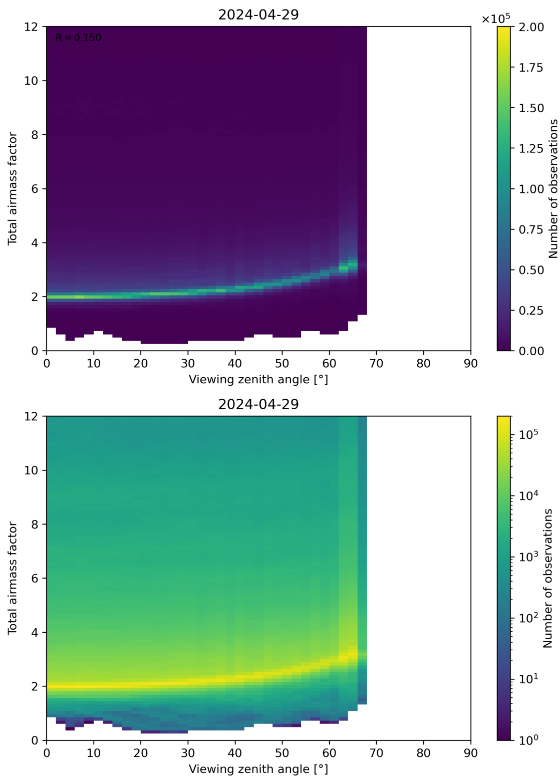
Figure 160: Scatter density plot of “Viewing zenith angle” against “Total airmass factor” for 2024-04-28 to 2024-04-30.
