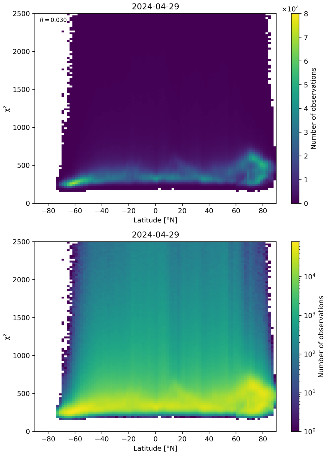
Figure 86: Scatter density plot of “Latitude” against “ \chi^2 ” for 2024-04-28 to 2024-04-30.
