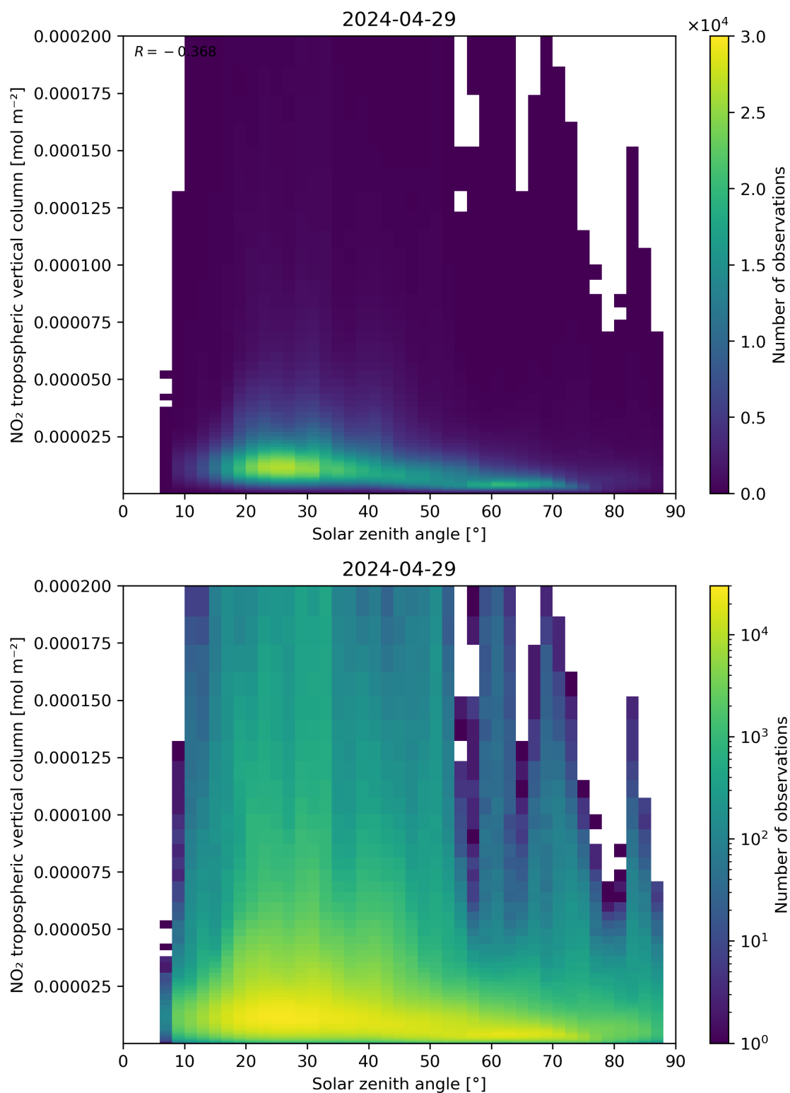
Figure 155: Scatter density plot of “Solar zenith angle” against “NO 2 tropospheric vertical column” for 2024-04-28 to 2024-04-30.
