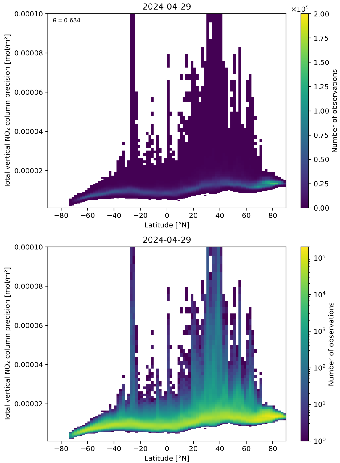
Figure 91: Scatter density plot of “Latitude” against “Total vertical NO 2 column precision” for 2024-04-28 to 2024-04-30.
