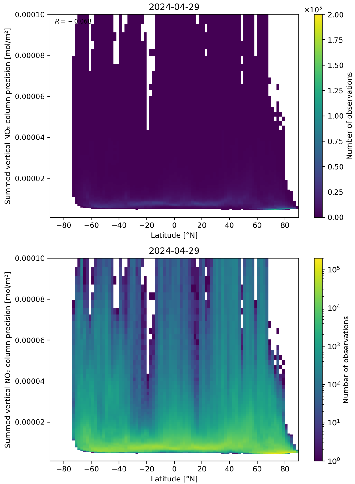
Figure 89: Scatter density plot of “Latitude” against “Summed vertical NO 2 column precision” for 2024-04-28 to 2024-04-30.
