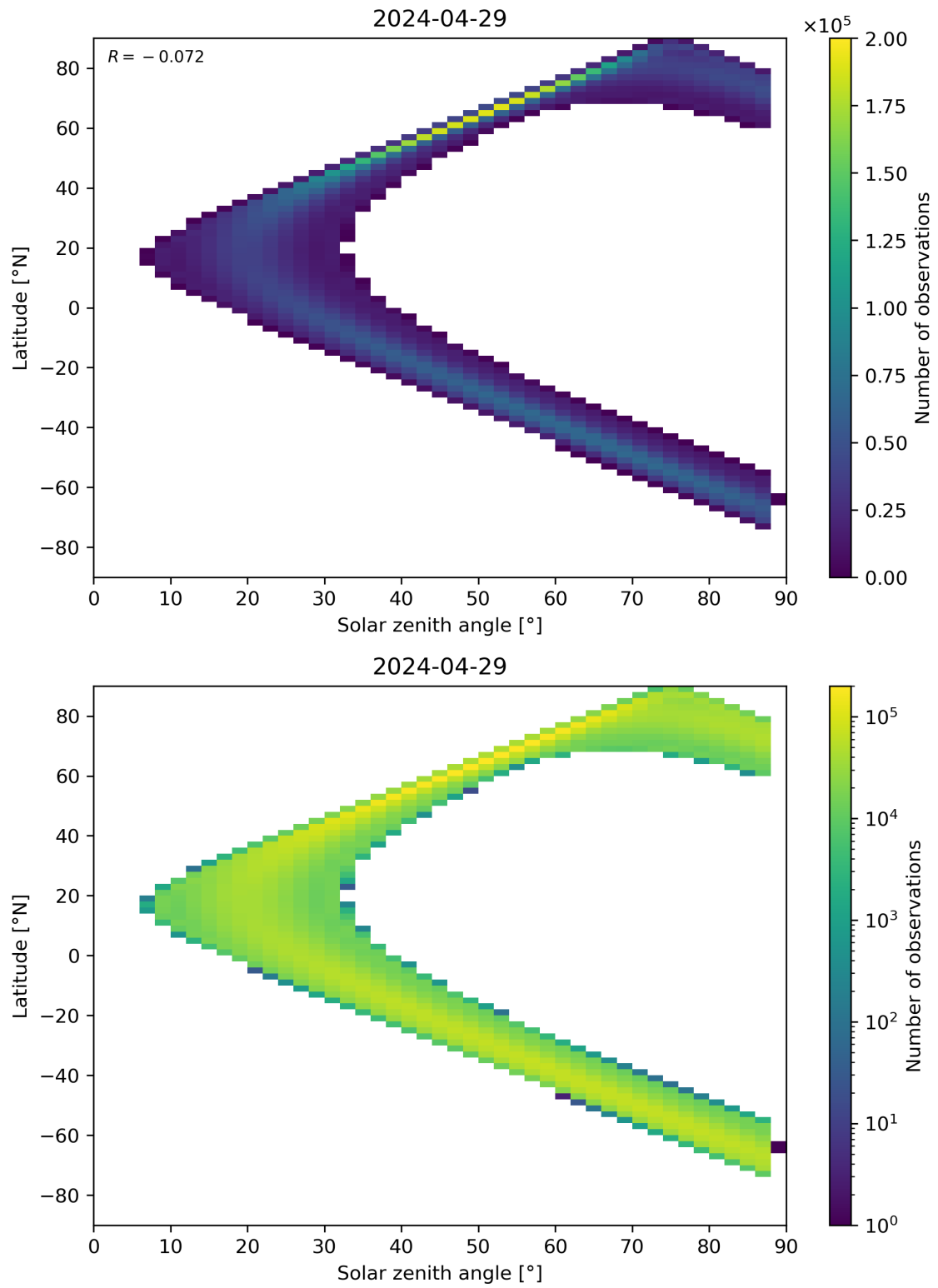
Figure 149: Scatter density plot of “Solar zenith angle” against “Latitude” for 2024-04-28 to 2024-04-30.
