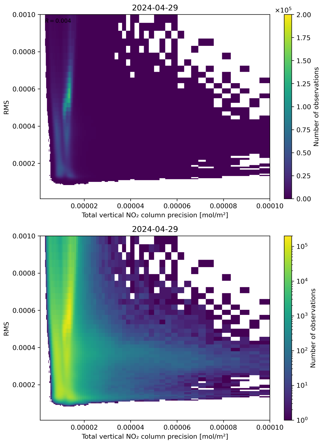
Figure 119: Scatter density plot of “Total vertical NO 2 column precision” against “RMS” for 2024-04-28 to 2024-04-30.
