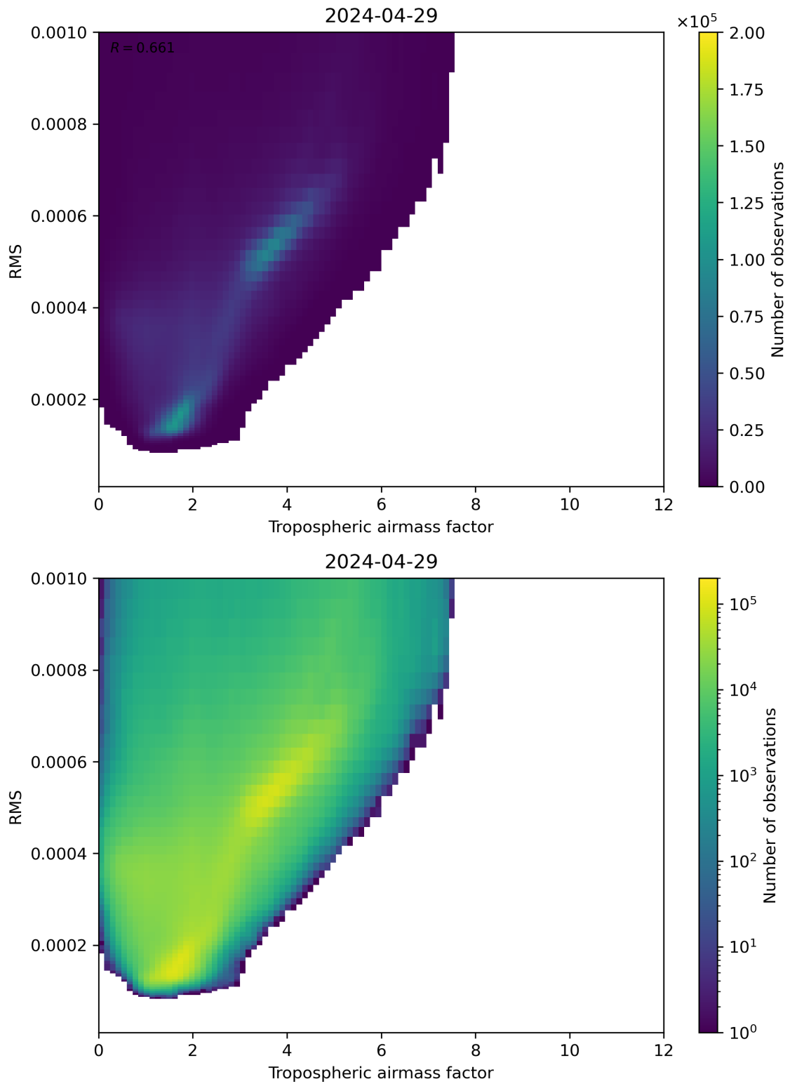
Figure 79: Scatter density plot of “Tropospheric airmass factor” against “RMS” for 2024-04-28 to 2024-04-30.
