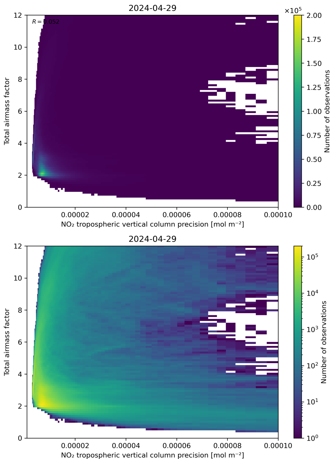
Figure 132: Scatter density plot of “NO 2 tropospheric vertical column precision” against “Total air mass factor” for 2024-04-28 to 2024-04-30.
