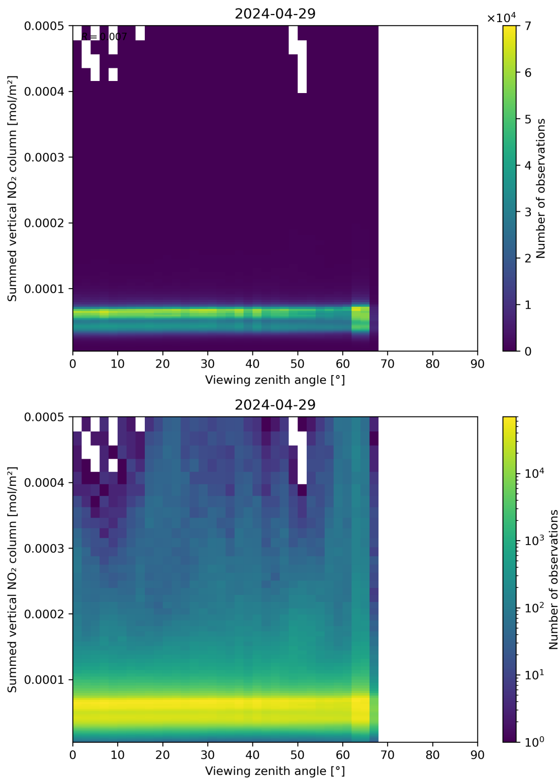
Figure 165: Scatter density plot of “Viewing zenith angle” against “Summed vertical NO 2 column” for 2024-04-28 to 2024-04-30.
