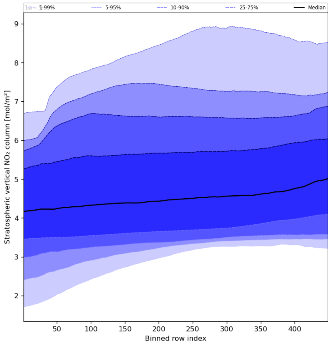
Figure 53: Along track statistics of “Stratospheric vertical NO 2 column” for 2024-04-28 to 2024-04-30
