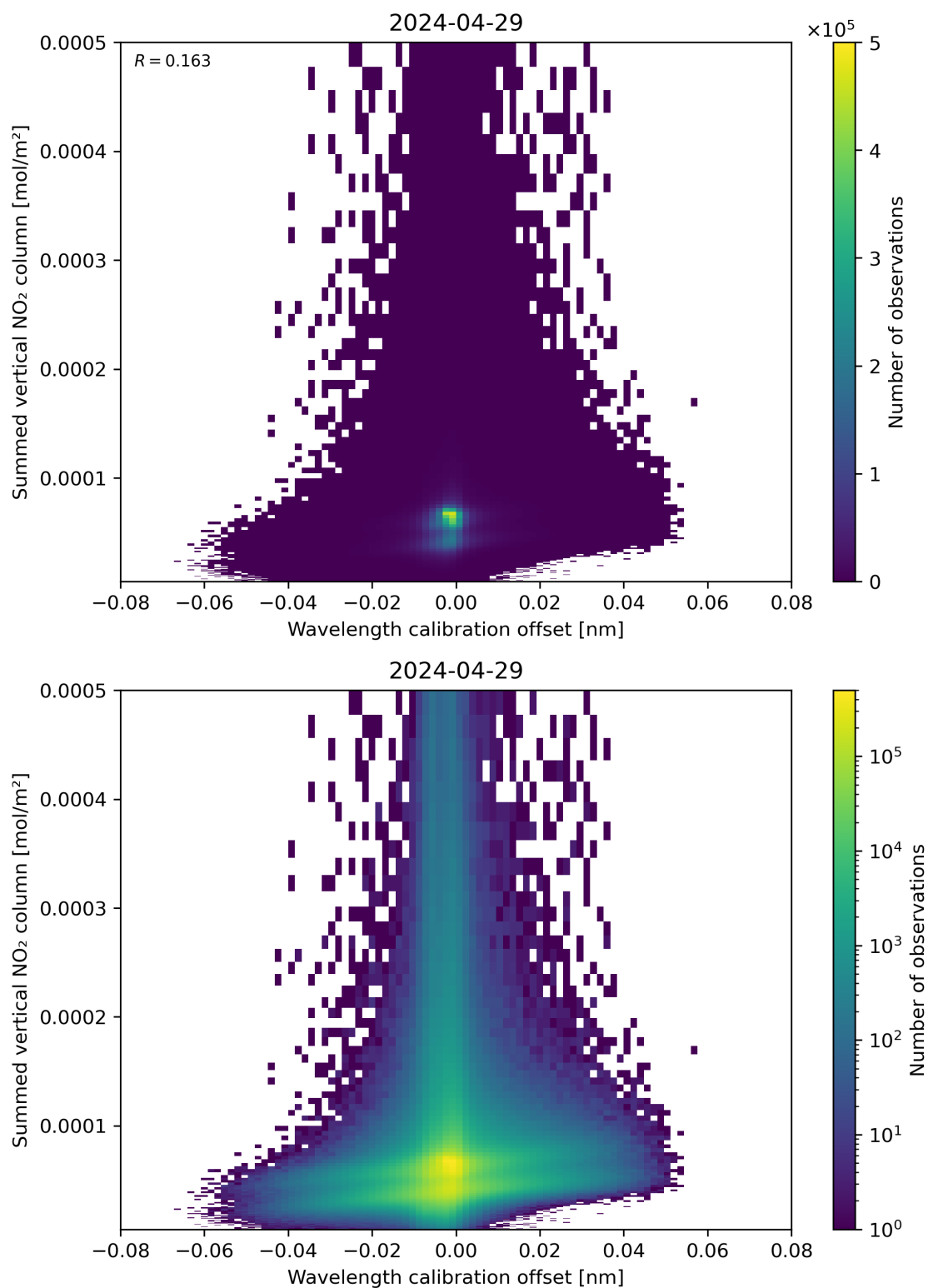
Figure 177: Scatter density plot of “Wavelength calibration offset” against “Summed vertical NO 2 column” for 2024-04-28 to 2024-04-30.
