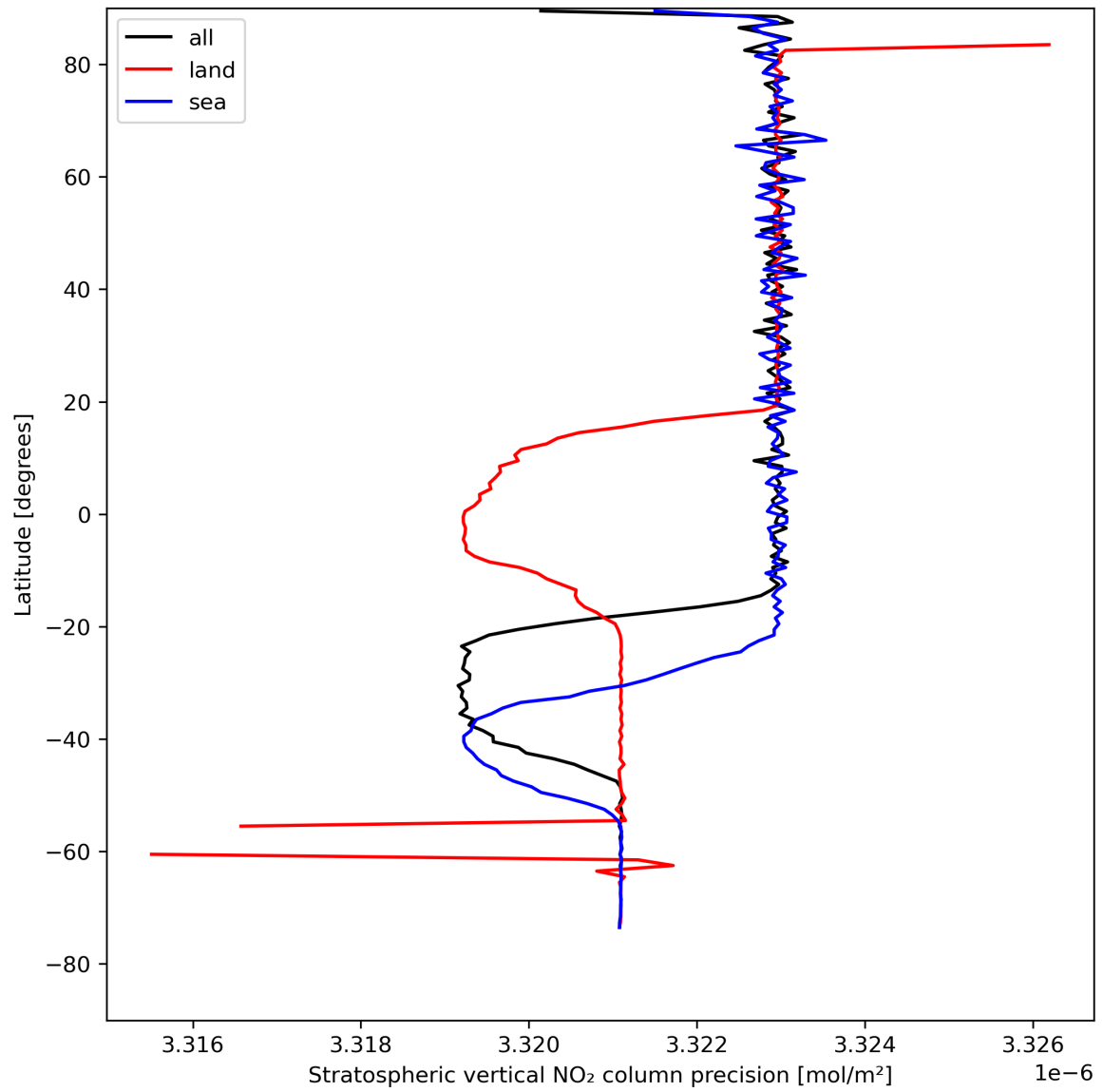
Figure 20: Zonal average of “Stratospheric vertical NO 2 column precision” for 2024-04-28 to 2024-04-30.
