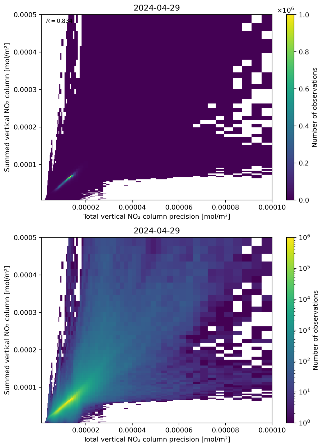
Figure 117: Scatter density plot of “Total vertical NO 2 column precision” against “Summed vertical NO 2 column” for 2024-04-28 to 2024-04-30.
