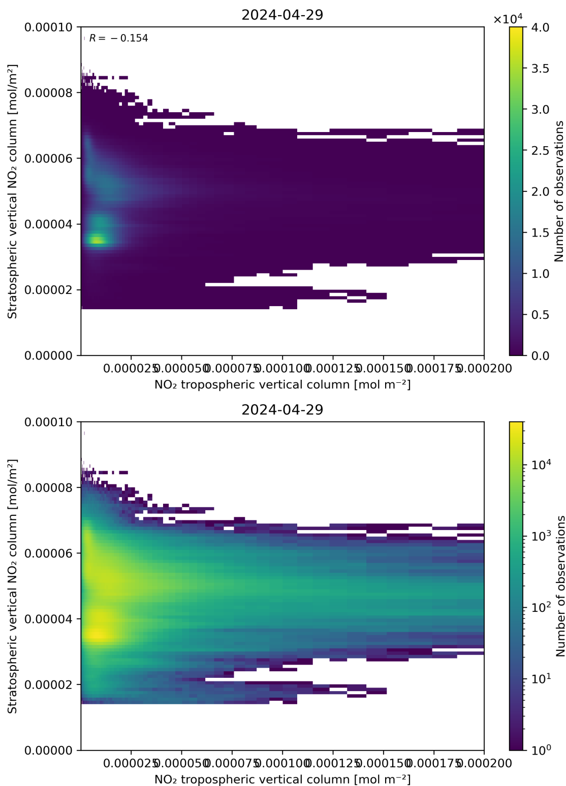
Figure 125: Scatter density plot of “NO 2 tropospheric vertical column” against “Stratospheric vertical NO 2 column” for 2024-04-28 to 2024-04-30.
