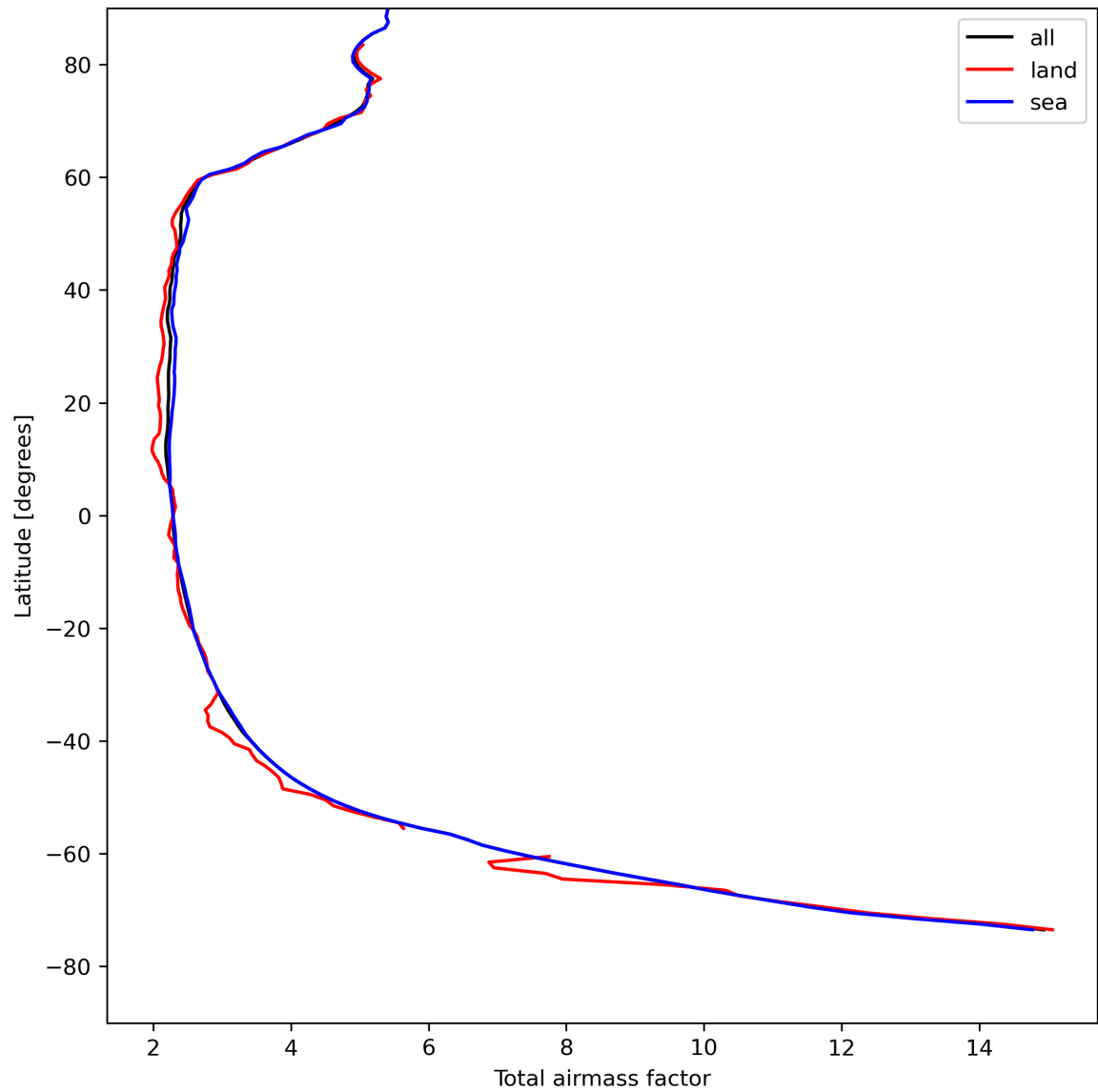
Figure 15: Zonal average of “Total airmass factor” for 2024-04-28 to 2024-04-30.
