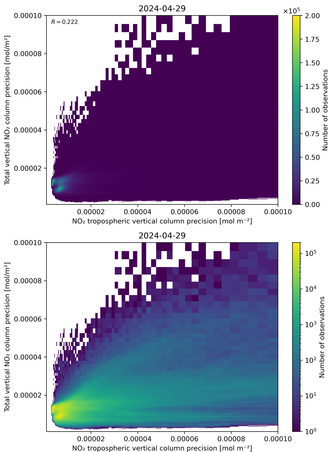
Figure 139: Scatter density plot of “NO 2 tropospheric vertical column precision” against “Total vertical NO 2 column precision” for 2024-04-28 to 2024-04-30.
