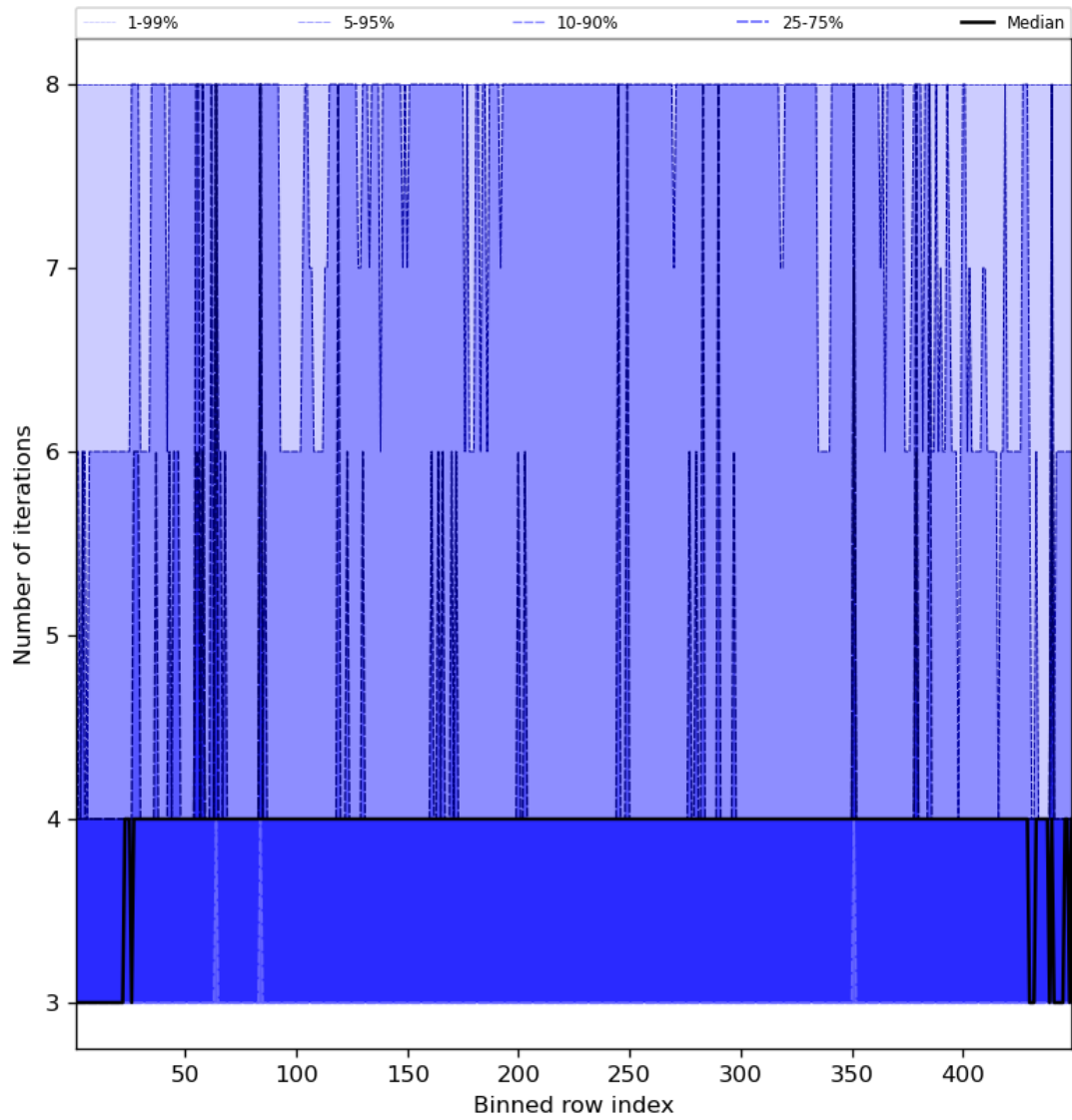
Figure 51: Along track statistics of “Number of iterations” for 2024-04-28 to 2024-04-30
