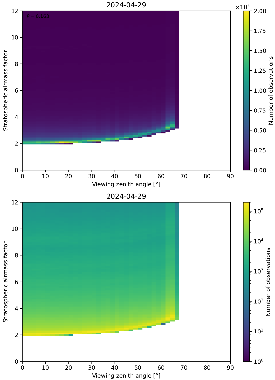
Figure 159: Scatter density plot of “Viewing zenith angle” against “Stratospheric airmass factor” for 2024-04-28 to 2024-04-30.
