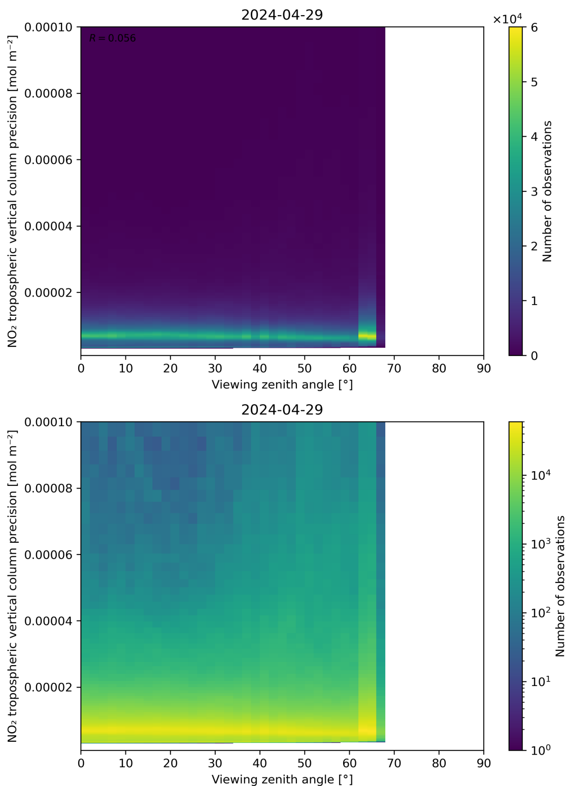
Figure 170: Scatter density plot of “Viewing zenith angle” against “NO 2 tropospheric vertical column precision” for 2024-04-28 to 2024-04-30.
