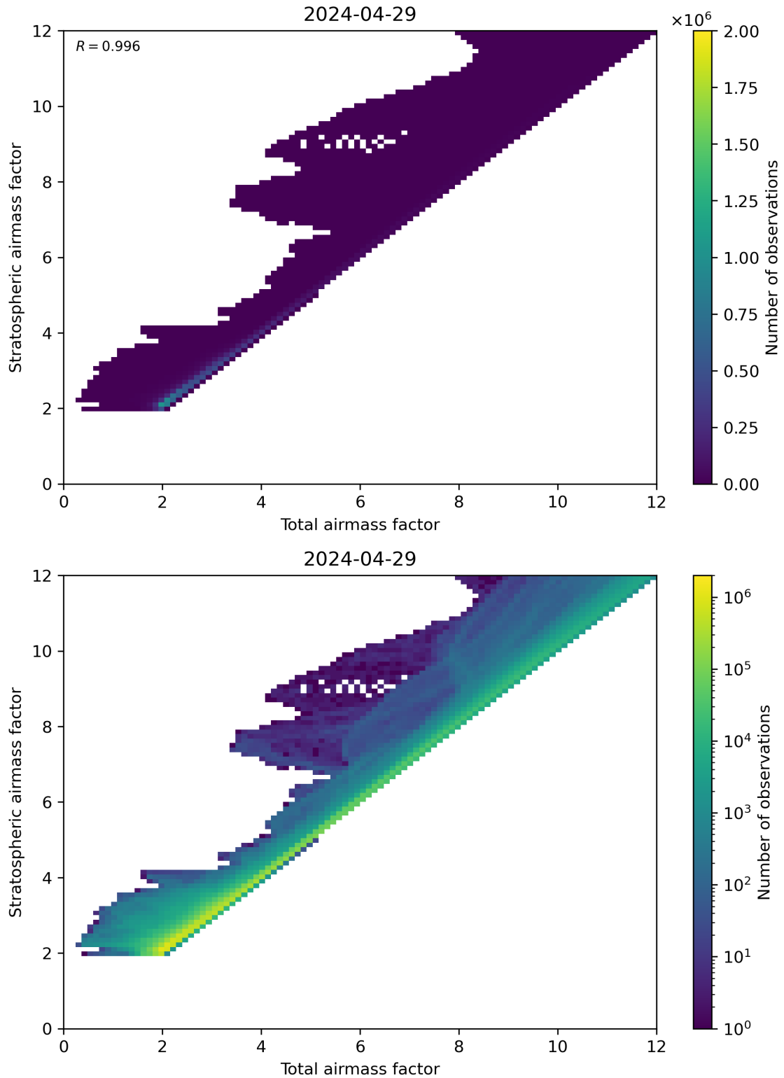
Figure 62: Scatter density plot of “Total airmass factor” against “Stratospheric airmass factor” for 2024-04-28 to 2024-04-30.
