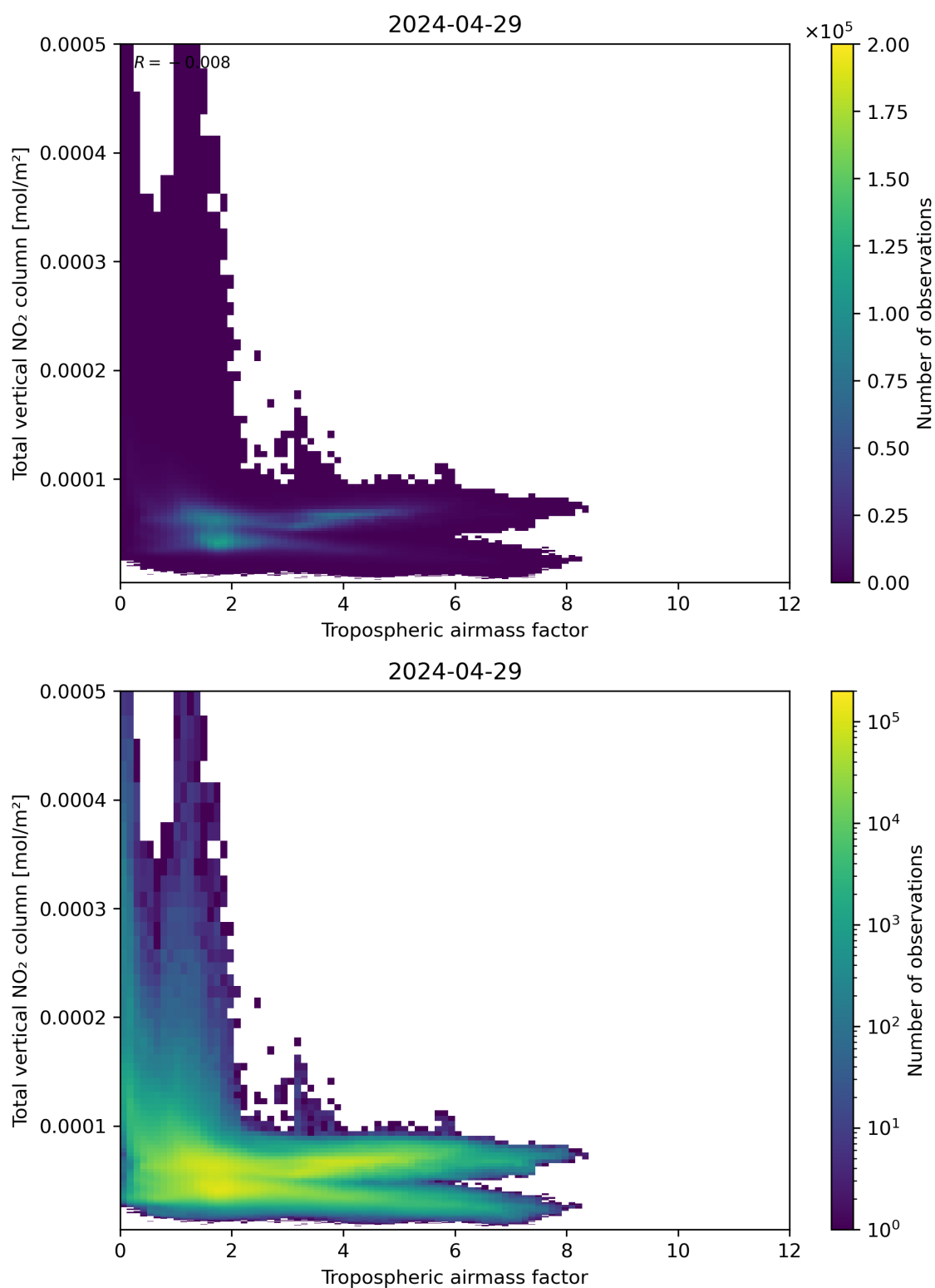
Figure 77: Scatter density plot of “Tropospheric airmass factor” against “Total vertical NO 2 column” for 2024-04-28 to 2024-04-30.
