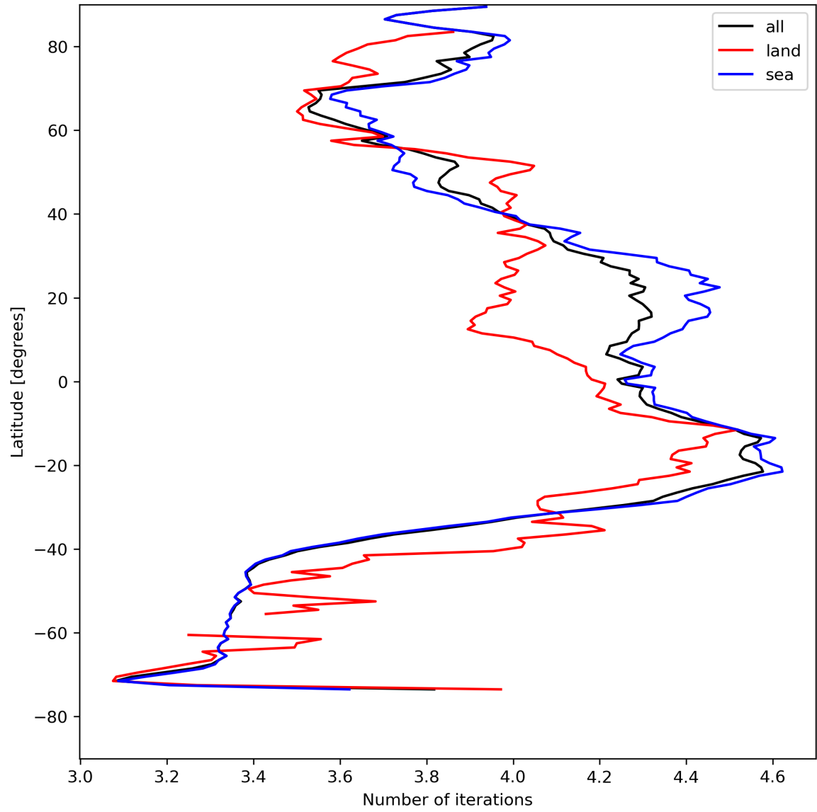
Figure 17: Zonal average of “Number of iterations” for 2024-04-28 to 2024-04-30.
