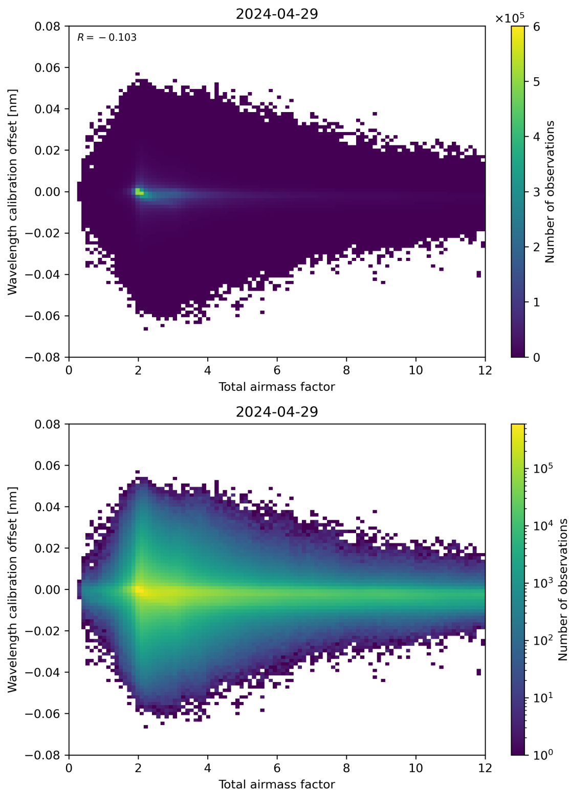
Figure 70: Scatter density plot of “Total airmass factor” against “Wavelength calibration offset” for 2024-04-28 to 2024-04-30.
