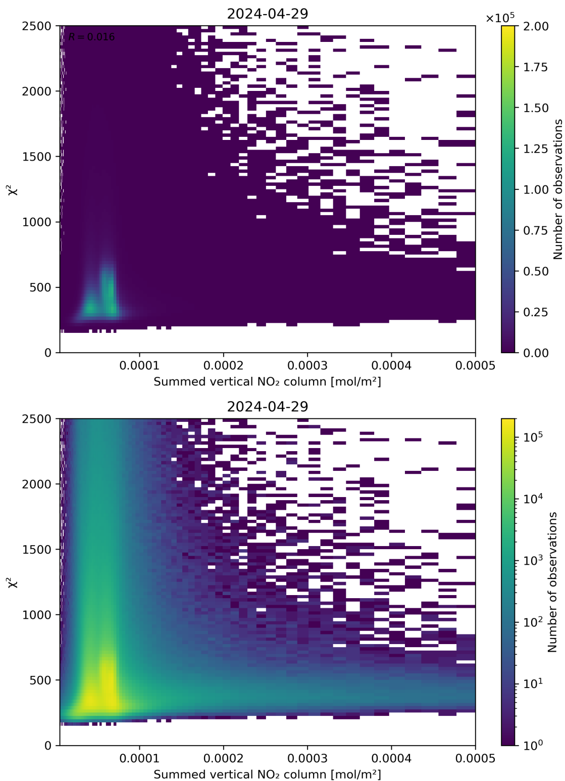
Figure 104: Scatter density plot of “Summed vertical NO 2 column” against “ \chi^2 ” for 2024-04-28 to 2024-04-30.
