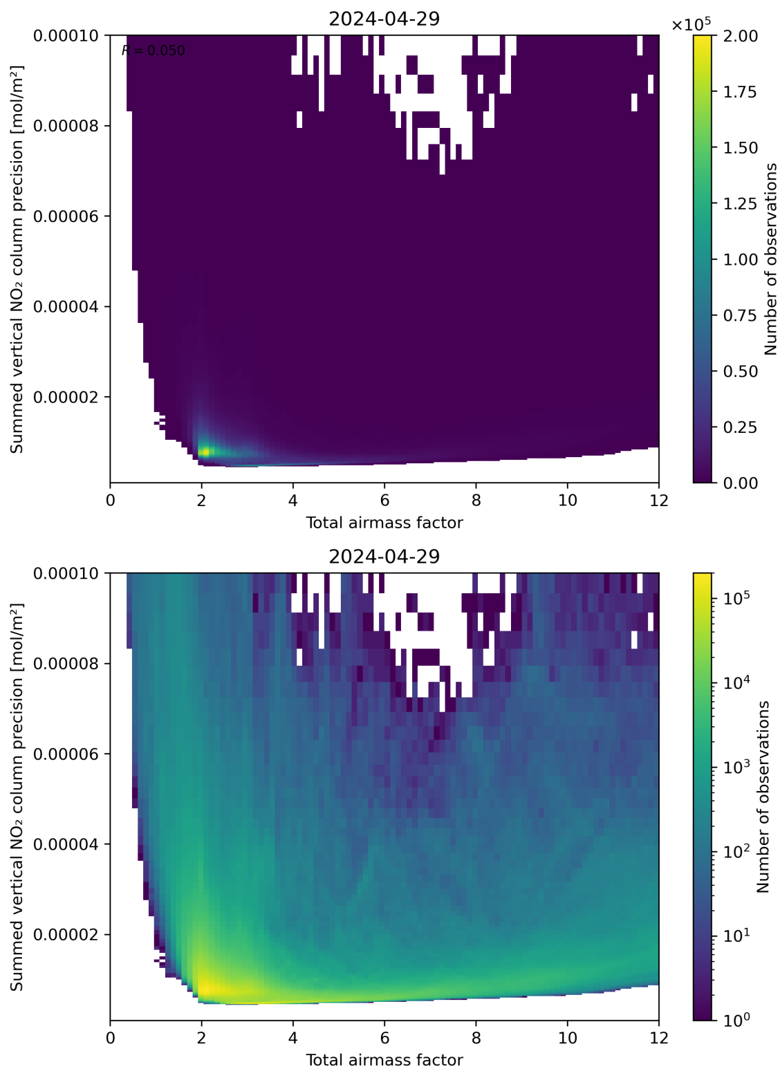
Figure 66: Scatter density plot of “Total airmass factor” against “Summed vertical NO 2 column precision” for 2024-04-28 to 2024-04-30.
