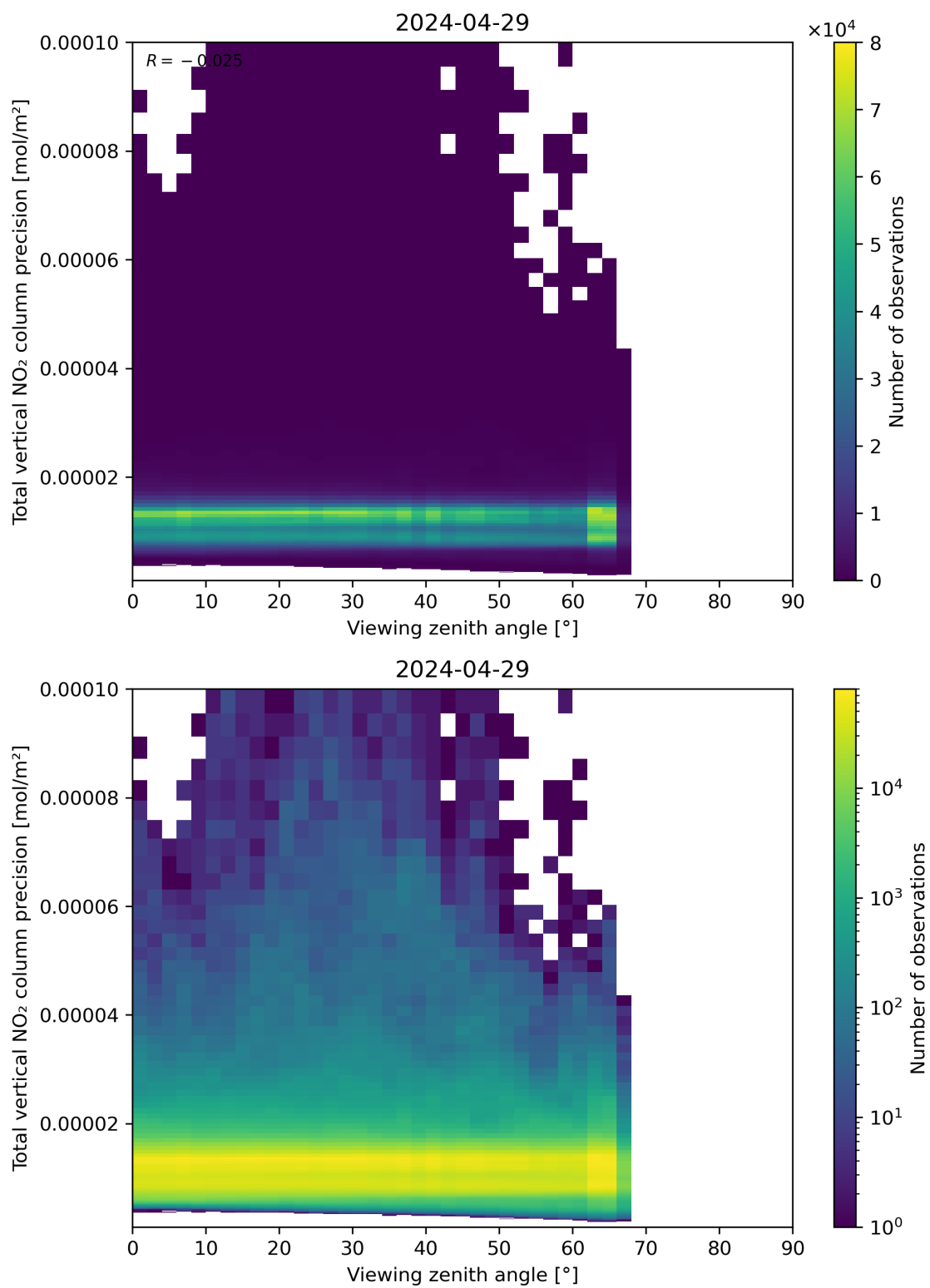
Figure 168: Scatter density plot of “Viewing zenith angle” against “Total vertical NO 2 column precision” for 2024-04-28 to 2024-04-30.
