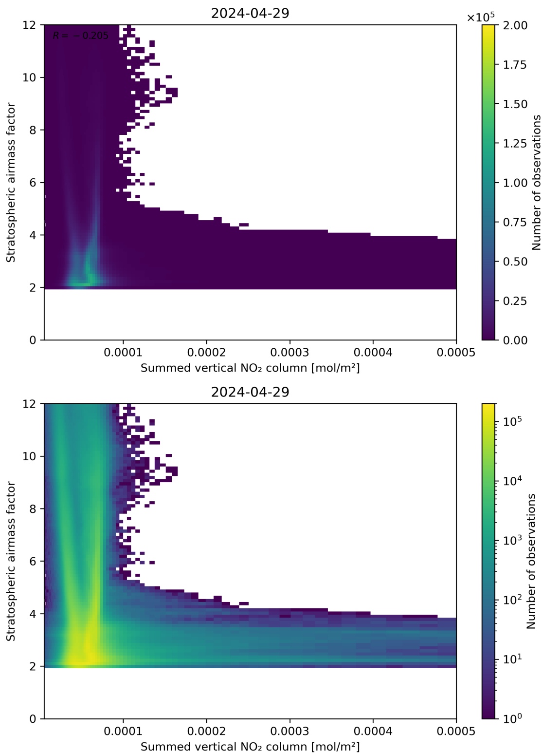
Figure 103: Scatter density plot of “Summed vertical NO 2 column” against “Stratospheric airmass factor” for 2024-04-28 to 2024-04-30.
