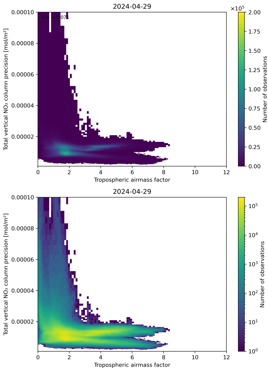
Figure 78: Scatter density plot of “Tropospheric air mass factor” against “Total vertical NO 2 column precision” for 2024-04-28 to 2024-04-30.
