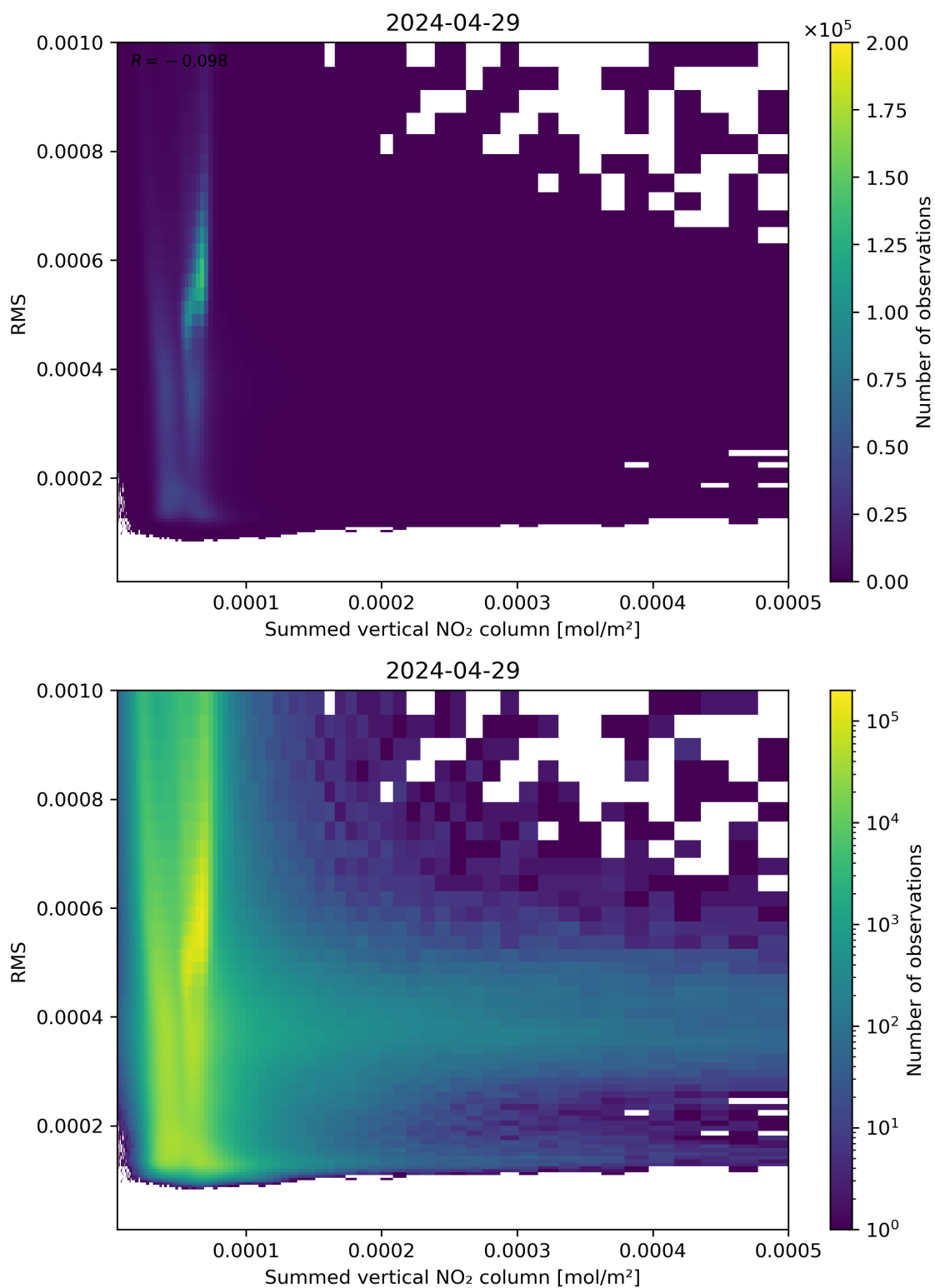
Figure 109: Scatter density plot of “Summed vertical NO 2 column” against “RMS” for 2024-04-28 to 2024-04-30.
