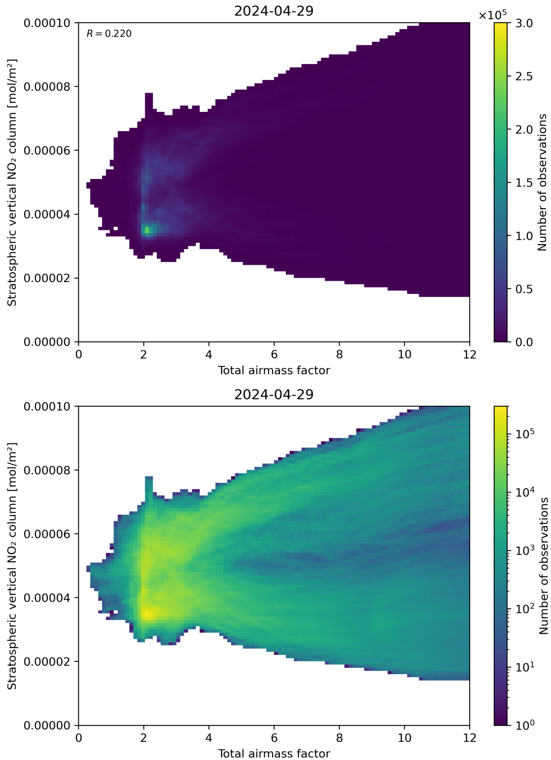
Figure 64: Scatter density plot of “Total airmass factor” against “Stratospheric vertical NO 2 column” for 2024-04-28 to 2024-04-30.
