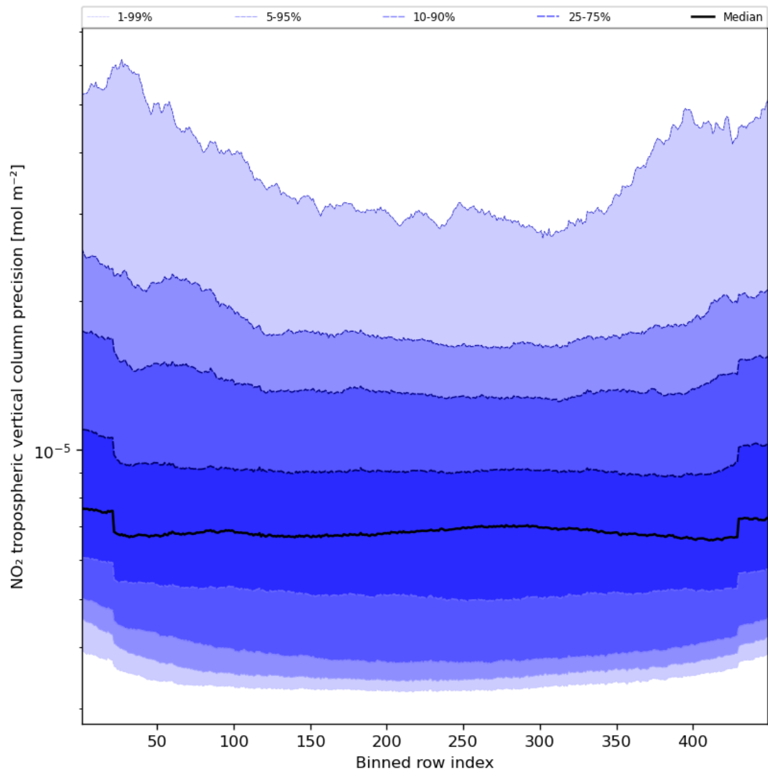
Figure 47: Along track statistics of “NO 2 tropospheric vertical column precision” for 2024-04-28 to 2024-04-30
