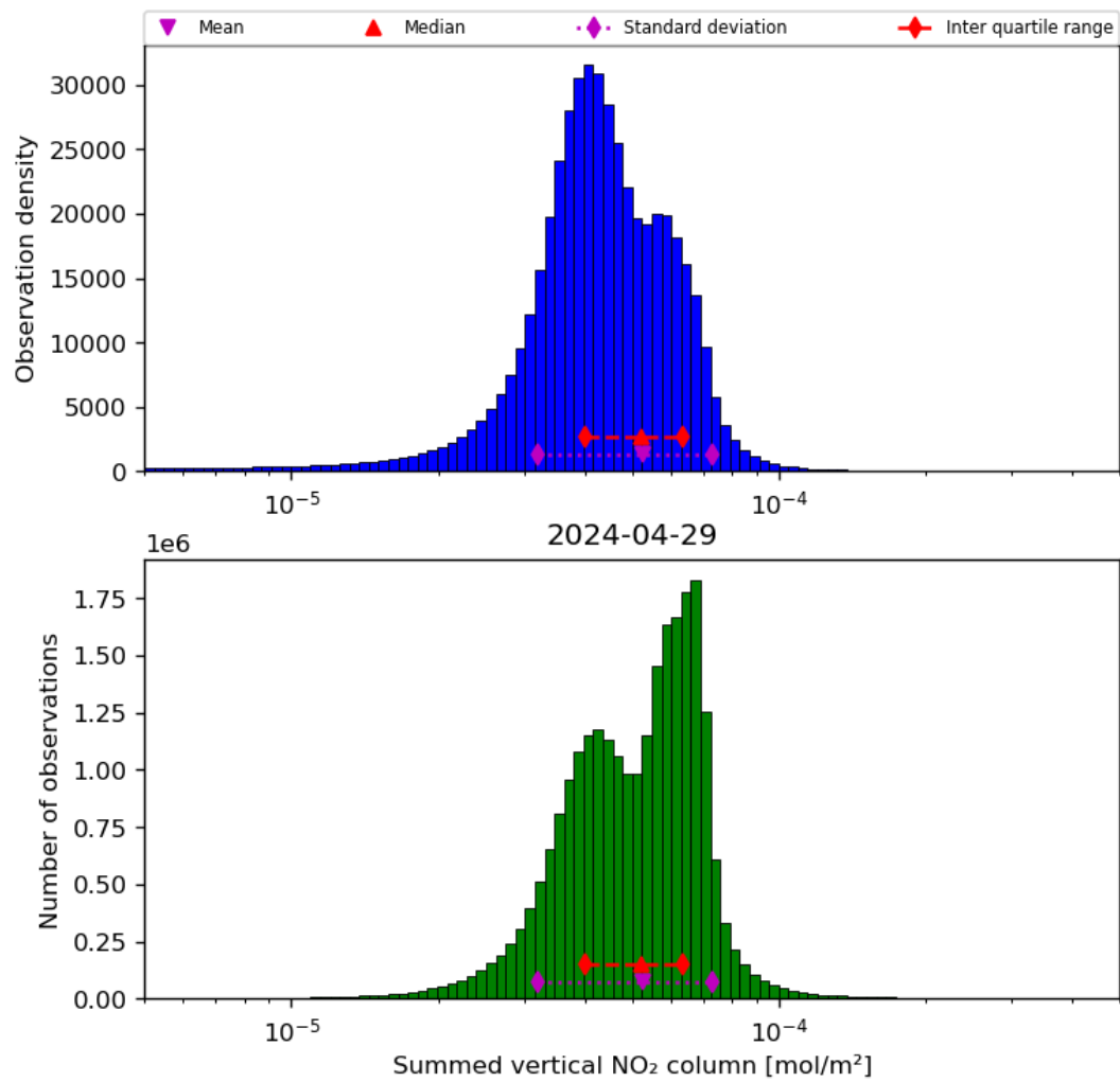
Figure 40: Histogram of “Summed vertical NO 2 column” for 2024-04-28 to 2024-04-30
