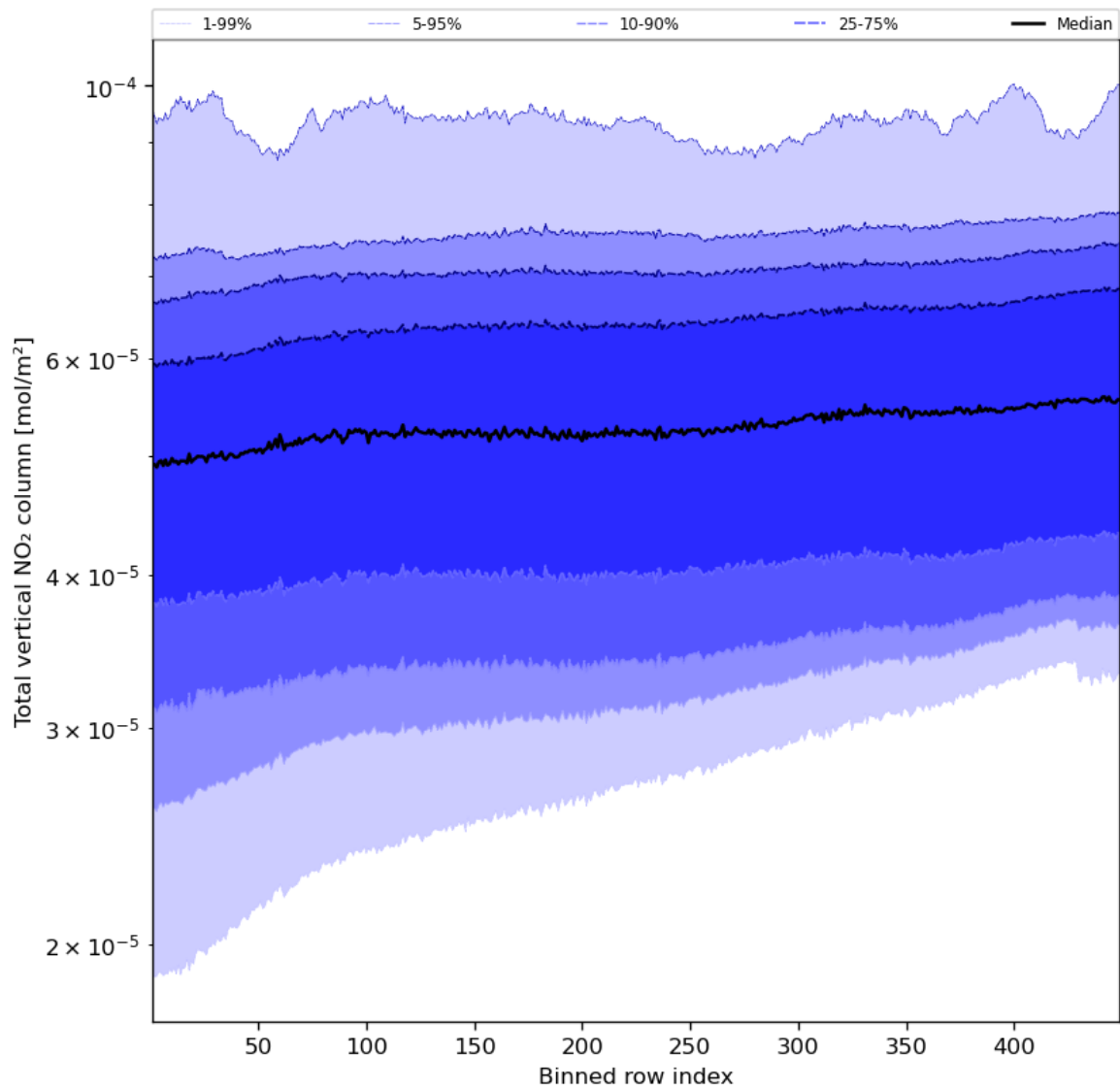
Figure 55: Along track statistics of “Total vertical NO 2 column” for 2024-04-28 to 2024-04-30
