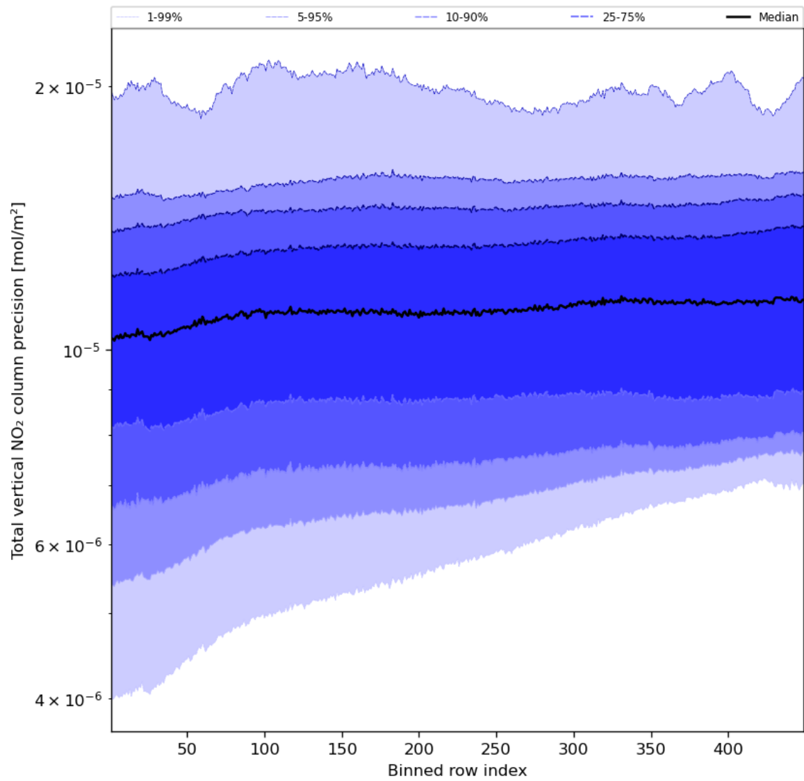
Figure 56: Along track statistics of “Total vertical NO 2 column precision” for 2024-04-28 to 2024-04-30
