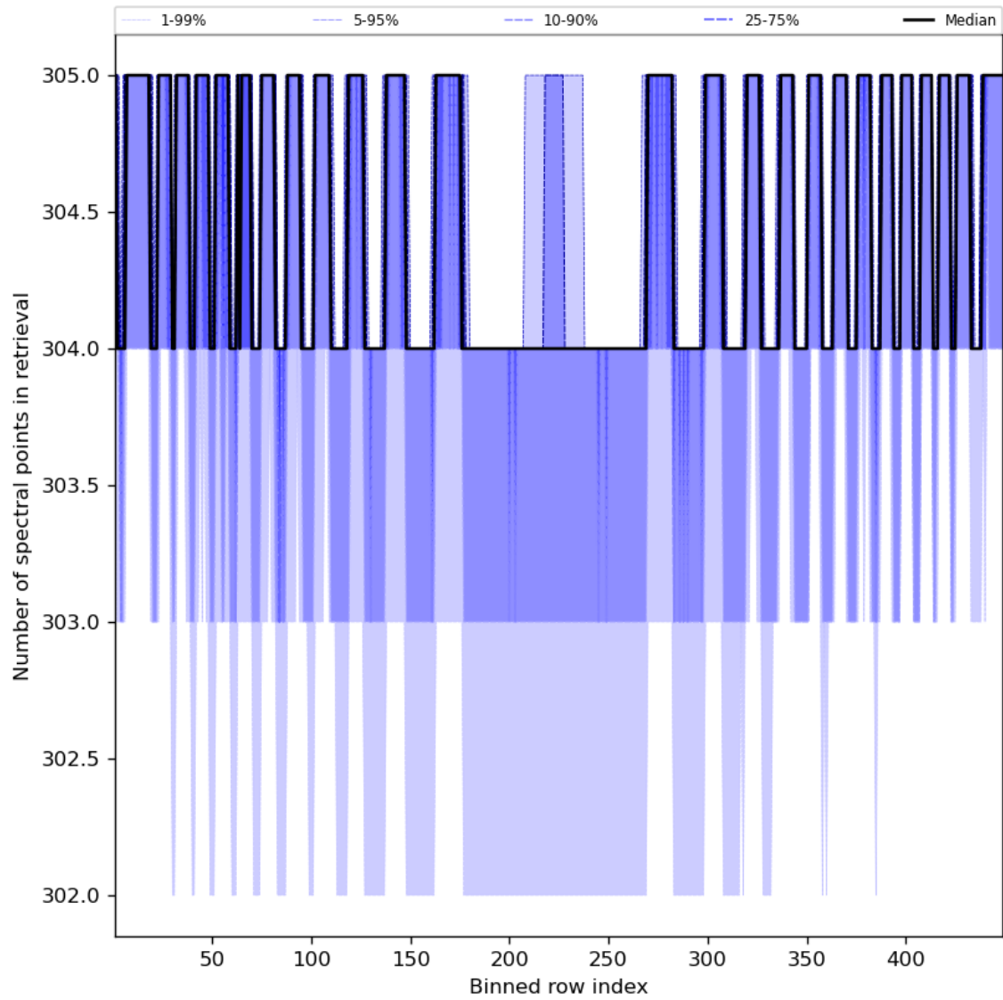
Figure 50: Along track statistics of “Number of spectral points in retrieval” for 2024-04-28 to 2024-04-30
