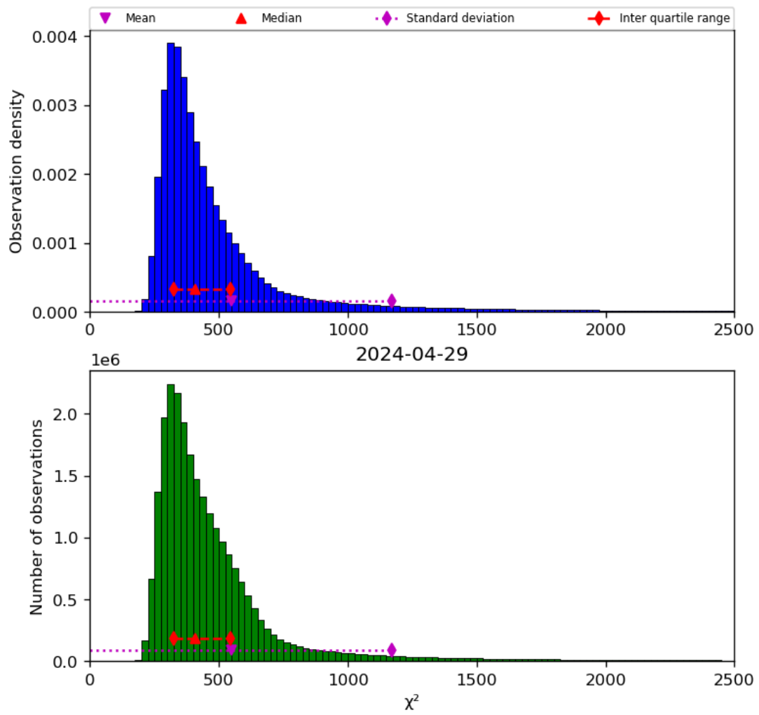
Figure 42: Histogram of “ \chi^2 ” for 2024-04-28 to 2024-04-30
