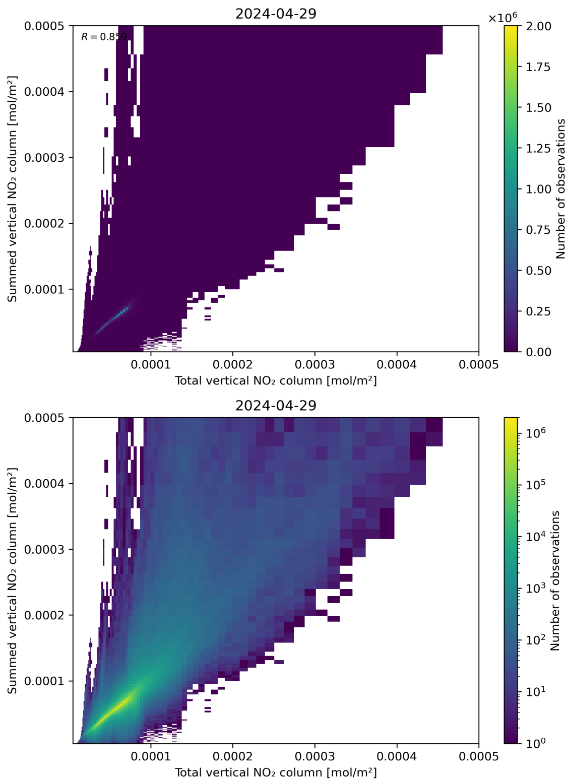
Figure 112: Scatter density plot of “Total vertical NO 2 column” against “Summed vertical NO 2 column” for 2024-04-28 to 2024-04-30.
