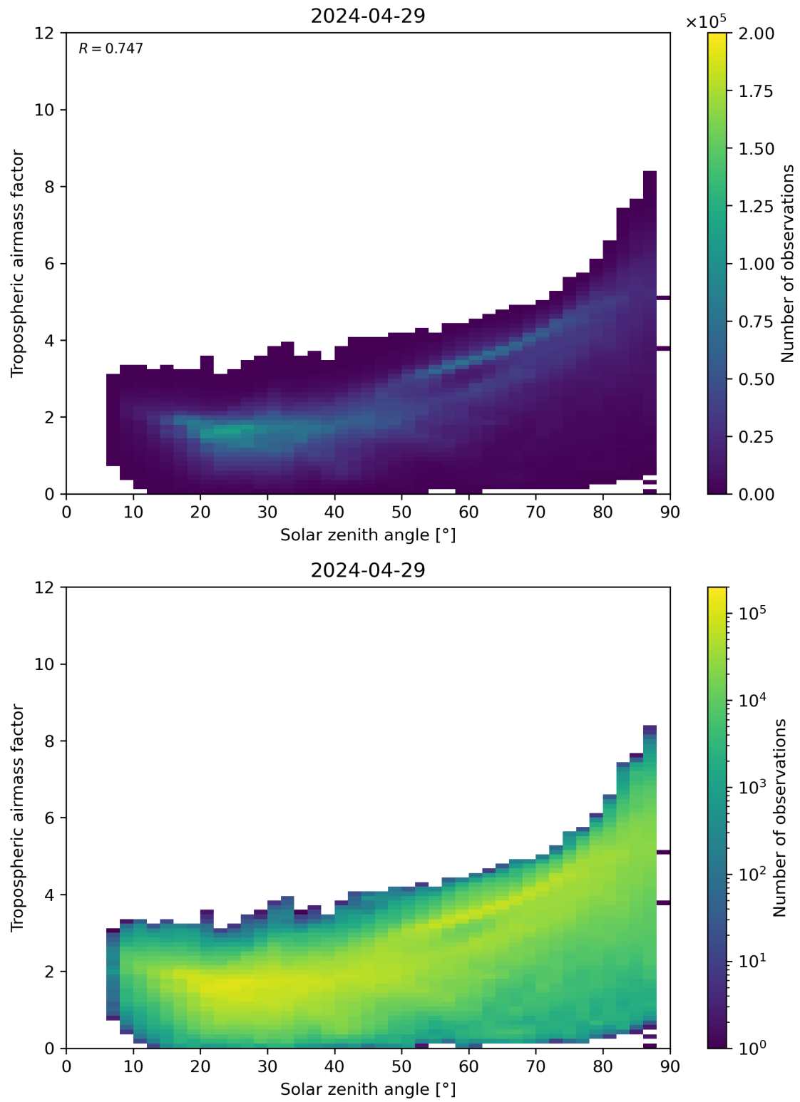
Figure 147: Scatter density plot of “Solar zenith angle” against “Tropospheric airmass factor” for 2024-04-28 to 2024-04-30.
