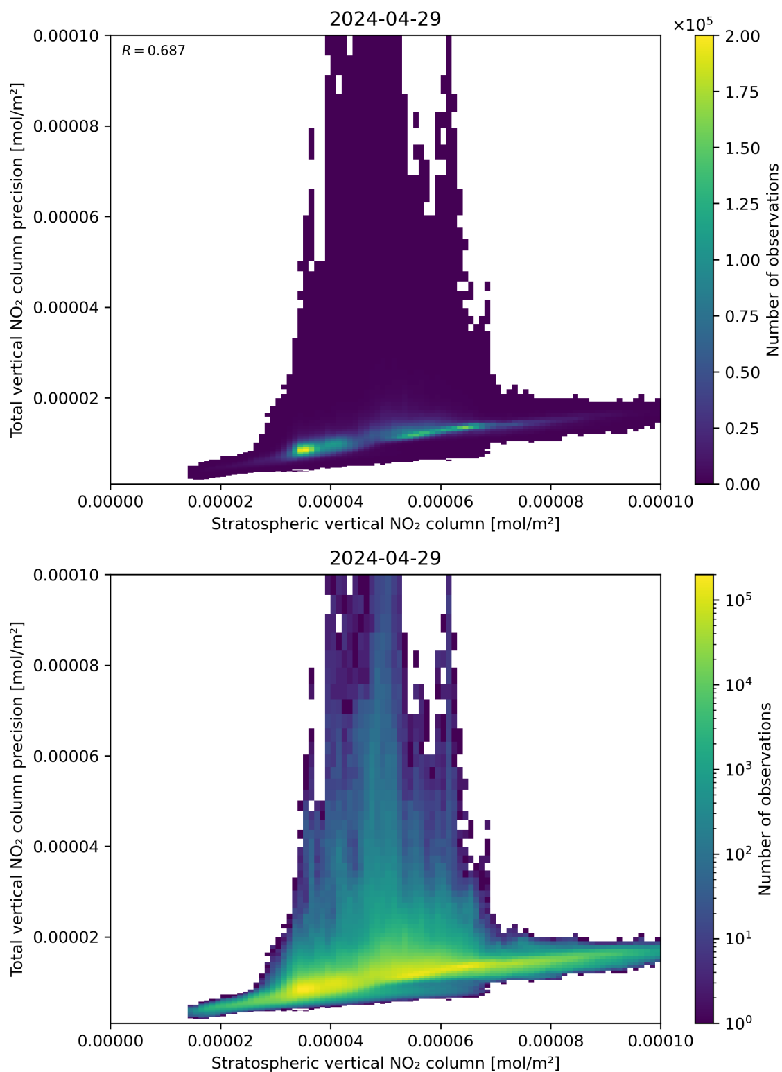
Figure 101: Scatter density plot of “Stratospheric vertical NO 2 column” against “Total vertical NO 2 column precision” for 2024-04-28 to 2024-04-30.
