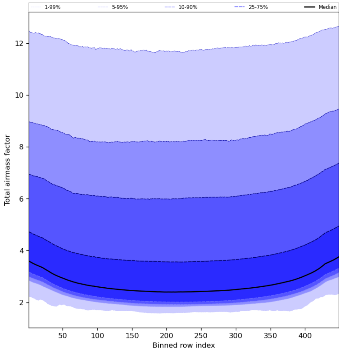
Figure 49: Along track statistics of “Total airmass factor” for 2024-04-28 to 2024-04-30
