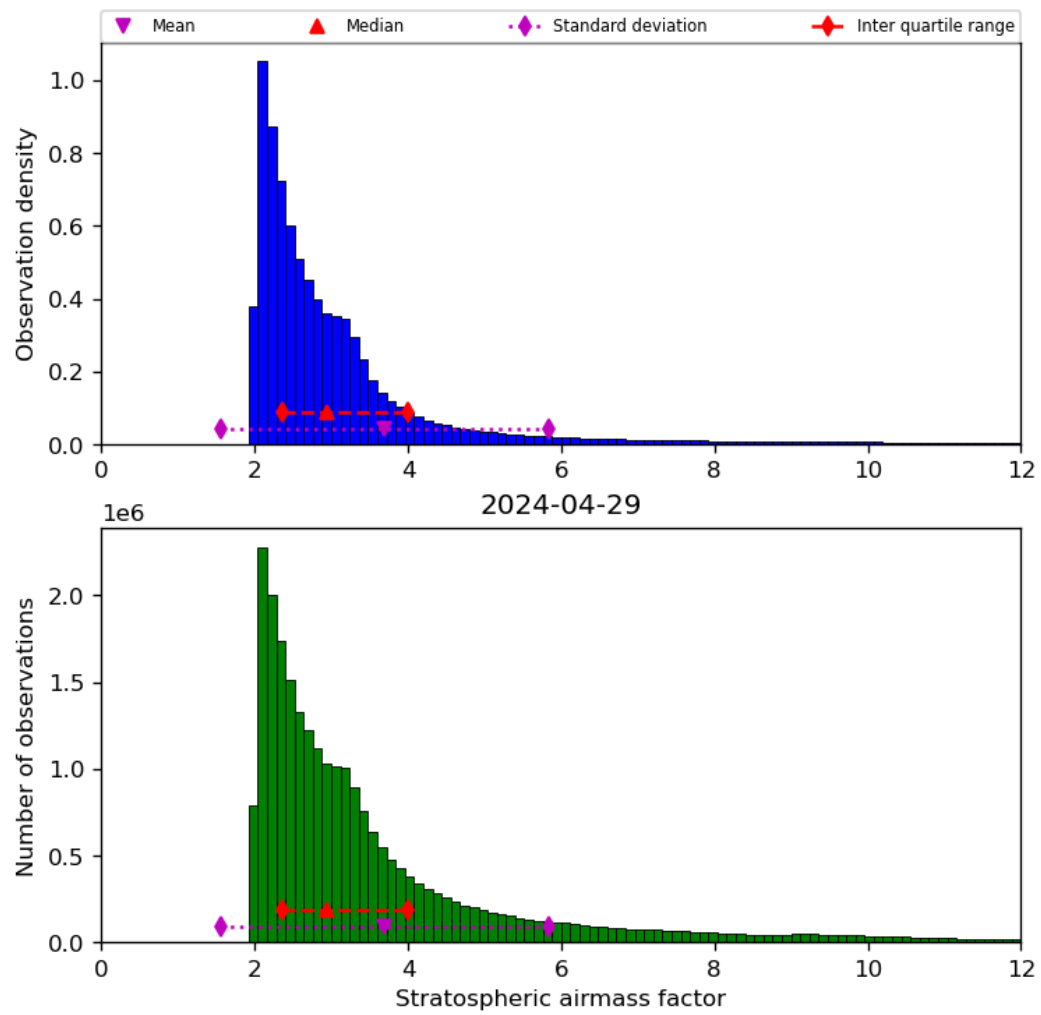
Figure 44: Histogram of “Stratospheric airmass factor” for 2024-04-28 to 2024-04-30
