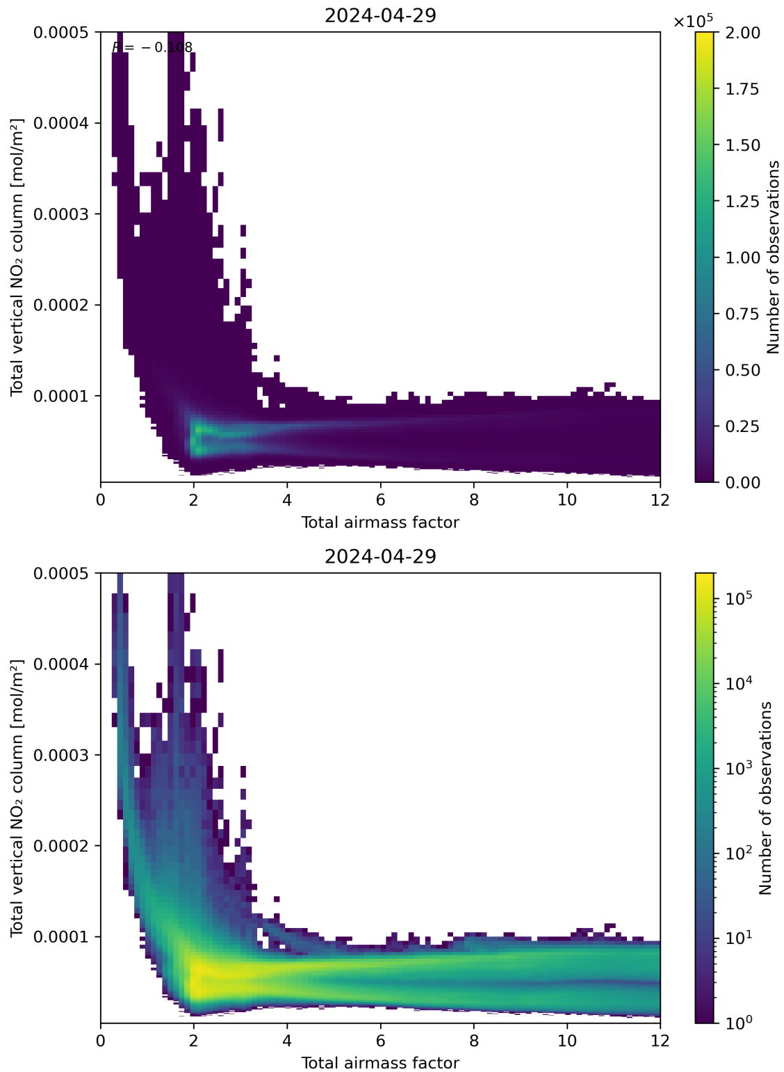
Figure 67: Scatter density plot of “Total airmass factor” against “Total vertical NO 2 column” for 2024-04-28 to 2024-04-30.
