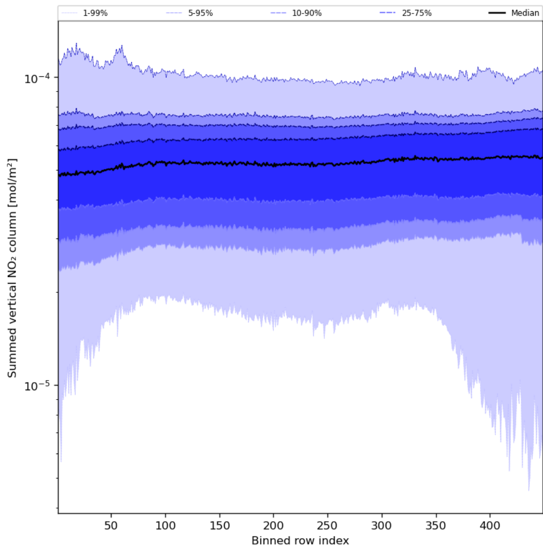
Figure 57: Along track statistics of “Summed vertical NO 2 column” for 2024-04-28 to 2024-04-30
