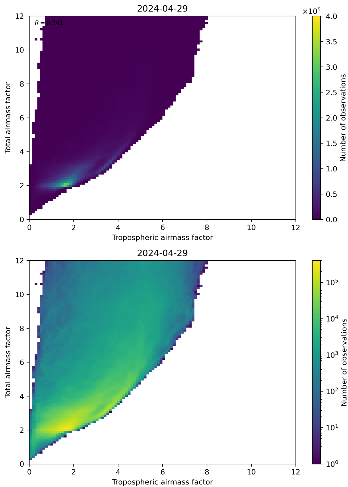
Figure 72: Scatter density plot of “Tropospheric airmass factor” against “Total airmass factor” for 2024-04-28 to 2024-04-30.
