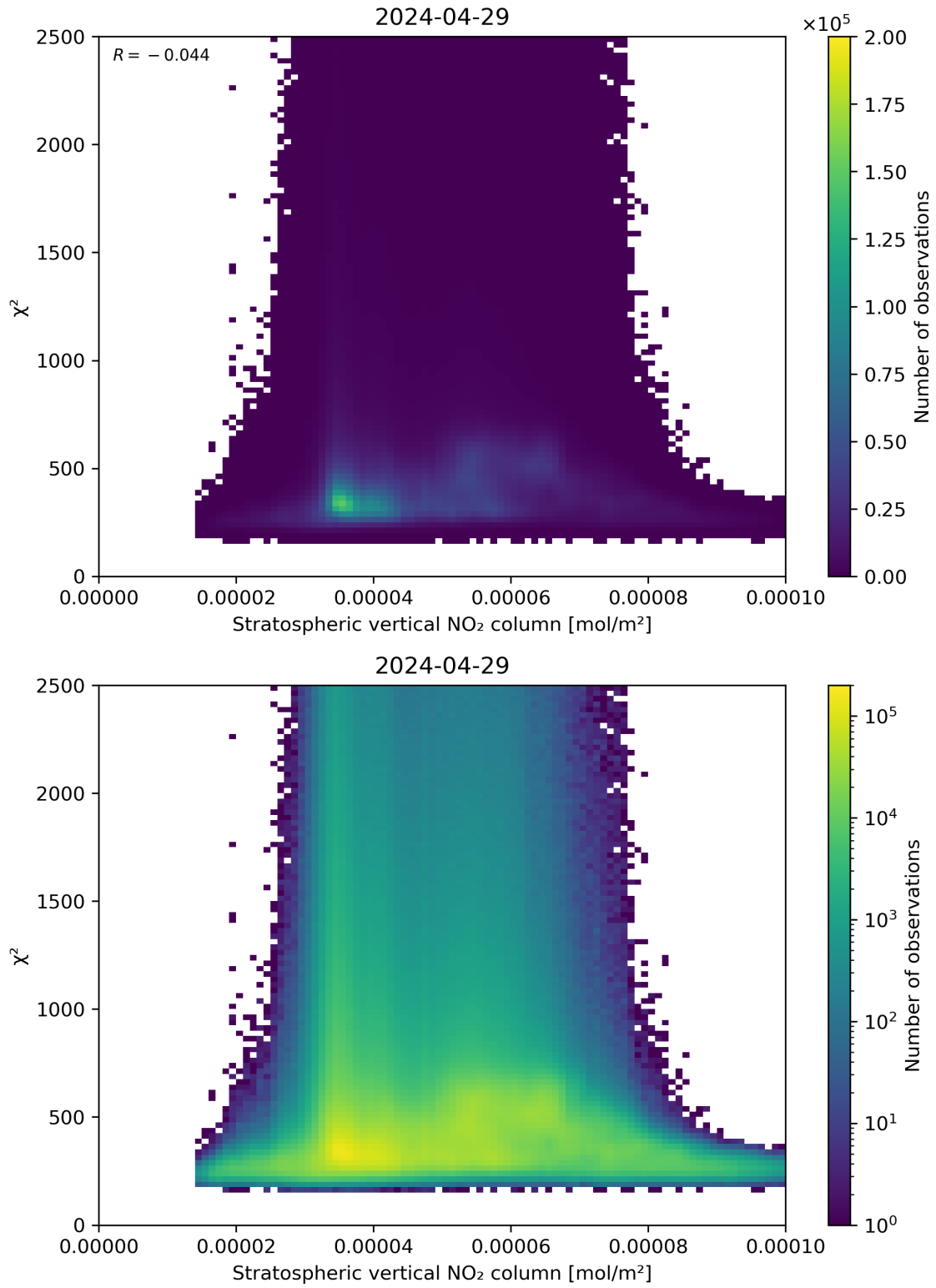
Figure 97: Scatter density plot of “Stratospheric vertical NO 2 column” against “ \chi^2 ” for 2024-04-28 to 2024-04-30.
