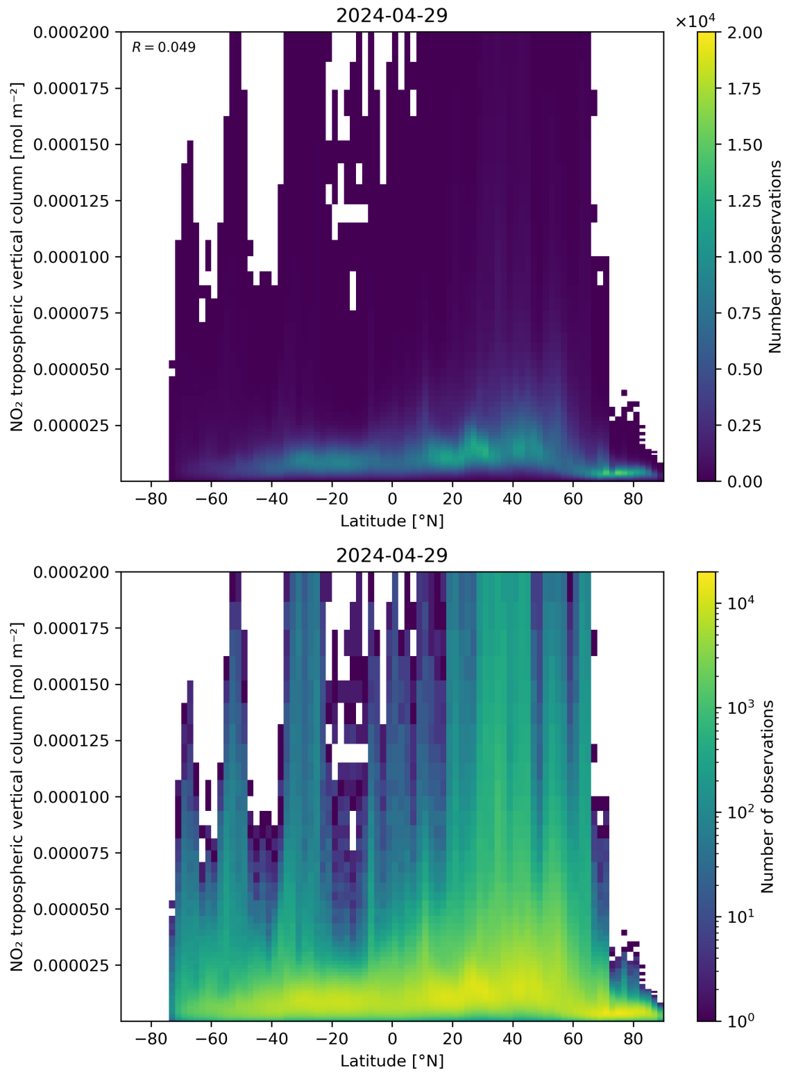
Figure 92: Scatter density plot of “Latitude” against “NO 2 tropospheric vertical column” for 2024-04-28 to 2024-04-30.
