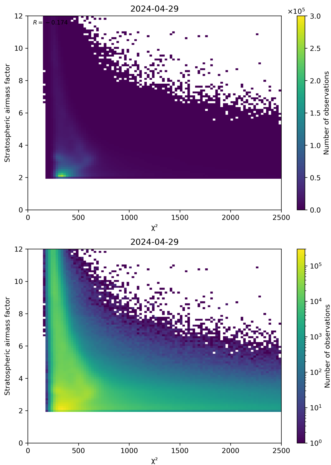
Figure 81: Scatter density plot of “ \chi^2 ” against “Stratospheric airmass factor” for 2024-04-28 to 2024-04-30.
