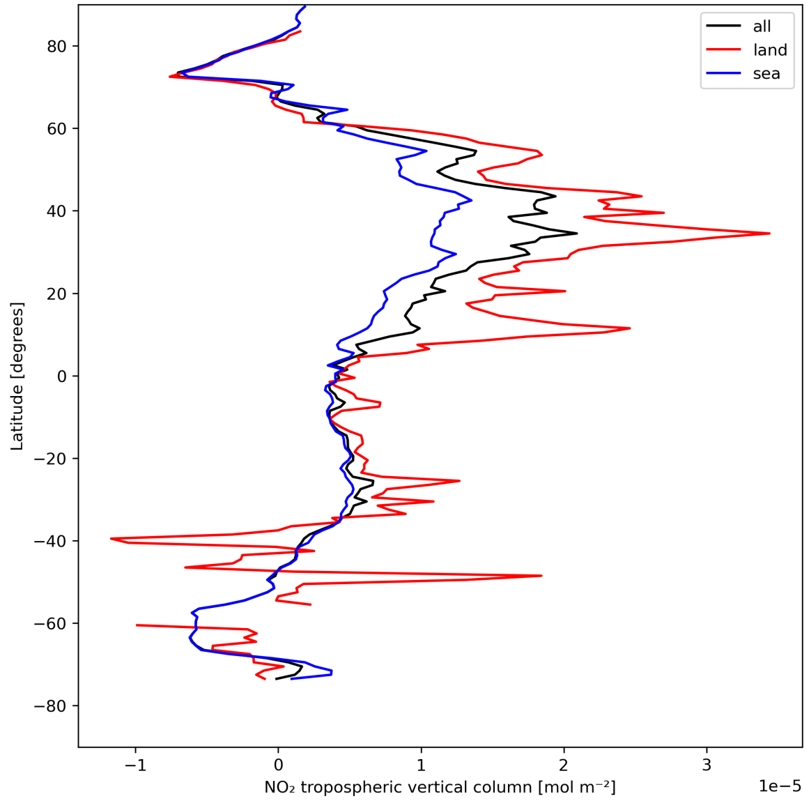
Figure 12: Zonal average of “NO 2 tropospheric vertical column” for 2024-04-28 to 2024-04-30.
