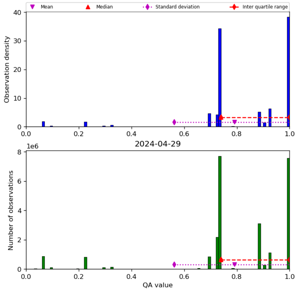
Figure 28: Histogram of “QA value” for 2024-04-28 to 2024-04-30
