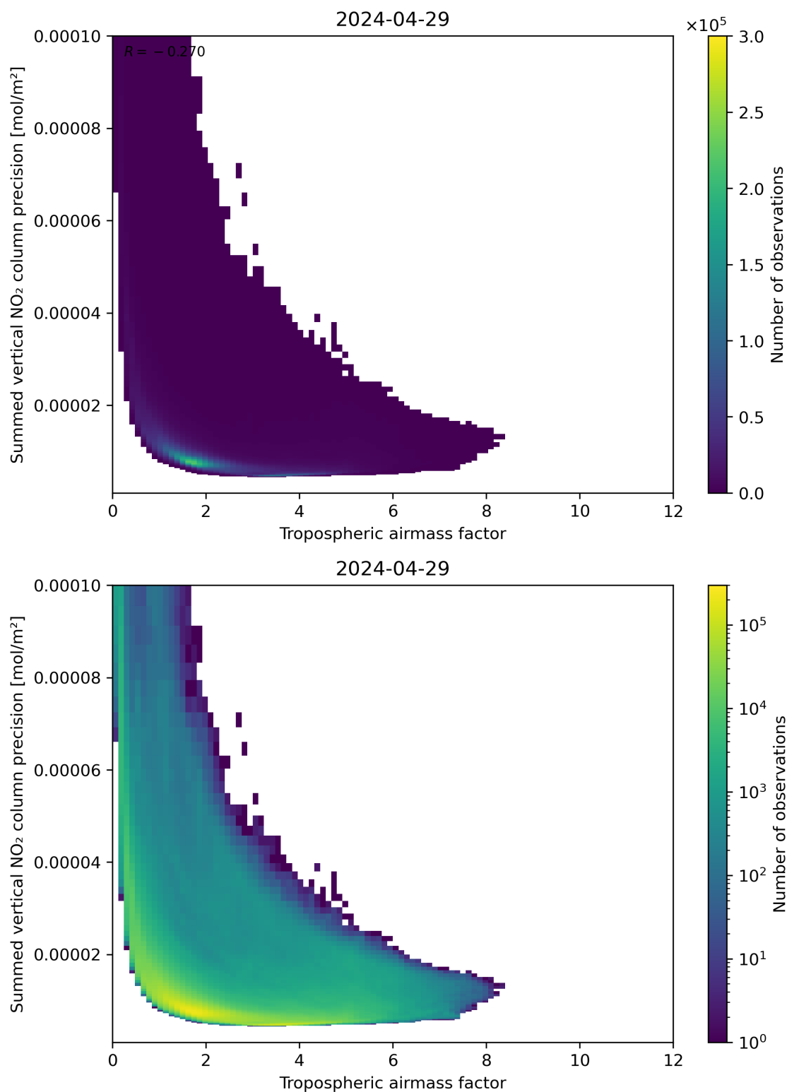
Figure 76: Scatter density plot of “Tropospheric air mass factor” against “Summed vertical NO 2 column precision” for 2024-04-28 to 2024-04-30.
