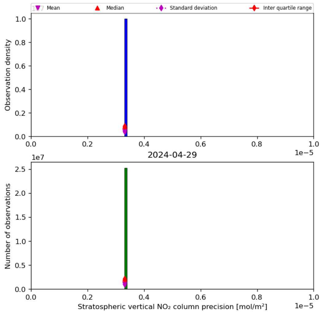
Figure 37: Histogram of “Stratospheric vertical NO 2 column precision” for 2024-04-28 to 2024-04-30
