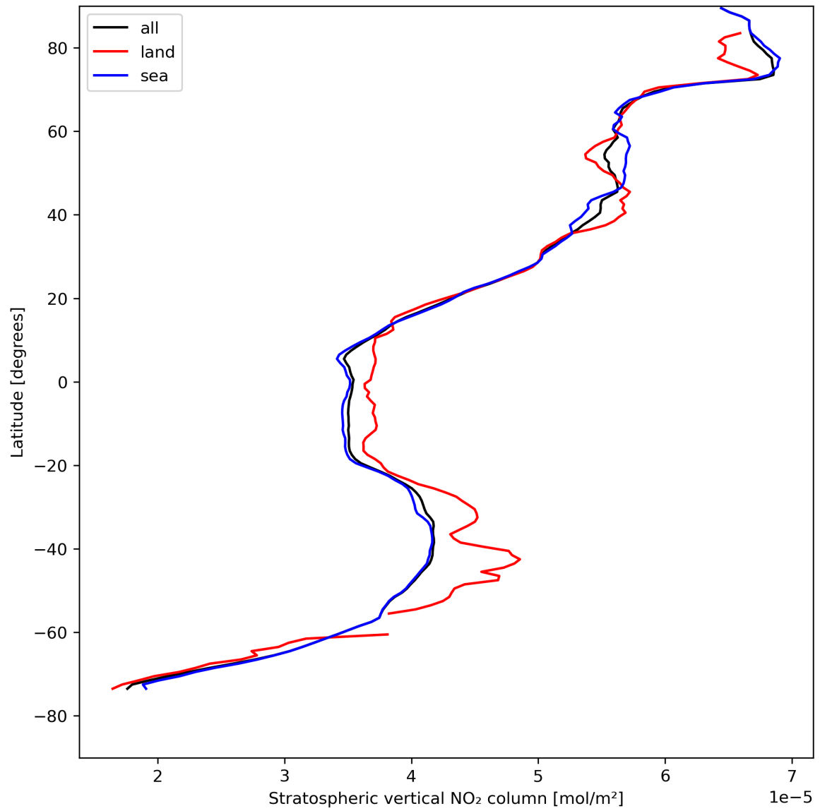
Figure 19: Zonal average of “Stratospheric vertical NO 2 column” for 2024-04-28 to 2024-04-30.
