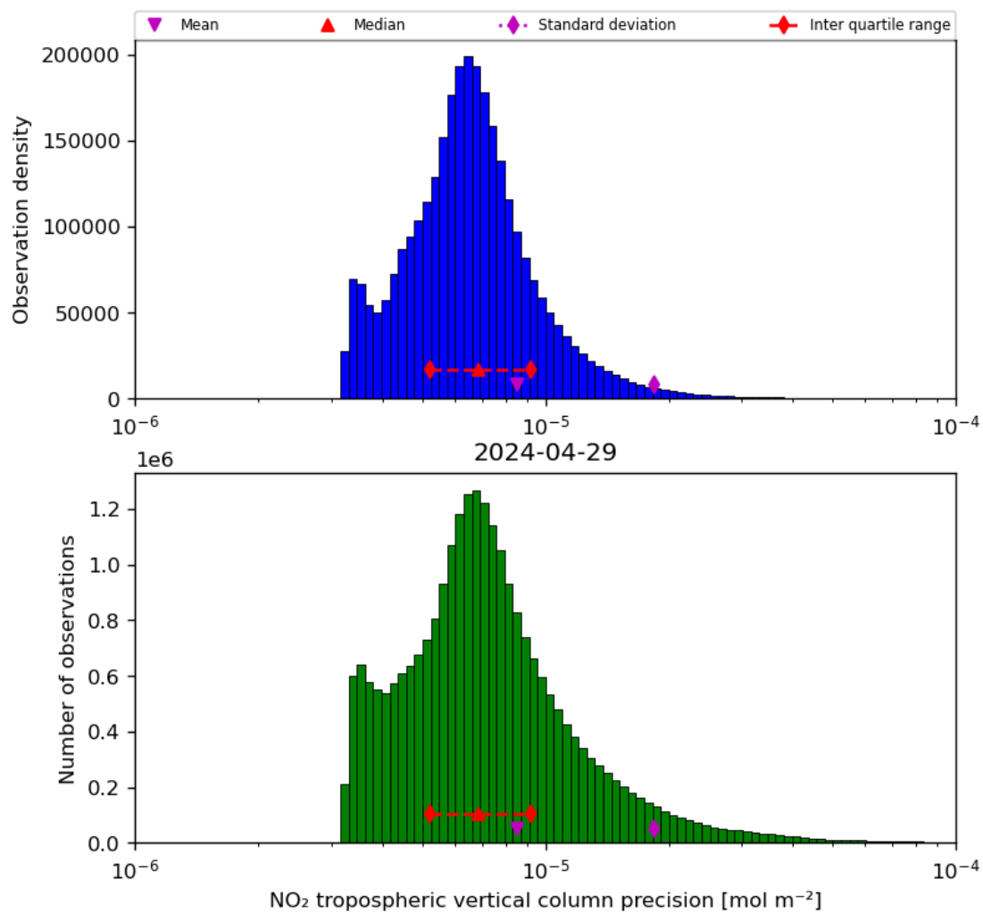
Figure 30: Histogram of “NO 2 tropospheric vertical column precision” for 2024-04-28 to 2024-04-30
