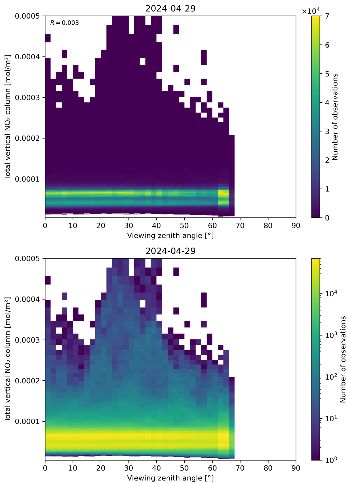
Figure 167: Scatter density plot of “Viewing zenith angle” against “Total vertical NO 2 column” for 2024-04-28 to 2024-04-30.
