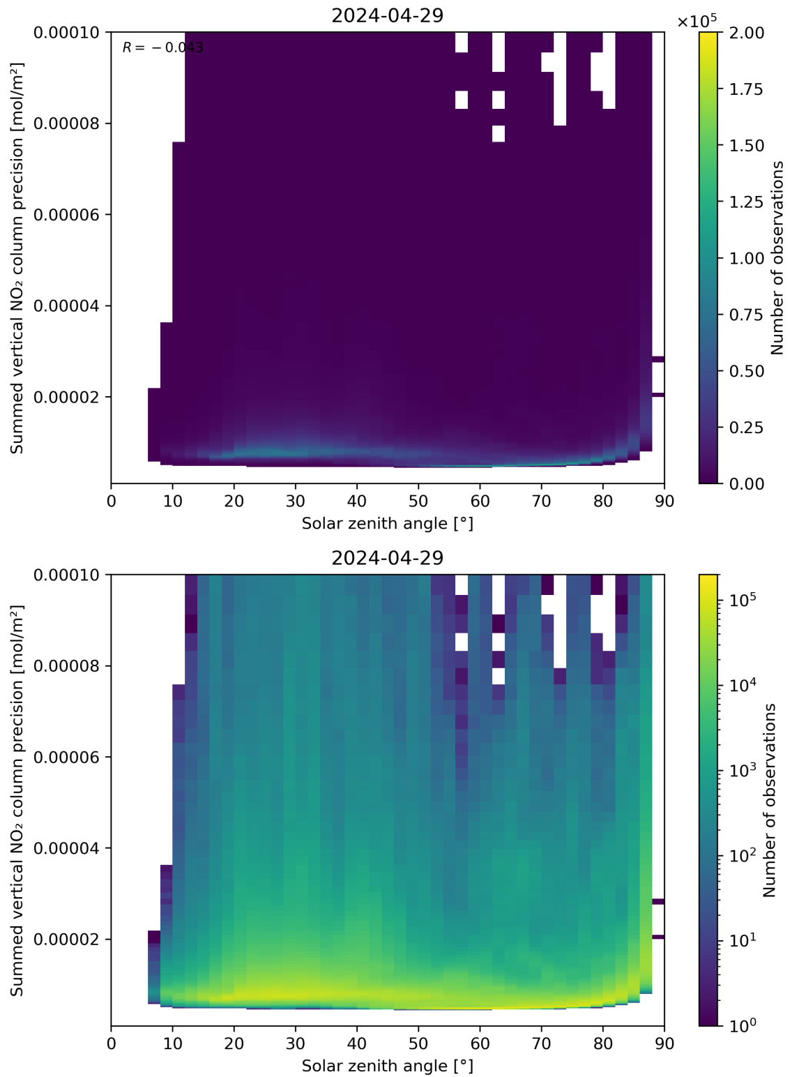
Figure 152: Scatter density plot of “Solar zenith angle” against “Summed vertical NO 2 column precision” for 2024-04-28 to 2024-04-30.
