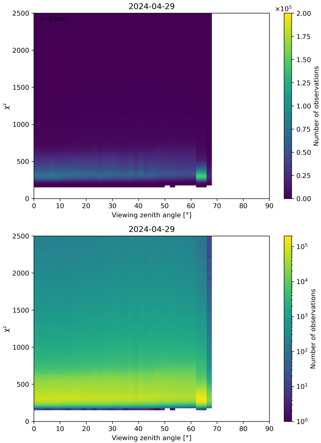
Figure 162: Scatter density plot of “Viewing zenith angle” against “ \chi^2 ” for 2024-04-28 to 2024-04-30.
