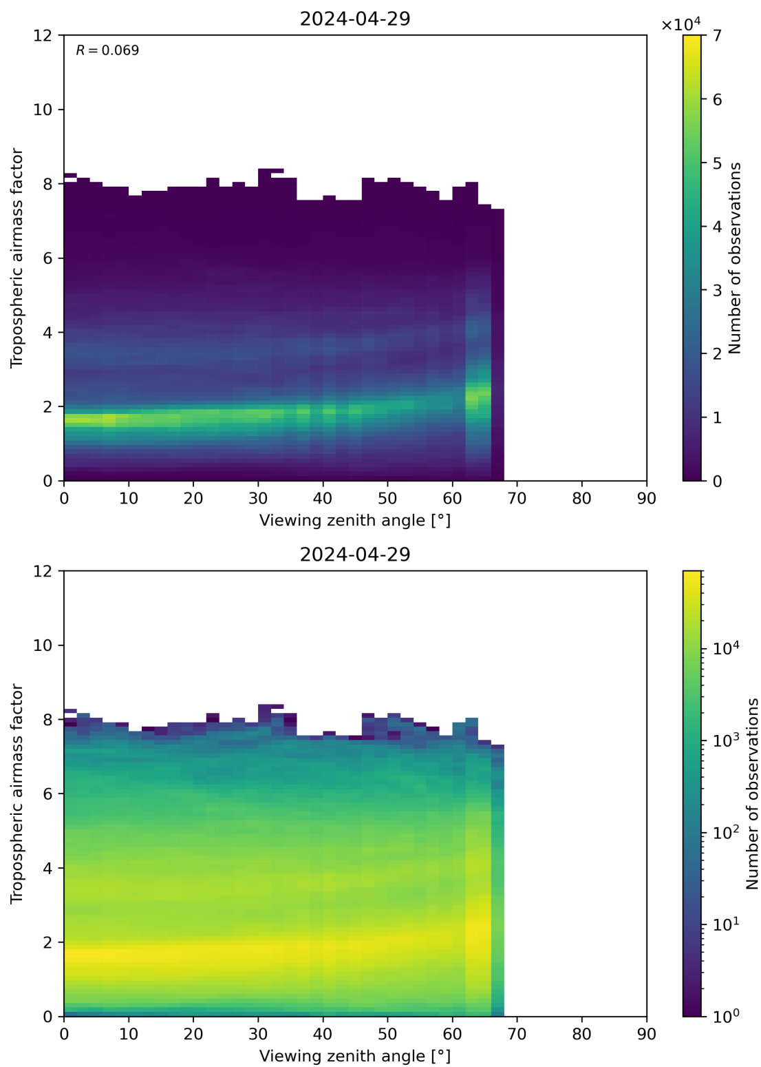
Figure 161: Scatter density plot of “Viewing zenith angle” against “Tropospheric airmass factor” for 2024-04-28 to 2024-04-30.
