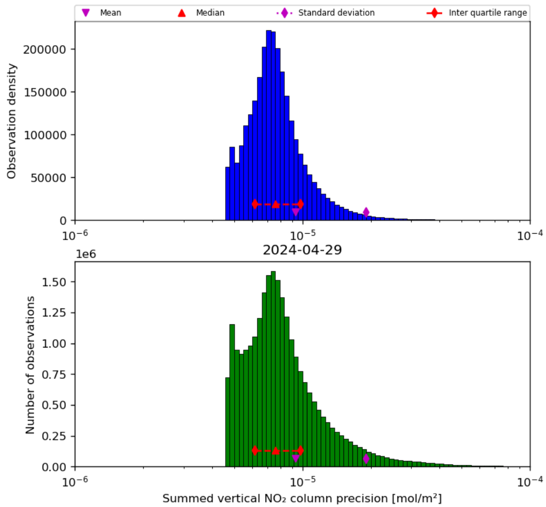
Figure 41: Histogram of “Summed vertical NO 2 column precision” for 2024-04-28 to 2024-04-30
