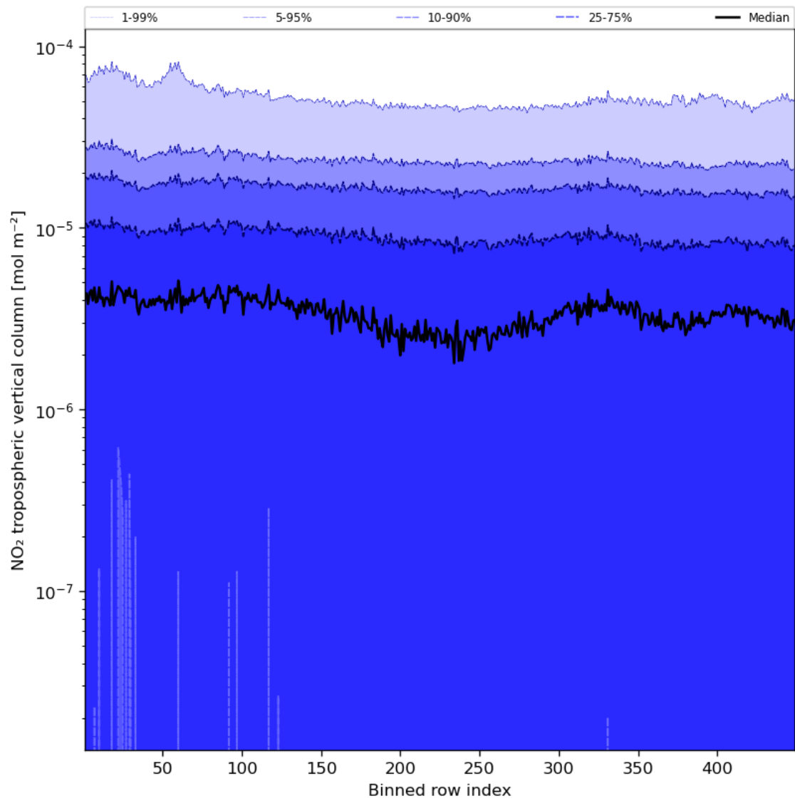
Figure 46: Along track statistics of “NO 2 tropospheric vertical column” for 2024-04-28 to 2024-04-30
