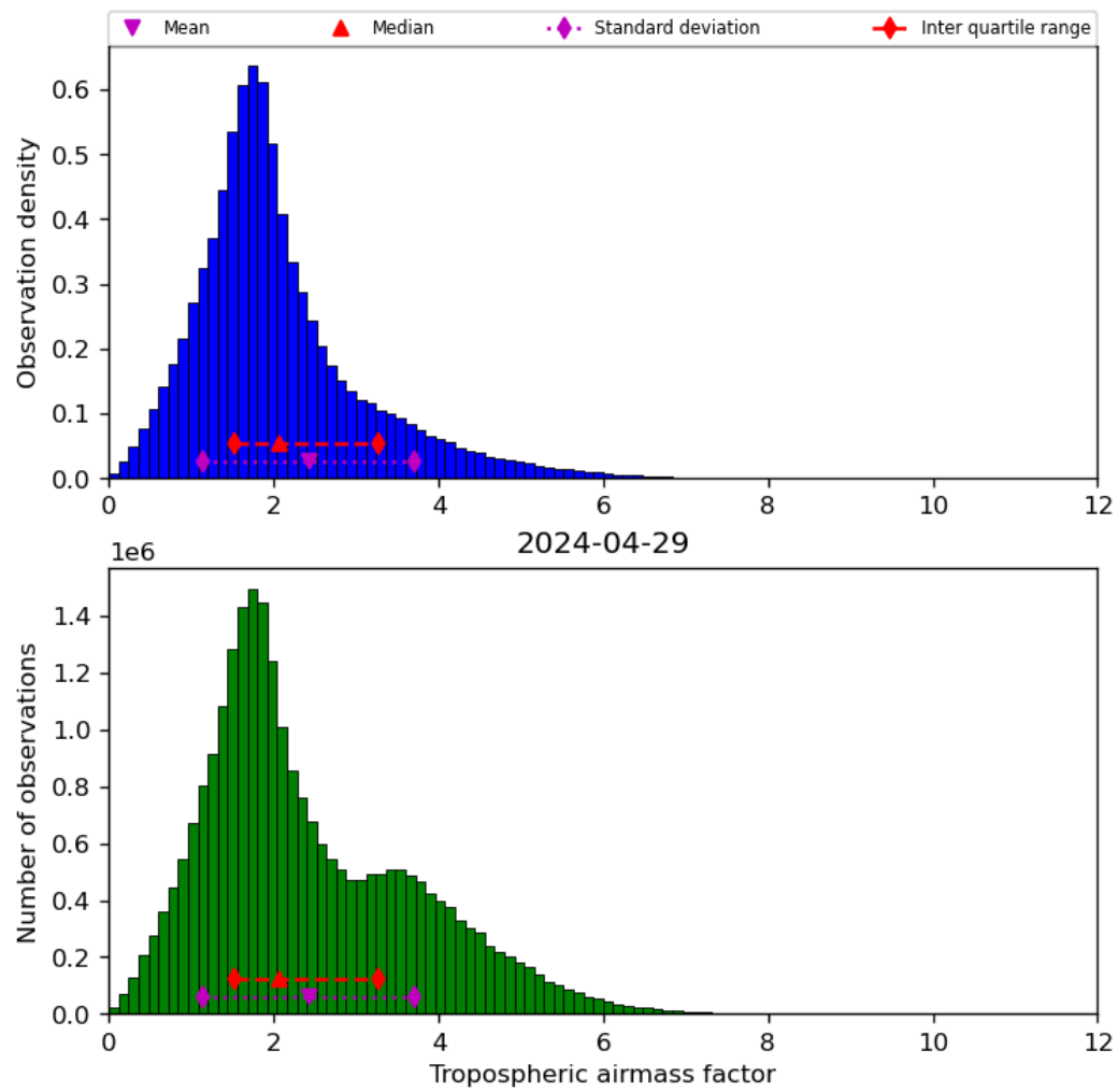
Figure 31: Histogram of “Tropospheric airmass factor” for 2024-04-28 to 2024-04-30
