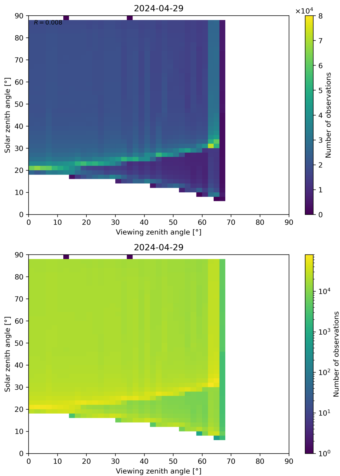
Figure 172: Scatter density plot of “Viewing zenith angle” against “Solar zenith angle” for 2024-04-28 to 2024-04-30.
