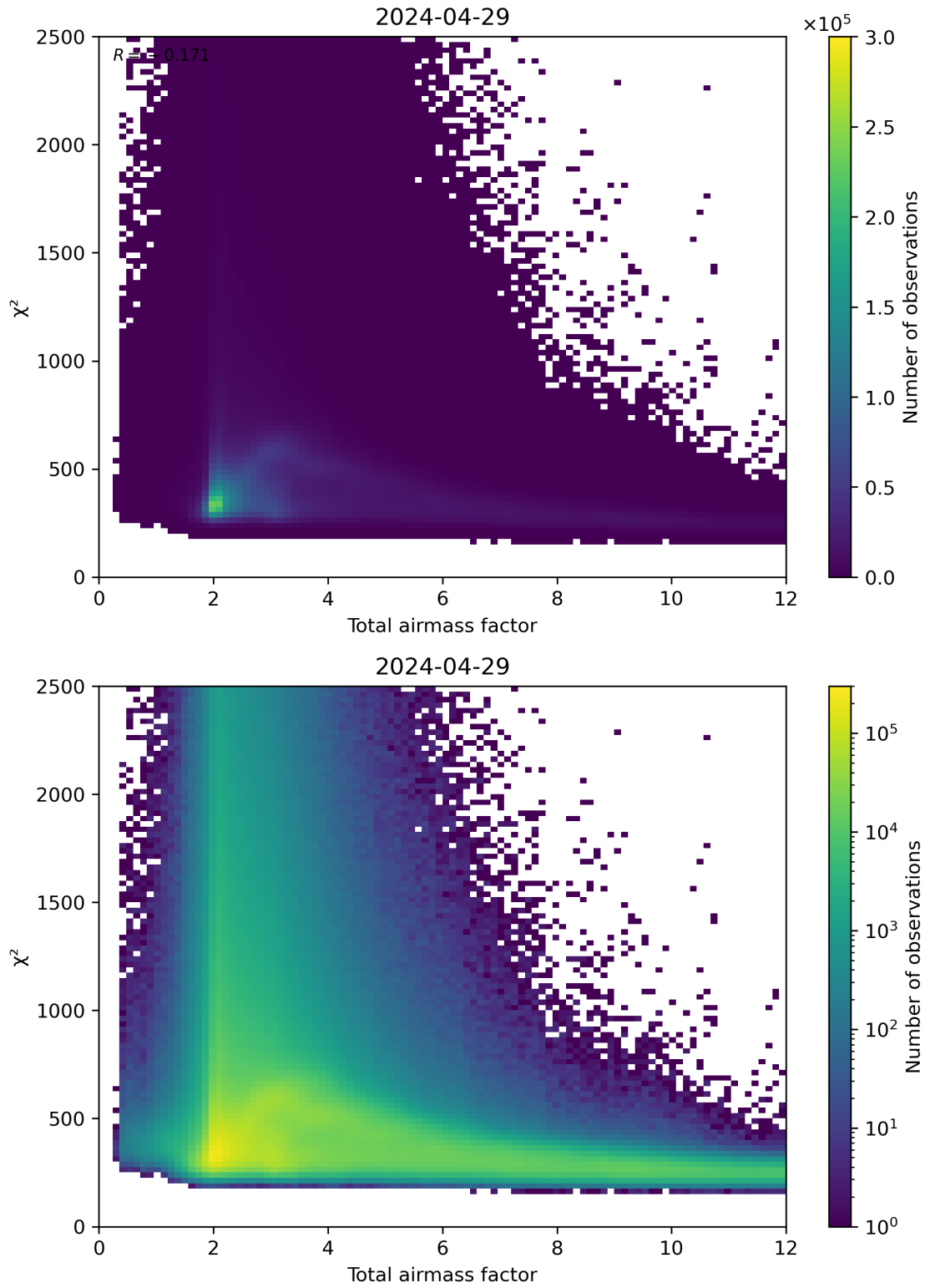
Figure 63: Scatter density plot of “Total airmass factor” against “ \chi^2 ” for 2024-04-28 to 2024-04-30.
