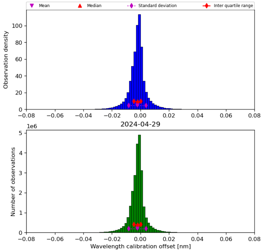
Figure 35: Histogram of “Wavelength calibration offset” for 2024-04-28 to 2024-04-30
