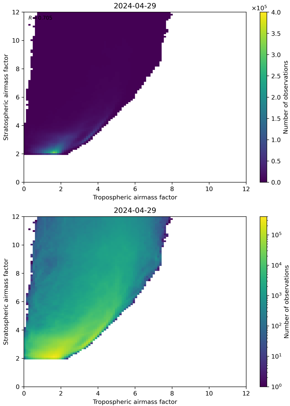
Figure 71: Scatter density plot of “Tropospheric airmass factor” against “Stratospheric airmass factor” for 2024-04-28 to 2024-04-30.
