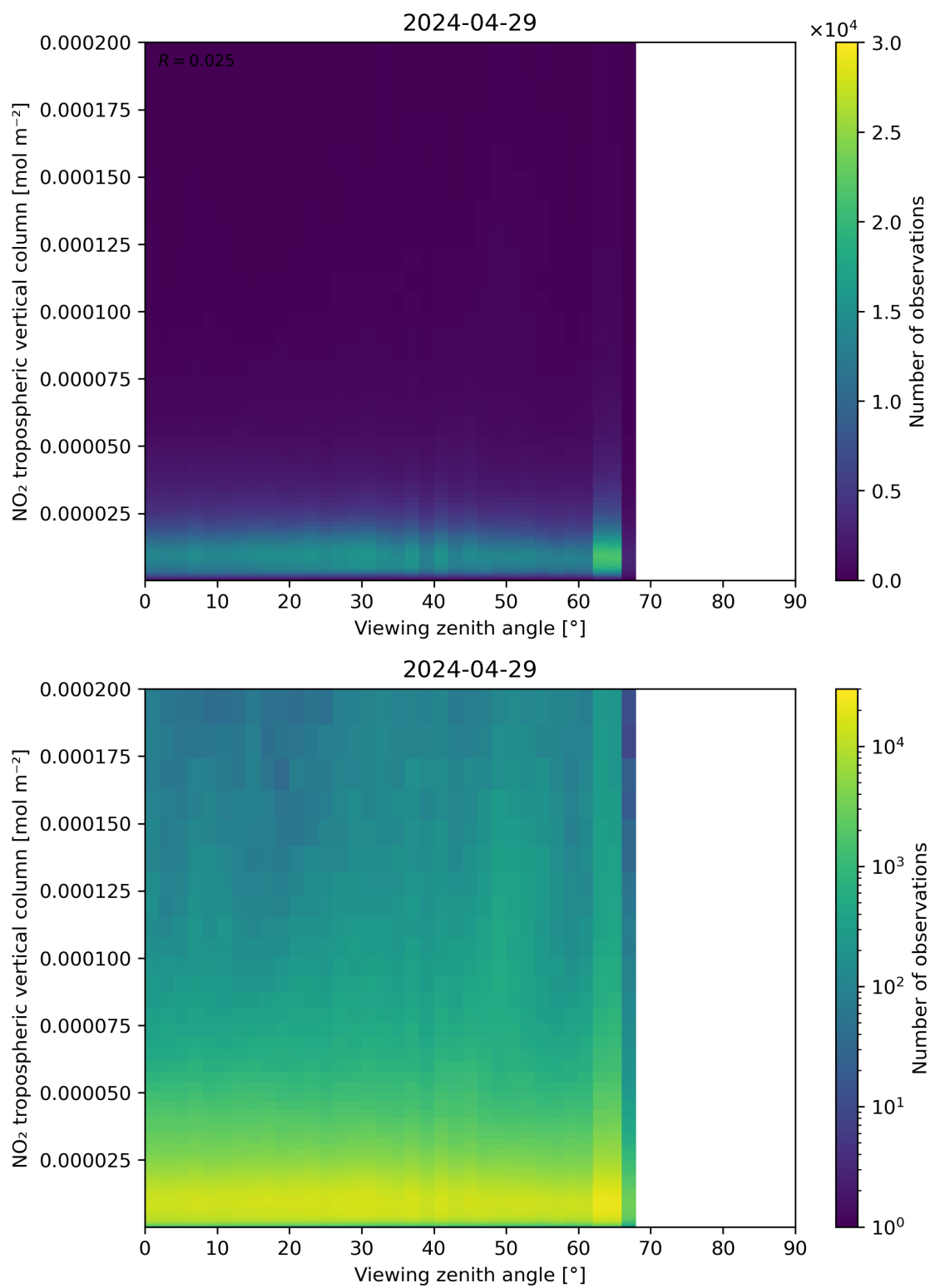
Figure 169: Scatter density plot of “Viewing zenith angle” against “NO 2 tropospheric vertical column” for 2024-04-28 to 2024-04-30.
