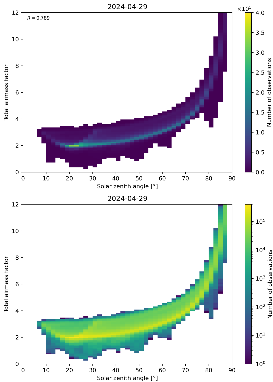
Figure 146: Scatter density plot of “Solar zenith angle” against “Total airmass factor” for 2024-04-28 to 2024-04-30.
