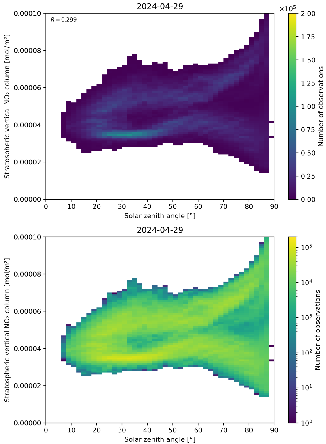
Figure 150: Scatter density plot of “Solar zenith angle” against “Stratospheric vertical NO 2 column” for 2024-04-28 to 2024-04-30.
