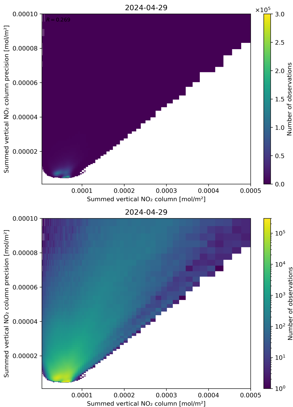
Figure 105: Scatter density plot of “Summed vertical NO 2 column” against “Summed vertical NO 2 column precision” for 2024-04-28 to 2024-04-30.
