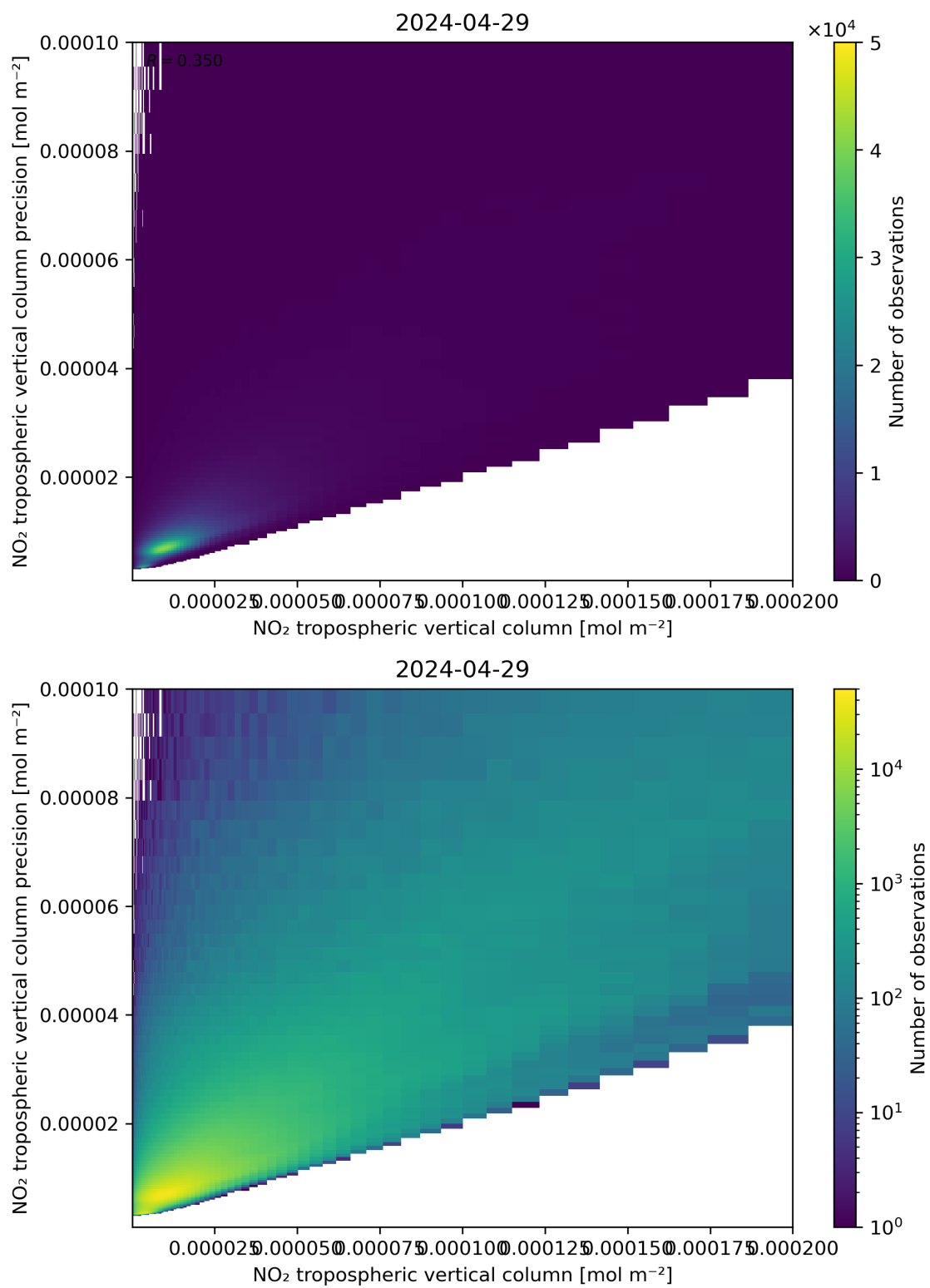
Figure 130: Scatter density plot of “NO 2 tropospheric vertical column” against “NO 2 tropospheric vertical column precision” for 2024-04-28 to 2024-04-30.
