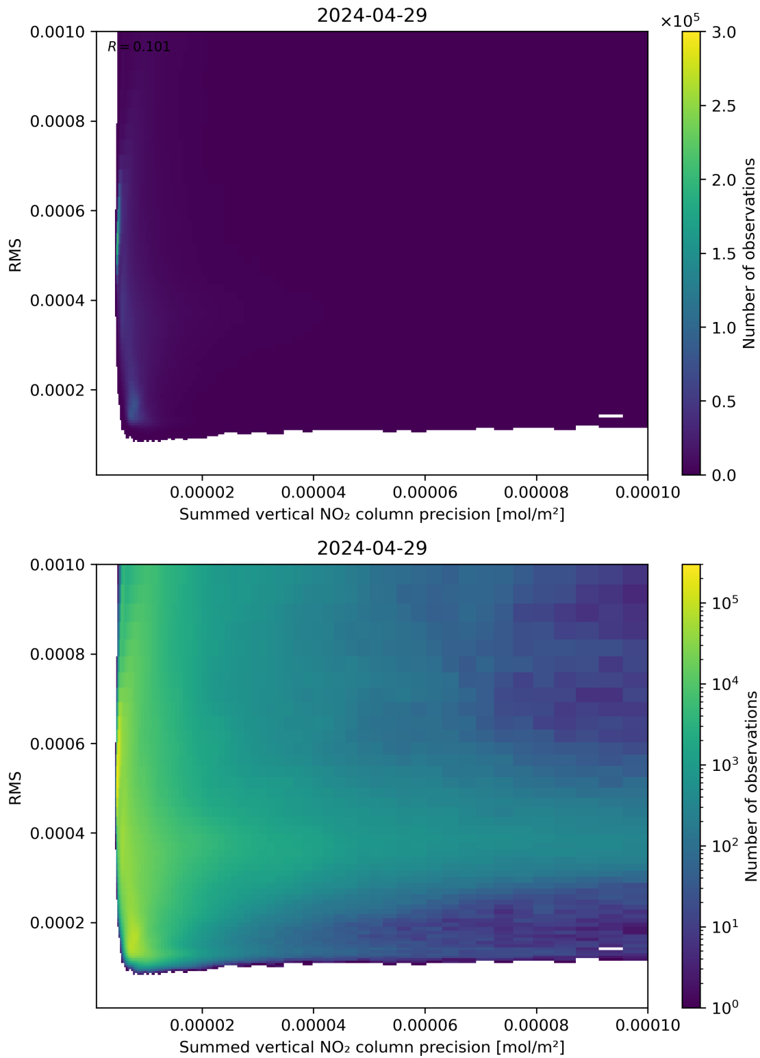
Figure 108: Scatter density plot of “Summed vertical NO 2 column precision” against “RMS” for 2024-04-28 to 2024-04-30.
