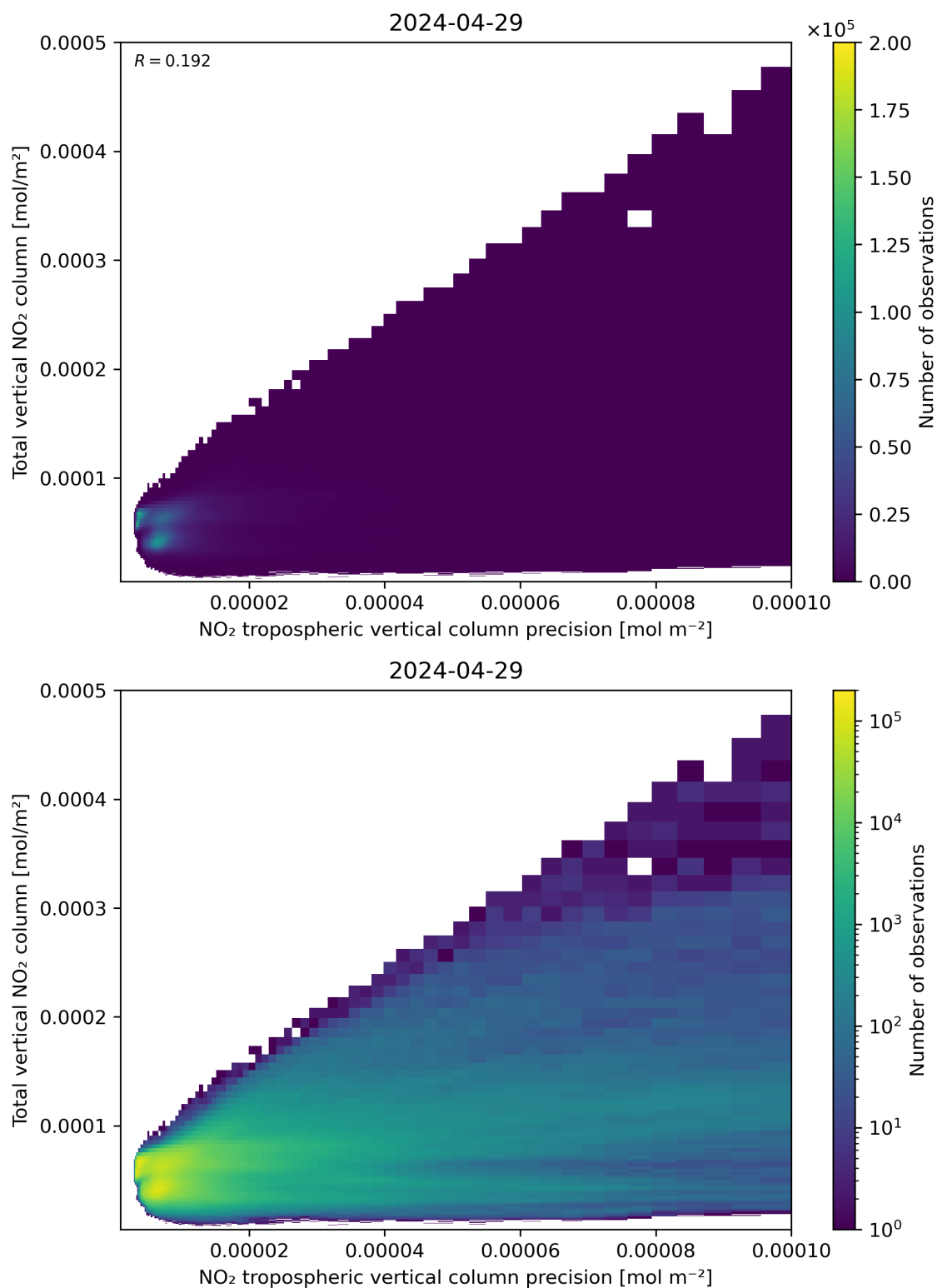
Figure 138: Scatter density plot of “NO 2 tropospheric vertical column precision” against “Total vertical NO 2 column” for 2024-04-28 to 2024-04-30.
