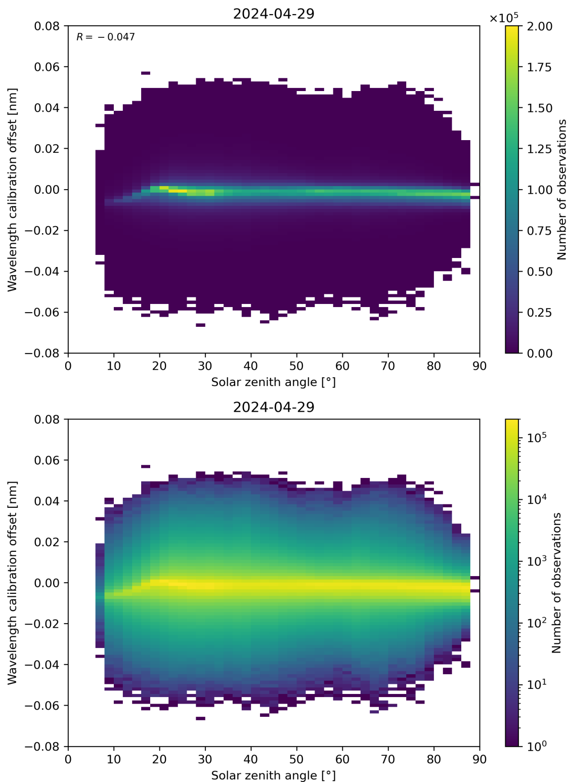
Figure 158: Scatter density plot of “Solar zenith angle” against “Wavelength calibration offset” for 2024-04-28 to 2024-04-30.
