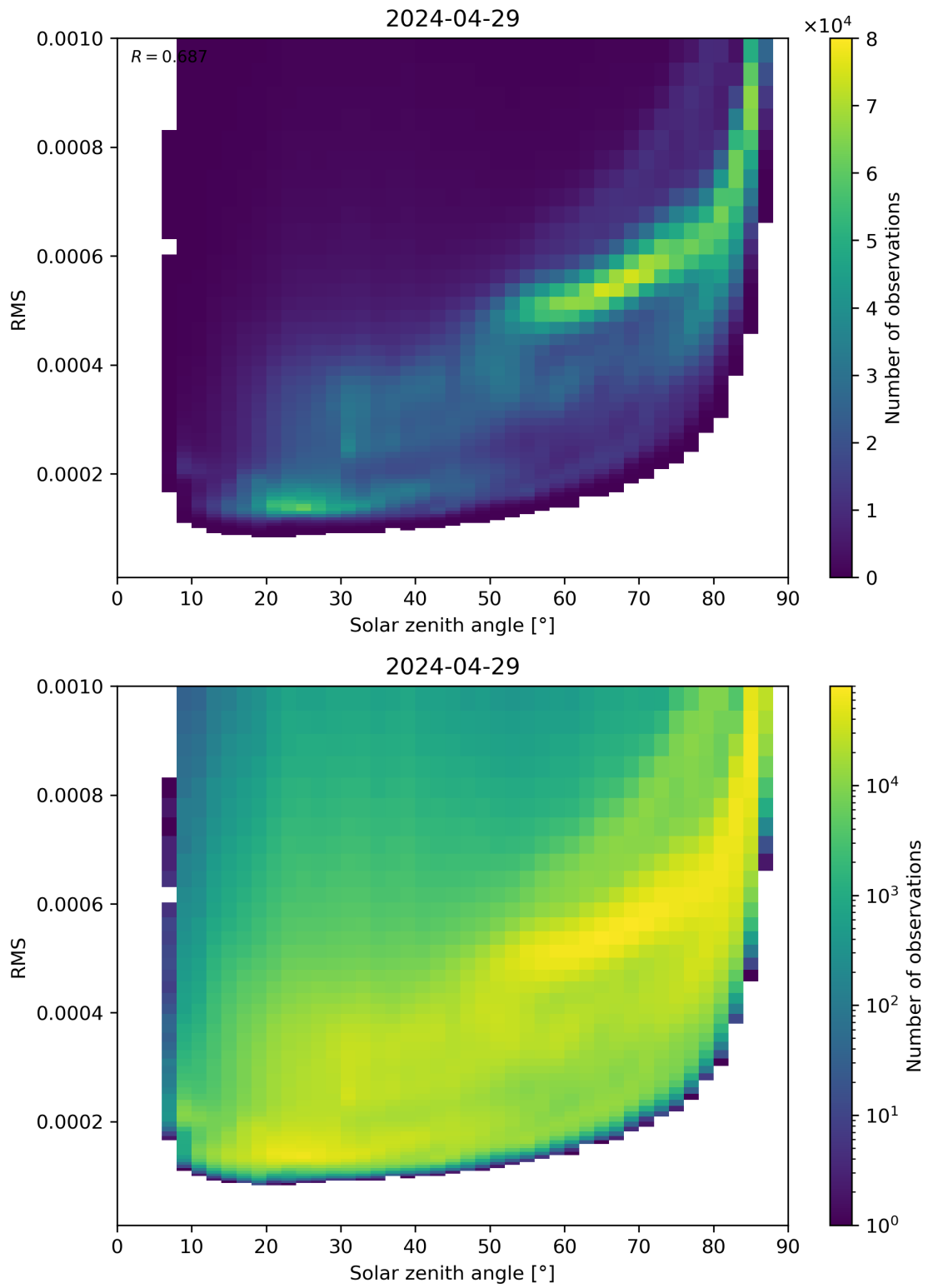
Figure 157: Scatter density plot of “Solar zenith angle” against “RMS” for 2024-04-28 to 2024-04-30.
