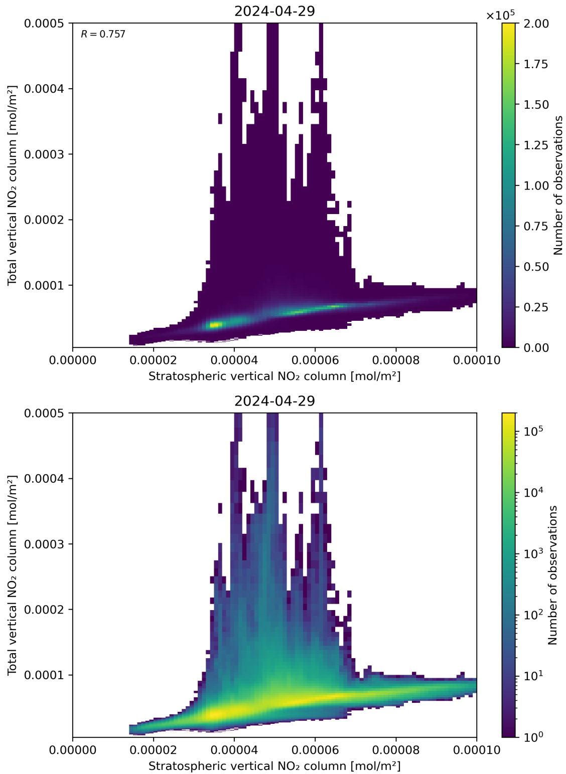
Figure 100: Scatter density plot of “Stratospheric vertical NO 2 column” against “Total vertical NO 2 column” for 2024-04-28 to 2024-04-30.
