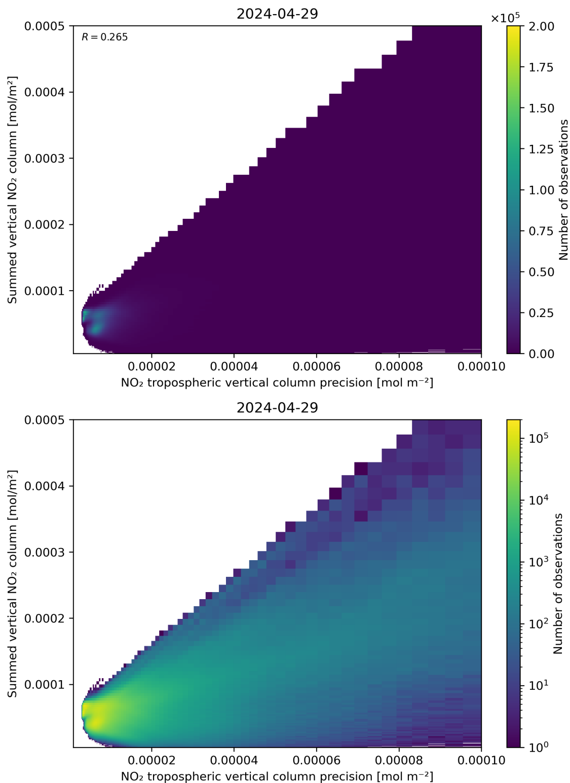
Figure 136: Scatter density plot of “NO 2 tropospheric vertical column precision” against “Summed vertical NO 2 column” for 2024-04-28 to 2024-04-30.
