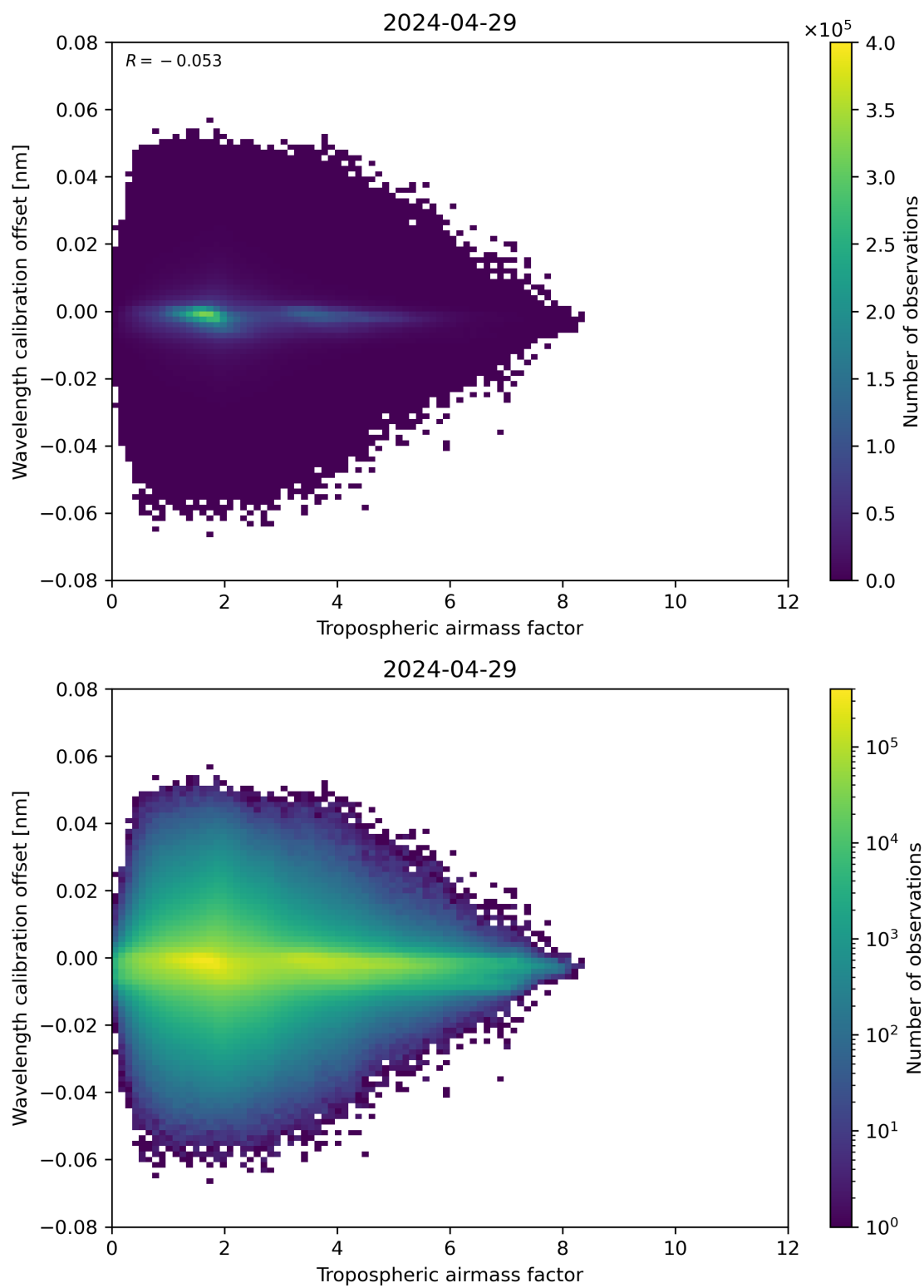
Figure 80: Scatter density plot of “Tropospheric airmass factor” against “Wavelength calibration offset” for 2024-04-28 to 2024-04-30.
