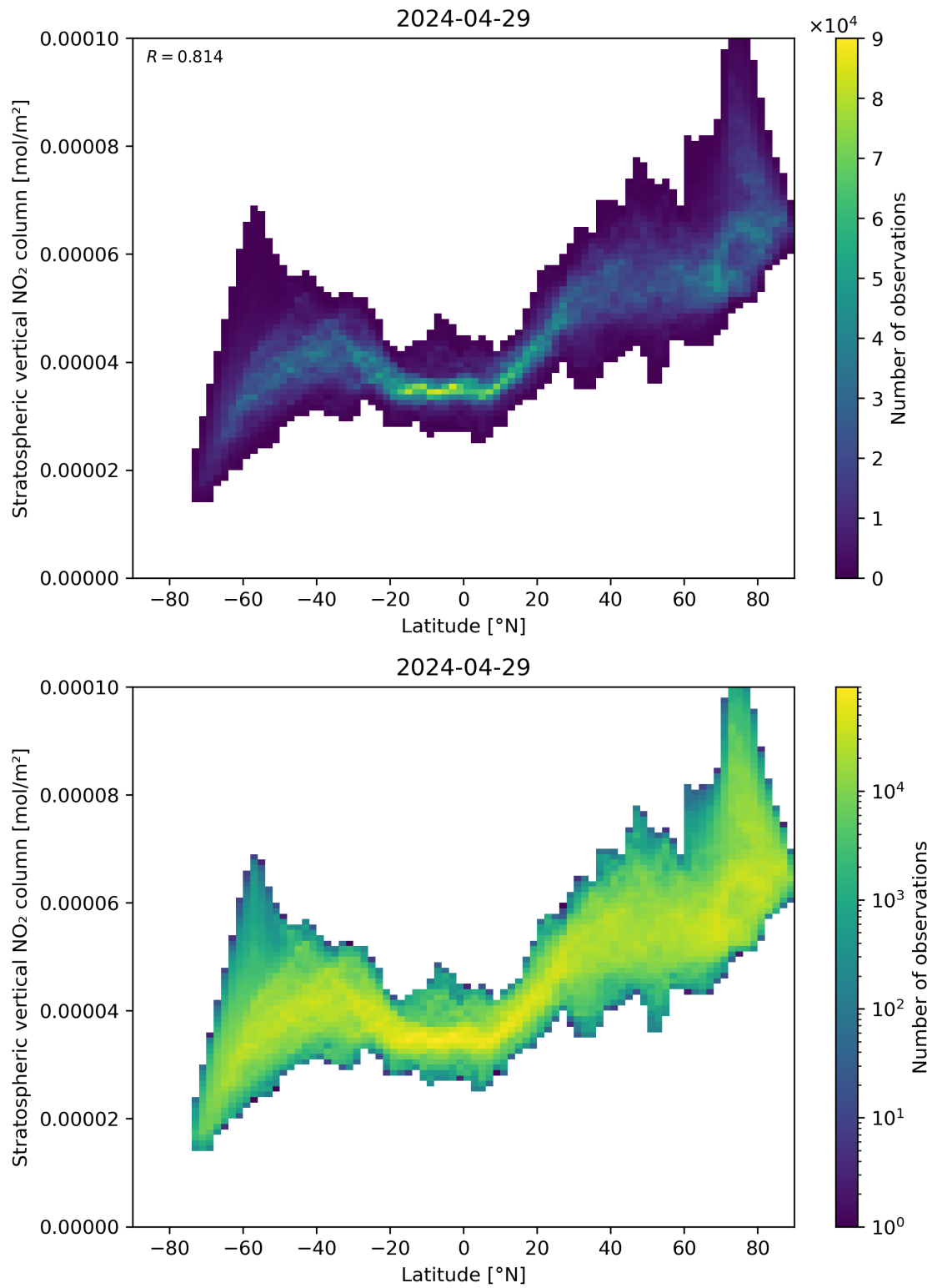
Figure 87: Scatter density plot of “Latitude” against “Stratospheric vertical NO 2 column” for 2024-04-28 to 2024-04-30.
