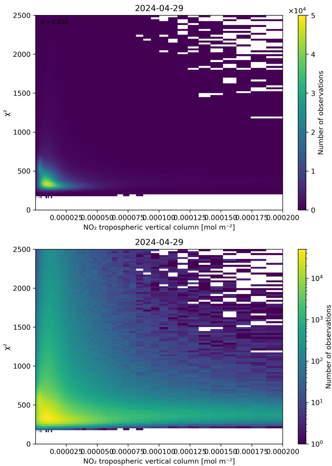
Figure 124: Scatter density plot of “NO 2 tropospheric vertical column” against “ \chi^2 ” for 2024-04-28 to 2024-04-30.
