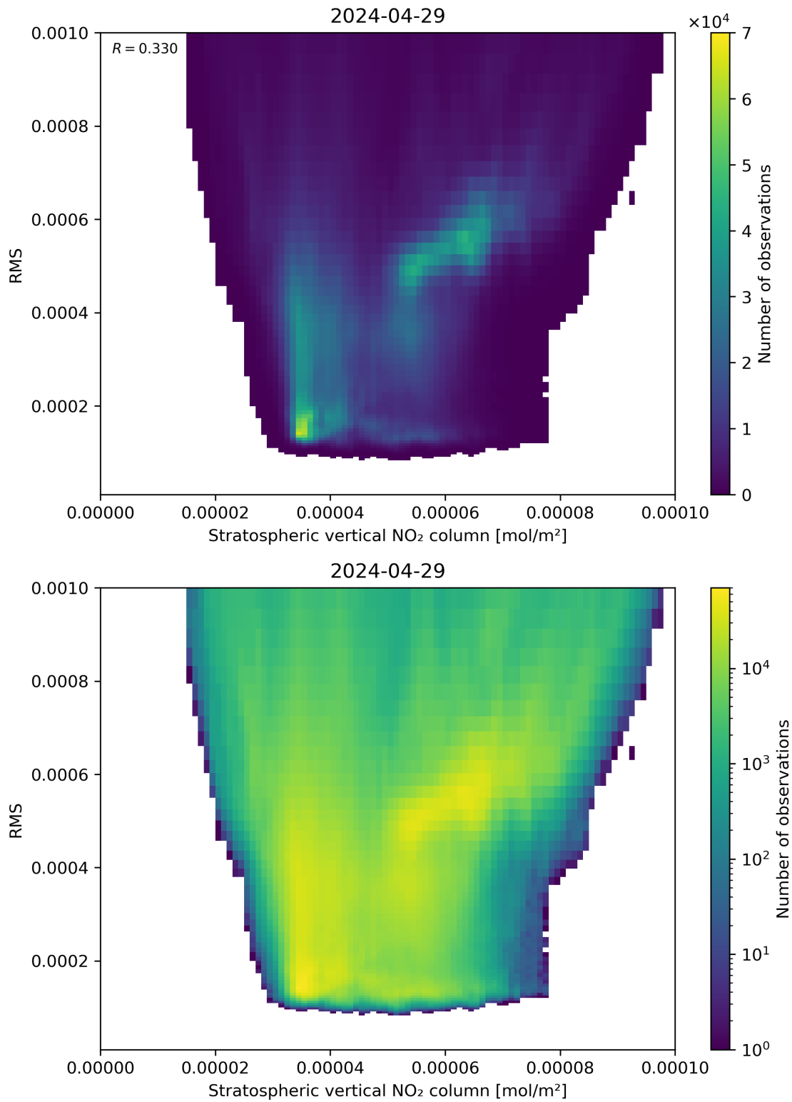
Figure 102: Scatter density plot of “Stratospheric vertical NO 2 column” against “RMS” for 2024-04-28 to 2024-04-30.
