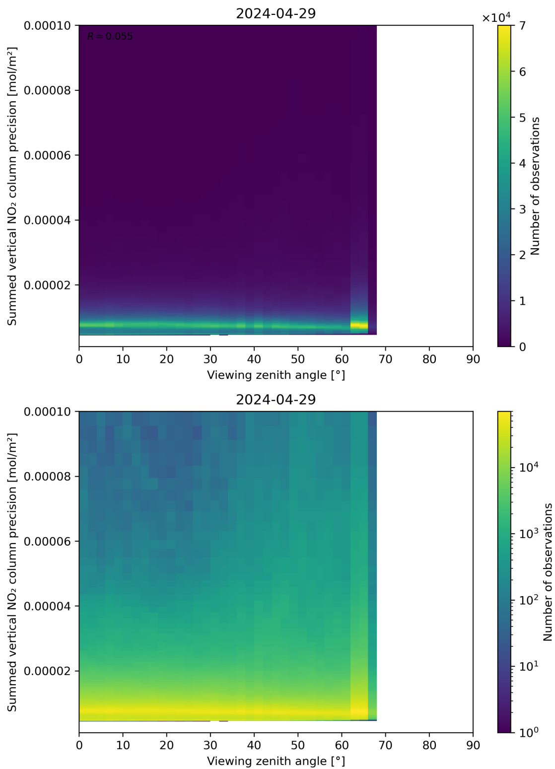
Figure 166: Scatter density plot of “Viewing zenith angle” against “Summed vertical NO 2 column precision” for 2024-04-28 to 2024-04-30.
