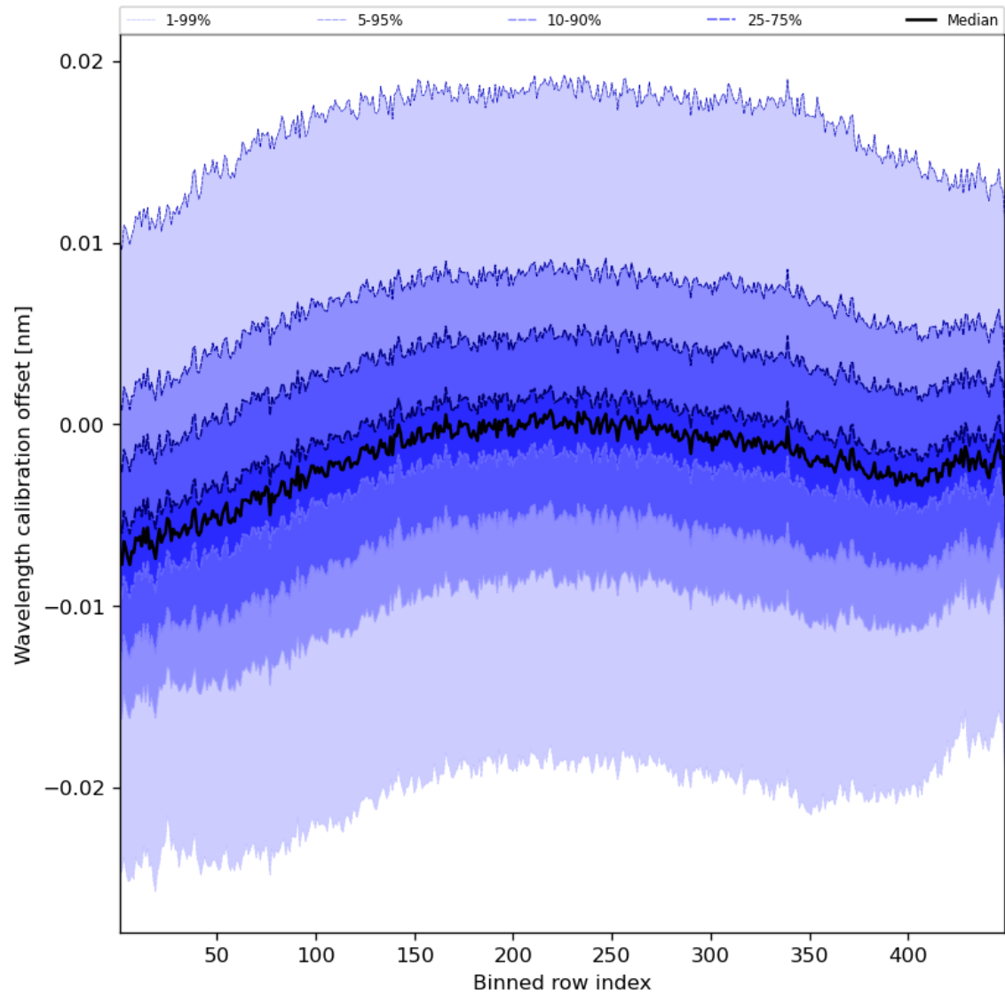
Figure 52: Along track statistics of “Wavelength calibration offset” for 2024-04-28 to 2024-04-30
