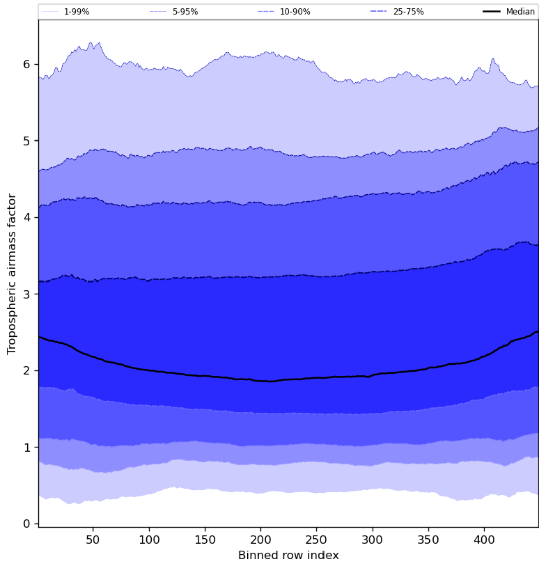
Figure 48: Along track statistics of “Tropospheric airmass factor” for 2024-04-28 to 2024-04-30
