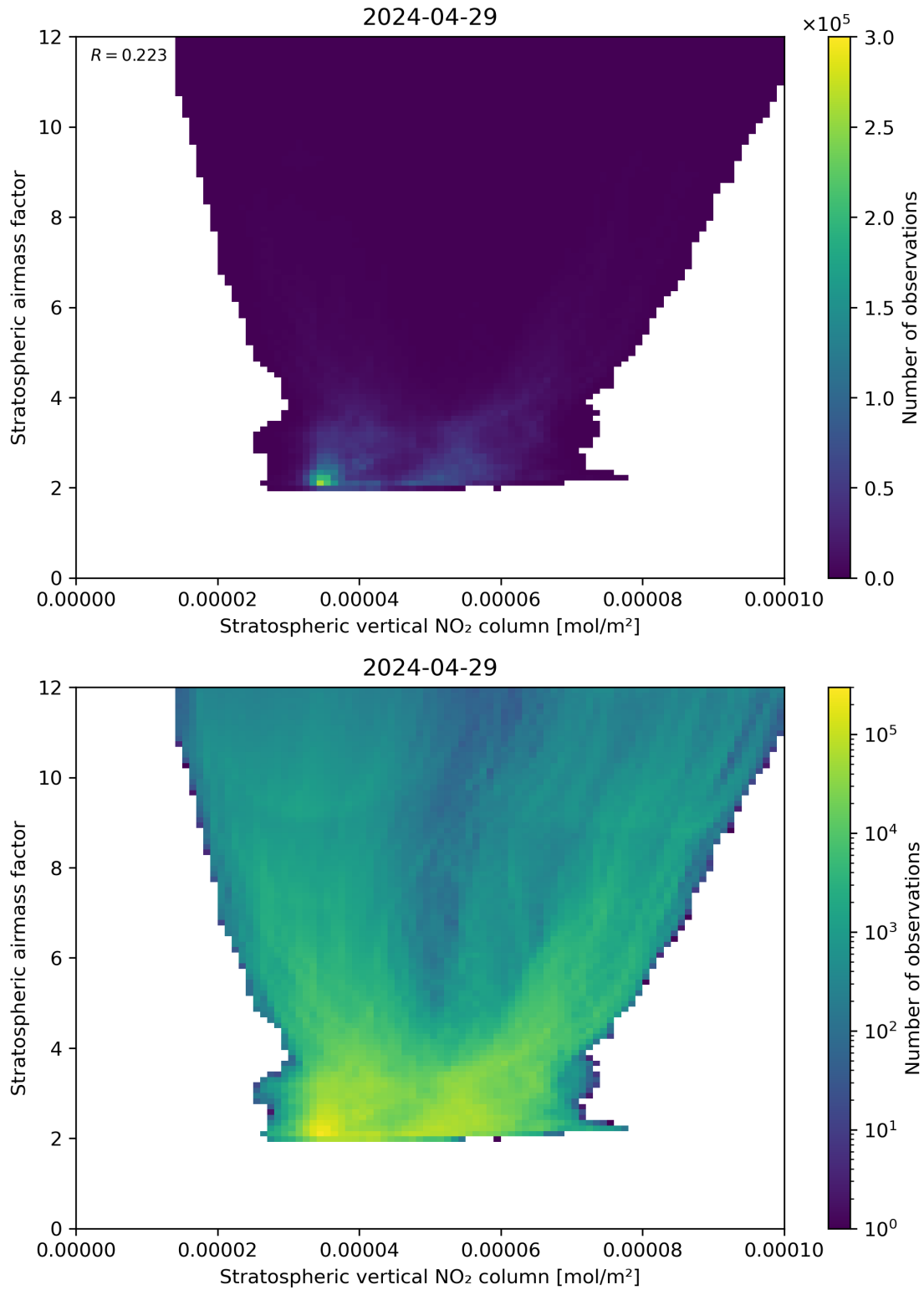
Figure 96: Scatter density plot of “Stratospheric vertical NO 2 column” against “Stratospheric airmass factor” for 2024-04-28 to 2024-04-30.
