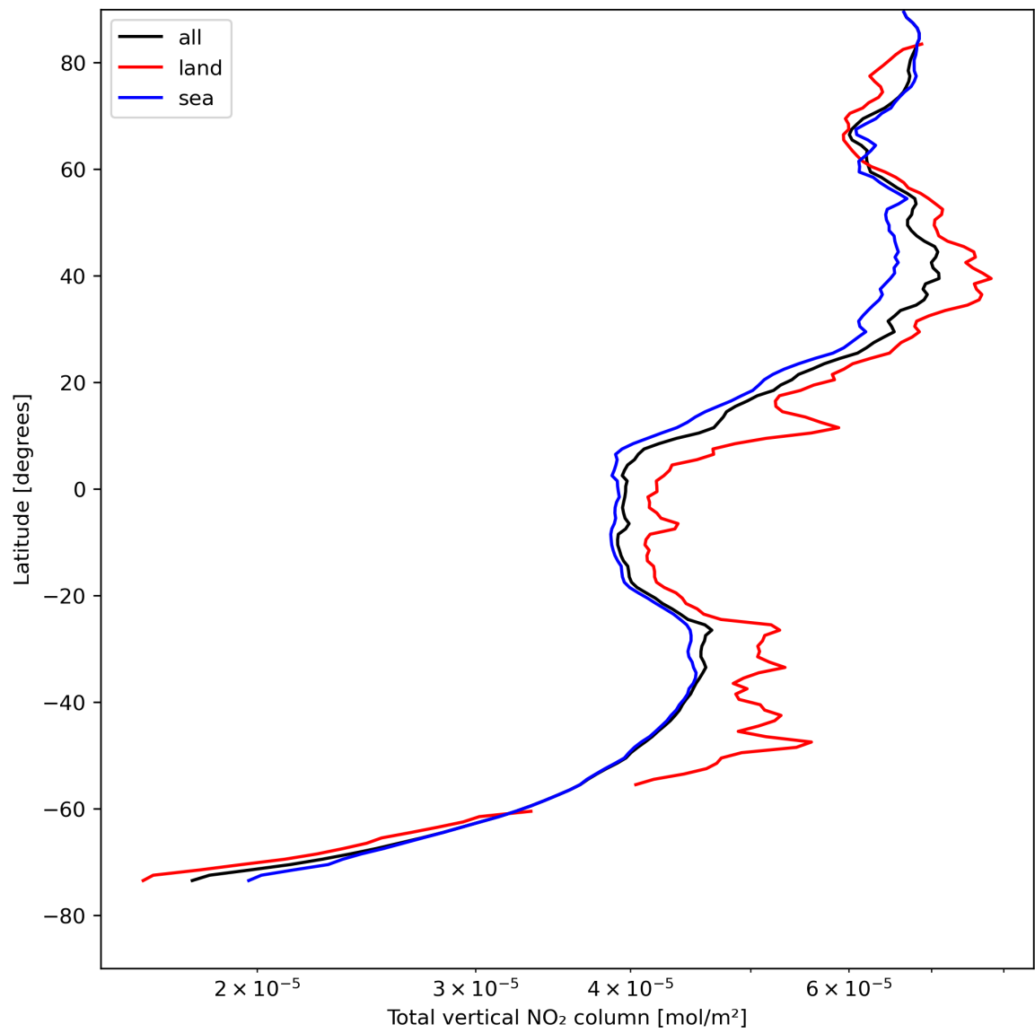
Figure 21: Zonal average of “Total vertical NO 2 column” for 2024-04-28 to 2024-04-30.
