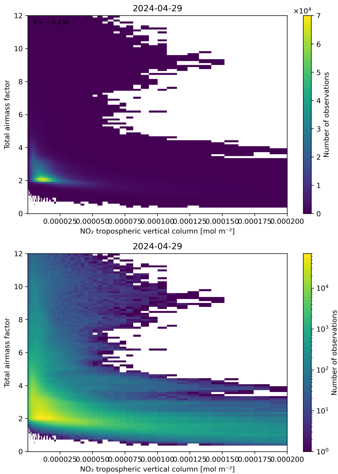
Figure 122: Scatter density plot of “NO 2 tropospheric vertical column” against “Total air mass factor” for 2024-04-28 to 2024-04-30.
