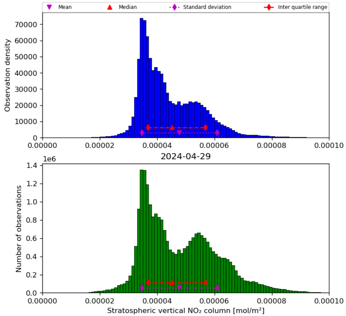
Figure 36: Histogram of “Stratospheric vertical NO 2 column” for 2024-04-28 to 2024-04-30
