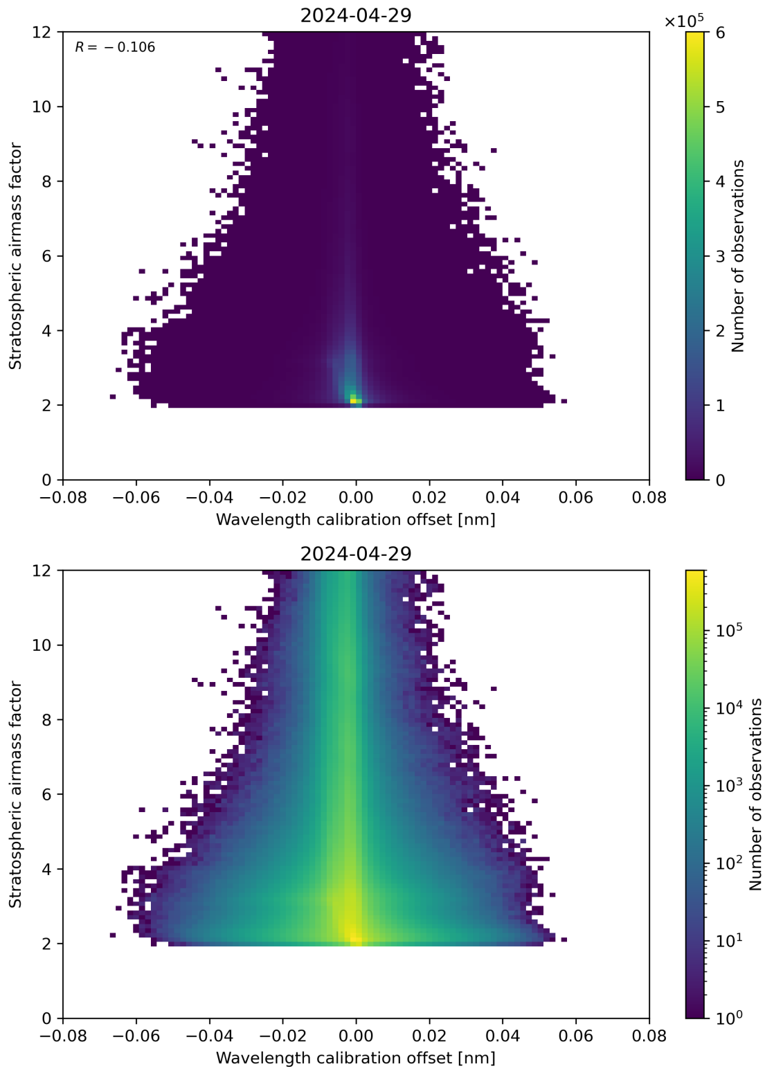
Figure 174: Scatter density plot of “Wavelength calibration offset” against “Stratospheric airmass factor” for 2024-04-28 to 2024-04-30.
