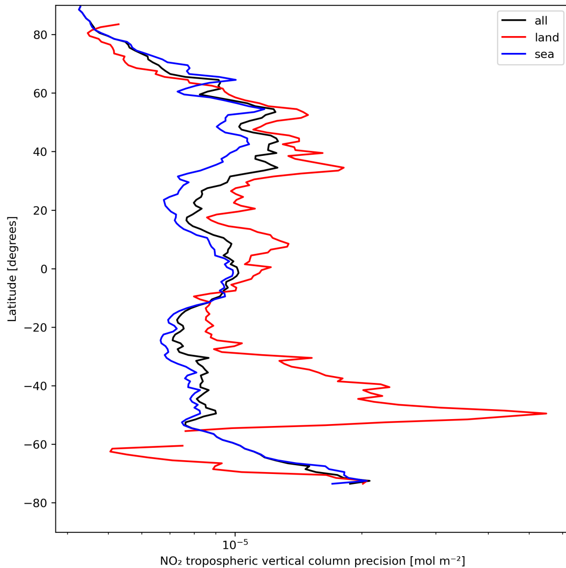
Figure 13: Zonal average of “NO 2 tropospheric vertical column precision” for 2024-04-28 to 2024-04-30.
