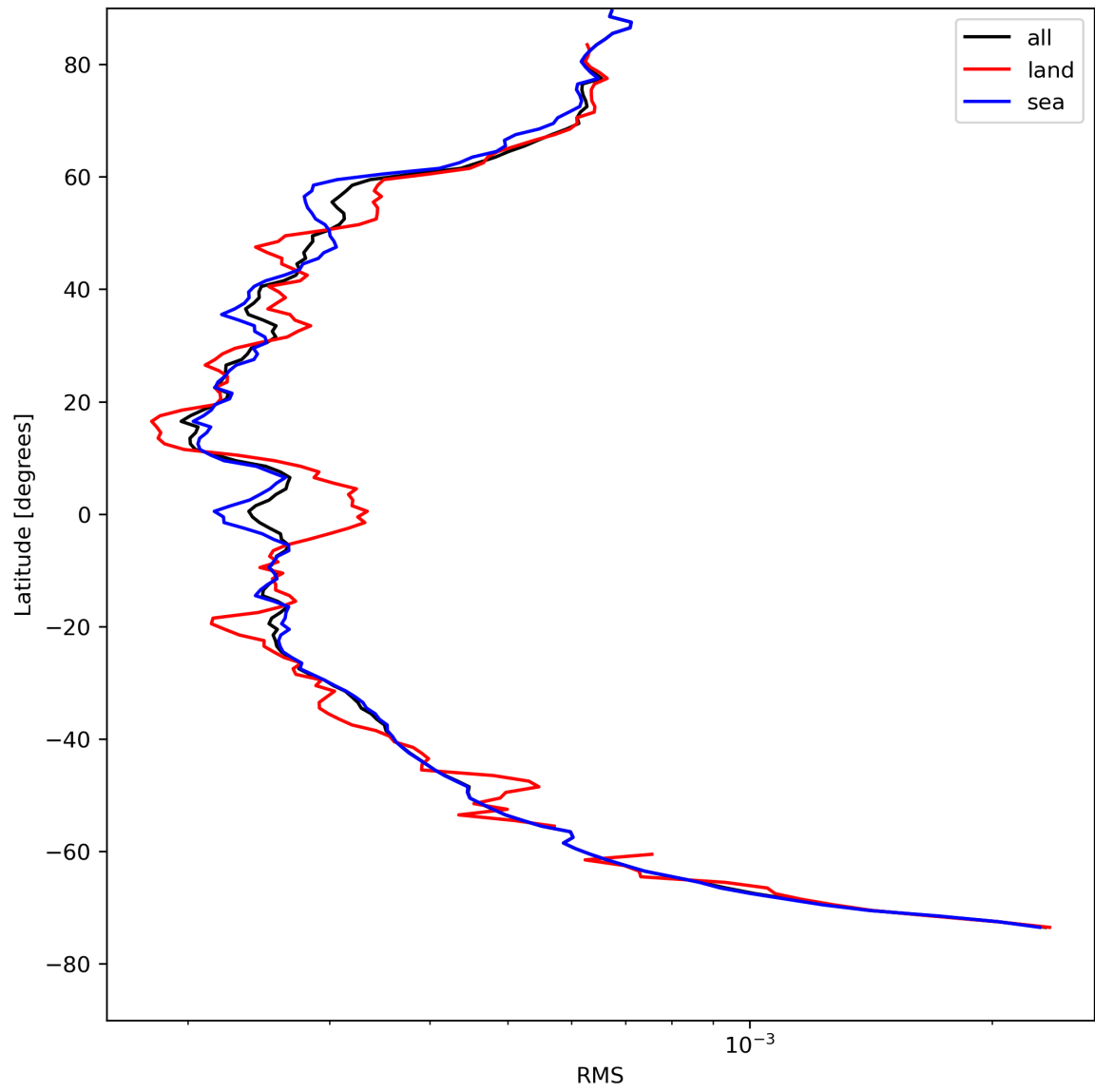
Figure 26: Zonal average of “RMS” for 2024-04-28 to 2024-04-30.
