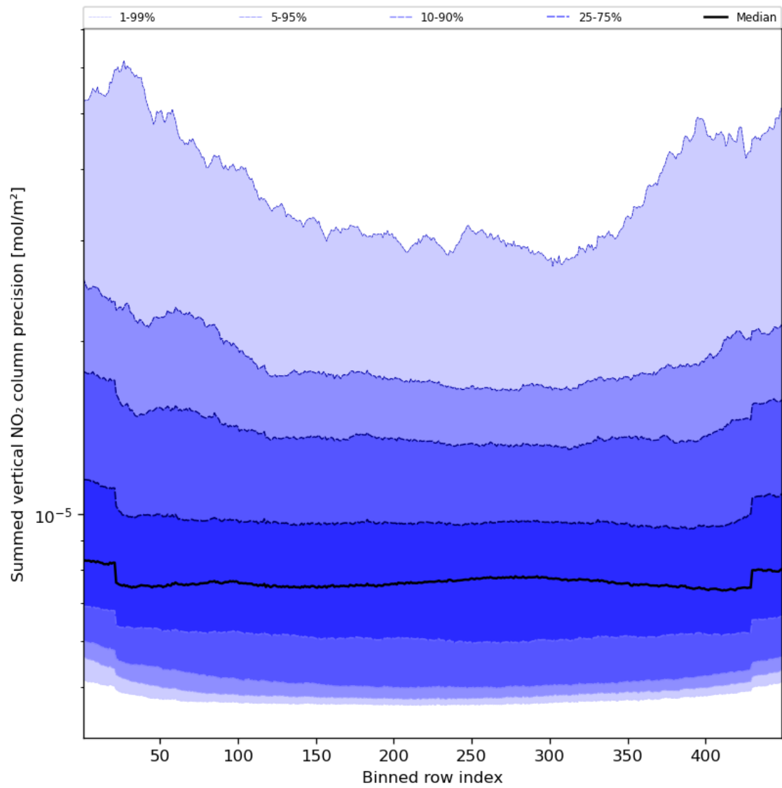
Figure 58: Along track statistics of “Summed vertical NO 2 column precision” for 2024-04-28 to 2024-04-30
