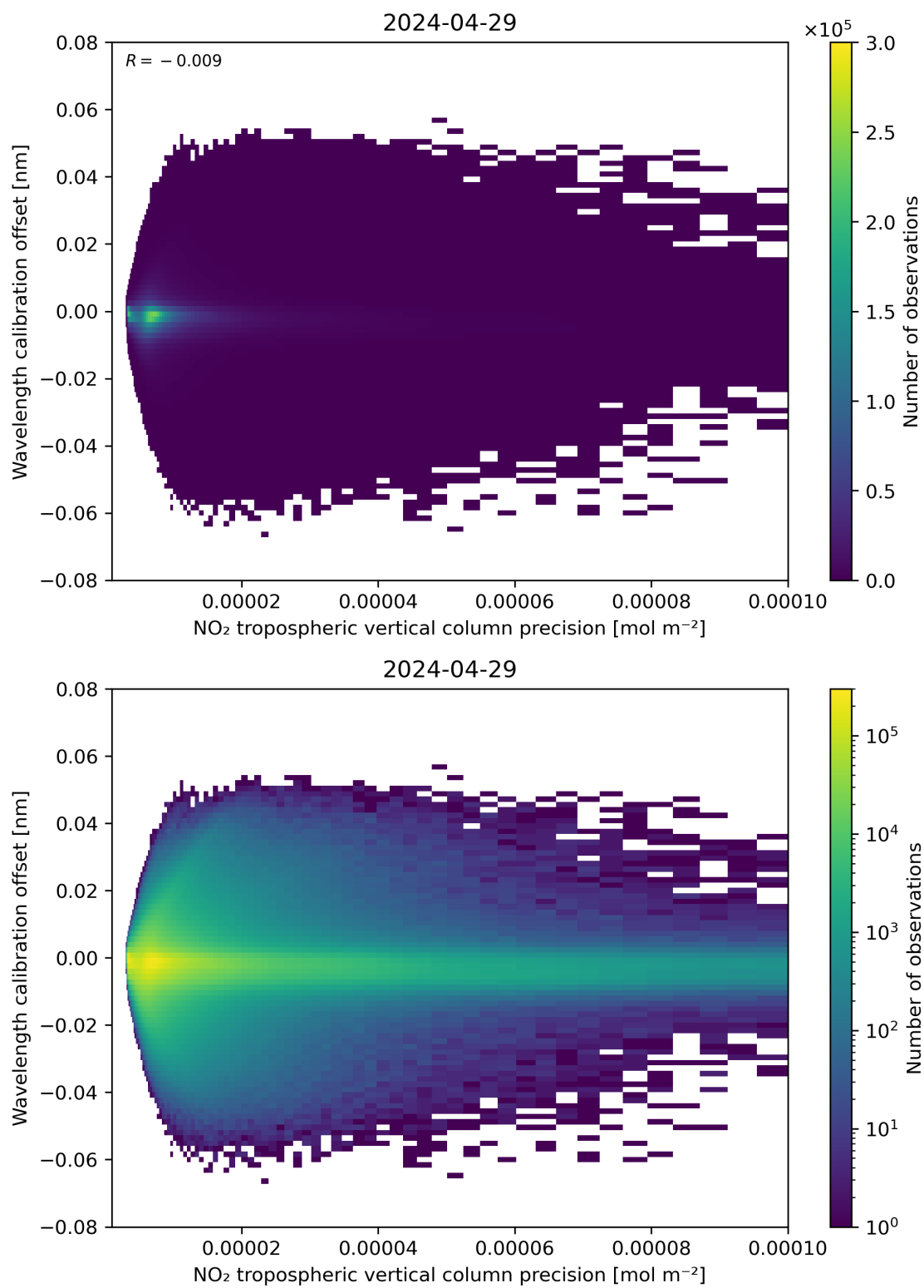
Figure 141: Scatter density plot of “NO 2 tropospheric vertical column precision” against “Wavelength calibration offset” for 2024-04-28 to 2024-04-30.
