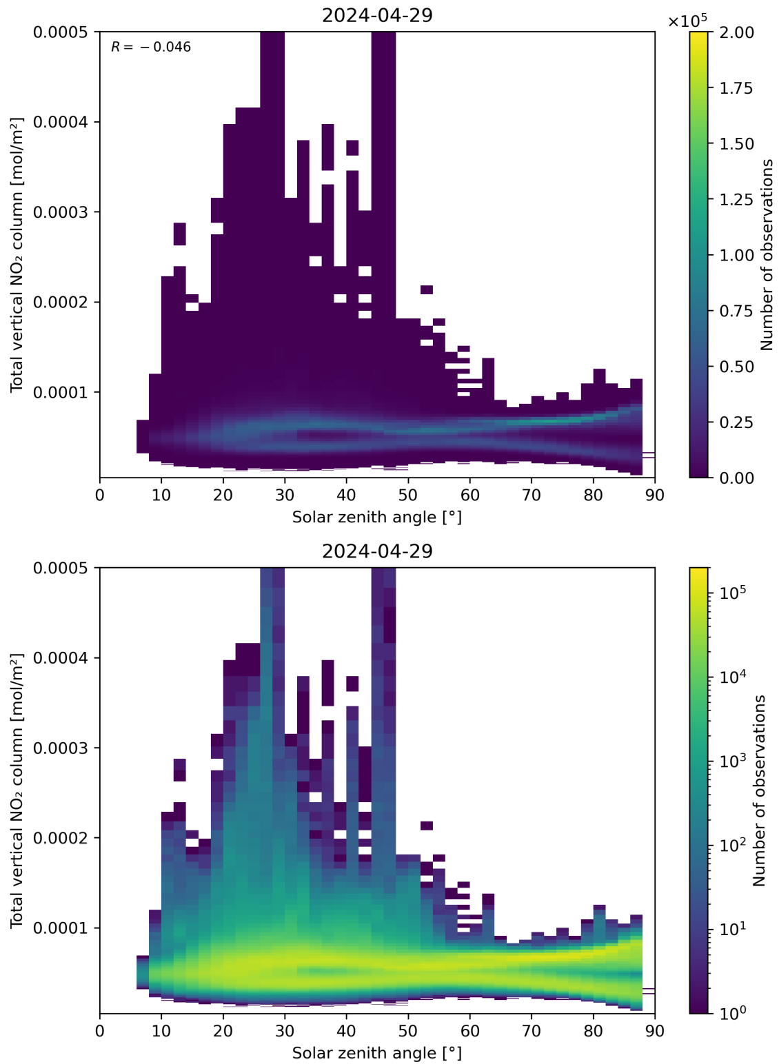
Figure 153: Scatter density plot of “Solar zenith angle” against “Total vertical NO 2 column” for 2024-04-28 to 2024-04-30.
