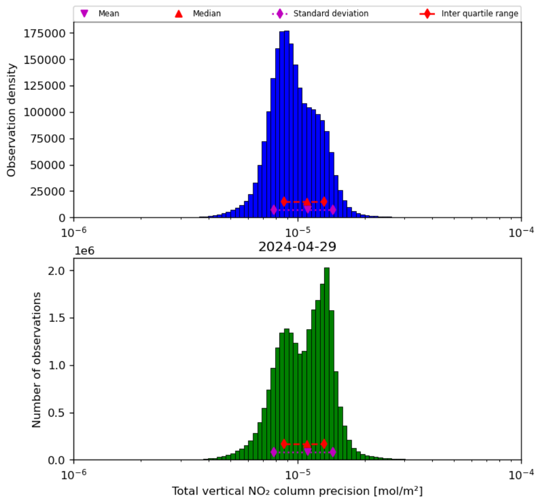
Figure 39: Histogram of “Total vertical NO 2 column precision” for 2024-04-28 to 2024-04-30
