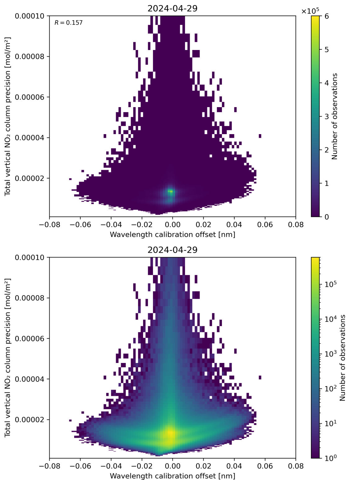
Figure 180: Scatter density plot of “Wavelength calibration offset” against “Total vertical NO 2 column precision” for 2024-04-28 to 2024-04-30.
