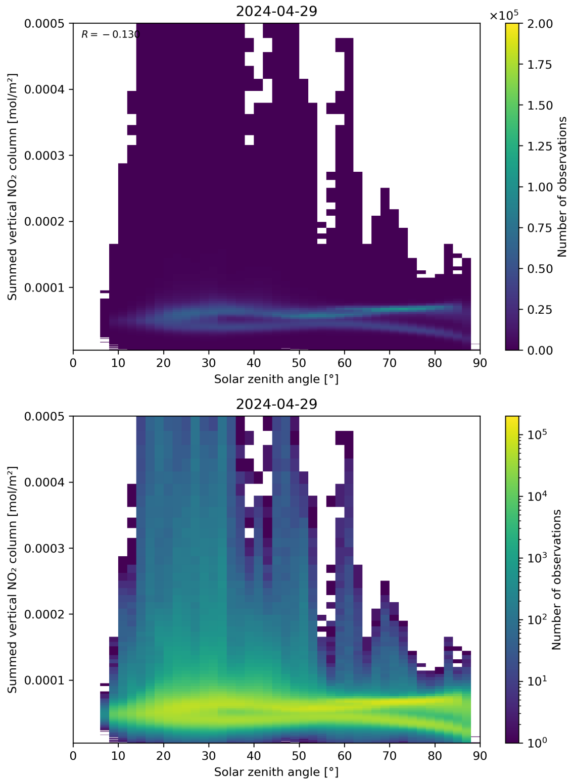
Figure 151: Scatter density plot of “Solar zenith angle” against “Summed vertical NO 2 column” for 2024-04-28 to 2024-04-30.
