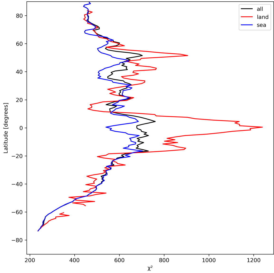
Figure 25: Zonal average of “ \chi^2 ” for 2024-04-28 to 2024-04-30.
