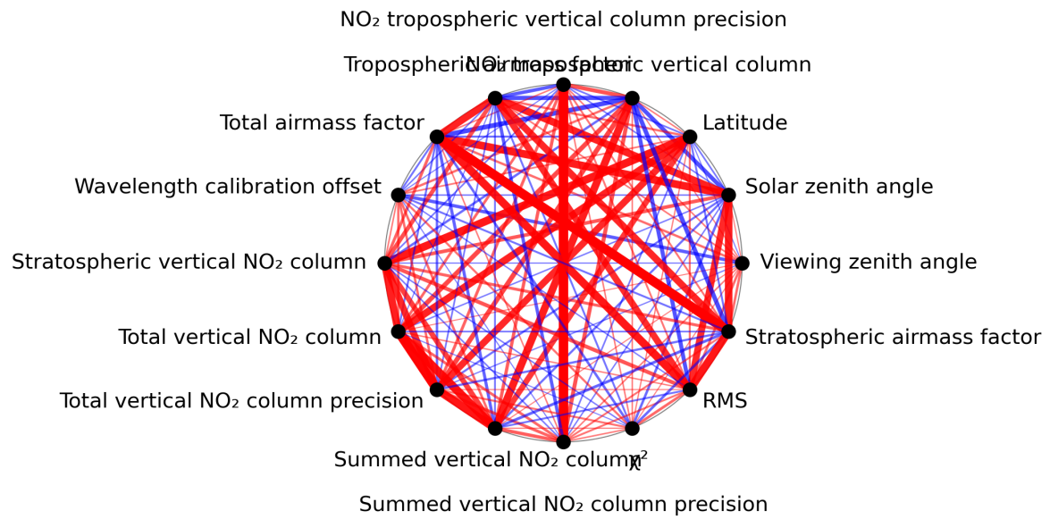
Figure 1: Map of correlation graph for 2024-04-28 to 2024-04-30.
