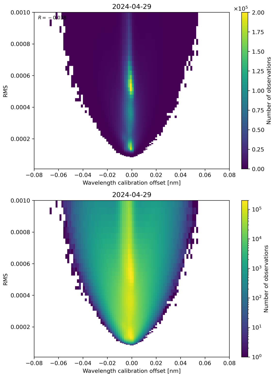
Figure 181: Scatter density plot of “Wavelength calibration offset” against “RMS” for 2024-04-28 to 2024-04-30.
