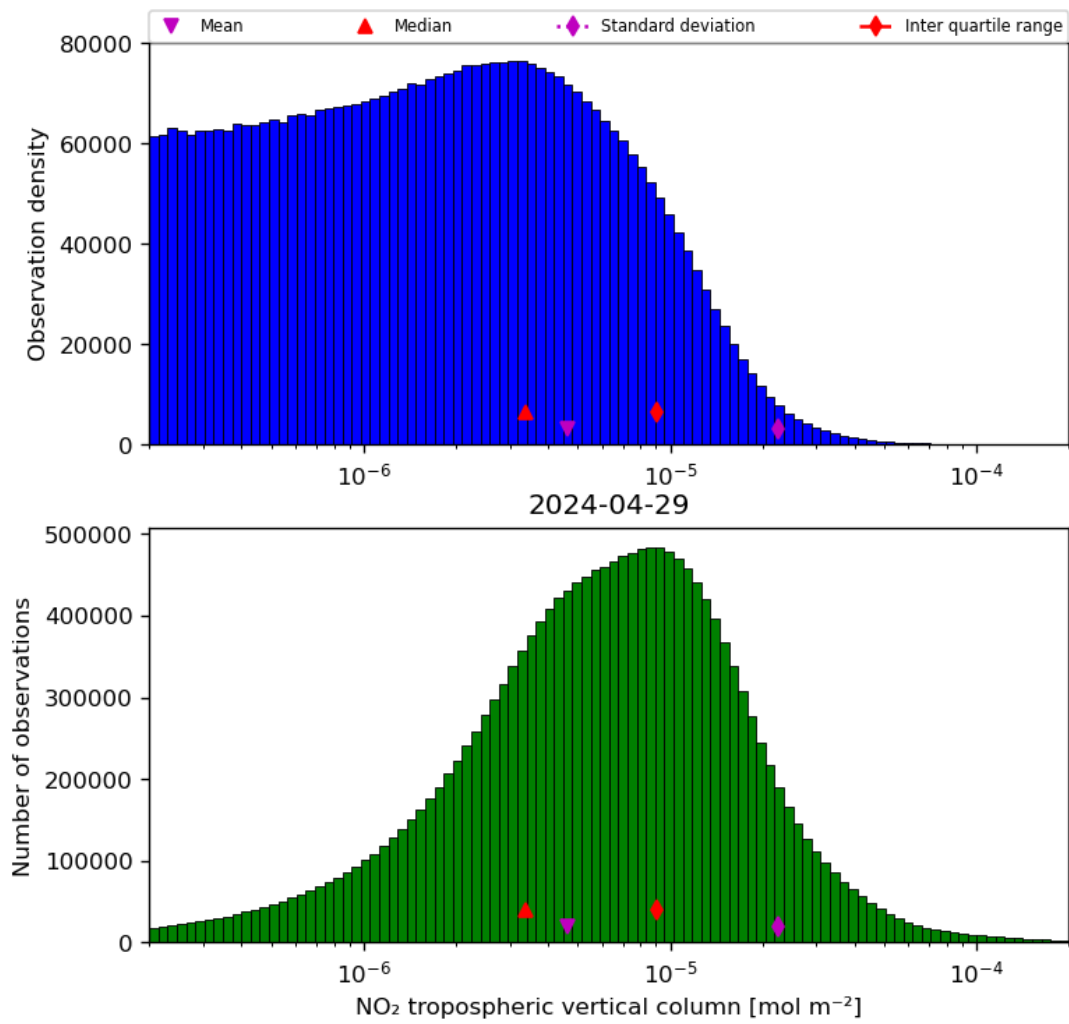
Figure 29: Histogram of “NO 2 tropospheric vertical column” for 2024-04-28 to 2024-04-30
