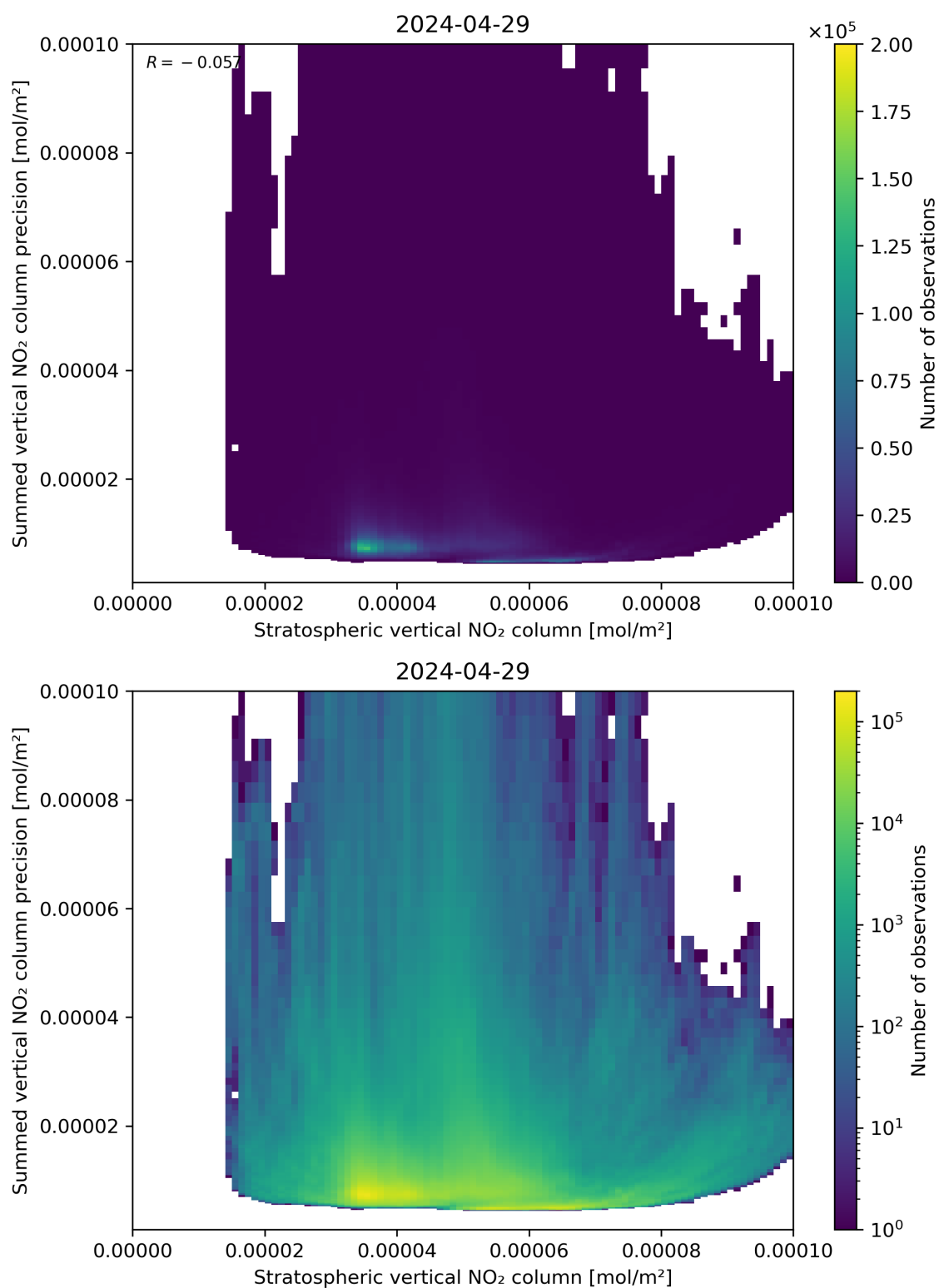
Figure 99: Scatter density plot of “Stratospheric vertical NO 2 column” against “Summed vertical NO 2 column precision” for 2024-04-28 to 2024-04-30.
