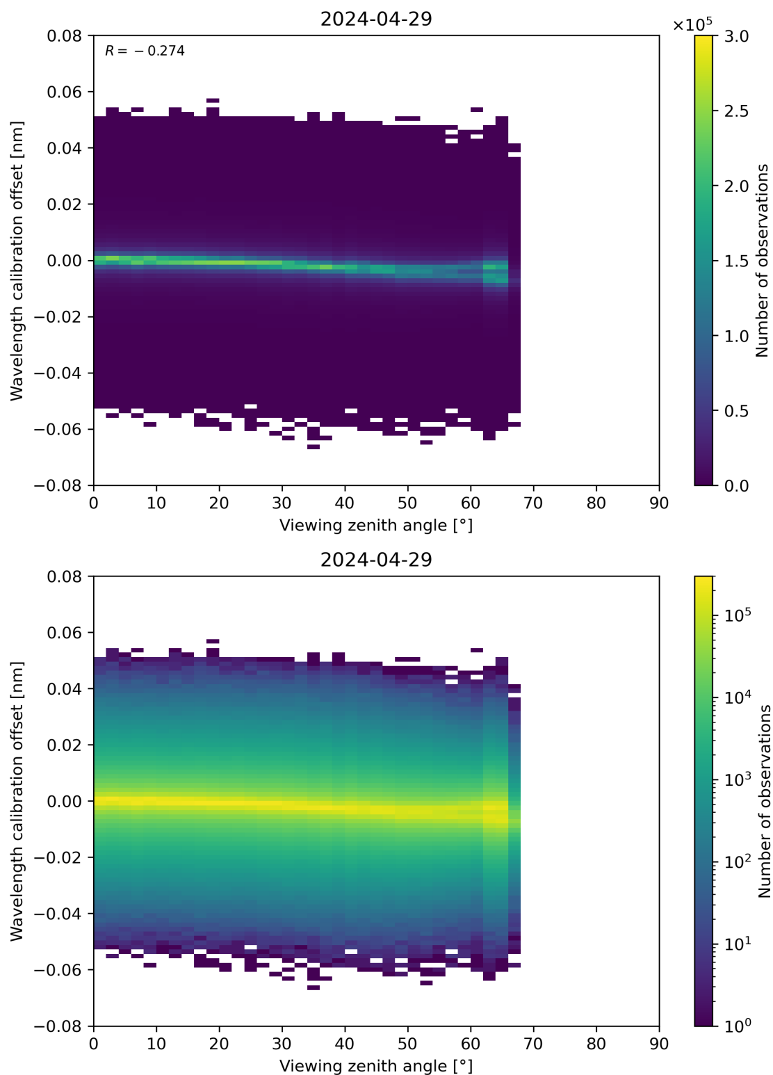
Figure 173: Scatter density plot of “Viewing zenith angle” against “Wavelength calibration offset” for 2024-04-28 to 2024-04-30.
