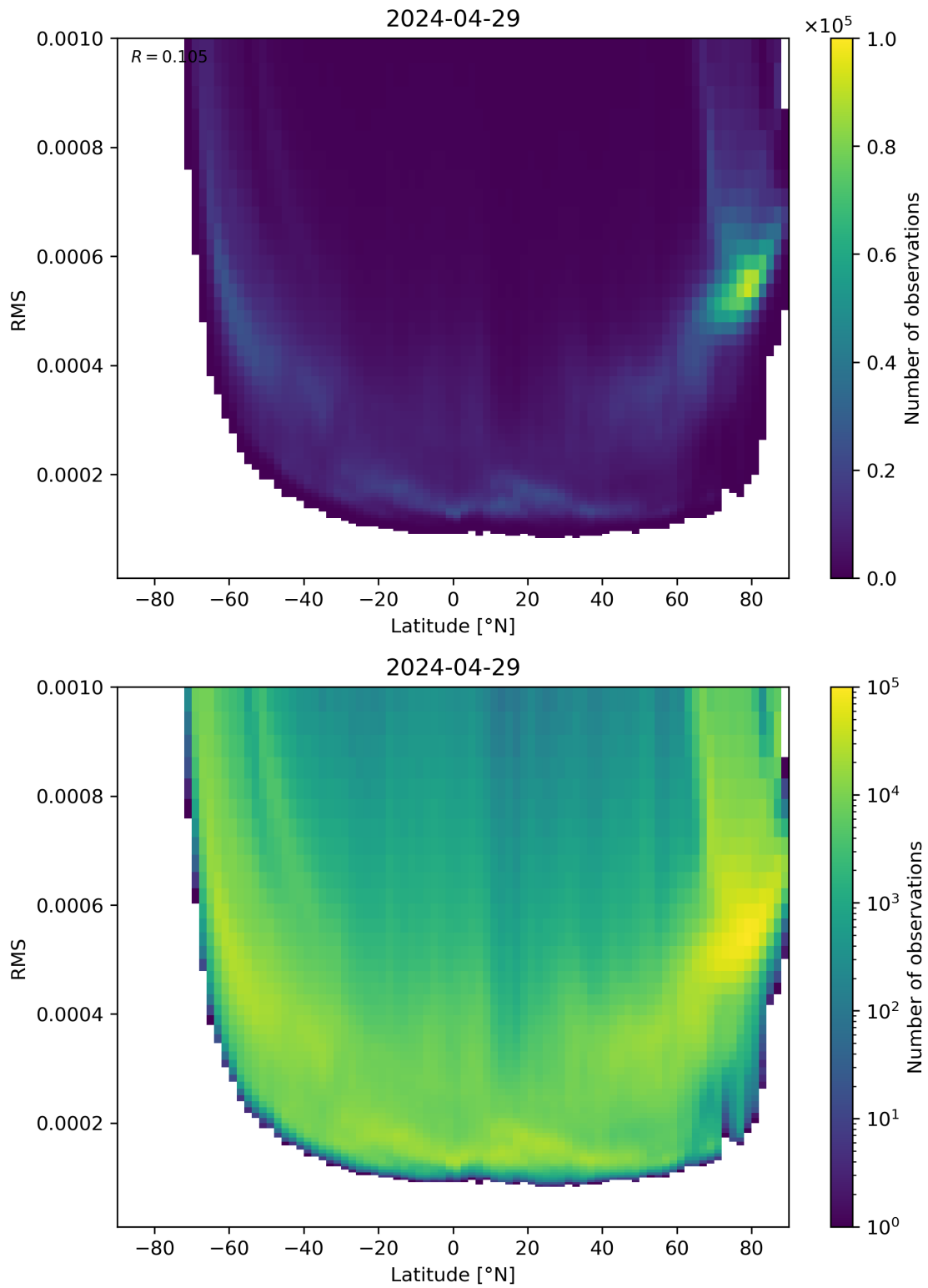
Figure 94: Scatter density plot of “Latitude” against “RMS” for 2024-04-28 to 2024-04-30.
