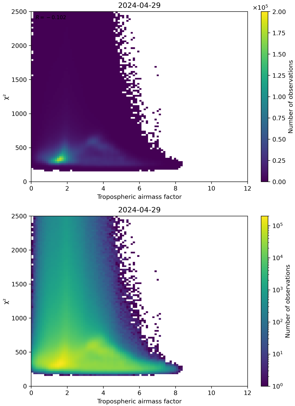
Figure 73: Scatter density plot of “Tropospheric airmass factor” against “ \chi^2 ” for 2024-04-28 to 2024-04-30.
