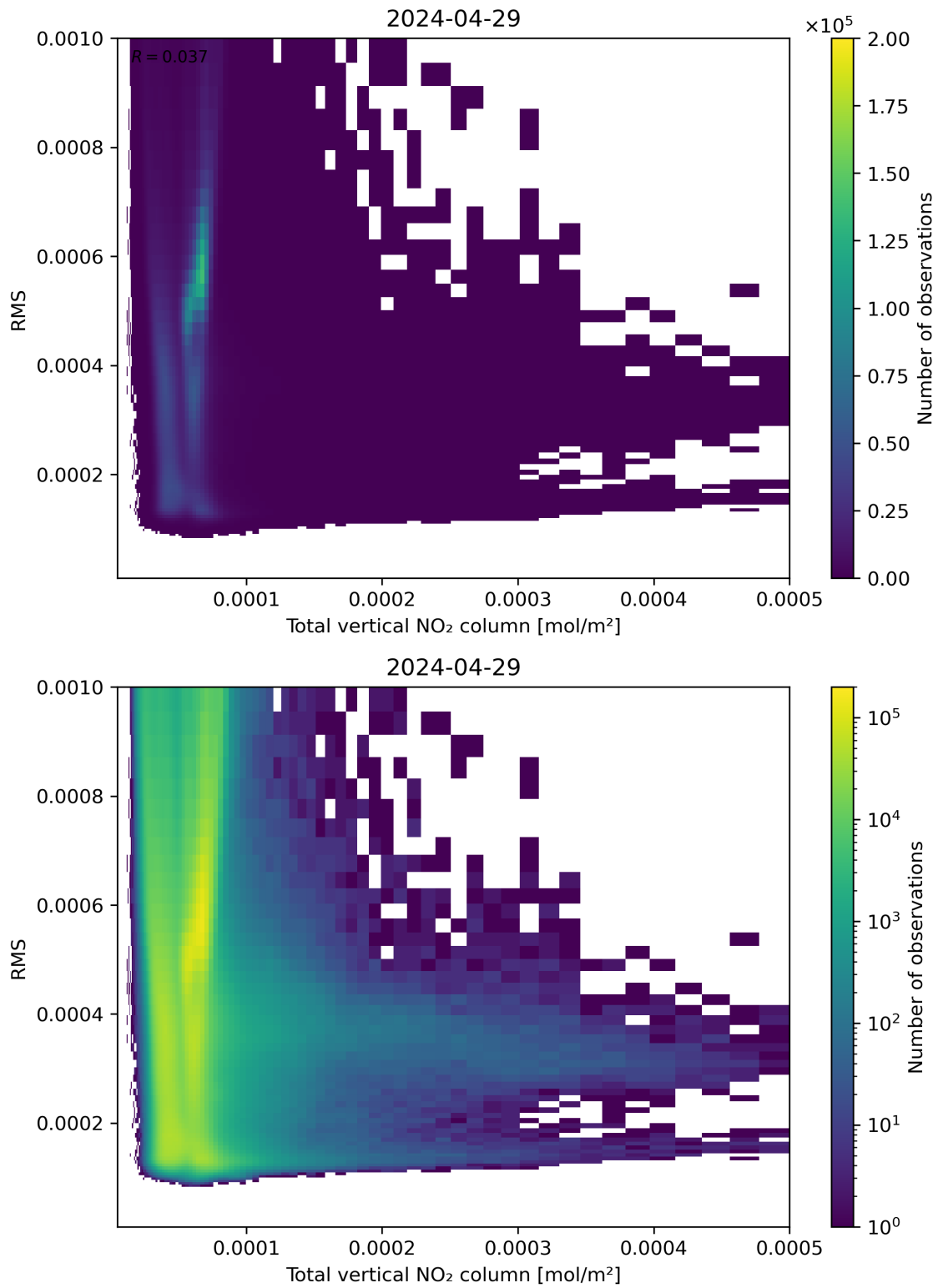
Figure 120: Scatter density plot of “Total vertical NO 2 column” against “RMS” for 2024-04-28 to 2024-04-30.
