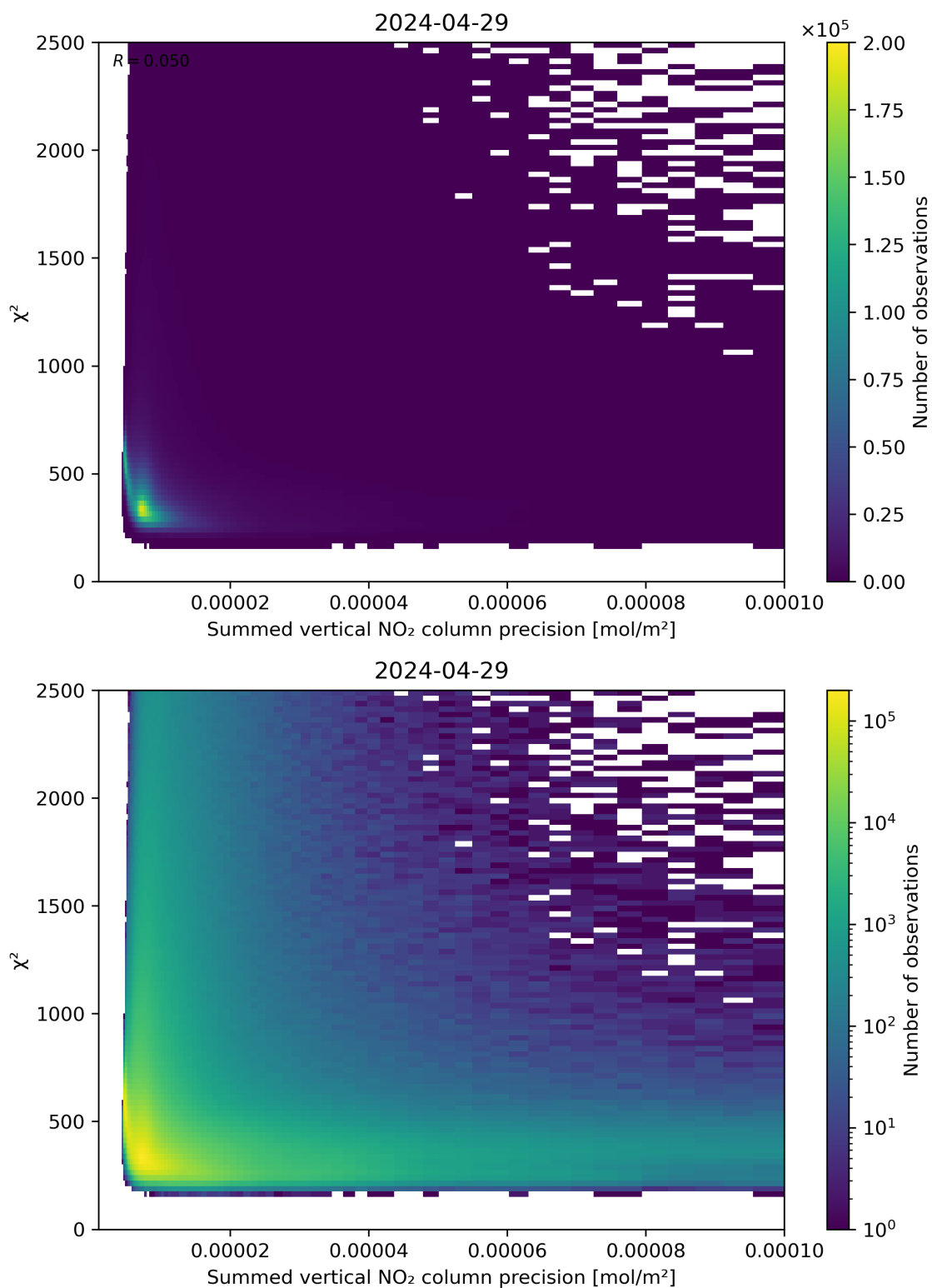
Figure 107: Scatter density plot of “Summed vertical NO 2 column precision” against “ \chi^2 ” for 2024-04-28 to 2024-04-30.
