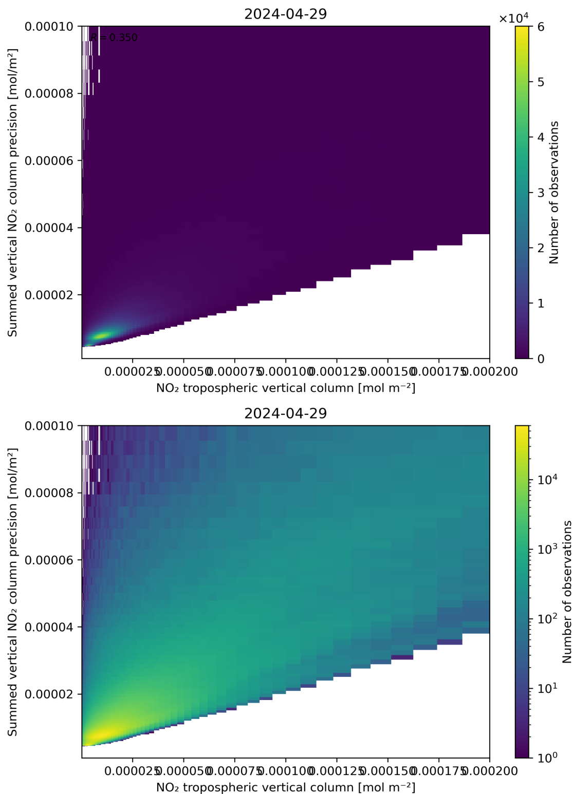
Figure 127: Scatter density plot of “NO 2 tropospheric vertical column” against “Summed vertical NO 2 column precision” for 2024-04-28 to 2024-04-30.
