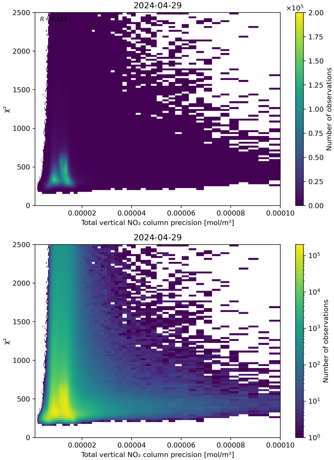
Figure 116: Scatter density plot of “Total vertical NO 2 column precision” against “ \chi^2 ” for 2024-04-28 to 2024-04-30.
