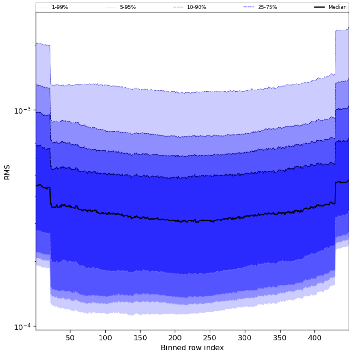
Figure 60: Along track statistics of “RMS” for 2024-04-28 to 2024-04-30
