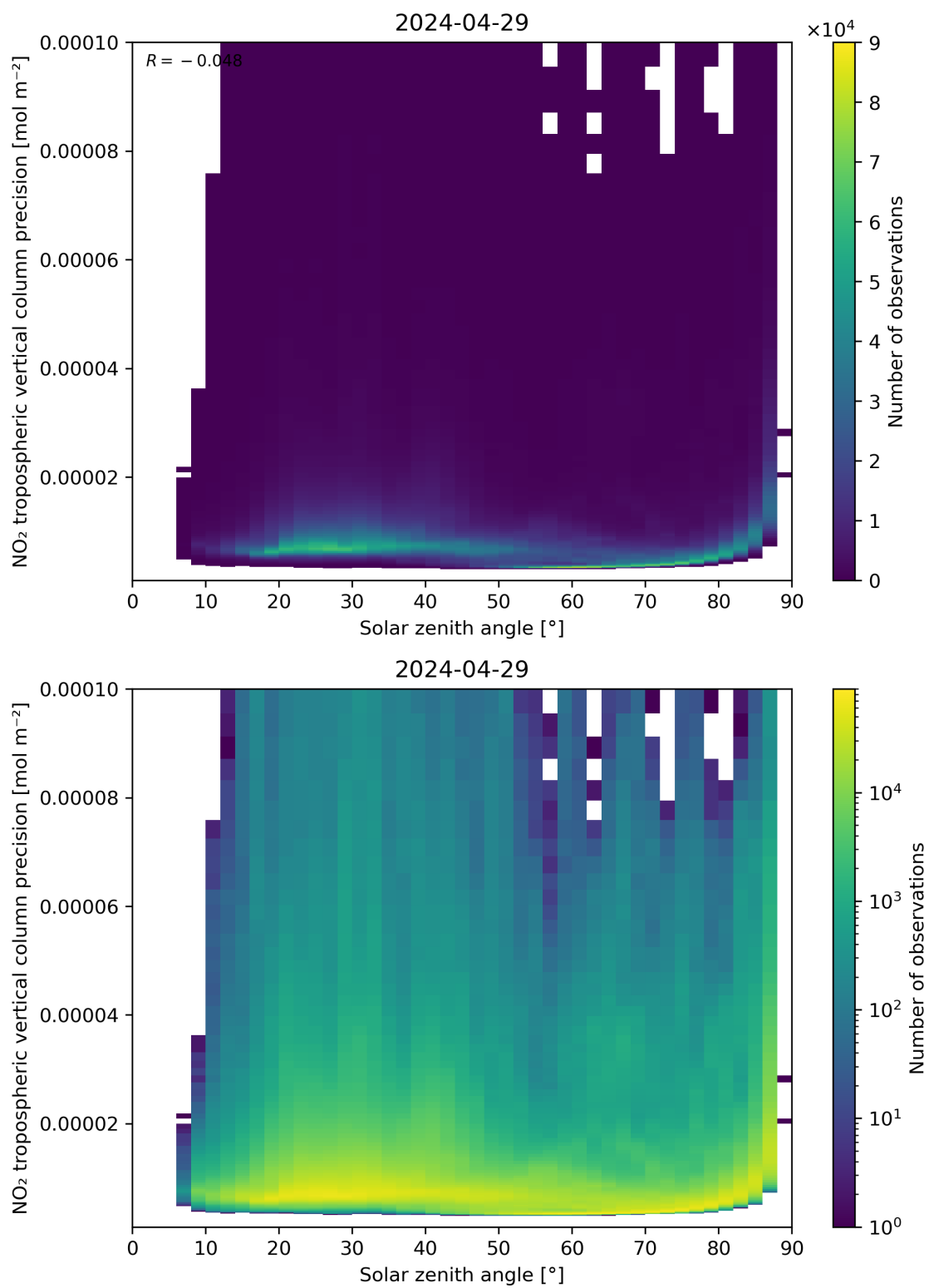
Figure 156: Scatter density plot of “Solar zenith angle” against “NO 2 tropospheric vertical column precision” for 2024-04-28 to 2024-04-30.
