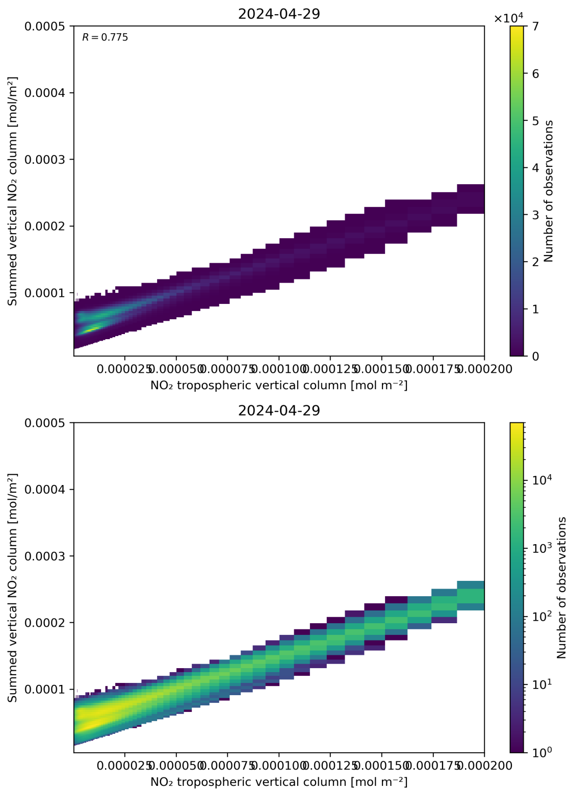
Figure 126: Scatter density plot of “NO 2 tropospheric vertical column” against “Summed vertical NO 2 column” for 2024-04-28 to 2024-04-30.
