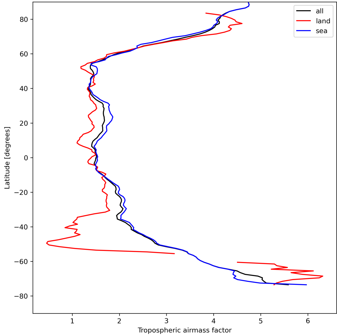
Figure 14: Zonal average of “Tropospheric airmass factor” for 2024-04-28 to 2024-04-30.
