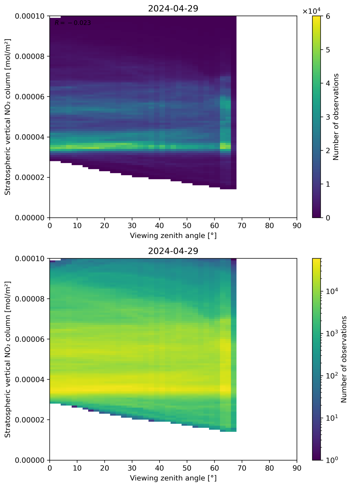
Figure 164: Scatter density plot of “Viewing zenith angle” against “Stratospheric vertical NO 2 column” for 2024-04-28 to 2024-04-30.
