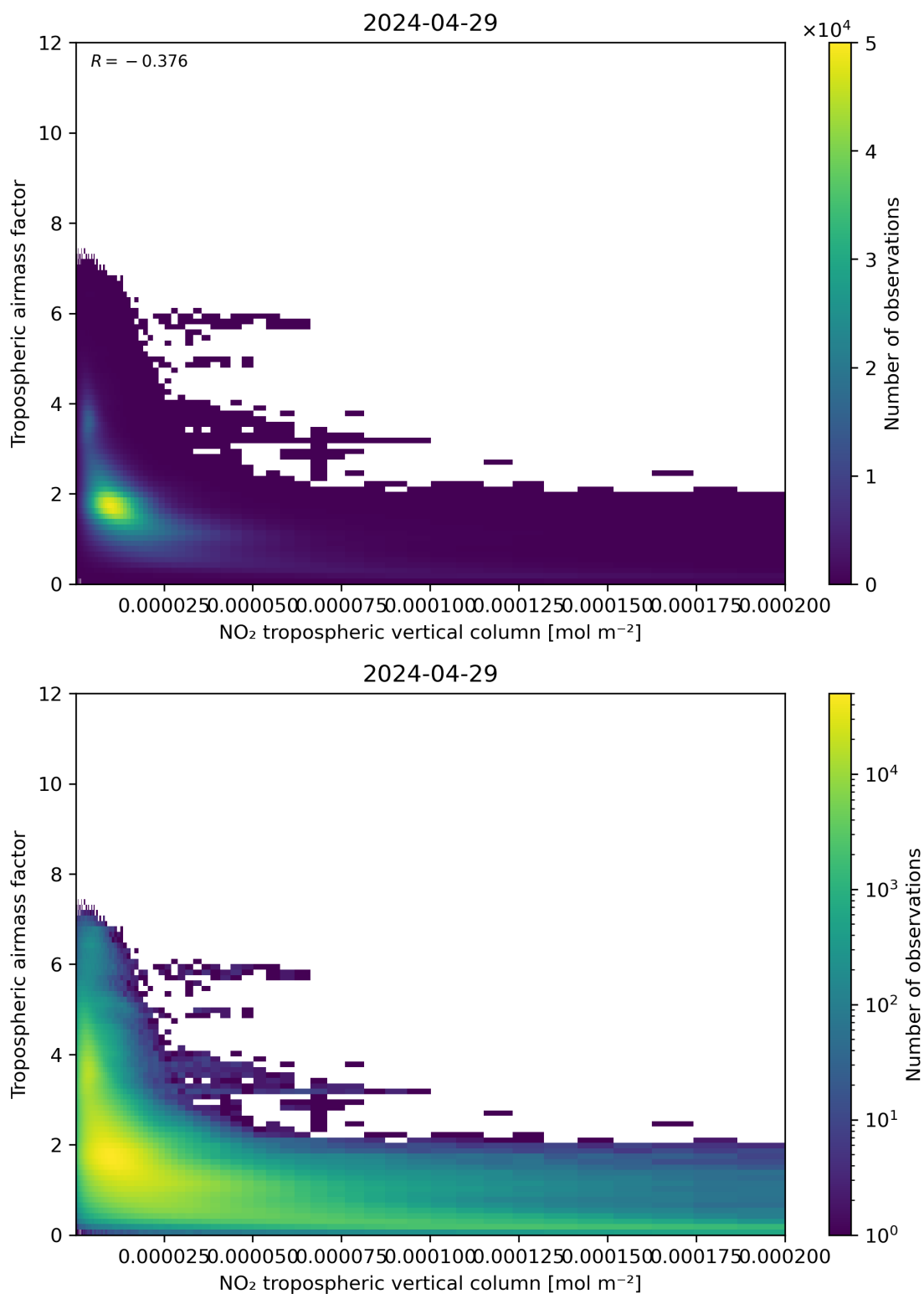
Figure 123: Scatter density plot of “NO 2 tropospheric vertical column” against “Tropospheric airmass factor” for 2024-04-28 to 2024-04-30.
