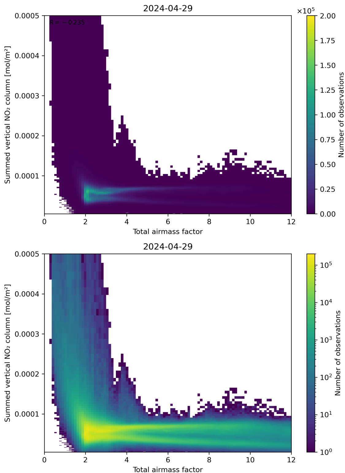
Figure 65: Scatter density plot of “Total airmass factor” against “Summed vertical NO 2 column” for 2024-04-28 to 2024-04-30.
