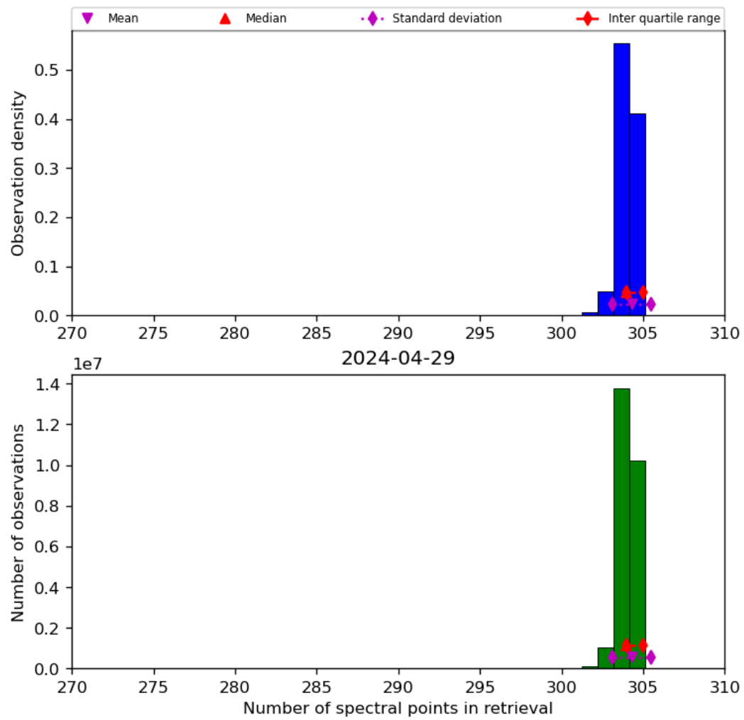
Figure 33: Histogram of “Number of spectral points in retrieval” for 2024-04-28 to 2024-04-30
