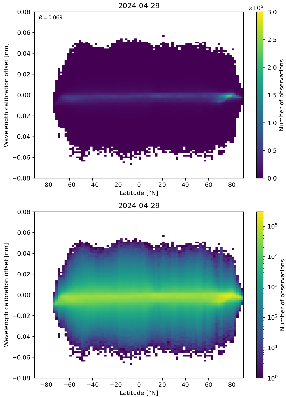
Figure 95: Scatter density plot of “Latitude” against “Wavelength calibration offset” for 2024-04-28 to 2024-04-30.
