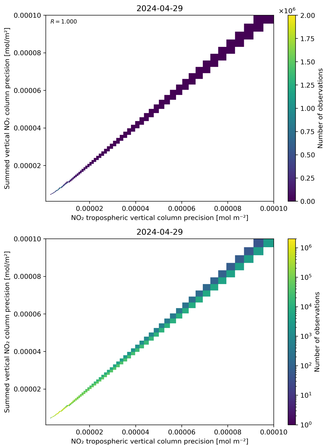
Figure 137: Scatter density plot of “NO 2 tropospheric vertical column precision” against “Summed vertical NO 2 column precision” for 2024-04-28 to 2024-04-30.
