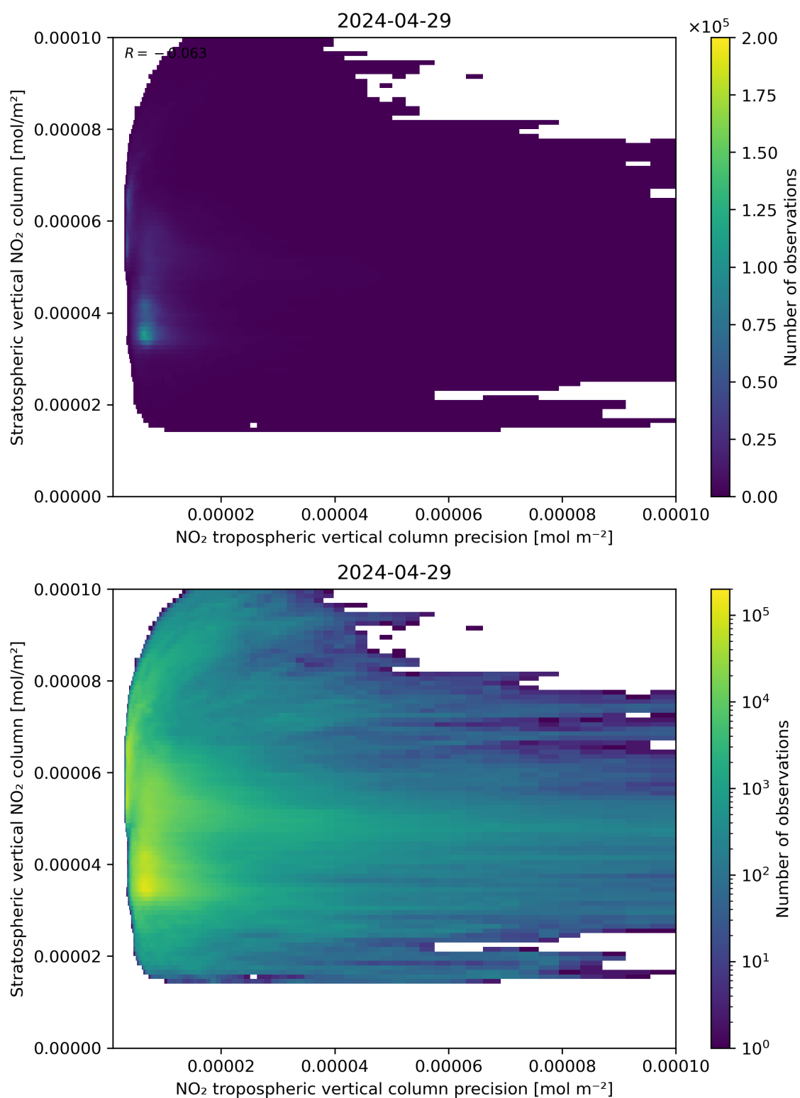
Figure 135: Scatter density plot of “NO 2 tropospheric vertical column precision” against “Stratospheric vertical NO 2 column” for 2024-04-28 to 2024-04-30.
