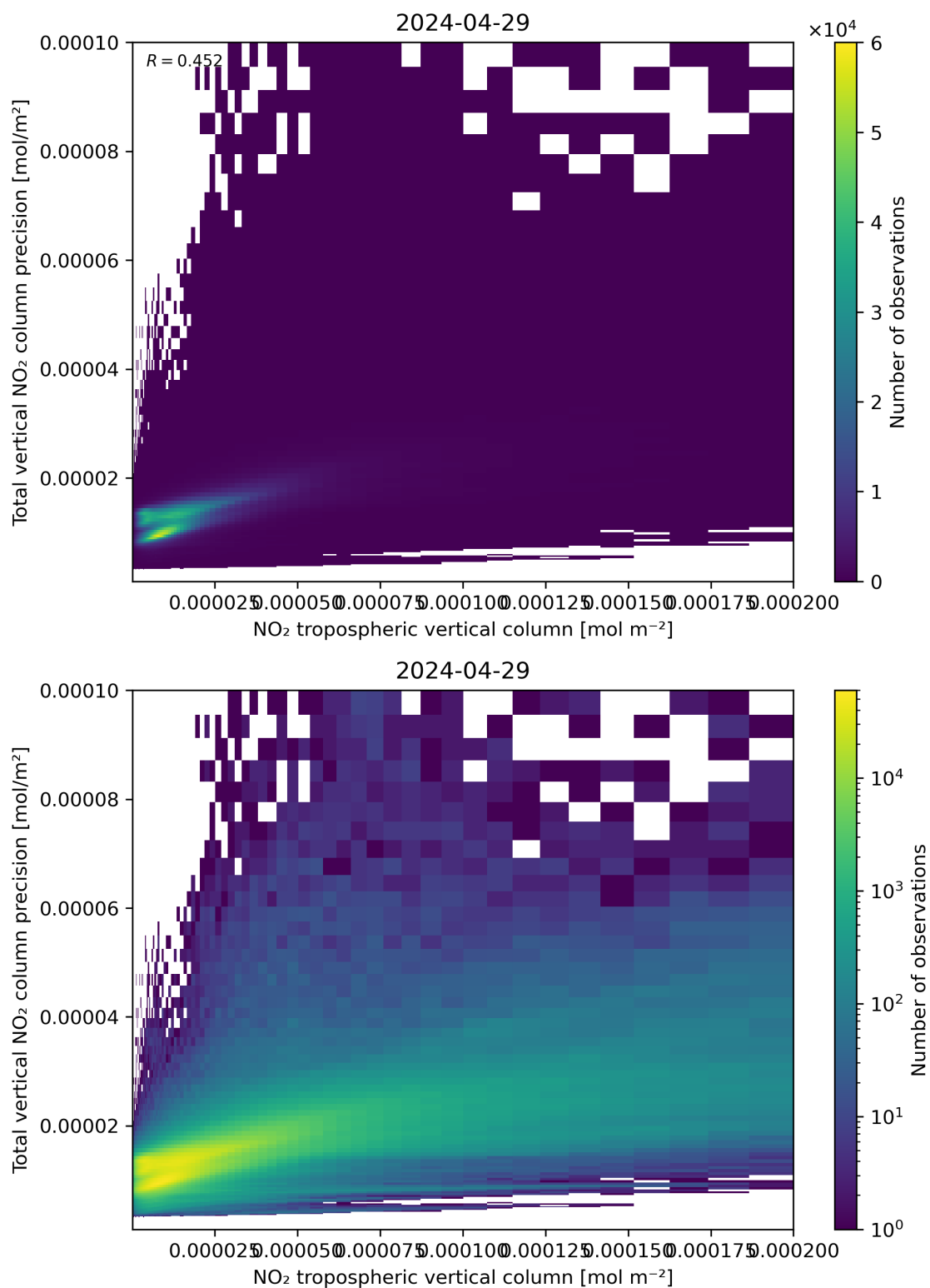
Figure 129: Scatter density plot of “NO 2 tropospheric vertical column” against “Total vertical NO 2 column precision” for 2024-04-28 to 2024-04-30.
