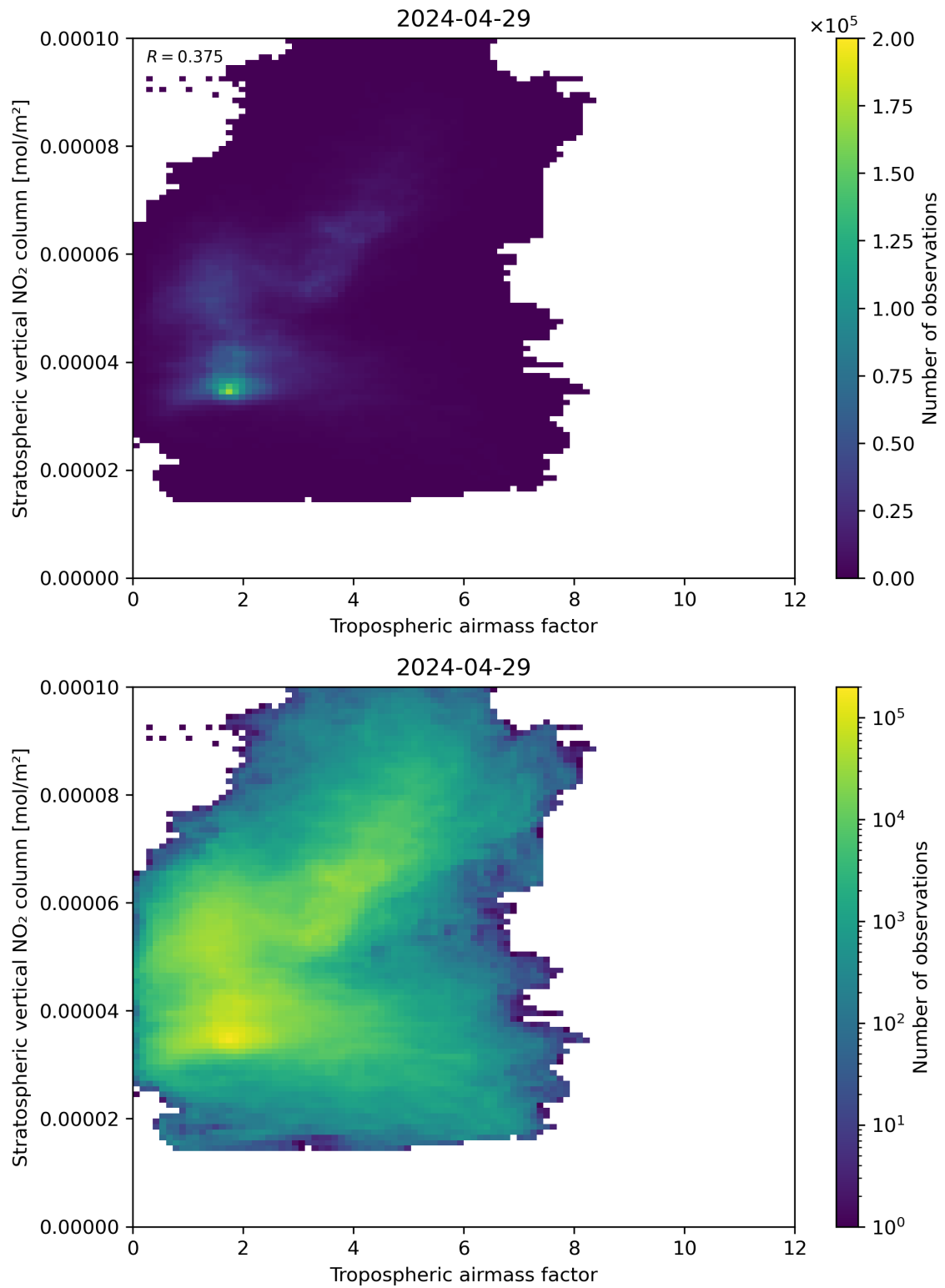
Figure 74: Scatter density plot of “Tropospheric air mass factor” against “Stratospheric vertical NO 2 column” for 2024-04-28 to 2024-04-30.
