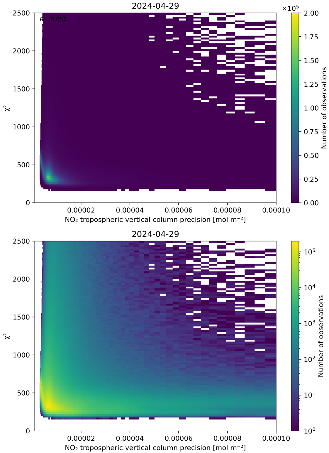
Figure 134: Scatter density plot of “NO 2 tropospheric vertical column precision” against “ \chi^2 ” for 2024-04-28 to 2024-04-30.
