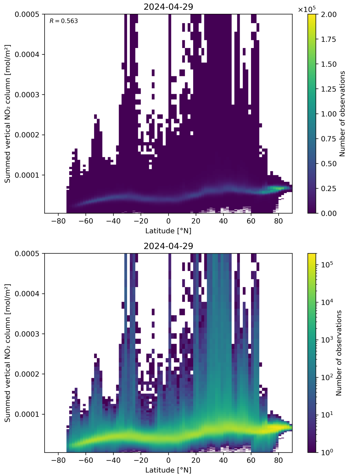
Figure 88: Scatter density plot of “Latitude” against “Summed vertical NO 2 column” for 2024-04-28 to 2024-04-30.
