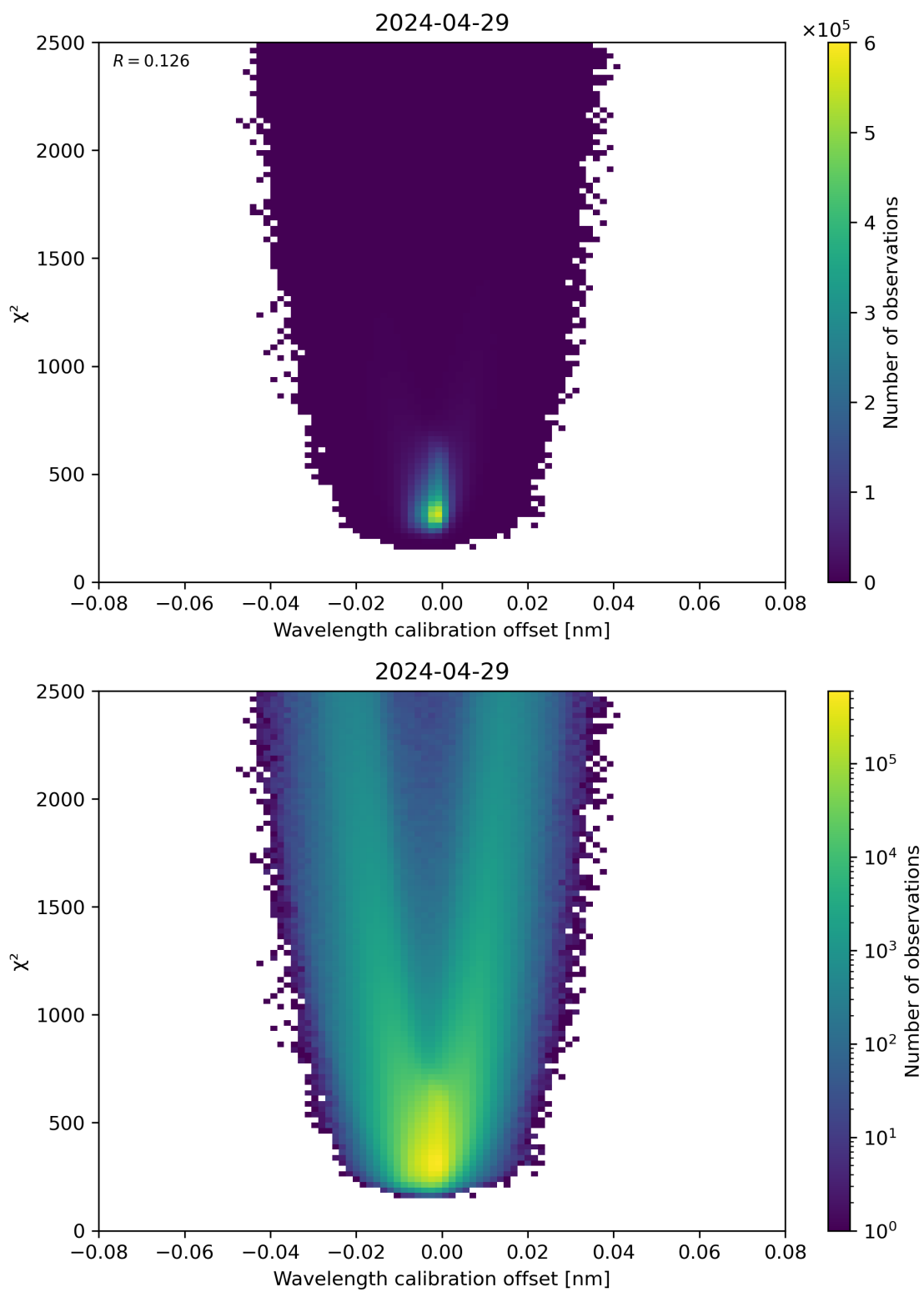
Figure 175: Scatter density plot of “Wavelength calibration offset” against “ \chi^2 ” for 2024-04-28 to 2024-04-30.
