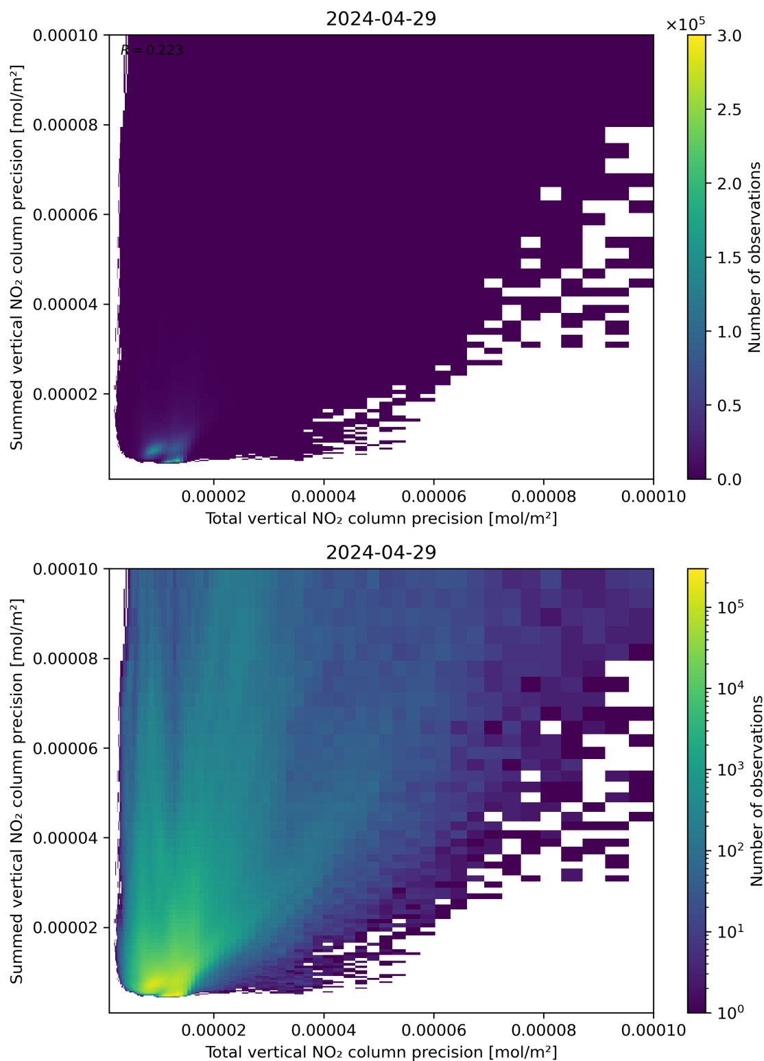
Figure 118: Scatter density plot of “Total vertical NO 2 column precision” against “Summed vertical NO 2 column precision” for 2024-04-28 to 2024-04-30.
