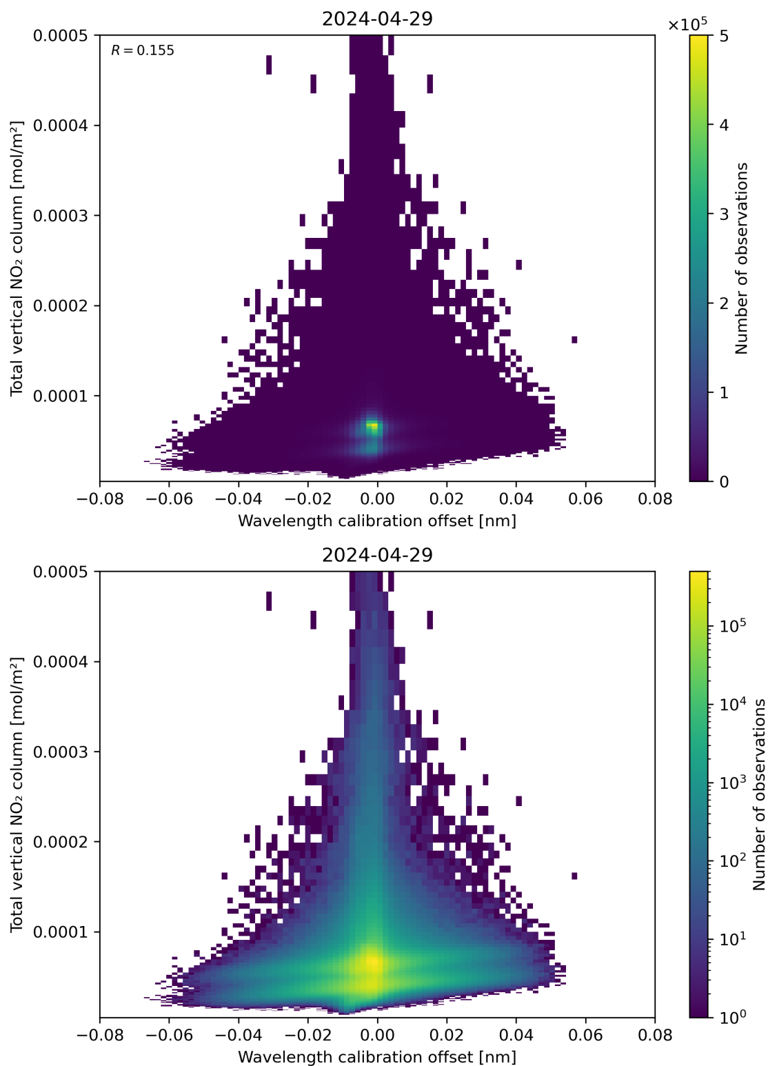
Figure 179: Scatter density plot of “Wavelength calibration offset” against “Total vertical NO 2 column” for 2024-04-28 to 2024-04-30.
