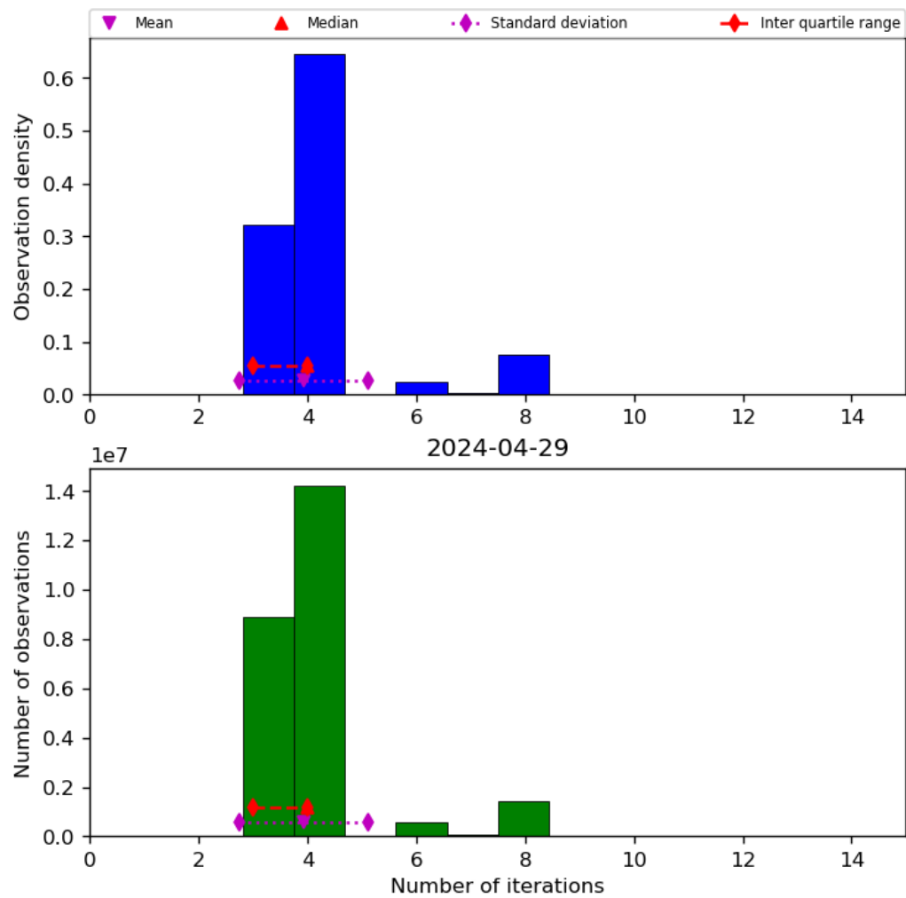
Figure 34: Histogram of “Number of iterations” for 2024-04-28 to 2024-04-30
