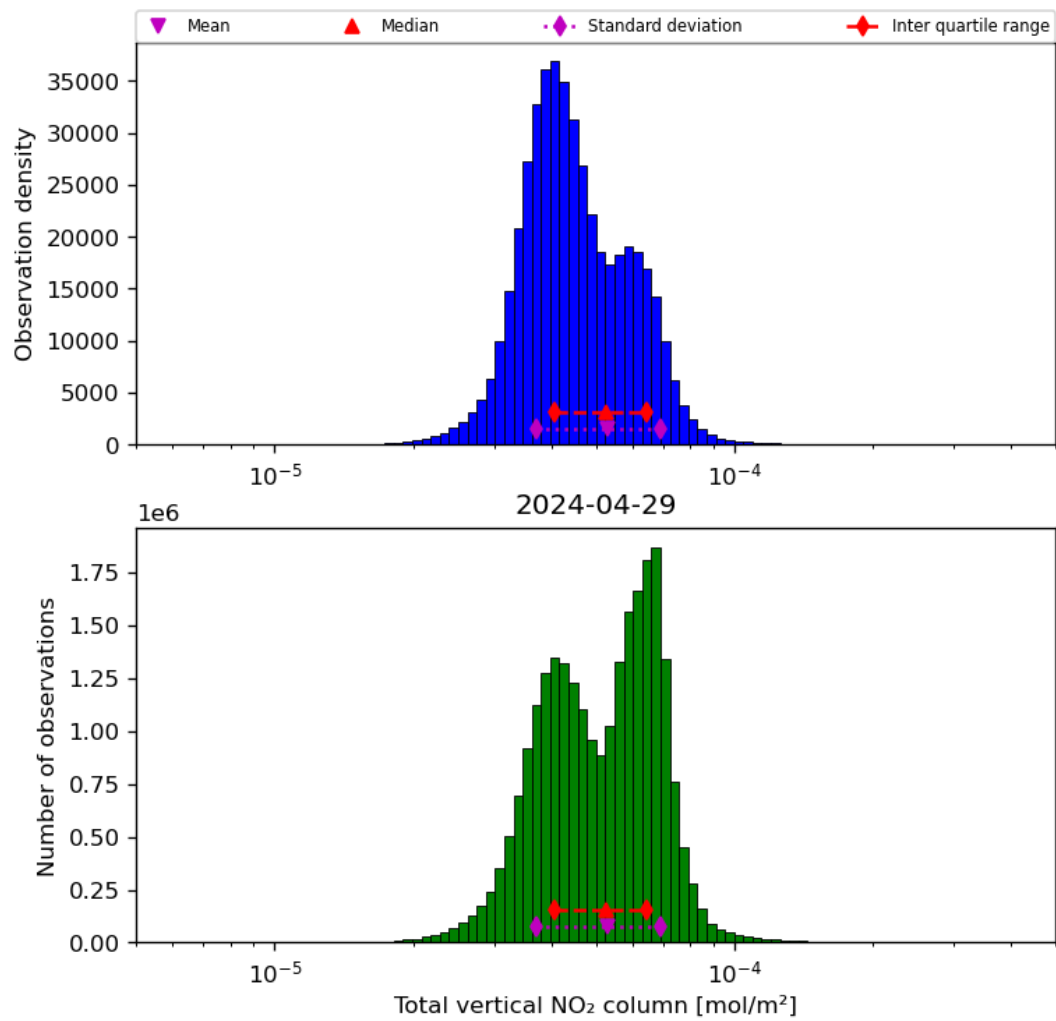
Figure 38: Histogram of "Total vertical NO 2 column" for 2024-04-28 to 2024-04-30
