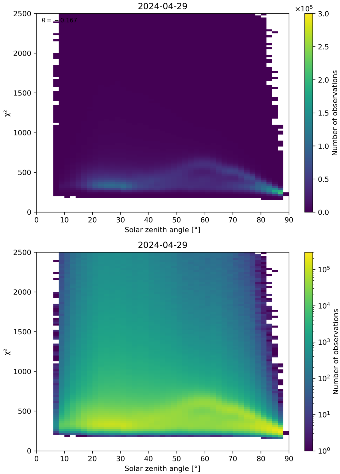
Figure 148: Scatter density plot of “Solar zenith angle” against “ \chi^2 ” for 2024-04-28 to 2024-04-30.
