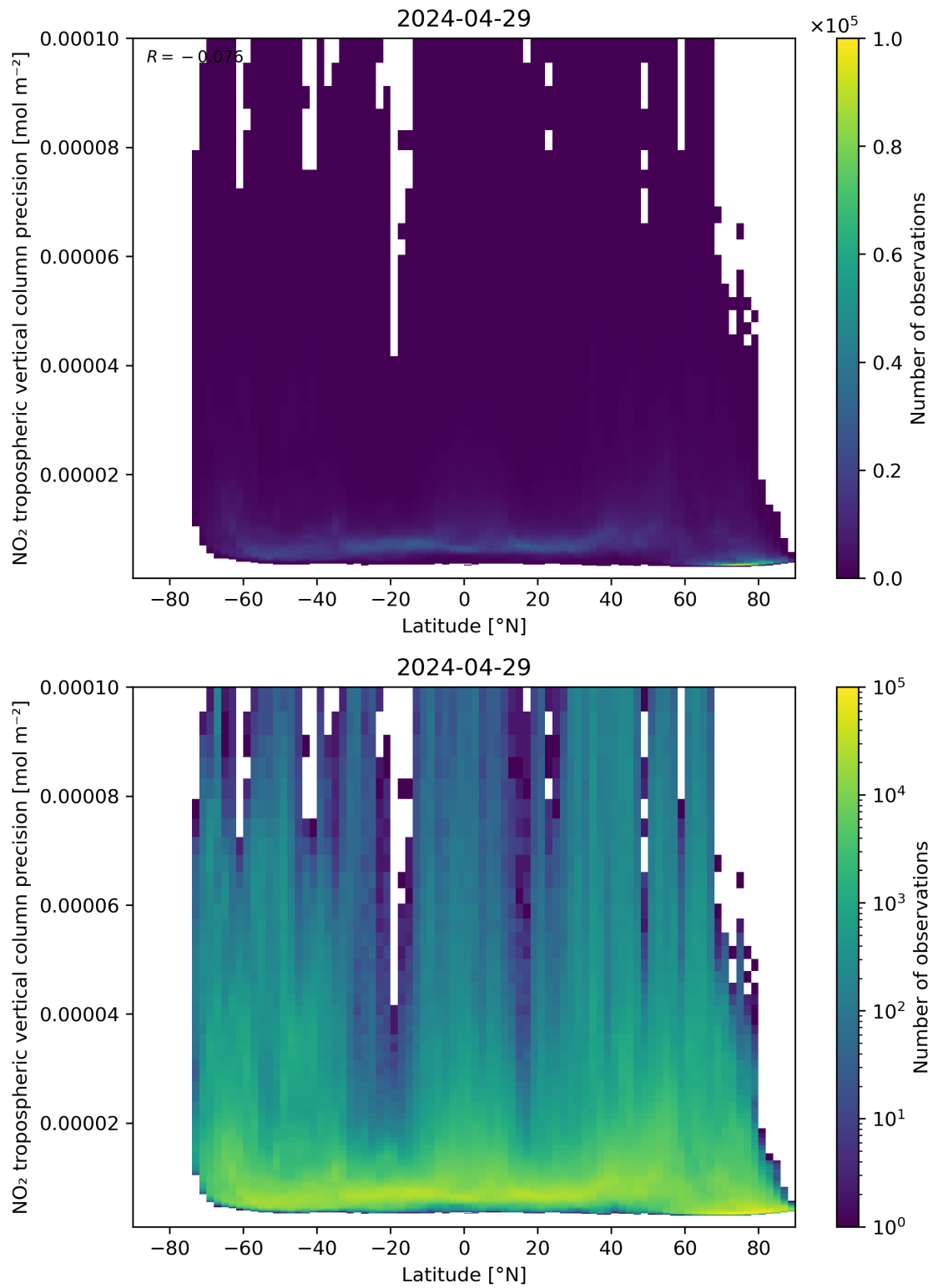
Figure 93: Scatter density plot of “Latitude” against “NO 2 tropospheric vertical column precision” for 2024-04-28 to 2024-04-30.
