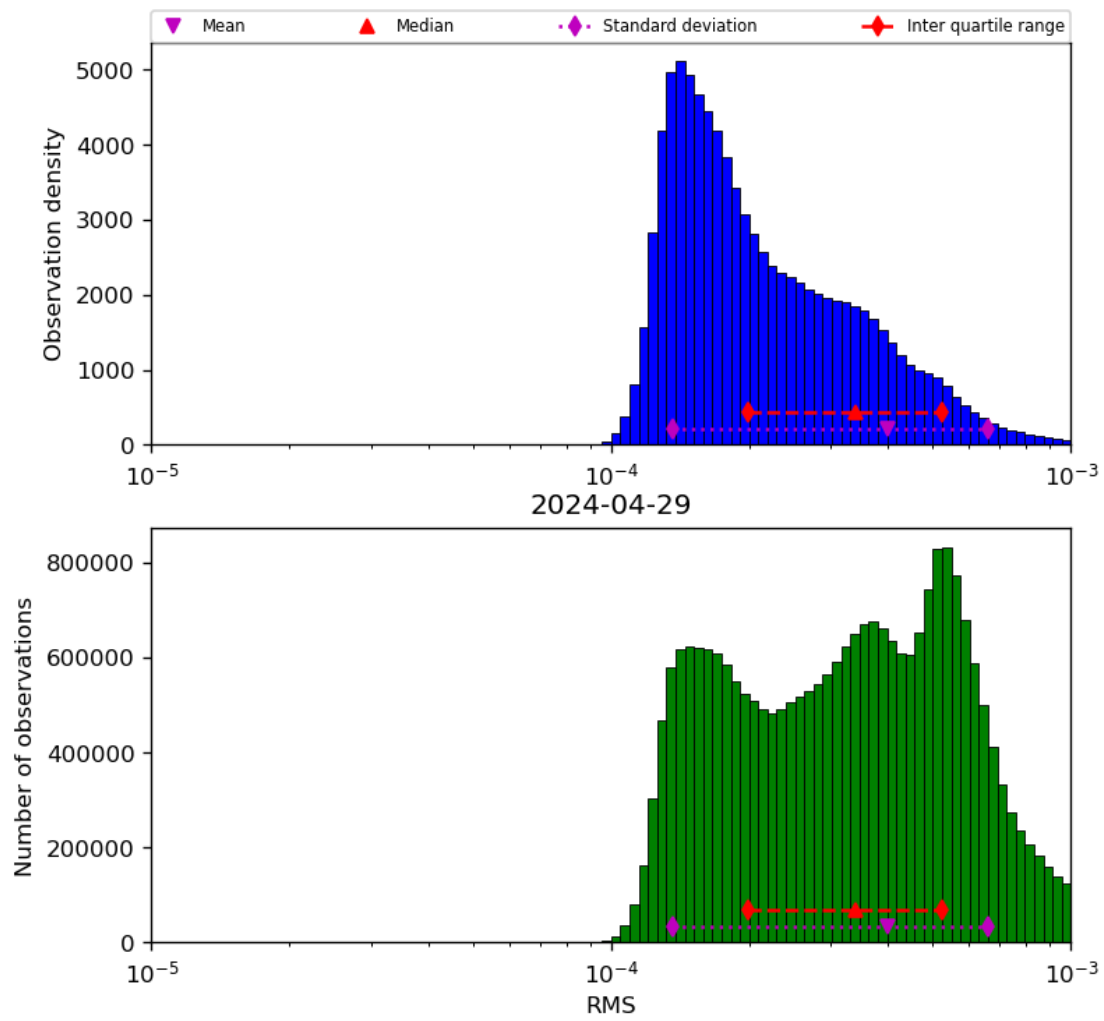
Figure 43: Histogram of “RMS” for 2024-04-28 to 2024-04-30
