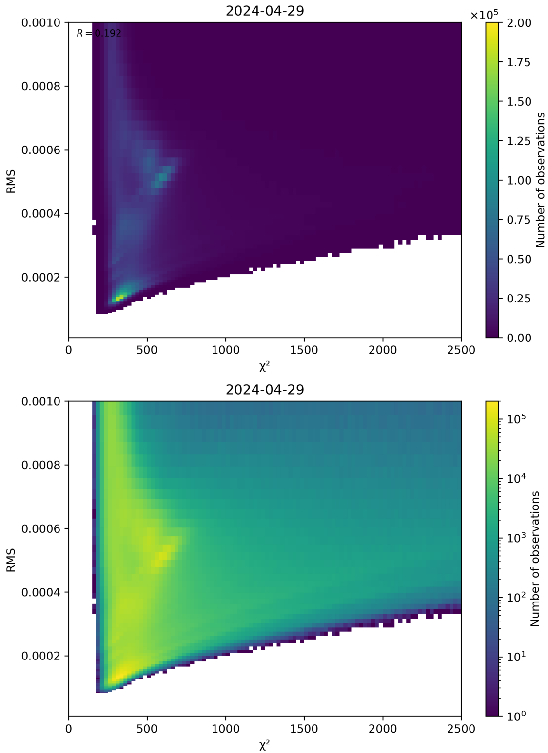
Figure 82: Scatter density plot of “ \chi^2 ” against “RMS” for 2024-04-28 to 2024-04-30.
