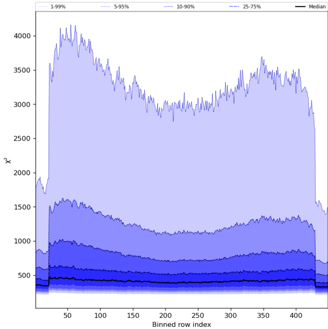
Figure 59: Along track statistics of “ \chi^2 ” for 2024-04-28 to 2024-04-30
