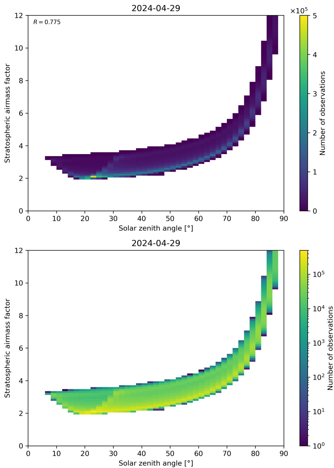
Figure 145: Scatter density plot of “Solar zenith angle” against “Stratospheric airmass factor” for 2024-04-28 to 2024-04-30.
