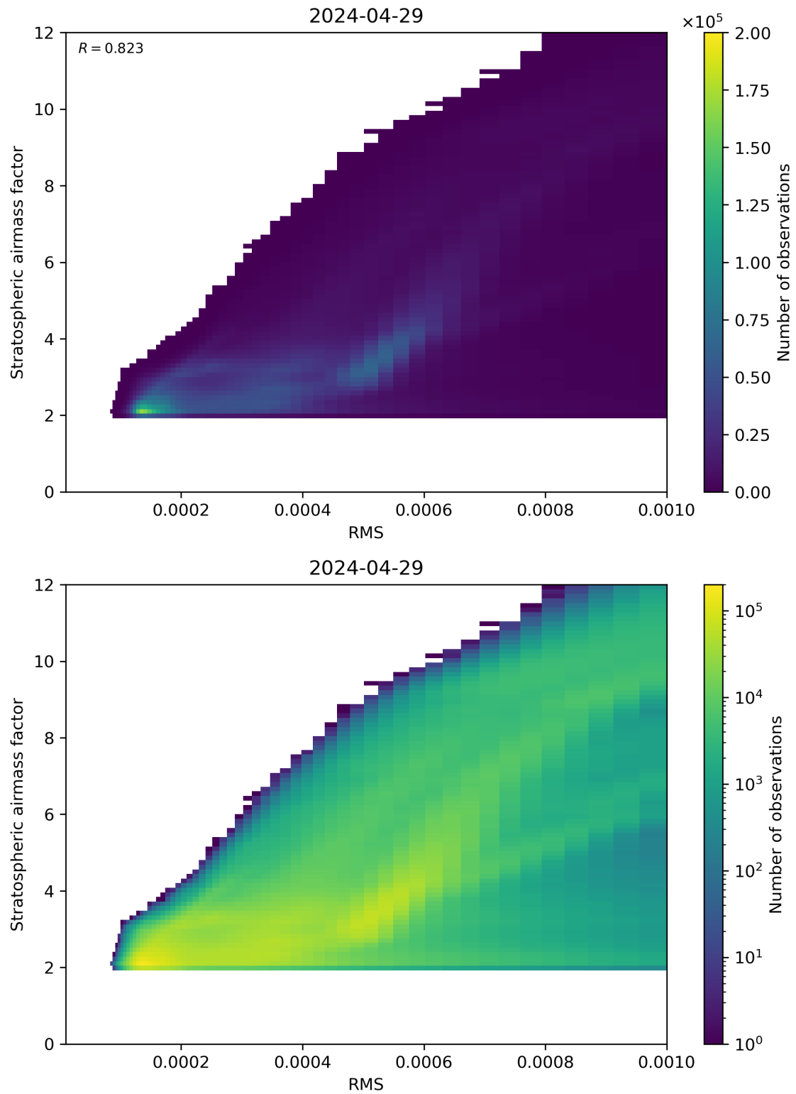
Figure 144: Scatter density plot of “RMS” against “Stratospheric airmass factor” for 2024-04-28 to 2024-04-30.
