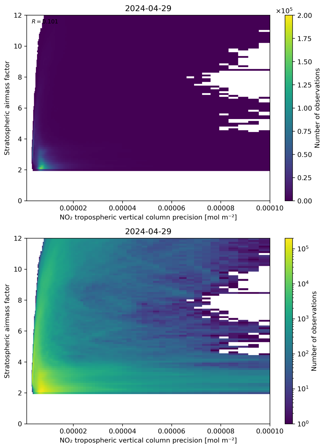
Figure 131: Scatter density plot of “NO 2 tropospheric vertical column precision” against “Stratospheric airmass factor” for 2024-04-28 to 2024-04-30.
