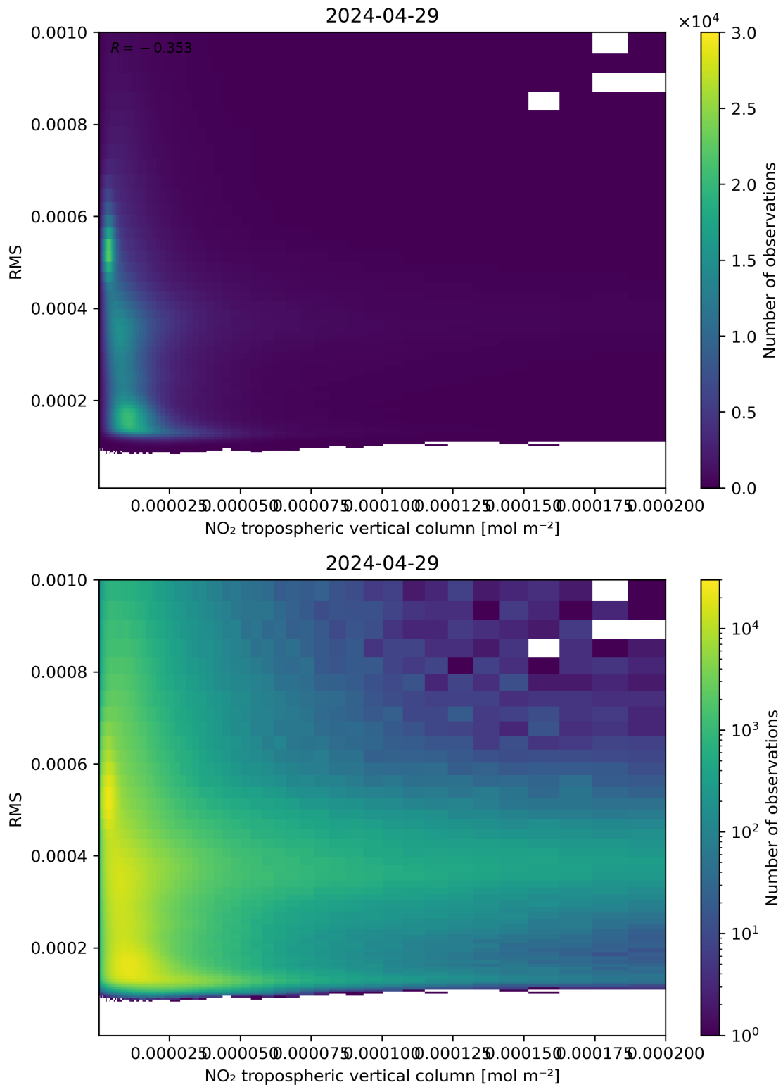
Figure 142: Scatter density plot of “NO 2 tropospheric vertical column” against “RMS” for 2024-04-28 to 2024-04-30.
