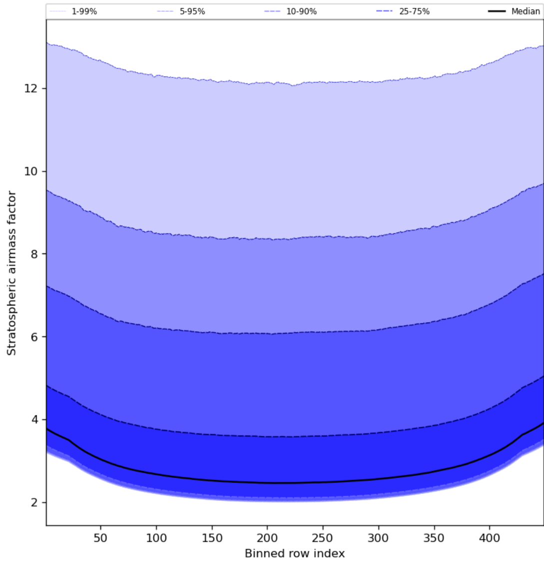
Figure 61: Along track statistics of “Stratospheric airmass factor” for 2024-04-28 to 2024-04-30
