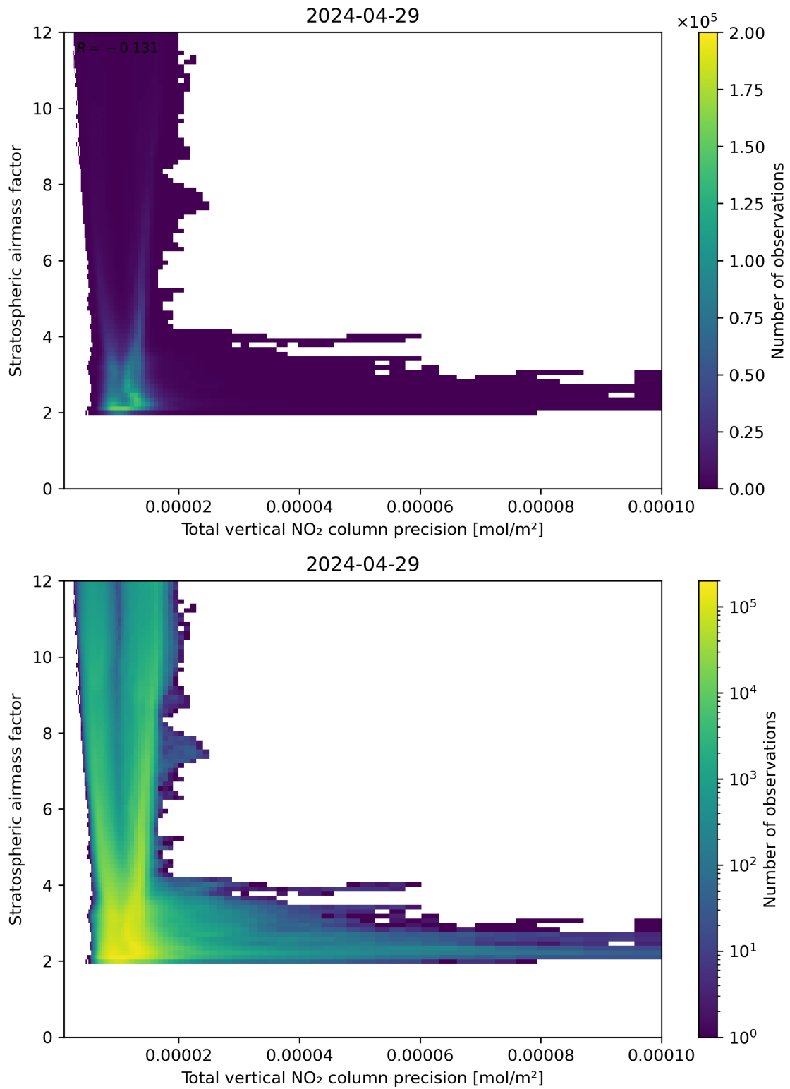
Figure 115: Scatter density plot of “Total vertical NO 2 column precision” against “Stratospheric air mass factor” for 2024-04-28 to 2024-04-30.
