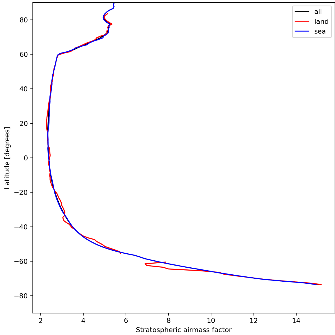
Figure 27: Zonal average of “Stratospheric airmass factor” for 2024-04-28 to 2024-04-30.
