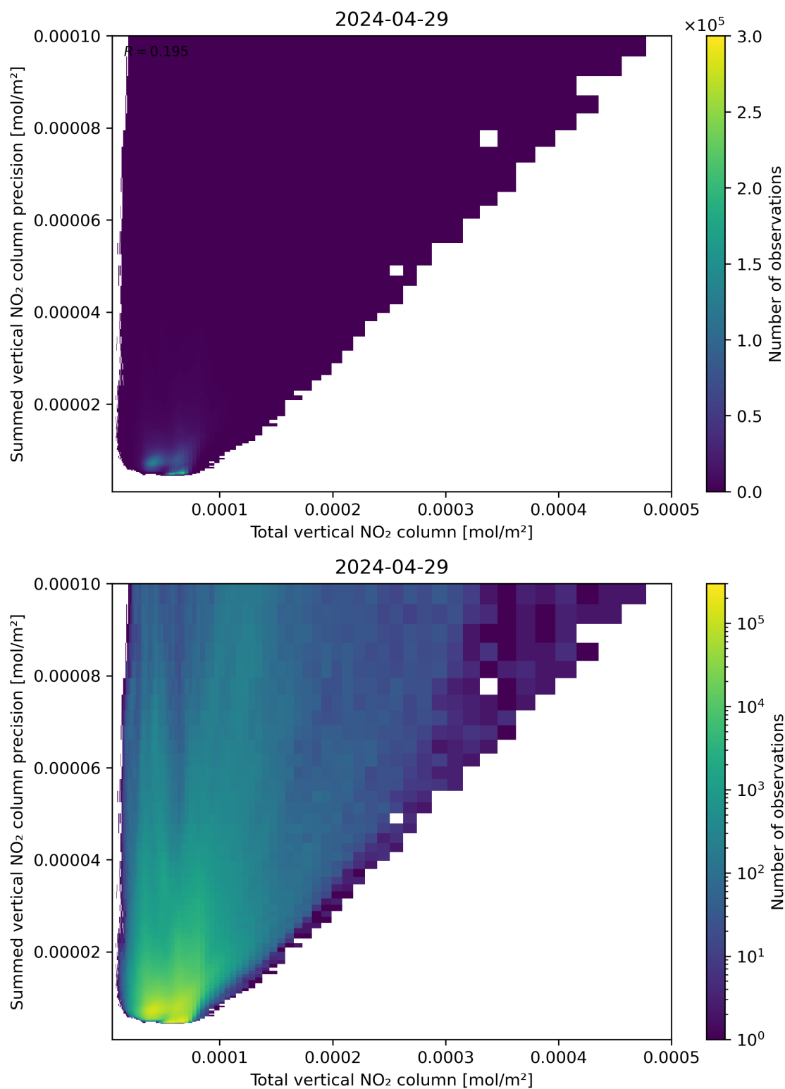
Figure 113: Scatter density plot of “Total vertical NO 2 column” against “Summed vertical NO 2 column precision” for 2024-04-28 to 2024-04-30.
