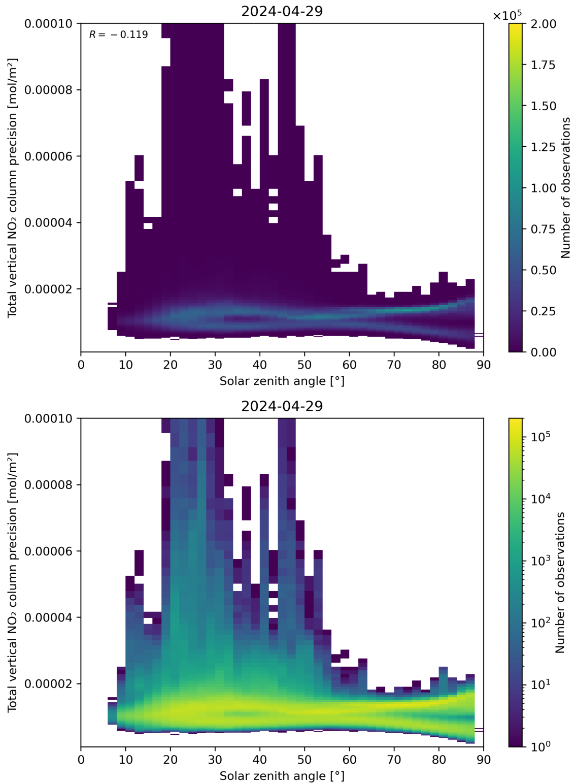
Figure 154: Scatter density plot of “Solar zenith angle” against “Total vertical NO 2 column precision” for 2024-04-28 to 2024-04-30.
