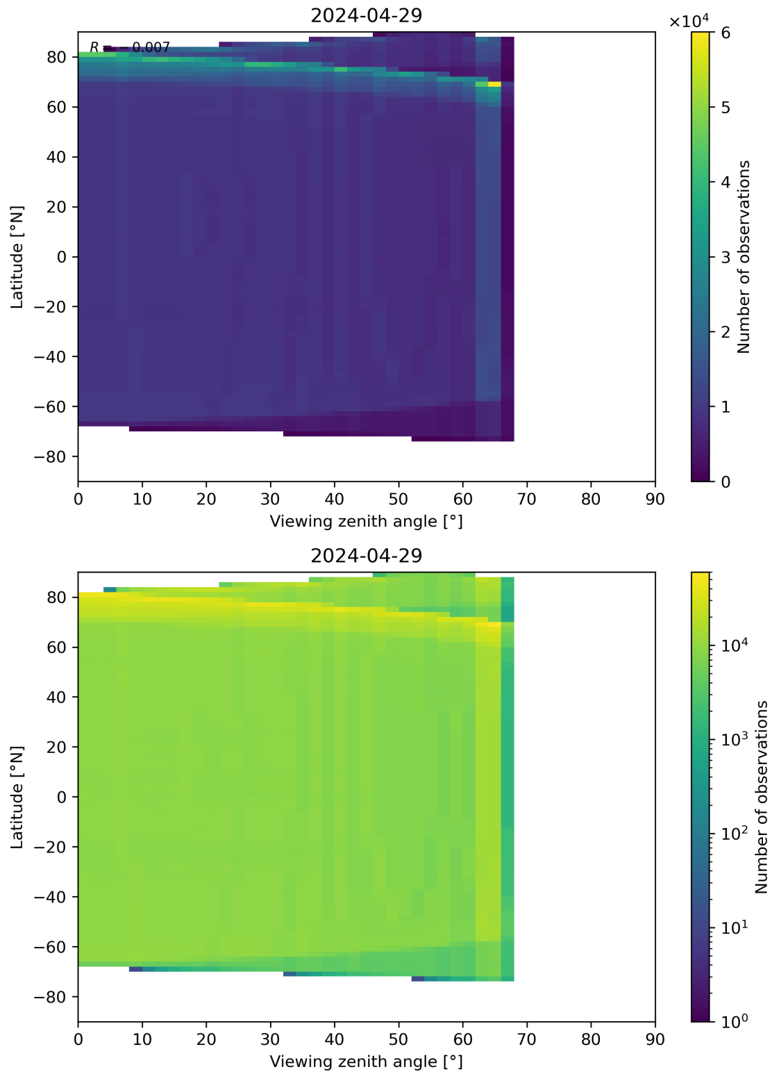
Figure 163: Scatter density plot of “Viewing zenith angle” against “Latitude” for 2024-04-28 to 2024-04-30.
