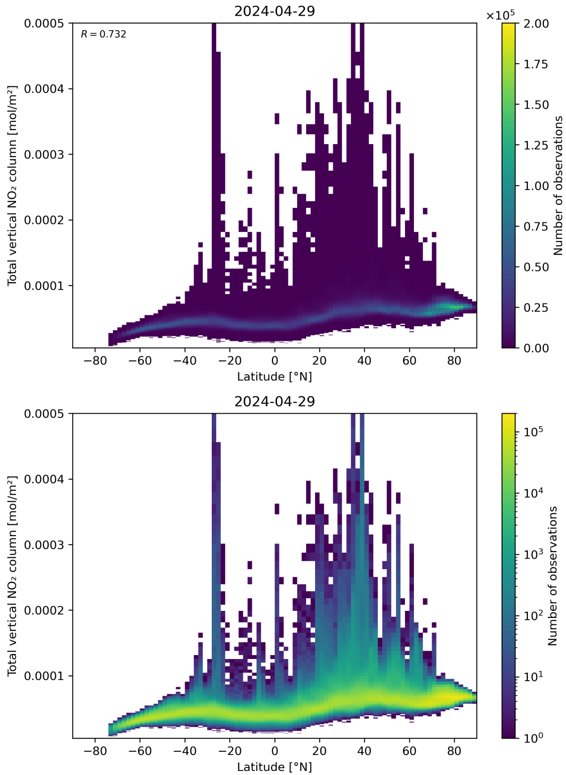
Figure 90: Scatter density plot of “Latitude” against “Total vertical NO 2 column” for 2024-04-28 to 2024-04-30.
