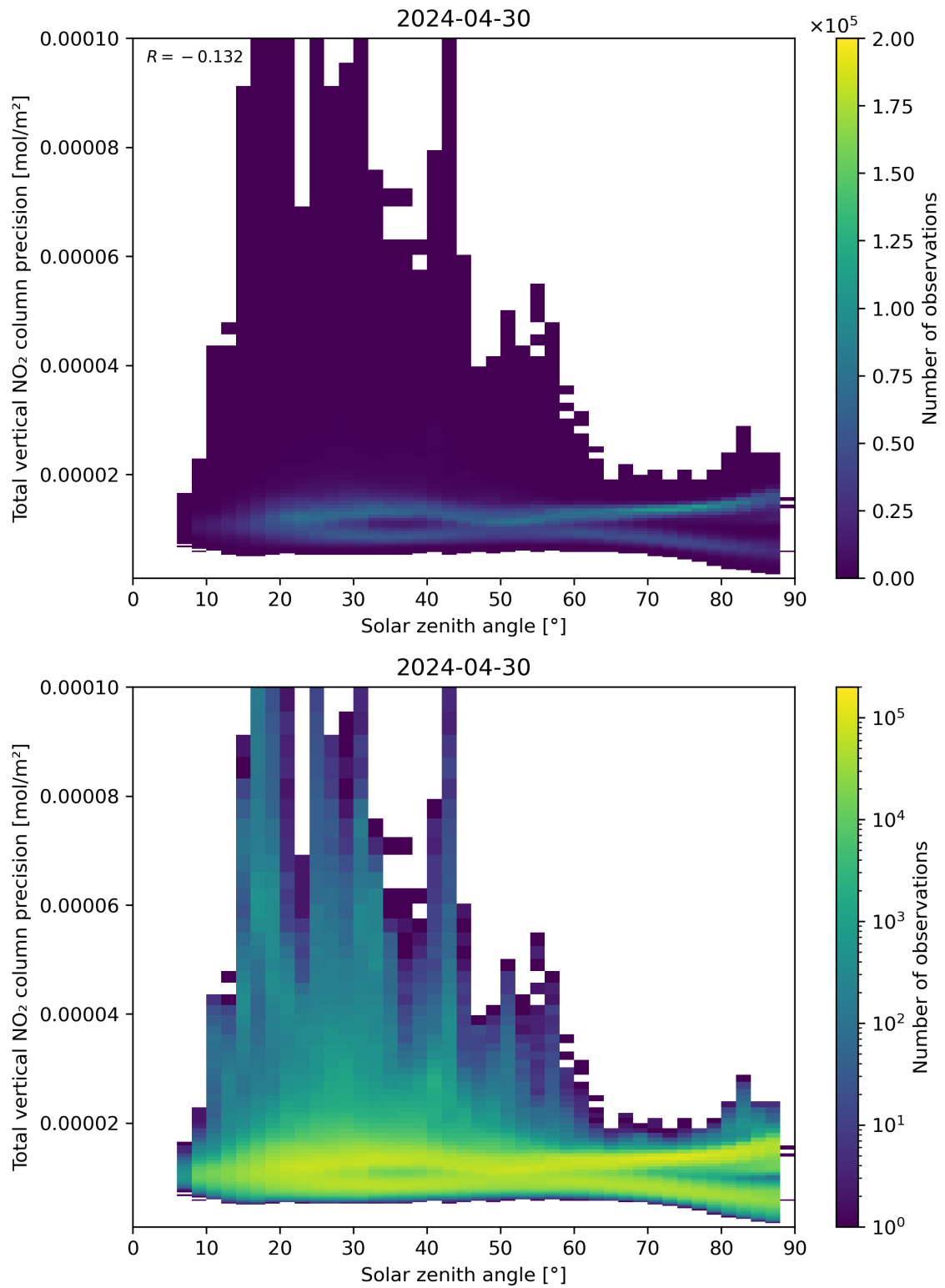
Figure 154: Scatter density plot of “Solar zenith angle” against “Total vertical NO 2 column precision” for 2024-04-29 to 2024-05-01.
