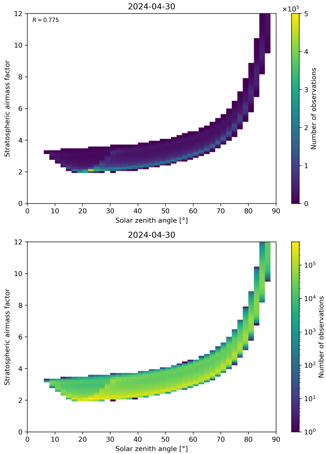
Figure 145: Scatter density plot of “Solar zenith angle” against “Stratospheric airmass factor” for 2024-04-29 to 2024-05-01.
