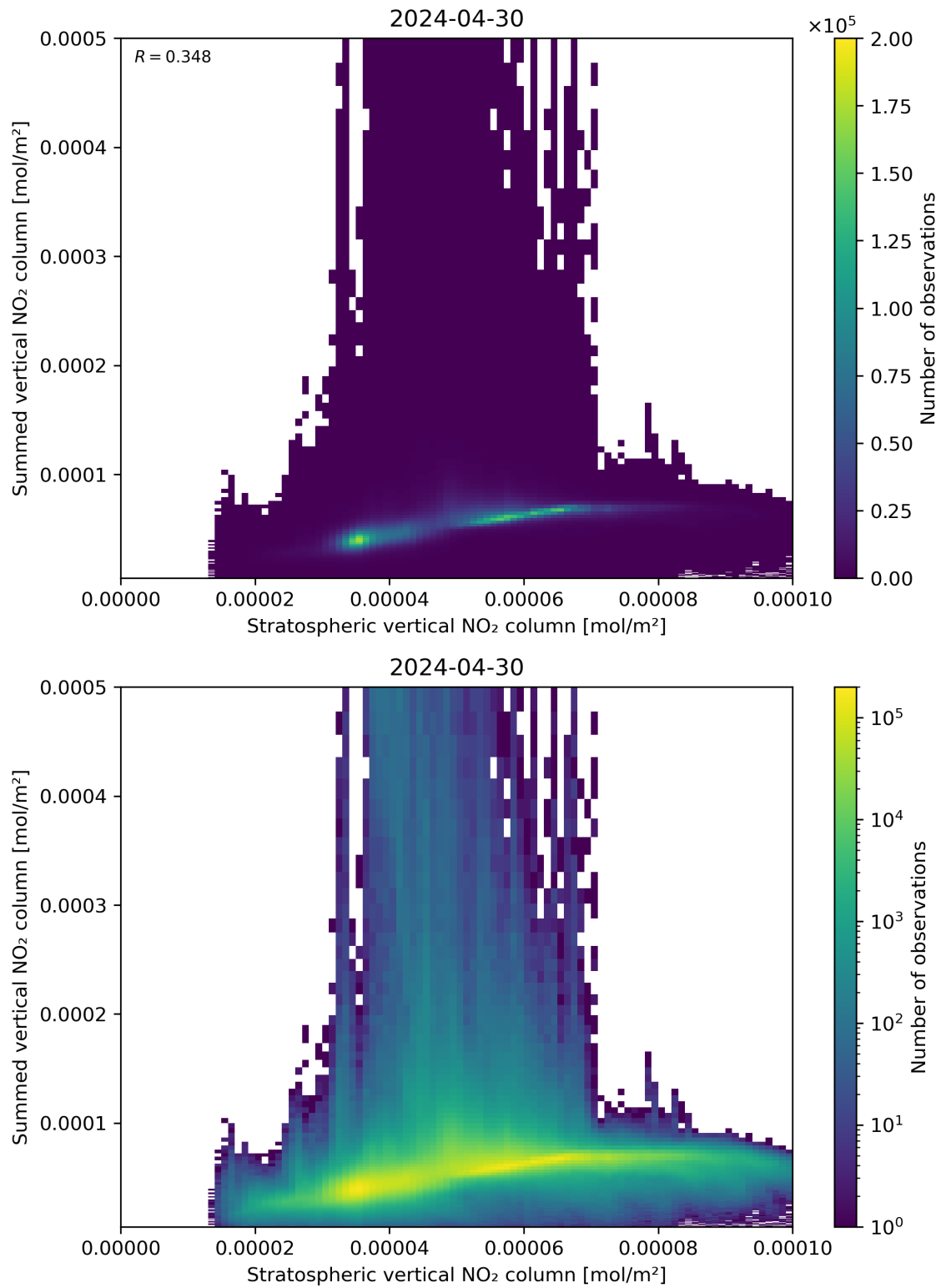
Figure 98: Scatter density plot of “Stratospheric vertical NO 2 column” against “Summed vertical NO 2 column” for 2024-04-29 to 2024-05-01.
