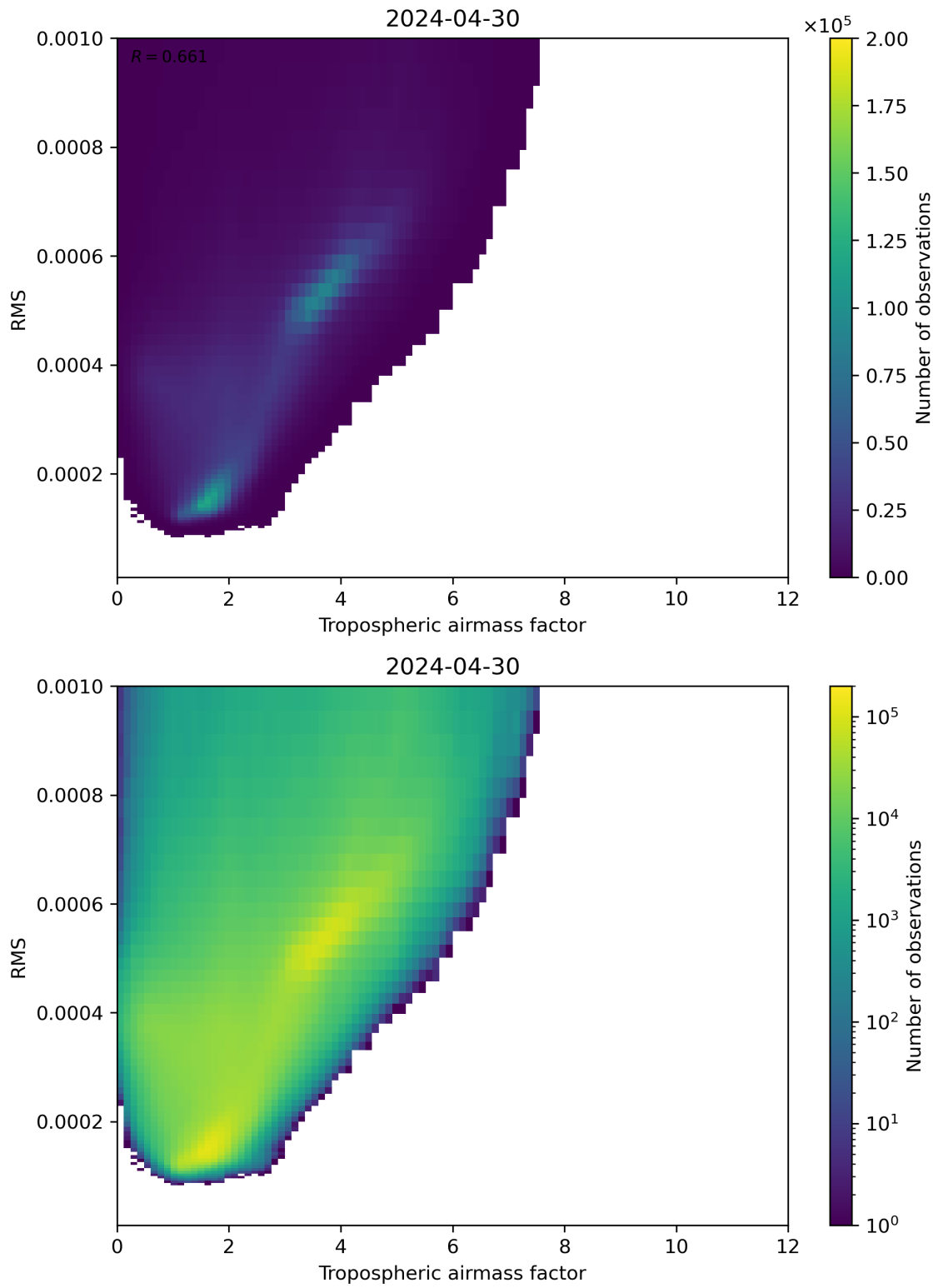
Figure 79: Scatter density plot of “Tropospheric airmass factor” against “RMS” for 2024-04-29 to 2024-05-01.
