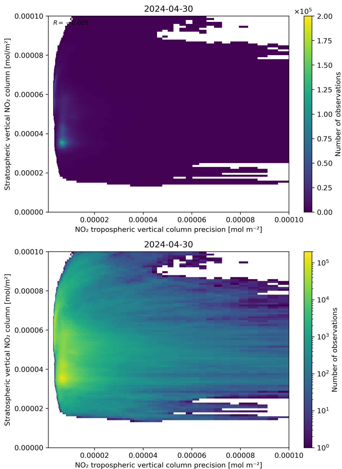
Figure 135: Scatter density plot of “NO 2 tropospheric vertical column precision” against “Stratospheric vertical NO 2 column” for 2024-04-29 to 2024-05-01.
