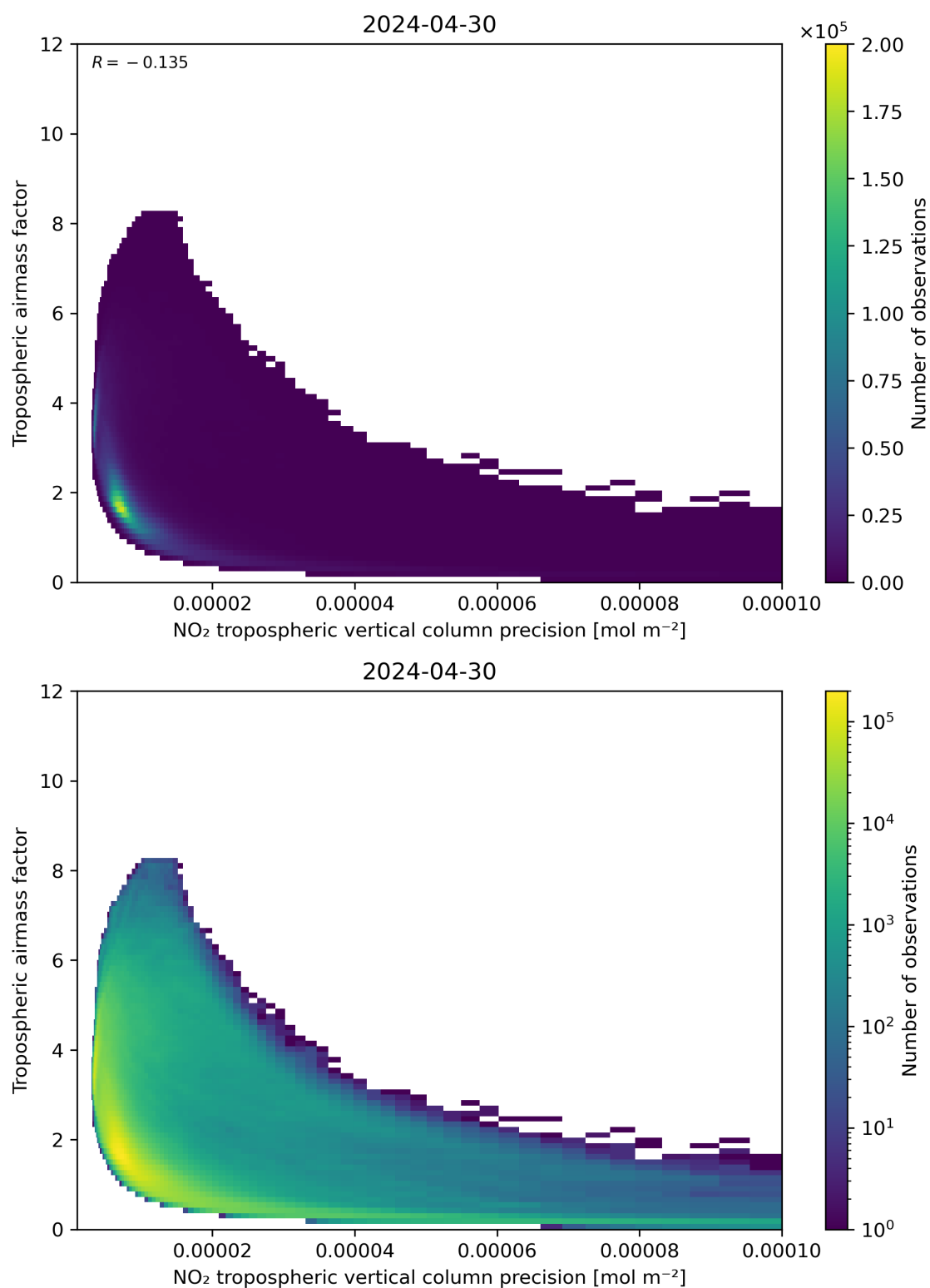
Figure 133: Scatter density plot of “NO 2 tropospheric vertical column precision” against “Tropospheric airmass factor” for 2024-04-29 to 2024-05-01.
