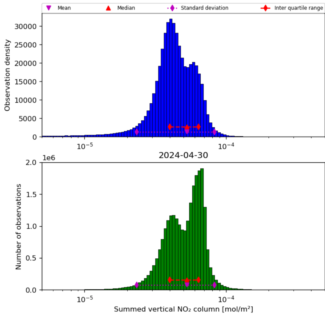
Figure 40: Histogram of “Summed vertical NO 2 column” for 2024-04-29 to 2024-05-01
