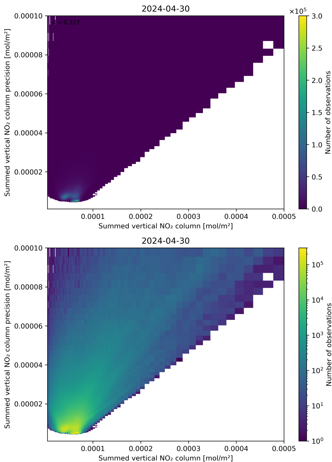
Figure 105: Scatter density plot of “Summed vertical NO 2 column” against “Summed vertical NO 2 column precision” for 2024-04-29 to 2024-05-01.
