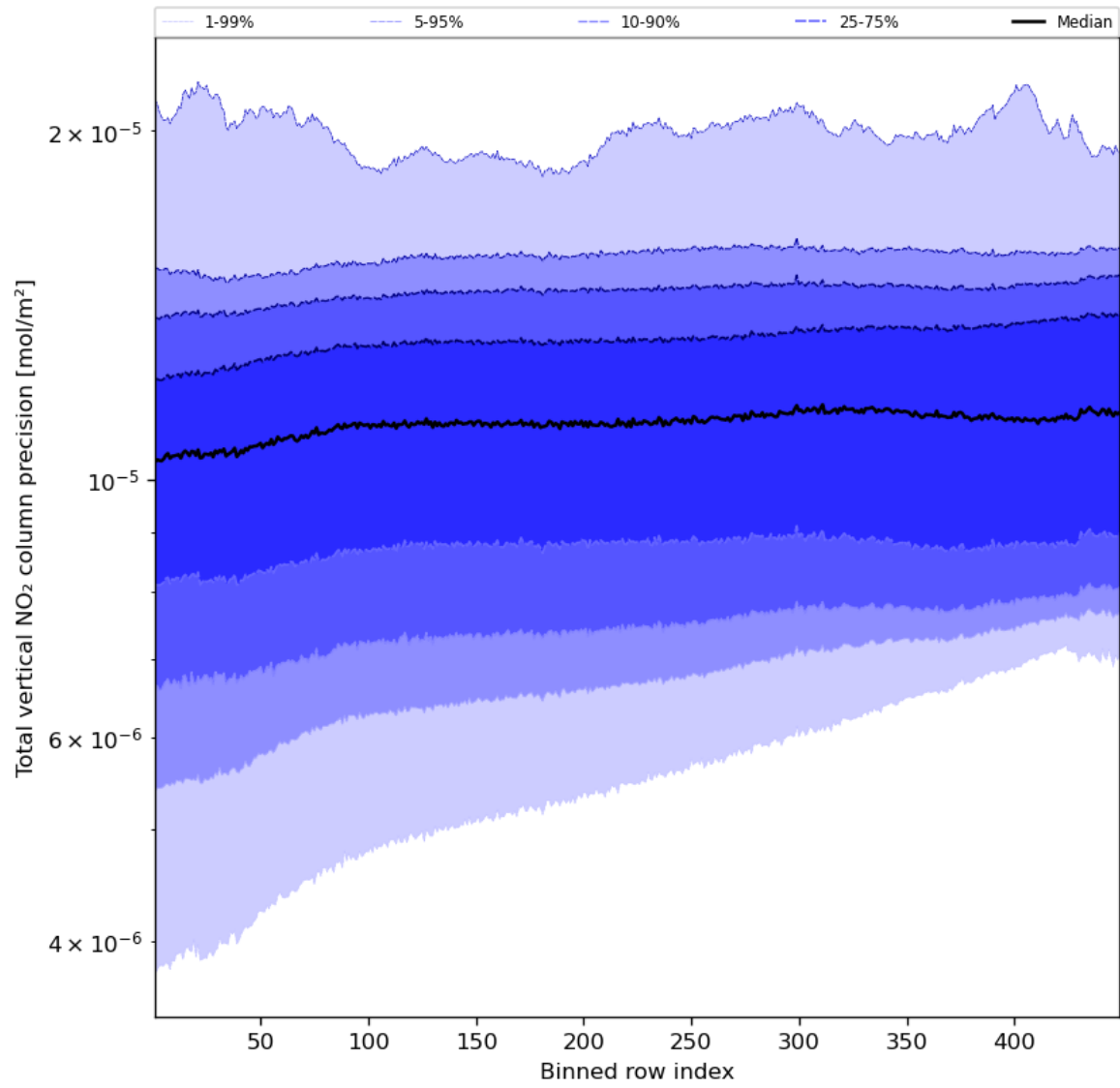
Figure 56: Along track statistics of “Total vertical NO 2 column precision” for 2024-04-29 to 2024-05-01
