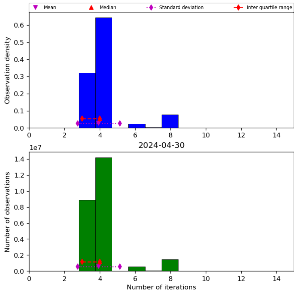
Figure 34: Histogram of “Number of iterations” for 2024-04-29 to 2024-05-01
