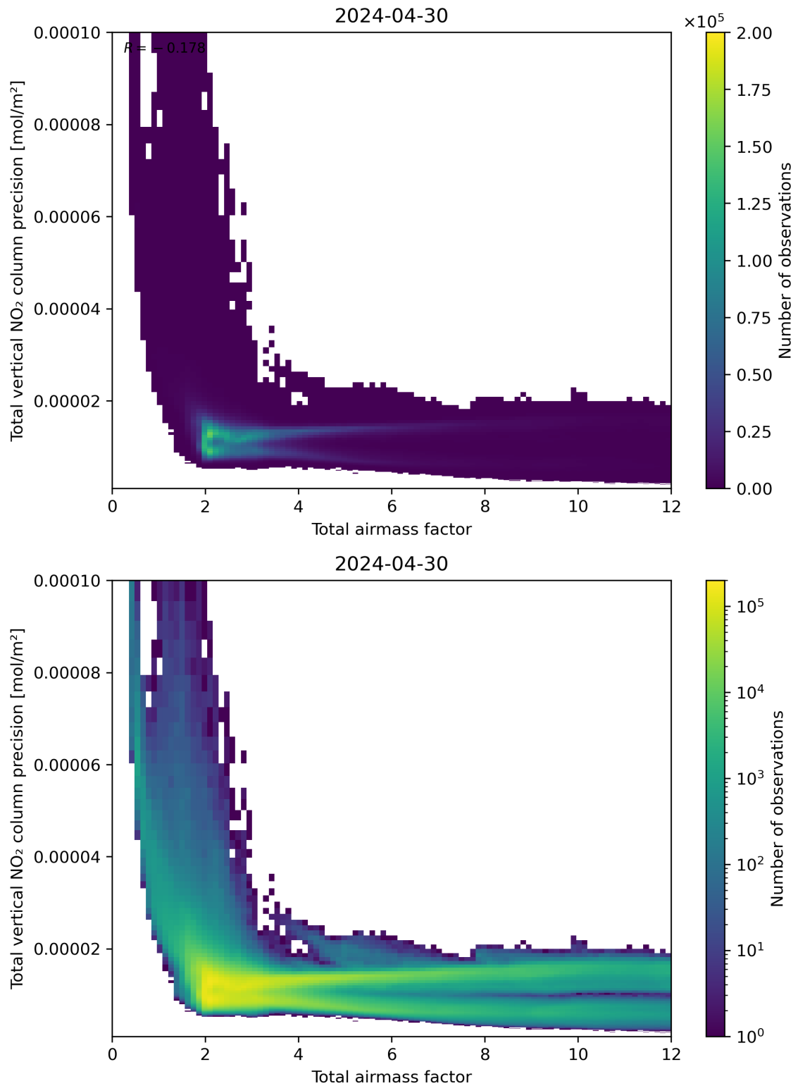
Figure 68: Scatter density plot of “Total airmass factor” against “Total vertical NO 2 column precision” for 2024-04-29 to 2024-05-01.
