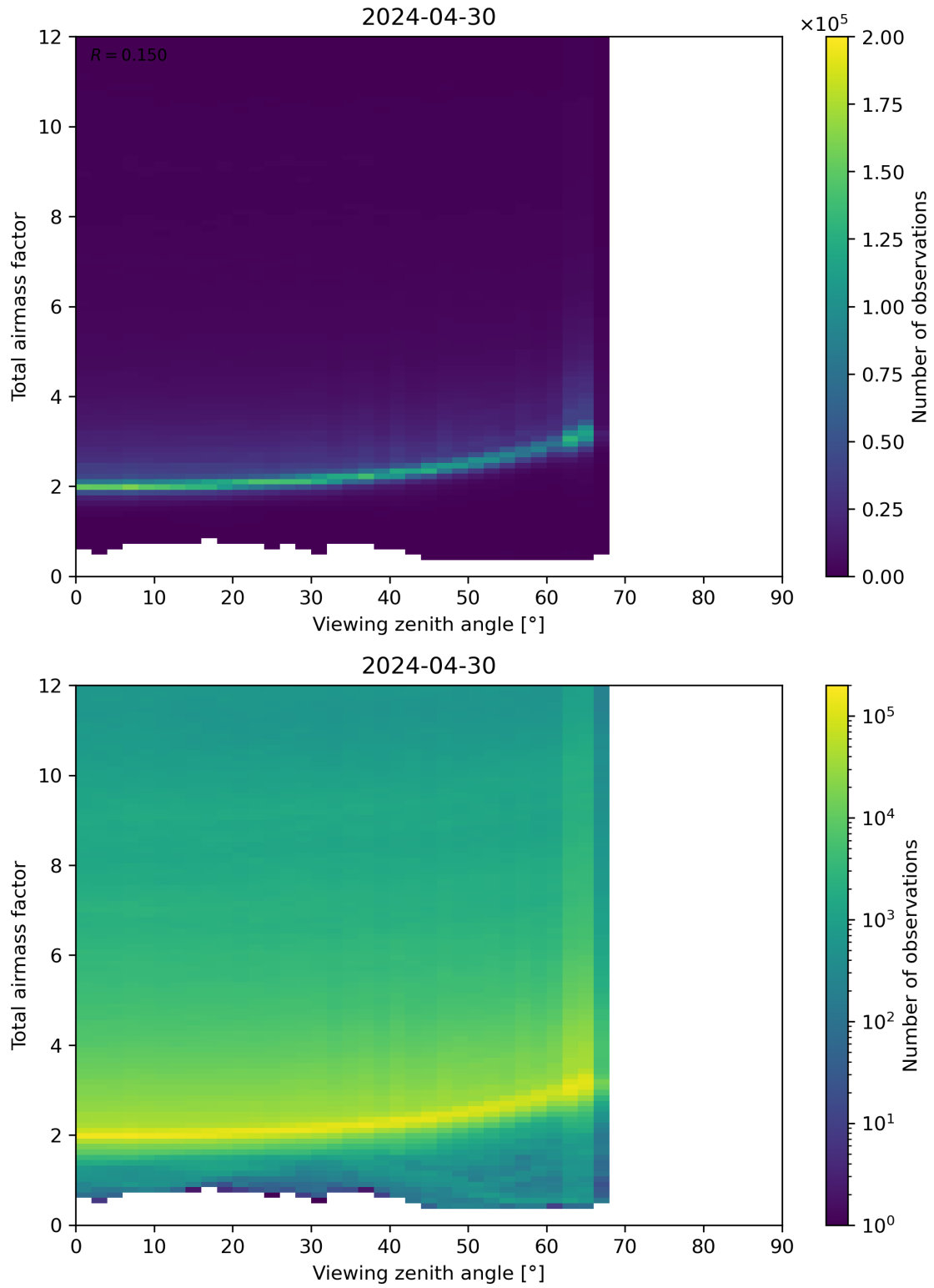
Figure 160: Scatter density plot of “Viewing zenith angle” against “Total airmass factor” for 2024-04-29 to 2024-05-01.
