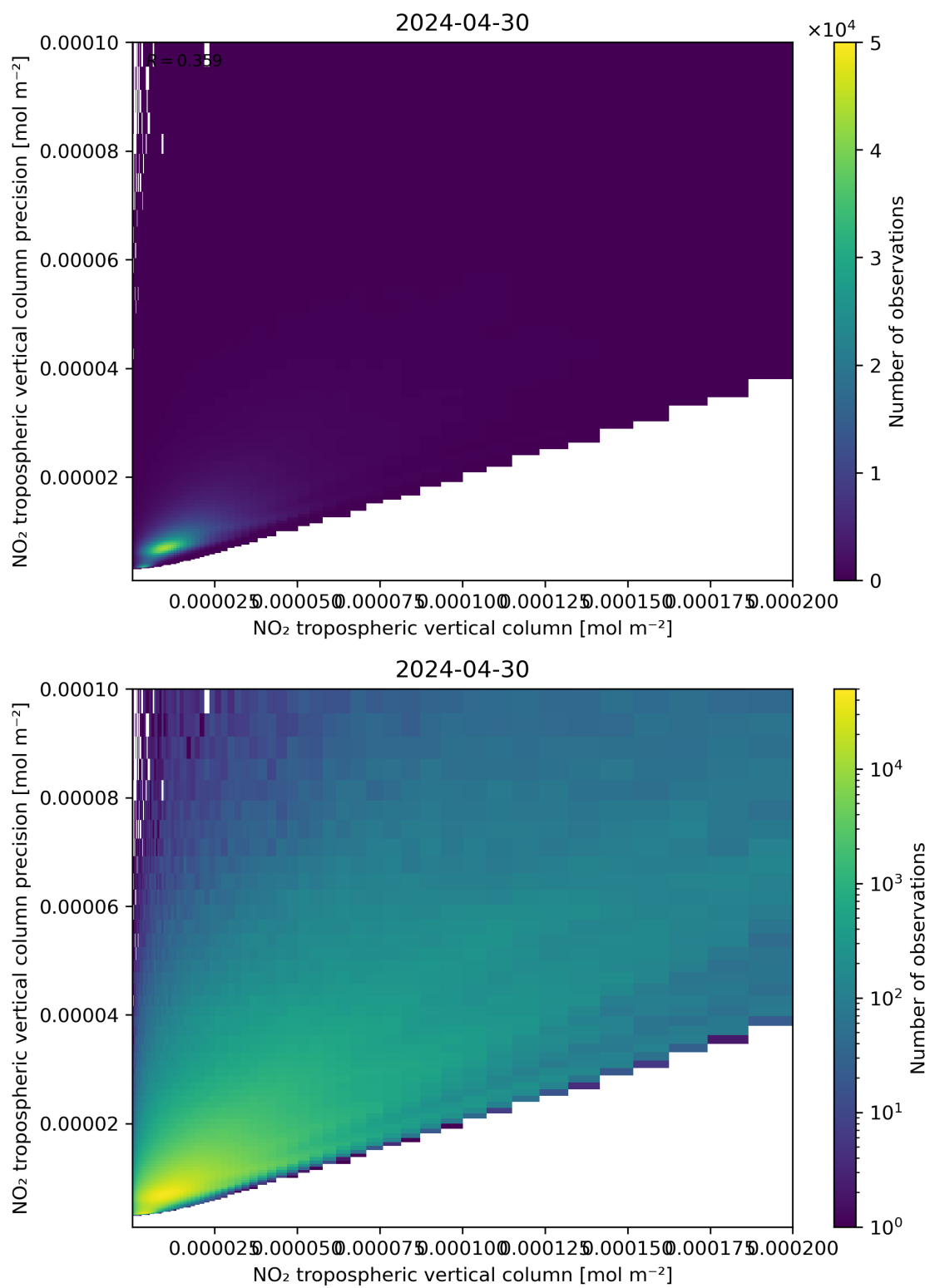
Figure 130: Scatter density plot of “NO 2 tropospheric vertical column” against “NO 2 tropospheric vertical column precision” for 2024-04-29 to 2024-05-01.
