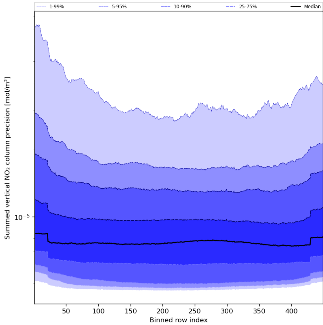
Figure 58: Along track statistics of “Summed vertical NO 2 column precision” for 2024-04-29 to 2024-05-01
