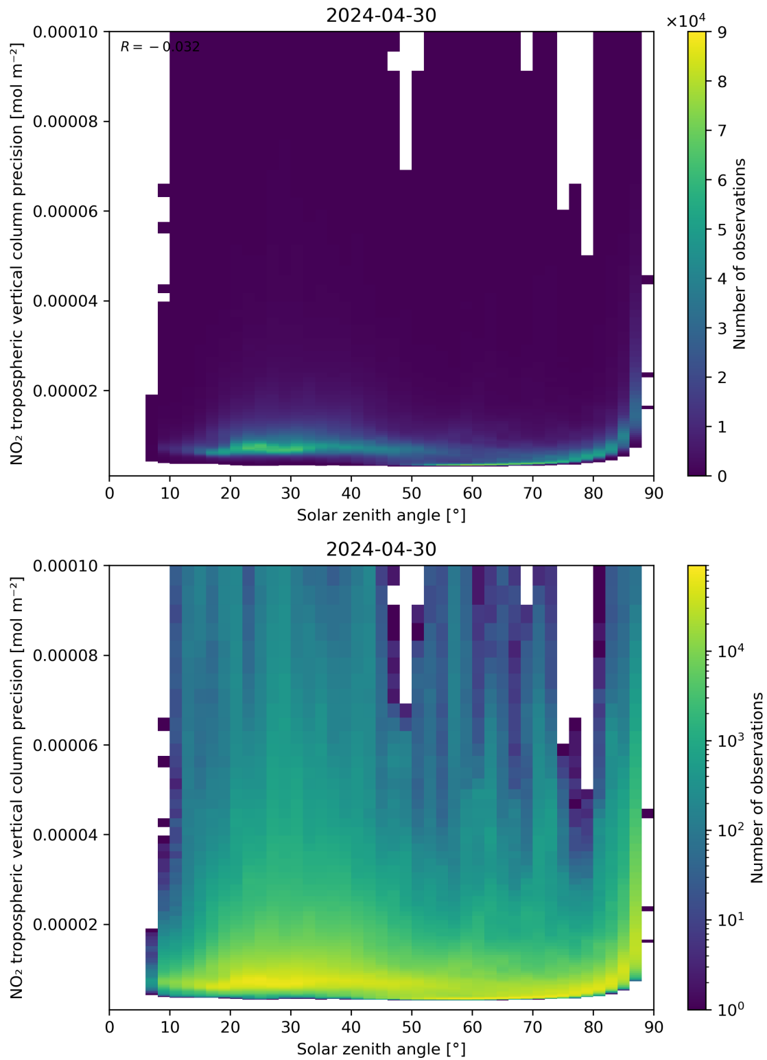
Figure 156: Scatter density plot of “Solar zenith angle” against “NO 2 tropospheric vertical column precision” for 2024-04-29 to 2024-05-01.
