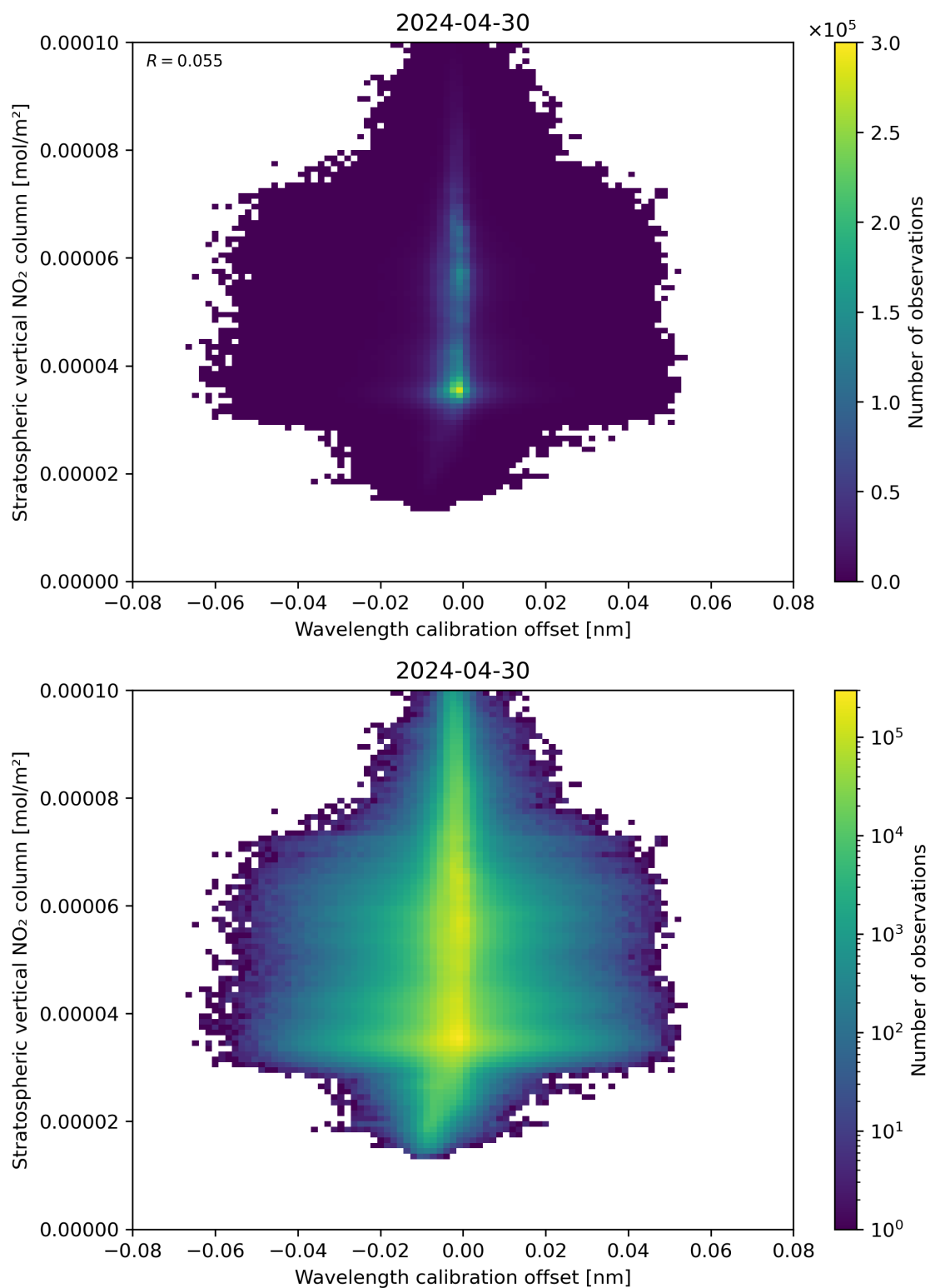
Figure 176: Scatter density plot of “Wavelength calibration offset” against “Stratospheric vertical NO 2 column” for 2024-04-29 to 2024-05-01.
