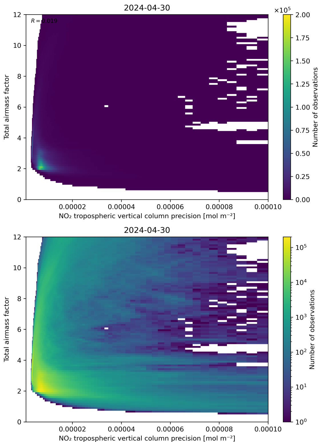
Figure 132: Scatter density plot of “NO 2 tropospheric vertical column precision” against “Total air mass factor” for 2024-04-29 to 2024-05-01.
