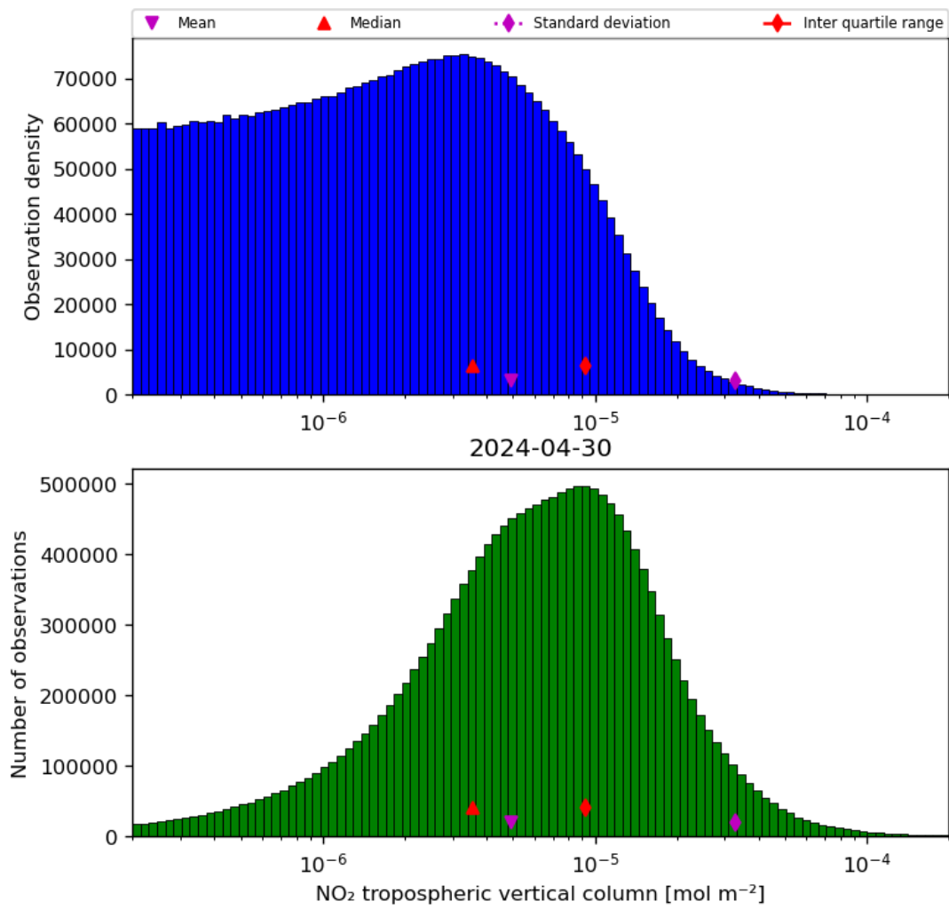
Figure 29: Histogram of “NO 2 tropospheric vertical column” for 2024-04-29 to 2024-05-01
