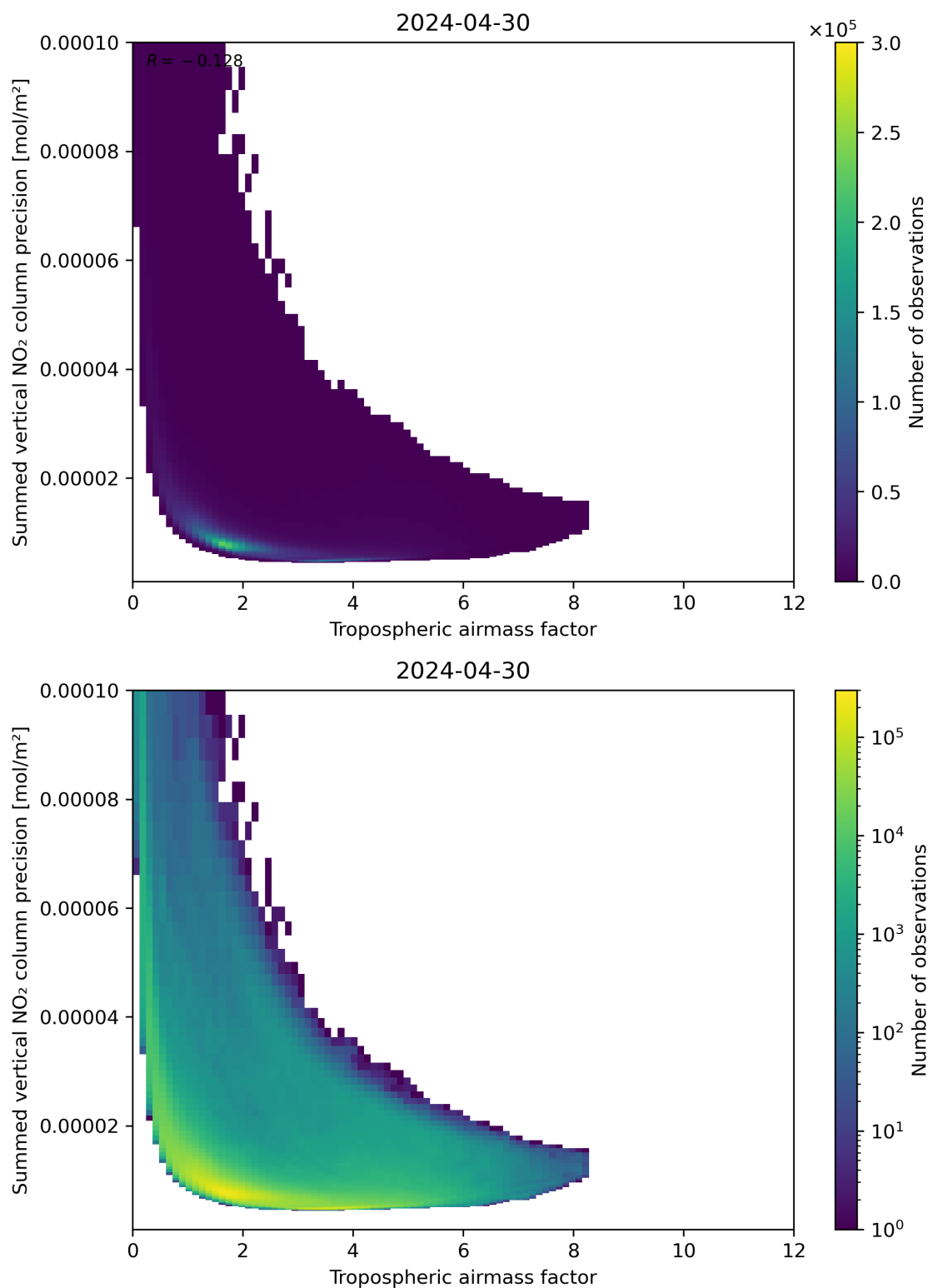
Figure 76: Scatter density plot of “Tropospheric air mass factor” against “Summed vertical NO 2 column precision” for 2024-04-29 to 2024-05-01.
