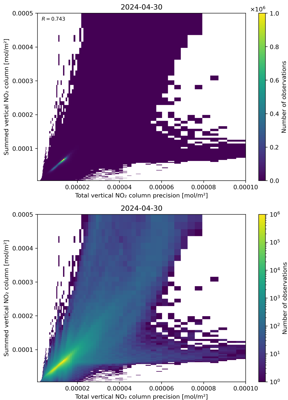
Figure 117: Scatter density plot of “Total vertical NO 2 column precision” against “Summed vertical NO 2 column” for 2024-04-29 to 2024-05-01.
