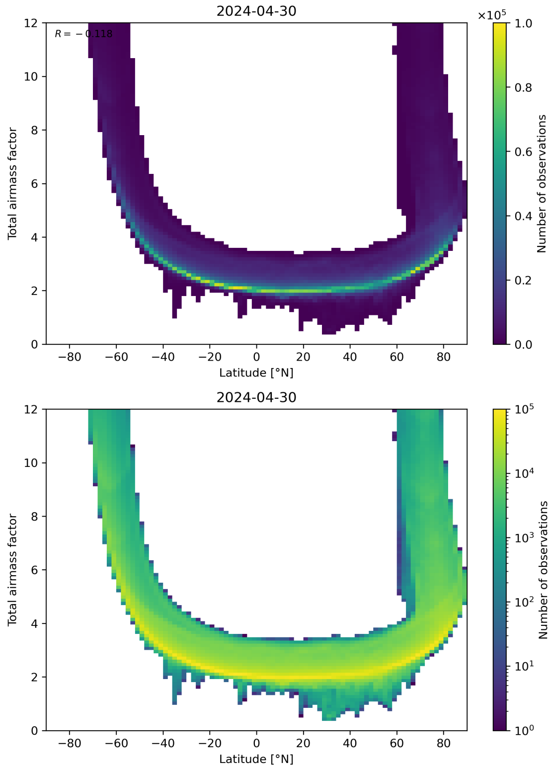
Figure 84: Scatter density plot of “Latitude” against “Total airmass factor” for 2024-04-29 to 2024-05-01.
