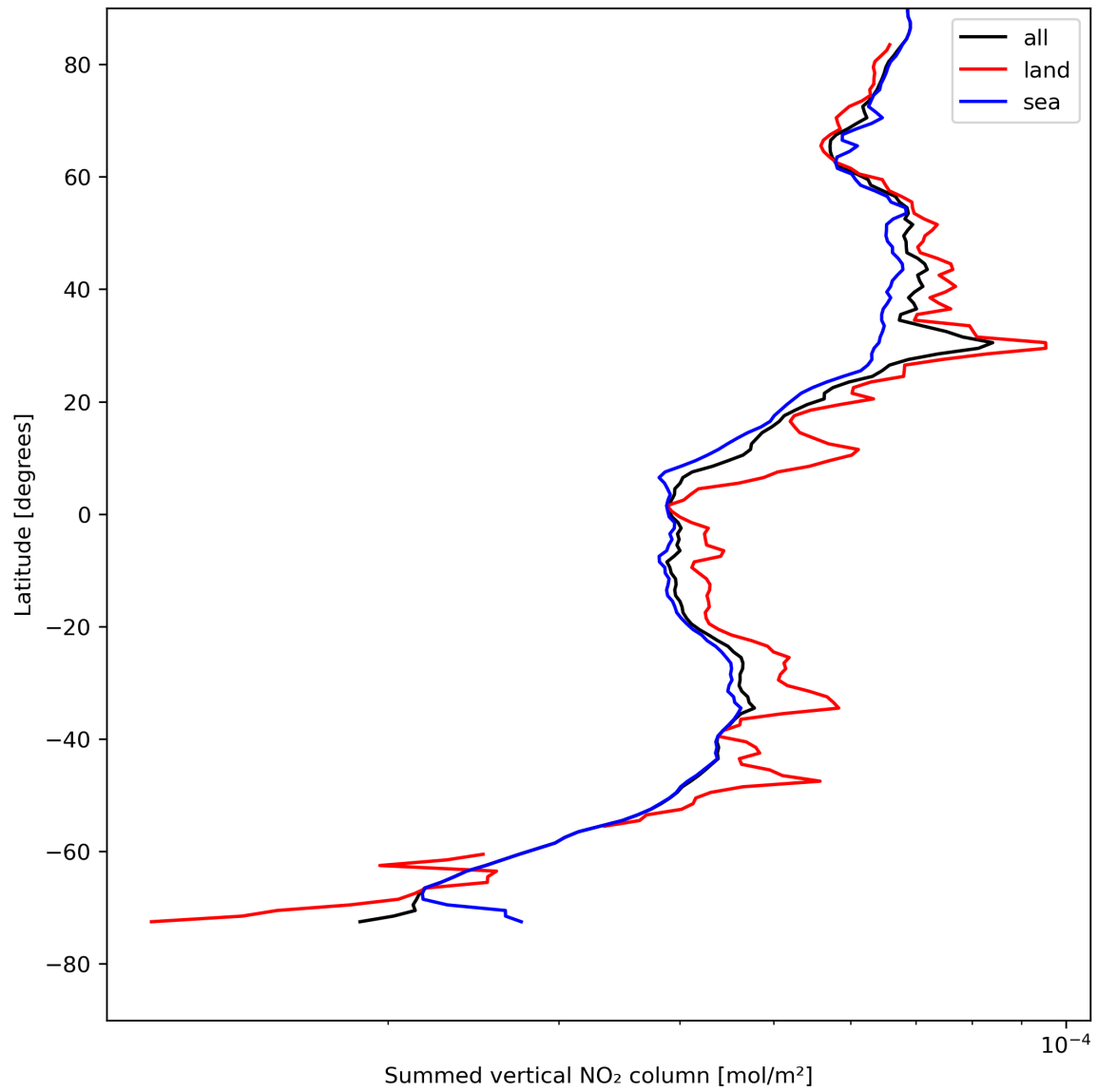
Figure 23: Zonal average of “Summed vertical NO 2 column” for 2024-04-29 to 2024-05-01.
