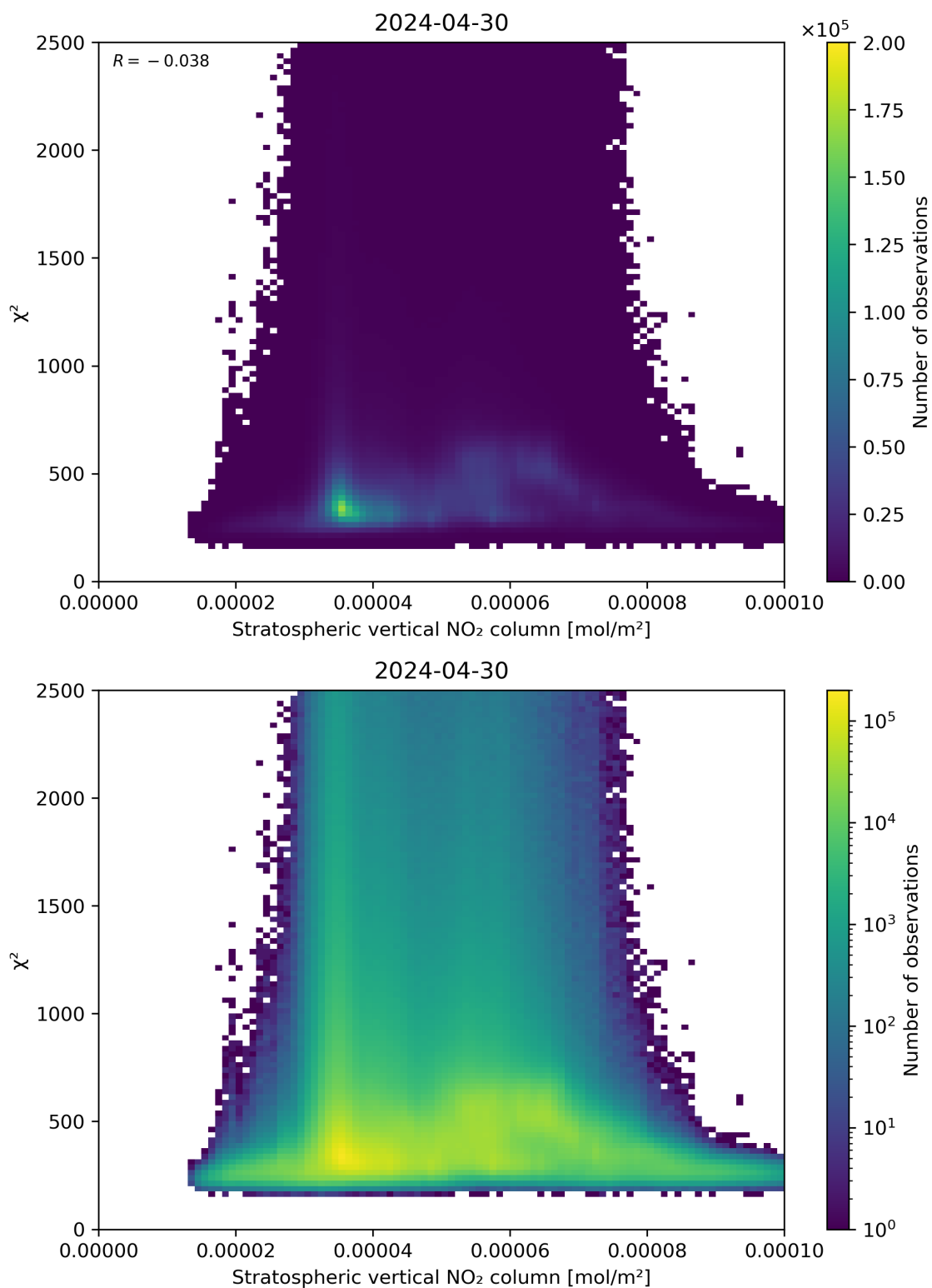
Figure 97: Scatter density plot of “Stratospheric vertical NO 2 column” against “ \chi^2 ” for 2024-04-29 to 2024-05-01.
