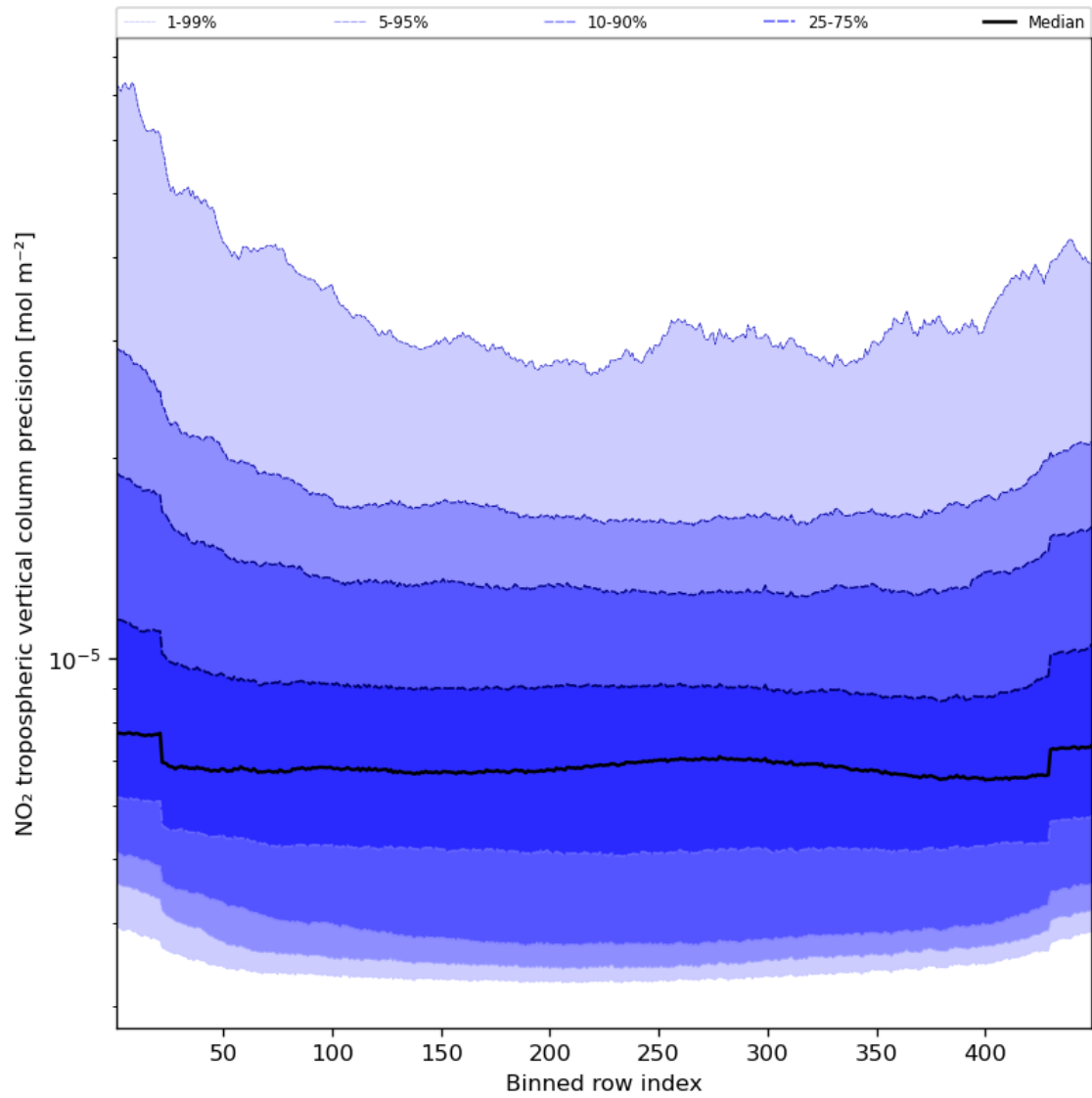
Figure 47: Along track statistics of “NO 2 tropospheric vertical column precision” for 2024-04-29 to 2024-05-01
