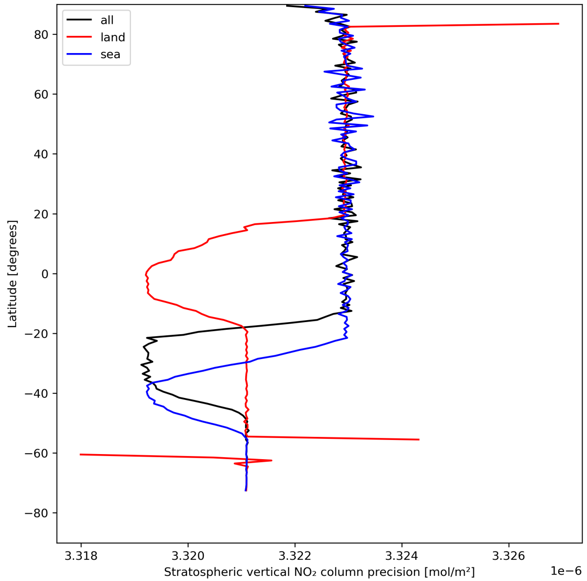
Figure 20: Zonal average of “Stratospheric vertical NO 2 column precision” for 2024-04-29 to 2024-05-01.
