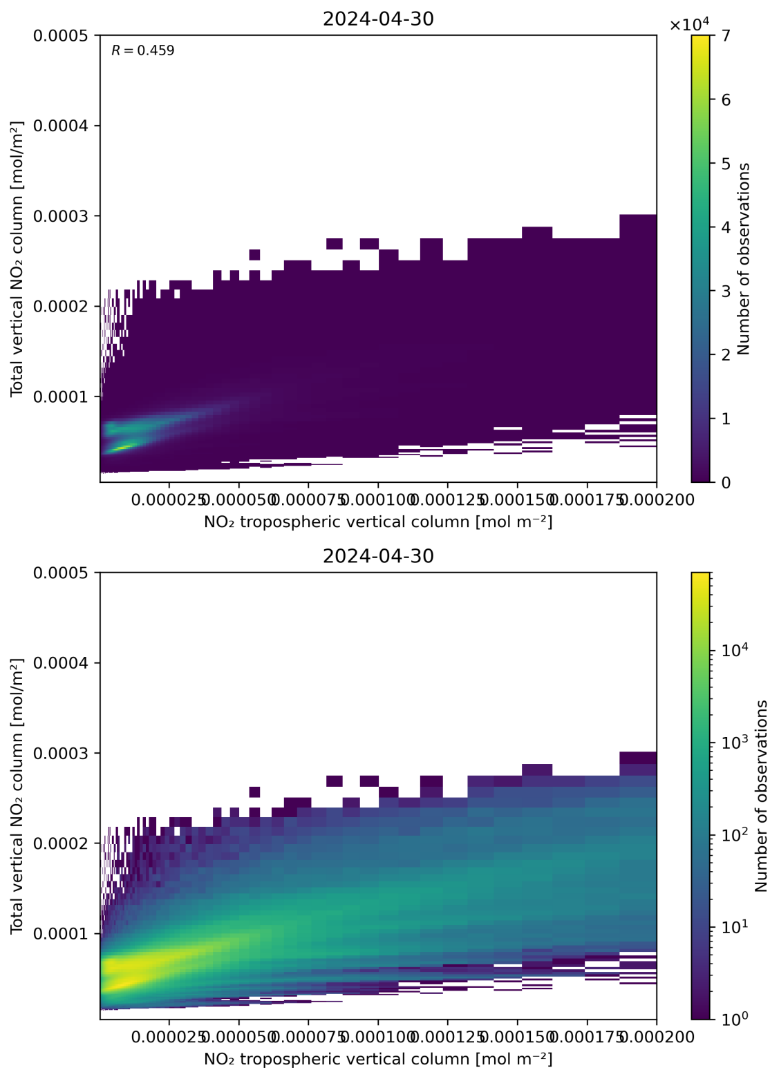
Figure 128: Scatter density plot of “NO 2 tropospheric vertical column” against “Total vertical NO 2 column” for 2024-04-29 to 2024-05-01.
