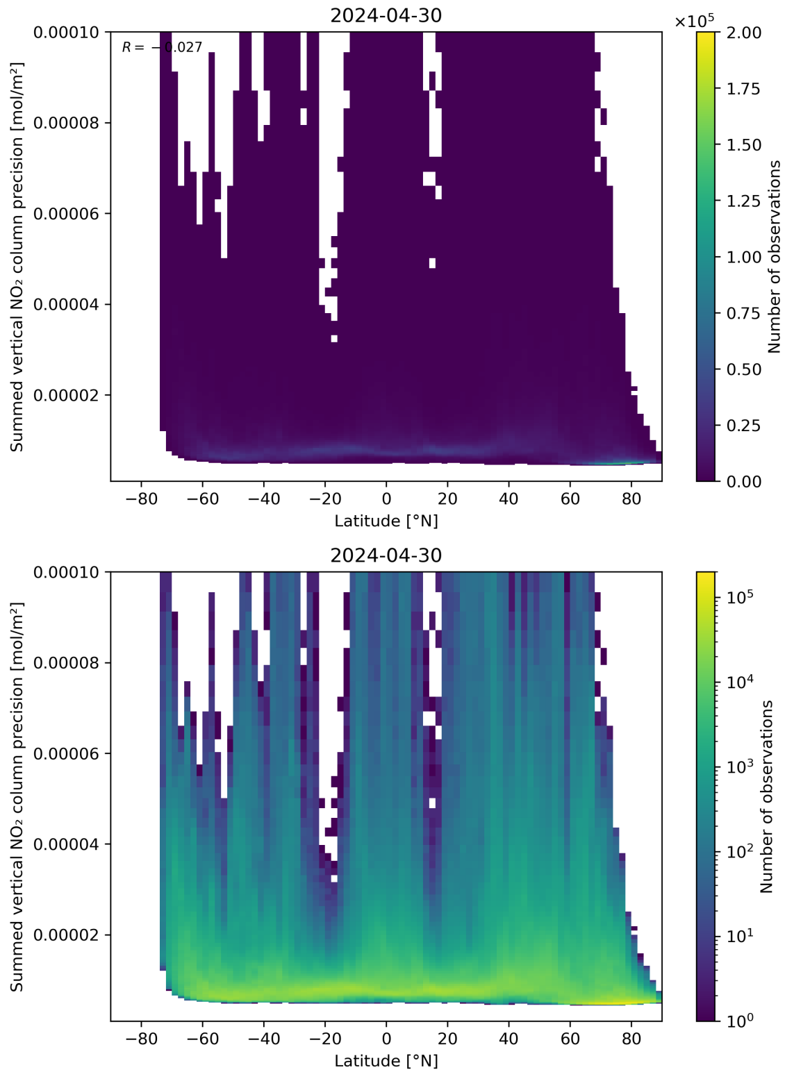
Figure 89: Scatter density plot of “Latitude” against “Summed vertical NO 2 column precision” for 2024-04-29 to 2024-05-01.
