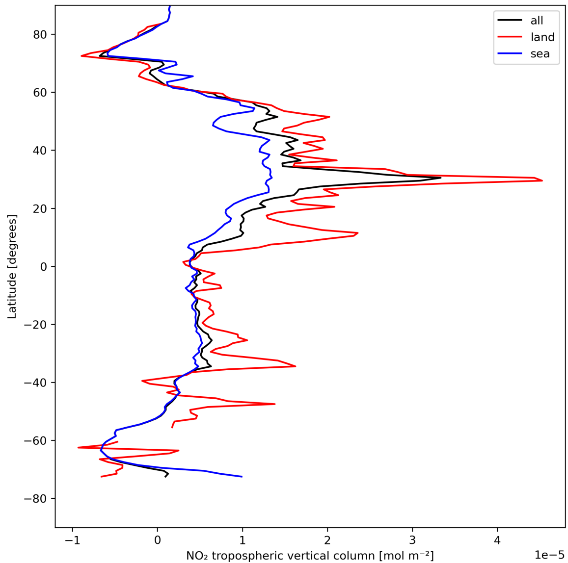
Figure 12: Zonal average of “NO 2 tropospheric vertical column” for 2024-04-29 to 2024-05-01.
