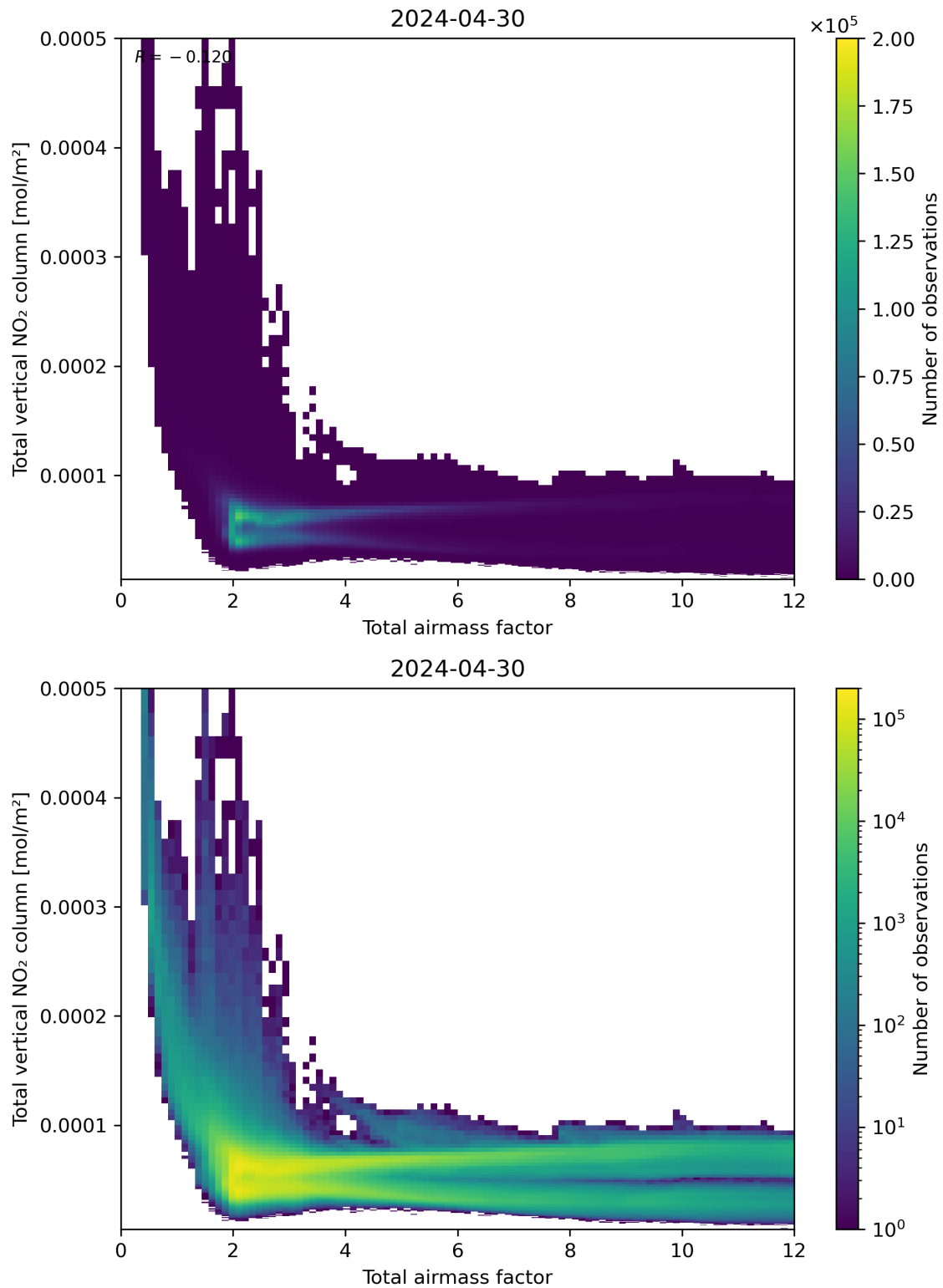
Figure 67: Scatter density plot of “Total airmass factor” against “Total vertical NO 2 column” for 2024-04-29 to 2024-05-01.
