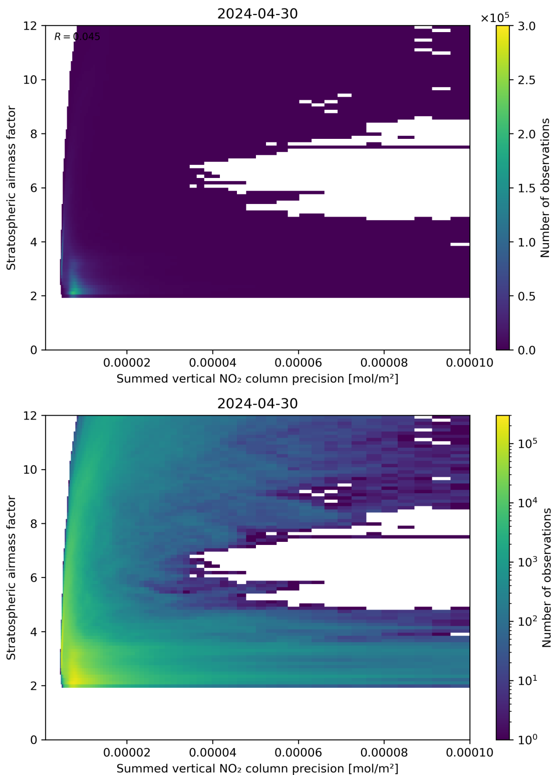
Figure 106: Scatter density plot of “Summed vertical NO 2 column precision” against “Stratospheric airmass factor” for 2024-04-29 to 2024-05-01.
