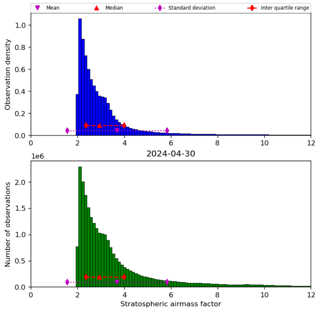
Figure 44: Histogram of “Stratospheric airmass factor” for 2024-04-29 to 2024-05-01
