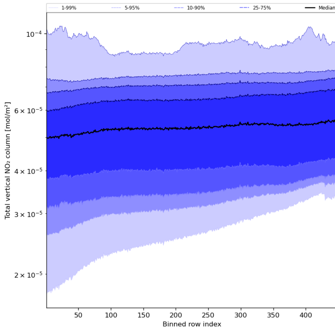
Figure 55: Along track statistics of “Total vertical NO 2 column” for 2024-04-29 to 2024-05-01
