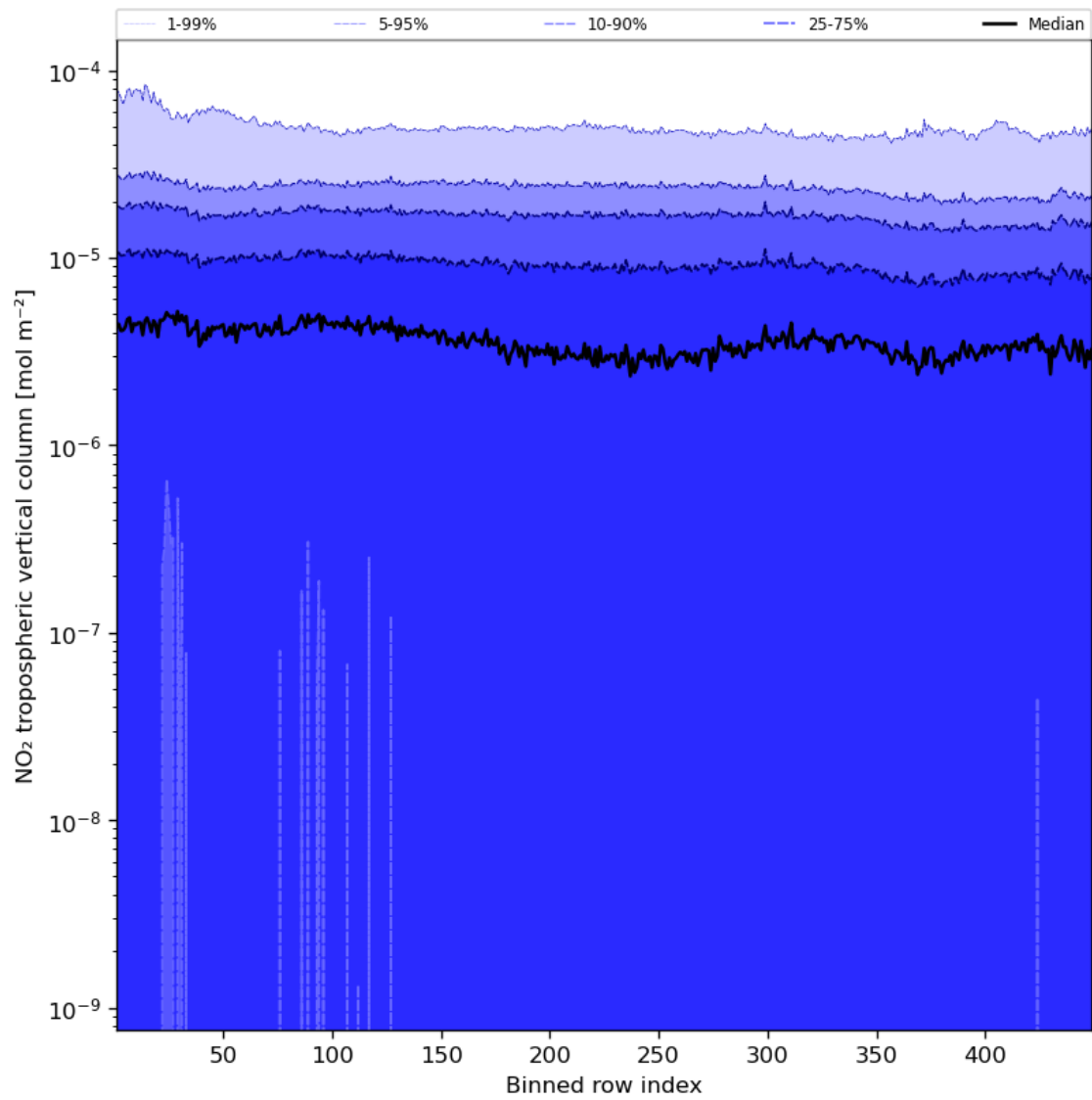
Figure 46: Along track statistics of “NO 2 tropospheric vertical column” for 2024-04-29 to 2024-05-01
