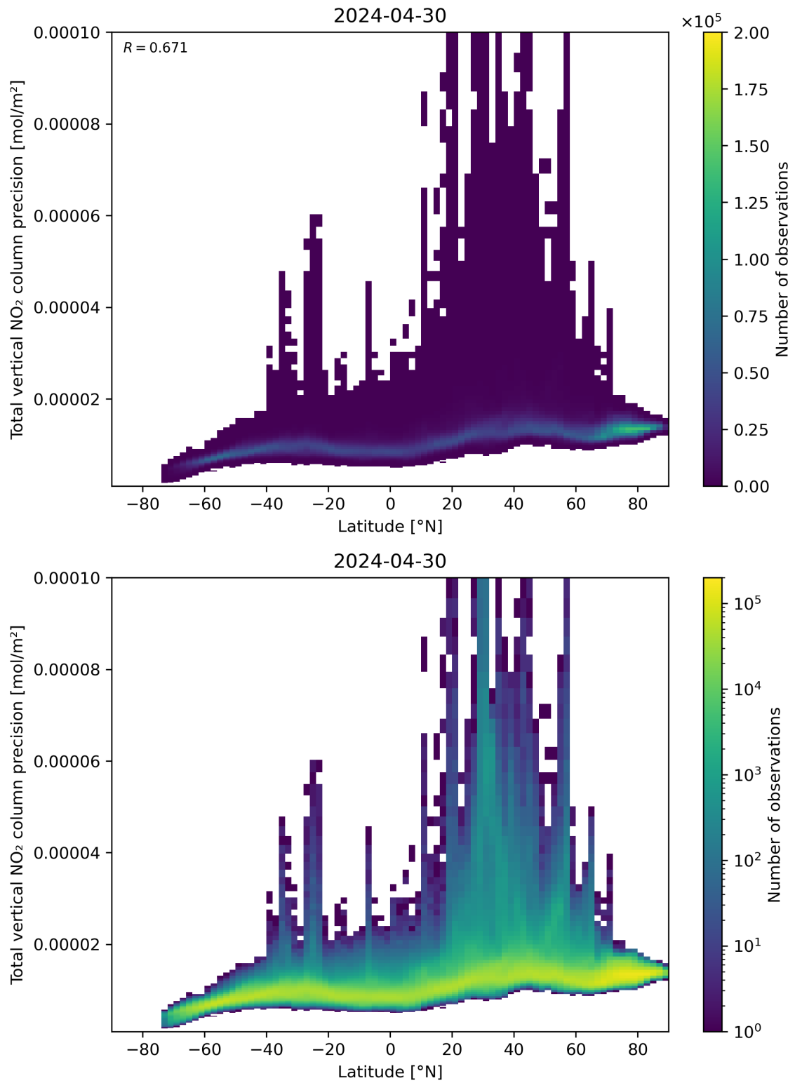
Figure 91: Scatter density plot of “Latitude” against “Total vertical NO 2 column precision” for 2024-04-29 to 2024-05-01.
