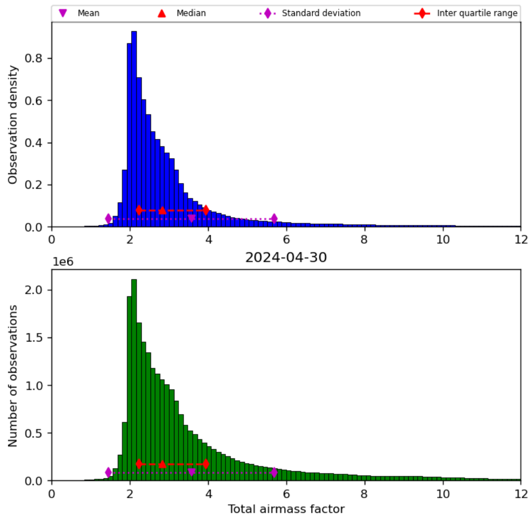
Figure 32: Histogram of “Total airmass factor” for 2024-04-29 to 2024-05-01
