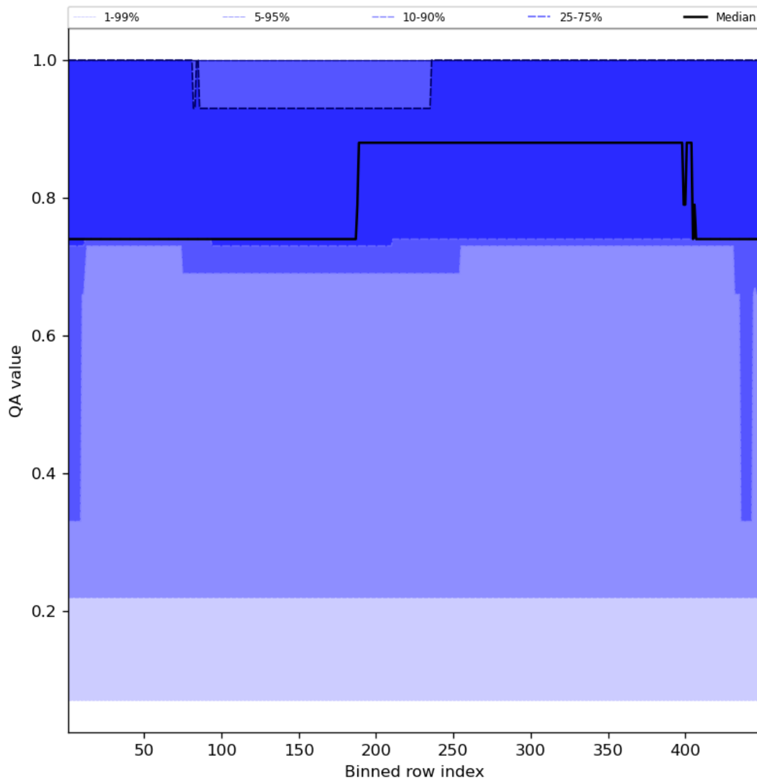
Figure 45: Along track statistics of “QA value” for 2024-04-29 to 2024-05-01
