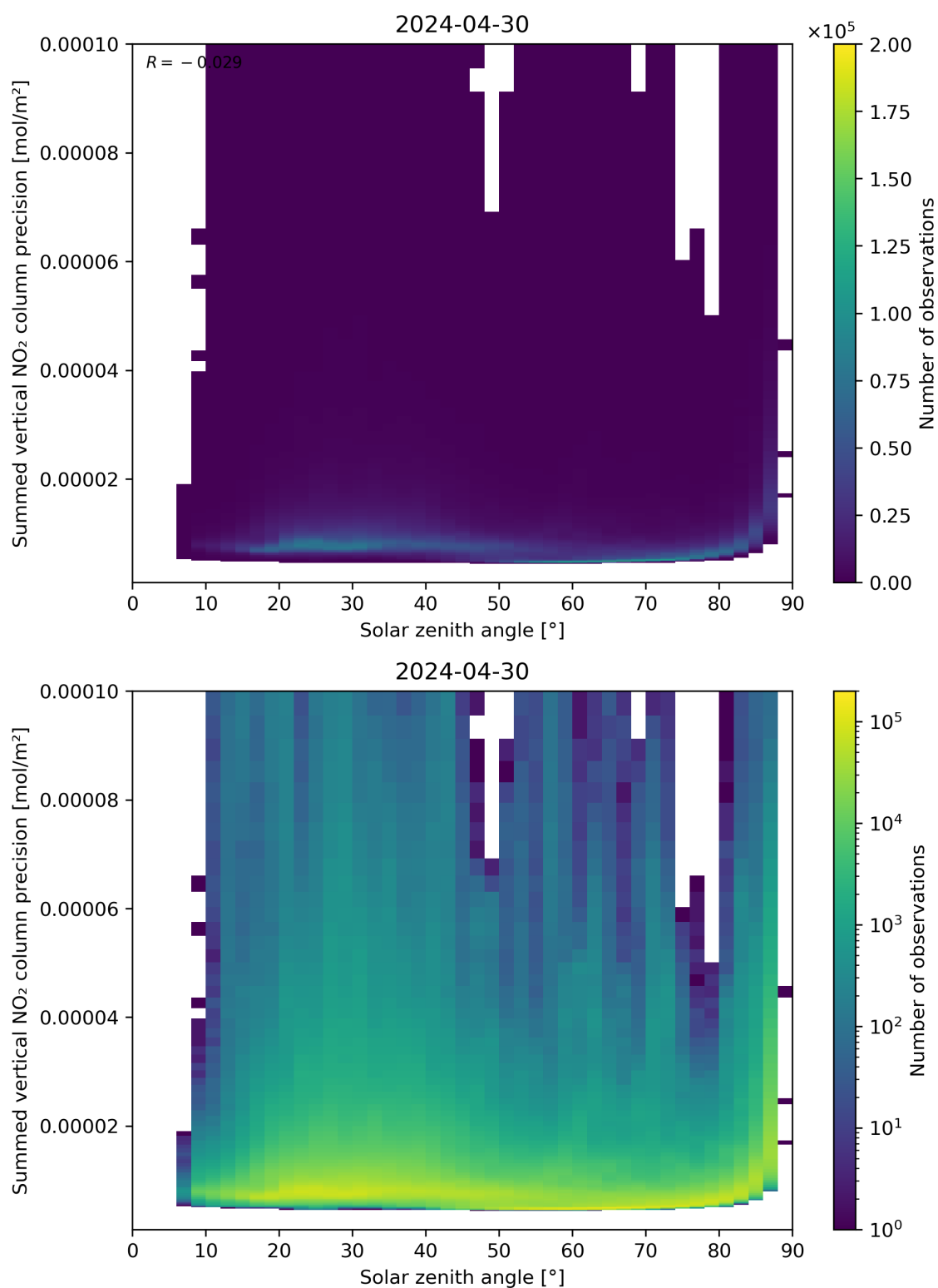
Figure 152: Scatter density plot of “Solar zenith angle” against “Summed vertical NO 2 column precision” for 2024-04-29 to 2024-05-01.
