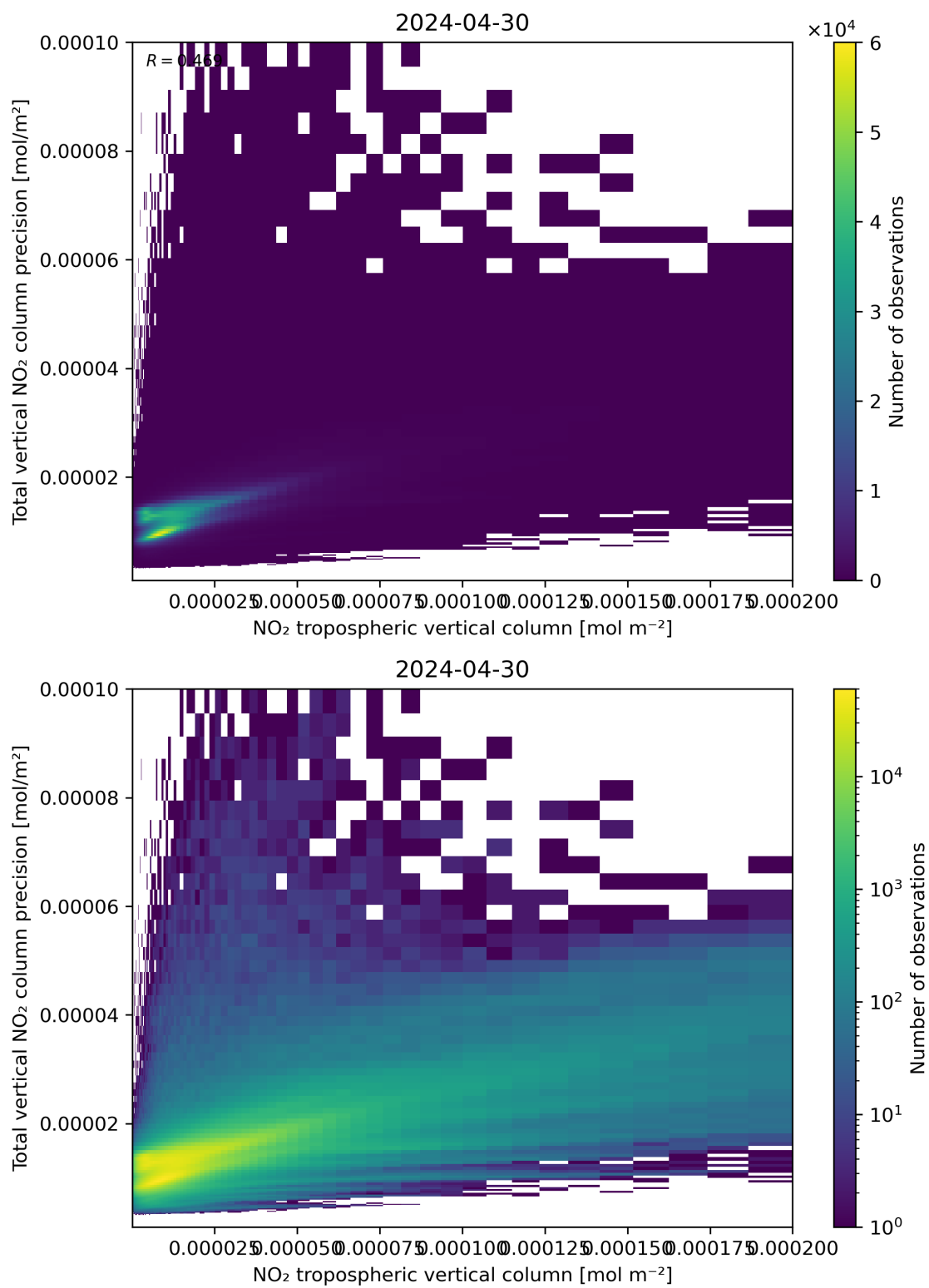
Figure 129: Scatter density plot of “NO 2 tropospheric vertical column” against “Total vertical NO 2 column precision” for 2024-04-29 to 2024-05-01.
