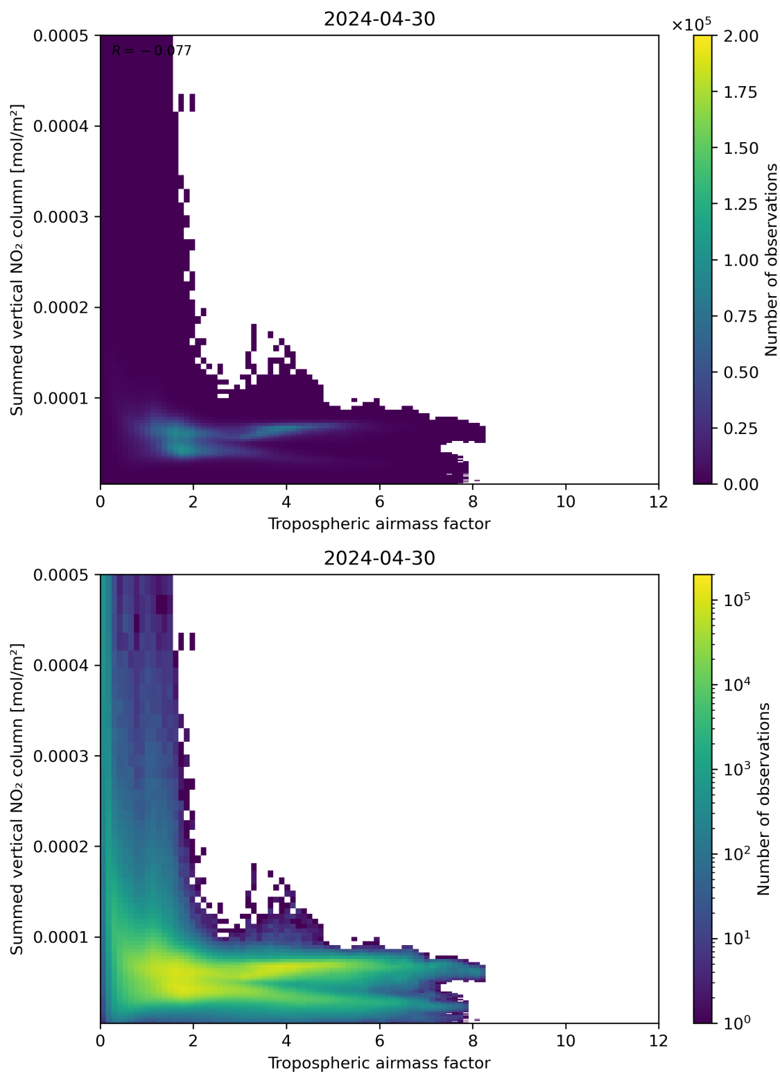
Figure 75: Scatter density plot of “Tropospheric airmass factor” against “Summed vertical NO 2 column” for 2024-04-29 to 2024-05-01.
