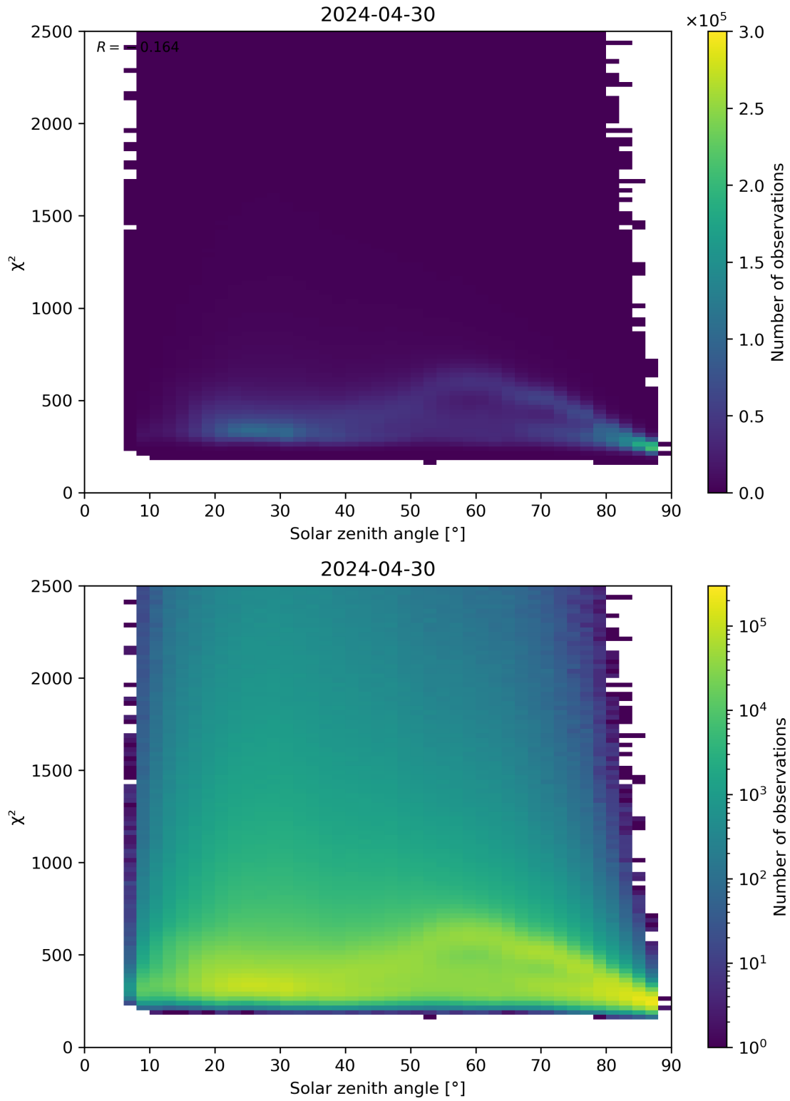
Figure 148: Scatter density plot of “Solar zenith angle” against “ \chi^2 ” for 2024-04-29 to 2024-05-01.
