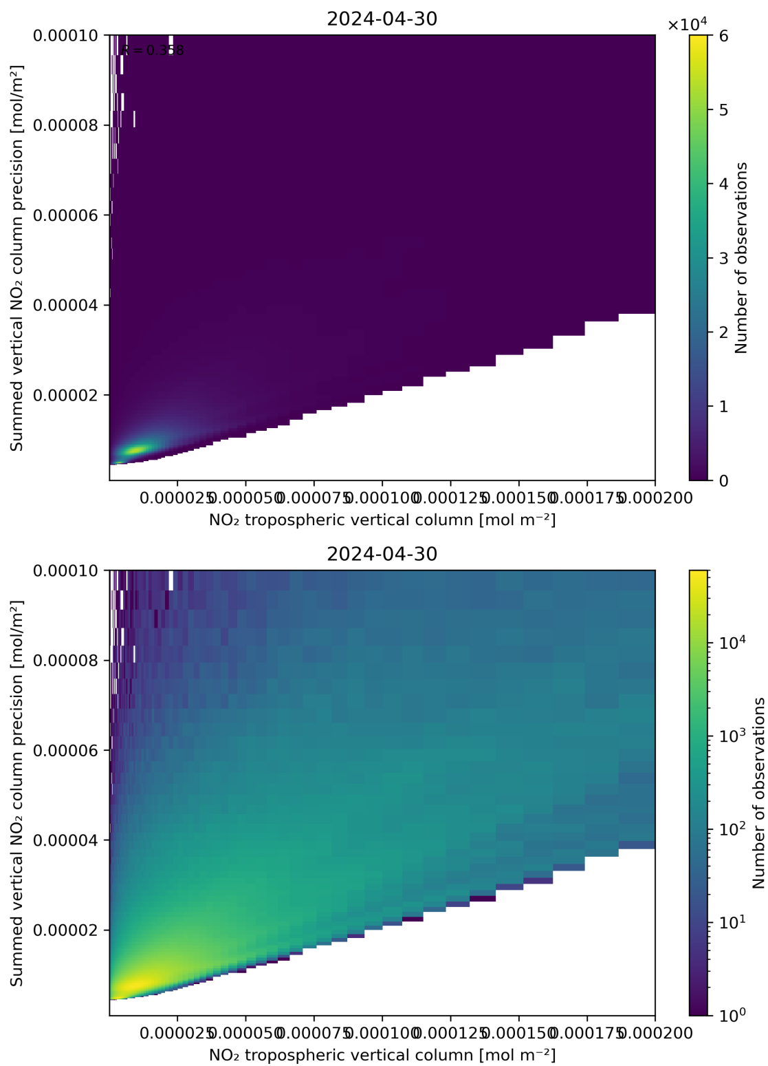
Figure 127: Scatter density plot of “NO 2 tropospheric vertical column” against “Summed vertical NO 2 column precision” for 2024-04-29 to 2024-05-01.
