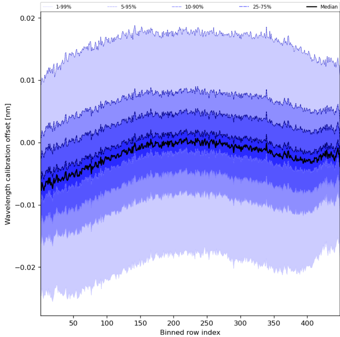
Figure 52: Along track statistics of “Wavelength calibration offset” for 2024-04-29 to 2024-05-01
