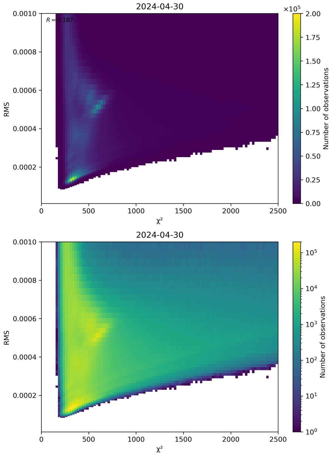
Figure 82: Scatter density plot of “ \chi^2 ” against “RMS” for 2024-04-29 to 2024-05-01.
