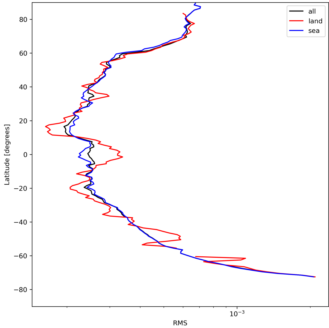
Figure 26: Zonal average of “RMS” for 2024-04-29 to 2024-05-01.
