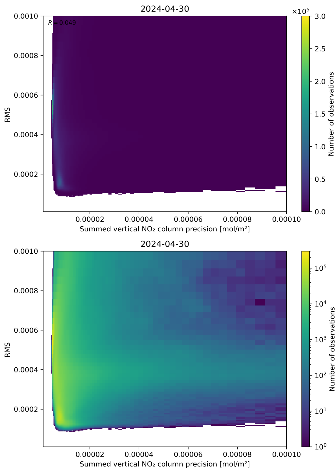
Figure 108: Scatter density plot of “Summed vertical NO 2 column precision” against “RMS” for 2024-04-29 to 2024-05-01.
