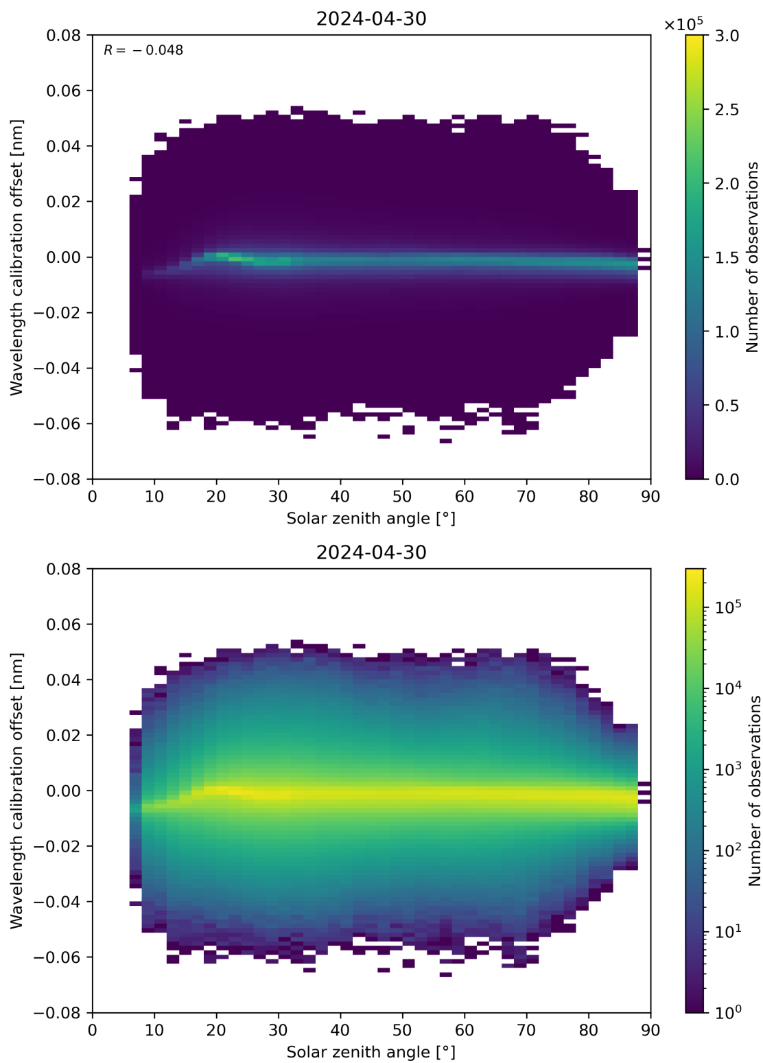
Figure 158: Scatter density plot of “Solar zenith angle” against “Wavelength calibration offset” for 2024-04-29 to 2024-05-01.
