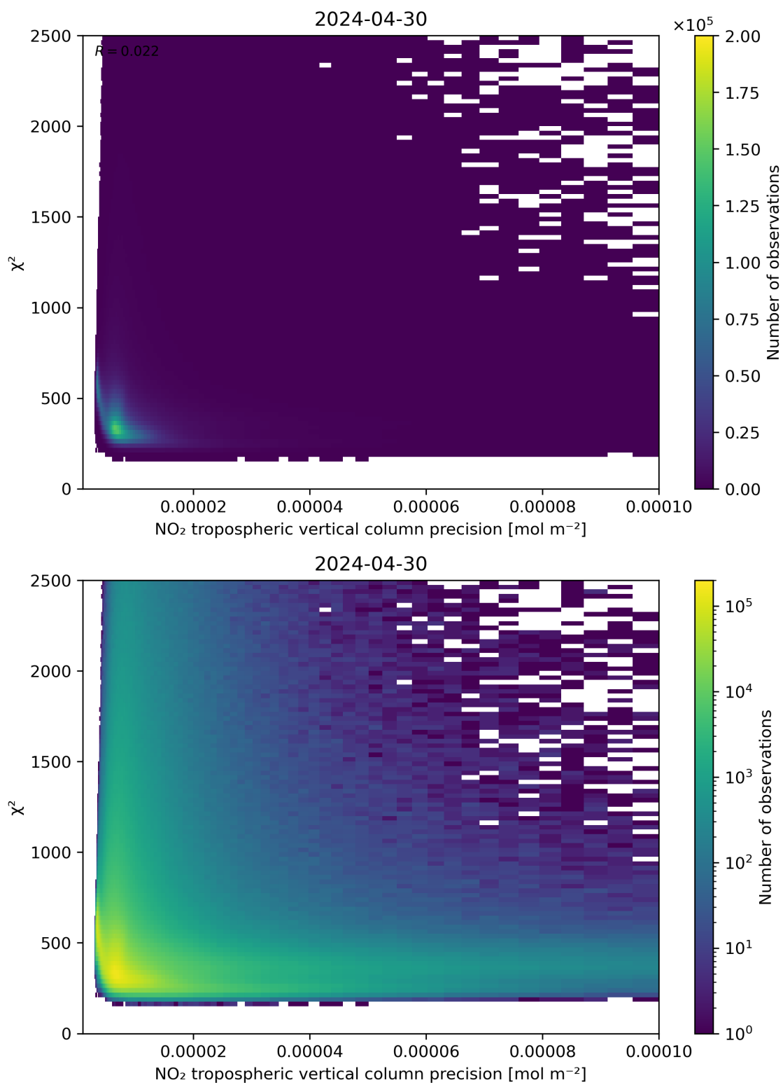
Figure 134: Scatter density plot of “NO 2 tropospheric vertical column precision” against “ \chi^2 ” for 2024-04-29 to 2024-05-01.
