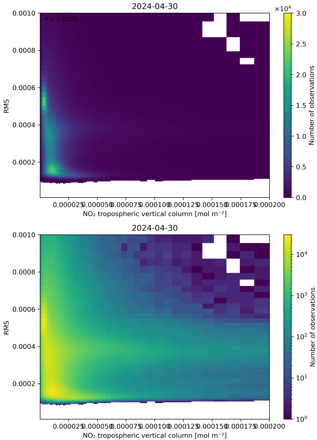
Figure 142: Scatter density plot of “NO 2 tropospheric vertical column” against “RMS” for 2024-04-29 to 2024-05-01.
