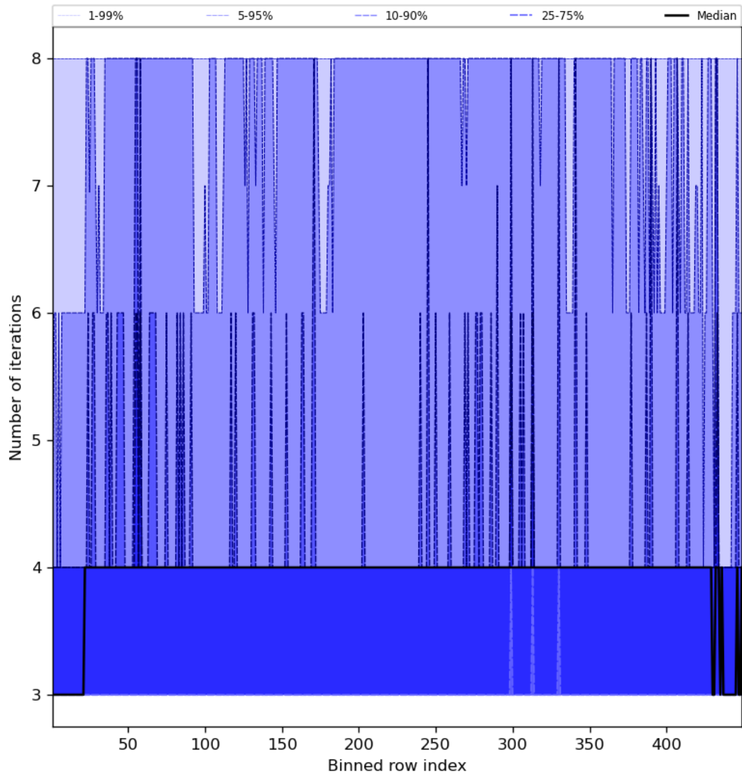
Figure 51: Along track statistics of “Number of iterations” for 2024-04-29 to 2024-05-01
