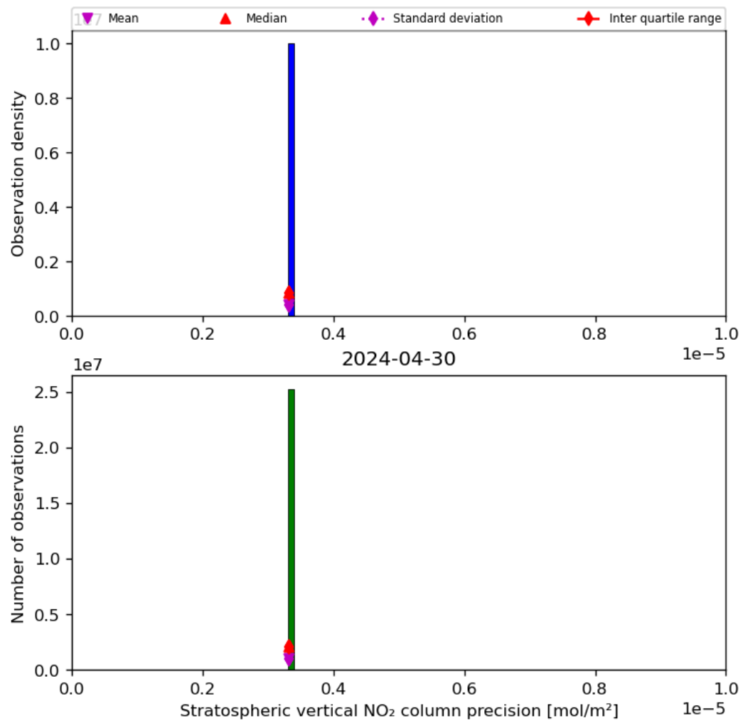
Figure 37: Histogram of “Stratospheric vertical NO 2 column precision” for 2024-04-29 to 2024-05-01
