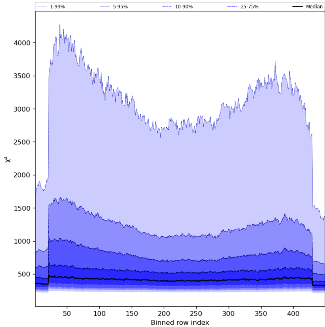
Figure 59: Along track statistics of “ \chi^2 ” for 2024-04-29 to 2024-05-01
