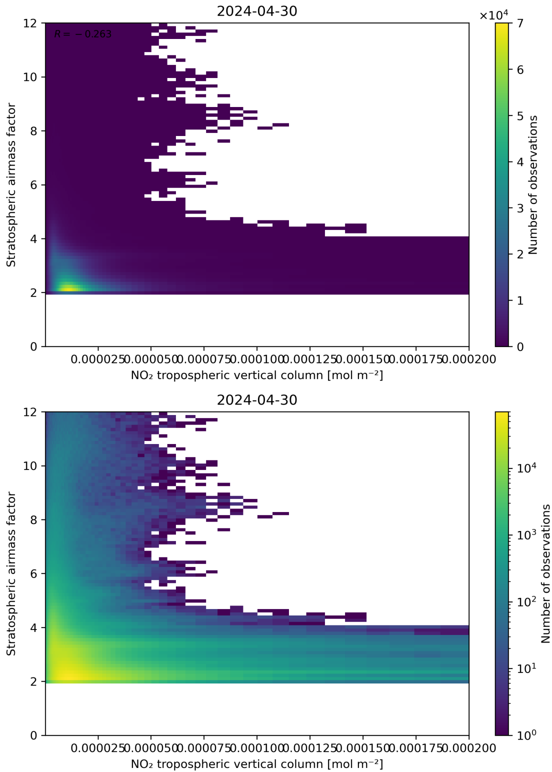
Figure 121: Scatter density plot of “NO 2 tropospheric vertical column” against “Stratospheric air mass factor” for 2024-04-29 to 2024-05-01.
