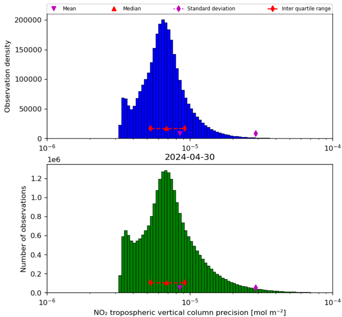
Figure 30: Histogram of “NO 2 tropospheric vertical column precision” for 2024-04-29 to 2024-05-01
