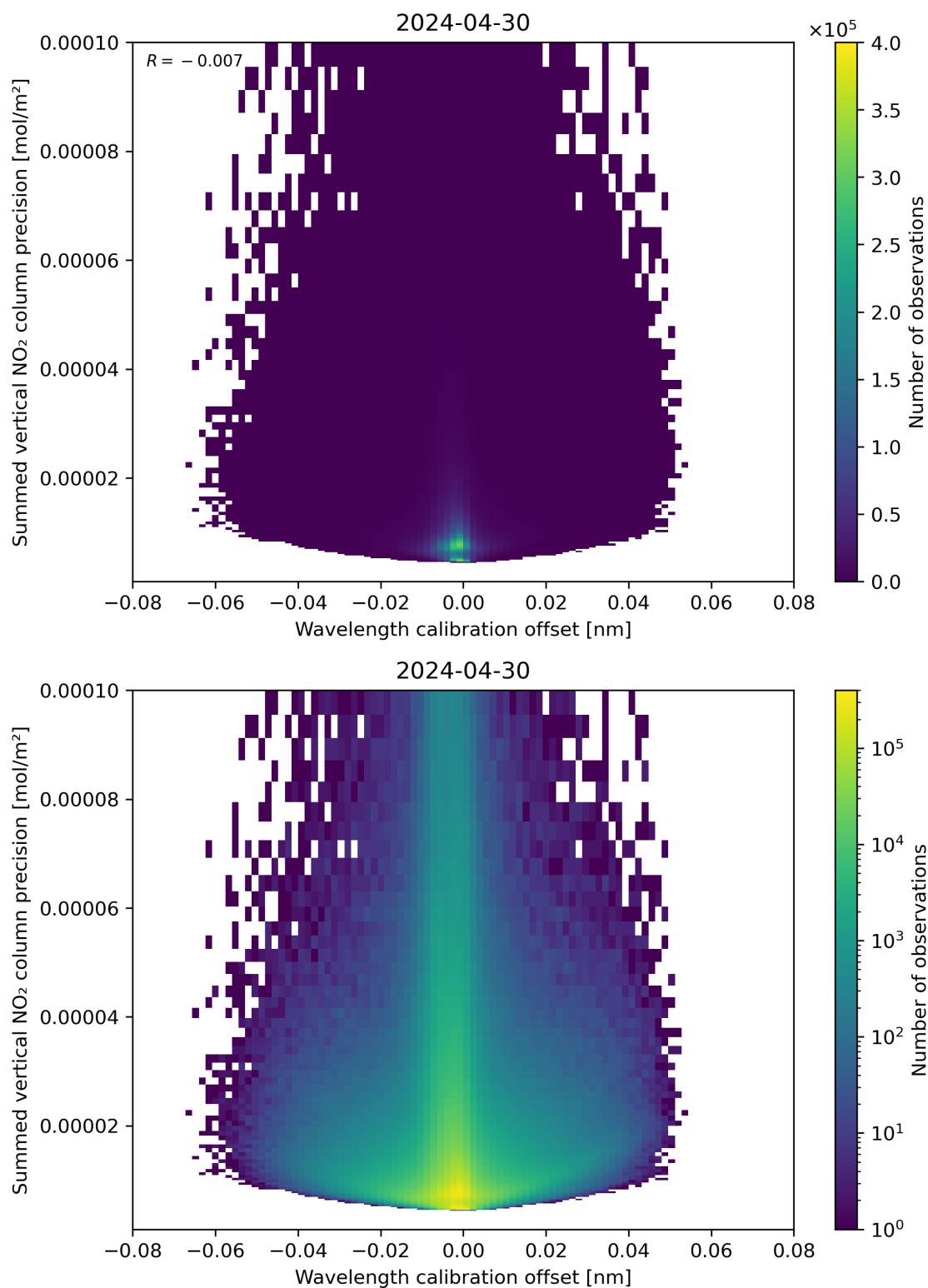
Figure 178: Scatter density plot of “Wavelength calibration offset” against “Summed vertical NO 2 column precision” for 2024-04-29 to 2024-05-01.
