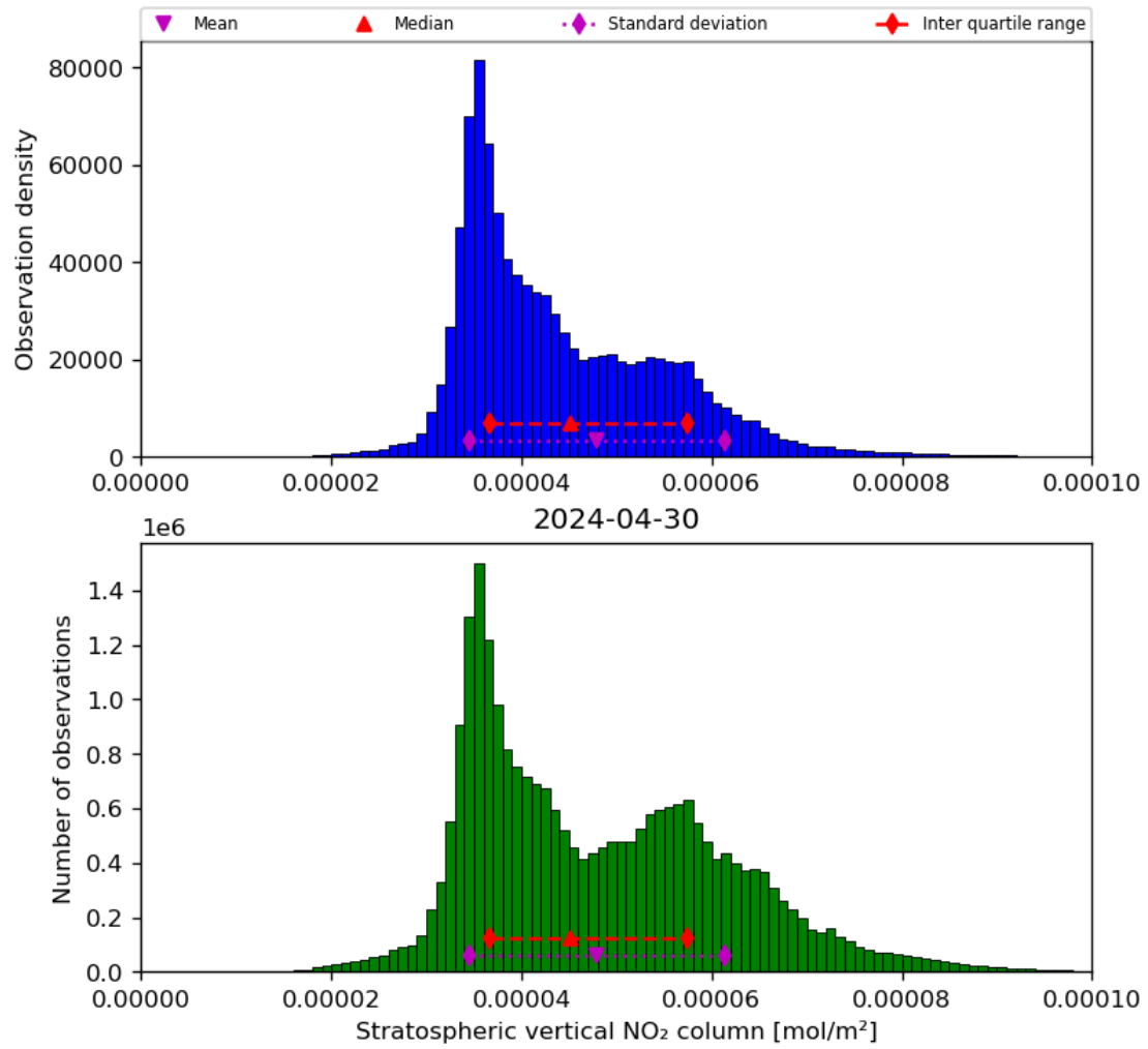
Figure 36: Histogram of “Stratospheric vertical NO 2 column” for 2024-04-29 to 2024-05-01
