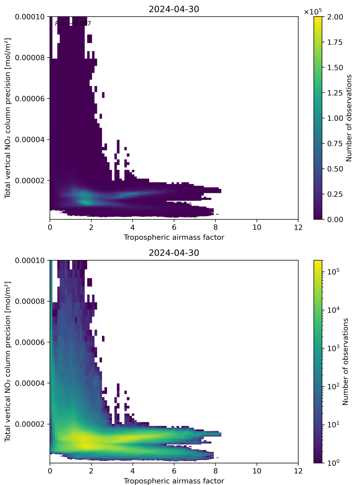
Figure 78: Scatter density plot of “Tropospheric air mass factor” against “Total vertical NO 2 column precision” for 2024-04-29 to 2024-05-01.
