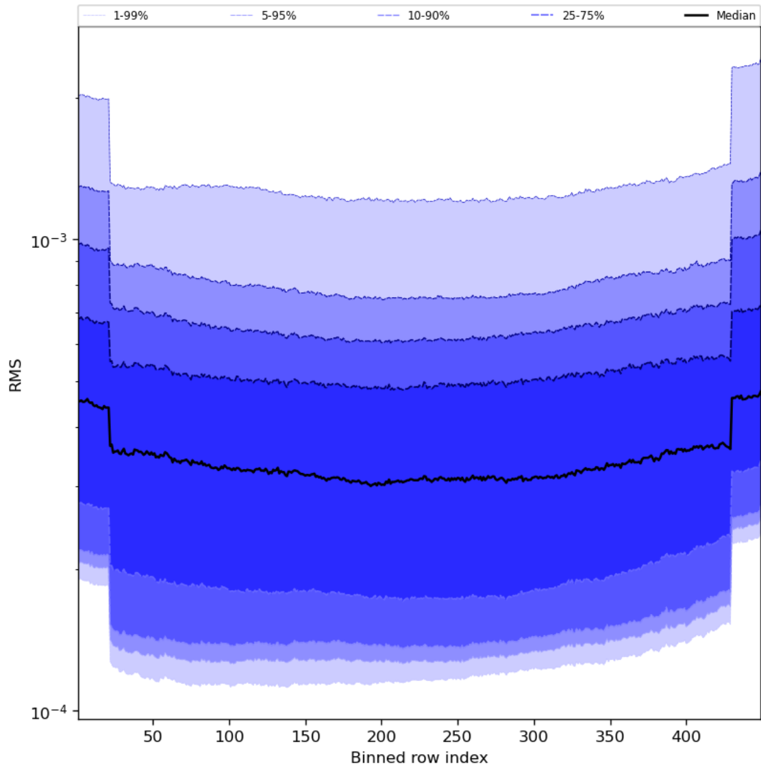
Figure 60: Along track statistics of “RMS” for 2024-04-29 to 2024-05-01
