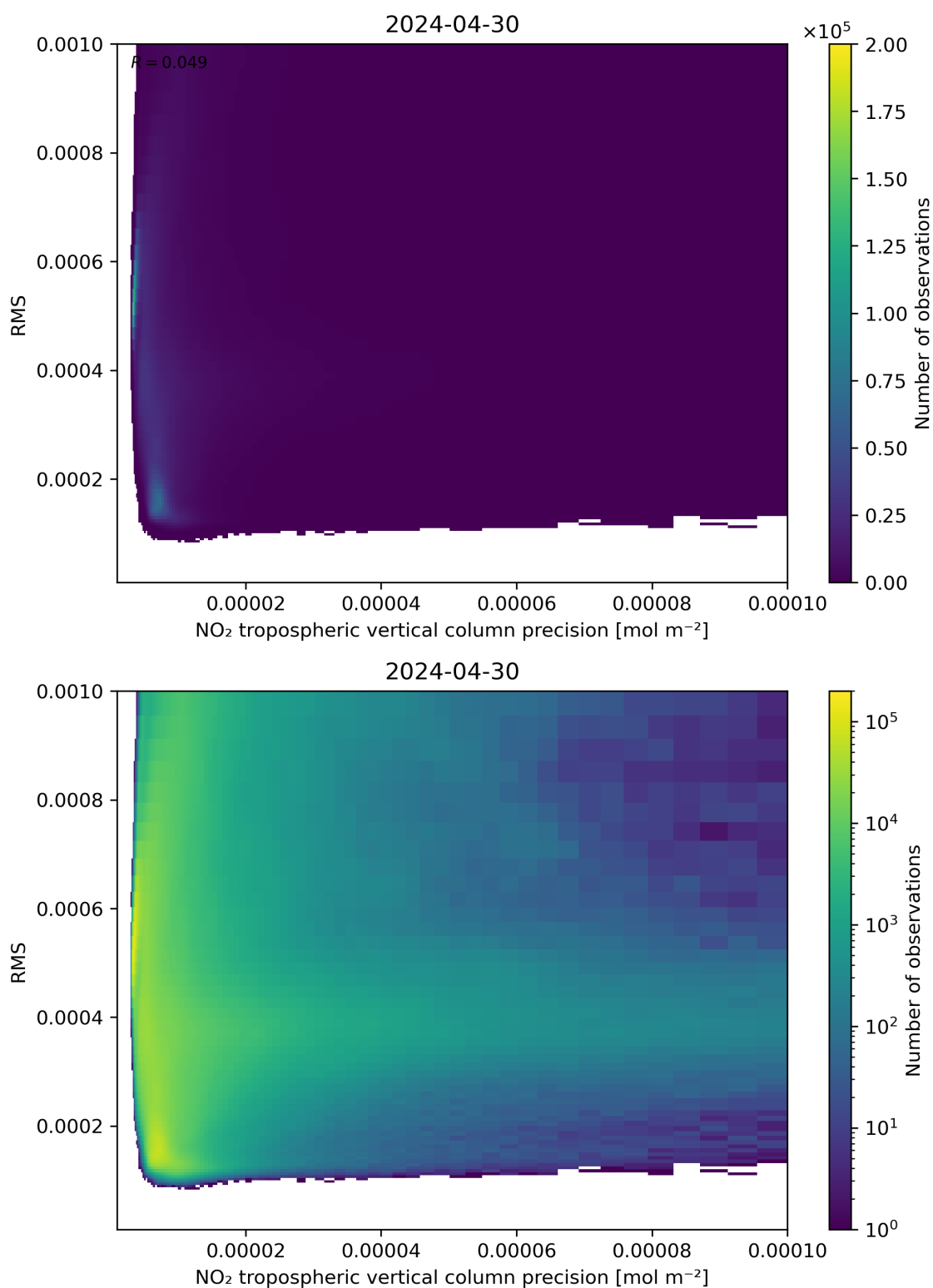
Figure 140: Scatter density plot of “NO 2 tropospheric vertical column precision” against “RMS” for 2024-04-29 to 2024-05-01.
