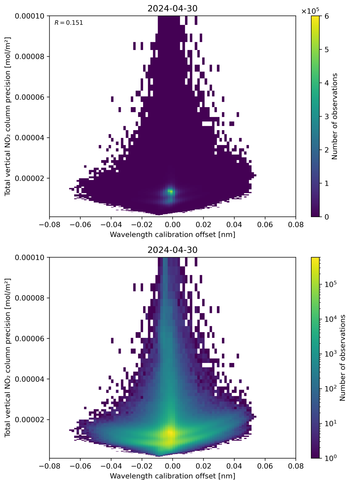
Figure 180: Scatter density plot of “Wavelength calibration offset” against “Total vertical NO 2 column precision” for 2024-04-29 to 2024-05-01.
