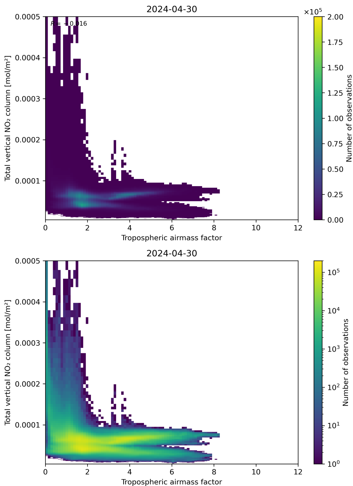
Figure 77: Scatter density plot of “Tropospheric airmass factor” against “Total vertical NO 2 column” for 2024-04-29 to 2024-05-01.
