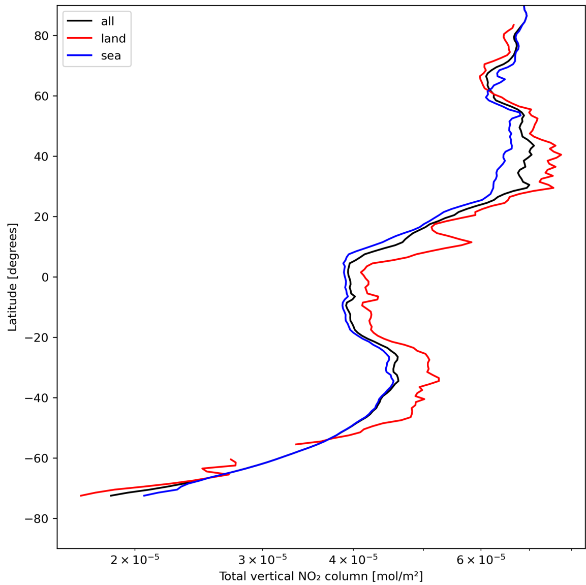
Figure 21: Zonal average of “Total vertical NO 2 column” for 2024-04-29 to 2024-05-01.
