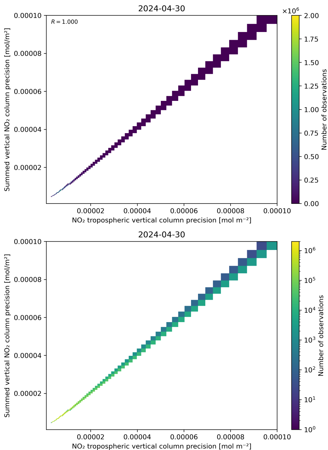
Figure 137: Scatter density plot of “NO 2 tropospheric vertical column precision” against “Summed vertical NO 2 column precision” for 2024-04-29 to 2024-05-01.
