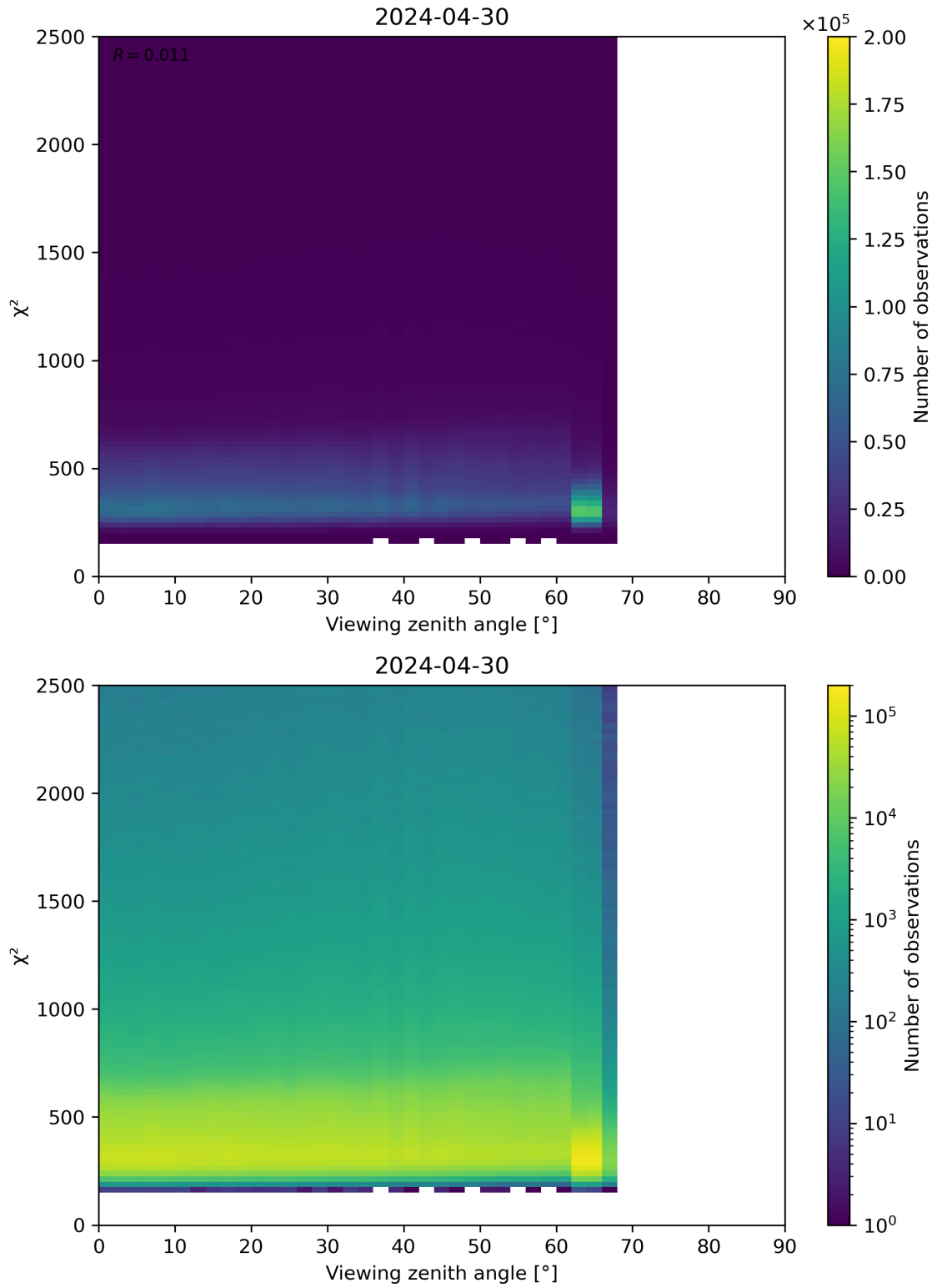
Figure 162: Scatter density plot of “Viewing zenith angle” against “ \chi^2 ” for 2024-04-29 to 2024-05-01.
