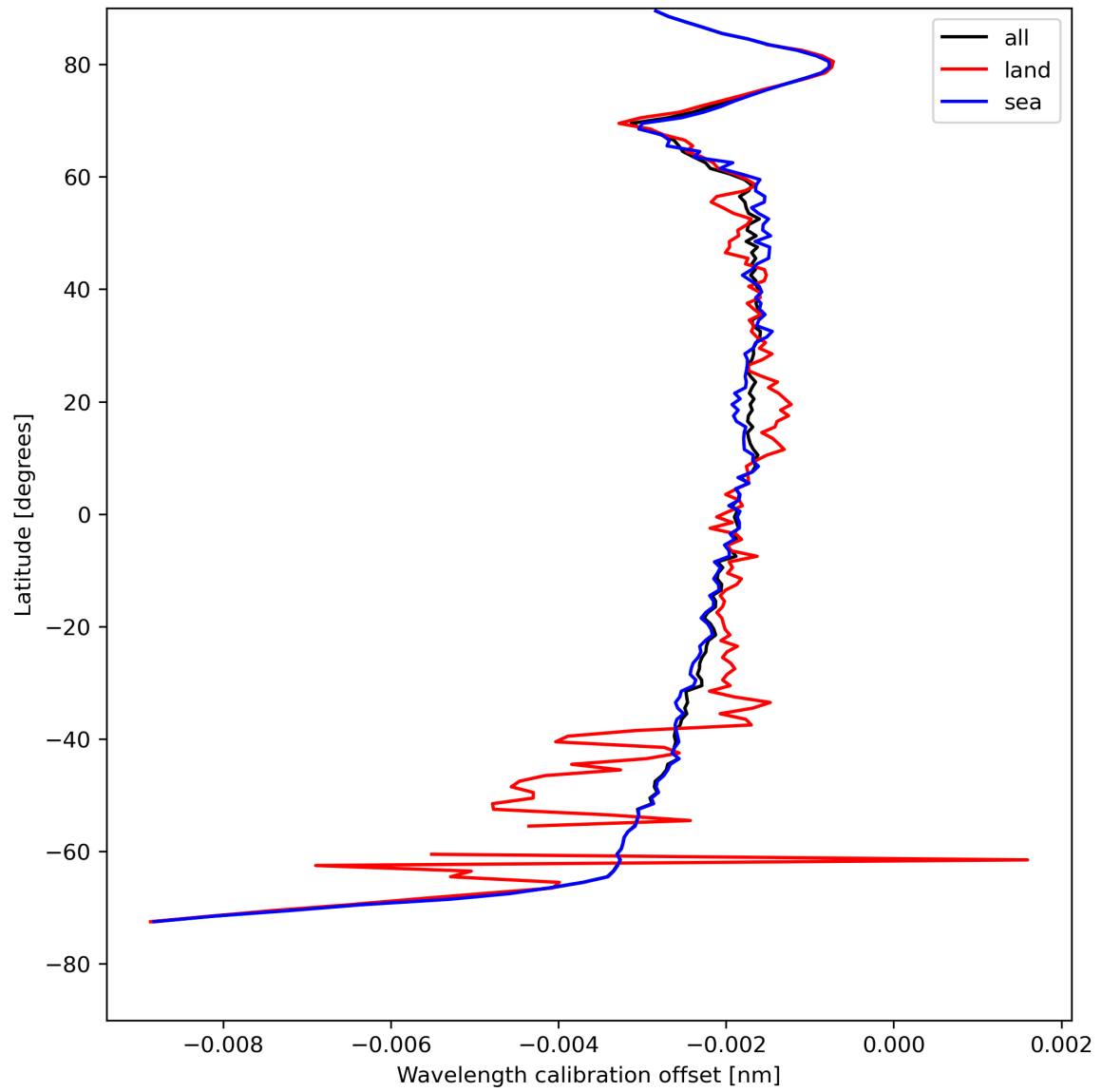
Figure 18: Zonal average of “Wavelength calibration offset” for 2024-04-29 to 2024-05-01.
