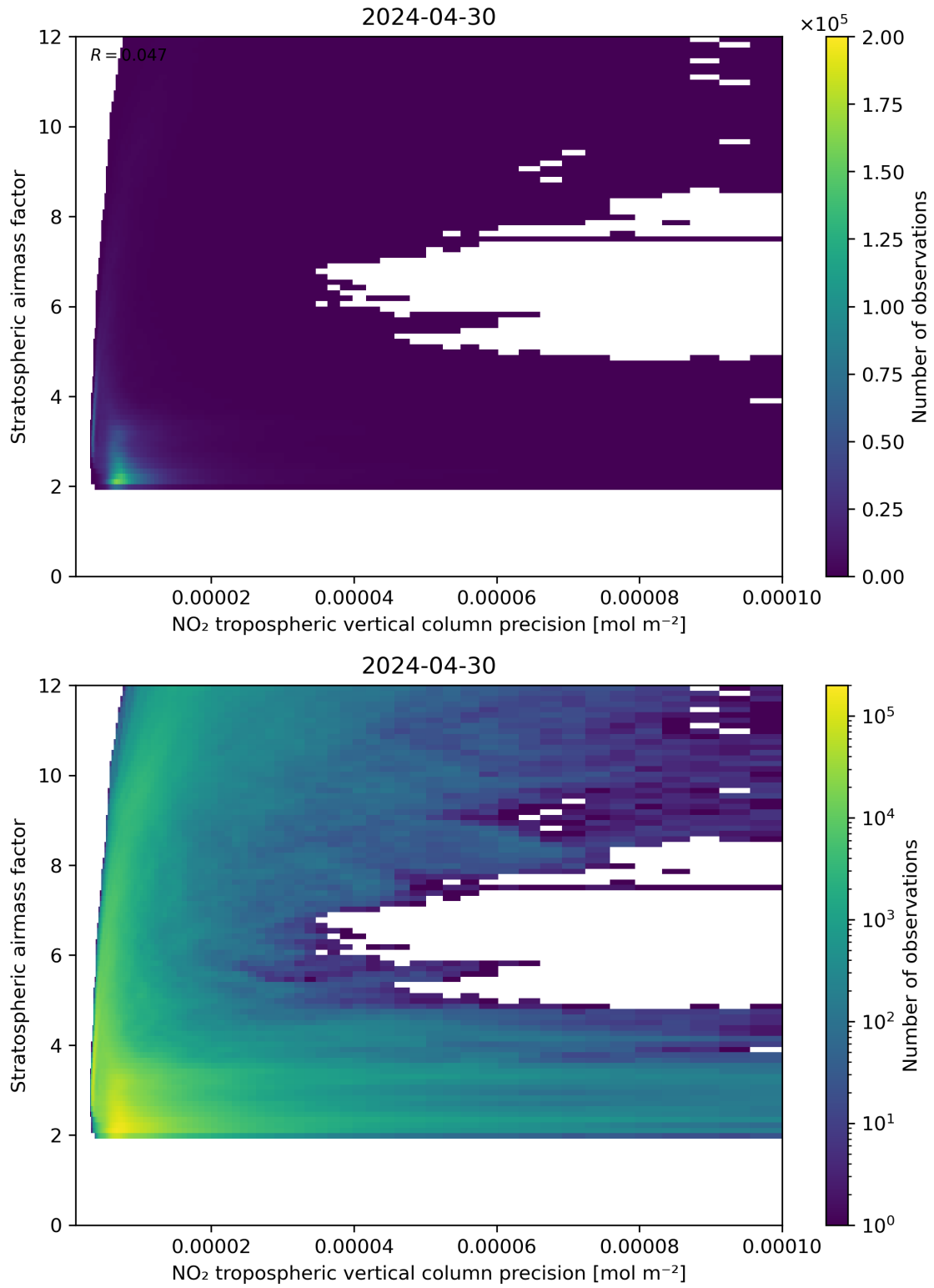
Figure 131: Scatter density plot of “NO 2 tropospheric vertical column precision” against “Stratospheric airmass factor” for 2024-04-29 to 2024-05-01.
