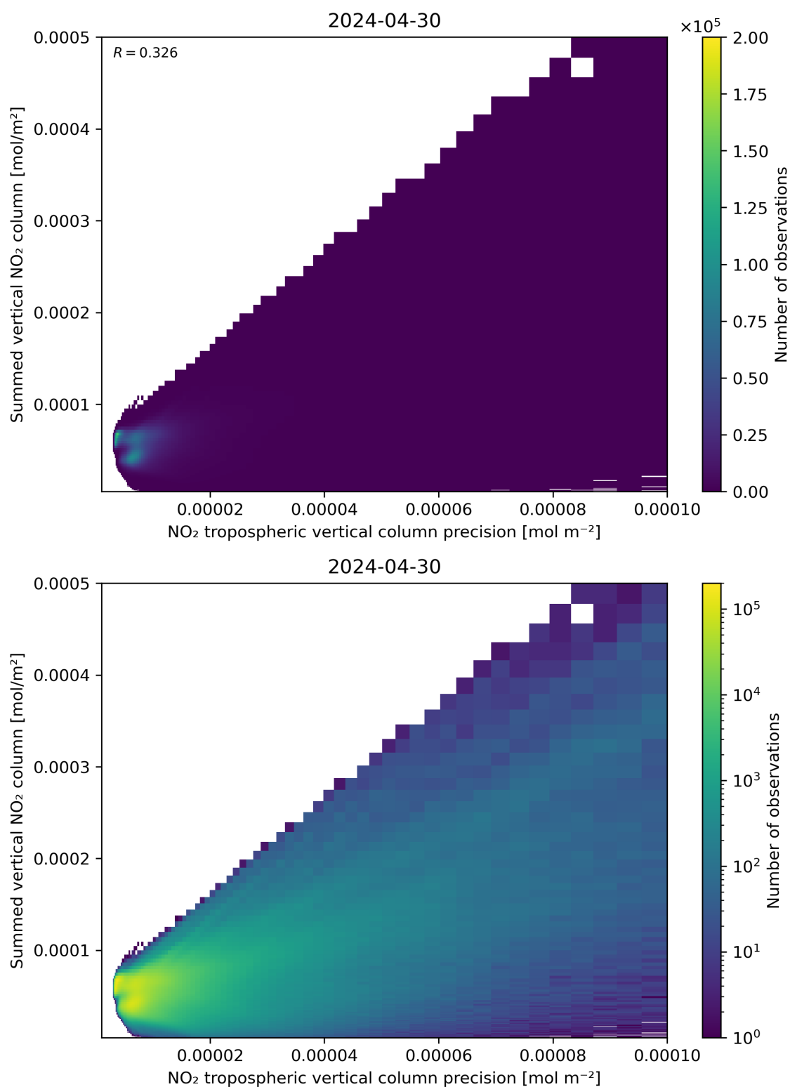
Figure 136: Scatter density plot of “NO 2 tropospheric vertical column precision” against “Summed vertical NO 2 column” for 2024-04-29 to 2024-05-01.
