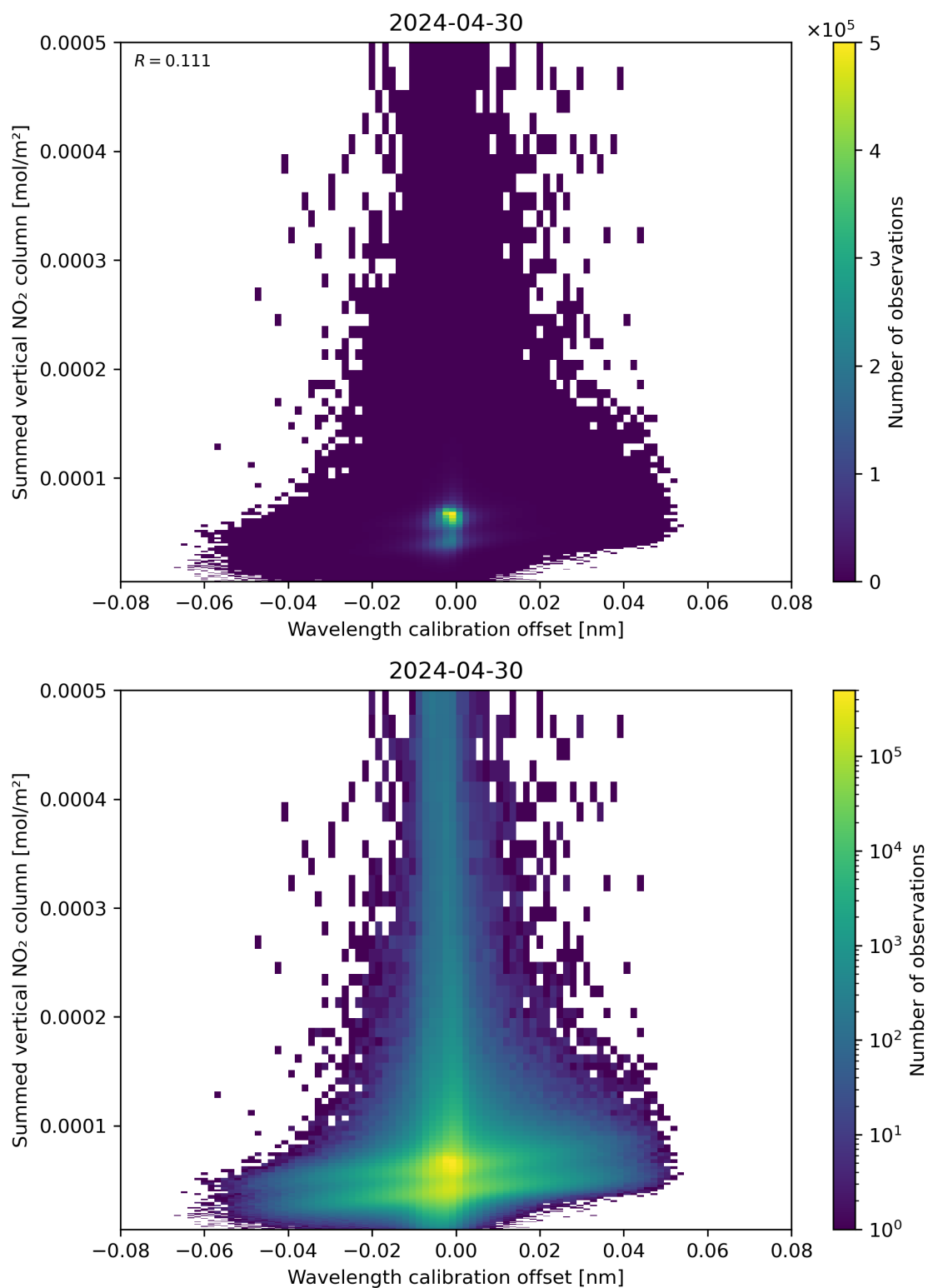
Figure 177: Scatter density plot of “Wavelength calibration offset” against “Summed vertical NO 2 column” for 2024-04-29 to 2024-05-01.
