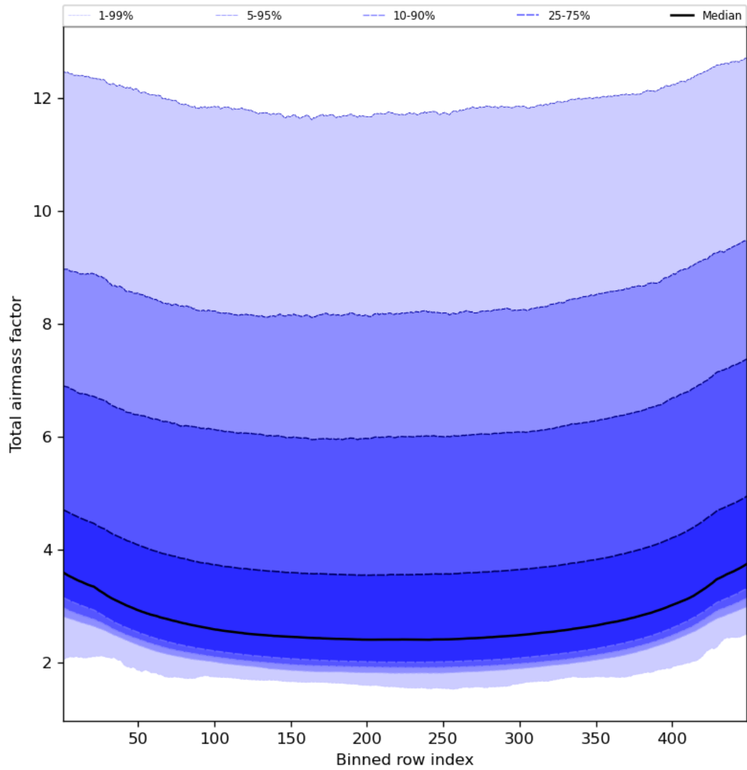
Figure 49: Along track statistics of “Total airmass factor” for 2024-04-29 to 2024-05-01
