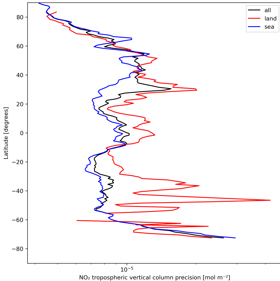
Figure 13: Zonal average of “NO 2 tropospheric vertical column precision” for 2024-04-29 to 2024-05-01.
