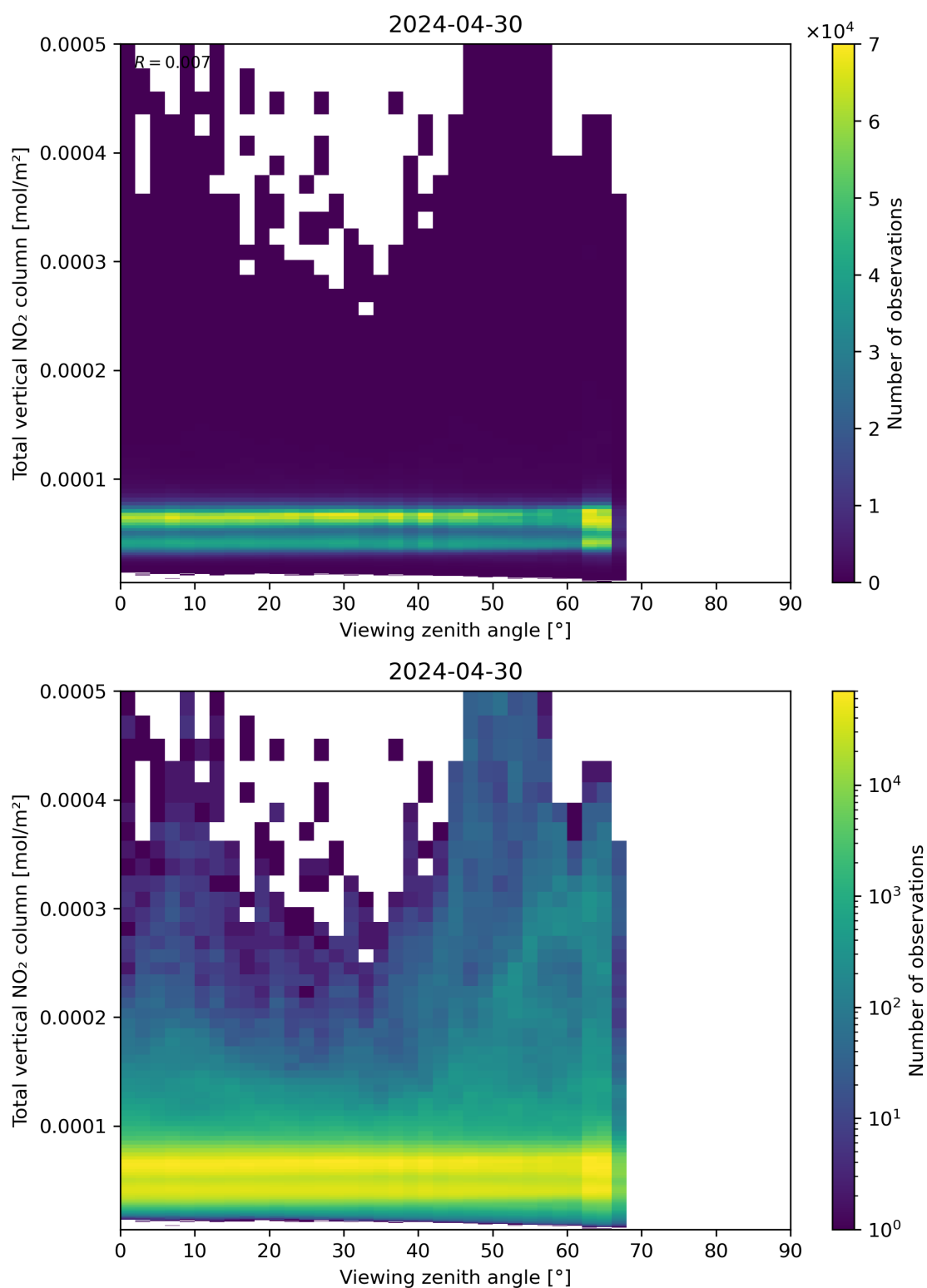
Figure 167: Scatter density plot of “Viewing zenith angle” against “Total vertical NO 2 column” for 2024-04-29 to 2024-05-01.
