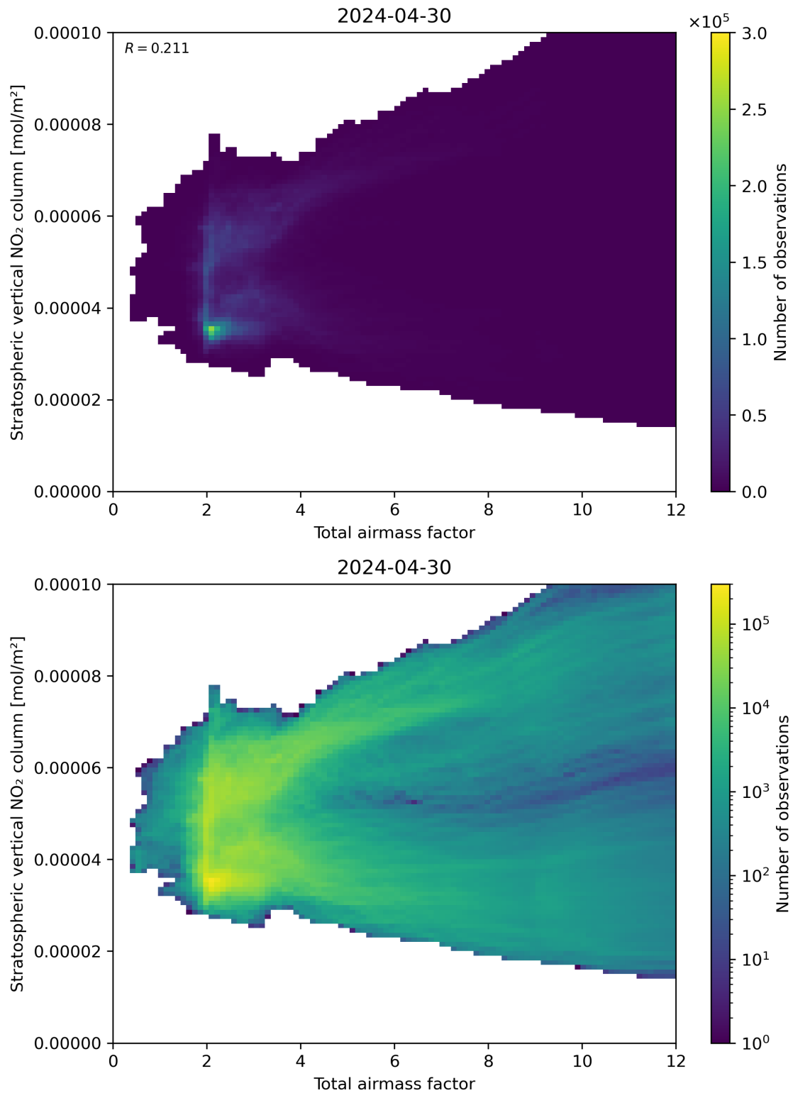
Figure 64: Scatter density plot of “Total airmass factor” against “Stratospheric vertical \text{NO}_2 column” for 2024-04-29 to 2024-05-01.
