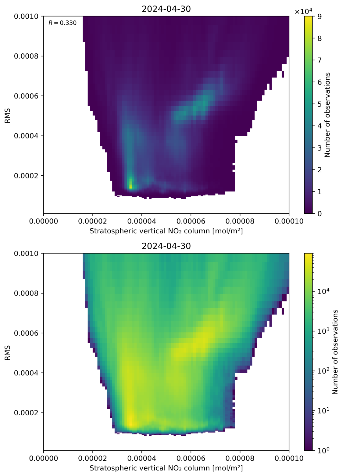
Figure 102: Scatter density plot of “Stratospheric vertical NO 2 column” against “RMS” for 2024-04-29 to 2024-05-01.
