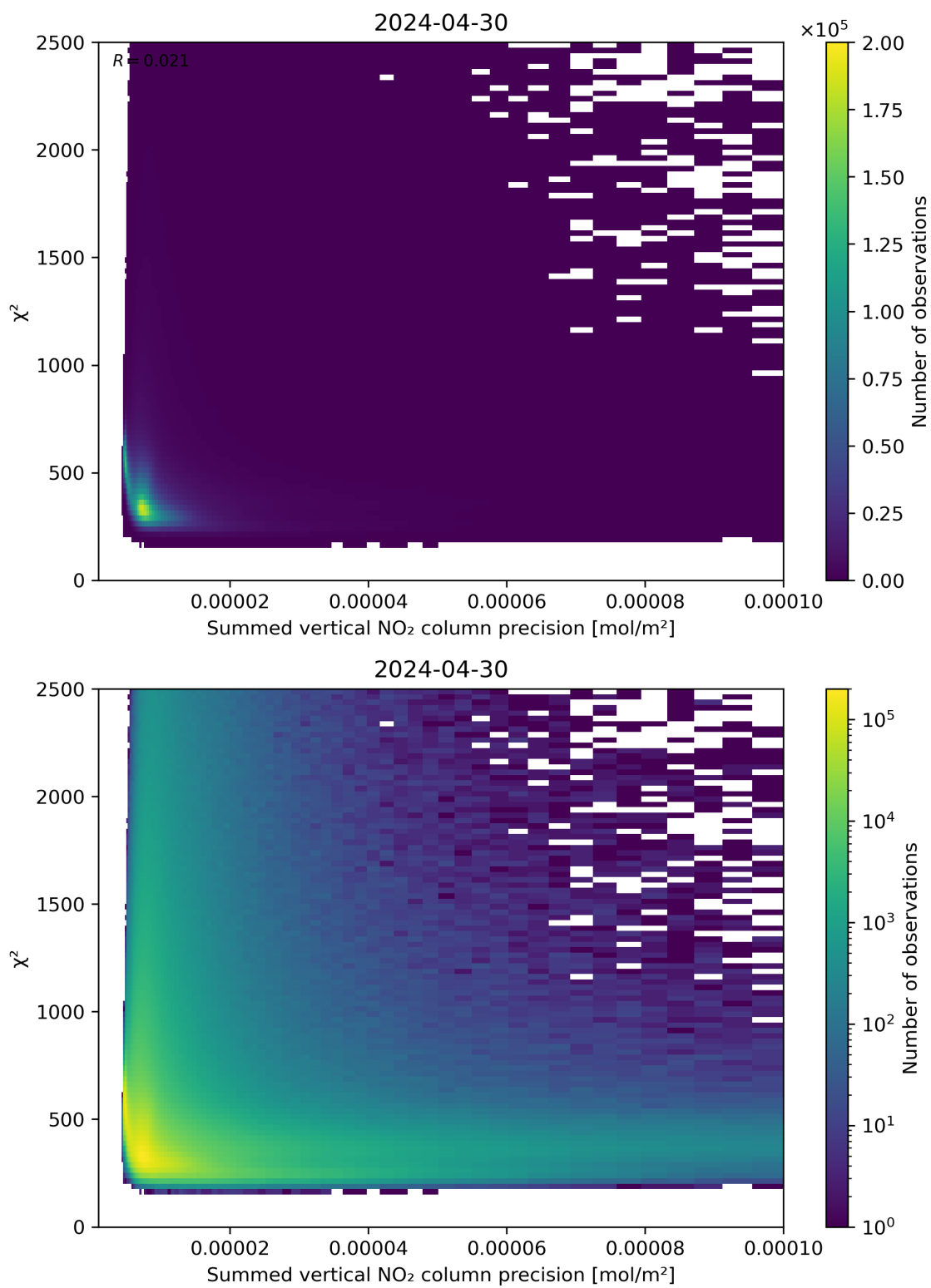
Figure 107: Scatter density plot of “Summed vertical NO 2 column precision” against “ \chi^2 ” for 2024-04-29 to 2024-05-01.
