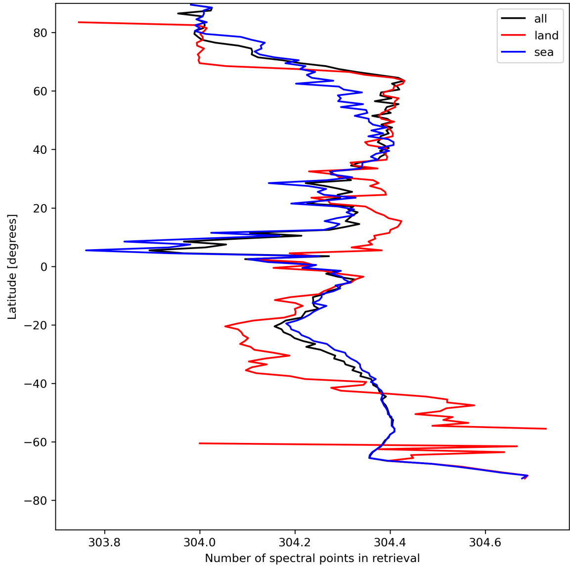
Figure 16: Zonal average of “Number of spectral points in retrieval” for 2024-04-29 to 2024-05-01.
