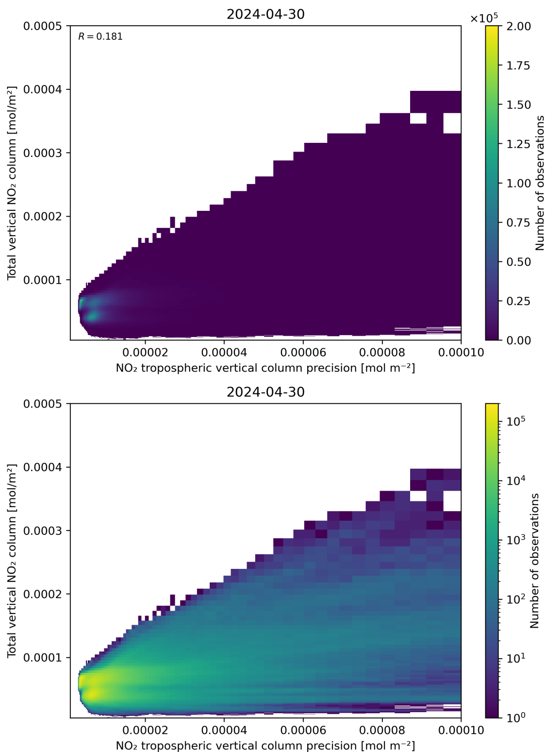
Figure 138: Scatter density plot of “NO 2 tropospheric vertical column precision” against “Total vertical NO 2 column” for 2024-04-29 to 2024-05-01.
