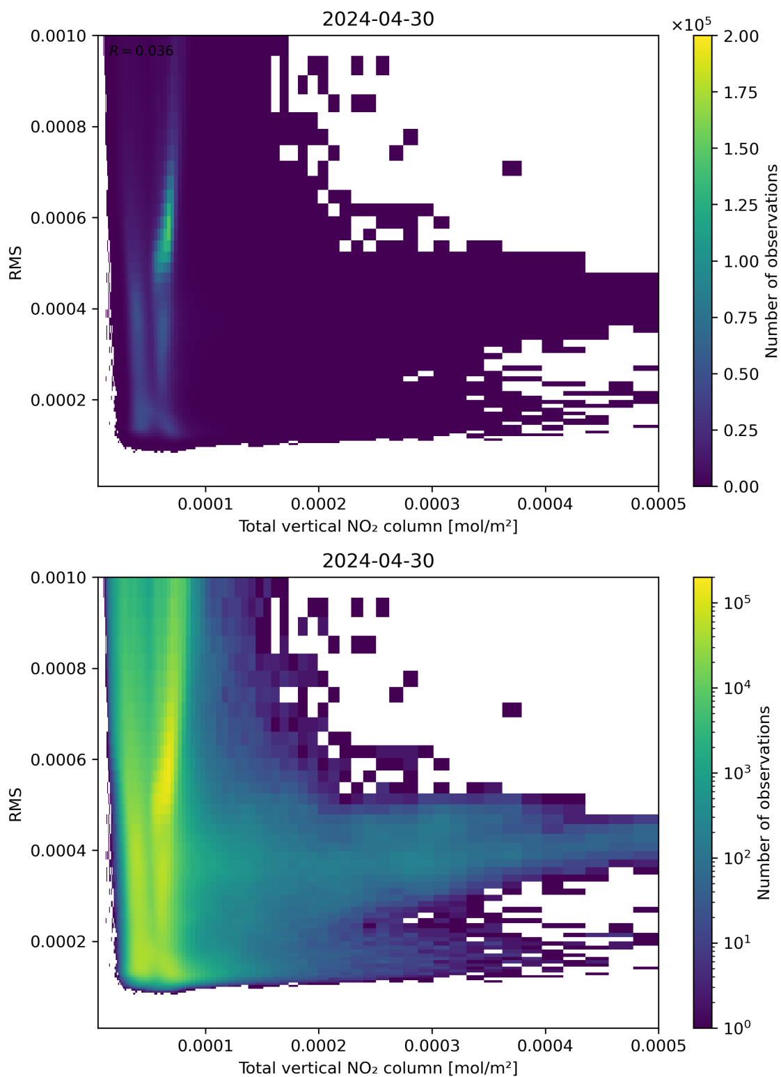
Figure 120: Scatter density plot of “Total vertical NO 2 column” against “RMS” for 2024-04-29 to 2024-05-01.
