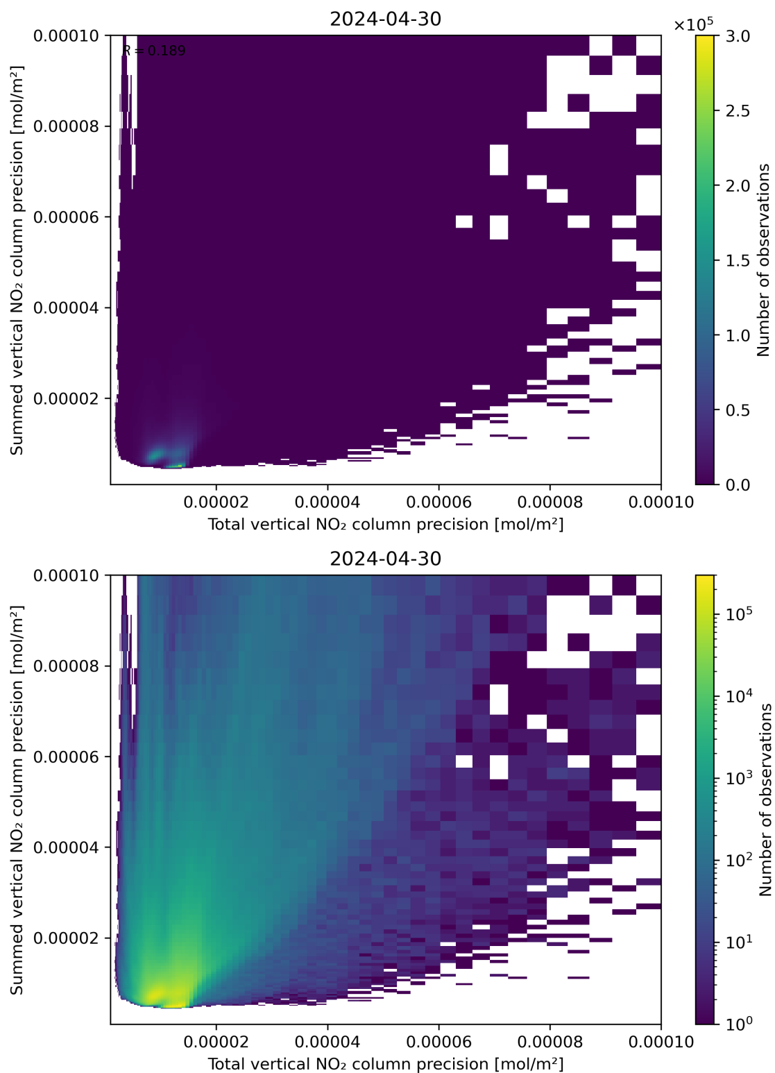
Figure 118: Scatter density plot of “Total vertical NO 2 column precision” against “Summed vertical NO 2 column precision” for 2024-04-29 to 2024-05-01.
