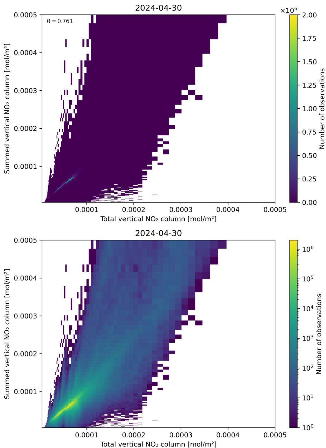
Figure 112: Scatter density plot of “Total vertical NO 2 column” against “Summed vertical NO 2 column” for 2024-04-29 to 2024-05-01.
