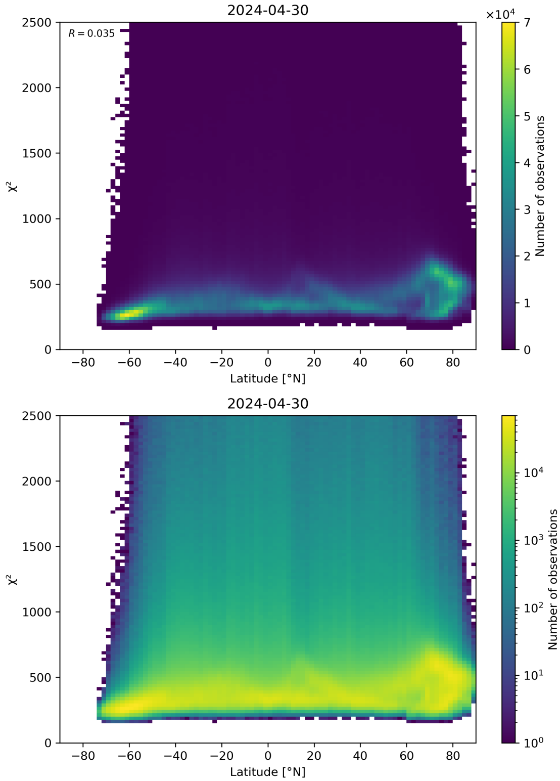
Figure 86: Scatter density plot of “Latitude” against “ \chi^2 ” for 2024-04-29 to 2024-05-01.
