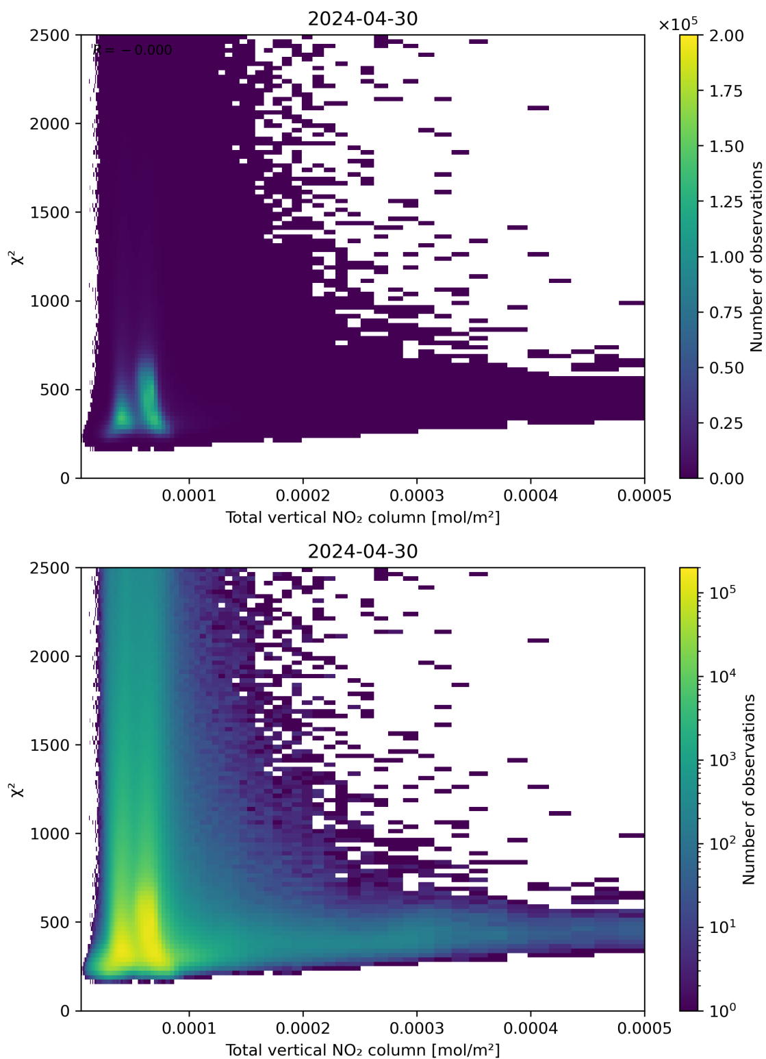
Figure 111: Scatter density plot of “Total vertical NO 2 column” against “ \chi^2 ” for 2024-04-29 to 2024-05-01.
