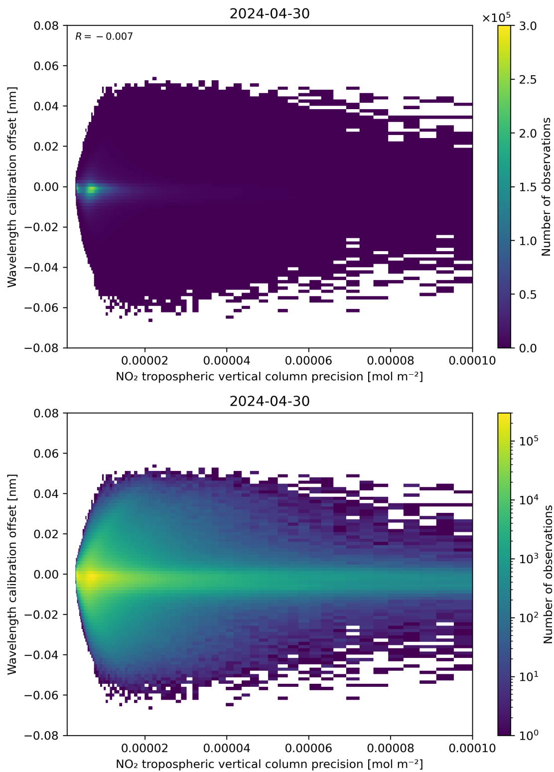
Figure 141: Scatter density plot of “NO 2 tropospheric vertical column precision” against “Wavelength calibration offset” for 2024-04-29 to 2024-05-01.
