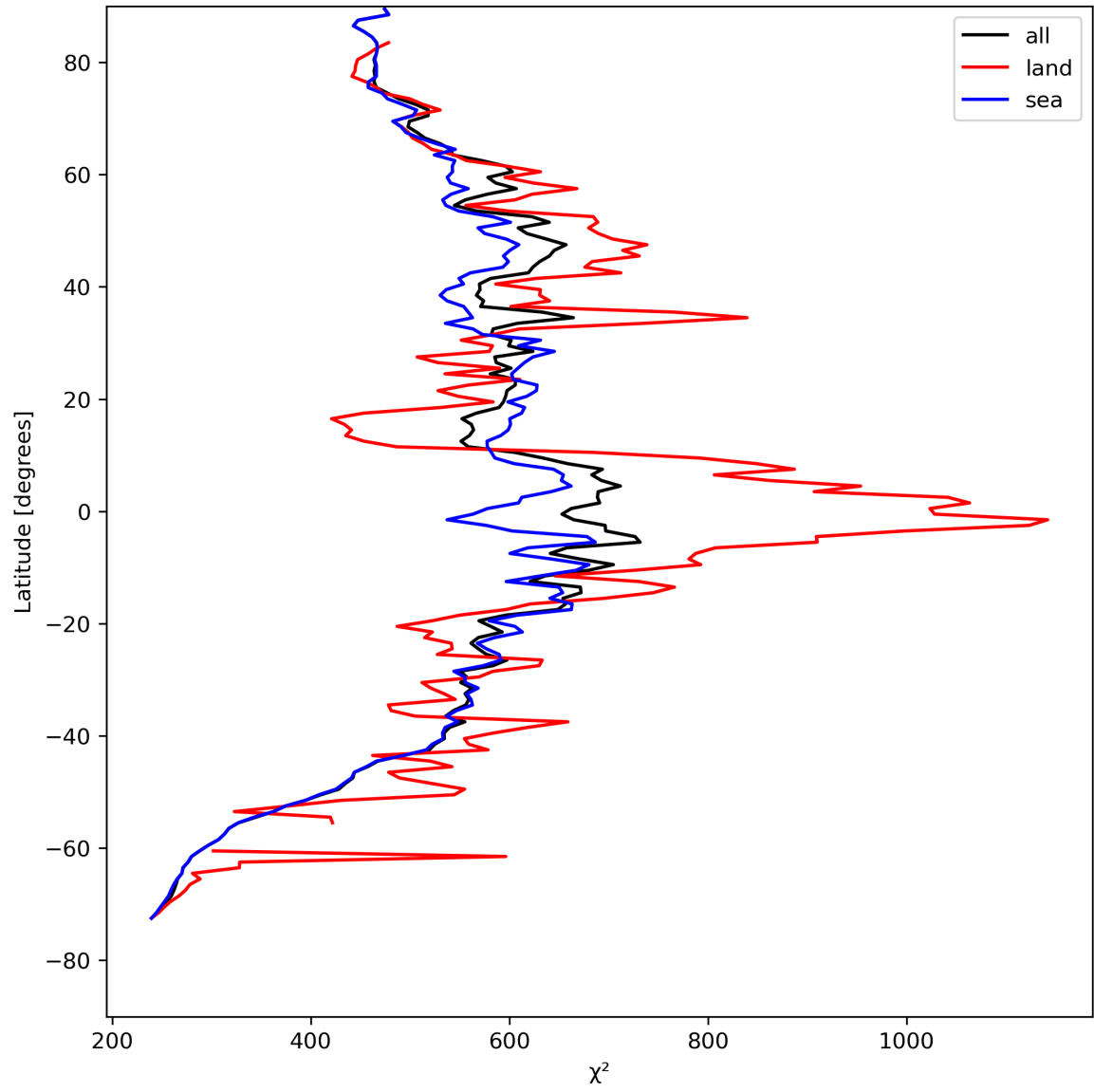
Figure 25: Zonal average of “ \chi^2 ” for 2024-04-29 to 2024-05-01.
