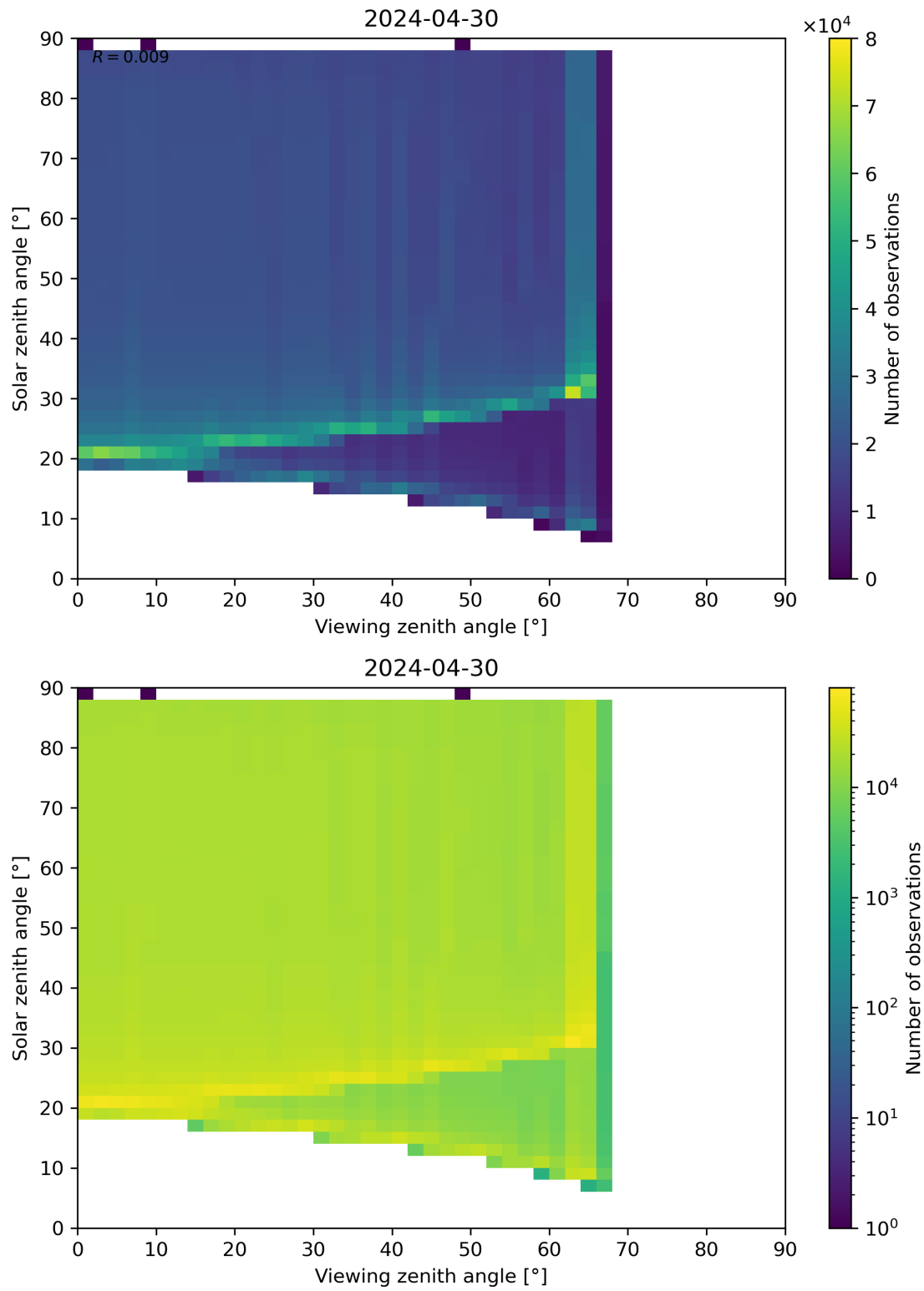
Figure 172: Scatter density plot of “Viewing zenith angle” against “Solar zenith angle” for 2024-04-29 to 2024-05-01.
