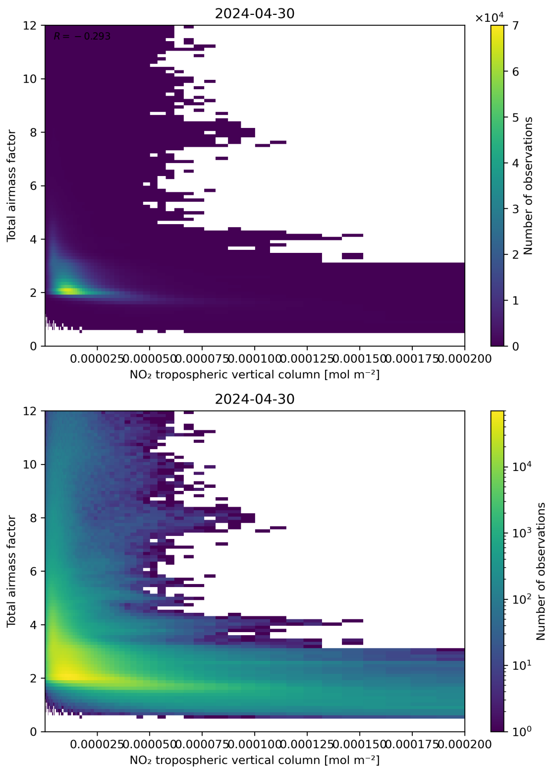
Figure 122: Scatter density plot of “NO 2 tropospheric vertical column” against “Total air mass factor” for 2024-04-29 to 2024-05-01.
