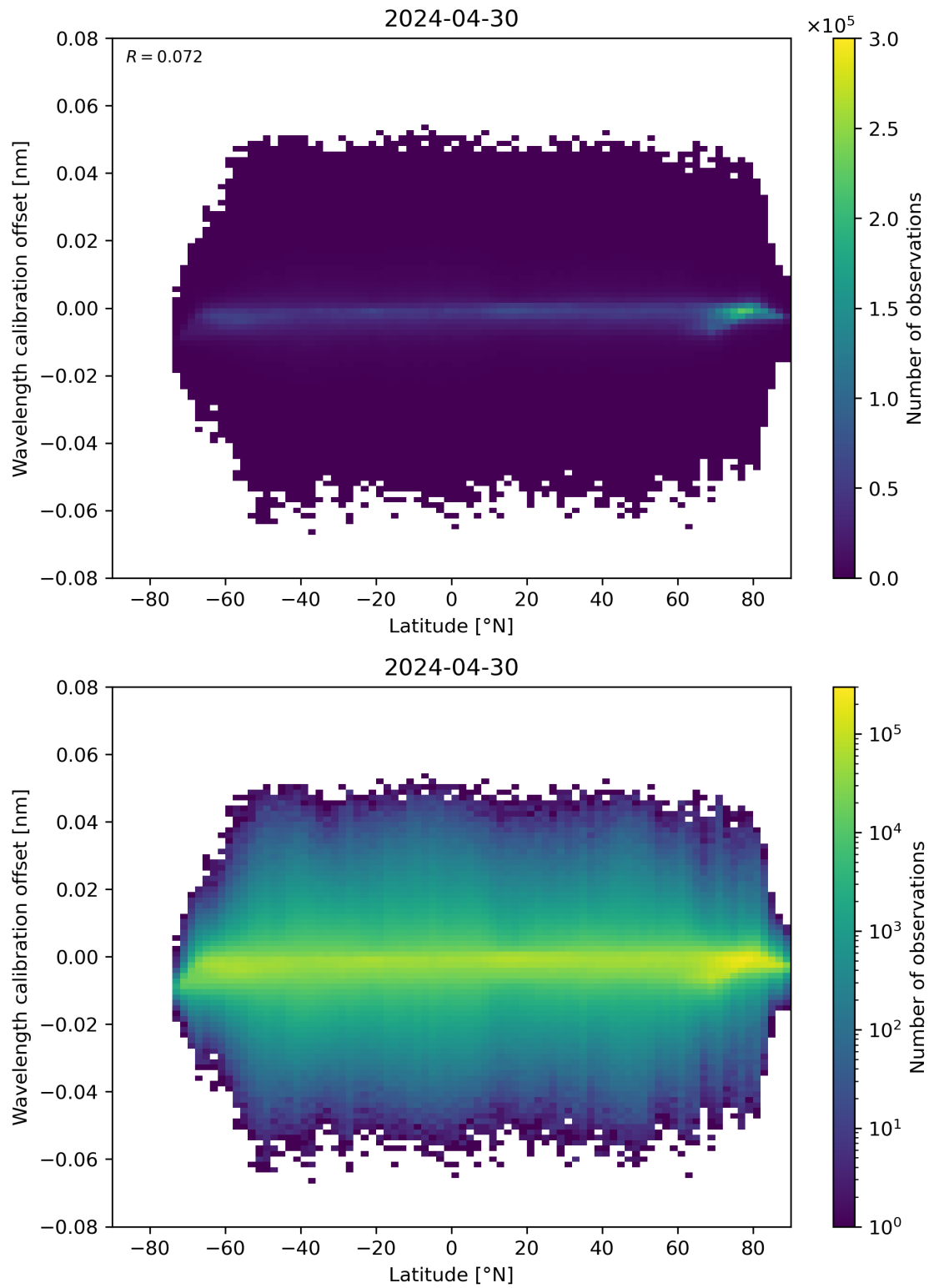
Figure 95: Scatter density plot of “Latitude” against “Wavelength calibration offset” for 2024-04-29 to 2024-05-01.
