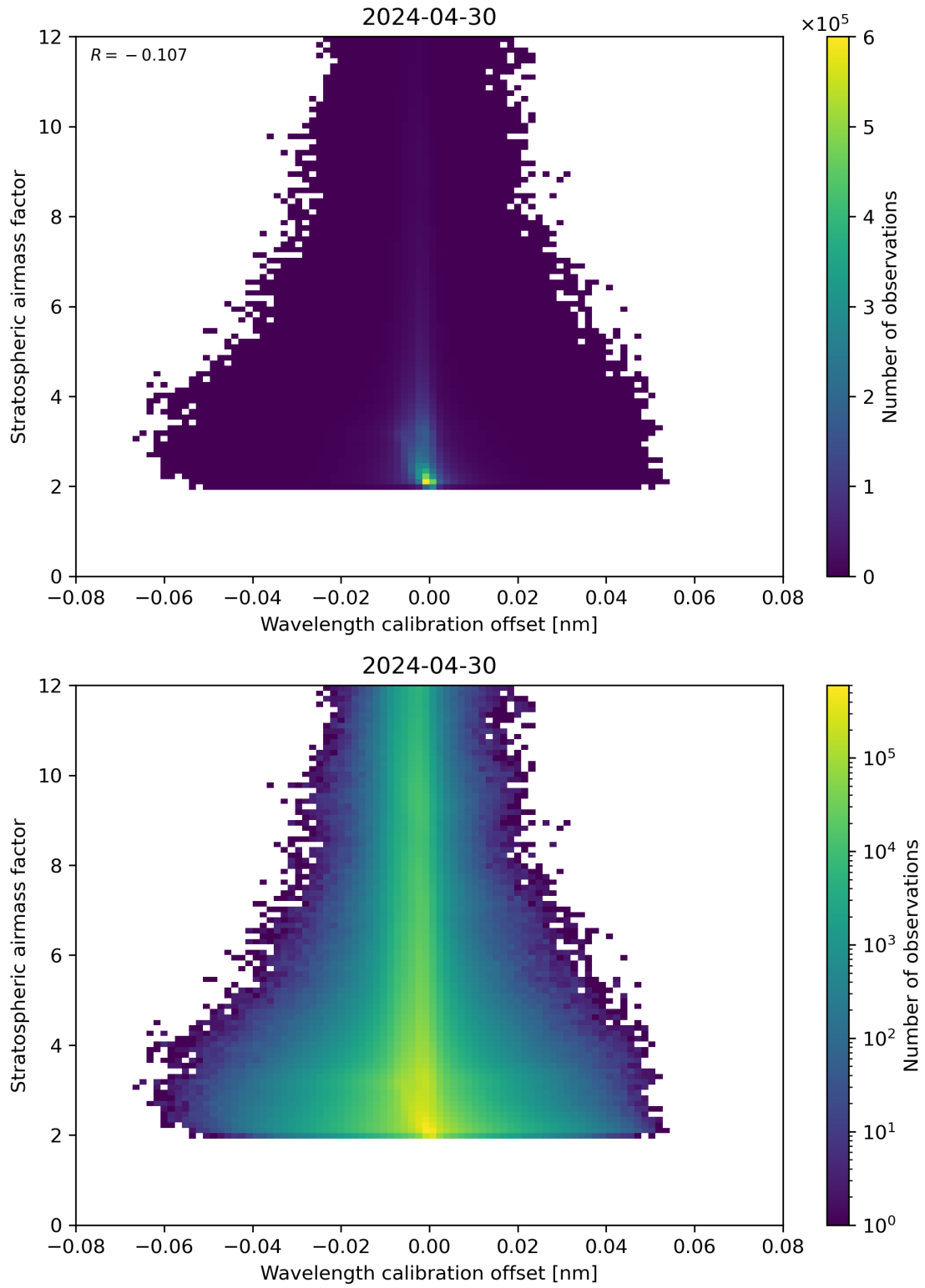
Figure 174: Scatter density plot of “Wavelength calibration offset” against “Stratospheric airmass factor” for 2024-04-29 to 2024-05-01.
