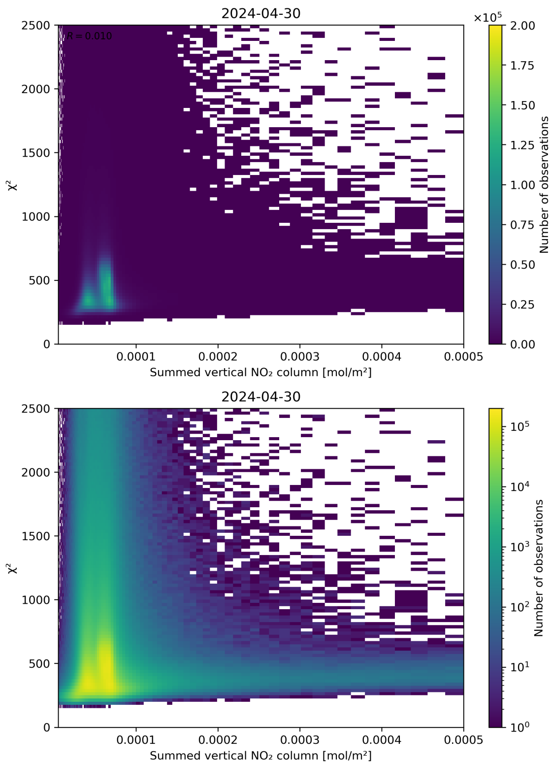
Figure 104: Scatter density plot of “Summed vertical NO 2 column” against “ \chi^2 ” for 2024-04-29 to 2024-05-01.
