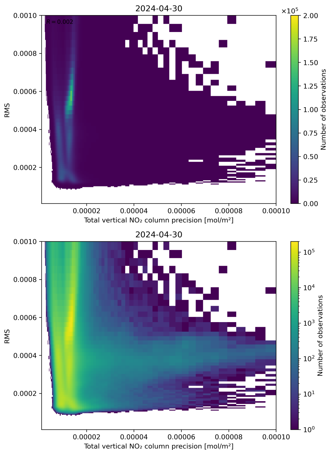
Figure 119: Scatter density plot of “Total vertical NO 2 column precision” against “RMS” for 2024-04-29 to 2024-05-01.
