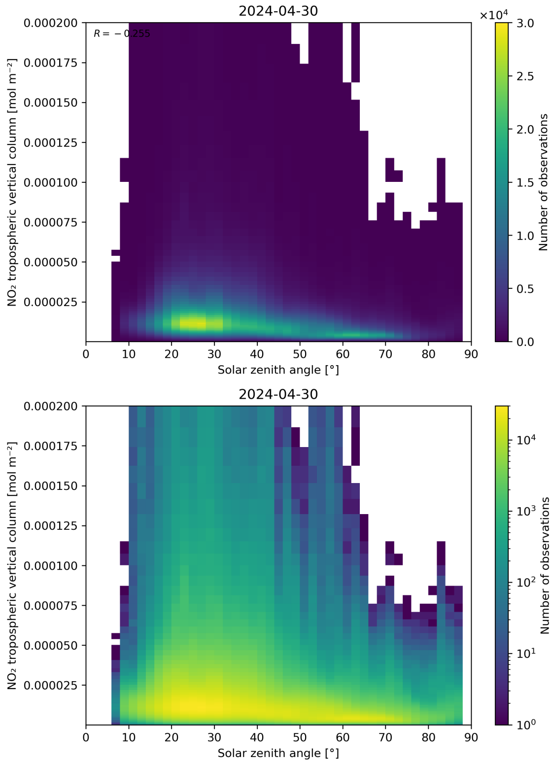
Figure 155: Scatter density plot of “Solar zenith angle” against “NO 2 tropospheric vertical column” for 2024-04-29 to 2024-05-01.
