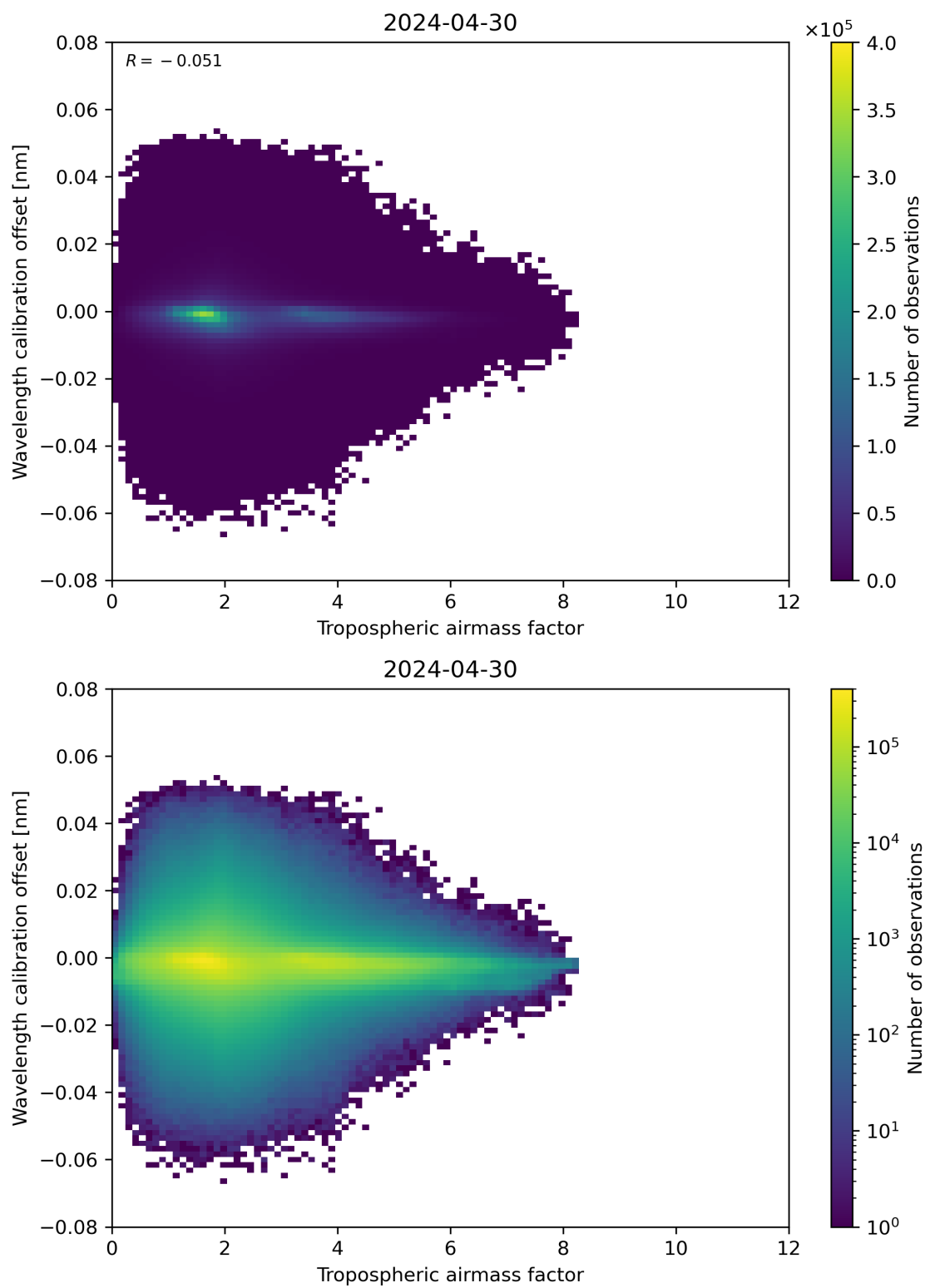
Figure 80: Scatter density plot of “Tropospheric air mass factor” against “Wavelength calibration offset” for 2024-04-29 to 2024-05-01.
