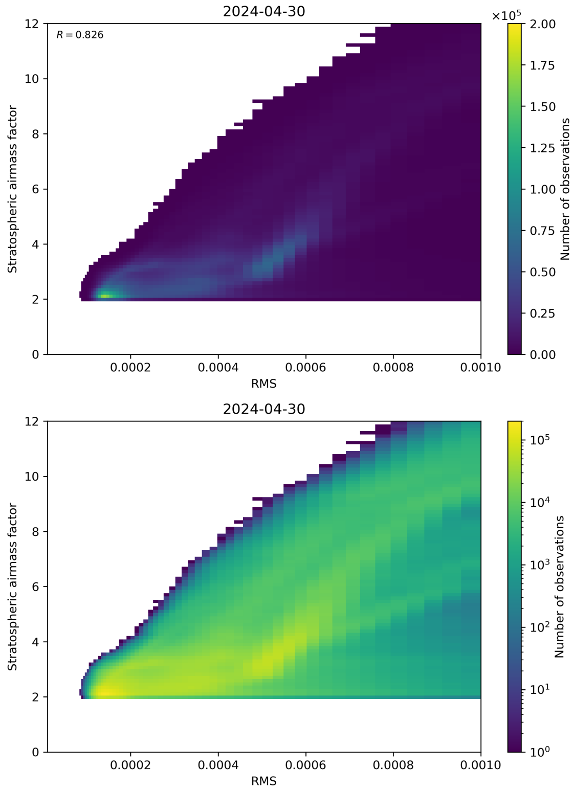
Figure 144: Scatter density plot of “RMS” against “Stratospheric airmass factor” for 2024-04-29 to 2024-05-01.
