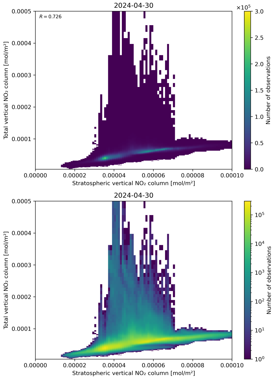
Figure 100: Scatter density plot of “Stratospheric vertical NO 2 column” against “Total vertical NO 2 column” for 2024-04-29 to 2024-05-01.
