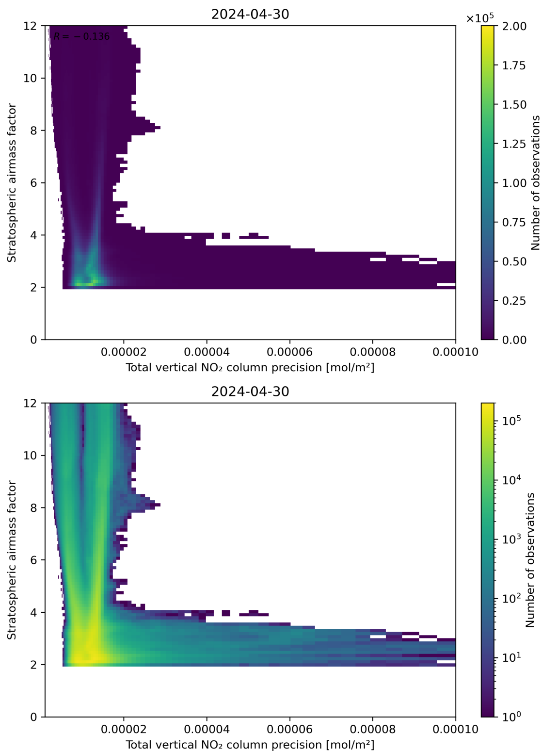
Figure 115: Scatter density plot of “Total vertical NO 2 column precision” against “Stratospheric air mass factor” for 2024-04-29 to 2024-05-01.
