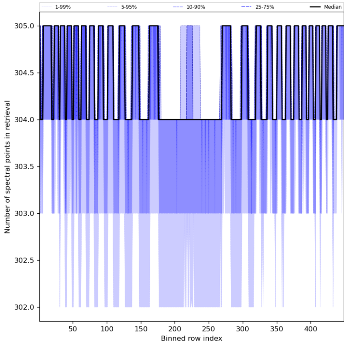
Figure 50: Along track statistics of “Number of spectral points in retrieval” for 2024-04-29 to 2024-05-01
