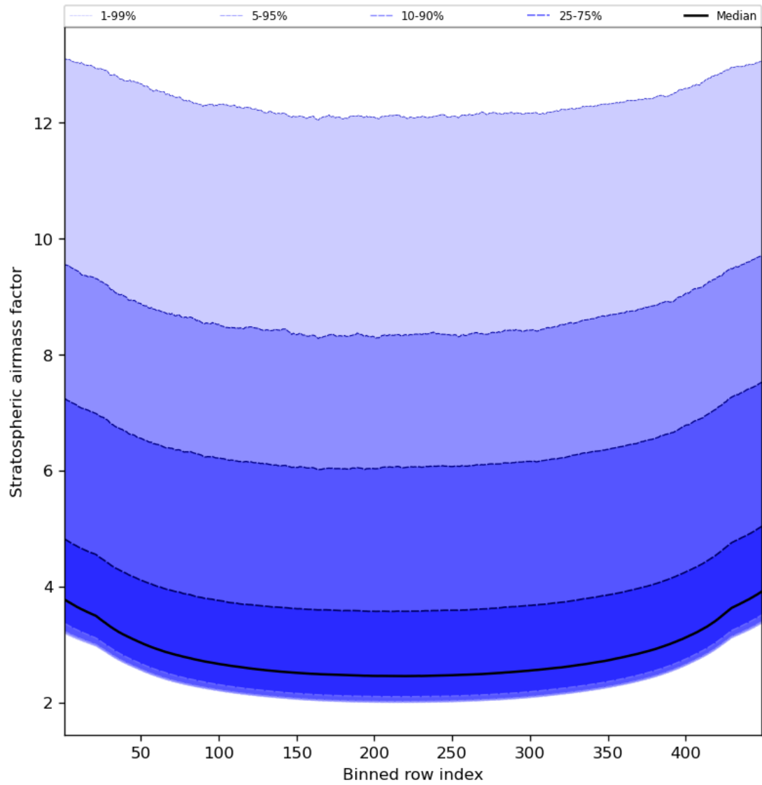
Figure 61: Along track statistics of “Stratospheric airmass factor” for 2024-04-29 to 2024-05-01
