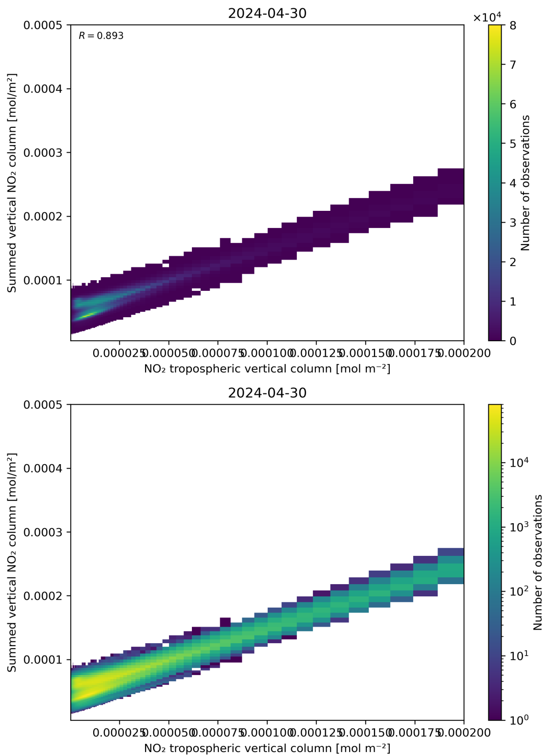
Figure 126: Scatter density plot of “NO 2 tropospheric vertical column” against “Summed vertical NO 2 column” for 2024-04-29 to 2024-05-01.
