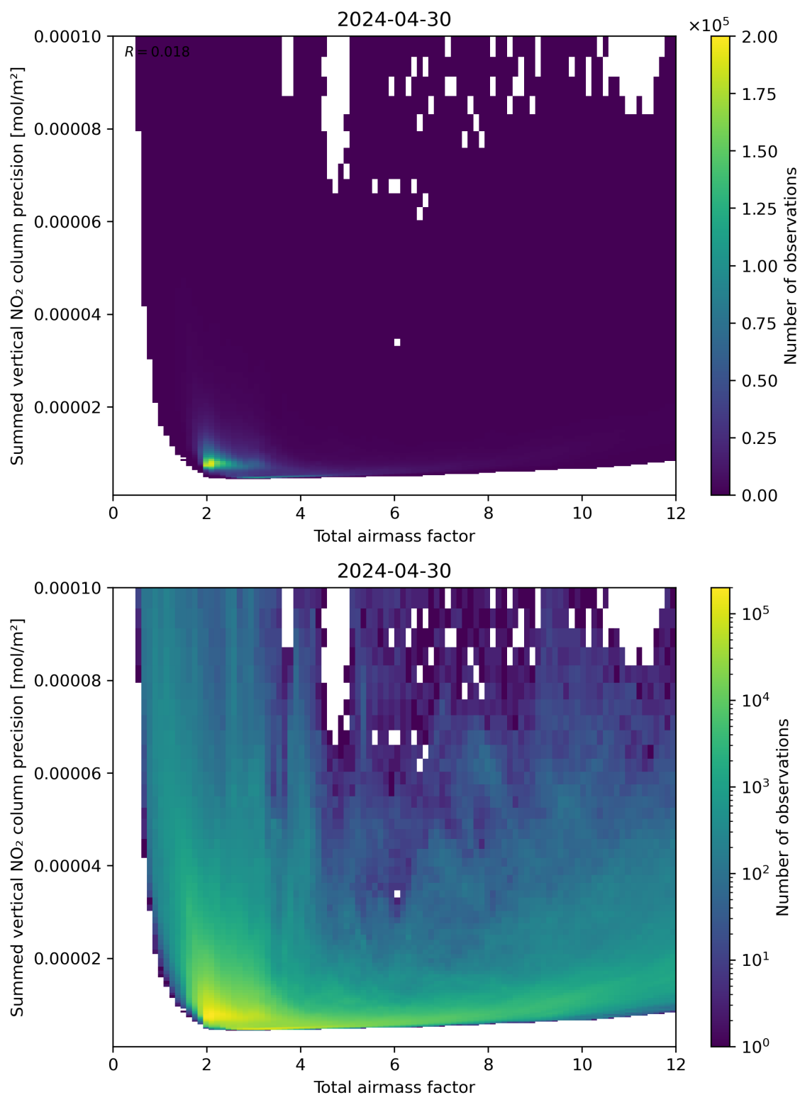
Figure 66: Scatter density plot of “Total airmass factor” against “Summed vertical NO 2 column precision” for 2024-04-29 to 2024-05-01.
