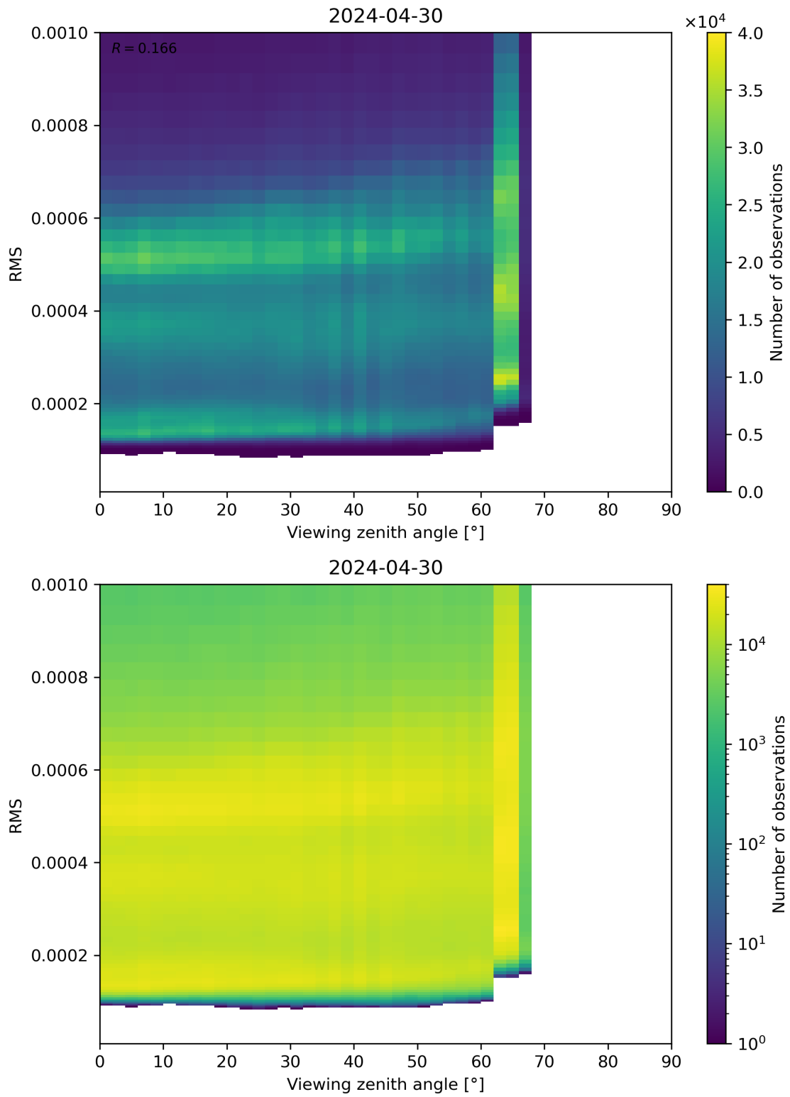
Figure 171: Scatter density plot of “Viewing zenith angle” against “RMS” for 2024-04-29 to 2024-05-01.
