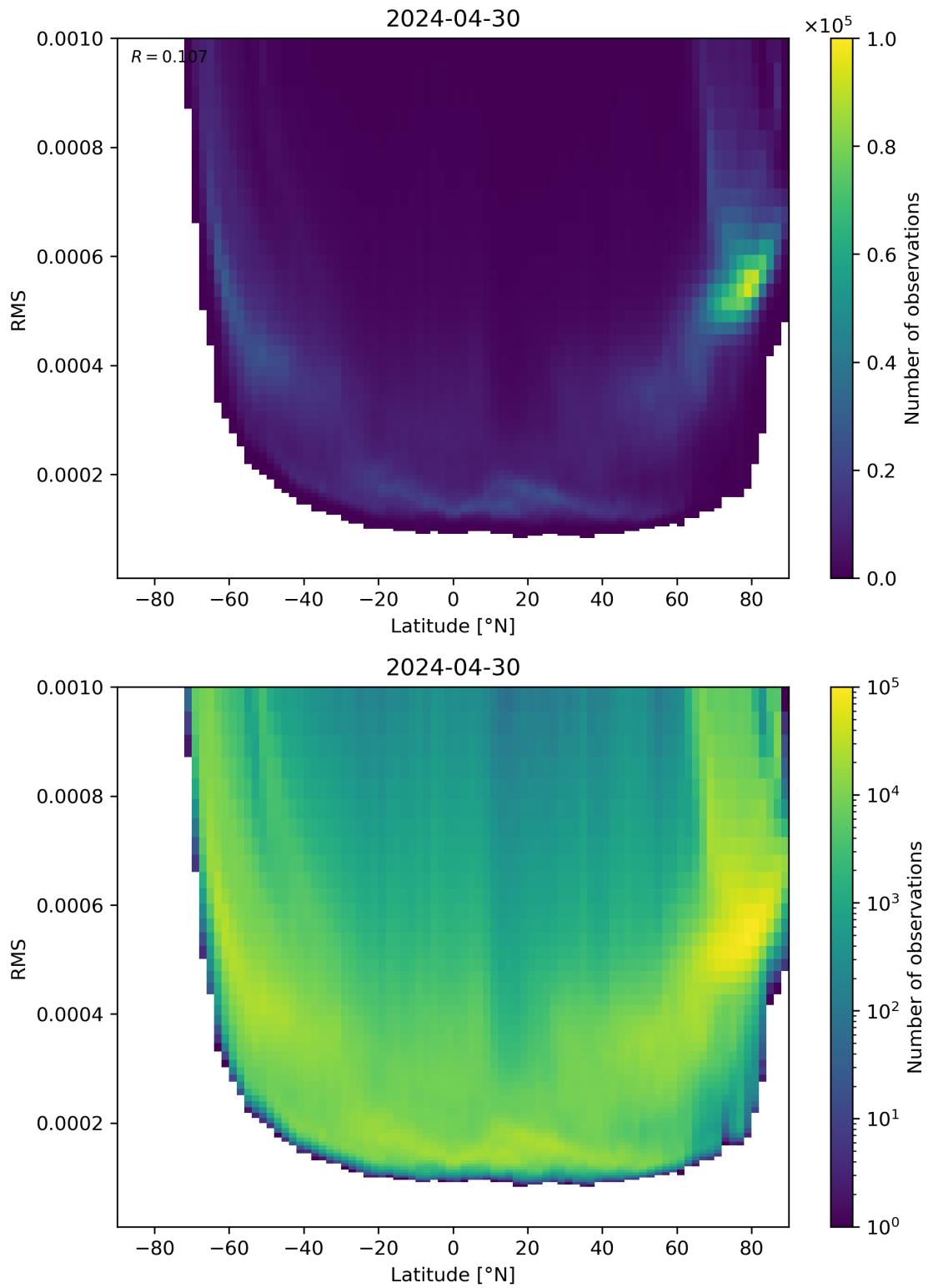
Figure 94: Scatter density plot of “Latitude” against “RMS” for 2024-04-29 to 2024-05-01.
