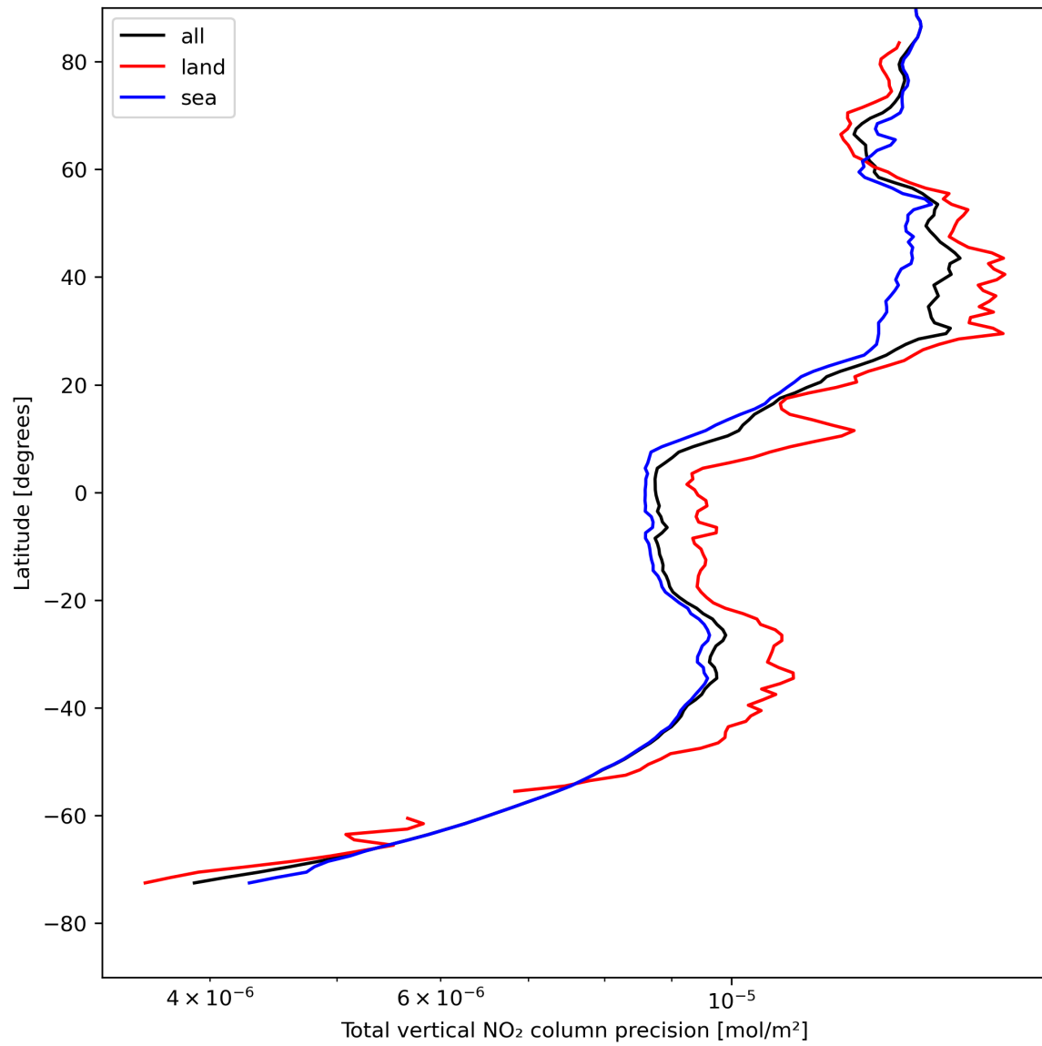
Figure 22: Zonal average of “Total vertical NO 2 column precision” for 2024-04-29 to 2024-05-01.
