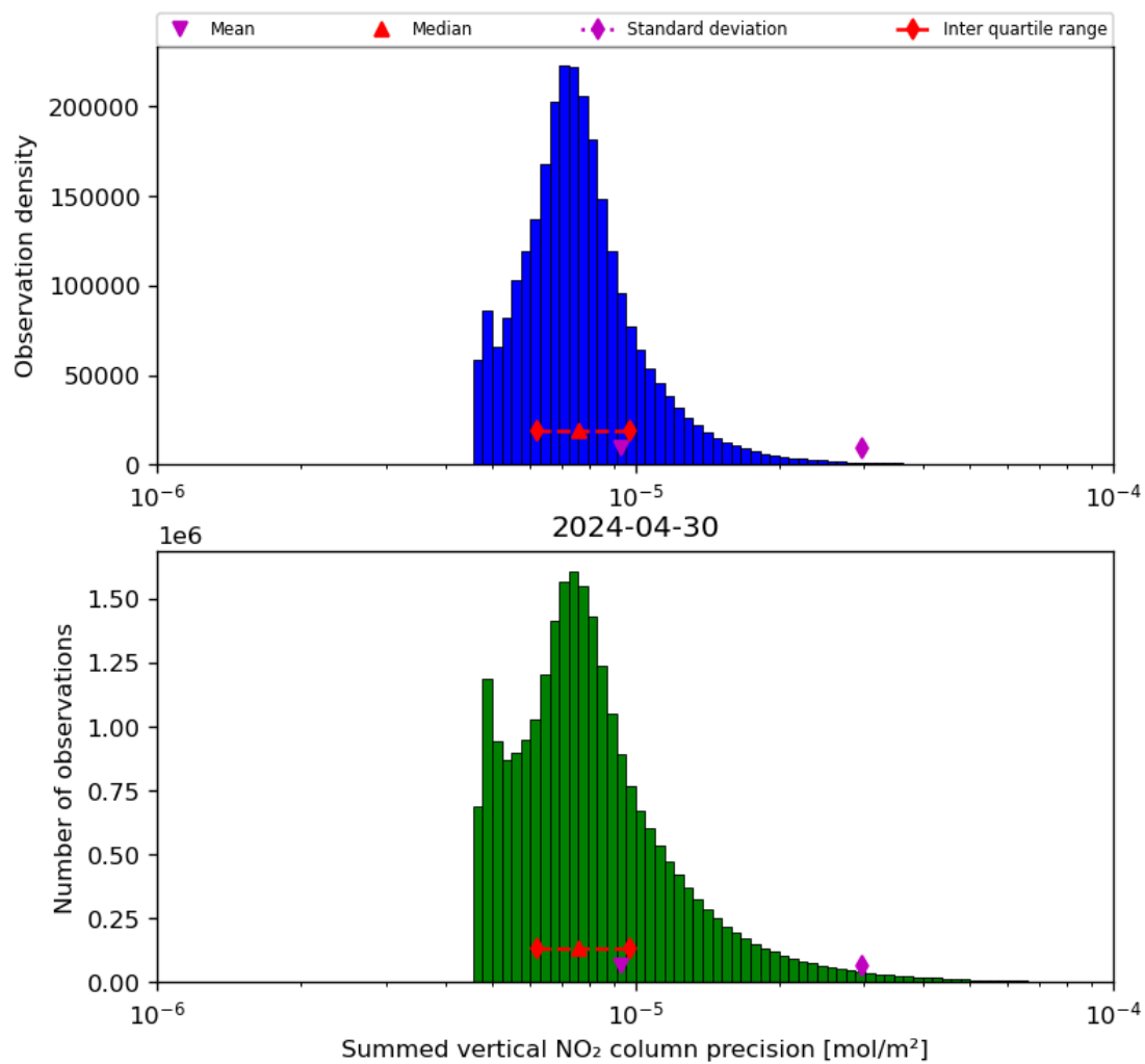
Figure 41: Histogram of "Summed vertical NO 2 column precision" for 2024-04-29 to 2024-05-01
