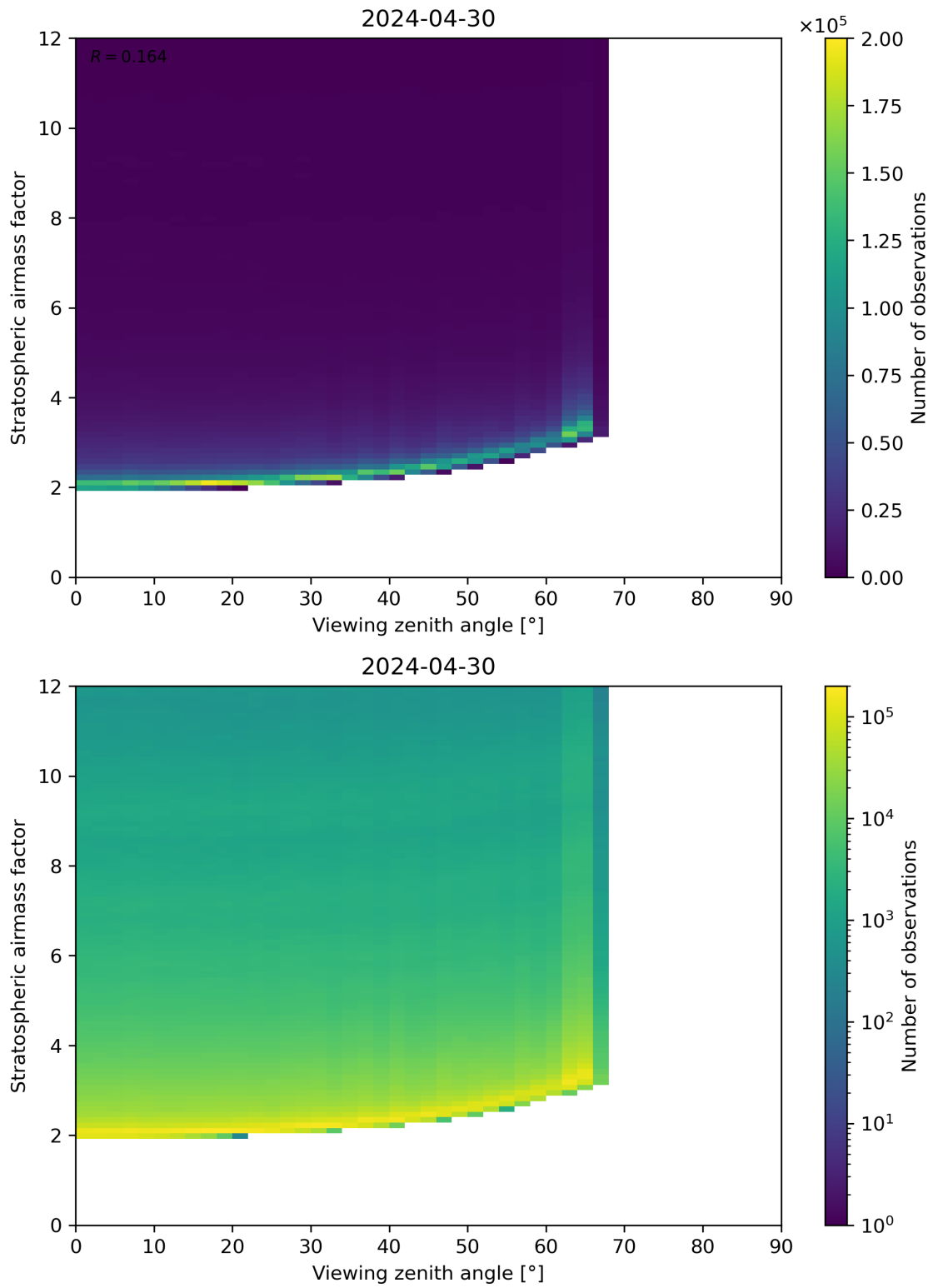
Figure 159: Scatter density plot of “Viewing zenith angle” against “Stratospheric airmass factor” for 2024-04-29 to 2024-05-01.
