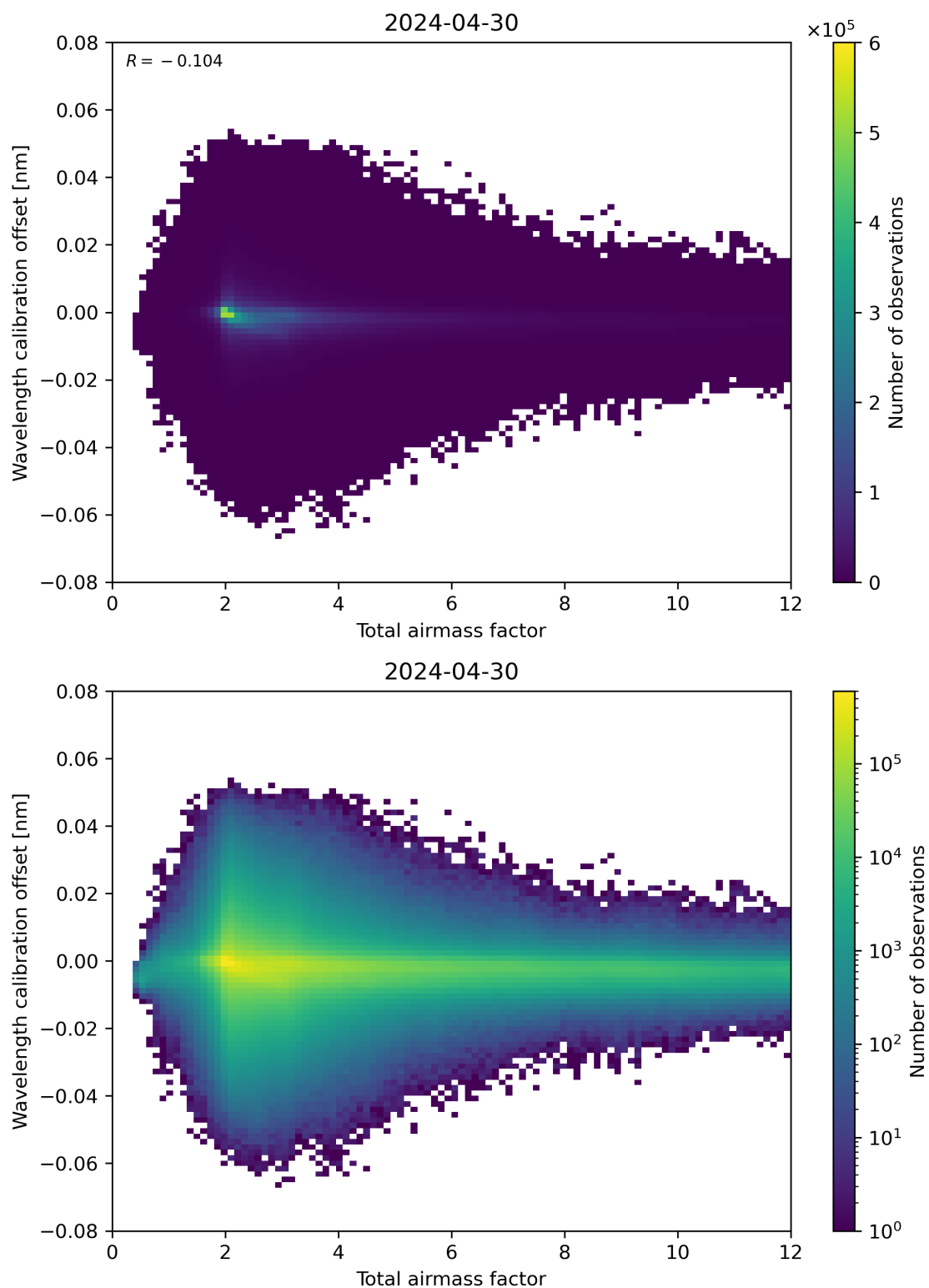
Figure 70: Scatter density plot of “Total airmass factor” against “Wavelength calibration offset” for 2024-04-29 to 2024-05-01.
