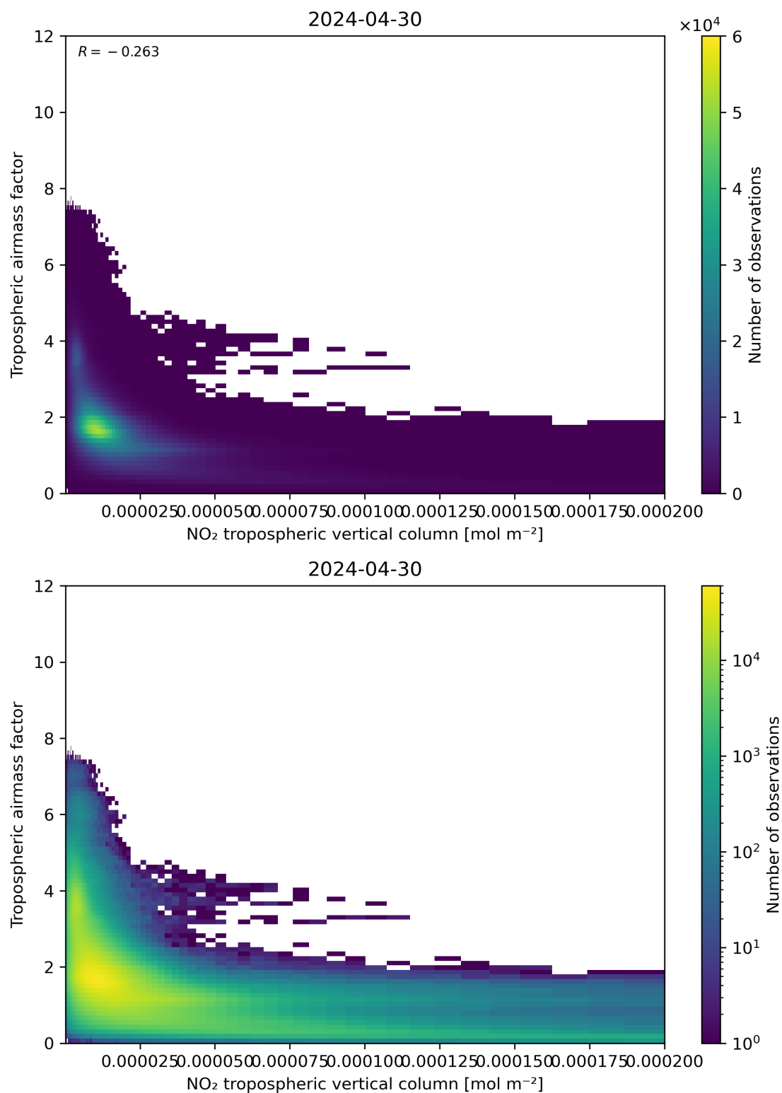
Figure 123: Scatter density plot of “NO 2 tropospheric vertical column” against “Tropospheric air mass factor” for 2024-04-29 to 2024-05-01.
