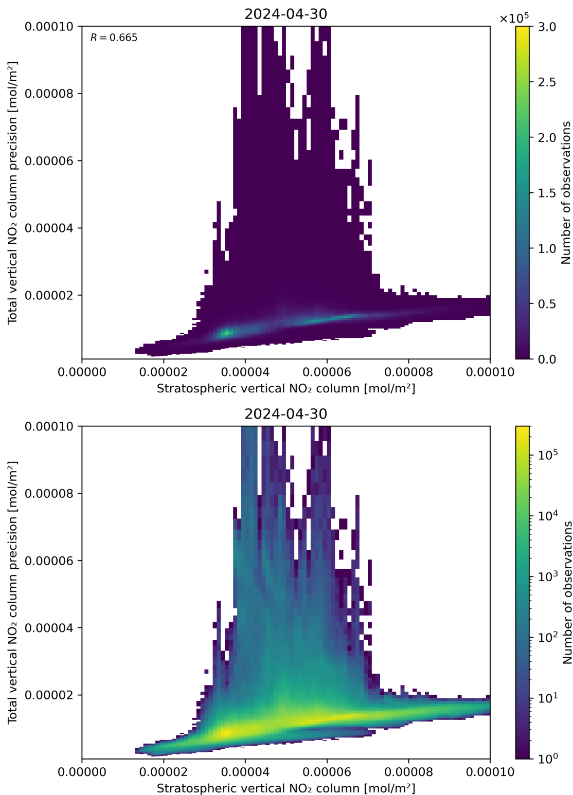
Figure 101: Scatter density plot of “Stratospheric vertical NO 2 column” against “Total vertical NO 2 column precision” for 2024-04-29 to 2024-05-01.
