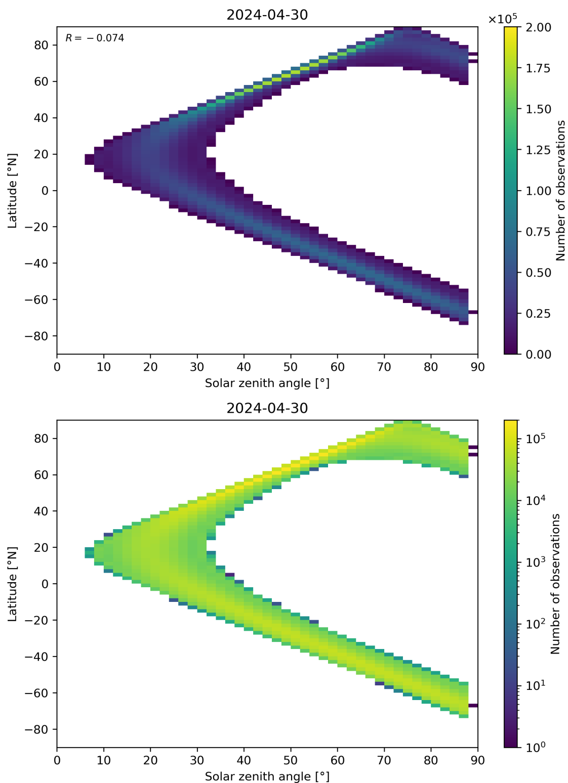
Figure 149: Scatter density plot of “Solar zenith angle” against “Latitude” for 2024-04-29 to 2024-05-01.
