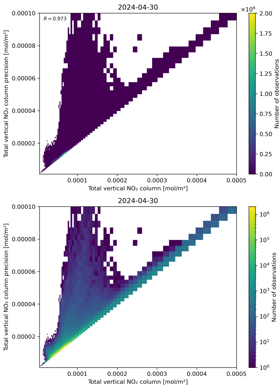
Figure 114: Scatter density plot of “Total vertical NO 2 column” against “Total vertical NO 2 column precision” for 2024-04-29 to 2024-05-01.
