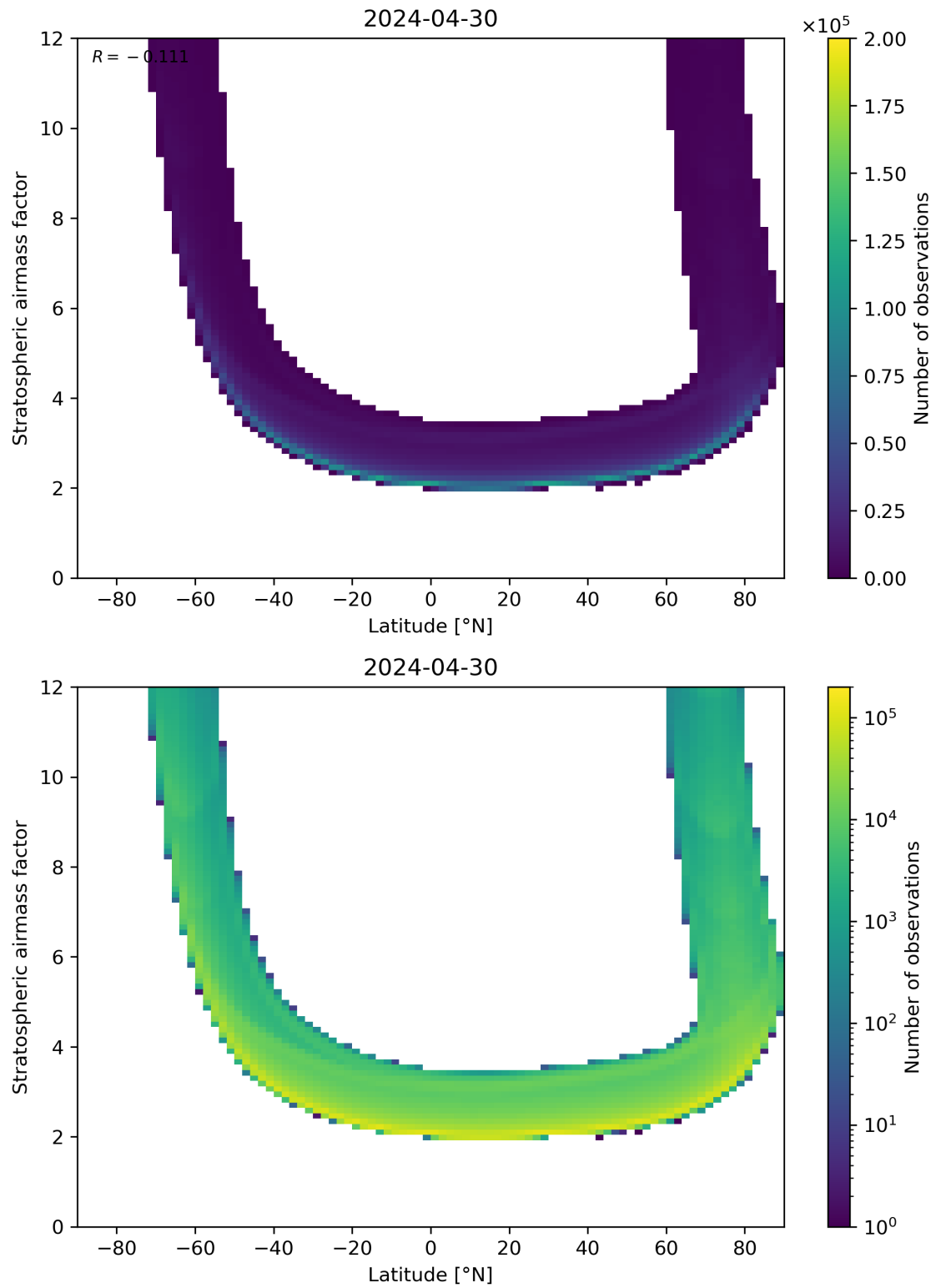
Figure 83: Scatter density plot of “Latitude” against “Stratospheric air mass factor” for 2024-04-29 to 2024-05-01.
