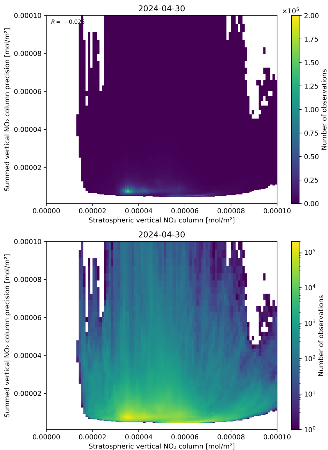
Figure 99: Scatter density plot of “Stratospheric vertical NO 2 column” against “Summed vertical NO 2 column precision” for 2024-04-29 to 2024-05-01.
