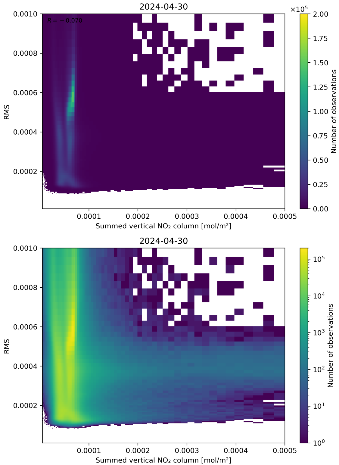
Figure 109: Scatter density plot of “Summed vertical NO 2 column” against “RMS” for 2024-04-29 to 2024-05-01.
