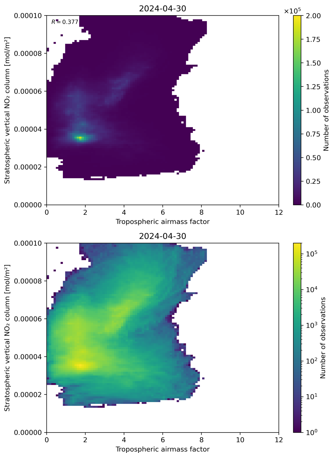
Figure 74: Scatter density plot of “Tropospheric air mass factor” against “Stratospheric vertical NO 2 column” for 2024-04-29 to 2024-05-01.
