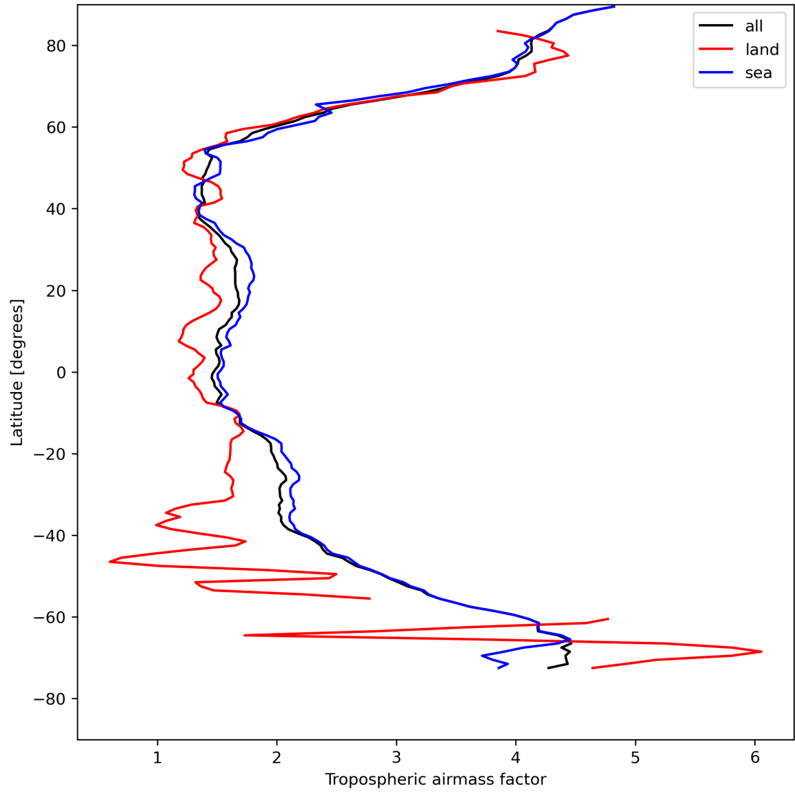
Figure 14: Zonal average of “Tropospheric airmass factor” for 2024-04-29 to 2024-05-01.
