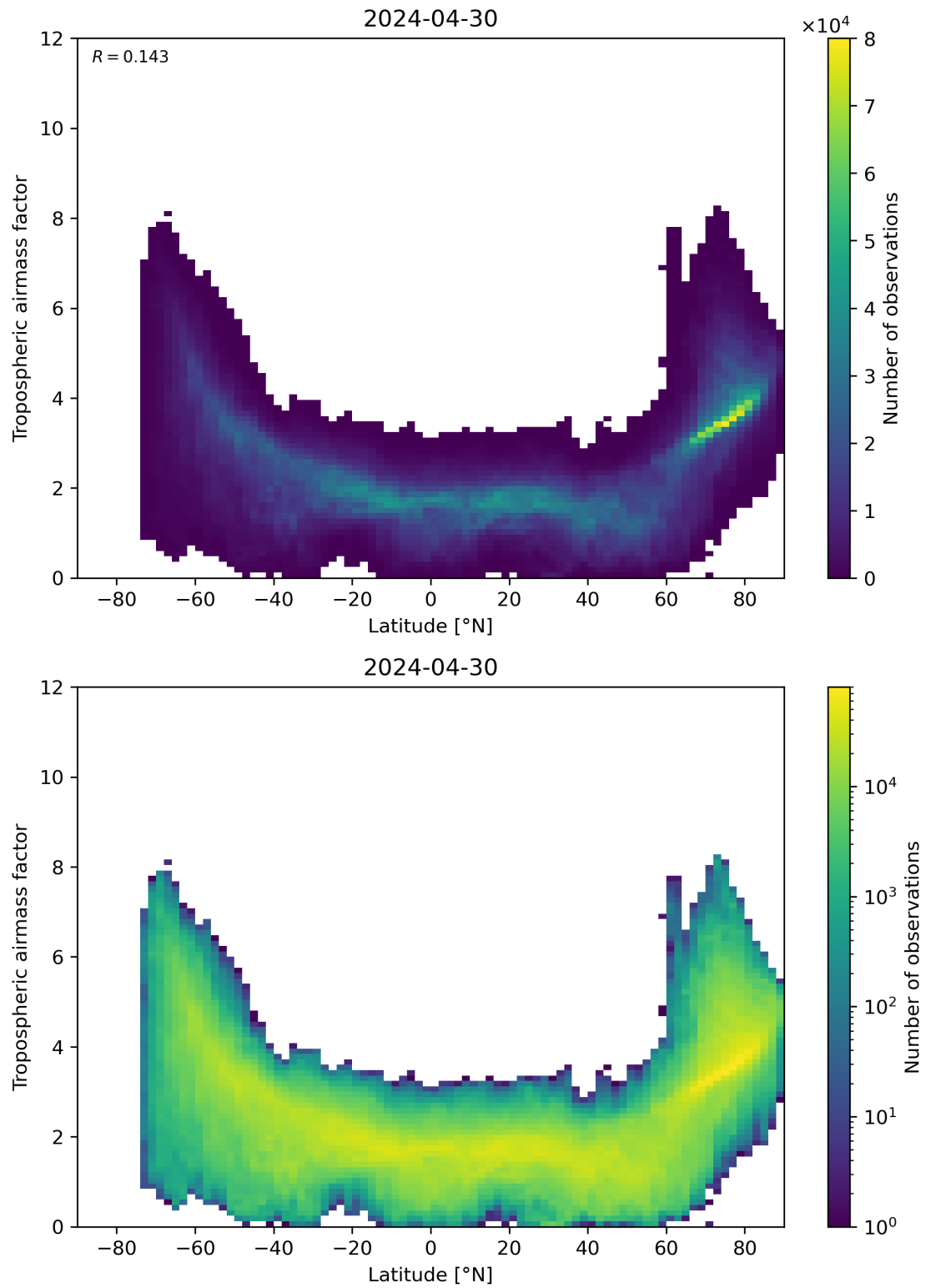
Figure 85: Scatter density plot of “Latitude” against “Tropospheric air mass factor” for 2024-04-29 to 2024-05-01.
