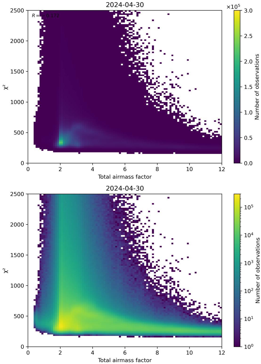
Figure 63: Scatter density plot of “Total airmass factor” against “ \chi^2 ” for 2024-04-29 to 2024-05-01.
