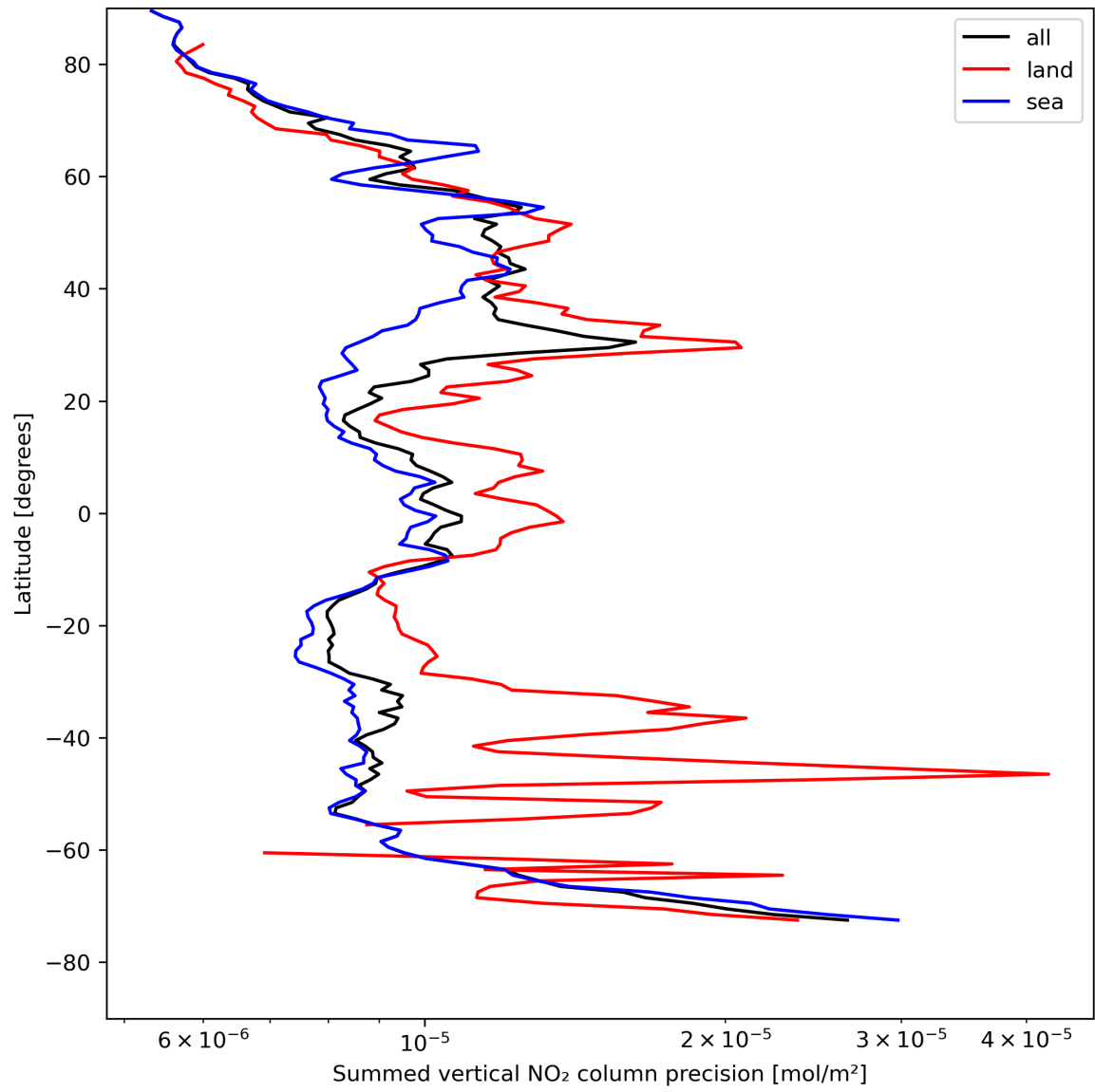
Figure 24: Zonal average of “Summed vertical NO 2 column precision” for 2024-04-29 to 2024-05-01.
