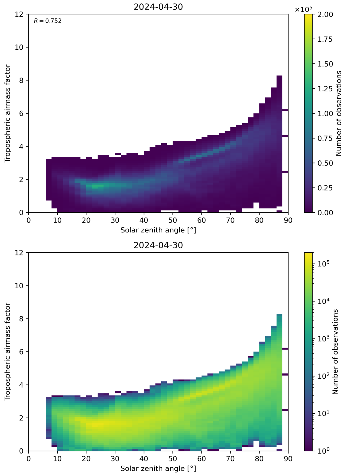
Figure 147: Scatter density plot of “Solar zenith angle” against “Tropospheric airmass factor” for 2024-04-29 to 2024-05-01.
