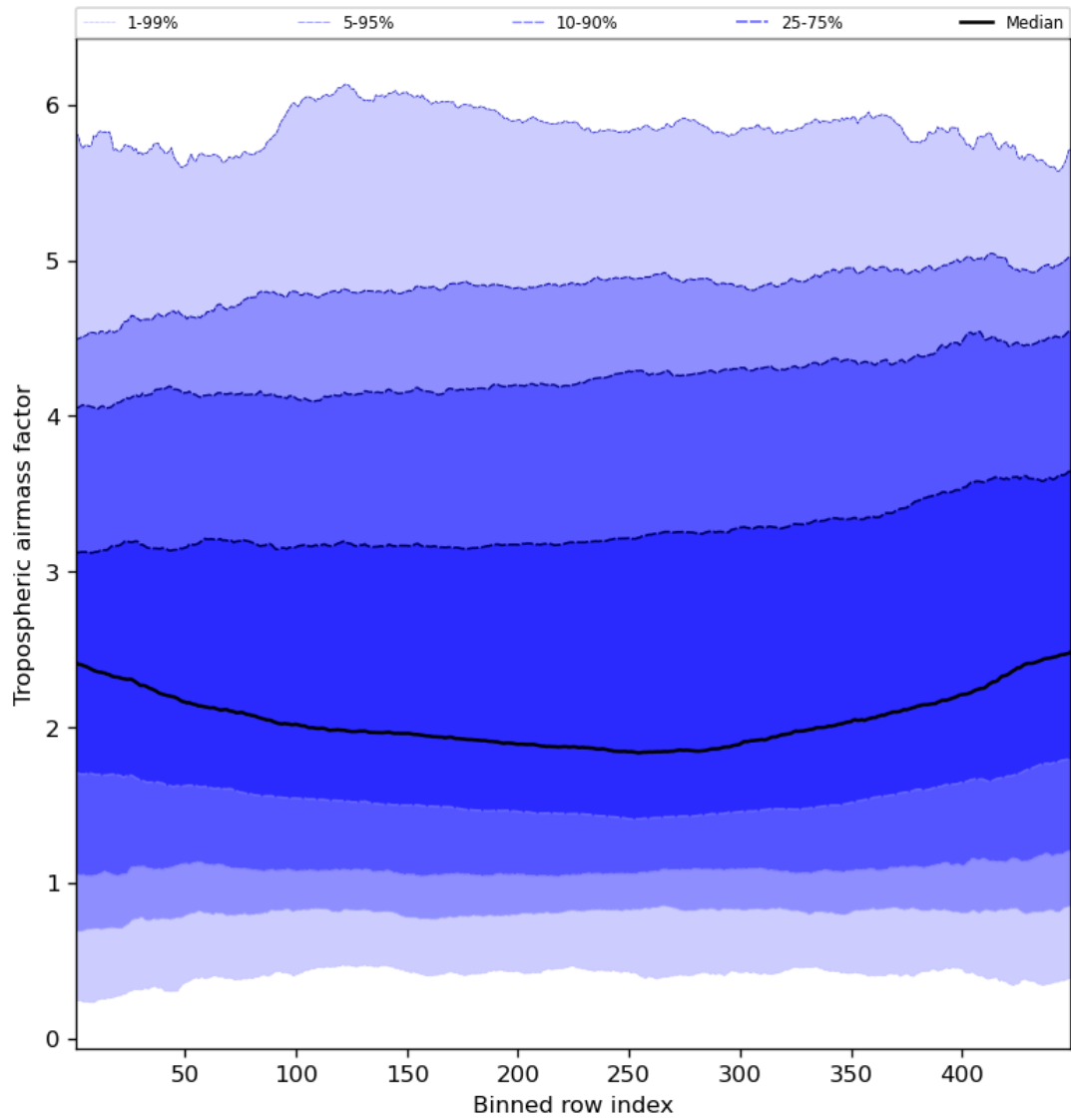
Figure 48: Along track statistics of “Tropospheric airmass factor” for 2024-04-29 to 2024-05-01
