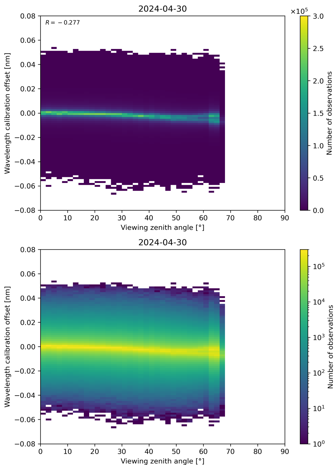
Figure 173: Scatter density plot of “Viewing zenith angle” against “Wavelength calibration offset” for 2024-04-29 to 2024-05-01.
