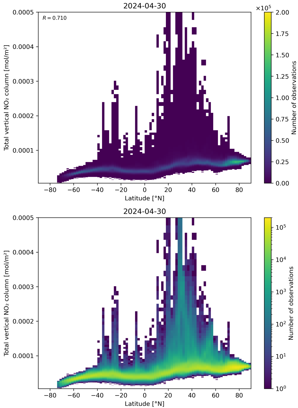
Figure 90: Scatter density plot of “Latitude” against “Total vertical NO 2 column” for 2024-04-29 to 2024-05-01.
