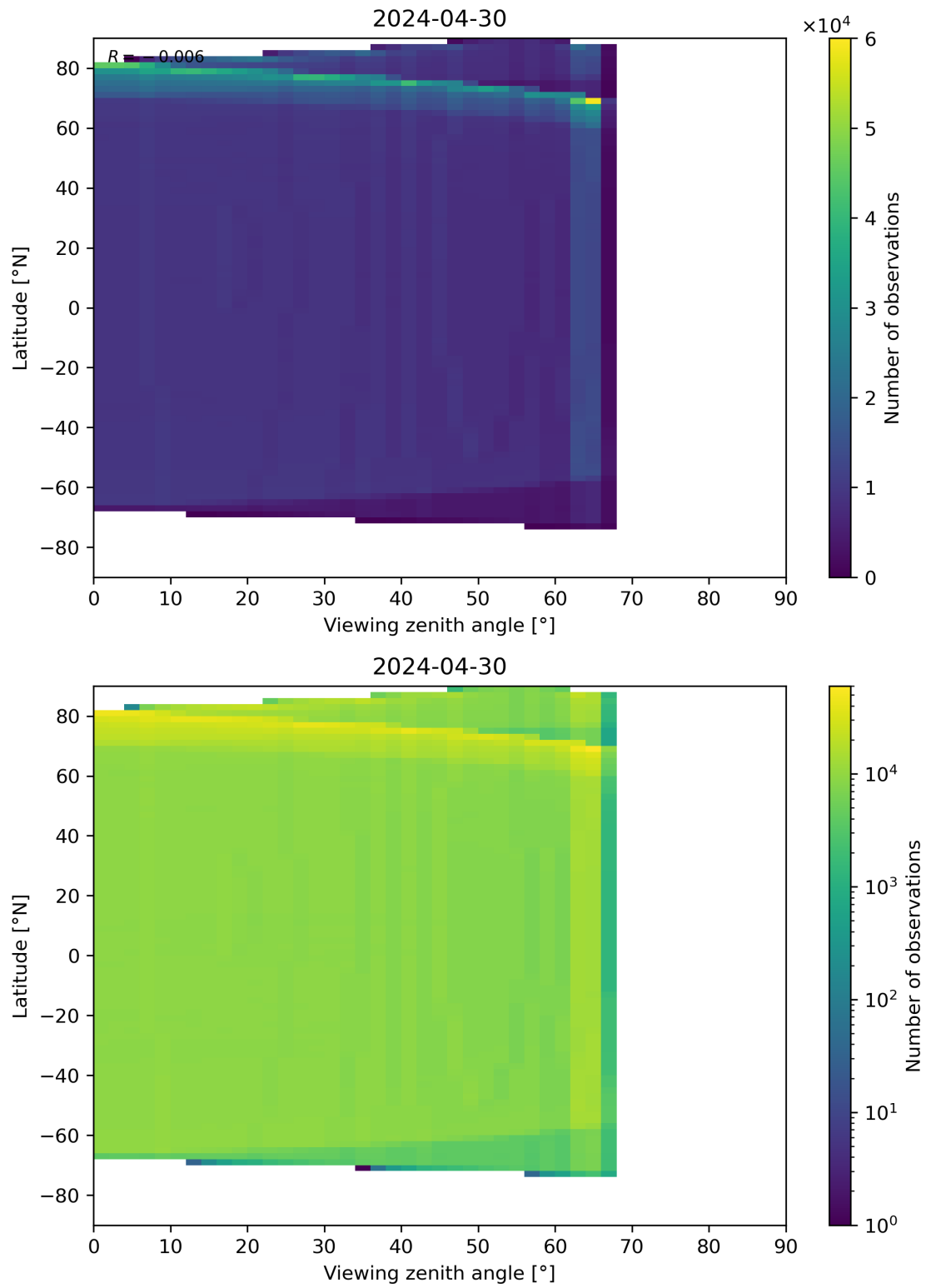
Figure 163: Scatter density plot of “Viewing zenith angle” against “Latitude” for 2024-04-29 to 2024-05-01.
