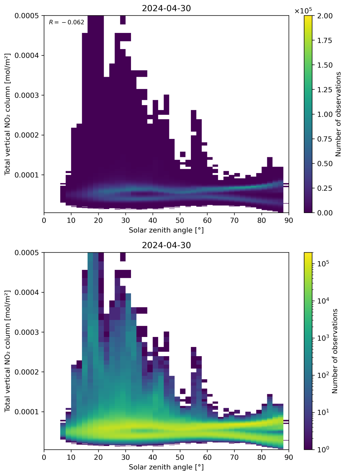
Figure 153: Scatter density plot of “Solar zenith angle” against “Total vertical NO 2 column” for 2024-04-29 to 2024-05-01.
