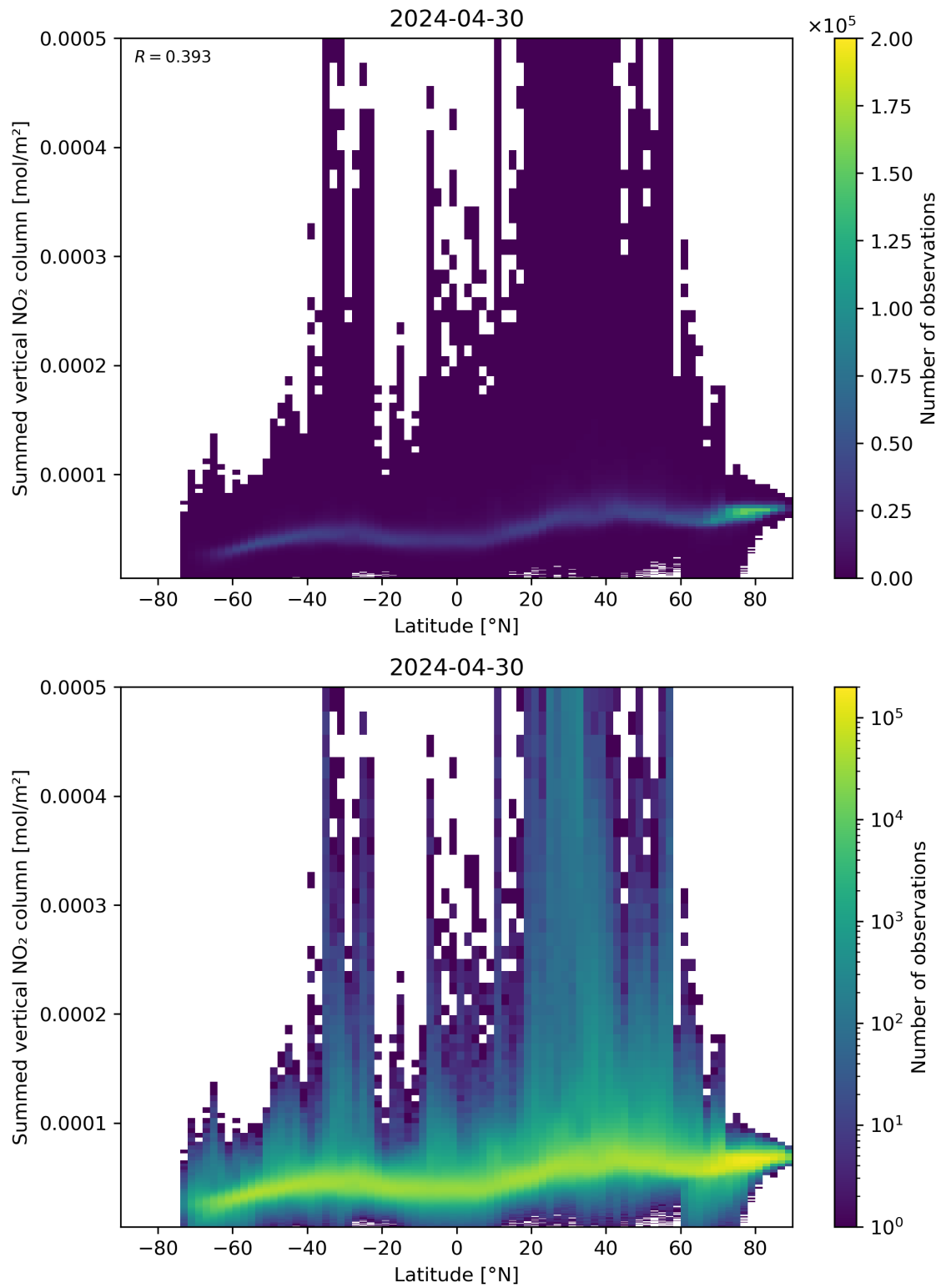
Figure 88: Scatter density plot of “Latitude” against “Summed vertical NO 2 column” for 2024-04-29 to 2024-05-01.
