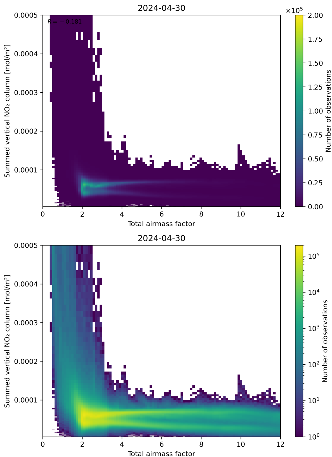
Figure 65: Scatter density plot of “Total air mass factor” against “Summed vertical NO 2 column” for 2024-04-29 to 2024-05-01.
