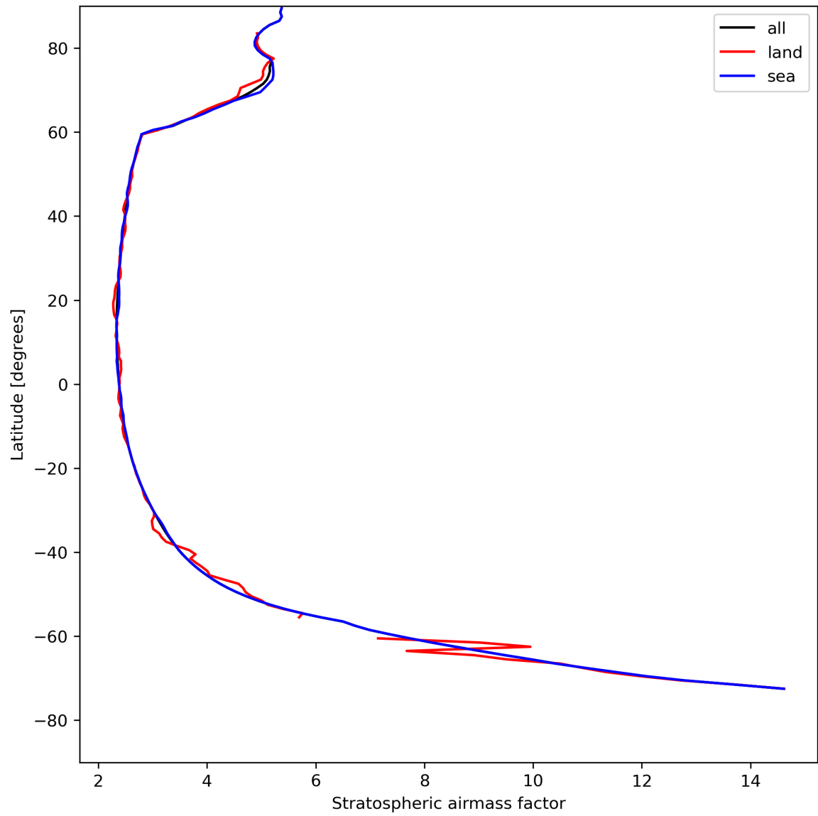
Figure 27: Zonal average of “Stratospheric airmass factor” for 2024-04-29 to 2024-05-01.
