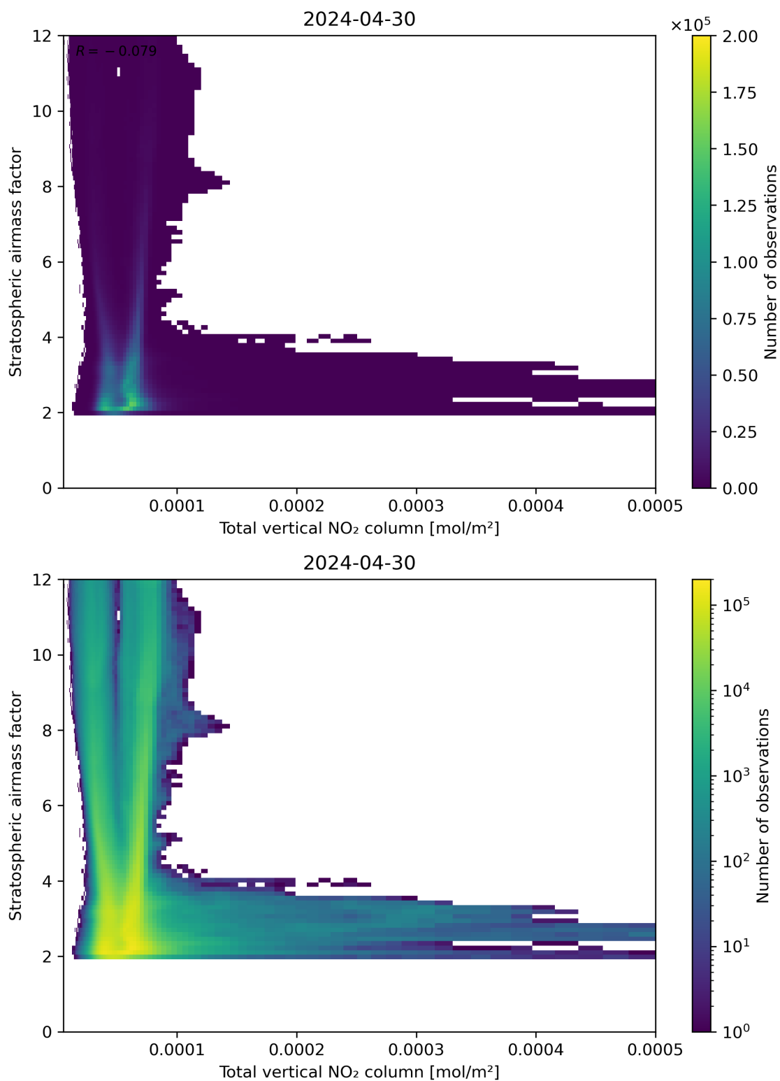
Figure 110: Scatter density plot of “Total vertical NO 2 column” against “Stratospheric airmass factor” for 2024-04-29 to 2024-05-01.
