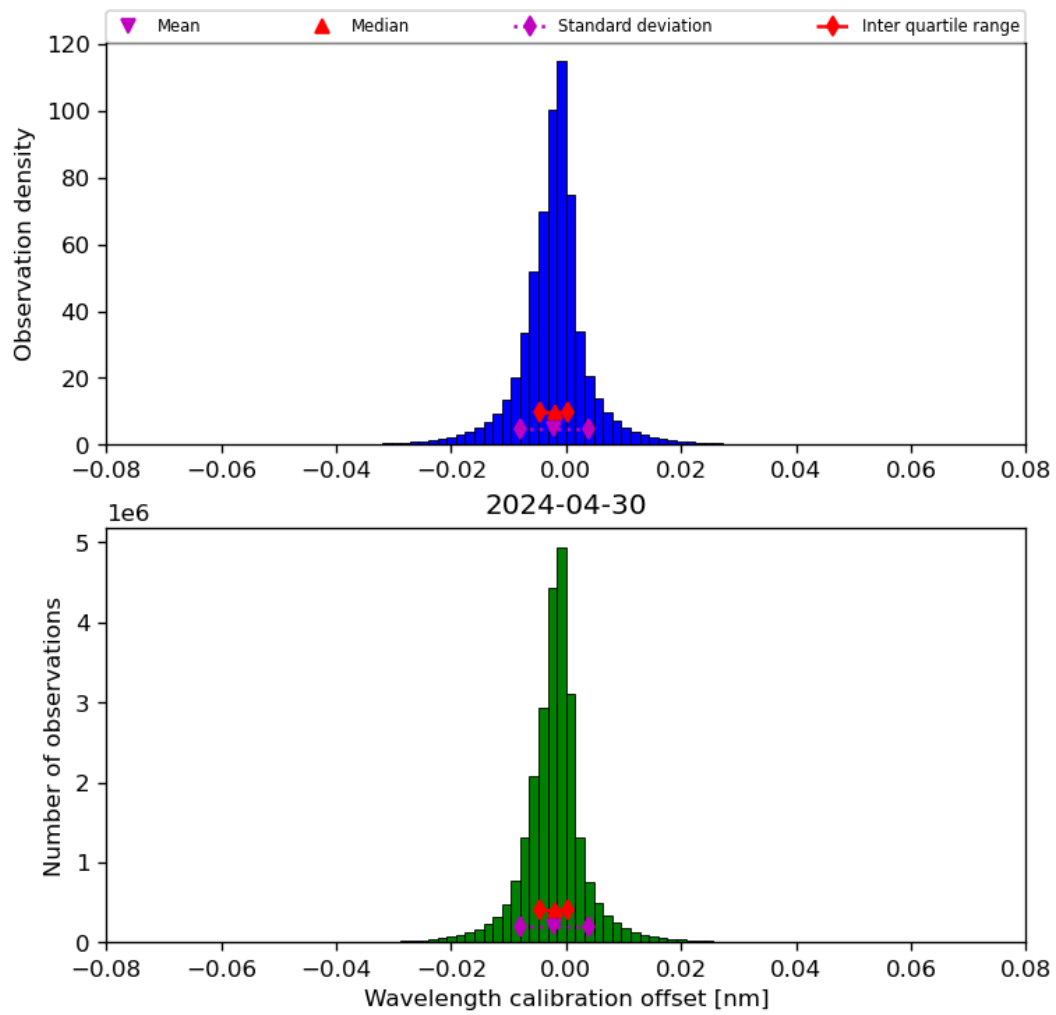
Figure 35: Histogram of “Wavelength calibration offset” for 2024-04-29 to 2024-05-01
