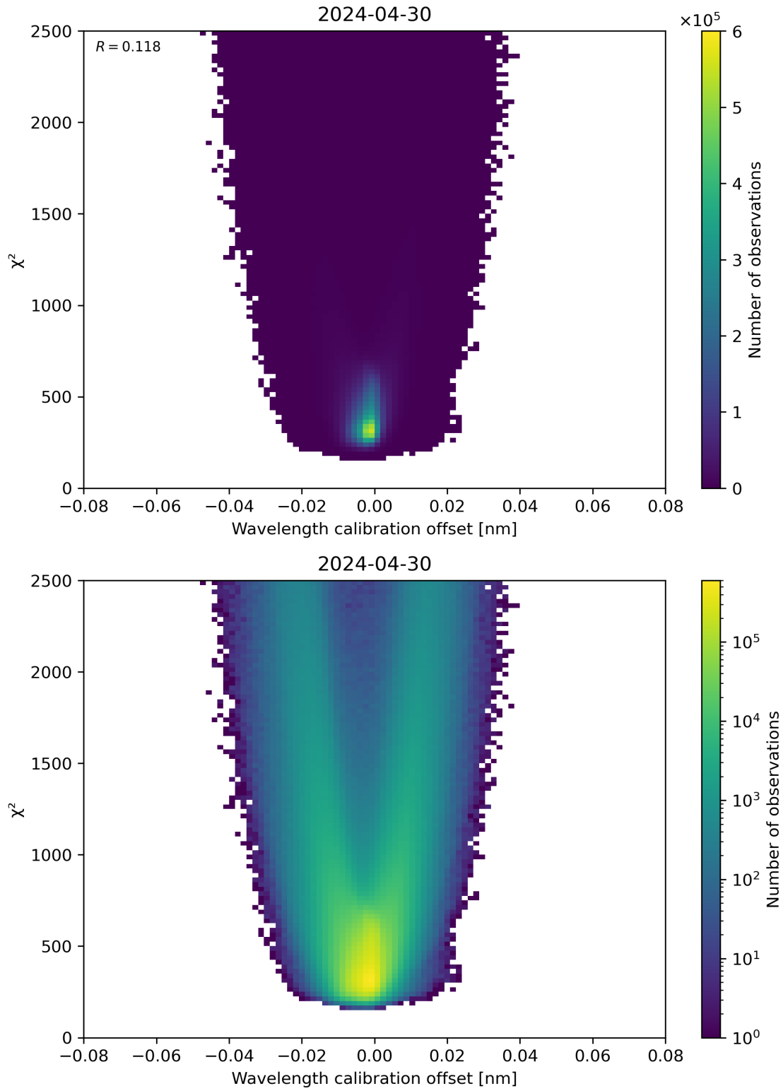
Figure 175: Scatter density plot of “Wavelength calibration offset” against “ \chi^2 ” for 2024-04-29 to 2024-05-01.
