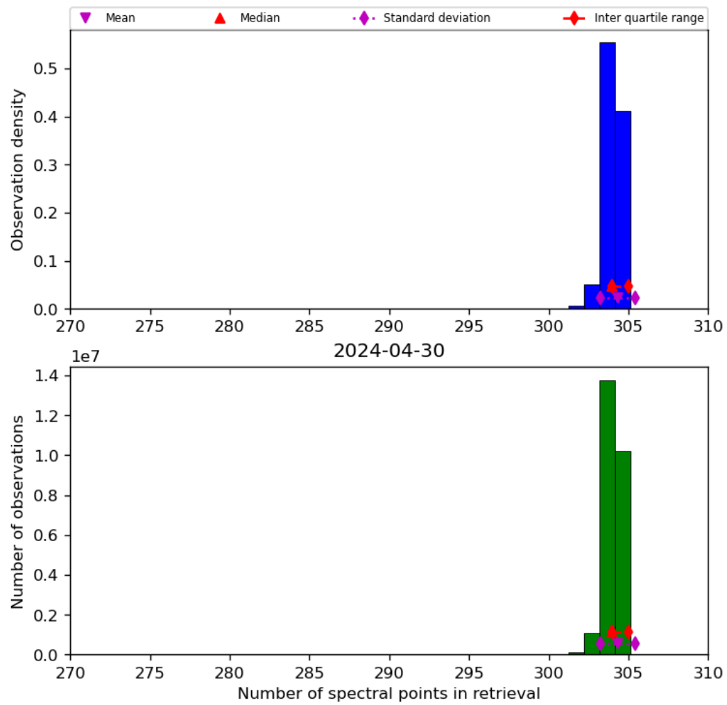
Figure 33: Histogram of “Number of spectral points in retrieval” for 2024-04-29 to 2024-05-01
