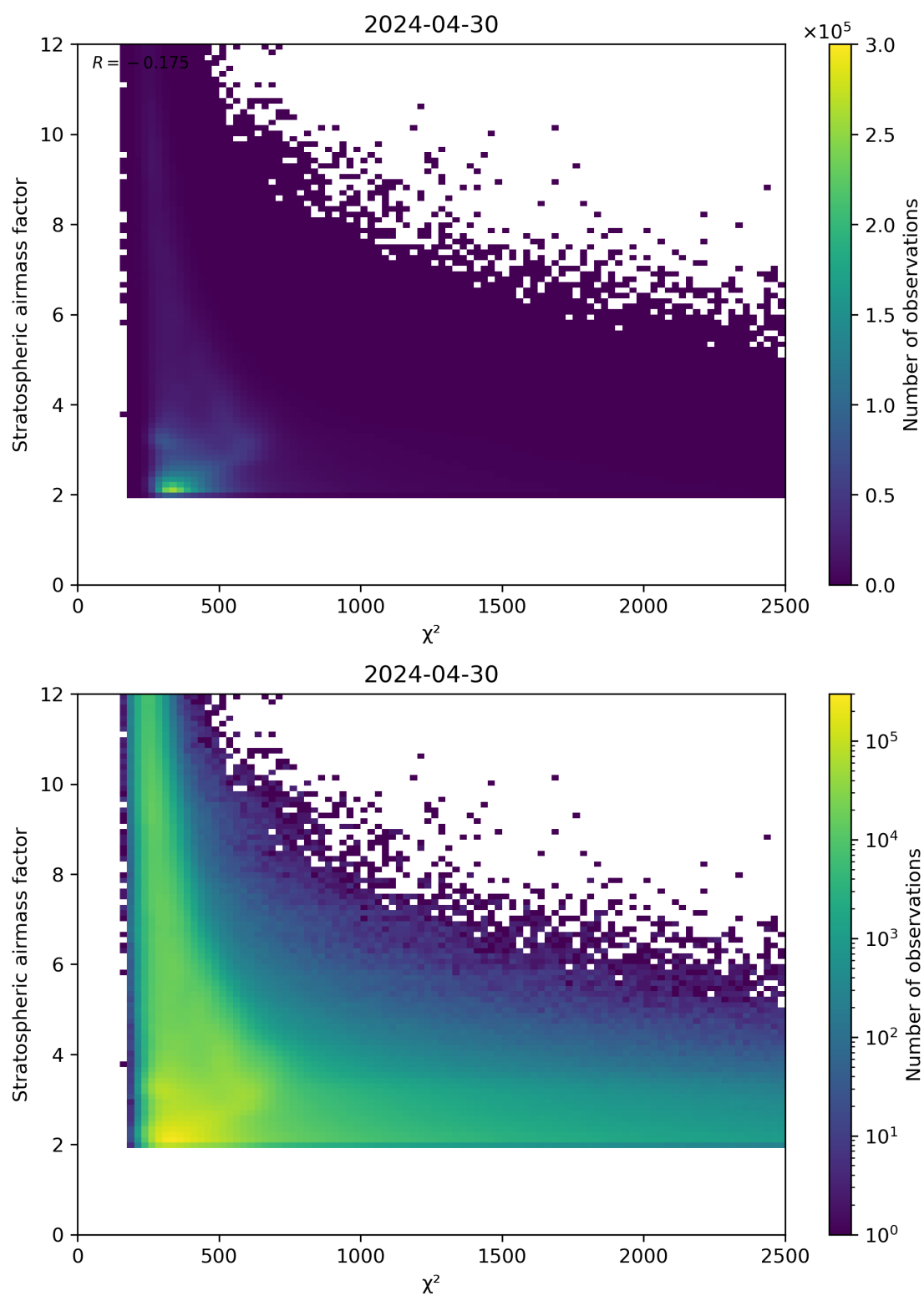
Figure 81: Scatter density plot of “ \chi^2 ” against “Stratospheric airmass factor” for 2024-04-29 to 2024-05-01.
