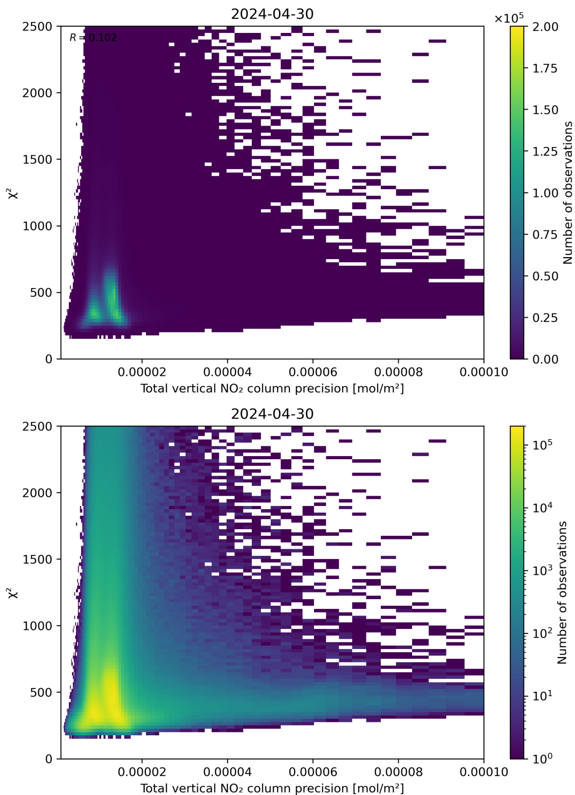
Figure 116: Scatter density plot of “Total vertical NO 2 column precision” against “ \chi^2 ” for 2024-04-29 to 2024-05-01.
