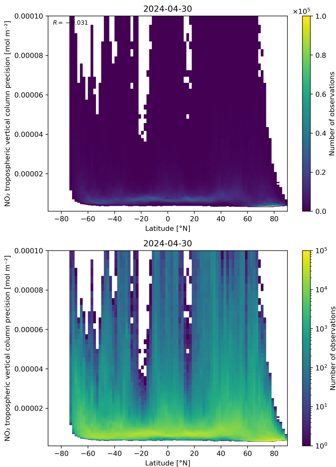
Figure 93: Scatter density plot of “Latitude” against “NO 2 tropospheric vertical column precision” for 2024-04-29 to 2024-05-01.
