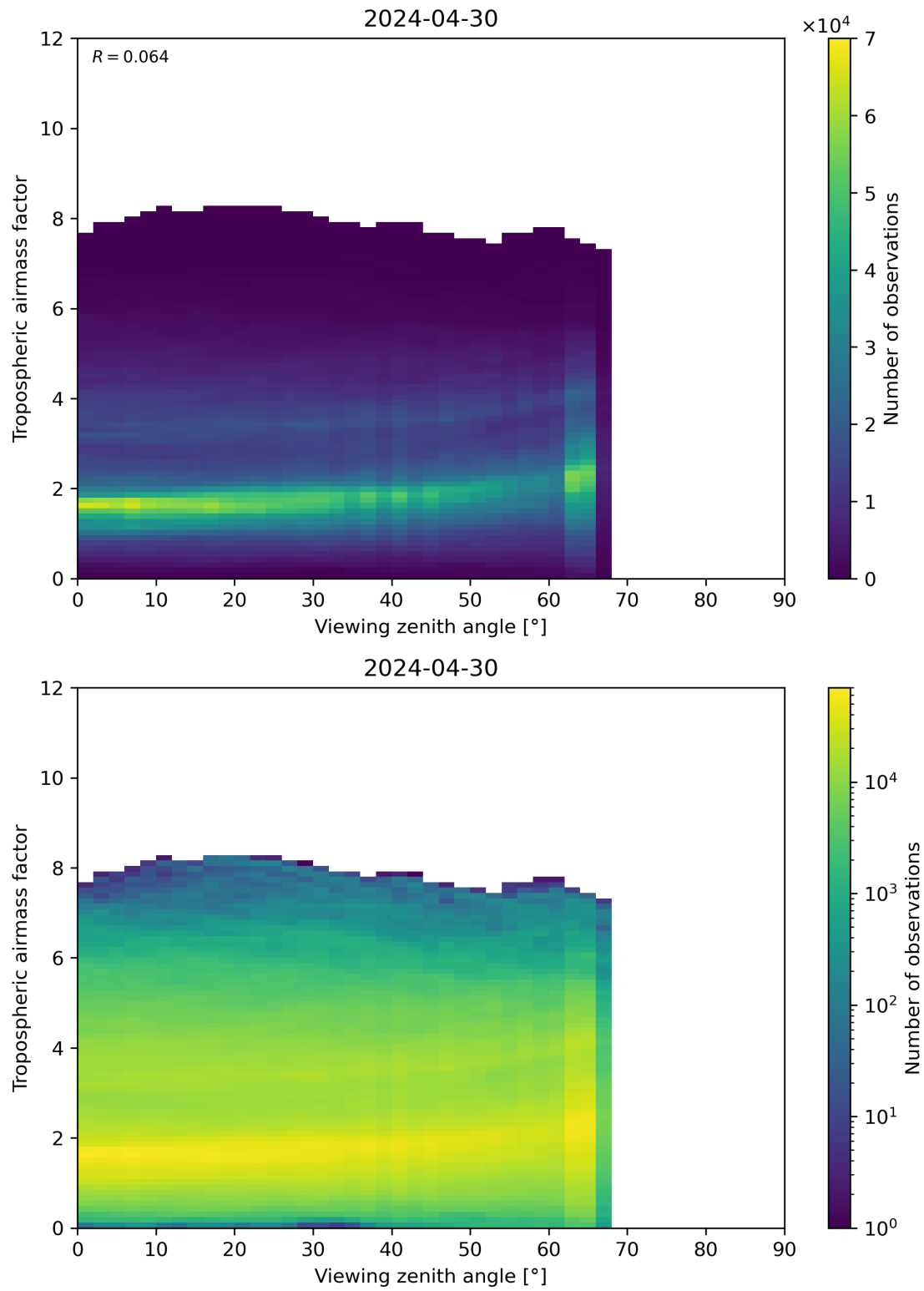
Figure 161: Scatter density plot of “Viewing zenith angle” against “Tropospheric airmass factor” for 2024-04-29 to 2024-05-01.
