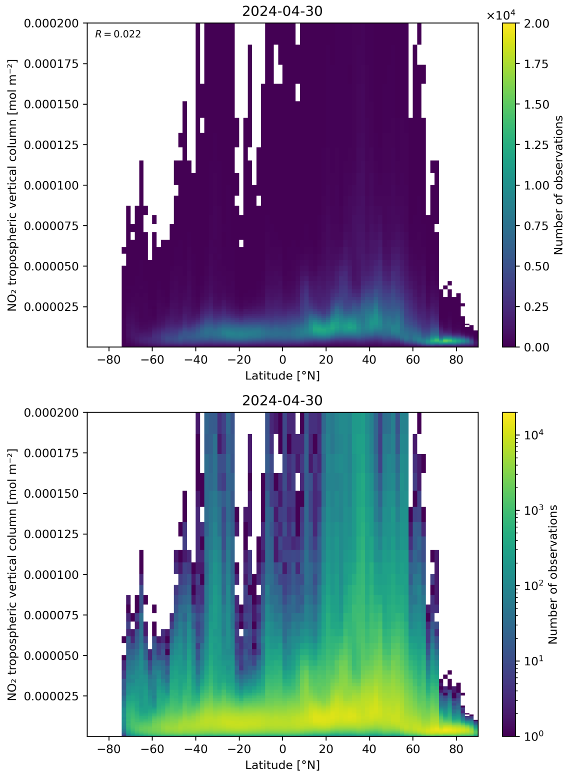
Figure 92: Scatter density plot of “Latitude” against “NO 2 tropospheric vertical column” for 2024-04-29 to 2024-05-01.
