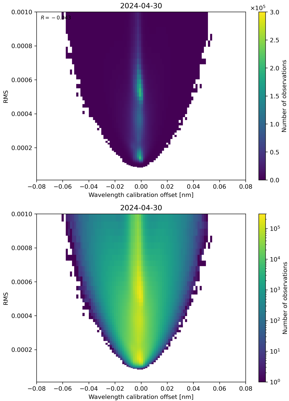
Figure 181: Scatter density plot of “Wavelength calibration offset” against “RMS” for 2024-04-29 to 2024-05-01.
