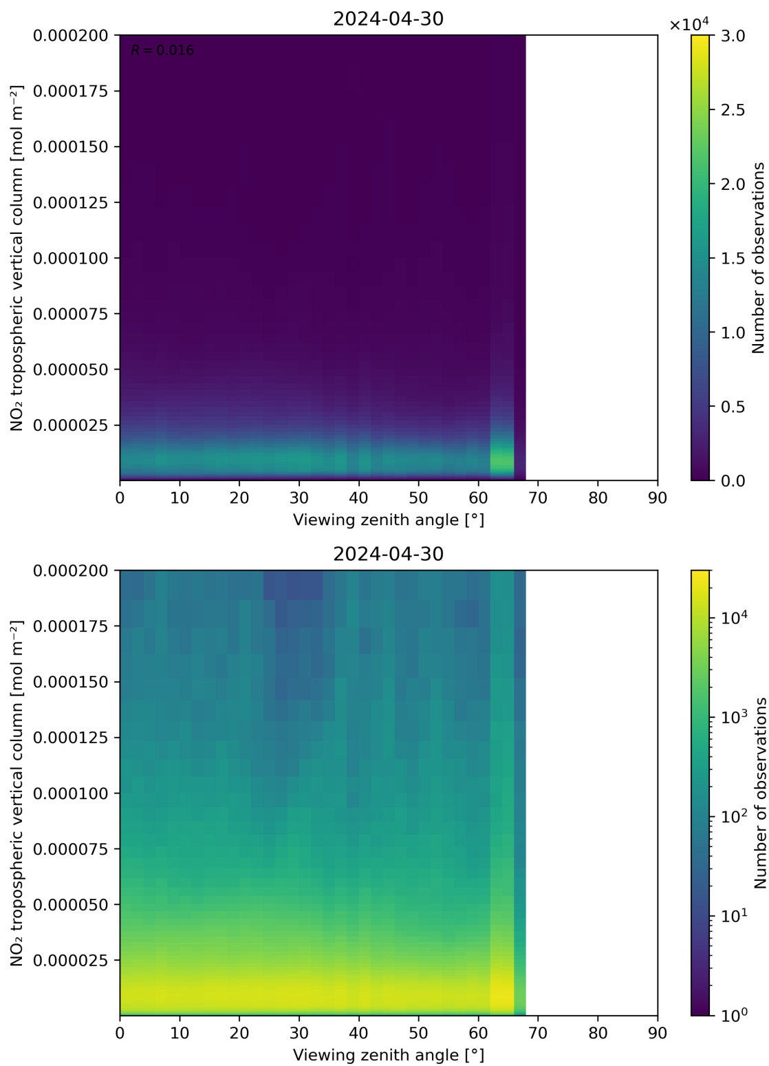
Figure 169: Scatter density plot of “Viewing zenith angle” against “NO 2 tropospheric vertical column” for 2024-04-29 to 2024-05-01.
