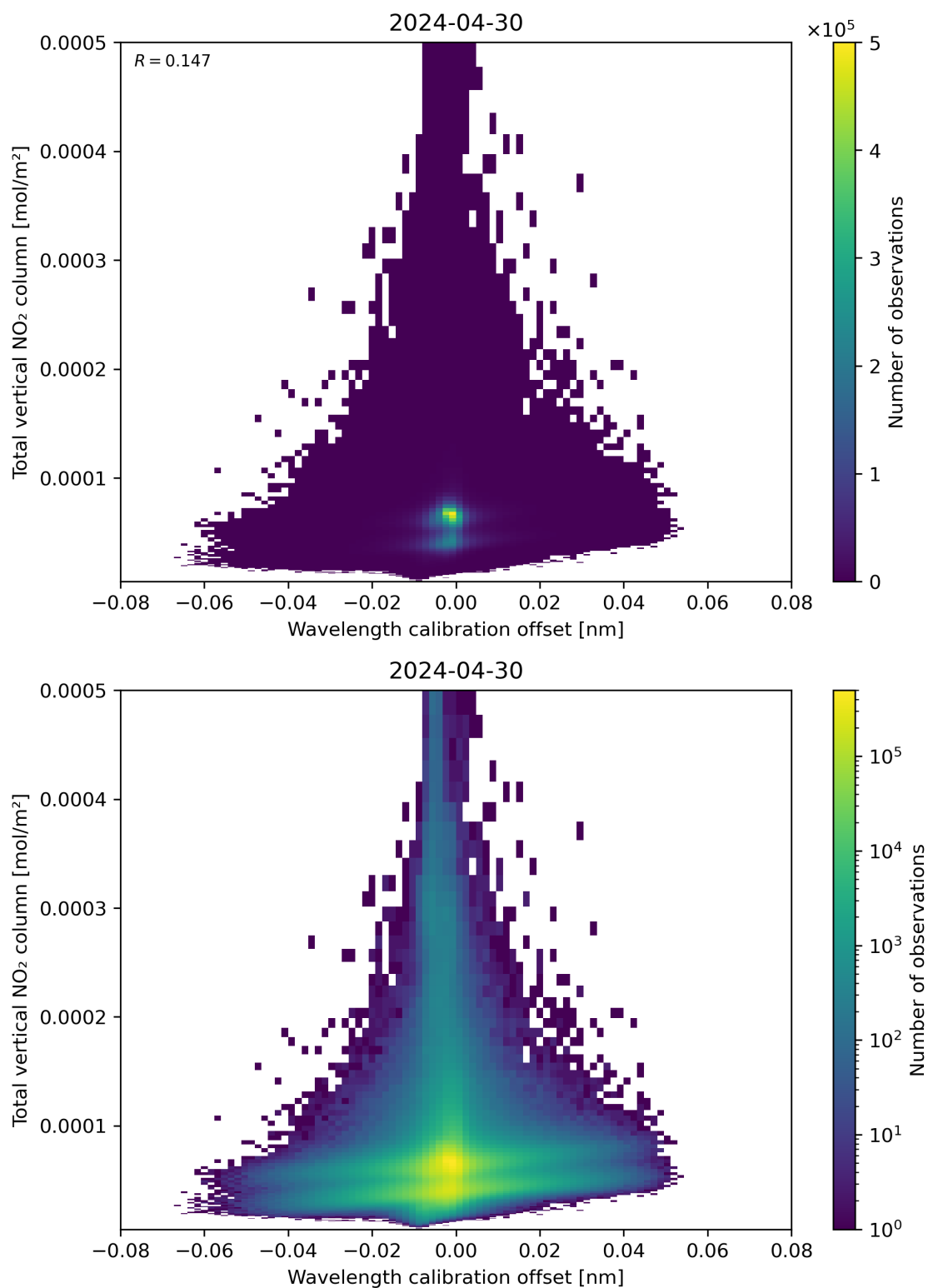
Figure 179: Scatter density plot of “Wavelength calibration offset” against “Total vertical NO 2 column” for 2024-04-29 to 2024-05-01.
