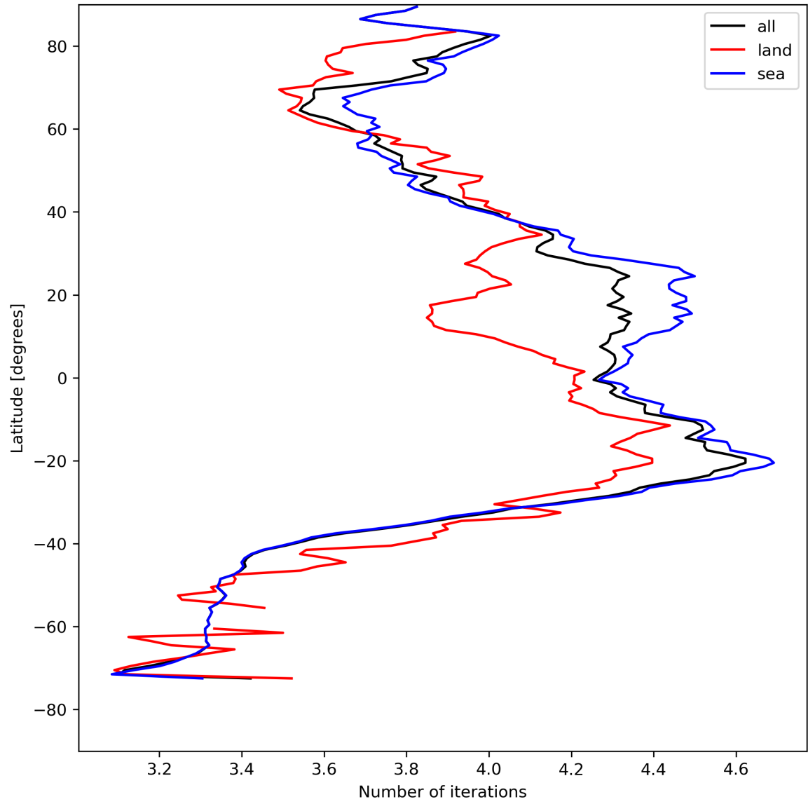
Figure 17: Zonal average of “Number of iterations” for 2024-04-29 to 2024-05-01.
