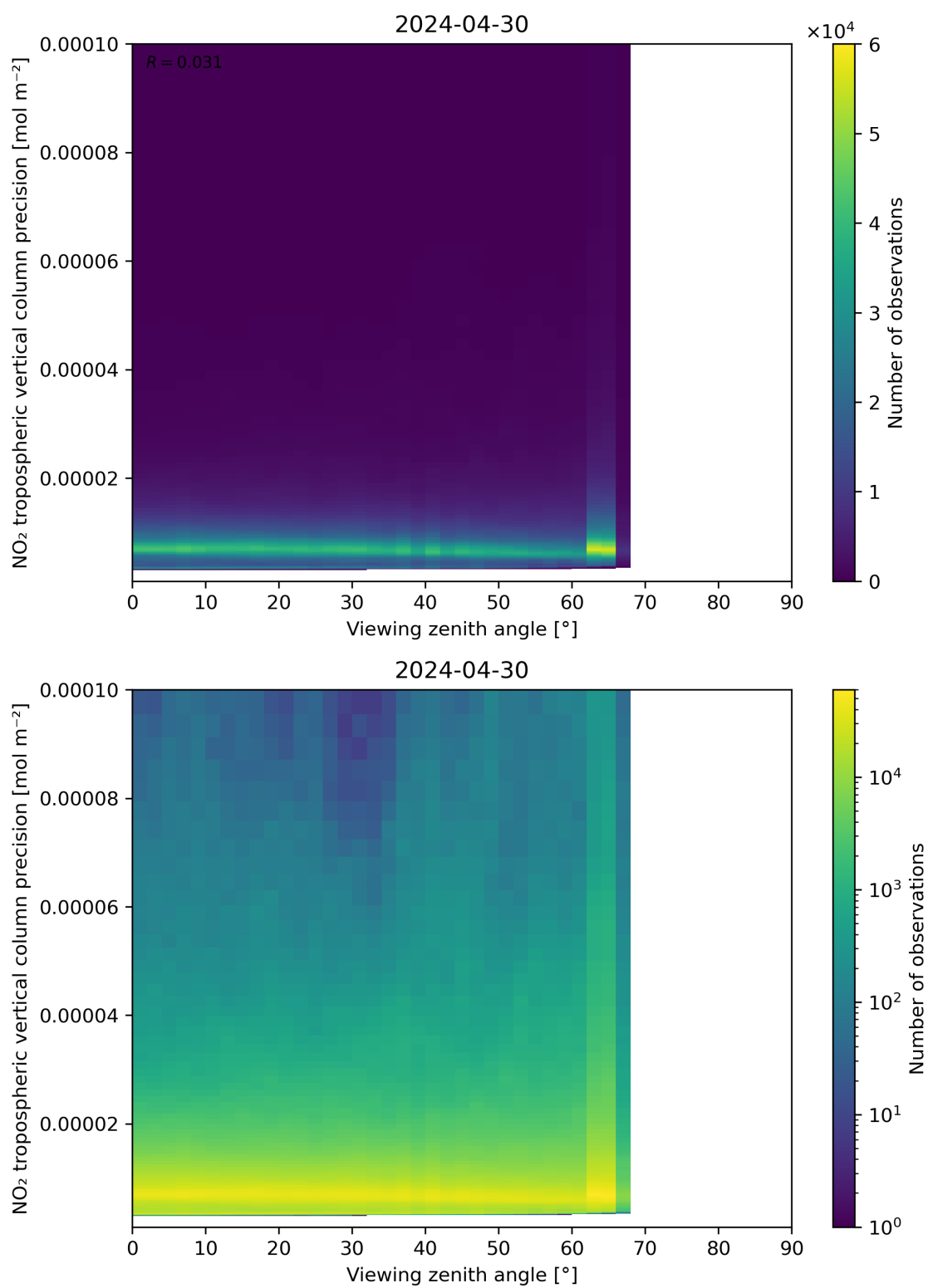
Figure 170: Scatter density plot of “Viewing zenith angle” against “NO 2 tropospheric vertical column precision” for 2024-04-29 to 2024-05-01.
