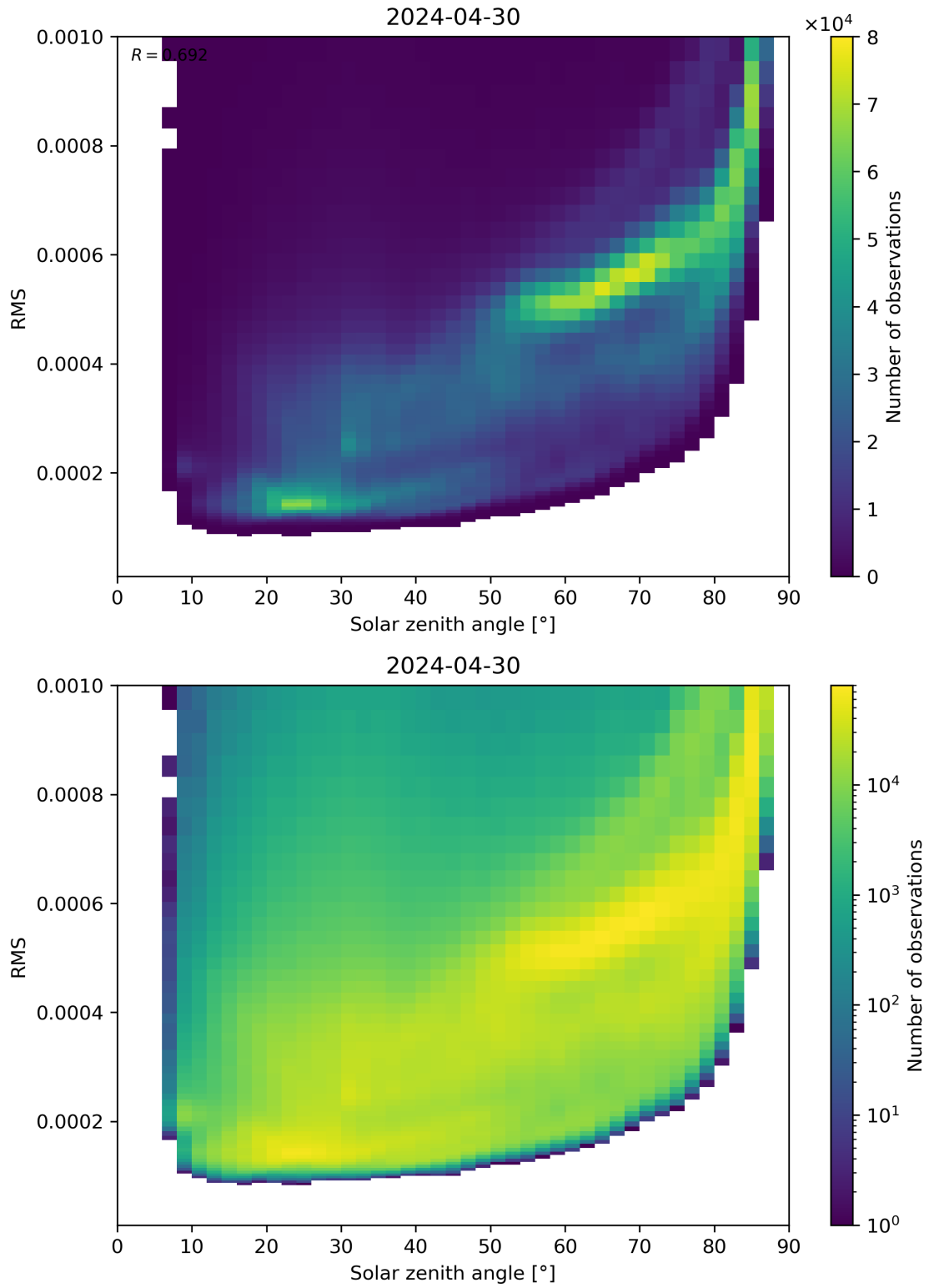
Figure 157: Scatter density plot of “Solar zenith angle” against “RMS” for 2024-04-29 to 2024-05-01.
