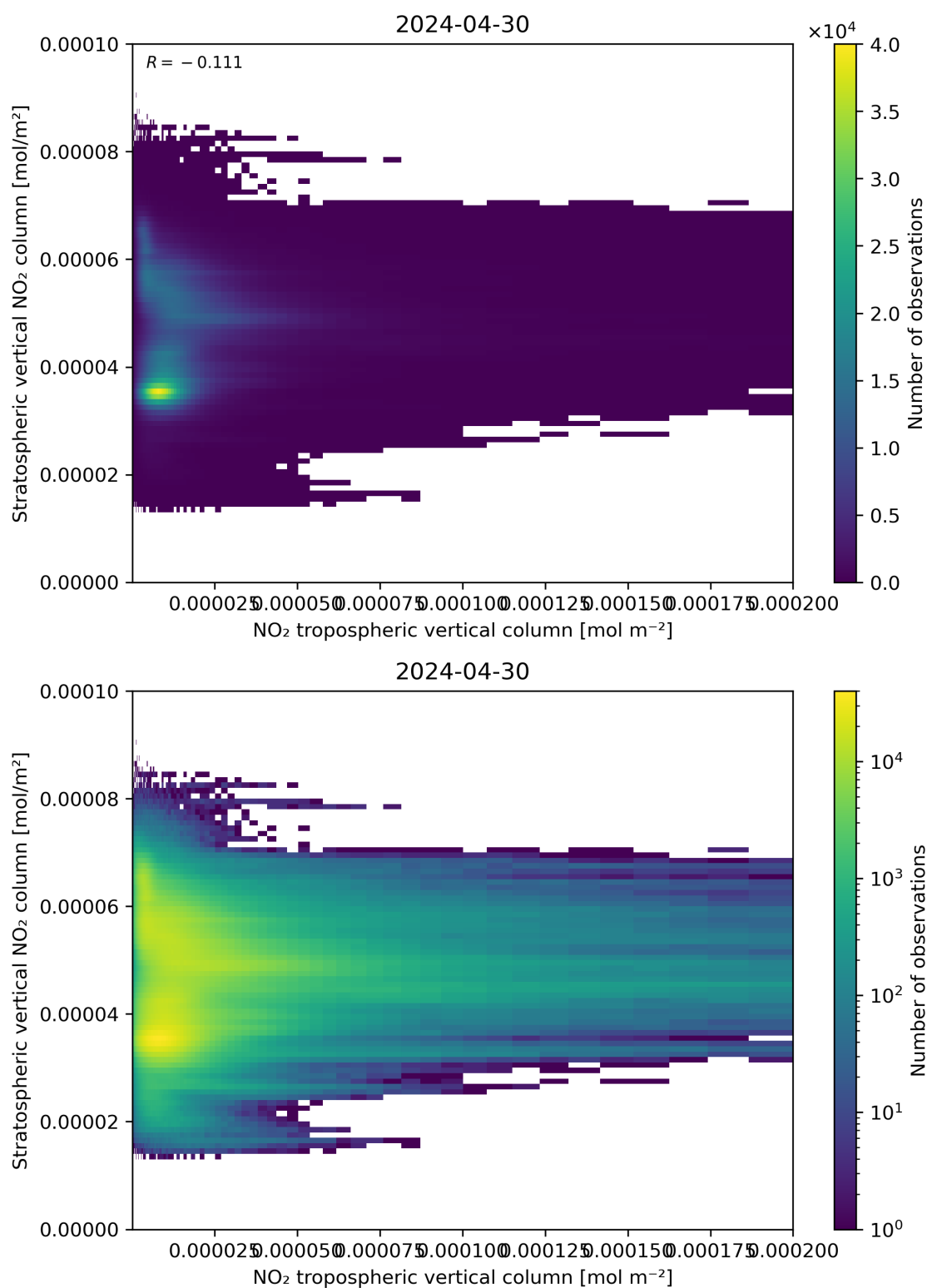
Figure 125: Scatter density plot of “NO 2 tropospheric vertical column” against “Stratospheric vertical NO 2 column” for 2024-04-29 to 2024-05-01.
