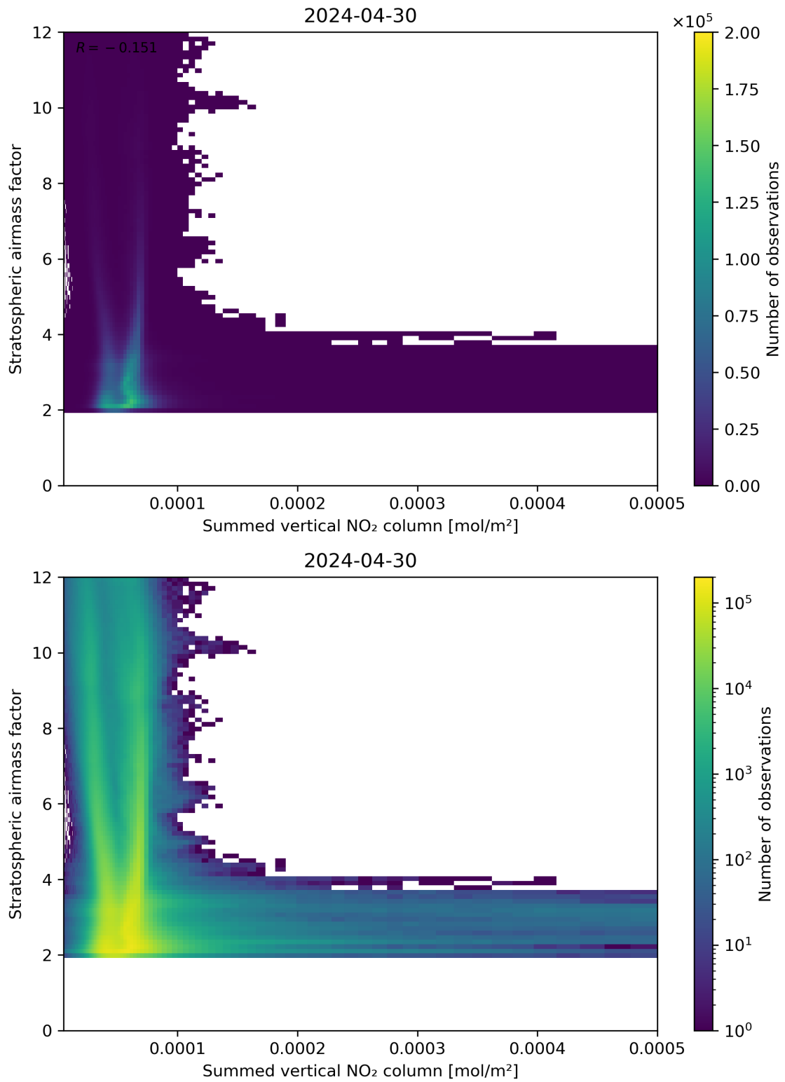
Figure 103: Scatter density plot of “Summed vertical NO 2 column” against “Stratospheric air mass factor” for 2024-04-29 to 2024-05-01.
