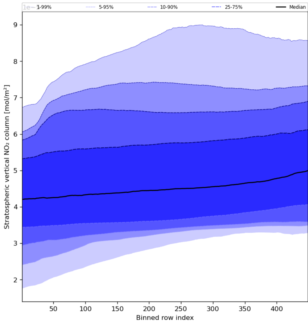
Figure 53: Along track statistics of “Stratospheric vertical NO 2 column” for 2024-04-29 to 2024-05-01
