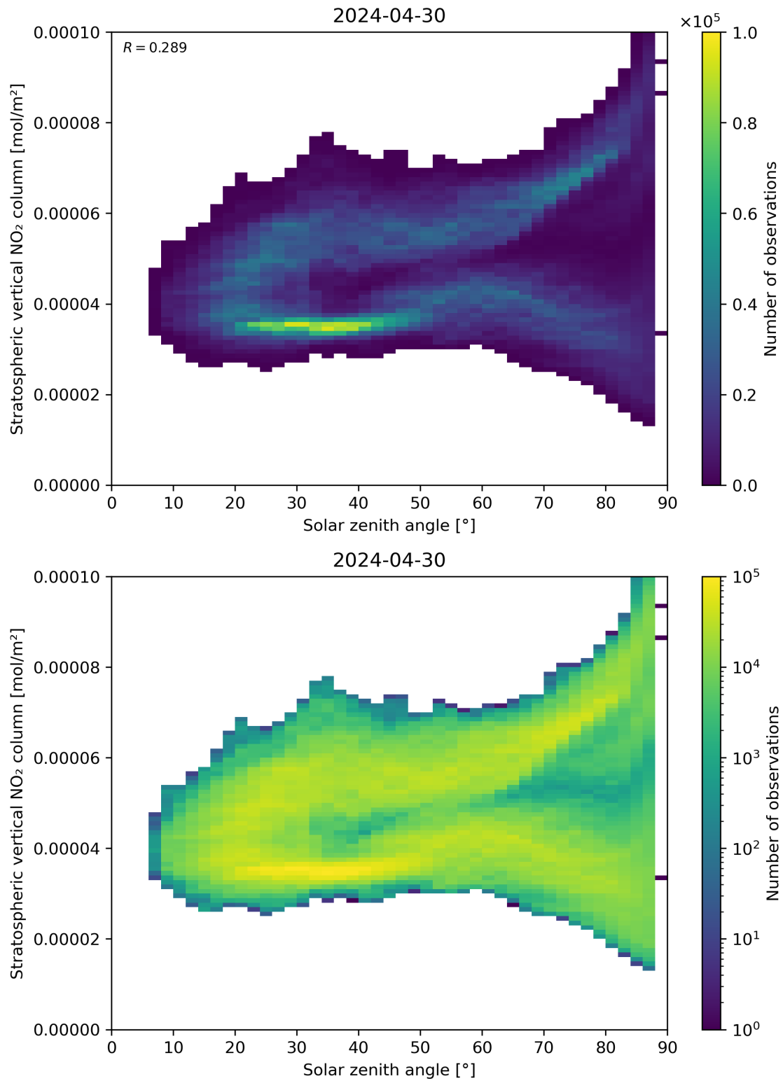
Figure 150: Scatter density plot of “Solar zenith angle” against “Stratospheric vertical NO 2 column” for 2024-04-29 to 2024-05-01.
