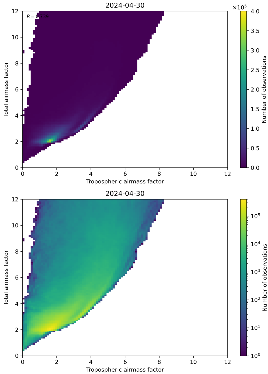
Figure 72: Scatter density plot of “Tropospheric airmass factor” against “Total airmass factor” for 2024-04-29 to 2024-05-01.
