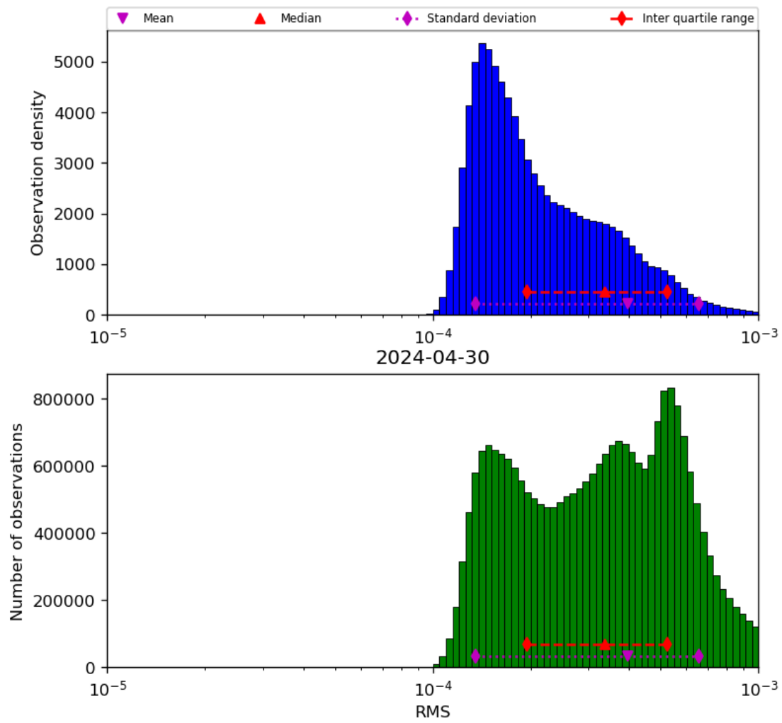
Figure 43: Histogram of “RMS” for 2024-04-29 to 2024-05-01
