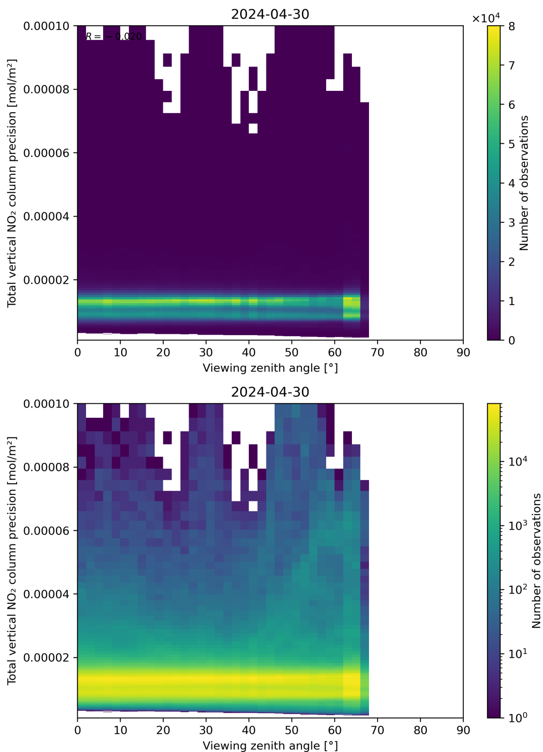
Figure 168: Scatter density plot of “Viewing zenith angle” against “Total vertical NO 2 column precision” for 2024-04-29 to 2024-05-01.
