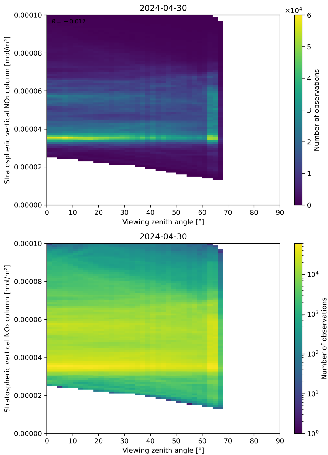
Figure 164: Scatter density plot of “Viewing zenith angle” against “Stratospheric vertical NO 2 column” for 2024-04-29 to 2024-05-01.
