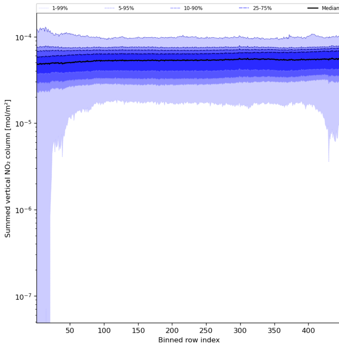
Figure 57: Along track statistics of “Summed vertical NO 2 column” for 2024-04-29 to 2024-05-01
