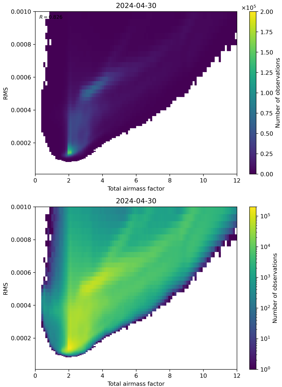
Figure 69: Scatter density plot of “Total airmass factor” against “RMS” for 2024-04-29 to 2024-05-01.
