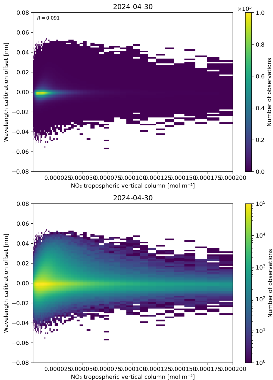
Figure 143: Scatter density plot of “NO 2 tropospheric vertical column” against “Wavelength calibration offset” for 2024-04-29 to 2024-05-01.
