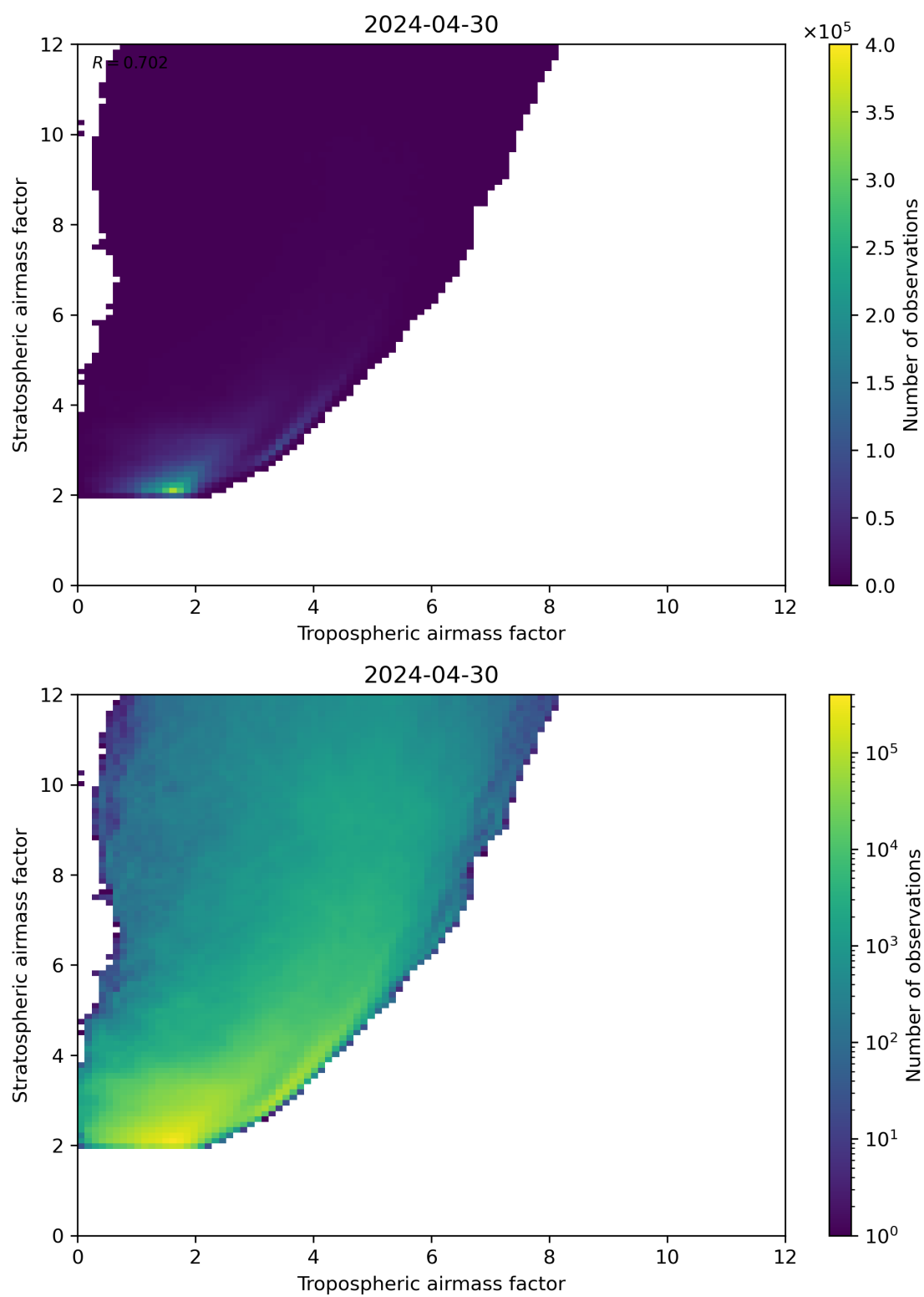
Figure 71: Scatter density plot of “Tropospheric airmass factor” against “Stratospheric airmass factor” for 2024-04-29 to 2024-05-01.
