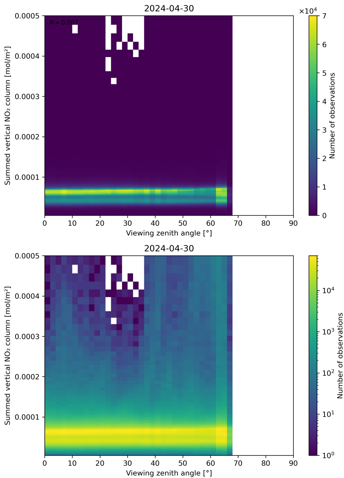
Figure 165: Scatter density plot of “Viewing zenith angle” against “Summed vertical NO 2 column” for 2024-04-29 to 2024-05-01.
