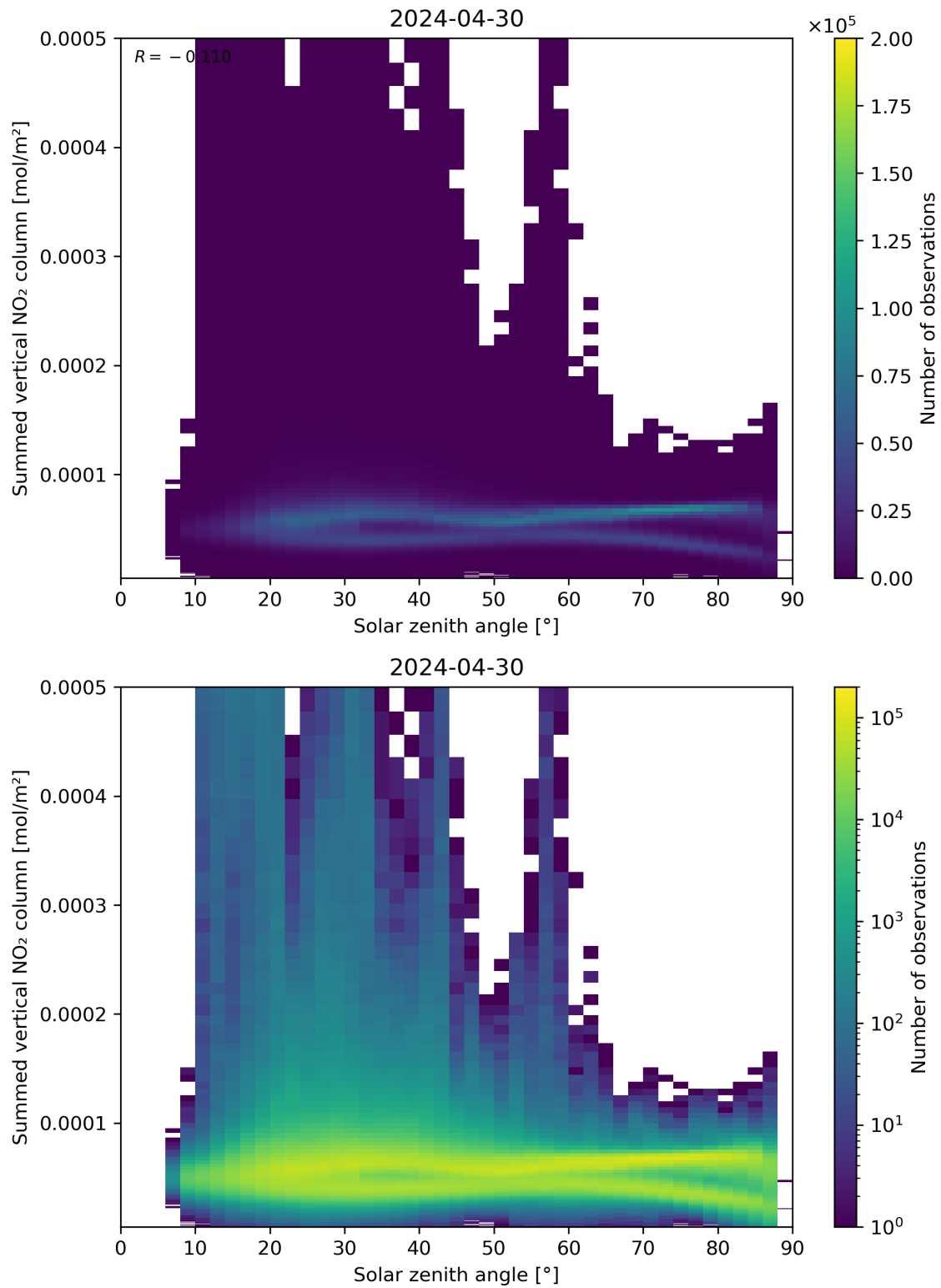
Figure 151: Scatter density plot of “Solar zenith angle” against “Summed vertical NO 2 column” for 2024-04-29 to 2024-05-01.
