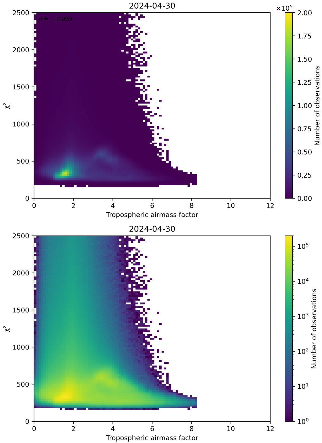
Figure 73: Scatter density plot of “Tropospheric airmass factor” against “ \chi^2 ” for 2024-04-29 to 2024-05-01.
