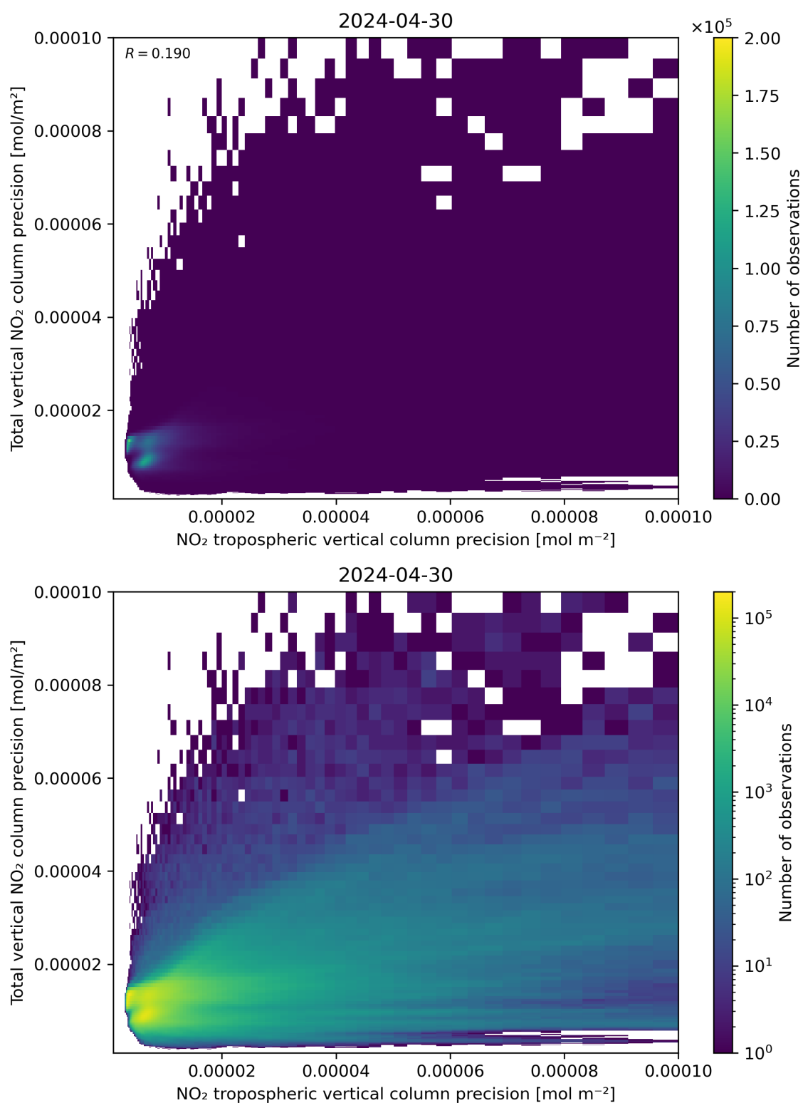
Figure 139: Scatter density plot of “NO 2 tropospheric vertical column precision” against “Total vertical NO 2 column precision” for 2024-04-29 to 2024-05-01.
