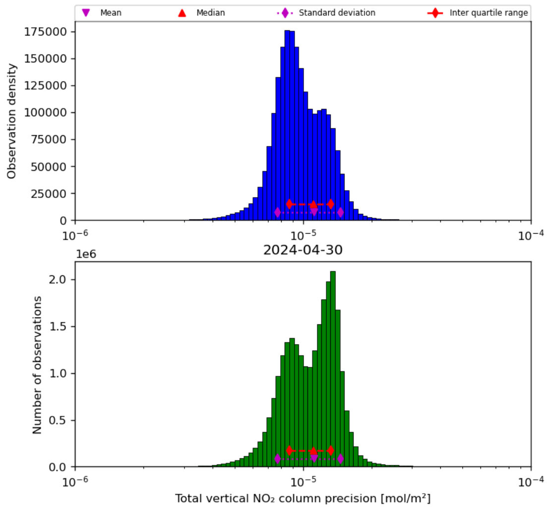
Figure 39: Histogram of “Total vertical NO 2 column precision” for 2024-04-29 to 2024-05-01
