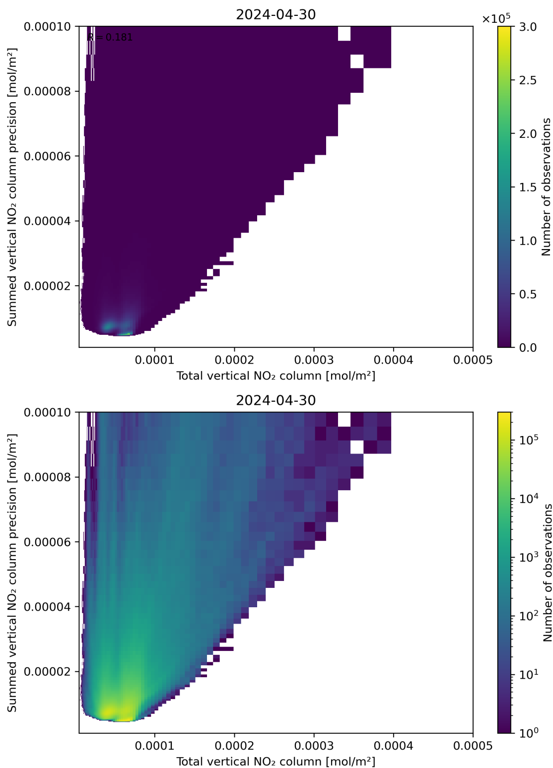
Figure 113: Scatter density plot of “Total vertical NO 2 column” against “Summed vertical NO 2 column precision” for 2024-04-29 to 2024-05-01.
