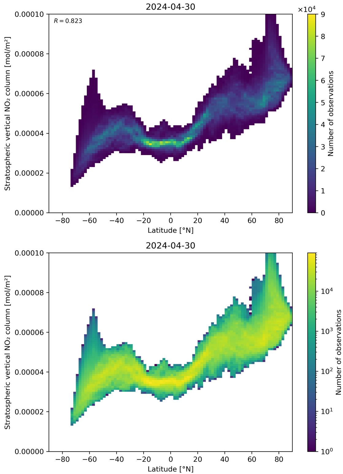
Figure 87: Scatter density plot of “Latitude” against “Stratospheric vertical NO 2 column” for 2024-04-29 to 2024-05-01.
