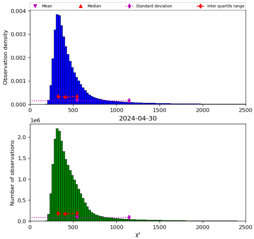
Figure 42: Histogram of “ \chi^2 ” for 2024-04-29 to 2024-05-01
