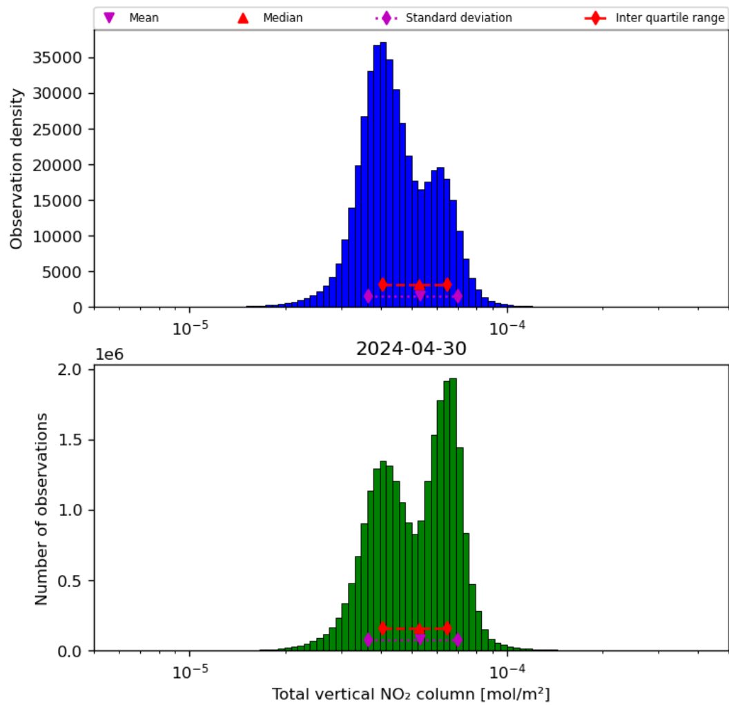
Figure 38: Histogram of “Total vertical NO 2 column” for 2024-04-29 to 2024-05-01
