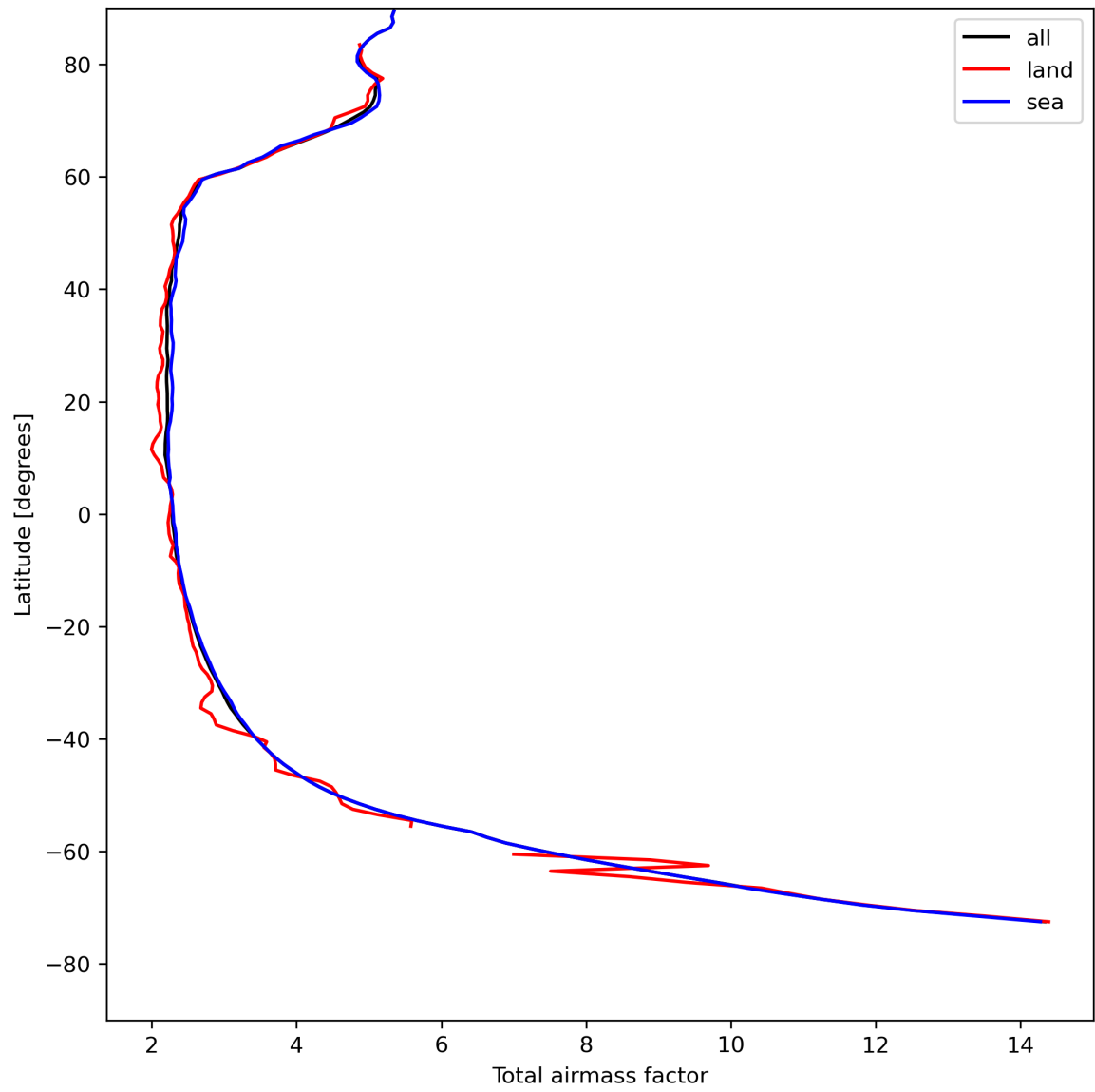
Figure 15: Zonal average of “Total airmass factor” for 2024-04-29 to 2024-05-01.
