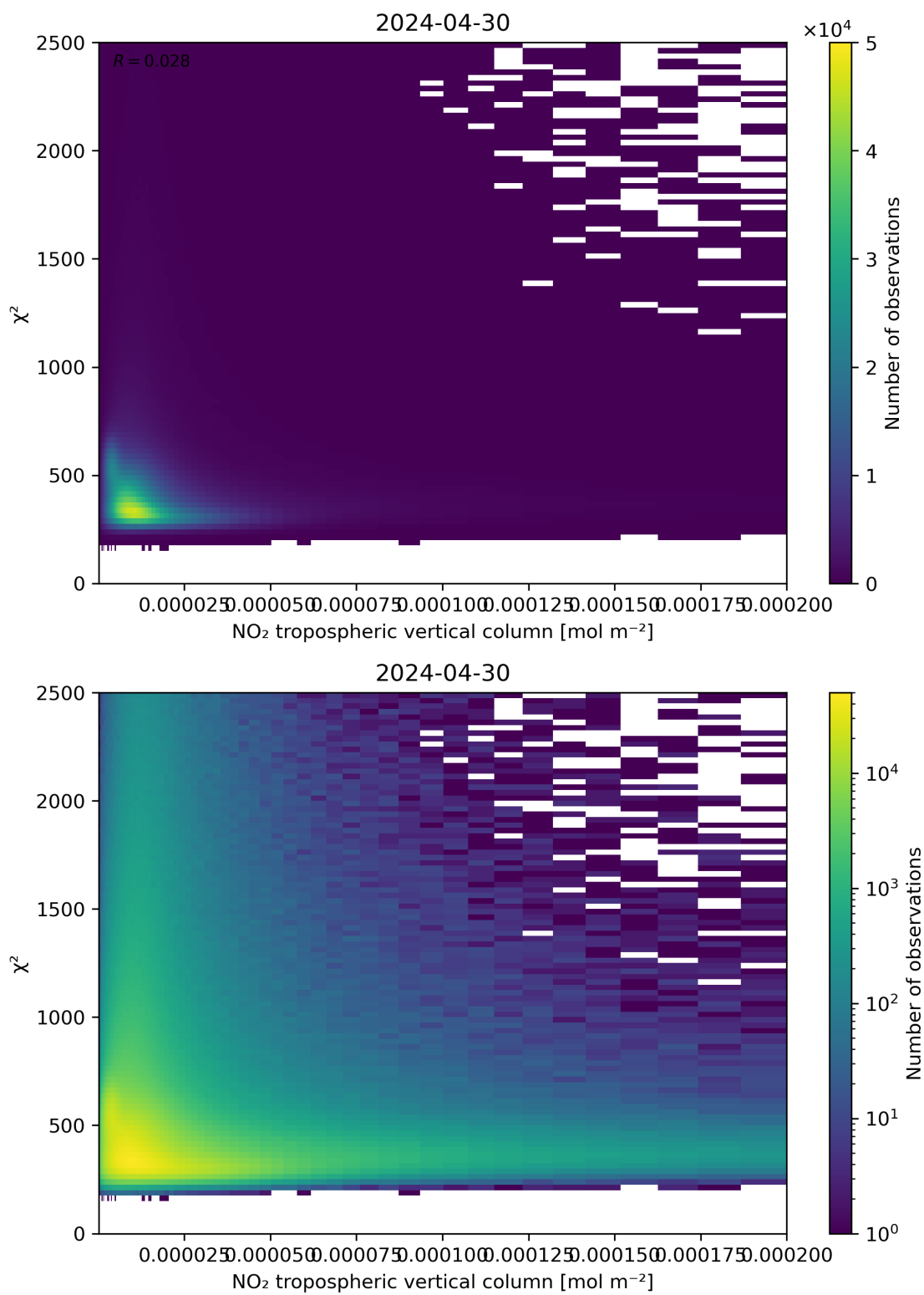
Figure 124: Scatter density plot of “NO 2 tropospheric vertical column” against “ \chi^2 ” for 2024-04-29 to 2024-05-01.
