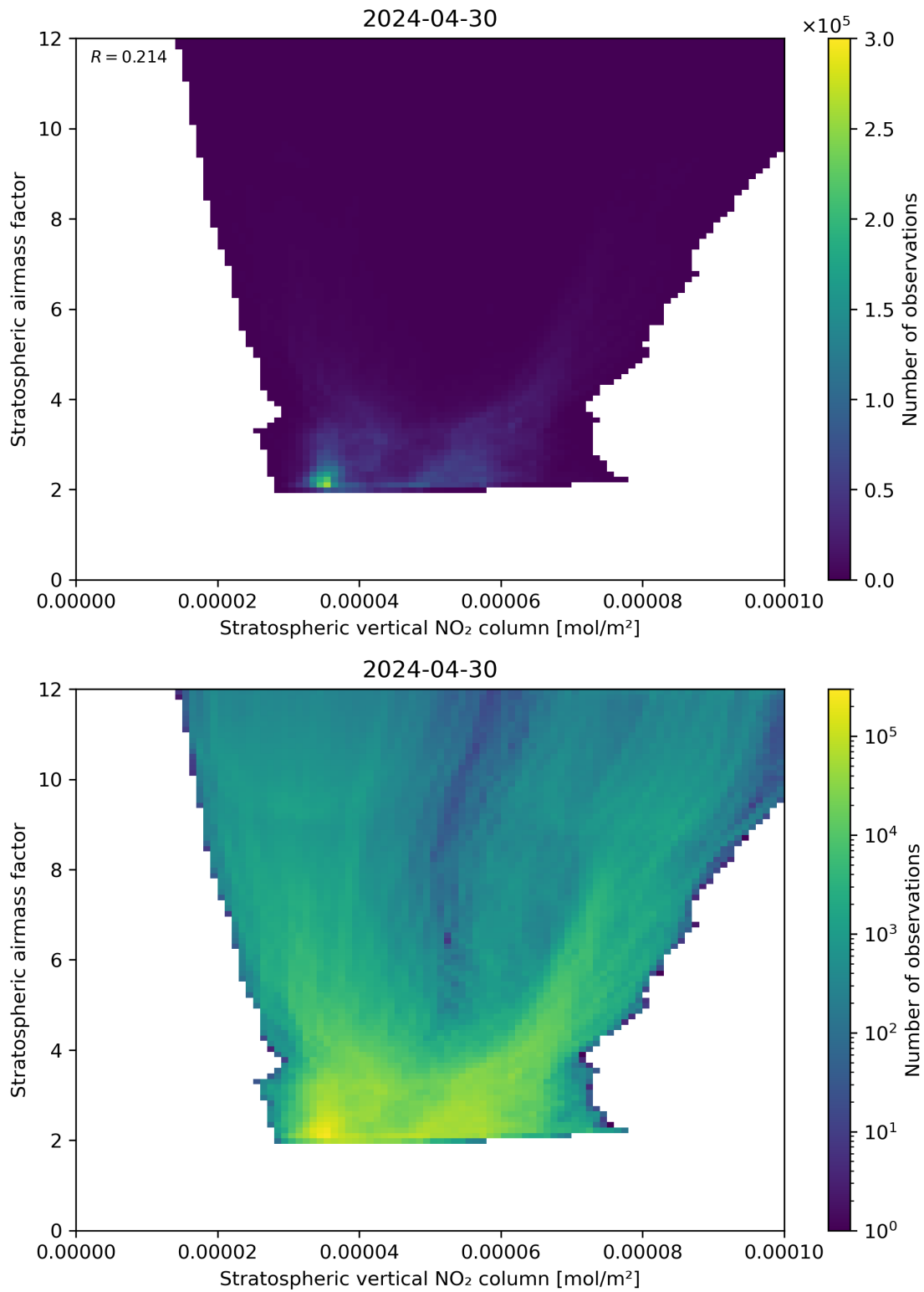
Figure 96: Scatter density plot of “Stratospheric vertical NO 2 column” against “Stratospheric airmass factor” for 2024-04-29 to 2024-05-01.
