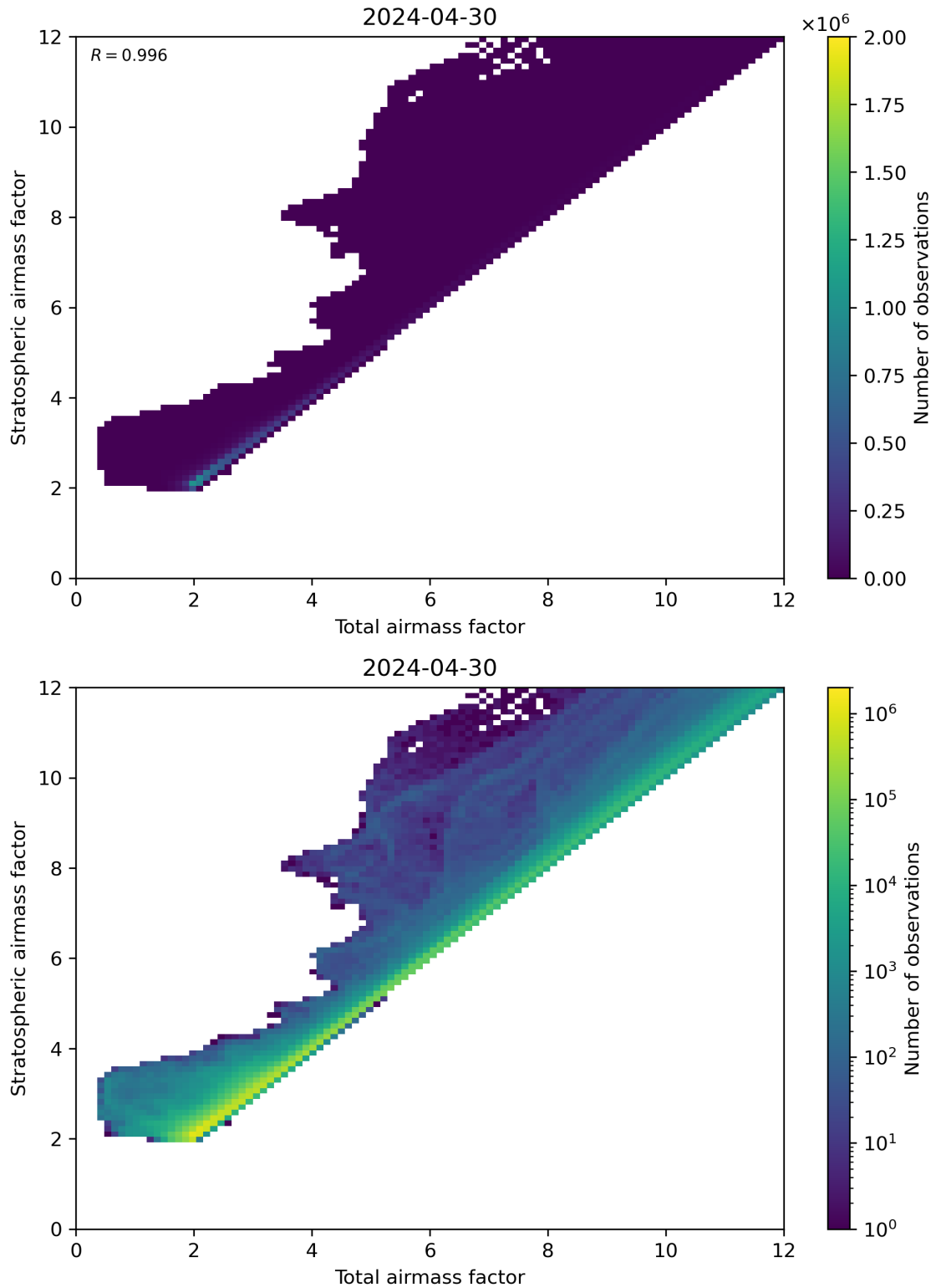
Figure 62: Scatter density plot of “Total airmass factor” against “Stratospheric airmass factor” for 2024-04-29 to 2024-05-01.
