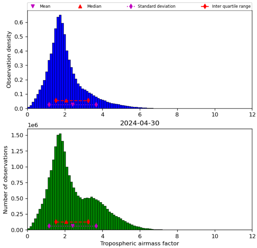
Figure 31: Histogram of “Tropospheric airmass factor” for 2024-04-29 to 2024-05-01
