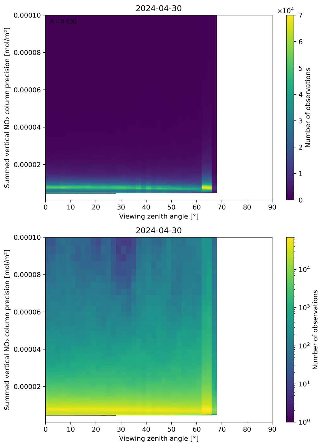
Figure 166: Scatter density plot of “Viewing zenith angle” against “Summed vertical NO 2 column precision” for 2024-04-29 to 2024-05-01.
