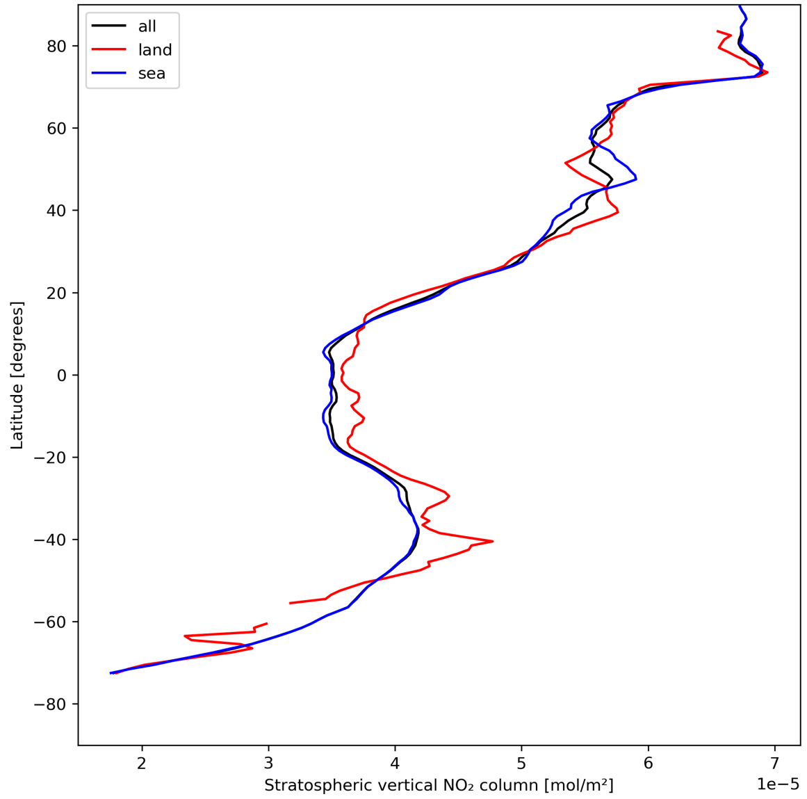
Figure 19: Zonal average of “Stratospheric vertical NO 2 column” for 2024-04-29 to 2024-05-01.
