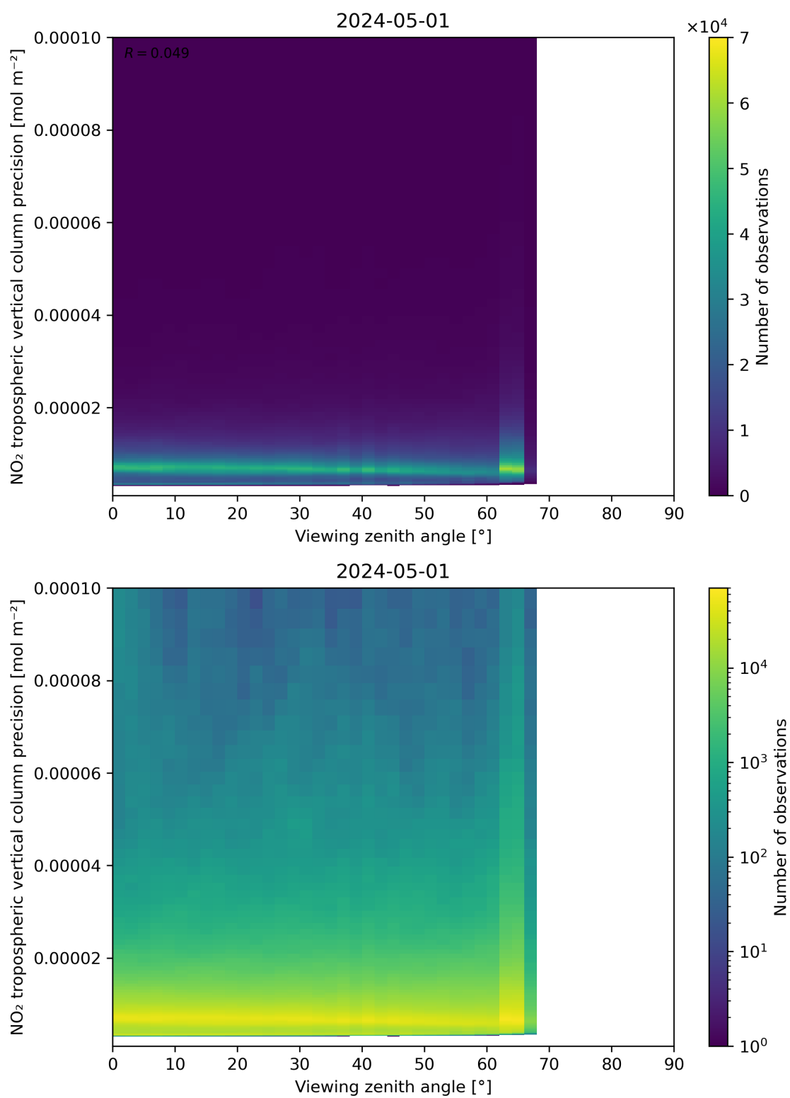
Figure 170: Scatter density plot of “Viewing zenith angle” against “NO 2 tropospheric vertical column precision” for 2024-04-30 to 2024-05-02.
