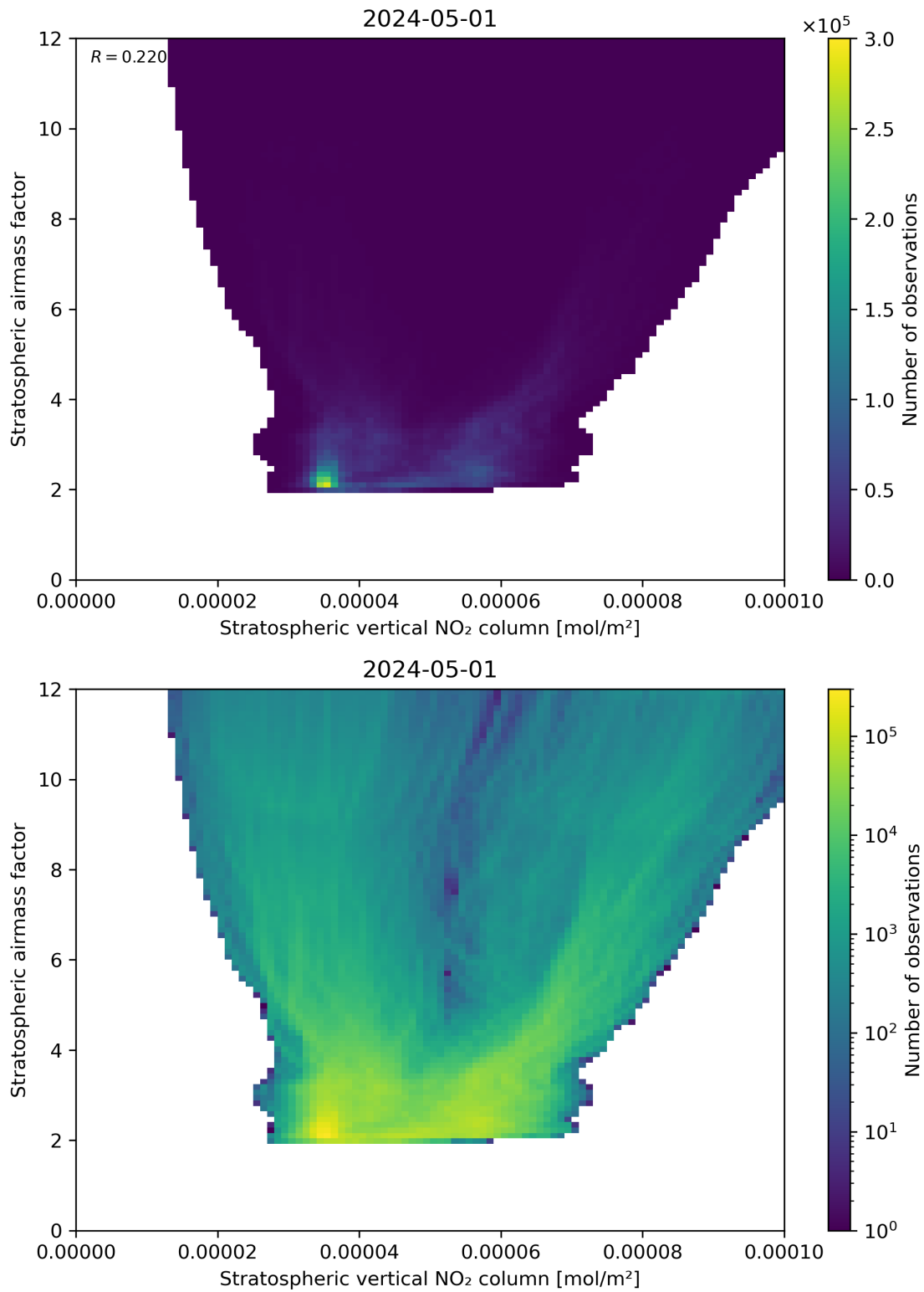
Figure 96: Scatter density plot of “Stratospheric vertical NO 2 column” against “Stratospheric airmass factor” for 2024-04-30 to 2024-05-02.
