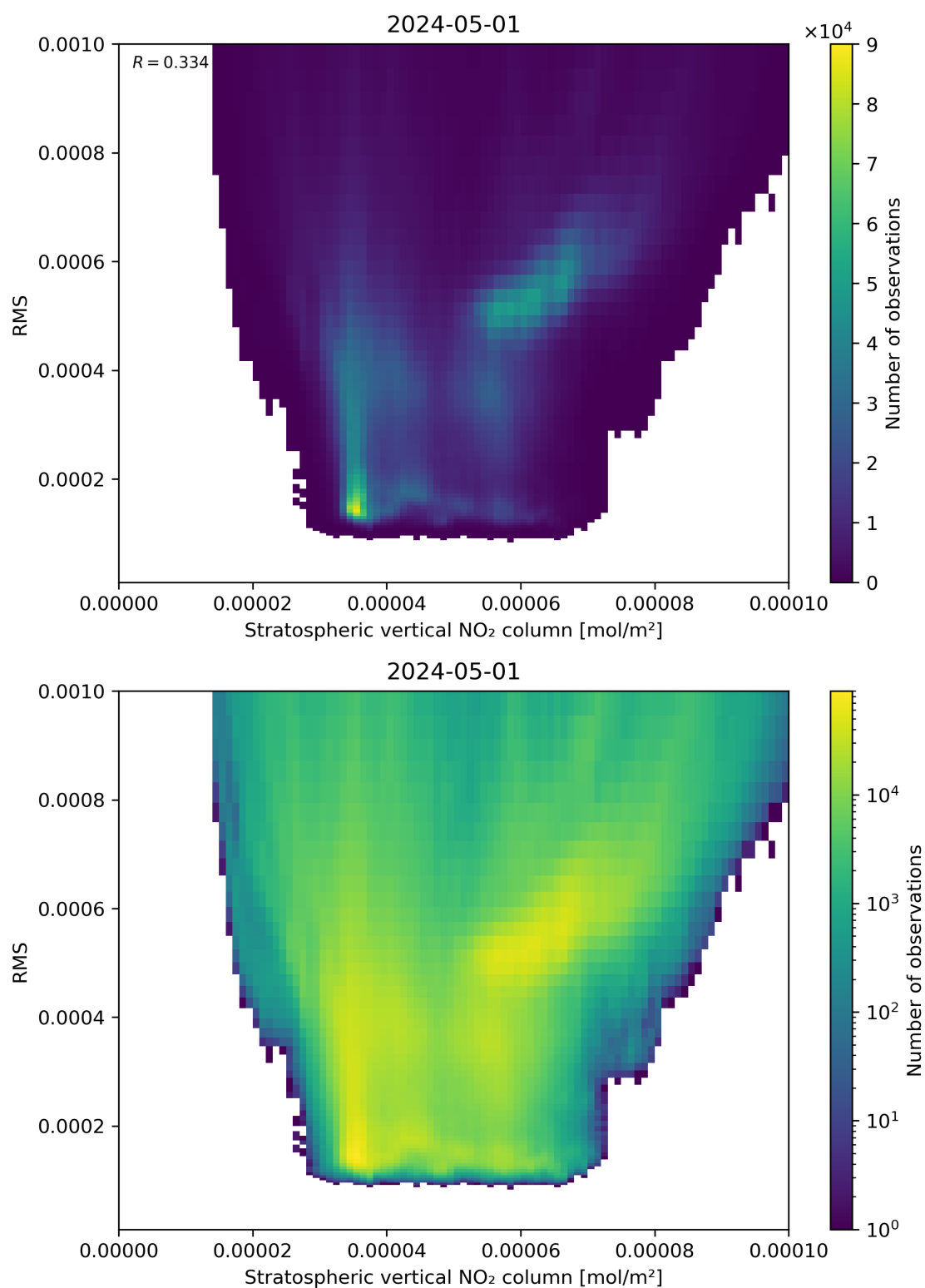
Figure 102: Scatter density plot of “Stratospheric vertical NO 2 column” against “RMS” for 2024-04-30 to 2024-05-02.
