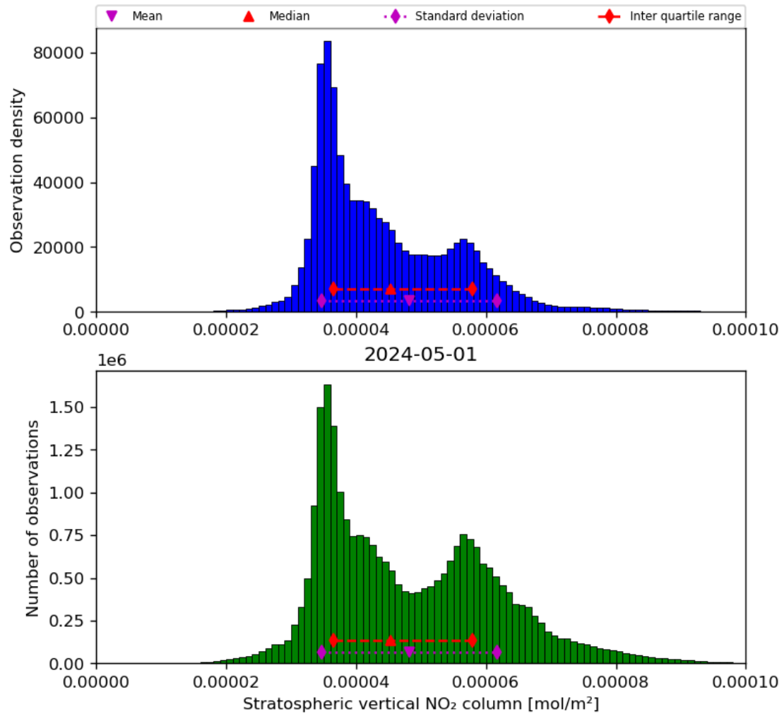
Figure 36: Histogram of “Stratospheric vertical NO 2 column” for 2024-04-30 to 2024-05-02
