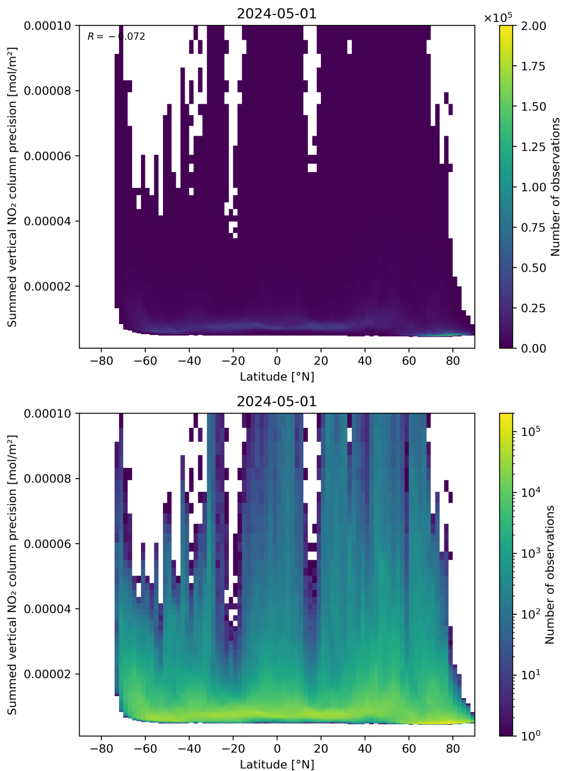
Figure 89: Scatter density plot of “Latitude” against “Summed vertical NO 2 column precision” for 2024-04-30 to 2024-05-02.
