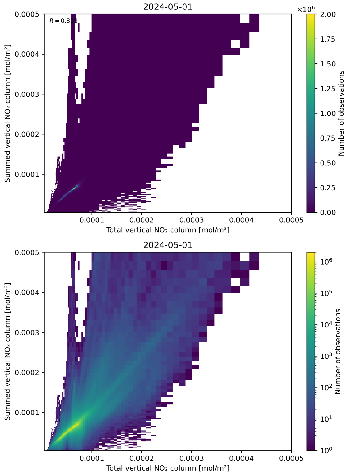
Figure 112: Scatter density plot of “Total vertical NO 2 column” against “Summed vertical NO 2 column” for 2024-04-30 to 2024-05-02.
