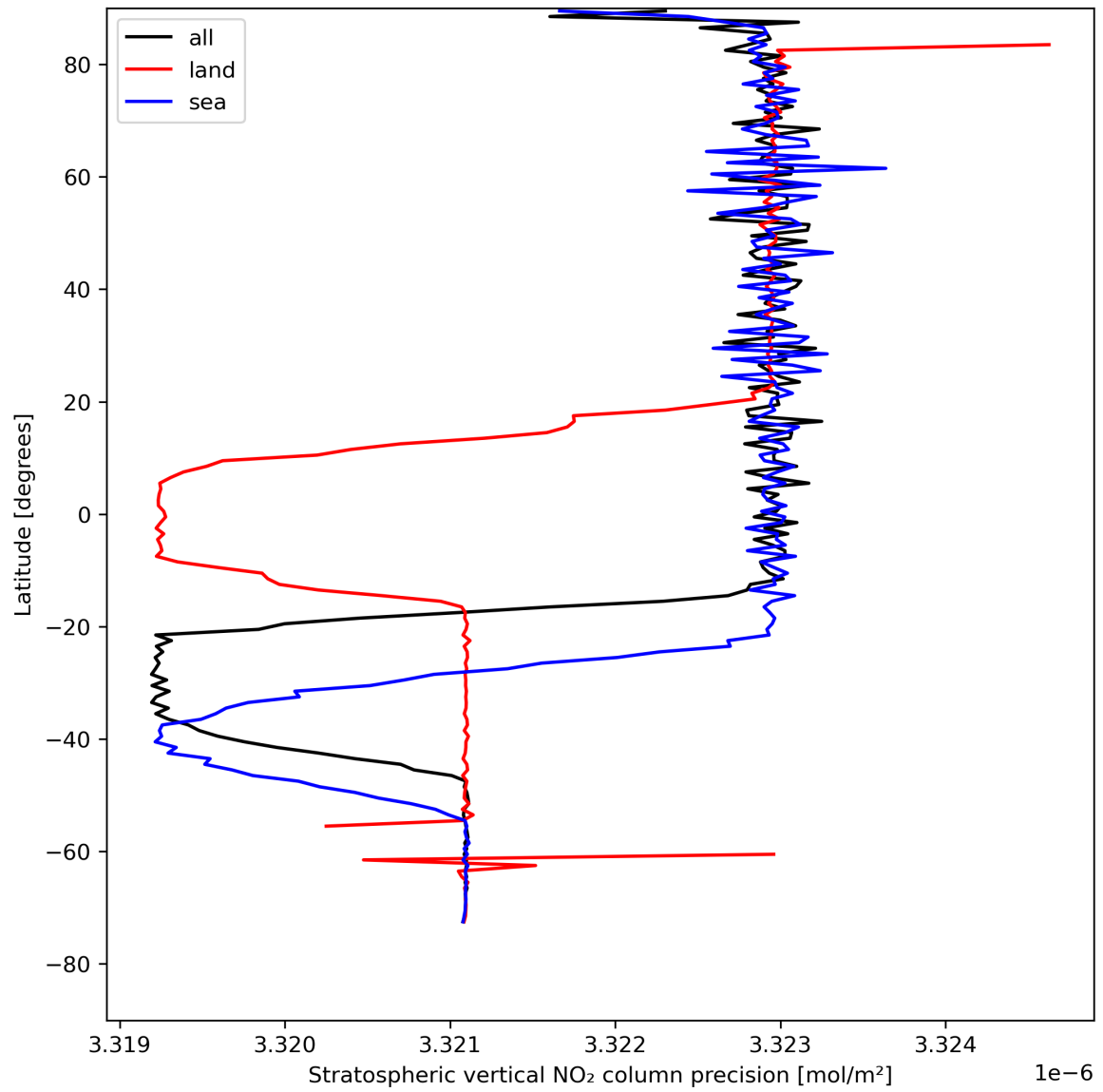
Figure 20: Zonal average of “Stratospheric vertical NO 2 column precision” for 2024-04-30 to 2024-05-02.
