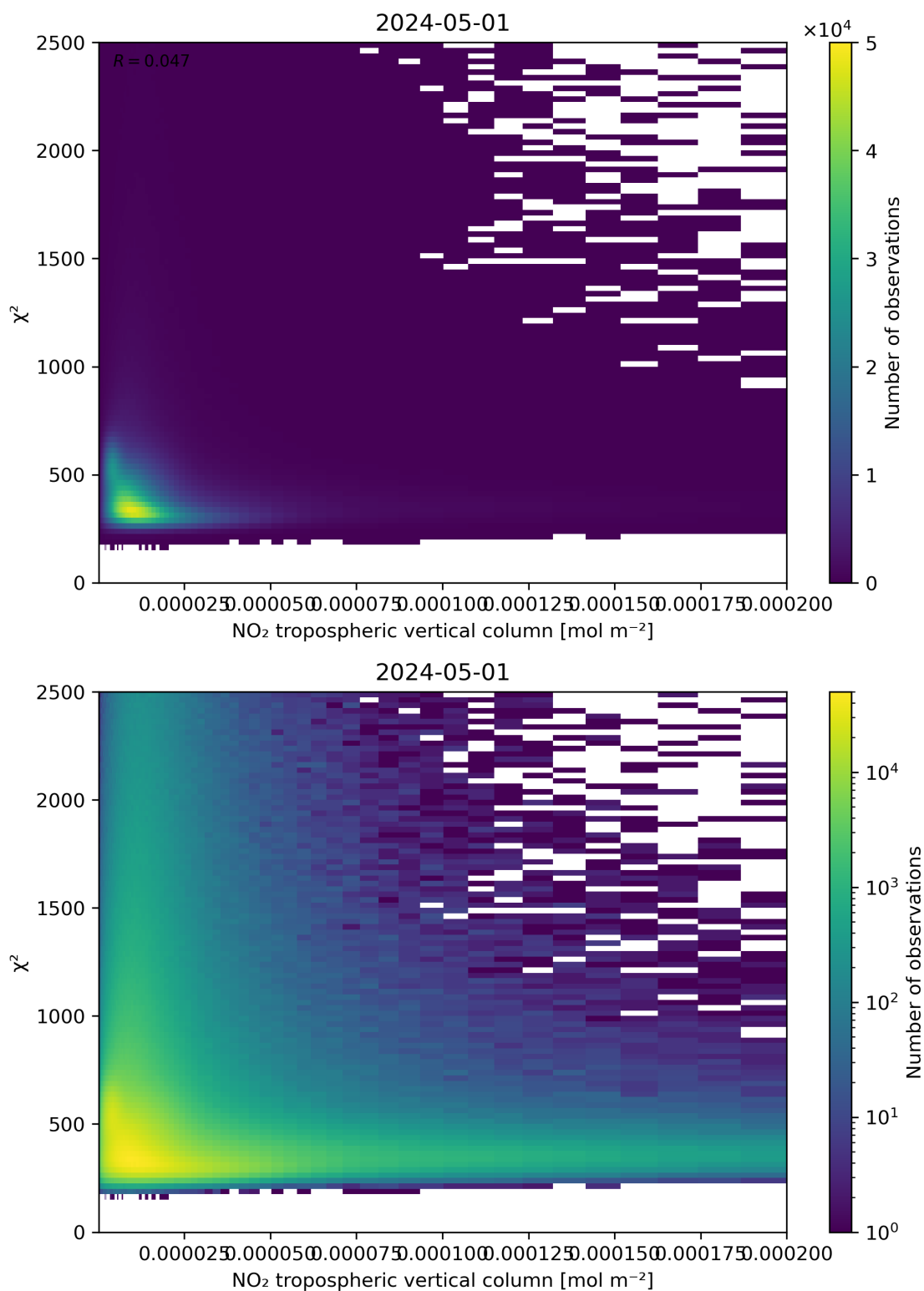
Figure 124: Scatter density plot of “NO 2 tropospheric vertical column” against “ \chi^2 ” for 2024-04-30 to 2024-05-02.
