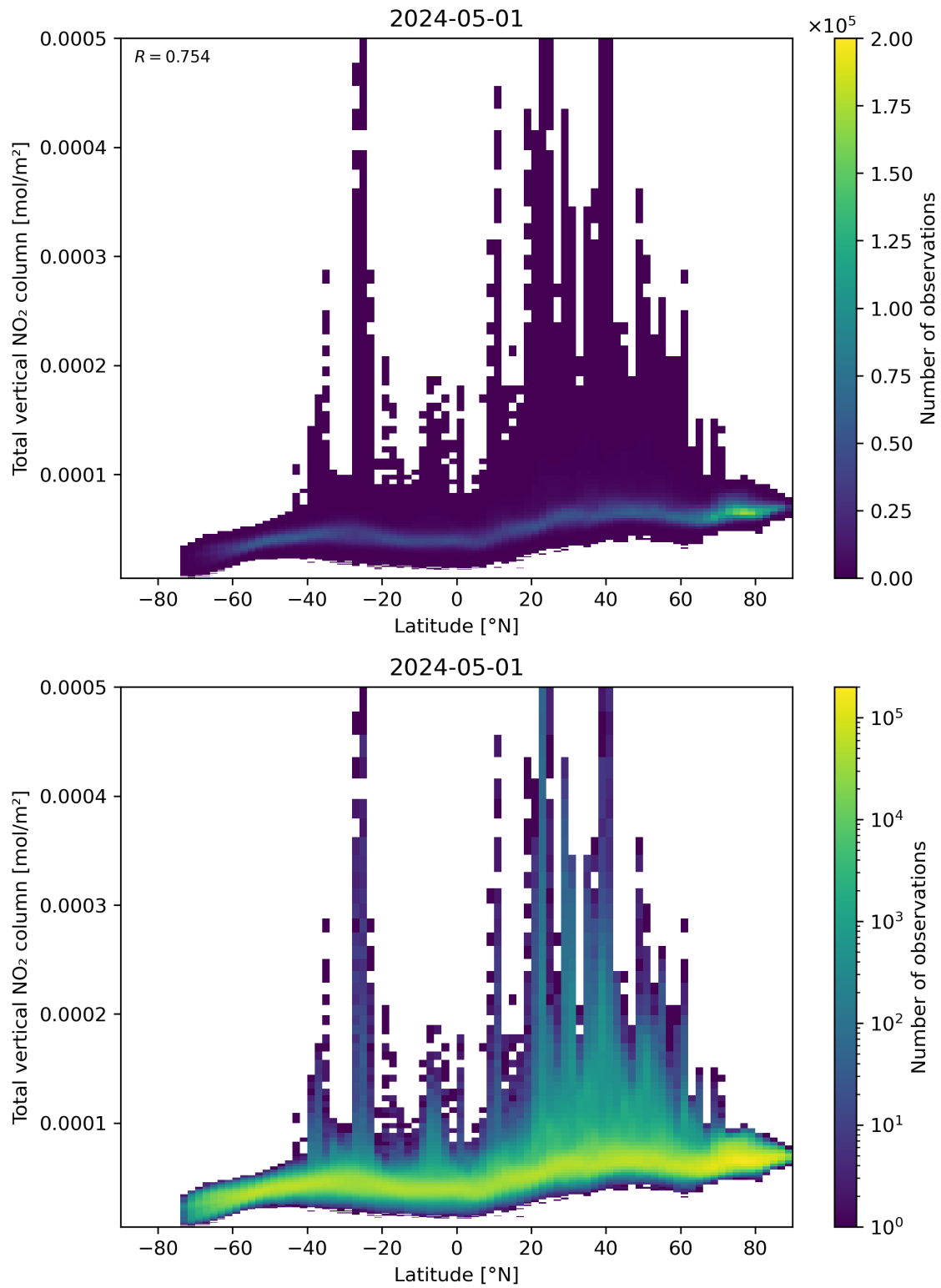
Figure 90: Scatter density plot of “Latitude” against “Total vertical NO 2 column” for 2024-04-30 to 2024-05-02.
