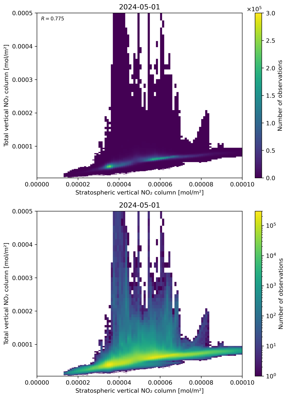
Figure 100: Scatter density plot of “Stratospheric vertical NO 2 column” against “Total vertical NO 2 column” for 2024-04-30 to 2024-05-02.
