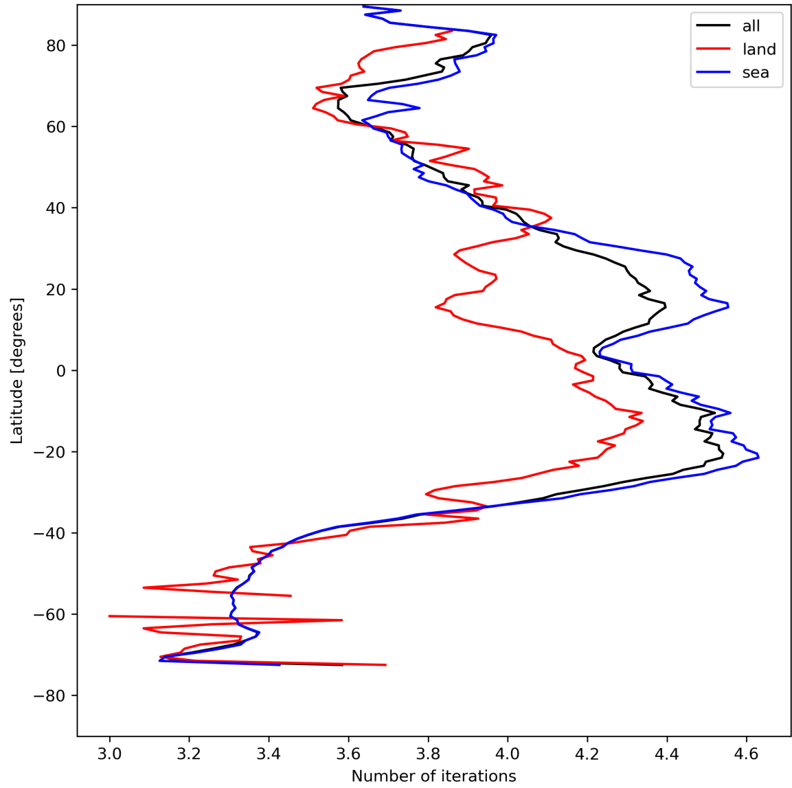
Figure 17: Zonal average of “Number of iterations” for 2024-04-30 to 2024-05-02.
