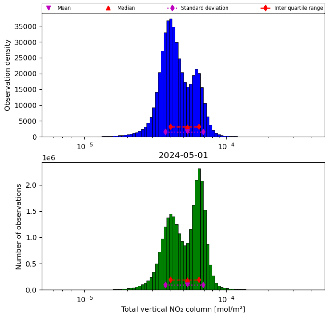
Figure 38: Histogram of “Total vertical NO 2 column” for 2024-04-30 to 2024-05-02
