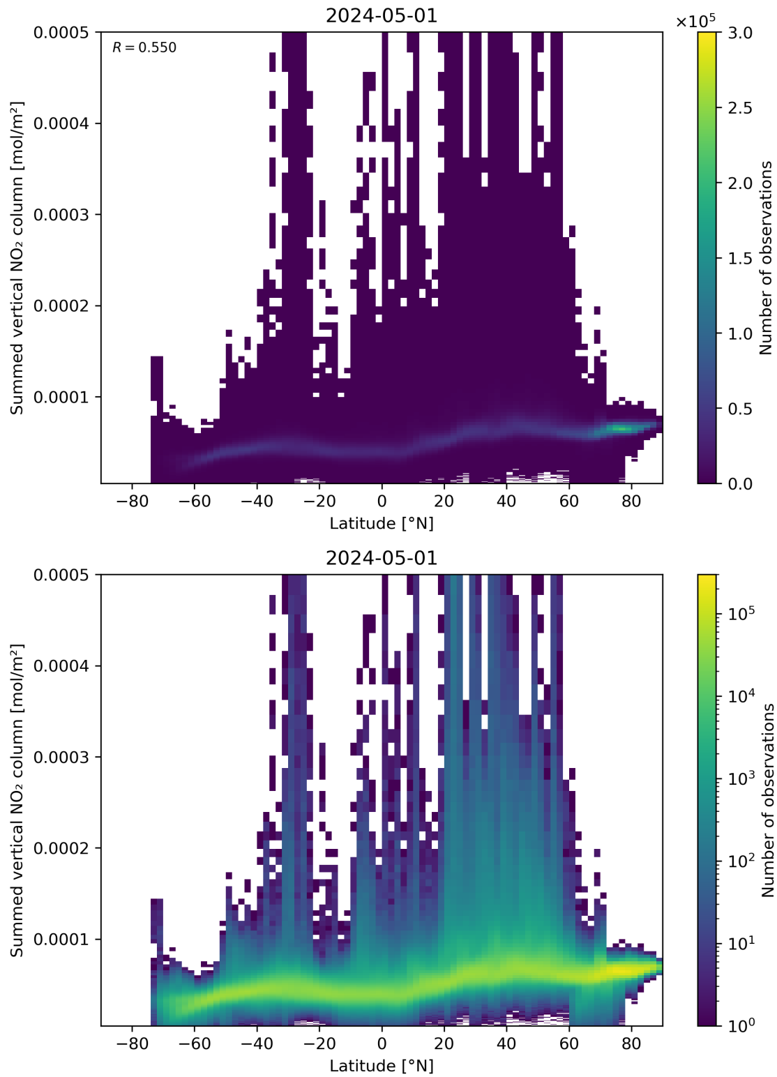
Figure 88: Scatter density plot of “Latitude” against “Summed vertical NO 2 column” for 2024-04-30 to 2024-05-02.
