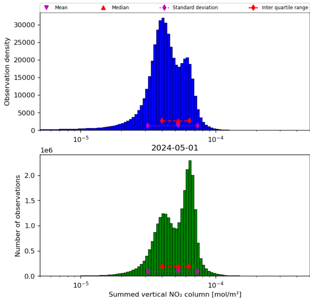
Figure 40: Histogram of "Summed vertical NO 2 column" for 2024-04-30 to 2024-05-02
