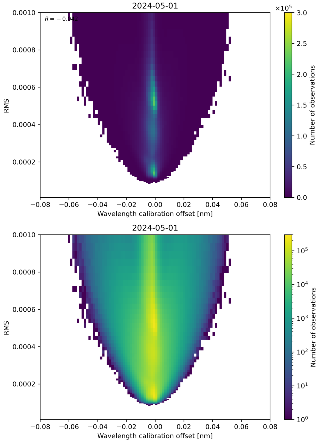
Figure 181: Scatter density plot of “Wavelength calibration offset” against “RMS” for 2024-04-30 to 2024-05-02.
