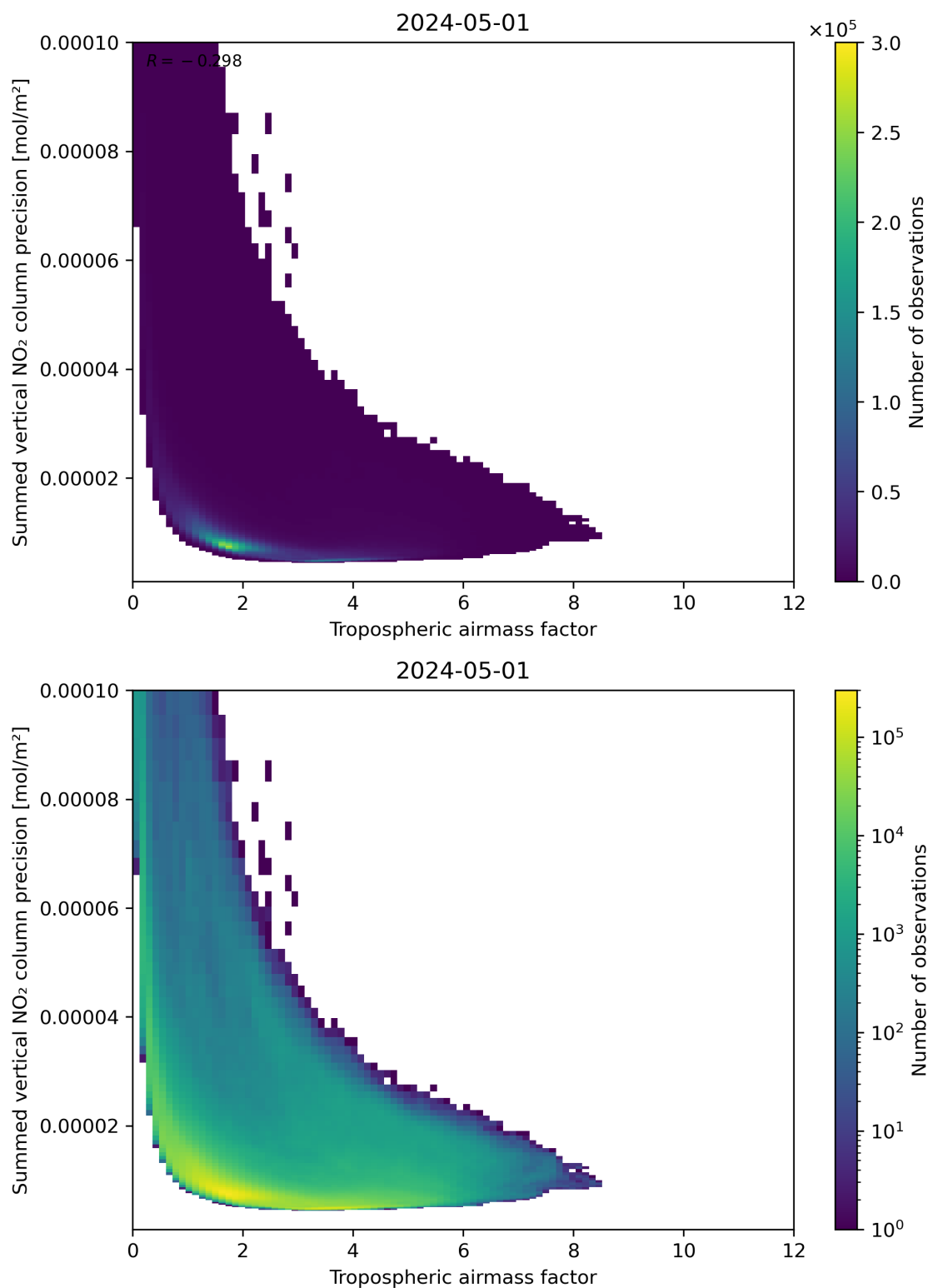
Figure 76: Scatter density plot of “Tropospheric air mass factor” against “Summed vertical NO 2 column precision” for 2024-04-30 to 2024-05-02.
