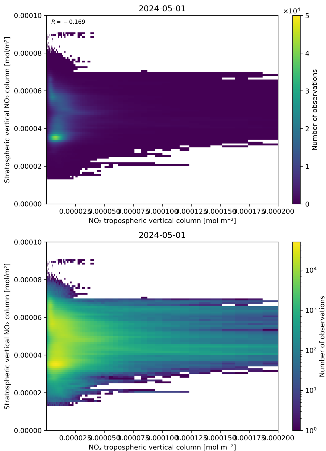
Figure 125: Scatter density plot of “NO 2 tropospheric vertical column” against “Stratospheric vertical NO 2 column” for 2024-04-30 to 2024-05-02.
