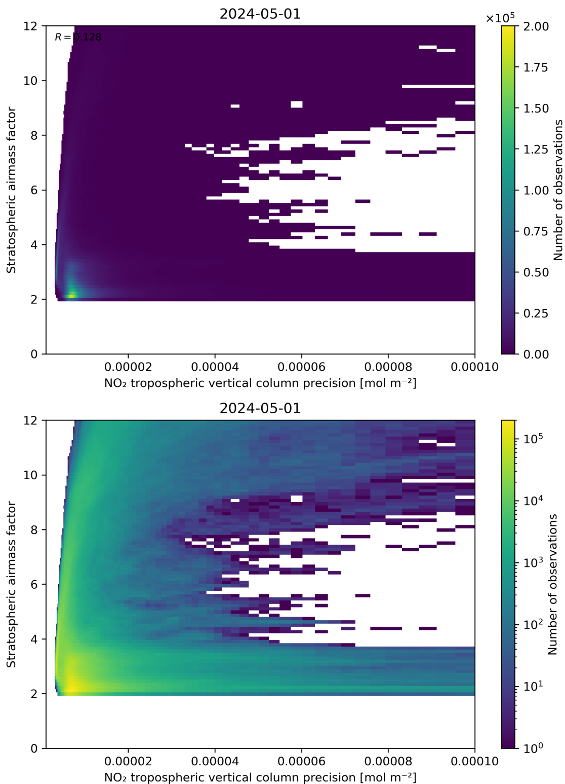
Figure 131: Scatter density plot of “NO 2 tropospheric vertical column precision” against “Stratospheric airmass factor” for 2024-04-30 to 2024-05-02.
