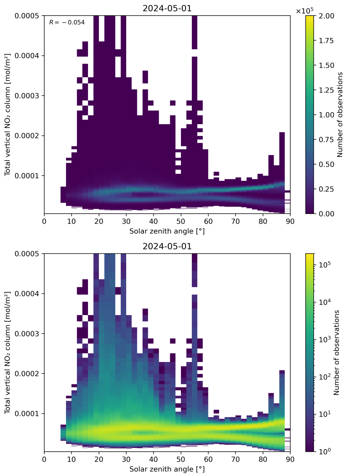
Figure 153: Scatter density plot of “Solar zenith angle” against “Total vertical NO 2 column” for 2024-04-30 to 2024-05-02.
