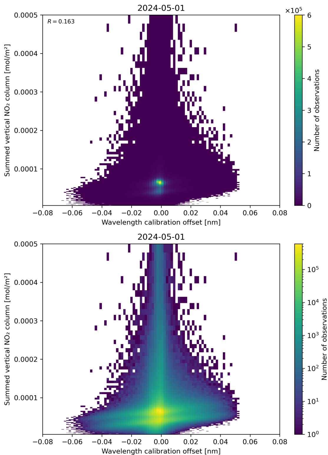
Figure 177: Scatter density plot of “Wavelength calibration offset” against “Summed vertical NO 2 column” for 2024-04-30 to 2024-05-02.
