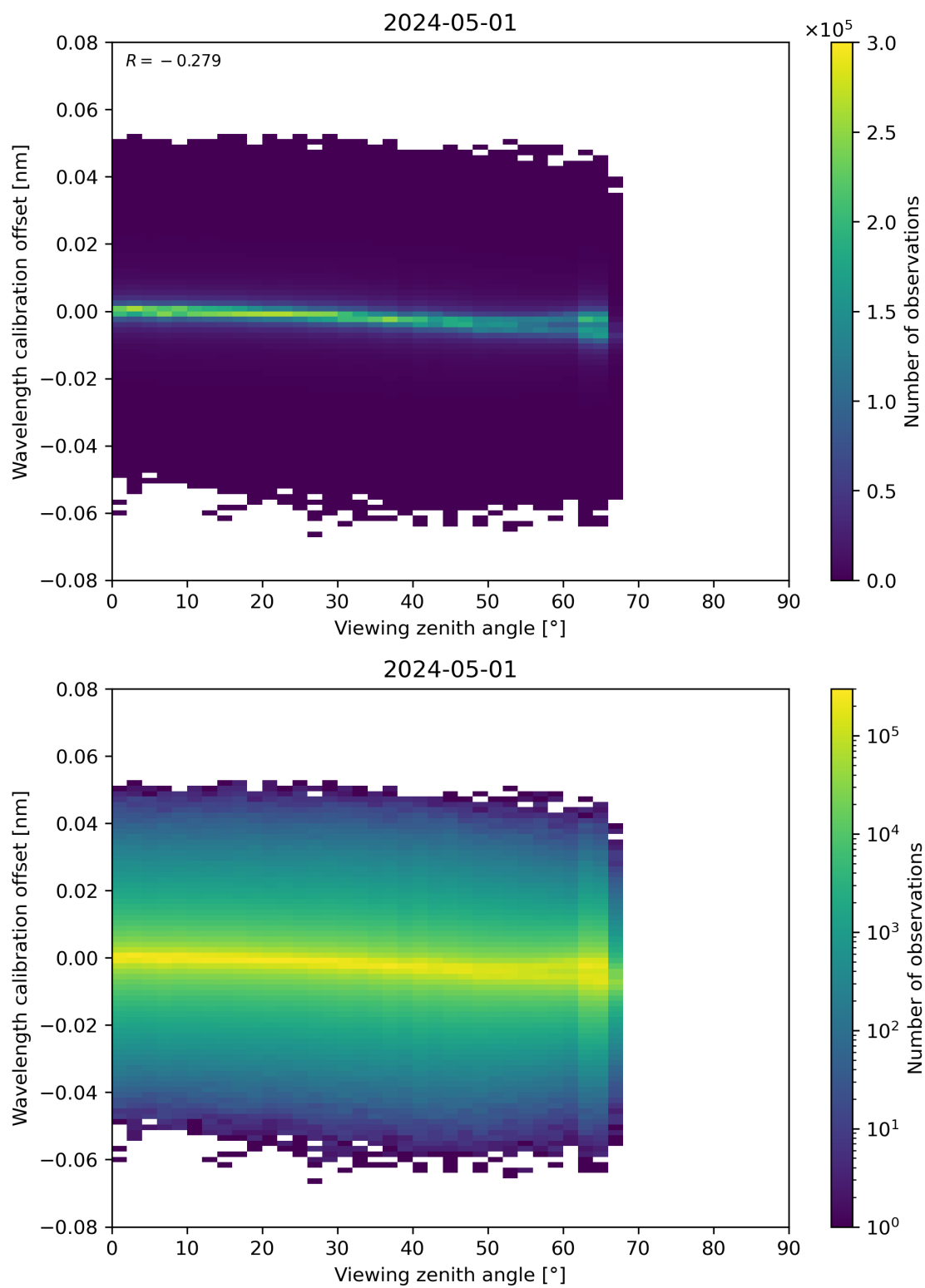
Figure 173: Scatter density plot of “Viewing zenith angle” against “Wavelength calibration offset” for 2024-04-30 to 2024-05-02.
