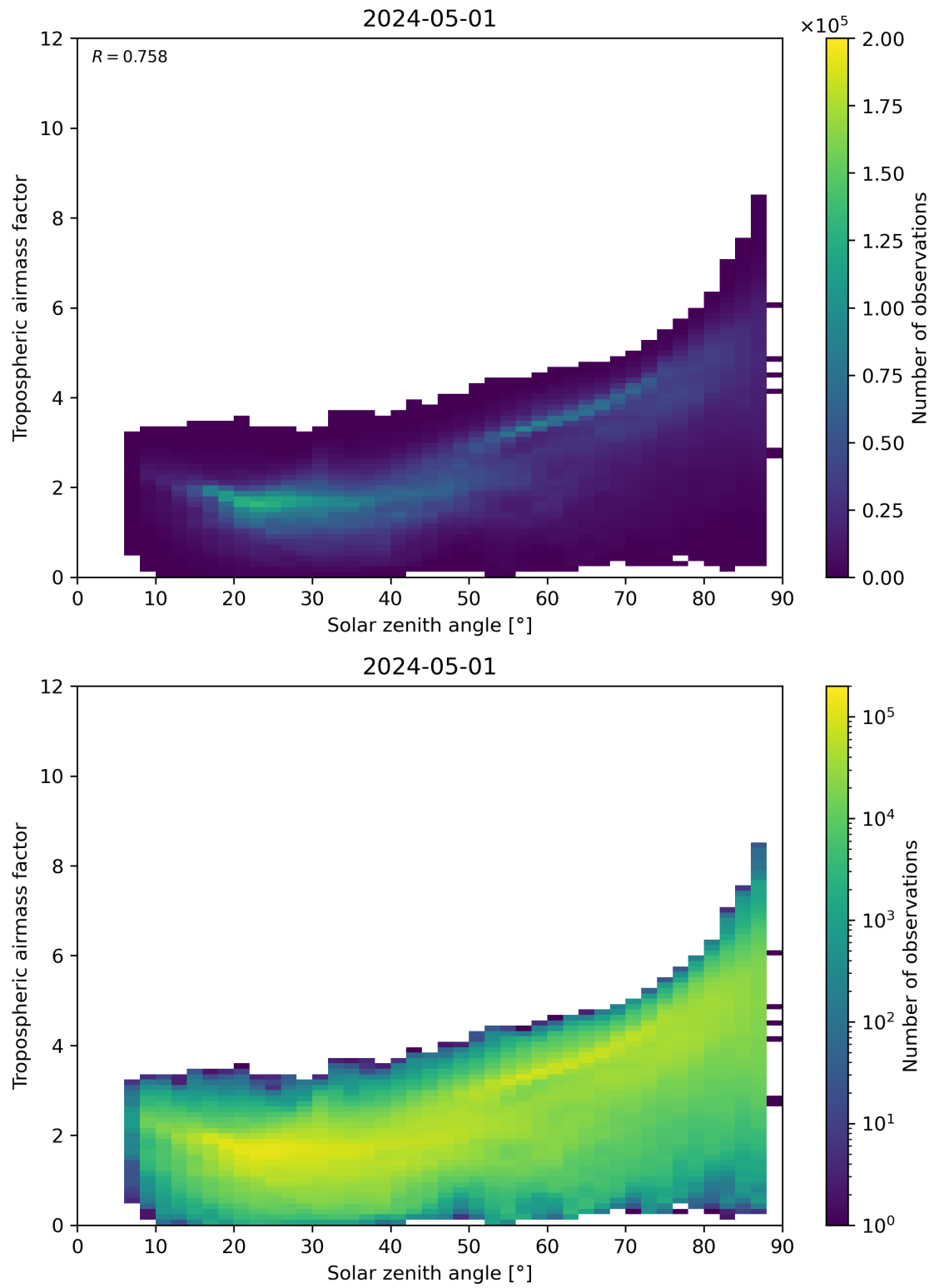
Figure 147: Scatter density plot of “Solar zenith angle” against “Tropospheric airmass factor” for 2024-04-30 to 2024-05-02.
