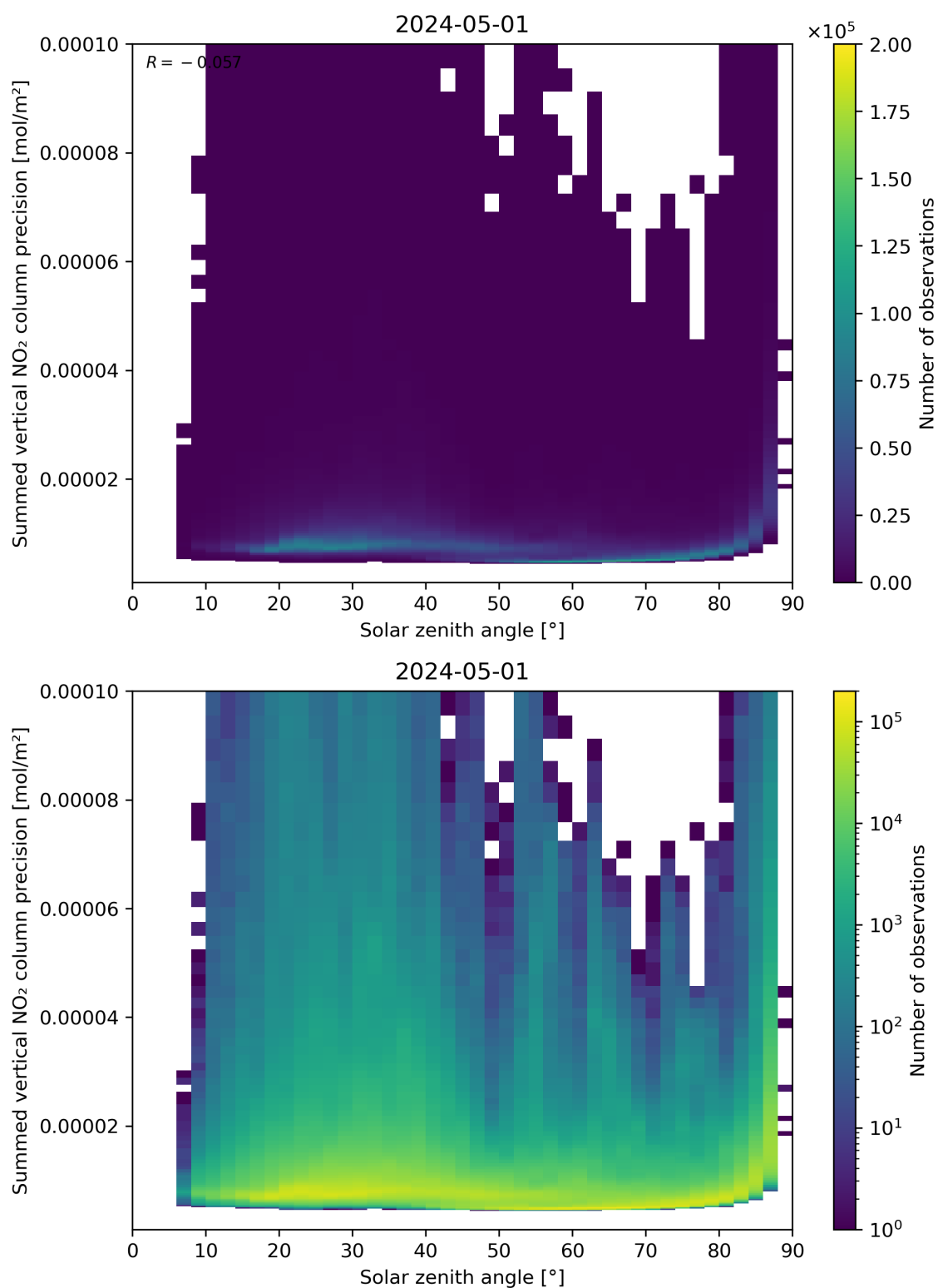
Figure 152: Scatter density plot of “Solar zenith angle” against “Summed vertical NO 2 column precision” for 2024-04-30 to 2024-05-02.
