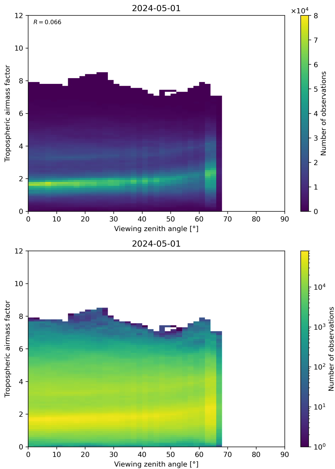
Figure 161: Scatter density plot of “Viewing zenith angle” against “Tropospheric airmass factor” for 2024-04-30 to 2024-05-02.
