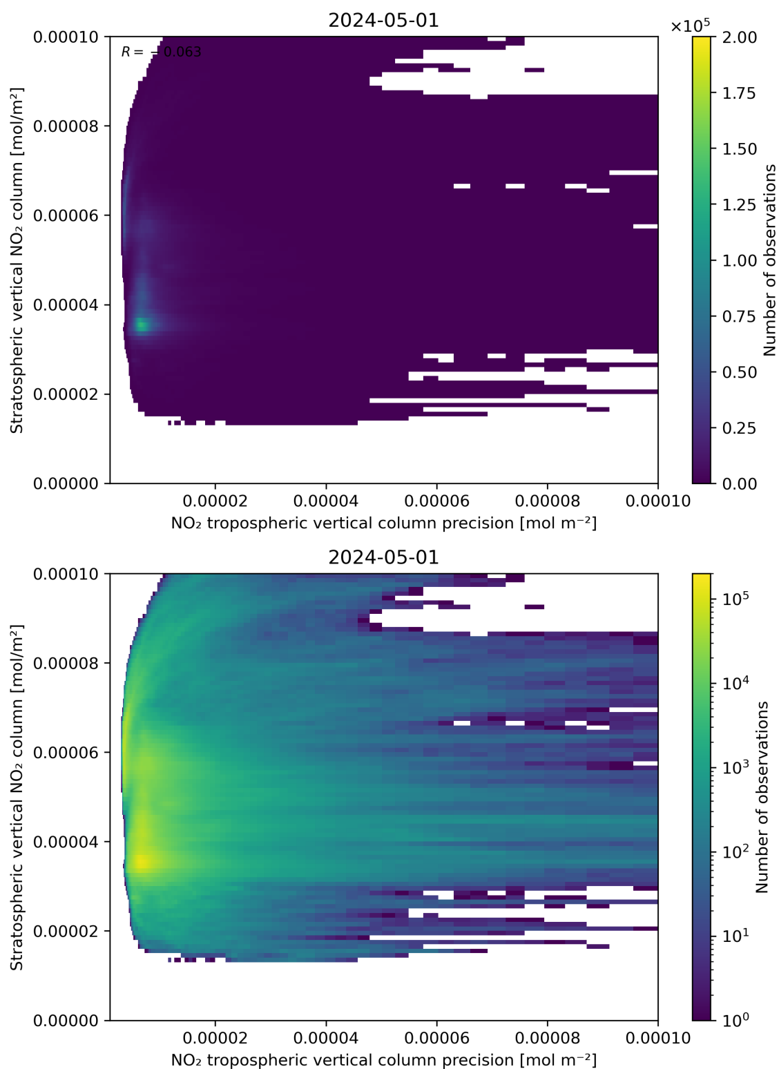
Figure 135: Scatter density plot of “NO 2 tropospheric vertical column precision” against “Stratospheric vertical NO 2 column” for 2024-04-30 to 2024-05-02.
