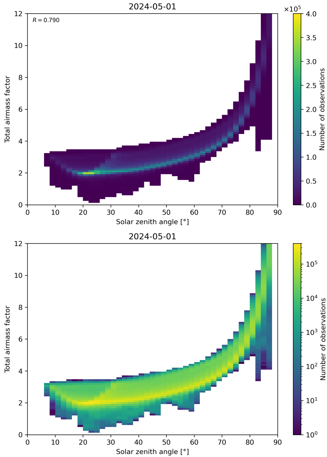
Figure 146: Scatter density plot of “Solar zenith angle” against “Total airmass factor” for 2024-04-30 to 2024-05-02.
