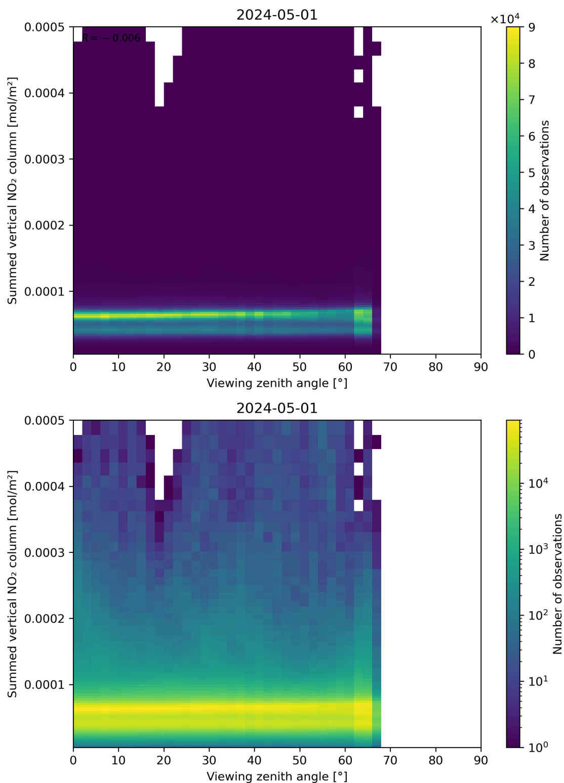
Figure 165: Scatter density plot of “Viewing zenith angle” against “Summed vertical NO 2 column” for 2024-04-30 to 2024-05-02.
