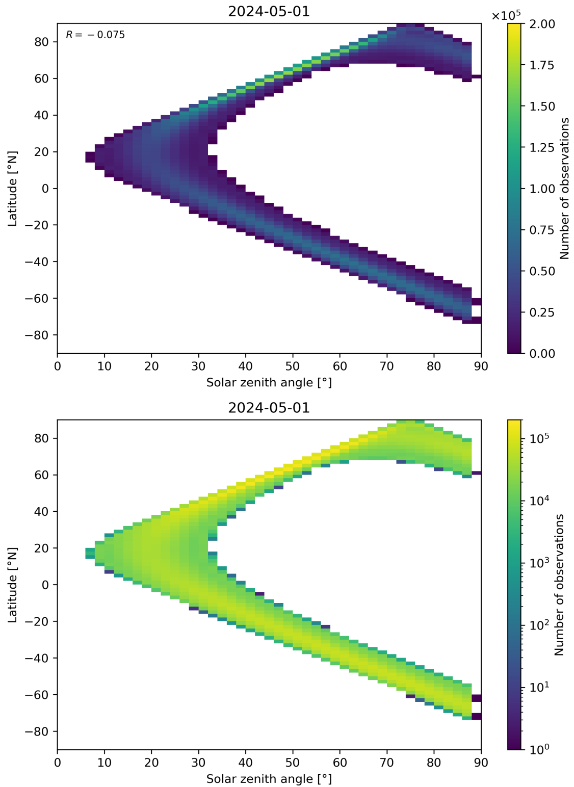
Figure 149: Scatter density plot of “Solar zenith angle” against “Latitude” for 2024-04-30 to 2024-05-02.
