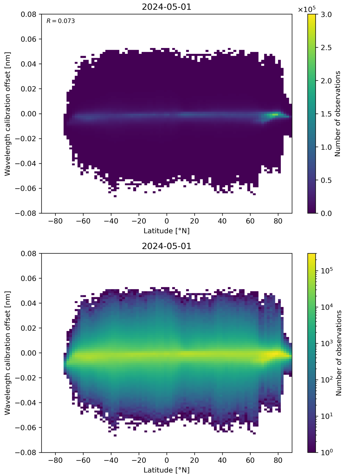
Figure 95: Scatter density plot of “Latitude” against “Wavelength calibration offset” for 2024-04-30 to 2024-05-02.
