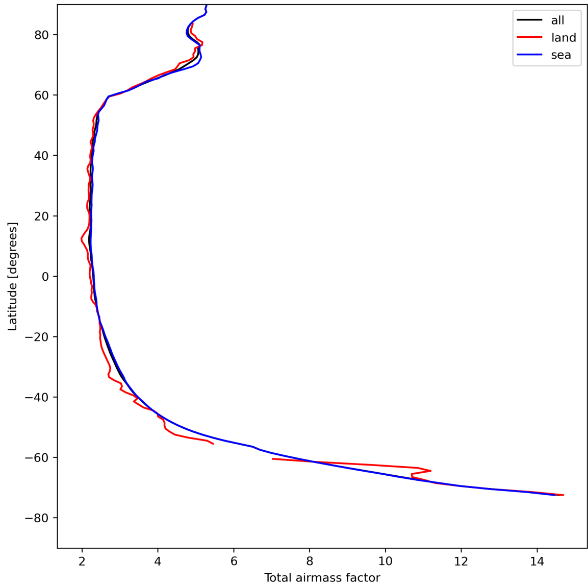
Figure 15: Zonal average of “Total airmass factor” for 2024-04-30 to 2024-05-02.
