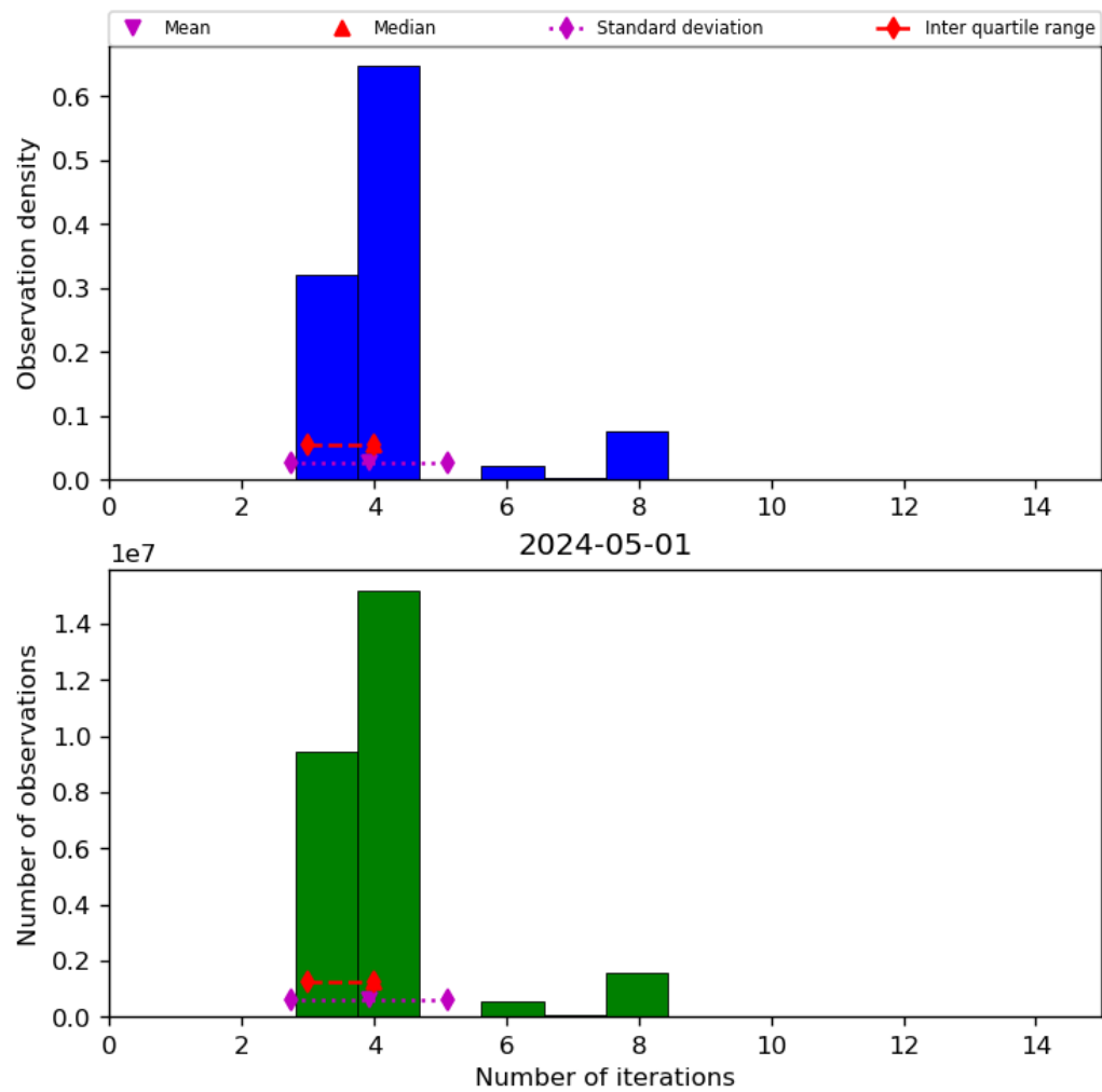
Figure 34: Histogram of "Number of iterations" for 2024-04-30 to 2024-05-02
