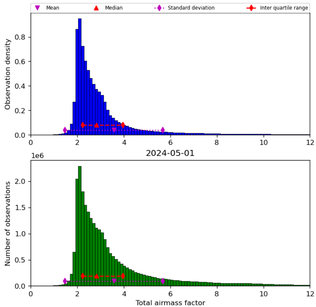
Figure 32: Histogram of “Total airmass factor” for 2024-04-30 to 2024-05-02
