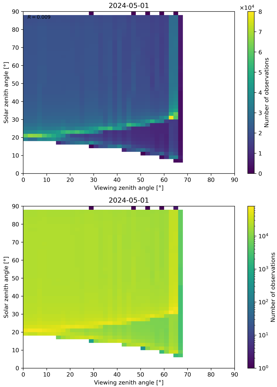
Figure 172: Scatter density plot of “Viewing zenith angle” against “Solar zenith angle” for 2024-04-30 to 2024-05-02.
