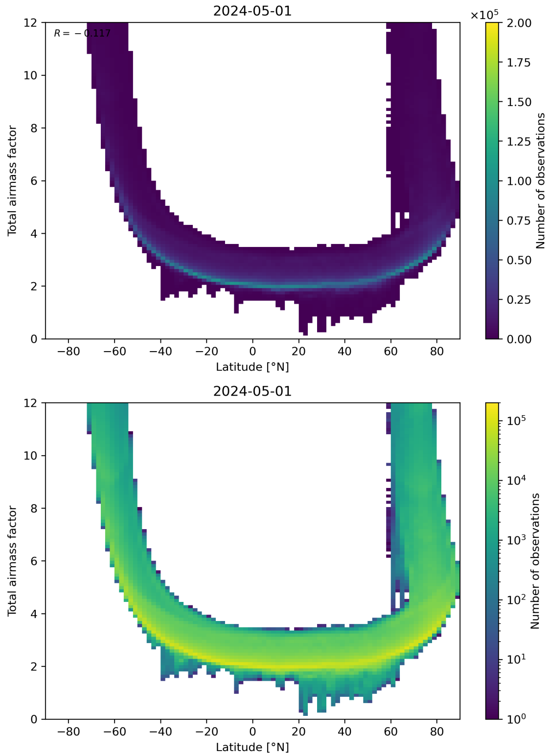
Figure 84: Scatter density plot of “Latitude” against “Total airmass factor” for 2024-04-30 to 2024-05-02.
