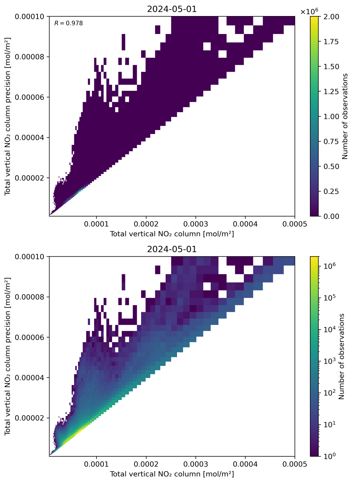
Figure 114: Scatter density plot of “Total vertical NO 2 column” against “Total vertical NO 2 column precision” for 2024-04-30 to 2024-05-02.
