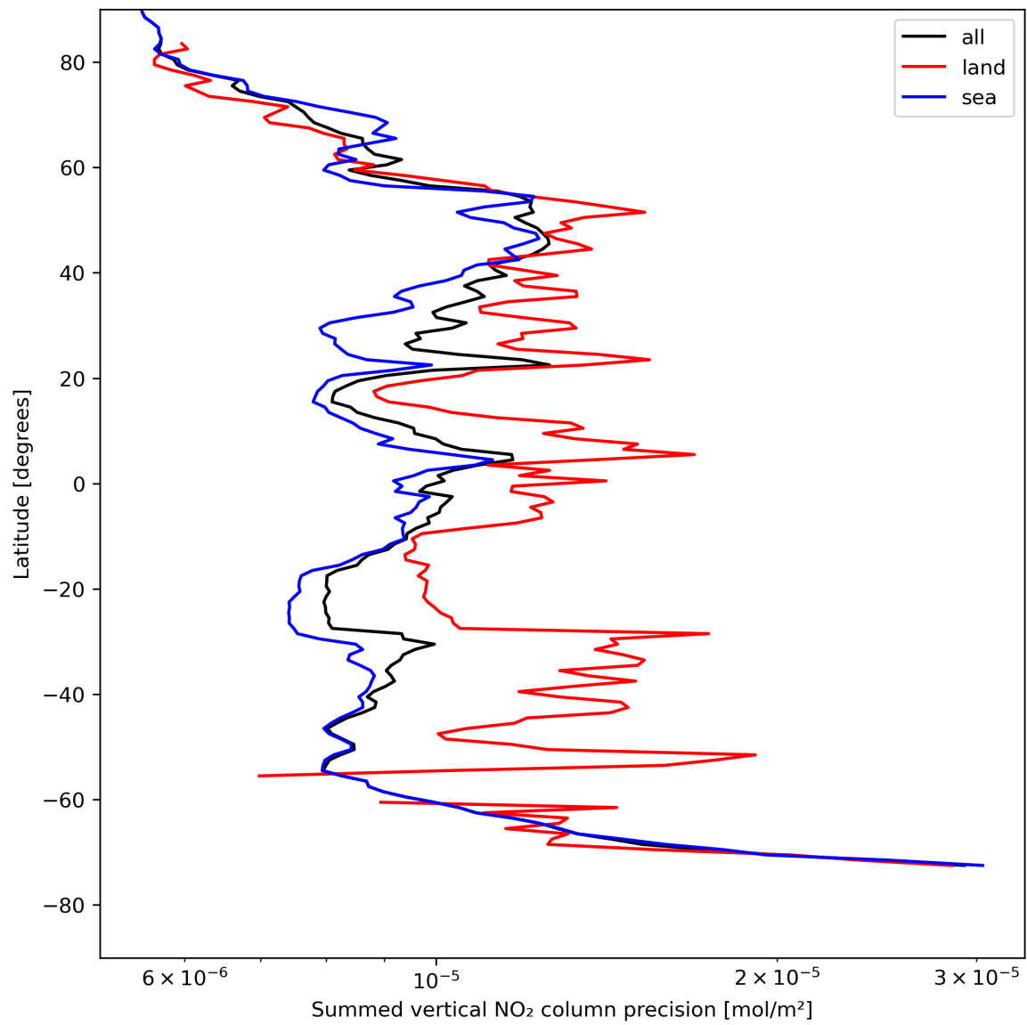
Figure 24: Zonal average of “Summed vertical NO 2 column precision” for 2024-04-30 to 2024-05-02.
