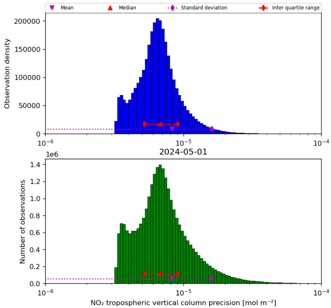
Figure 30: Histogram of “NO 2 tropospheric vertical column precision” for 2024-04-30 to 2024-05-02
