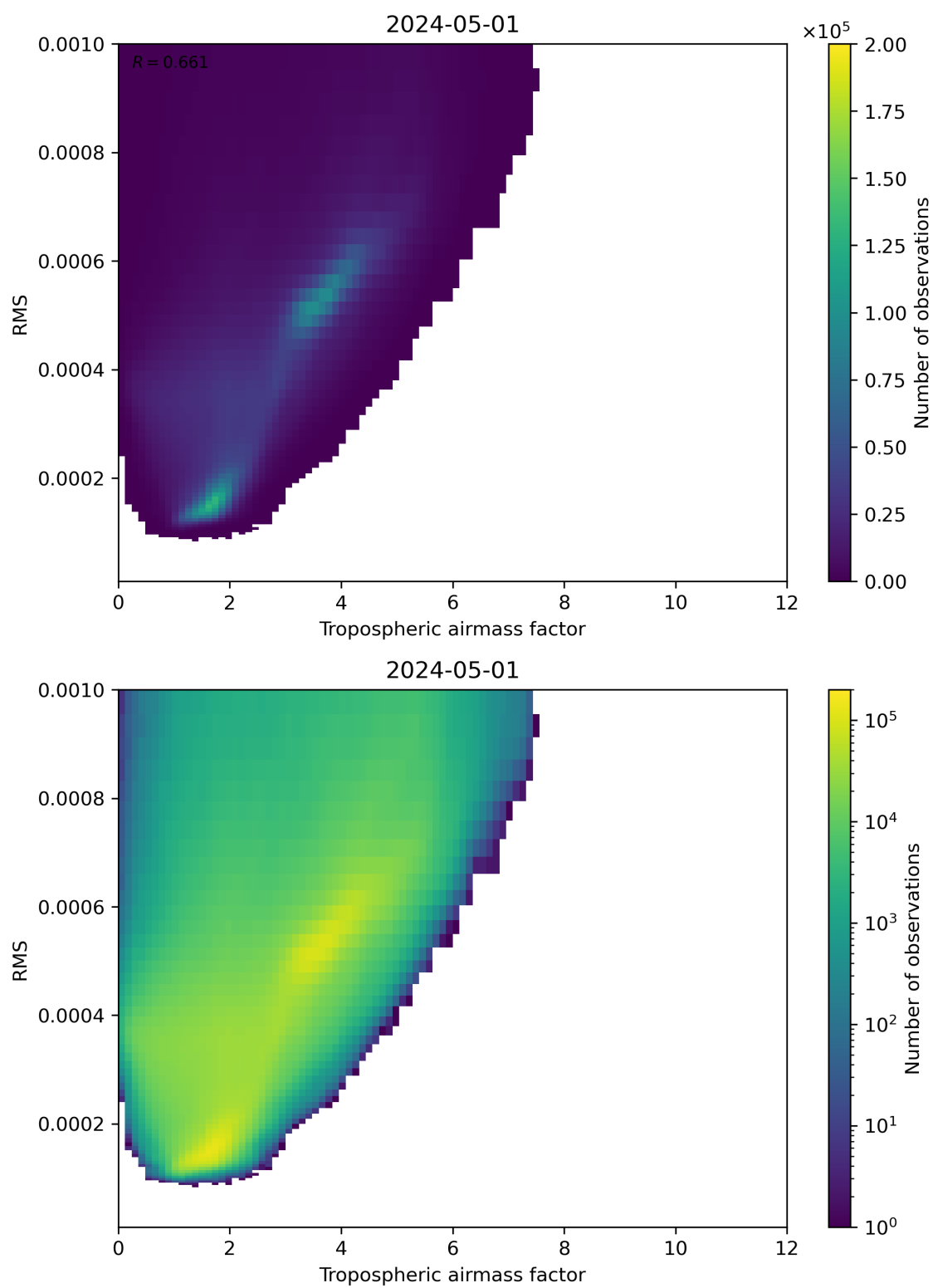
Figure 79: Scatter density plot of “Tropospheric airmass factor” against “RMS” for 2024-04-30 to 2024-05-02.
