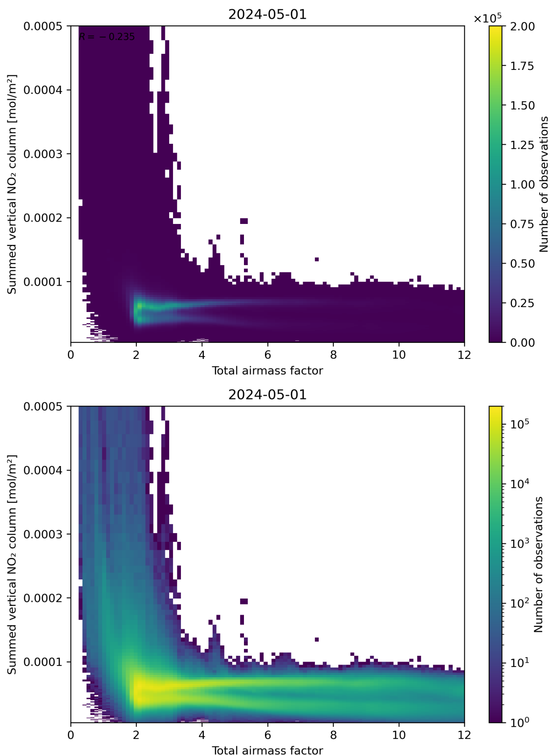
Figure 65: Scatter density plot of “Total airmass factor” against “Summed vertical NO 2 column” for 2024-04-30 to 2024-05-02.
