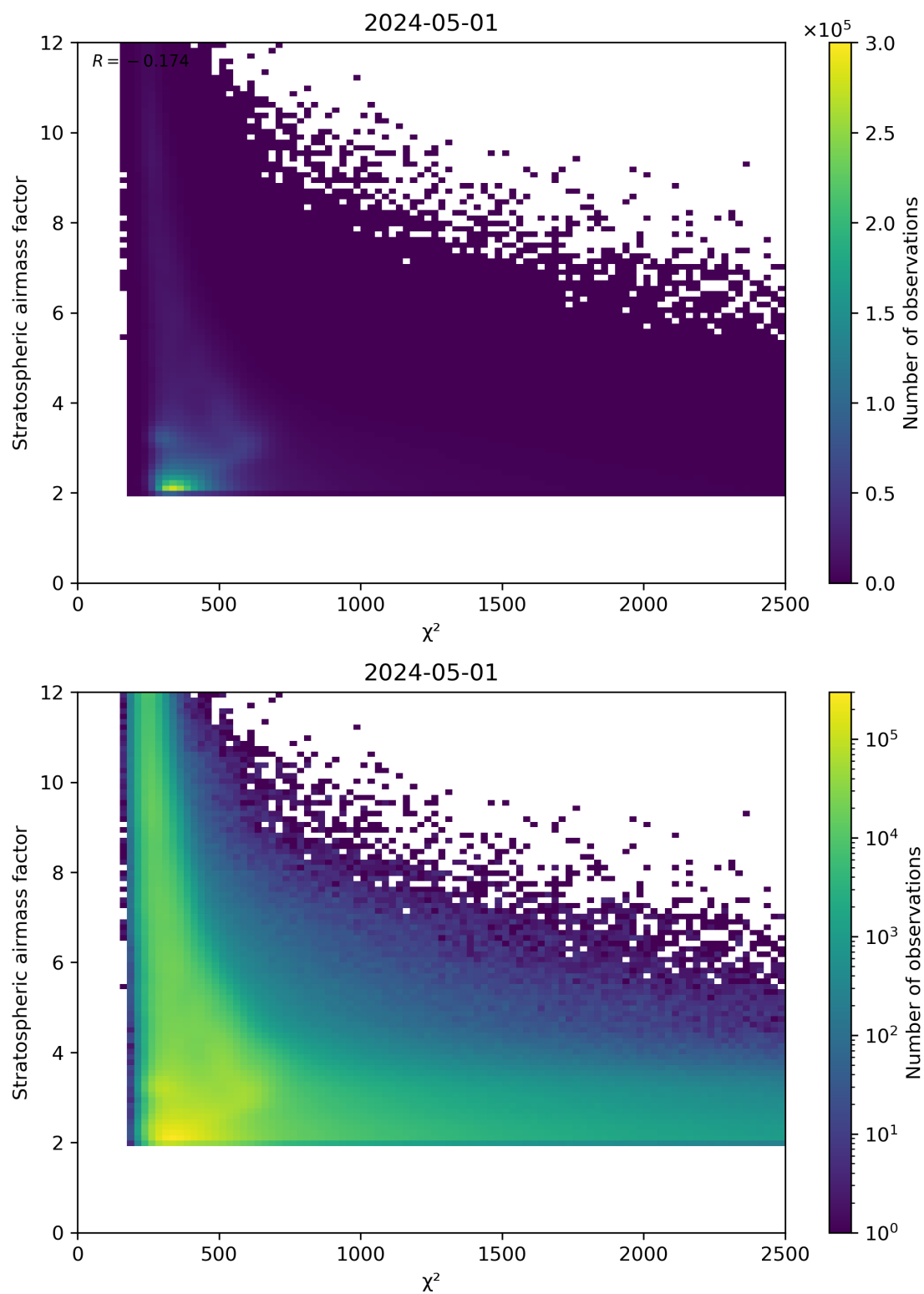
Figure 81: Scatter density plot of “ \chi^2 ” against “Stratospheric airmass factor” for 2024-04-30 to 2024-05-02.
