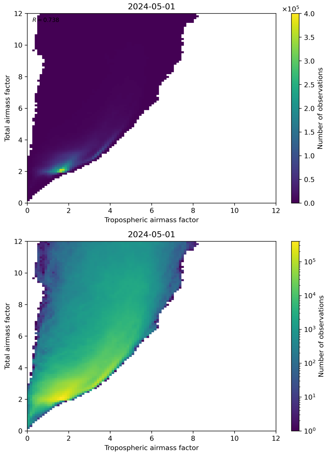
Figure 72: Scatter density plot of “Tropospheric airmass factor” against “Total airmass factor” for 2024-04-30 to 2024-05-02.
