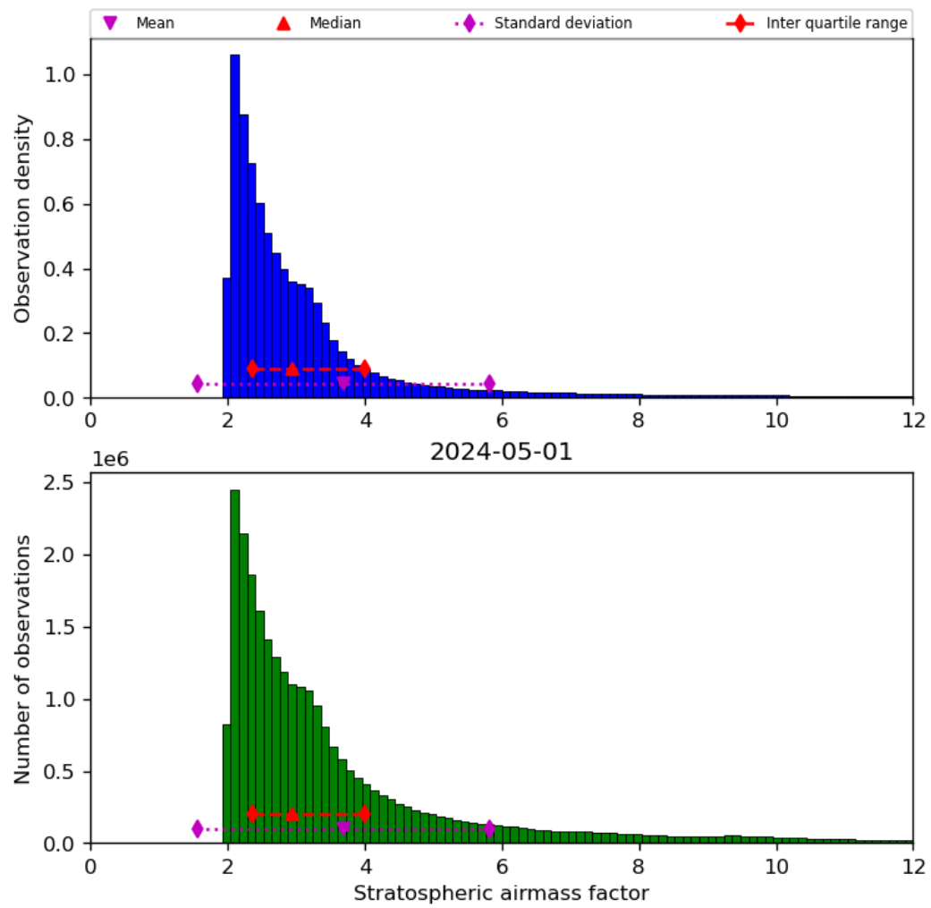
Figure 44: Histogram of “Stratospheric airmass factor” for 2024-04-30 to 2024-05-02
