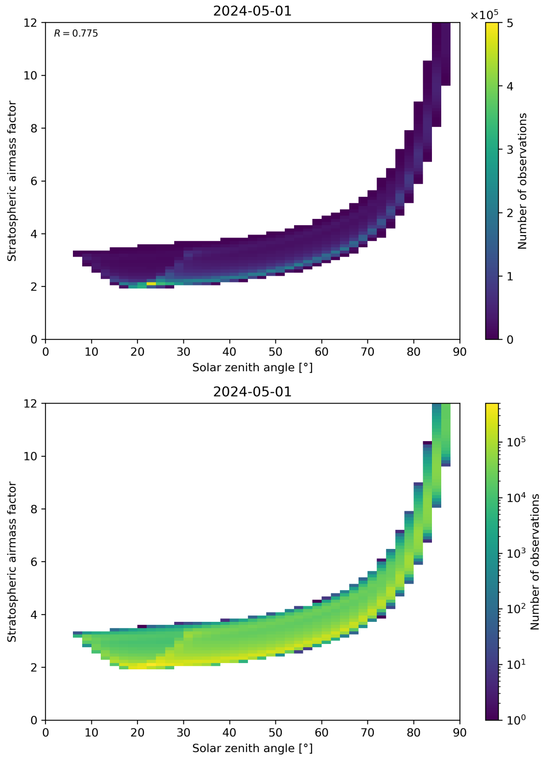
Figure 145: Scatter density plot of “Solar zenith angle” against “Stratospheric airmass factor” for 2024-04-30 to 2024-05-02.
