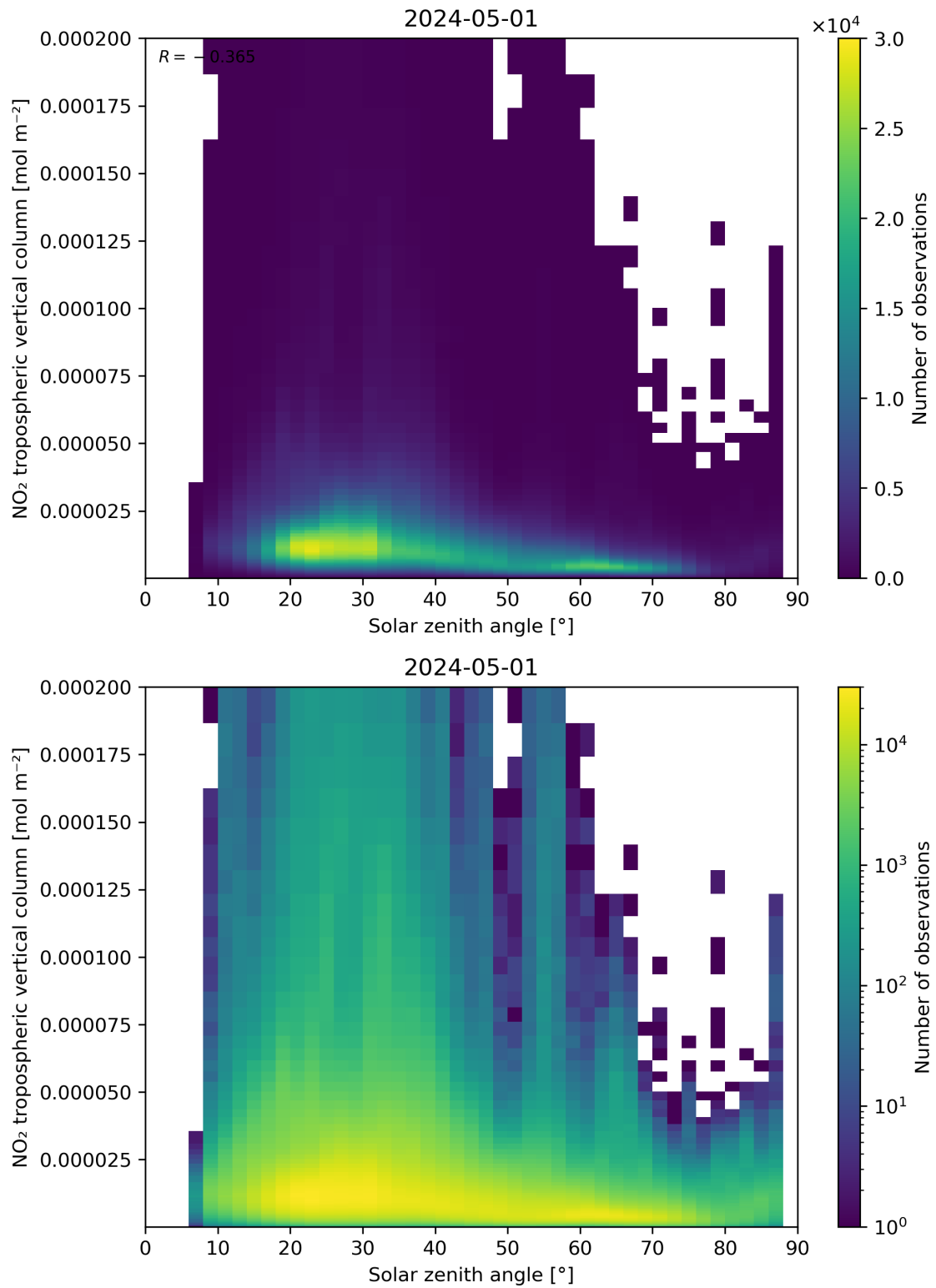
Figure 155: Scatter density plot of “Solar zenith angle” against “NO 2 tropospheric vertical column” for 2024-04-30 to 2024-05-02.
