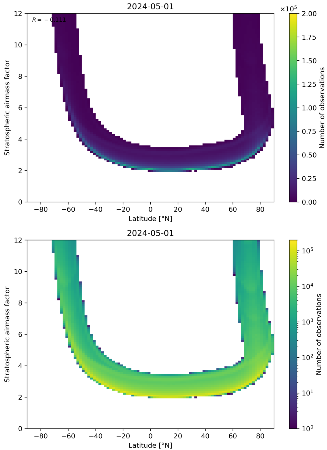
Figure 83: Scatter density plot of “Latitude” against “Stratospheric air mass factor” for 2024-04-30 to 2024-05-02.
