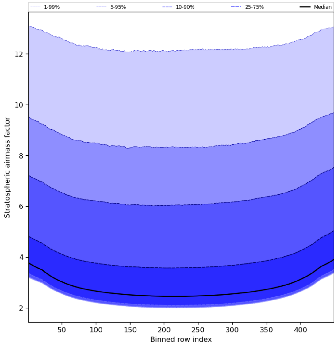
Figure 61: Along track statistics of “Stratospheric airmass factor” for 2024-04-30 to 2024-05-02
