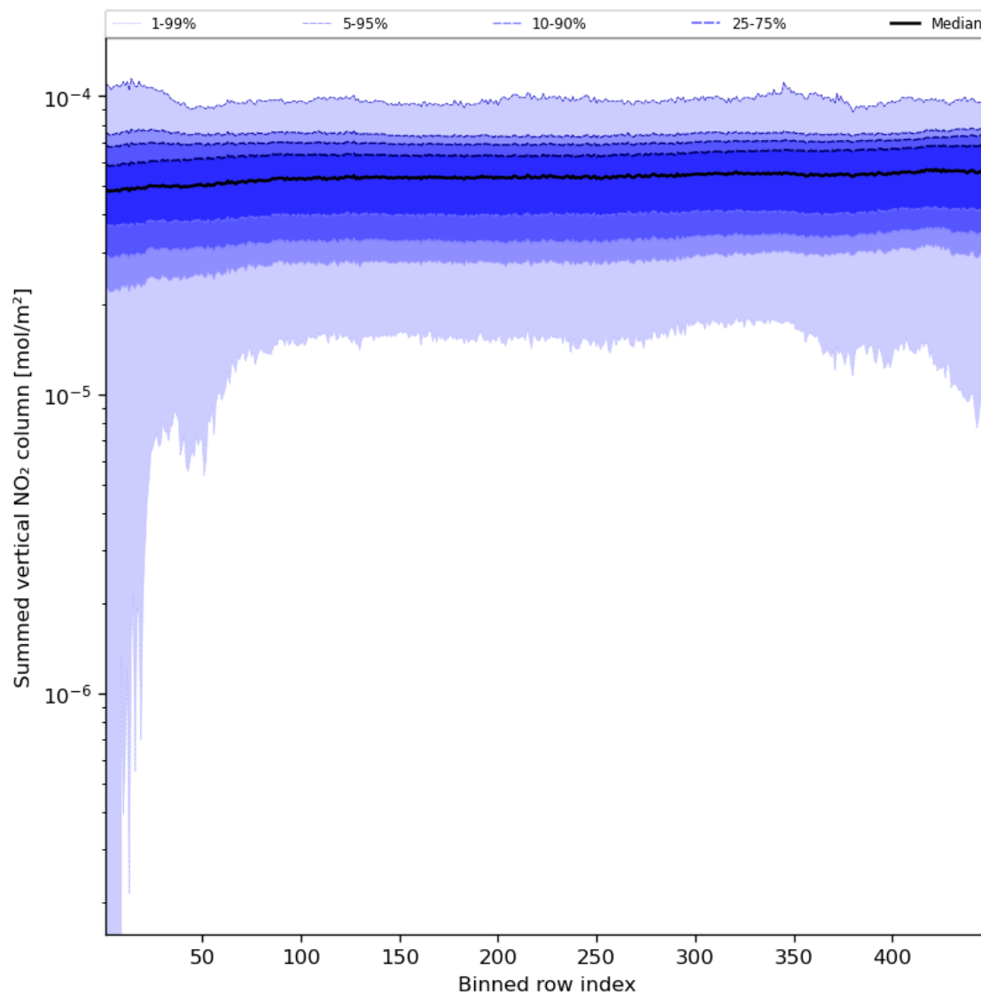
Figure 57: Along track statistics of “Summed vertical NO 2 column” for 2024-04-30 to 2024-05-02
