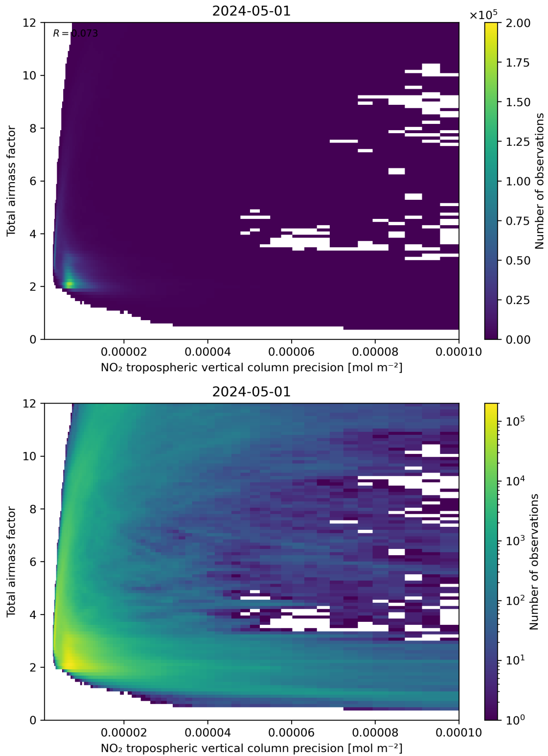
Figure 132: Scatter density plot of “NO 2 tropospheric vertical column precision” against “Total air mass factor” for 2024-04-30 to 2024-05-02.
