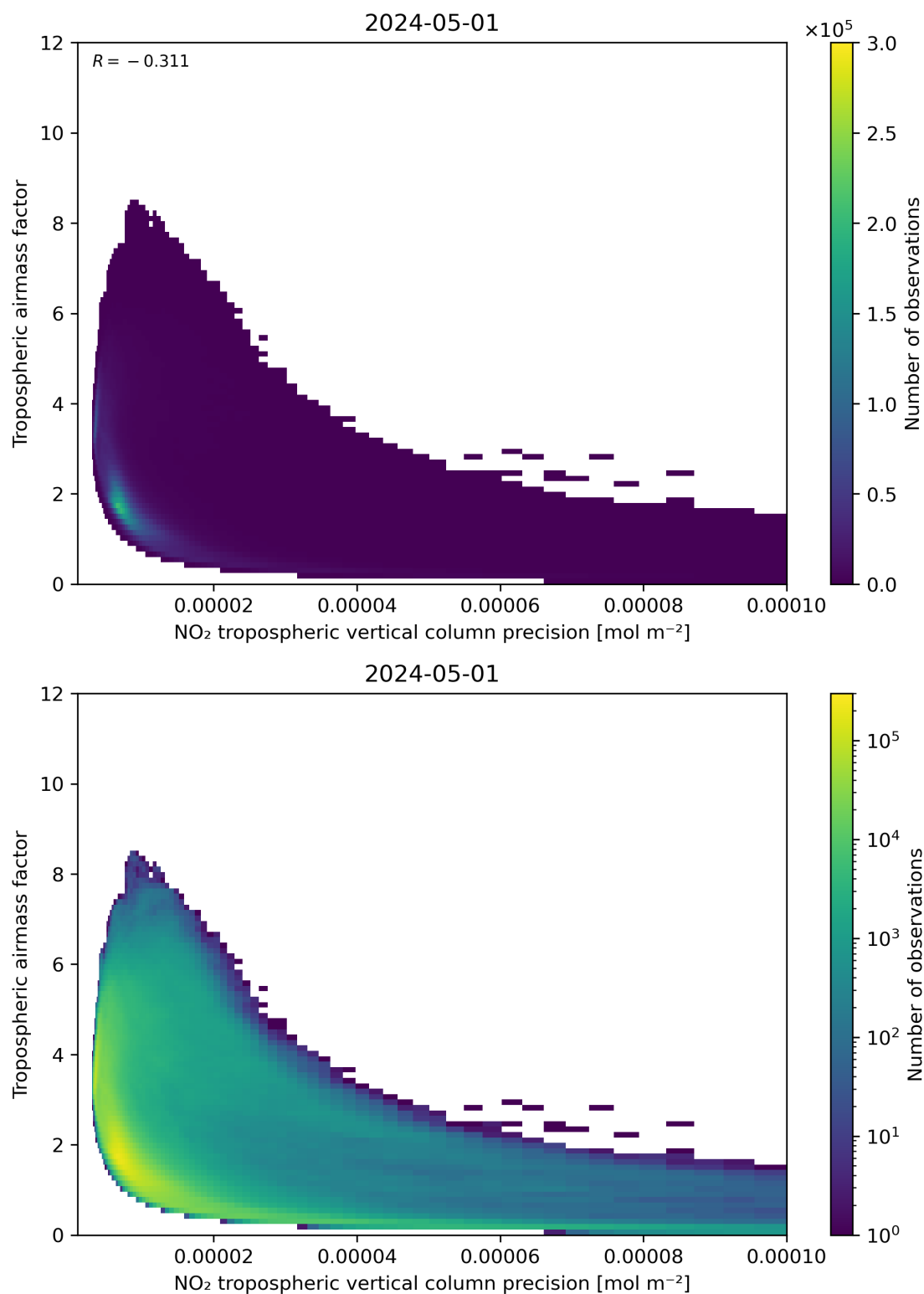
Figure 133: Scatter density plot of “NO 2 tropospheric vertical column precision” against “Tropospheric airmass factor” for 2024-04-30 to 2024-05-02.
