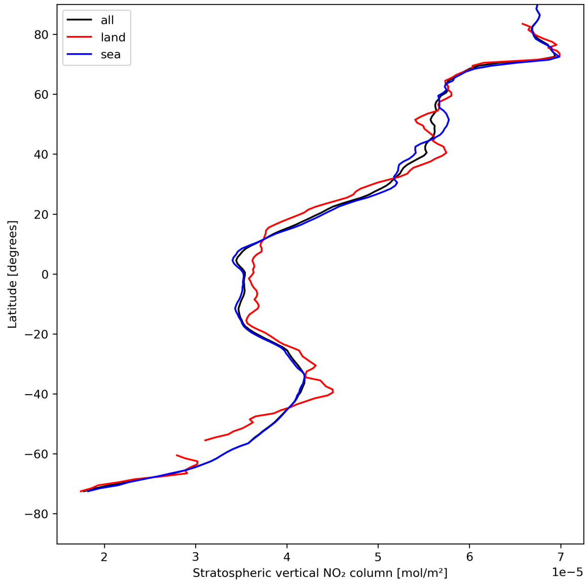
Figure 19: Zonal average of “Stratospheric vertical NO 2 column” for 2024-04-30 to 2024-05-02.
