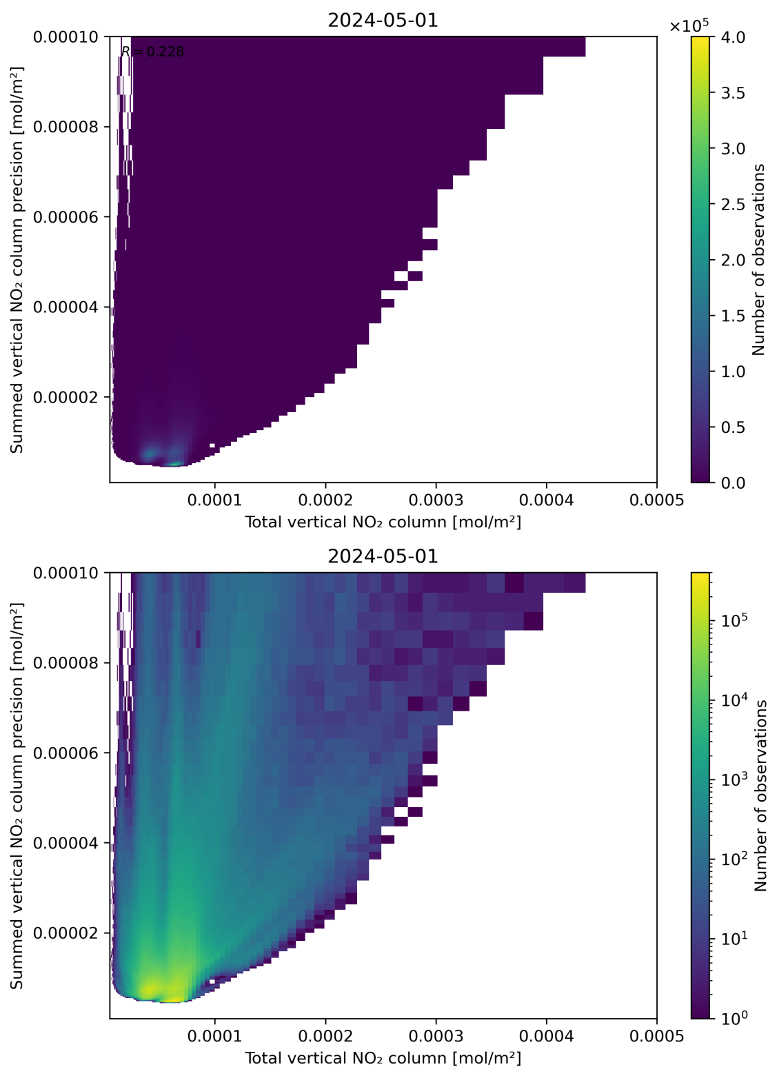
Figure 113: Scatter density plot of “Total vertical NO 2 column” against “Summed vertical NO 2 column precision” for 2024-04-30 to 2024-05-02.
