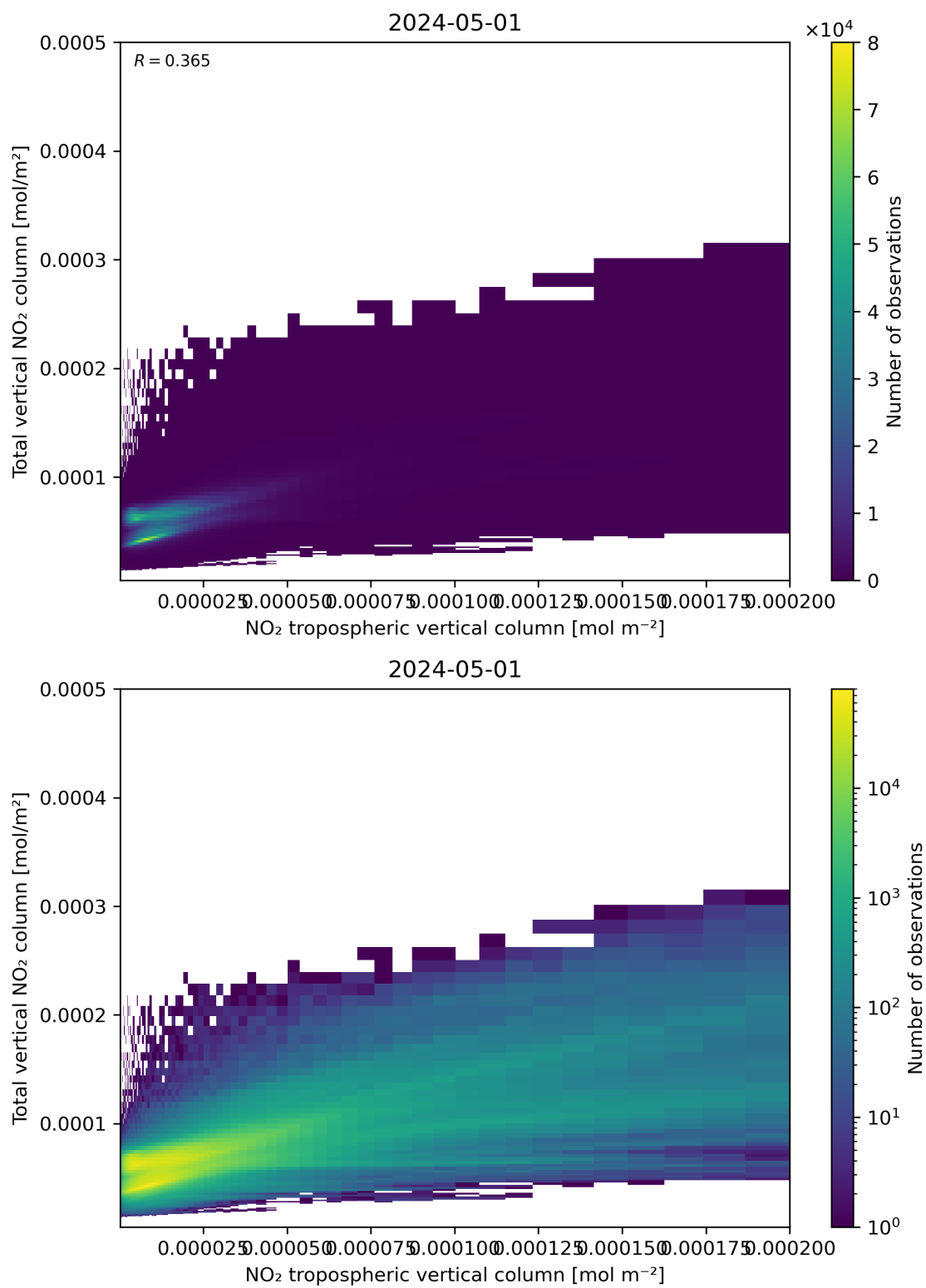
Figure 128: Scatter density plot of “NO 2 tropospheric vertical column” against “Total vertical NO 2 column” for 2024-04-30 to 2024-05-02.
