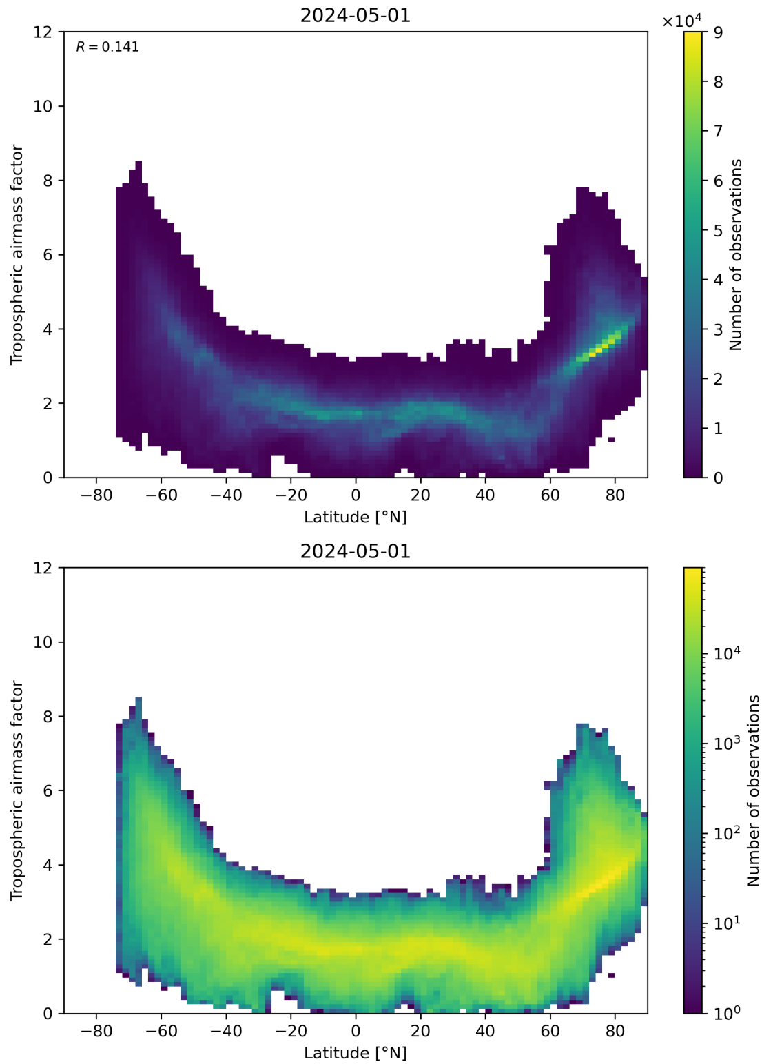
Figure 85: Scatter density plot of “Latitude” against “Tropospheric airmass factor” for 2024-04-30 to 2024-05-02.
