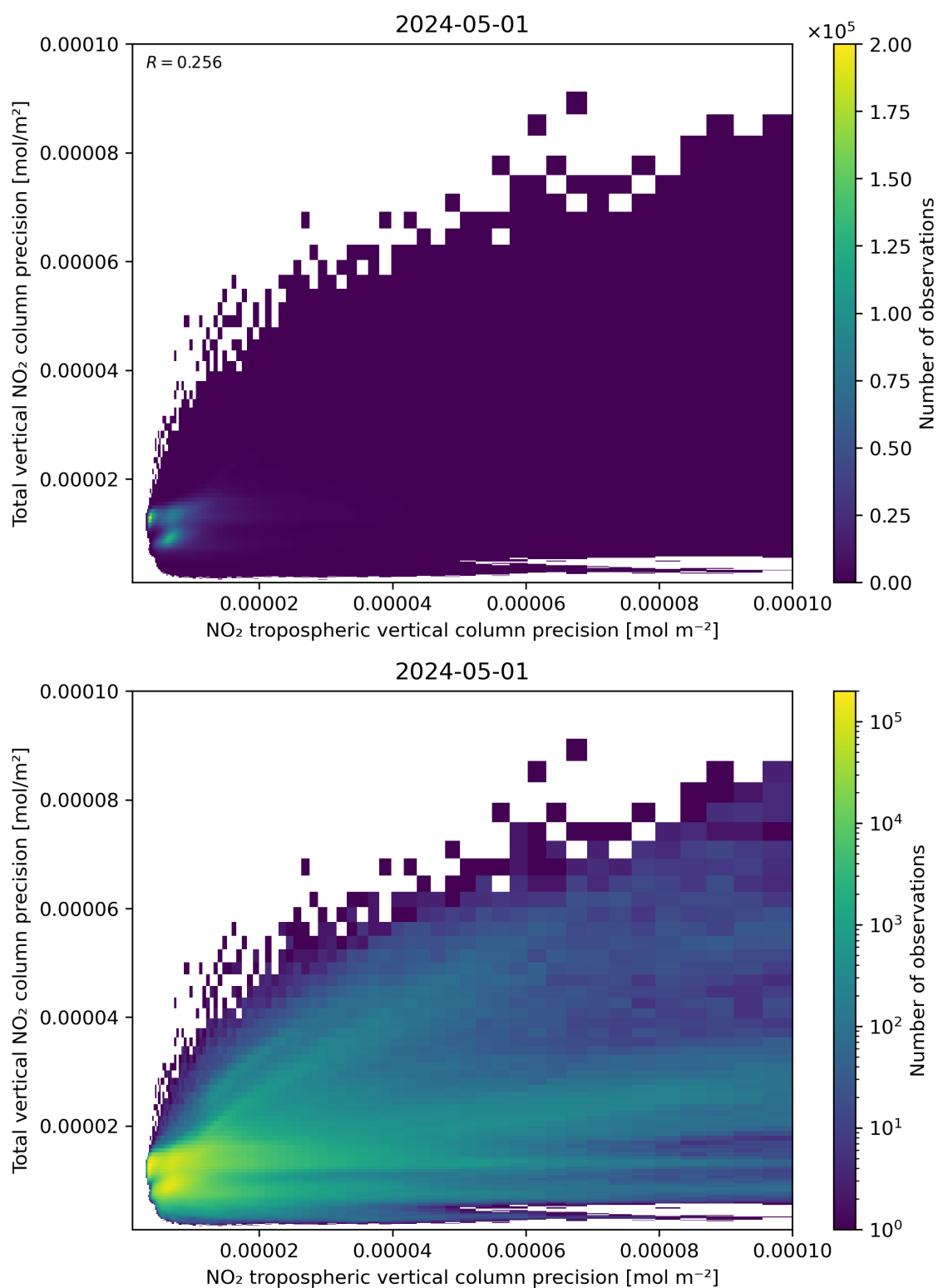
Figure 139: Scatter density plot of “NO 2 tropospheric vertical column precision” against “Total vertical NO 2 column precision” for 2024-04-30 to 2024-05-02.
