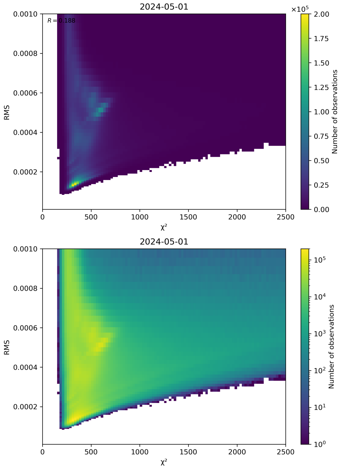
Figure 82: Scatter density plot of “ \chi^2 ” against “RMS” for 2024-04-30 to 2024-05-02.
