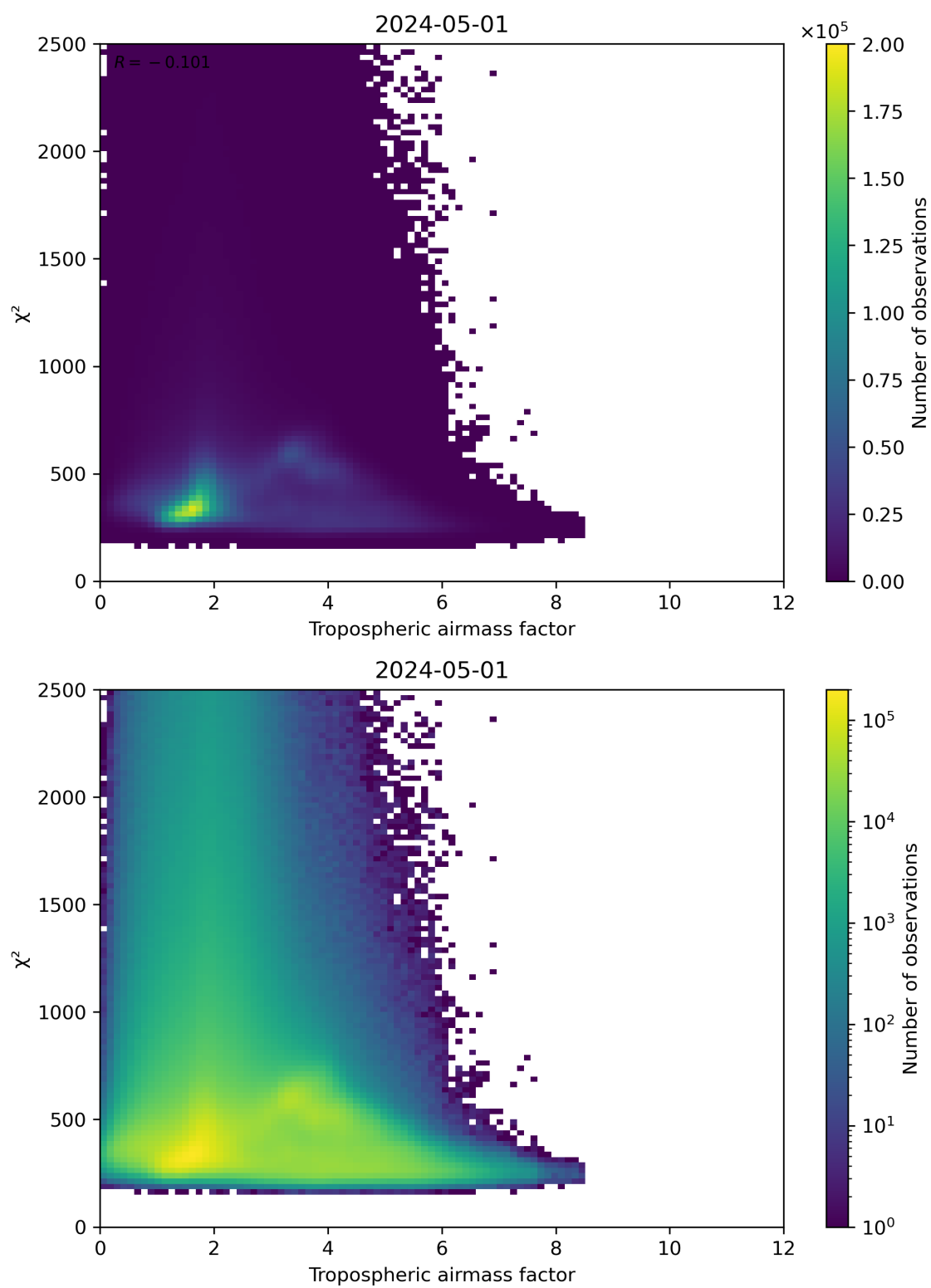
Figure 73: Scatter density plot of “Tropospheric airmass factor” against “ \chi^2 ” for 2024-04-30 to 2024-05-02.
