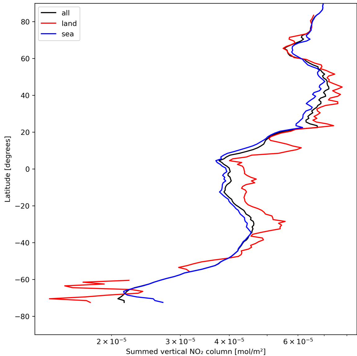
Figure 23: Zonal average of “Summed vertical NO 2 column” for 2024-04-30 to 2024-05-02.
