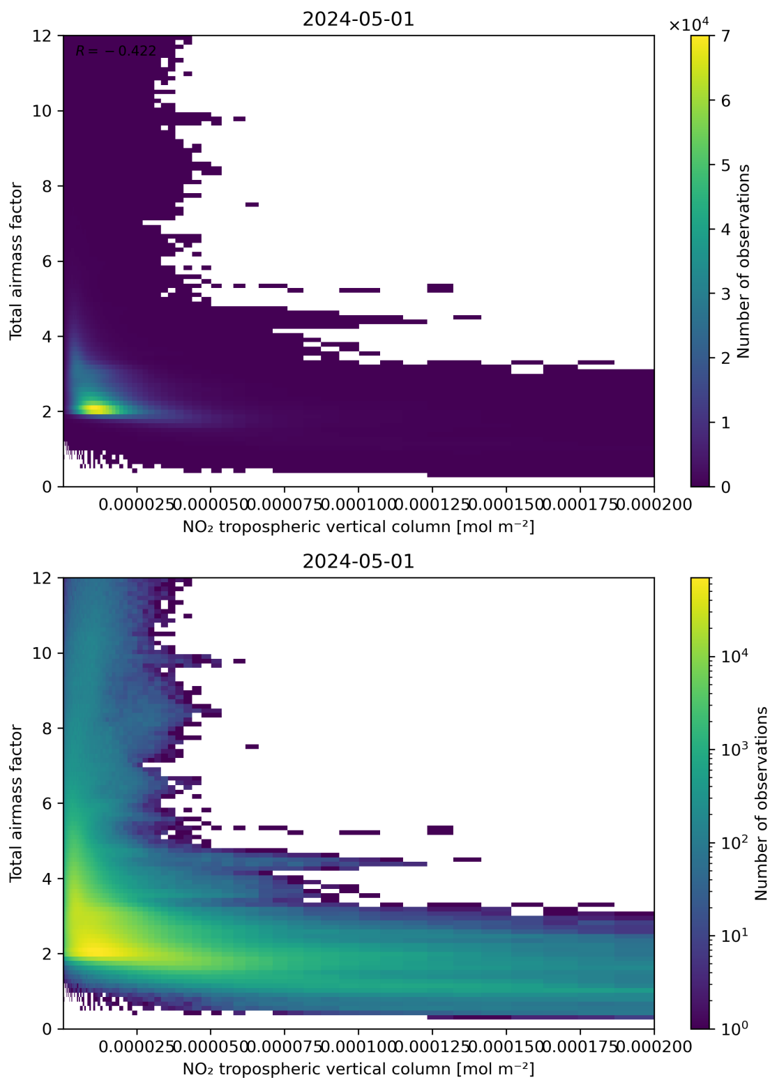
Figure 122: Scatter density plot of “NO 2 tropospheric vertical column” against “Total air mass factor” for 2024-04-30 to 2024-05-02.
