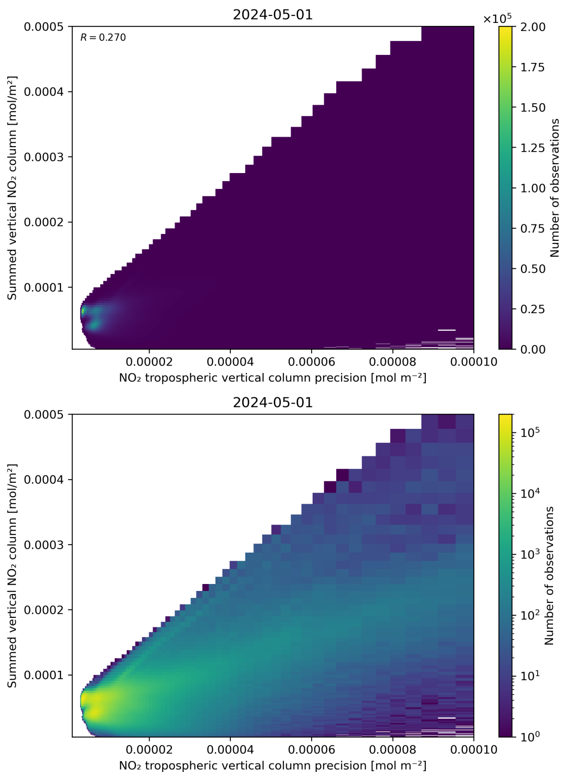
Figure 136: Scatter density plot of “NO 2 tropospheric vertical column precision” against “Summed vertical NO 2 column” for 2024-04-30 to 2024-05-02.
