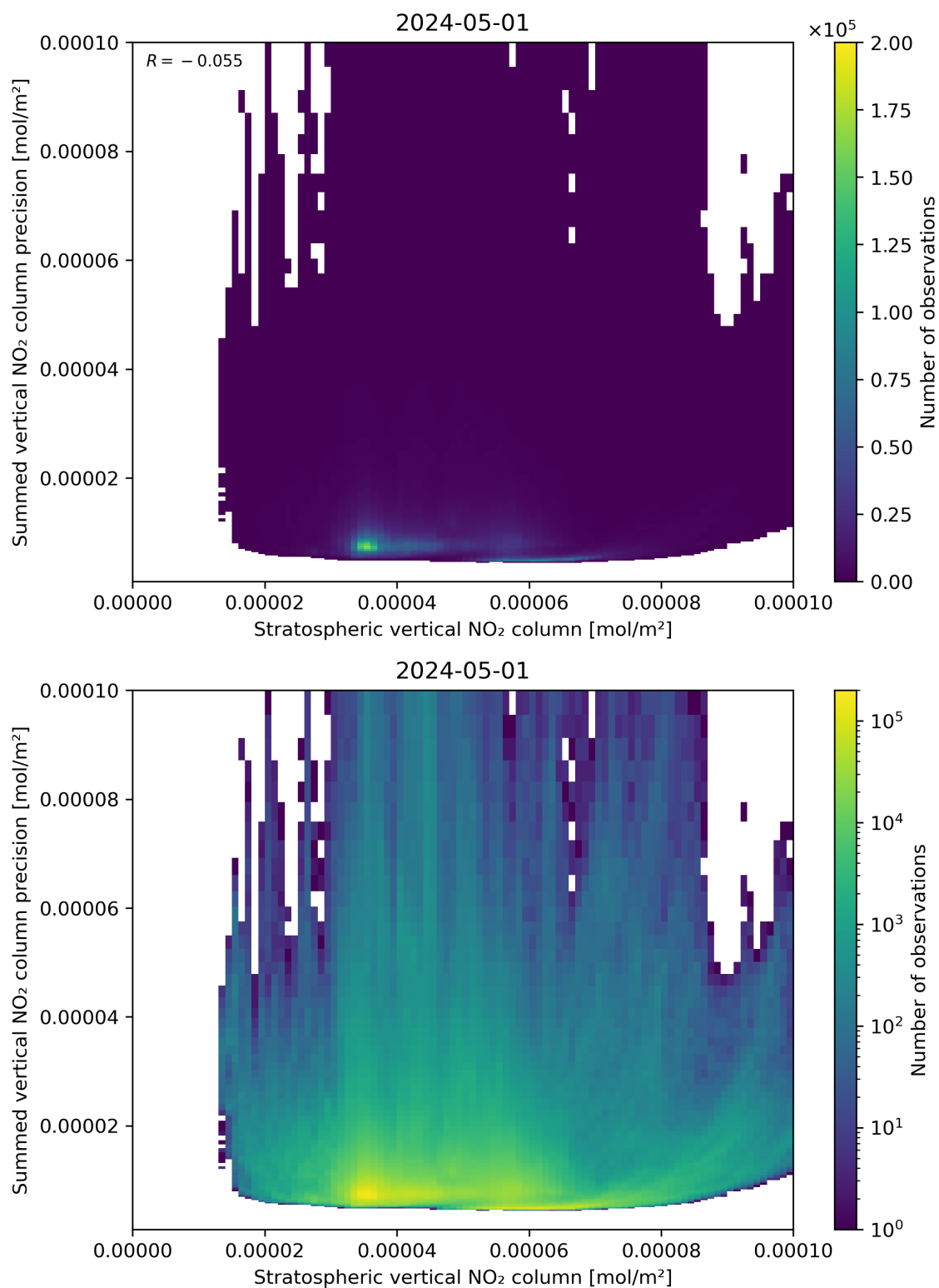
Figure 99: Scatter density plot of “Stratospheric vertical NO 2 column” against “Summed vertical NO 2 column precision” for 2024-04-30 to 2024-05-02.
