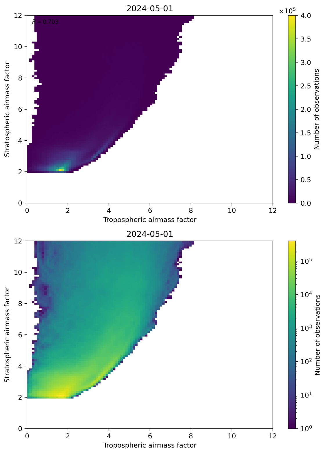
Figure 71: Scatter density plot of “Tropospheric airmass factor” against “Stratospheric airmass factor” for 2024-04-30 to 2024-05-02.
