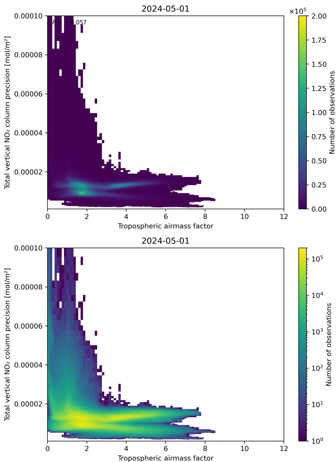
Figure 78: Scatter density plot of “Tropospheric air mass factor” against “Total vertical NO 2 column precision” for 2024-04-30 to 2024-05-02.
