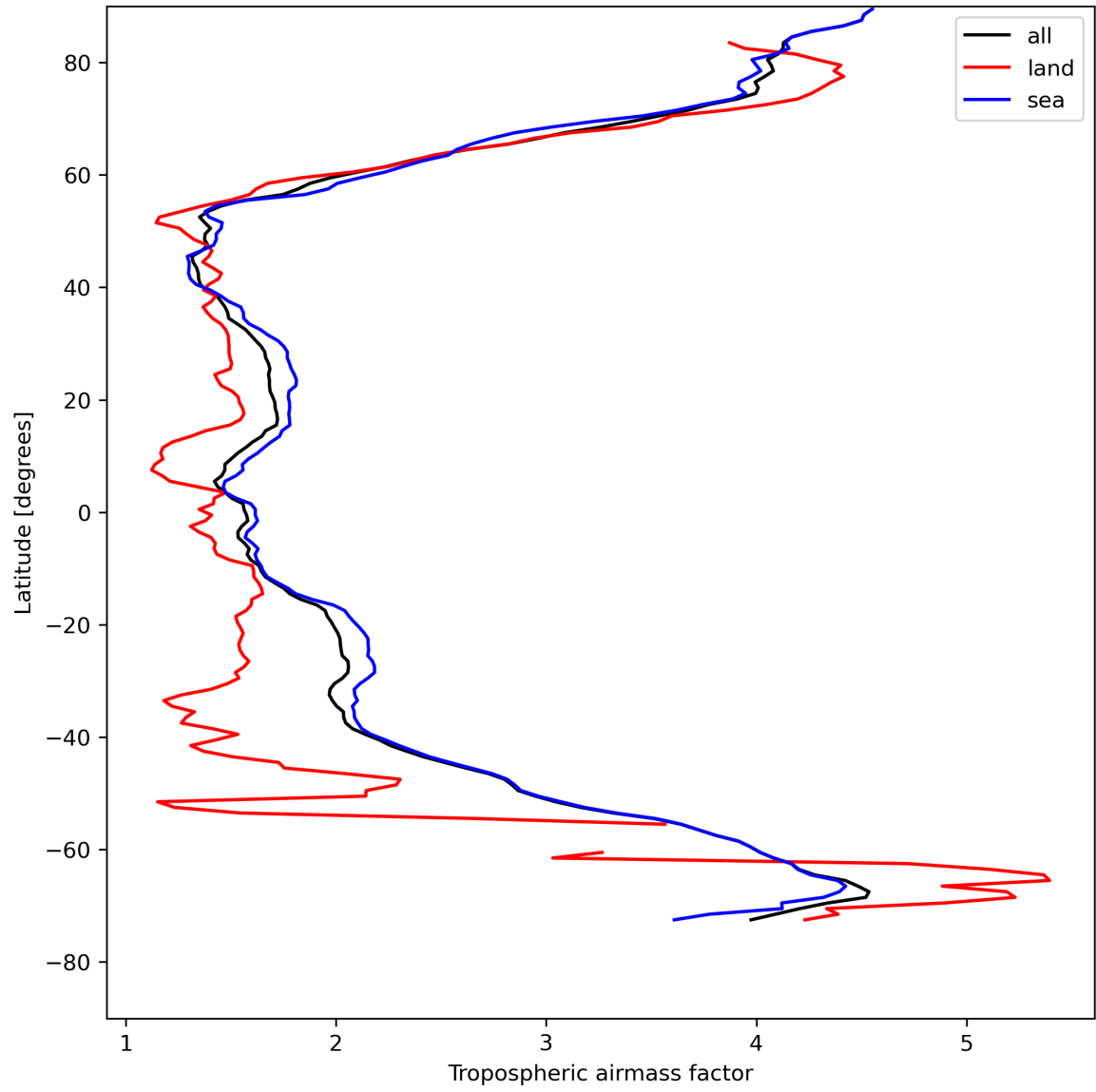
Figure 14: Zonal average of “Tropospheric airmass factor” for 2024-04-30 to 2024-05-02.
