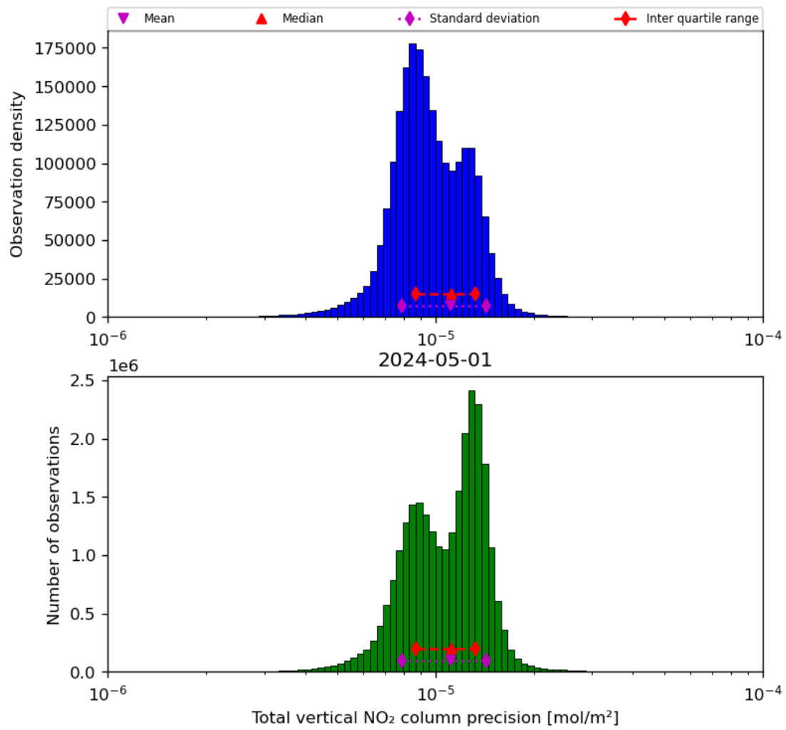
Figure 39: Histogram of "Total vertical NO 2 column precision" for 2024-04-30 to 2024-05-02
