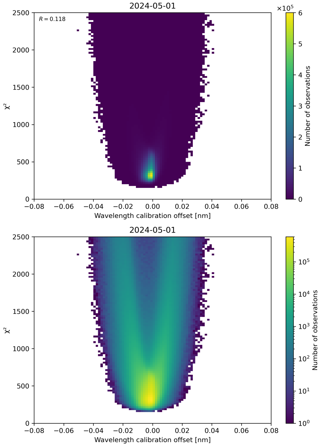
Figure 175: Scatter density plot of “Wavelength calibration offset” against “ \chi^2 ” for 2024-04-30 to 2024-05-02.
