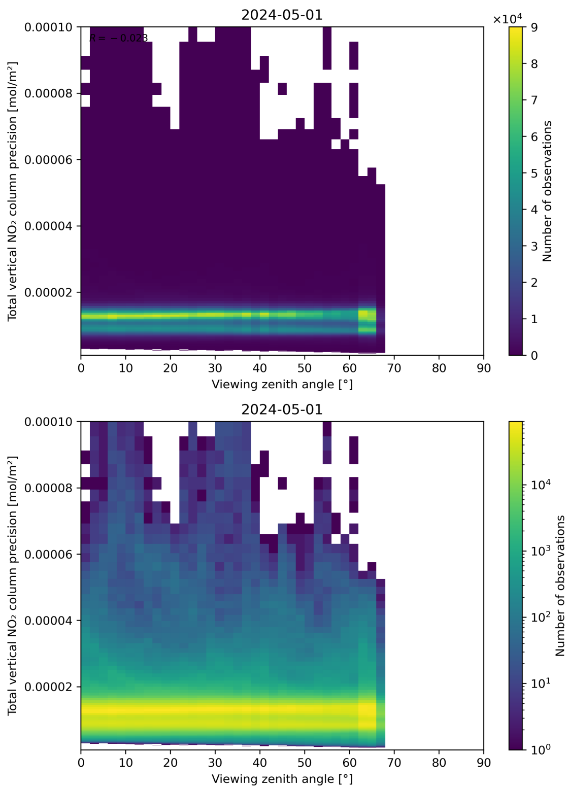
Figure 168: Scatter density plot of “Viewing zenith angle” against “Total vertical NO 2 column precision” for 2024-04-30 to 2024-05-02.
