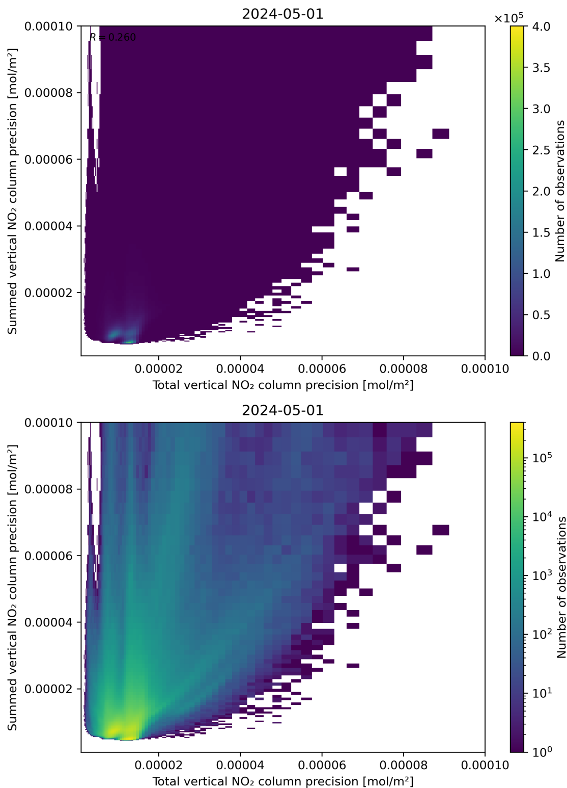
Figure 118: Scatter density plot of “Total vertical NO 2 column precision” against “Summed vertical NO 2 column precision” for 2024-04-30 to 2024-05-02.
