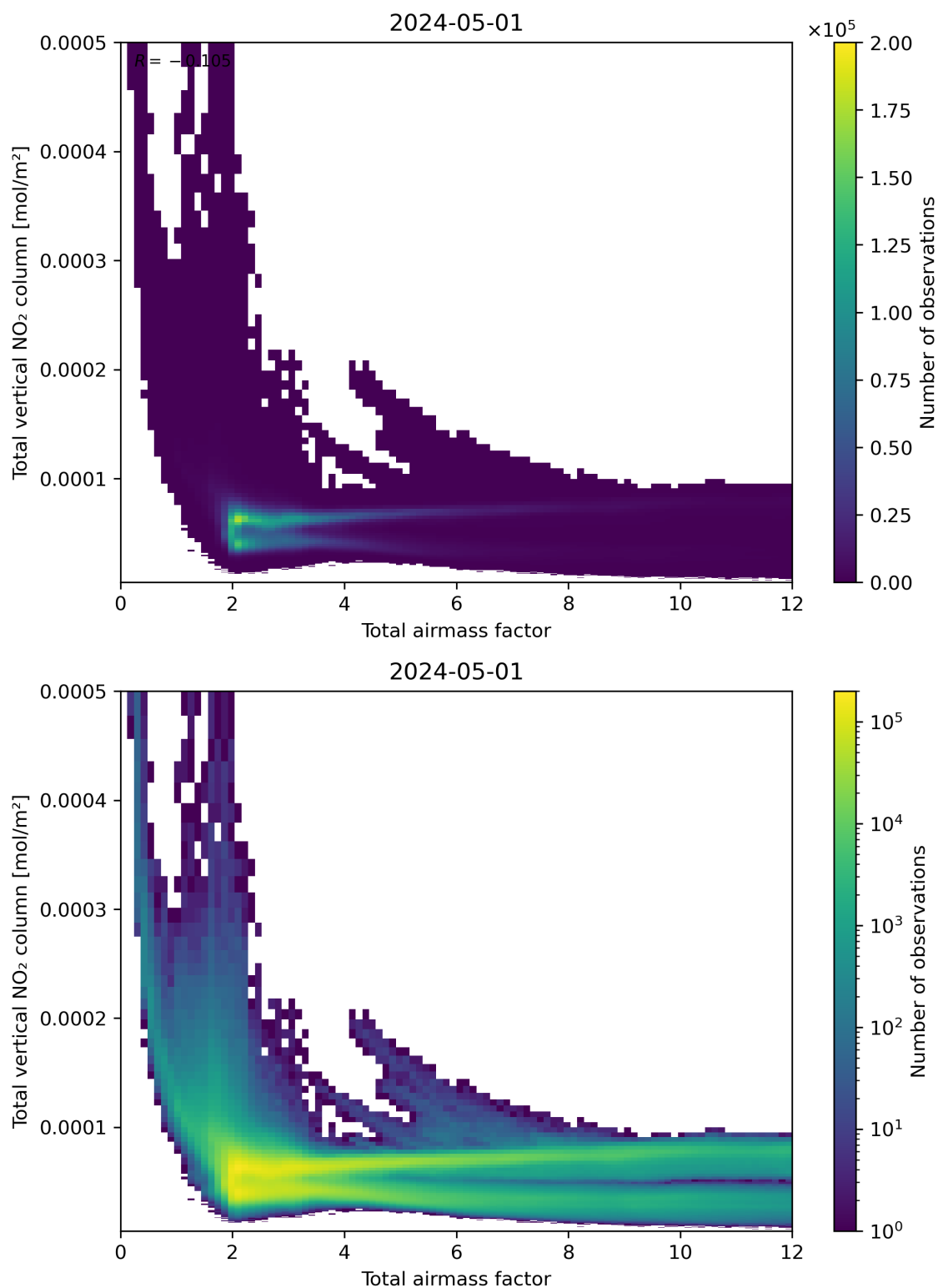
Figure 67: Scatter density plot of “Total airmass factor” against “Total vertical NO 2 column” for 2024-04-30 to 2024-05-02.
