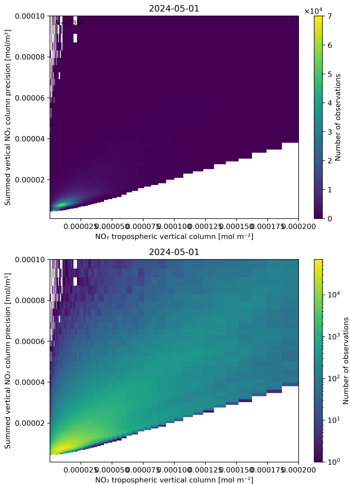
Figure 127: Scatter density plot of “NO 2 tropospheric vertical column” against “Summed vertical NO 2 column precision” for 2024-04-30 to 2024-05-02.
