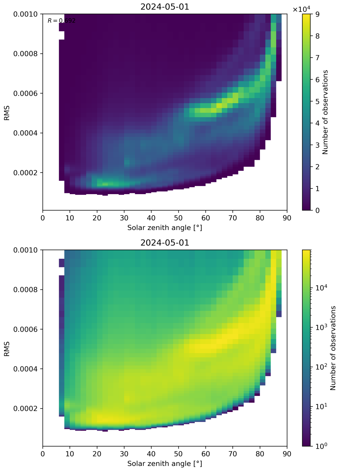
Figure 157: Scatter density plot of “Solar zenith angle” against “RMS” for 2024-04-30 to 2024-05-02.
