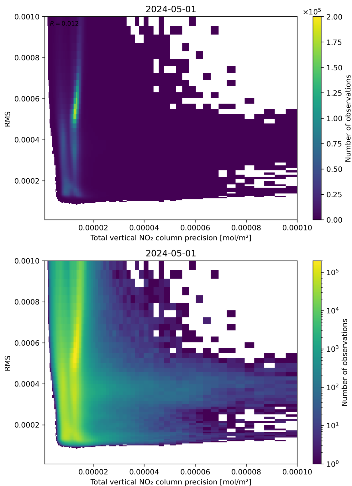
Figure 119: Scatter density plot of “Total vertical NO 2 column precision” against “RMS” for 2024-04-30 to 2024-05-02.
