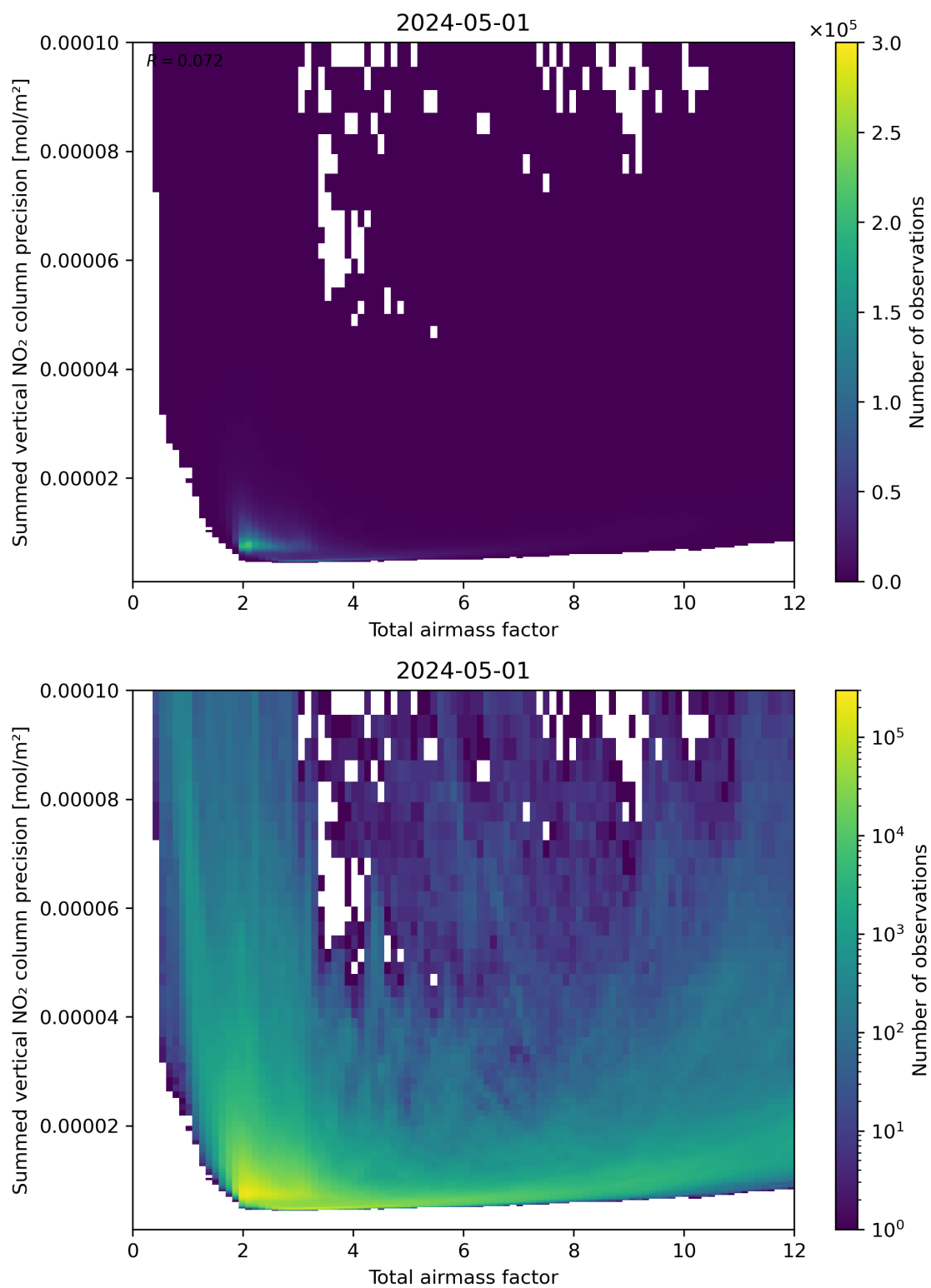
Figure 66: Scatter density plot of “Total airmass factor” against “Summed vertical NO 2 column precision” for 2024-04-30 to 2024-05-02.
