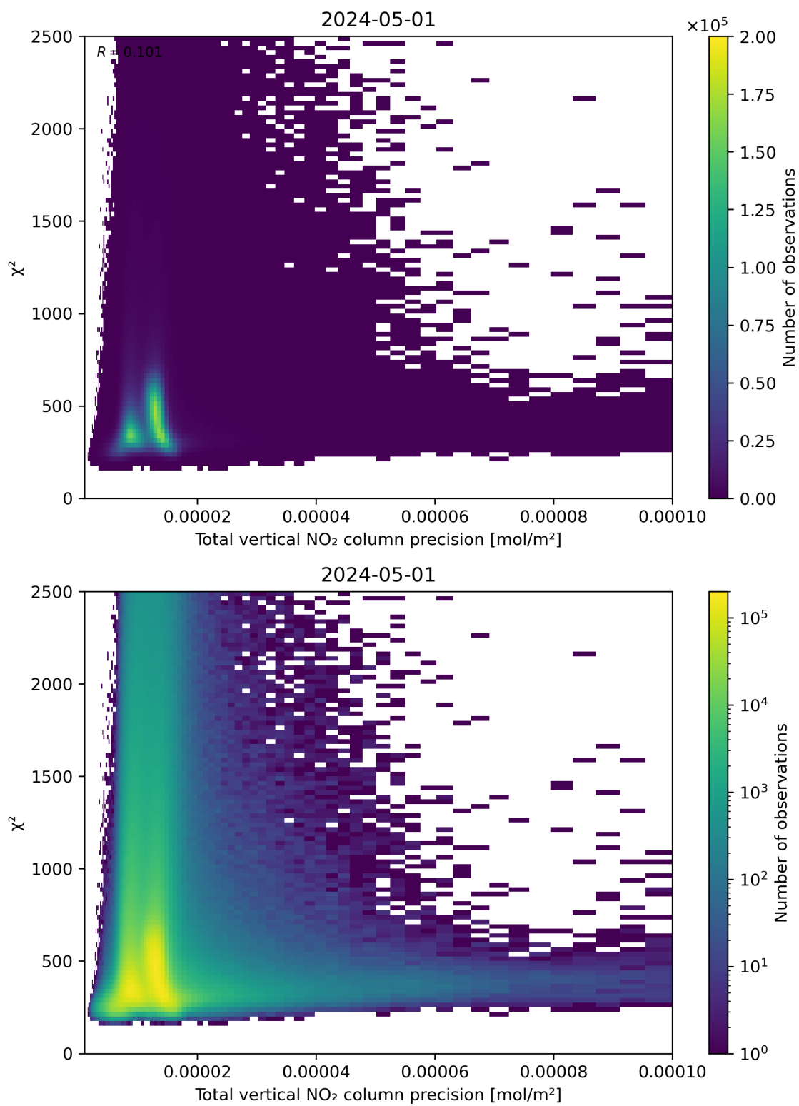
Figure 116: Scatter density plot of “Total vertical NO 2 column precision” against “ \chi^2 ” for 2024-04-30 to 2024-05-02.
