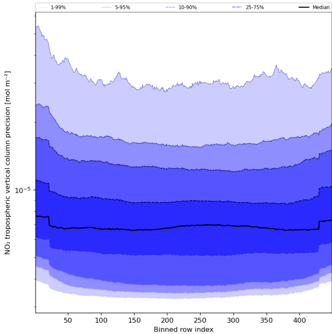
Figure 47: Along track statistics of “NO 2 tropospheric vertical column precision” for 2024-04-30 to 2024-05-02
