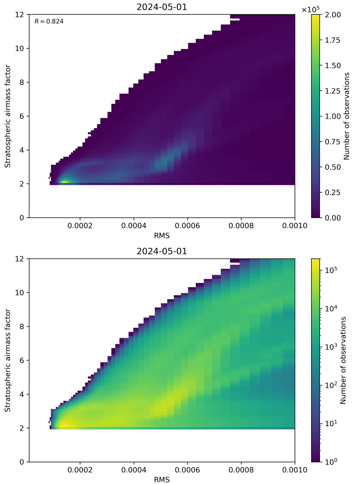
Figure 144: Scatter density plot of “RMS” against “Stratospheric airmass factor” for 2024-04-30 to 2024-05-02.
