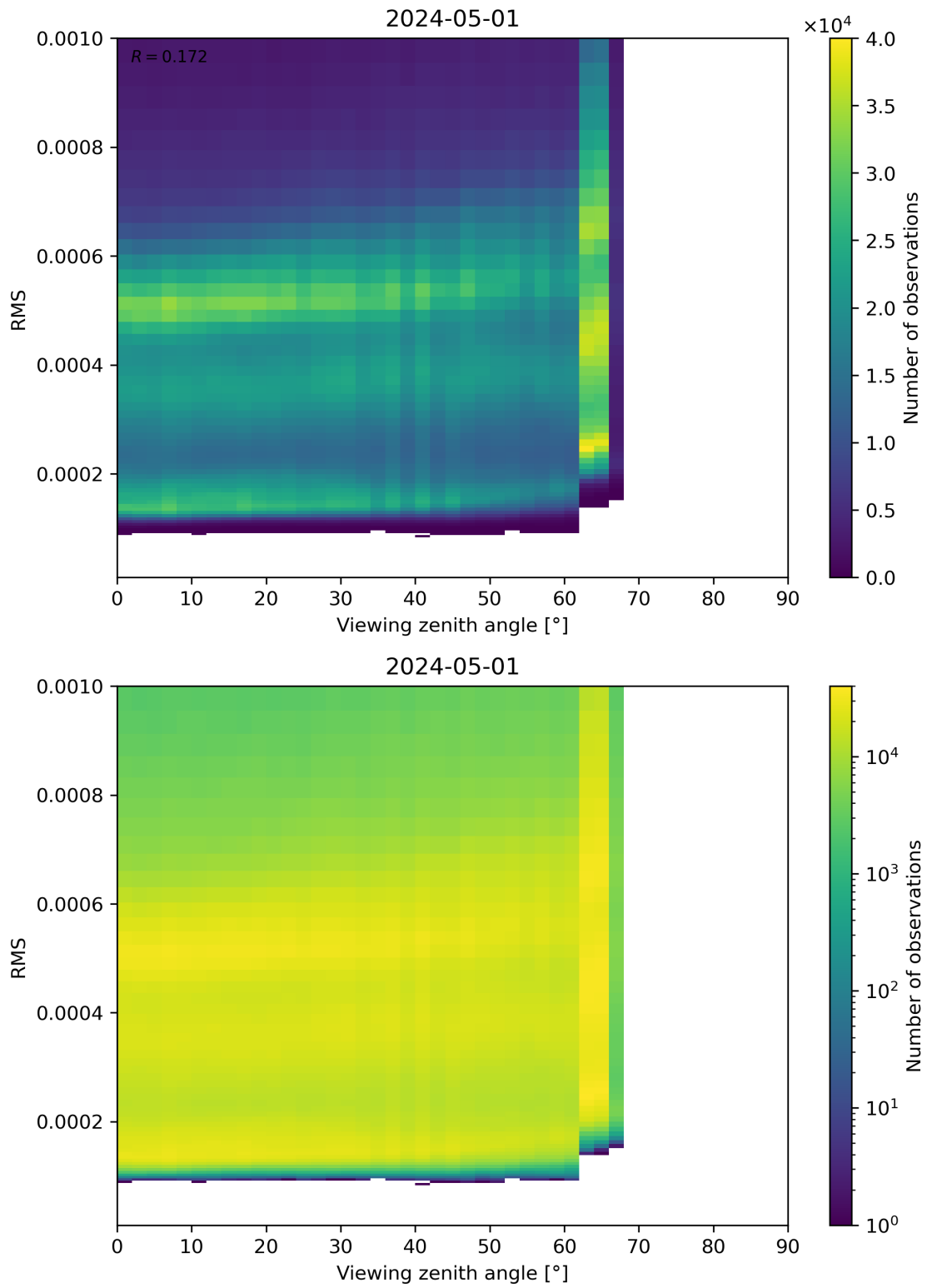
Figure 171: Scatter density plot of “Viewing zenith angle” against “RMS” for 2024-04-30 to 2024-05-02.
