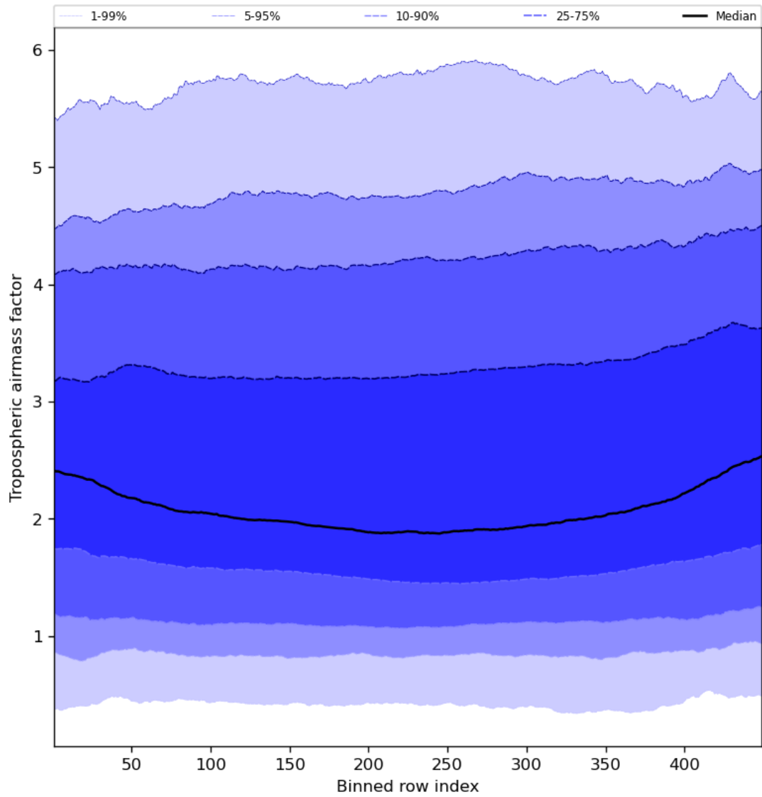
Figure 48: Along track statistics of “Tropospheric airmass factor” for 2024-04-30 to 2024-05-02
