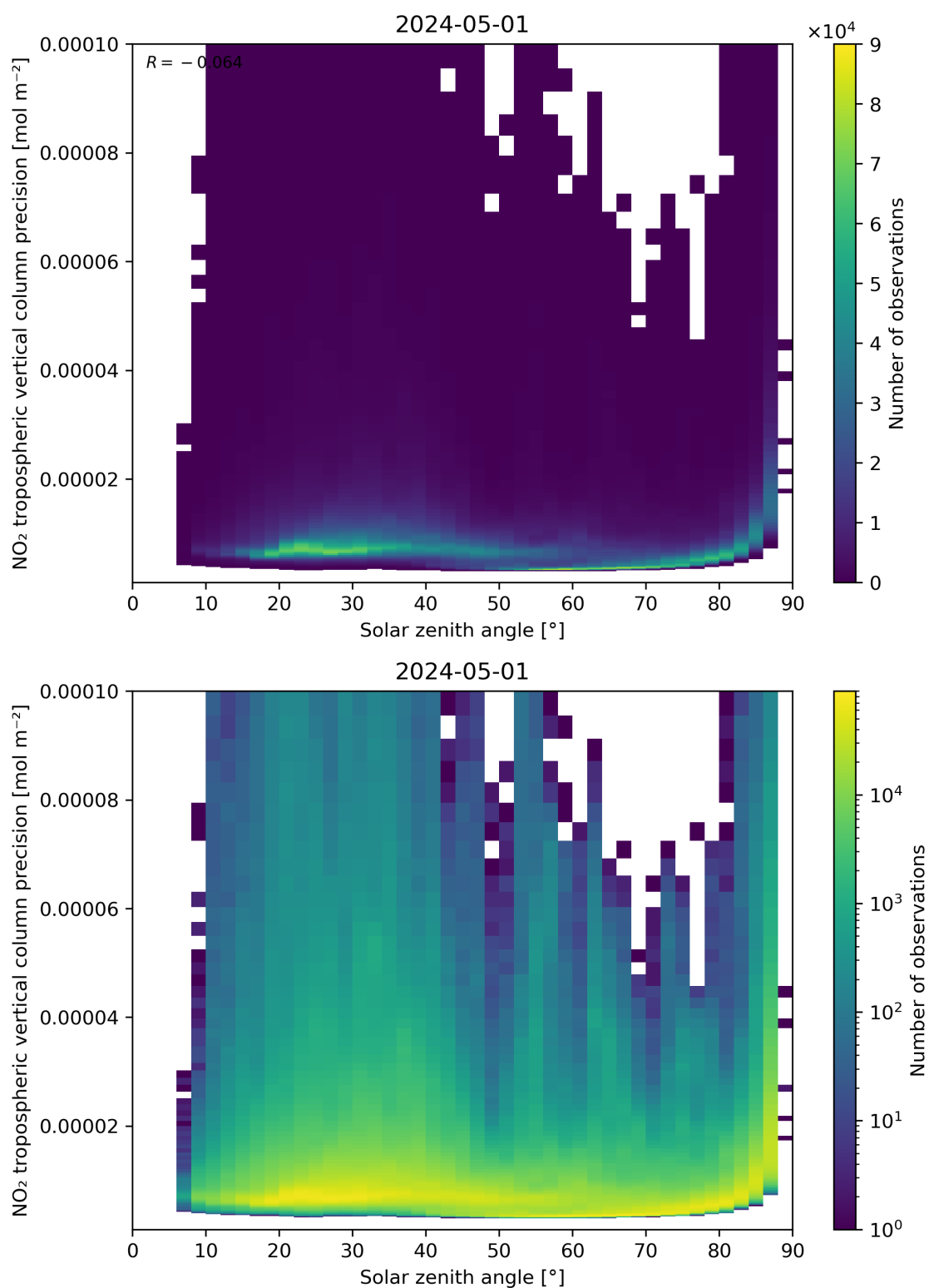
Figure 156: Scatter density plot of “Solar zenith angle” against “NO 2 tropospheric vertical column precision” for 2024-04-30 to 2024-05-02.
