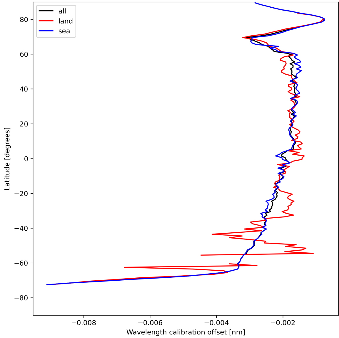
Figure 18: Zonal average of “Wavelength calibration offset” for 2024-04-30 to 2024-05-02.
