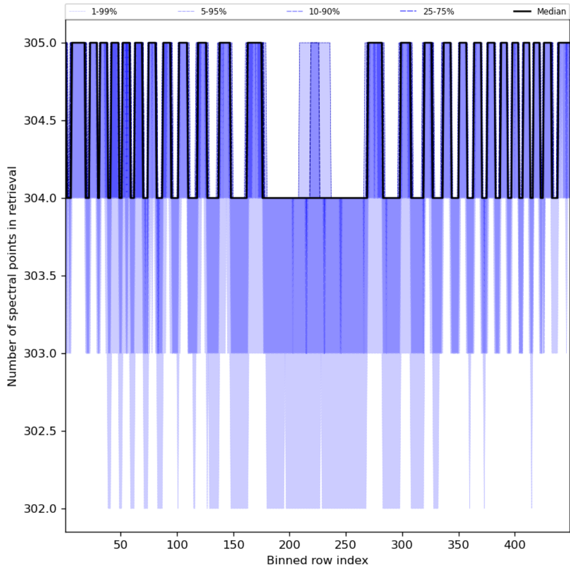
Figure 50: Along track statistics of “Number of spectral points in retrieval” for 2024-04-30 to 2024-05-02
