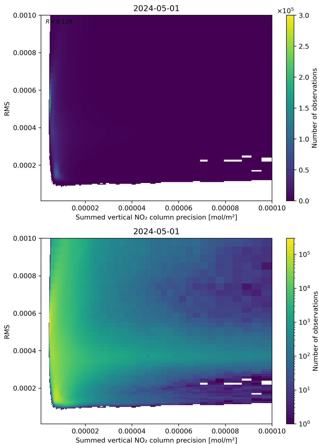
Figure 108: Scatter density plot of “Summed vertical NO 2 column precision” against “RMS” for 2024-04-30 to 2024-05-02.
