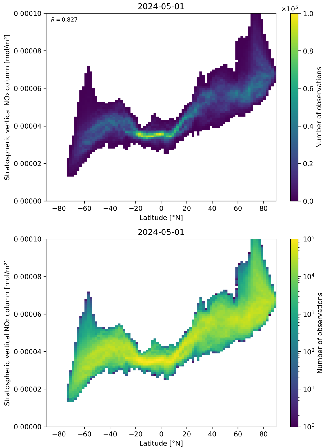
Figure 87: Scatter density plot of “Latitude” against “Stratospheric vertical NO 2 column” for 2024-04-30 to 2024-05-02.
