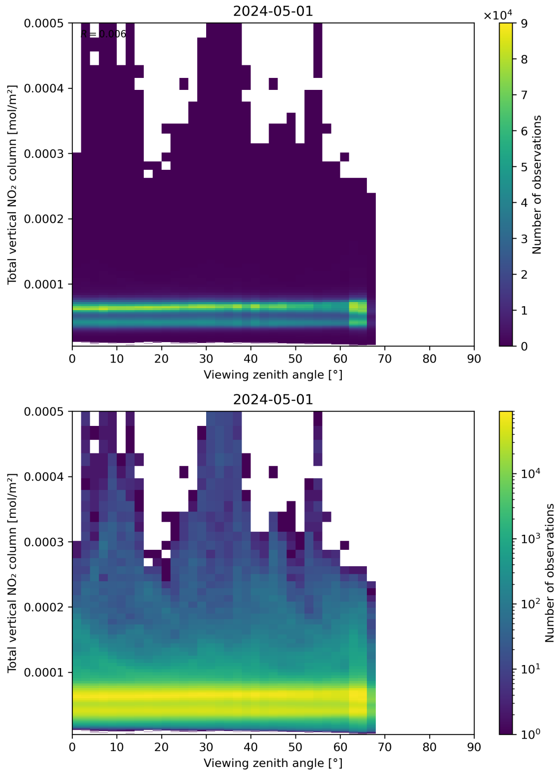
Figure 167: Scatter density plot of “Viewing zenith angle” against “Total vertical NO 2 column” for 2024-04-30 to 2024-05-02.
