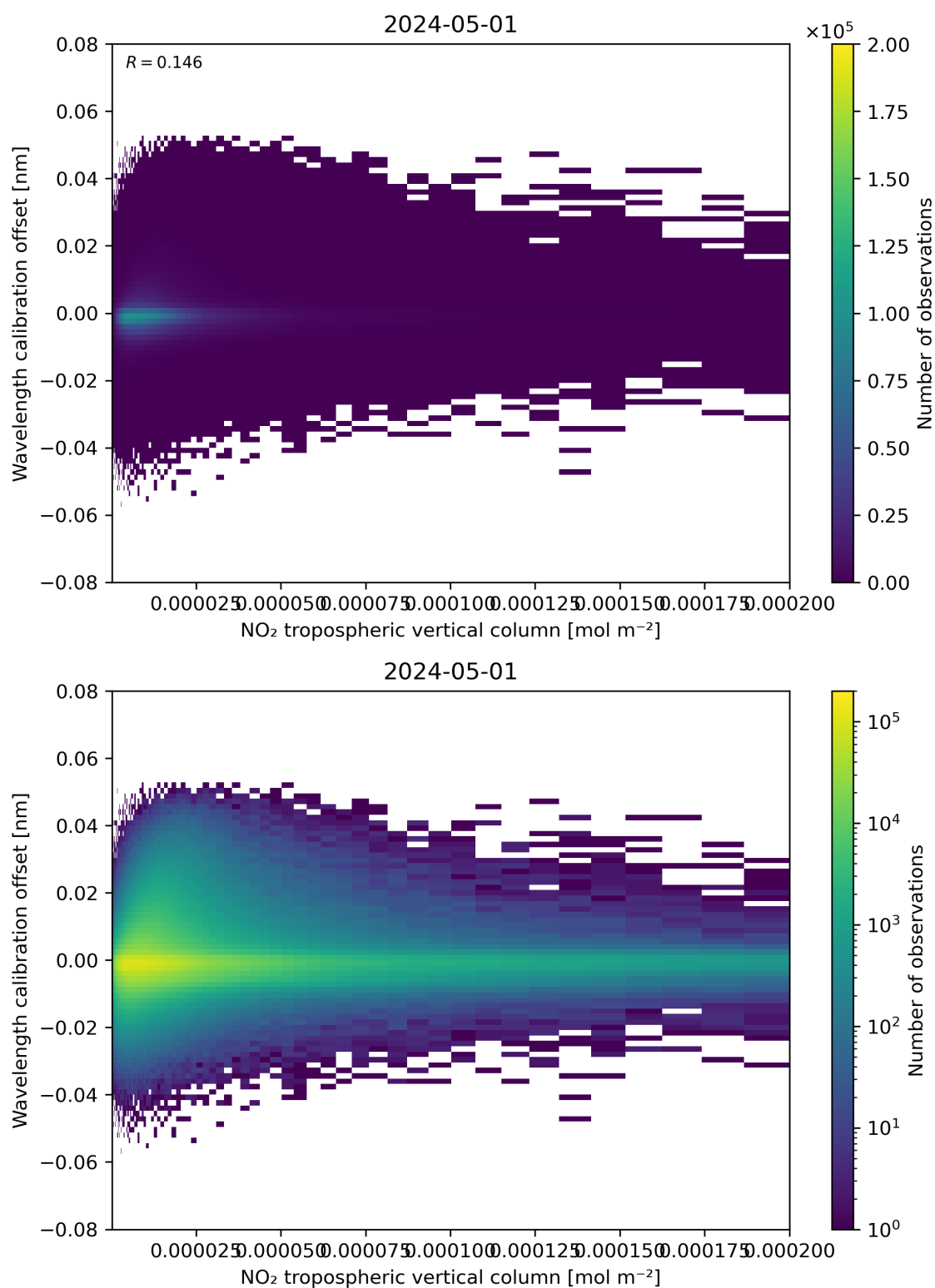
Figure 143: Scatter density plot of “NO 2 tropospheric vertical column” against “Wavelength calibration offset” for 2024-04-30 to 2024-05-02.
