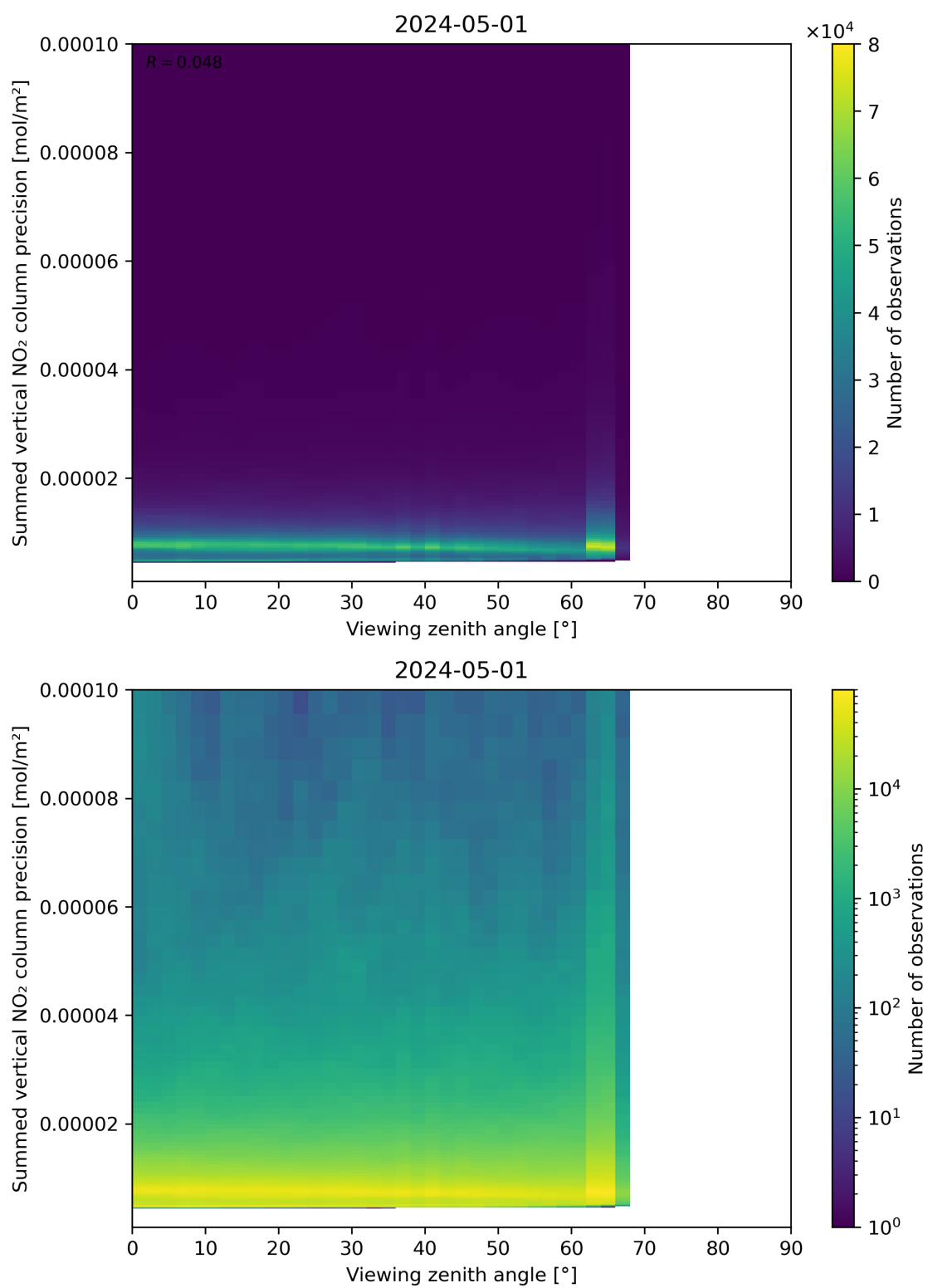
Figure 166: Scatter density plot of “Viewing zenith angle” against “Summed vertical NO 2 column precision” for 2024-04-30 to 2024-05-02.
