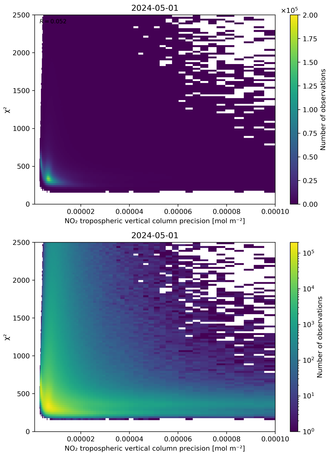
Figure 134: Scatter density plot of “NO 2 tropospheric vertical column precision” against “ \chi^2 ” for 2024-04-30 to 2024-05-02.
