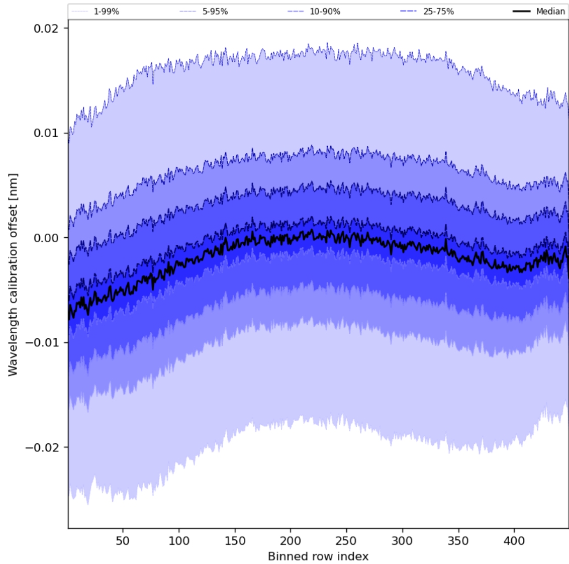
Figure 52: Along track statistics of “Wavelength calibration offset” for 2024-04-30 to 2024-05-02
