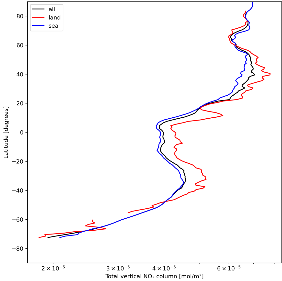
Figure 21: Zonal average of “Total vertical NO 2 column” for 2024-04-30 to 2024-05-02.
