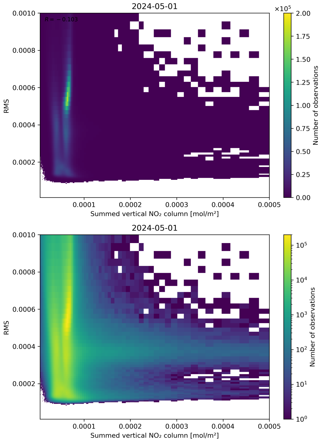
Figure 109: Scatter density plot of “Summed vertical NO 2 column” against “RMS” for 2024-04-30 to 2024-05-02.
