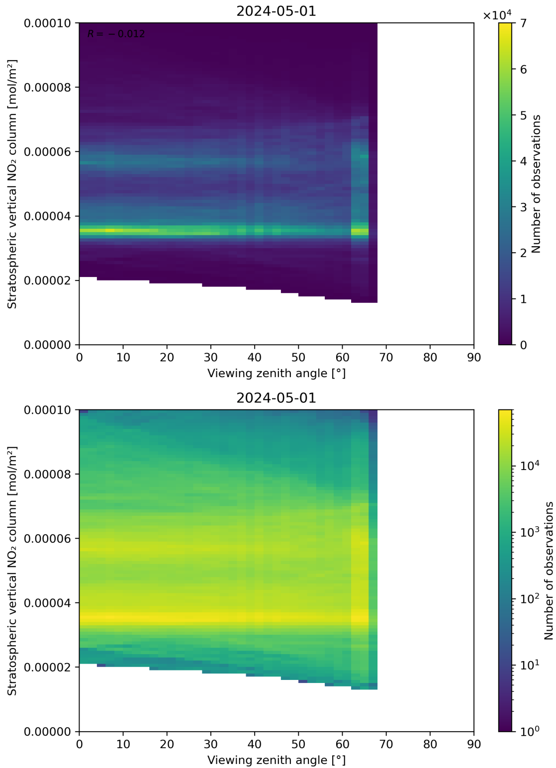
Figure 164: Scatter density plot of “Viewing zenith angle” against “Stratospheric vertical NO 2 column” for 2024-04-30 to 2024-05-02.
