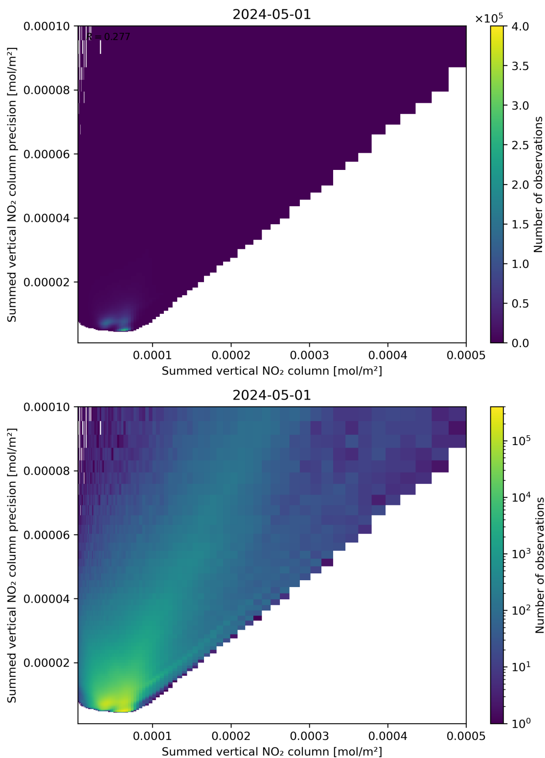
Figure 105: Scatter density plot of “Summed vertical NO 2 column” against “Summed vertical NO 2 column precision” for 2024-04-30 to 2024-05-02.
