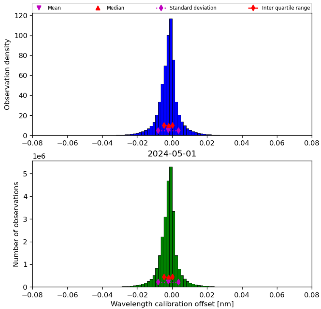
Figure 35: Histogram of “Wavelength calibration offset” for 2024-04-30 to 2024-05-02
