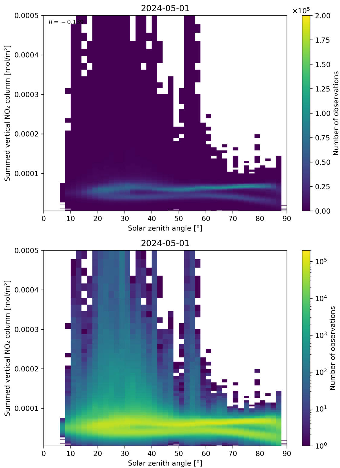
Figure 151: Scatter density plot of “Solar zenith angle” against “Summed vertical NO 2 column” for 2024-04-30 to 2024-05-02.
