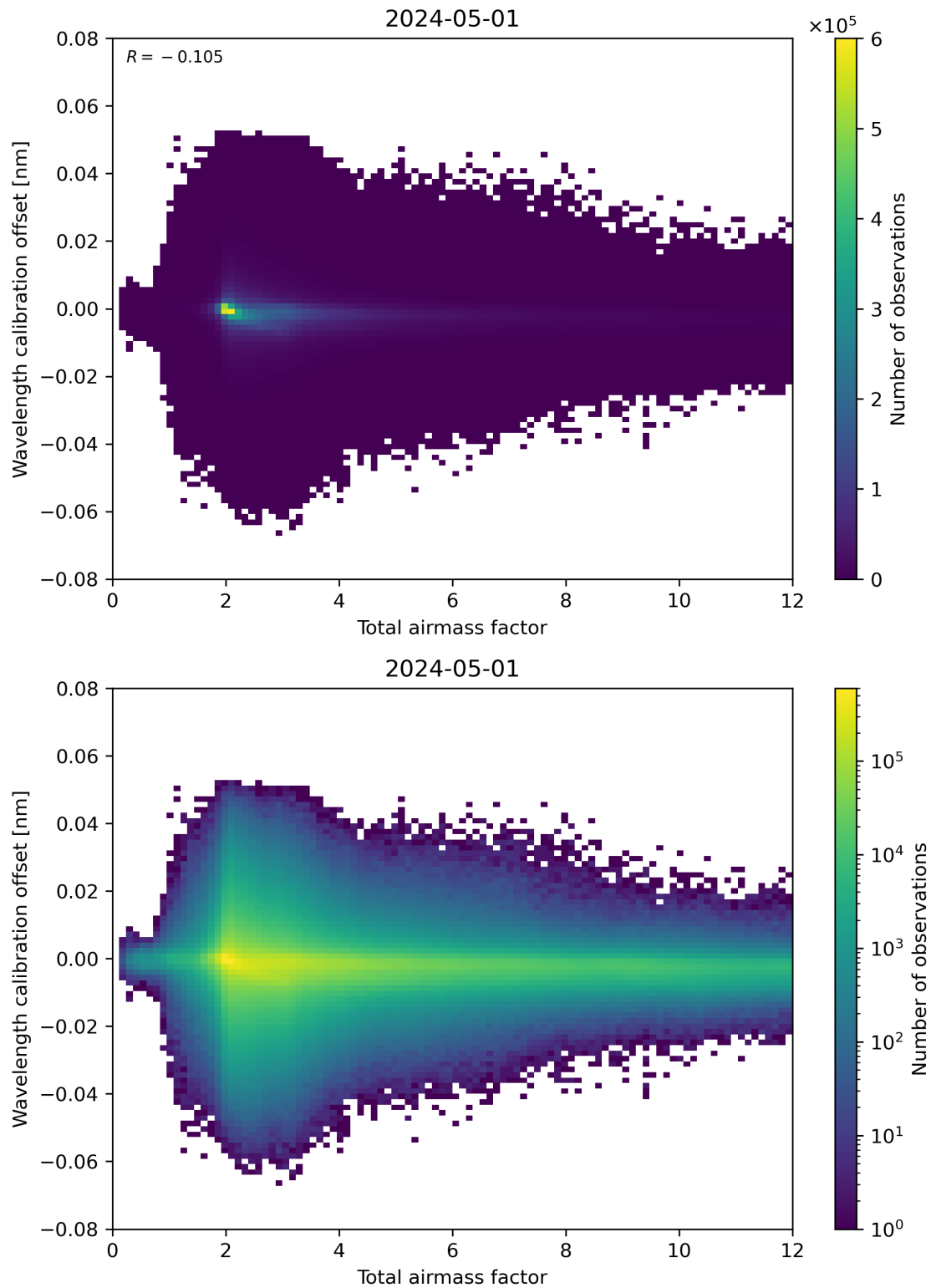
Figure 70: Scatter density plot of “Total airmass factor” against “Wavelength calibration offset” for 2024-04-30 to 2024-05-02.
