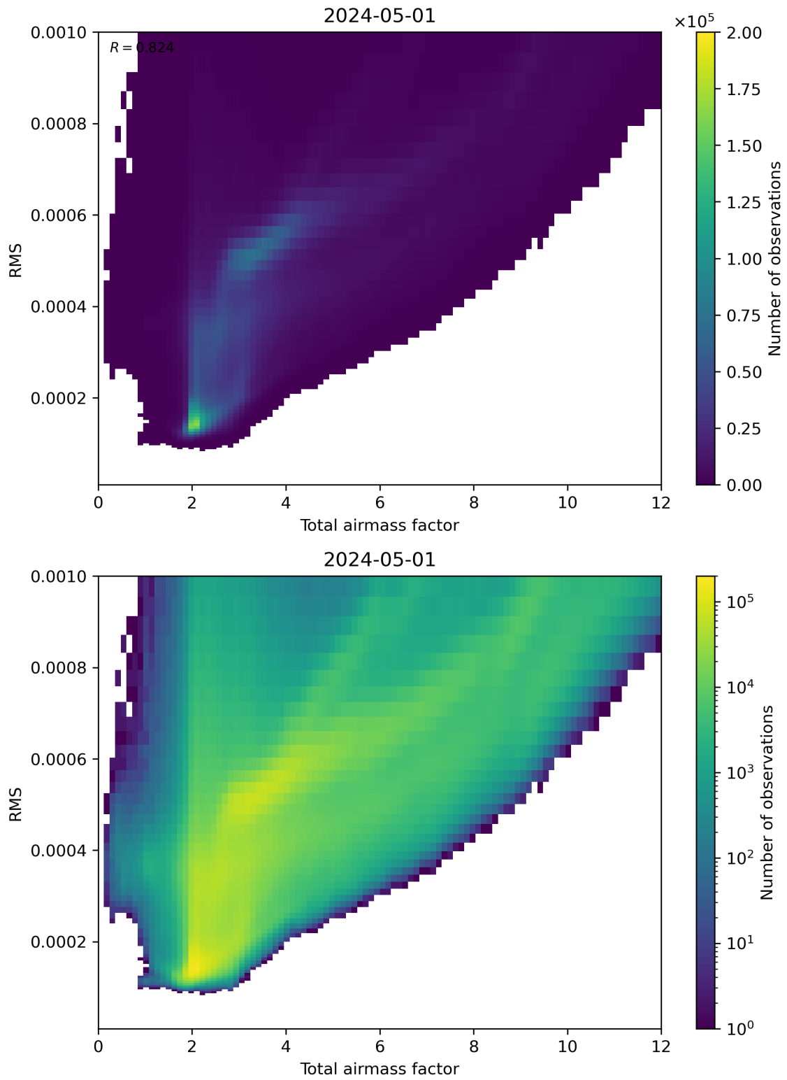
Figure 69: Scatter density plot of “Total airmass factor” against “RMS” for 2024-04-30 to 2024-05-02.
