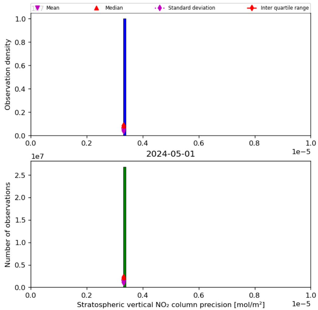
Figure 37: Histogram of “Stratospheric vertical NO 2 column precision” for 2024-04-30 to 2024-05-02
