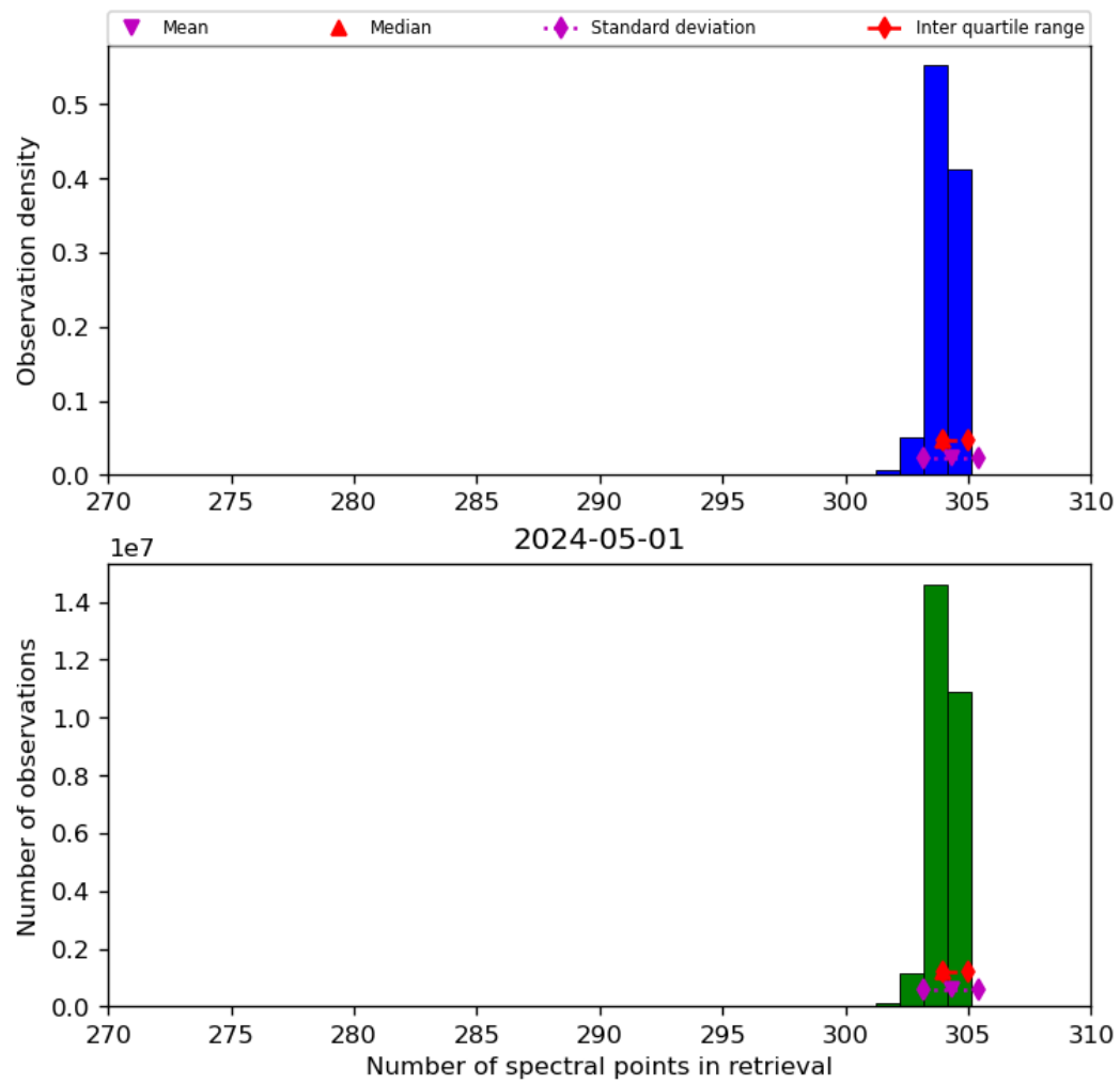
Figure 33: Histogram of “Number of spectral points in retrieval” for 2024-04-30 to 2024-05-02
