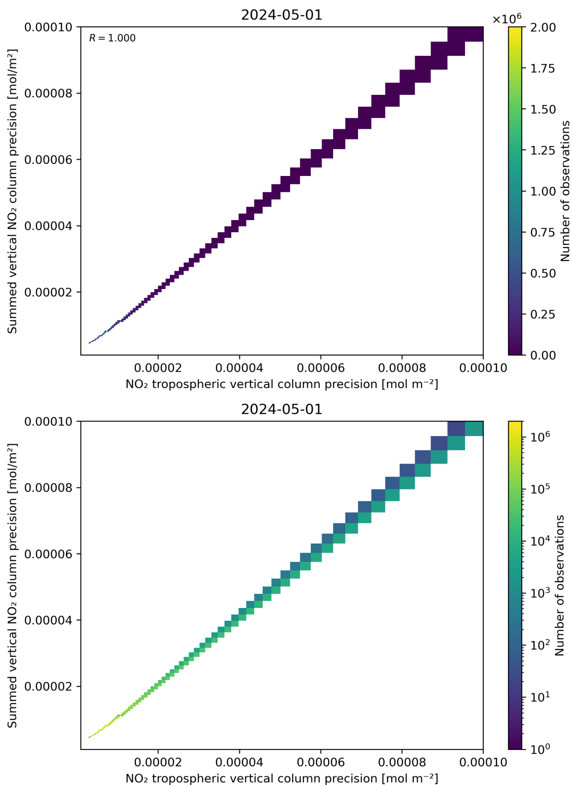
Figure 137: Scatter density plot of “NO 2 tropospheric vertical column precision” against “Summed vertical NO 2 column precision” for 2024-04-30 to 2024-05-02.
