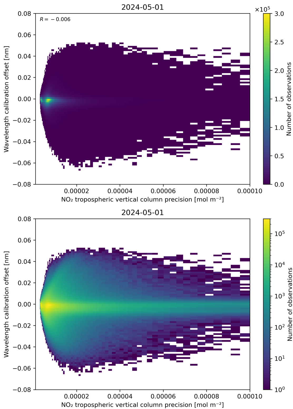
Figure 141: Scatter density plot of “NO 2 tropospheric vertical column precision” against “Wavelength calibration offset” for 2024-04-30 to 2024-05-02.
