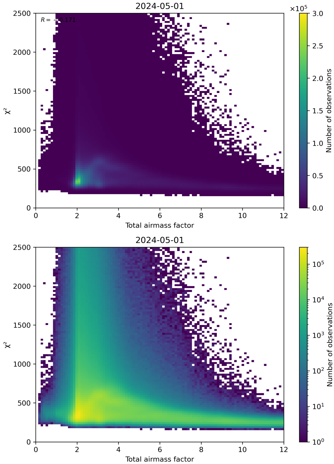
Figure 63: Scatter density plot of “Total airmass factor” against “ \chi^2 ” for 2024-04-30 to 2024-05-02.
