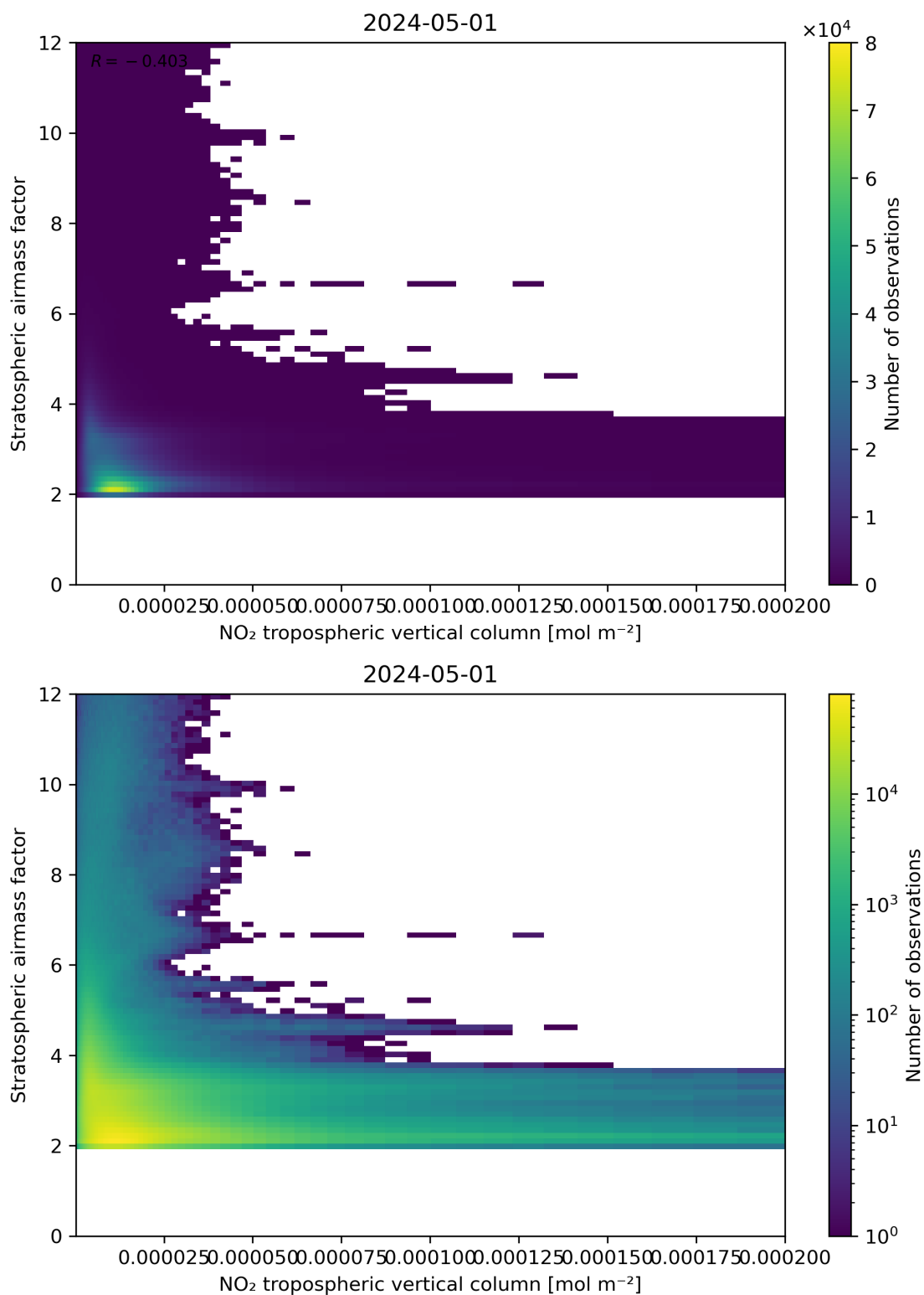
Figure 121: Scatter density plot of “NO 2 tropospheric vertical column” against “Stratospheric air mass factor” for 2024-04-30 to 2024-05-02.
