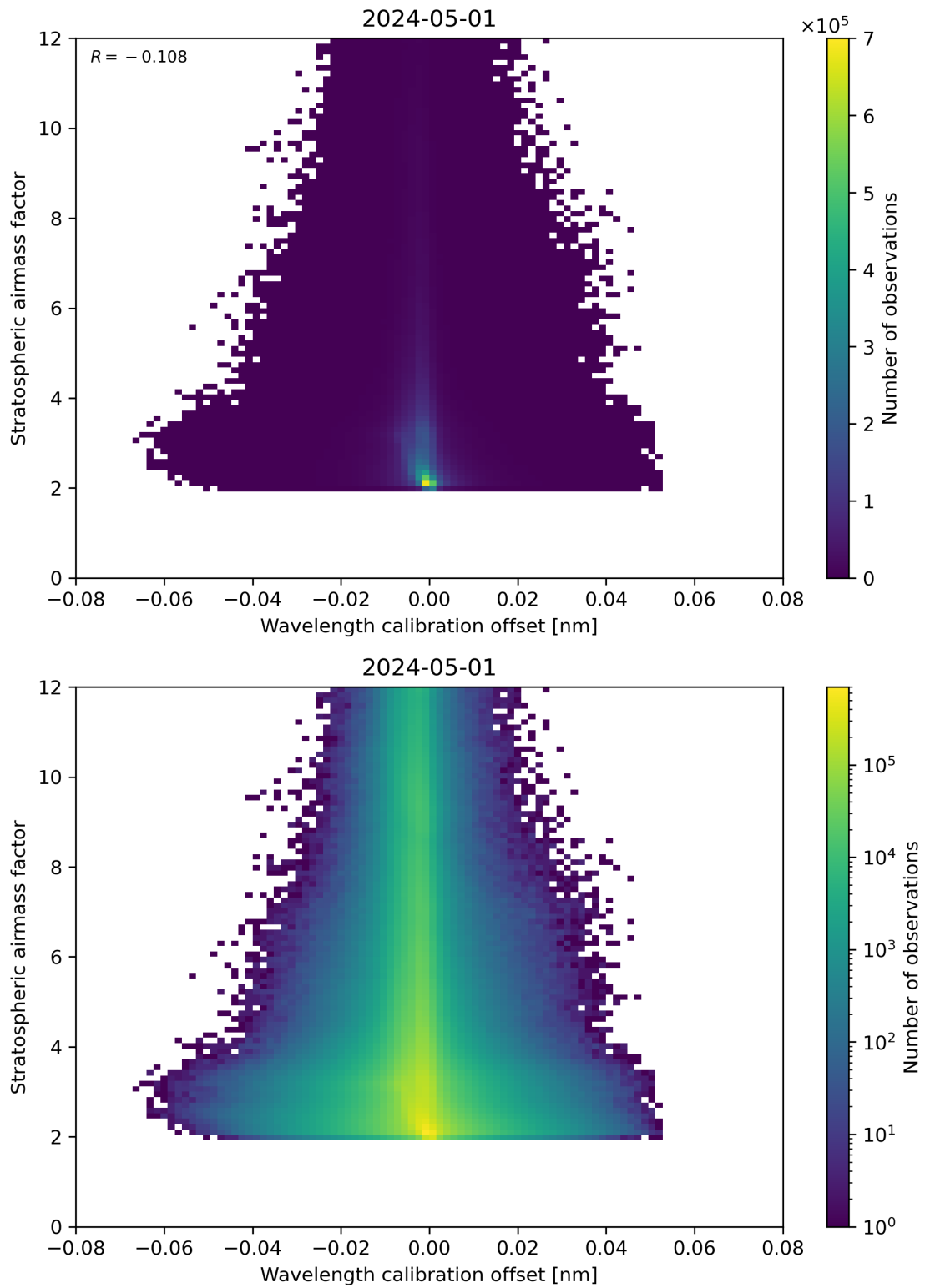
Figure 174: Scatter density plot of “Wavelength calibration offset” against “Stratospheric airmass factor” for 2024-04-30 to 2024-05-02.
