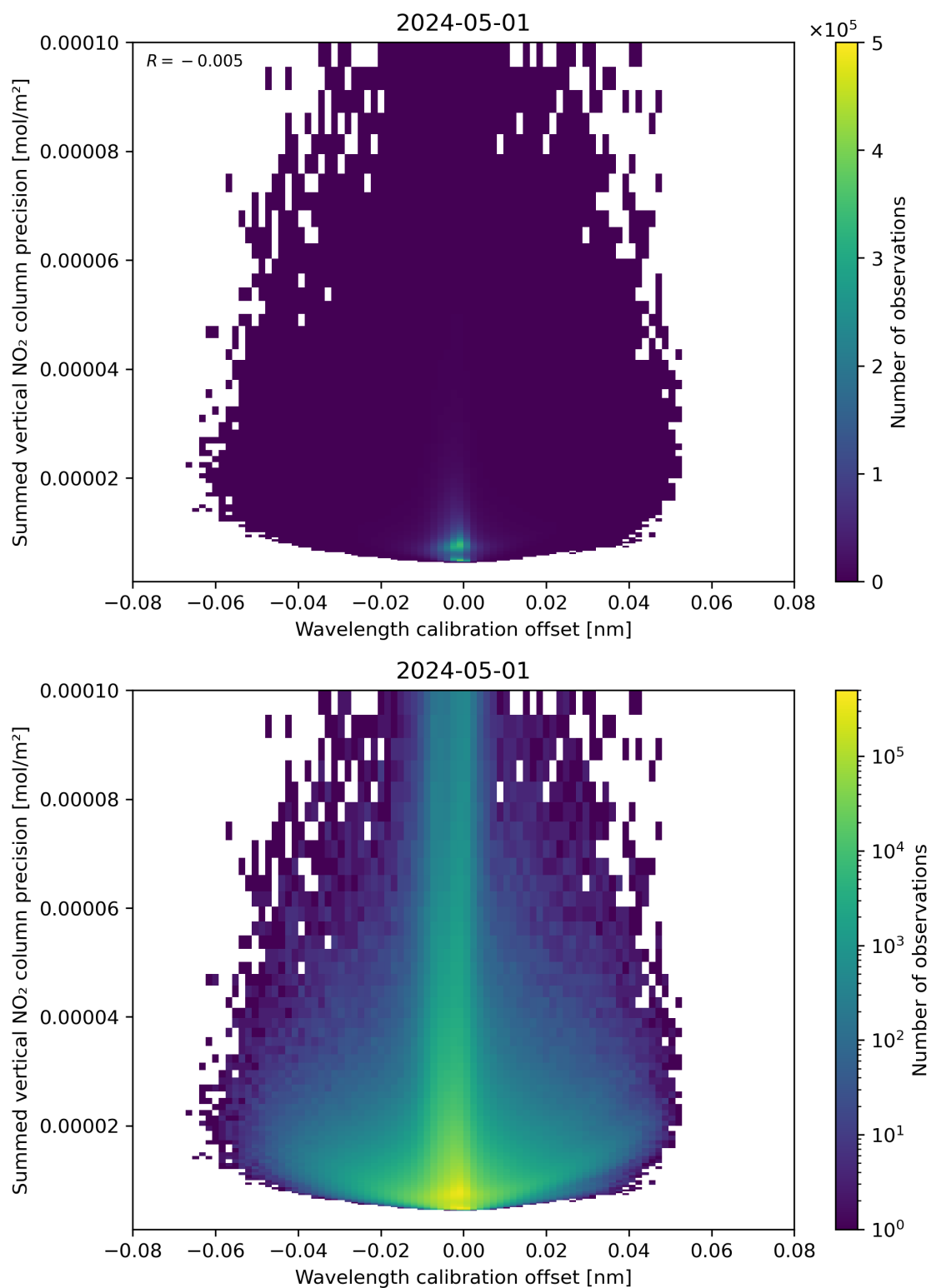
Figure 178: Scatter density plot of “Wavelength calibration offset” against “Summed vertical NO 2 column precision” for 2024-04-30 to 2024-05-02.
