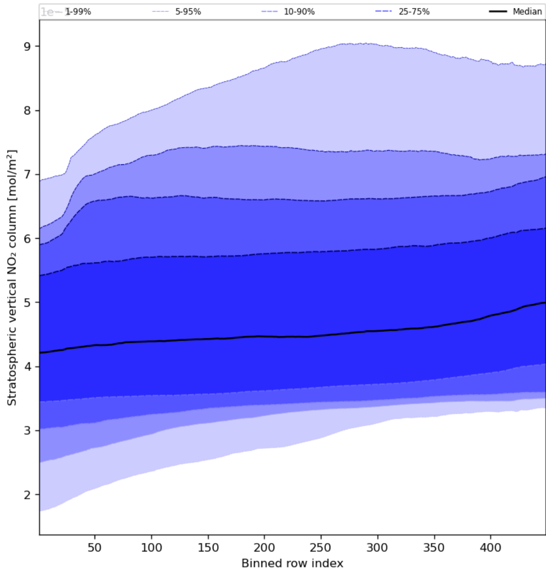
Figure 53: Along track statistics of “Stratospheric vertical NO 2 column” for 2024-04-30 to 2024-05-02
