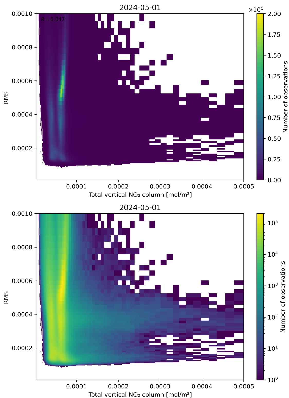
Figure 120: Scatter density plot of “Total vertical NO 2 column” against “RMS” for 2024-04-30 to 2024-05-02.
