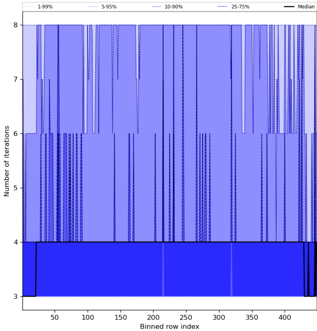
Figure 51: Along track statistics of “Number of iterations” for 2024-04-30 to 2024-05-02
