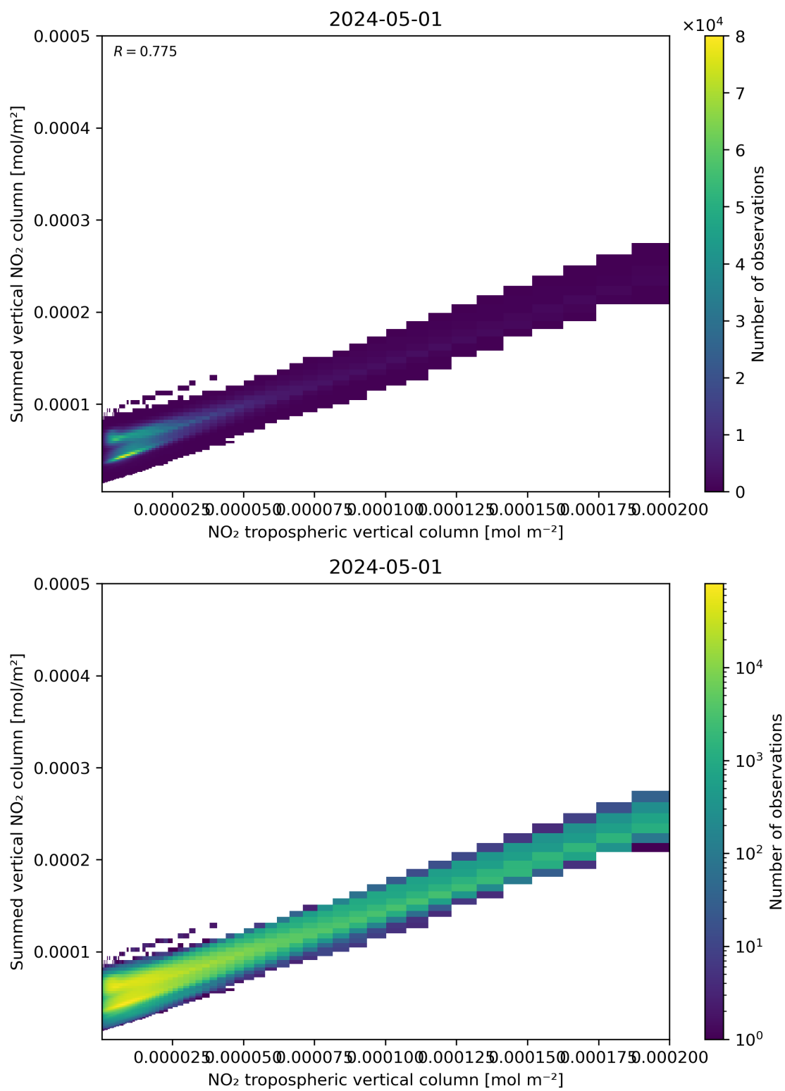
Figure 126: Scatter density plot of “NO 2 tropospheric vertical column” against “Summed vertical NO 2 column” for 2024-04-30 to 2024-05-02.
