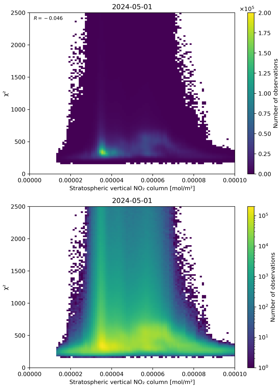
Figure 97: Scatter density plot of “Stratospheric vertical NO 2 column” against “ \chi^2 ” for 2024-04-30 to 2024-05-02.
