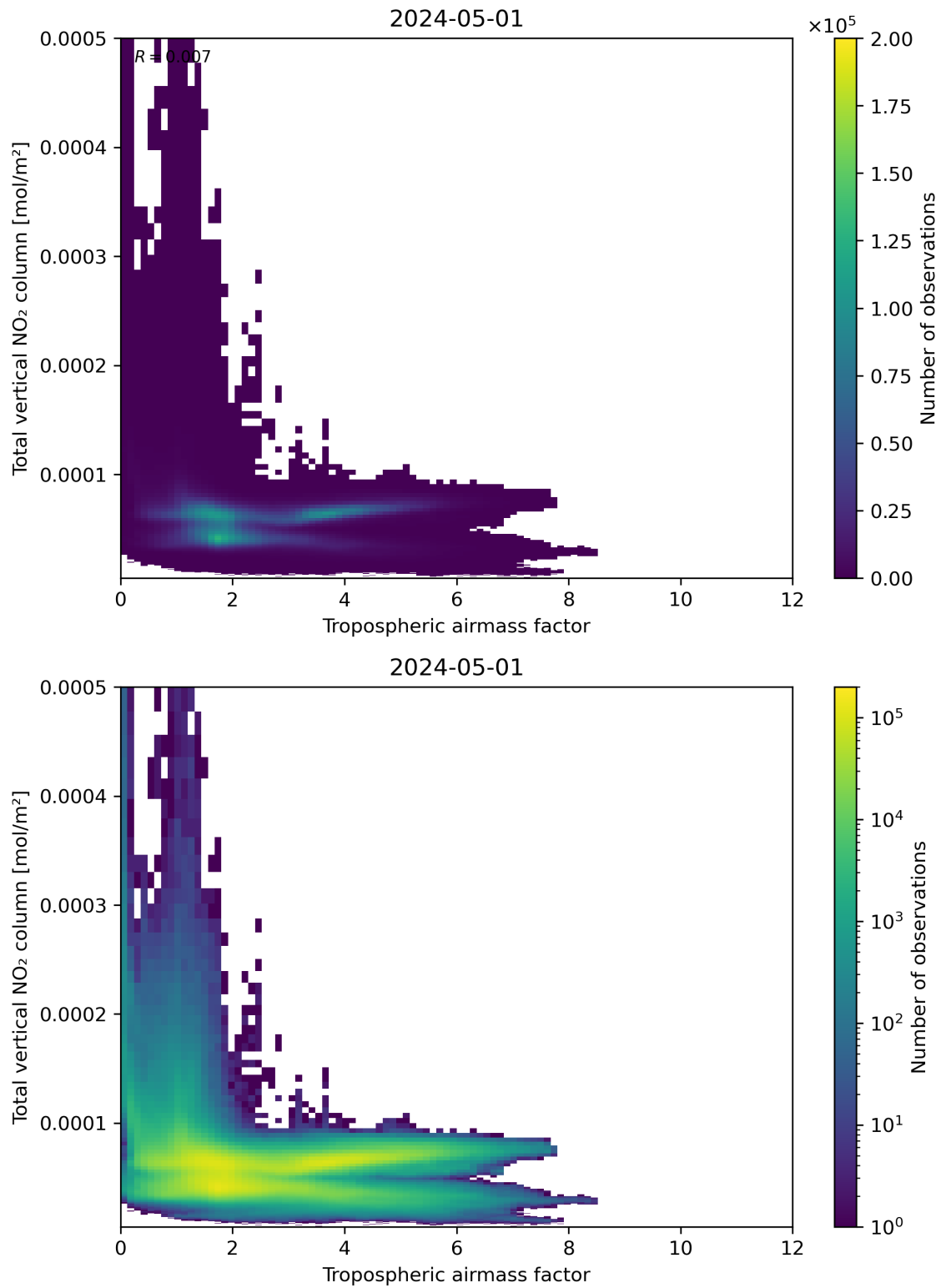
Figure 77: Scatter density plot of “Tropospheric airmass factor” against “Total vertical NO 2 column” for 2024-04-30 to 2024-05-02.
