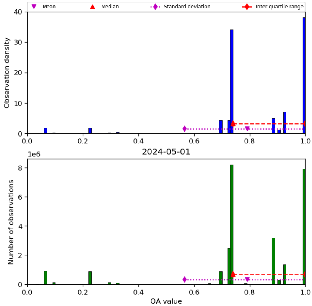
Figure 28: Histogram of “QA value” for 2024-04-30 to 2024-05-02
