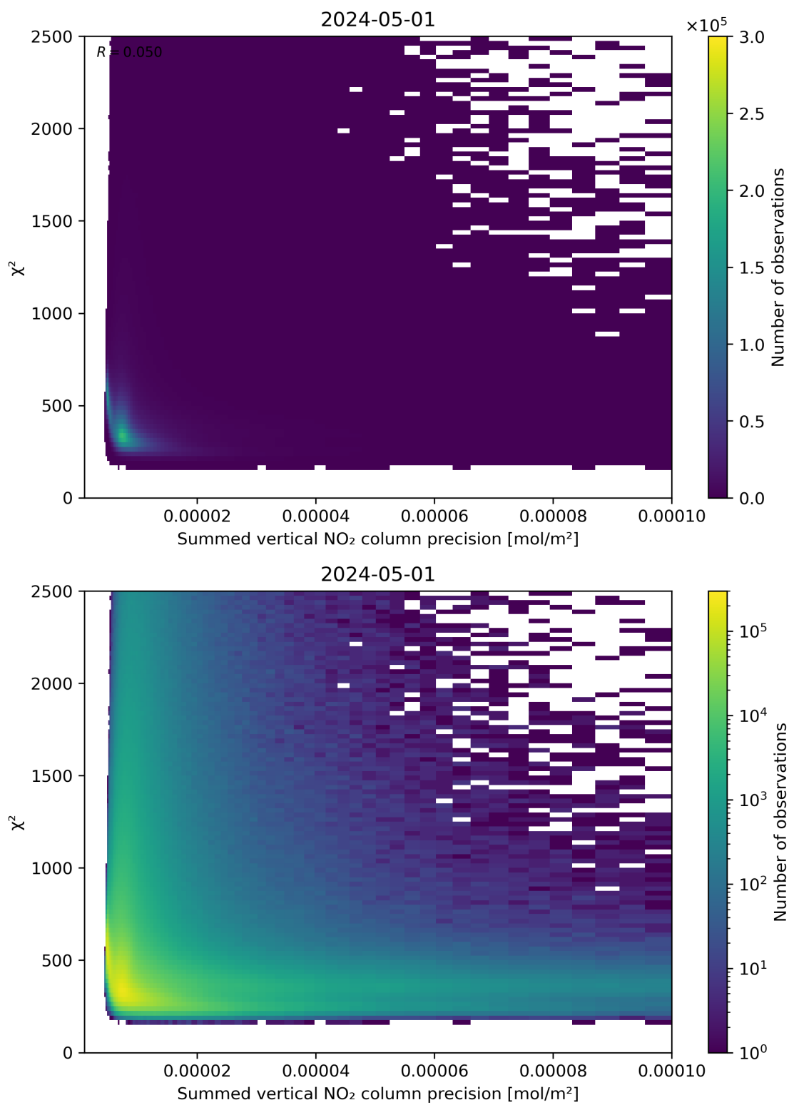
Figure 107: Scatter density plot of “Summed vertical NO 2 column precision” against “ \chi^2 ” for 2024-04-30 to 2024-05-02.
