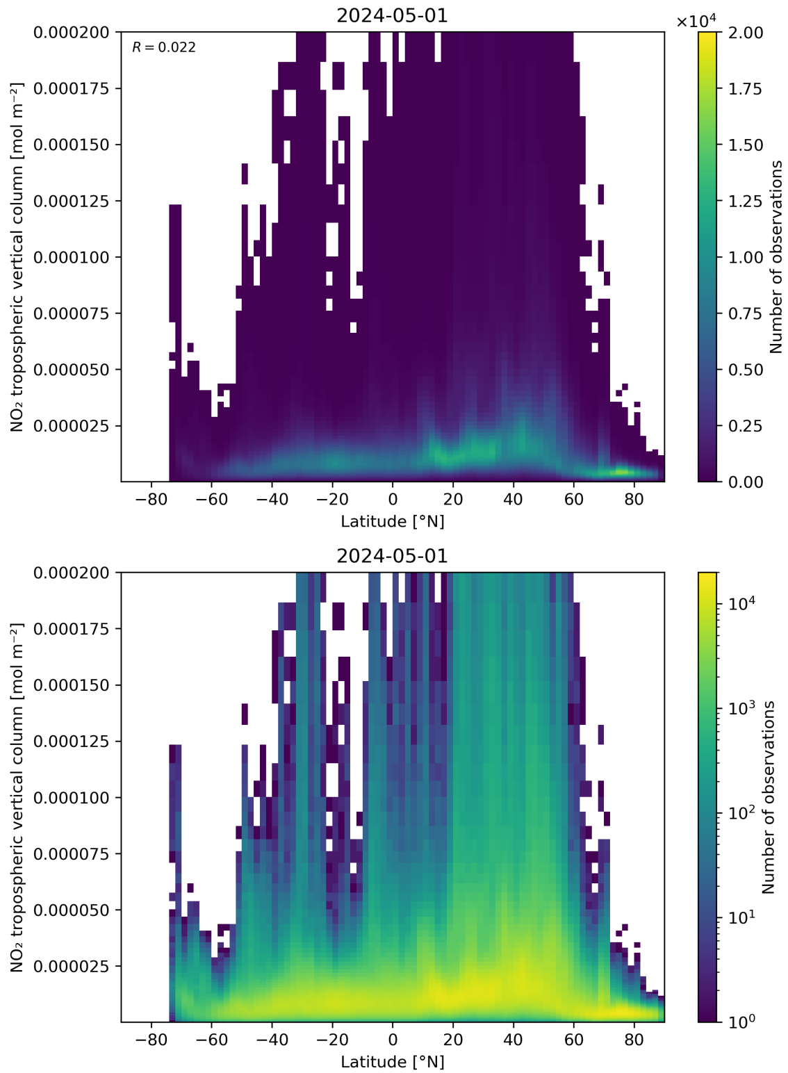
Figure 92: Scatter density plot of “Latitude” against “NO 2 tropospheric vertical column” for 2024-04-30 to 2024-05-02.
