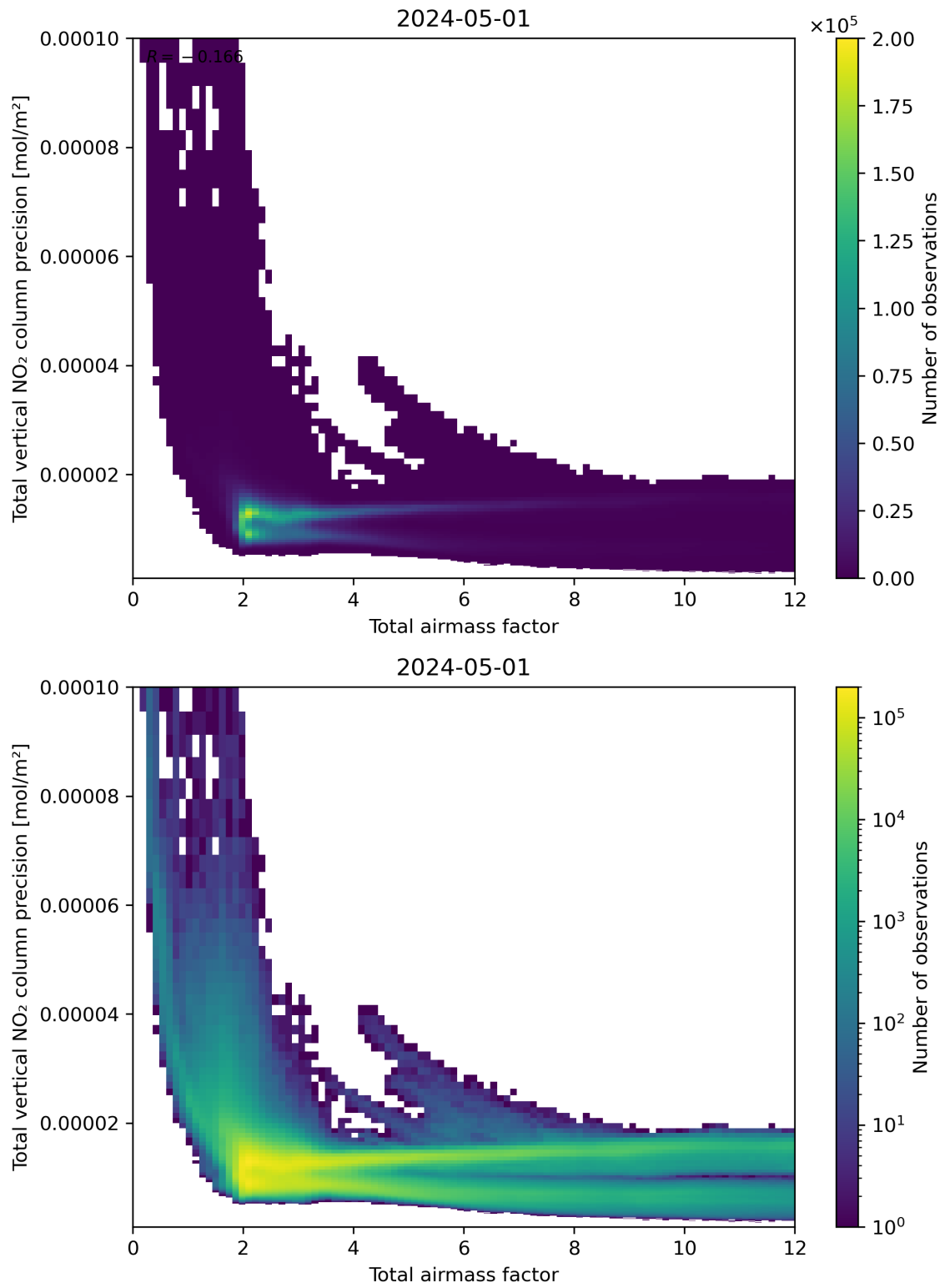
Figure 68: Scatter density plot of “Total airmass factor” against “Total vertical NO 2 column precision” for 2024-04-30 to 2024-05-02.
