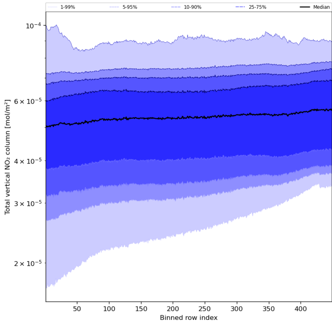
Figure 55: Along track statistics of “Total vertical NO 2 column” for 2024-04-30 to 2024-05-02
