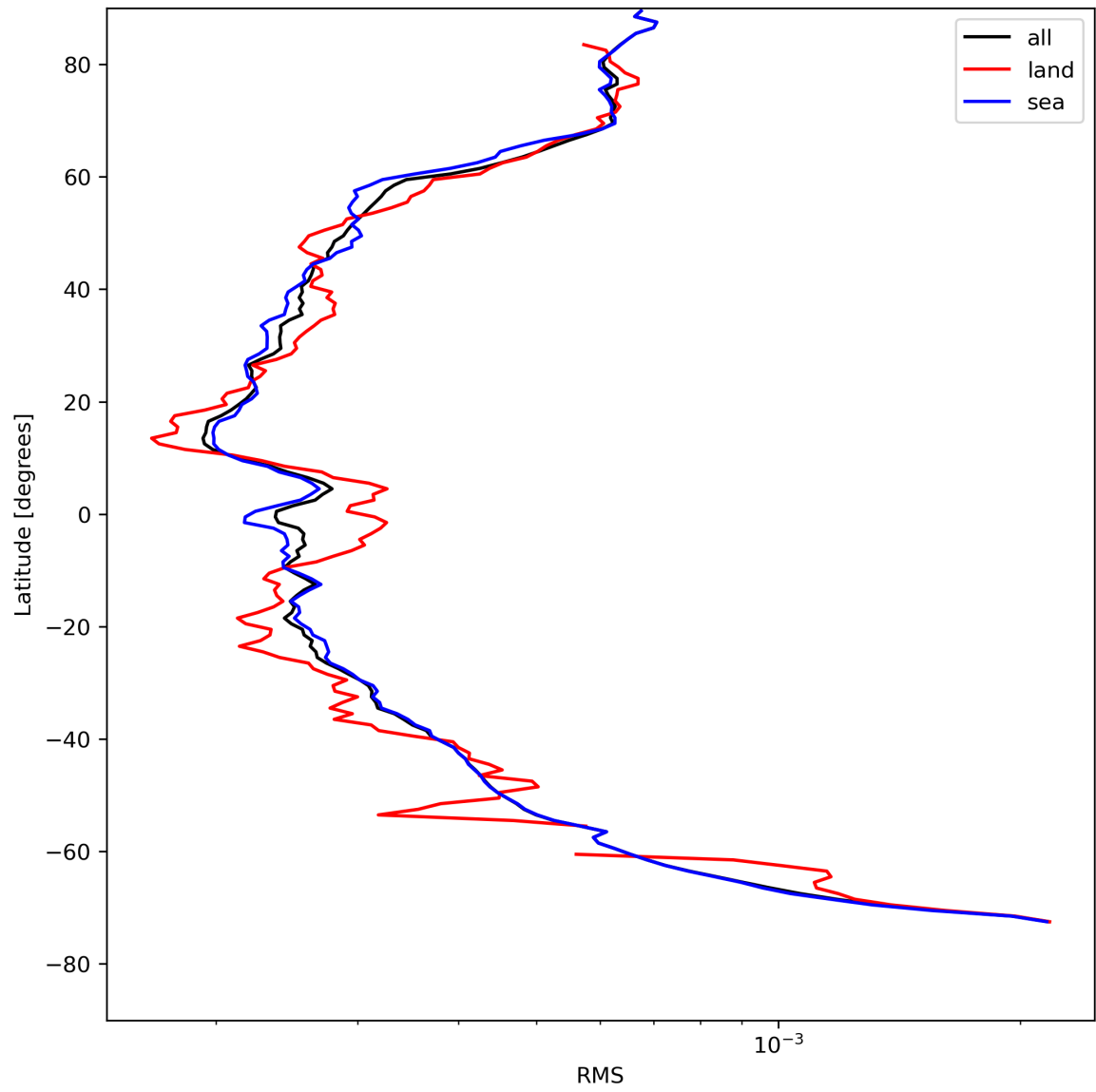
Figure 26: Zonal average of “RMS” for 2024-04-30 to 2024-05-02.
