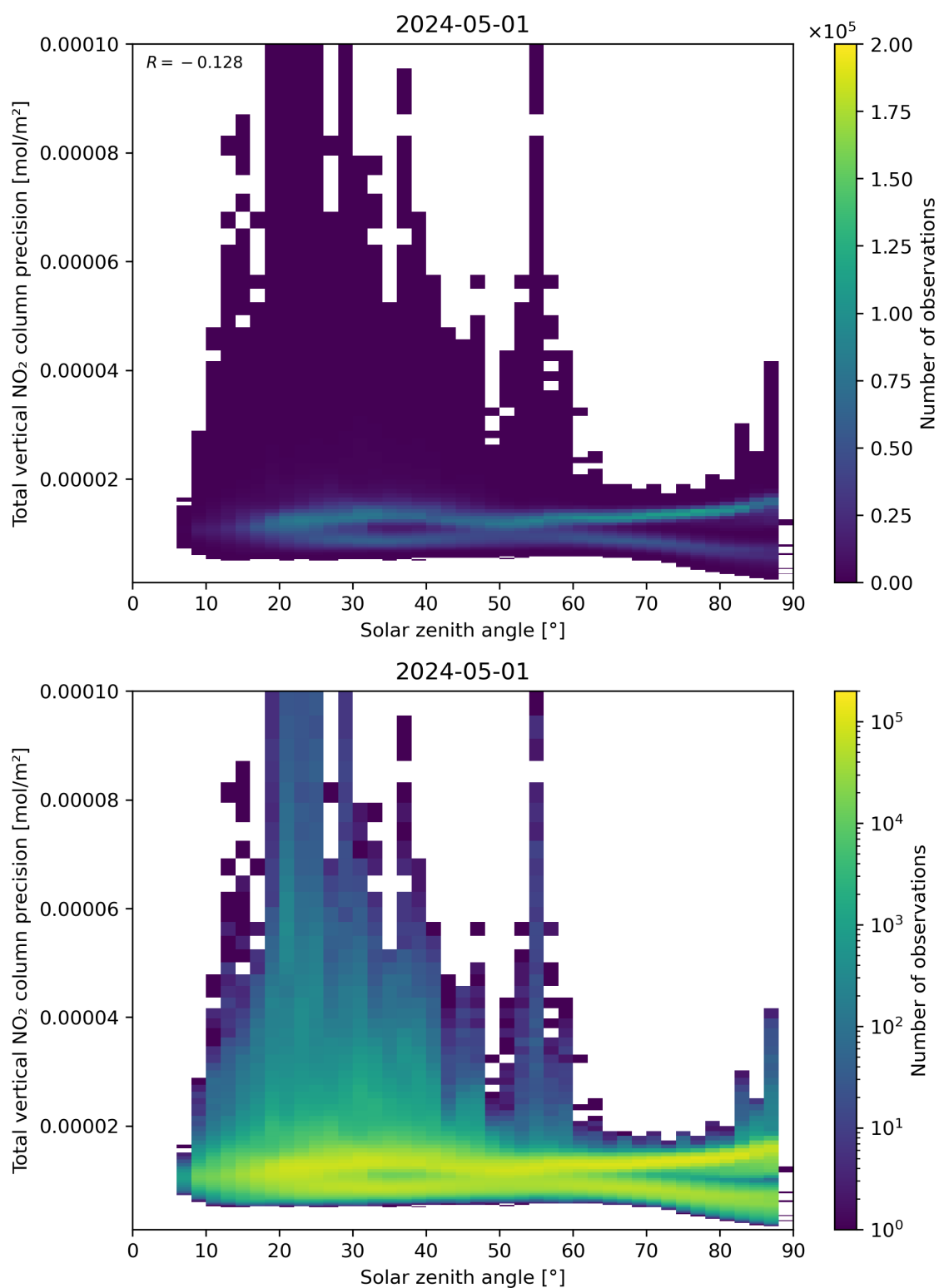
Figure 154: Scatter density plot of “Solar zenith angle” against “Total vertical NO 2 column precision” for 2024-04-30 to 2024-05-02.
