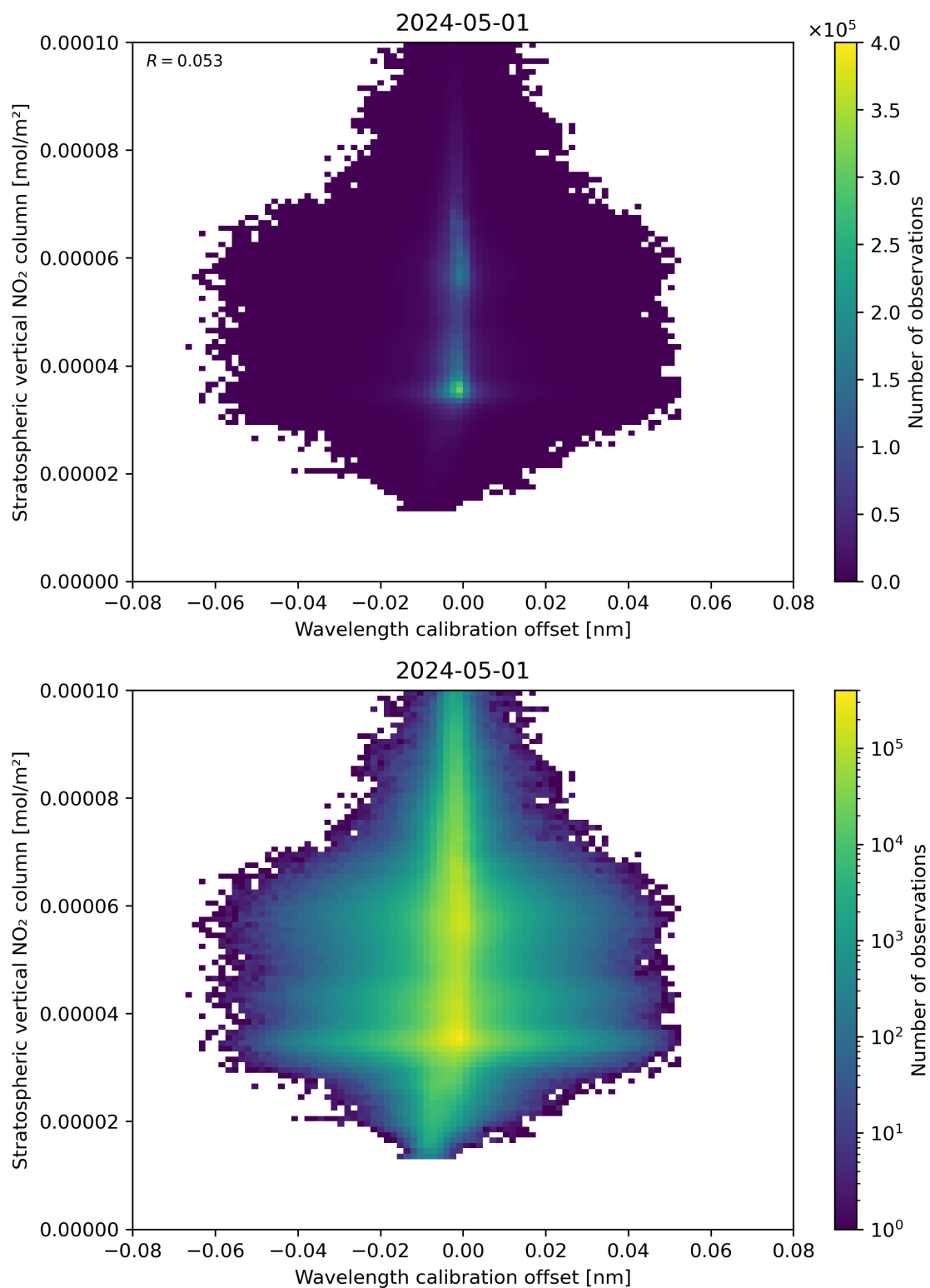
Figure 176: Scatter density plot of “Wavelength calibration offset” against “Stratospheric vertical NO 2 column” for 2024-04-30 to 2024-05-02.
