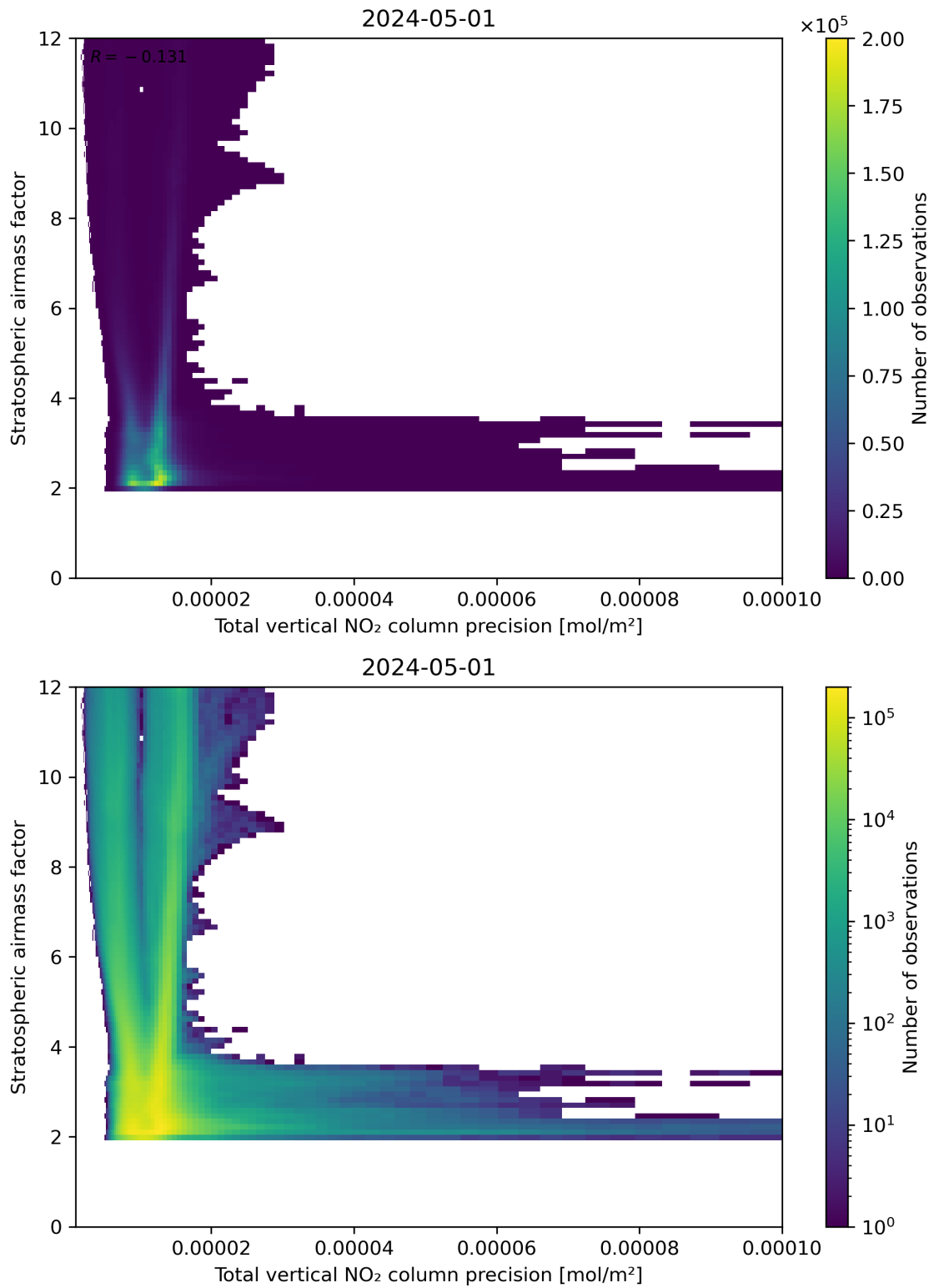
Figure 115: Scatter density plot of “Total vertical NO 2 column precision” against “Stratospheric air mass factor” for 2024-04-30 to 2024-05-02.
