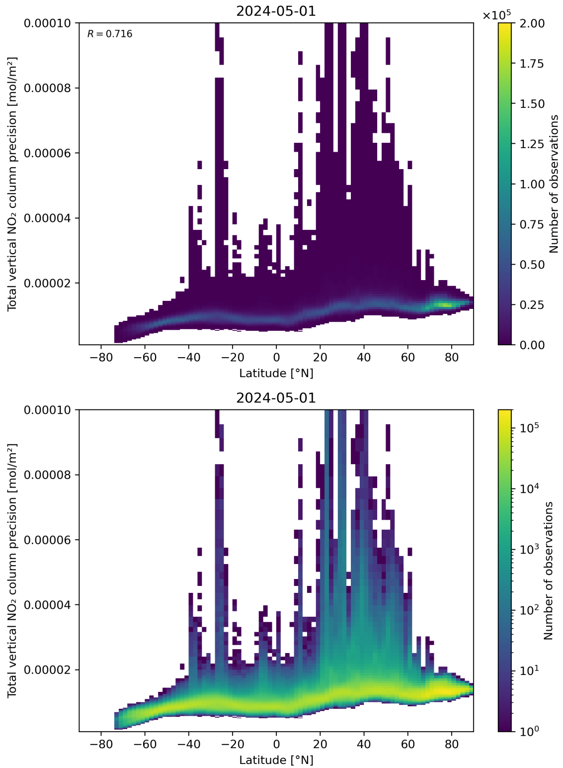
Figure 91: Scatter density plot of “Latitude” against “Total vertical NO 2 column precision” for 2024-04-30 to 2024-05-02.
