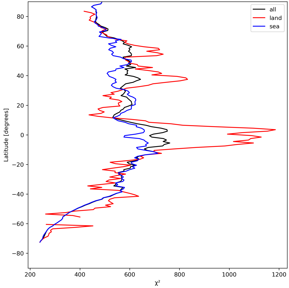
Figure 25: Zonal average of “ \chi^2 ” for 2024-04-30 to 2024-05-02.
