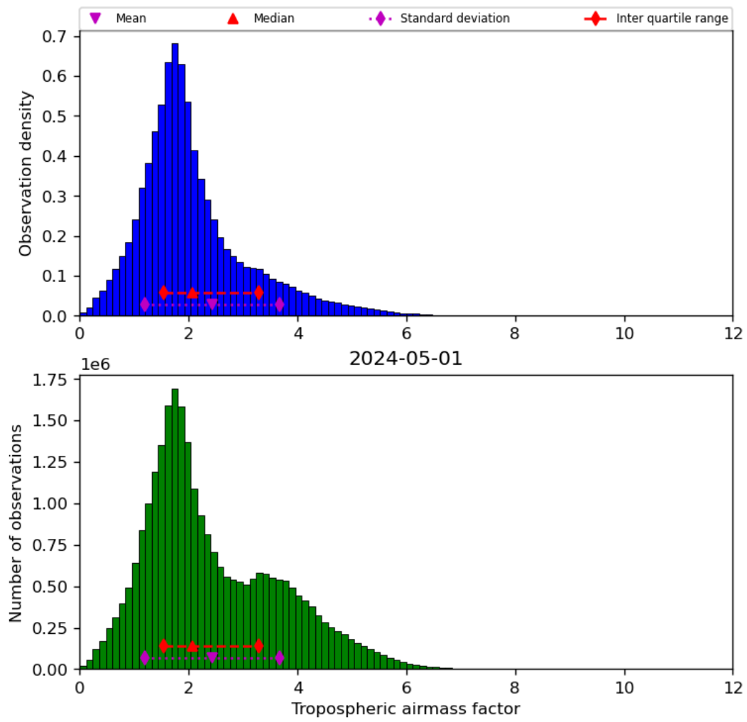
Figure 31: Histogram of “Tropospheric airmass factor” for 2024-04-30 to 2024-05-02
