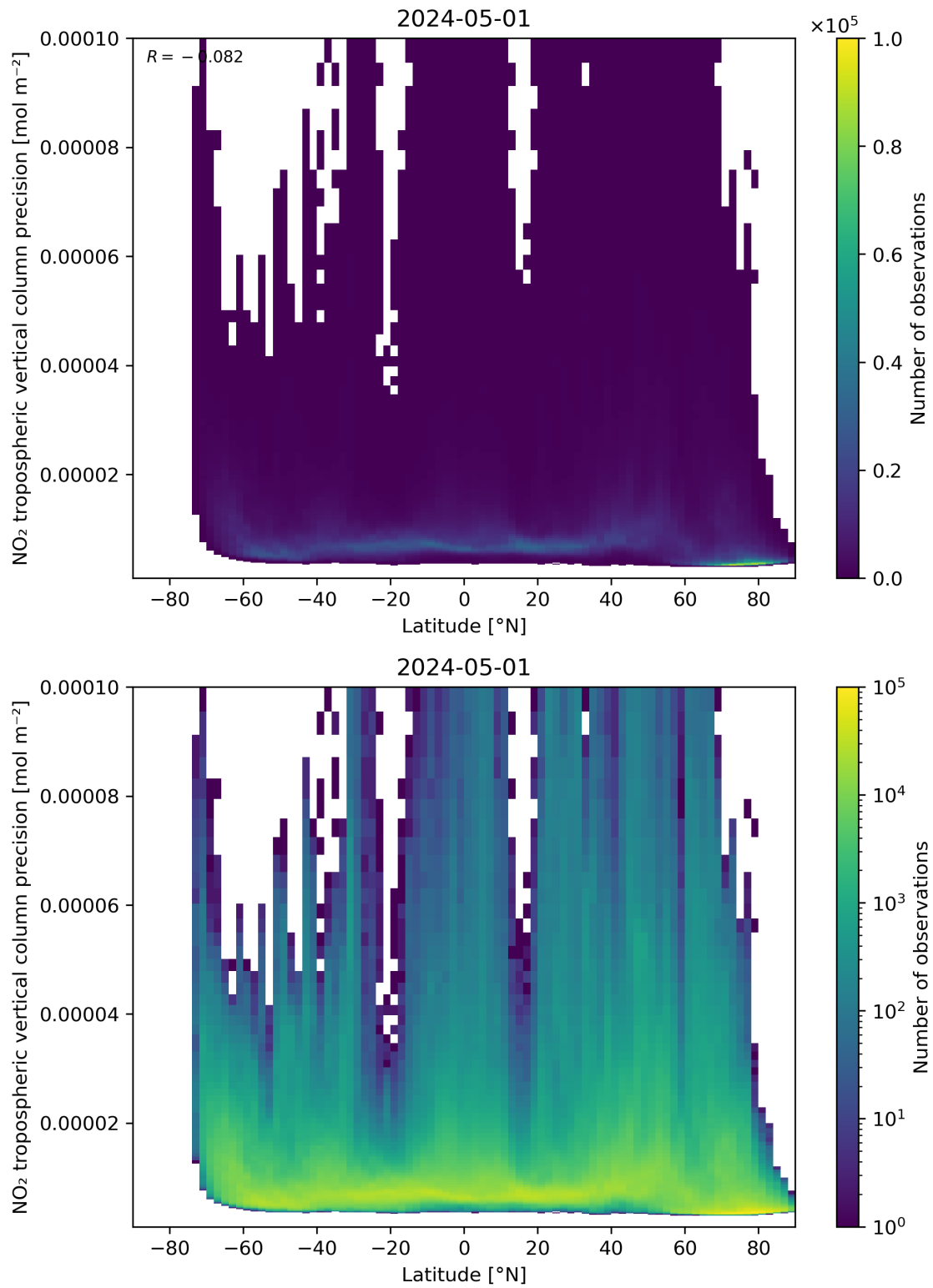
Figure 93: Scatter density plot of “Latitude” against “NO 2 tropospheric vertical column precision” for 2024-04-30 to 2024-05-02.
