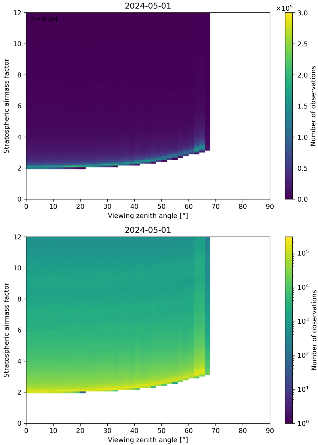
Figure 159: Scatter density plot of “Viewing zenith angle” against “Stratospheric airmass factor” for 2024-04-30 to 2024-05-02.
