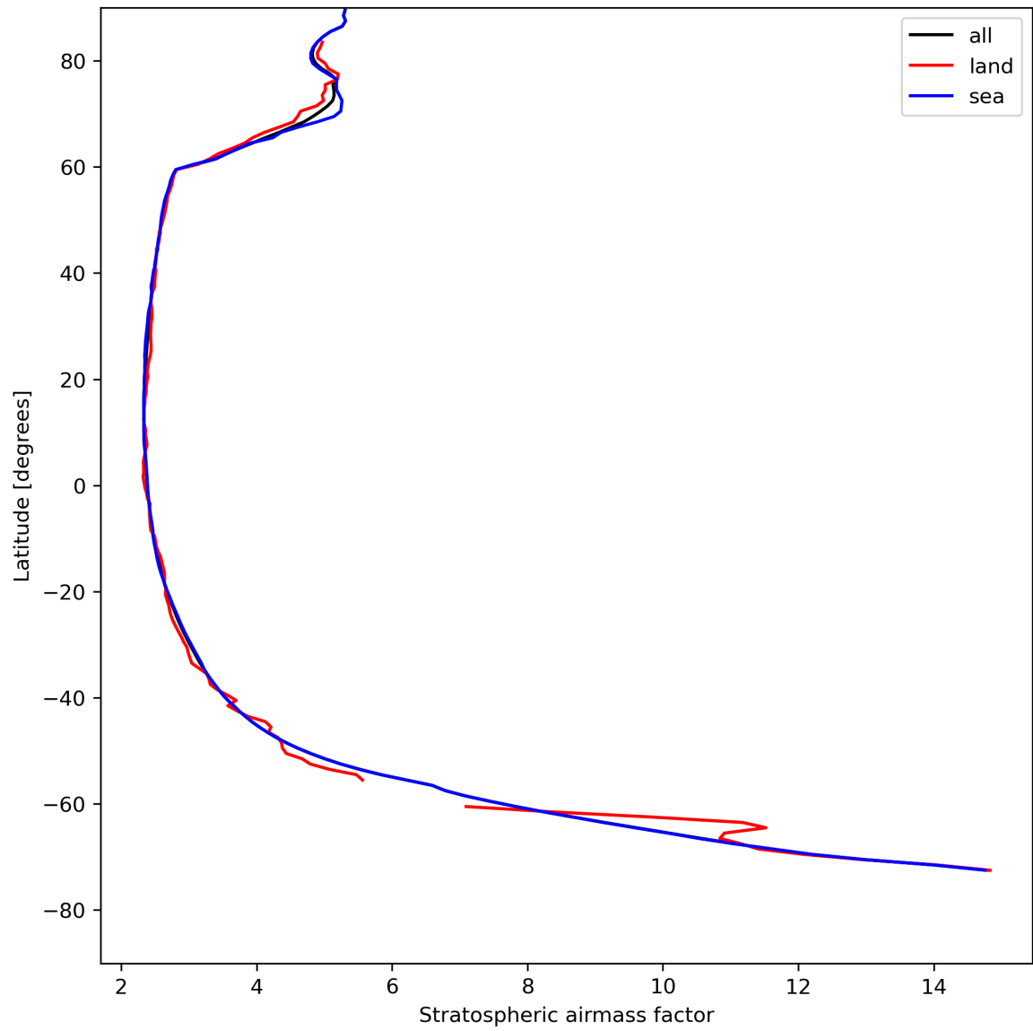
Figure 27: Zonal average of “Stratospheric airmass factor” for 2024-04-30 to 2024-05-02.
