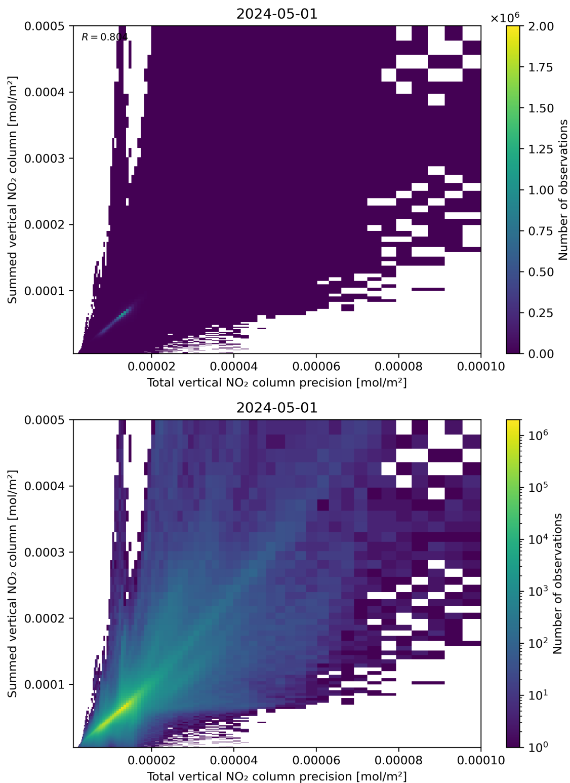
Figure 117: Scatter density plot of “Total vertical NO 2 column precision” against “Summed vertical NO 2 column” for 2024-04-30 to 2024-05-02.
