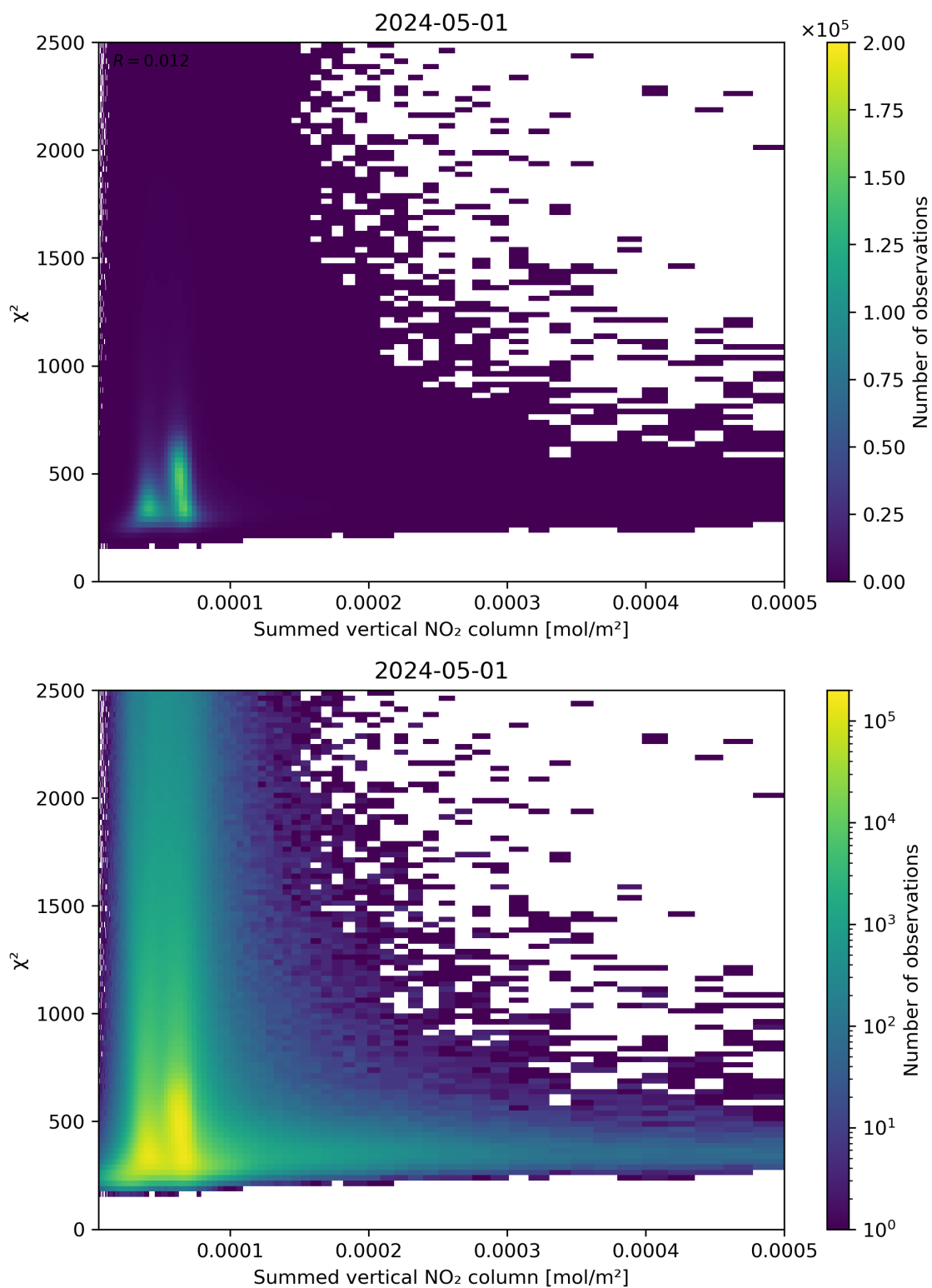
Figure 104: Scatter density plot of “Summed vertical NO 2 column” against “ \chi^2 ” for 2024-04-30 to 2024-05-02.
