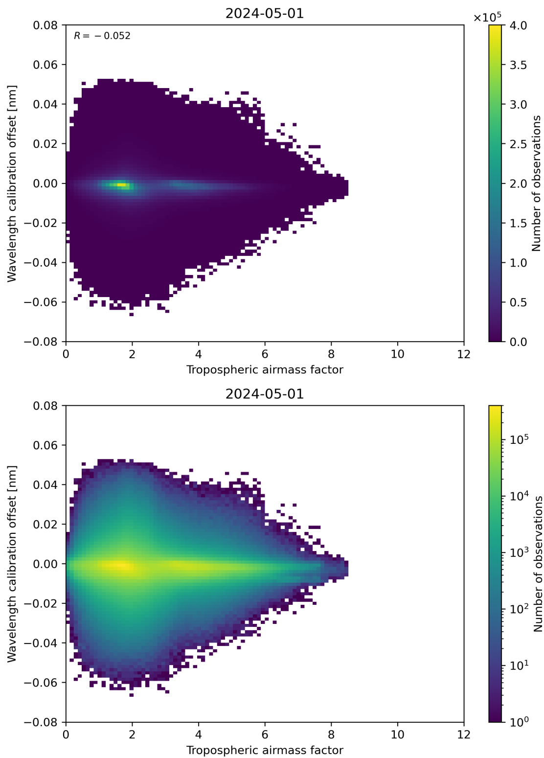
Figure 80: Scatter density plot of “Tropospheric airmass factor” against “Wavelength calibration offset” for 2024-04-30 to 2024-05-02.
