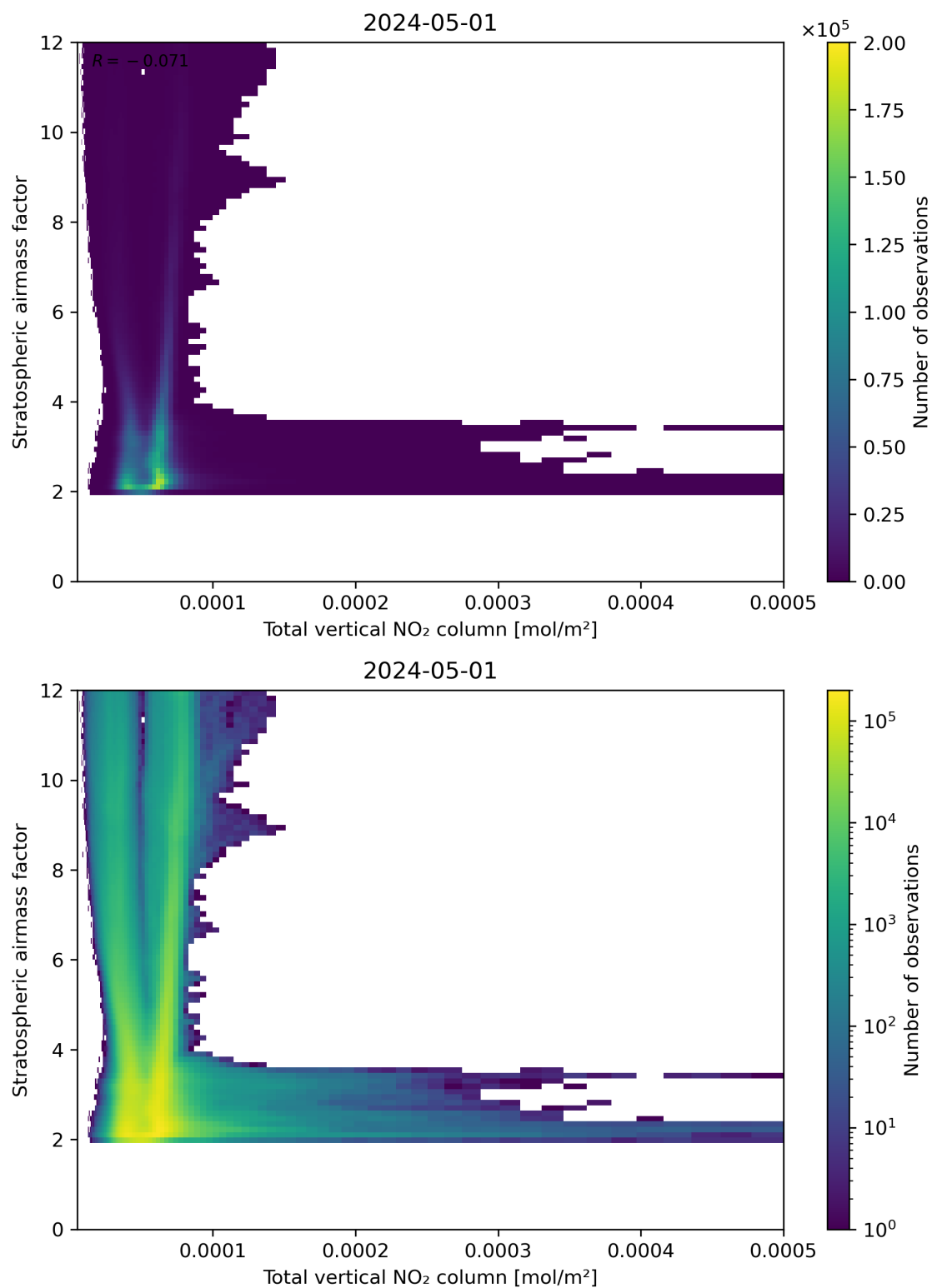
Figure 110: Scatter density plot of “Total vertical NO 2 column” against “Stratospheric airmass factor” for 2024-04-30 to 2024-05-02.
