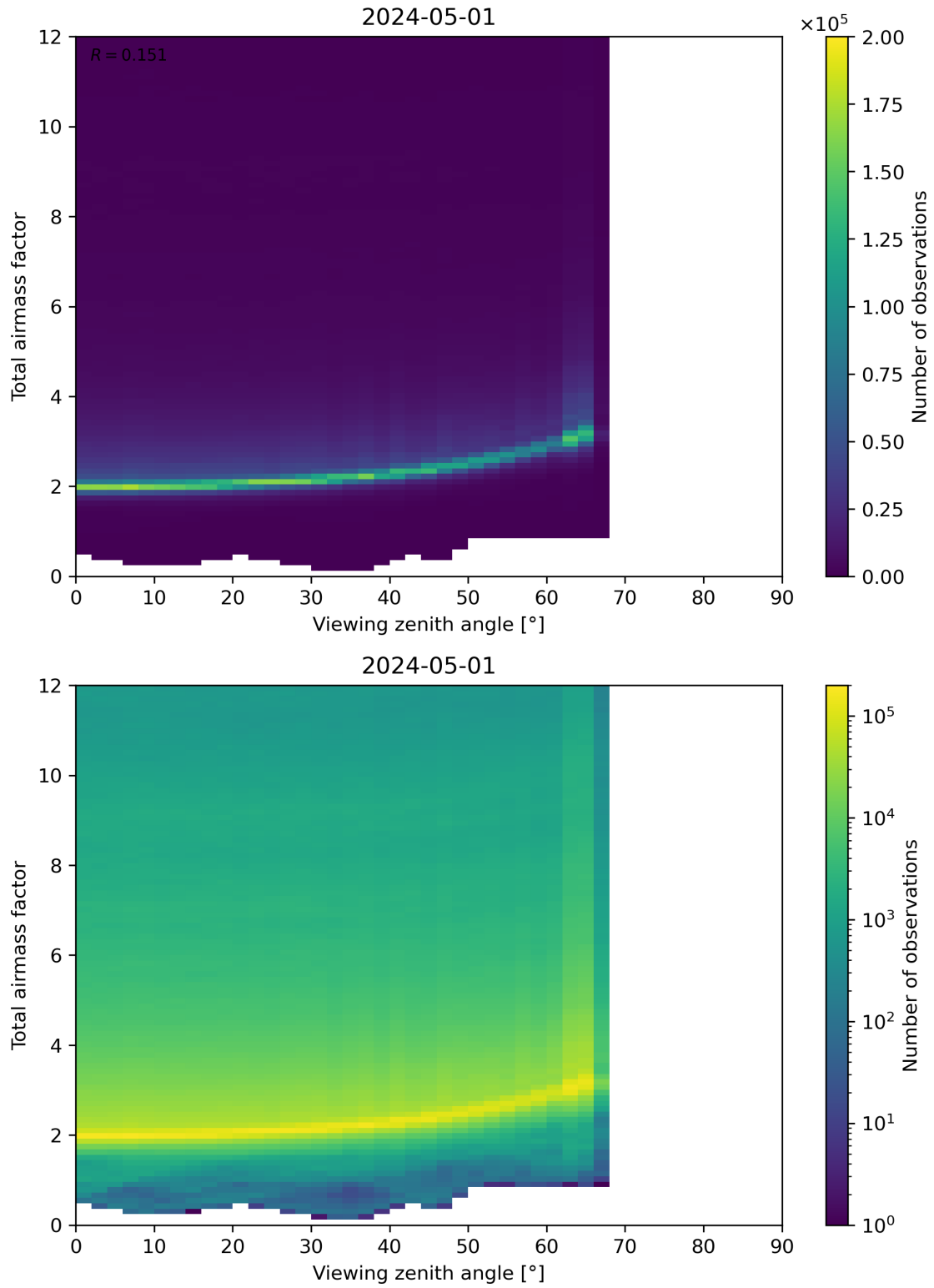
Figure 160: Scatter density plot of “Viewing zenith angle” against “Total airmass factor” for 2024-04-30 to 2024-05-02.
