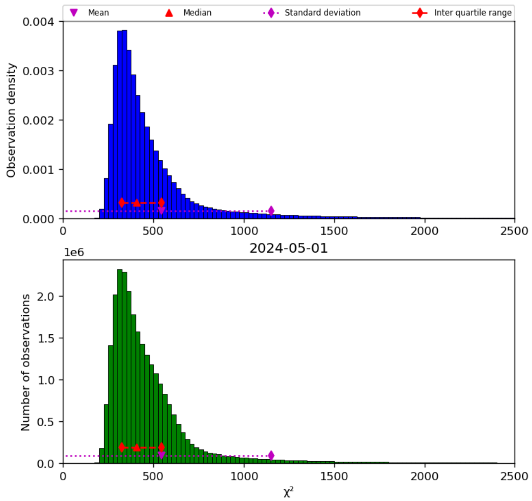
Figure 42: Histogram of " \chi^2 " for 2024-04-30 to 2024-05-02
