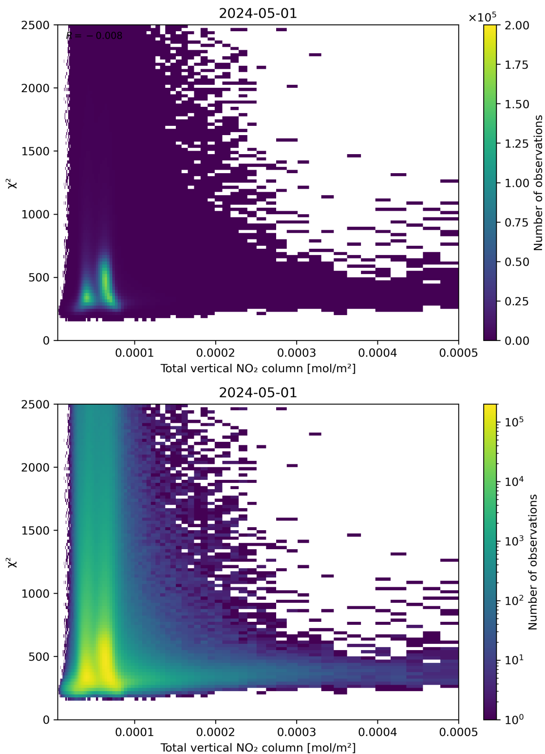
Figure 111: Scatter density plot of “Total vertical NO 2 column” against “ \chi^2 ” for 2024-04-30 to 2024-05-02.
