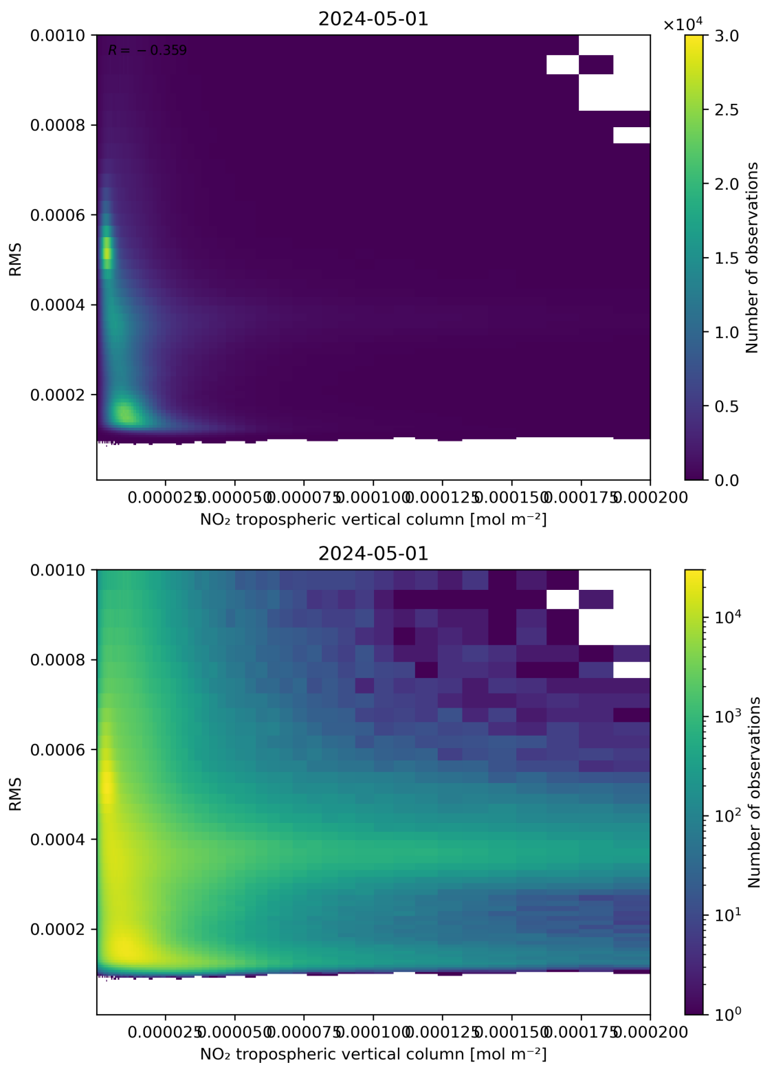
Figure 142: Scatter density plot of “NO 2 tropospheric vertical column” against “RMS” for 2024-04-30 to 2024-05-02.
