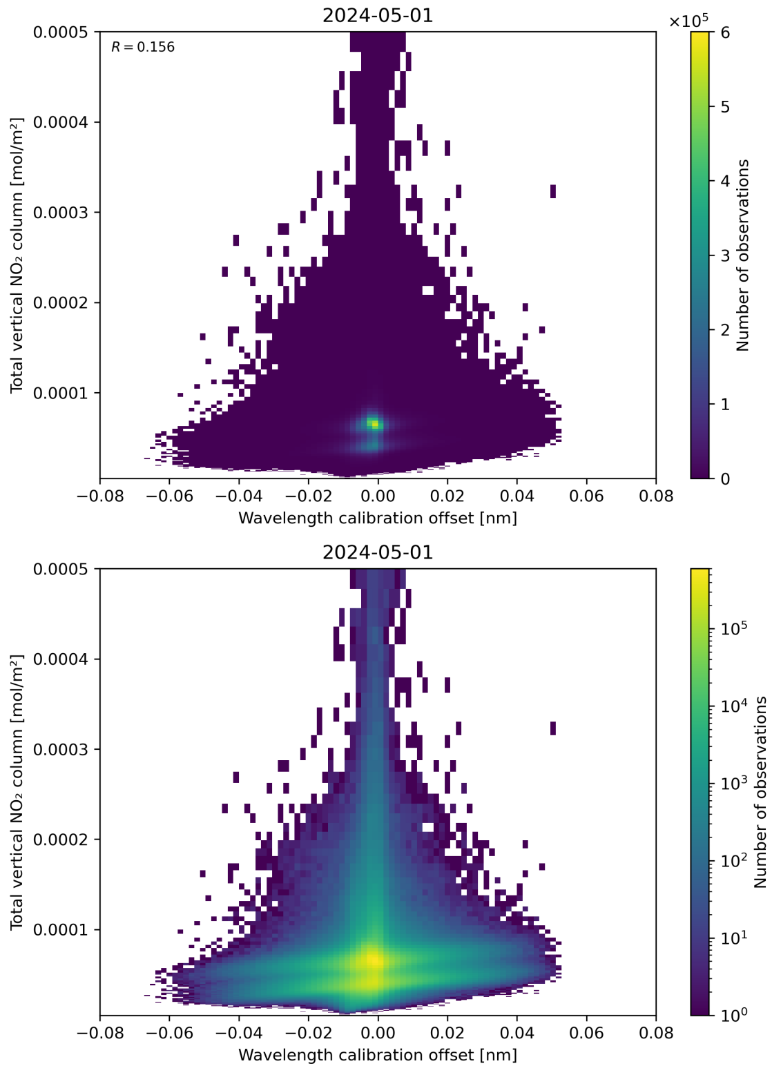
Figure 179: Scatter density plot of “Wavelength calibration offset” against “Total vertical NO 2 column” for 2024-04-30 to 2024-05-02.
