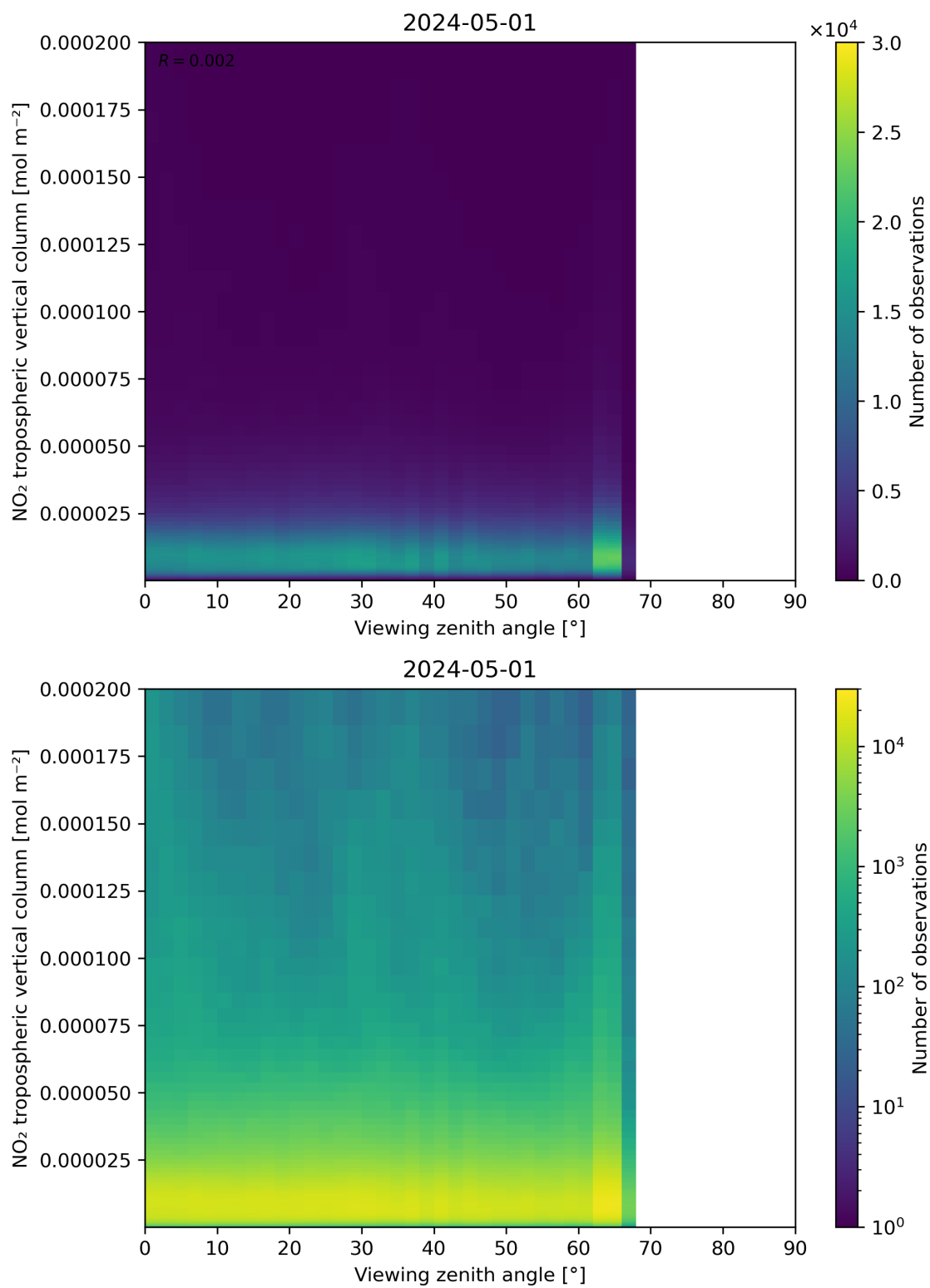
Figure 169: Scatter density plot of “Viewing zenith angle” against “NO 2 tropospheric vertical column” for 2024-04-30 to 2024-05-02.
