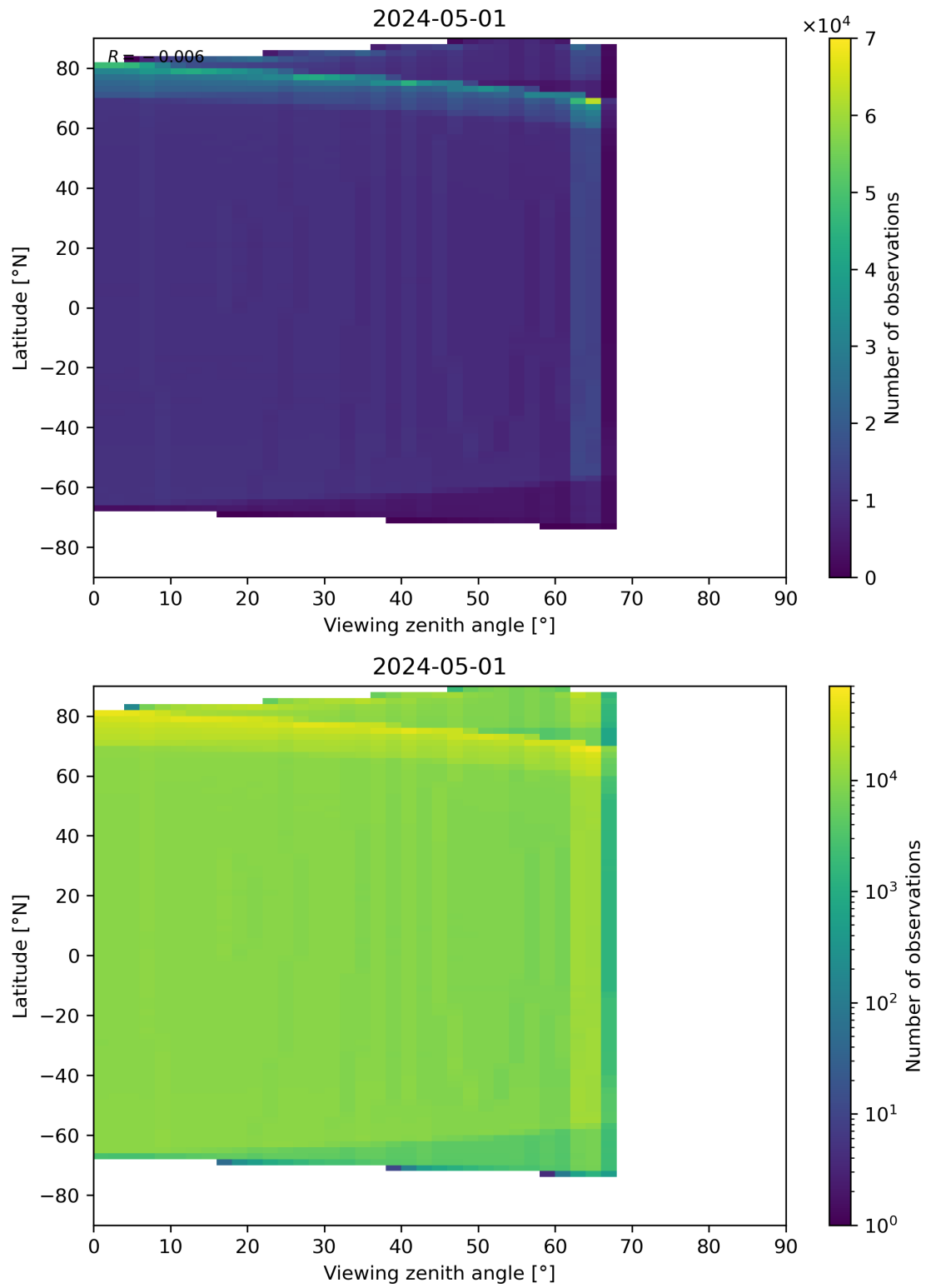
Figure 163: Scatter density plot of “Viewing zenith angle” against “Latitude” for 2024-04-30 to 2024-05-02.
