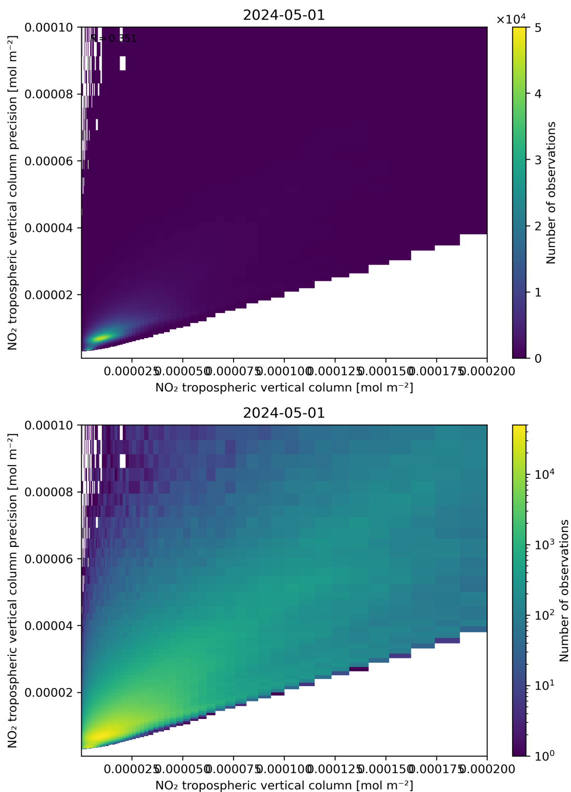
Figure 130: Scatter density plot of “NO 2 tropospheric vertical column” against “NO 2 tropospheric vertical column precision” for 2024-04-30 to 2024-05-02.
