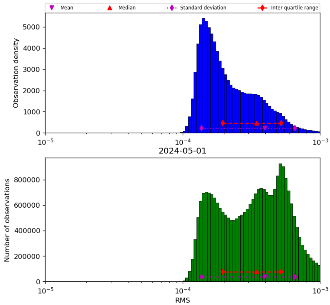
Figure 43: Histogram of “RMS” for 2024-04-30 to 2024-05-02
