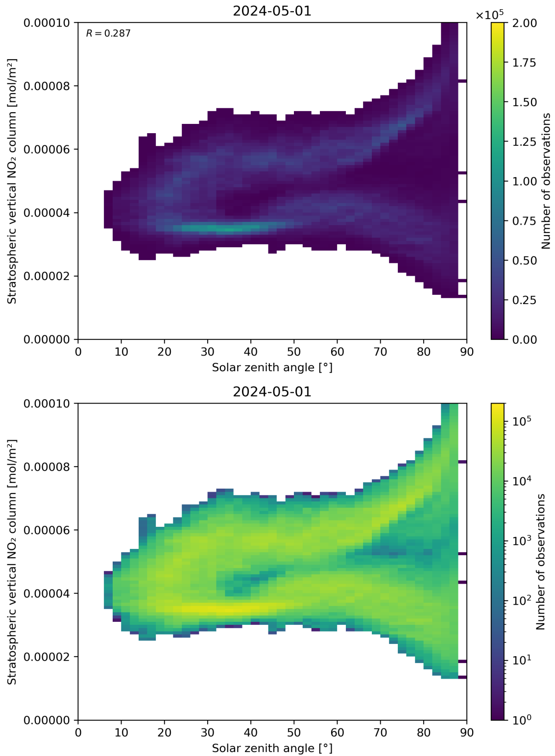
Figure 150: Scatter density plot of “Solar zenith angle” against “Stratospheric vertical NO 2 column” for 2024-04-30 to 2024-05-02.
