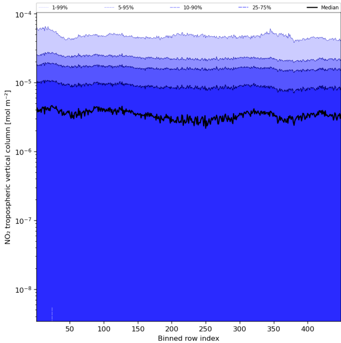
Figure 46: Along track statistics of “NO 2 tropospheric vertical column” for 2024-04-30 to 2024-05-02
