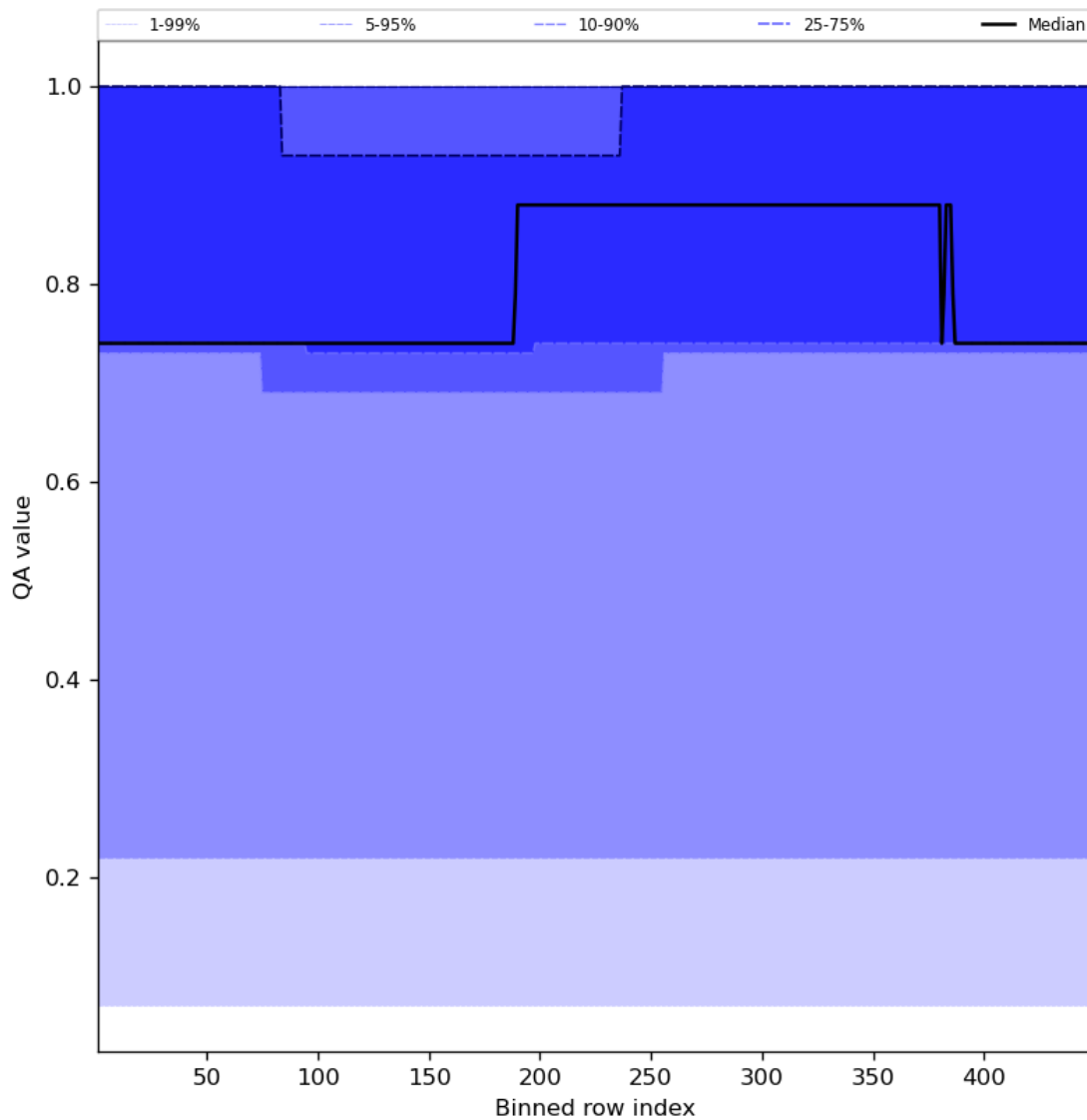
Figure 45: Along track statistics of “QA value” for 2024-04-30 to 2024-05-02
