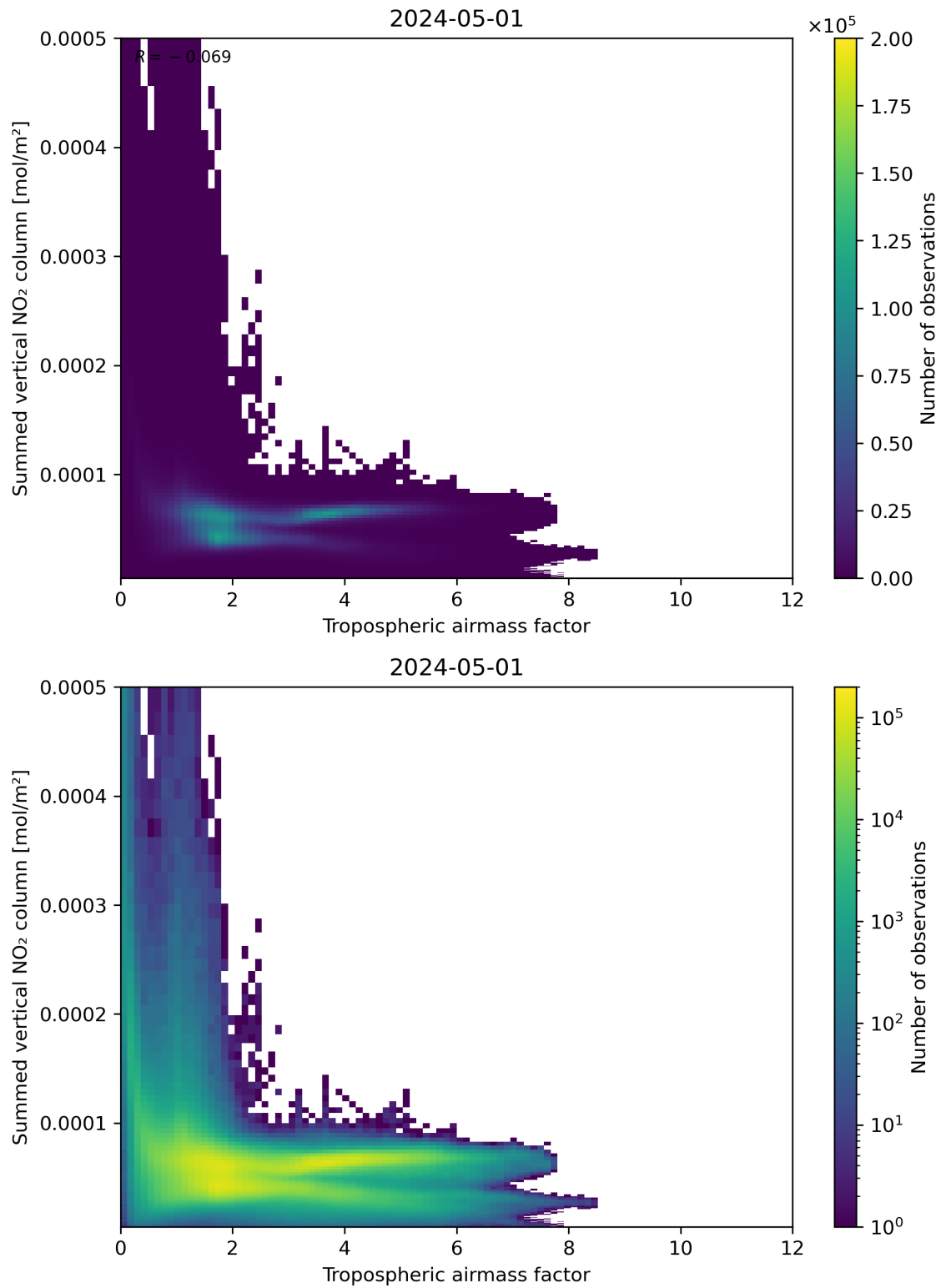
Figure 75: Scatter density plot of “Tropospheric airmass factor” against “Summed vertical NO 2 column” for 2024-04-30 to 2024-05-02.
