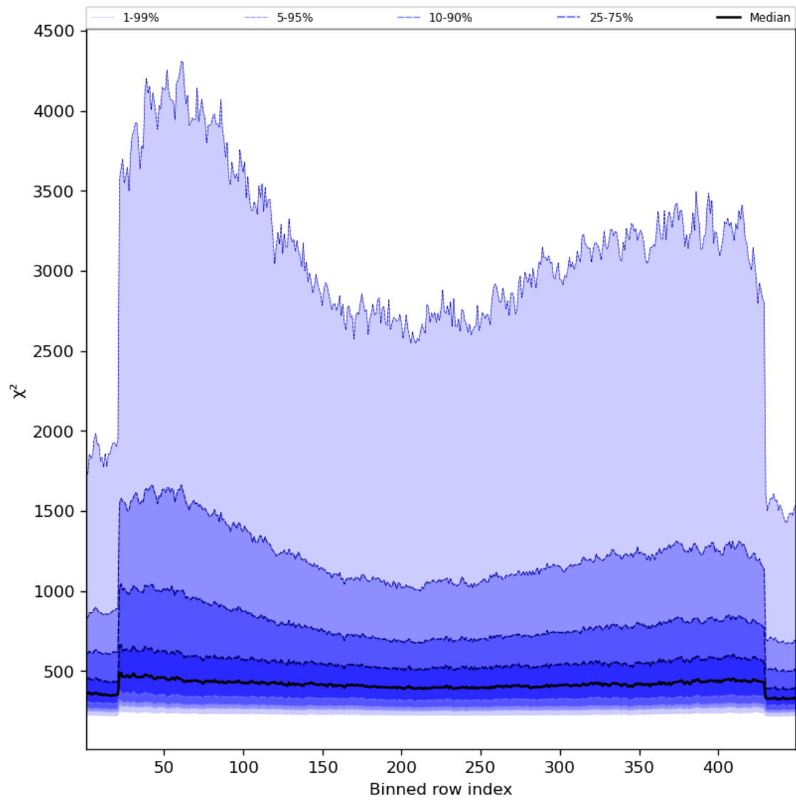
Figure 59: Along track statistics of “ \chi^2 ” for 2024-04-30 to 2024-05-02
