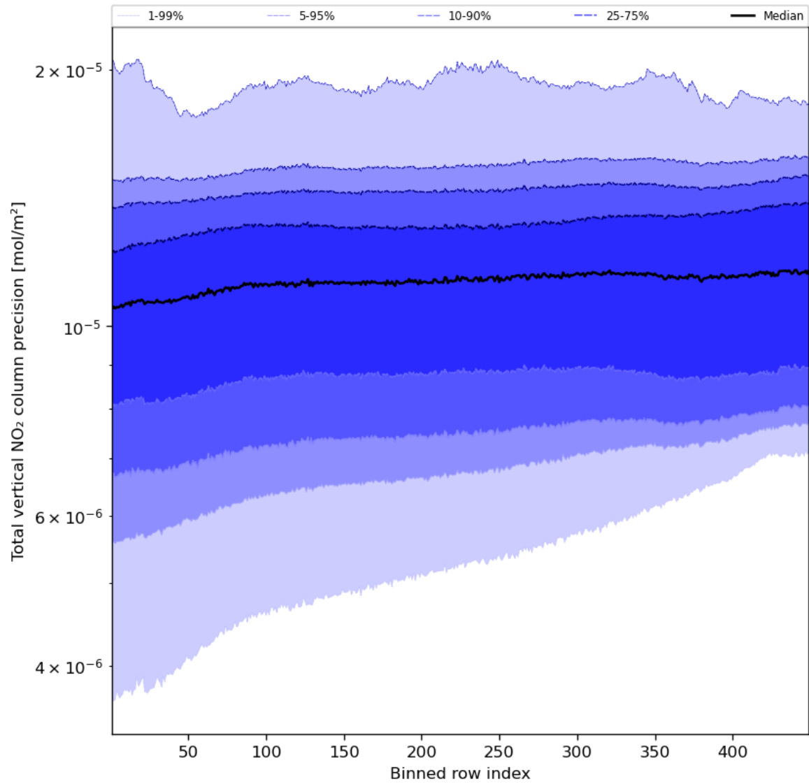
Figure 56: Along track statistics of “Total vertical NO 2 column precision” for 2024-04-30 to 2024-05-02
