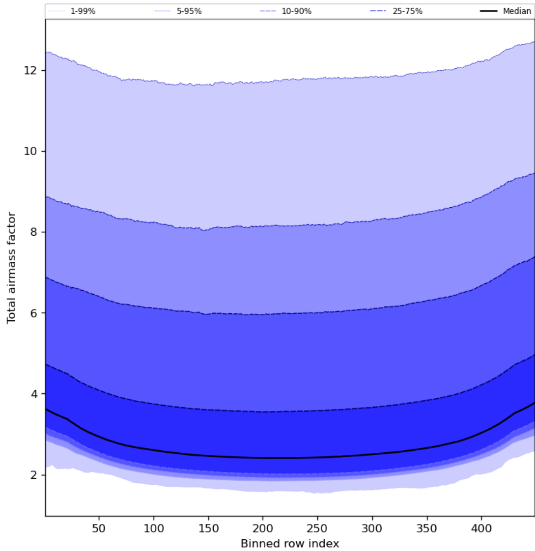
Figure 49: Along track statistics of “Total airmass factor” for 2024-04-30 to 2024-05-02
