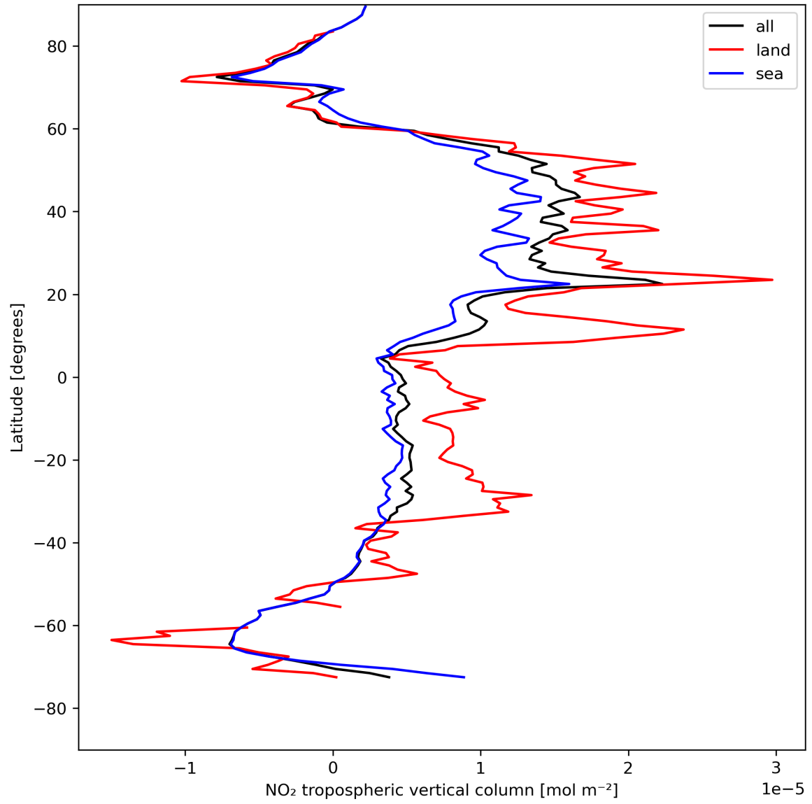
Figure 12: Zonal average of “NO 2 tropospheric vertical column” for 2024-04-30 to 2024-05-02.
