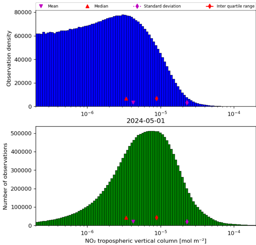
Figure 29: Histogram of “NO 2 tropospheric vertical column” for 2024-04-30 to 2024-05-02
