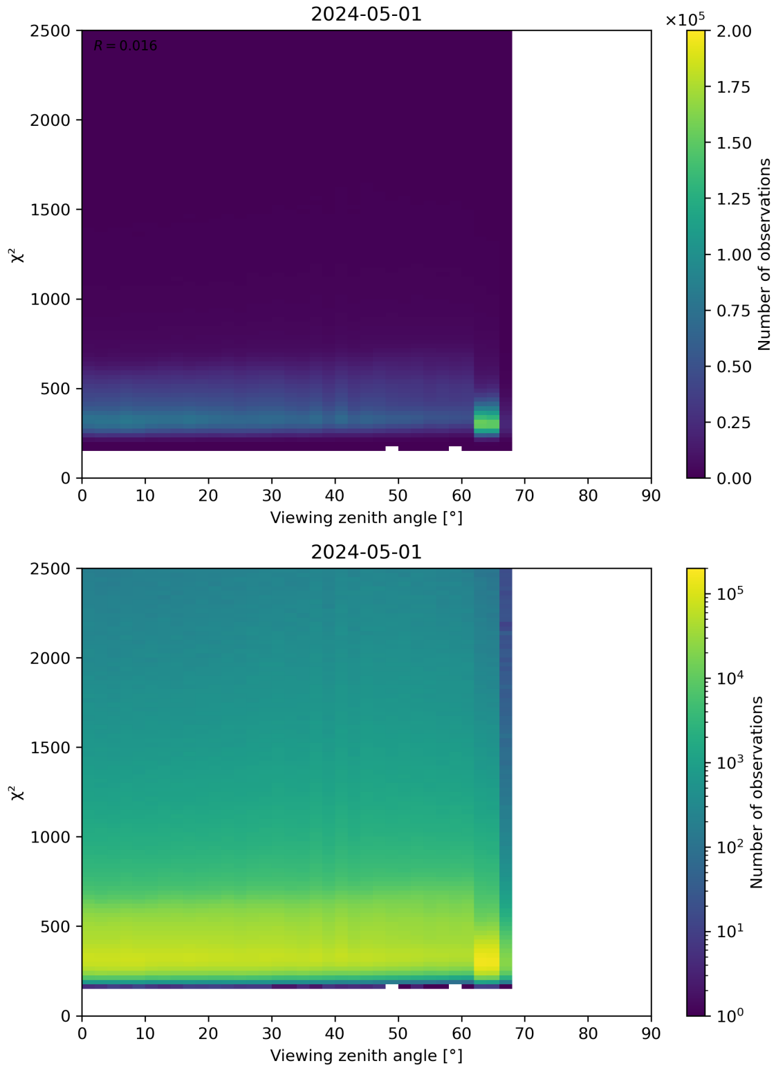
Figure 162: Scatter density plot of “Viewing zenith angle” against “ \chi^2 ” for 2024-04-30 to 2024-05-02.
