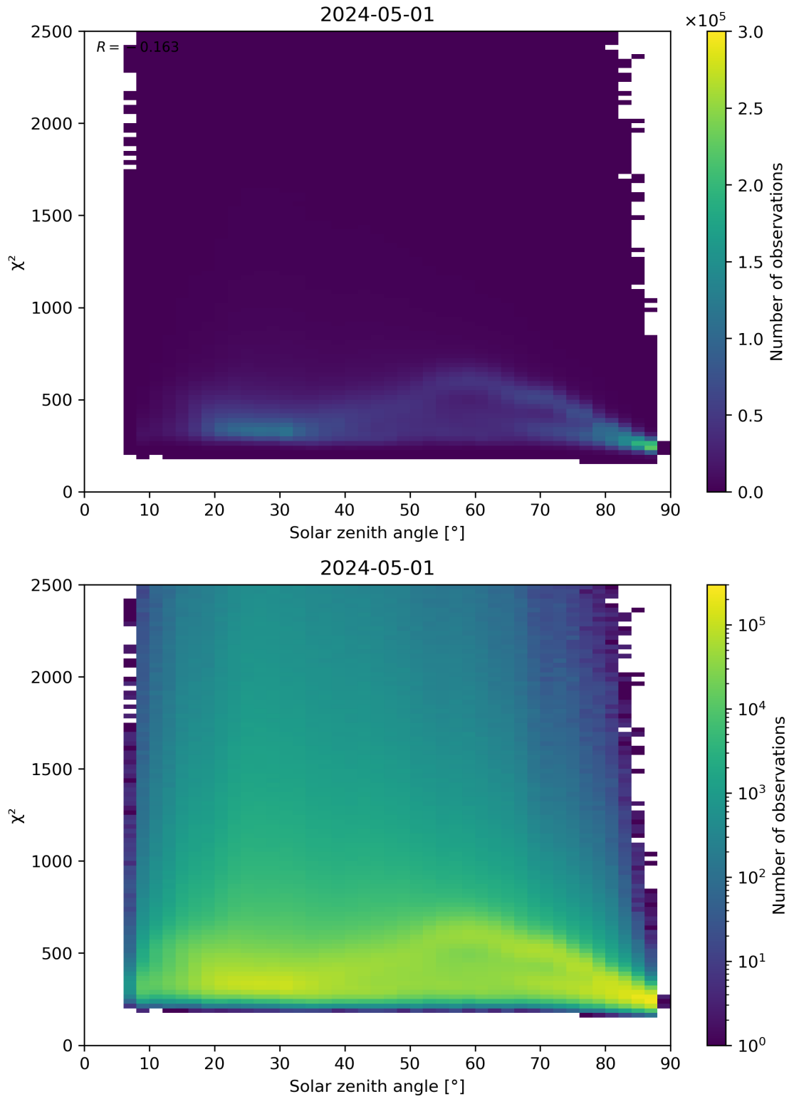
Figure 148: Scatter density plot of “Solar zenith angle” against “ \chi^2 ” for 2024-04-30 to 2024-05-02.
