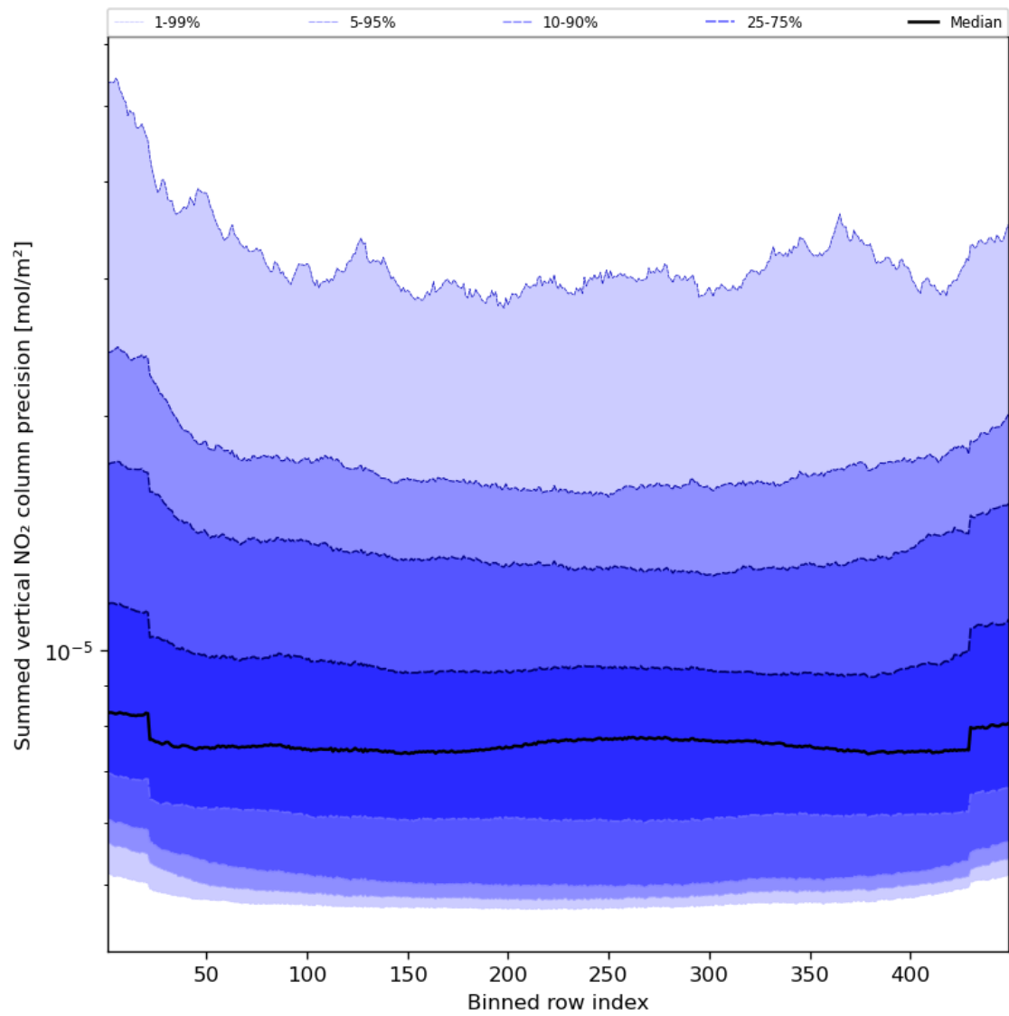
Figure 58: Along track statistics of “Summed vertical NO 2 column precision” for 2024-04-30 to 2024-05-02
