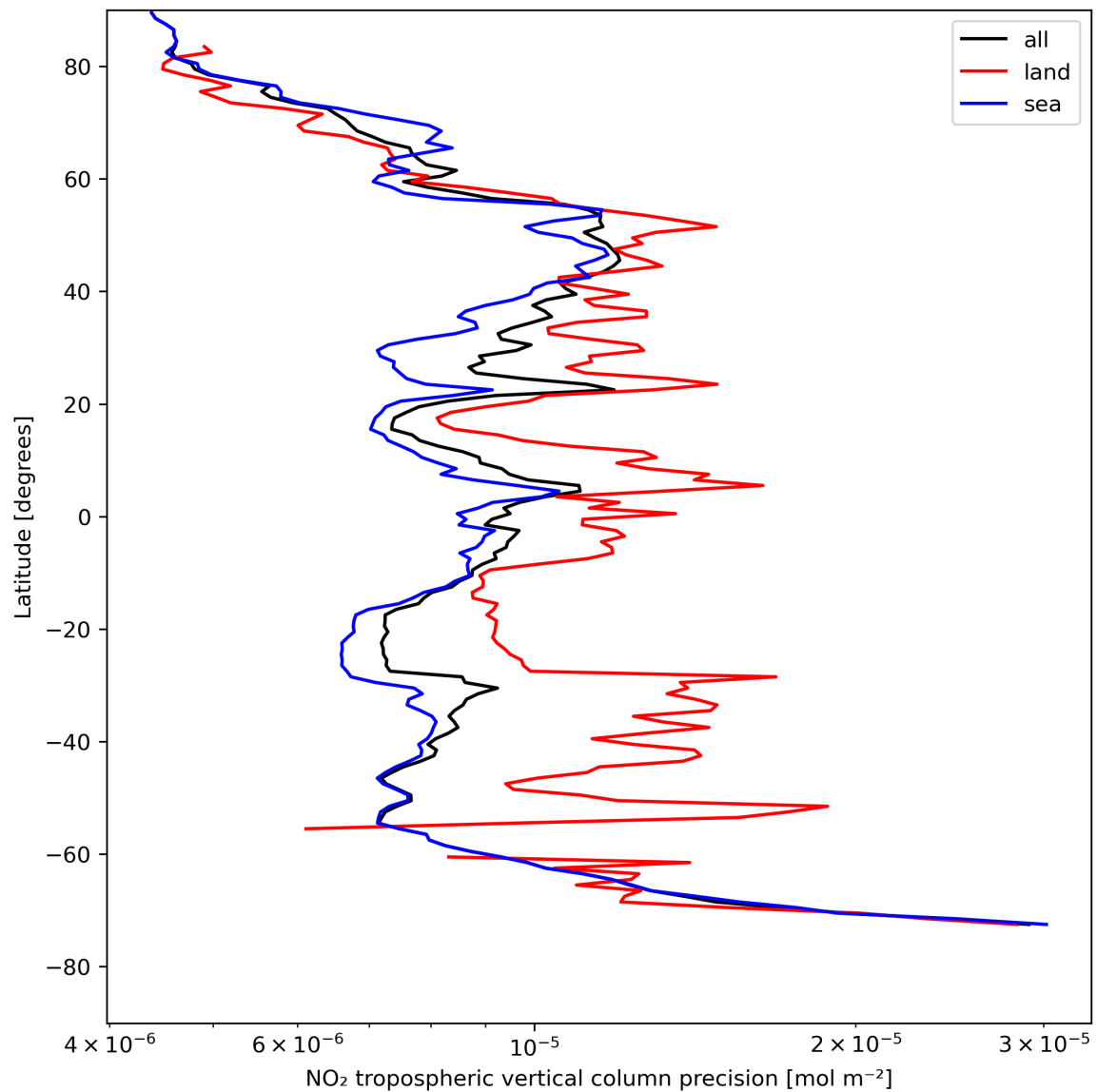
Figure 13: Zonal average of “NO 2 tropospheric vertical column precision” for 2024-04-30 to 2024-05-02.
