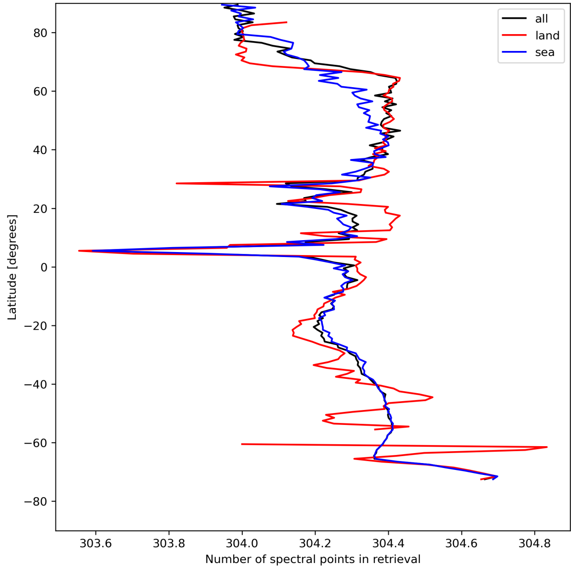
Figure 16: Zonal average of “Number of spectral points in retrieval” for 2024-04-30 to 2024-05-02.
