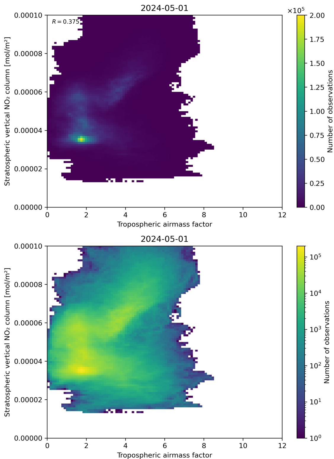
Figure 74: Scatter density plot of “Tropospheric air mass factor” against “Stratospheric vertical NO 2 column” for 2024-04-30 to 2024-05-02.
