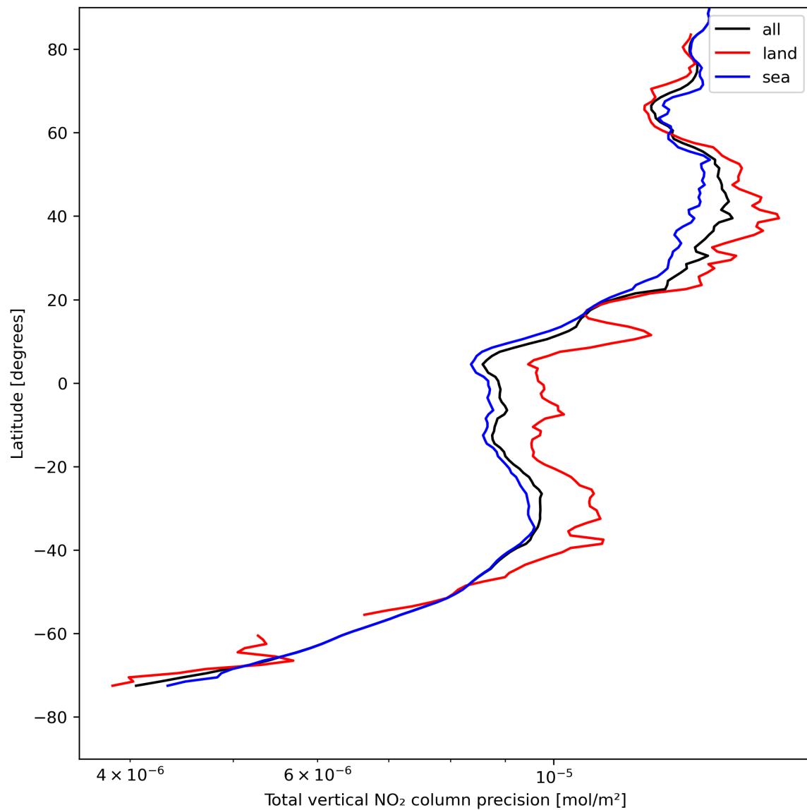
Figure 22: Zonal average of “Total vertical NO 2 column precision” for 2024-04-30 to 2024-05-02.
