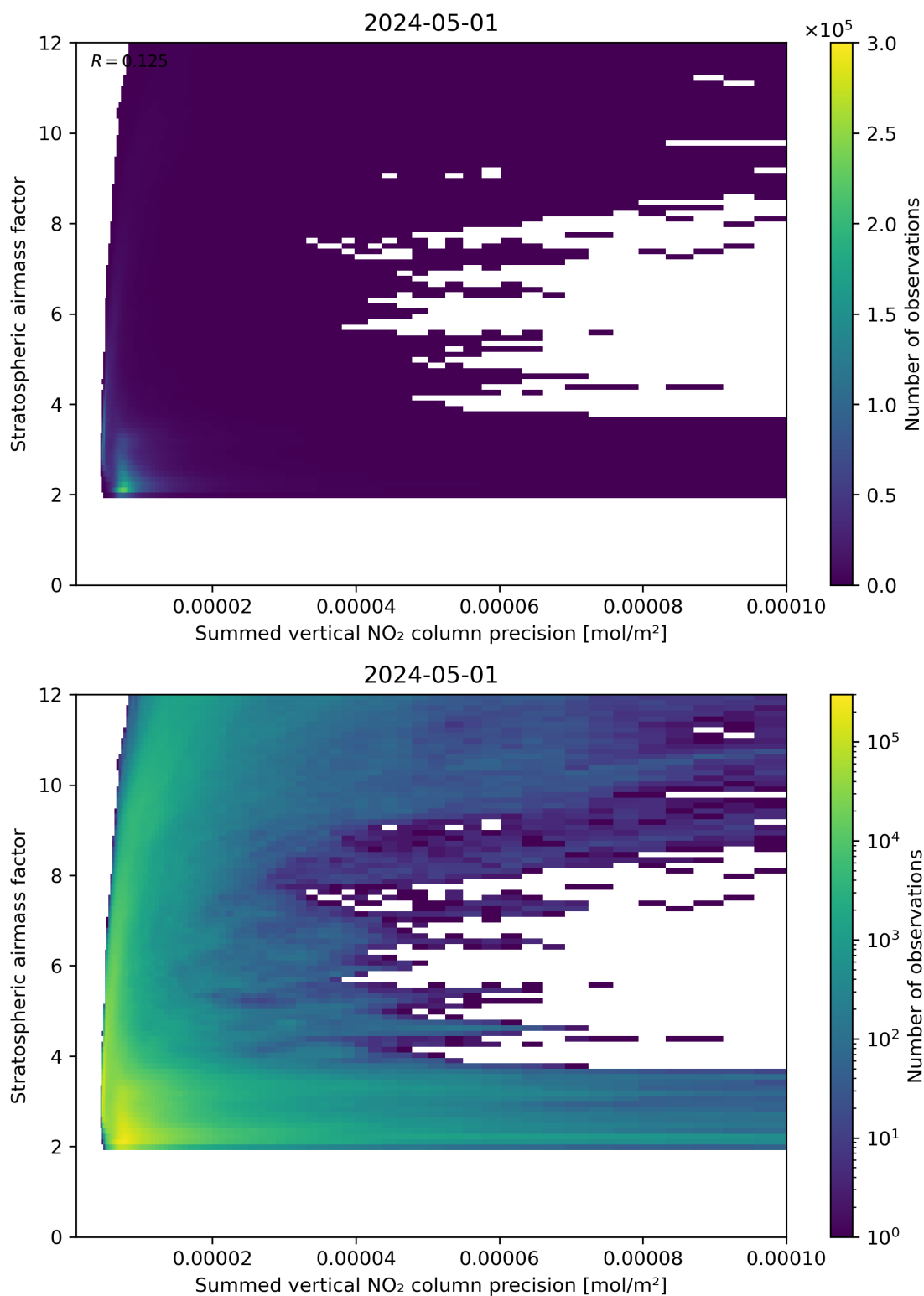
Figure 106: Scatter density plot of “Summed vertical NO 2 column precision” against “Stratospheric airmass factor” for 2024-04-30 to 2024-05-02.
