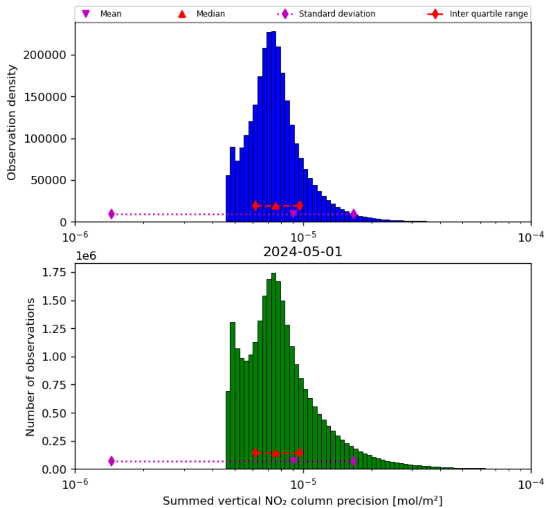
Figure 41: Histogram of "Summed vertical NO 2 column precision" for 2024-04-30 to 2024-05-02
