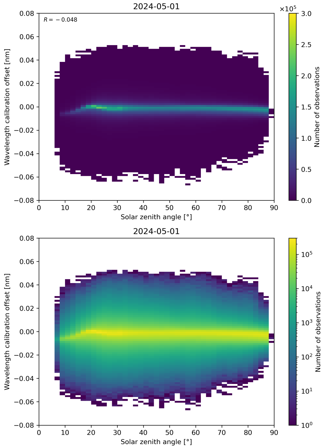
Figure 158: Scatter density plot of “Solar zenith angle” against “Wavelength calibration offset” for 2024-04-30 to 2024-05-02.
