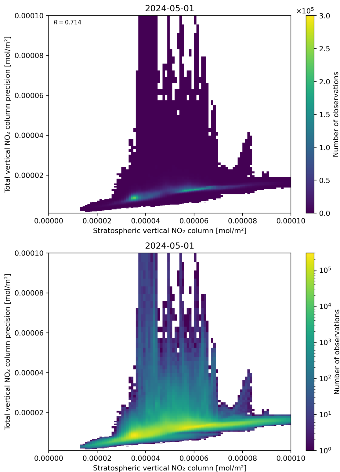
Figure 101: Scatter density plot of “Stratospheric vertical NO 2 column” against “Total vertical NO 2 column precision” for 2024-04-30 to 2024-05-02.
