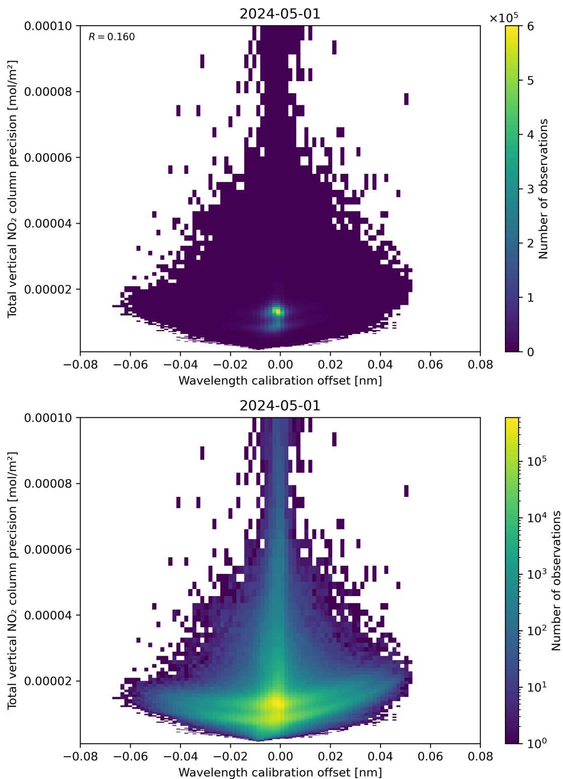
Figure 180: Scatter density plot of “Wavelength calibration offset” against “Total vertical NO 2 column precision” for 2024-04-30 to 2024-05-02.
