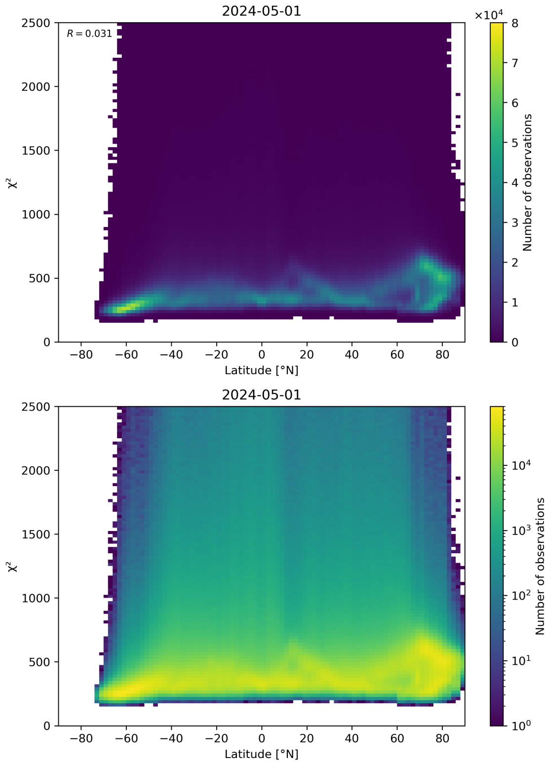
Figure 86: Scatter density plot of “Latitude” against “ \chi^2 ” for 2024-04-30 to 2024-05-02.
