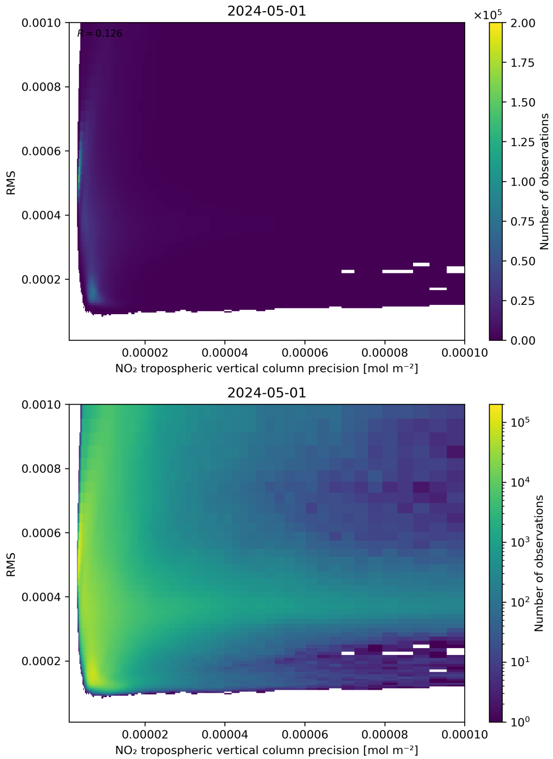
Figure 140: Scatter density plot of “NO 2 tropospheric vertical column precision” against “RMS” for 2024-04-30 to 2024-05-02.
