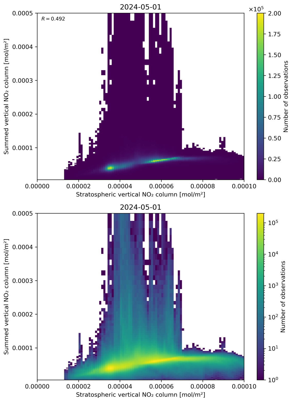
Figure 98: Scatter density plot of “Stratospheric vertical NO 2 column” against “Summed vertical NO 2 column” for 2024-04-30 to 2024-05-02.
