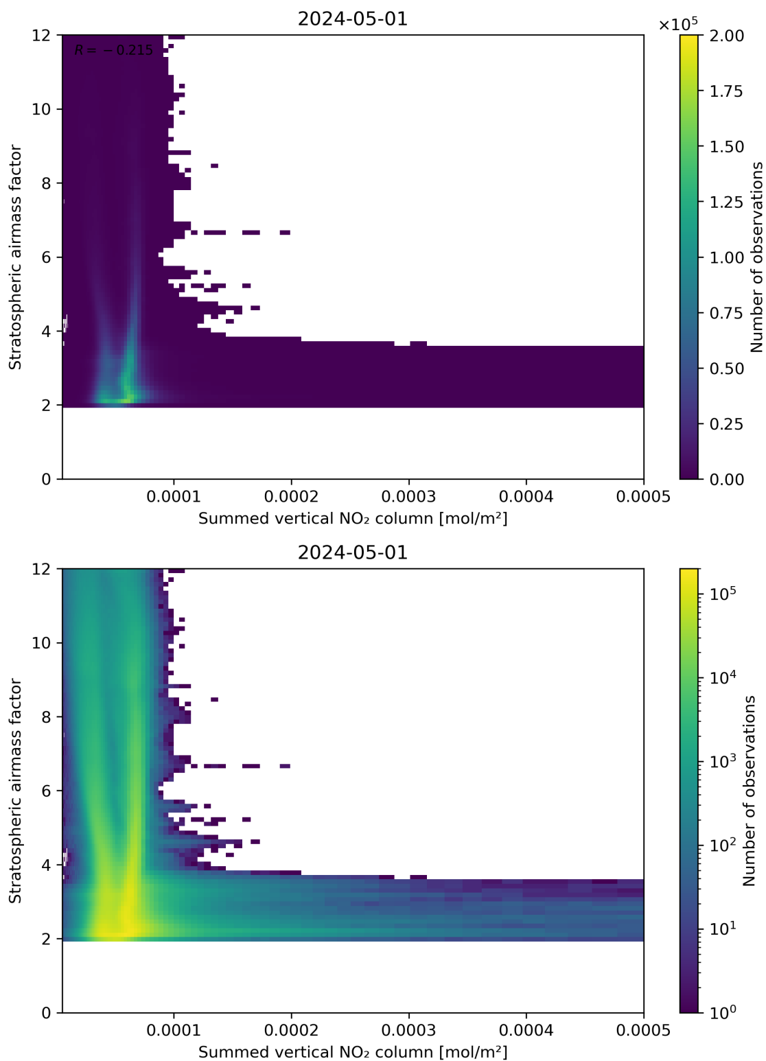
Figure 103: Scatter density plot of “Summed vertical NO 2 column” against “Stratospheric airmass factor” for 2024-04-30 to 2024-05-02.
