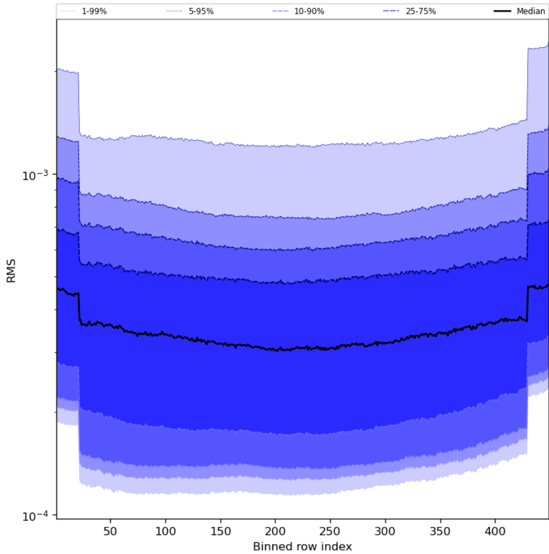
Figure 60: Along track statistics of “RMS” for 2024-04-30 to 2024-05-02
