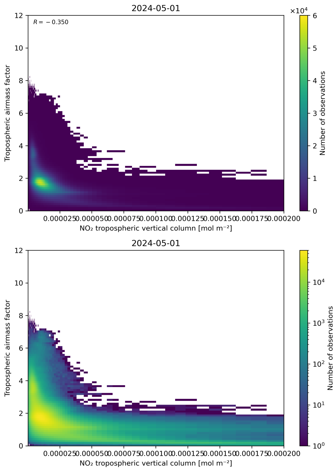
Figure 123: Scatter density plot of “NO 2 tropospheric vertical column” against “Tropospheric air mass factor” for 2024-04-30 to 2024-05-02.
