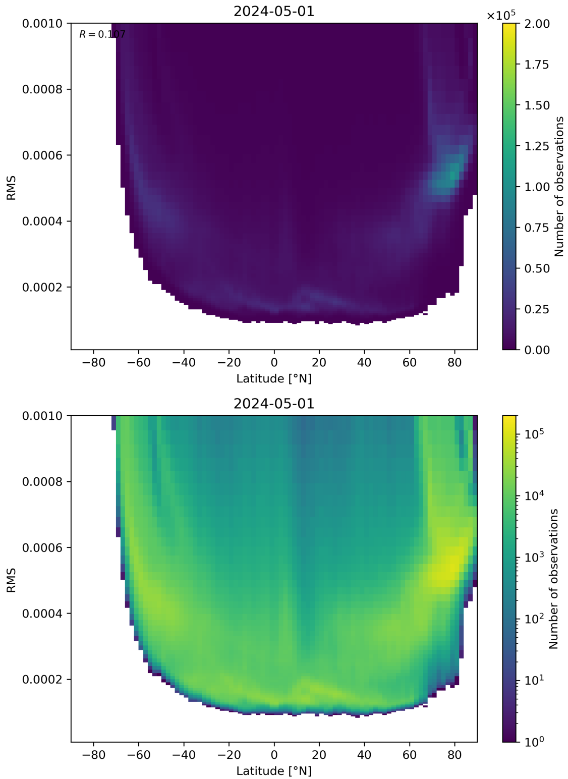
Figure 94: Scatter density plot of “Latitude” against “RMS” for 2024-04-30 to 2024-05-02.
