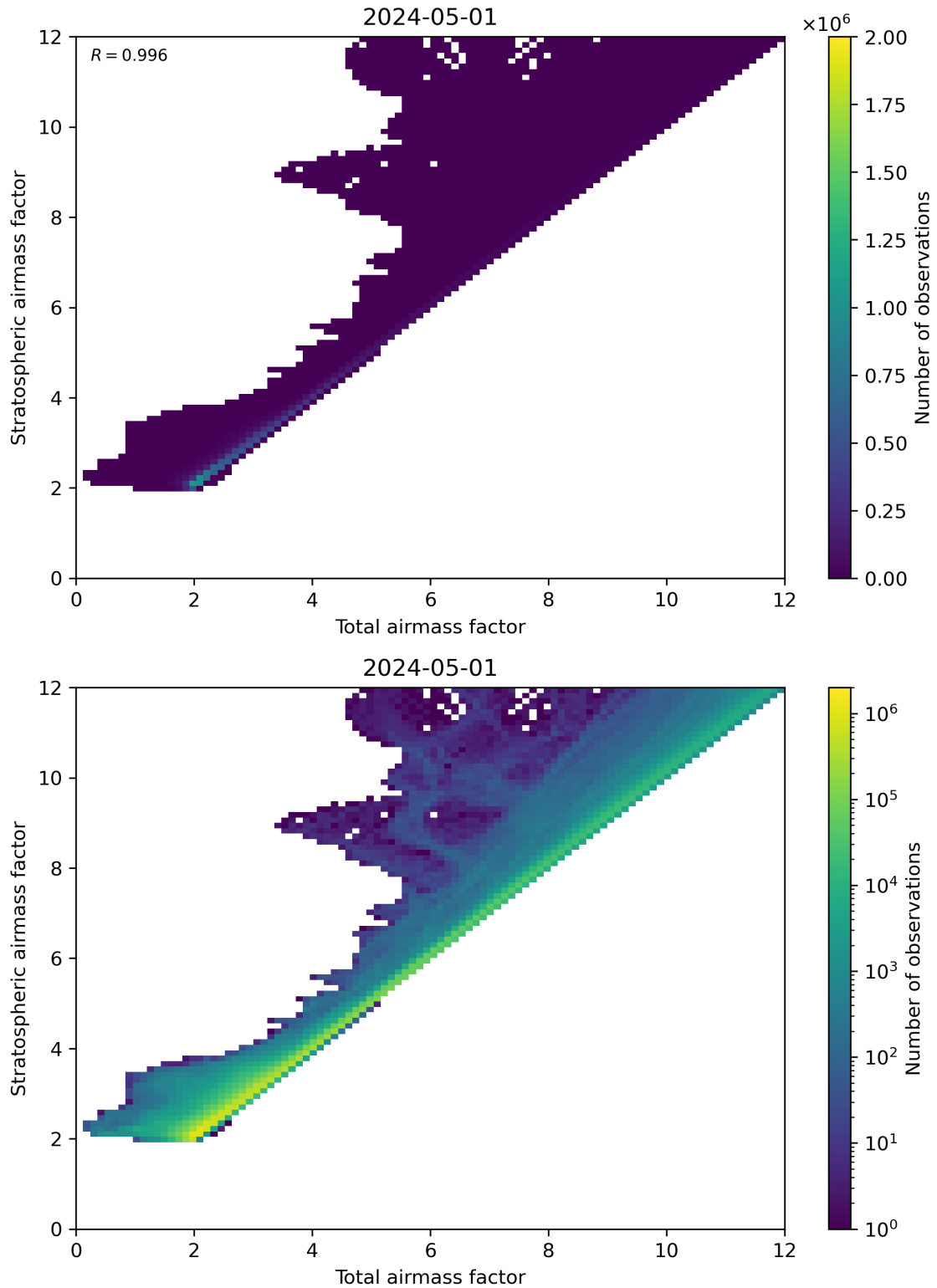
Figure 62: Scatter density plot of “Total airmass factor” against “Stratospheric airmass factor” for 2024-04-30 to 2024-05-02.
