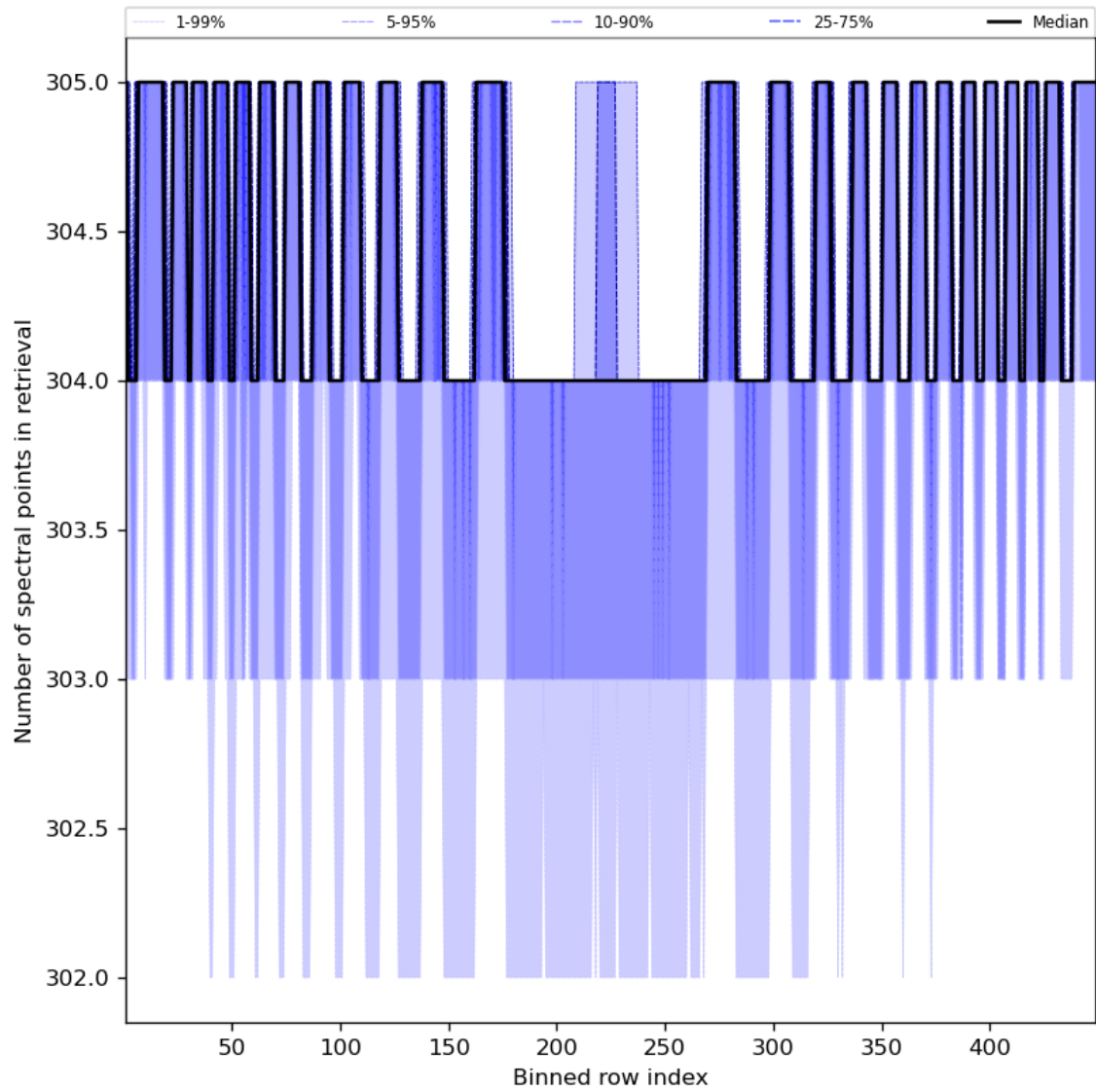
Figure 50: Along track statistics of “Number of spectral points in retrieval” for 2024-05-02 to 2024-05-03
