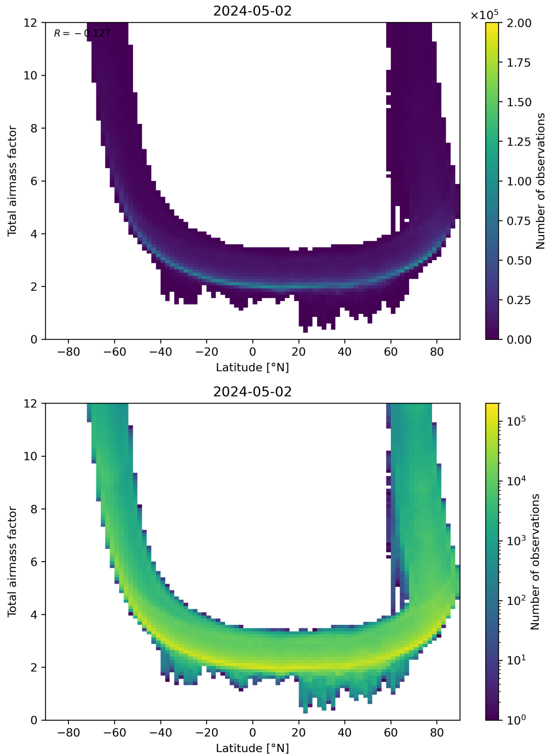
Figure 84: Scatter density plot of “Latitude” against “Total airmass factor” for 2024-05-02 to 2024-05-03.
