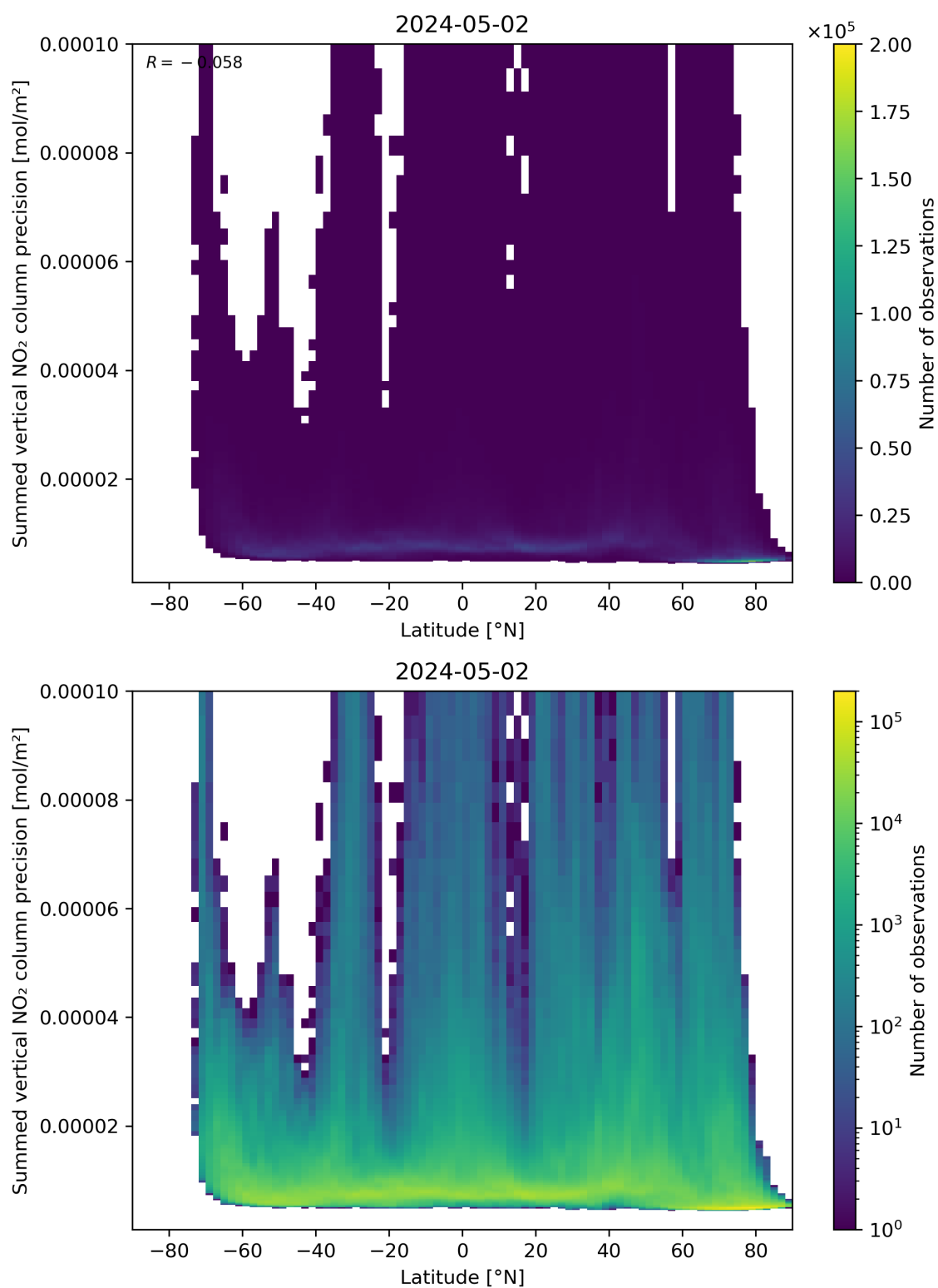
Figure 89: Scatter density plot of “Latitude” against “Summed vertical NO 2 column precision” for 2024-05-02 to 2024-05-03.
