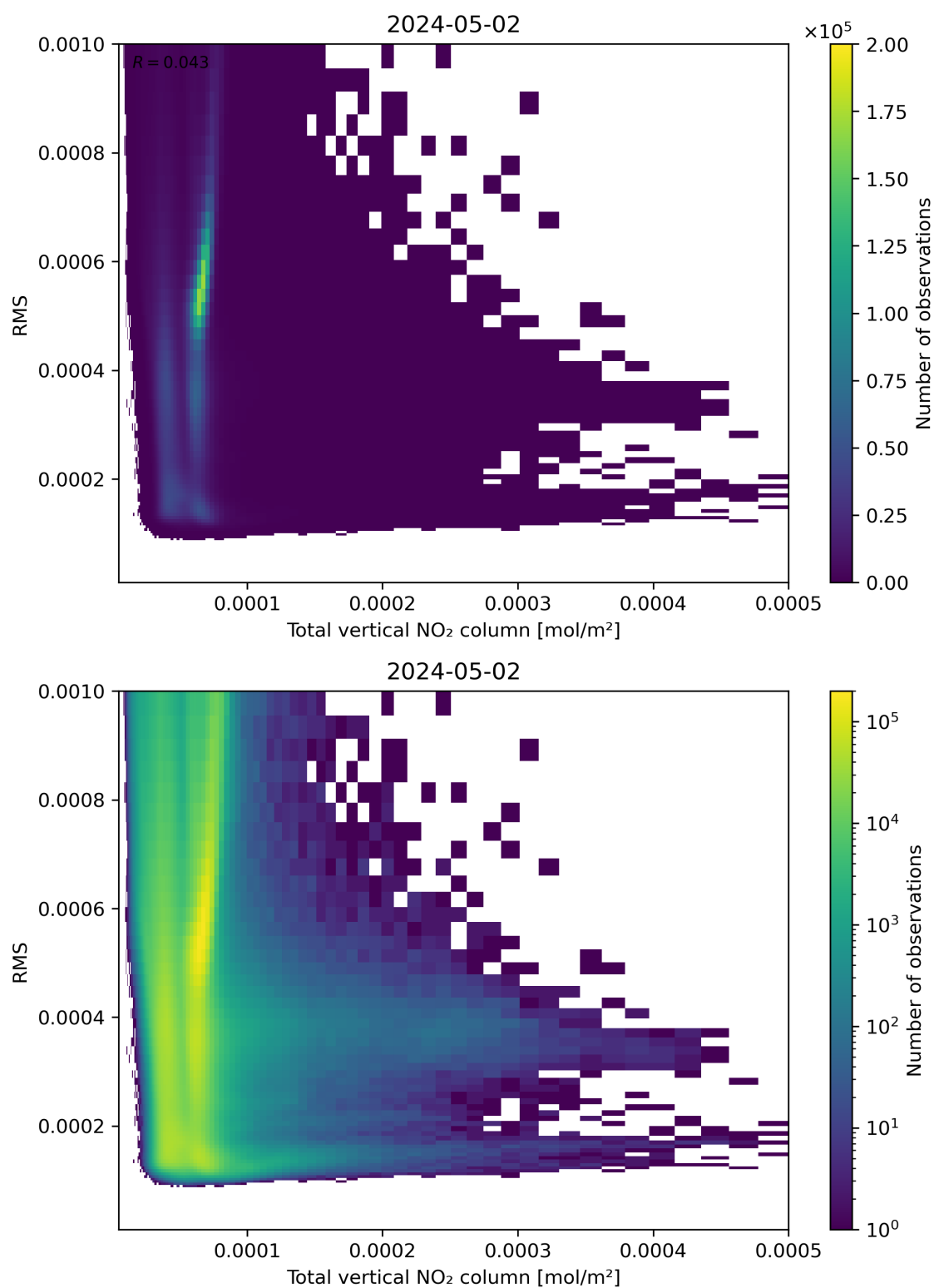
Figure 120: Scatter density plot of “Total vertical NO 2 column” against “RMS” for 2024-05-02 to 2024-05-03.
