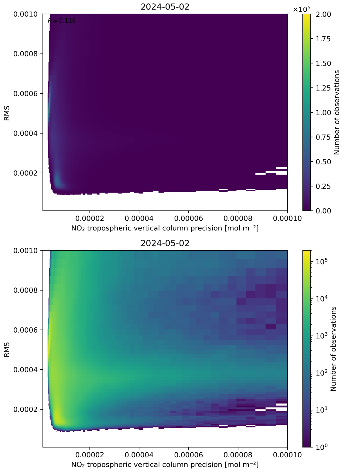
Figure 140: Scatter density plot of “NO 2 tropospheric vertical column precision” against “RMS” for 2024-05-02 to 2024-05-03.
