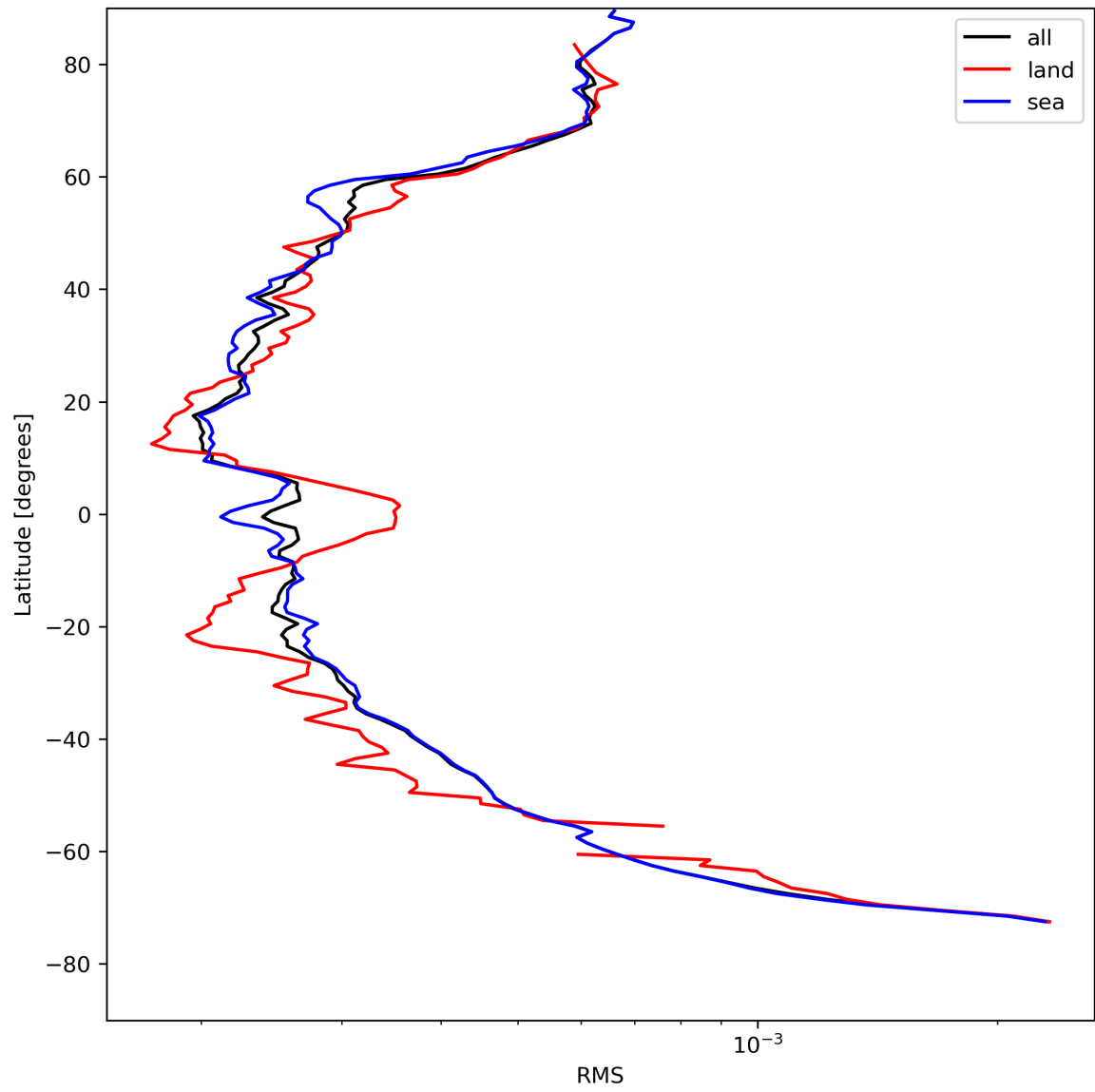
Figure 26: Zonal average of “RMS” for 2024-05-02 to 2024-05-03.
