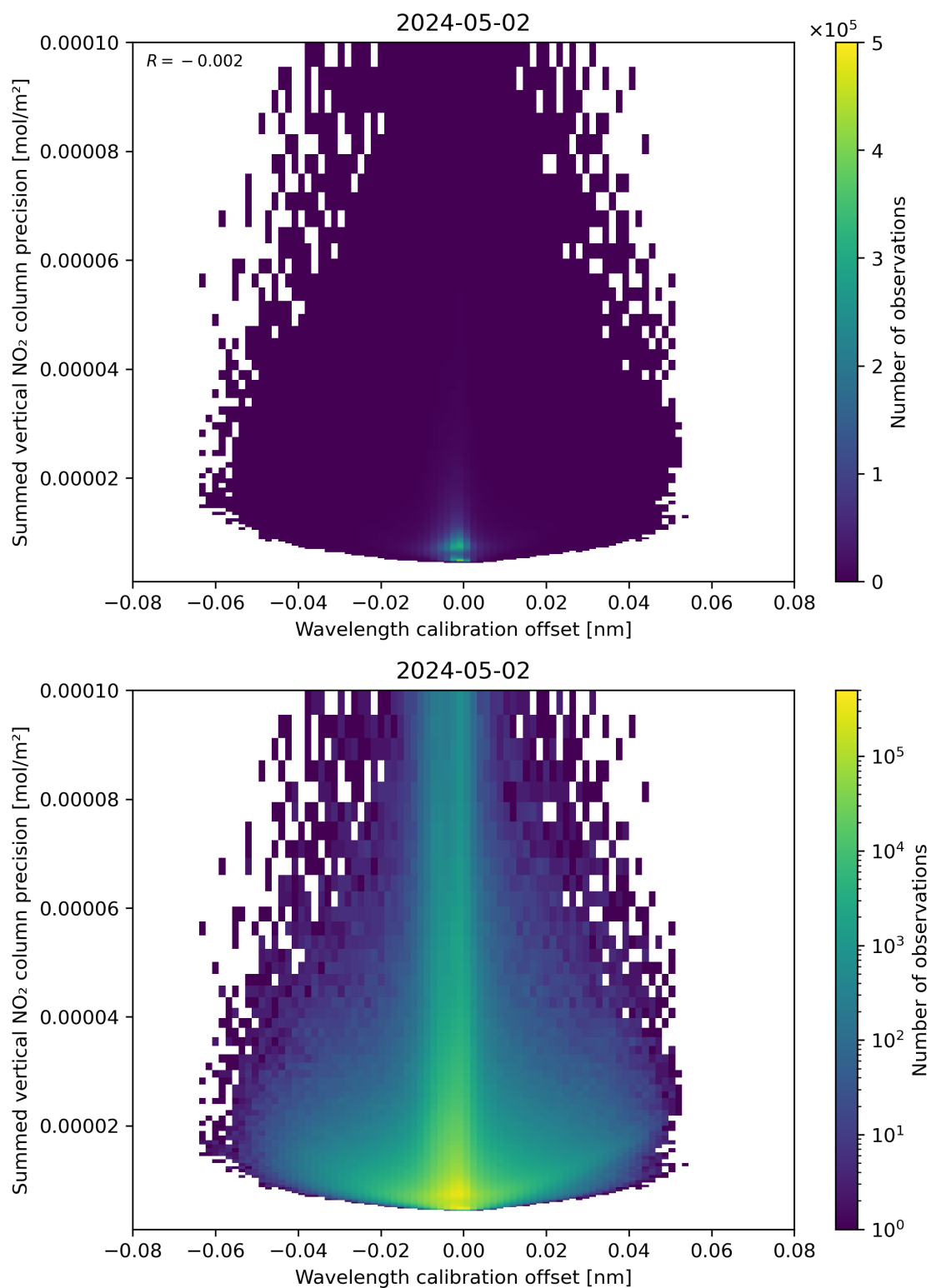
Figure 178: Scatter density plot of “Wavelength calibration offset” against “Summed vertical NO 2 column precision” for 2024-05-02 to 2024-05-03.
