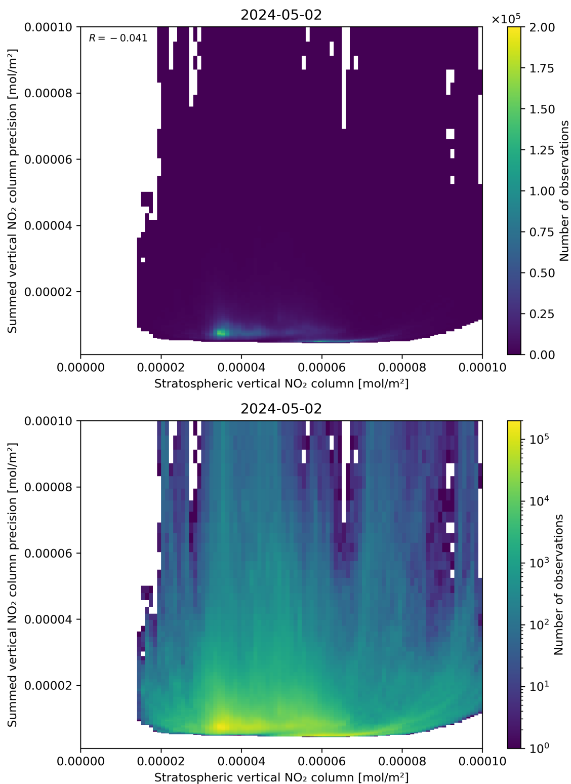
Figure 99: Scatter density plot of “Stratospheric vertical NO 2 column” against “Summed vertical NO 2 column precision” for 2024-05-02 to 2024-05-03.
