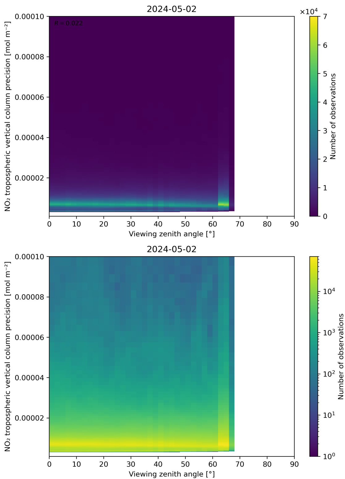
Figure 170: Scatter density plot of “Viewing zenith angle” against “NO 2 tropospheric vertical column precision” for 2024-05-02 to 2024-05-03.
