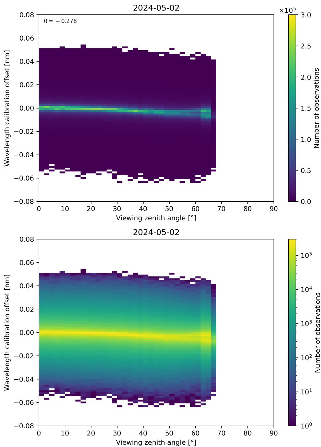
Figure 173: Scatter density plot of “Viewing zenith angle” against “Wavelength calibration offset” for 2024-05-02 to 2024-05-03.
