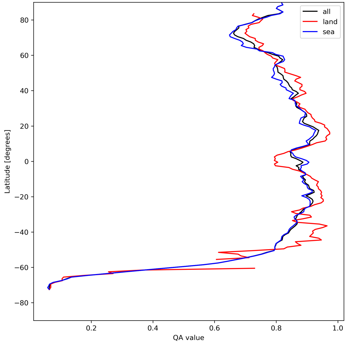
Figure 11: Zonal average of “QA value” for 2024-05-02 to 2024-05-03.
