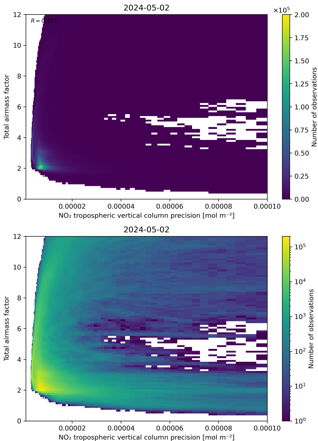
Figure 132: Scatter density plot of “NO 2 tropospheric vertical column precision” against “Total air mass factor” for 2024-05-02 to 2024-05-03.
