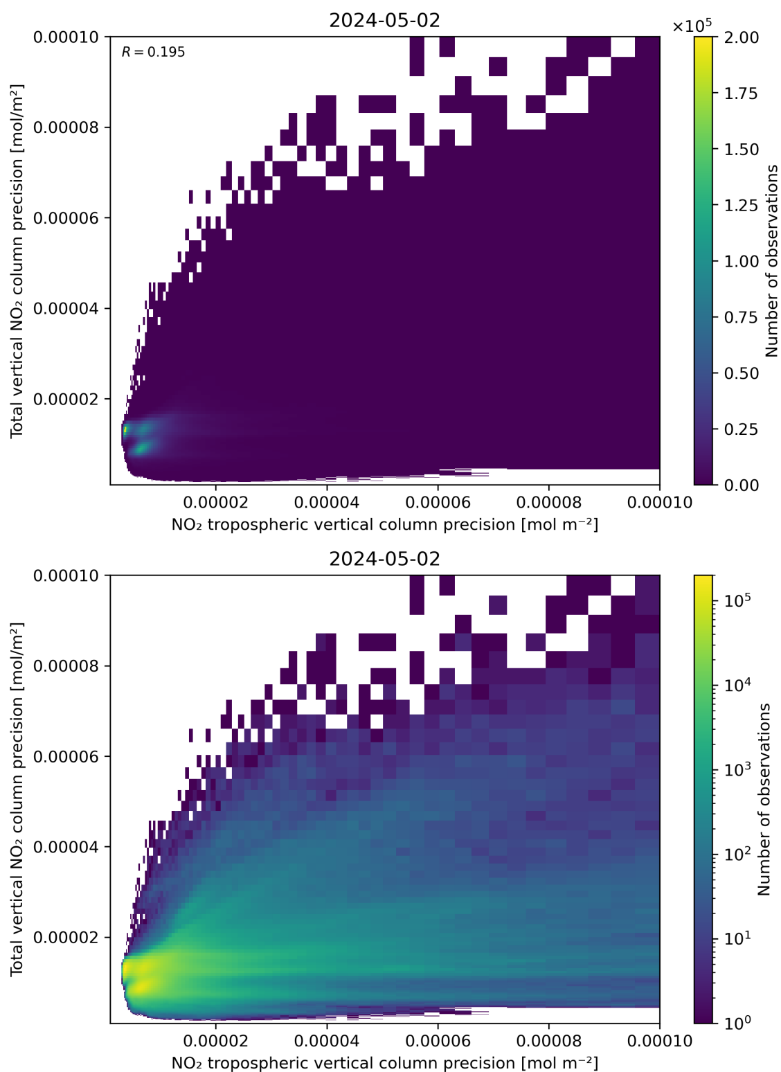
Figure 139: Scatter density plot of “NO 2 tropospheric vertical column precision” against “Total vertical NO 2 column precision” for 2024-05-02 to 2024-05-03.
