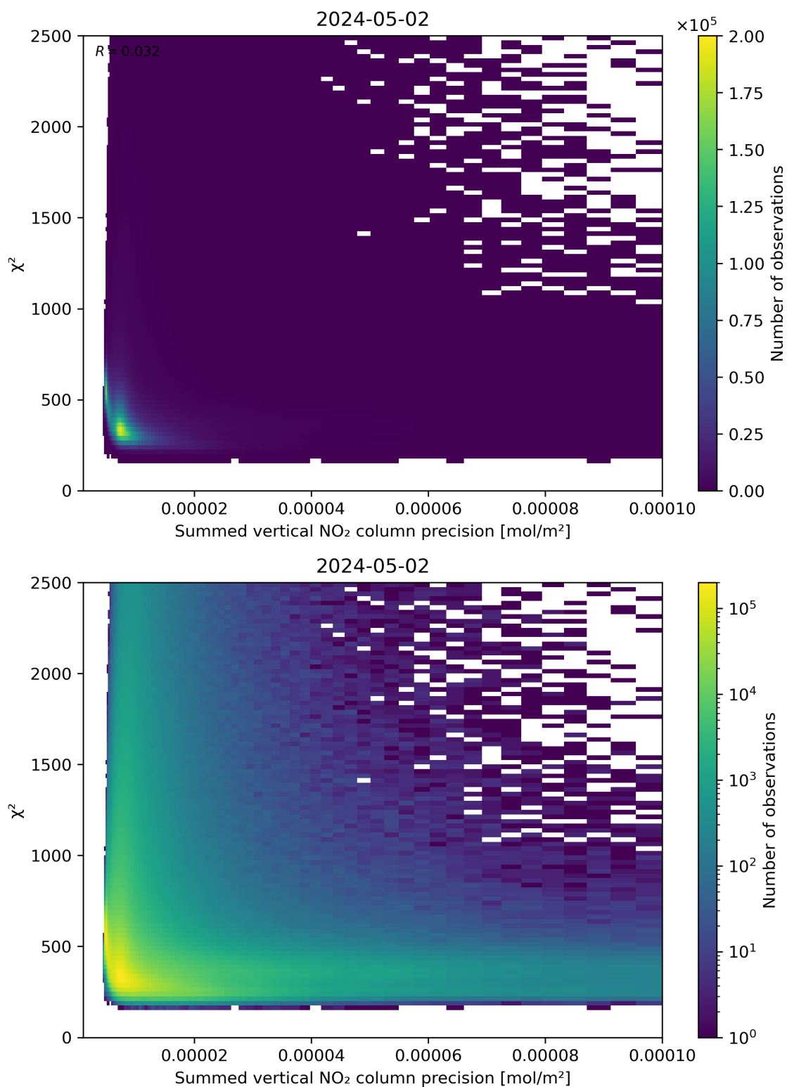
Figure 107: Scatter density plot of “Summed vertical NO 2 column precision” against “ \chi^2 ” for 2024-05-02 to 2024-05-03.
