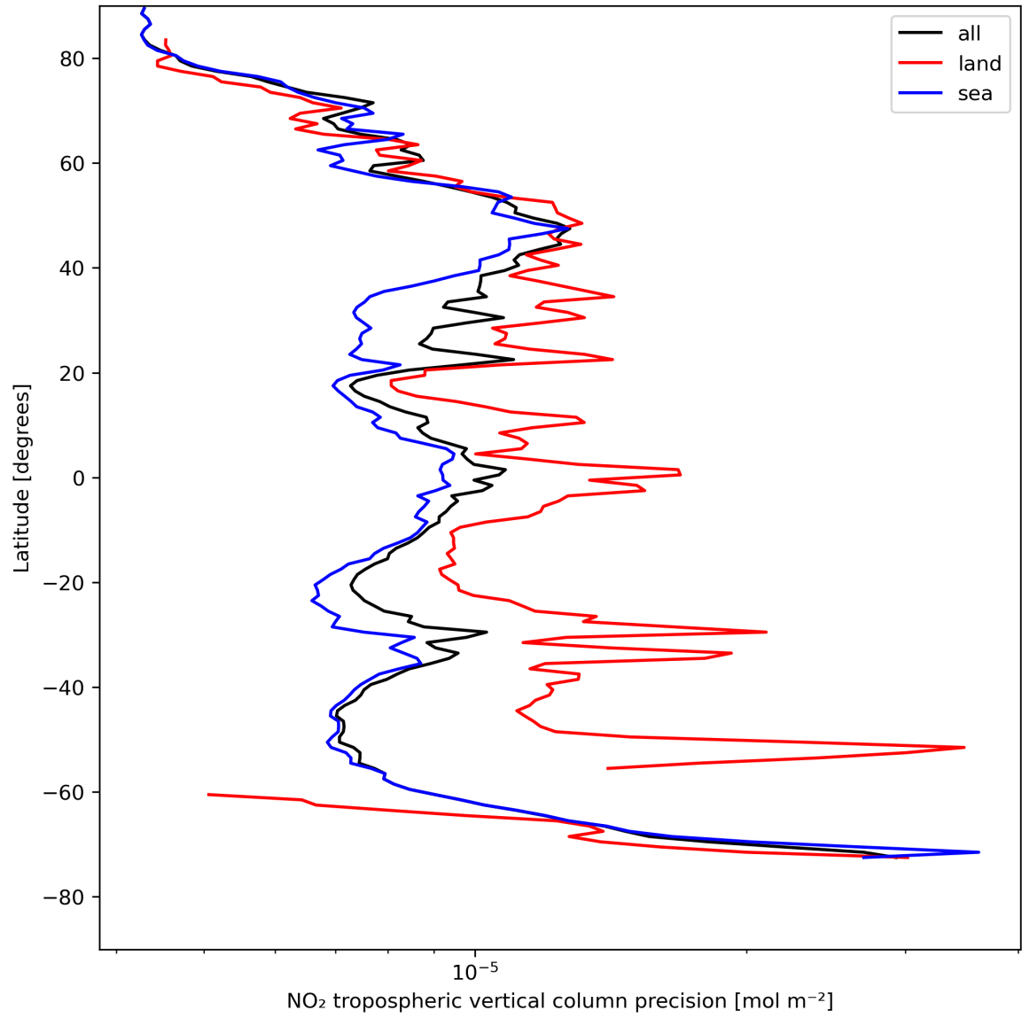
Figure 13: Zonal average of “NO 2 tropospheric vertical column precision” for 2024-05-02 to 2024-05-03.
