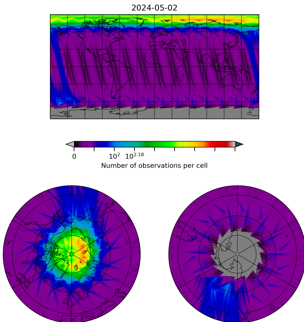
Figure 10: Map of the number of observations for 2024-05-02 to 2024-05-03
