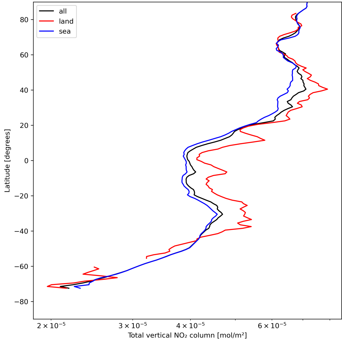
Figure 21: Zonal average of “Total vertical NO 2 column” for 2024-05-02 to 2024-05-03.
