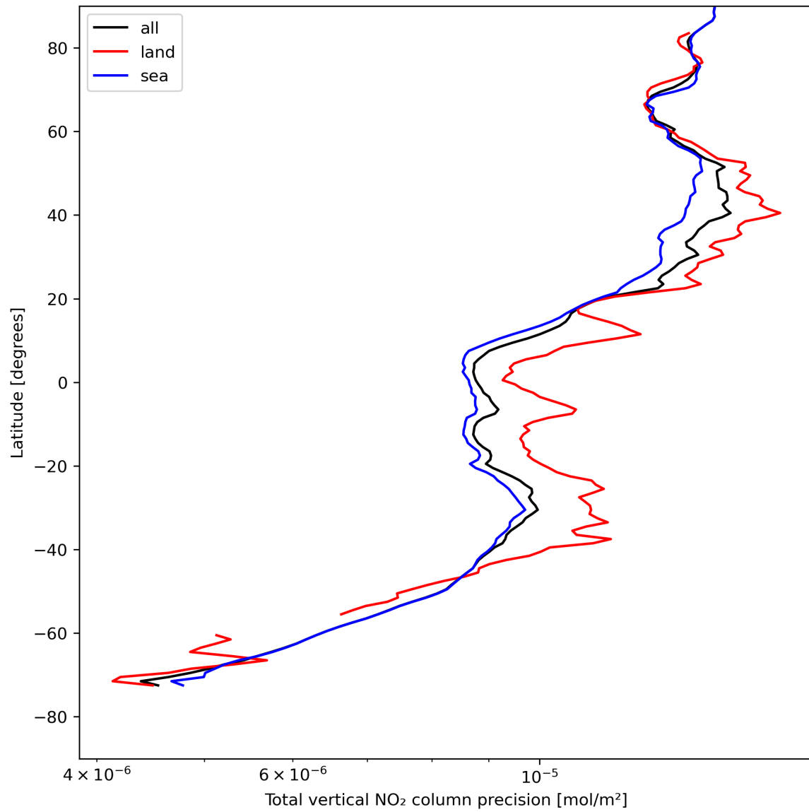
Figure 22: Zonal average of “Total vertical NO 2 column precision” for 2024-05-02 to 2024-05-03.
