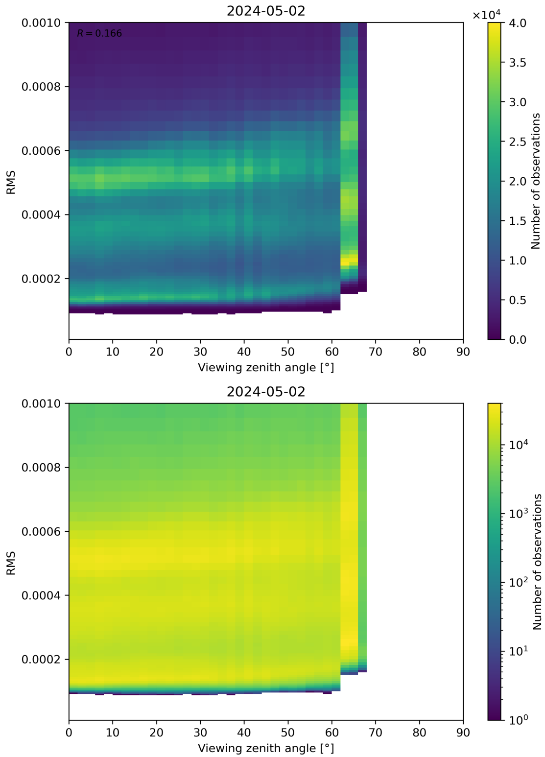
Figure 171: Scatter density plot of “Viewing zenith angle” against “RMS” for 2024-05-02 to 2024-05-03.
