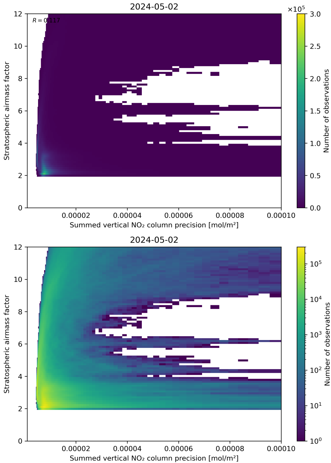
Figure 106: Scatter density plot of “Summed vertical NO 2 column precision” against “Stratospheric airmass factor” for 2024-05-02 to 2024-05-03.
