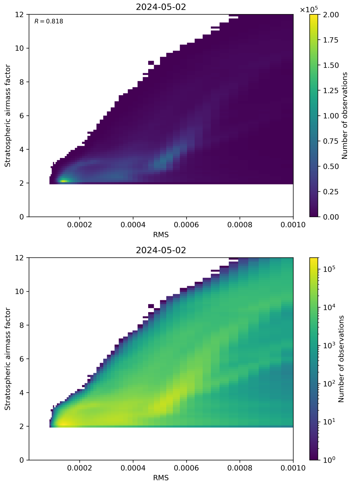
Figure 144: Scatter density plot of “RMS” against “Stratospheric airmass factor” for 2024-05-02 to 2024-05-03.
