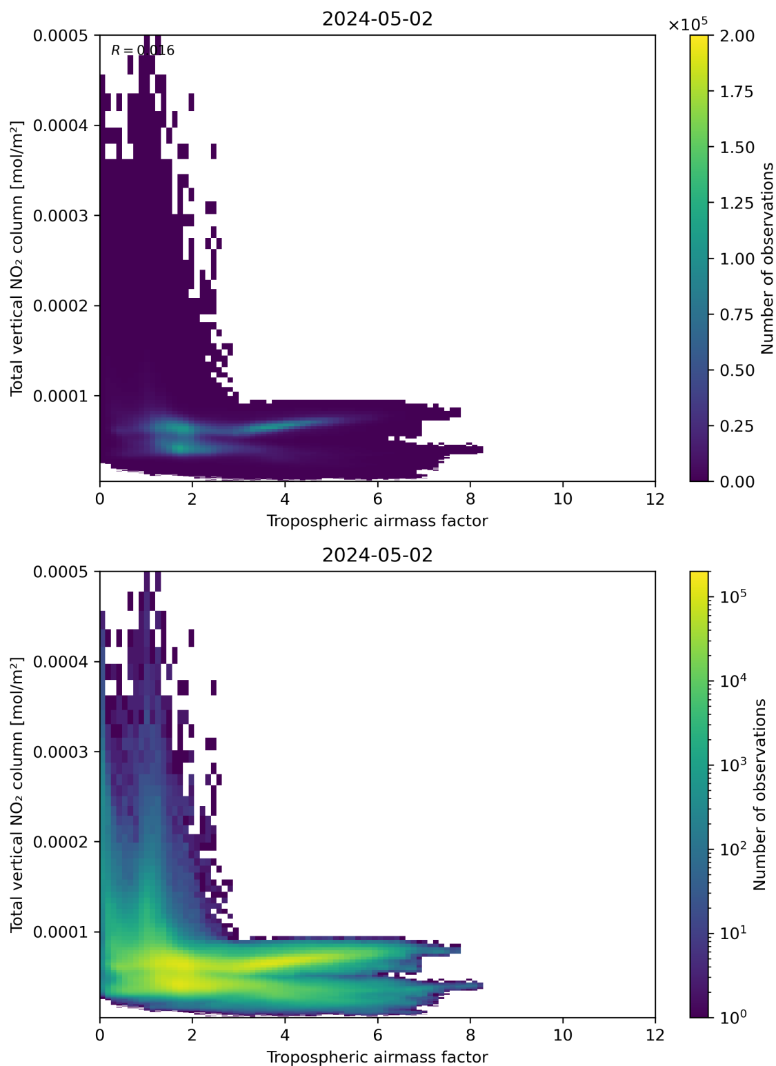
Figure 77: Scatter density plot of “Tropospheric airmass factor” against “Total vertical NO 2 column” for 2024-05-02 to 2024-05-03.
