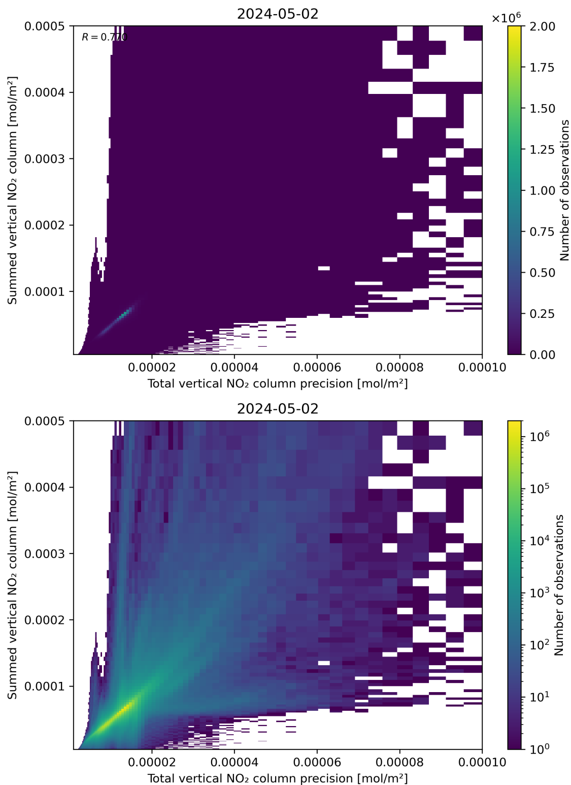
Figure 117: Scatter density plot of “Total vertical NO 2 column precision” against “Summed vertical NO 2 column” for 2024-05-02 to 2024-05-03.
