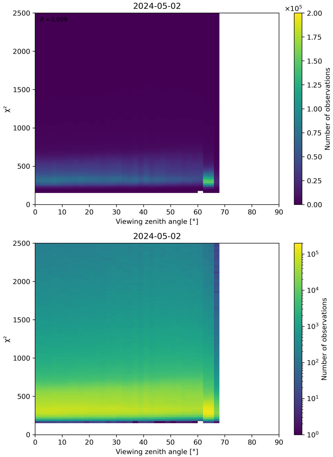
Figure 162: Scatter density plot of “Viewing zenith angle” against “ \chi^2 ” for 2024-05-02 to 2024-05-03.
