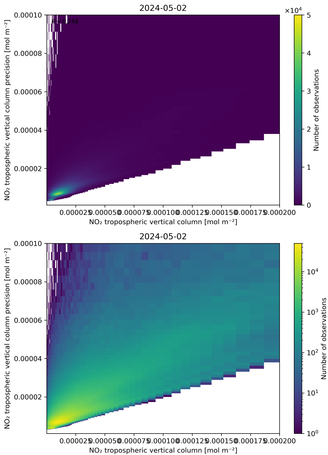
Figure 130: Scatter density plot of “NO 2 tropospheric vertical column” against “NO 2 tropospheric vertical column precision” for 2024-05-02 to 2024-05-03.
