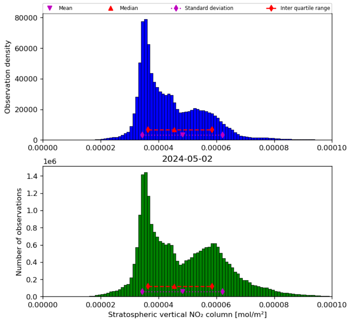
Figure 36: Histogram of “Stratospheric vertical NO 2 column” for 2024-05-02 to 2024-05-03
