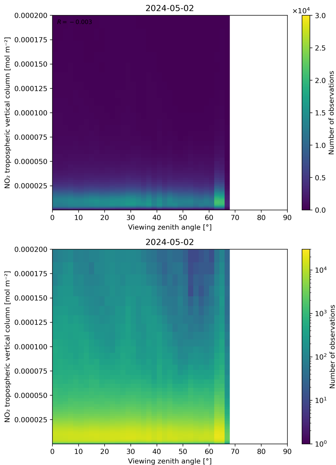
Figure 169: Scatter density plot of “Viewing zenith angle” against “NO 2 tropospheric vertical column” for 2024-05-02 to 2024-05-03.
