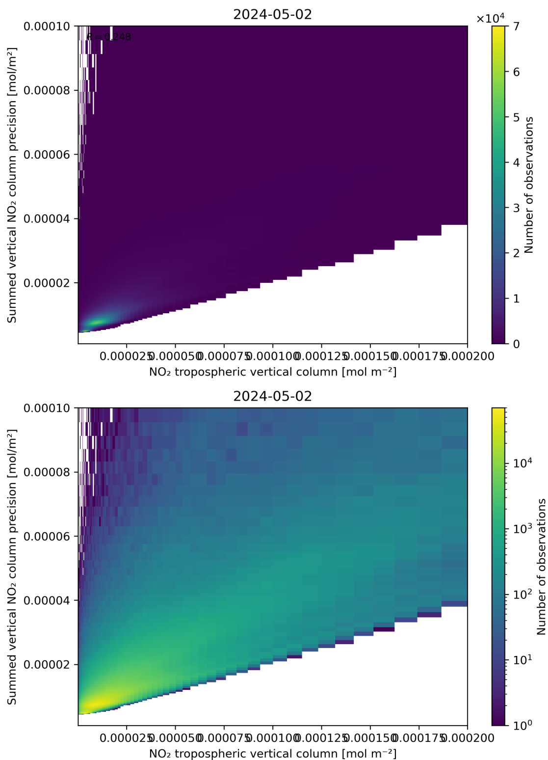
Figure 127: Scatter density plot of “NO 2 tropospheric vertical column” against “Summed vertical NO 2 column precision” for 2024-05-02 to 2024-05-03.
