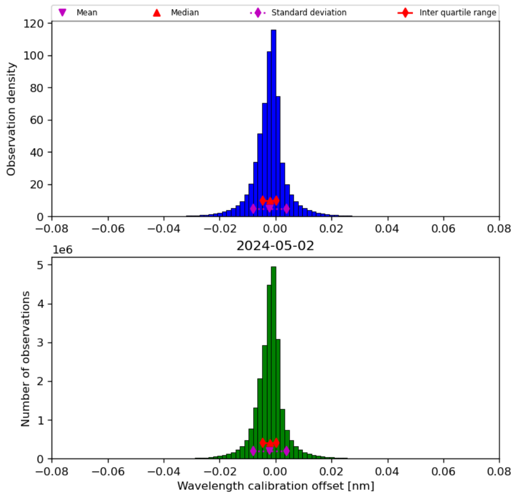
Figure 35: Histogram of “Wavelength calibration offset” for 2024-05-02 to 2024-05-03
