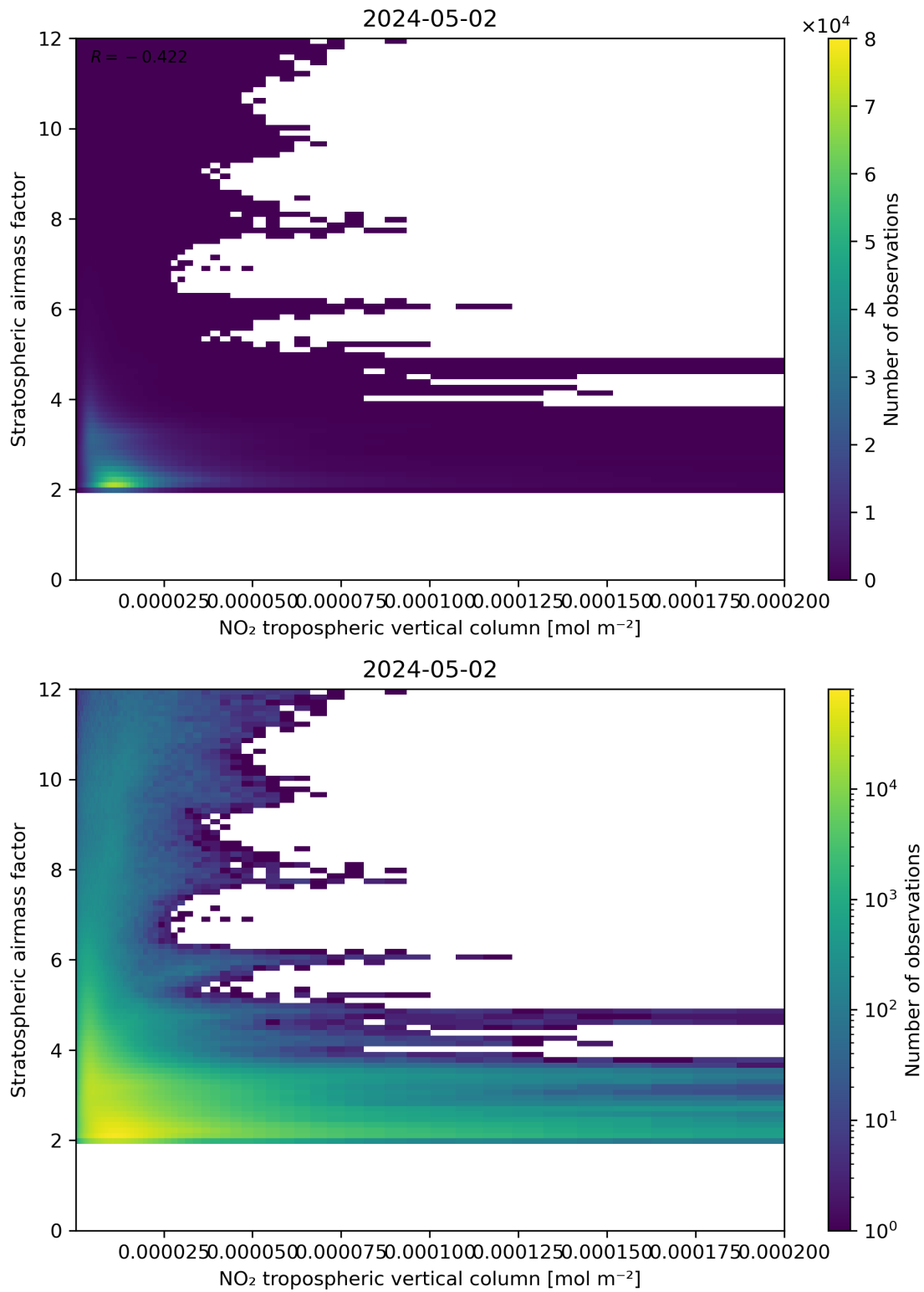
Figure 121: Scatter density plot of “NO 2 tropospheric vertical column” against “Stratospheric air mass factor” for 2024-05-02 to 2024-05-03.
