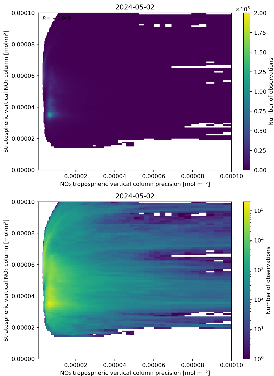
Figure 135: Scatter density plot of “NO 2 tropospheric vertical column precision” against “Stratospheric vertical NO 2 column” for 2024-05-02 to 2024-05-03.
