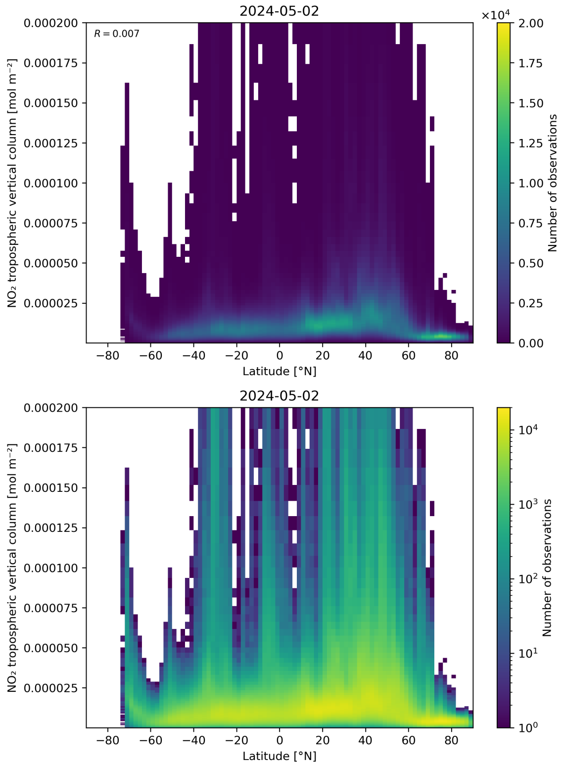
Figure 92: Scatter density plot of “Latitude” against “NO 2 tropospheric vertical column” for 2024-05-02 to 2024-05-03.
