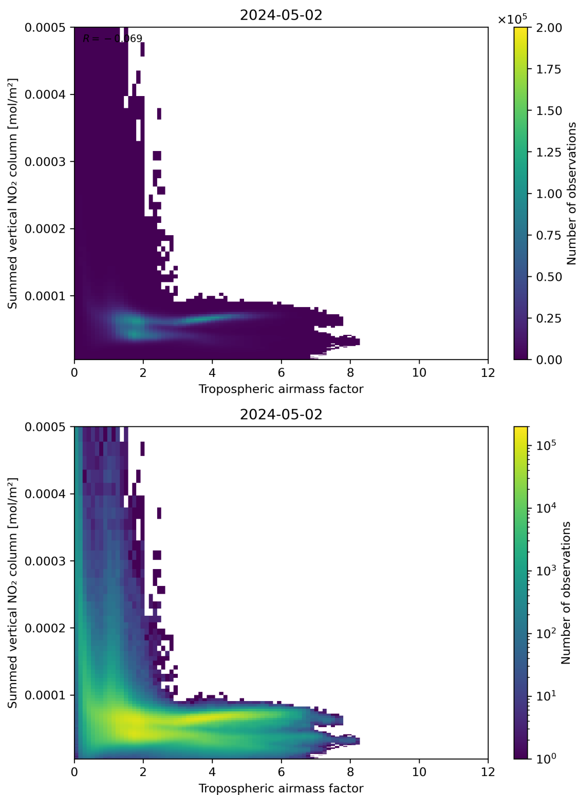
Figure 75: Scatter density plot of “Tropospheric air mass factor” against “Summed vertical NO 2 column” for 2024-05-02 to 2024-05-03.
