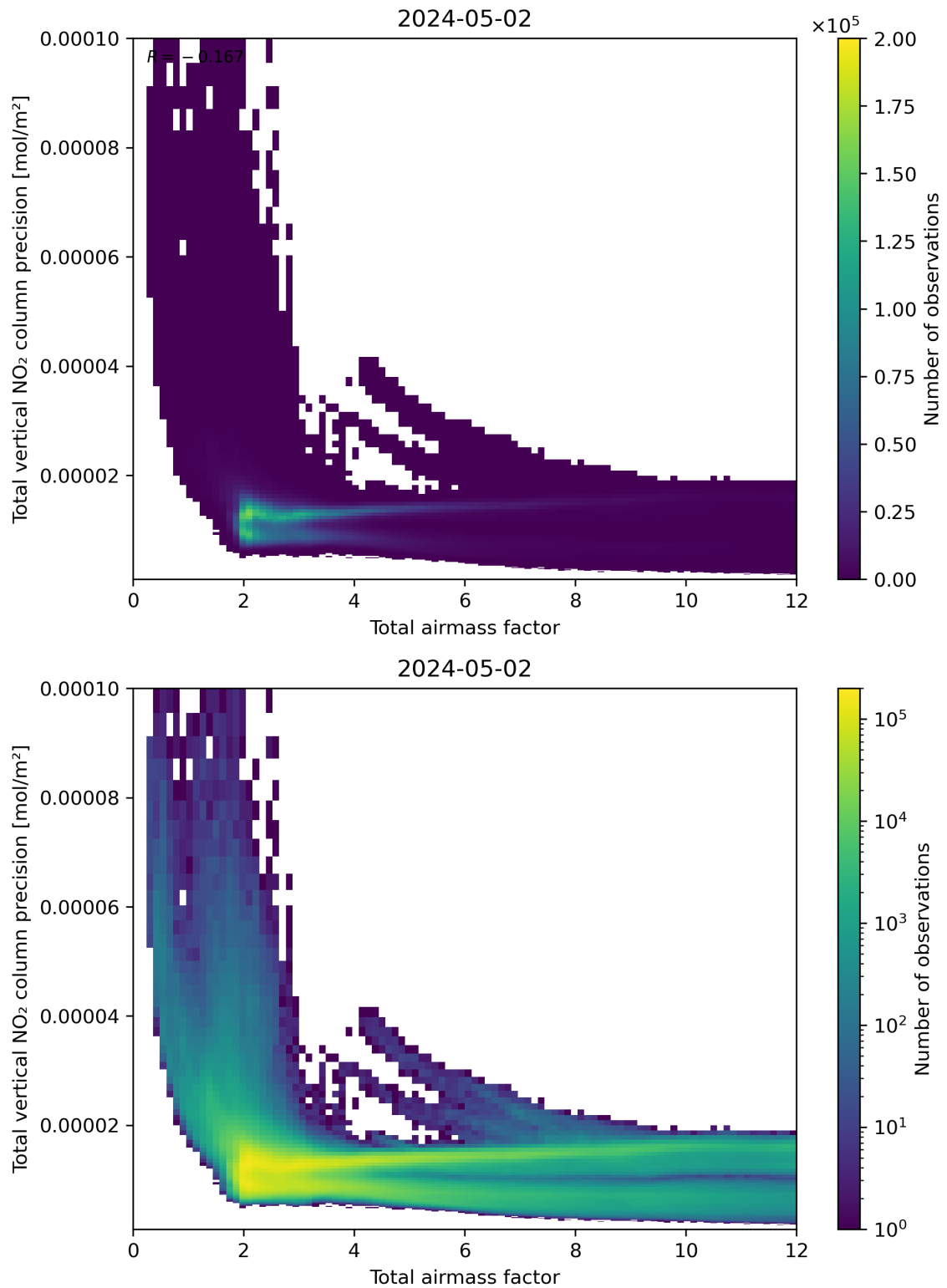
Figure 68: Scatter density plot of “Total airmass factor” against “Total vertical NO 2 column precision” for 2024-05-02 to 2024-05-03.
