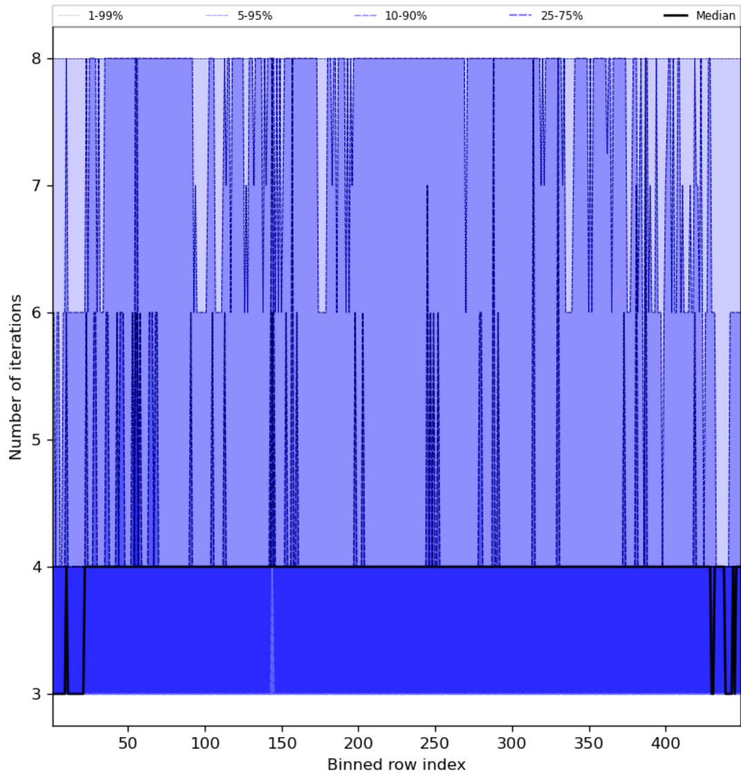
Figure 51: Along track statistics of “Number of iterations” for 2024-05-02 to 2024-05-03
