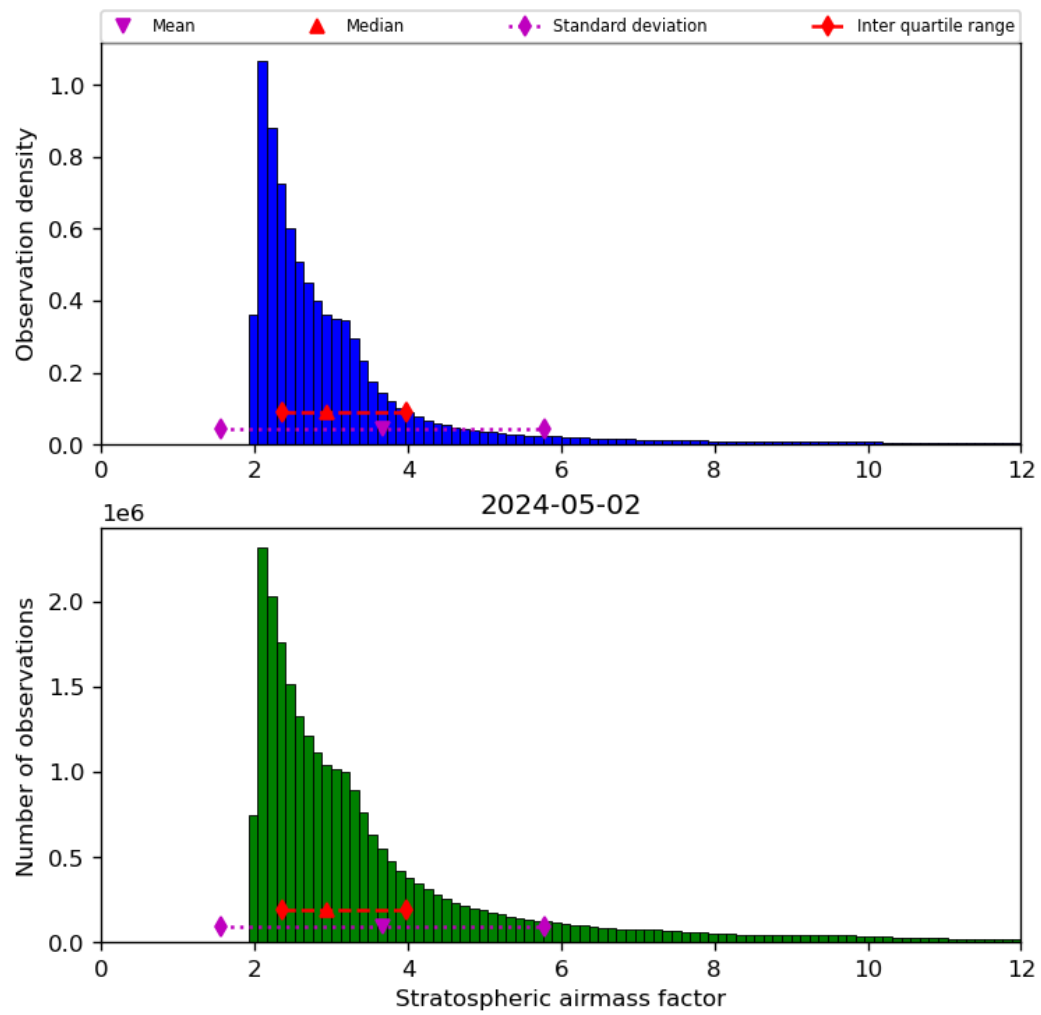
Figure 44: Histogram of “Stratospheric airmass factor” for 2024-05-02 to 2024-05-03
