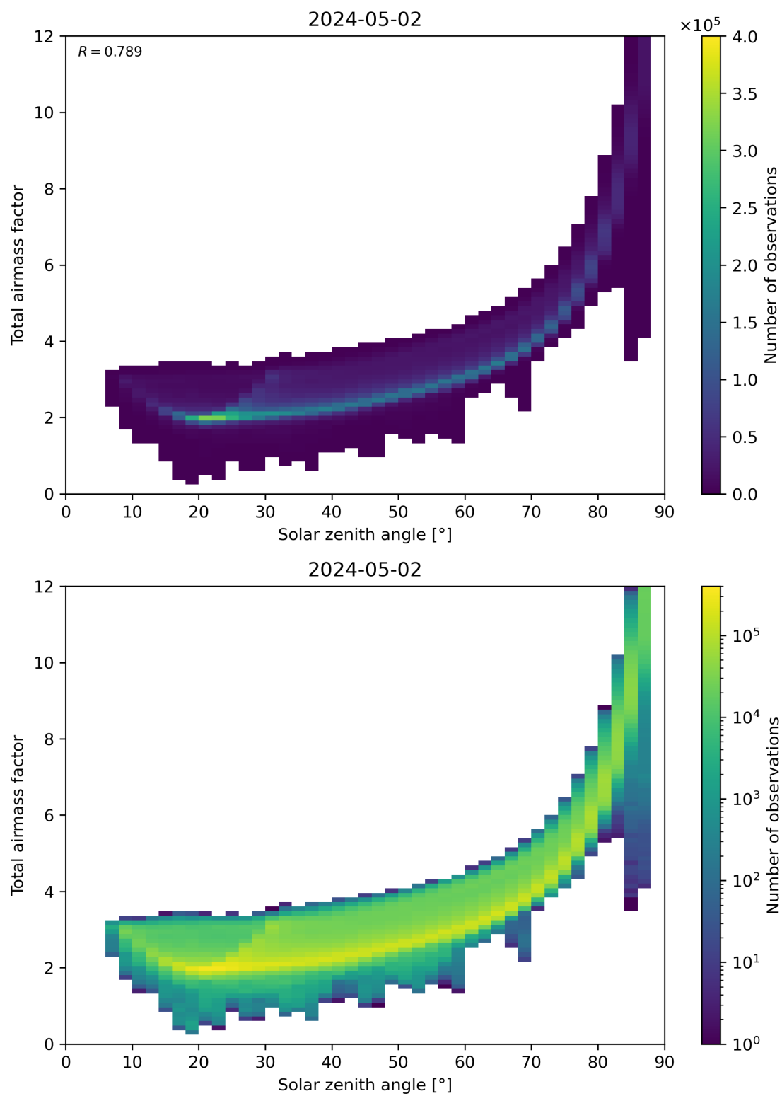
Figure 146: Scatter density plot of “Solar zenith angle” against “Total airmass factor” for 2024-05-02 to 2024-05-03.
