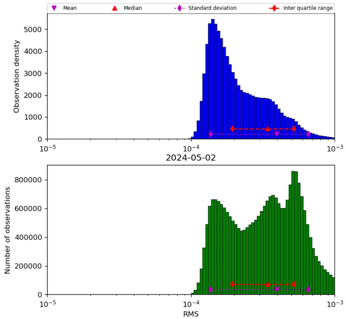
Figure 43: Histogram of “RMS” for 2024-05-02 to 2024-05-03
