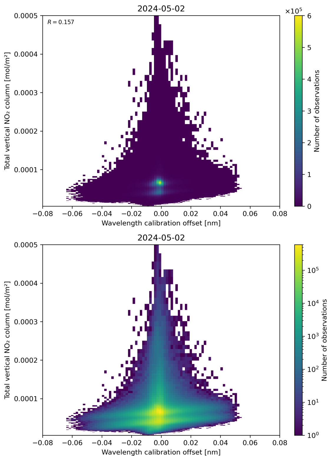
Figure 179: Scatter density plot of “Wavelength calibration offset” against “Total vertical NO 2 column” for 2024-05-02 to 2024-05-03.
