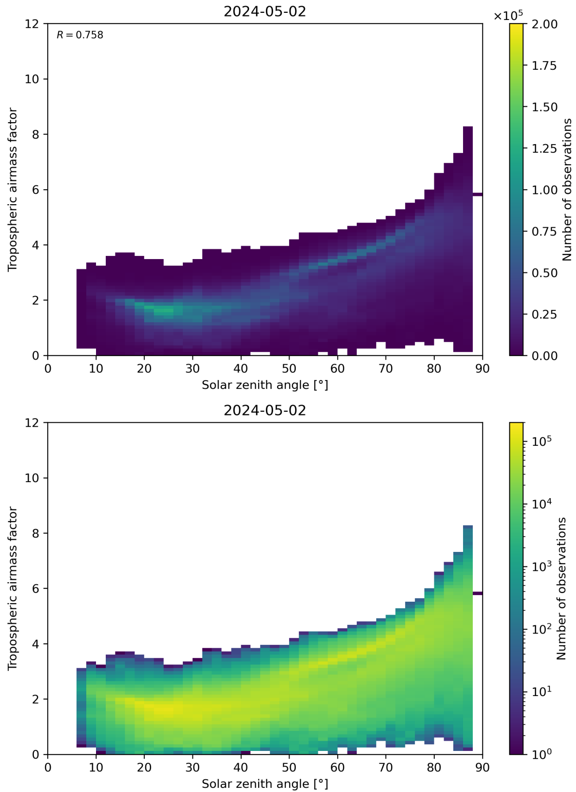
Figure 147: Scatter density plot of “Solar zenith angle” against “Tropospheric airmass factor” for 2024-05-02 to 2024-05-03.
