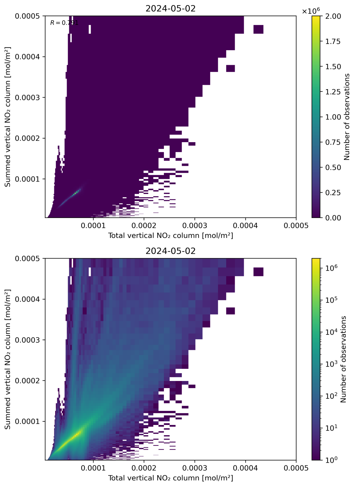
Figure 112: Scatter density plot of “Total vertical NO 2 column” against “Summed vertical NO 2 column” for 2024-05-02 to 2024-05-03.
