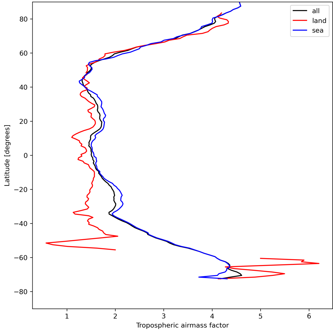
Figure 14: Zonal average of “Tropospheric airmass factor” for 2024-05-02 to 2024-05-03.
