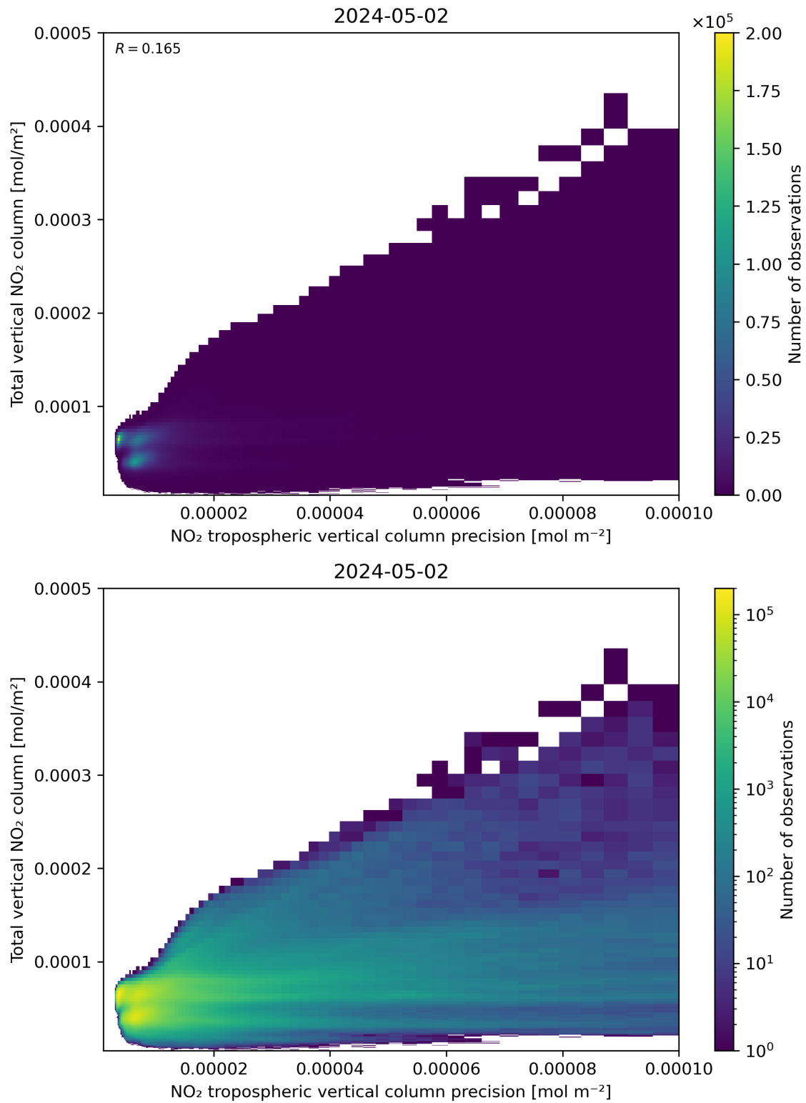
Figure 138: Scatter density plot of “NO 2 tropospheric vertical column precision” against “Total vertical NO 2 column” for 2024-05-02 to 2024-05-03.
