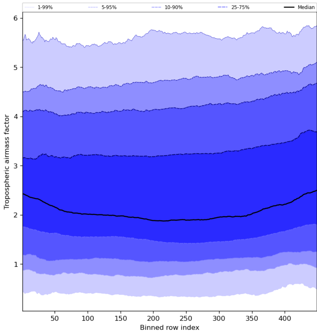
Figure 48: Along track statistics of “Tropospheric airmass factor” for 2024-05-02 to 2024-05-03
