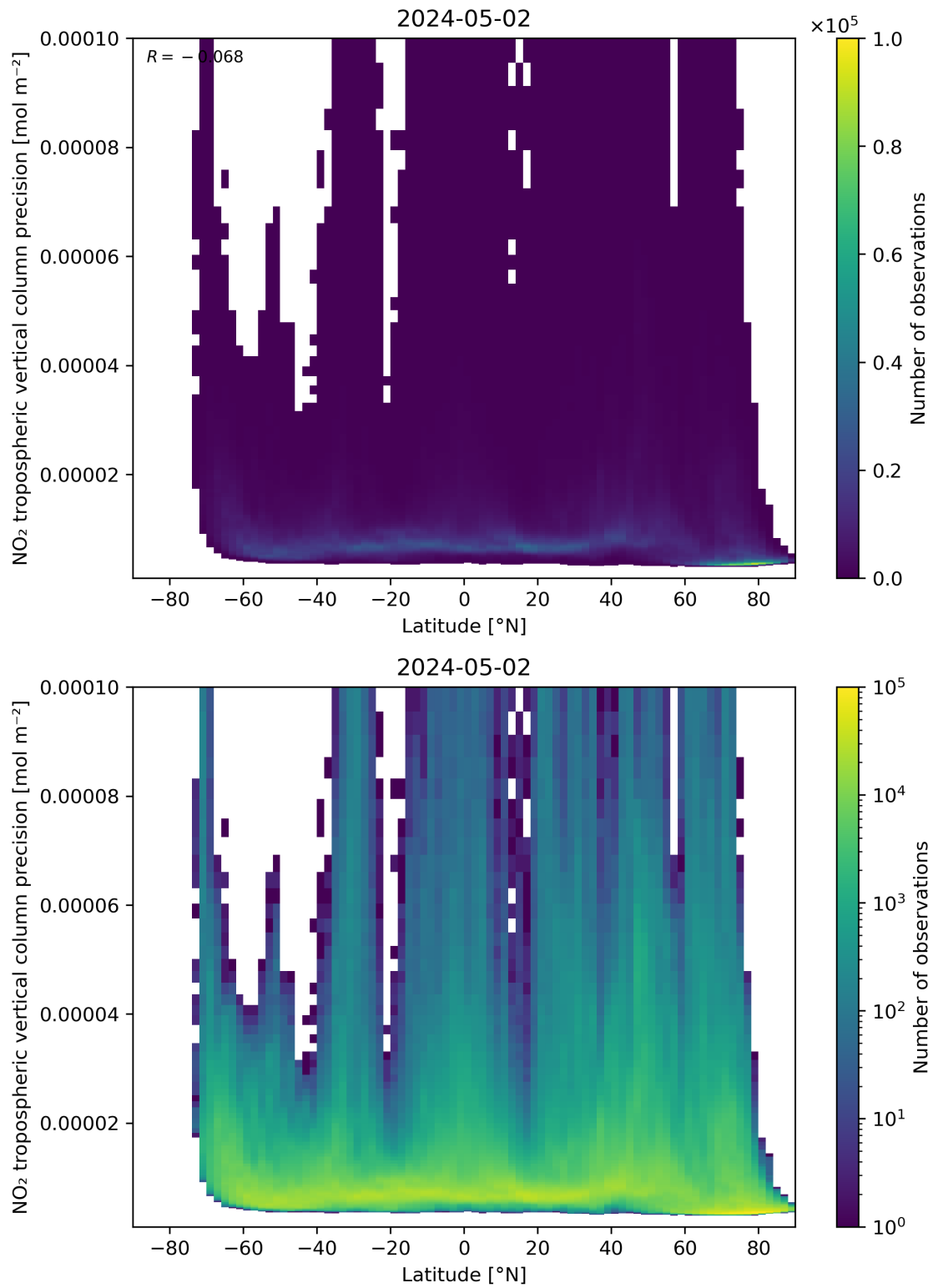
Figure 93: Scatter density plot of “Latitude” against “NO 2 tropospheric vertical column precision” for 2024-05-02 to 2024-05-03.
