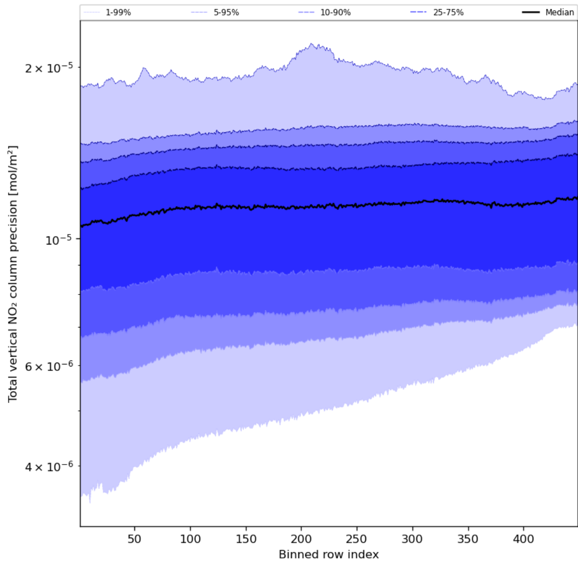
Figure 56: Along track statistics of “Total vertical NO 2 column precision” for 2024-05-02 to 2024-05-03
