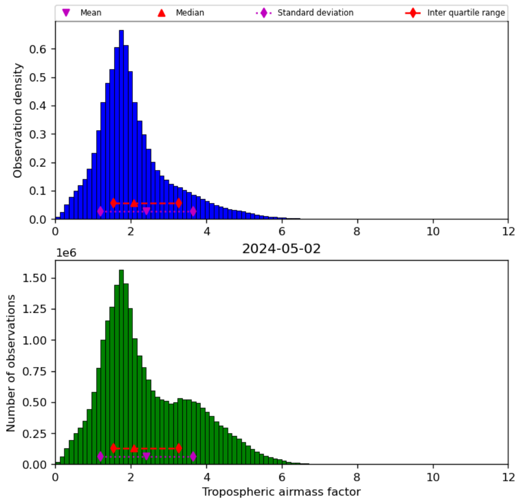
Figure 31: Histogram of “Tropospheric airmass factor” for 2024-05-02 to 2024-05-03
