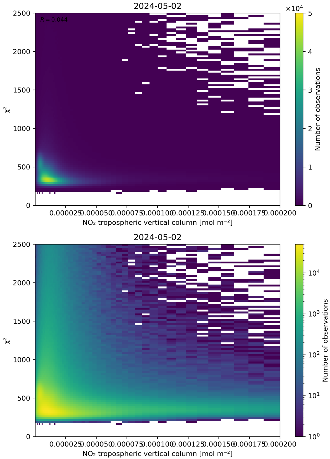
Figure 124: Scatter density plot of “NO 2 tropospheric vertical column” against “ \chi^2 ” for 2024-05-02 to 2024-05-03.
