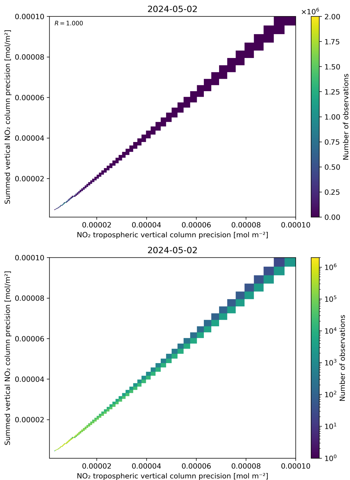
Figure 137: Scatter density plot of “NO 2 tropospheric vertical column precision” against “Summed vertical NO 2 column precision” for 2024-05-02 to 2024-05-03.
