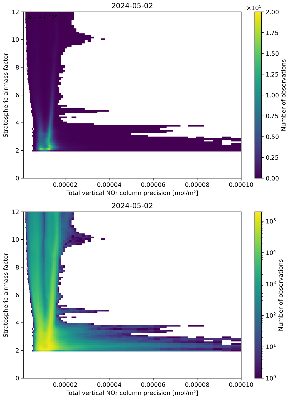
Figure 115: Scatter density plot of “Total vertical NO 2 column precision” against “Stratospheric air mass factor” for 2024-05-02 to 2024-05-03.
