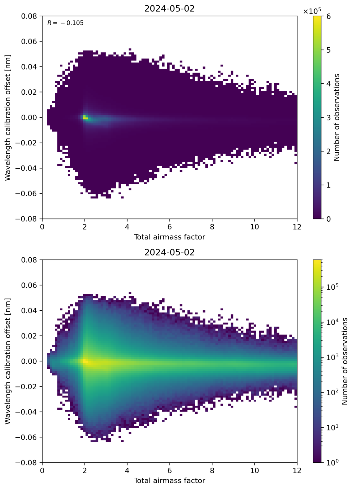
Figure 70: Scatter density plot of “Total airmass factor” against “Wavelength calibration offset” for 2024-05-02 to 2024-05-03.
