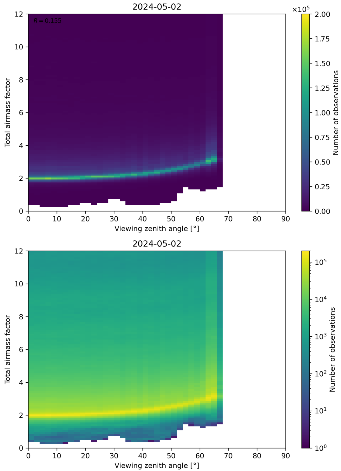
Figure 160: Scatter density plot of “Viewing zenith angle” against “Total airmass factor” for 2024-05-02 to 2024-05-03.
