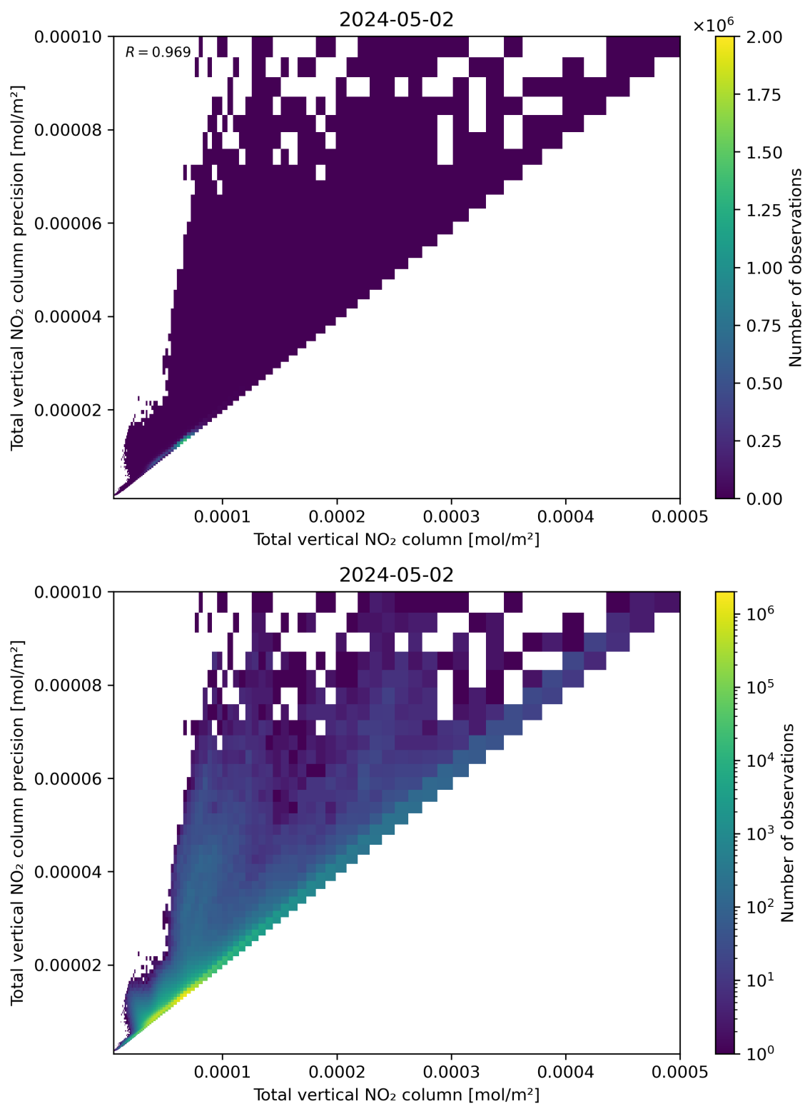
Figure 114: Scatter density plot of “Total vertical NO 2 column” against “Total vertical NO 2 column precision” for 2024-05-02 to 2024-05-03.
