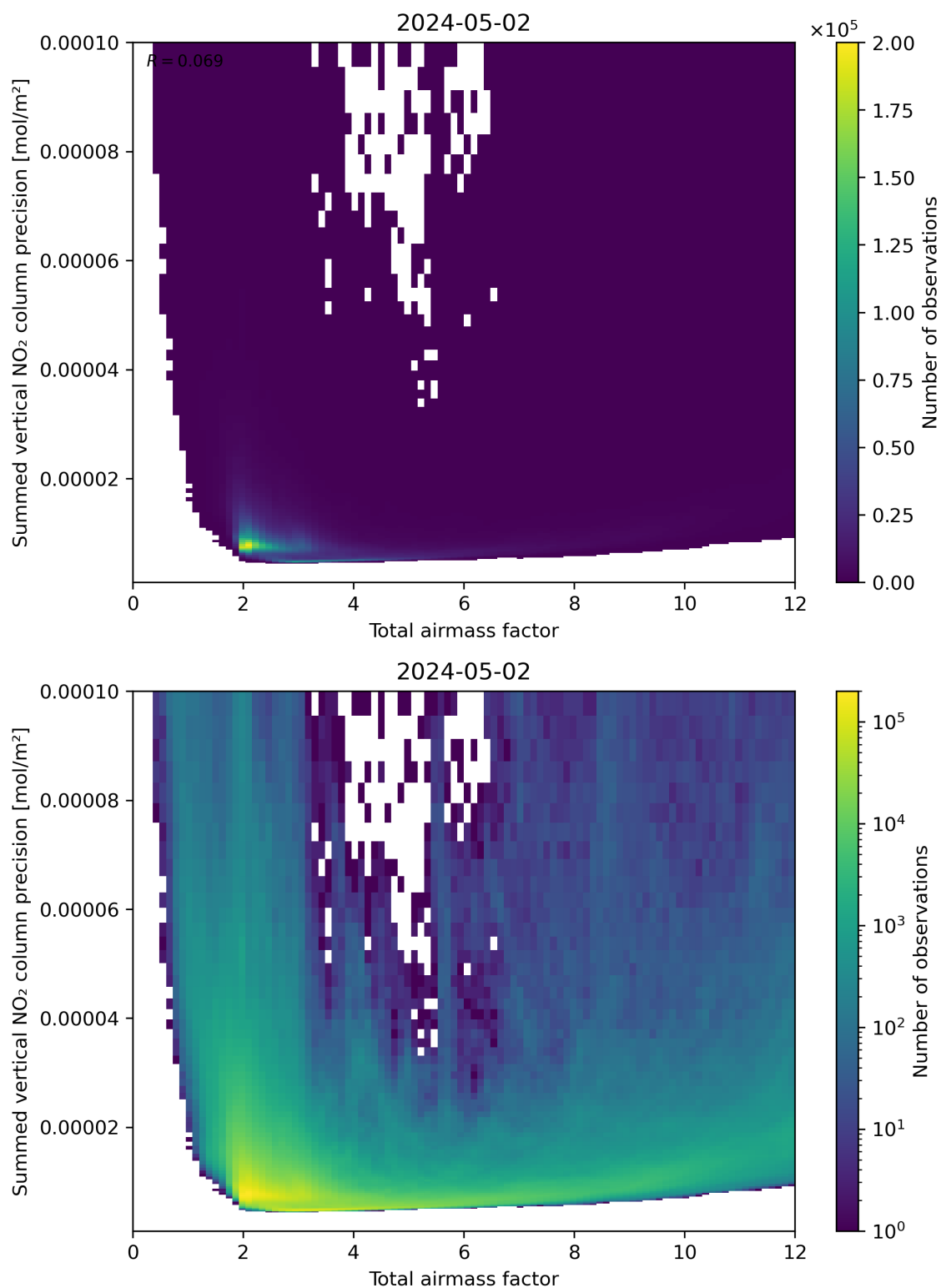
Figure 66: Scatter density plot of “Total airmass factor” against “Summed vertical NO 2 column precision” for 2024-05-02 to 2024-05-03.
