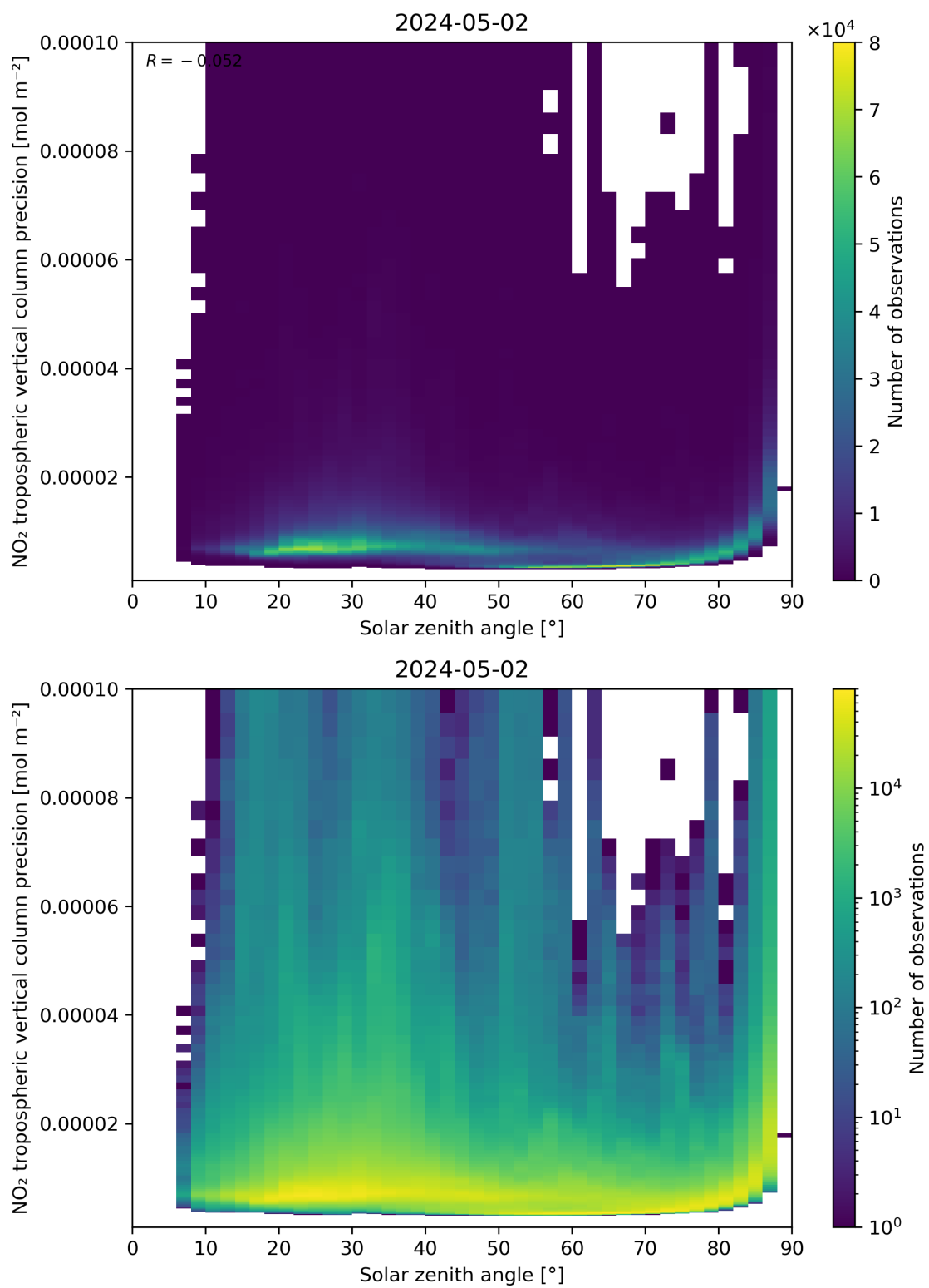
Figure 156: Scatter density plot of “Solar zenith angle” against “NO 2 tropospheric vertical column precision” for 2024-05-02 to 2024-05-03.
