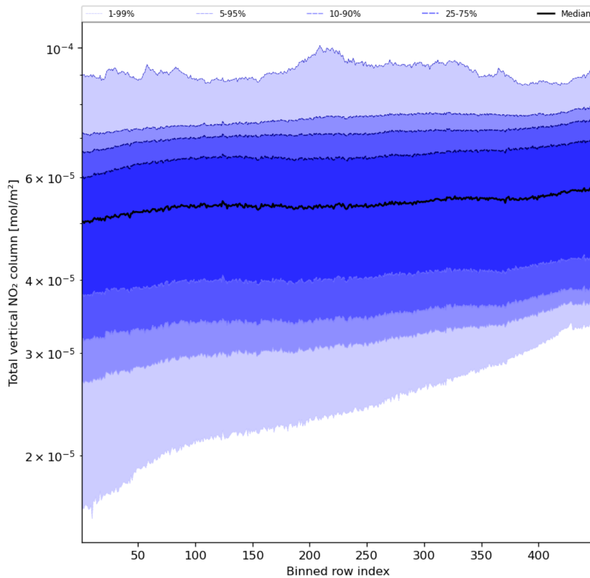
Figure 55: Along track statistics of “Total vertical NO 2 column” for 2024-05-02 to 2024-05-03
