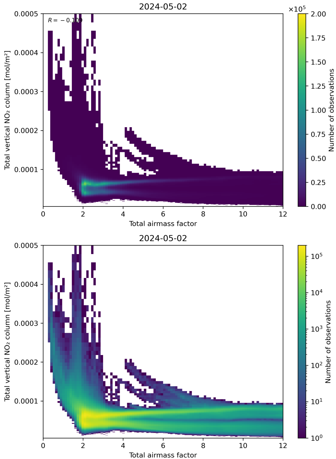
Figure 67: Scatter density plot of “Total airmass factor” against “Total vertical NO 2 column” for 2024-05-02 to 2024-05-03.
