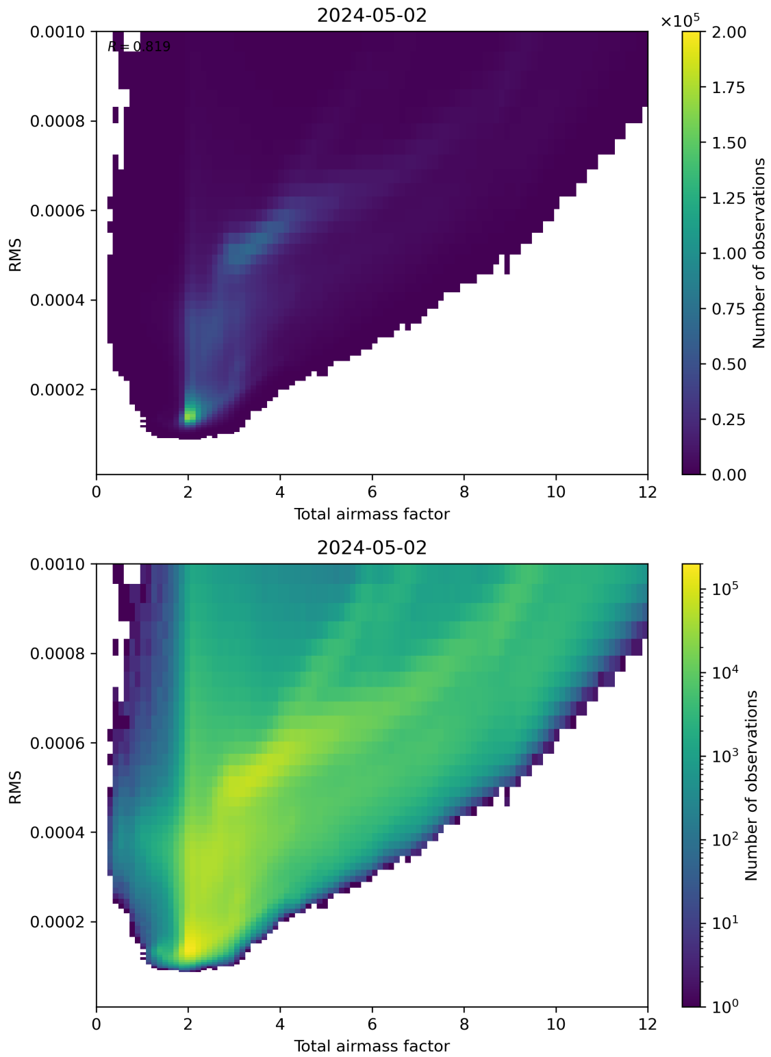
Figure 69: Scatter density plot of “Total airmass factor” against “RMS” for 2024-05-02 to 2024-05-03.
