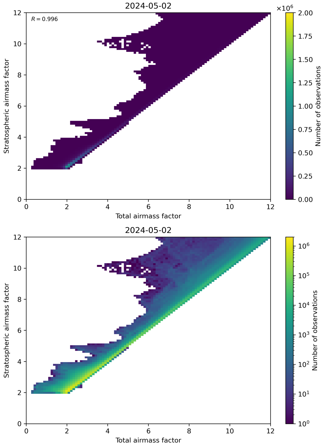
Figure 62: Scatter density plot of “Total airmass factor” against “Stratospheric airmass factor” for 2024-05-02 to 2024-05-03.
