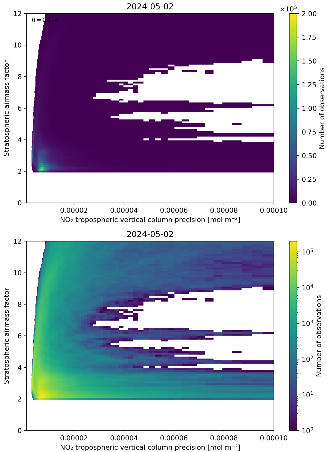
Figure 131: Scatter density plot of “NO 2 tropospheric vertical column precision” against “Stratospheric airmass factor” for 2024-05-02 to 2024-05-03.
