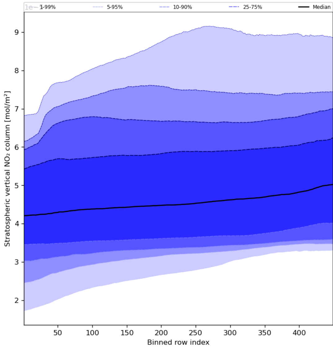
Figure 53: Along track statistics of “Stratospheric vertical NO 2 column” for 2024-05-02 to 2024-05-03
