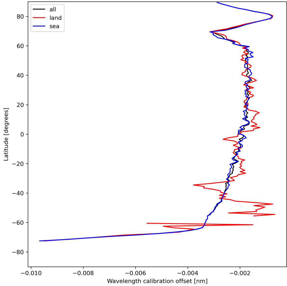
Figure 18: Zonal average of “Wavelength calibration offset” for 2024-05-02 to 2024-05-03.
