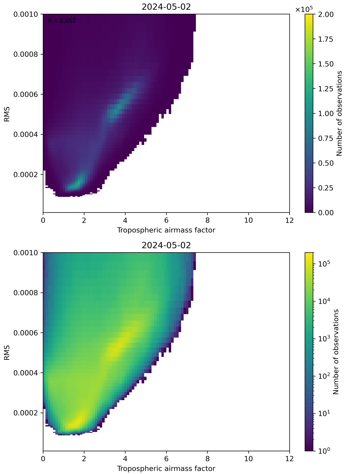
Figure 79: Scatter density plot of “Tropospheric airmass factor” against “RMS” for 2024-05-02 to 2024-05-03.
