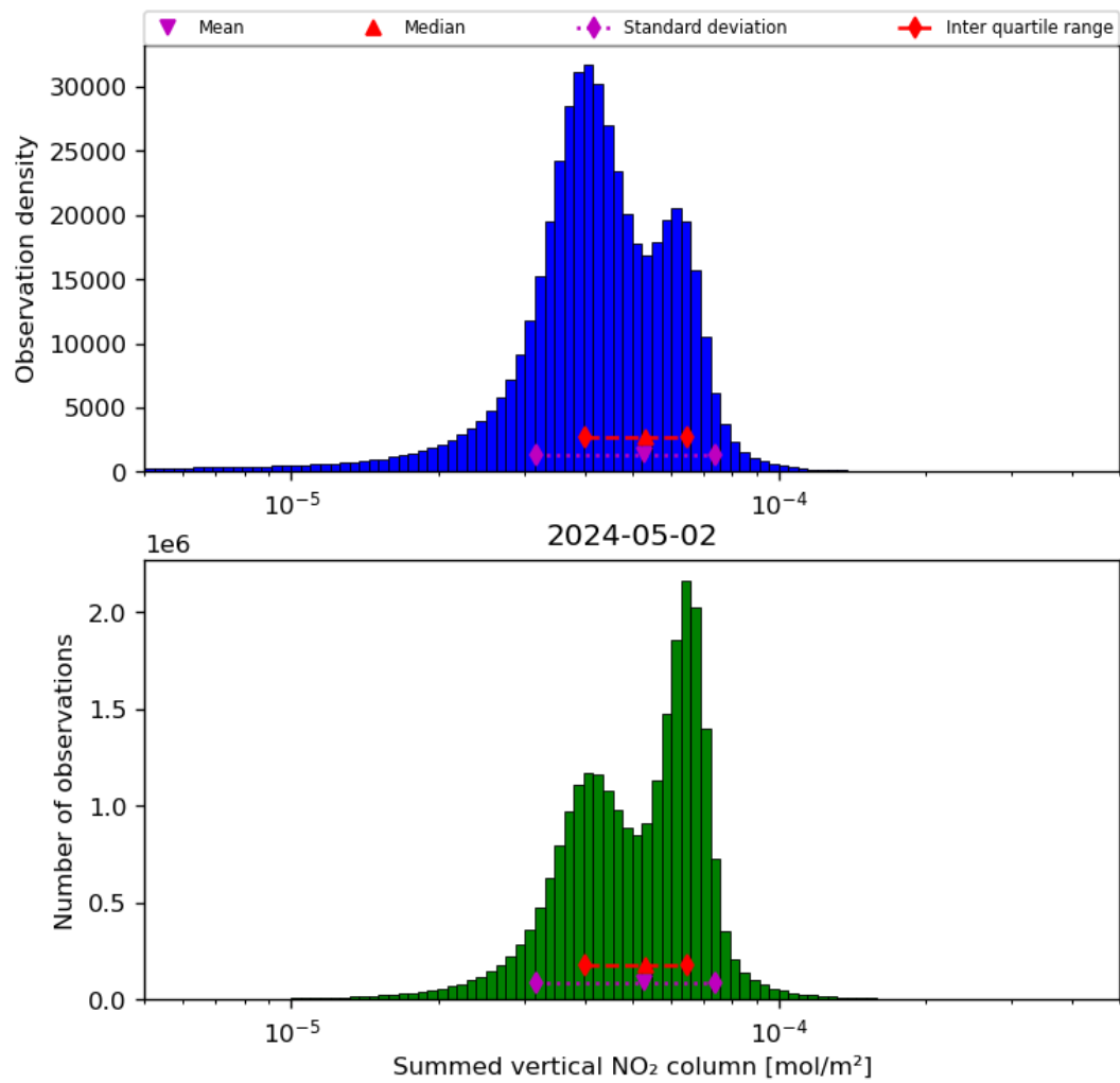
Figure 40: Histogram of “Summed vertical NO 2 column” for 2024-05-02 to 2024-05-03
