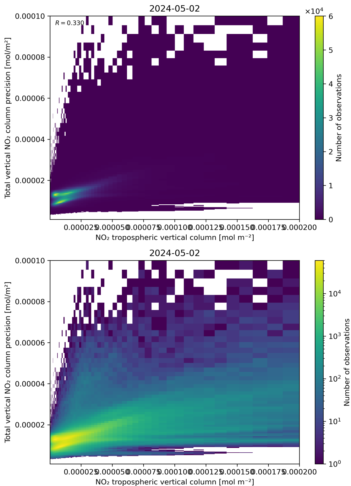
Figure 129: Scatter density plot of “NO 2 tropospheric vertical column” against “Total vertical NO 2 column precision” for 2024-05-02 to 2024-05-03.
