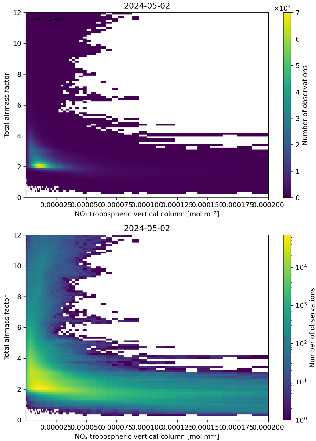
Figure 122: Scatter density plot of “NO 2 tropospheric vertical column” against “Total air mass factor” for 2024-05-02 to 2024-05-03.
