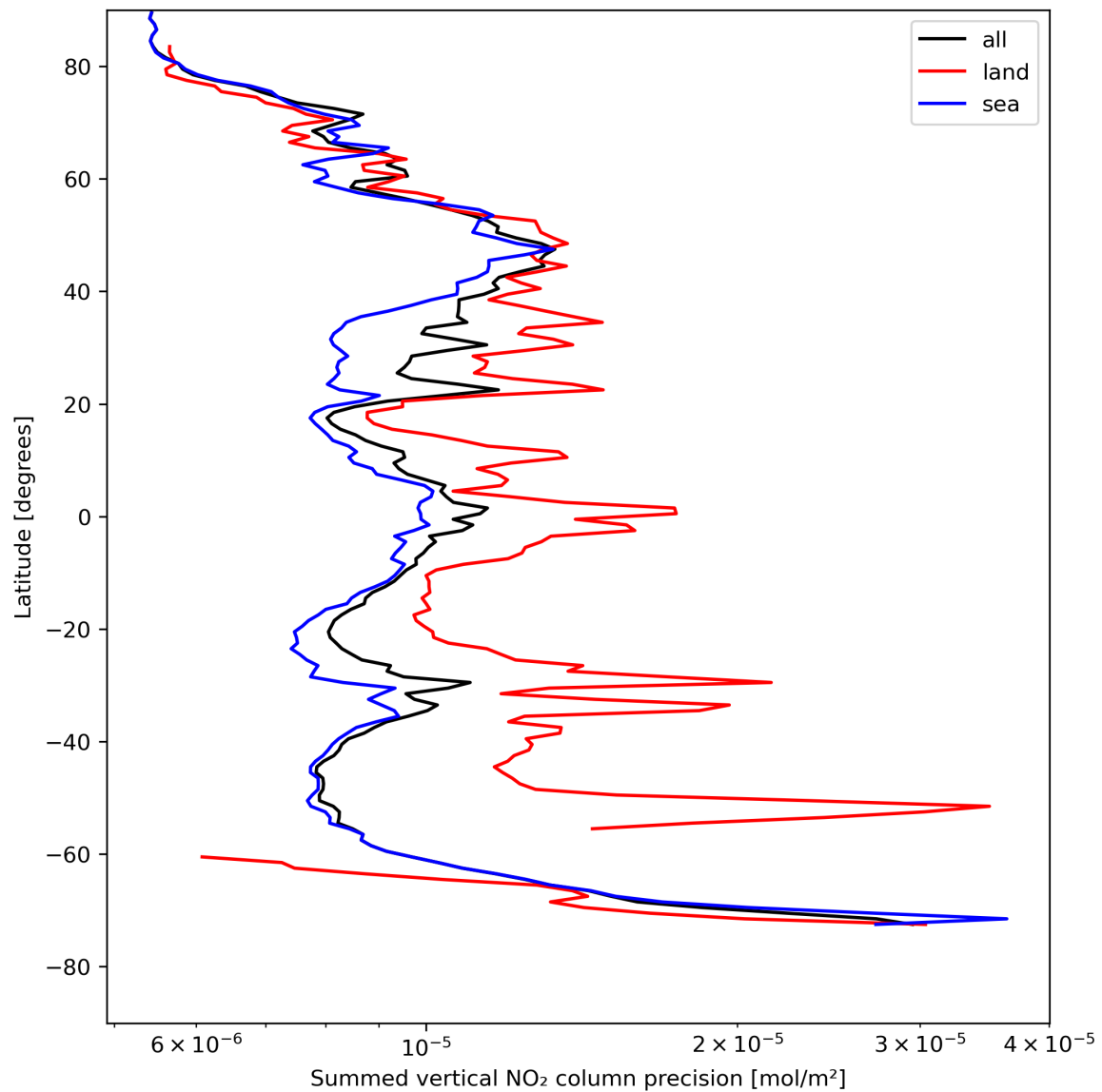
Figure 24: Zonal average of “Summed vertical NO 2 column precision” for 2024-05-02 to 2024-05-03.
