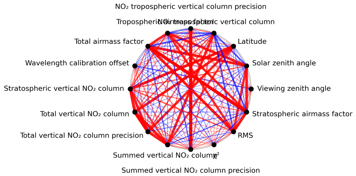
Figure 1: Map of correlation graph for 2024-05-02 to 2024-05-03.
