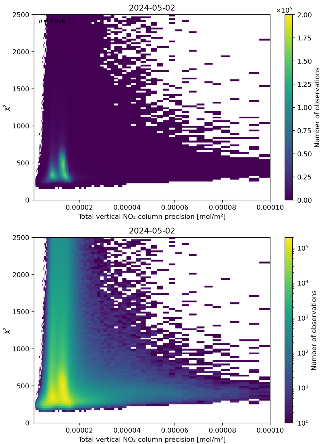
Figure 116: Scatter density plot of “Total vertical NO 2 column precision” against “ \chi^2 ” for 2024-05-02 to 2024-05-03.
