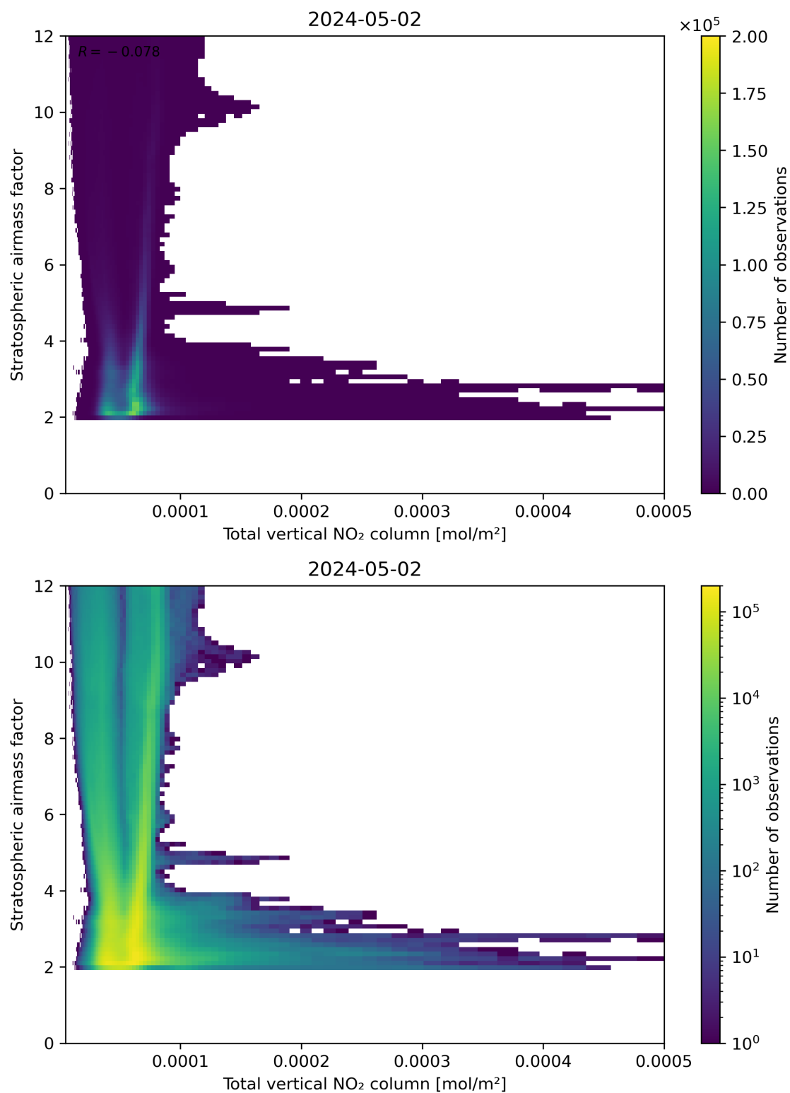
Figure 110: Scatter density plot of “Total vertical NO 2 column” against “Stratospheric airmass factor” for 2024-05-02 to 2024-05-03.
