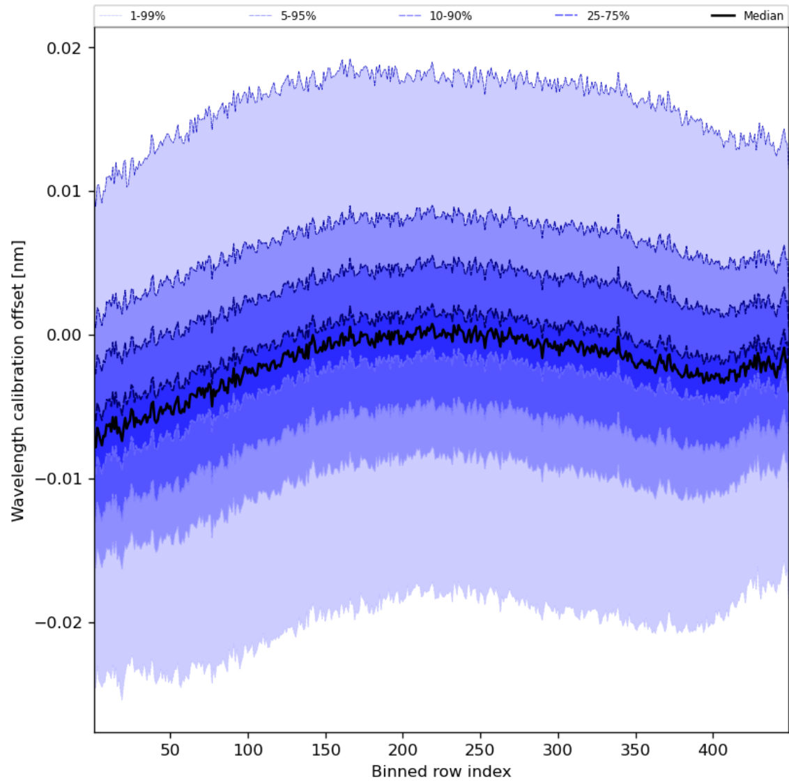
Figure 52: Along track statistics of “Wavelength calibration offset” for 2024-05-02 to 2024-05-03
