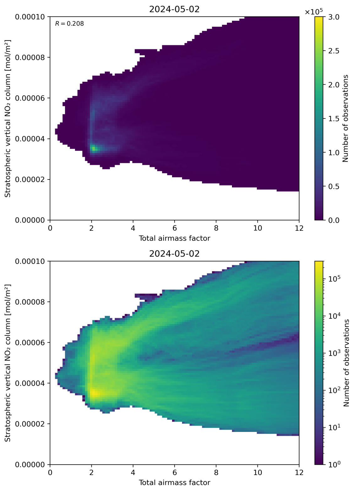
Figure 64: Scatter density plot of “Total airmass factor” against “Stratospheric vertical \text{NO}_2 column” for 2024-05-02 to 2024-05-03.
