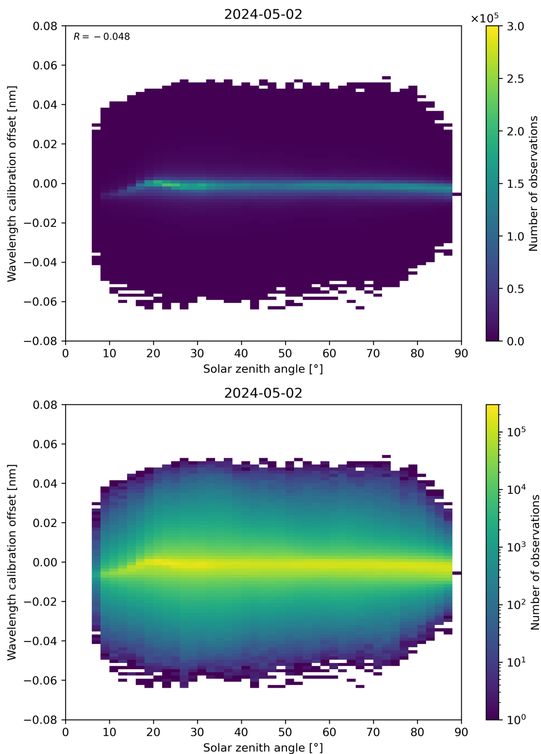
Figure 158: Scatter density plot of “Solar zenith angle” against “Wavelength calibration offset” for 2024-05-02 to 2024-05-03.
