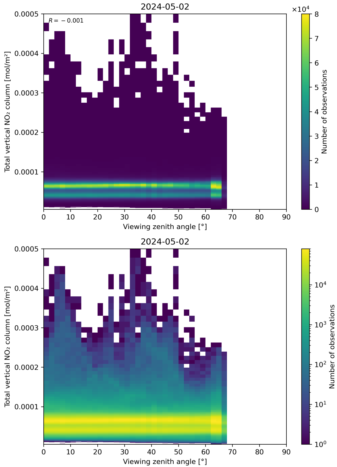
Figure 167: Scatter density plot of “Viewing zenith angle” against “Total vertical NO 2 column” for 2024-05-02 to 2024-05-03.
