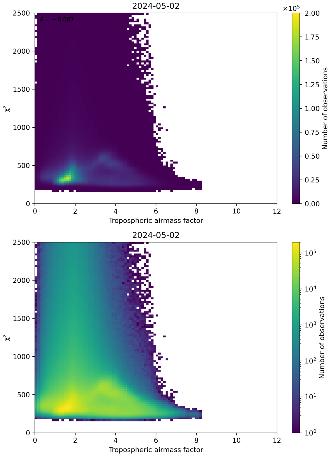
Figure 73: Scatter density plot of “Tropospheric airmass factor” against “ \chi^2 ” for 2024-05-02 to 2024-05-03.
