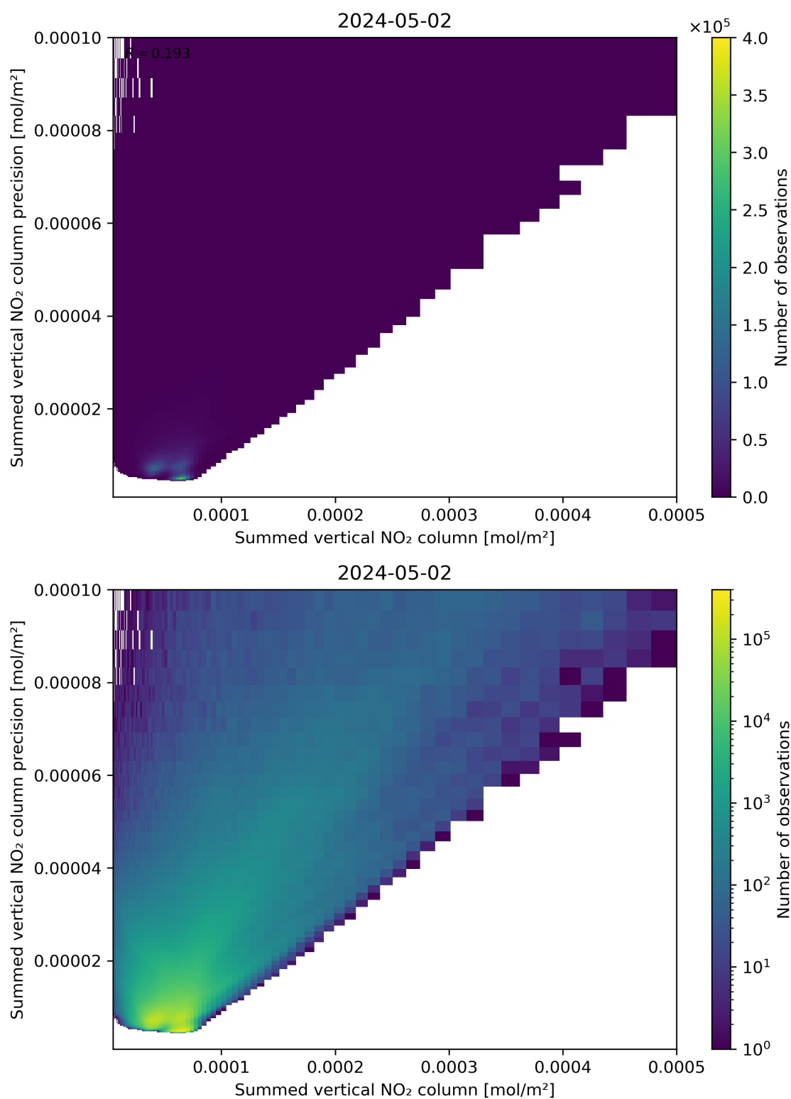
Figure 105: Scatter density plot of “Summed vertical NO 2 column” against “Summed vertical NO 2 column precision” for 2024-05-02 to 2024-05-03.
