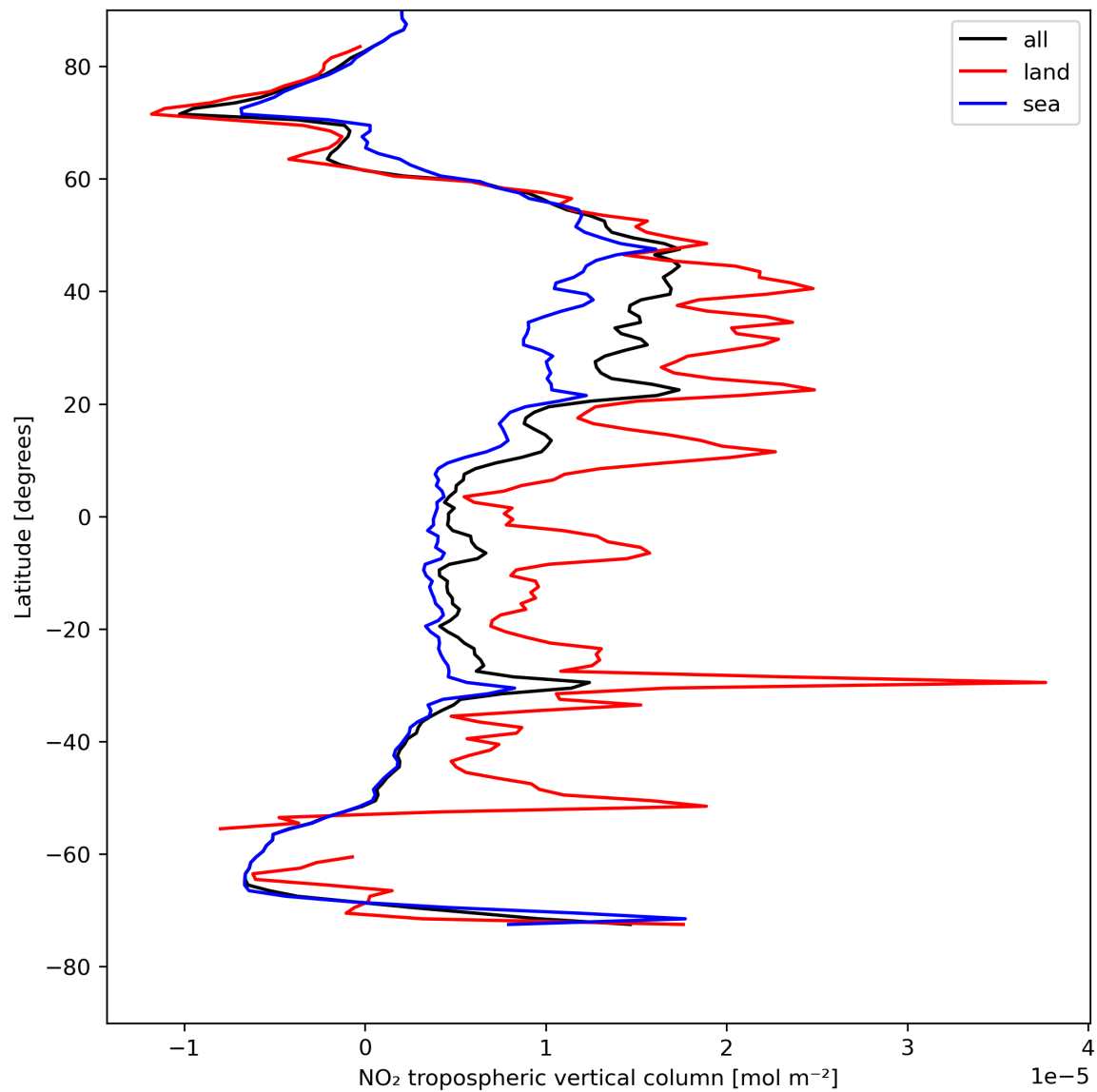
Figure 12: Zonal average of “NO 2 tropospheric vertical column” for 2024-05-02 to 2024-05-03.
