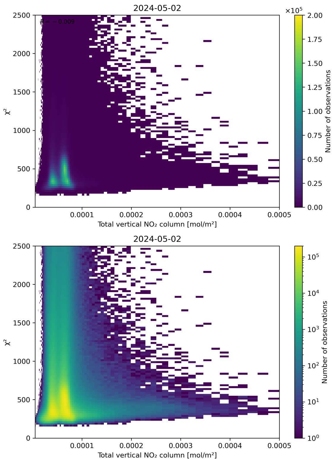
Figure 111: Scatter density plot of “Total vertical NO 2 column” against “ \chi^2 ” for 2024-05-02 to 2024-05-03.
