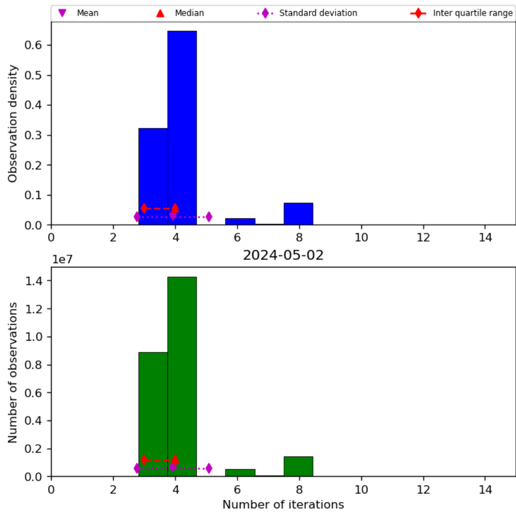
Figure 34: Histogram of “Number of iterations” for 2024-05-02 to 2024-05-03
