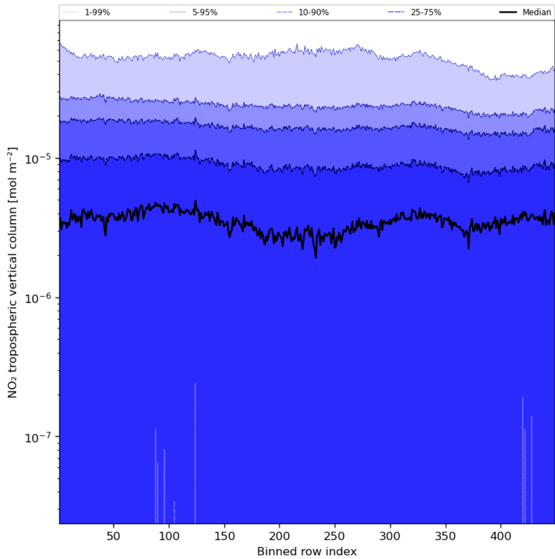
Figure 46: Along track statistics of “NO 2 tropospheric vertical column” for 2024-05-02 to 2024-05-03
