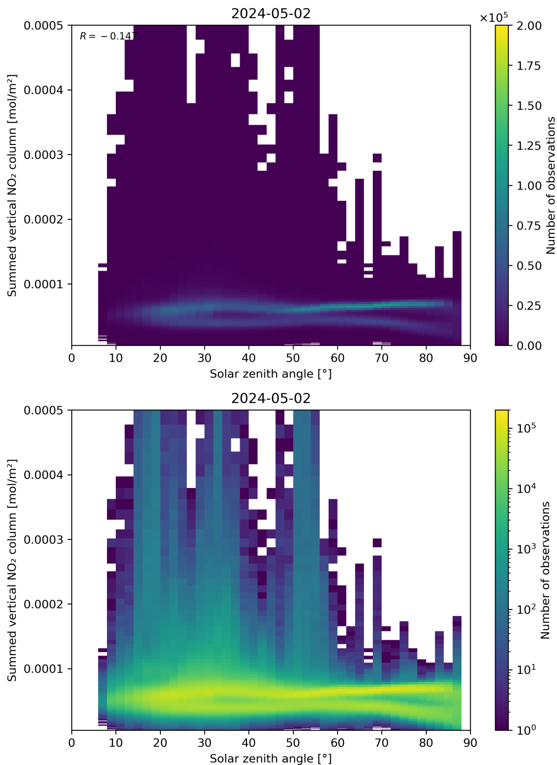
Figure 151: Scatter density plot of “Solar zenith angle” against “Summed vertical NO 2 column” for 2024-05-02 to 2024-05-03.
