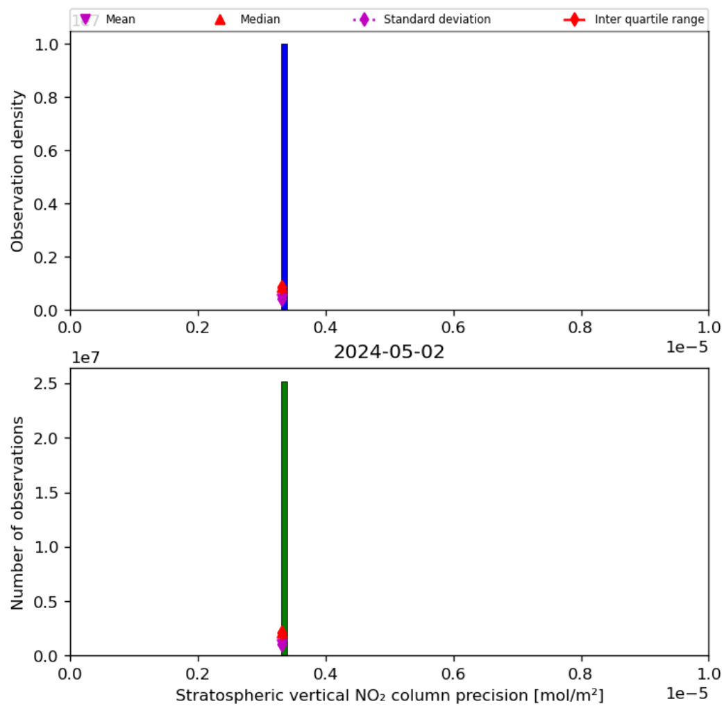
Figure 37: Histogram of “Stratospheric vertical NO 2 column precision” for 2024-05-02 to 2024-05-03
