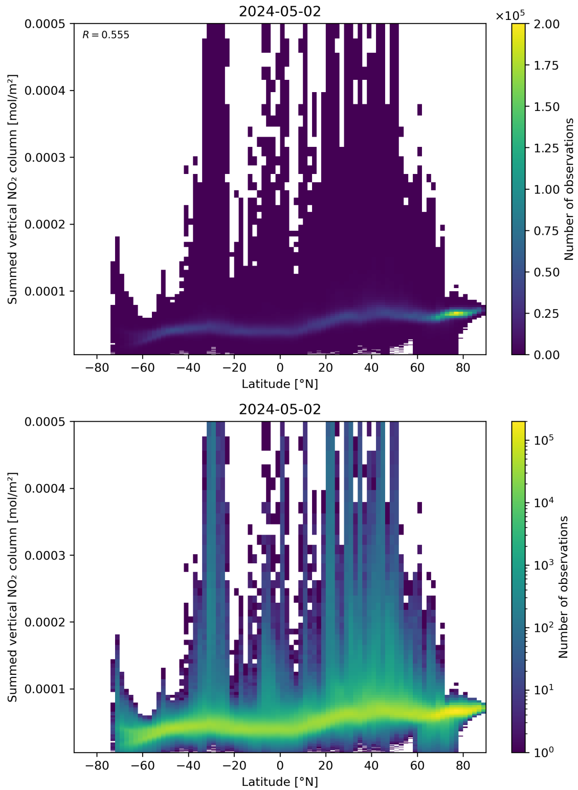
Figure 88: Scatter density plot of “Latitude” against “Summed vertical NO 2 column” for 2024-05-02 to 2024-05-03.
