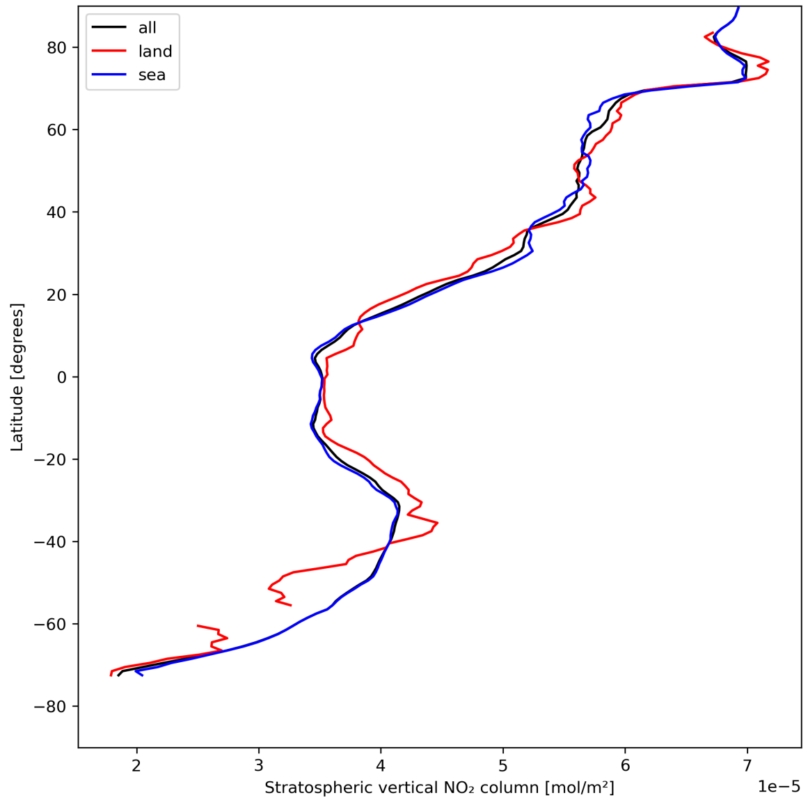
Figure 19: Zonal average of “Stratospheric vertical NO 2 column” for 2024-05-02 to 2024-05-03.
