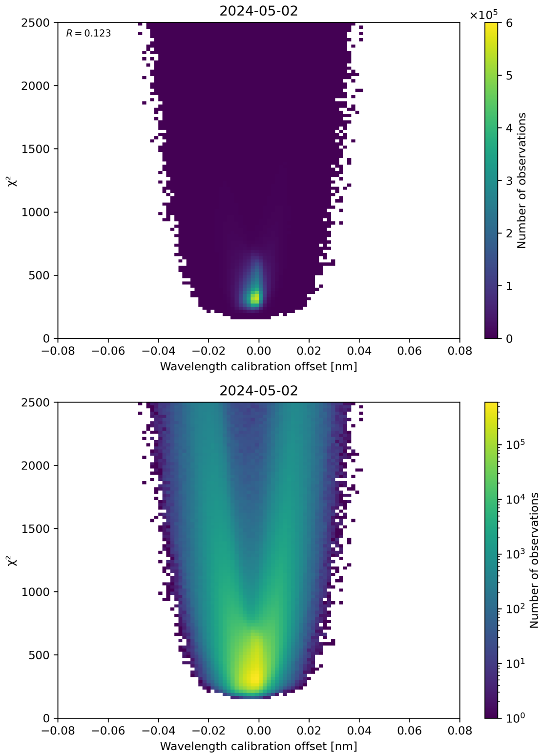
Figure 175: Scatter density plot of “Wavelength calibration offset” against “ \chi^2 ” for 2024-05-02 to 2024-05-03.
