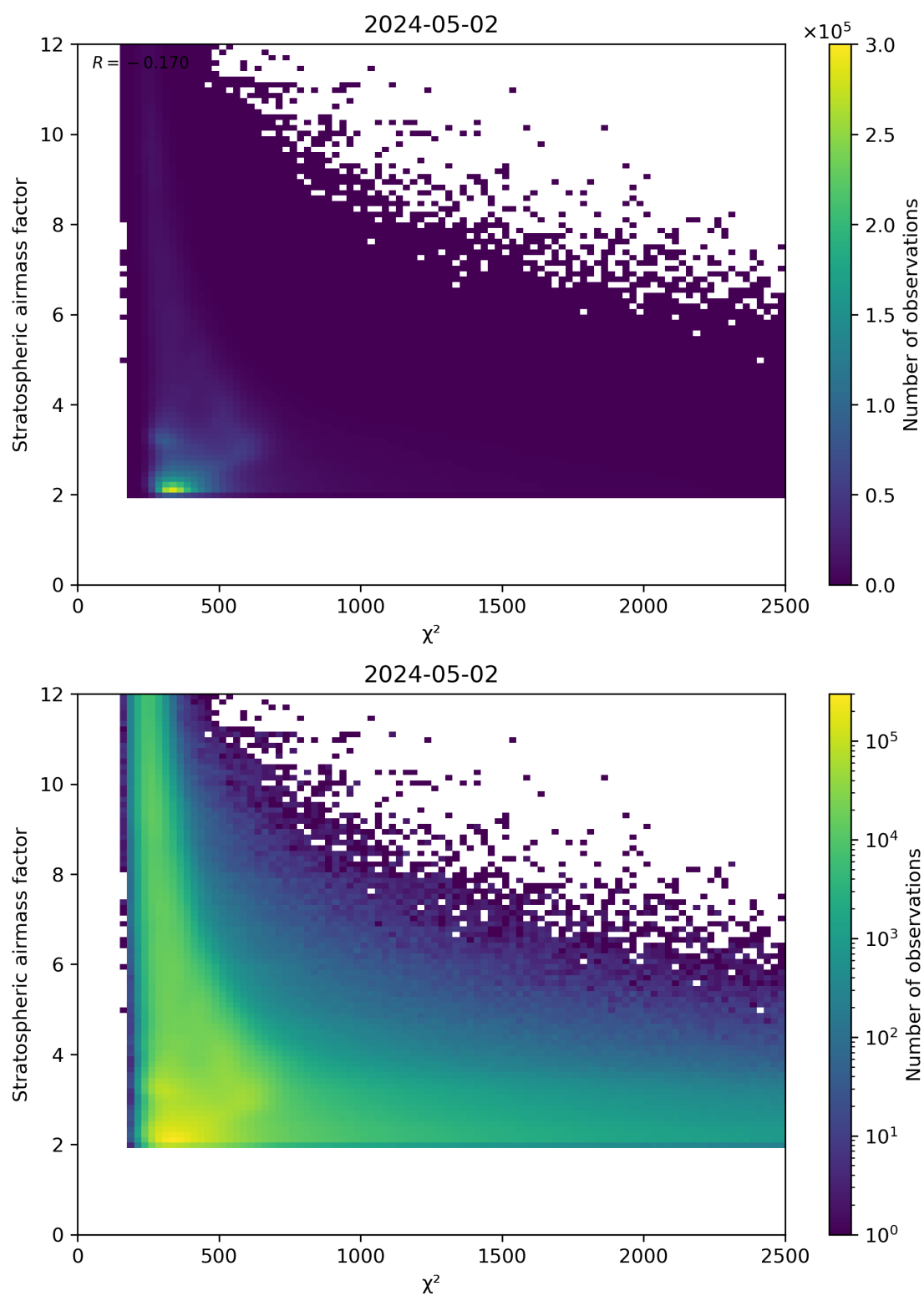
Figure 81: Scatter density plot of “ \chi^2 ” against “Stratospheric airmass factor” for 2024-05-02 to 2024-05-03.
