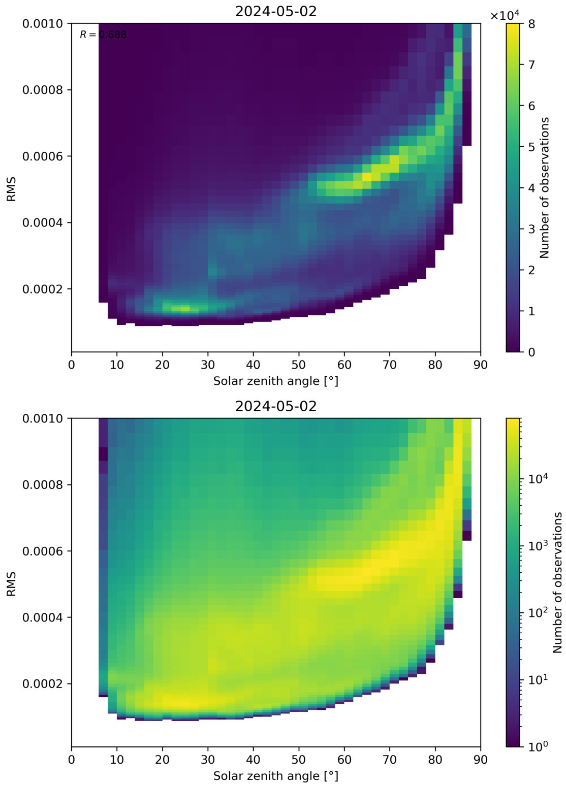
Figure 157: Scatter density plot of “Solar zenith angle” against “RMS” for 2024-05-02 to 2024-05-03.
