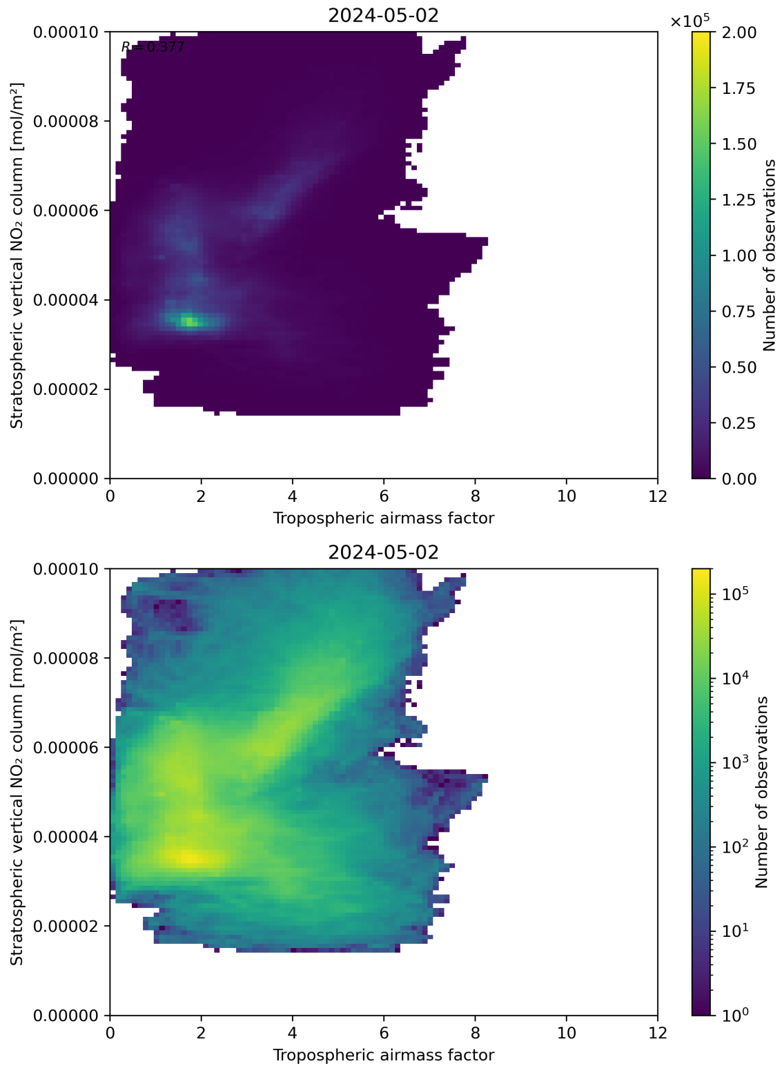
Figure 74: Scatter density plot of “Tropospheric air mass factor” against “Stratospheric vertical NO 2 column” for 2024-05-02 to 2024-05-03.
