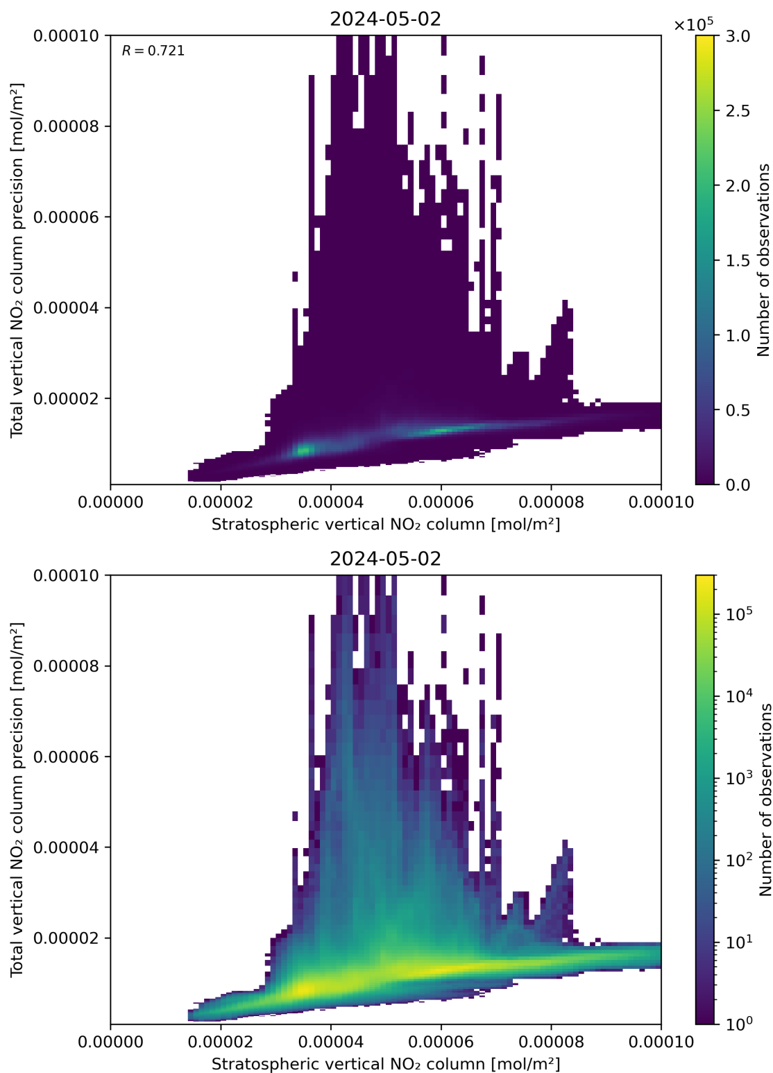
Figure 101: Scatter density plot of “Stratospheric vertical NO 2 column” against “Total vertical NO 2 column precision” for 2024-05-02 to 2024-05-03.
