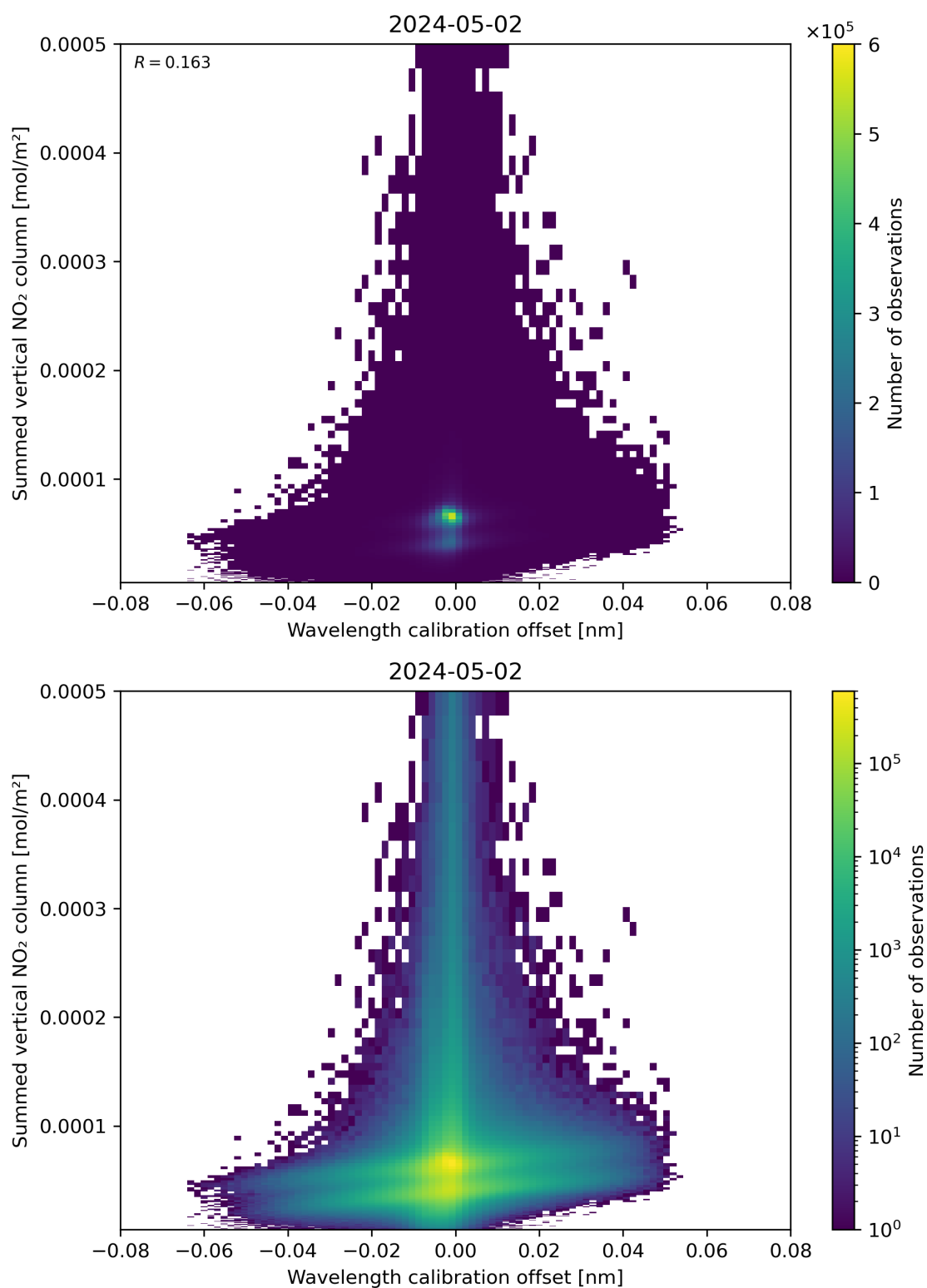
Figure 177: Scatter density plot of “Wavelength calibration offset” against “Summed vertical NO 2 column” for 2024-05-02 to 2024-05-03.
