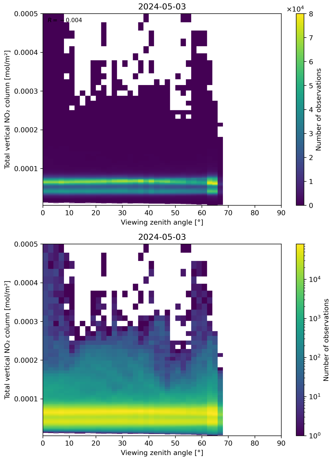
Figure 167: Scatter density plot of “Viewing zenith angle” against “Total vertical NO 2 column” for 2024-05-02 to 2024-05-04.
