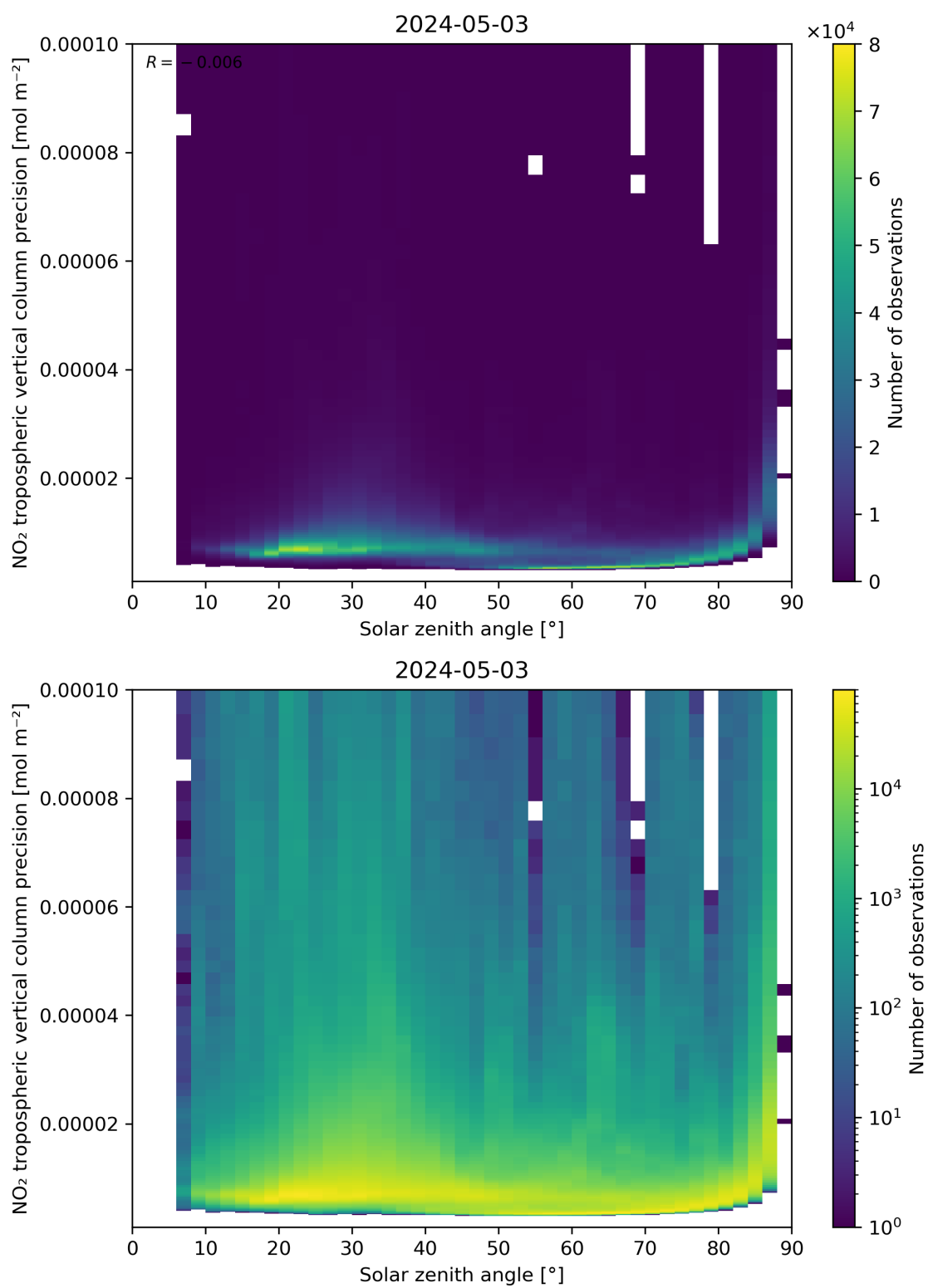
Figure 156: Scatter density plot of “Solar zenith angle” against “NO 2 tropospheric vertical column precision” for 2024-05-02 to 2024-05-04.
