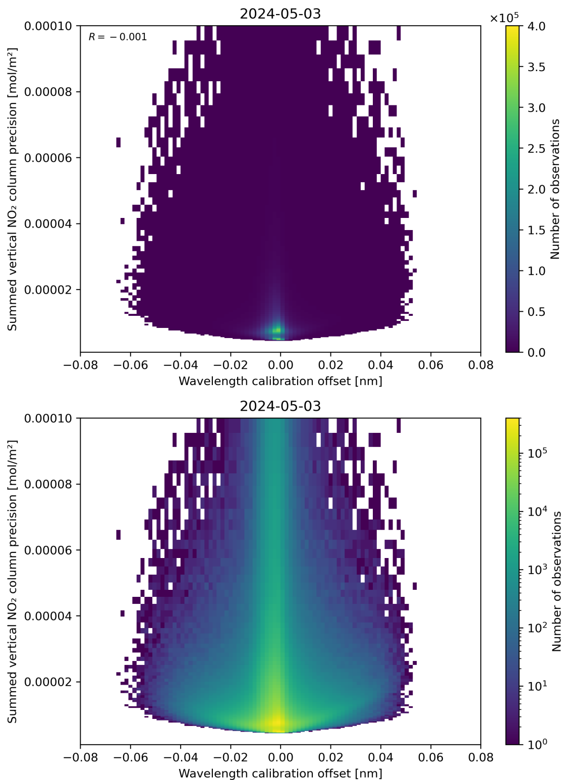
Figure 178: Scatter density plot of “Wavelength calibration offset” against “Summed vertical NO 2 column precision” for 2024-05-02 to 2024-05-04.
