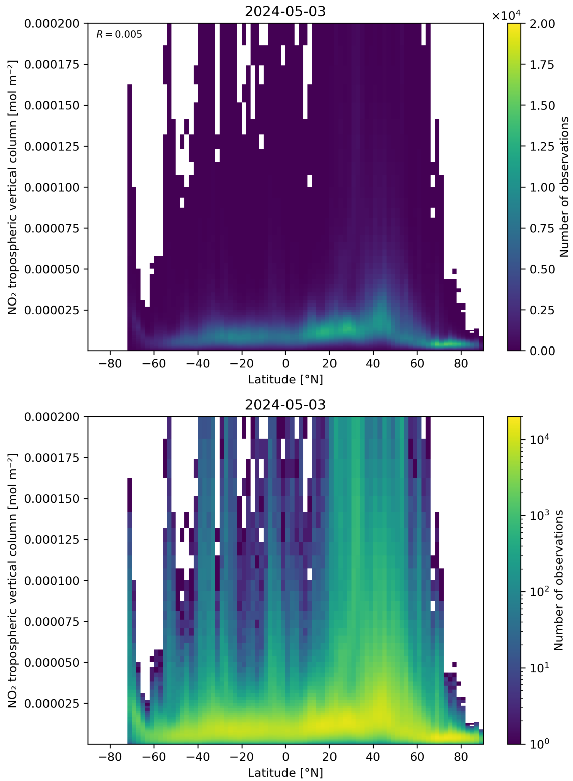
Figure 92: Scatter density plot of “Latitude” against “NO 2 tropospheric vertical column” for 2024-05-02 to 2024-05-04.
