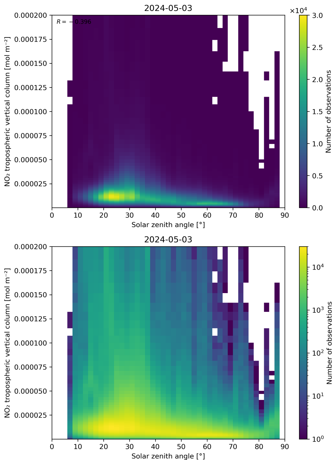
Figure 155: Scatter density plot of “Solar zenith angle” against “NO 2 tropospheric vertical column” for 2024-05-02 to 2024-05-04.
