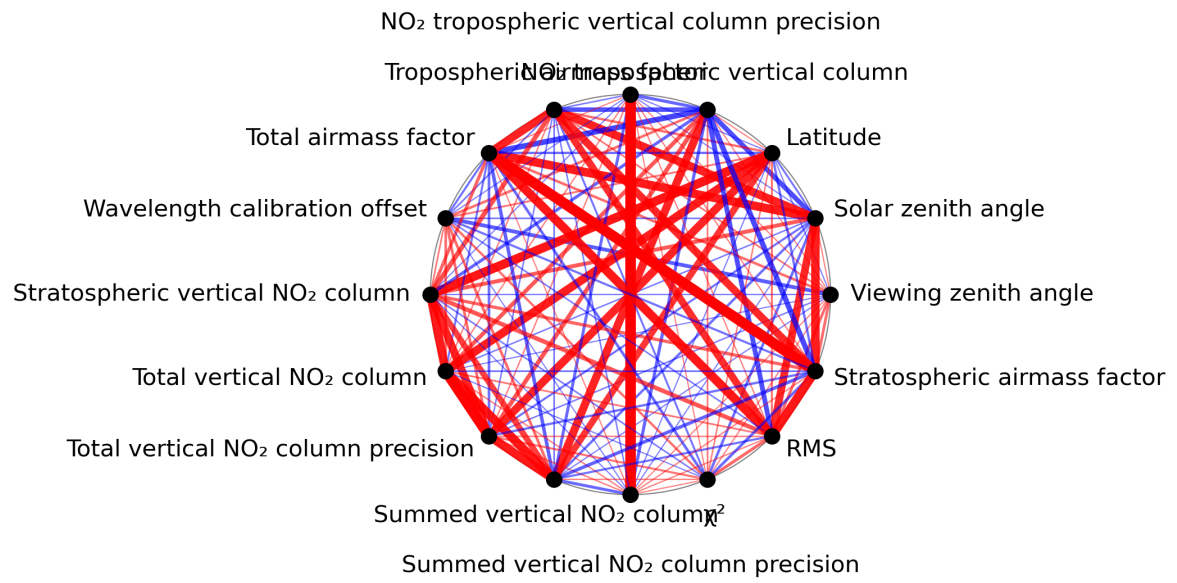
Figure 1: Map of correlation graph for 2024-05-02 to 2024-05-04.
