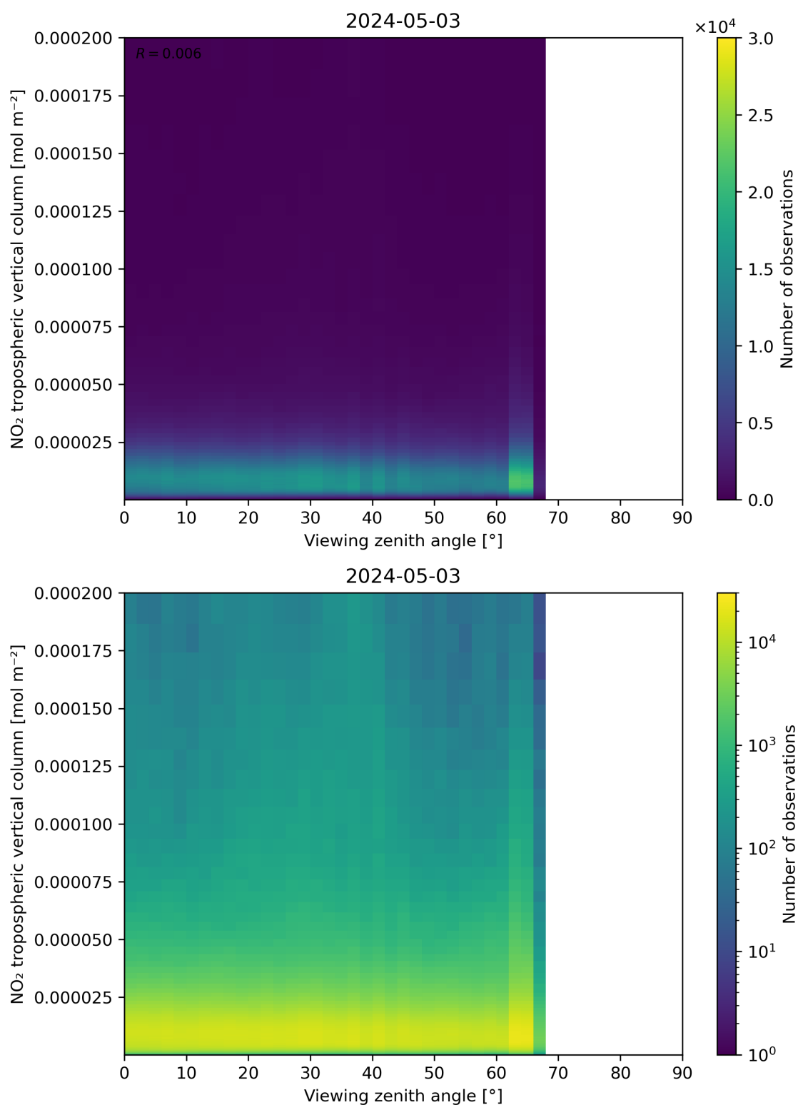
Figure 169: Scatter density plot of “Viewing zenith angle” against “NO 2 tropospheric vertical column” for 2024-05-02 to 2024-05-04.
