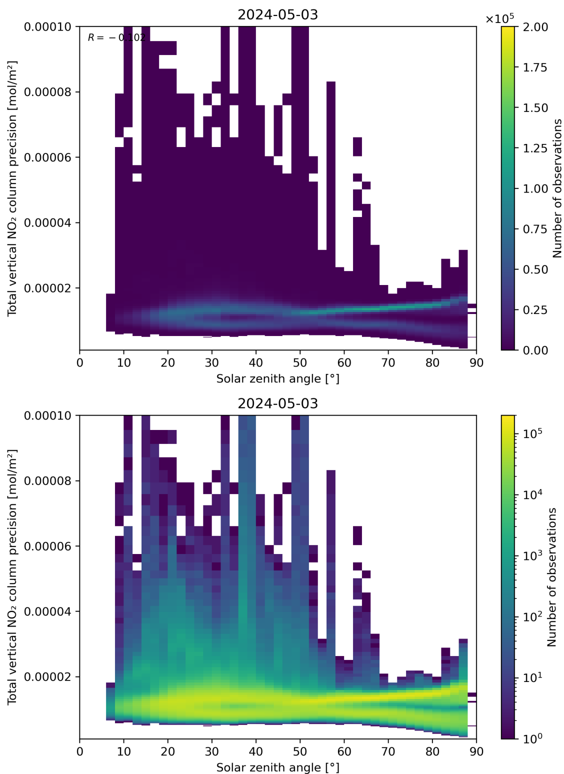
Figure 154: Scatter density plot of “Solar zenith angle” against “Total vertical NO 2 column precision” for 2024-05-02 to 2024-05-04.
