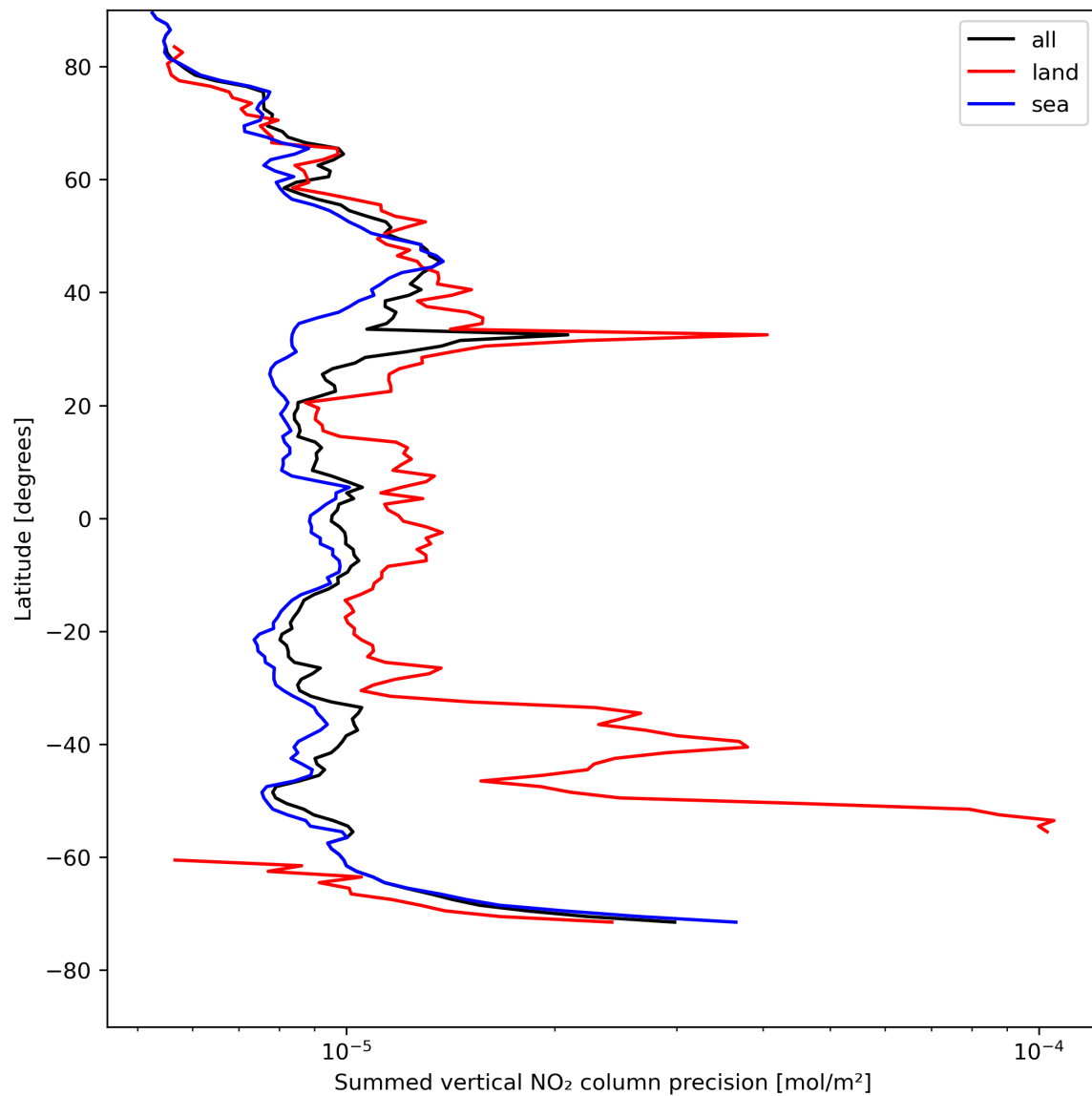
Figure 24: Zonal average of “Summed vertical NO 2 column precision” for 2024-05-02 to 2024-05-04.
