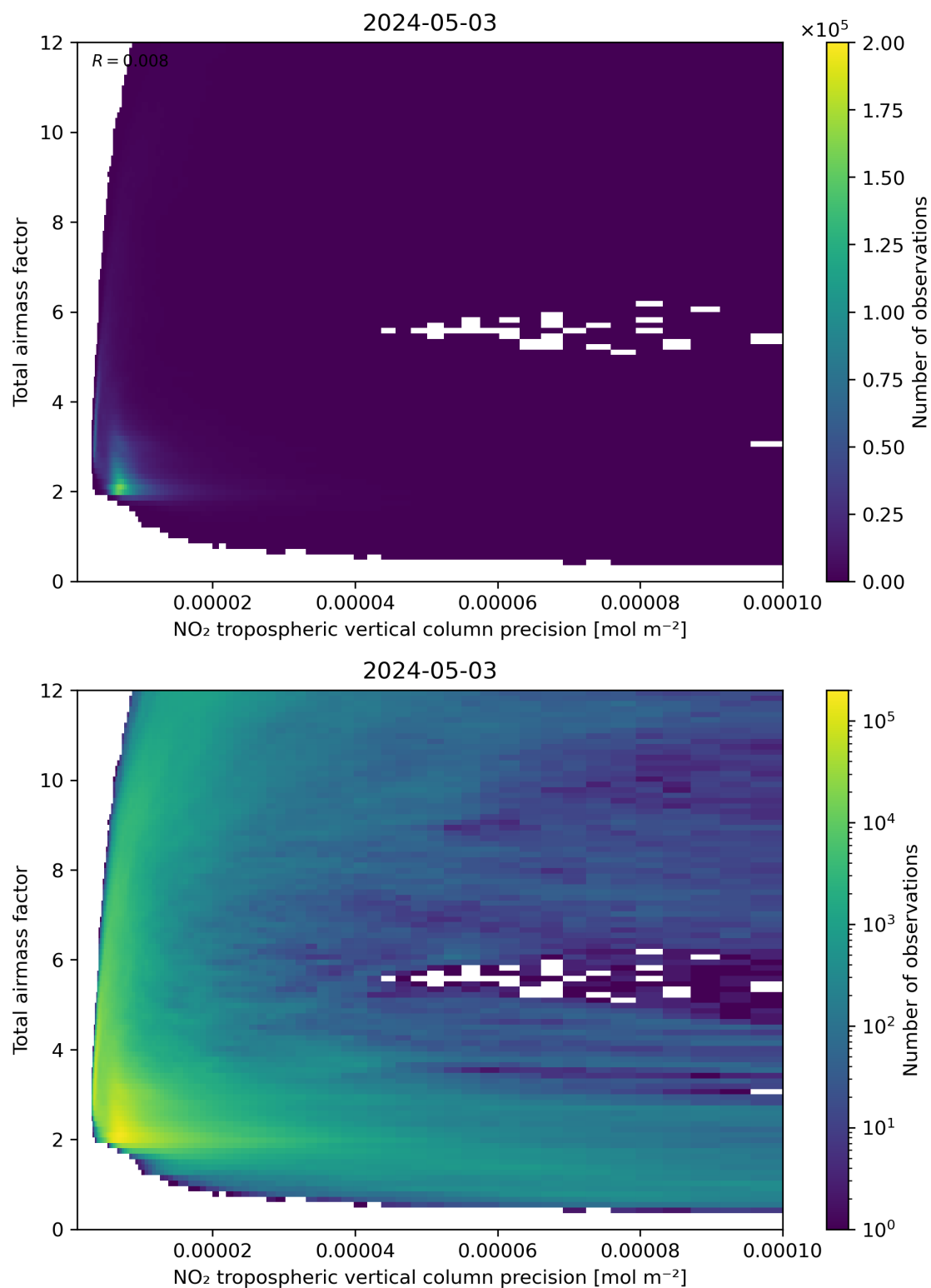
Figure 132: Scatter density plot of “NO 2 tropospheric vertical column precision” against “Total air mass factor” for 2024-05-02 to 2024-05-04.
