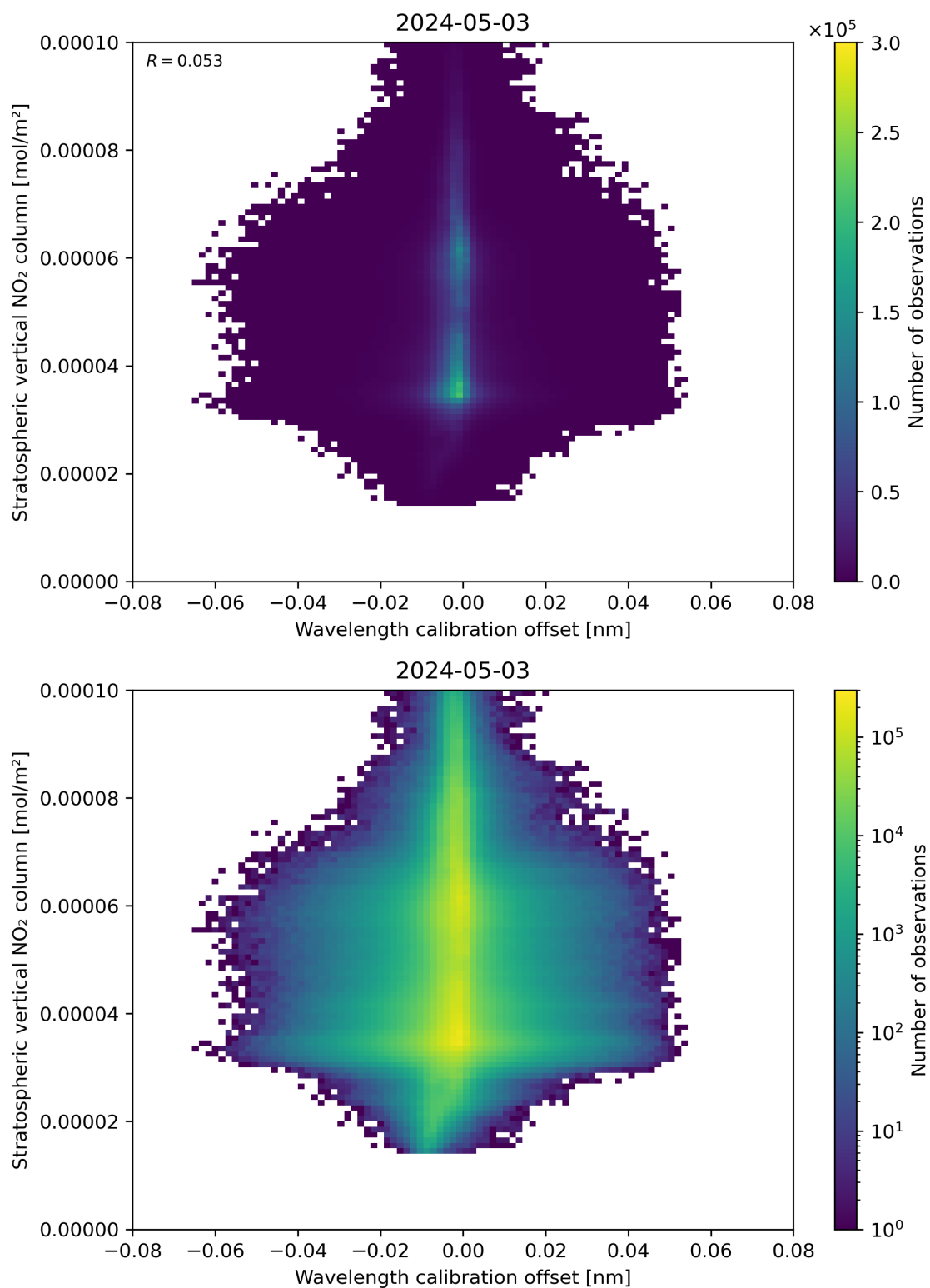
Figure 176: Scatter density plot of “Wavelength calibration offset” against “Stratospheric vertical NO 2 column” for 2024-05-02 to 2024-05-04.
