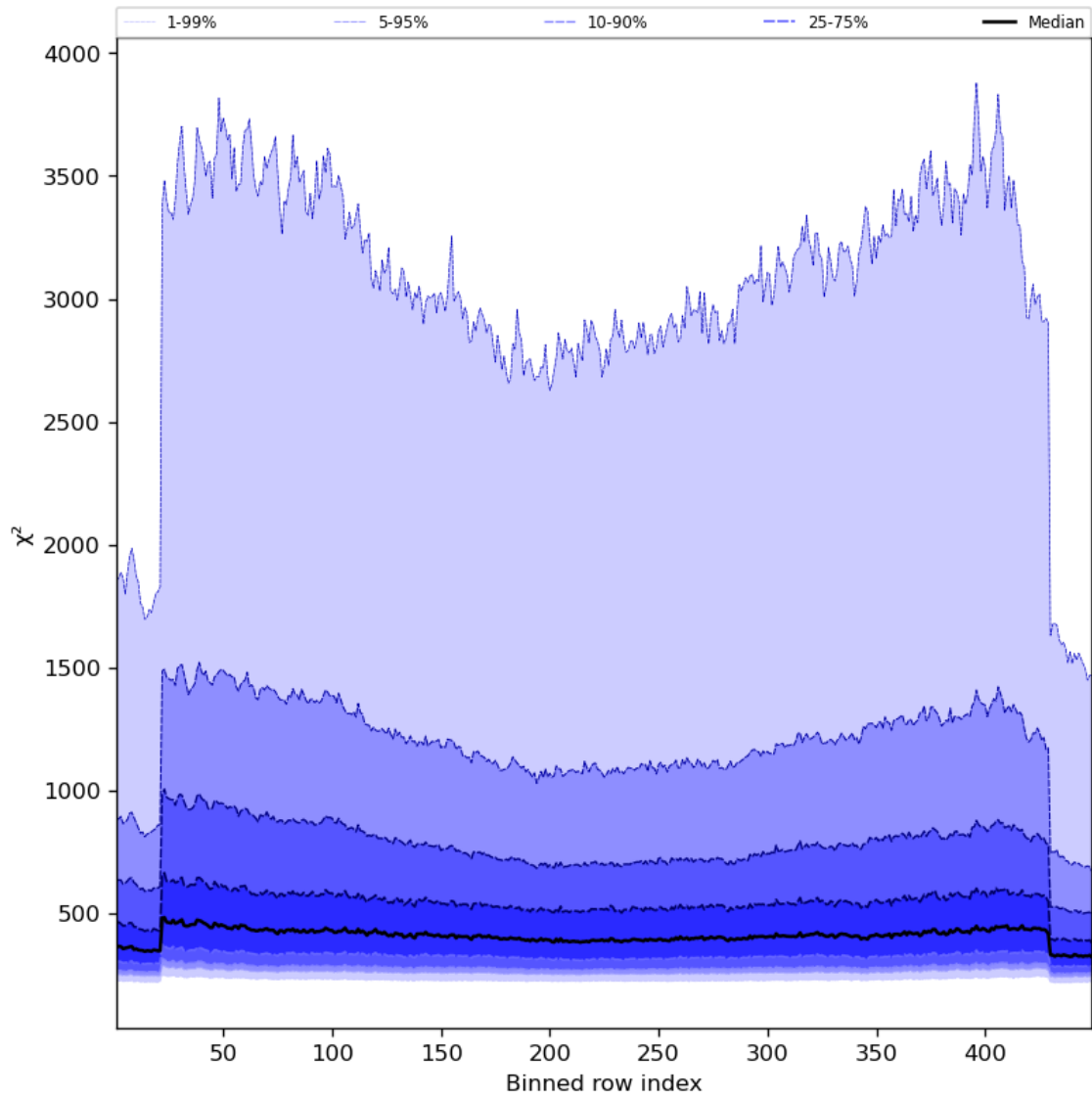
Figure 59: Along track statistics of “ \chi^2 ” for 2024-05-02 to 2024-05-04
