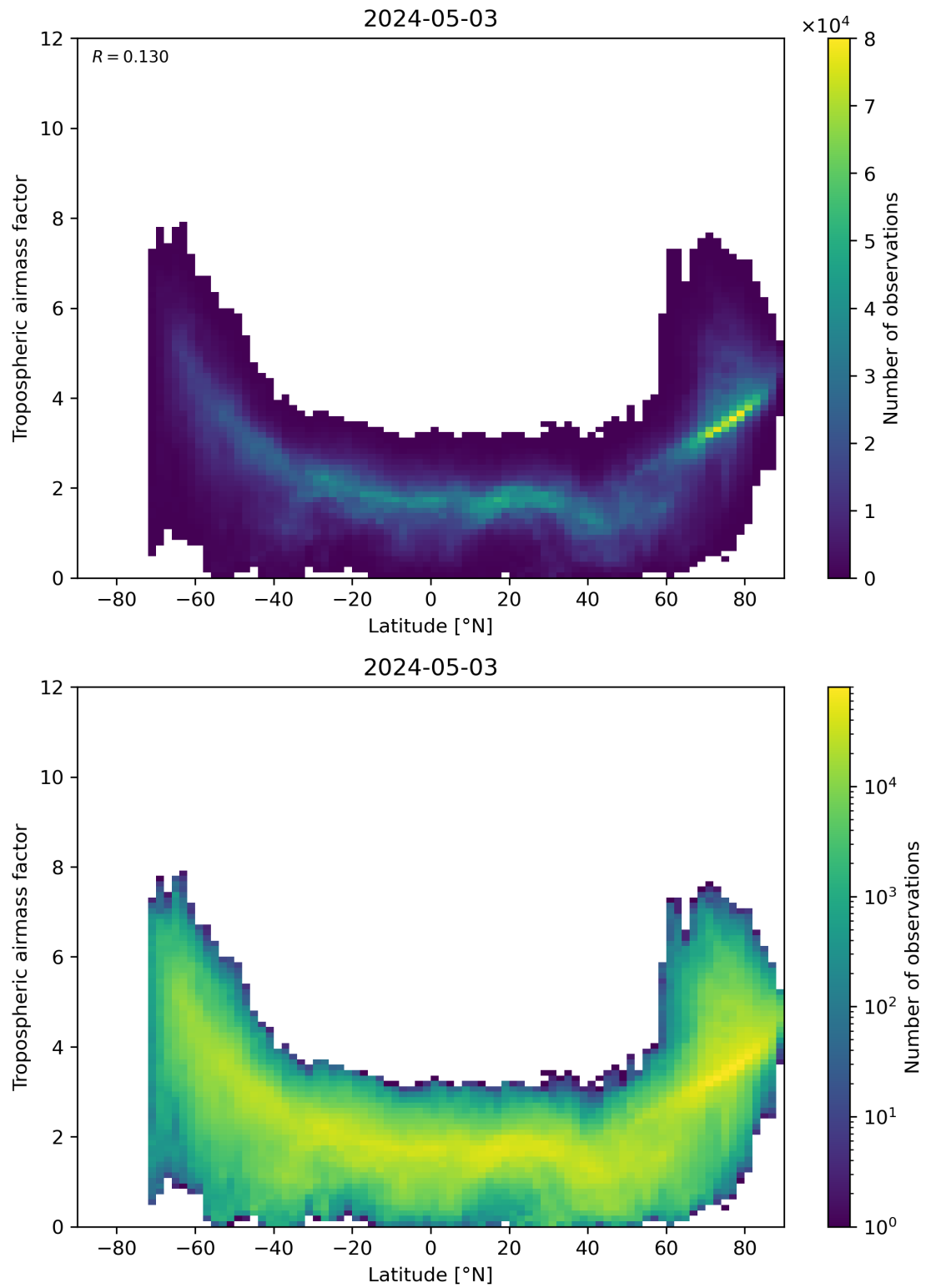
Figure 85: Scatter density plot of “Latitude” against “Tropospheric airmass factor” for 2024-05-02 to 2024-05-04.
