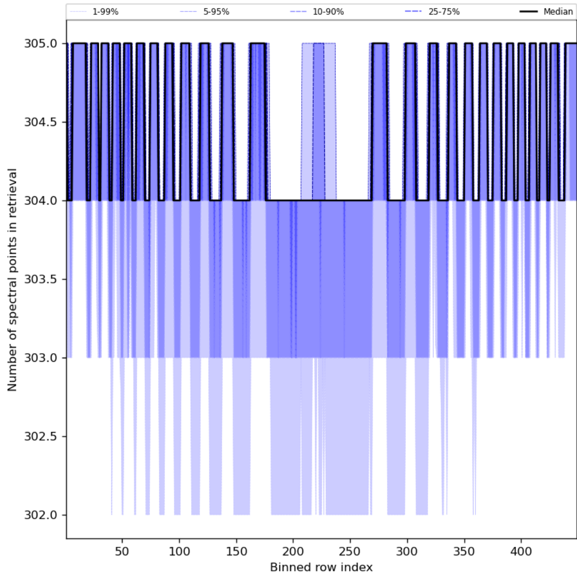
Figure 50: Along track statistics of “Number of spectral points in retrieval” for 2024-05-02 to 2024-05-04
