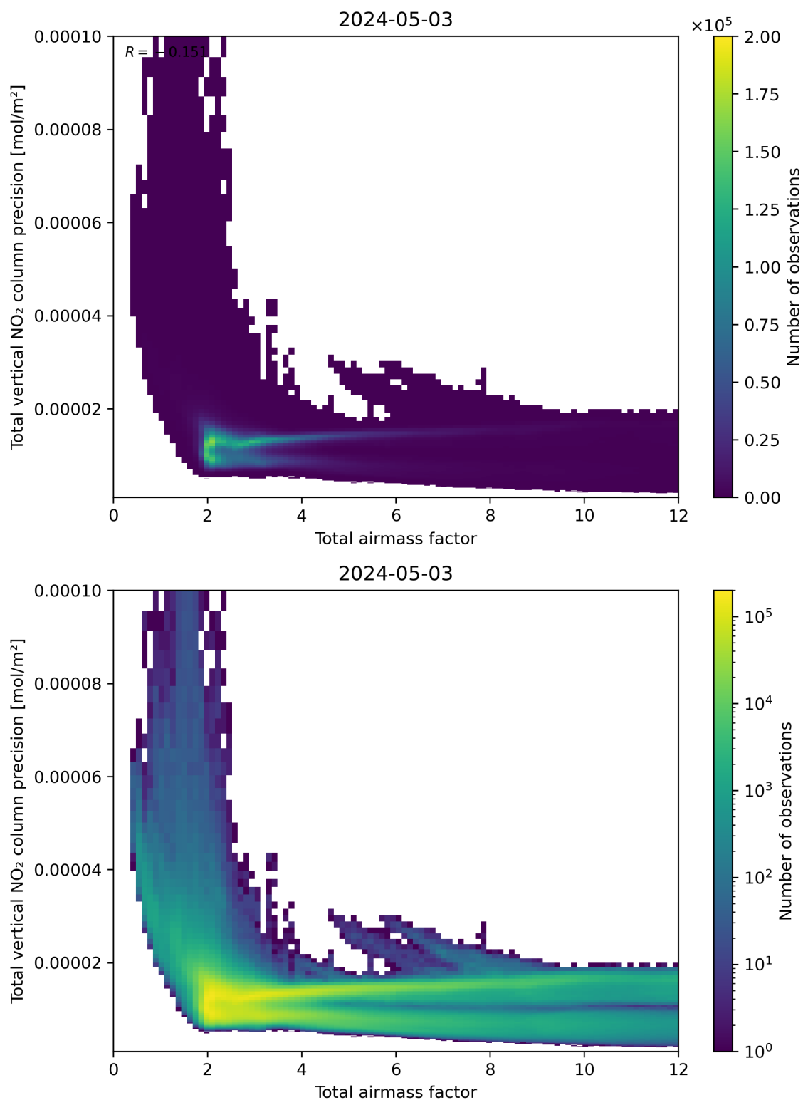
Figure 68: Scatter density plot of “Total airmass factor” against “Total vertical NO 2 column precision” for 2024-05-02 to 2024-05-04.
