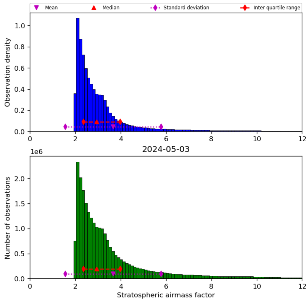
Figure 44: Histogram of “Stratospheric airmass factor” for 2024-05-02 to 2024-05-04
