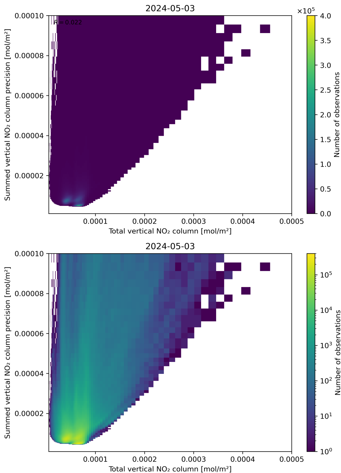
Figure 113: Scatter density plot of “Total vertical NO 2 column” against “Summed vertical NO 2 column precision” for 2024-05-02 to 2024-05-04.
