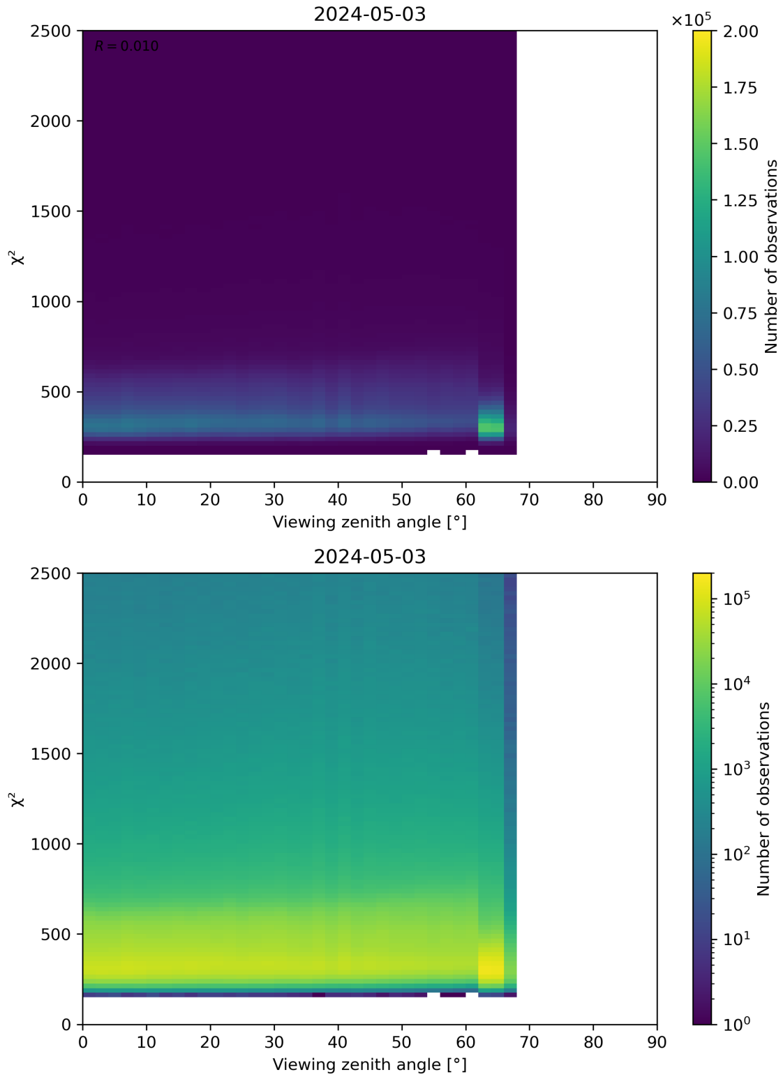
Figure 162: Scatter density plot of “Viewing zenith angle” against “ \chi^2 ” for 2024-05-02 to 2024-05-04.
