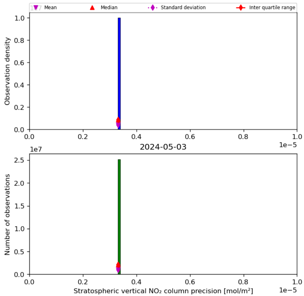
Figure 37: Histogram of “Stratospheric vertical NO 2 column precision” for 2024-05-02 to 2024-05-04
