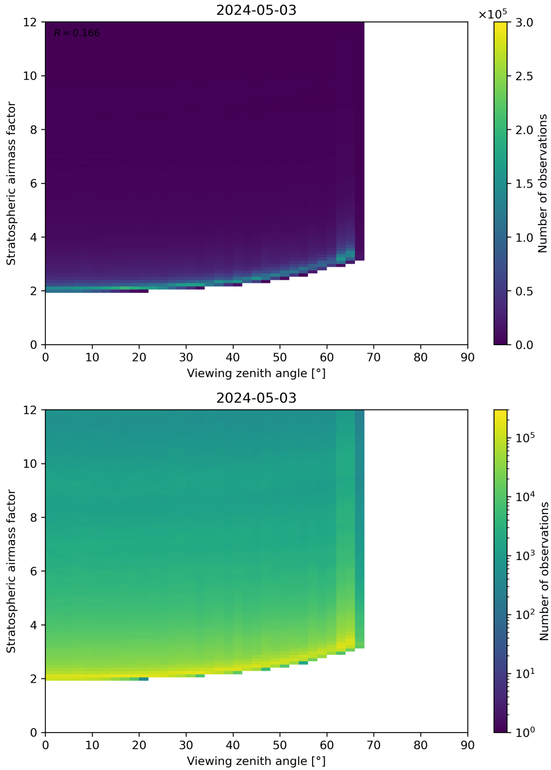
Figure 159: Scatter density plot of “Viewing zenith angle” against “Stratospheric airmass factor” for 2024-05-02 to 2024-05-04.
