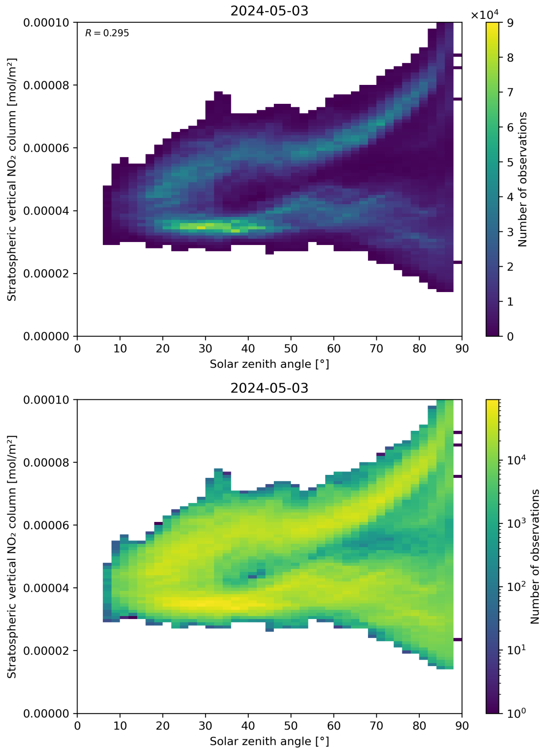
Figure 150: Scatter density plot of “Solar zenith angle” against “Stratospheric vertical NO 2 column” for 2024-05-02 to 2024-05-04.
