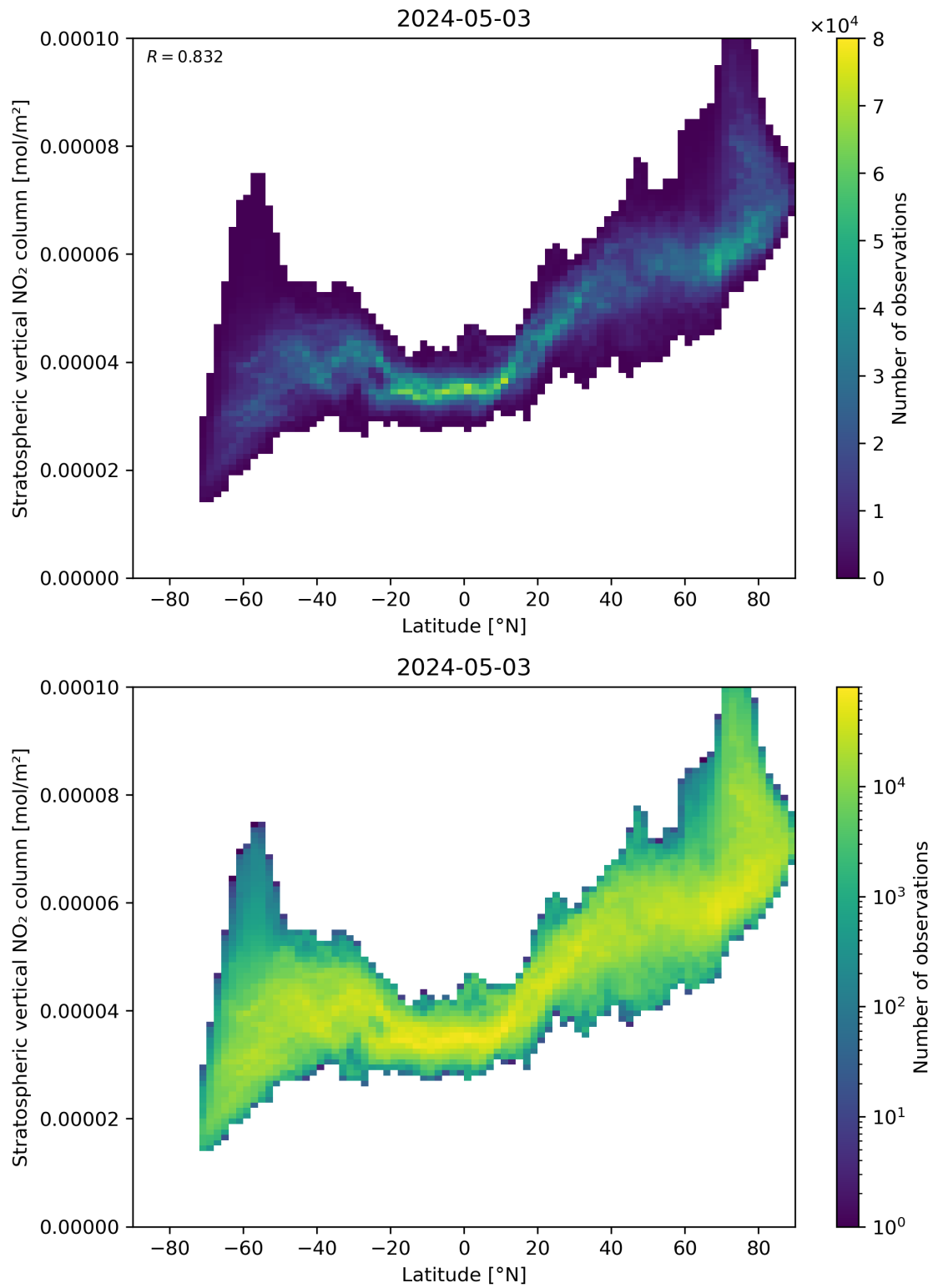
Figure 87: Scatter density plot of “Latitude” against “Stratospheric vertical NO 2 column” for 2024-05-02 to 2024-05-04.
