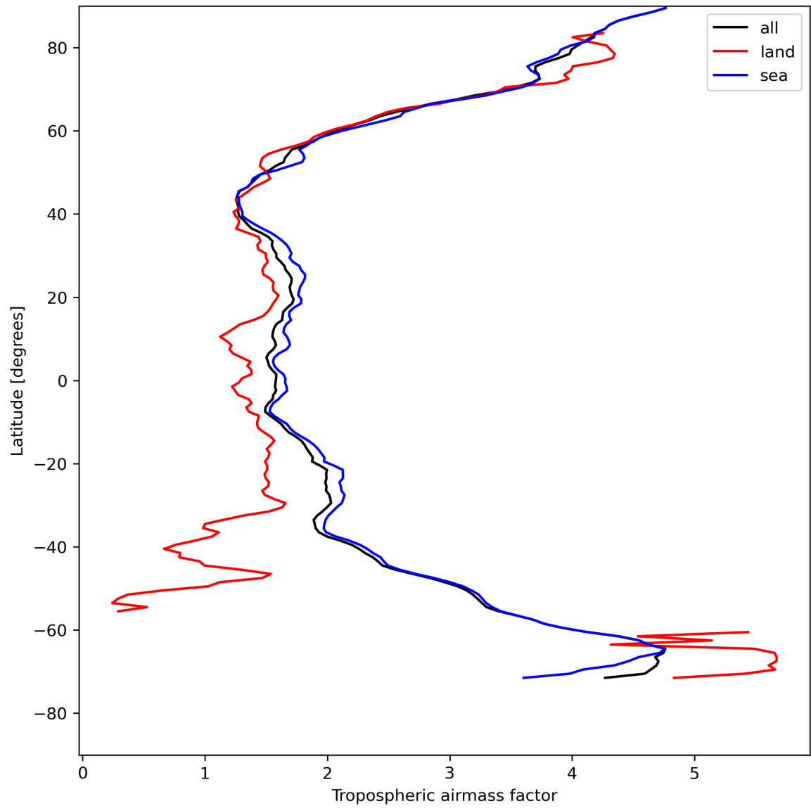
Figure 14: Zonal average of “Tropospheric airmass factor” for 2024-05-02 to 2024-05-04.
