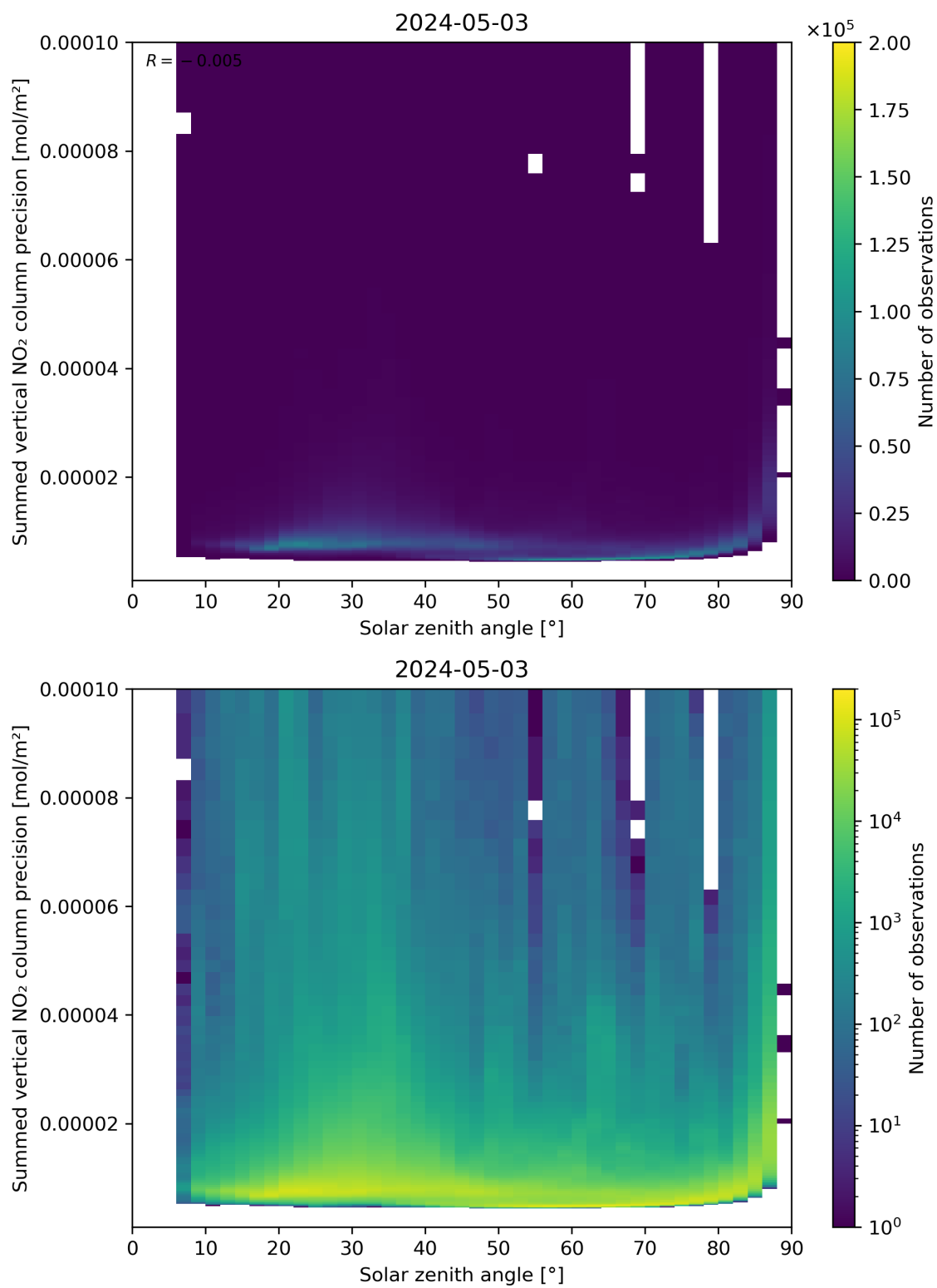
Figure 152: Scatter density plot of “Solar zenith angle” against “Summed vertical NO 2 column precision” for 2024-05-02 to 2024-05-04.
