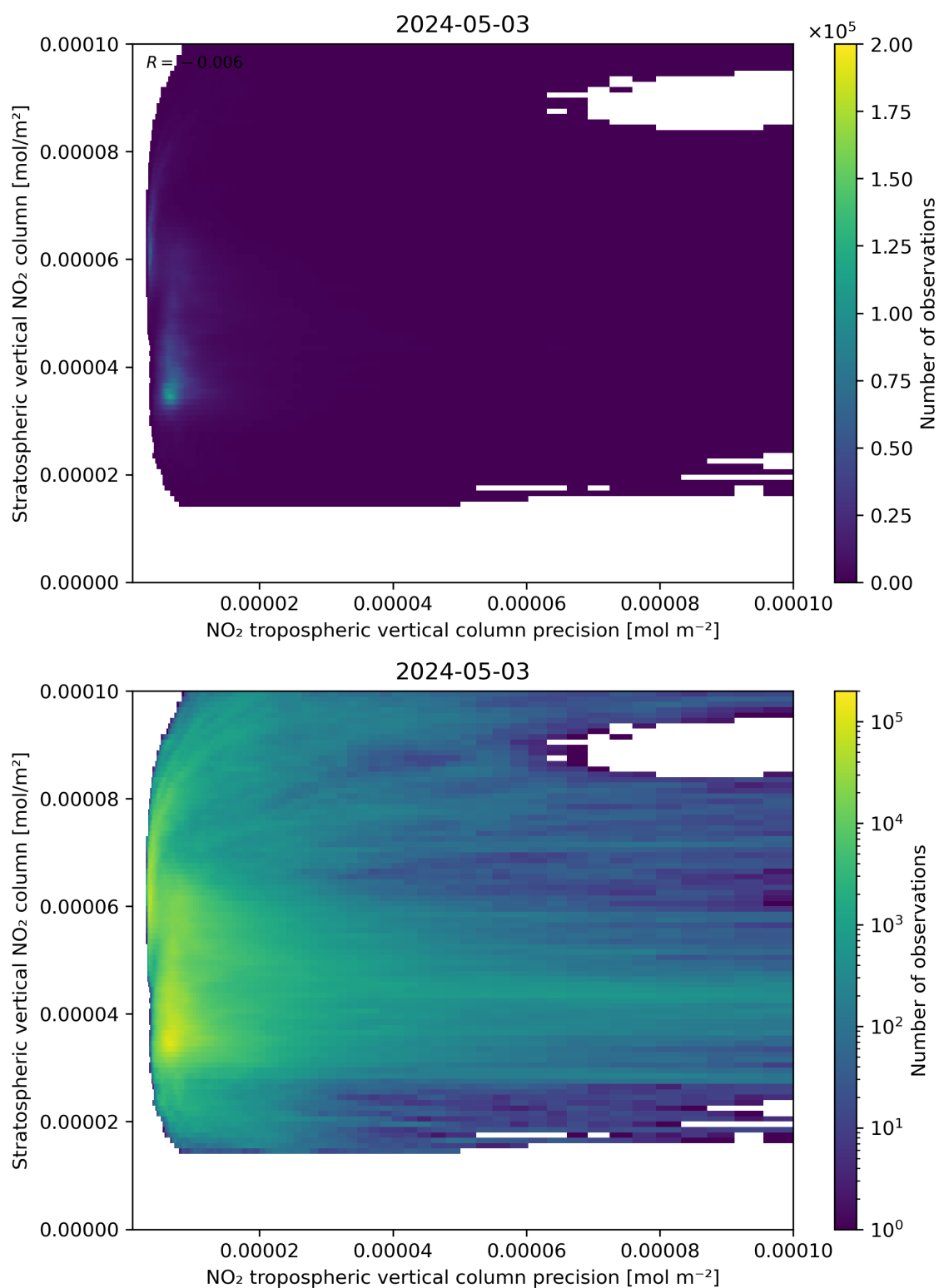
Figure 135: Scatter density plot of “NO 2 tropospheric vertical column precision” against “Stratospheric vertical NO 2 column” for 2024-05-02 to 2024-05-04.
