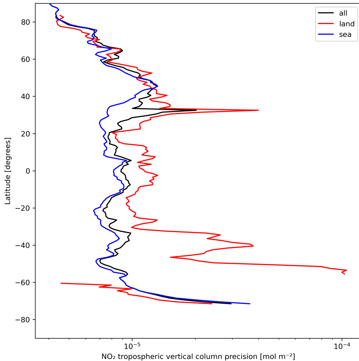
Figure 13: Zonal average of “NO 2 tropospheric vertical column precision” for 2024-05-02 to 2024-05-04.
