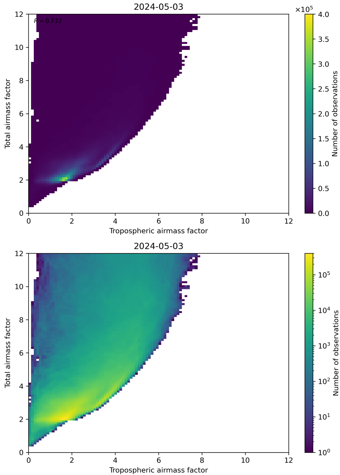
Figure 72: Scatter density plot of “Tropospheric airmass factor” against “Total airmass factor” for 2024-05-02 to 2024-05-04.
