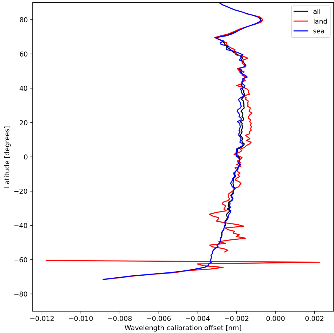
Figure 18: Zonal average of “Wavelength calibration offset” for 2024-05-02 to 2024-05-04.
