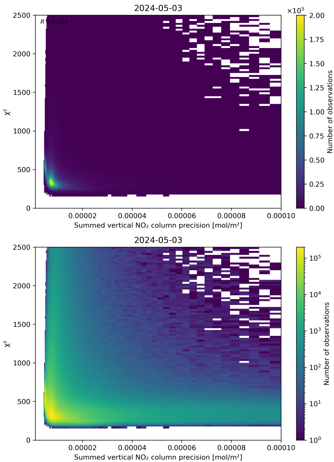
Figure 107: Scatter density plot of “Summed vertical NO 2 column precision” against “ \chi^2 ” for 2024-05-02 to 2024-05-04.
