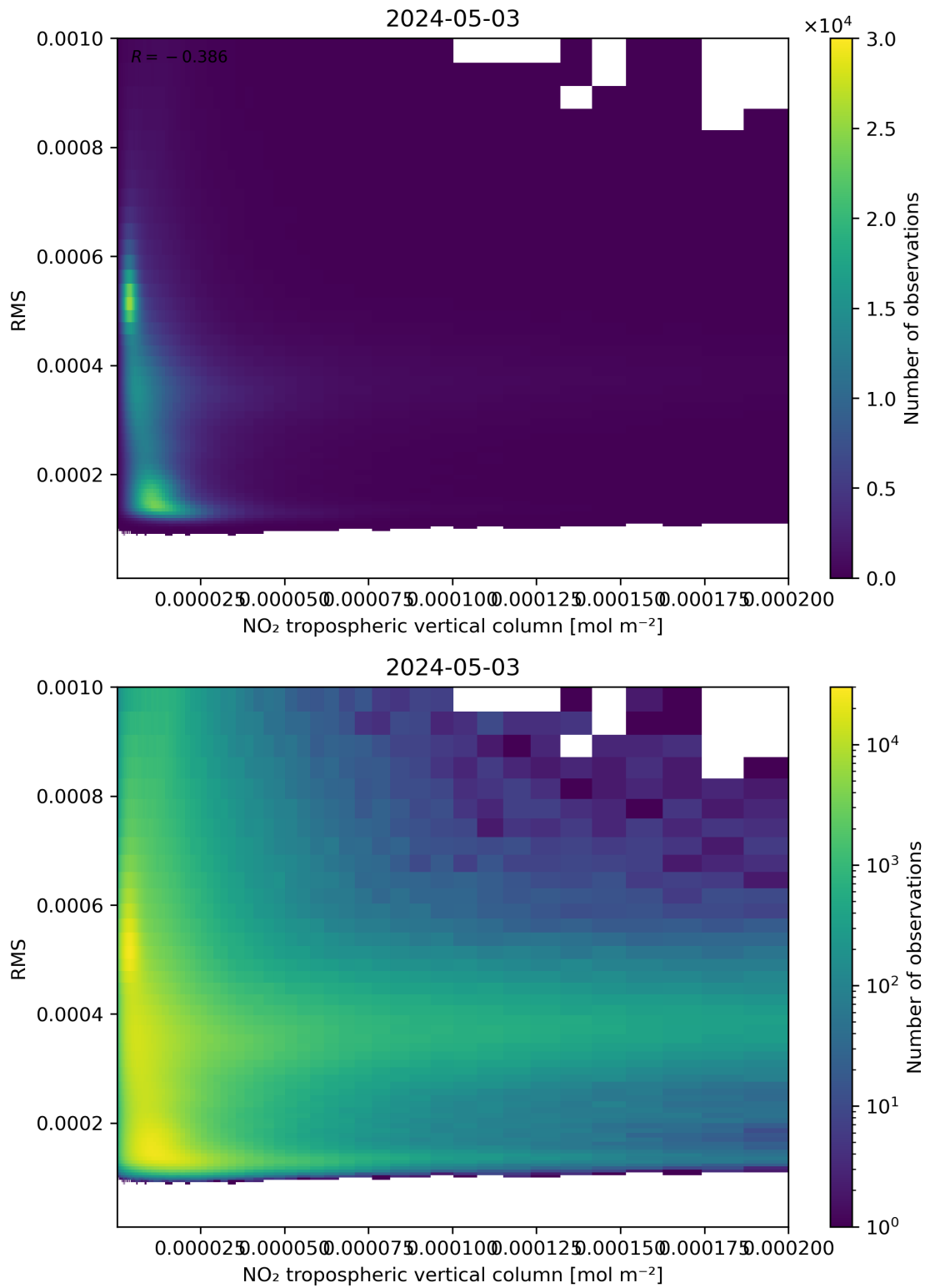
Figure 142: Scatter density plot of “NO 2 tropospheric vertical column” against “RMS” for 2024-05-02 to 2024-05-04.
