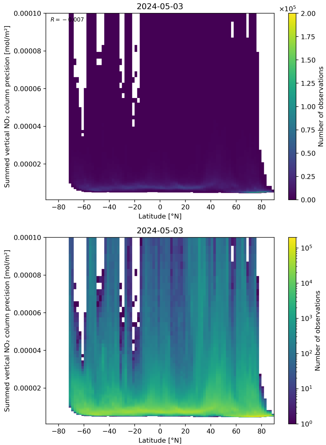
Figure 89: Scatter density plot of “Latitude” against “Summed vertical NO 2 column precision” for 2024-05-02 to 2024-05-04.
