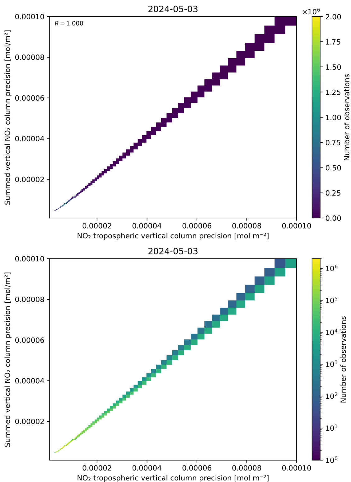
Figure 137: Scatter density plot of “NO 2 tropospheric vertical column precision” against “Summed vertical NO 2 column precision” for 2024-05-02 to 2024-05-04.
