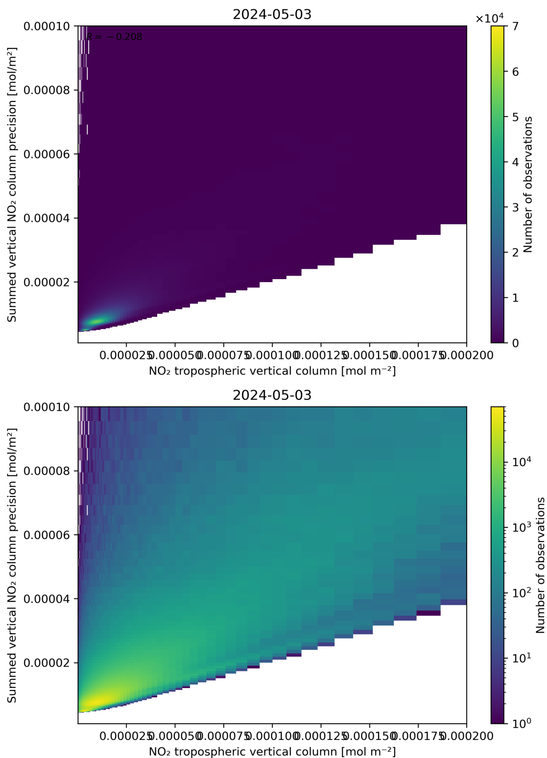
Figure 127: Scatter density plot of “NO 2 tropospheric vertical column” against “Summed vertical NO 2 column precision” for 2024-05-02 to 2024-05-04.
