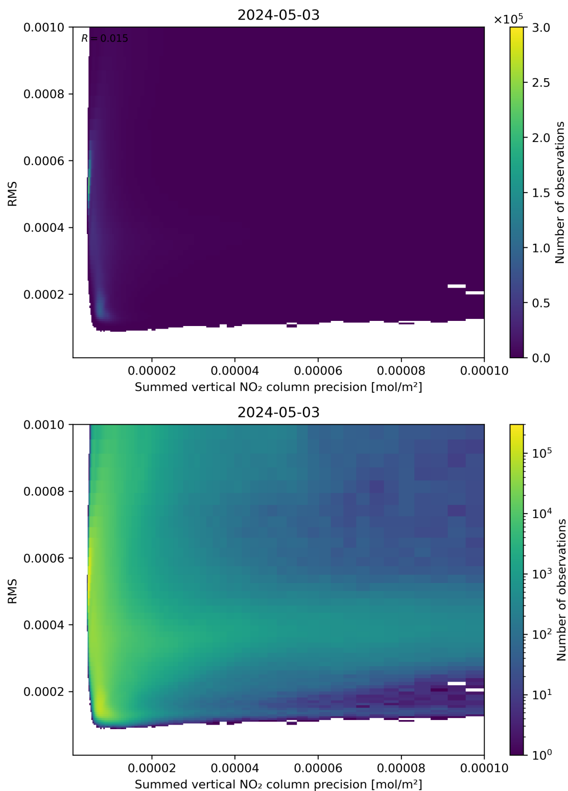
Figure 108: Scatter density plot of “Summed vertical NO 2 column precision” against “RMS” for 2024-05-02 to 2024-05-04.
