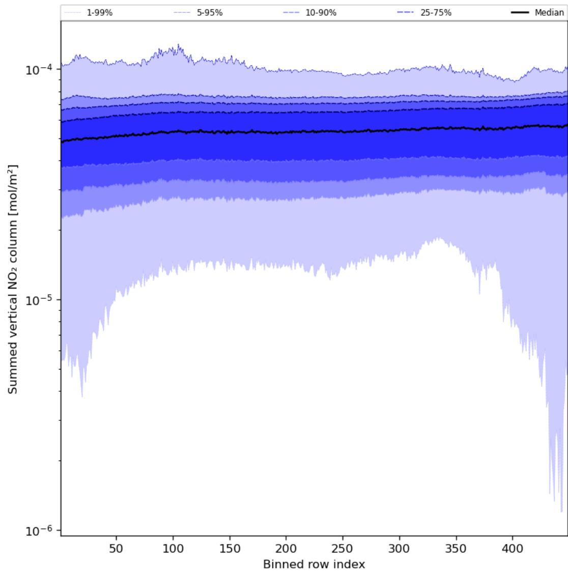
Figure 57: Along track statistics of “Summed vertical NO 2 column” for 2024-05-02 to 2024-05-04
