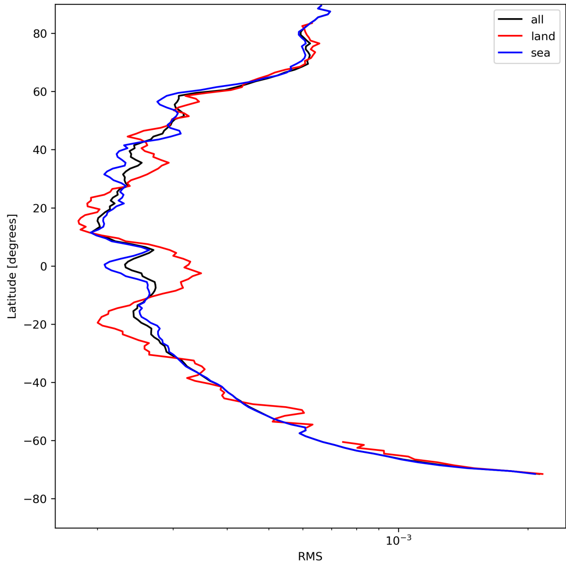
Figure 26: Zonal average of “RMS” for 2024-05-02 to 2024-05-04.
