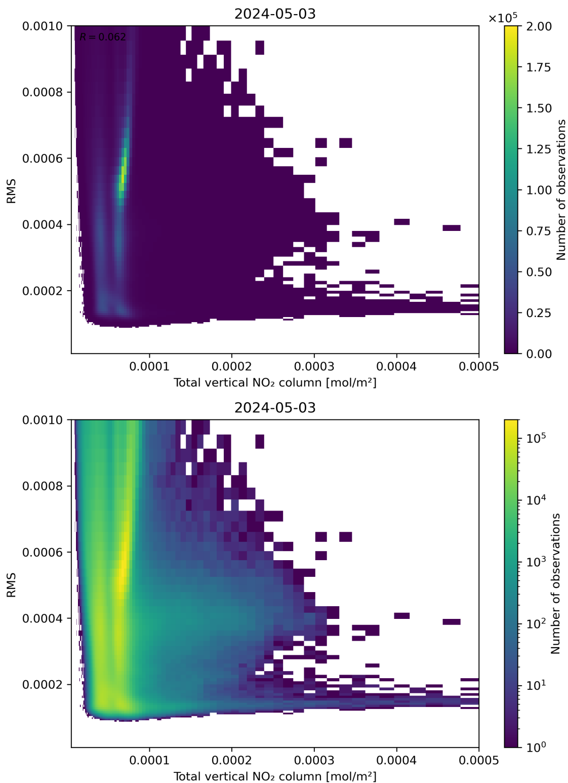
Figure 120: Scatter density plot of “Total vertical NO 2 column” against “RMS” for 2024-05-02 to 2024-05-04.
