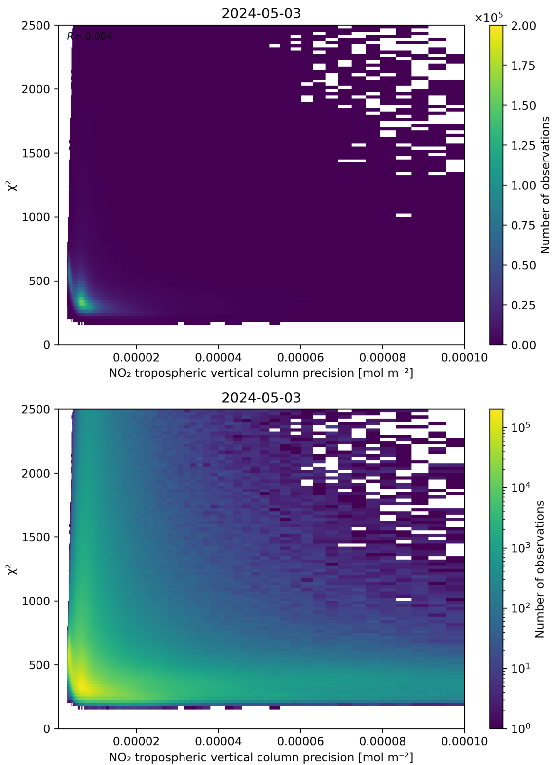
Figure 134: Scatter density plot of “NO 2 tropospheric vertical column precision” against “ \chi^2 ” for 2024-05-02 to 2024-05-04.
