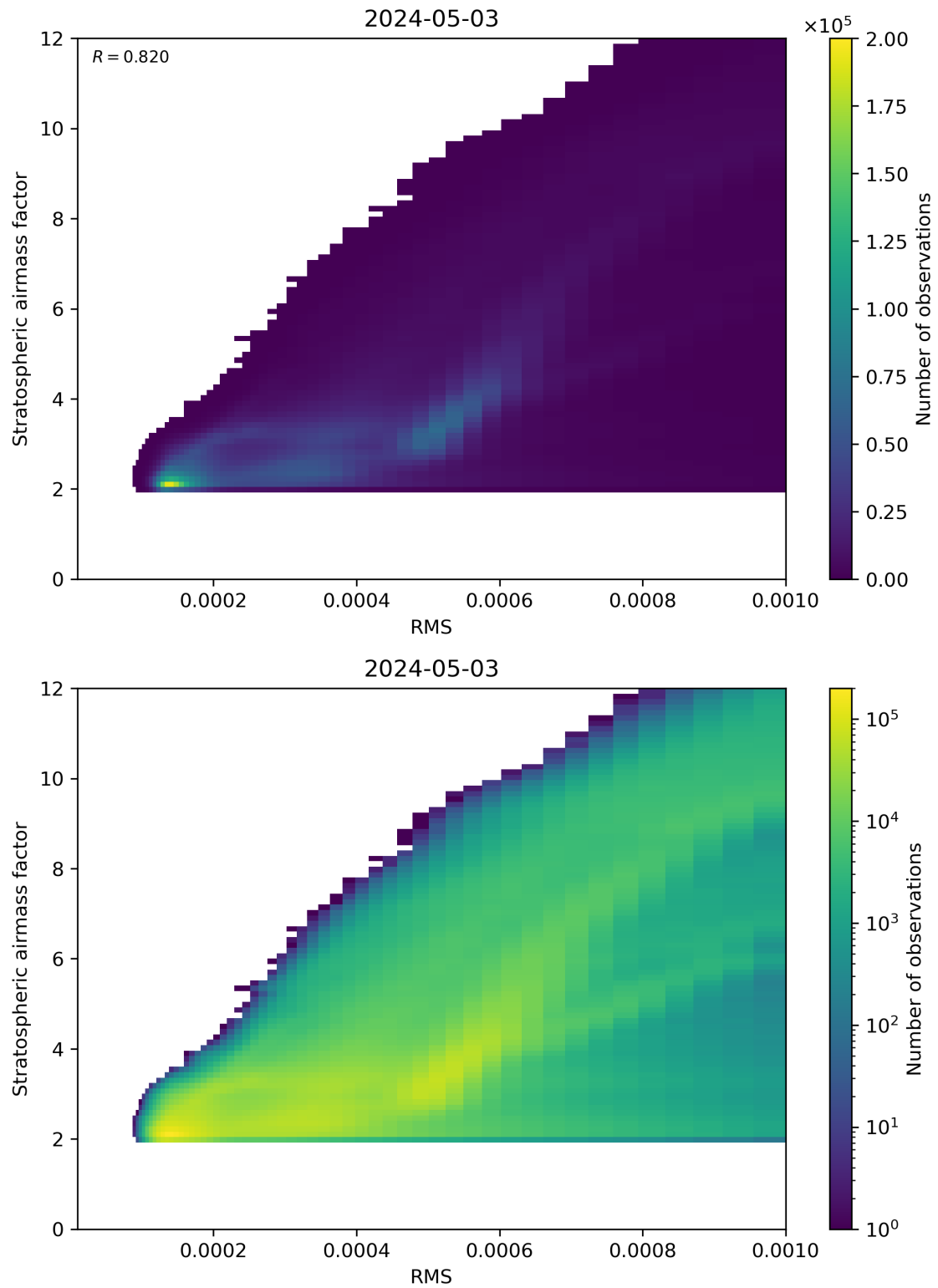
Figure 144: Scatter density plot of “RMS” against “Stratospheric airmass factor” for 2024-05-02 to 2024-05-04.
