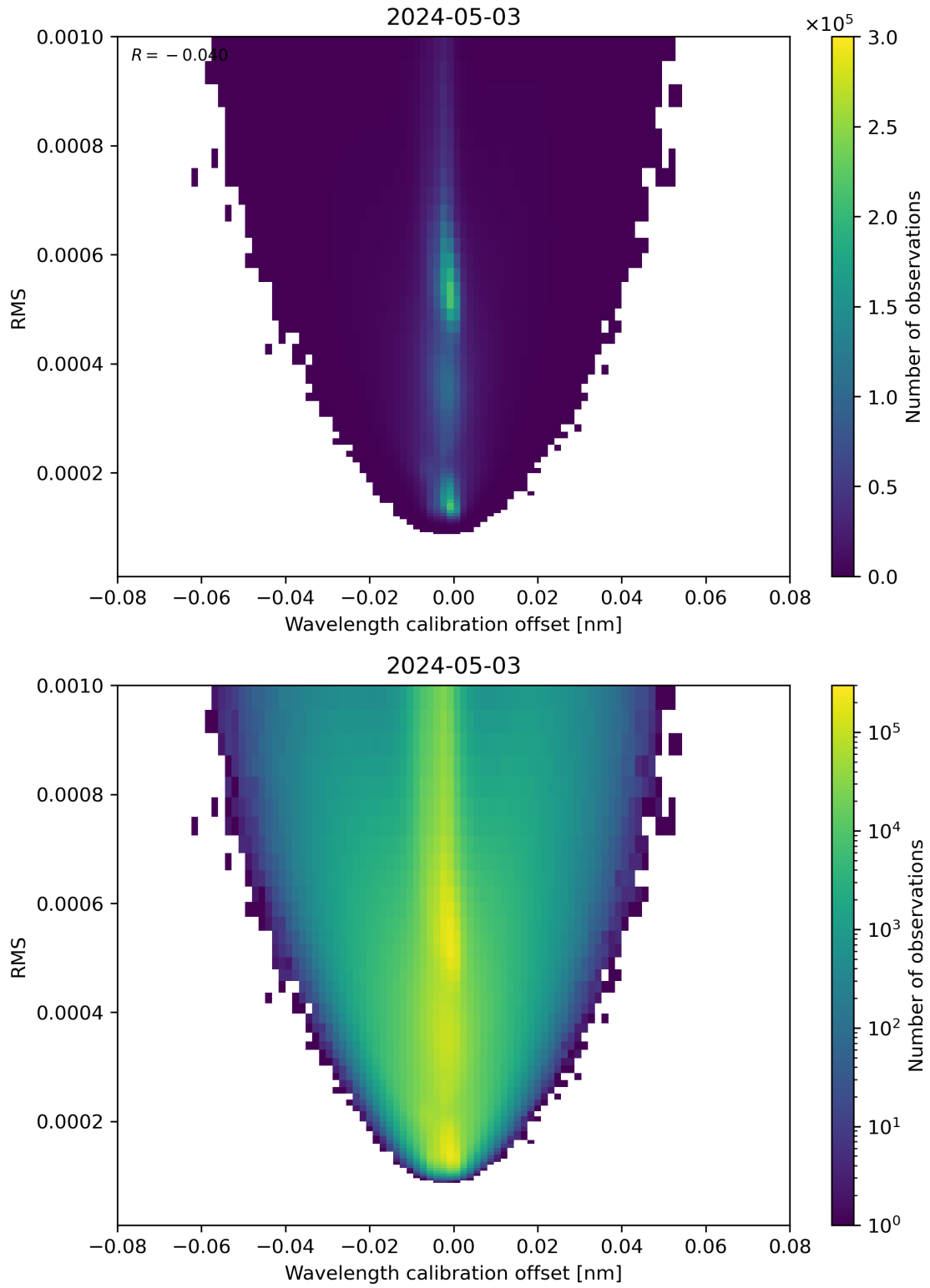
Figure 181: Scatter density plot of “Wavelength calibration offset” against “RMS” for 2024-05-02 to 2024-05-04.
