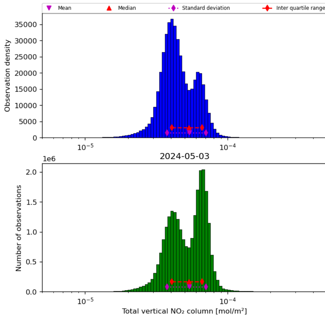
Figure 38: Histogram of “Total vertical NO 2 column” for 2024-05-02 to 2024-05-04
