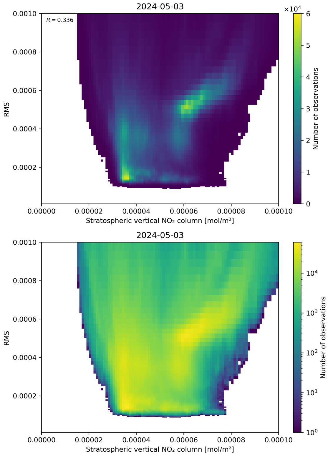
Figure 102: Scatter density plot of “Stratospheric vertical NO 2 column” against “RMS” for 2024-05-02 to 2024-05-04.
