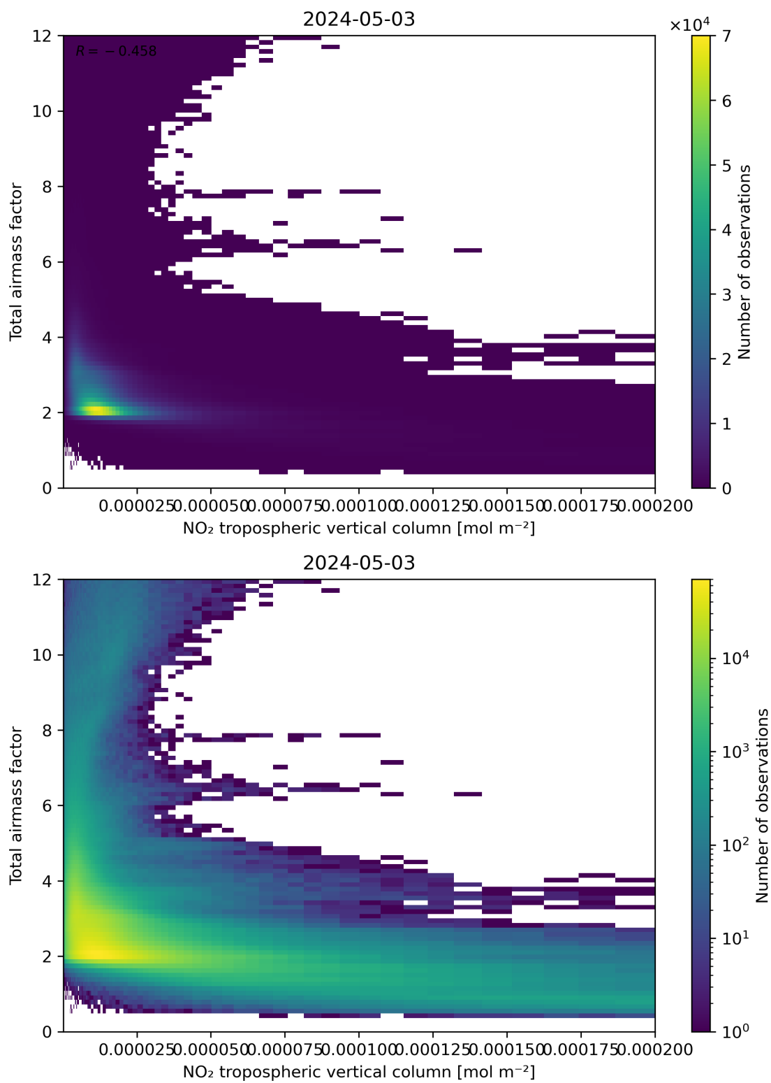
Figure 122: Scatter density plot of “NO 2 tropospheric vertical column” against “Total air mass factor” for 2024-05-02 to 2024-05-04.
