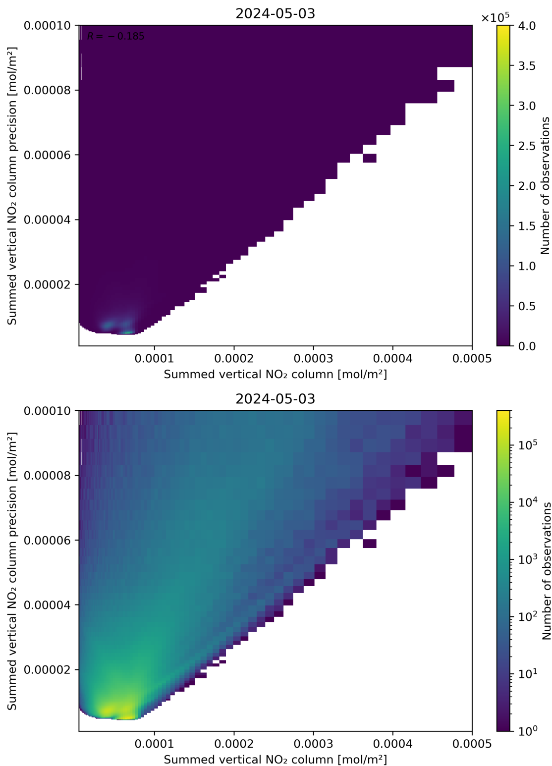
Figure 105: Scatter density plot of “Summed vertical NO 2 column” against “Summed vertical NO 2 column precision” for 2024-05-02 to 2024-05-04.
