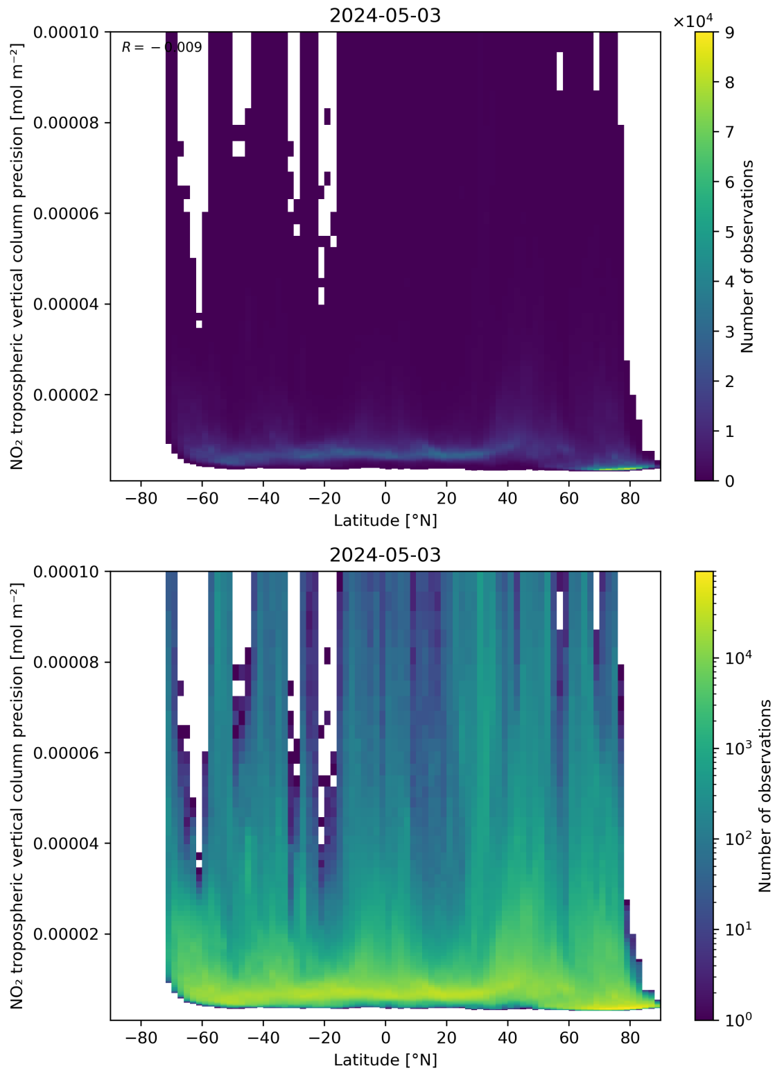
Figure 93: Scatter density plot of “Latitude” against “NO 2 tropospheric vertical column precision” for 2024-05-02 to 2024-05-04.
