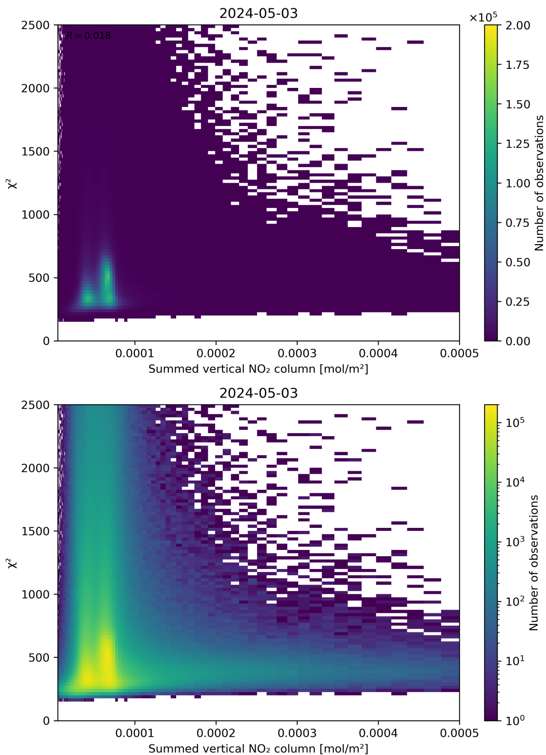
Figure 104: Scatter density plot of “Summed vertical NO 2 column” against “ \chi^2 ” for 2024-05-02 to 2024-05-04.
