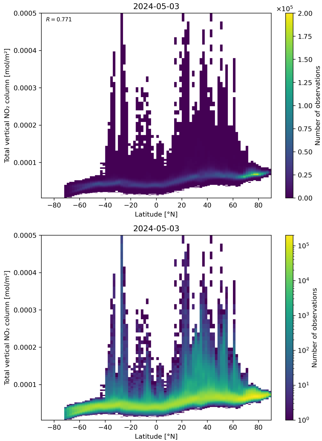
Figure 90: Scatter density plot of “Latitude” against “Total vertical NO 2 column” for 2024-05-02 to 2024-05-04.
