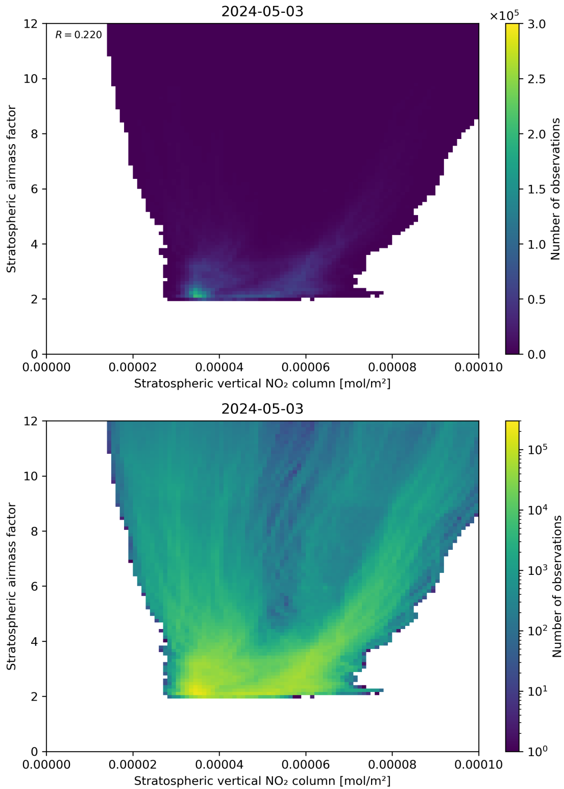
Figure 96: Scatter density plot of “Stratospheric vertical NO 2 column” against “Stratospheric airmass factor” for 2024-05-02 to 2024-05-04.
