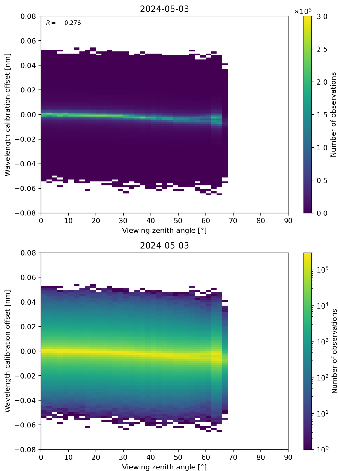
Figure 173: Scatter density plot of “Viewing zenith angle” against “Wavelength calibration offset” for 2024-05-02 to 2024-05-04.
