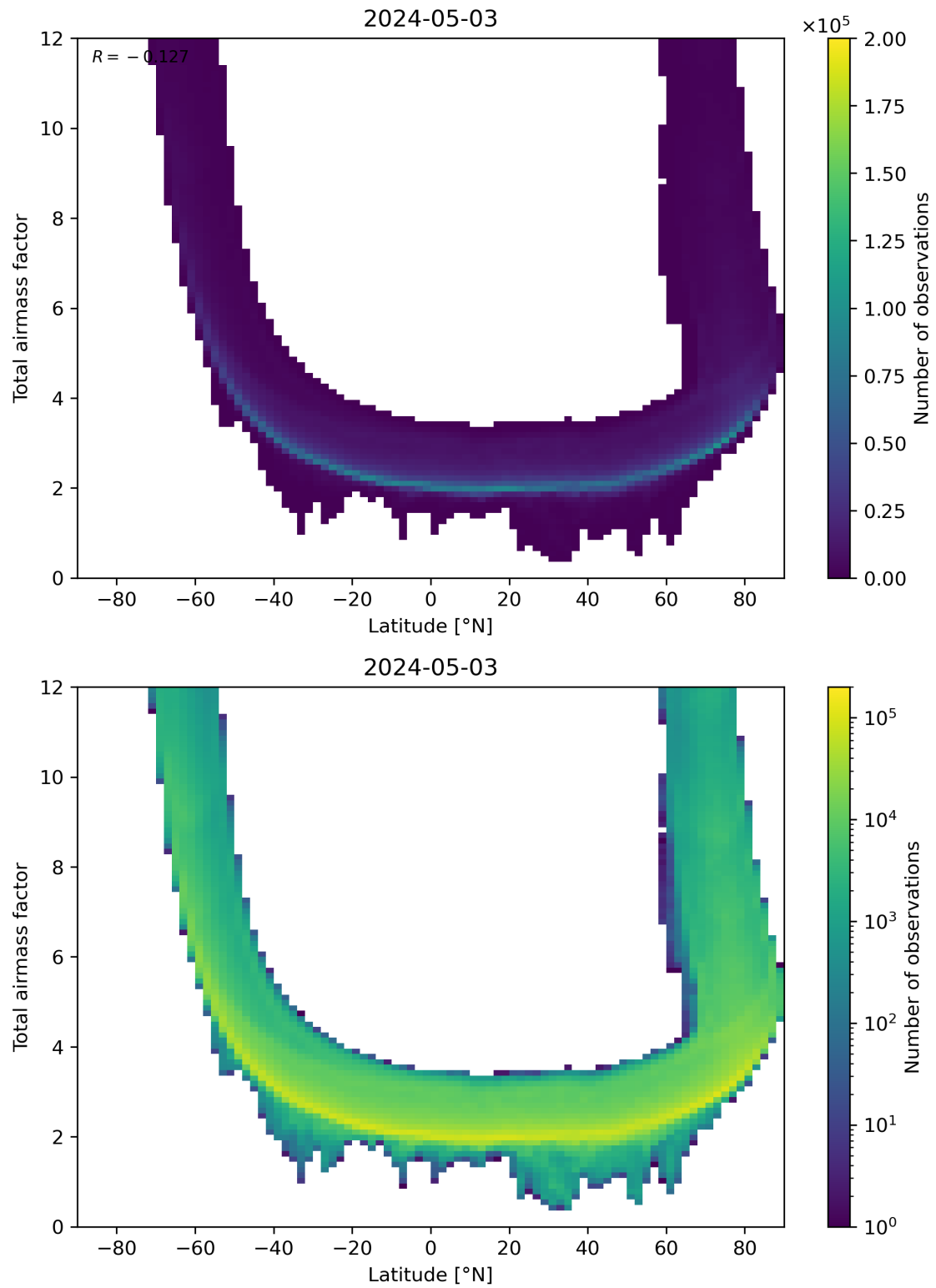
Figure 84: Scatter density plot of “Latitude” against “Total airmass factor” for 2024-05-02 to 2024-05-04.
