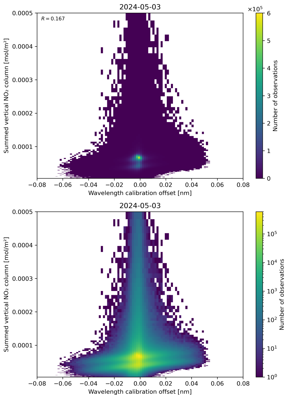
Figure 177: Scatter density plot of “Wavelength calibration offset” against “Summed vertical NO 2 column” for 2024-05-02 to 2024-05-04.
