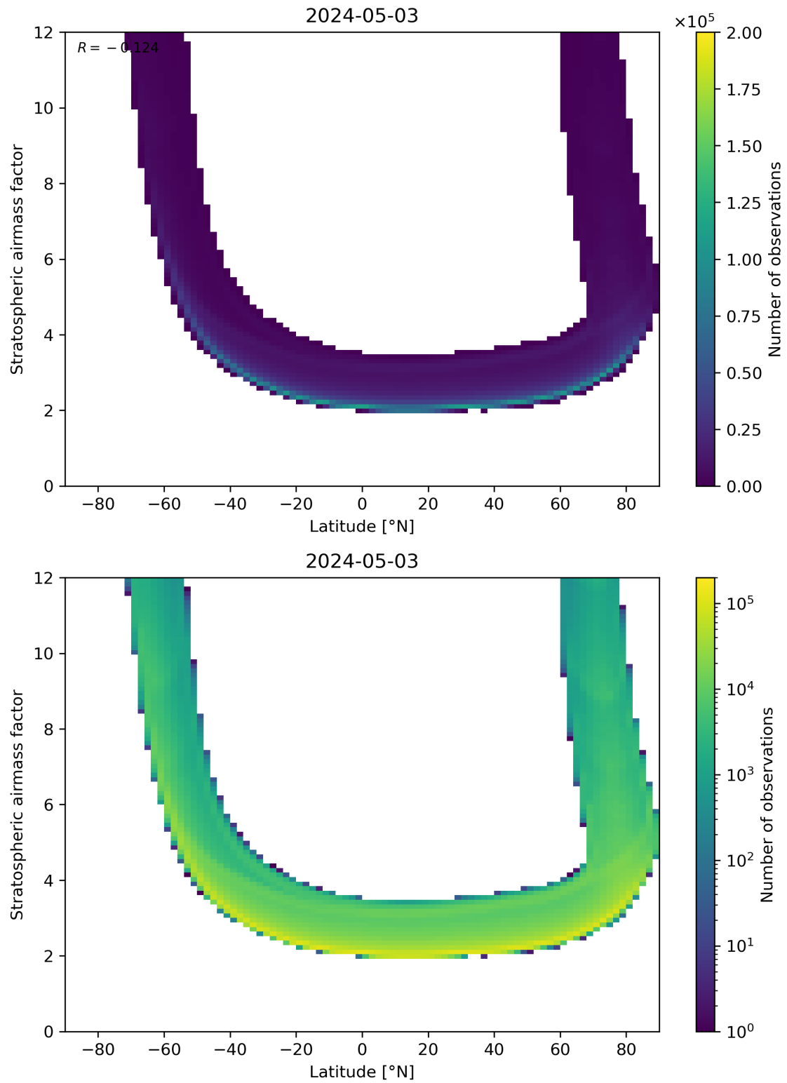
Figure 83: Scatter density plot of “Latitude” against “Stratospheric air mass factor” for 2024-05-02 to 2024-05-04.
