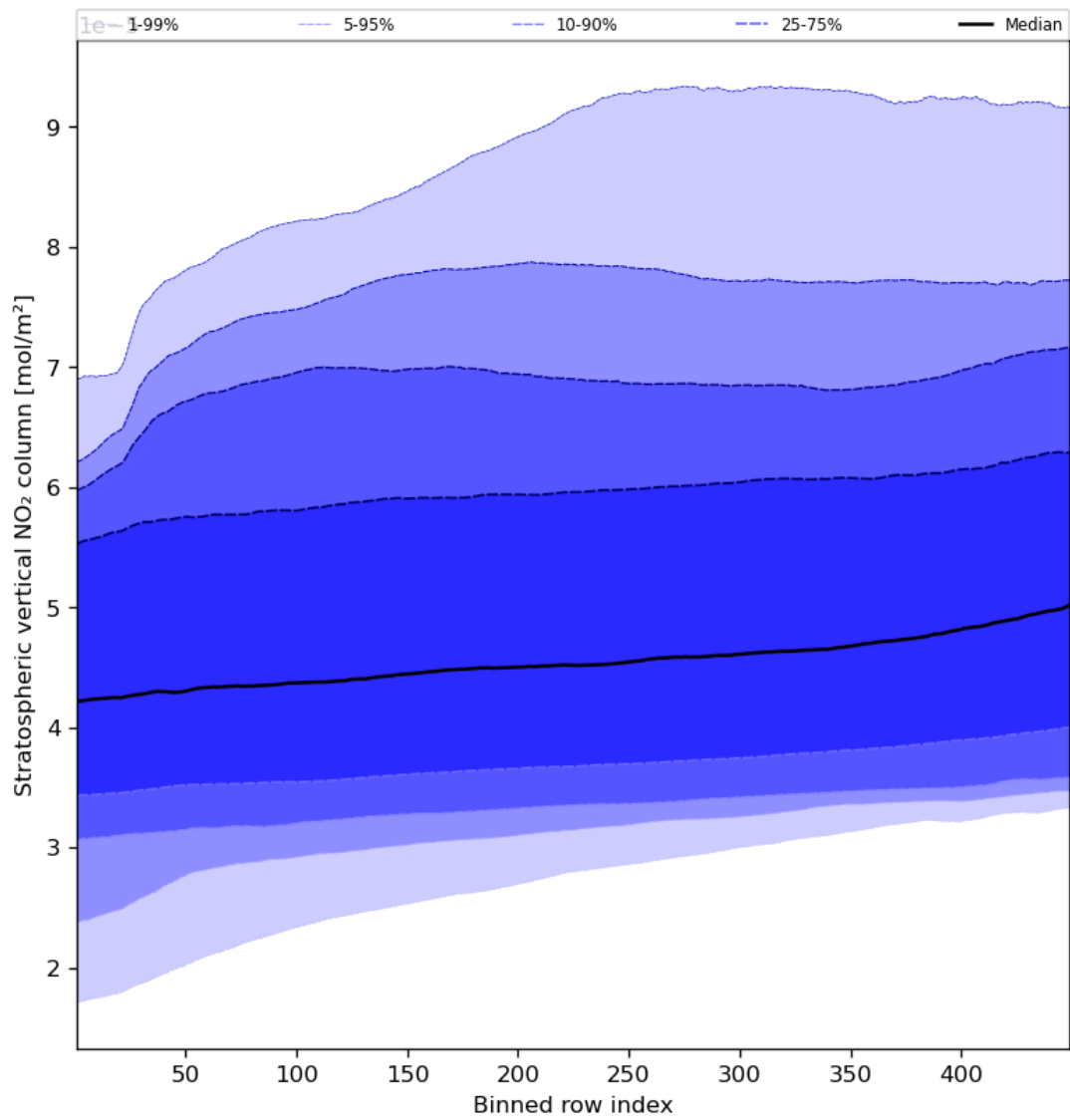
Figure 53: Along track statistics of “Stratospheric vertical NO 2 column” for 2024-05-02 to 2024-05-04
