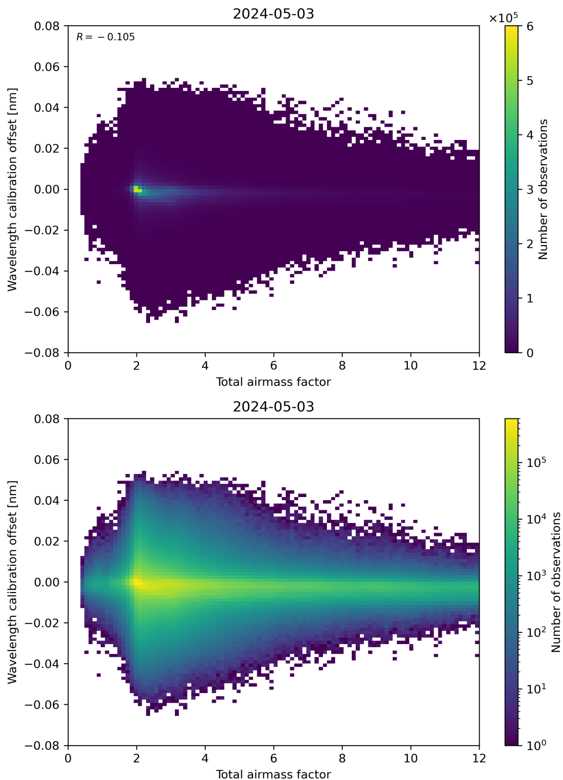
Figure 70: Scatter density plot of “Total airmass factor” against “Wavelength calibration offset” for 2024-05-02 to 2024-05-04.
