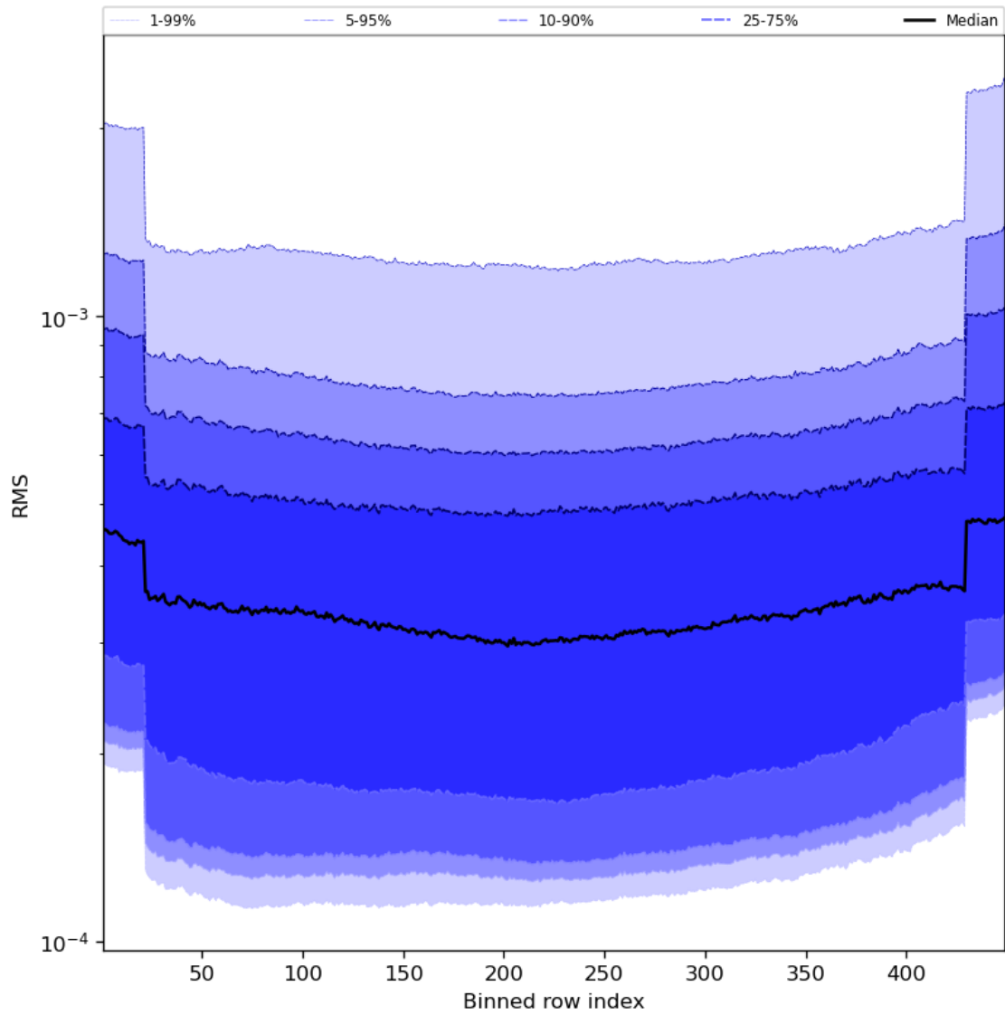
Figure 60: Along track statistics of “RMS” for 2024-05-02 to 2024-05-04
