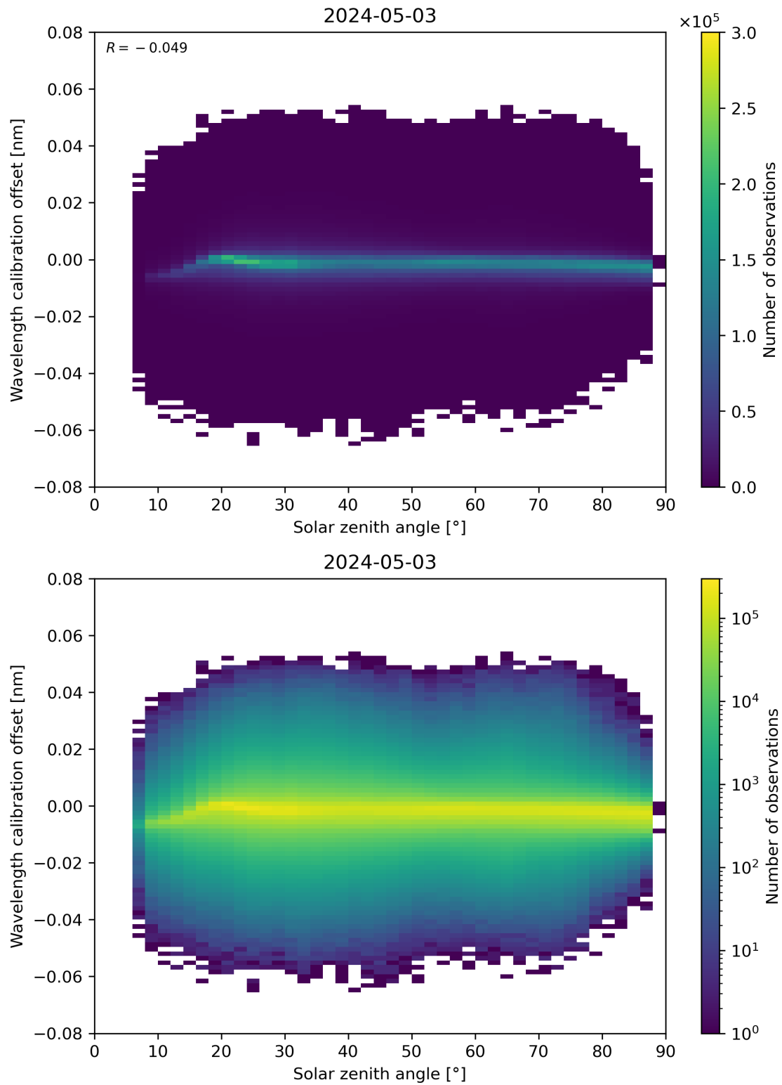
Figure 158: Scatter density plot of “Solar zenith angle” against “Wavelength calibration offset” for 2024-05-02 to 2024-05-04.
