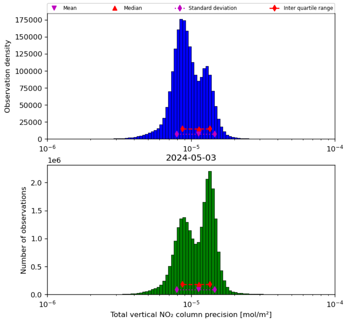
Figure 39: Histogram of "Total vertical NO 2 column precision" for 2024-05-02 to 2024-05-04
