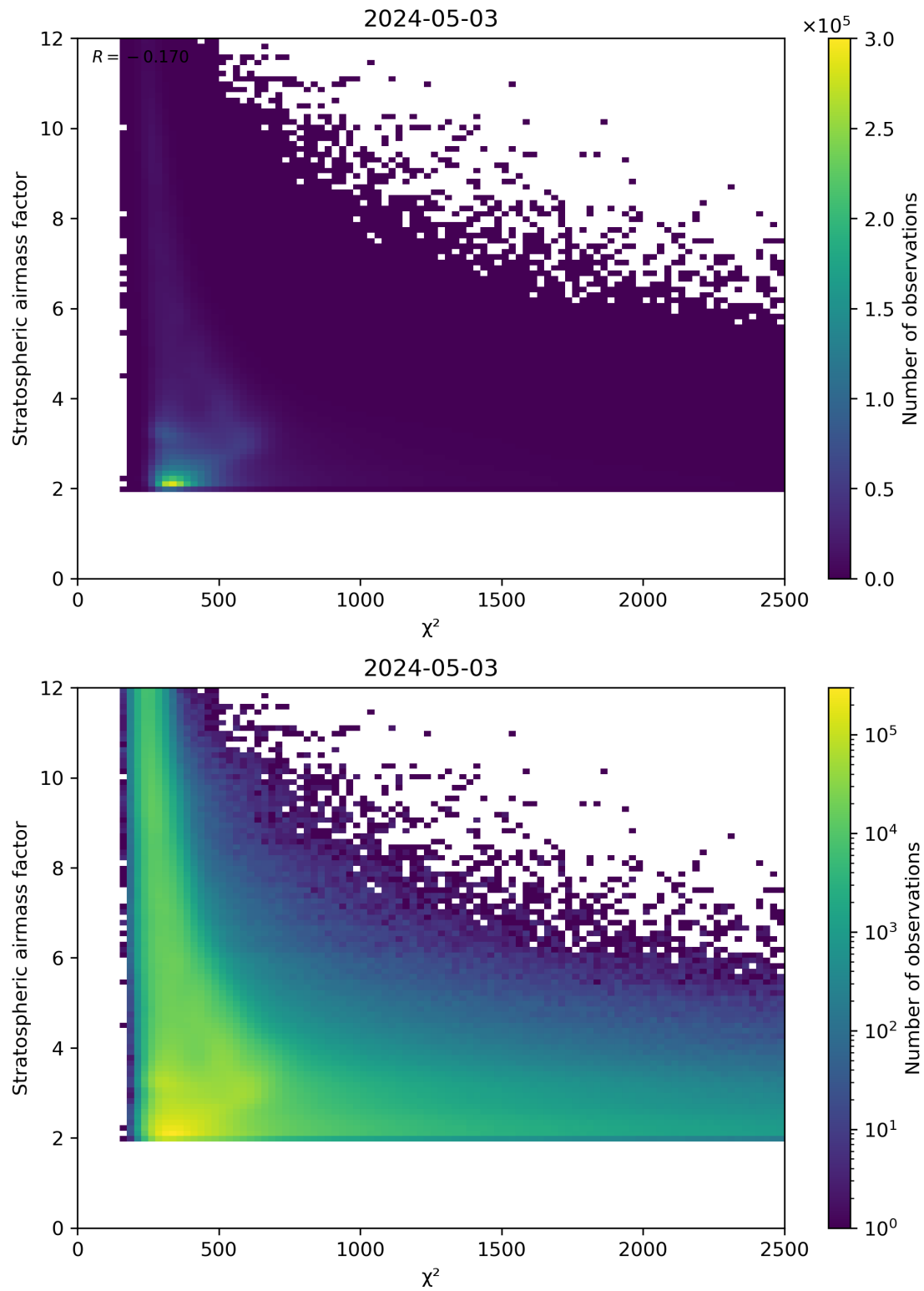
Figure 81: Scatter density plot of “ \chi^2 ” against “Stratospheric airmass factor” for 2024-05-02 to 2024-05-04.
