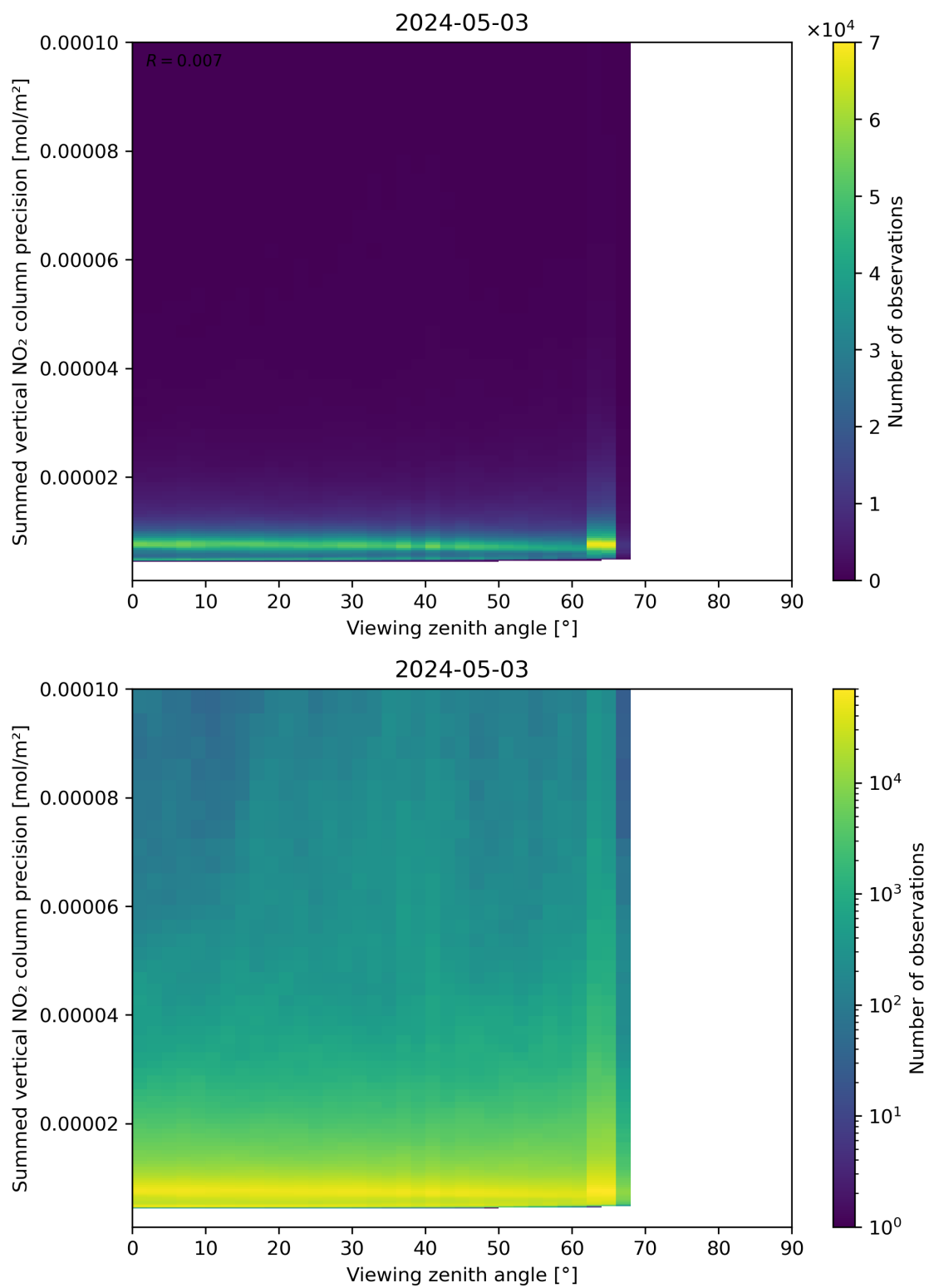
Figure 166: Scatter density plot of “Viewing zenith angle” against “Summed vertical NO 2 column precision” for 2024-05-02 to 2024-05-04.
