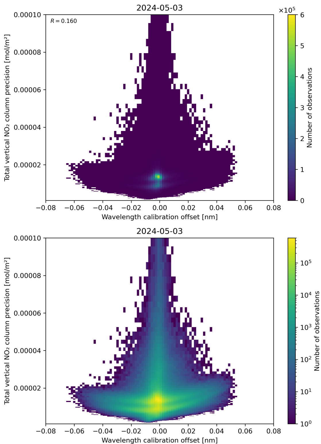
Figure 180: Scatter density plot of “Wavelength calibration offset” against “Total vertical NO 2 column precision” for 2024-05-02 to 2024-05-04.
