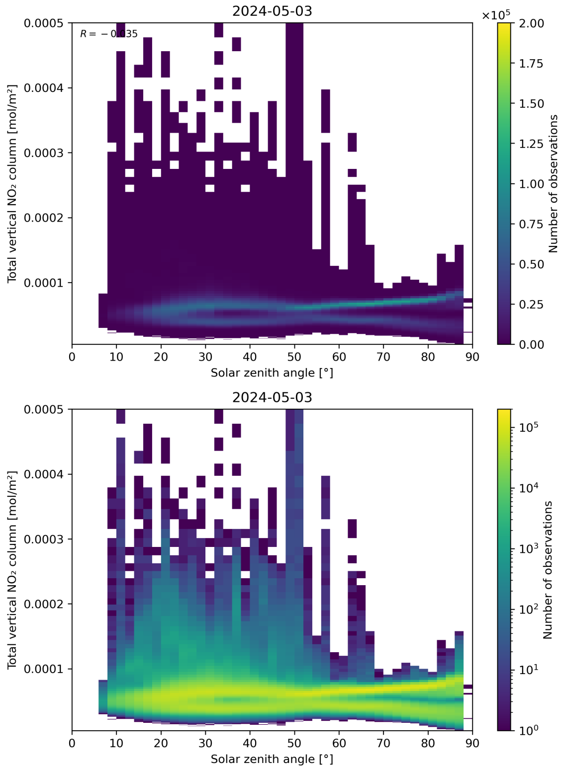
Figure 153: Scatter density plot of “Solar zenith angle” against “Total vertical NO 2 column” for 2024-05-02 to 2024-05-04.
