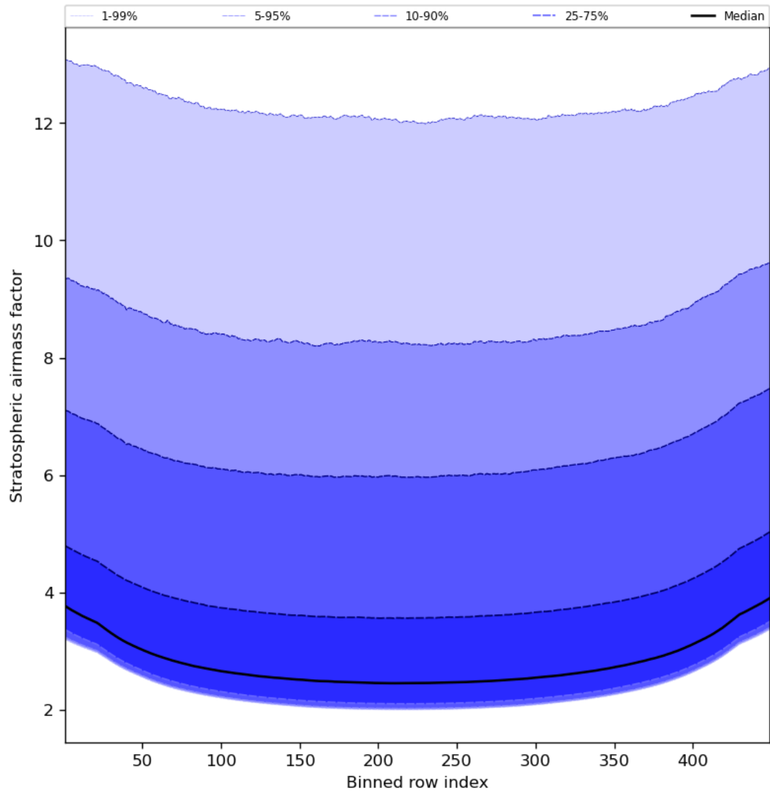
Figure 61: Along track statistics of “Stratospheric airmass factor” for 2024-05-02 to 2024-05-04
