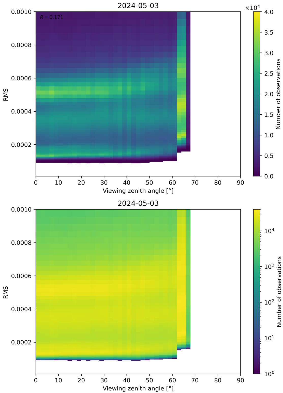
Figure 171: Scatter density plot of “Viewing zenith angle” against “RMS” for 2024-05-02 to 2024-05-04.
