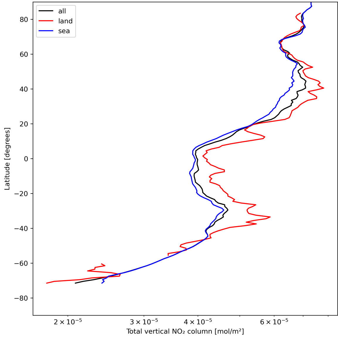
Figure 21: Zonal average of “Total vertical NO 2 column” for 2024-05-02 to 2024-05-04.
