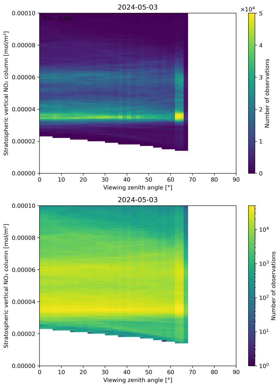
Figure 164: Scatter density plot of “Viewing zenith angle” against “Stratospheric vertical NO 2 column” for 2024-05-02 to 2024-05-04.
