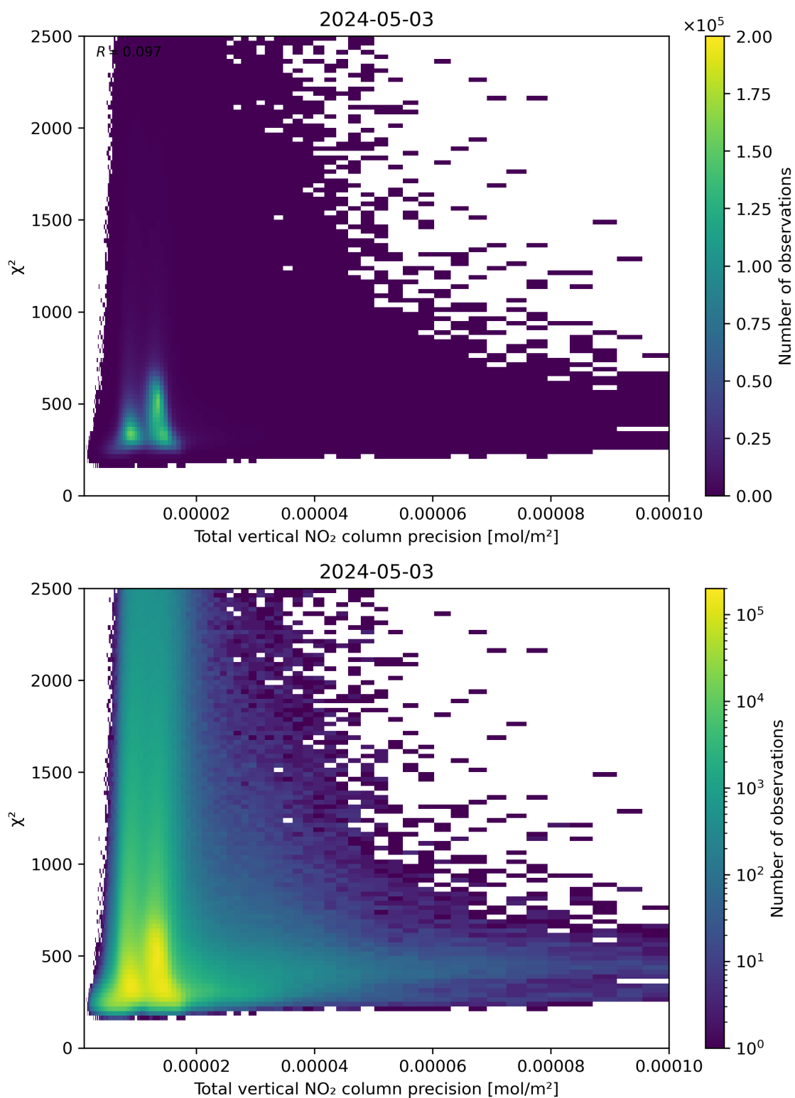
Figure 116: Scatter density plot of “Total vertical NO 2 column precision” against “ \chi^2 ” for 2024-05-02 to 2024-05-04.
