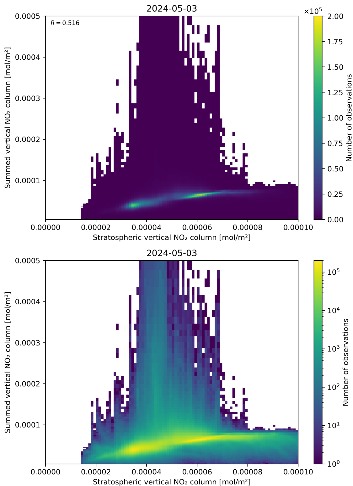
Figure 98: Scatter density plot of “Stratospheric vertical NO 2 column” against “Summed vertical NO 2 column” for 2024-05-02 to 2024-05-04.
