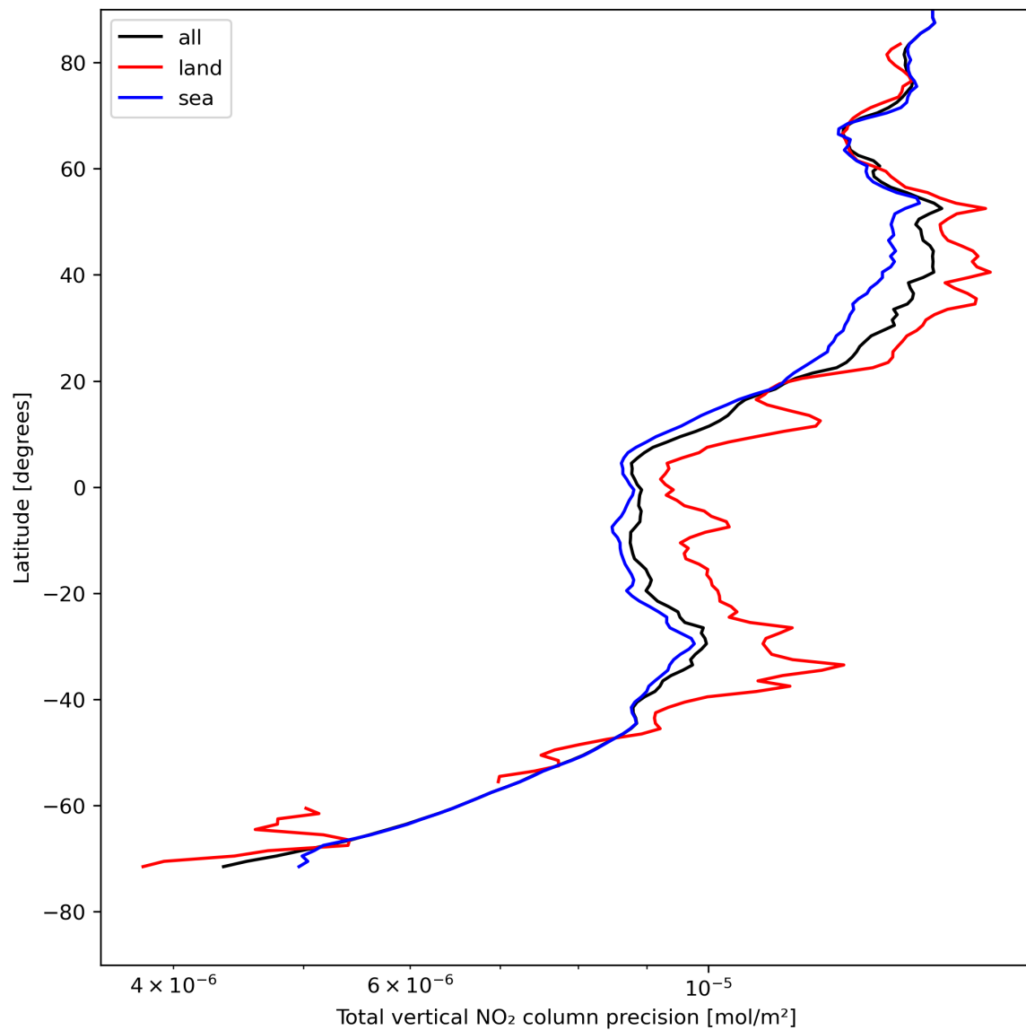
Figure 22: Zonal average of “Total vertical NO 2 column precision” for 2024-05-02 to 2024-05-04.
