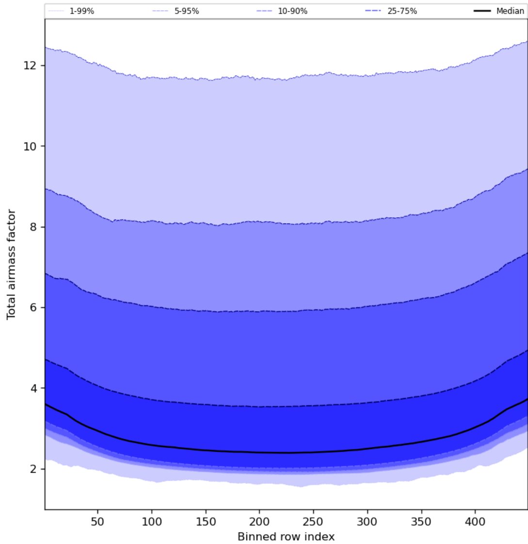
Figure 49: Along track statistics of “Total airmass factor” for 2024-05-02 to 2024-05-04
