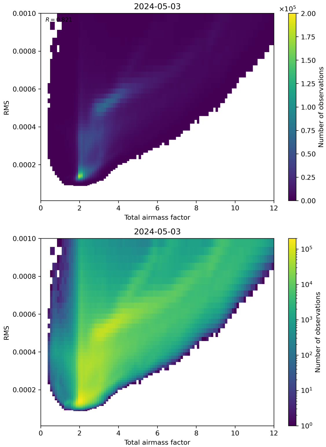
Figure 69: Scatter density plot of “Total airmass factor” against “RMS” for 2024-05-02 to 2024-05-04.
