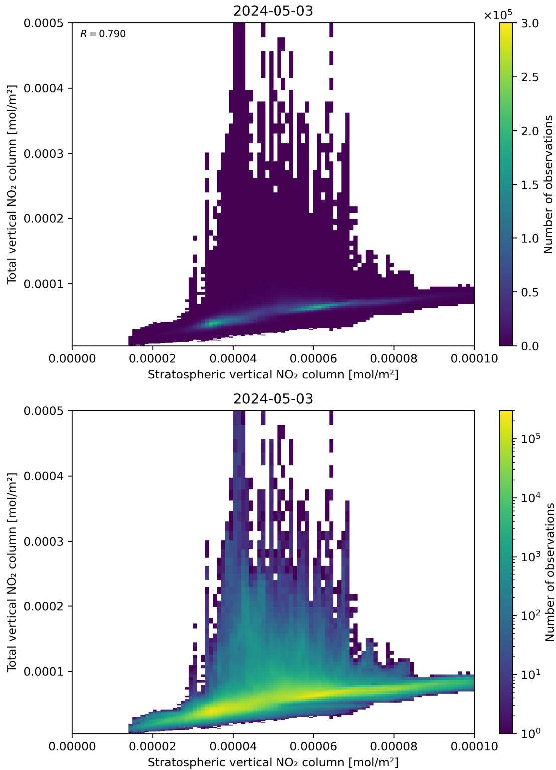
Figure 100: Scatter density plot of “Stratospheric vertical NO 2 column” against “Total vertical NO 2 column” for 2024-05-02 to 2024-05-04.
