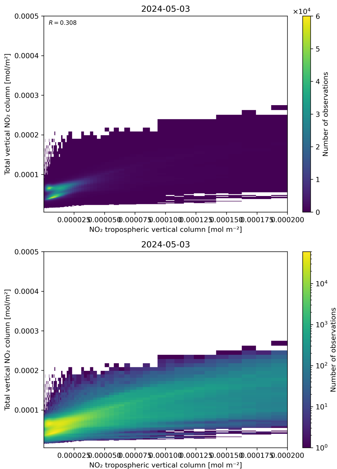
Figure 128: Scatter density plot of “NO 2 tropospheric vertical column” against “Total vertical NO 2 column” for 2024-05-02 to 2024-05-04.
