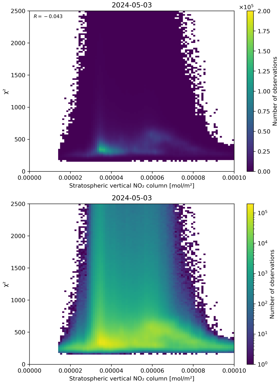
Figure 97: Scatter density plot of “Stratospheric vertical NO 2 column” against “ \chi^2 ” for 2024-05-02 to 2024-05-04.
