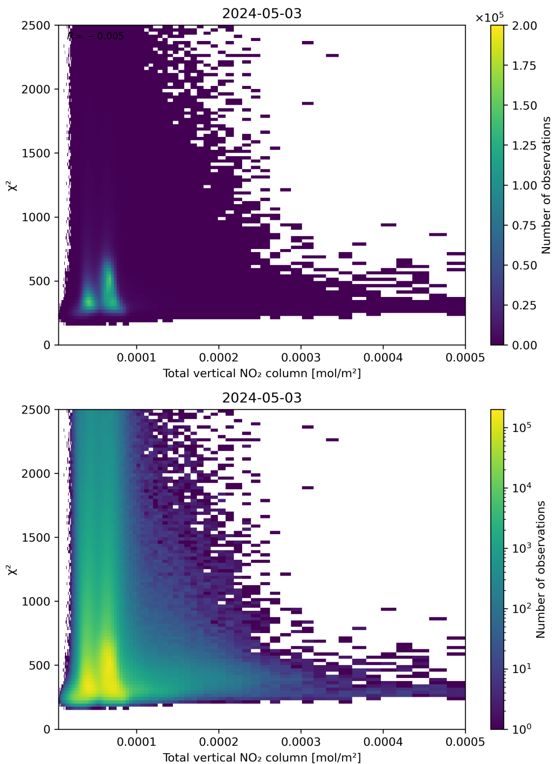
Figure 111: Scatter density plot of “Total vertical NO 2 column” against “ \chi^2 ” for 2024-05-02 to 2024-05-04.
