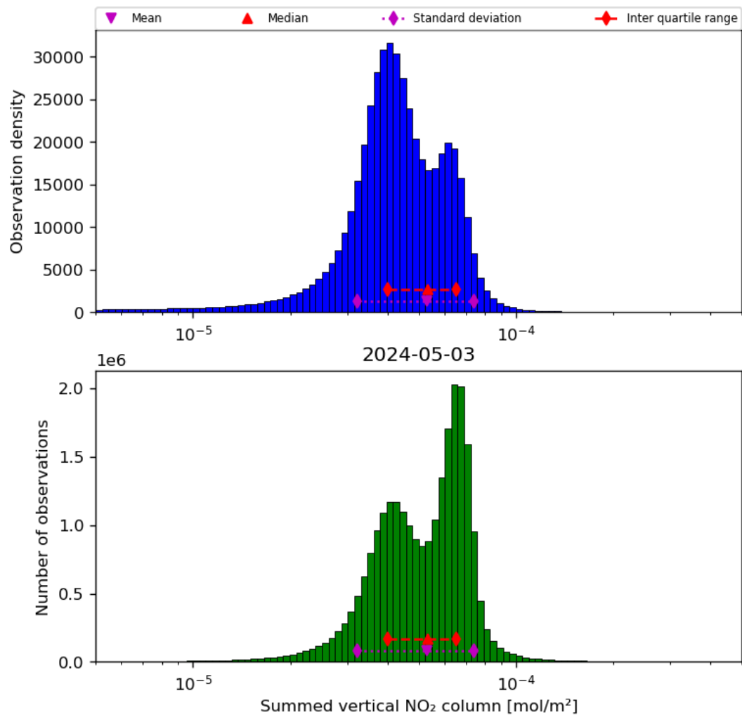
Figure 40: Histogram of “Summed vertical NO 2 column” for 2024-05-02 to 2024-05-04
