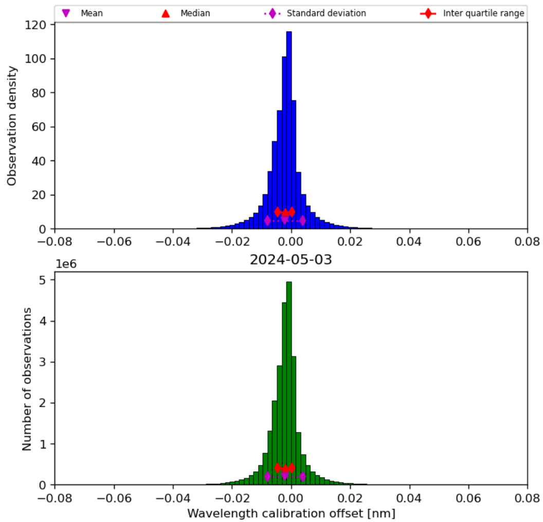
Figure 35: Histogram of “Wavelength calibration offset” for 2024-05-02 to 2024-05-04
