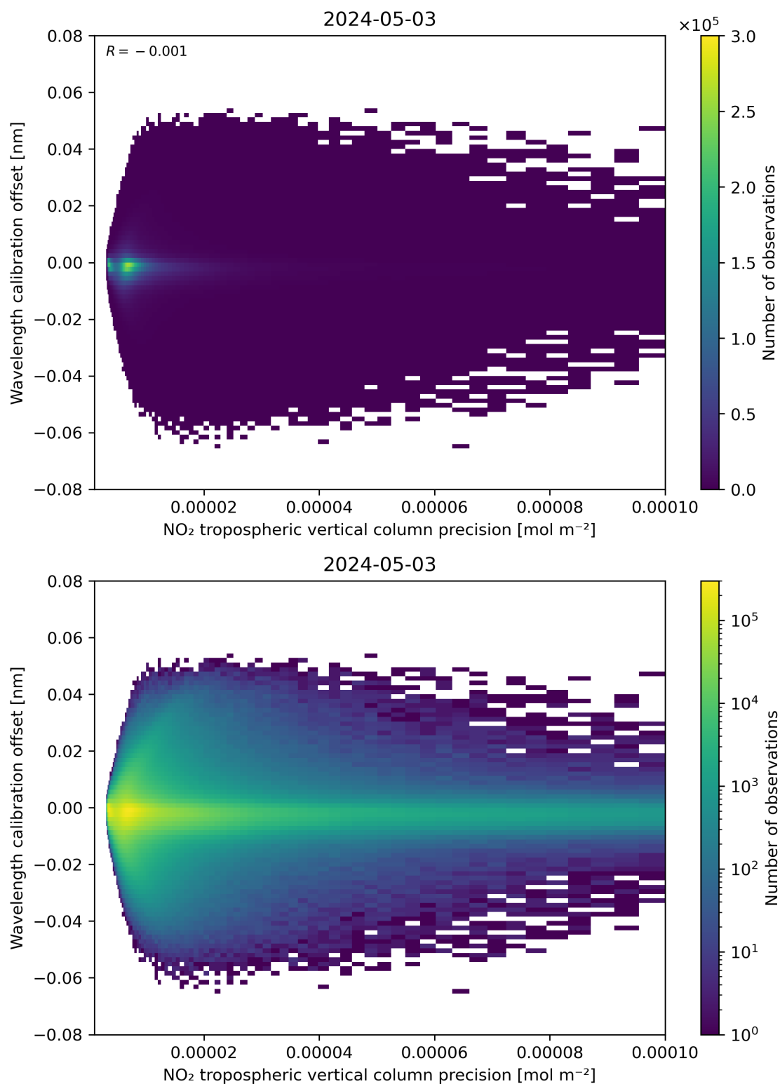
Figure 141: Scatter density plot of “NO 2 tropospheric vertical column precision” against “Wavelength calibration offset” for 2024-05-02 to 2024-05-04.
