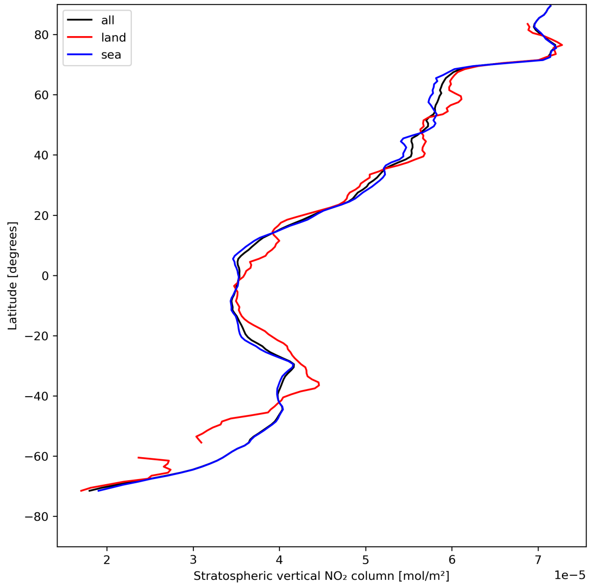
Figure 19: Zonal average of “Stratospheric vertical NO 2 column” for 2024-05-02 to 2024-05-04.
