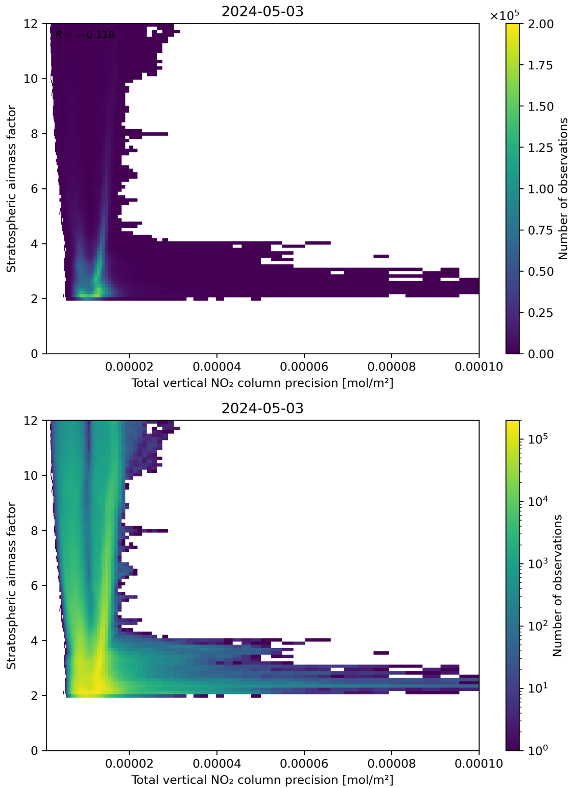
Figure 115: Scatter density plot of “Total vertical NO 2 column precision” against “Stratospheric air mass factor” for 2024-05-02 to 2024-05-04.
