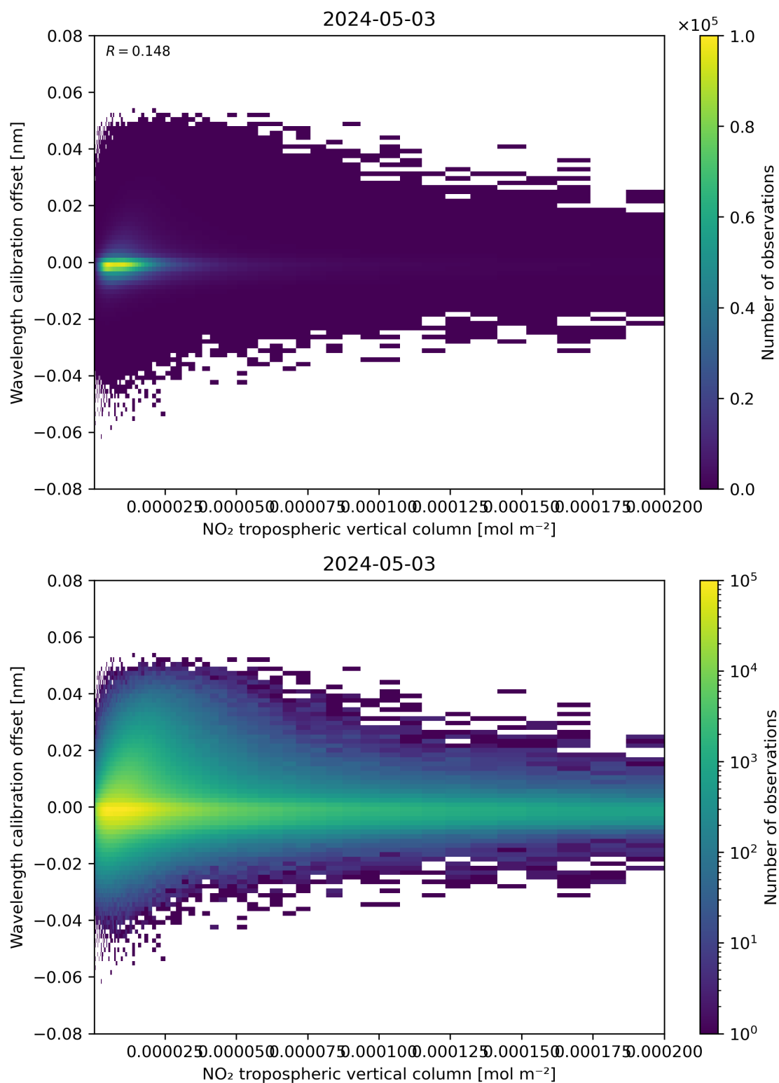
Figure 143: Scatter density plot of “NO 2 tropospheric vertical column” against “Wavelength calibration offset” for 2024-05-02 to 2024-05-04.
