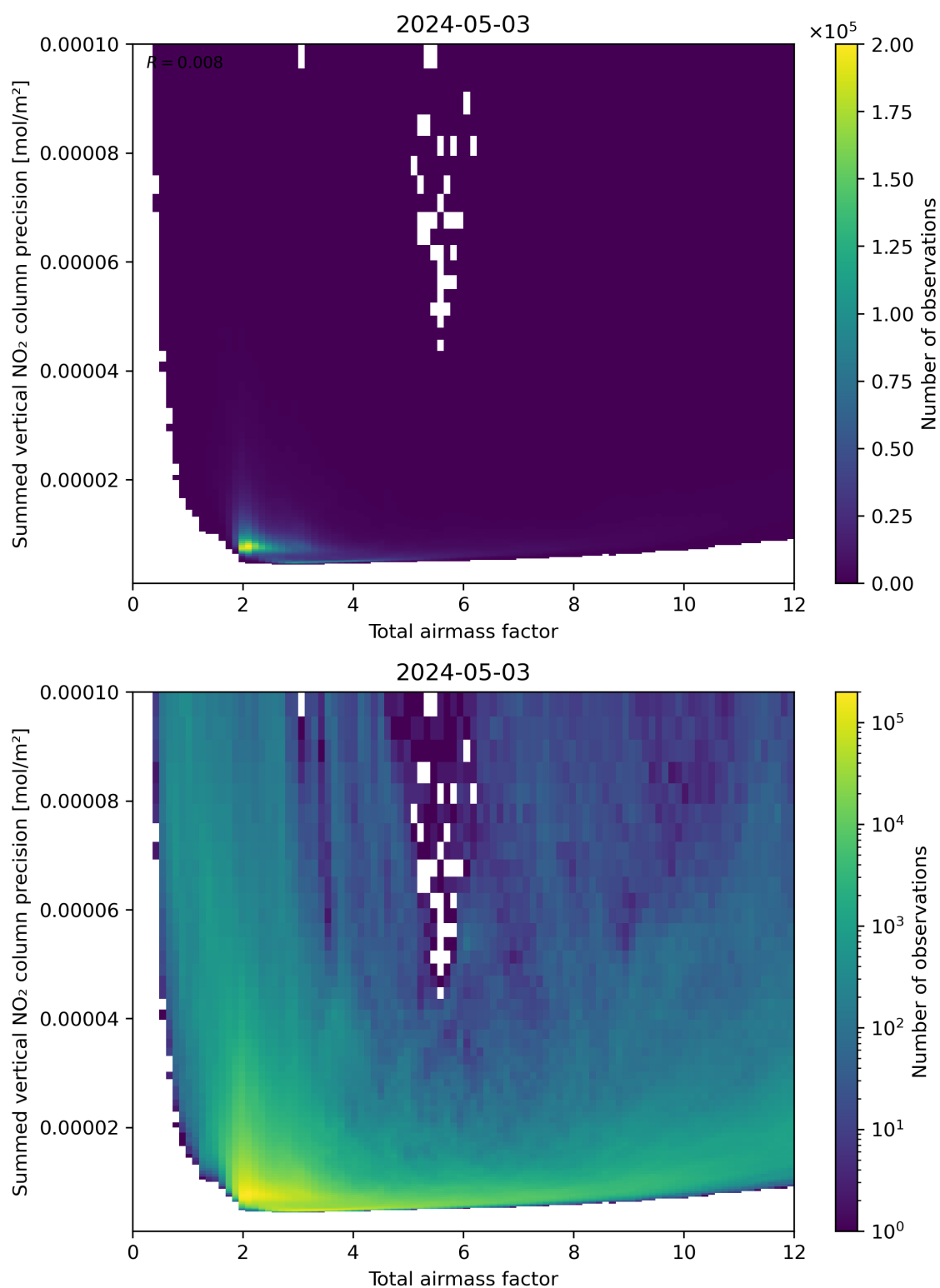
Figure 66: Scatter density plot of “Total airmass factor” against “Summed vertical NO 2 column precision” for 2024-05-02 to 2024-05-04.
