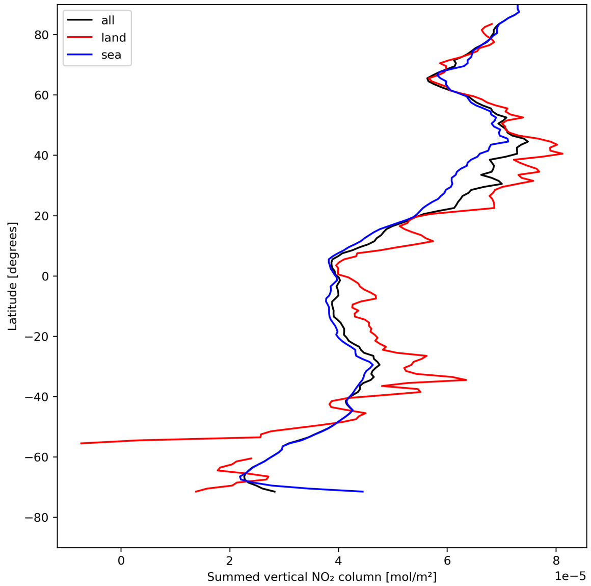
Figure 23: Zonal average of “Summed vertical NO 2 column” for 2024-05-02 to 2024-05-04.
