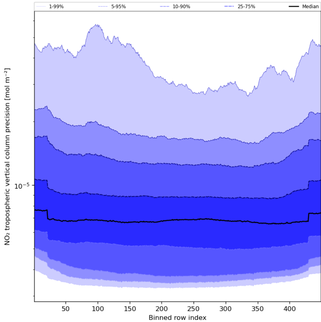
Figure 47: Along track statistics of “NO 2 tropospheric vertical column precision” for 2024-05-02 to 2024-05-04
