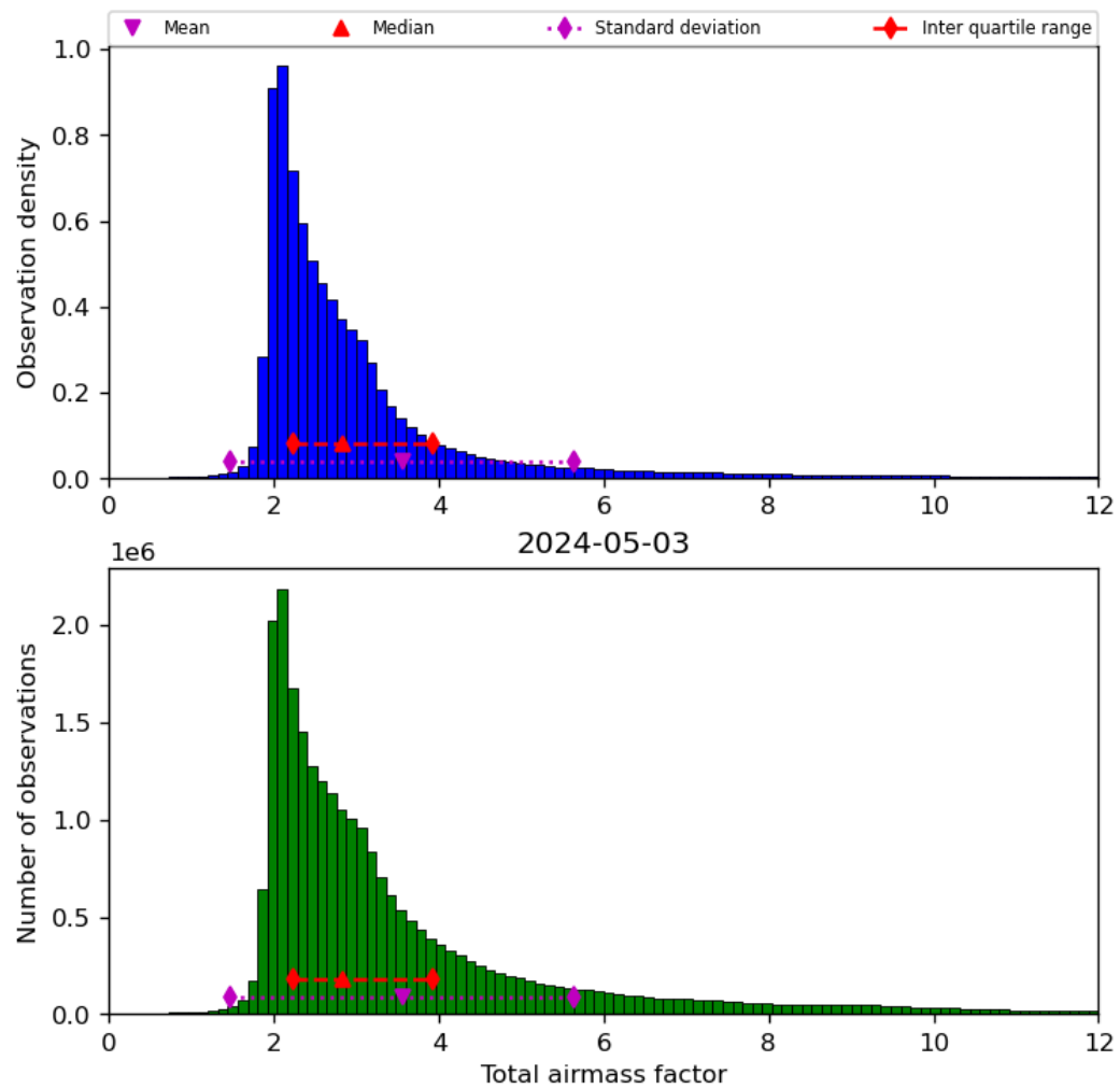
Figure 32: Histogram of “Total airmass factor” for 2024-05-02 to 2024-05-04
