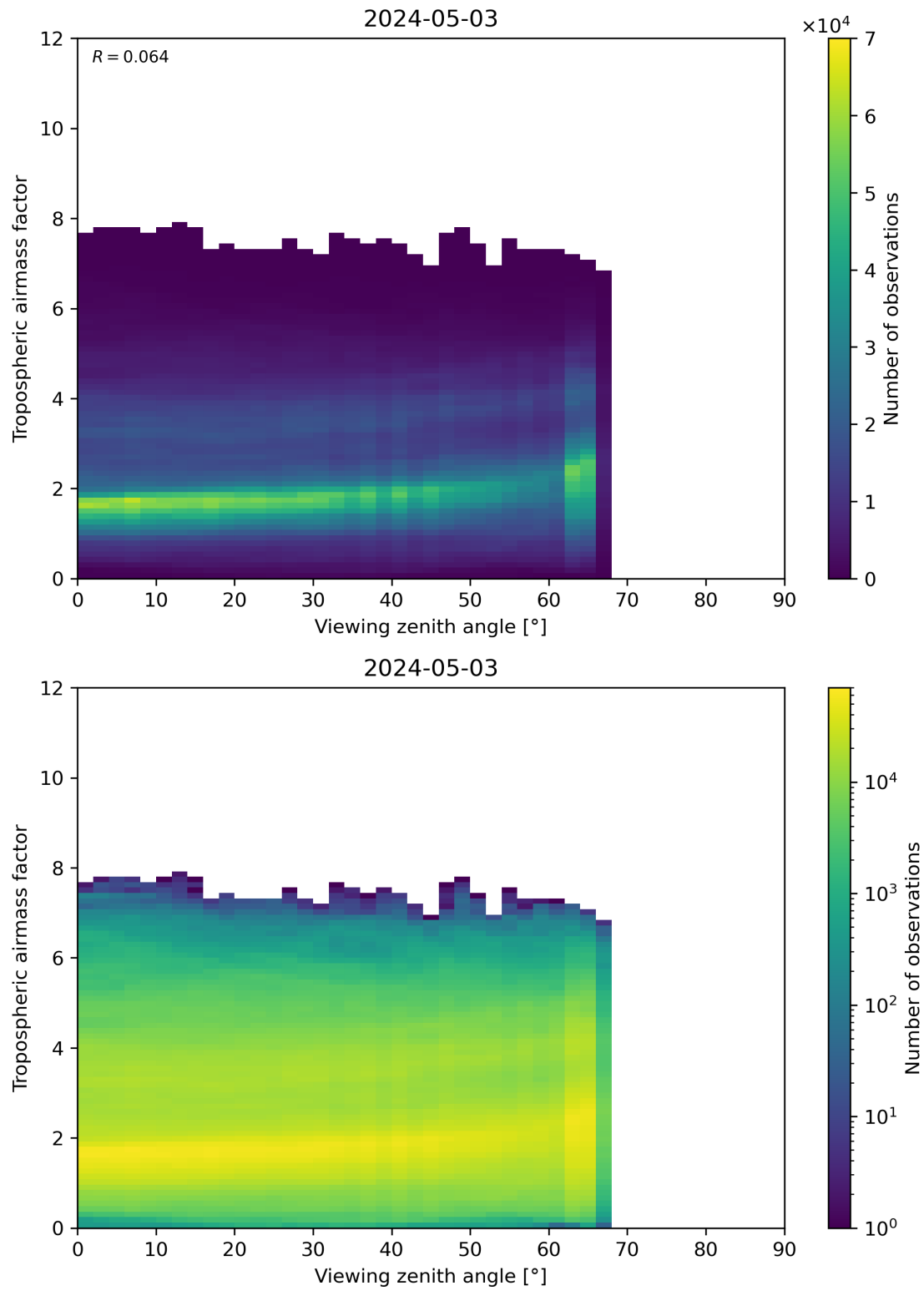
Figure 161: Scatter density plot of “Viewing zenith angle” against “Tropospheric airmass factor” for 2024-05-02 to 2024-05-04.
