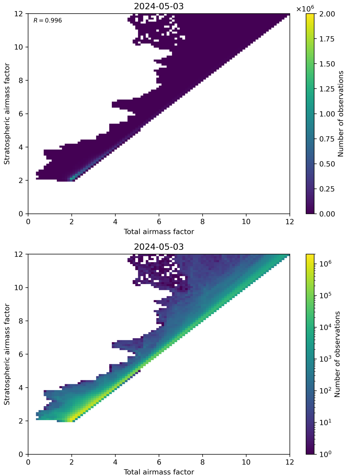
Figure 62: Scatter density plot of “Total airmass factor” against “Stratospheric airmass factor” for 2024-05-02 to 2024-05-04.
