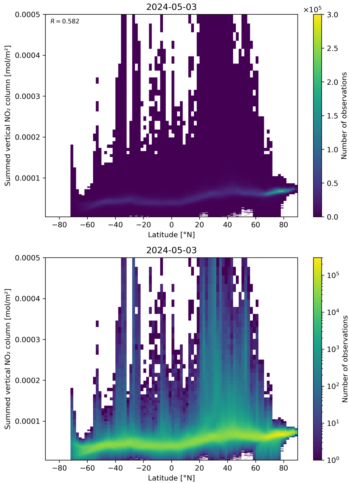
Figure 88: Scatter density plot of “Latitude” against “Summed vertical NO 2 column” for 2024-05-02 to 2024-05-04.
