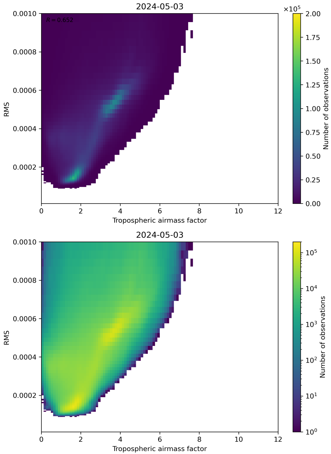
Figure 79: Scatter density plot of “Tropospheric airmass factor” against “RMS” for 2024-05-02 to 2024-05-04.
