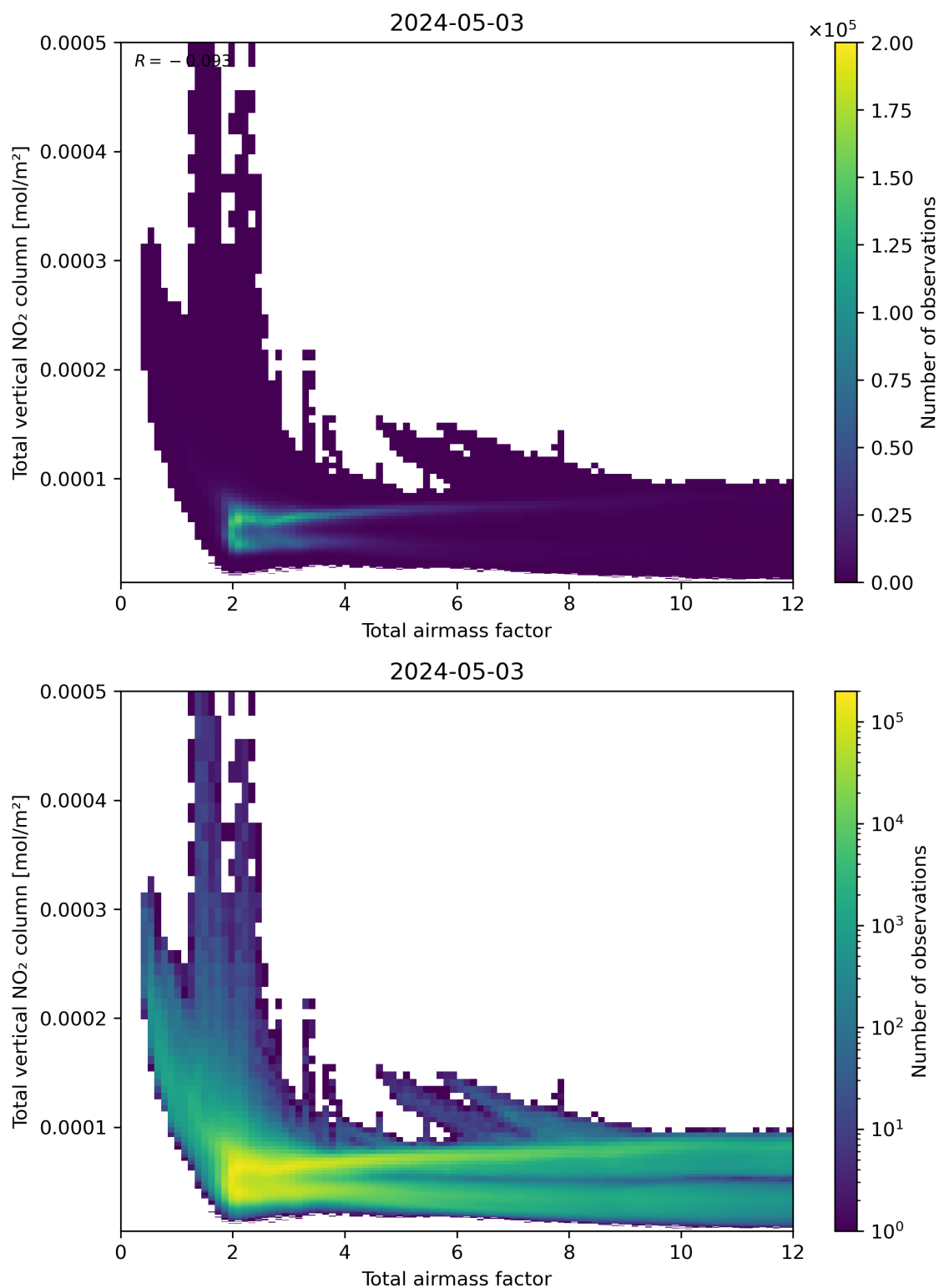
Figure 67: Scatter density plot of “Total airmass factor” against “Total vertical NO 2 column” for 2024-05-02 to 2024-05-04.
