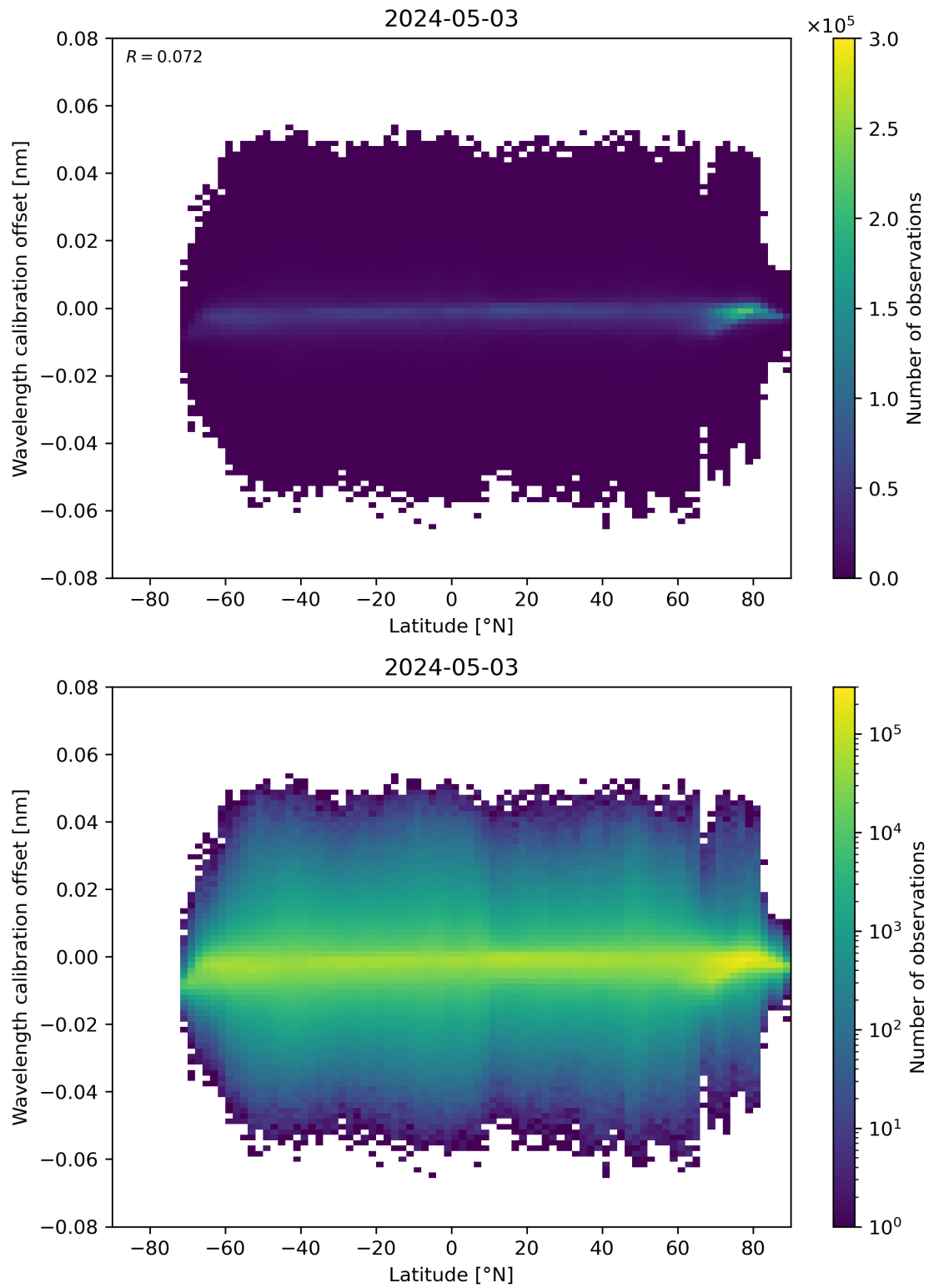
Figure 95: Scatter density plot of “Latitude” against “Wavelength calibration offset” for 2024-05-02 to 2024-05-04.
