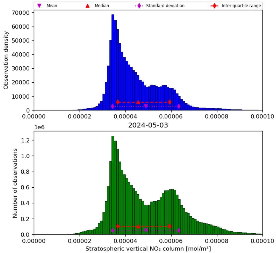
Figure 36: Histogram of “Stratospheric vertical NO 2 column” for 2024-05-02 to 2024-05-04
