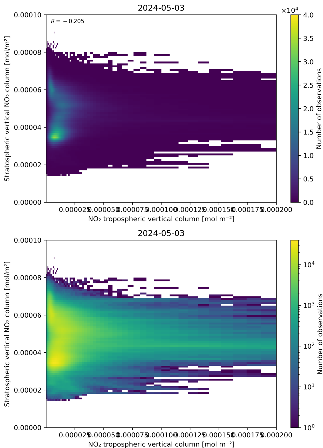
Figure 125: Scatter density plot of “NO 2 tropospheric vertical column” against “Stratospheric vertical NO 2 column” for 2024-05-02 to 2024-05-04.
