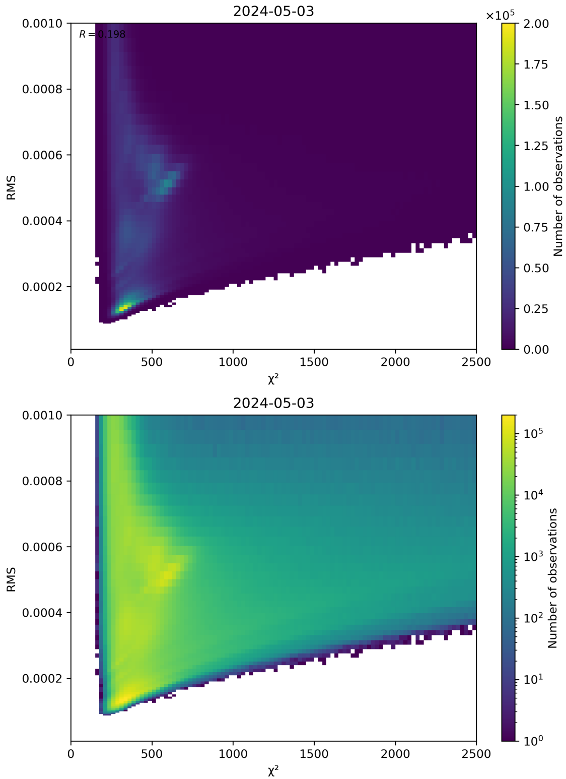
Figure 82: Scatter density plot of “ \chi^2 ” against “RMS” for 2024-05-02 to 2024-05-04.
