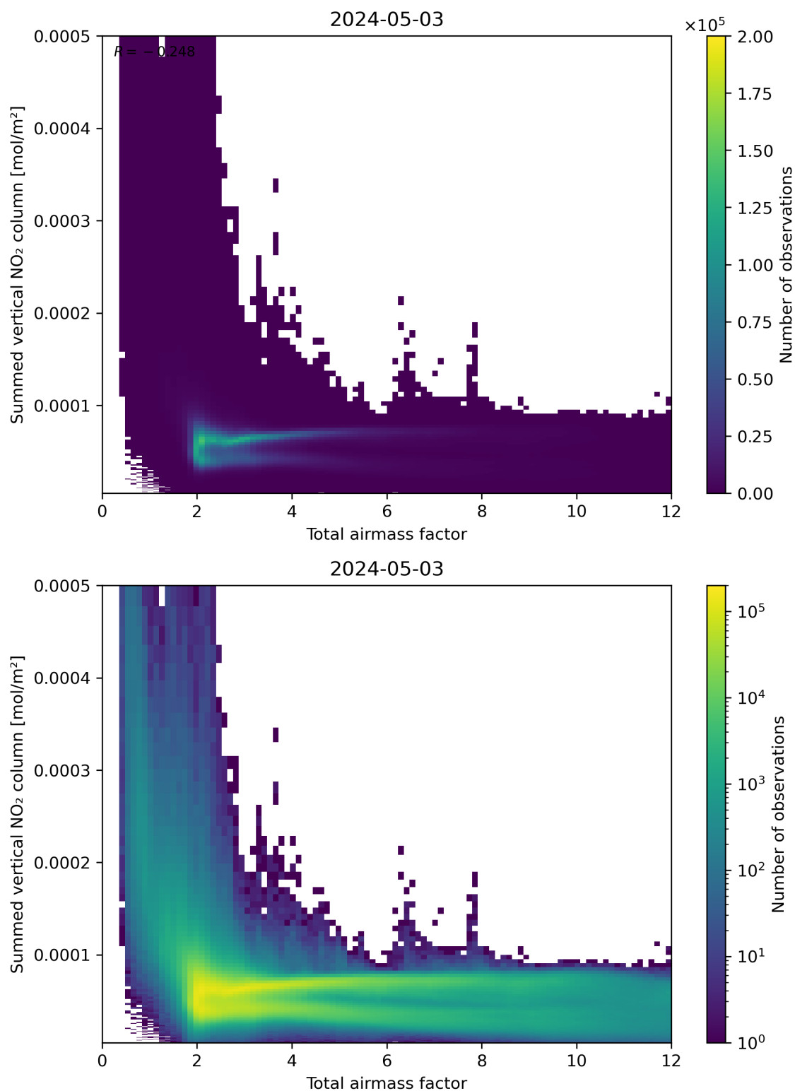
Figure 65: Scatter density plot of “Total airmass factor” against “Summed vertical NO 2 column” for 2024-05-02 to 2024-05-04.
