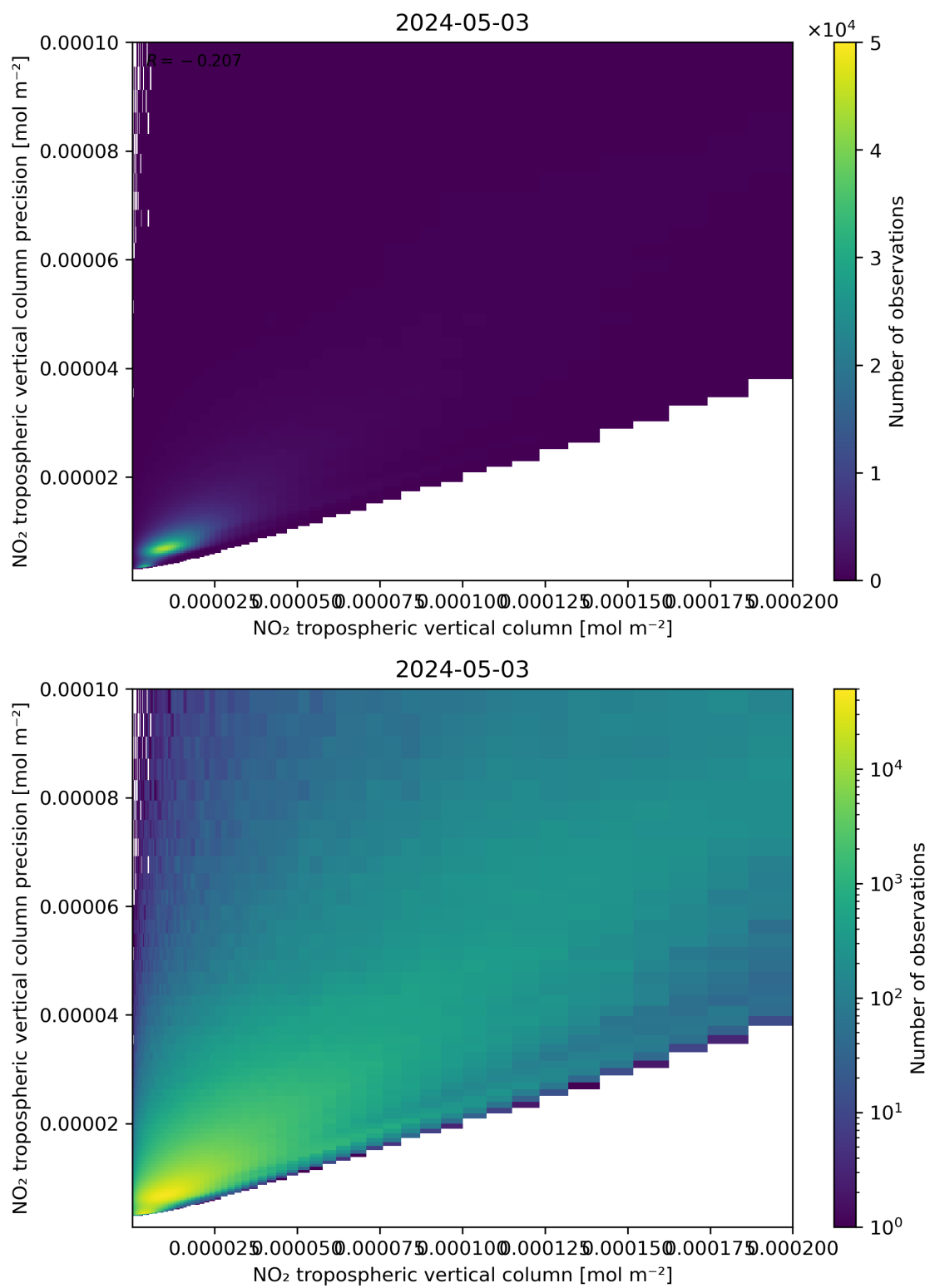
Figure 130: Scatter density plot of “NO 2 tropospheric vertical column” against “NO 2 tropospheric vertical column precision” for 2024-05-02 to 2024-05-04.
