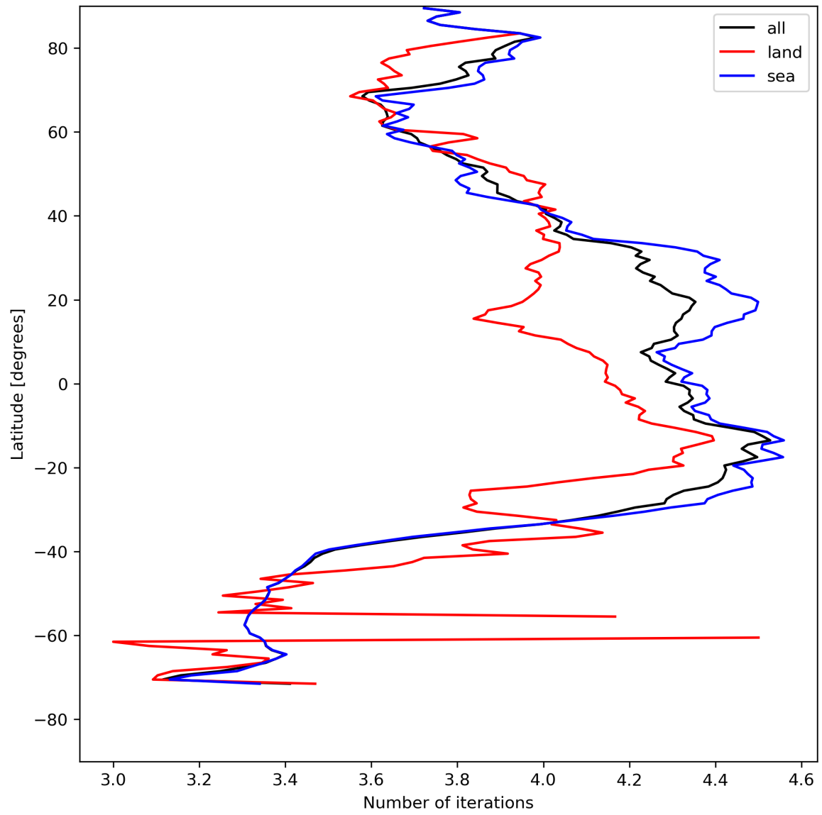
Figure 17: Zonal average of “Number of iterations” for 2024-05-02 to 2024-05-04.
