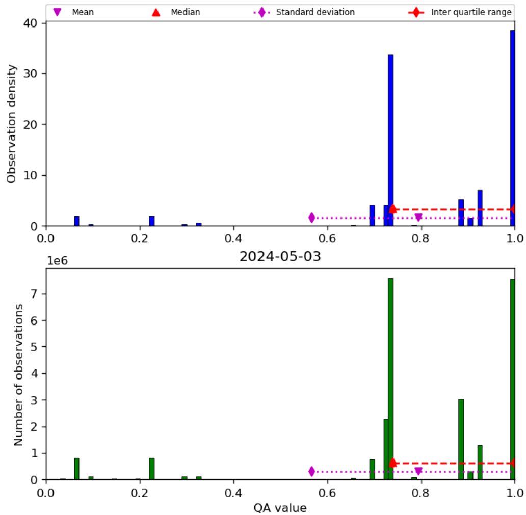
Figure 28: Histogram of “QA value” for 2024-05-02 to 2024-05-04
