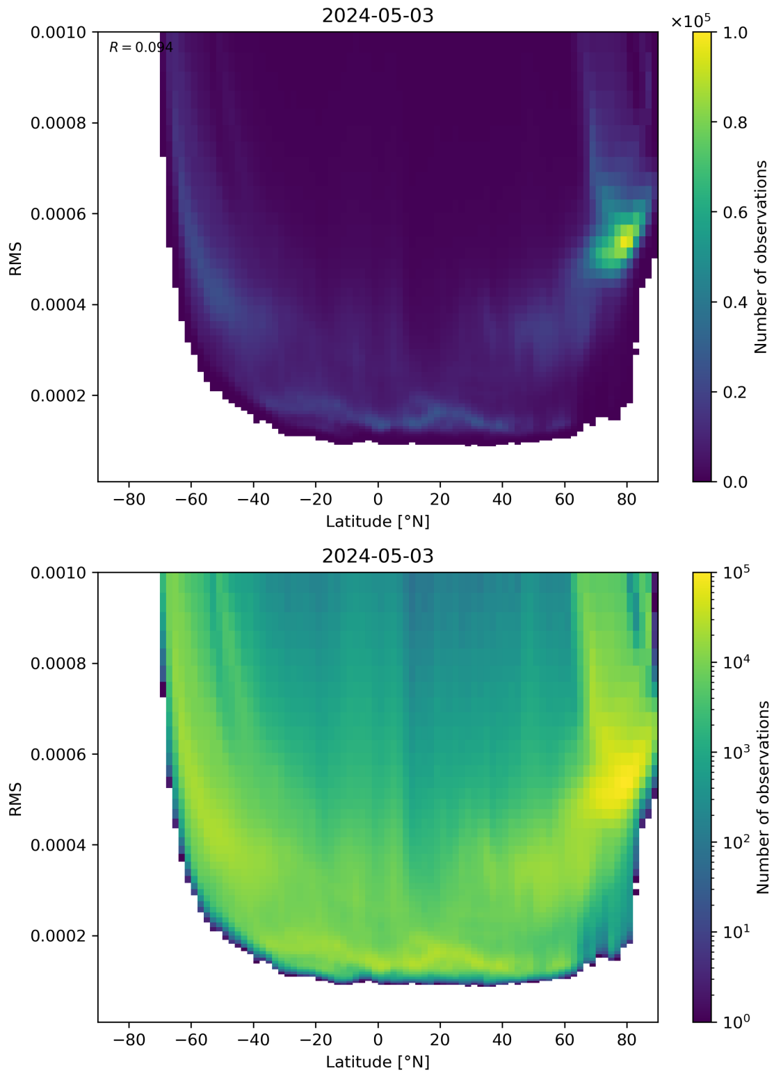
Figure 94: Scatter density plot of “Latitude” against “RMS” for 2024-05-02 to 2024-05-04.
