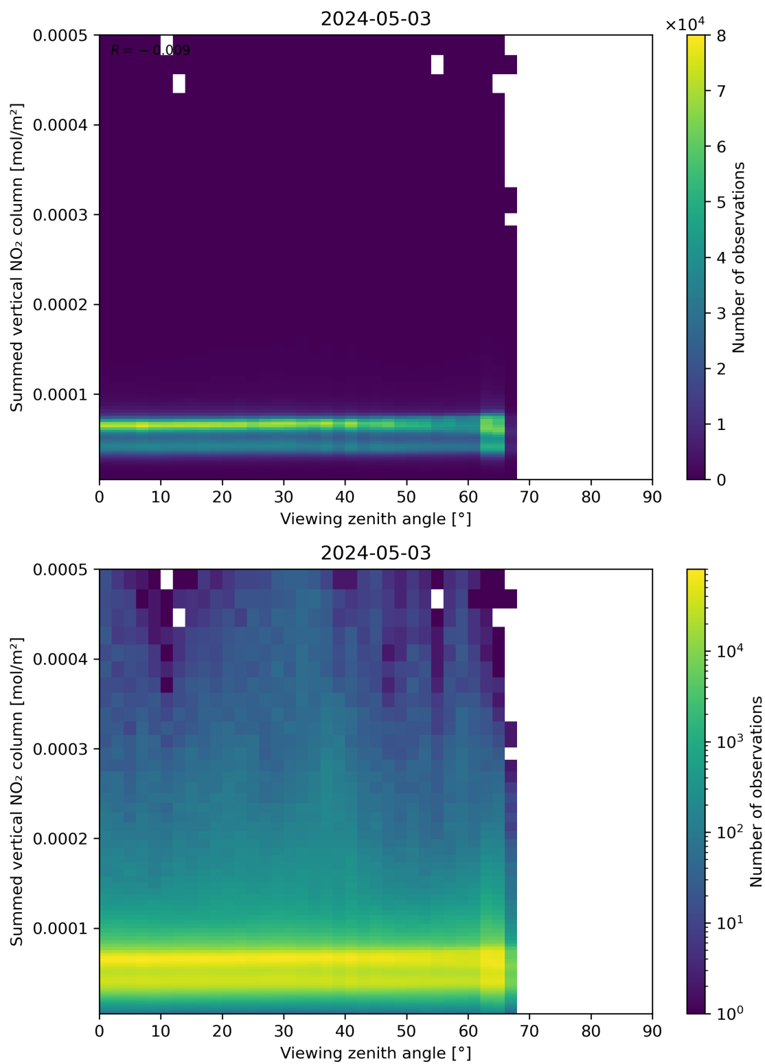
Figure 165: Scatter density plot of “Viewing zenith angle” against “Summed vertical NO 2 column” for 2024-05-02 to 2024-05-04.
