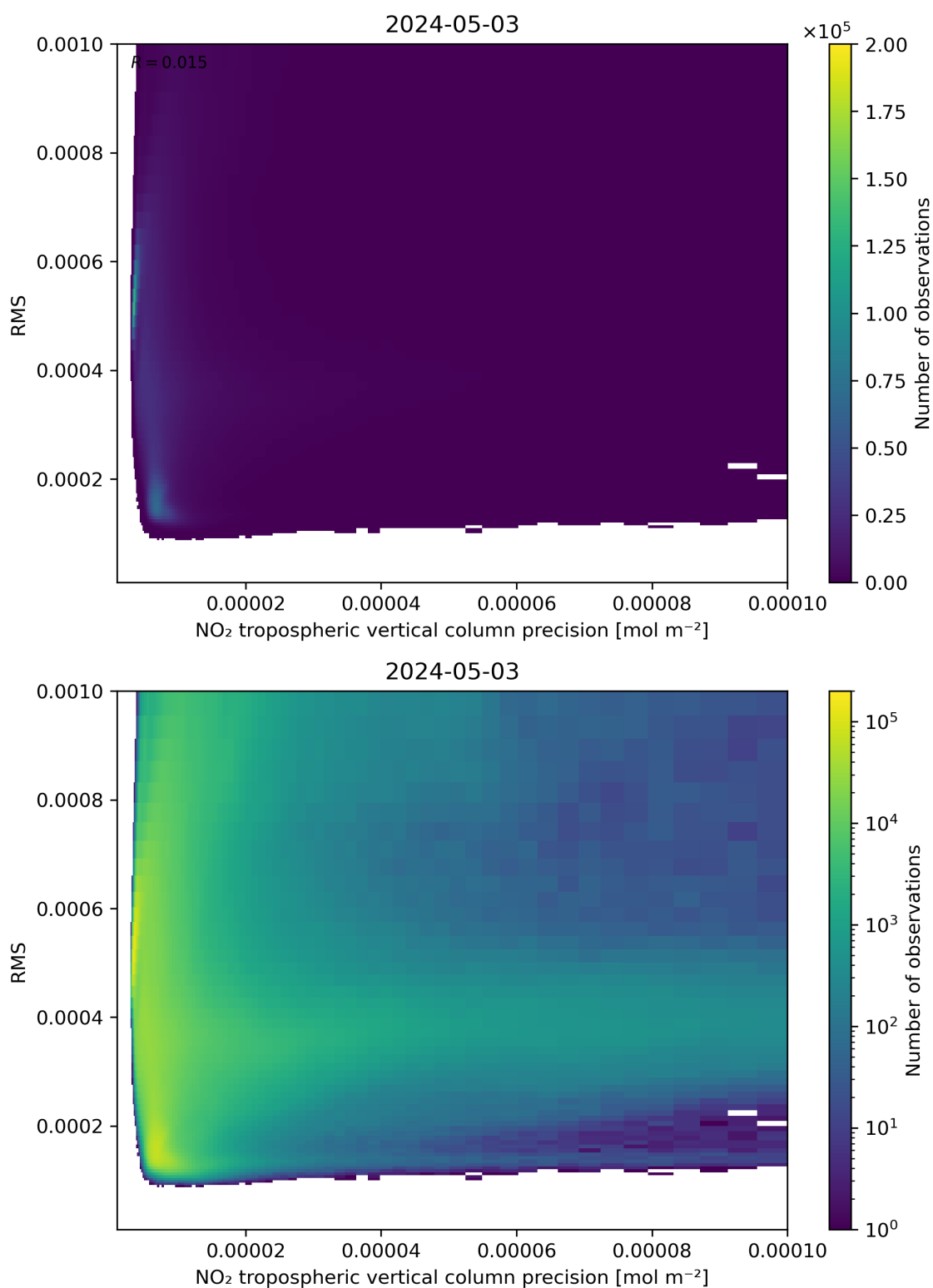
Figure 140: Scatter density plot of “NO 2 tropospheric vertical column precision” against “RMS” for 2024-05-02 to 2024-05-04.
