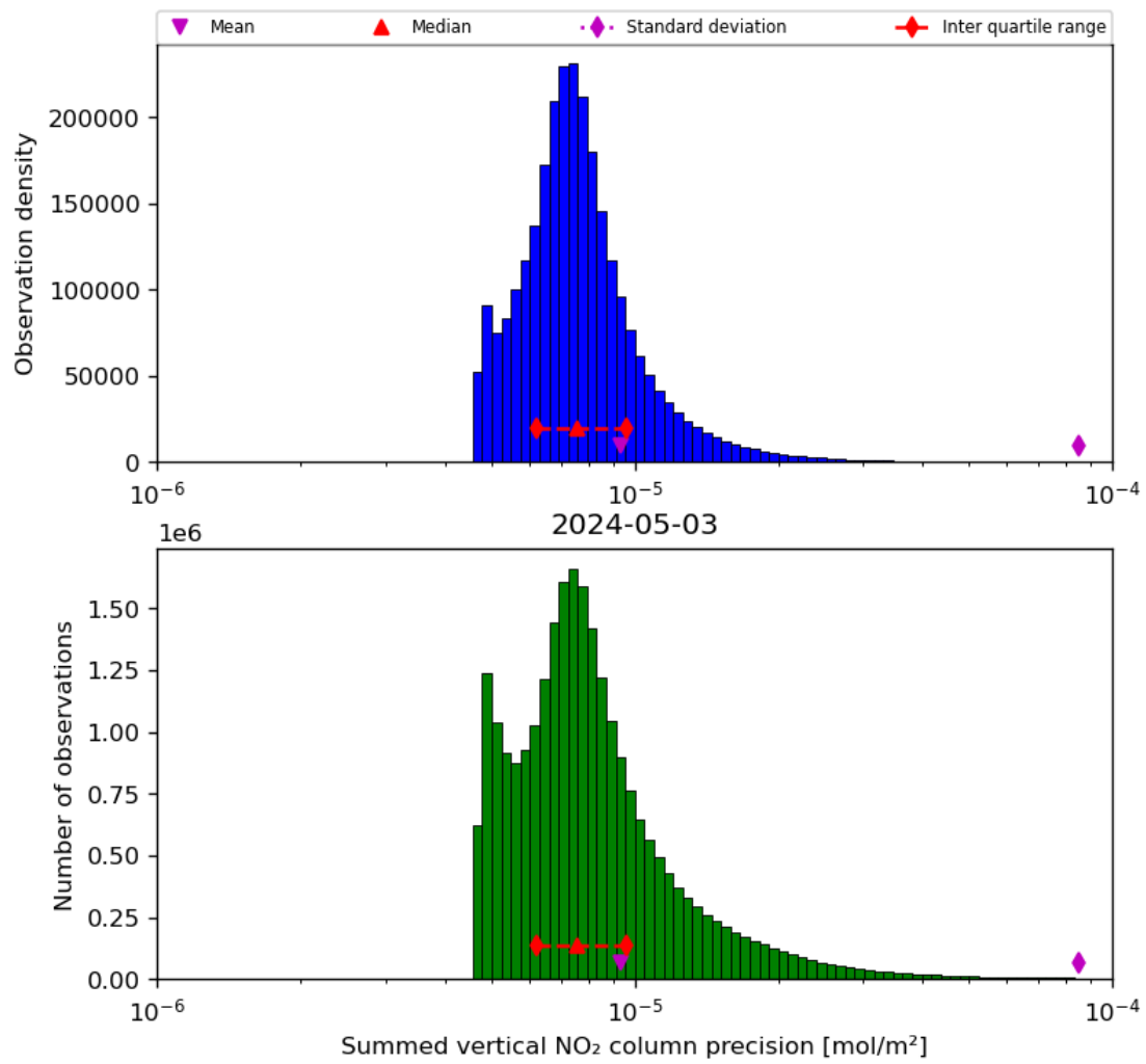
Figure 41: Histogram of "Summed vertical NO 2 column precision" for 2024-05-02 to 2024-05-04
