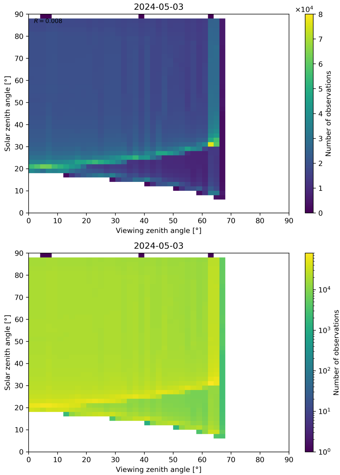
Figure 172: Scatter density plot of “Viewing zenith angle” against “Solar zenith angle” for 2024-05-02 to 2024-05-04.
