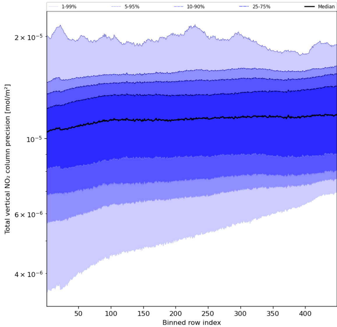
Figure 56: Along track statistics of “Total vertical NO 2 column precision” for 2024-05-02 to 2024-05-04
