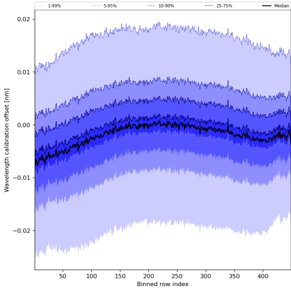
Figure 52: Along track statistics of “Wavelength calibration offset” for 2024-05-02 to 2024-05-04
