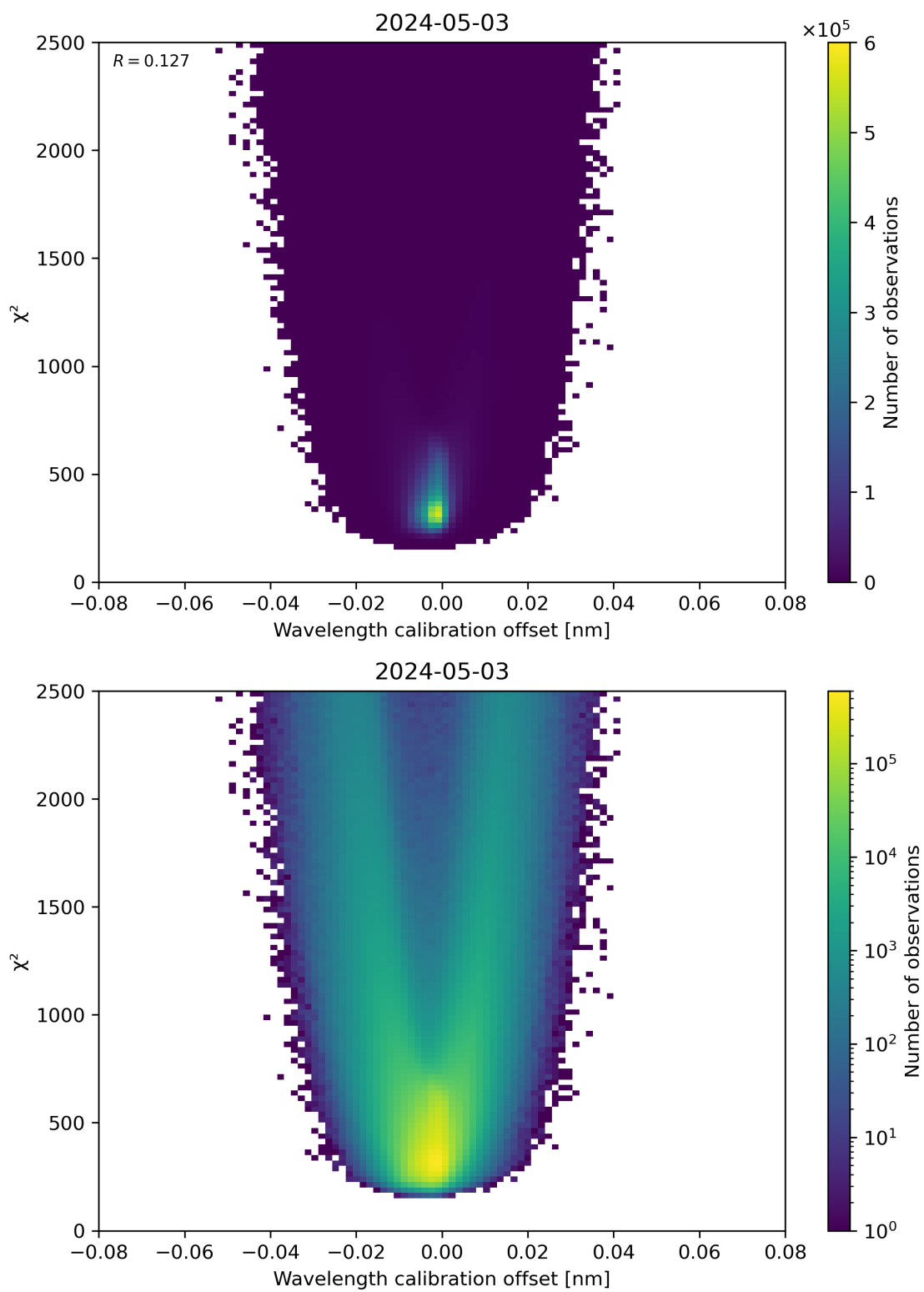
Figure 175: Scatter density plot of “Wavelength calibration offset” against “ \chi^2 ” for 2024-05-02 to 2024-05-04.
