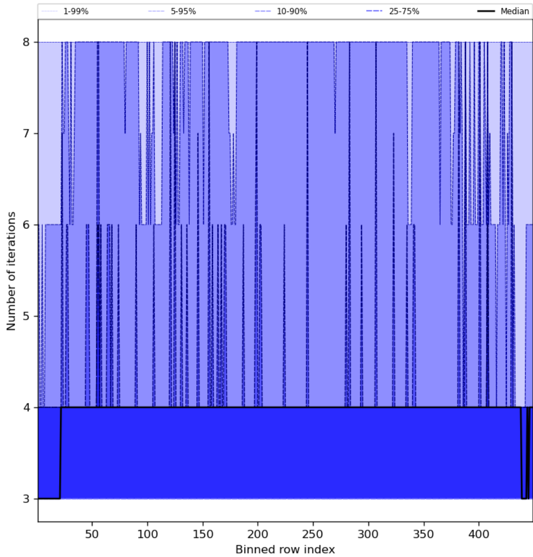
Figure 51: Along track statistics of “Number of iterations” for 2024-05-02 to 2024-05-04
