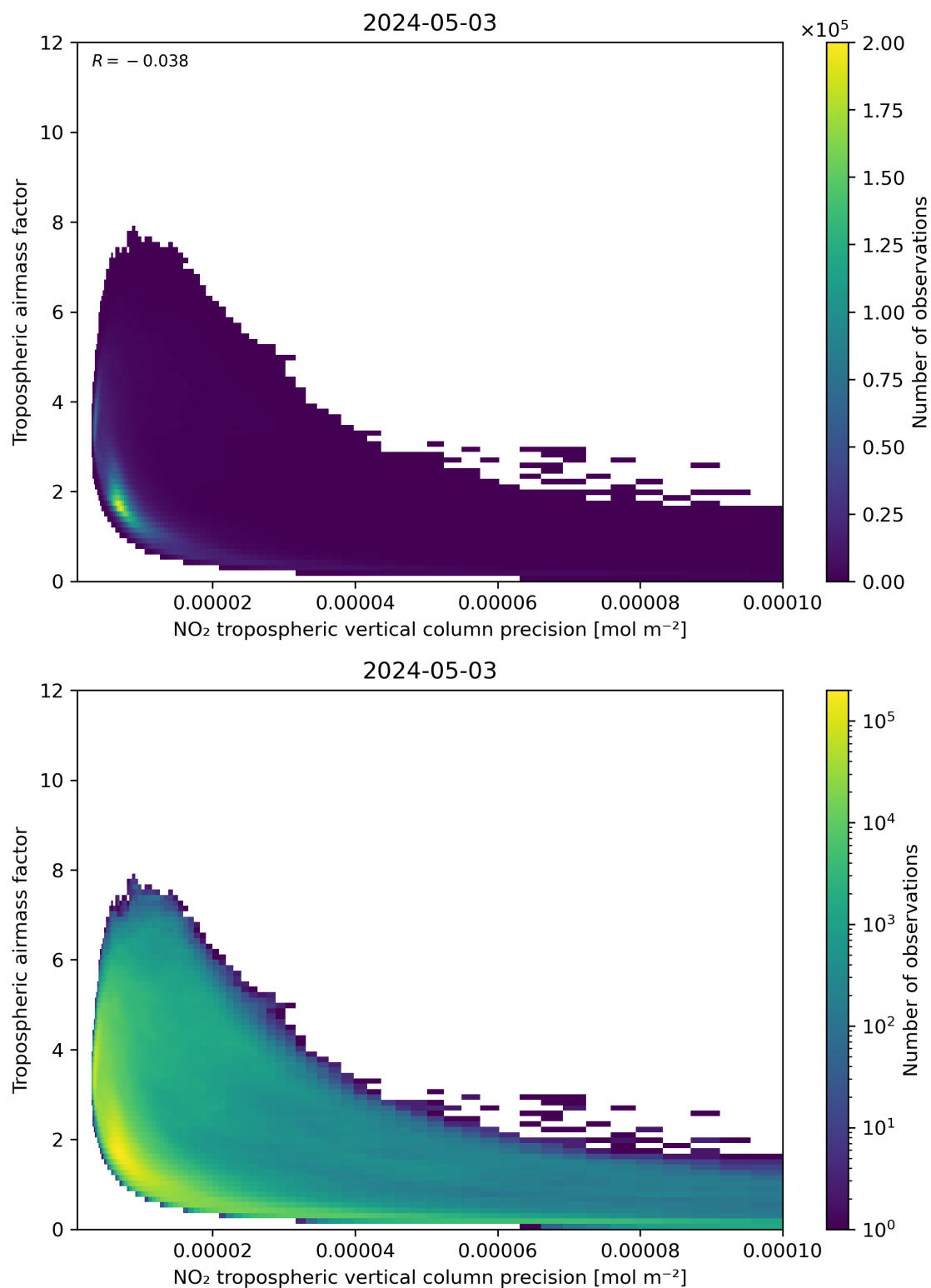
Figure 133: Scatter density plot of “NO 2 tropospheric vertical column precision” against “Tropospheric airmass factor” for 2024-05-02 to 2024-05-04.
