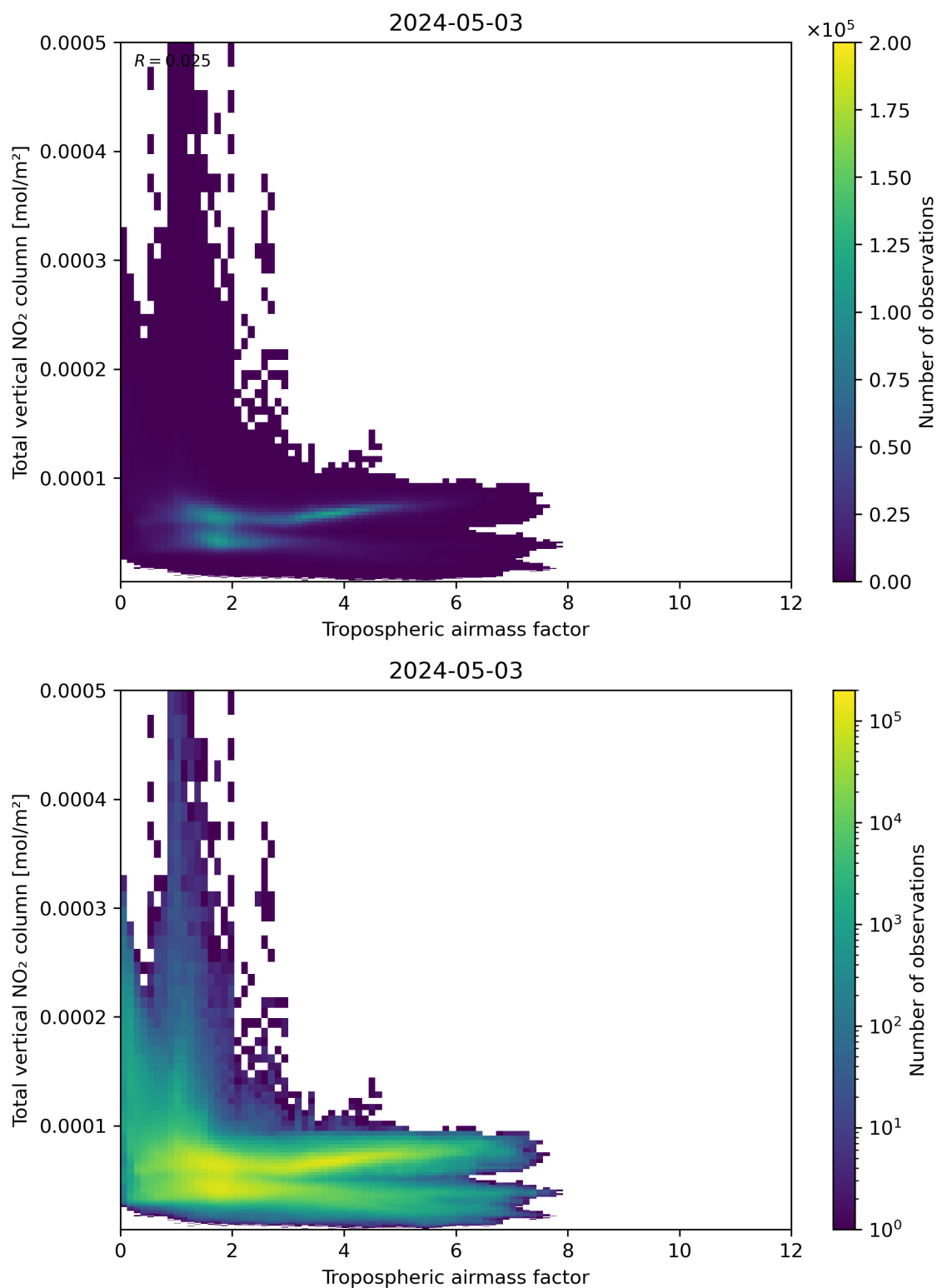
Figure 77: Scatter density plot of “Tropospheric airmass factor” against “Total vertical NO 2 column” for 2024-05-02 to 2024-05-04.
