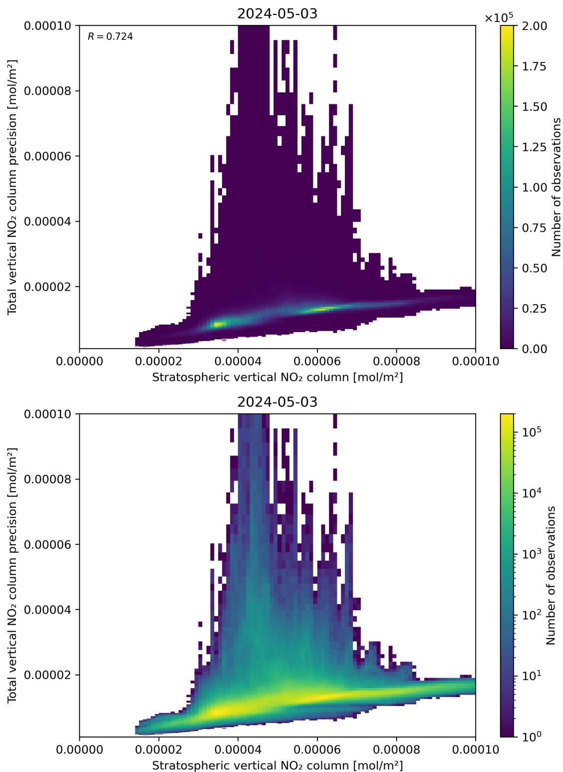
Figure 101: Scatter density plot of “Stratospheric vertical NO 2 column” against “Total vertical NO 2 column precision” for 2024-05-02 to 2024-05-04.
