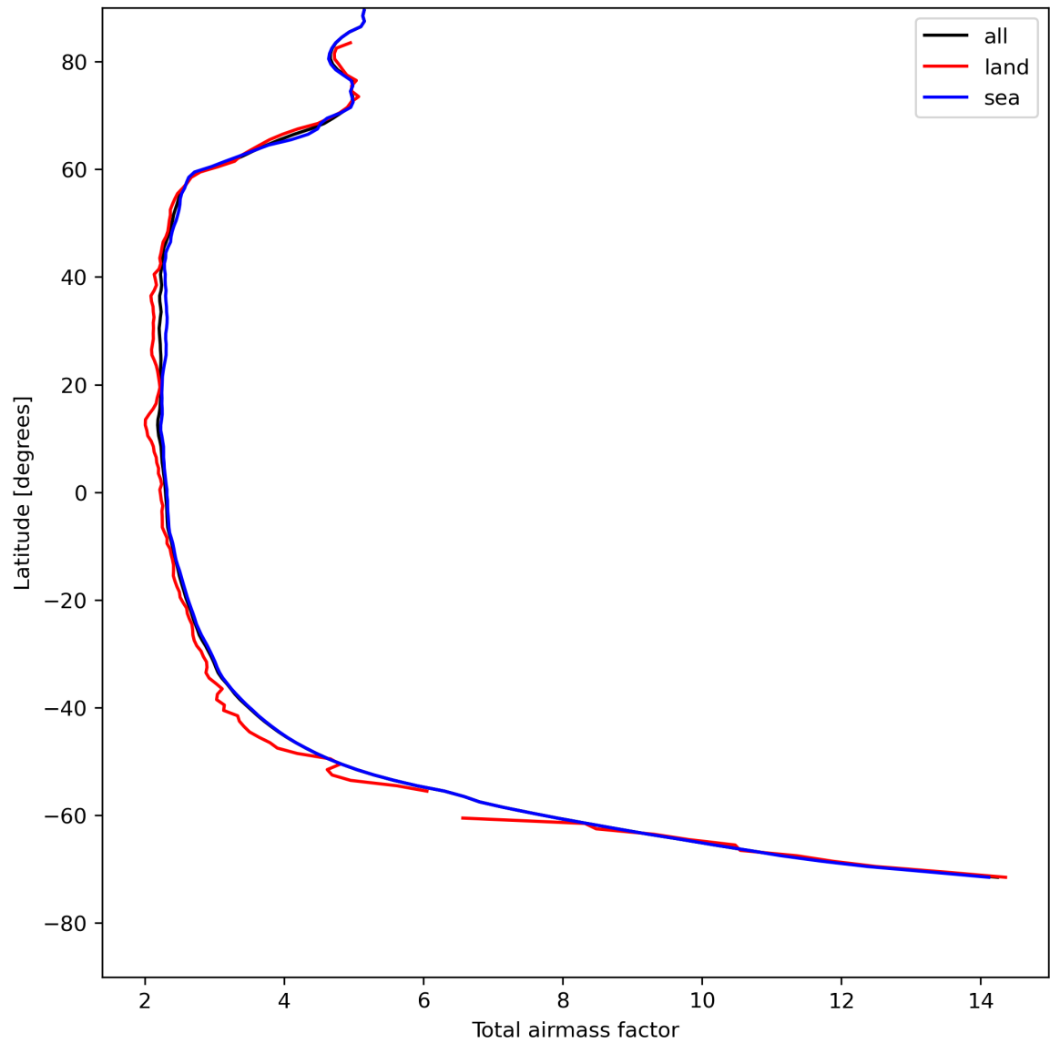
Figure 15: Zonal average of “Total airmass factor” for 2024-05-02 to 2024-05-04.
