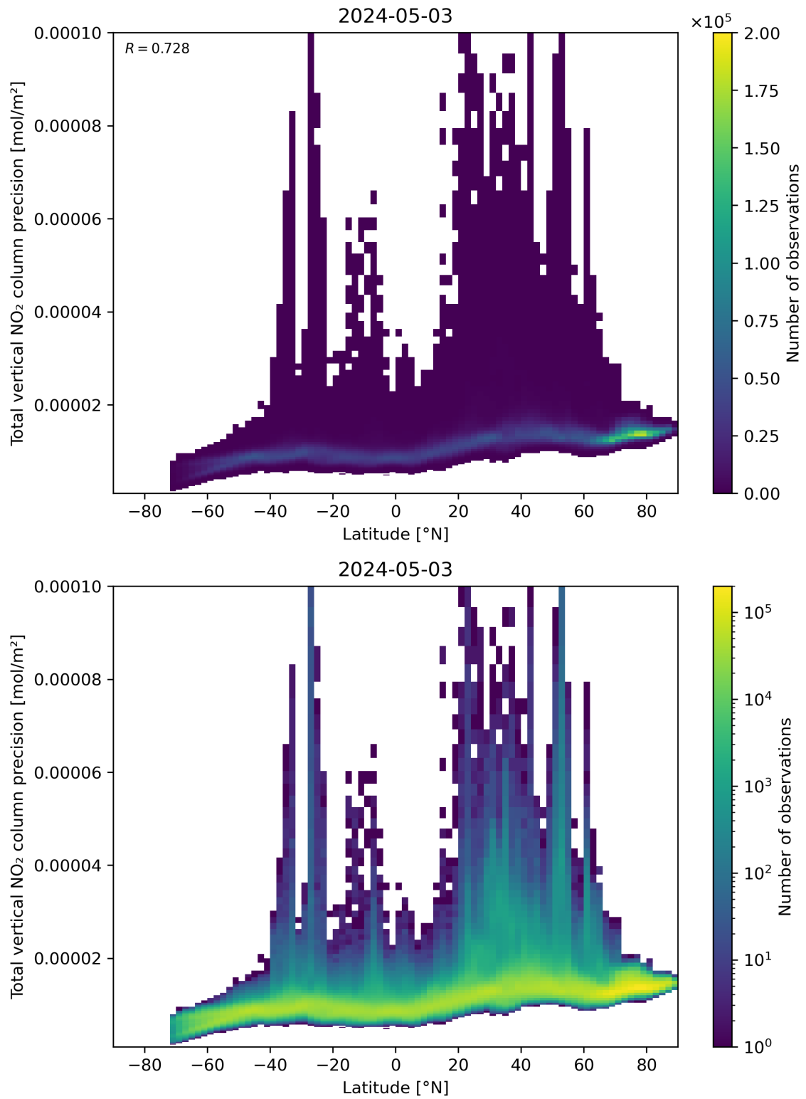
Figure 91: Scatter density plot of “Latitude” against “Total vertical NO 2 column precision” for 2024-05-02 to 2024-05-04.
