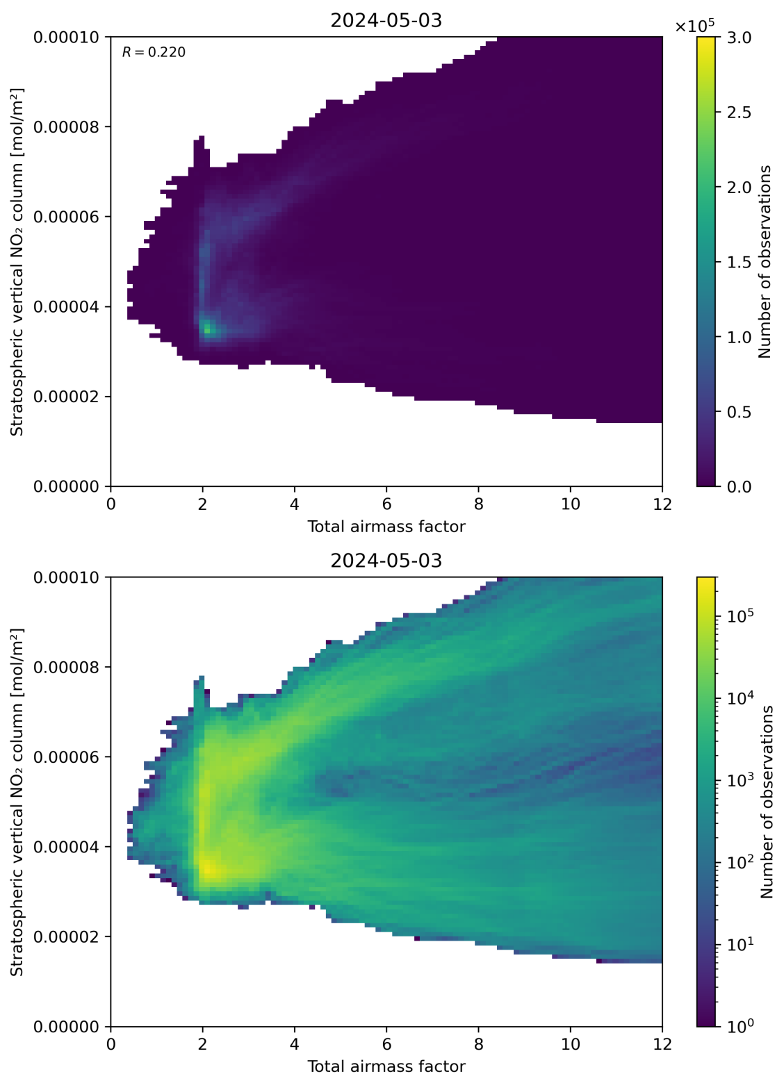
Figure 64: Scatter density plot of “Total airmass factor” against “Stratospheric vertical NO 2 column” for 2024-05-02 to 2024-05-04.
