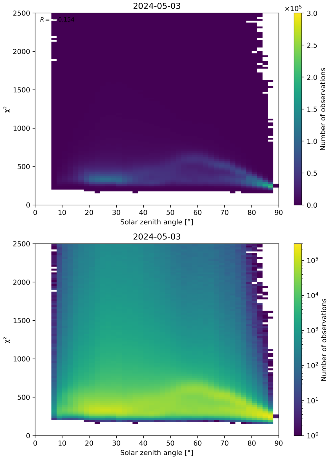
Figure 148: Scatter density plot of “Solar zenith angle” against “ \chi^2 ” for 2024-05-02 to 2024-05-04.
