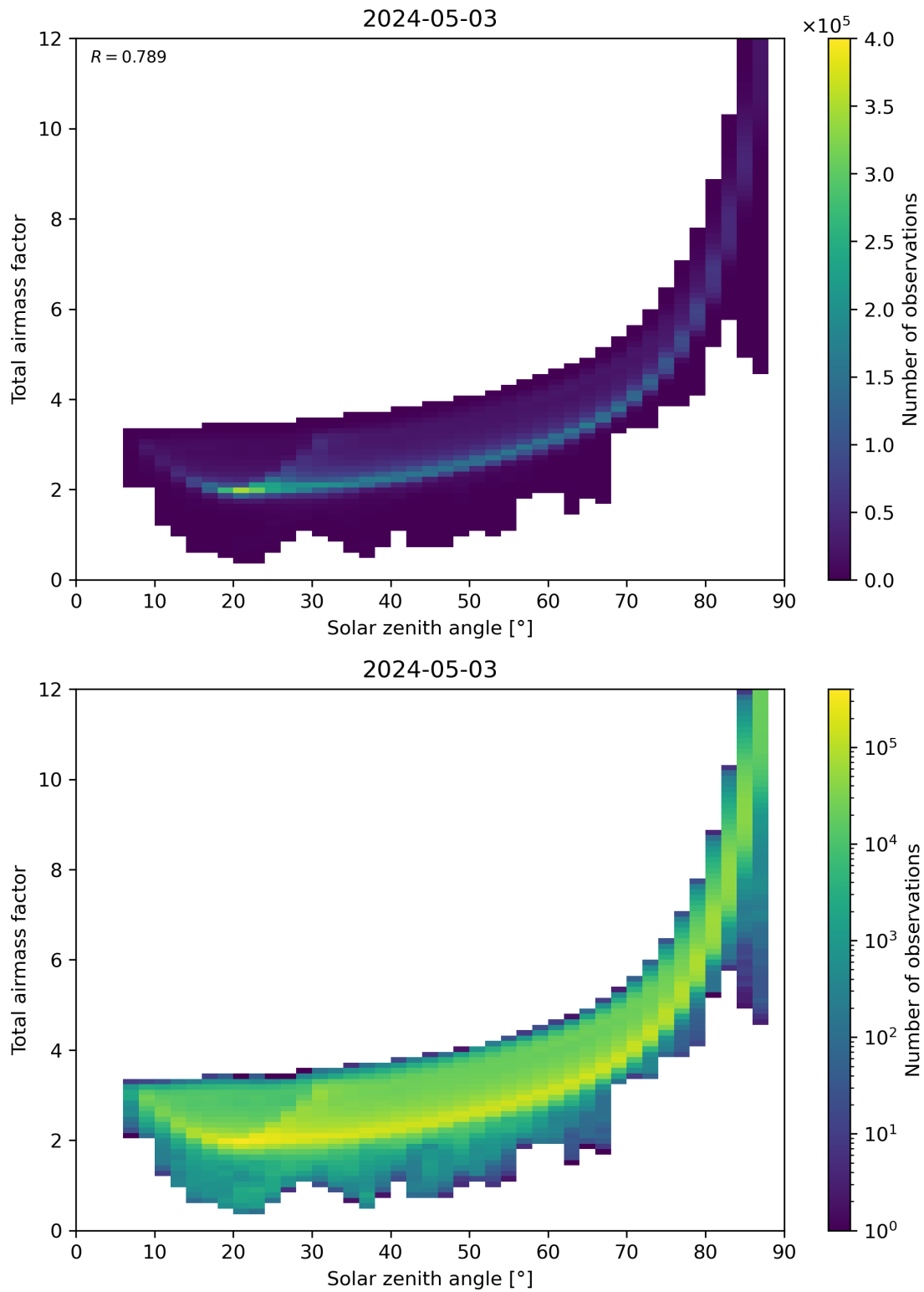
Figure 146: Scatter density plot of “Solar zenith angle” against “Total air mass factor” for 2024-05-02 to 2024-05-04.
