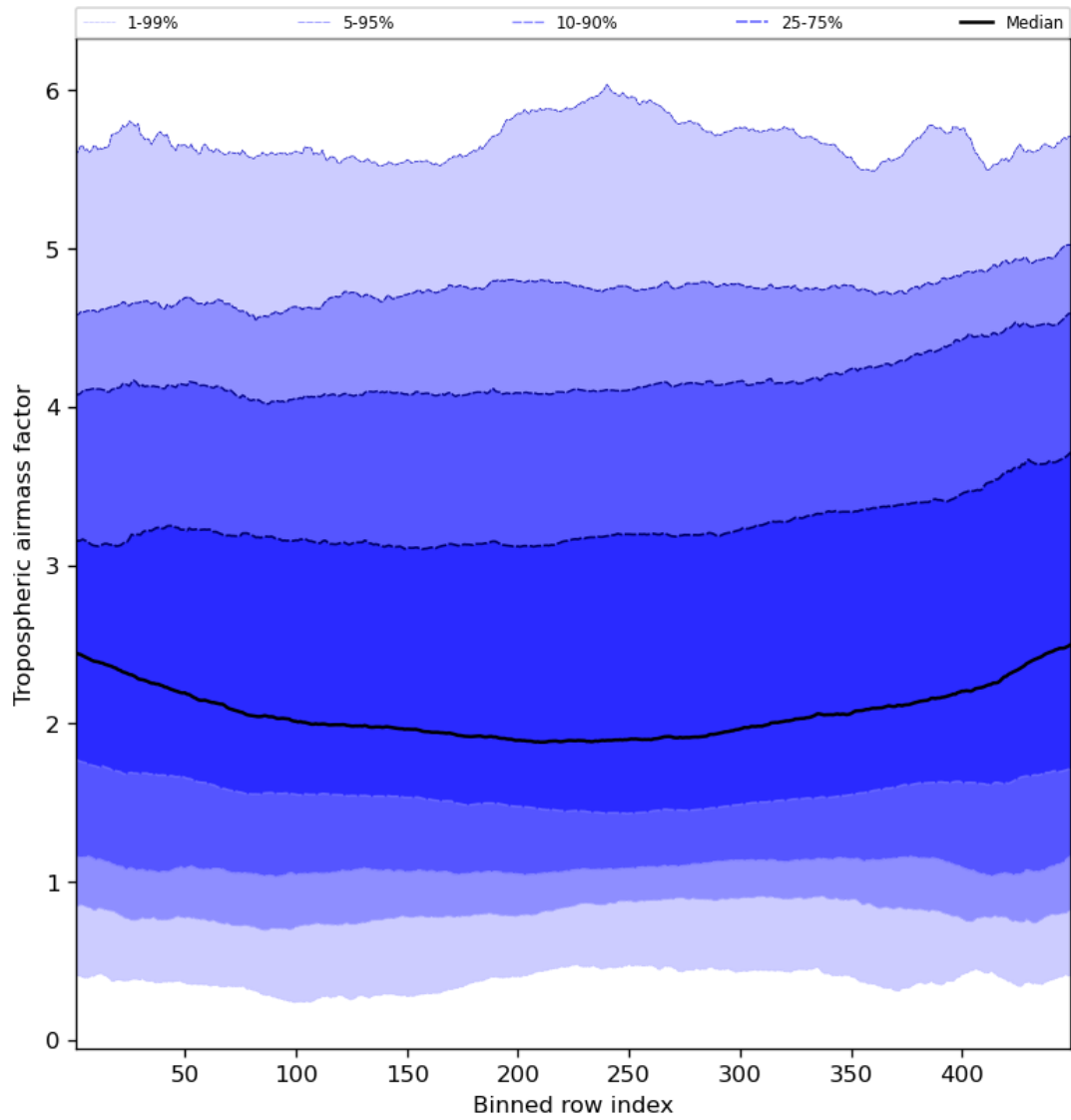
Figure 48: Along track statistics of “Tropospheric airmass factor” for 2024-05-02 to 2024-05-04
