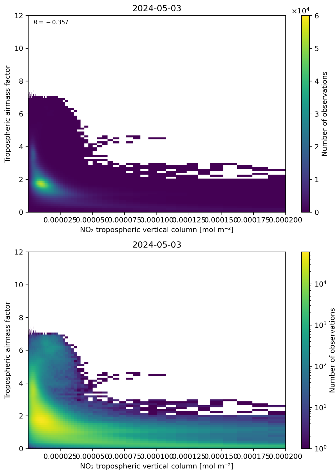
Figure 123: Scatter density plot of “NO 2 tropospheric vertical column” against “Tropospheric air mass factor” for 2024-05-02 to 2024-05-04.
