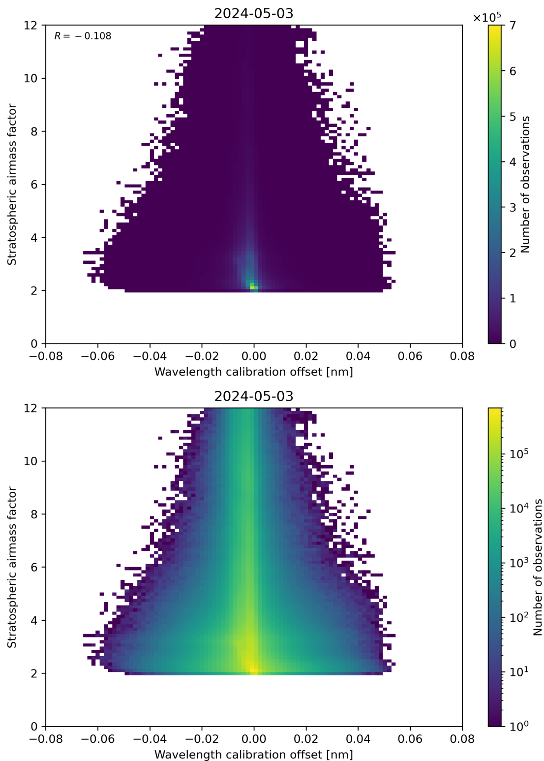
Figure 174: Scatter density plot of “Wavelength calibration offset” against “Stratospheric airmass factor” for 2024-05-02 to 2024-05-04.
