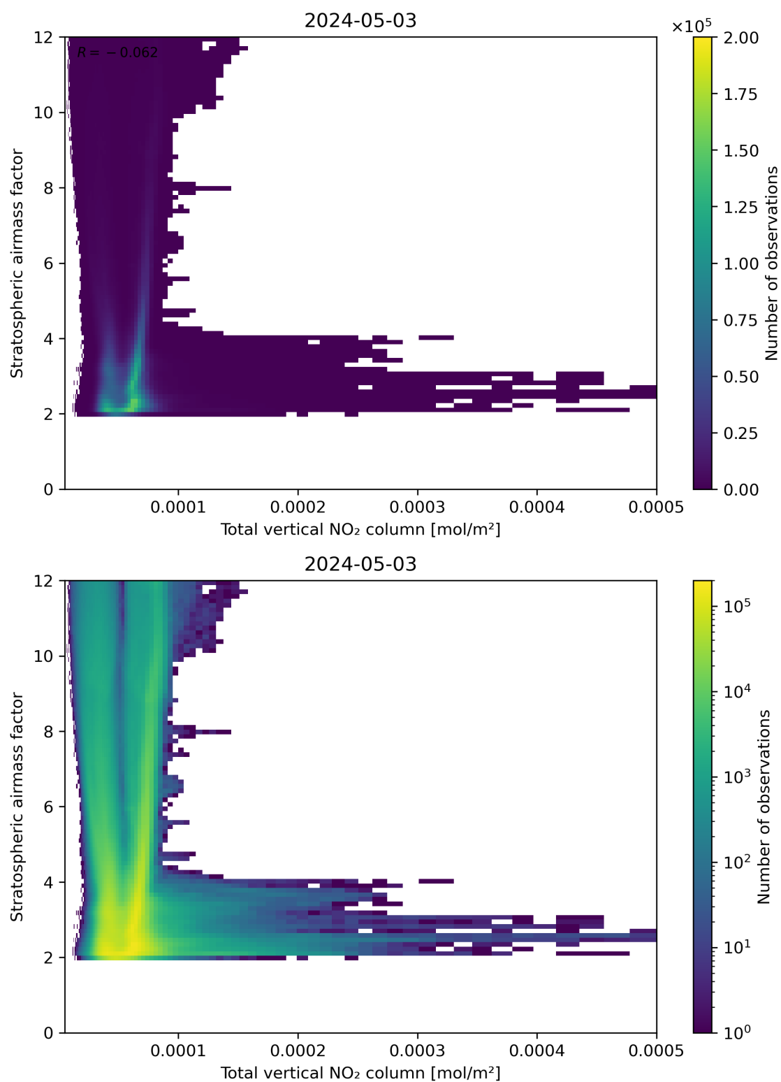
Figure 110: Scatter density plot of “Total vertical NO 2 column” against “Stratospheric airmass factor” for 2024-05-02 to 2024-05-04.
