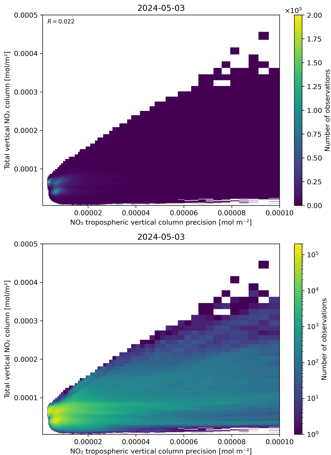
Figure 138: Scatter density plot of “NO 2 tropospheric vertical column precision” against “Total vertical NO 2 column” for 2024-05-02 to 2024-05-04.
