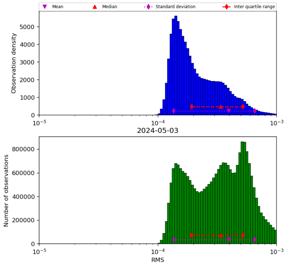
Figure 43: Histogram of “RMS” for 2024-05-02 to 2024-05-04
