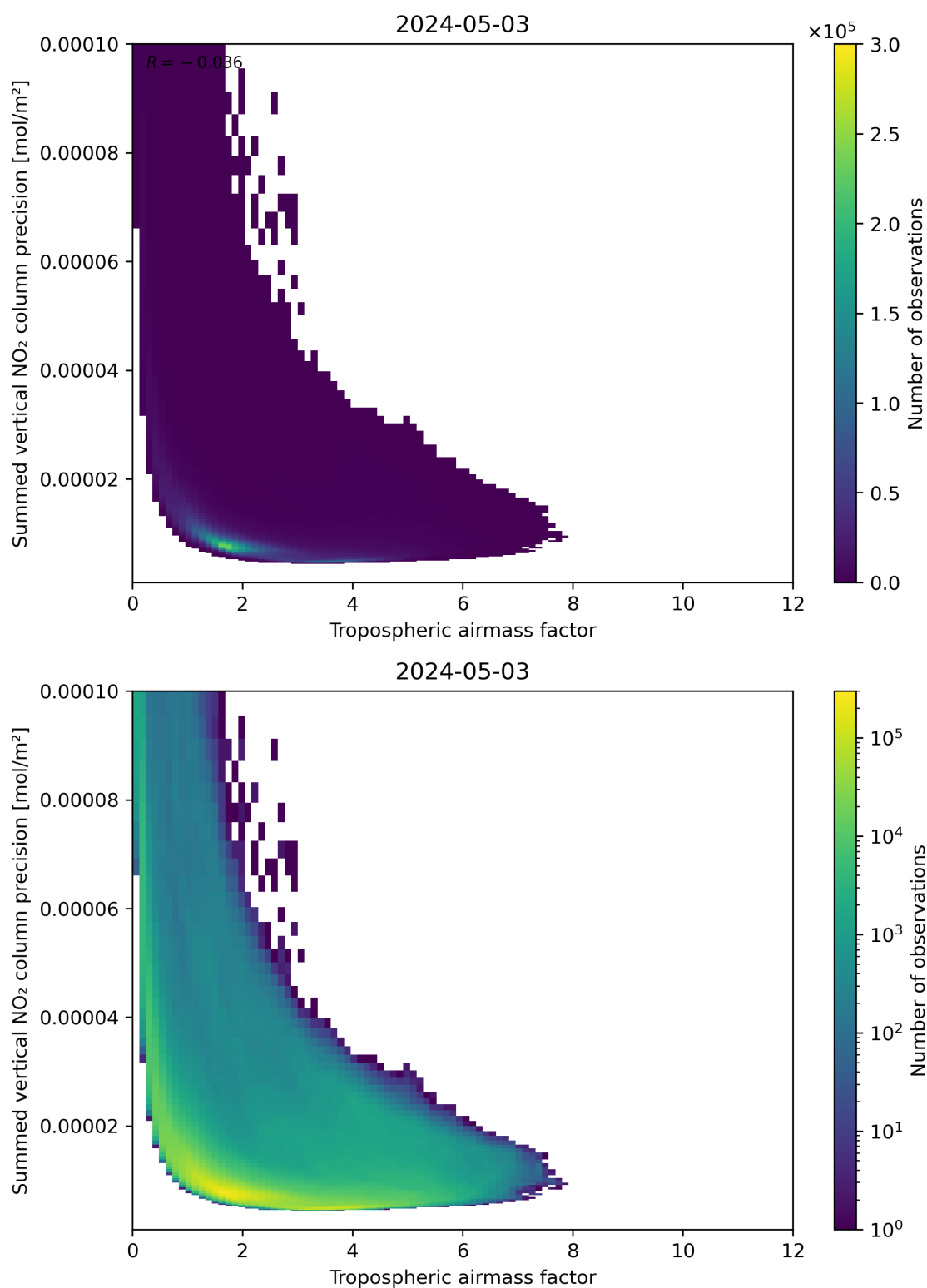
Figure 76: Scatter density plot of “Tropospheric air mass factor” against “Summed vertical NO 2 column precision” for 2024-05-02 to 2024-05-04.
