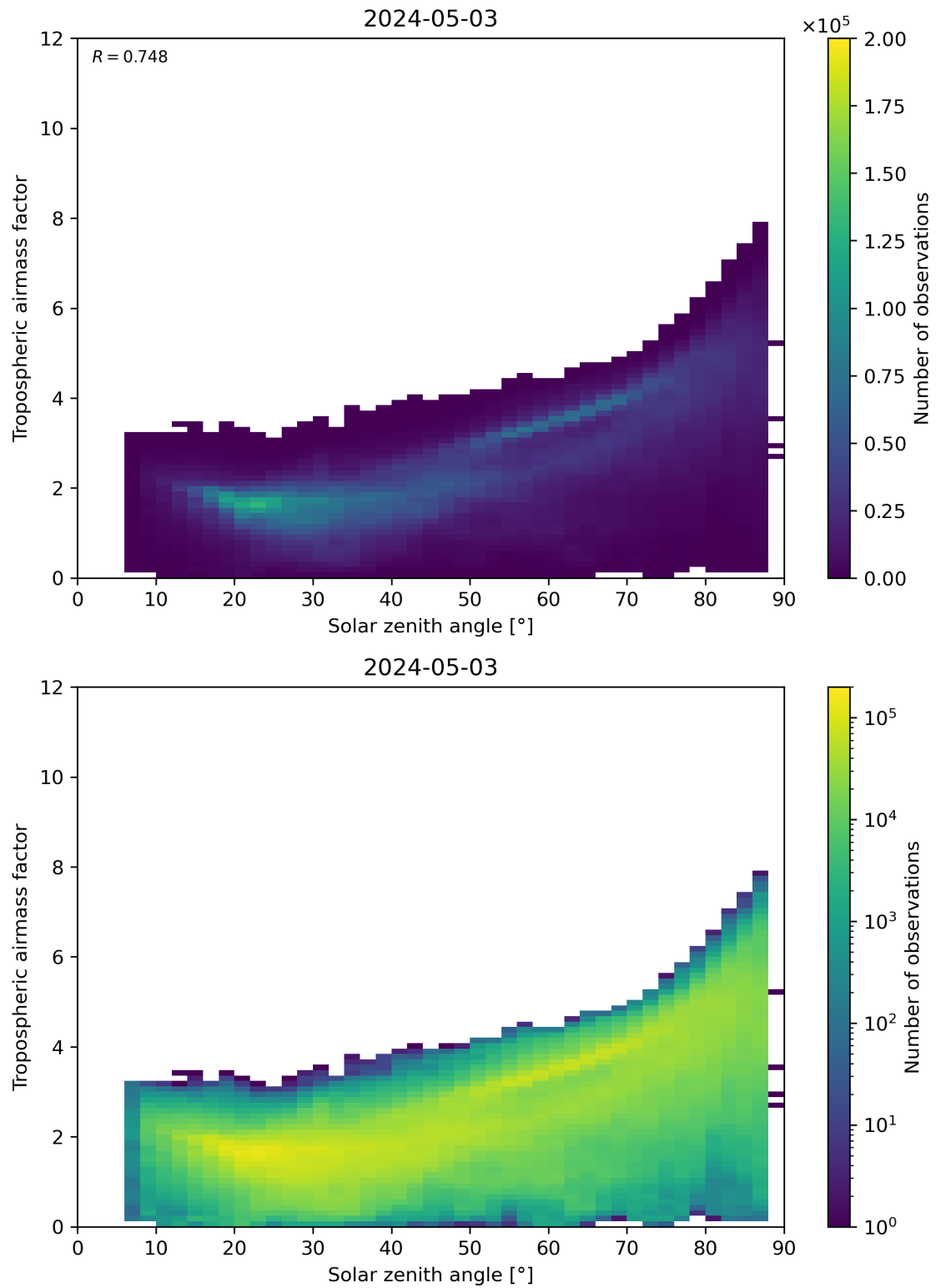
Figure 147: Scatter density plot of “Solar zenith angle” against “Tropospheric airmass factor” for 2024-05-02 to 2024-05-04.
