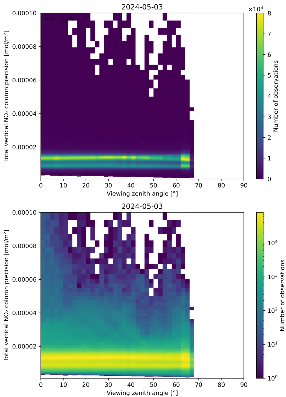
Figure 168: Scatter density plot of “Viewing zenith angle” against “Total vertical NO 2 column precision” for 2024-05-02 to 2024-05-04.
