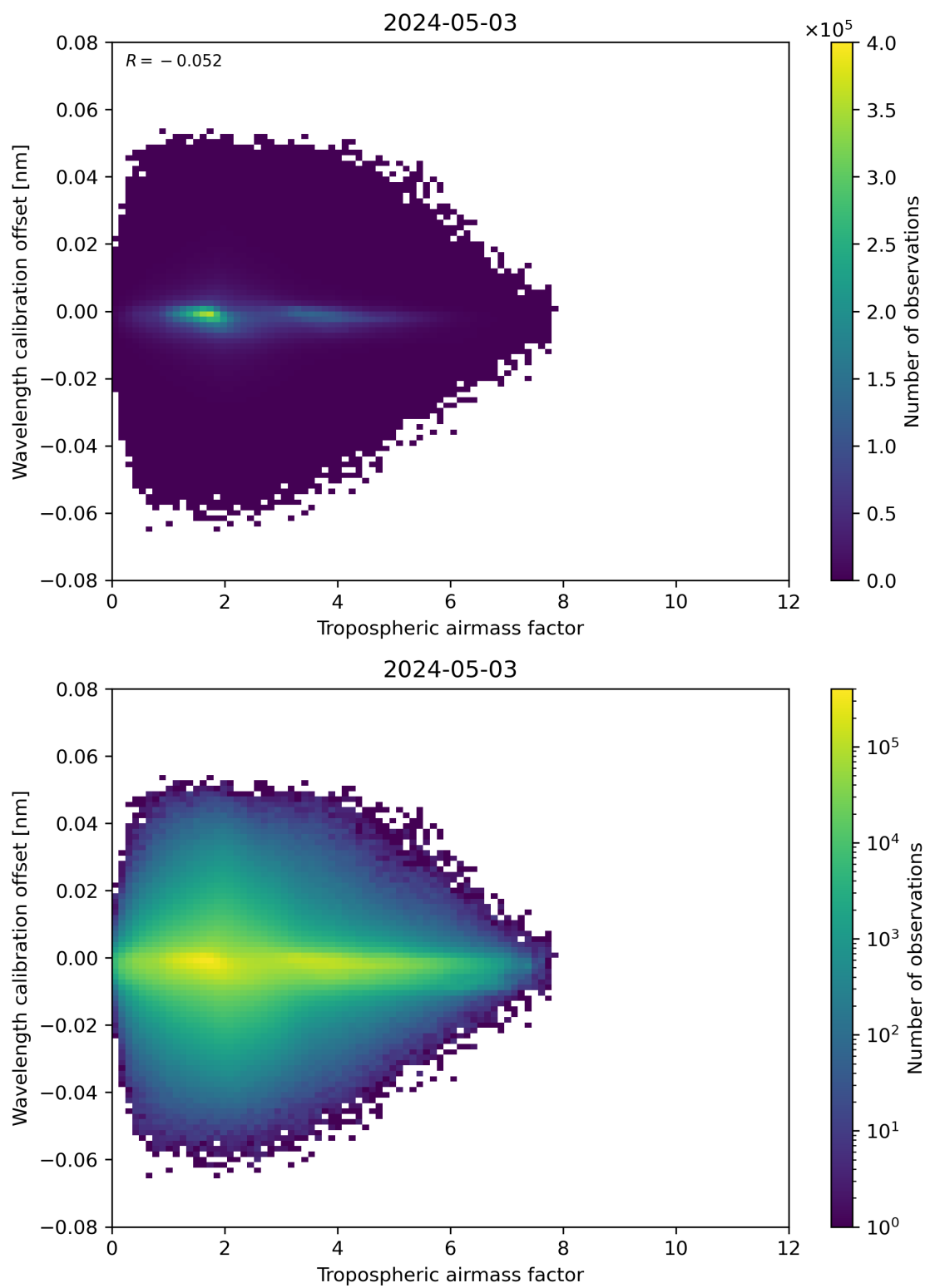
Figure 80: Scatter density plot of “Tropospheric airmass factor” against “Wavelength calibration offset” for 2024-05-02 to 2024-05-04.
