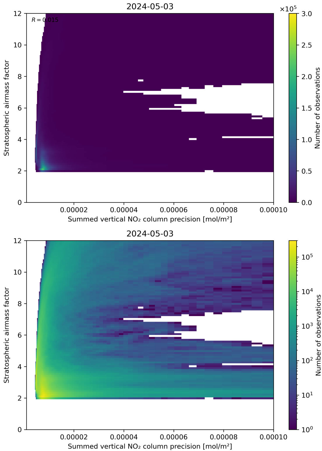
Figure 106: Scatter density plot of “Summed vertical NO 2 column precision” against “Stratospheric airmass factor” for 2024-05-02 to 2024-05-04.
