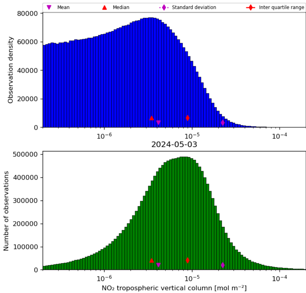
Figure 29: Histogram of “NO 2 tropospheric vertical column” for 2024-05-02 to 2024-05-04
