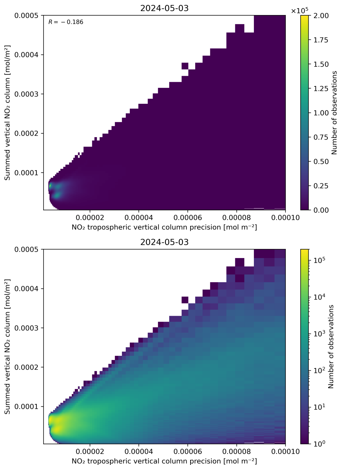
Figure 136: Scatter density plot of “NO 2 tropospheric vertical column precision” against “Summed vertical NO 2 column” for 2024-05-02 to 2024-05-04.
