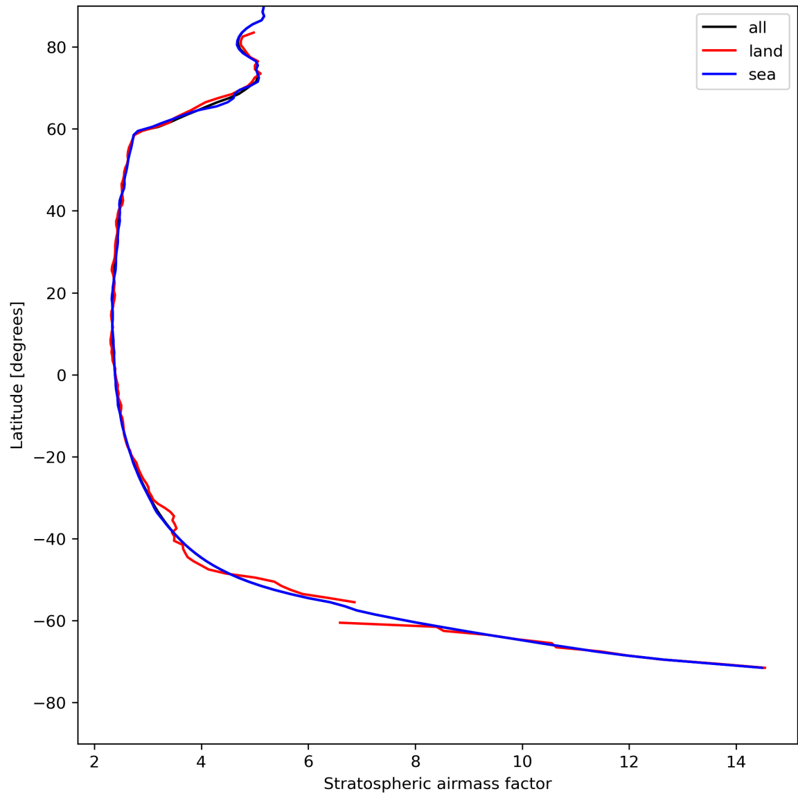
Figure 27: Zonal average of “Stratospheric air mass factor” for 2024-05-02 to 2024-05-04.
