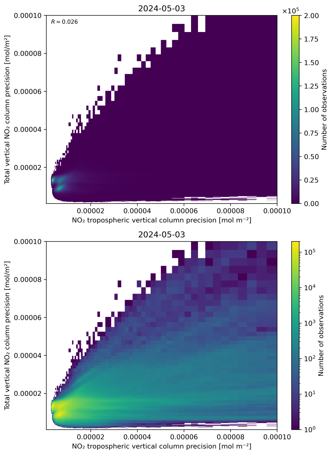
Figure 139: Scatter density plot of “NO 2 tropospheric vertical column precision” against “Total vertical NO 2 column precision” for 2024-05-02 to 2024-05-04.
