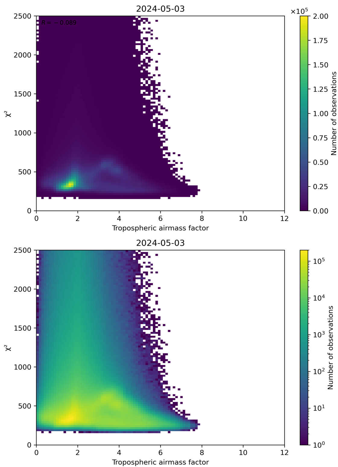
Figure 73: Scatter density plot of “Tropospheric airmass factor” against “ \chi^2 ” for 2024-05-02 to 2024-05-04.
