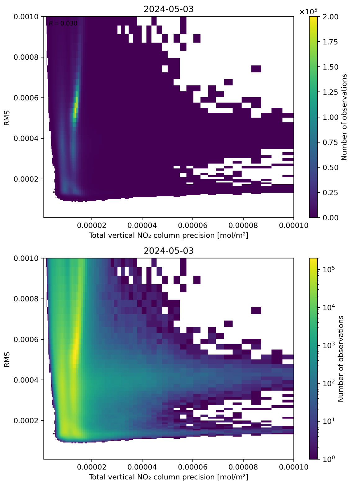
Figure 119: Scatter density plot of “Total vertical NO 2 column precision” against “RMS” for 2024-05-02 to 2024-05-04.
