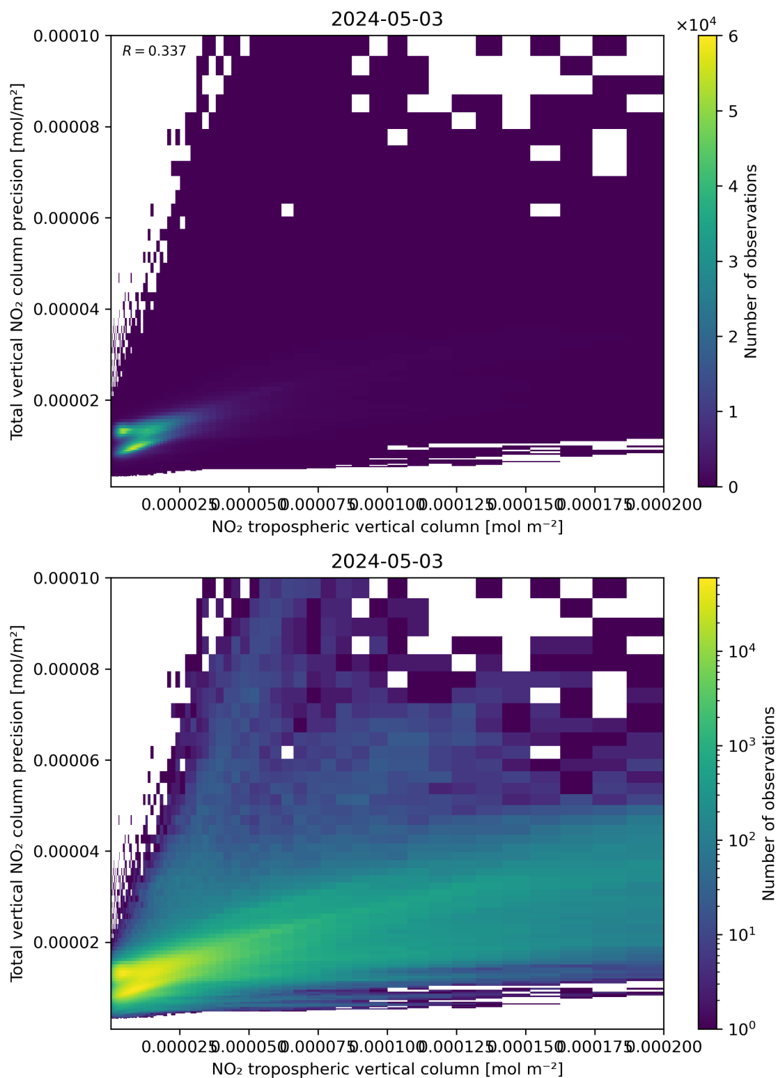
Figure 129: Scatter density plot of “NO 2 tropospheric vertical column” against “Total vertical NO 2 column precision” for 2024-05-02 to 2024-05-04.
