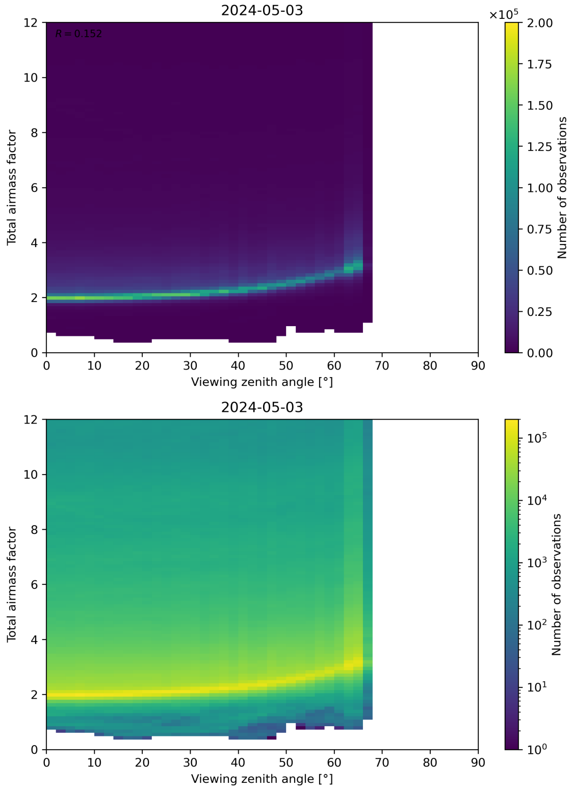
Figure 160: Scatter density plot of “Viewing zenith angle” against “Total airmass factor” for 2024-05-02 to 2024-05-04.
