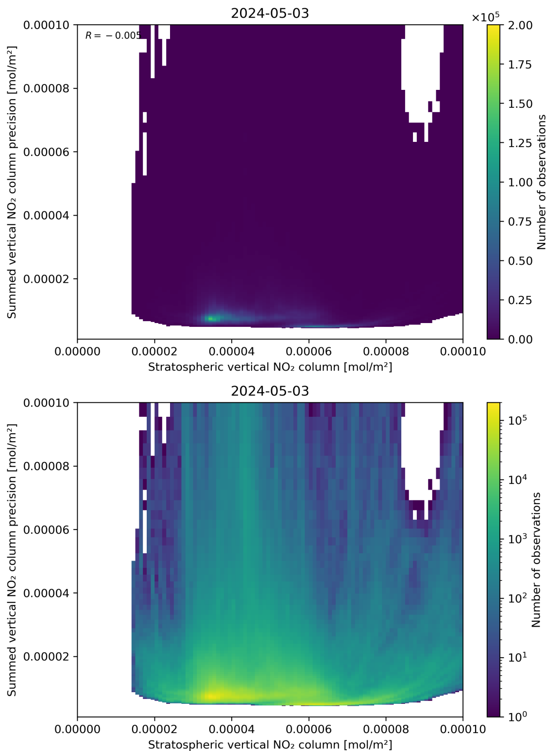
Figure 99: Scatter density plot of “Stratospheric vertical NO 2 column” against “Summed vertical NO 2 column precision” for 2024-05-02 to 2024-05-04.
