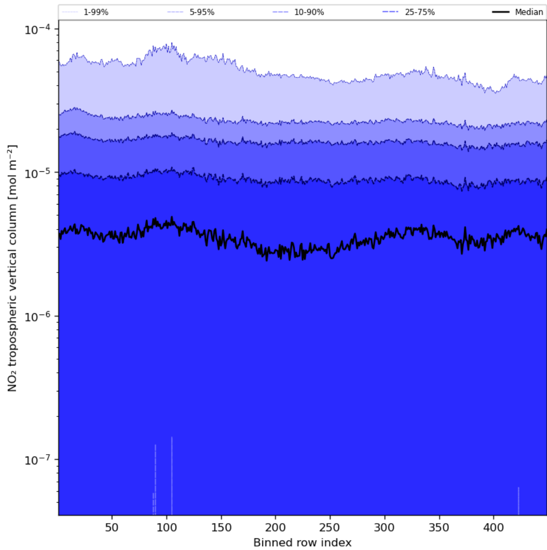
Figure 46: Along track statistics of “NO 2 tropospheric vertical column” for 2024-05-02 to 2024-05-04
