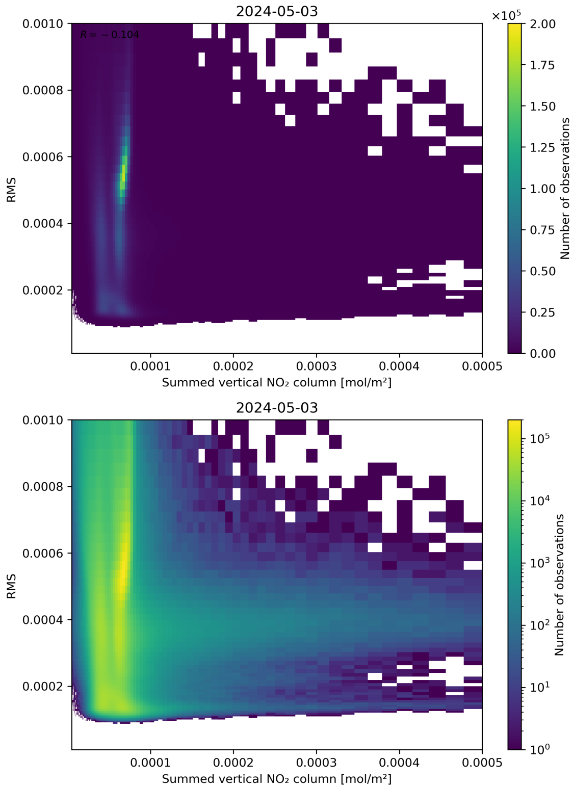
Figure 109: Scatter density plot of “Summed vertical NO 2 column” against “RMS” for 2024-05-02 to 2024-05-04.
