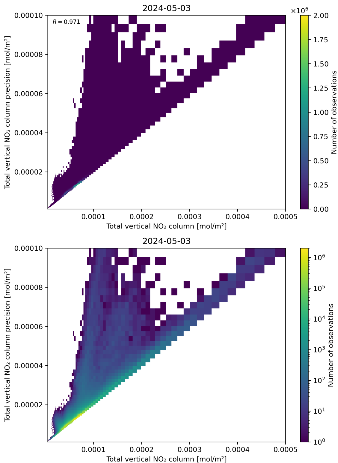
Figure 114: Scatter density plot of “Total vertical NO 2 column” against “Total vertical NO 2 column precision” for 2024-05-02 to 2024-05-04.
