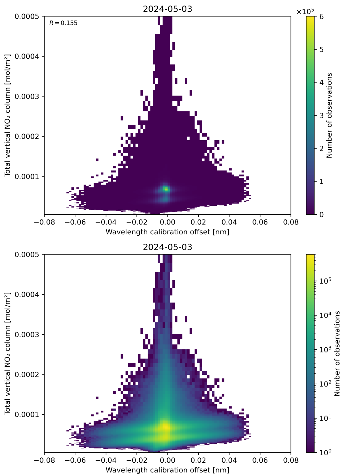
Figure 179: Scatter density plot of “Wavelength calibration offset” against “Total vertical NO 2 column” for 2024-05-02 to 2024-05-04.
