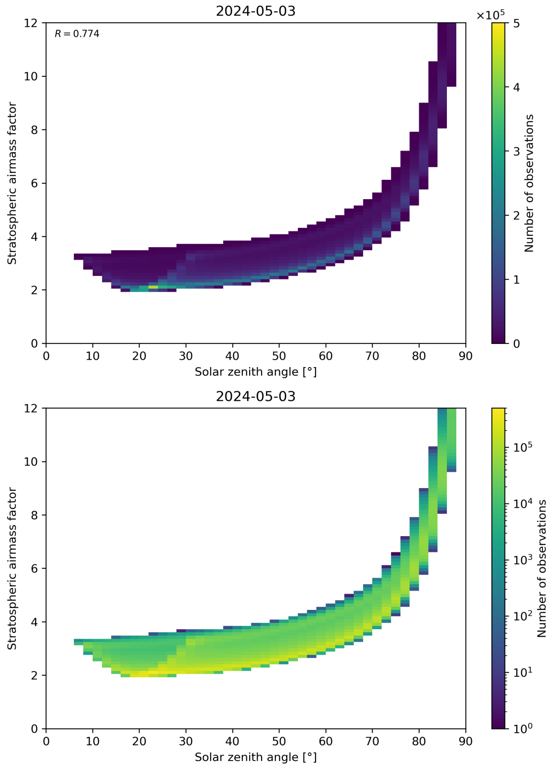
Figure 145: Scatter density plot of “Solar zenith angle” against “Stratospheric airmass factor” for 2024-05-02 to 2024-05-04.
