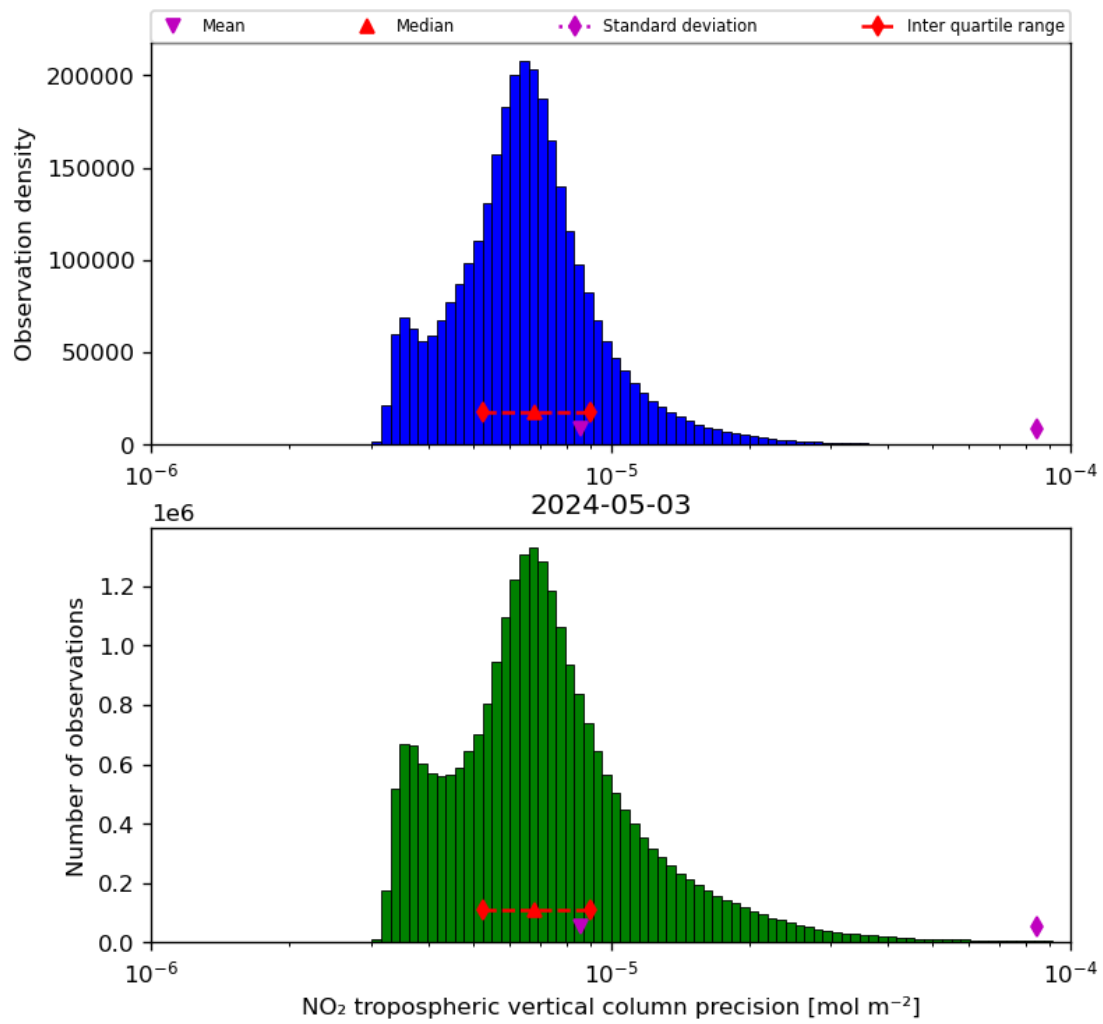
Figure 30: Histogram of “NO 2 tropospheric vertical column precision” for 2024-05-02 to 2024-05-04
