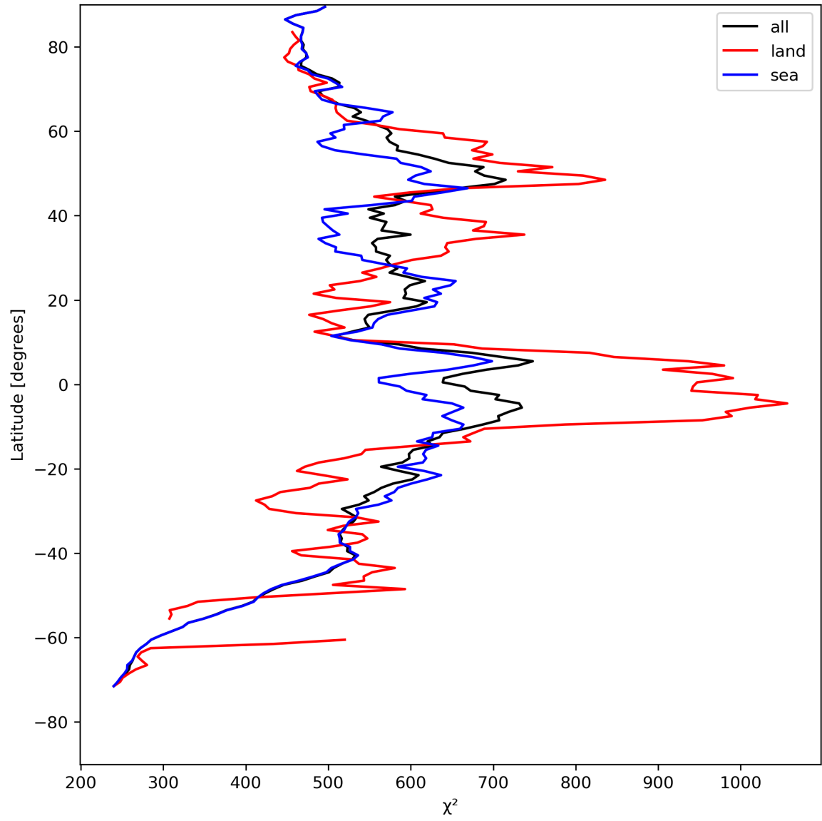
Figure 25: Zonal average of “ \chi^2 ” for 2024-05-02 to 2024-05-04.
