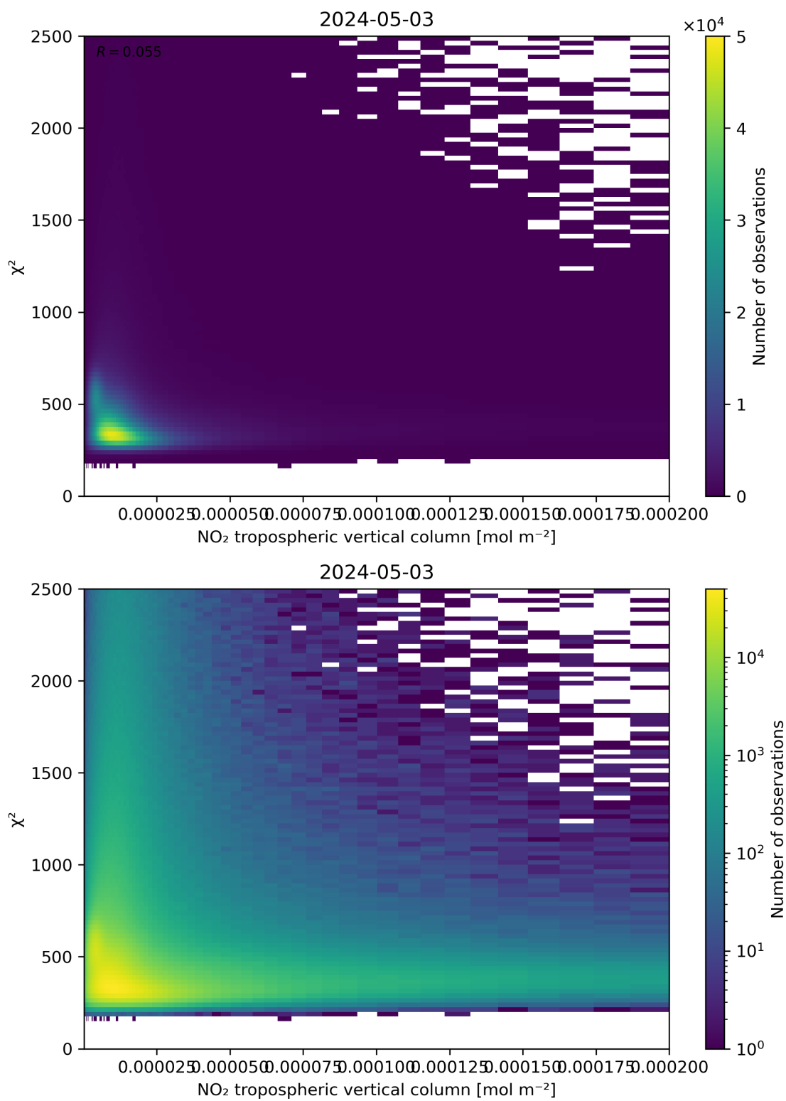
Figure 124: Scatter density plot of “NO 2 tropospheric vertical column” against “ \chi^2 ” for 2024-05-02 to 2024-05-04.
