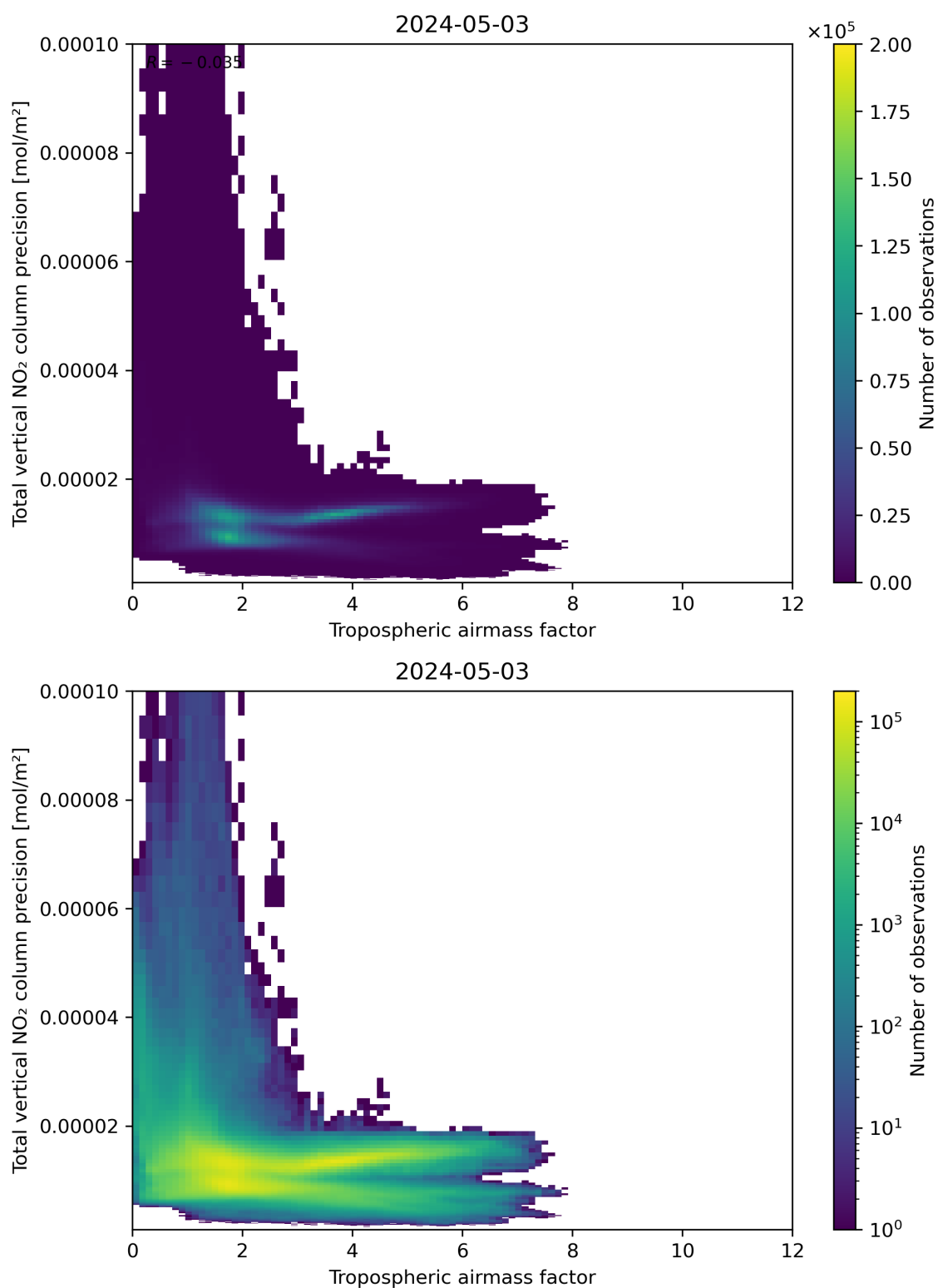
Figure 78: Scatter density plot of “Tropospheric air mass factor” against “Total vertical NO 2 column precision” for 2024-05-02 to 2024-05-04.
