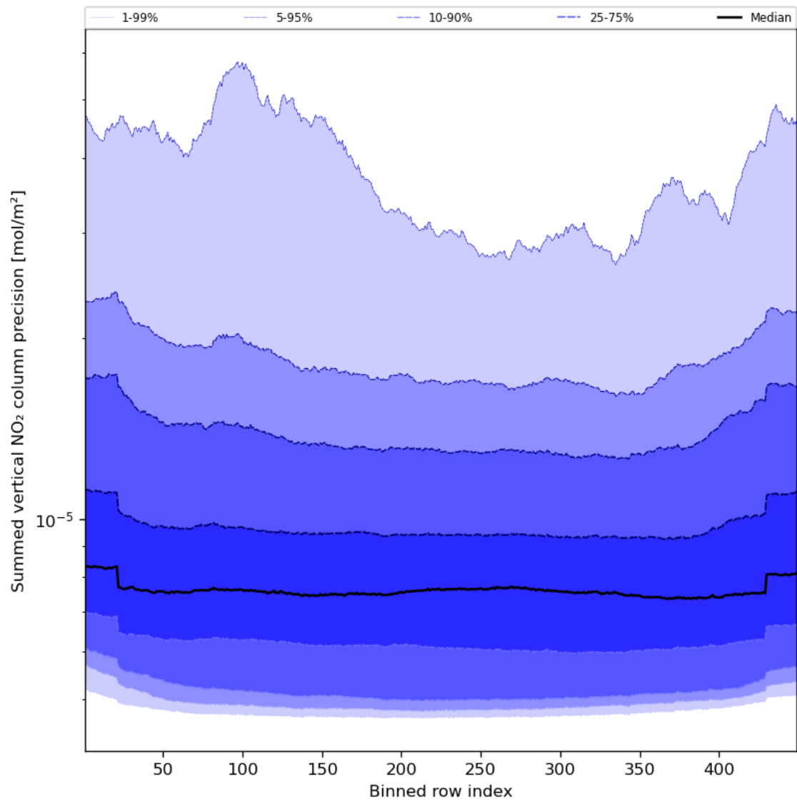
Figure 58: Along track statistics of “Summed vertical NO 2 column precision” for 2024-05-02 to 2024-05-04
