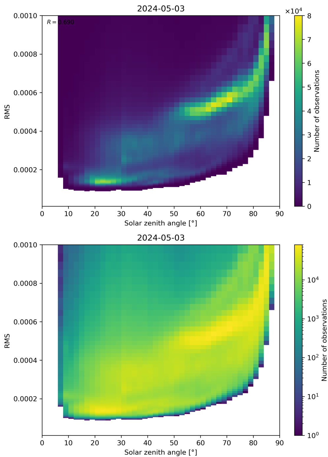
Figure 157: Scatter density plot of “Solar zenith angle” against “RMS” for 2024-05-02 to 2024-05-04.
