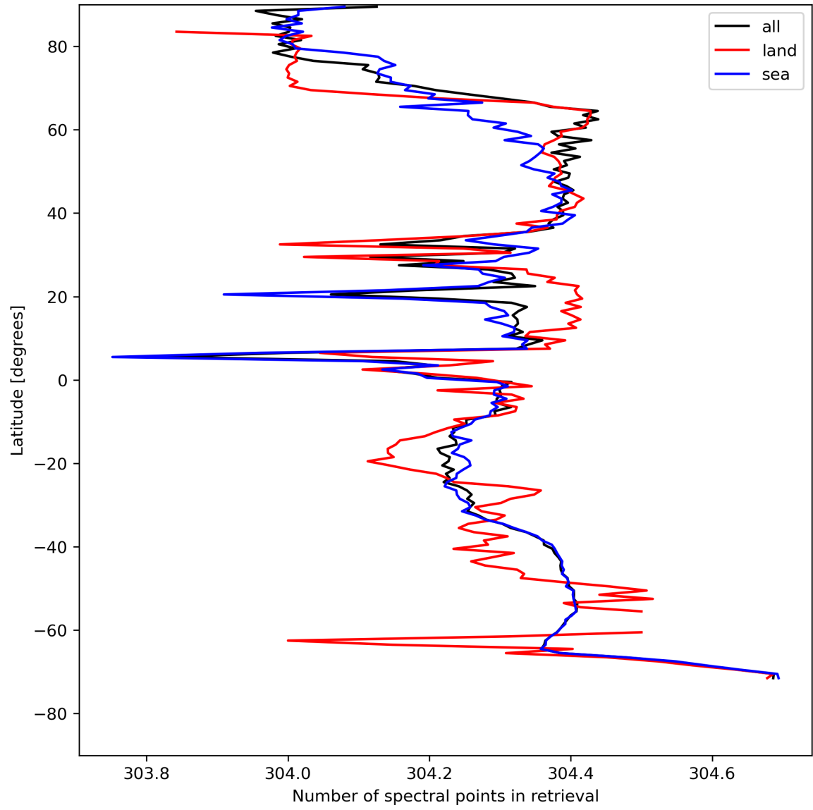
Figure 16: Zonal average of “Number of spectral points in retrieval” for 2024-05-02 to 2024-05-04.
