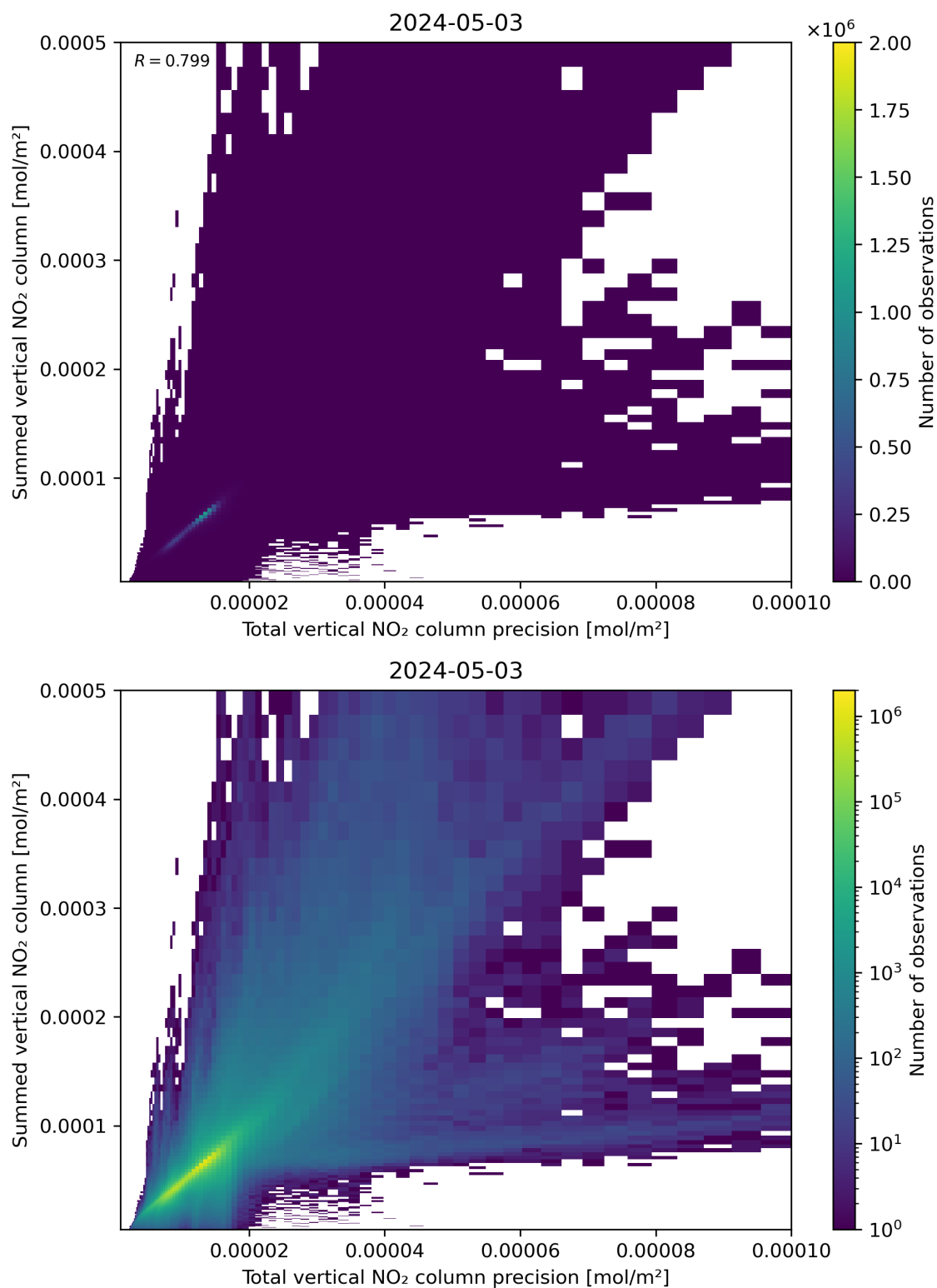
Figure 117: Scatter density plot of “Total vertical NO 2 column precision” against “Summed vertical NO 2 column” for 2024-05-02 to 2024-05-04.
