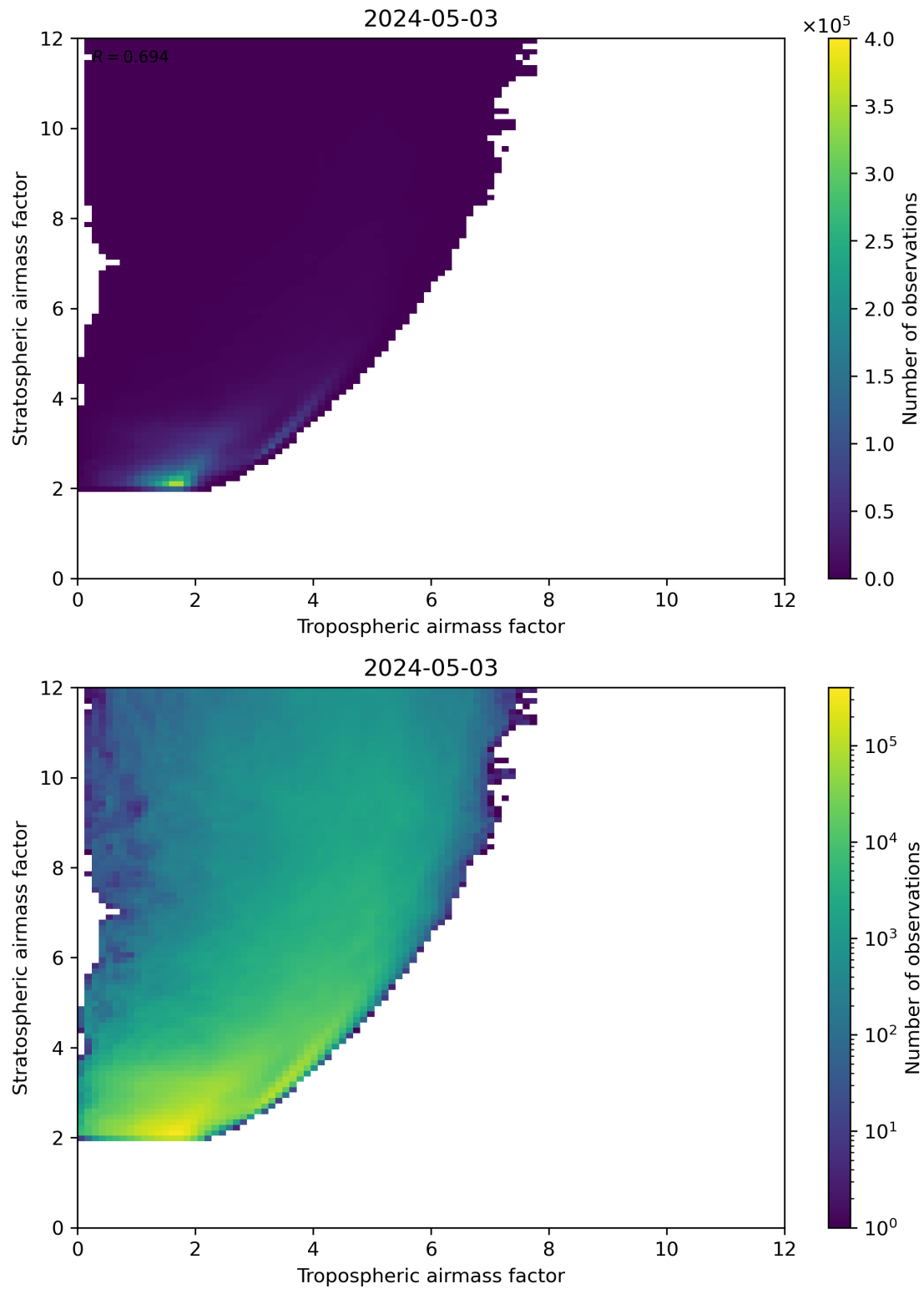
Figure 71: Scatter density plot of “Tropospheric airmass factor” against “Stratospheric airmass factor” for 2024-05-02 to 2024-05-04.
