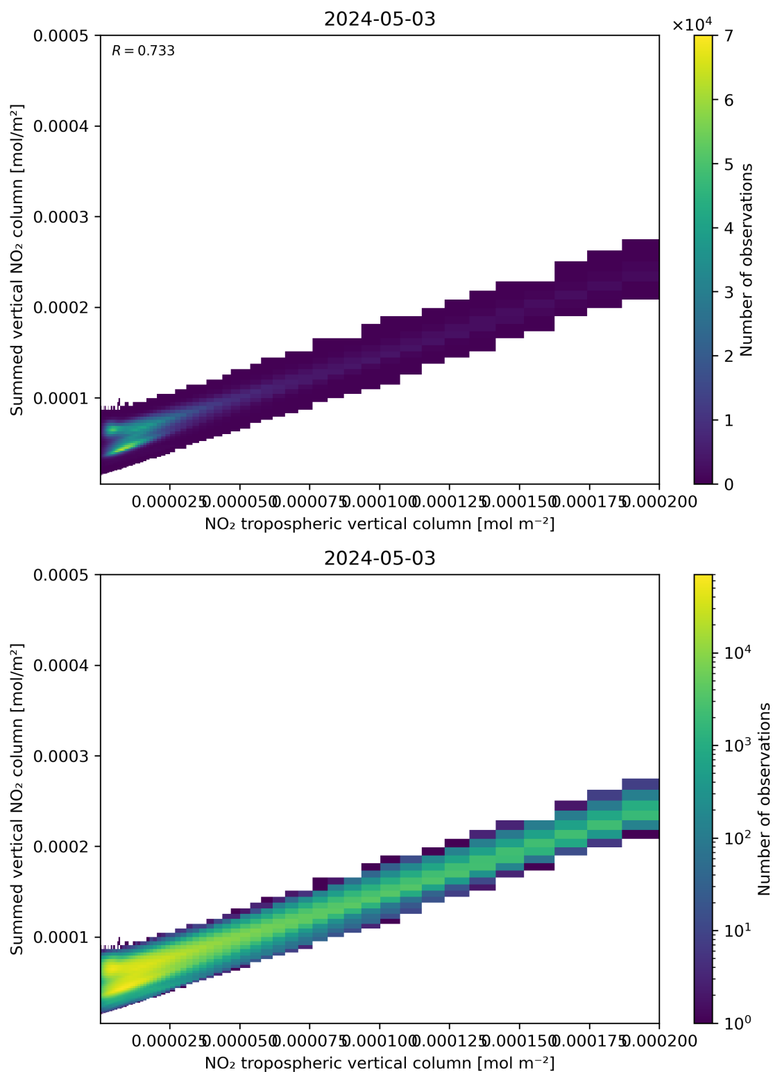
Figure 126: Scatter density plot of “NO 2 tropospheric vertical column” against “Summed vertical NO 2 column” for 2024-05-02 to 2024-05-04.
