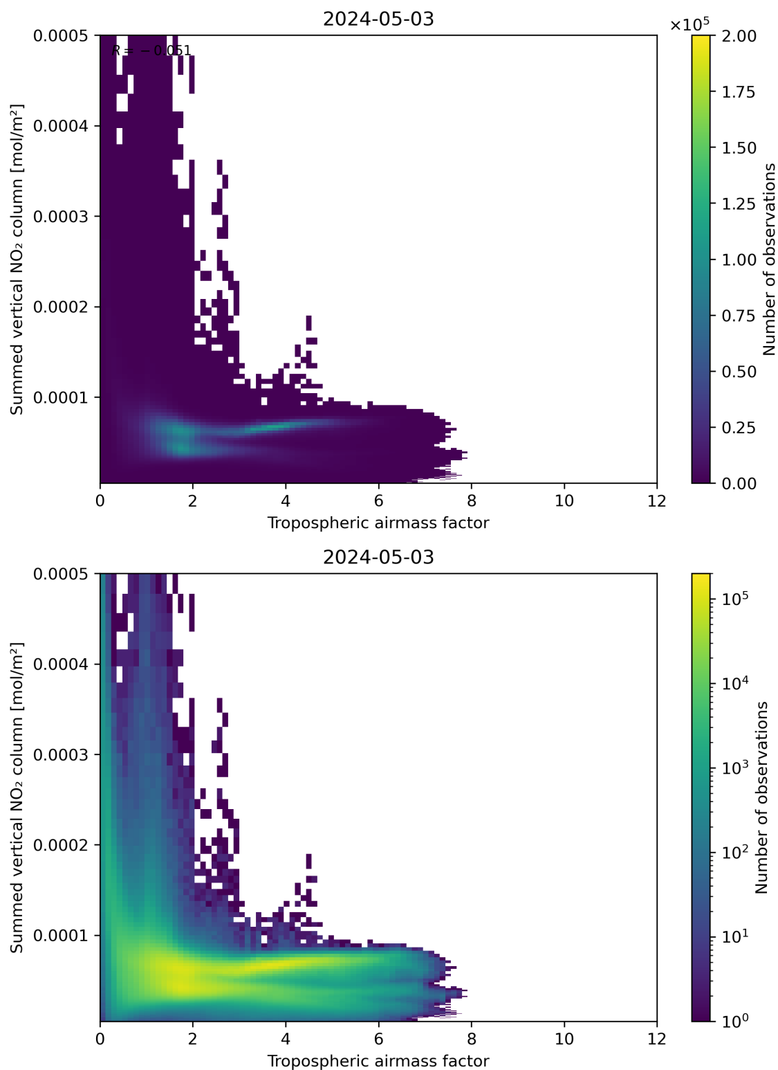
Figure 75: Scatter density plot of “Tropospheric airmass factor” against “Summed vertical NO 2 column” for 2024-05-02 to 2024-05-04.
