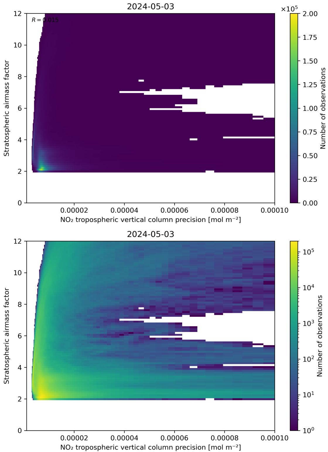
Figure 131: Scatter density plot of “NO 2 tropospheric vertical column precision” against “Stratospheric airmass factor” for 2024-05-02 to 2024-05-04.
