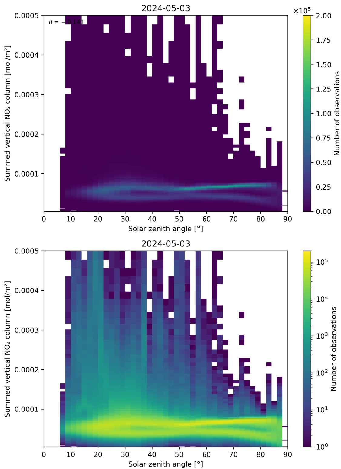
Figure 151: Scatter density plot of “Solar zenith angle” against “Summed vertical NO 2 column” for 2024-05-02 to 2024-05-04.
