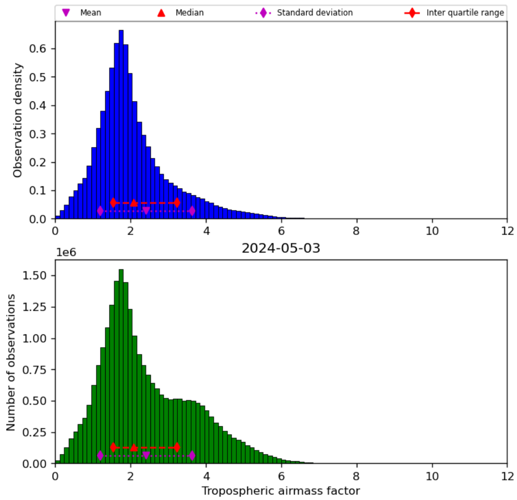
Figure 31: Histogram of “Tropospheric airmass factor” for 2024-05-02 to 2024-05-04
