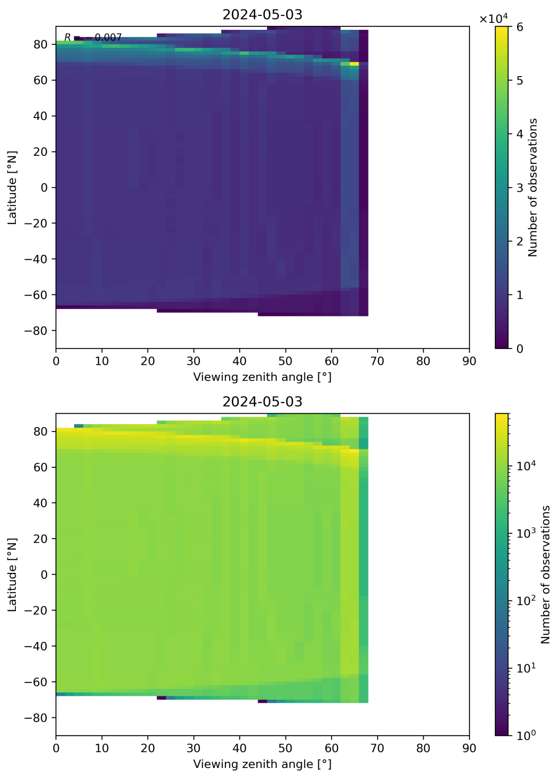
Figure 163: Scatter density plot of “Viewing zenith angle” against “Latitude” for 2024-05-02 to 2024-05-04.
