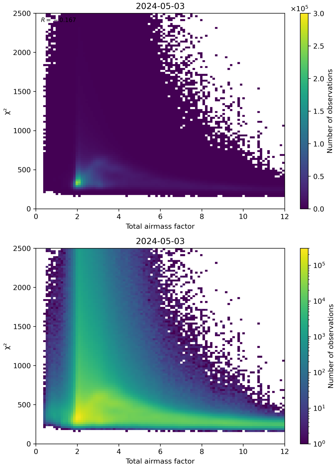
Figure 63: Scatter density plot of “Total airmass factor” against “ \chi^2 ” for 2024-05-02 to 2024-05-04.
