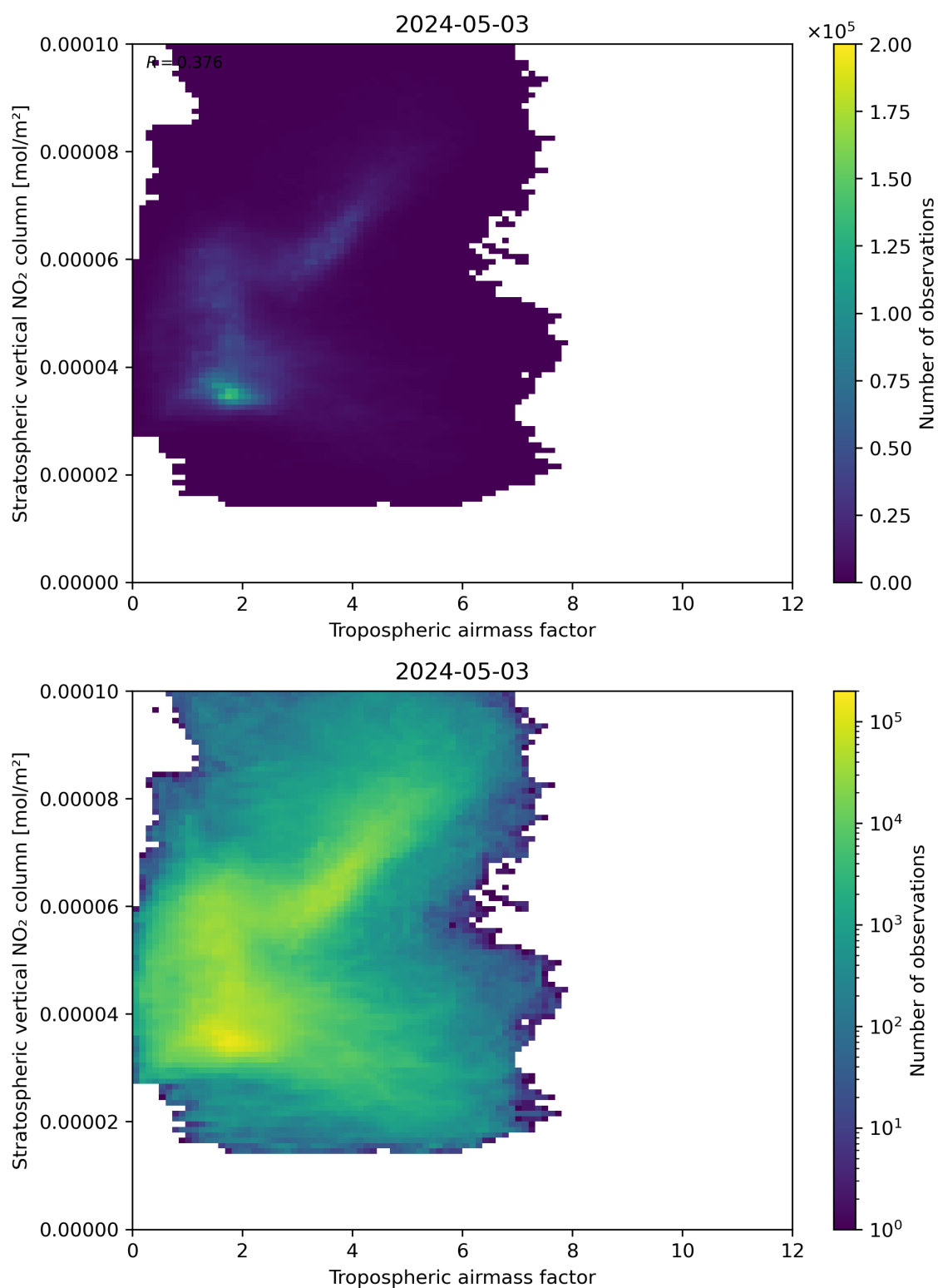
Figure 74: Scatter density plot of “Tropospheric air mass factor” against “Stratospheric vertical NO 2 column” for 2024-05-02 to 2024-05-04.
