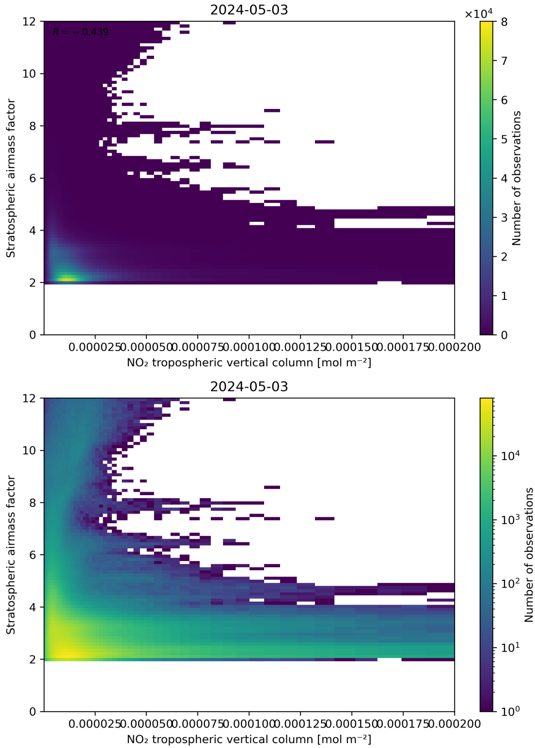
Figure 121: Scatter density plot of “NO 2 tropospheric vertical column” against “Stratospheric air mass factor” for 2024-05-02 to 2024-05-04.
