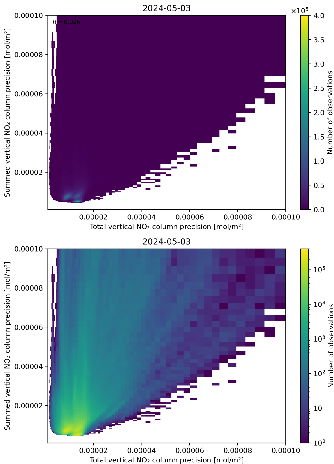
Figure 118: Scatter density plot of “Total vertical NO 2 column precision” against “Summed vertical NO 2 column precision” for 2024-05-02 to 2024-05-04.
