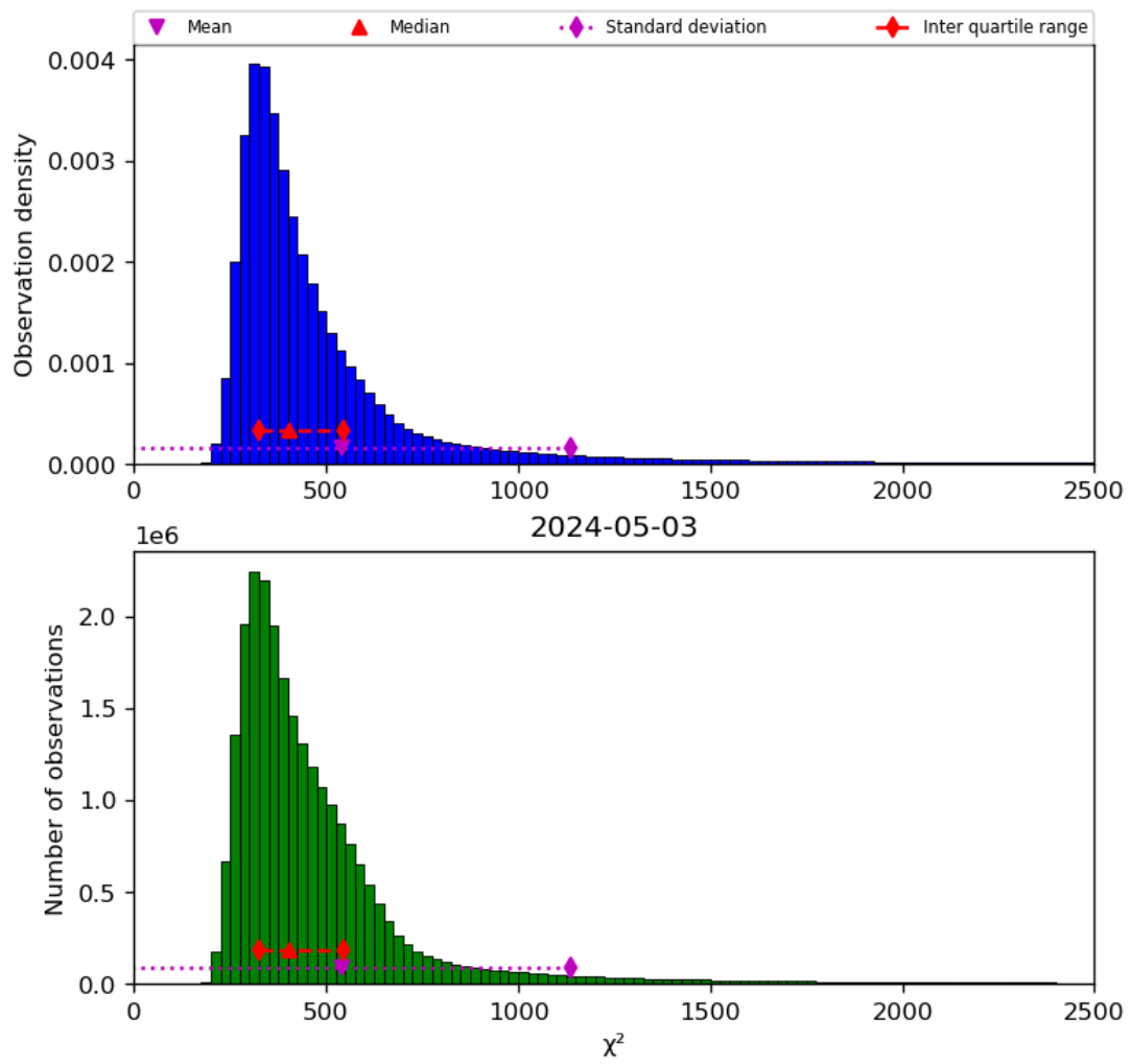
Figure 42: Histogram of “ \chi^2 ” for 2024-05-02 to 2024-05-04
