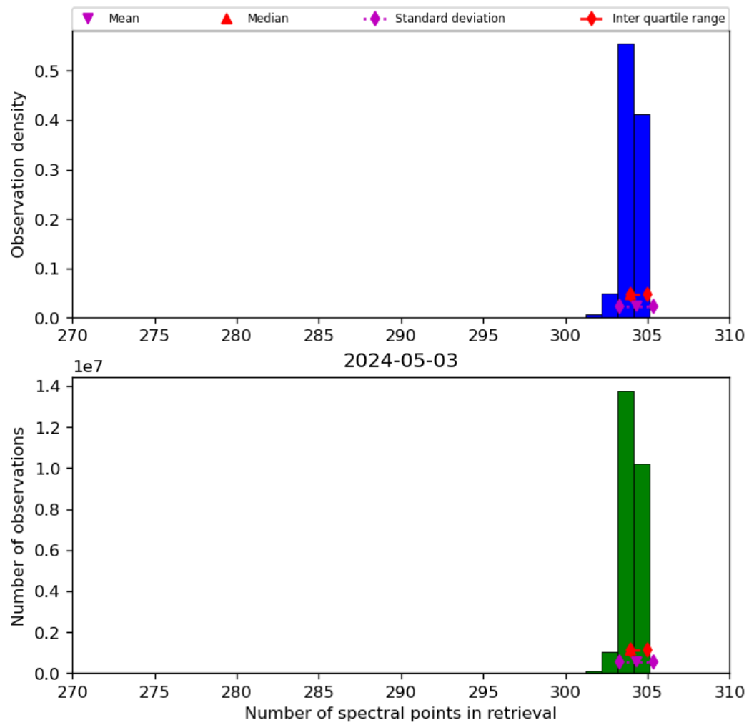
Figure 33: Histogram of “Number of spectral points in retrieval” for 2024-05-02 to 2024-05-04
