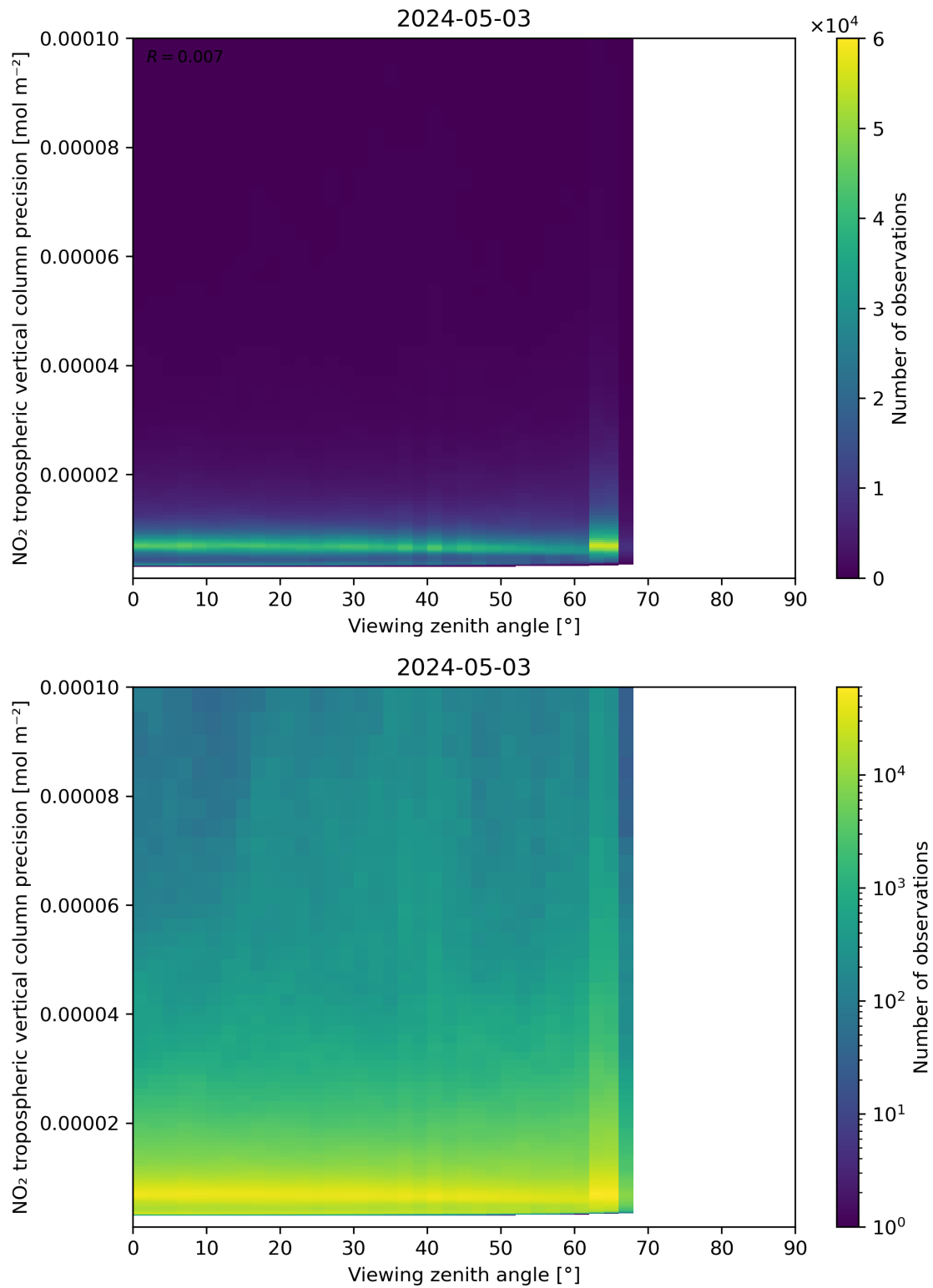
Figure 170: Scatter density plot of “Viewing zenith angle” against “NO 2 tropospheric vertical column precision” for 2024-05-02 to 2024-05-04.
