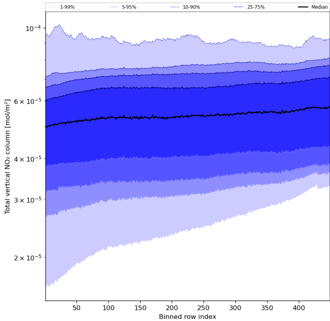
Figure 55: Along track statistics of “Total vertical NO 2 column” for 2024-05-02 to 2024-05-04
