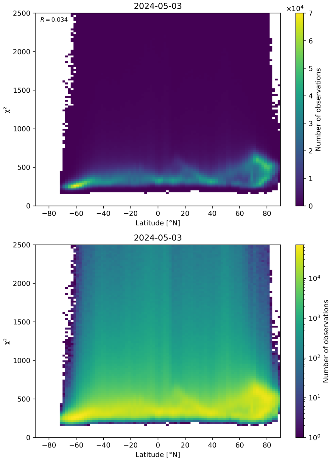
Figure 86: Scatter density plot of “Latitude” against “ \chi^2 ” for 2024-05-02 to 2024-05-04.
