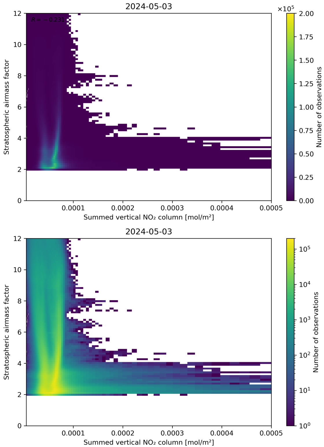
Figure 103: Scatter density plot of “Summed vertical NO 2 column” against “Stratospheric airmass factor” for 2024-05-02 to 2024-05-04.
