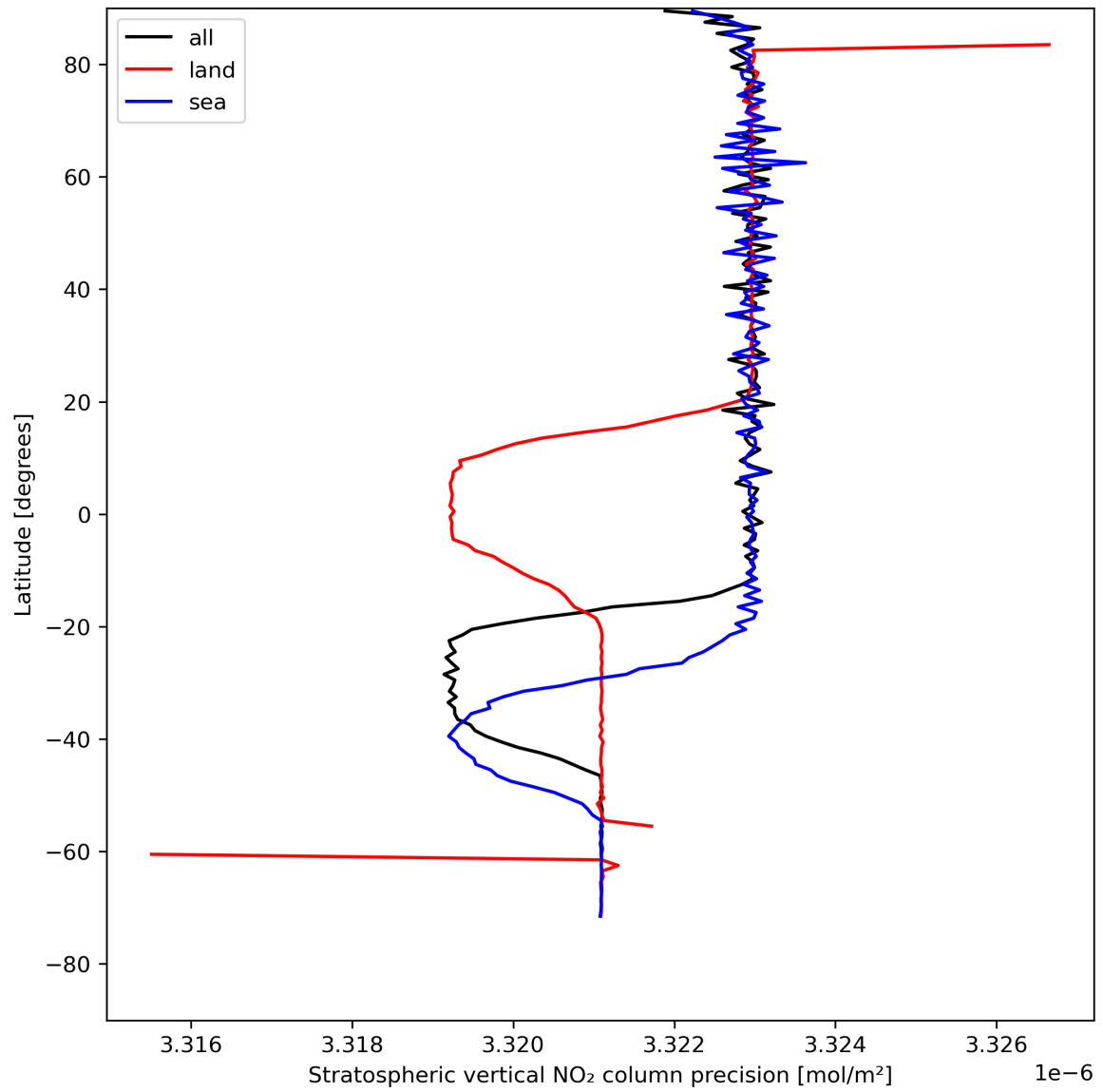
Figure 20: Zonal average of “Stratospheric vertical NO 2 column precision” for 2024-05-02 to 2024-05-04.
