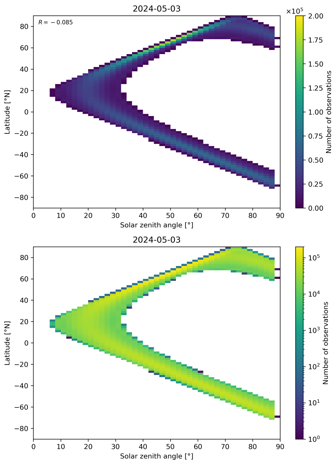
Figure 149: Scatter density plot of “Solar zenith angle” against “Latitude” for 2024-05-02 to 2024-05-04.
