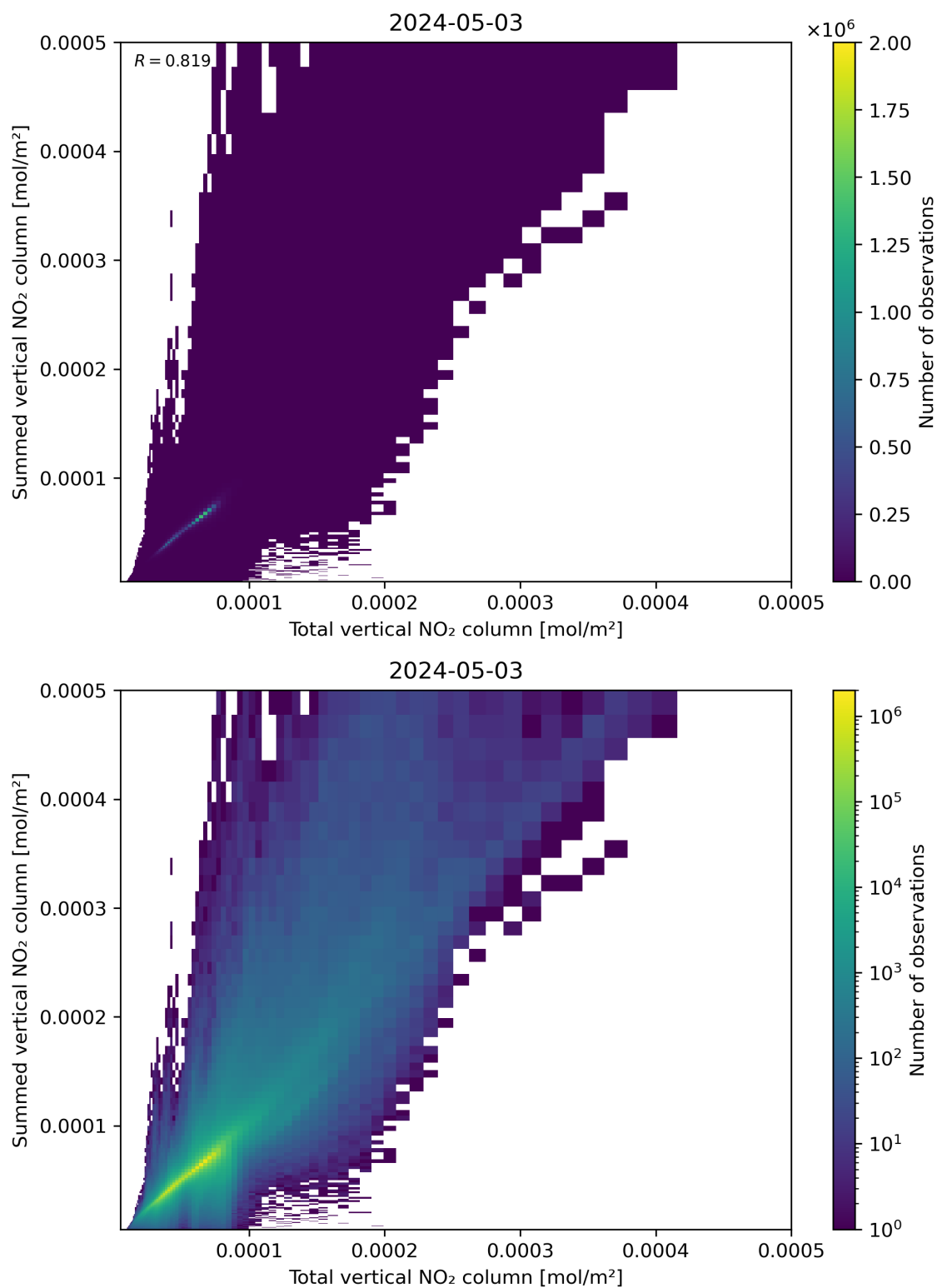
Figure 112: Scatter density plot of “Total vertical NO 2 column” against “Summed vertical NO 2 column” for 2024-05-02 to 2024-05-04.
