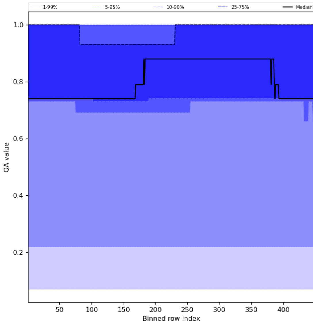
Figure 45: Along track statistics of “QA value” for 2024-05-02 to 2024-05-04
