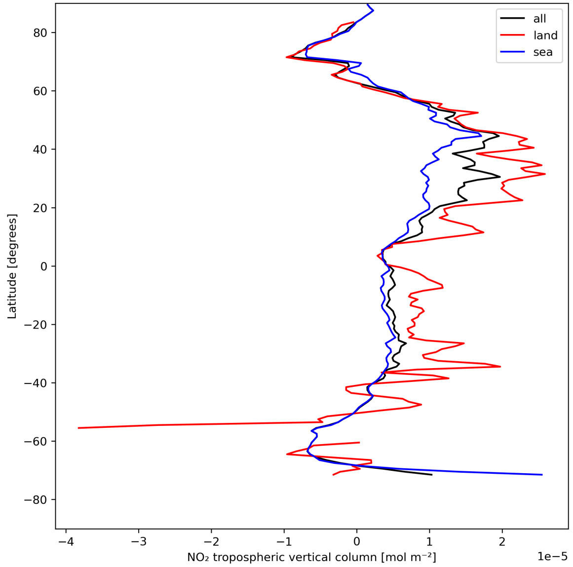
Figure 12: Zonal average of “NO 2 tropospheric vertical column” for 2024-05-02 to 2024-05-04.
