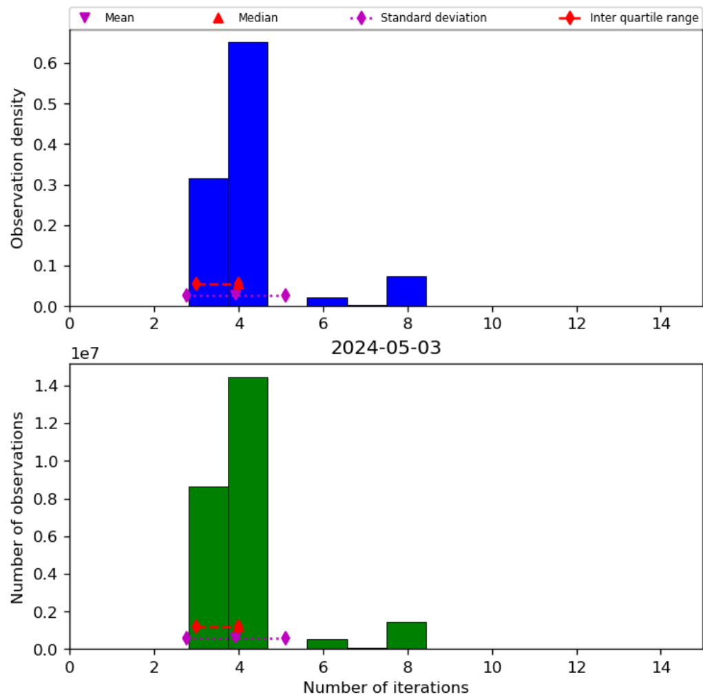
Figure 34: Histogram of "Number of iterations" for 2024-05-02 to 2024-05-04
