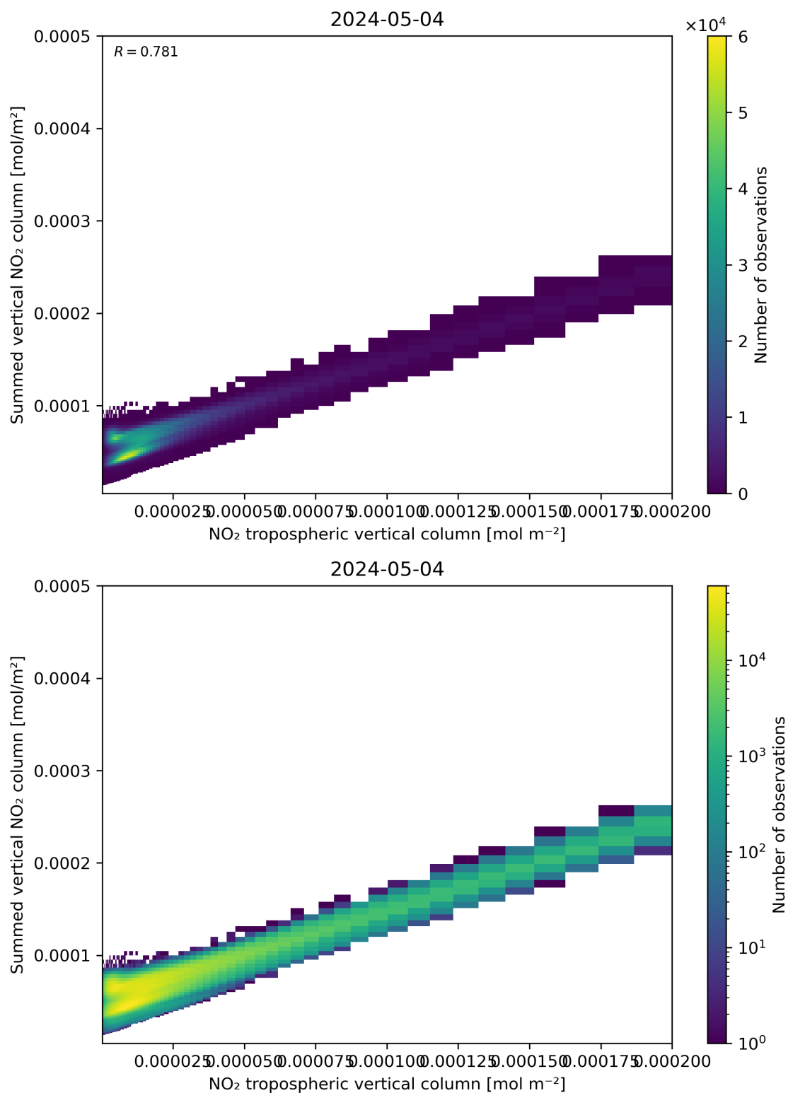
Figure 126: Scatter density plot of “NO 2 tropospheric vertical column” against “Summed vertical NO 2 column” for 2024-05-03 to 2024-05-05.
