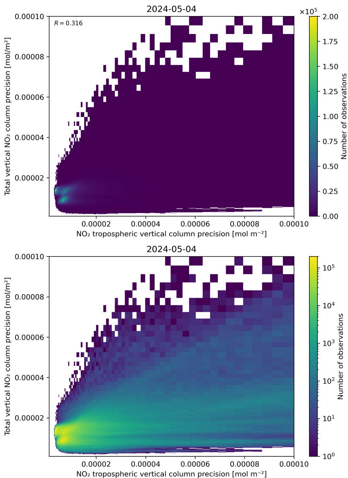
Figure 139: Scatter density plot of “NO 2 tropospheric vertical column precision” against “Total vertical NO 2 column precision” for 2024-05-03 to 2024-05-05.
