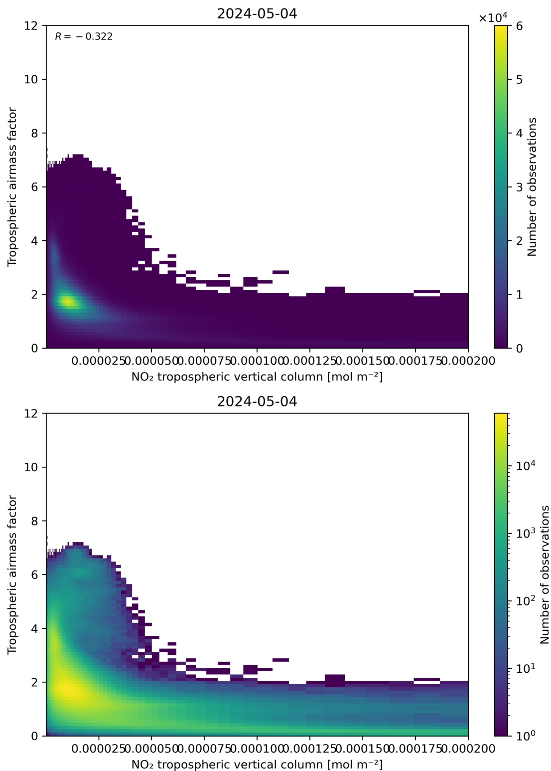
Figure 123: Scatter density plot of “NO 2 tropospheric vertical column” against “Tropospheric airmass factor” for 2024-05-03 to 2024-05-05.
