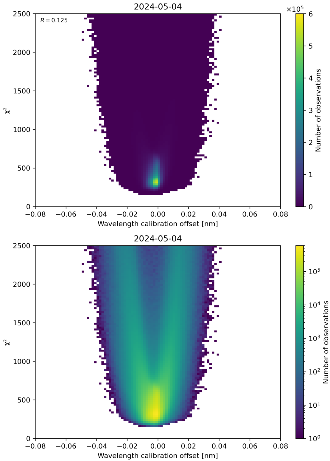
Figure 175: Scatter density plot of “Wavelength calibration offset” against “ \chi^2 ” for 2024-05-03 to 2024-05-05.
