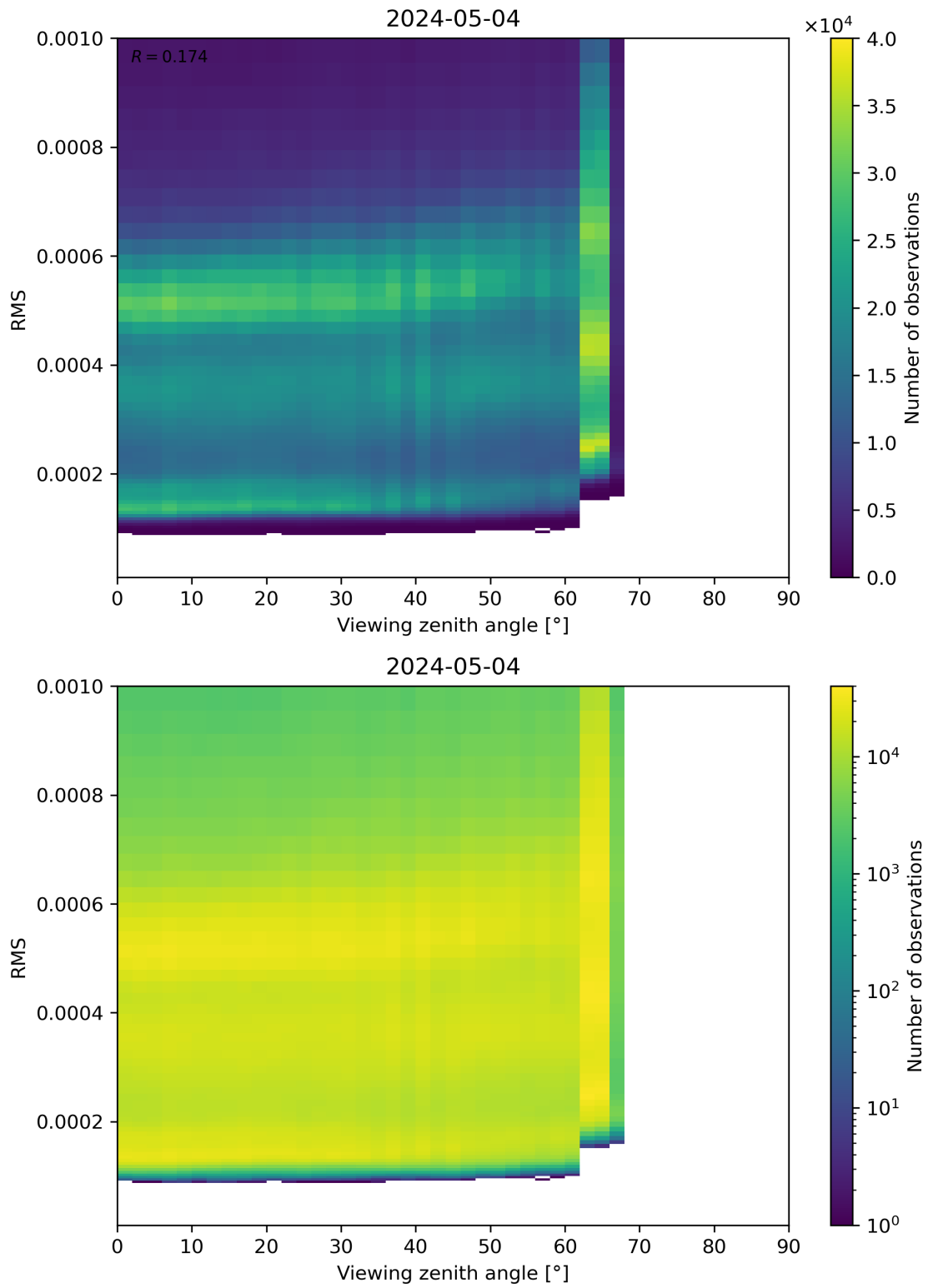
Figure 171: Scatter density plot of “Viewing zenith angle” against “RMS” for 2024-05-03 to 2024-05-05.
