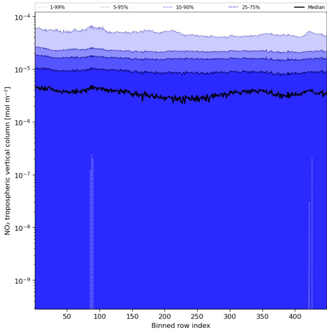
Figure 46: Along track statistics of “NO 2 tropospheric vertical column” for 2024-05-03 to 2024-05-05
