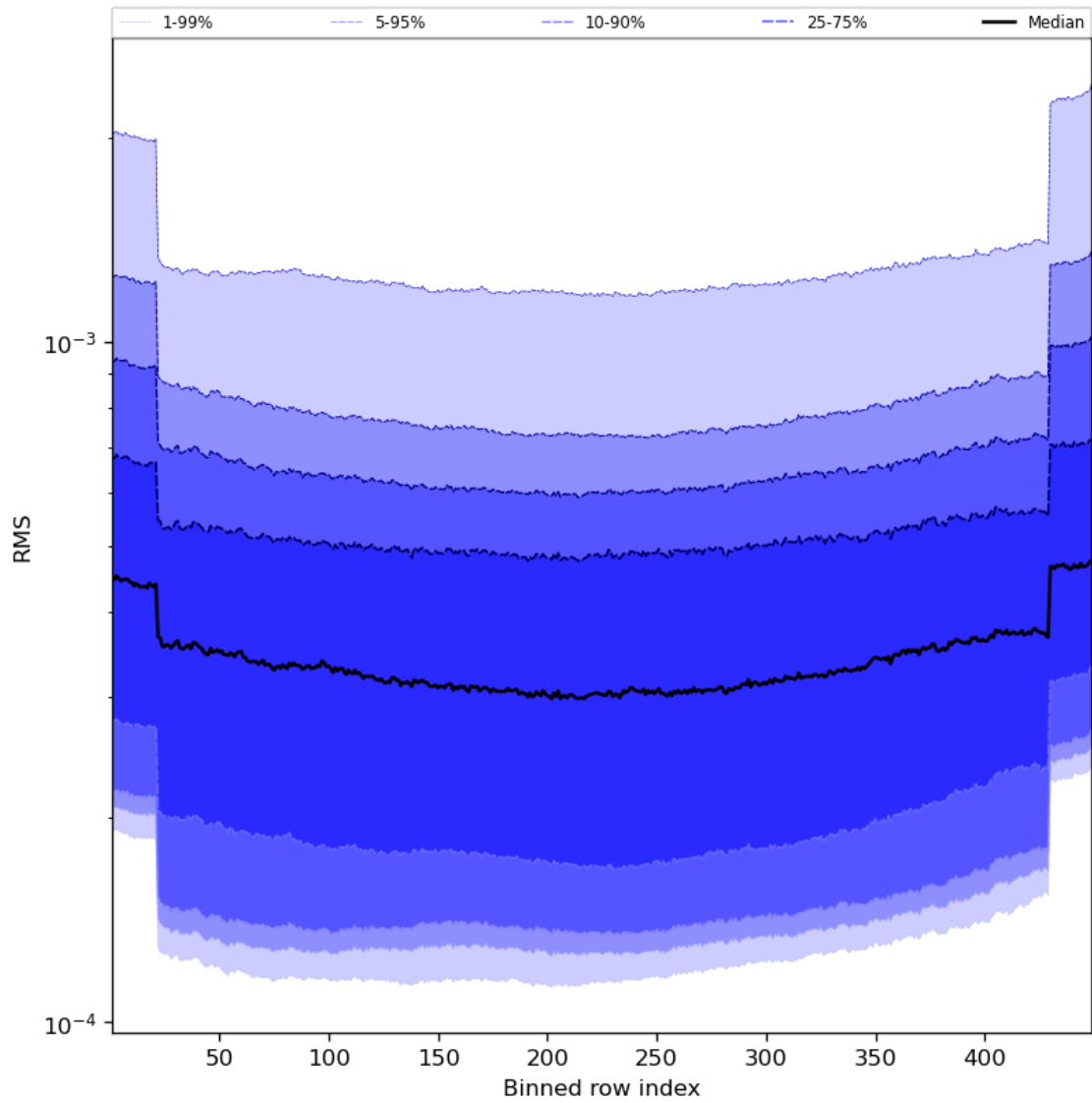
Figure 60: Along track statistics of “RMS” for 2024-05-03 to 2024-05-05
