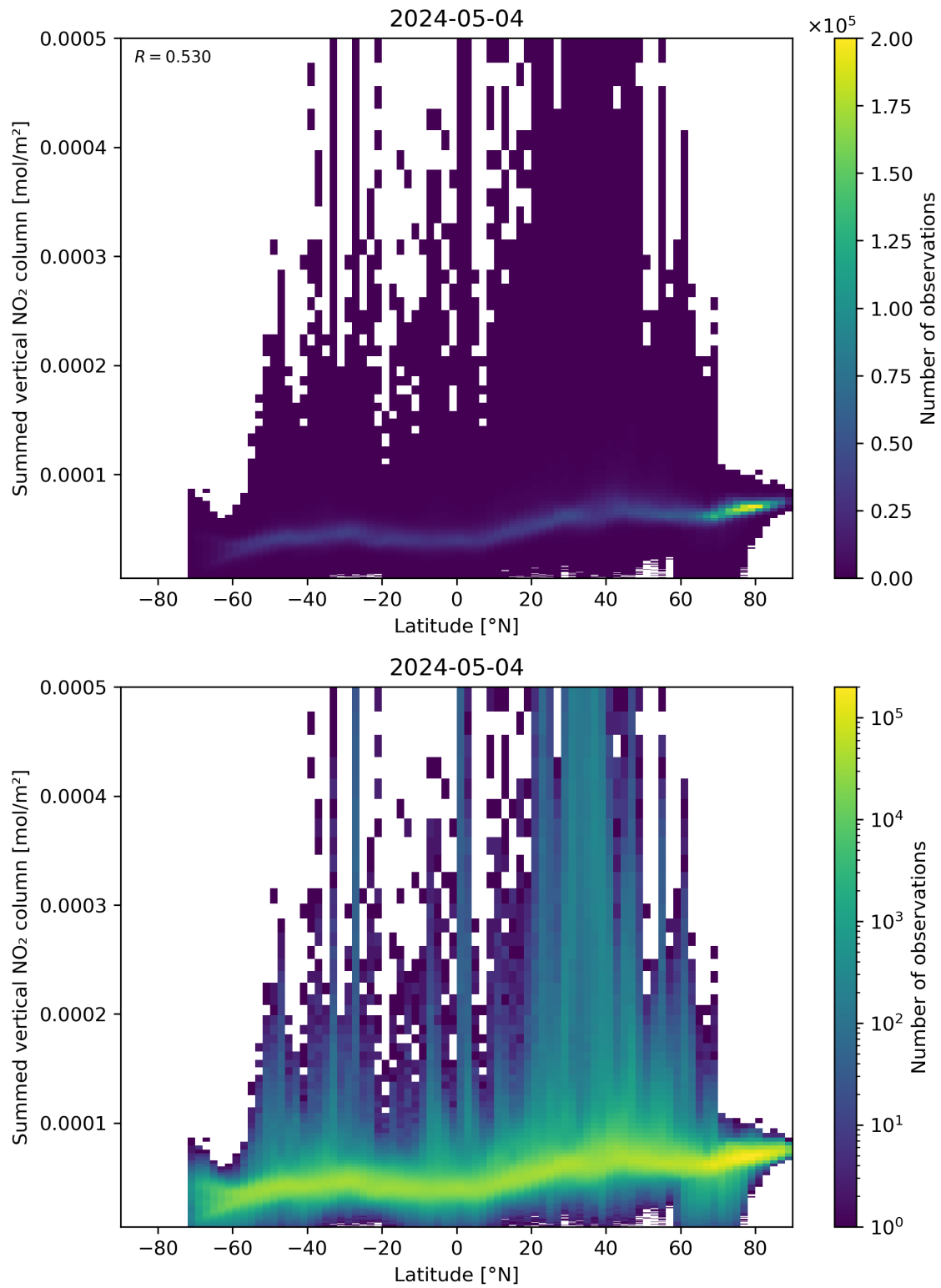
Figure 88: Scatter density plot of “Latitude” against “Summed vertical NO 2 column” for 2024-05-03 to 2024-05-05.
