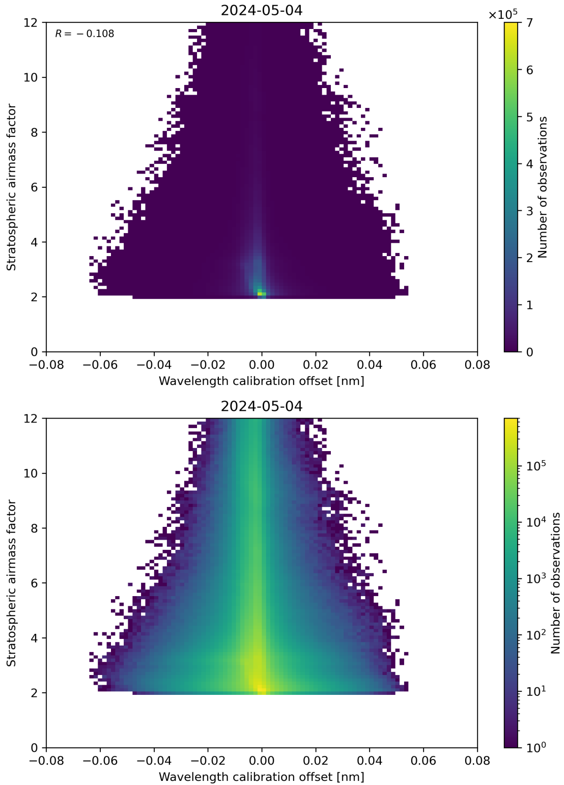
Figure 174: Scatter density plot of “Wavelength calibration offset” against “Stratospheric airmass factor” for 2024-05-03 to 2024-05-05.
