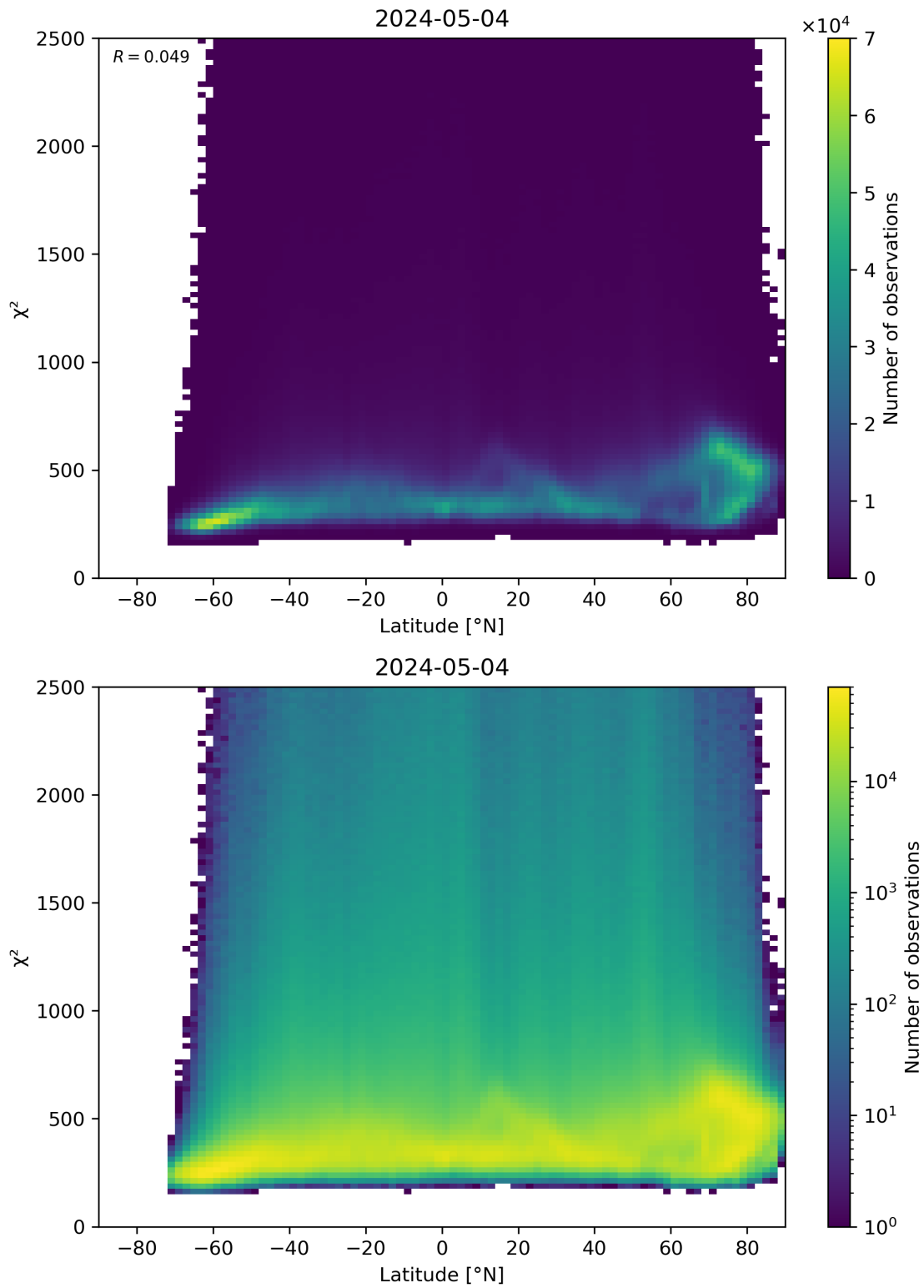
Figure 86: Scatter density plot of “Latitude” against “ \chi^2 ” for 2024-05-03 to 2024-05-05.
