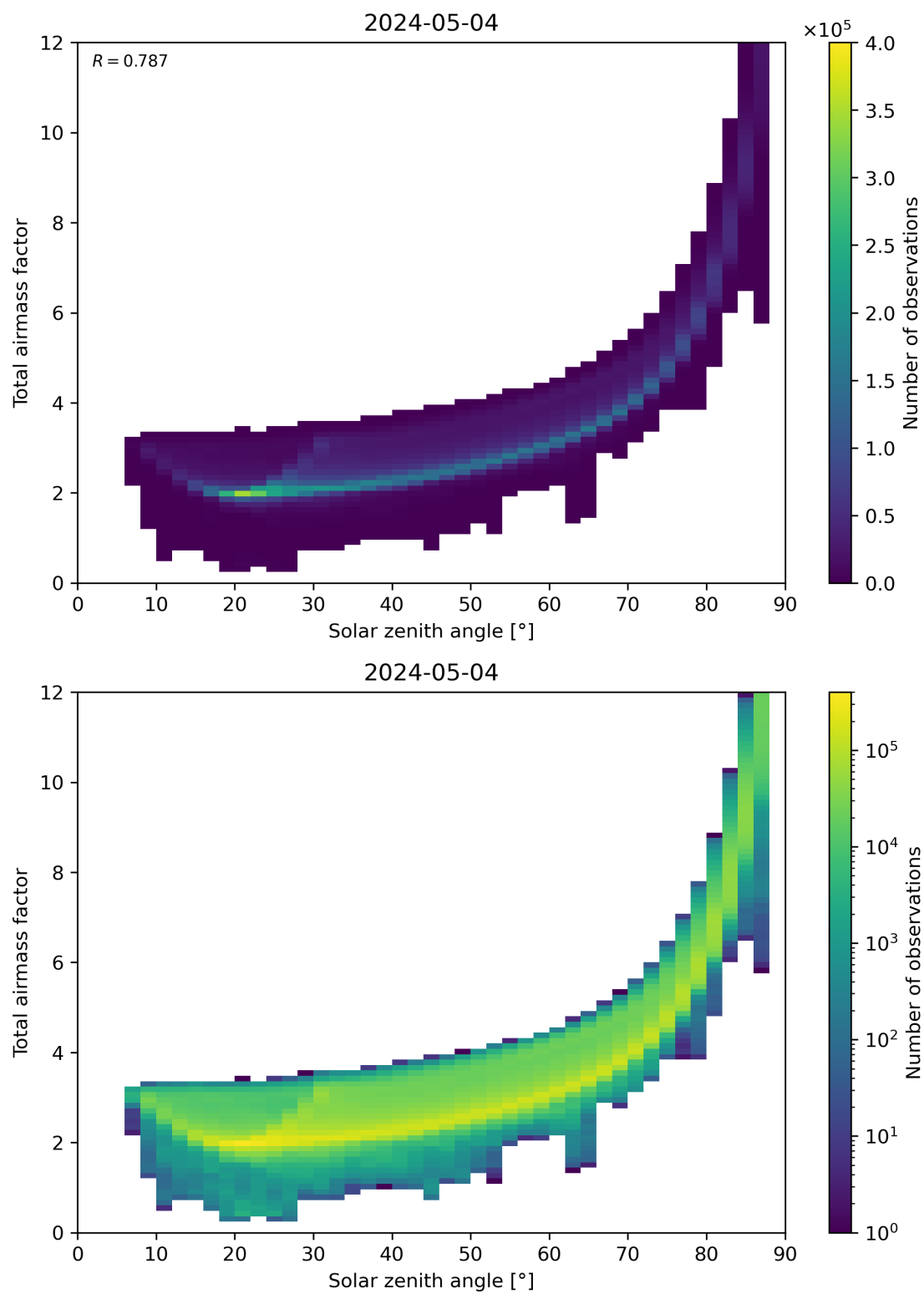
Figure 146: Scatter density plot of “Solar zenith angle” against “Total airmass factor” for 2024-05-03 to 2024-05-05.
