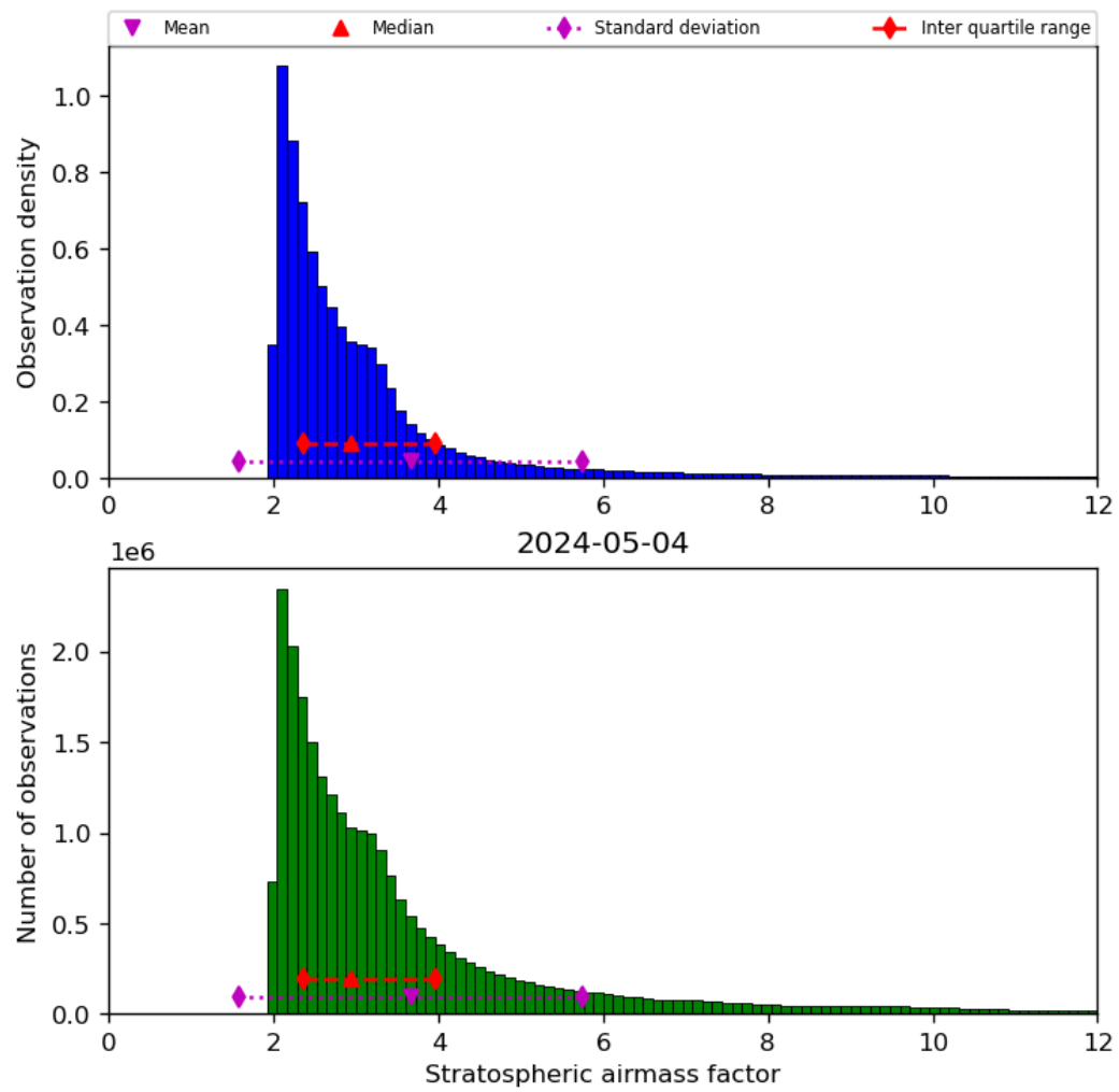
Figure 44: Histogram of “Stratospheric airmass factor” for 2024-05-03 to 2024-05-05
