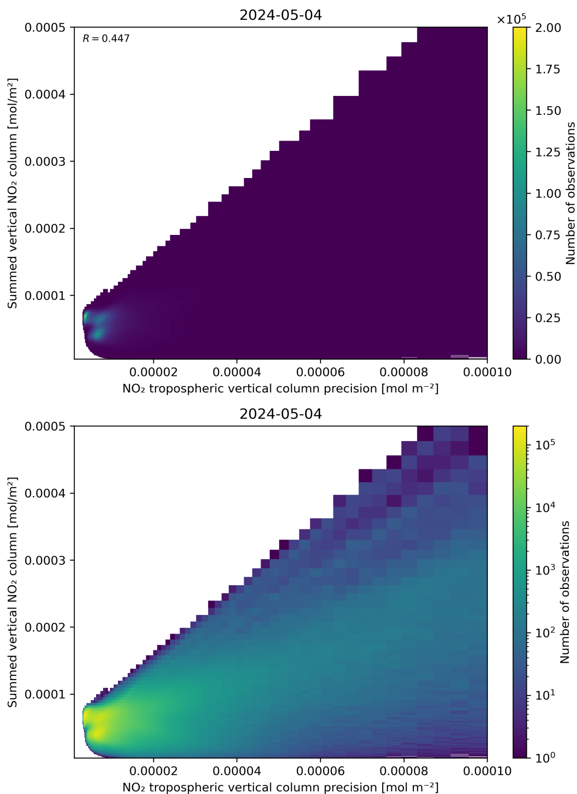
Figure 136: Scatter density plot of “NO 2 tropospheric vertical column precision” against “Summed vertical NO 2 column” for 2024-05-03 to 2024-05-05.
