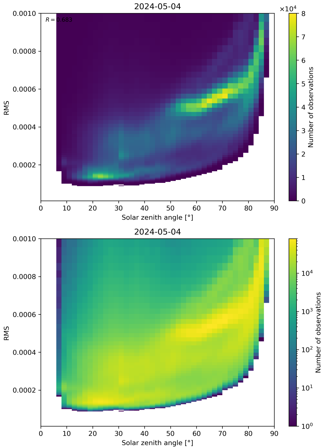
Figure 157: Scatter density plot of “Solar zenith angle” against “RMS” for 2024-05-03 to 2024-05-05.
