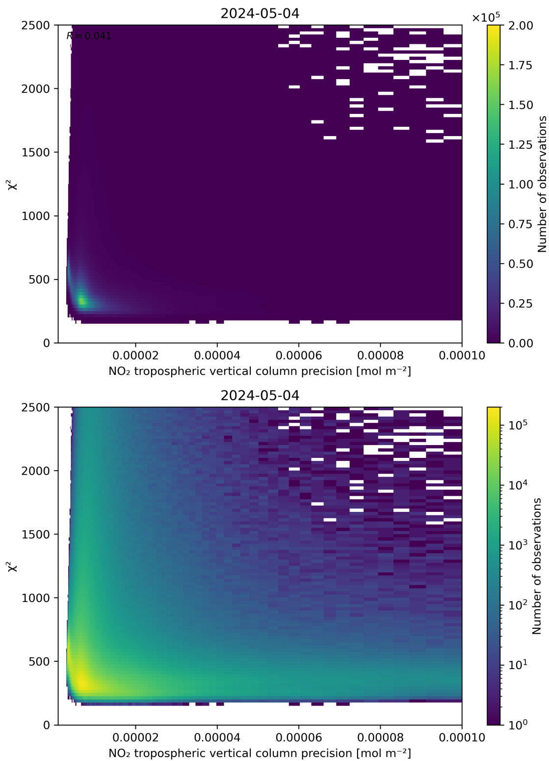
Figure 134: Scatter density plot of “NO 2 tropospheric vertical column precision” against “ \chi^2 ” for 2024-05-03 to 2024-05-05.
