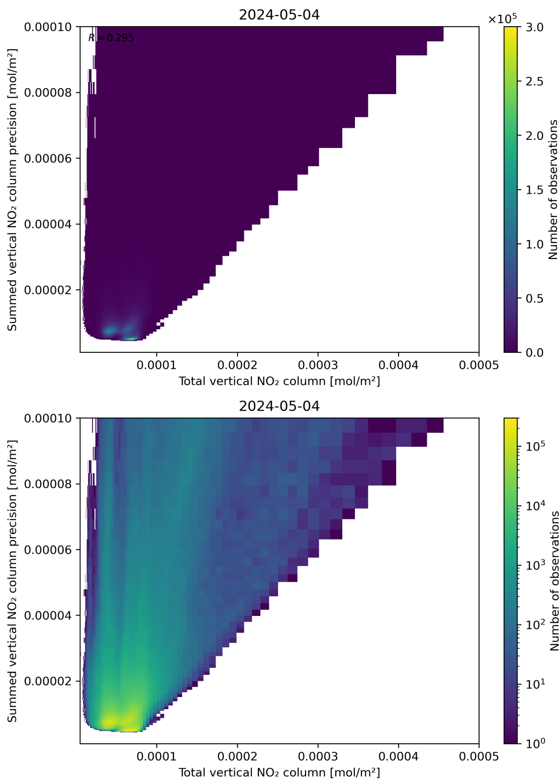
Figure 113: Scatter density plot of “Total vertical NO 2 column” against “Summed vertical NO 2 column precision” for 2024-05-03 to 2024-05-05.
