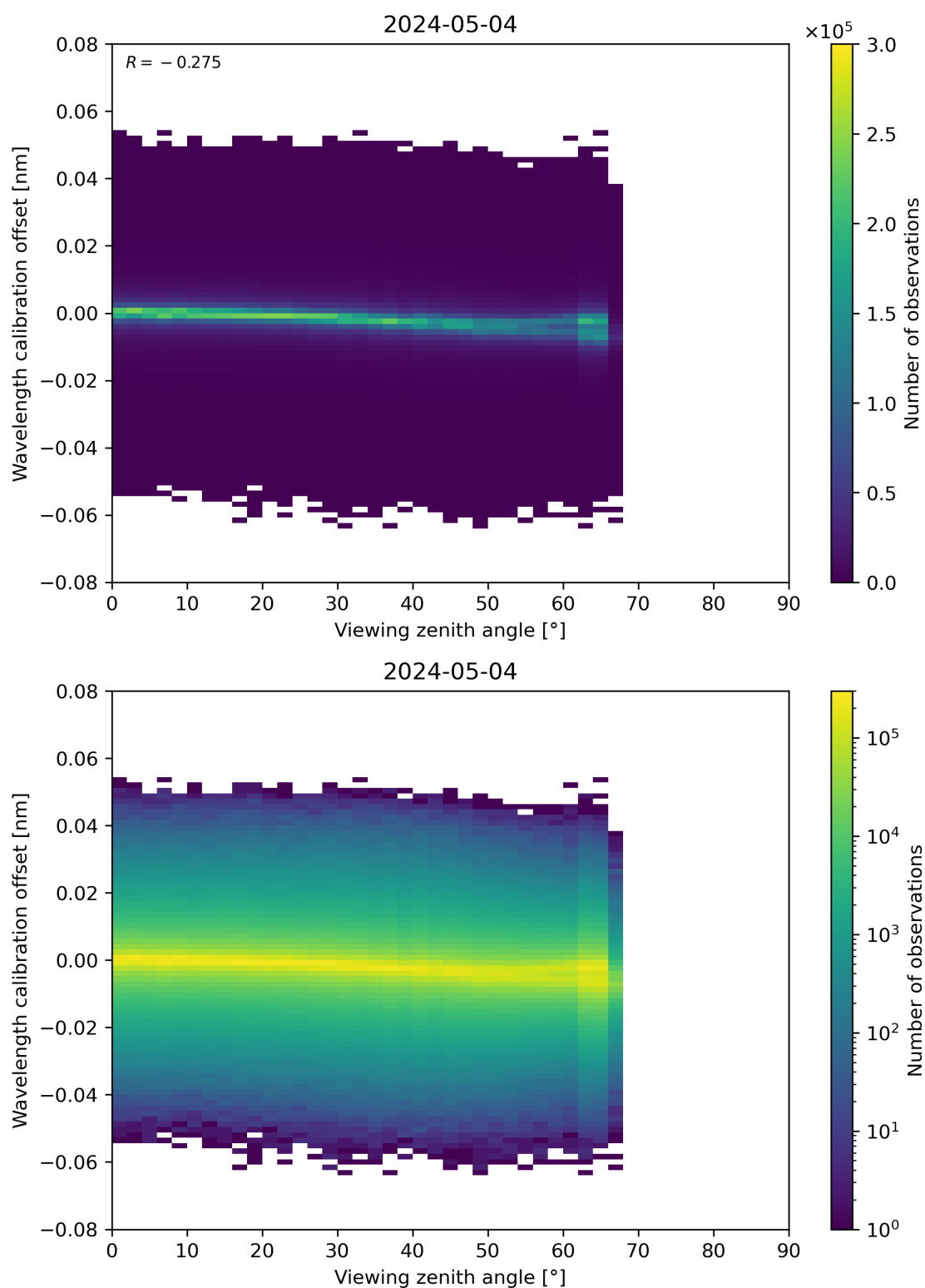
Figure 173: Scatter density plot of “Viewing zenith angle” against “Wavelength calibration offset” for 2024-05-03 to 2024-05-05.
