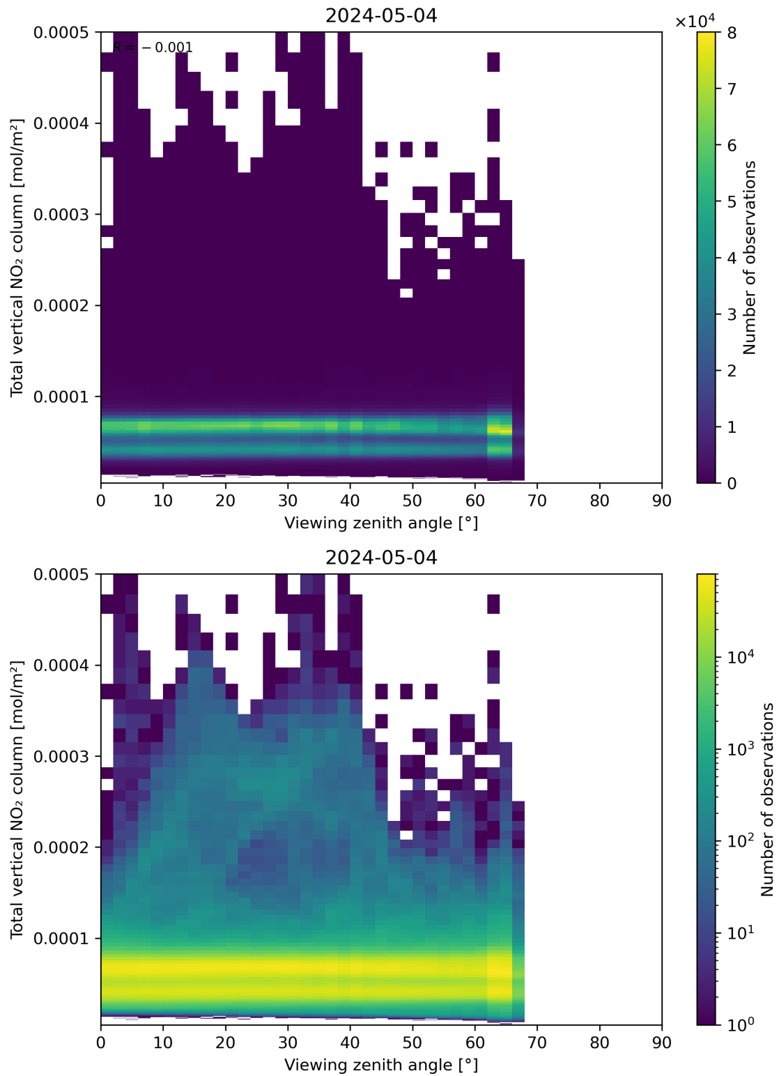
Figure 167: Scatter density plot of “Viewing zenith angle” against “Total vertical NO 2 column” for 2024-05-03 to 2024-05-05.
