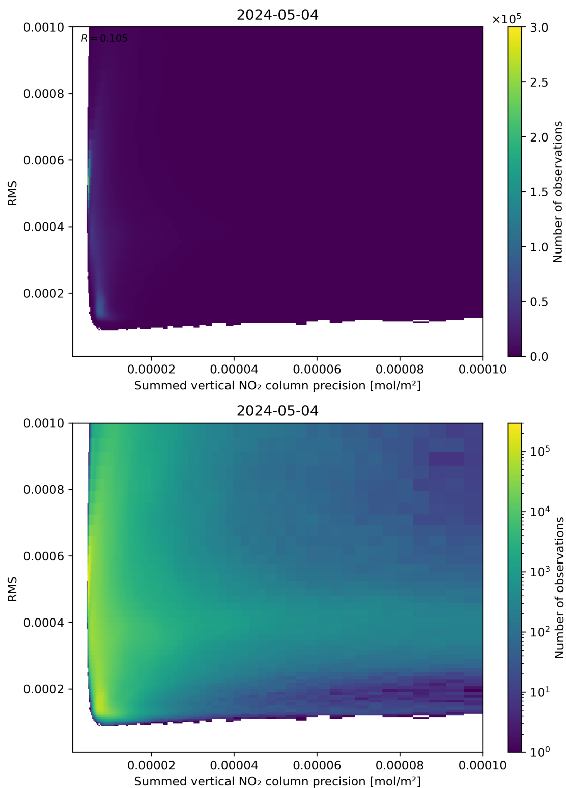
Figure 108: Scatter density plot of “Summed vertical NO 2 column precision” against “RMS” for 2024-05-03 to 2024-05-05.
