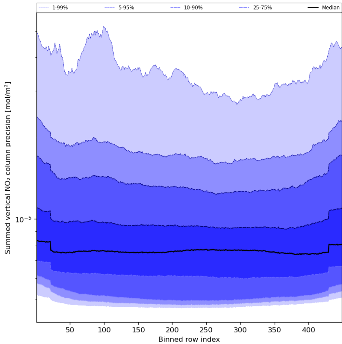
Figure 58: Along track statistics of “Summed vertical NO 2 column precision” for 2024-05-03 to 2024-05-05
