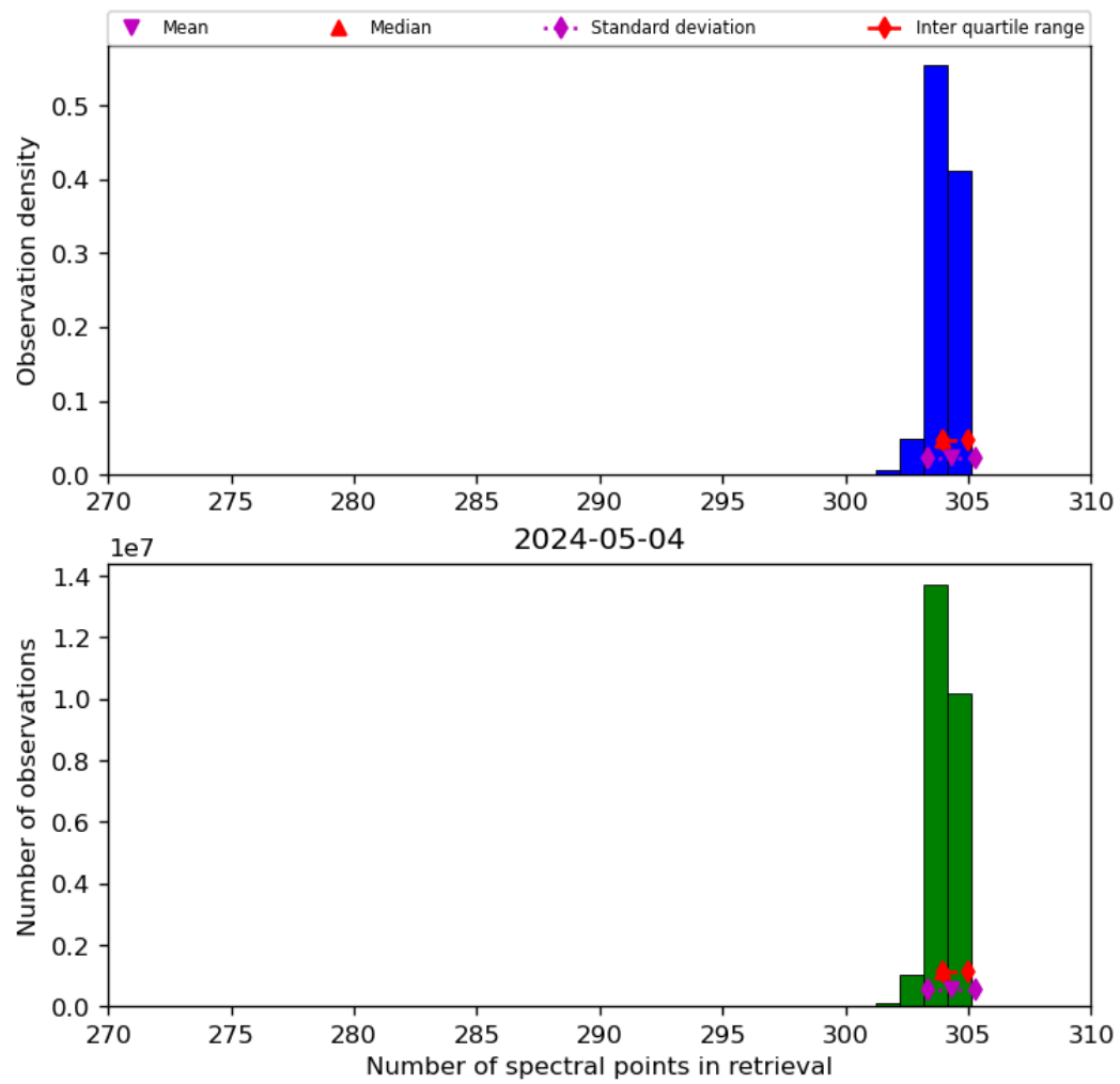
Figure 33: Histogram of “Number of spectral points in retrieval” for 2024-05-03 to 2024-05-05
