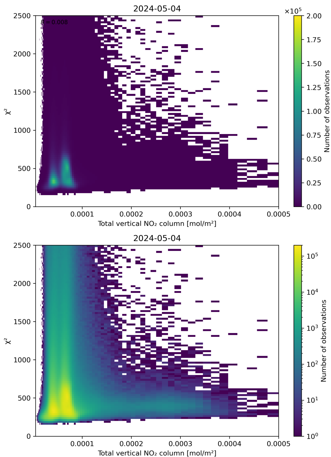
Figure 111: Scatter density plot of “Total vertical NO 2 column” against “ \chi^2 ” for 2024-05-03 to 2024-05-05.
