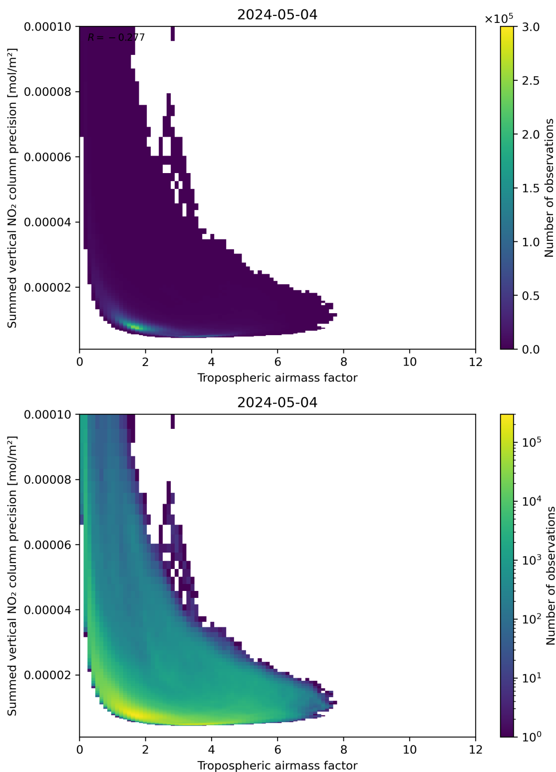
Figure 76: Scatter density plot of “Tropospheric air mass factor” against “Summed vertical NO 2 column precision” for 2024-05-03 to 2024-05-05.
