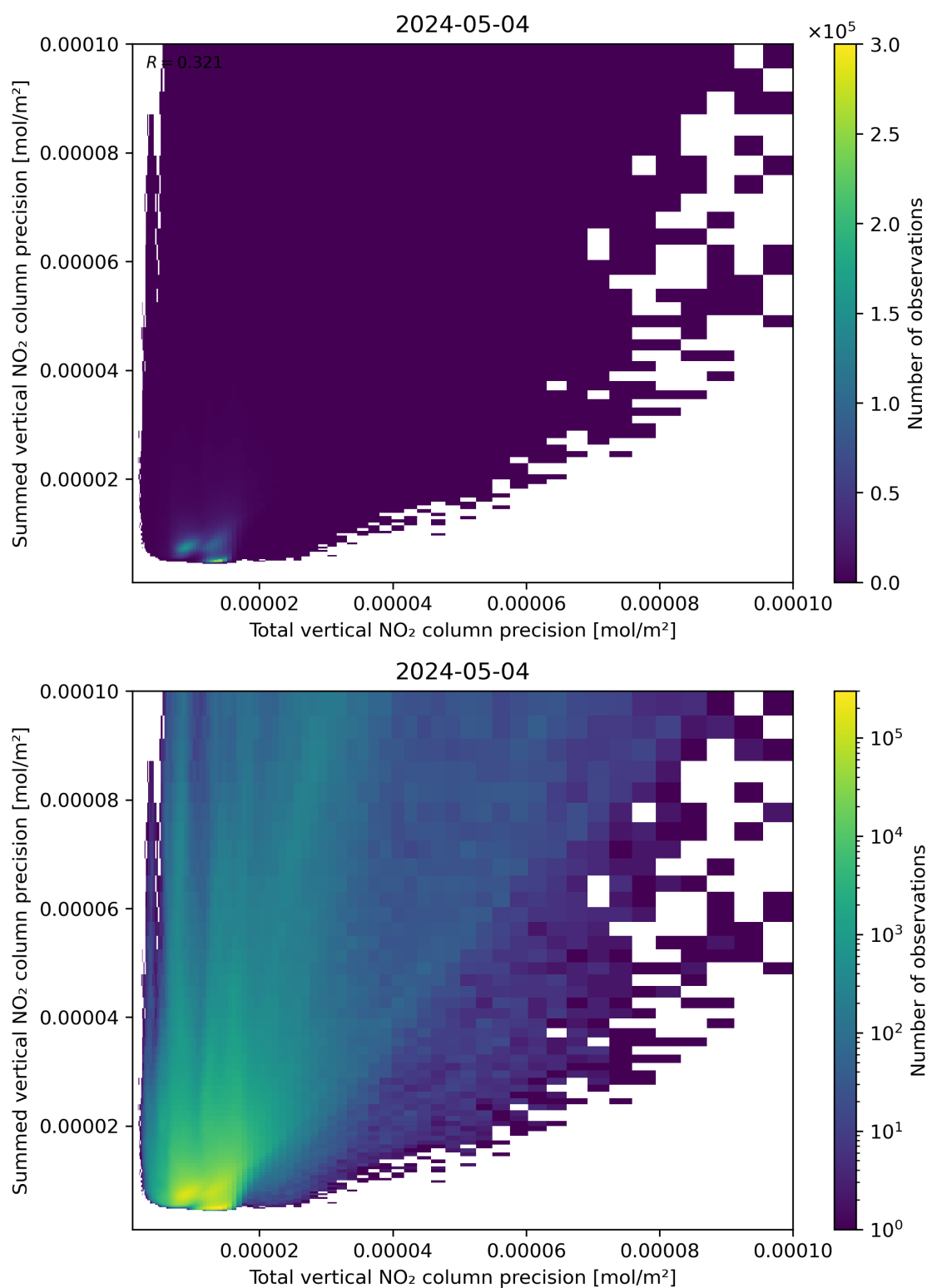
Figure 118: Scatter density plot of “Total vertical NO 2 column precision” against “Summed vertical NO 2 column precision” for 2024-05-03 to 2024-05-05.
