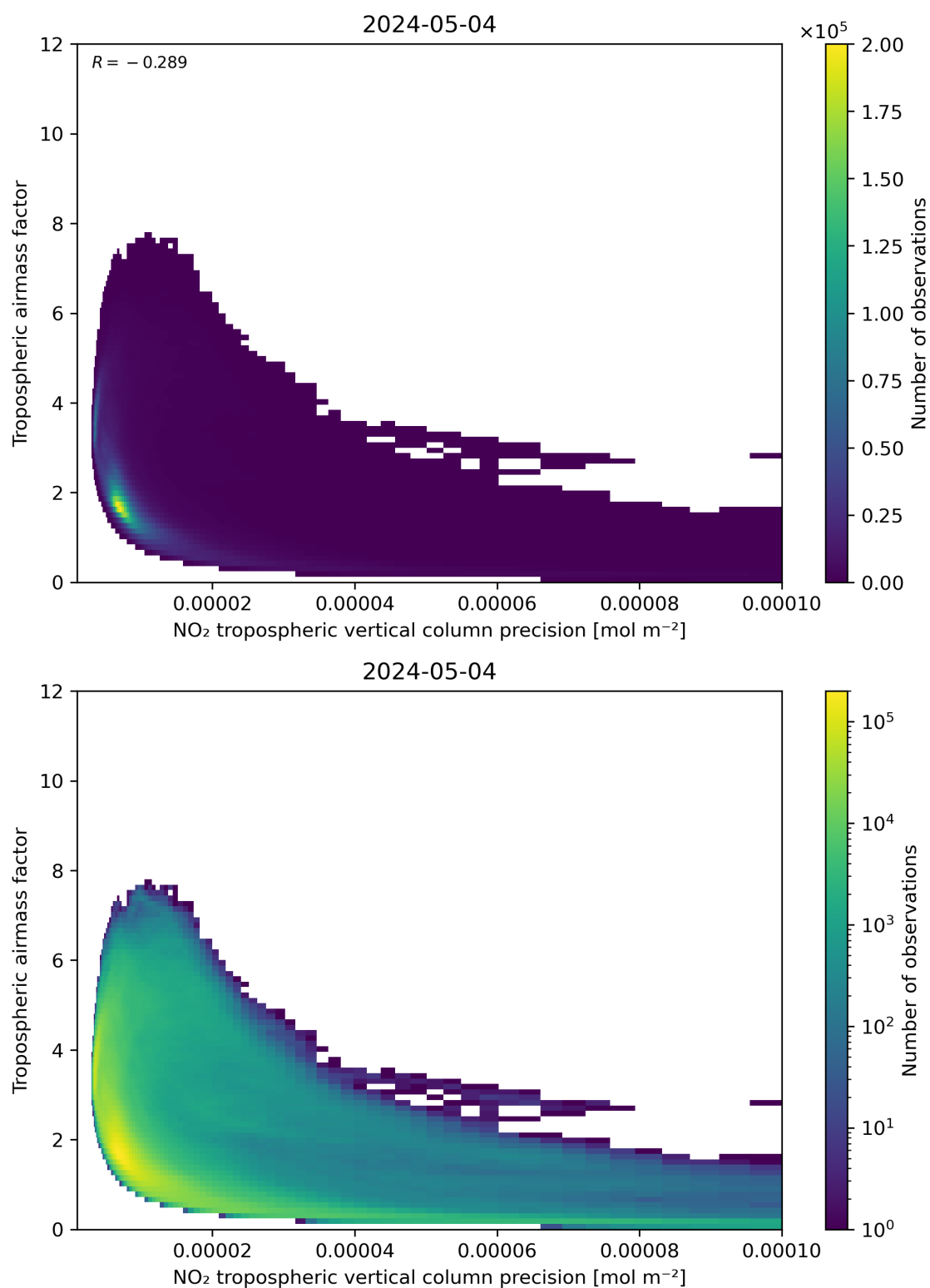
Figure 133: Scatter density plot of “NO 2 tropospheric vertical column precision” against “Tropospheric air mass factor” for 2024-05-03 to 2024-05-05.
