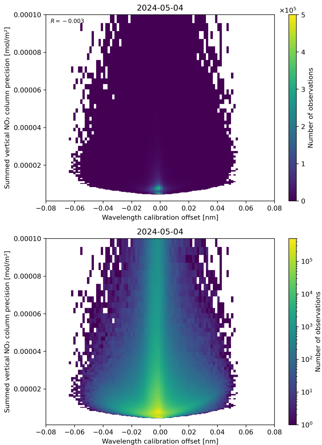
Figure 178: Scatter density plot of “Wavelength calibration offset” against “Summed vertical NO 2 column precision” for 2024-05-03 to 2024-05-05.
