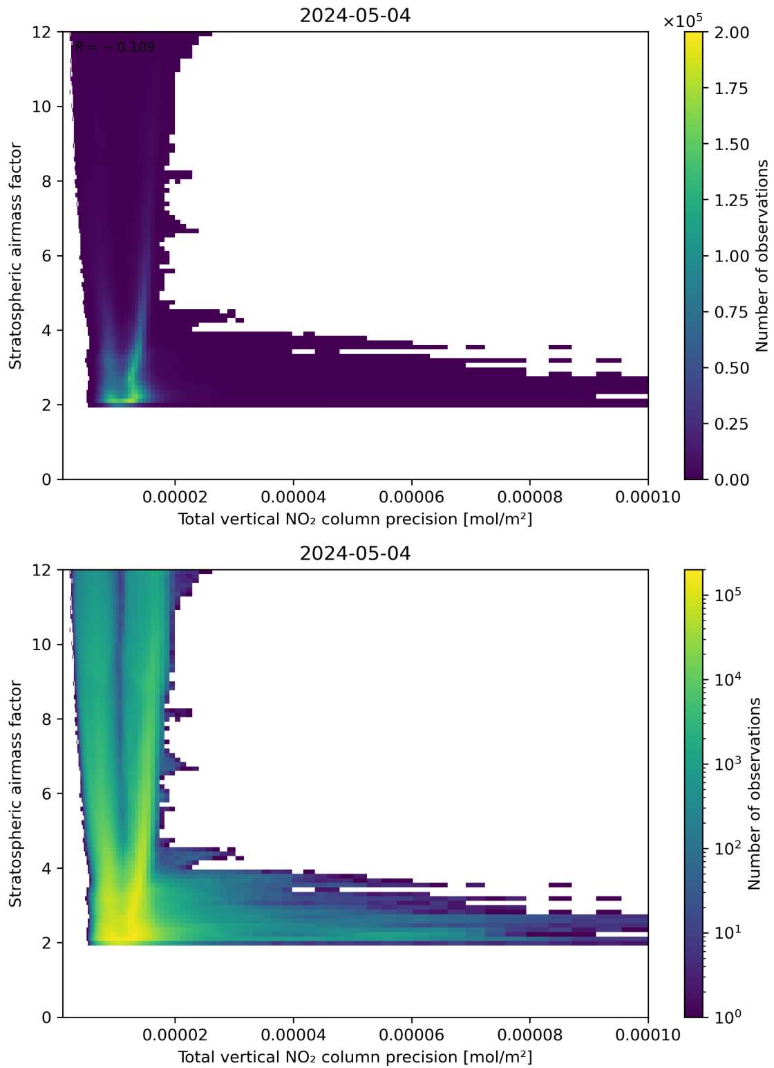
Figure 115: Scatter density plot of “Total vertical NO 2 column precision” against “Stratospheric air mass factor” for 2024-05-03 to 2024-05-05.
