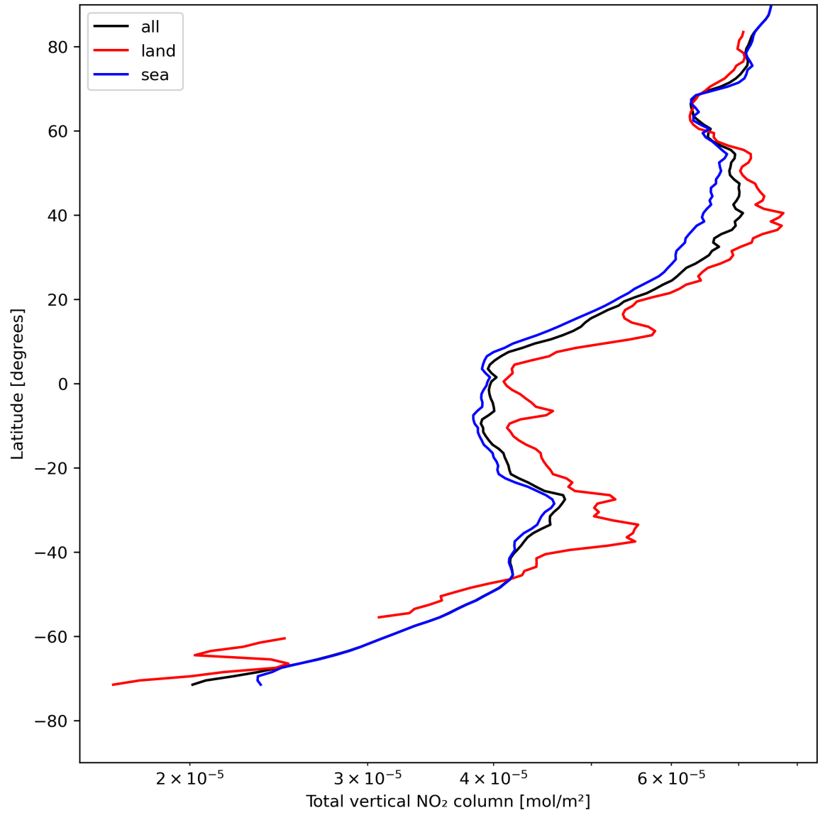
Figure 21: Zonal average of “Total vertical NO 2 column” for 2024-05-03 to 2024-05-05.
