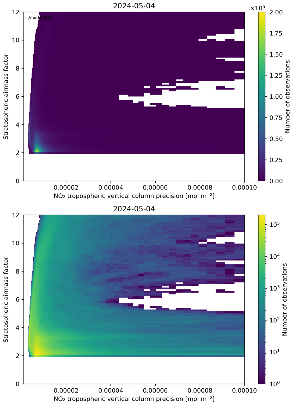
Figure 131: Scatter density plot of “NO 2 tropospheric vertical column precision” against “Stratospheric airmass factor” for 2024-05-03 to 2024-05-05.
