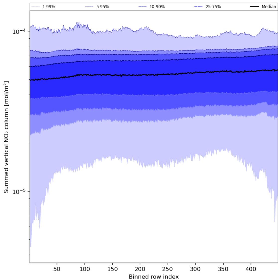
Figure 57: Along track statistics of “Summed vertical NO 2 column” for 2024-05-03 to 2024-05-05
