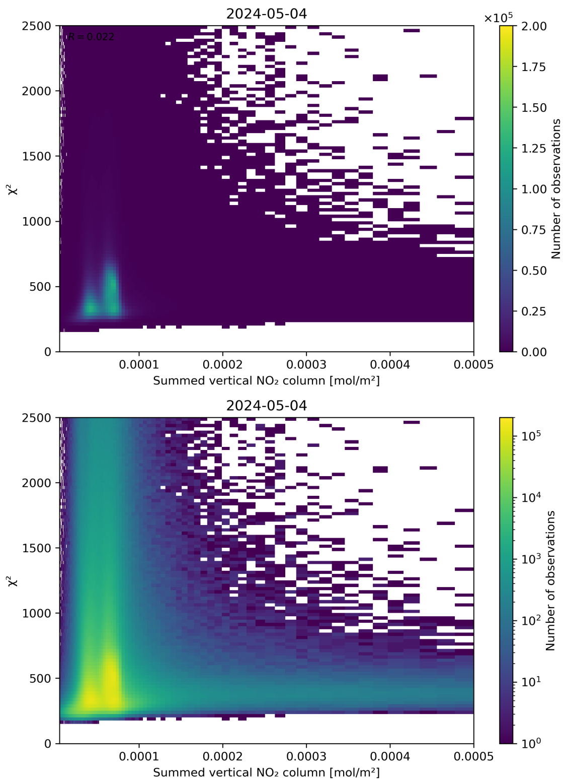
Figure 104: Scatter density plot of “Summed vertical NO 2 column” against “ \chi^2 ” for 2024-05-03 to 2024-05-05.
