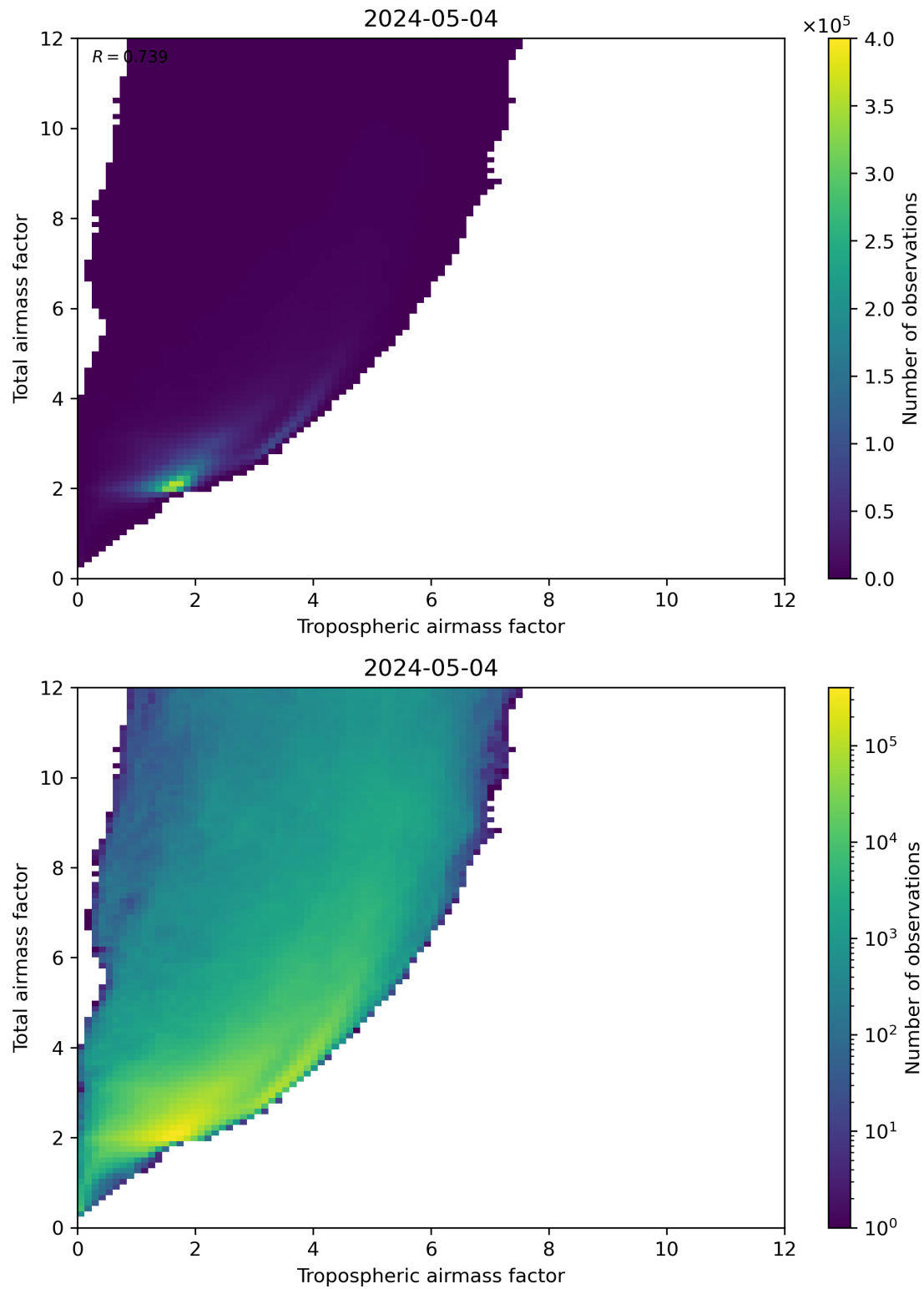
Figure 72: Scatter density plot of “Tropospheric airmass factor” against “Total airmass factor” for 2024-05-03 to 2024-05-05.
