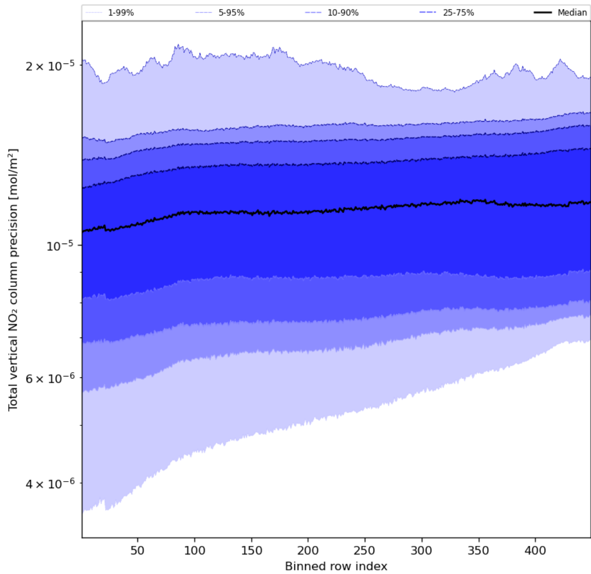
Figure 56: Along track statistics of “Total vertical NO 2 column precision” for 2024-05-03 to 2024-05-05
