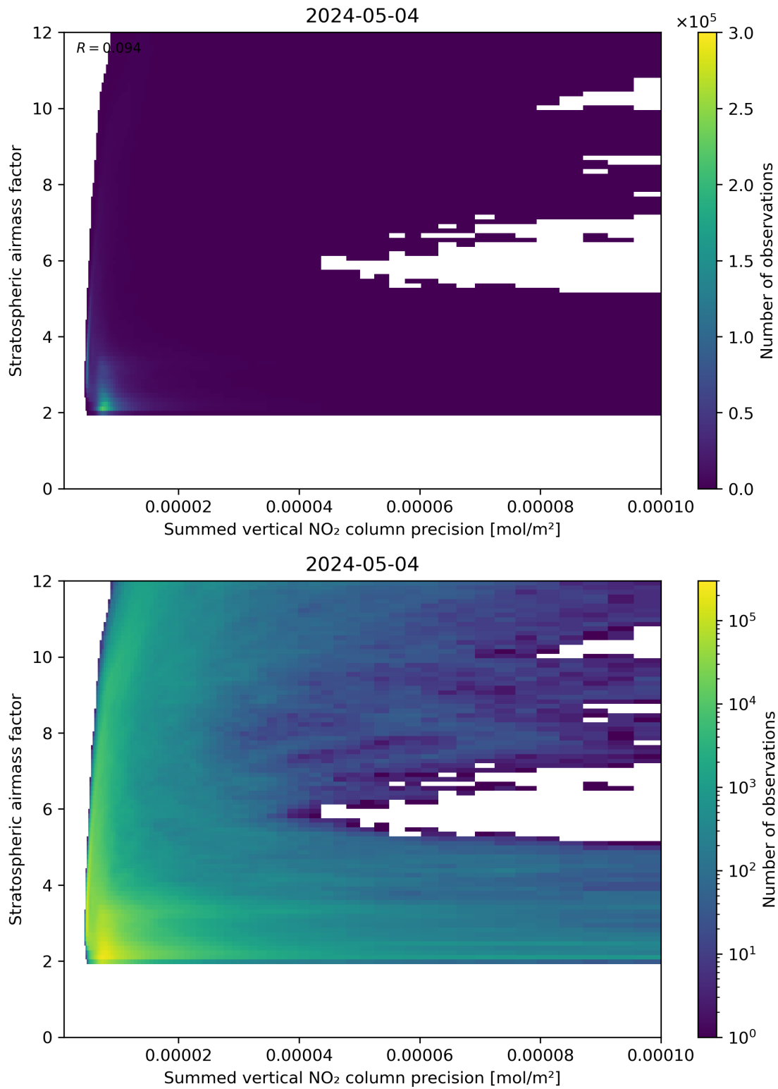
Figure 106: Scatter density plot of “Summed vertical NO 2 column precision” against “Stratospheric airmass factor” for 2024-05-03 to 2024-05-05.
