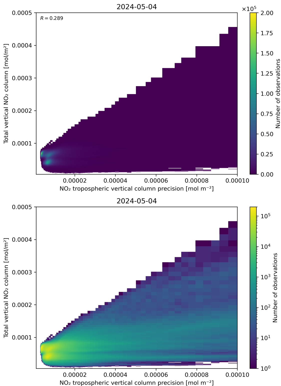
Figure 138: Scatter density plot of “NO 2 tropospheric vertical column precision” against “Total vertical NO 2 column” for 2024-05-03 to 2024-05-05.
