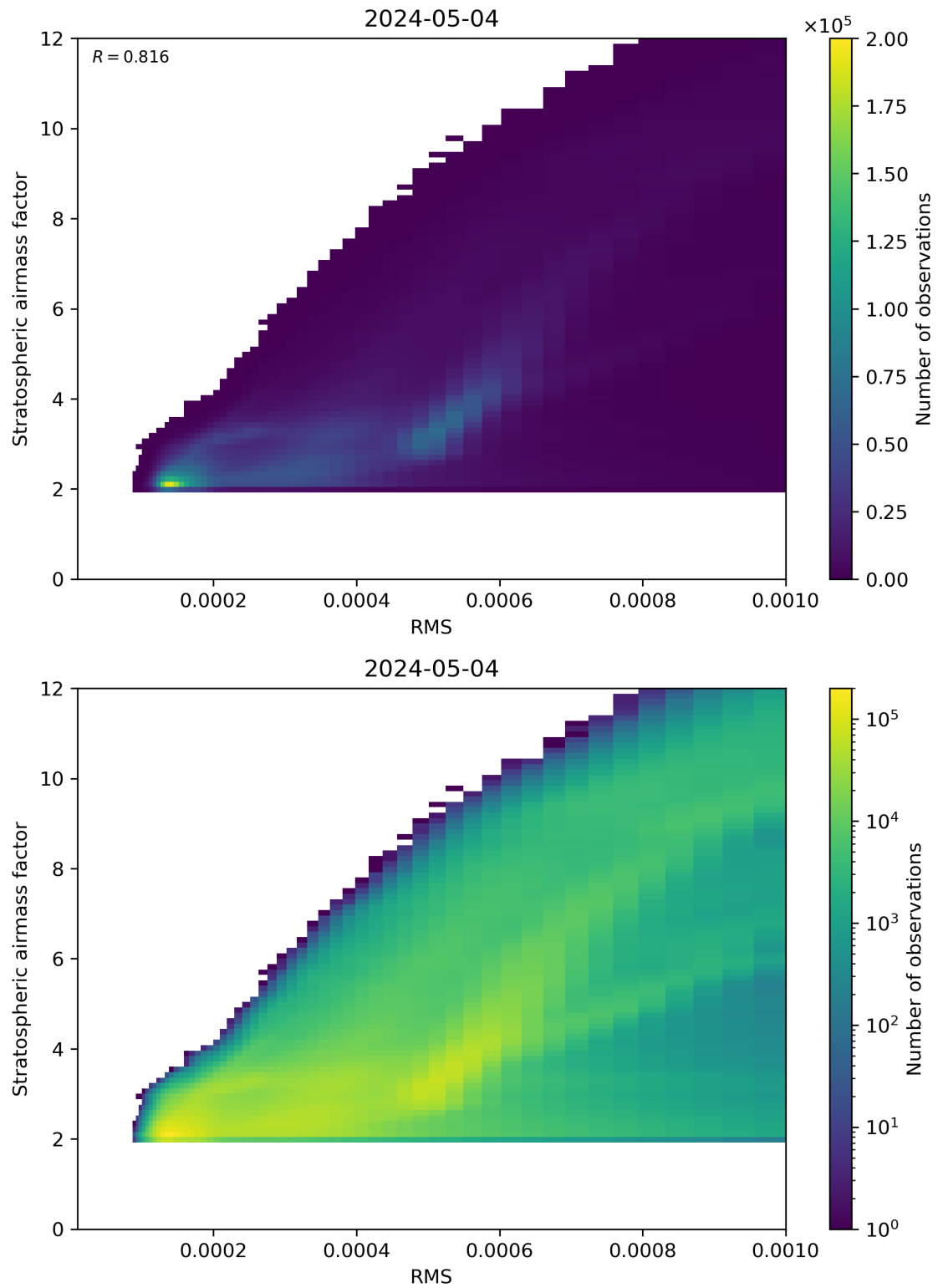
Figure 144: Scatter density plot of “RMS” against “Stratospheric airmass factor” for 2024-05-03 to 2024-05-05.
