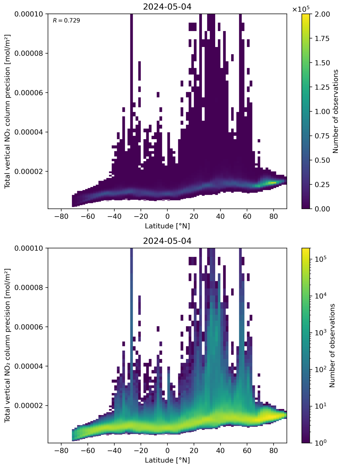
Figure 91: Scatter density plot of “Latitude” against “Total vertical NO 2 column precision” for 2024-05-03 to 2024-05-05.
