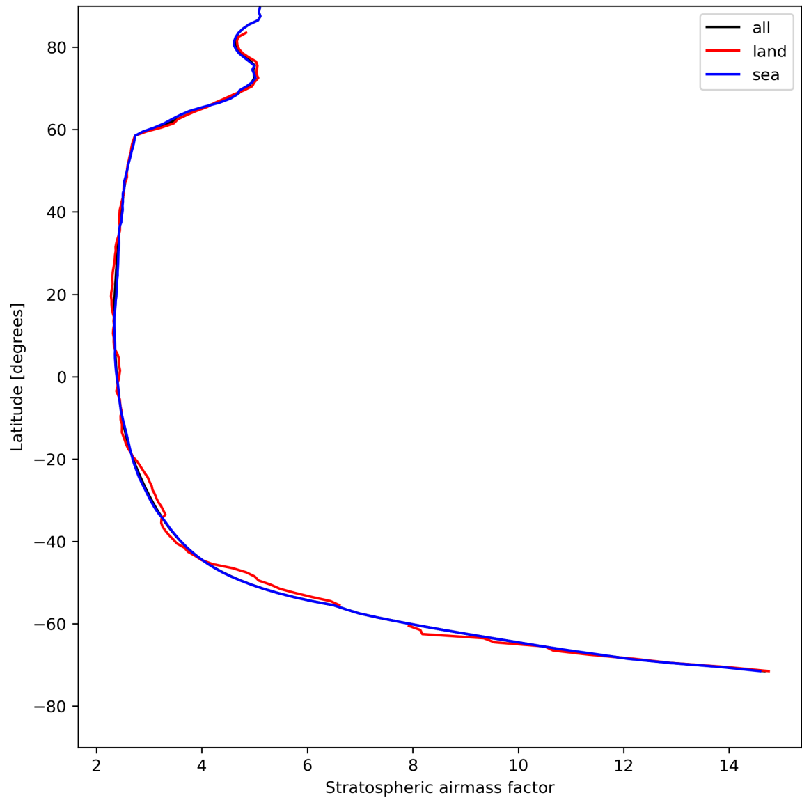
Figure 27: Zonal average of “Stratospheric air mass factor” for 2024-05-03 to 2024-05-05.
