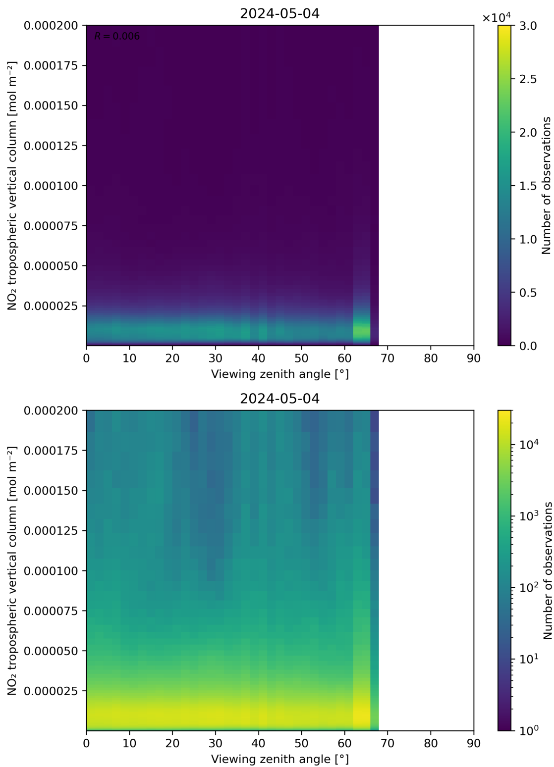
Figure 169: Scatter density plot of “Viewing zenith angle” against “NO 2 tropospheric vertical column” for 2024-05-03 to 2024-05-05.
