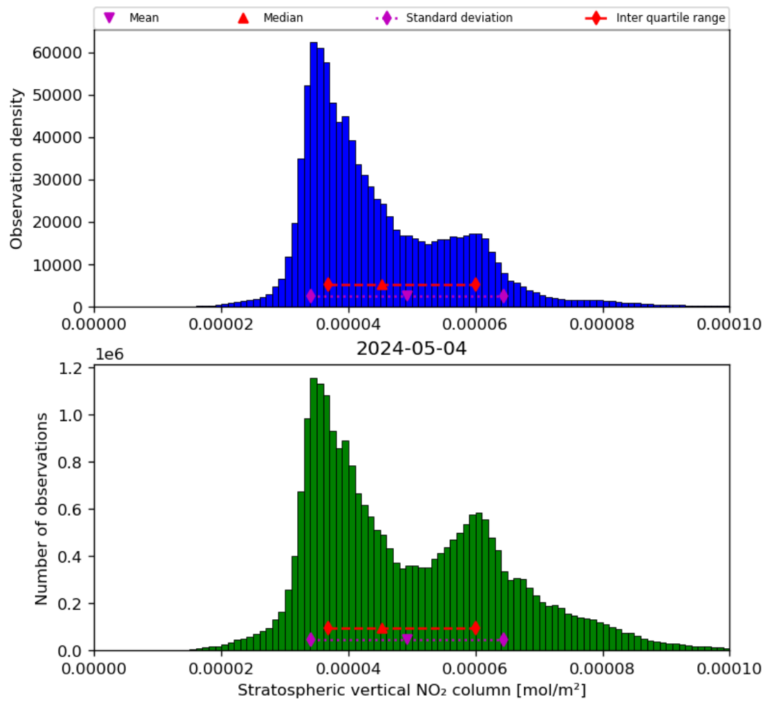
Figure 36: Histogram of “Stratospheric vertical NO 2 column” for 2024-05-03 to 2024-05-05
