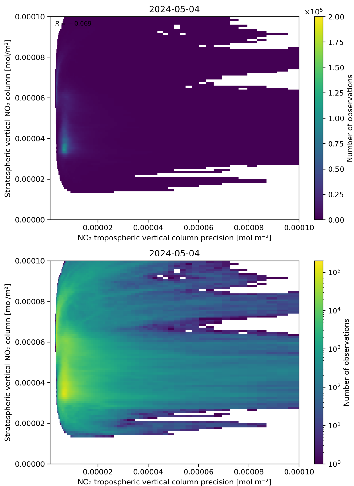
Figure 135: Scatter density plot of “NO 2 tropospheric vertical column precision” against “Stratospheric vertical NO 2 column” for 2024-05-03 to 2024-05-05.
