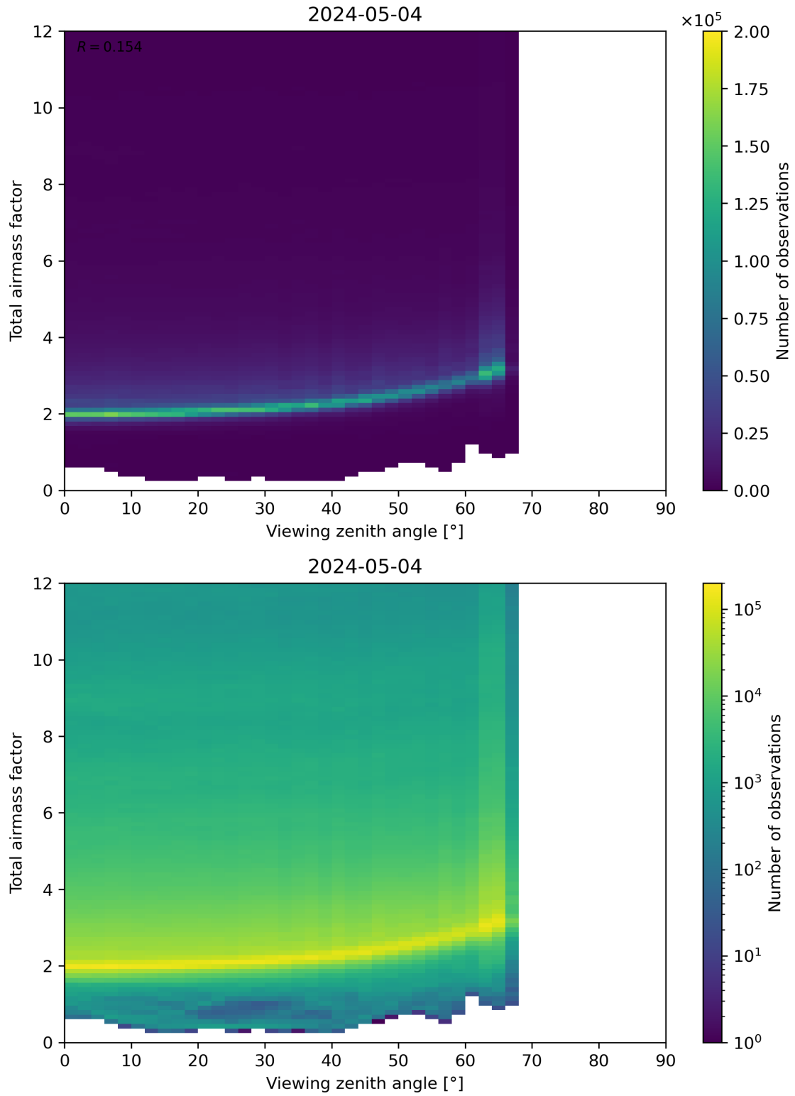
Figure 160: Scatter density plot of “Viewing zenith angle” against “Total airmass factor” for 2024-05-03 to 2024-05-05.
