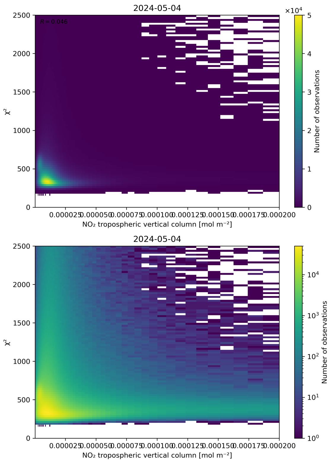
Figure 124: Scatter density plot of “NO 2 tropospheric vertical column” against “ \chi^2 ” for 2024-05-03 to 2024-05-05.
