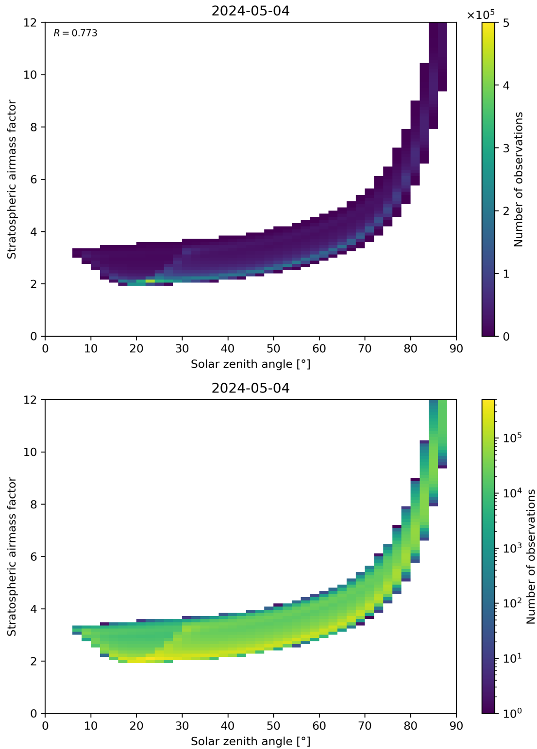
Figure 145: Scatter density plot of “Solar zenith angle” against “Stratospheric airmass factor” for 2024-05-03 to 2024-05-05.
