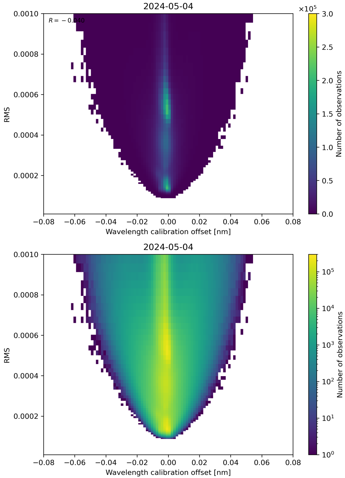
Figure 181: Scatter density plot of “Wavelength calibration offset” against “RMS” for 2024-05-03 to 2024-05-05.
