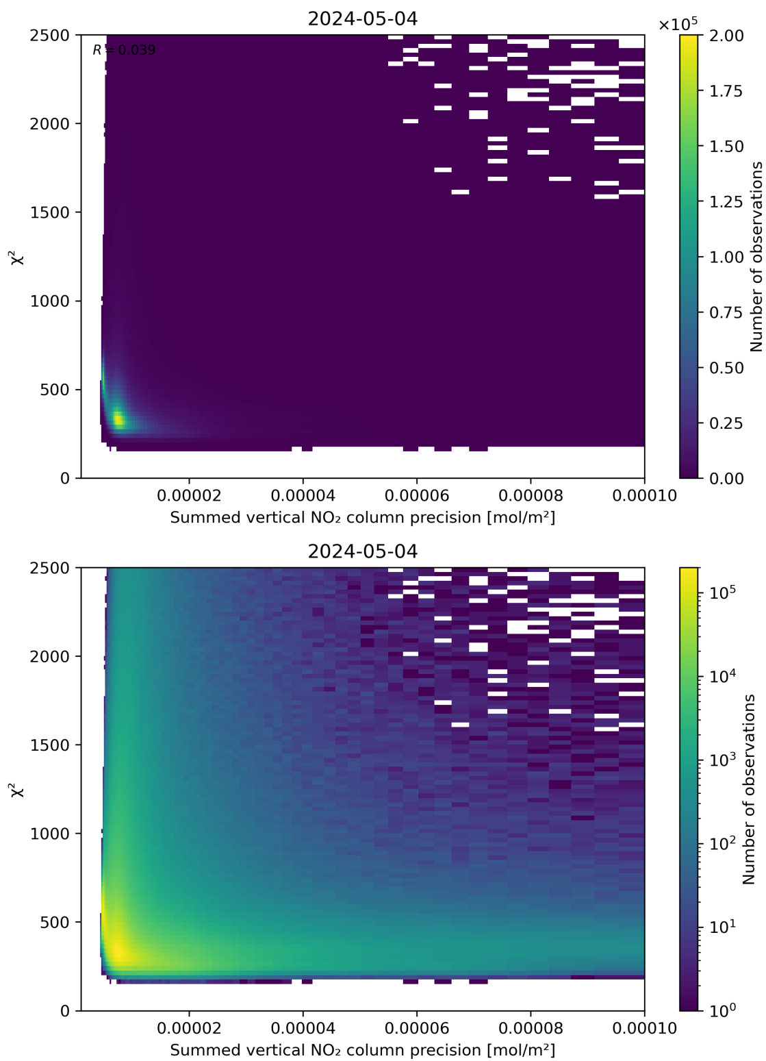
Figure 107: Scatter density plot of “Summed vertical NO 2 column precision” against “ \chi^2 ” for 2024-05-03 to 2024-05-05.
