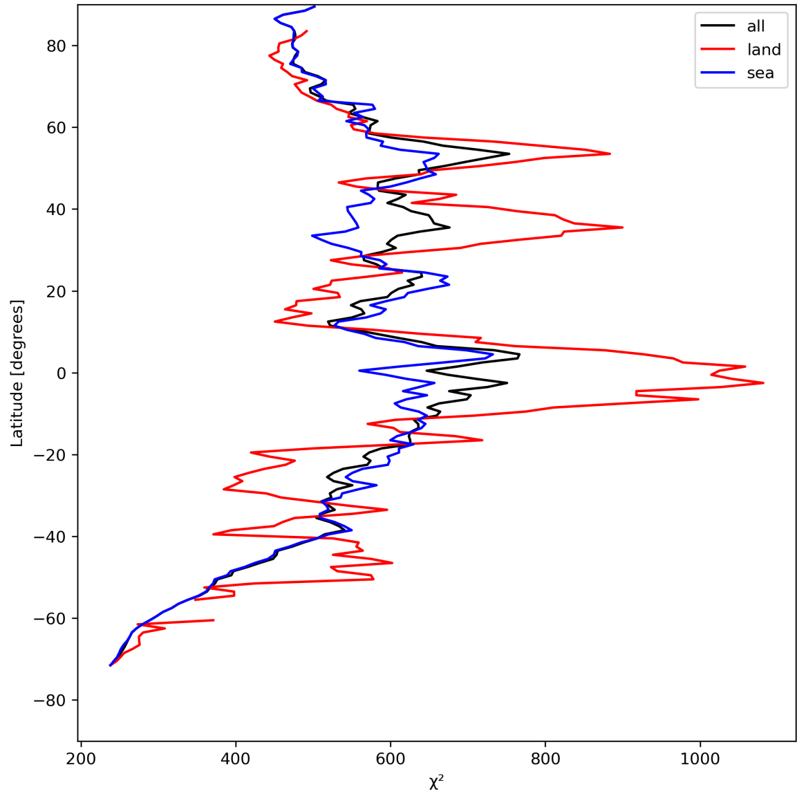
Figure 25: Zonal average of “ \chi^2 ” for 2024-05-03 to 2024-05-05.
