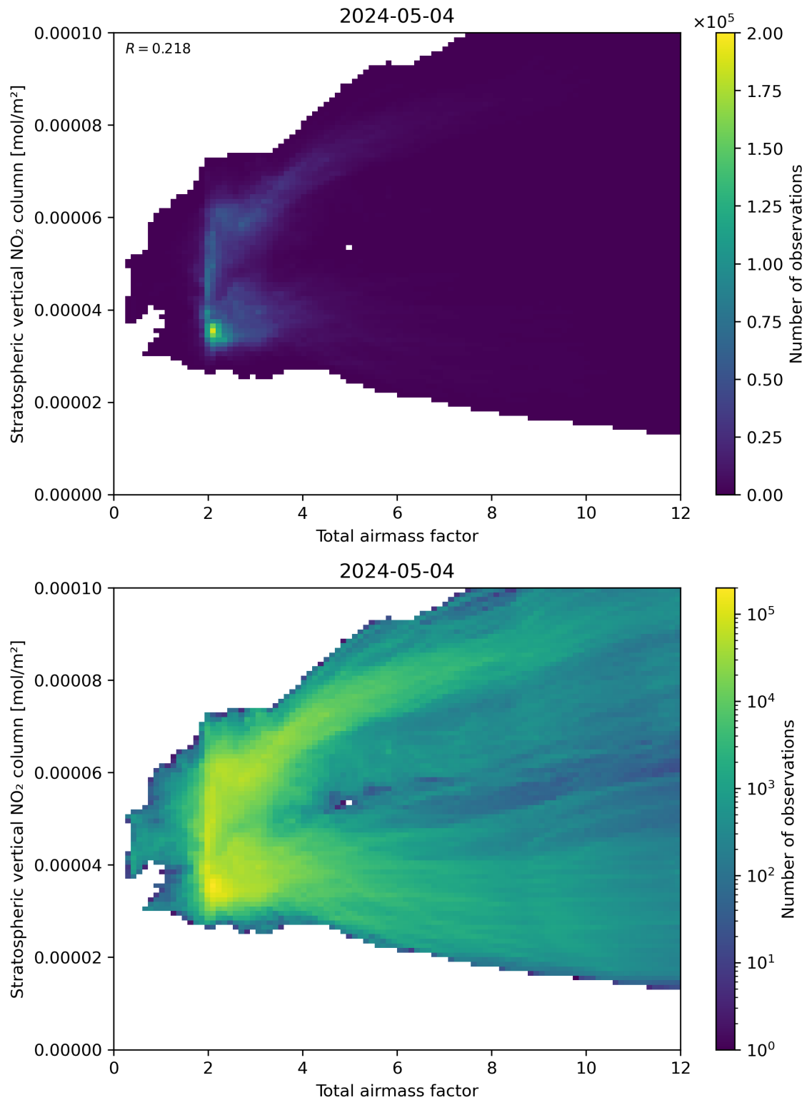
Figure 64: Scatter density plot of “Total airmass factor” against “Stratospheric vertical NO 2 column” for 2024-05-03 to 2024-05-05.
