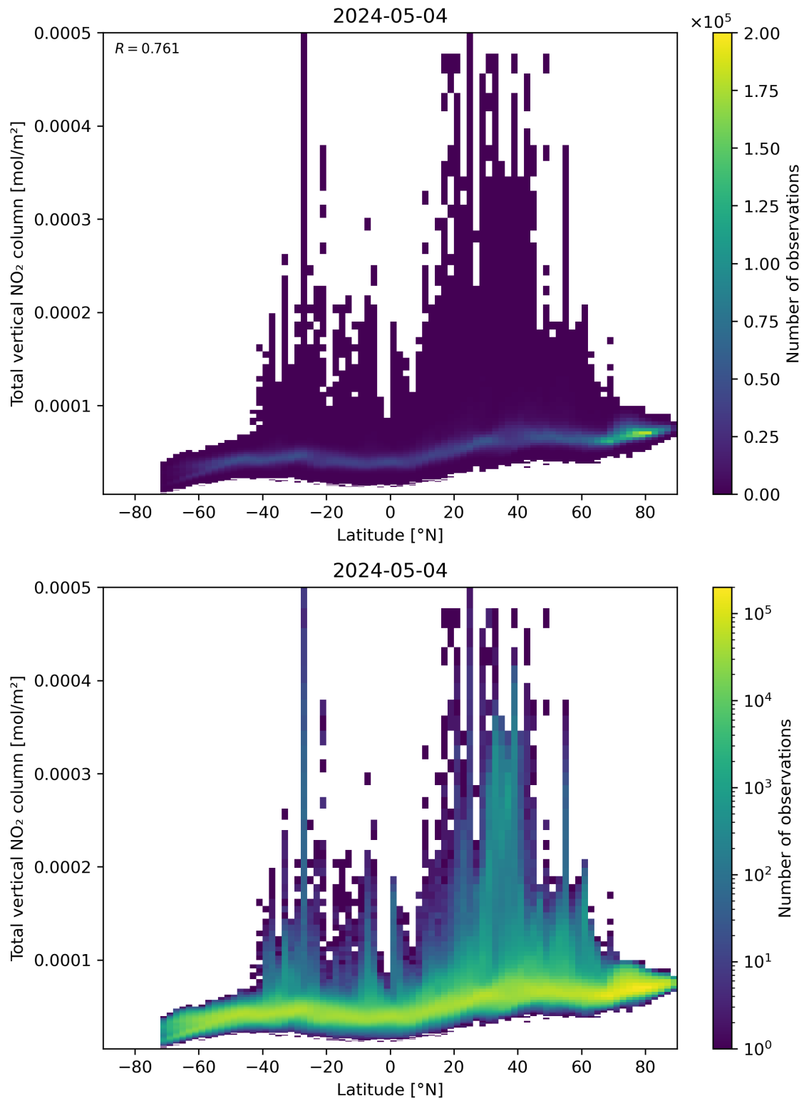
Figure 90: Scatter density plot of “Latitude” against “Total vertical NO 2 column” for 2024-05-03 to 2024-05-05.
