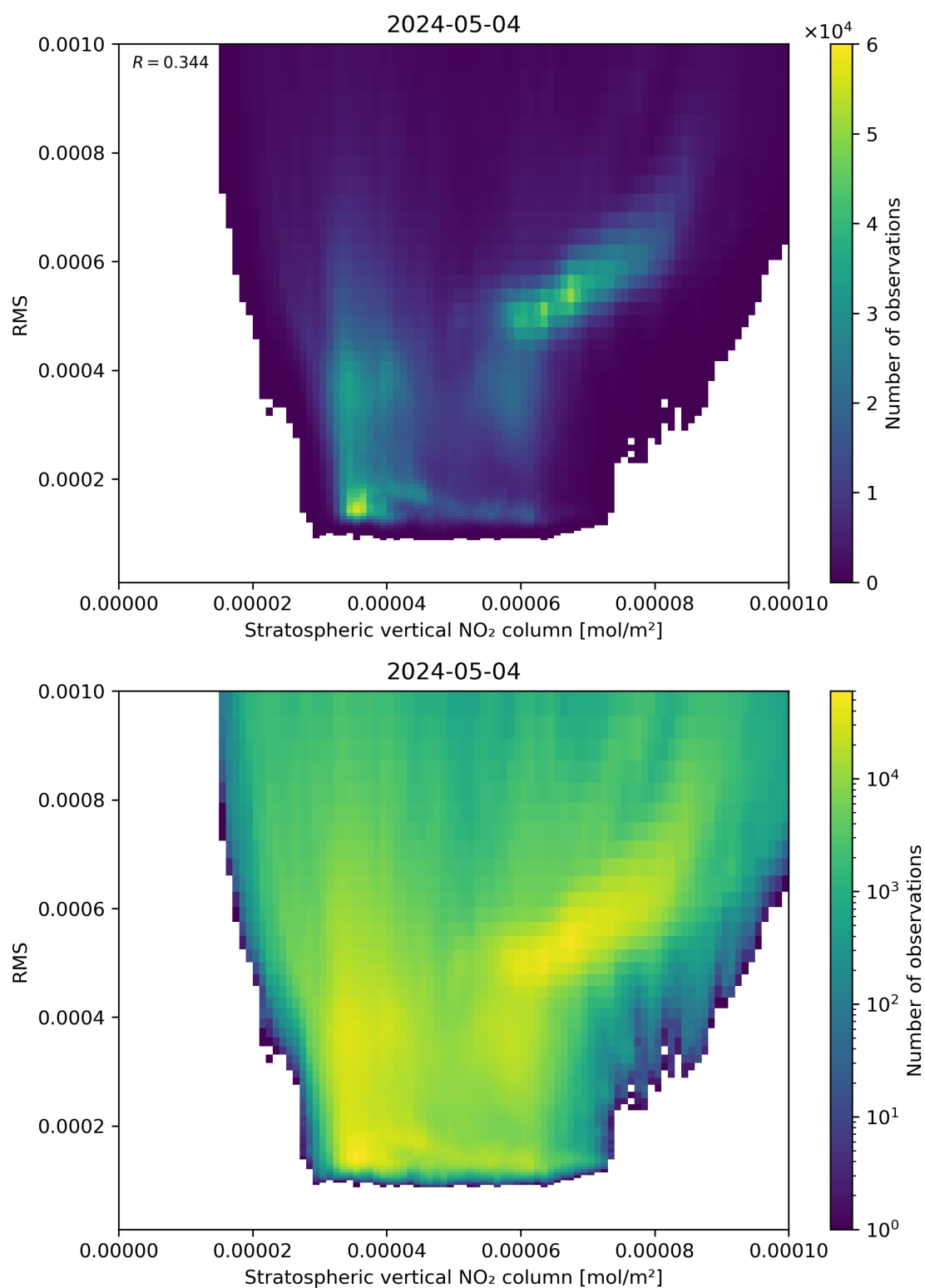
Figure 102: Scatter density plot of “Stratospheric vertical NO 2 column” against “RMS” for 2024-05-03 to 2024-05-05.
