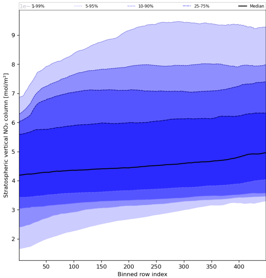
Figure 53: Along track statistics of “Stratospheric vertical NO 2 column” for 2024-05-03 to 2024-05-05
