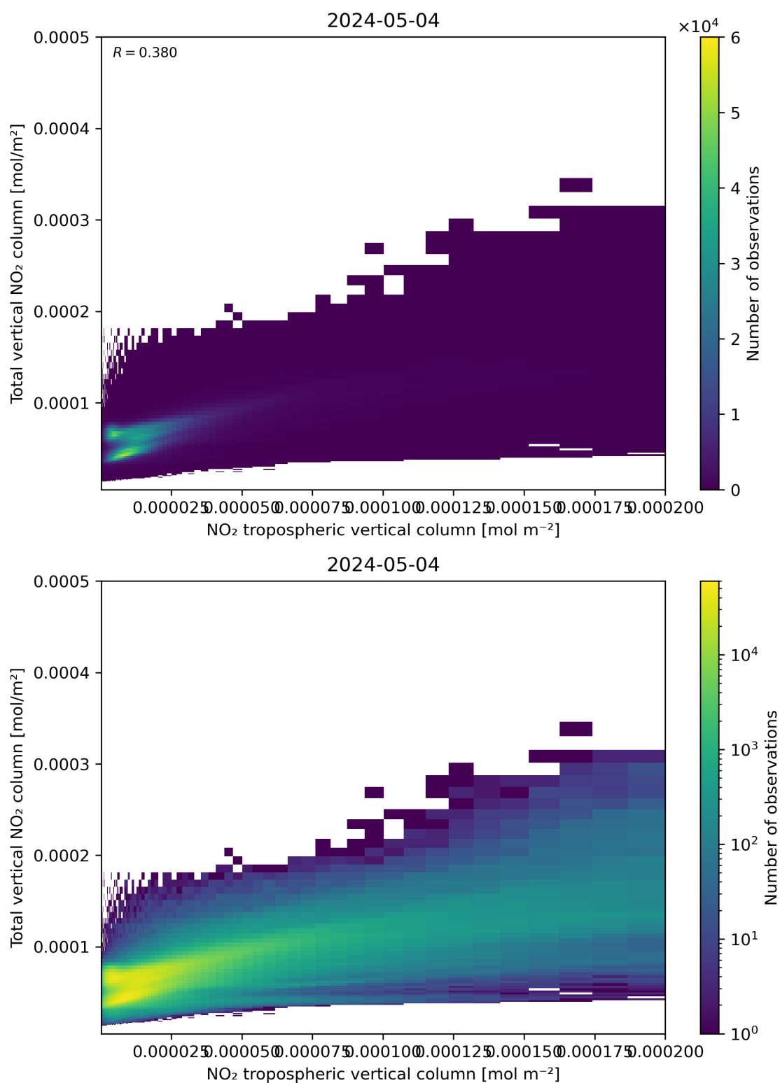
Figure 128: Scatter density plot of “NO 2 tropospheric vertical column” against “Total vertical NO 2 column” for 2024-05-03 to 2024-05-05.
