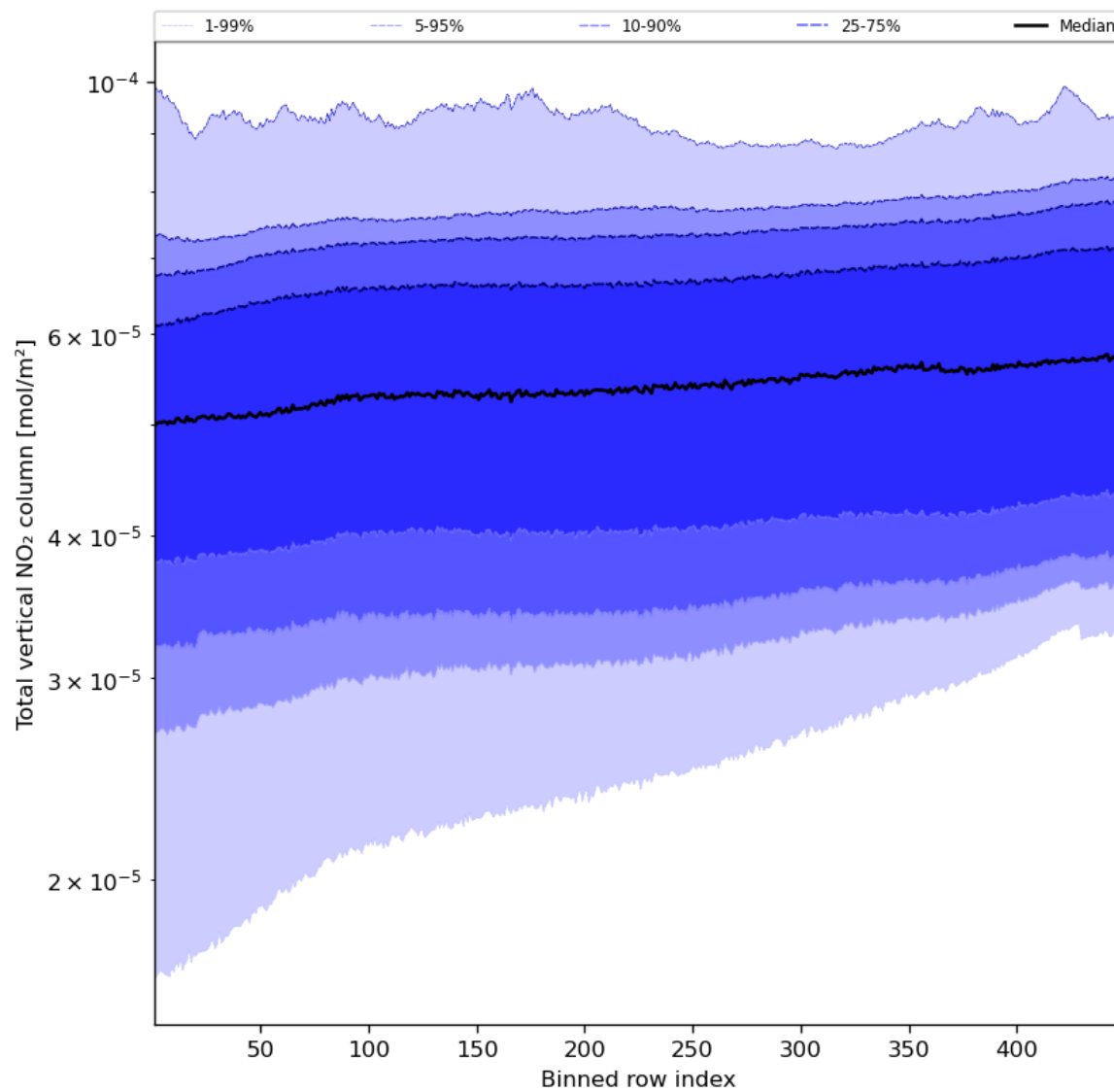
Figure 55: Along track statistics of “Total vertical NO 2 column” for 2024-05-03 to 2024-05-05
