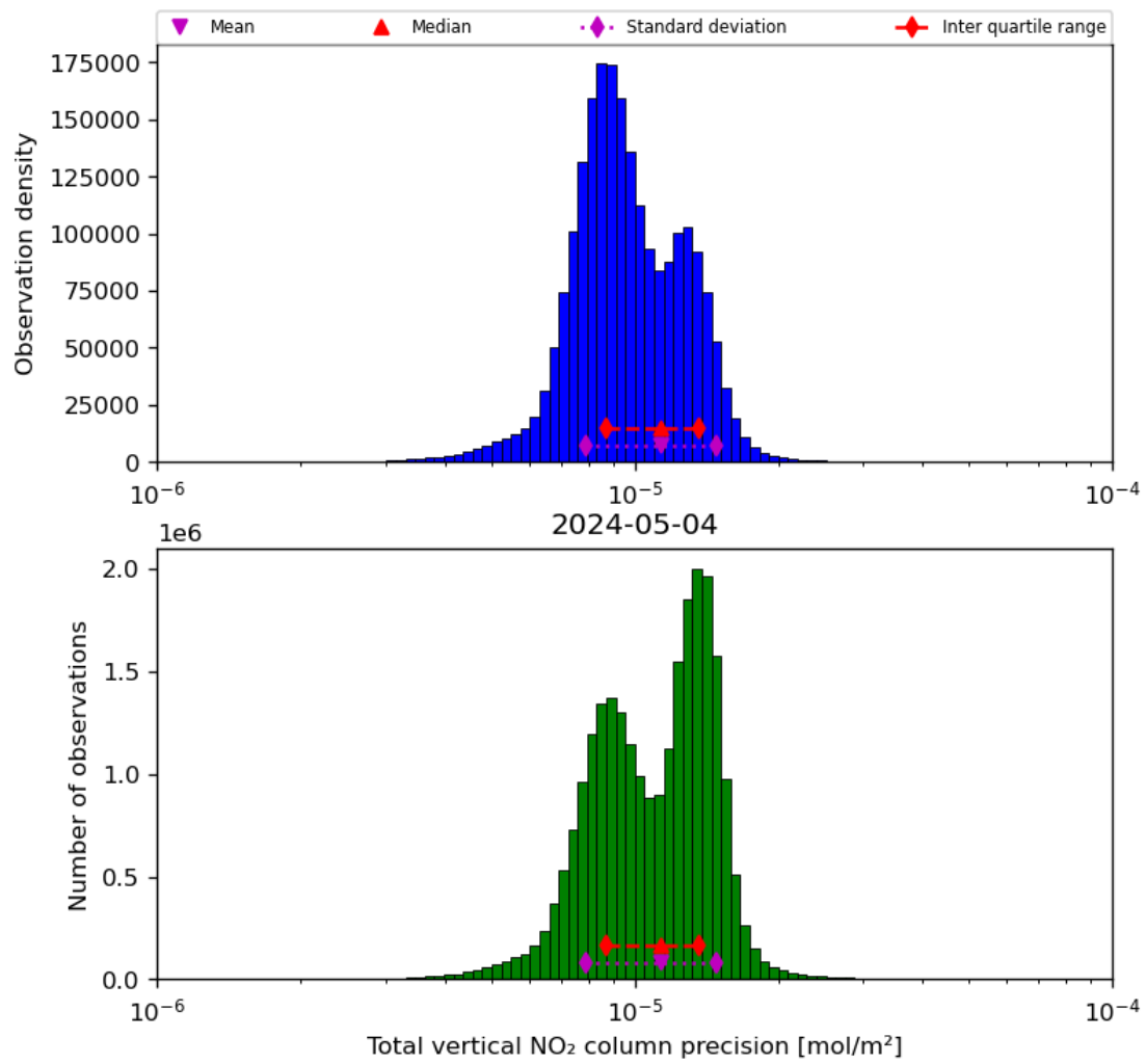
Figure 39: Histogram of “Total vertical NO 2 column precision” for 2024-05-03 to 2024-05-05
