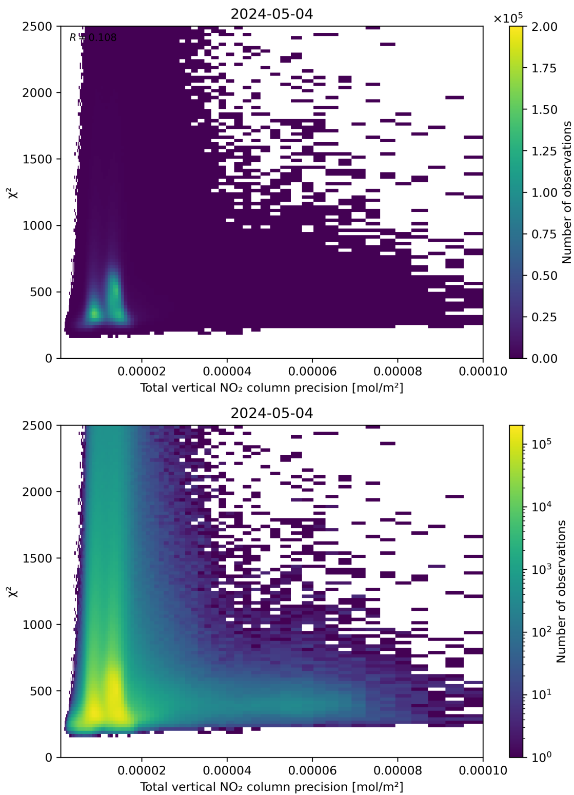
Figure 116: Scatter density plot of “Total vertical NO 2 column precision” against “ \chi^2 ” for 2024-05-03 to 2024-05-05.
