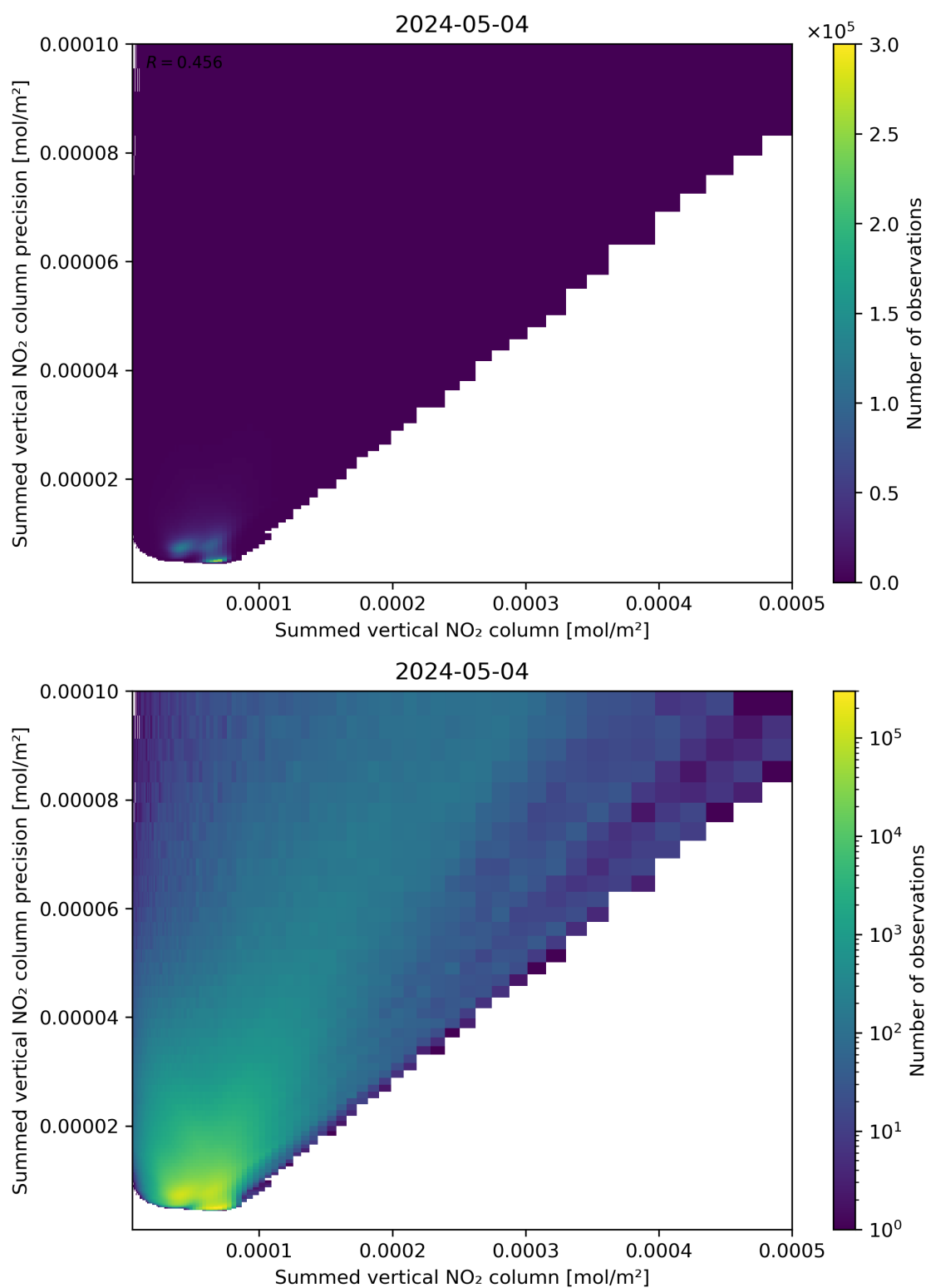
Figure 105: Scatter density plot of “Summed vertical NO 2 column” against “Summed vertical NO 2 column precision” for 2024-05-03 to 2024-05-05.
