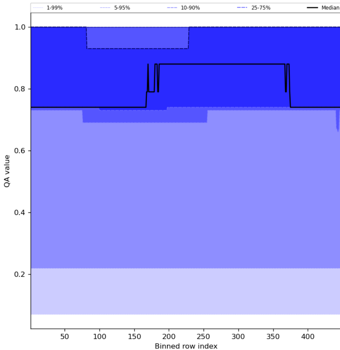
Figure 45: Along track statistics of “QA value” for 2024-05-03 to 2024-05-05
