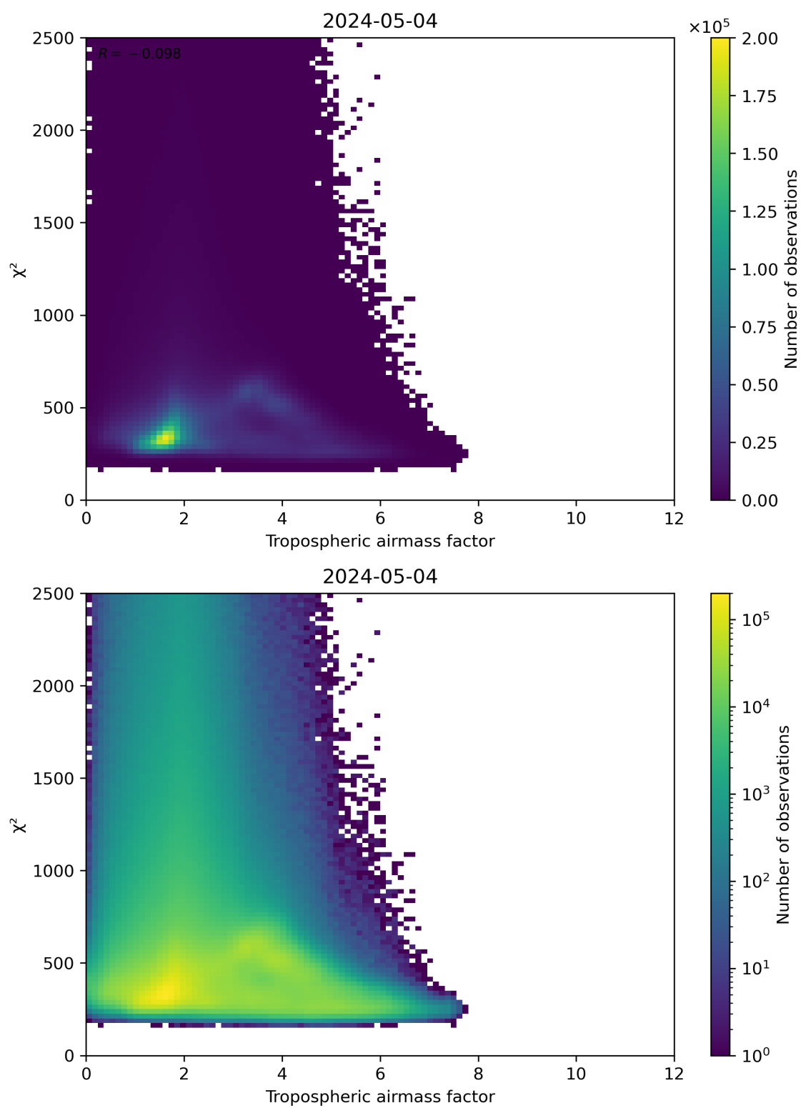
Figure 73: Scatter density plot of “Tropospheric airmass factor” against “ \chi^2 ” for 2024-05-03 to 2024-05-05.
