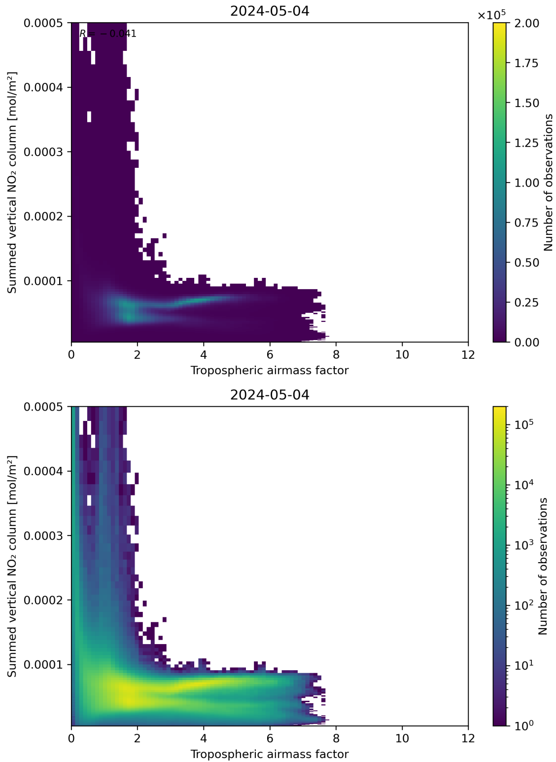
Figure 75: Scatter density plot of “Tropospheric airmass factor” against “Summed vertical NO 2 column” for 2024-05-03 to 2024-05-05.
