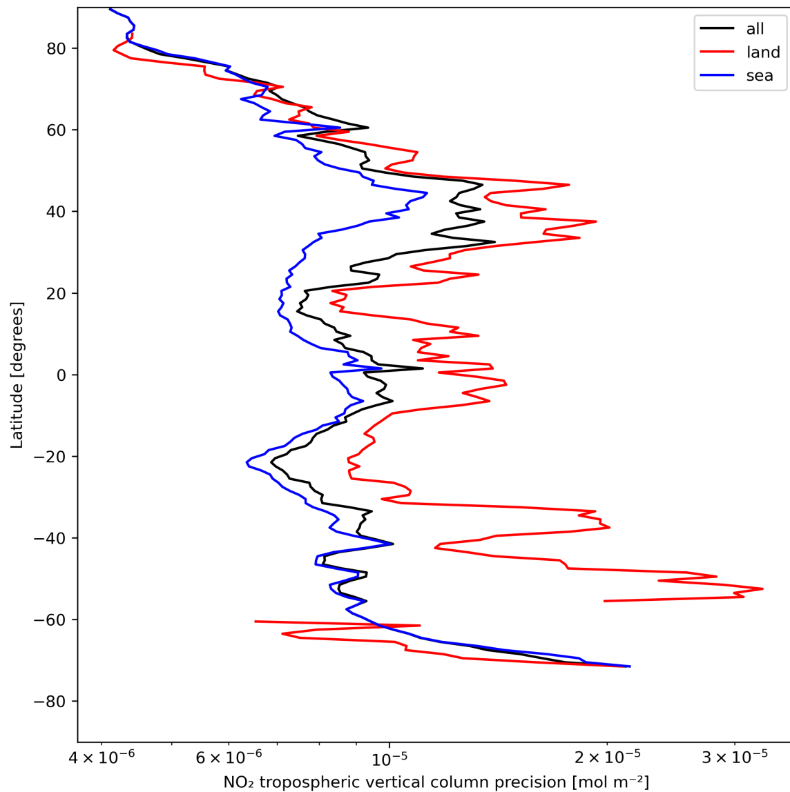
Figure 13: Zonal average of “NO 2 tropospheric vertical column precision” for 2024-05-03 to 2024-05-05.
