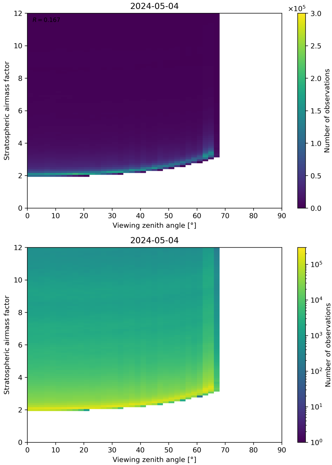
Figure 159: Scatter density plot of “Viewing zenith angle” against “Stratospheric airmass factor” for 2024-05-03 to 2024-05-05.
