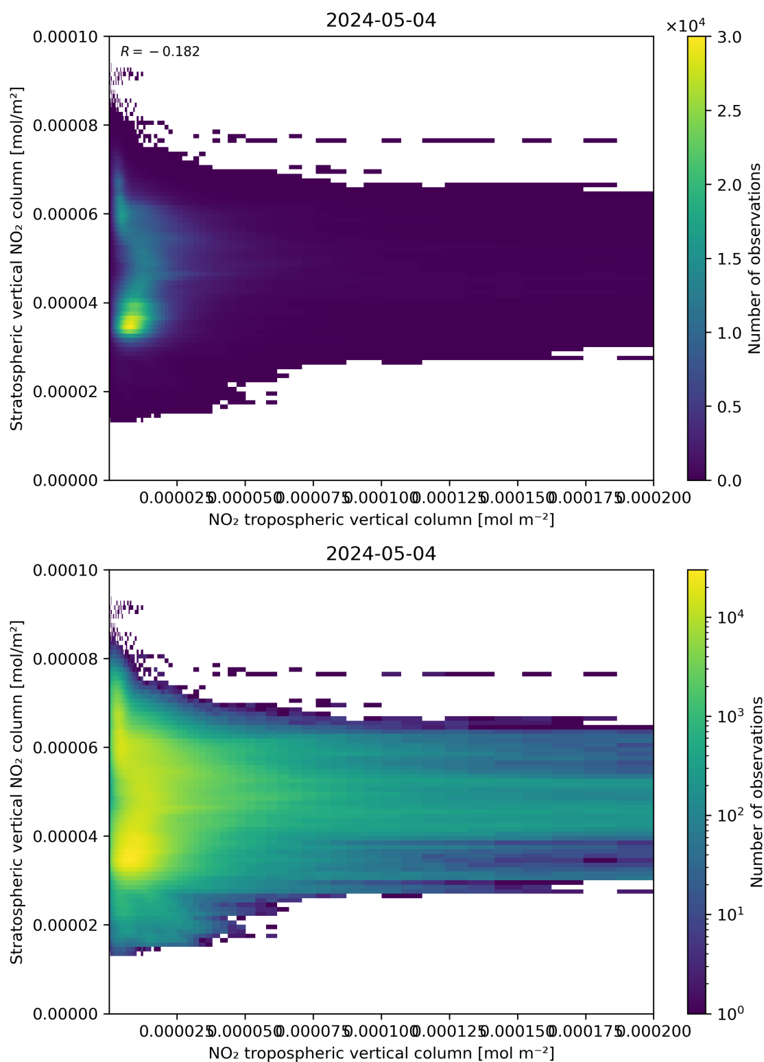
Figure 125: Scatter density plot of “NO 2 tropospheric vertical column” against “Stratospheric vertical NO 2 column” for 2024-05-03 to 2024-05-05.
