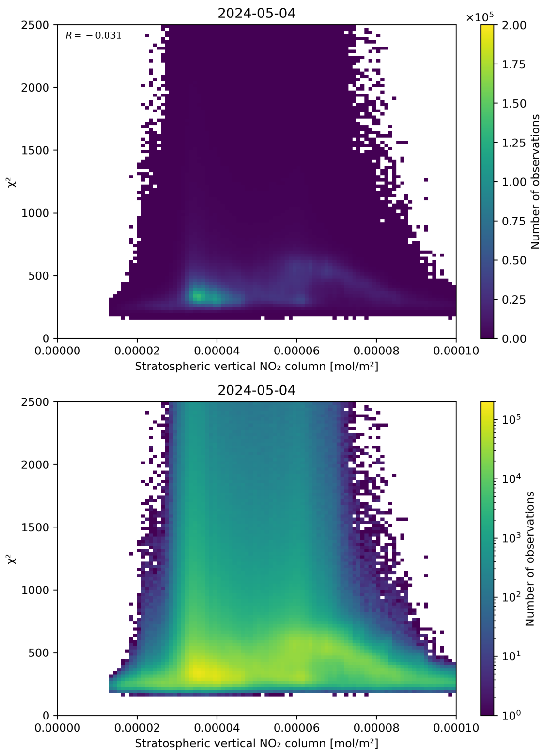
Figure 97: Scatter density plot of “Stratospheric vertical NO 2 column” against “ \chi^2 ” for 2024-05-03 to 2024-05-05.
