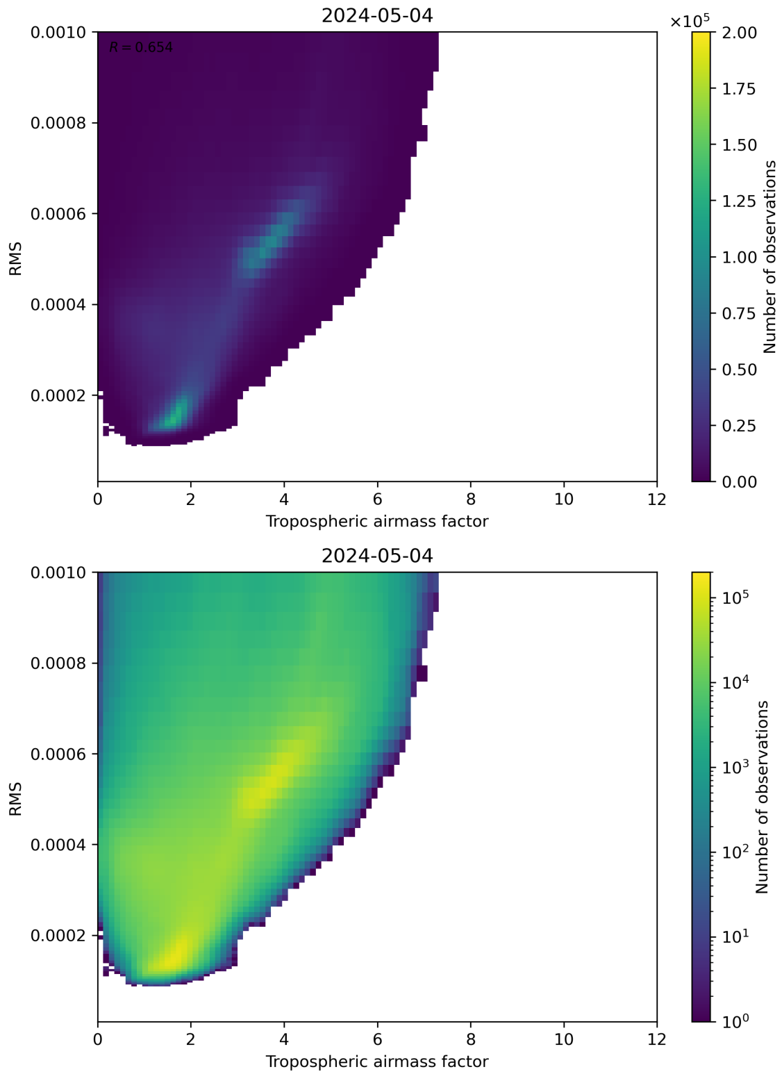
Figure 79: Scatter density plot of “Tropospheric airmass factor” against “RMS” for 2024-05-03 to 2024-05-05.
