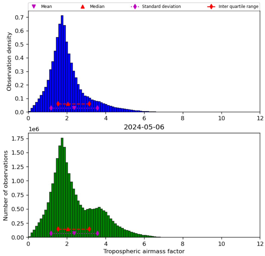
Figure 31: Histogram of “Tropospheric airmass factor” for 2024-05-05 to 2024-05-07
