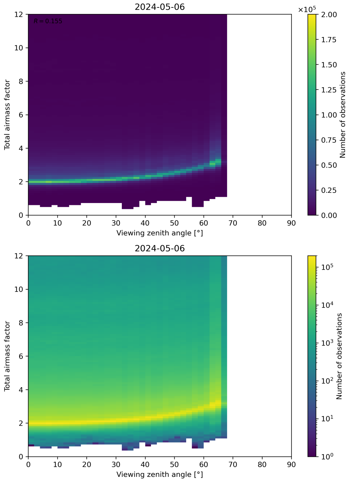
Figure 160: Scatter density plot of “Viewing zenith angle” against “Total airmass factor” for 2024-05-05 to 2024-05-07.
