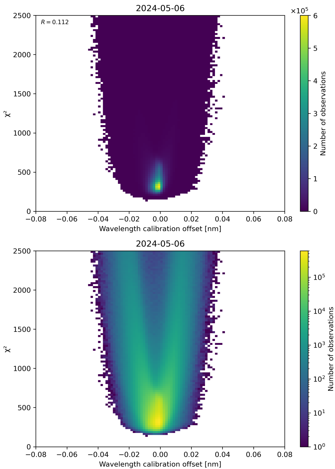
Figure 175: Scatter density plot of “Wavelength calibration offset” against “ \chi^2 ” for 2024-05-05 to 2024-05-07.
