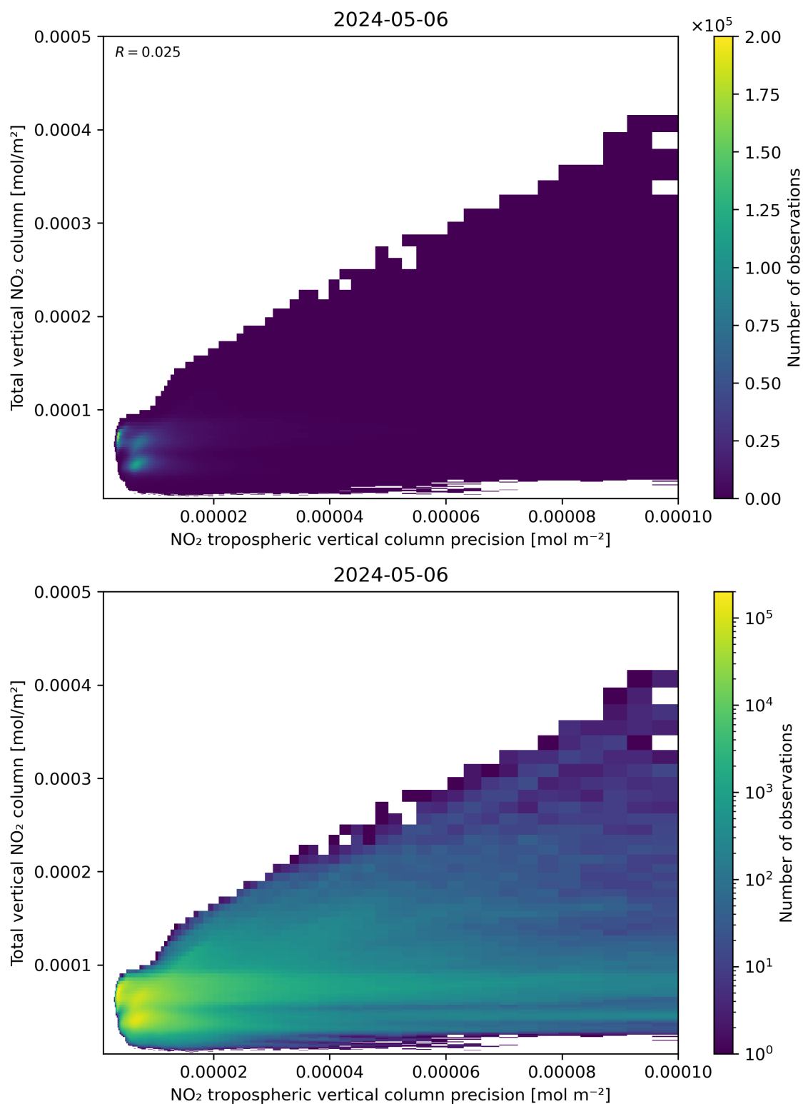
Figure 138: Scatter density plot of “NO 2 tropospheric vertical column precision” against “Total vertical NO 2 column” for 2024-05-05 to 2024-05-07.
