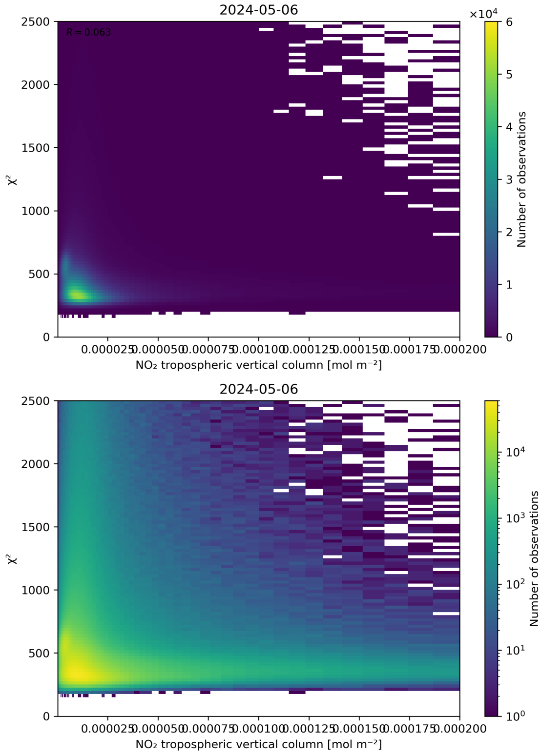
Figure 124: Scatter density plot of “NO 2 tropospheric vertical column” against “ \chi^2 ” for 2024-05-05 to 2024-05-07.
