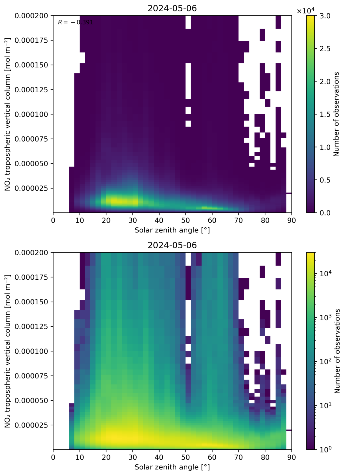
Figure 155: Scatter density plot of “Solar zenith angle” against “NO 2 tropospheric vertical column” for 2024-05-05 to 2024-05-07.
