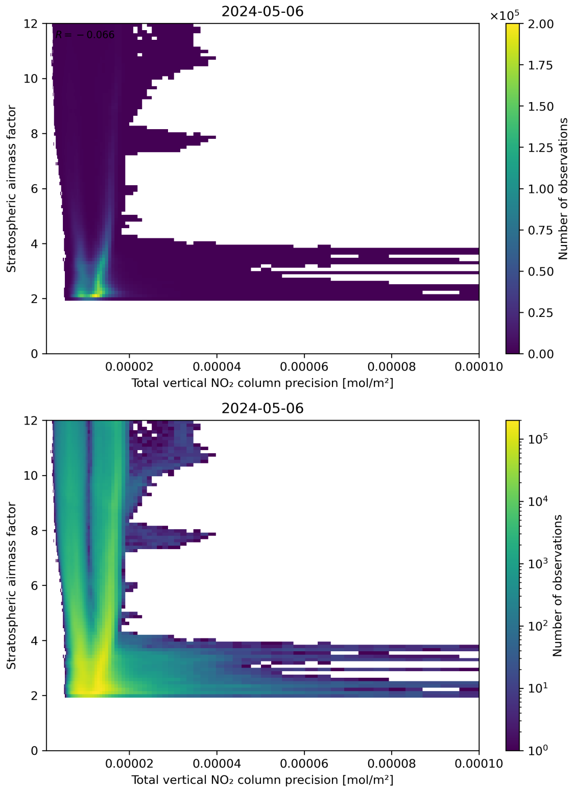
Figure 115: Scatter density plot of “Total vertical NO 2 column precision” against “Stratospheric air mass factor” for 2024-05-05 to 2024-05-07.
