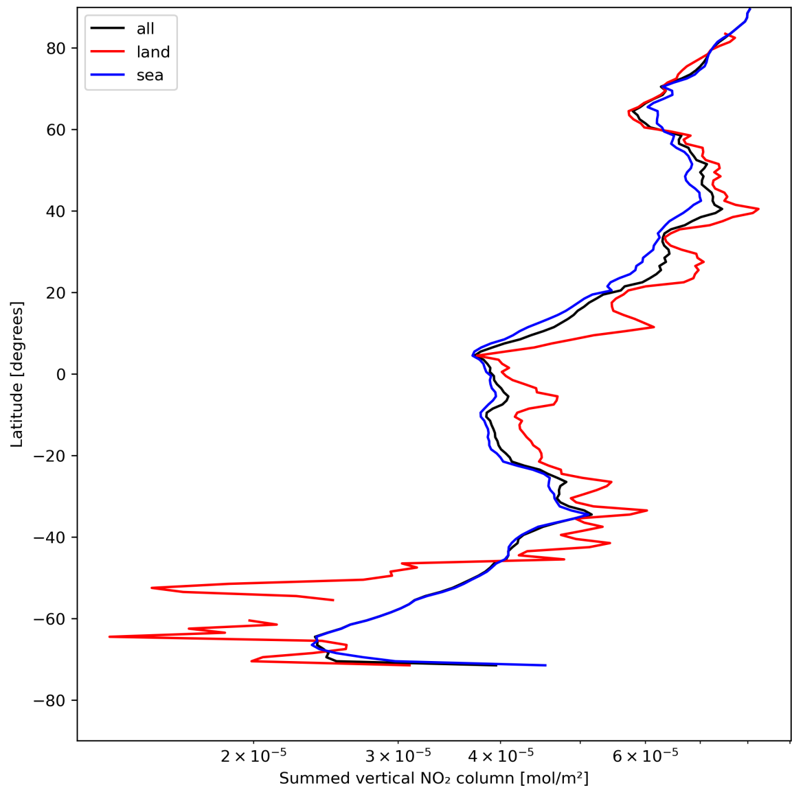
Figure 23: Zonal average of “Summed vertical NO 2 column” for 2024-05-05 to 2024-05-07.
