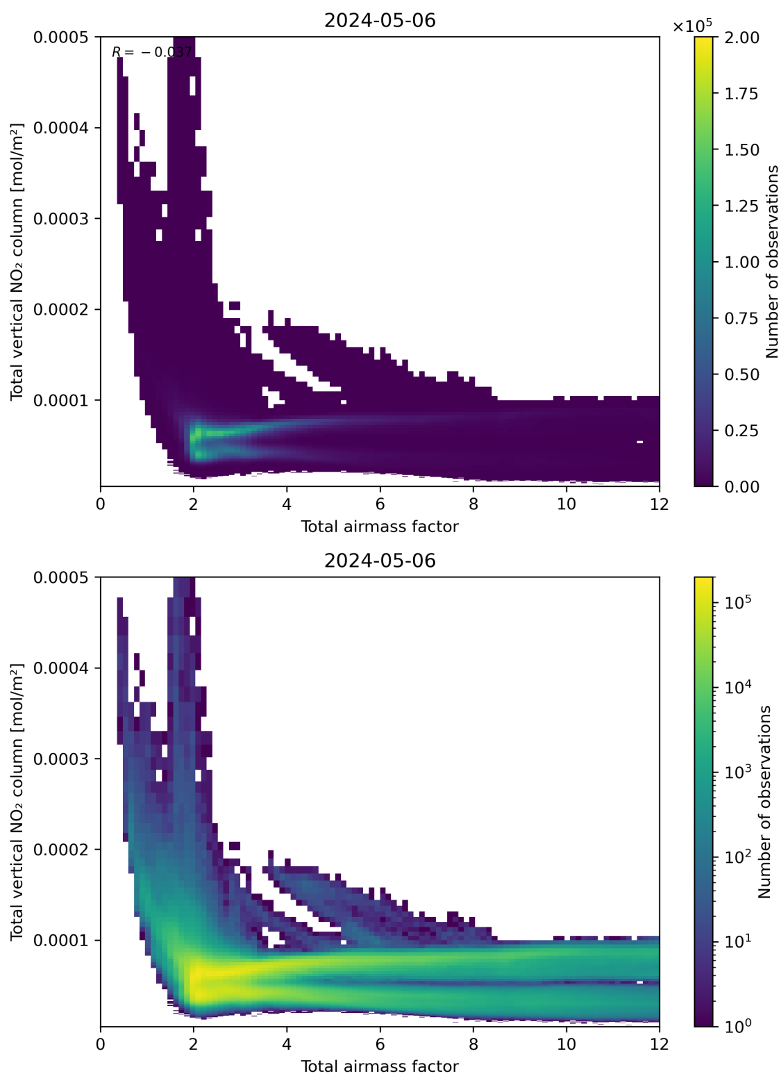
Figure 67: Scatter density plot of “Total airmass factor” against “Total vertical NO 2 column” for 2024-05-05 to 2024-05-07.
