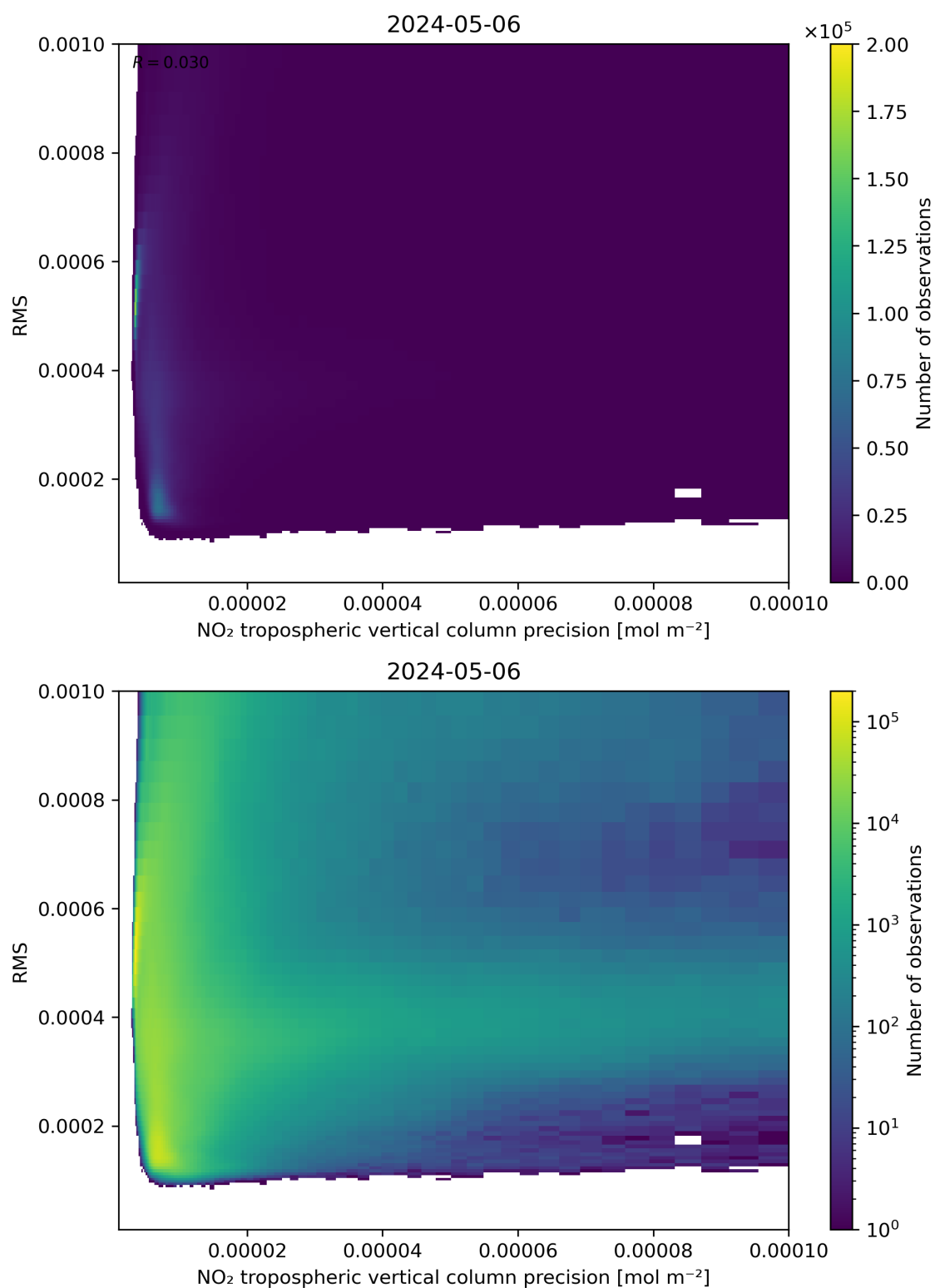
Figure 140: Scatter density plot of “NO 2 tropospheric vertical column precision” against “RMS” for 2024-05-05 to 2024-05-07.
