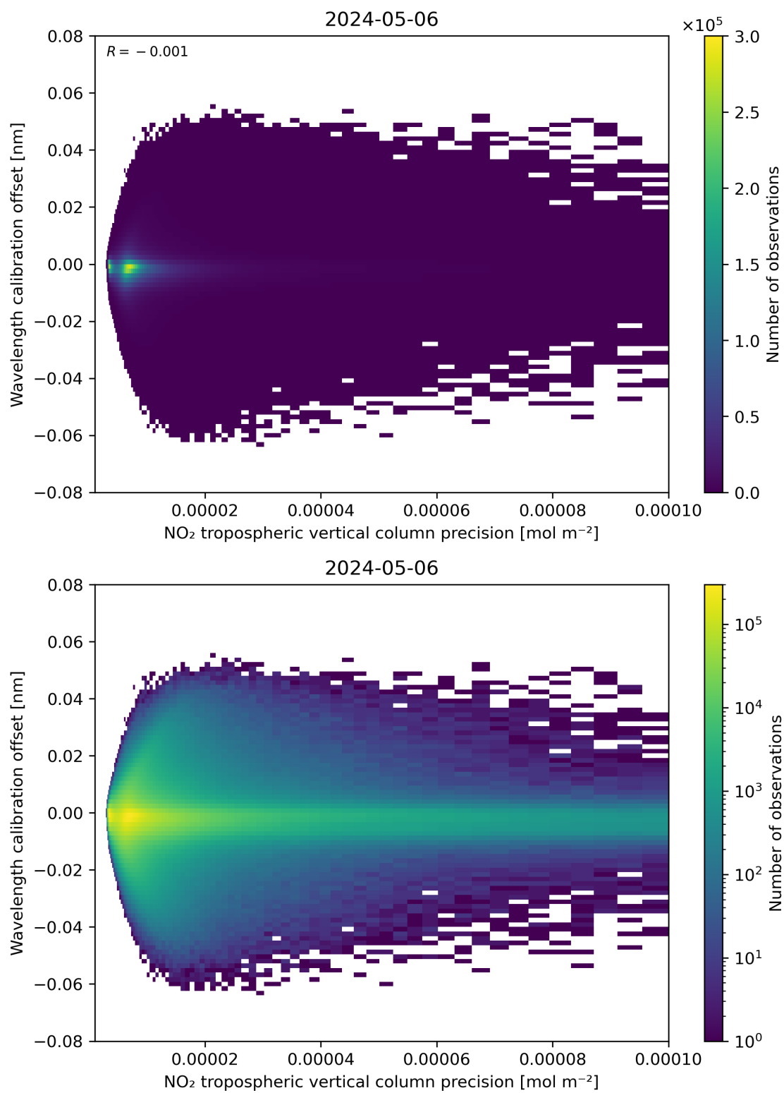
Figure 141: Scatter density plot of “NO 2 tropospheric vertical column precision” against “Wavelength calibration offset” for 2024-05-05 to 2024-05-07.
