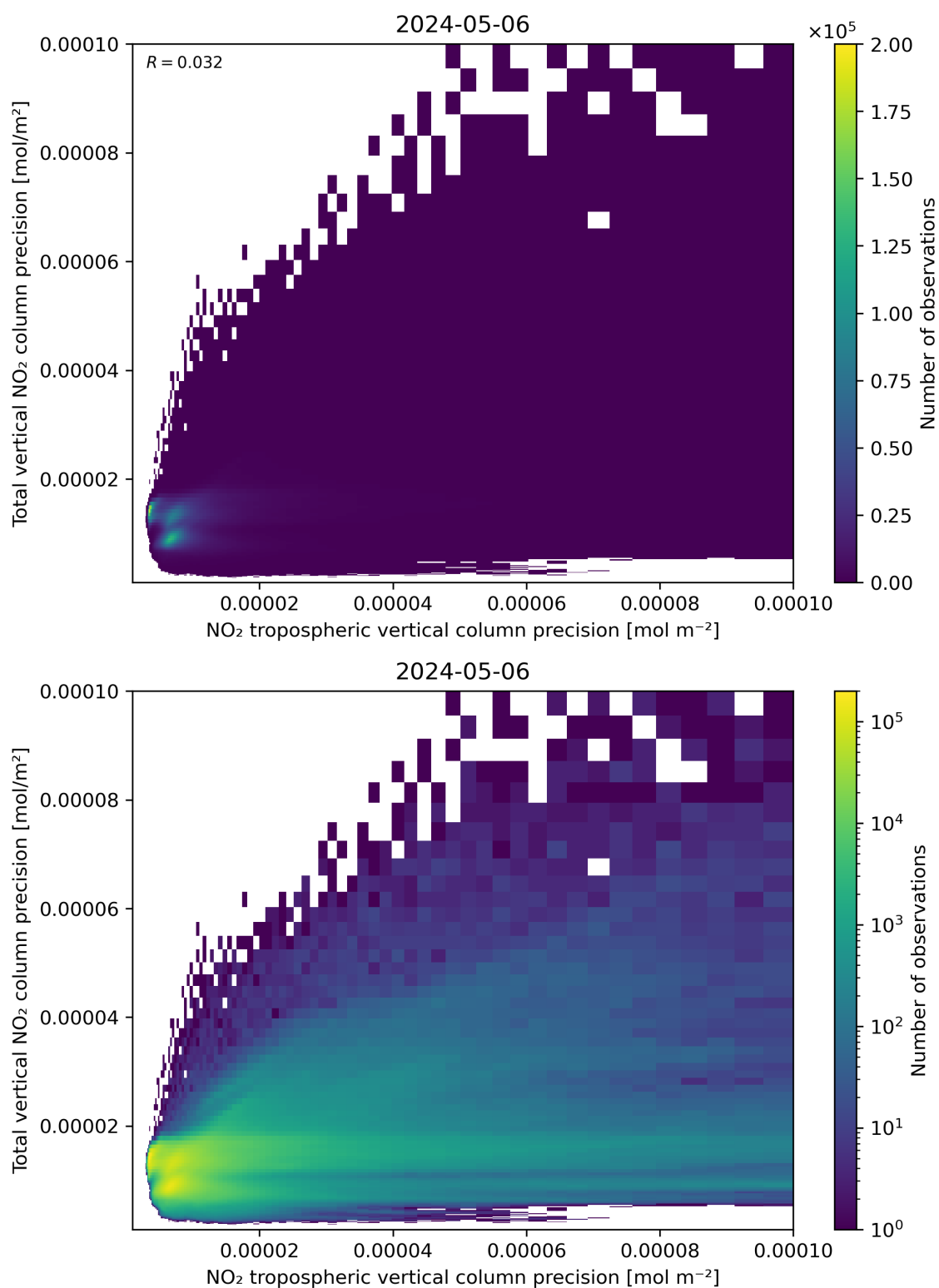
Figure 139: Scatter density plot of “NO 2 tropospheric vertical column precision” against “Total vertical NO 2 column precision” for 2024-05-05 to 2024-05-07.
