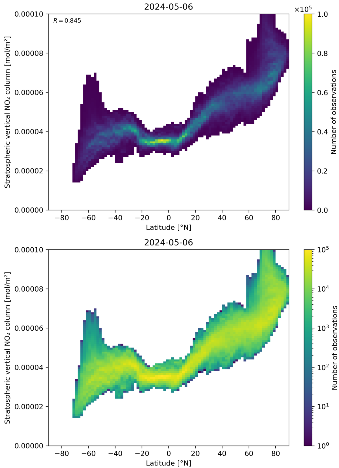
Figure 87: Scatter density plot of “Latitude” against “Stratospheric vertical NO 2 column” for 2024-05-05 to 2024-05-07.
