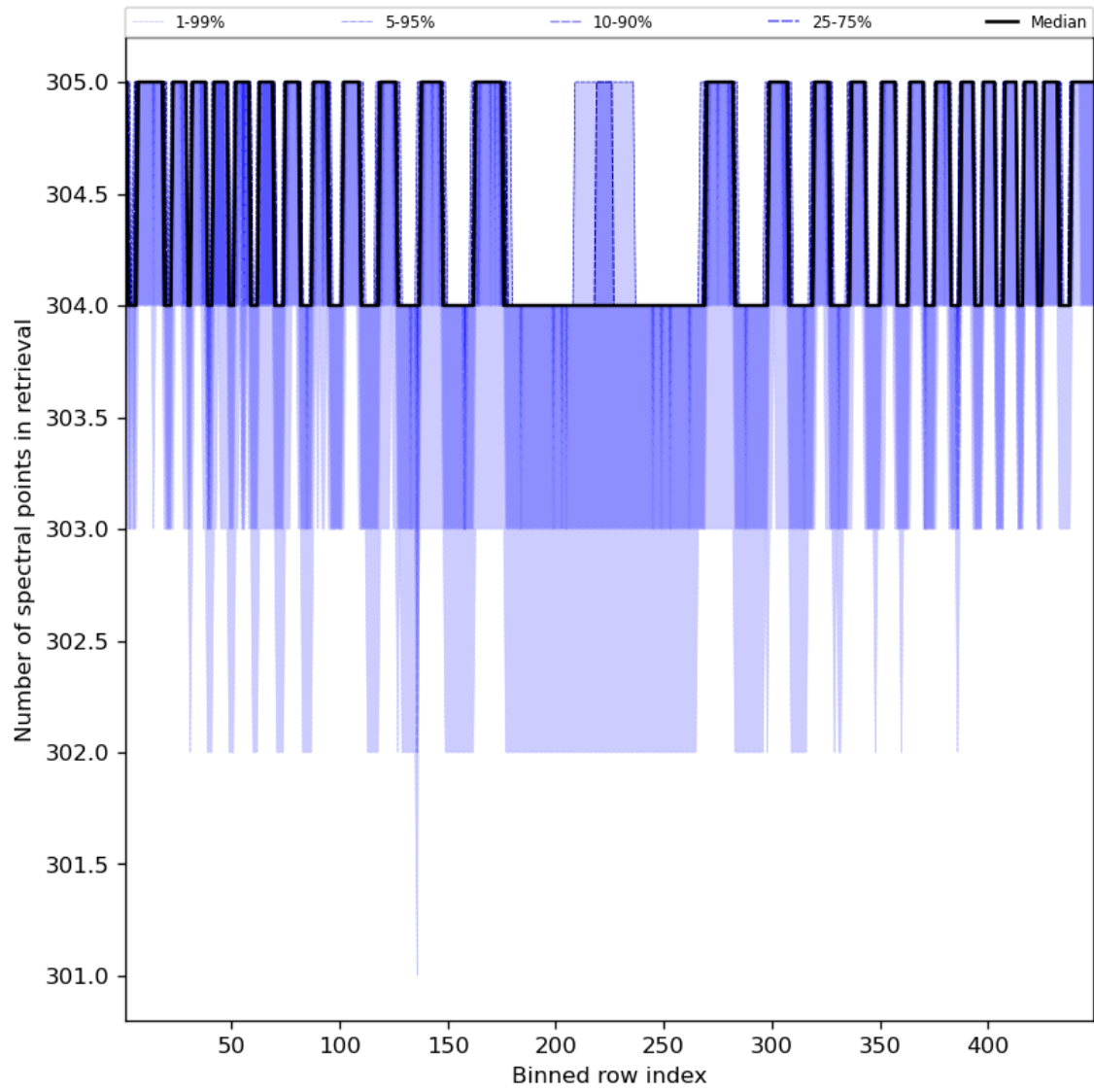
Figure 50: Along track statistics of “Number of spectral points in retrieval” for 2024-05-05 to 2024-05-07
