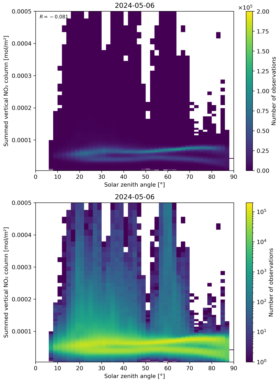
Figure 151: Scatter density plot of “Solar zenith angle” against “Summed vertical NO 2 column” for 2024-05-05 to 2024-05-07.
