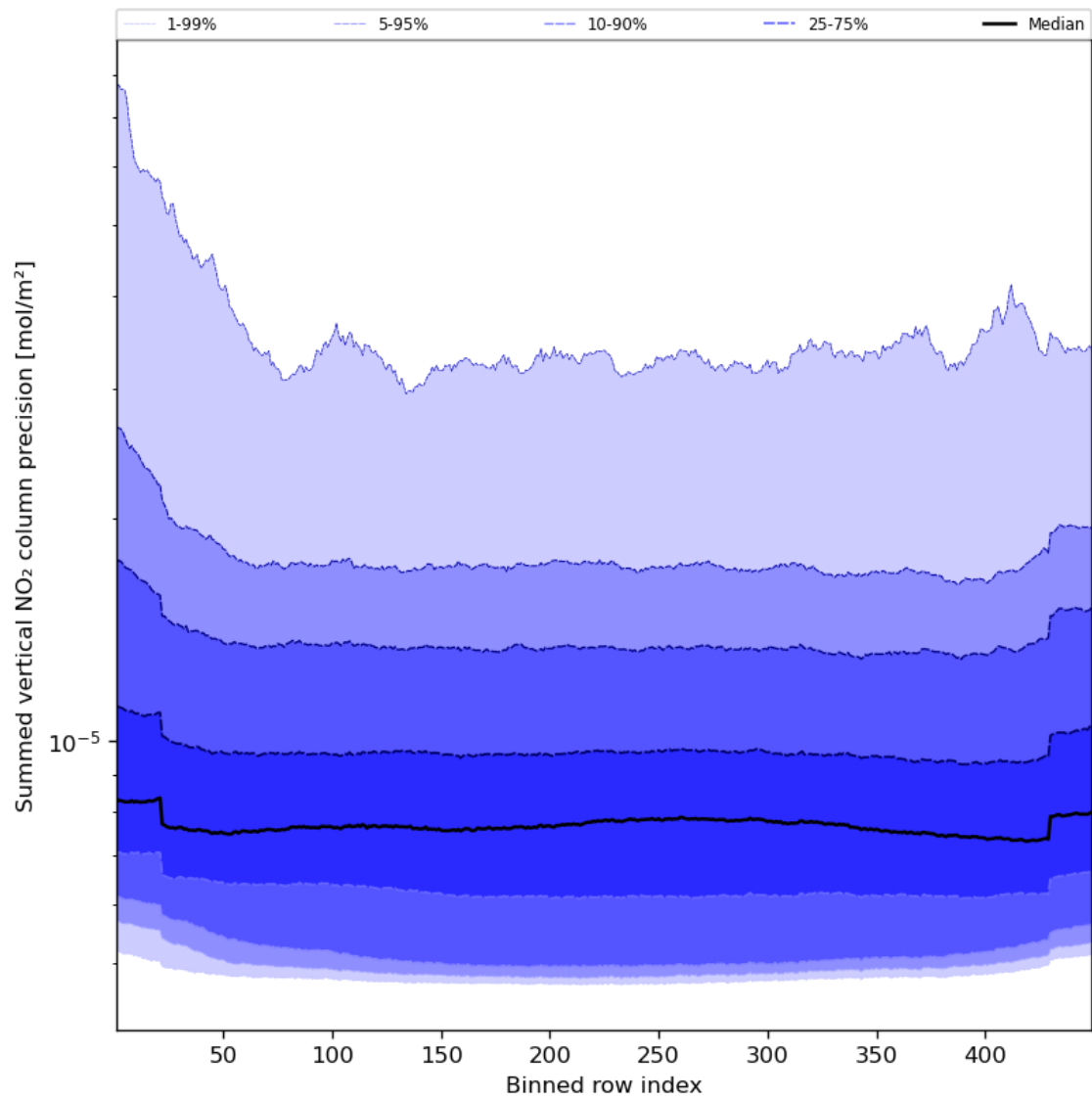
Figure 58: Along track statistics of “Summed vertical NO 2 column precision” for 2024-05-05 to 2024-05-07
