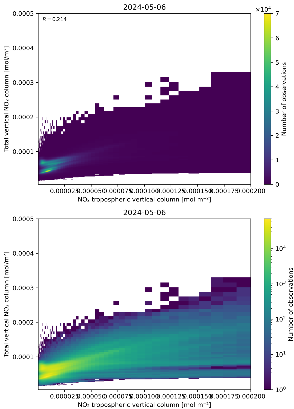
Figure 128: Scatter density plot of “NO 2 tropospheric vertical column” against “Total vertical NO 2 column” for 2024-05-05 to 2024-05-07.
