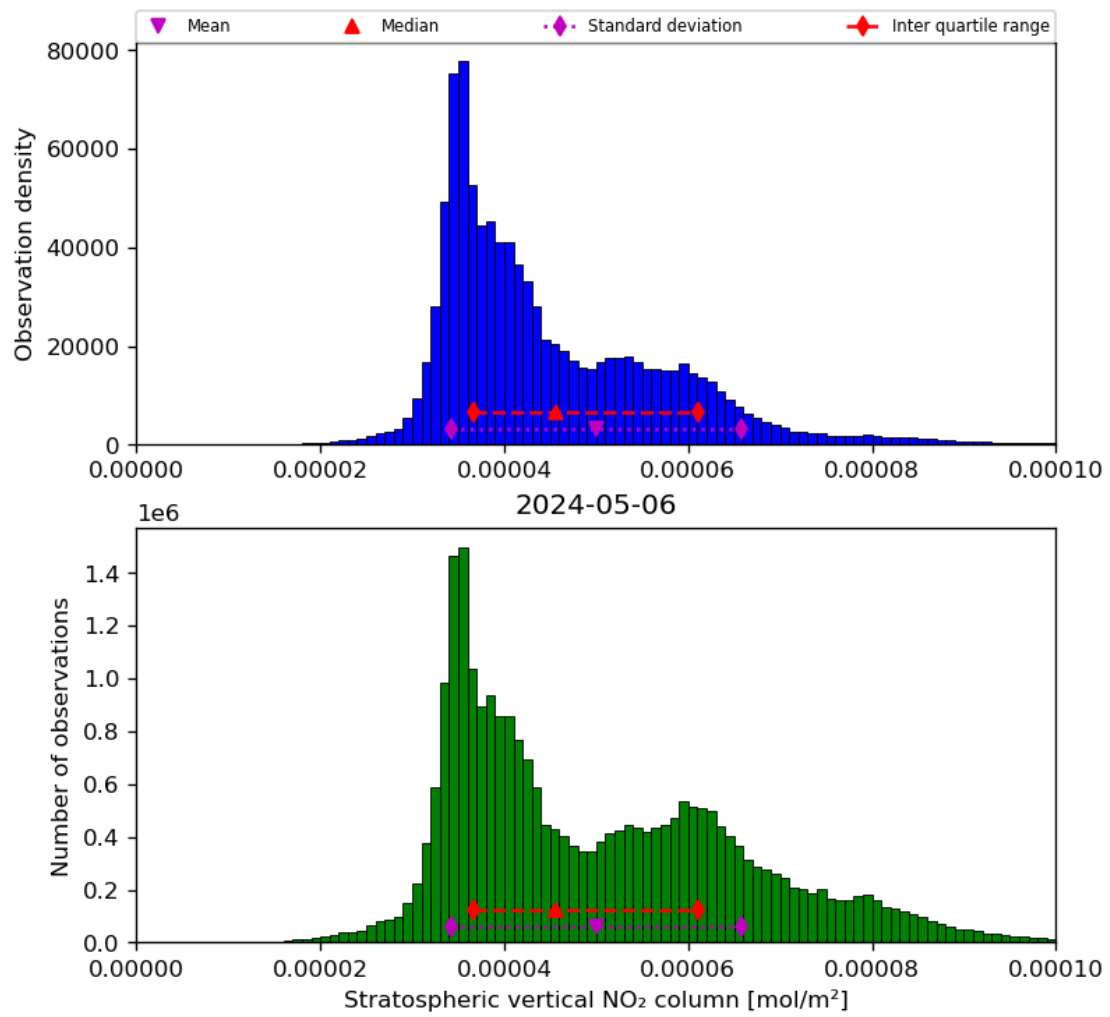
Figure 36: Histogram of “Stratospheric vertical NO 2 column” for 2024-05-05 to 2024-05-07
