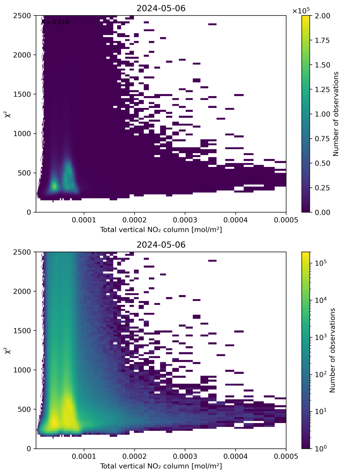
Figure 111: Scatter density plot of “Total vertical NO 2 column” against “ \chi^2 ” for 2024-05-05 to 2024-05-07.
