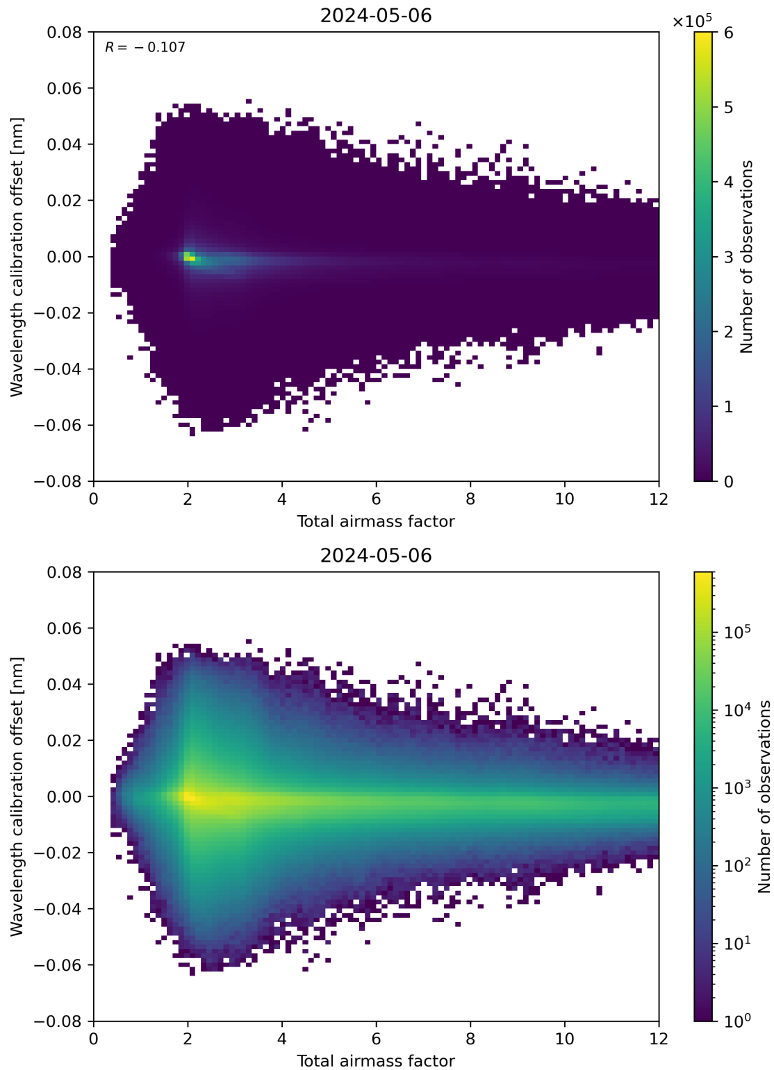
Figure 70: Scatter density plot of “Total airmass factor” against “Wavelength calibration offset” for 2024-05-05 to 2024-05-07.
