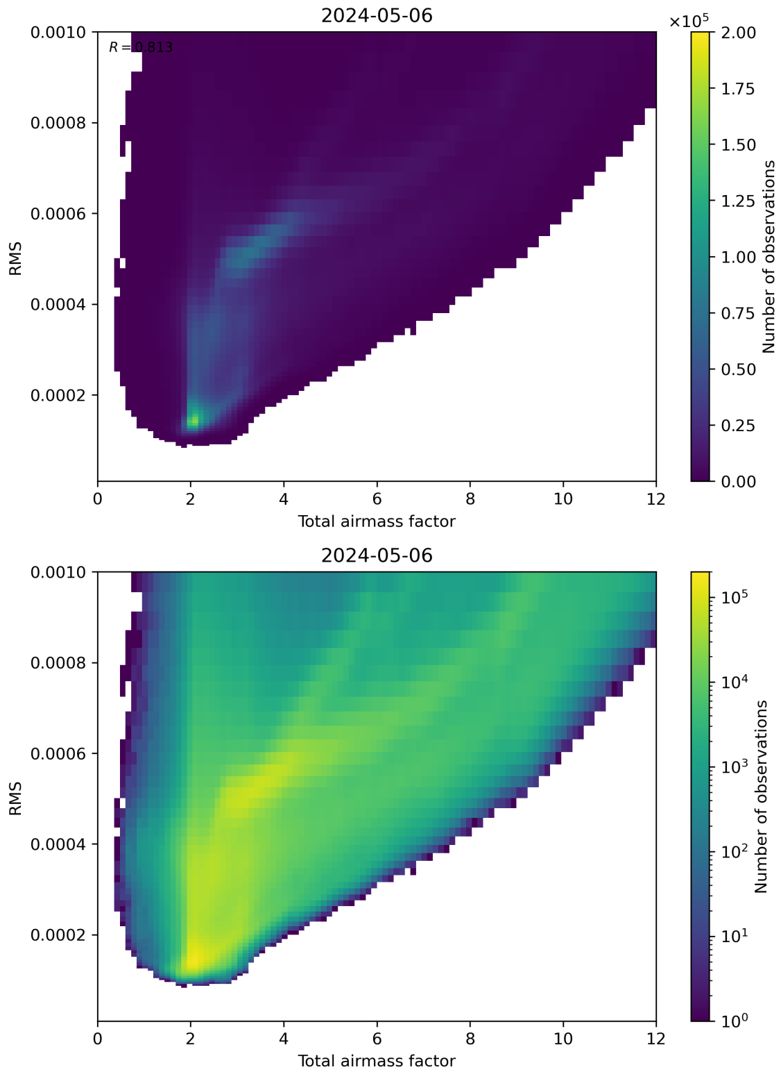
Figure 69: Scatter density plot of “Total airmass factor” against “RMS” for 2024-05-05 to 2024-05-07.
