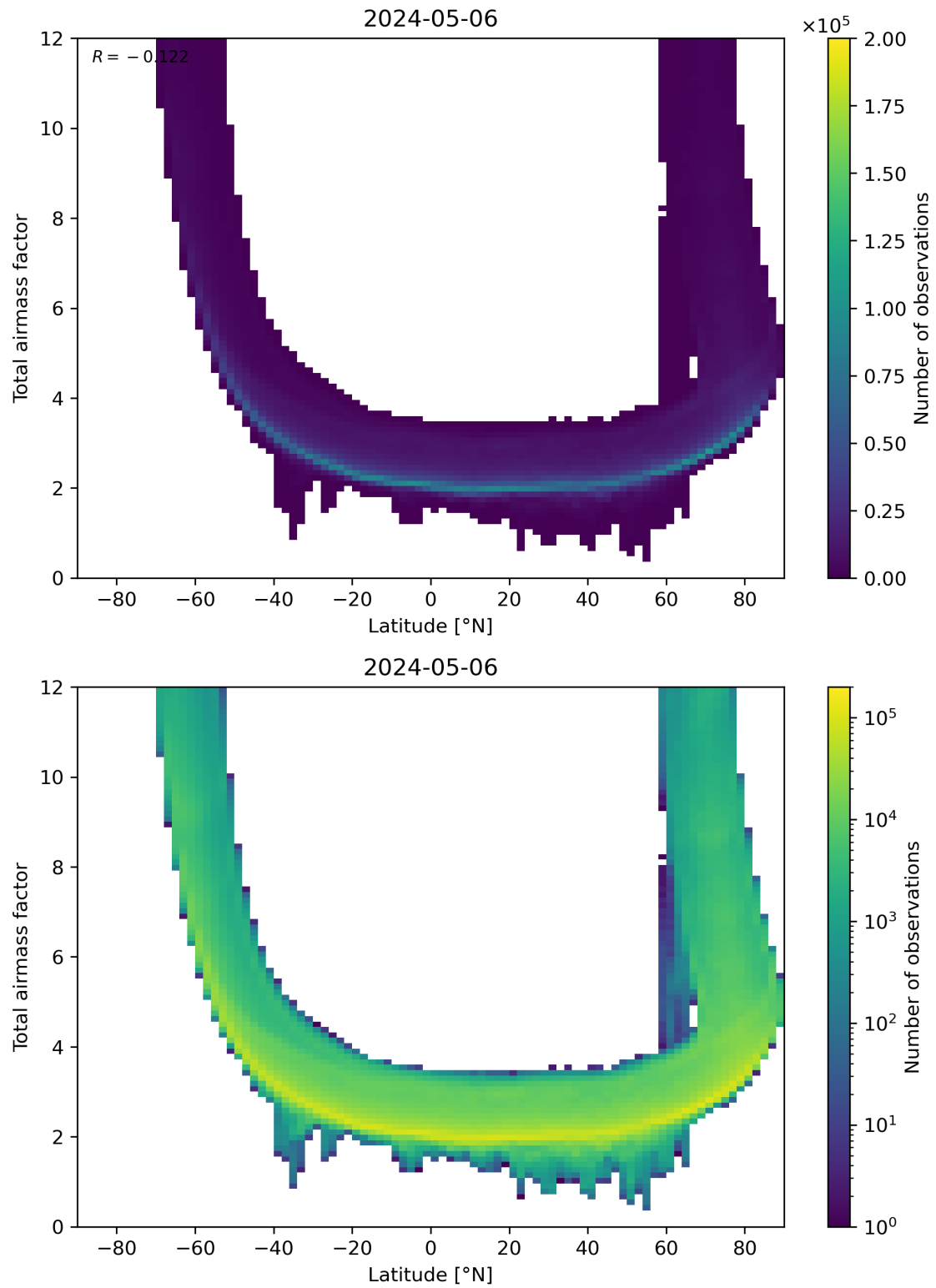
Figure 84: Scatter density plot of “Latitude” against “Total airmass factor” for 2024-05-05 to 2024-05-07.
