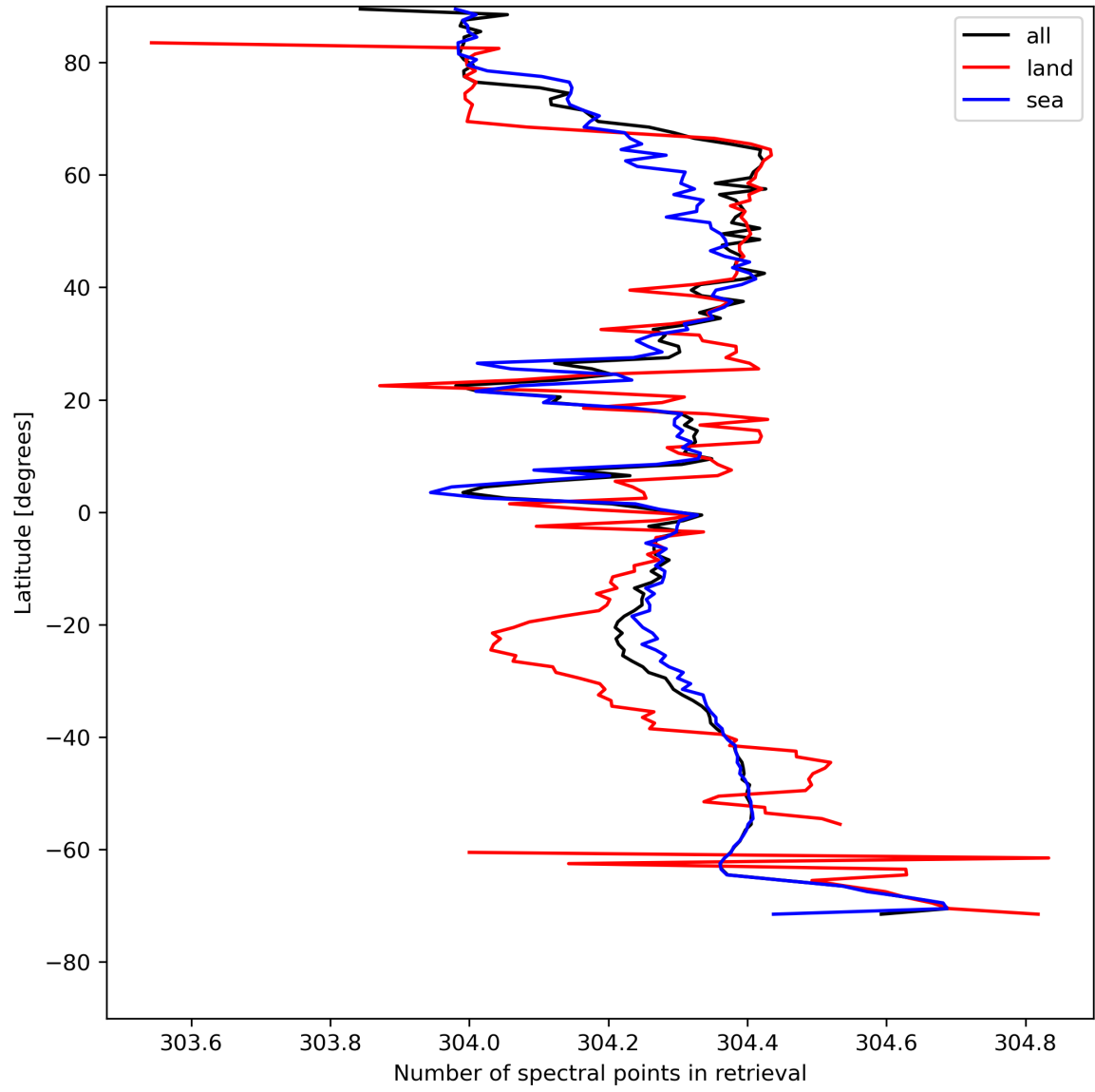
Figure 16: Zonal average of “Number of spectral points in retrieval” for 2024-05-05 to 2024-05-07.
