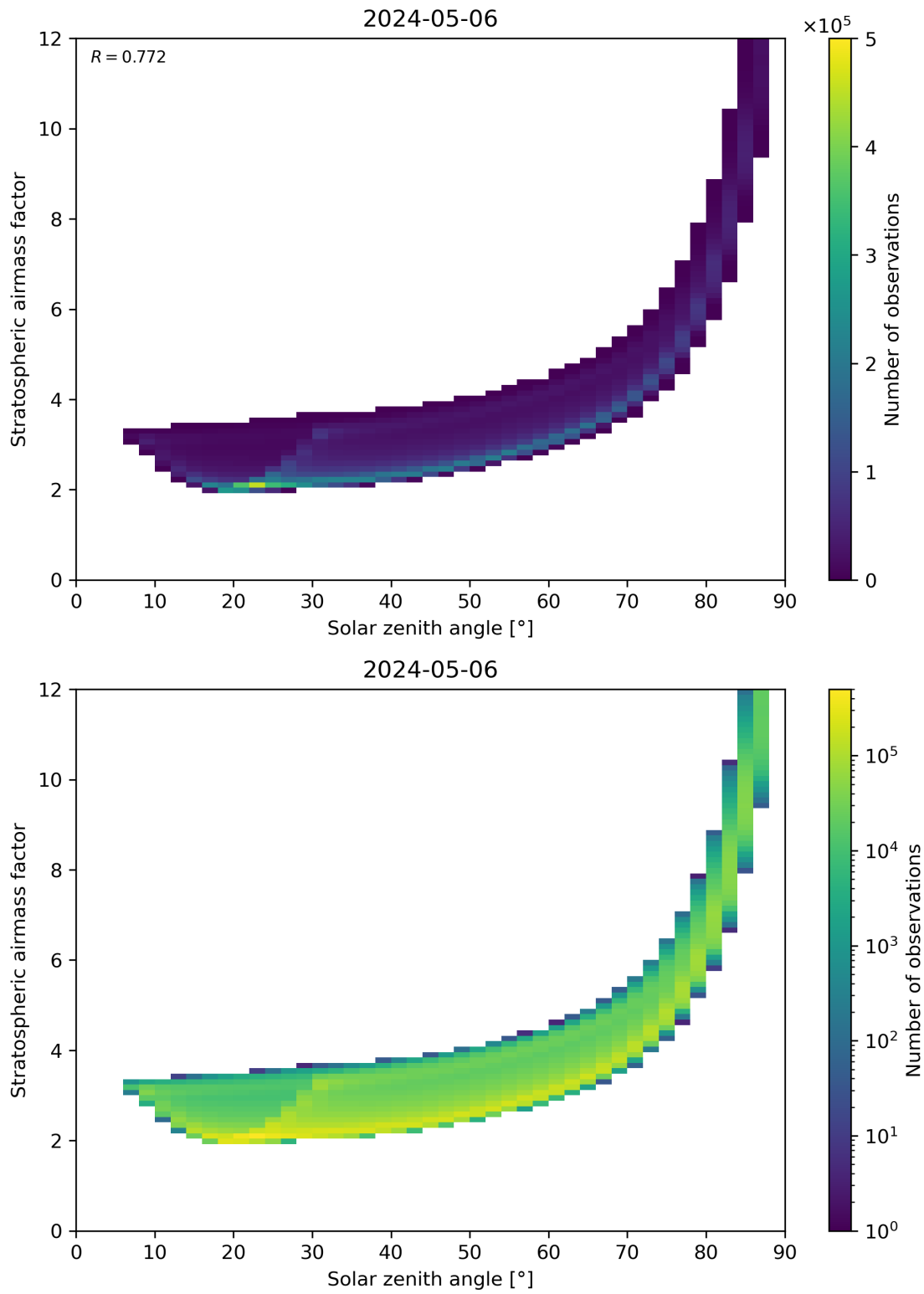
Figure 145: Scatter density plot of “Solar zenith angle” against “Stratospheric airmass factor” for 2024-05-05 to 2024-05-07.
