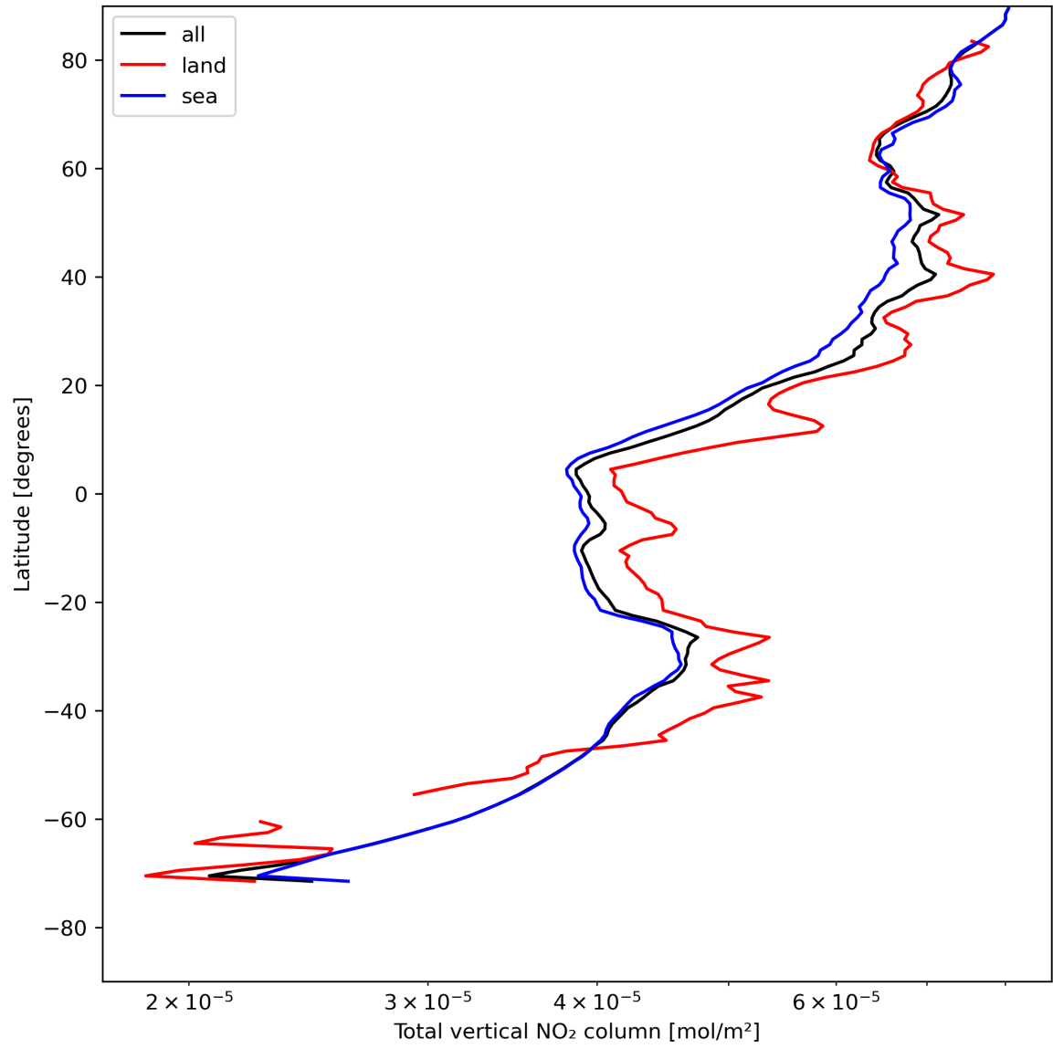
Figure 21: Zonal average of “Total vertical NO 2 column” for 2024-05-05 to 2024-05-07.
