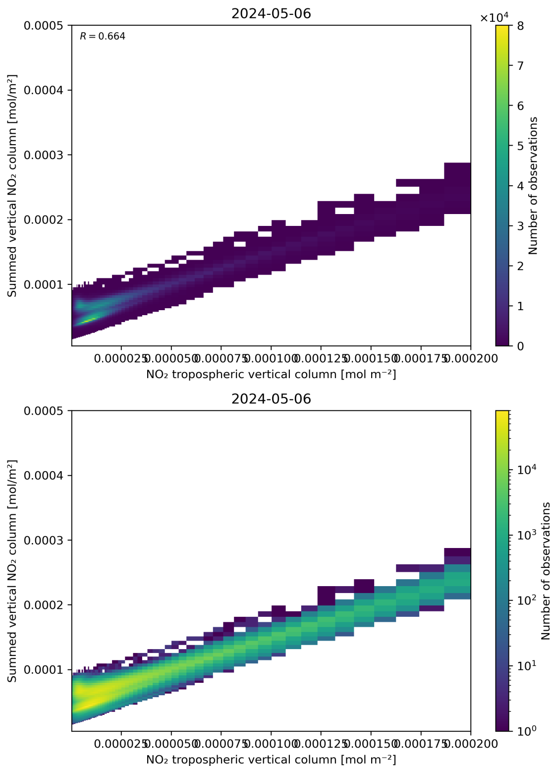
Figure 126: Scatter density plot of “NO 2 tropospheric vertical column” against “Summed vertical NO 2 column” for 2024-05-05 to 2024-05-07.
