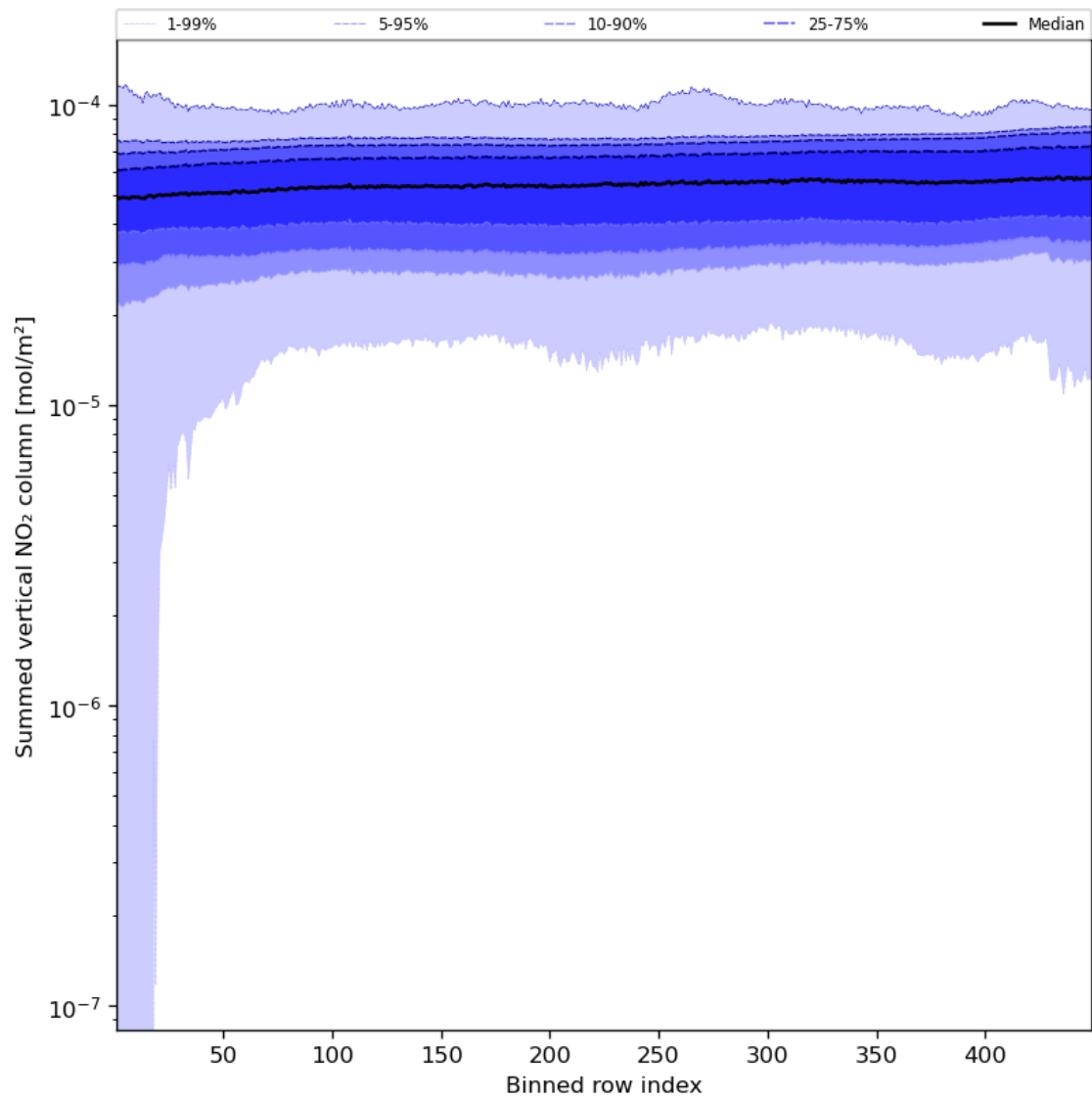
Figure 57: Along track statistics of “Summed vertical NO 2 column” for 2024-05-05 to 2024-05-07
