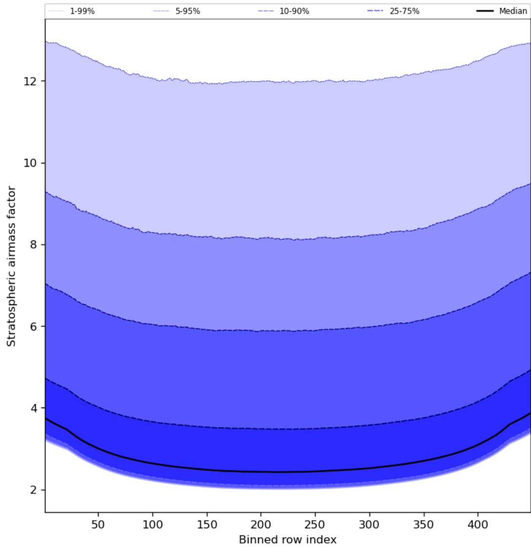
Figure 61: Along track statistics of “Stratospheric airmass factor” for 2024-05-05 to 2024-05-07
