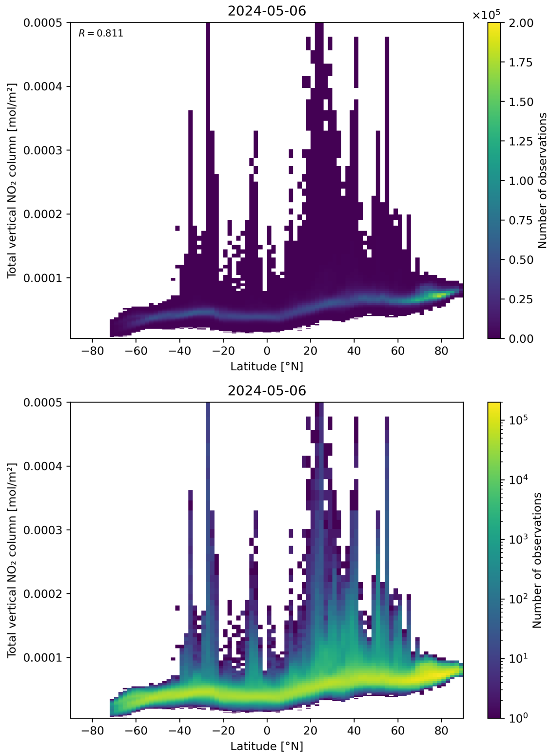
Figure 90: Scatter density plot of “Latitude” against “Total vertical NO 2 column” for 2024-05-05 to 2024-05-07.
