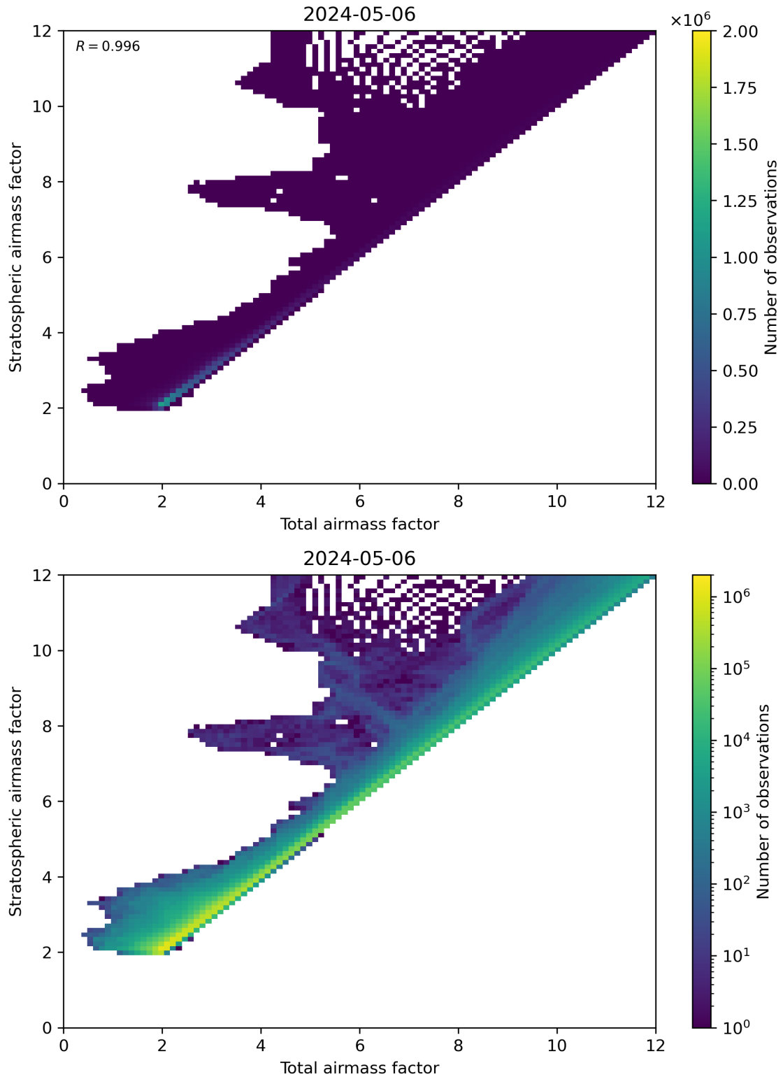
Figure 62: Scatter density plot of “Total airmass factor” against “Stratospheric airmass factor” for 2024-05-05 to 2024-05-07.
