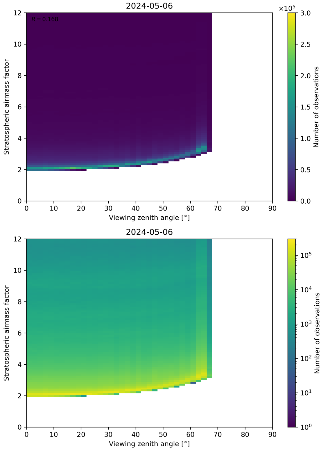
Figure 159: Scatter density plot of “Viewing zenith angle” against “Stratospheric airmass factor” for 2024-05-05 to 2024-05-07.
