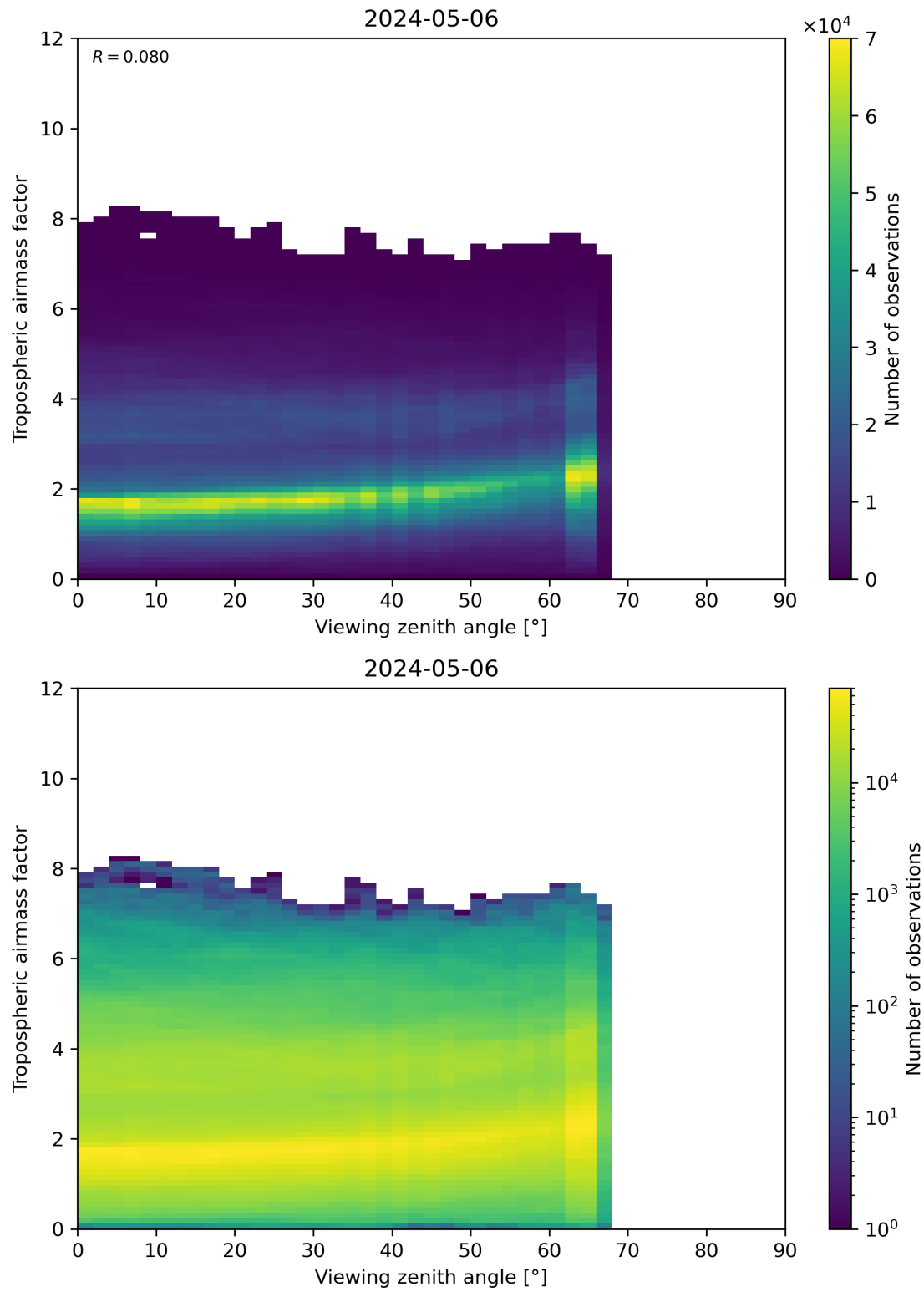
Figure 161: Scatter density plot of “Viewing zenith angle” against “Tropospheric airmass factor” for 2024-05-05 to 2024-05-07.
