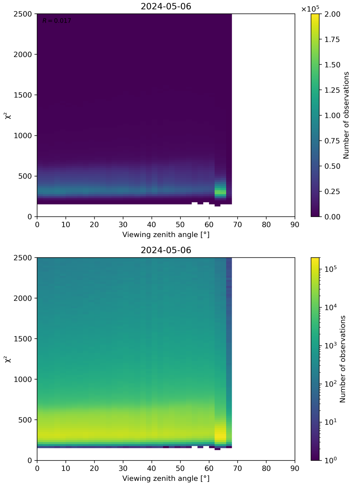
Figure 162: Scatter density plot of “Viewing zenith angle” against “ \chi^2 ” for 2024-05-05 to 2024-05-07.
