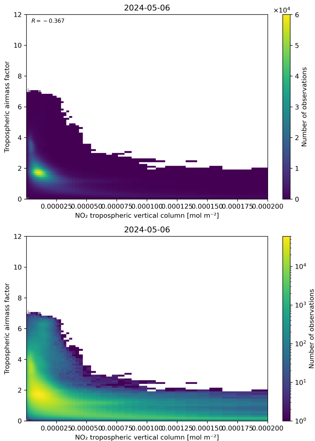
Figure 123: Scatter density plot of “NO 2 tropospheric vertical column” against “Tropospheric air mass factor” for 2024-05-05 to 2024-05-07.
