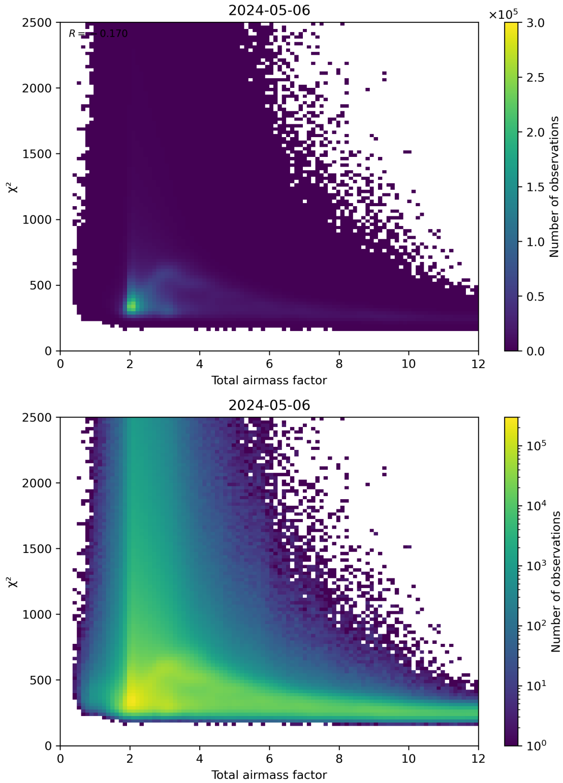
Figure 63: Scatter density plot of “Total airmass factor” against “ \chi^2 ” for 2024-05-05 to 2024-05-07.
