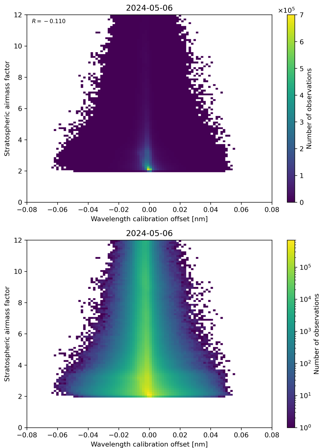
Figure 174: Scatter density plot of “Wavelength calibration offset” against “Stratospheric airmass factor” for 2024-05-05 to 2024-05-07.
