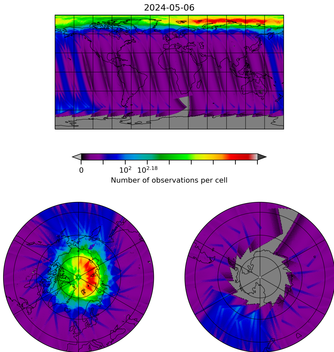
Figure 10: Map of the number of observations for 2024-05-05 to 2024-05-07
