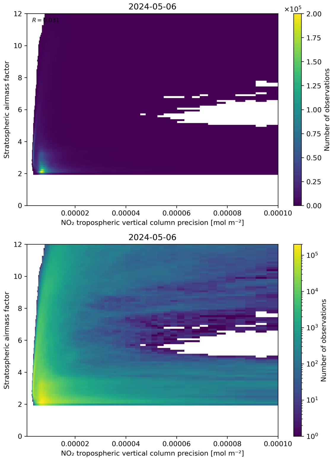
Figure 131: Scatter density plot of “NO 2 tropospheric vertical column precision” against “Stratospheric airmass factor” for 2024-05-05 to 2024-05-07.
