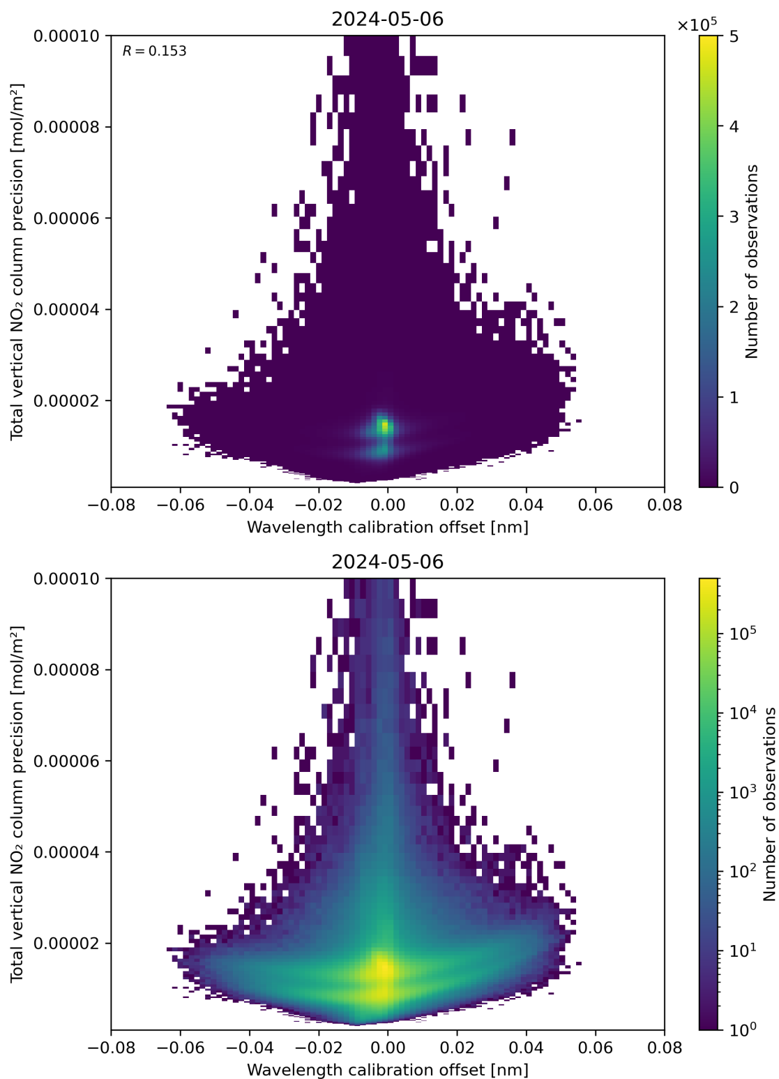
Figure 180: Scatter density plot of “Wavelength calibration offset” against “Total vertical NO 2 column precision” for 2024-05-05 to 2024-05-07.
