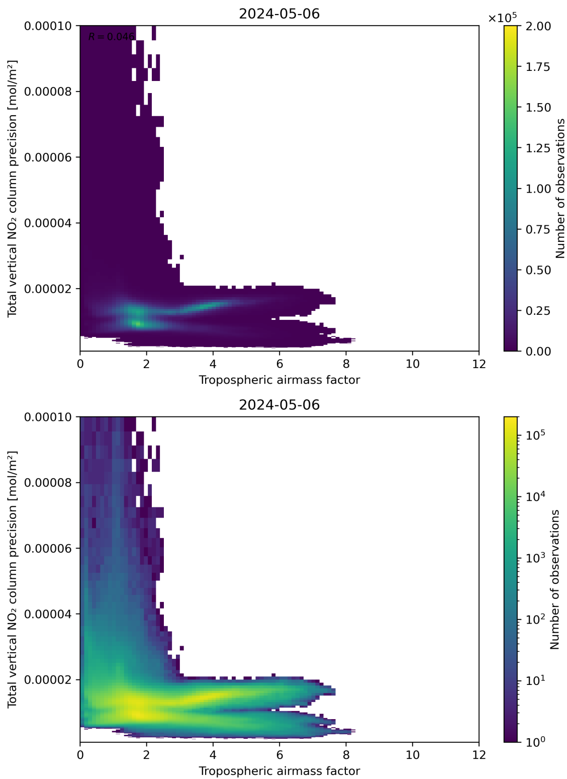
Figure 78: Scatter density plot of “Tropospheric air mass factor” against “Total vertical NO 2 column precision” for 2024-05-05 to 2024-05-07.
