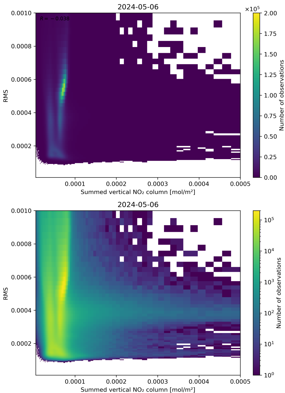
Figure 109: Scatter density plot of “Summed vertical NO 2 column” against “RMS” for 2024-05-05 to 2024-05-07.
