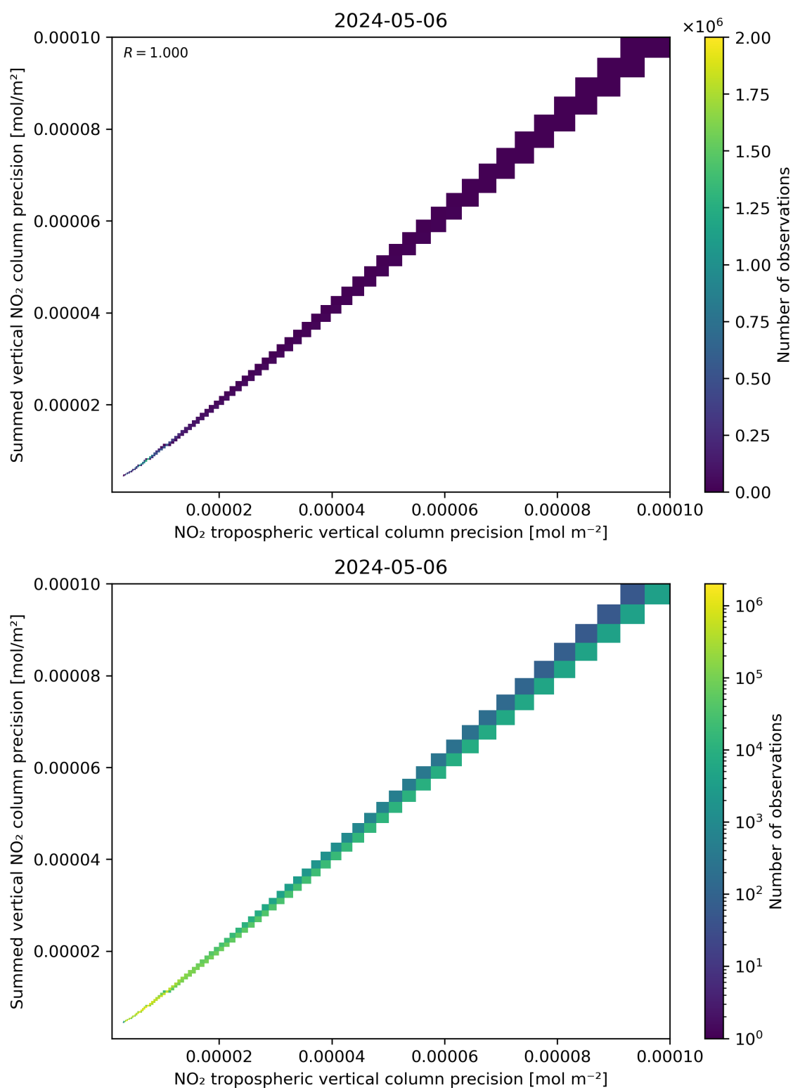
Figure 137: Scatter density plot of “NO 2 tropospheric vertical column precision” against “Summed vertical NO 2 column precision” for 2024-05-05 to 2024-05-07.
