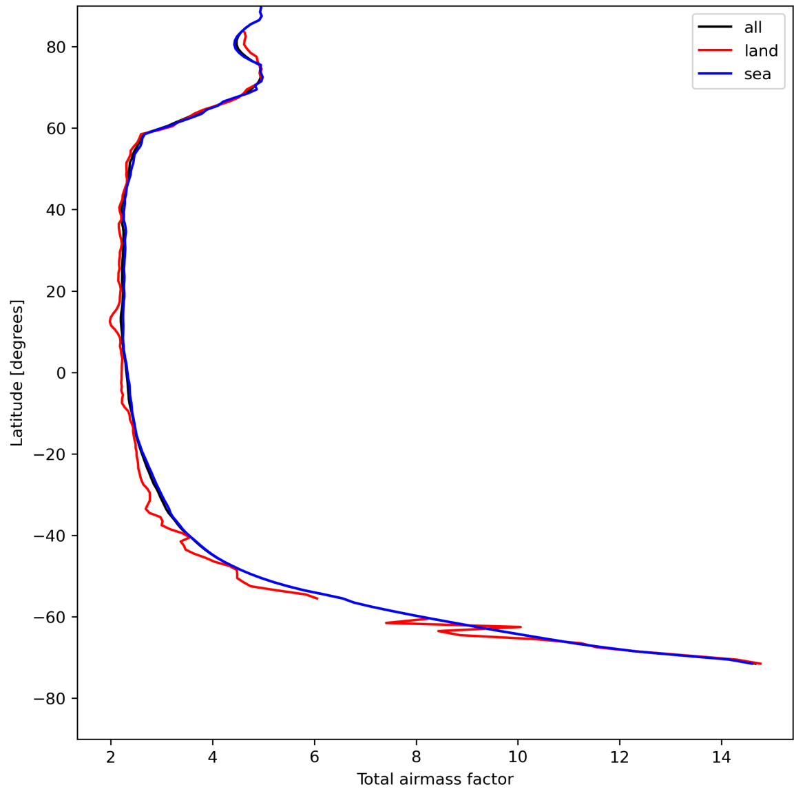
Figure 15: Zonal average of “Total airmass factor” for 2024-05-05 to 2024-05-07.
