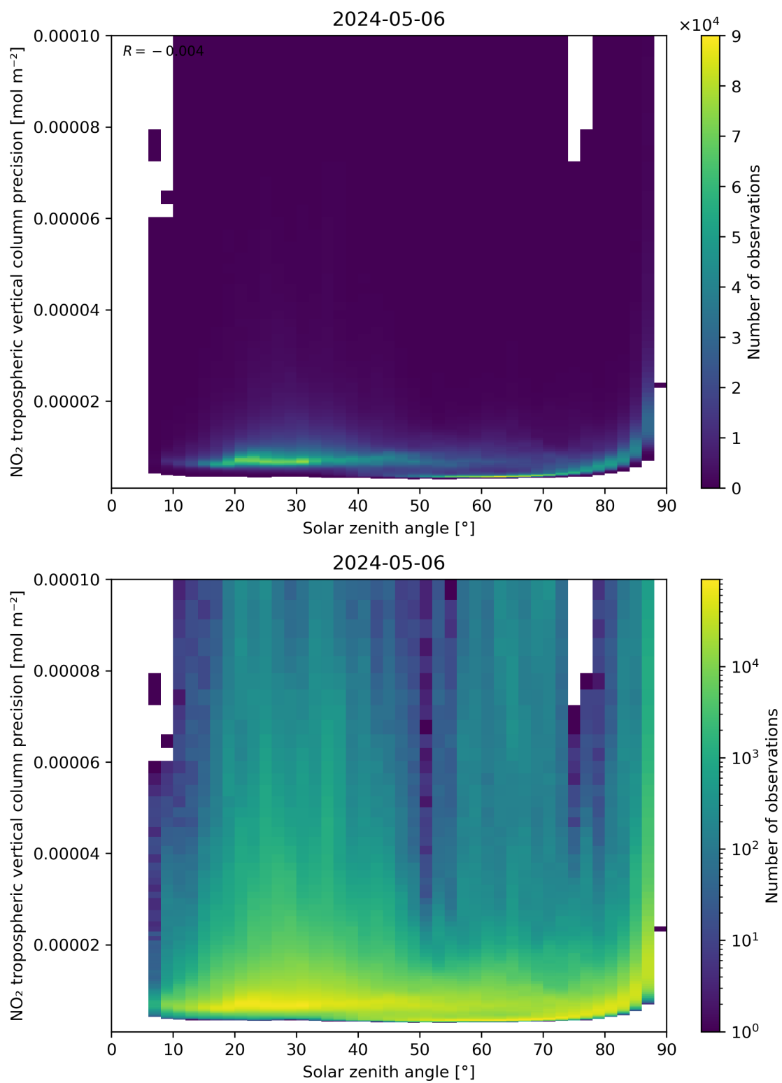
Figure 156: Scatter density plot of “Solar zenith angle” against “NO 2 tropospheric vertical column precision” for 2024-05-05 to 2024-05-07.
