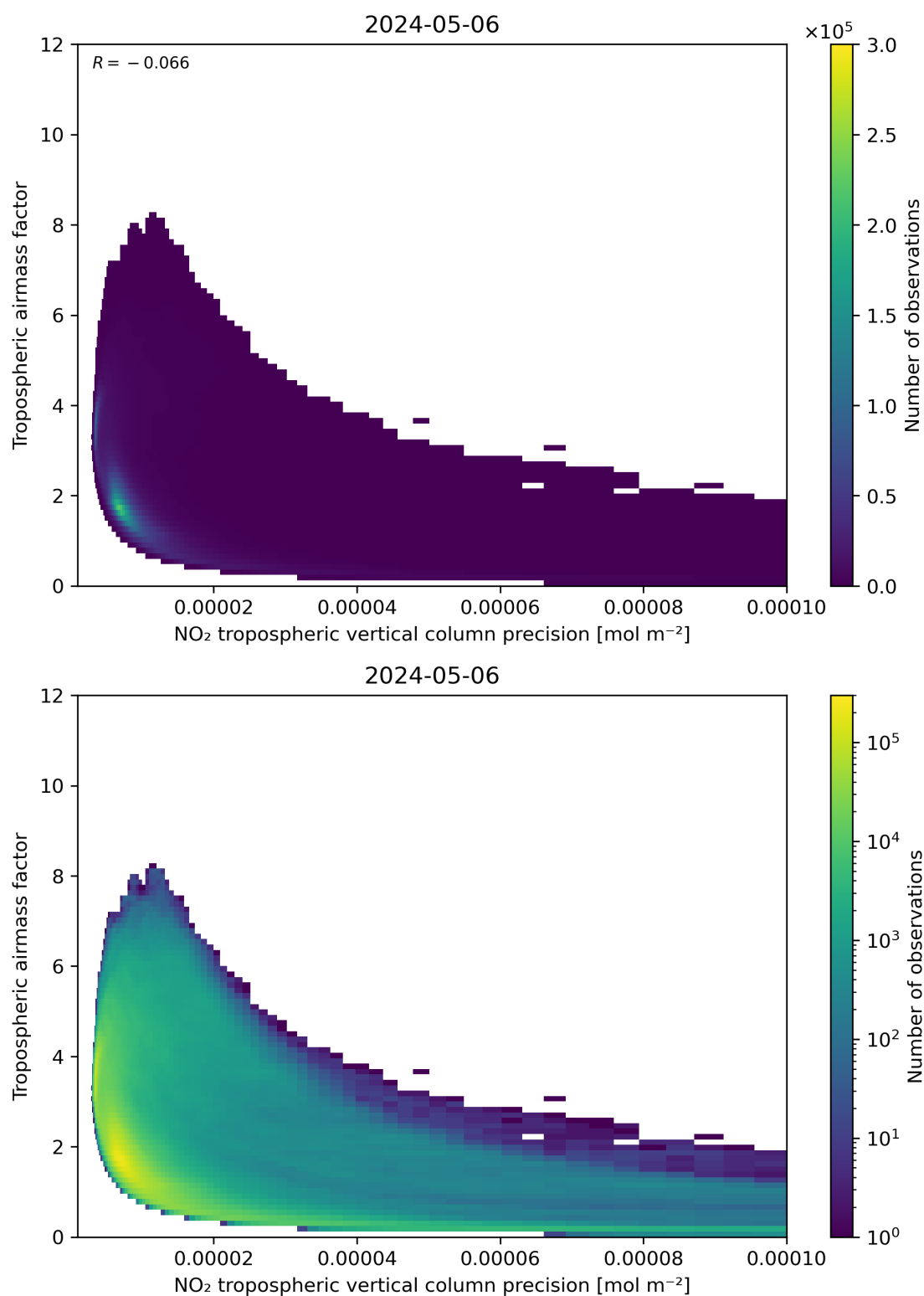
Figure 133: Scatter density plot of “NO 2 tropospheric vertical column precision” against “Tropospheric airmass factor” for 2024-05-05 to 2024-05-07.
