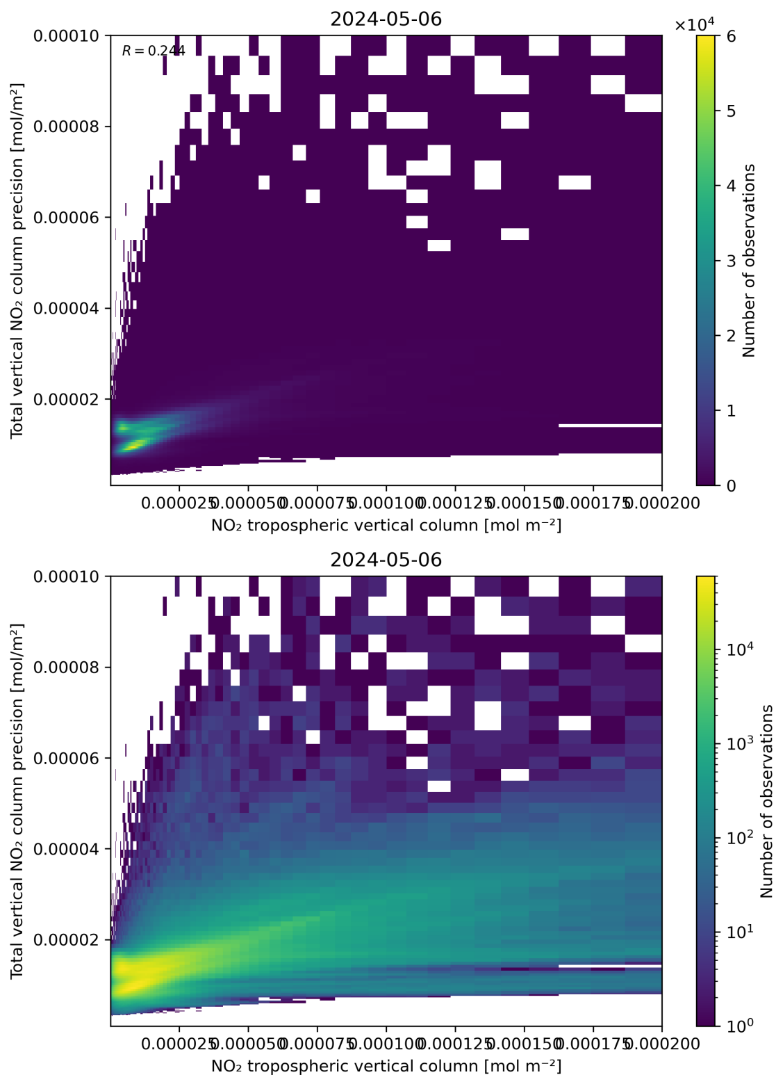
Figure 129: Scatter density plot of “NO 2 tropospheric vertical column” against “Total vertical NO 2 column precision” for 2024-05-05 to 2024-05-07.
