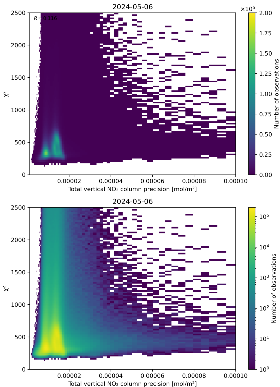
Figure 116: Scatter density plot of “Total vertical NO 2 column precision” against “ \chi^2 ” for 2024-05-05 to 2024-05-07.
