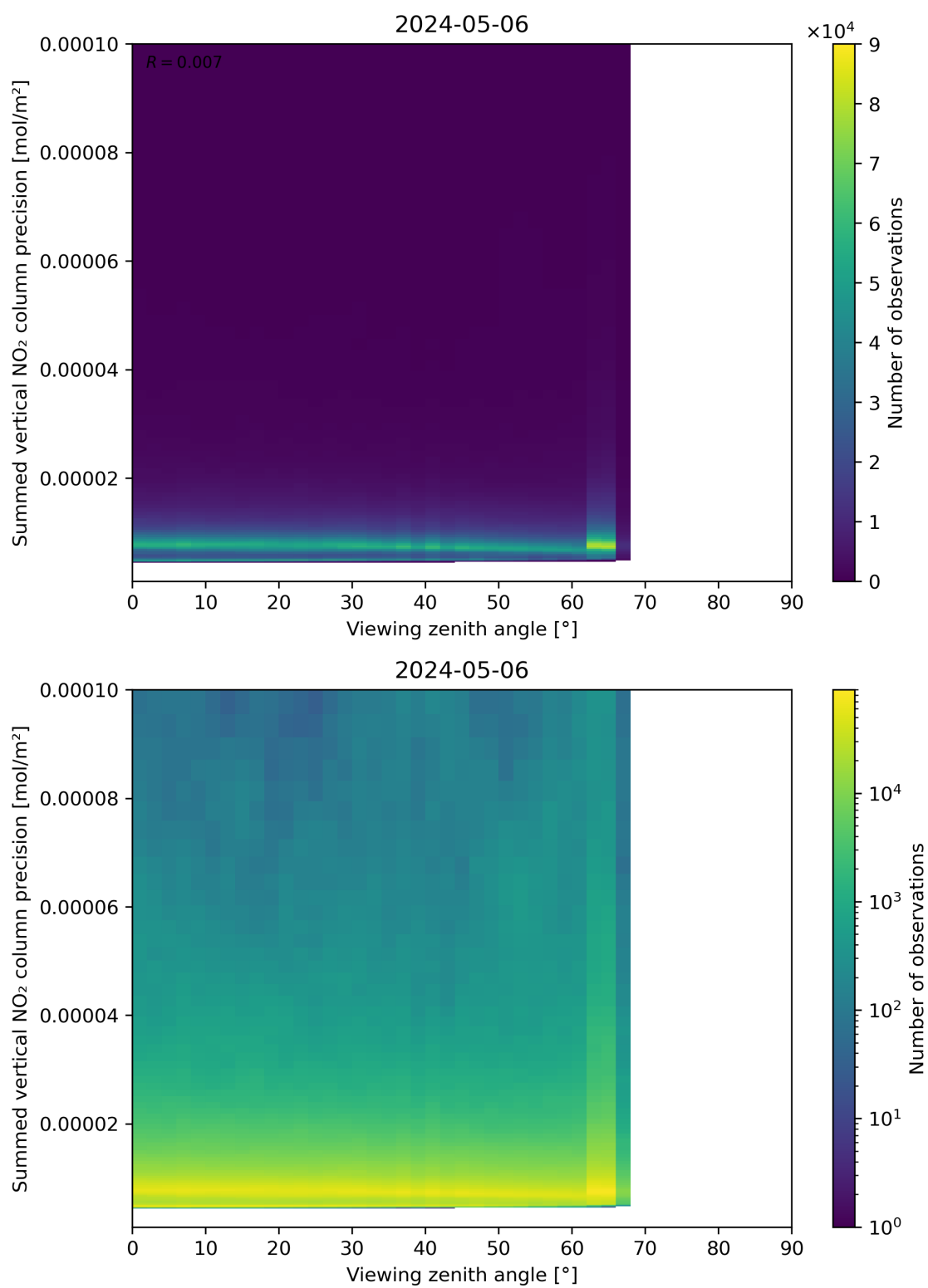
Figure 166: Scatter density plot of “Viewing zenith angle” against “Summed vertical NO 2 column precision” for 2024-05-05 to 2024-05-07.
