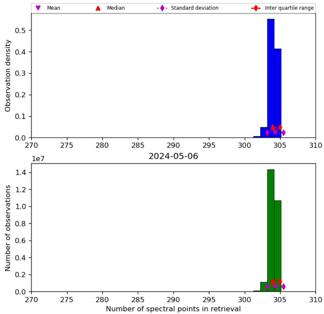
Figure 33: Histogram of “Number of spectral points in retrieval” for 2024-05-05 to 2024-05-07
