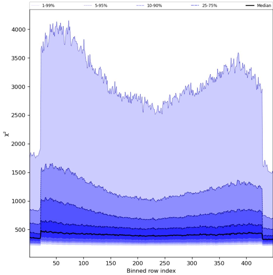
Figure 59: Along track statistics of “ \chi^2 ” for 2024-05-05 to 2024-05-07
