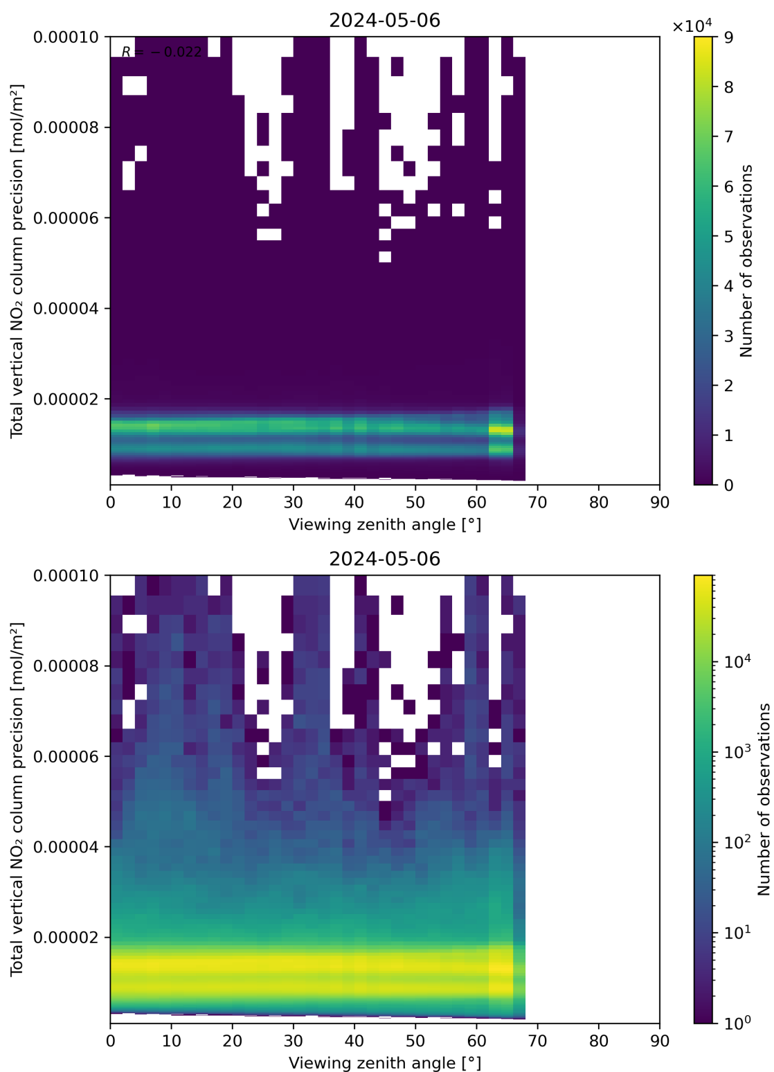
Figure 168: Scatter density plot of “Viewing zenith angle” against “Total vertical NO 2 column precision” for 2024-05-05 to 2024-05-07.
