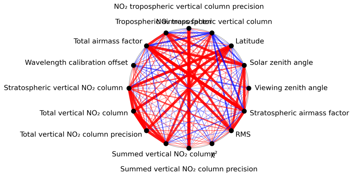
Figure 1: Map of correlation graph for 2024-05-05 to 2024-05-07.
