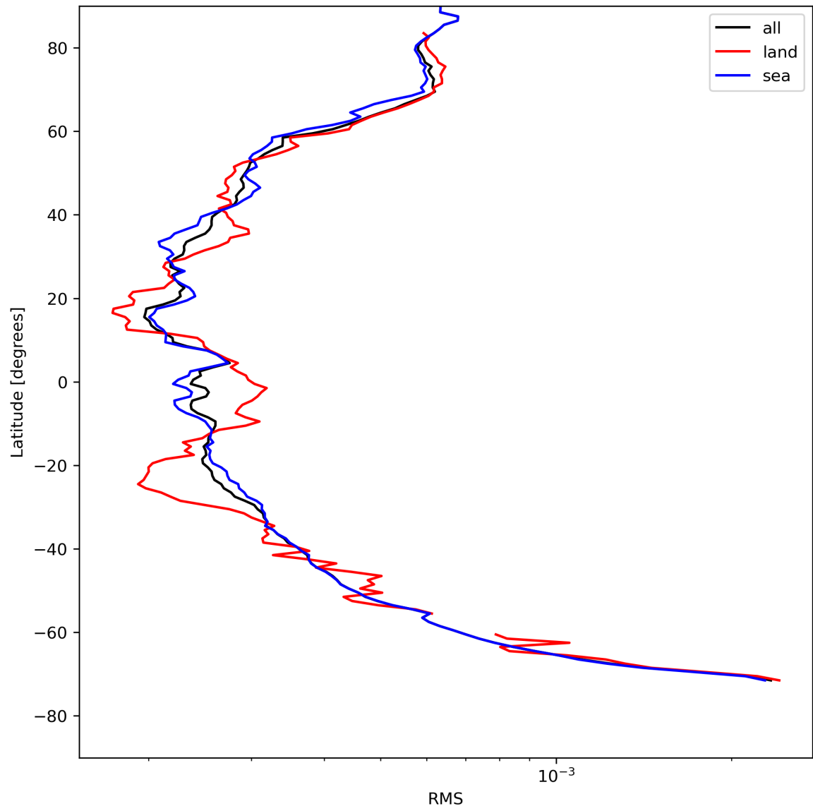
Figure 26: Zonal average of “RMS” for 2024-05-05 to 2024-05-07.
