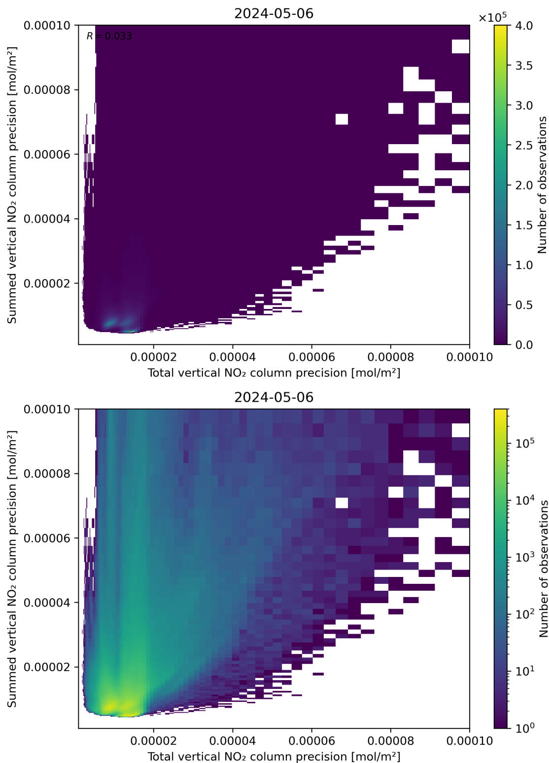
Figure 118: Scatter density plot of “Total vertical NO 2 column precision” against “Summed vertical NO 2 column precision” for 2024-05-05 to 2024-05-07.
