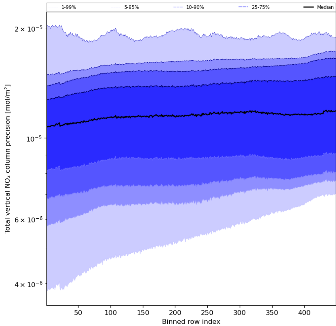
Figure 56: Along track statistics of “Total vertical NO 2 column precision” for 2024-05-05 to 2024-05-07
