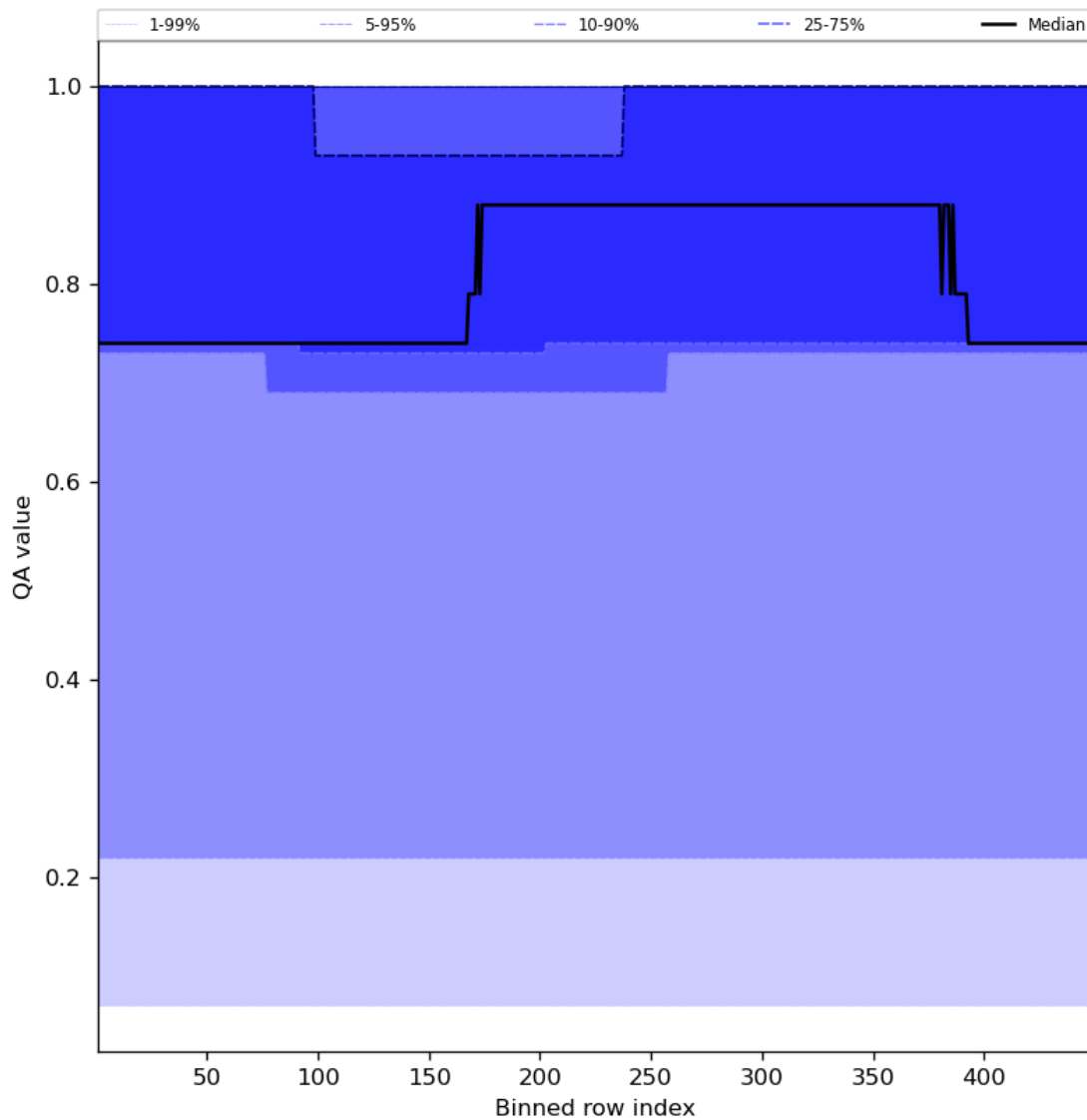
Figure 45: Along track statistics of “QA value” for 2024-05-05 to 2024-05-07
