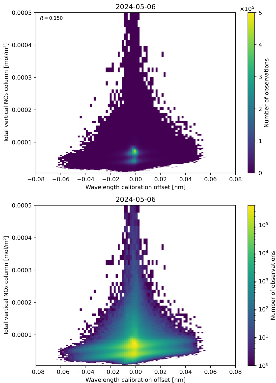
Figure 179: Scatter density plot of “Wavelength calibration offset” against “Total vertical NO 2 column” for 2024-05-05 to 2024-05-07.
