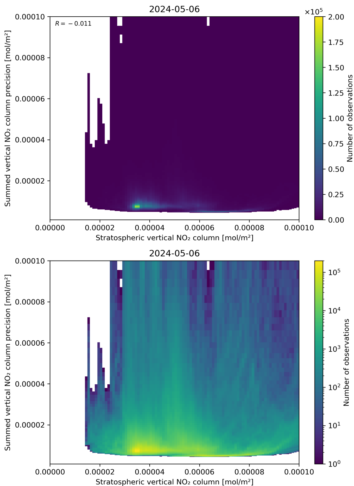
Figure 99: Scatter density plot of “Stratospheric vertical NO 2 column” against “Summed vertical NO 2 column precision” for 2024-05-05 to 2024-05-07.
