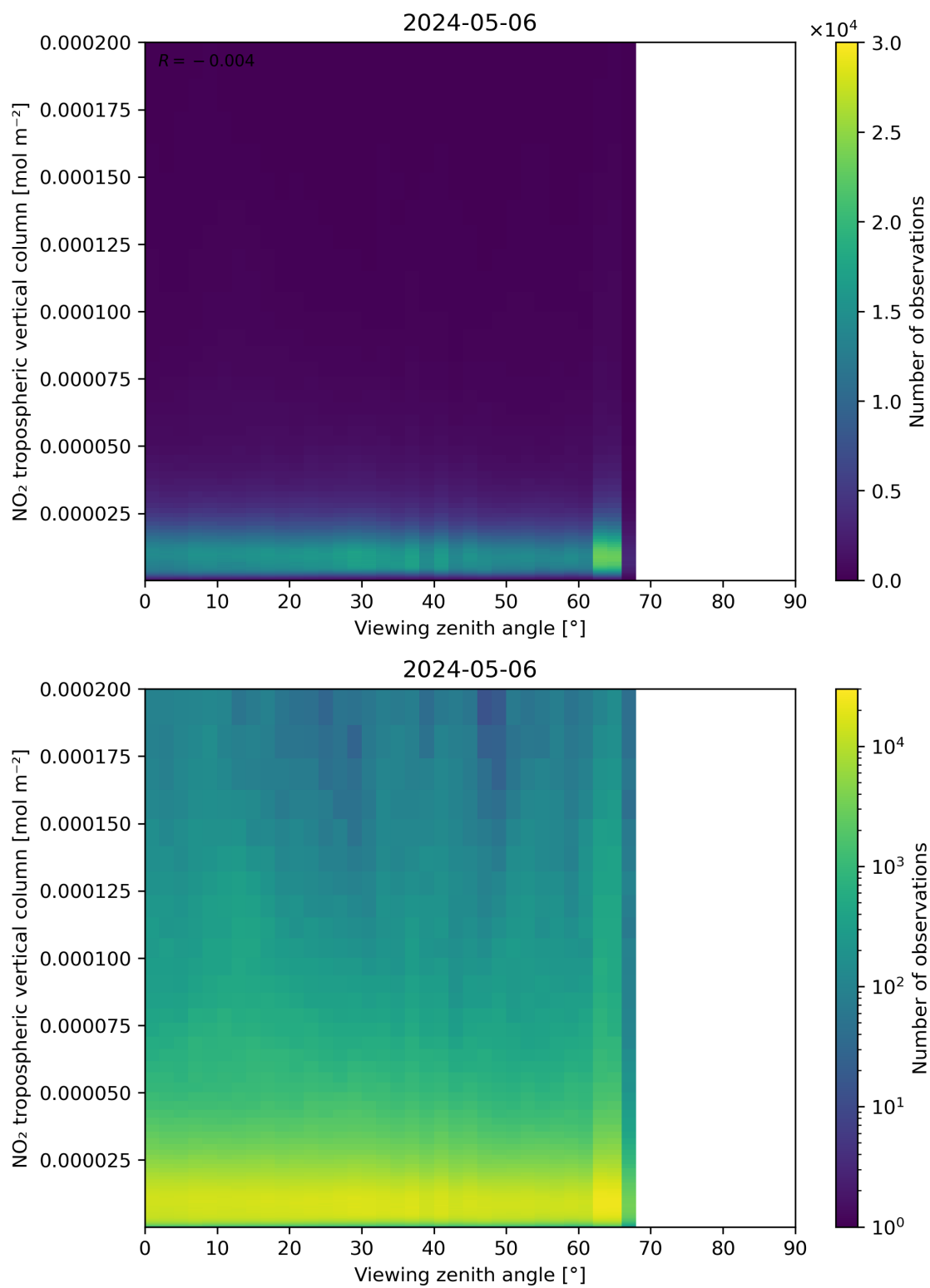
Figure 169: Scatter density plot of “Viewing zenith angle” against “NO 2 tropospheric vertical column” for 2024-05-05 to 2024-05-07.
