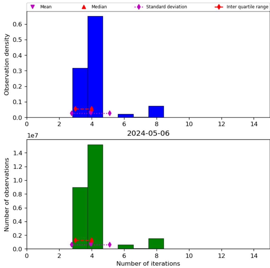
Figure 34: Histogram of “Number of iterations” for 2024-05-05 to 2024-05-07
