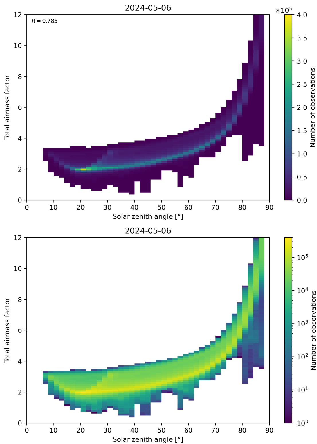
Figure 146: Scatter density plot of “Solar zenith angle” against “Total air mass factor” for 2024-05-05 to 2024-05-07.
