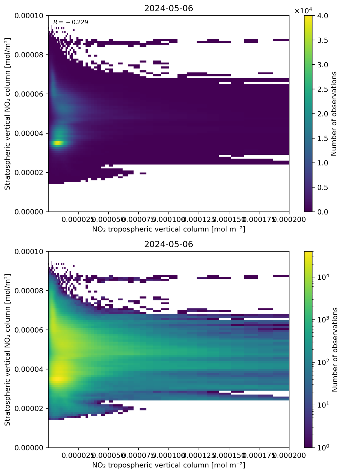
Figure 125: Scatter density plot of “NO 2 tropospheric vertical column” against “Stratospheric vertical NO 2 column” for 2024-05-05 to 2024-05-07.
