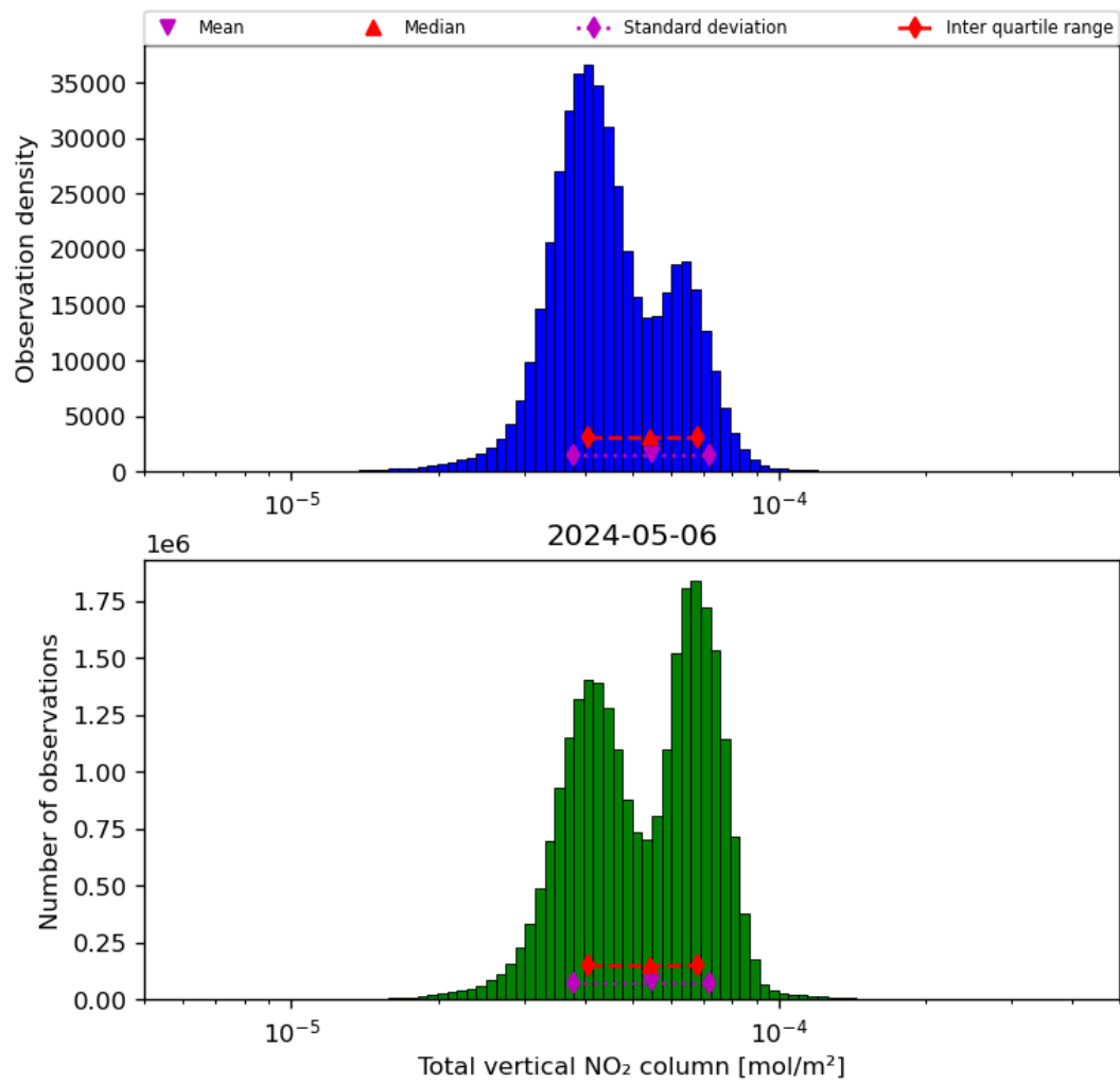
Figure 38: Histogram of “Total vertical NO 2 column” for 2024-05-05 to 2024-05-07
