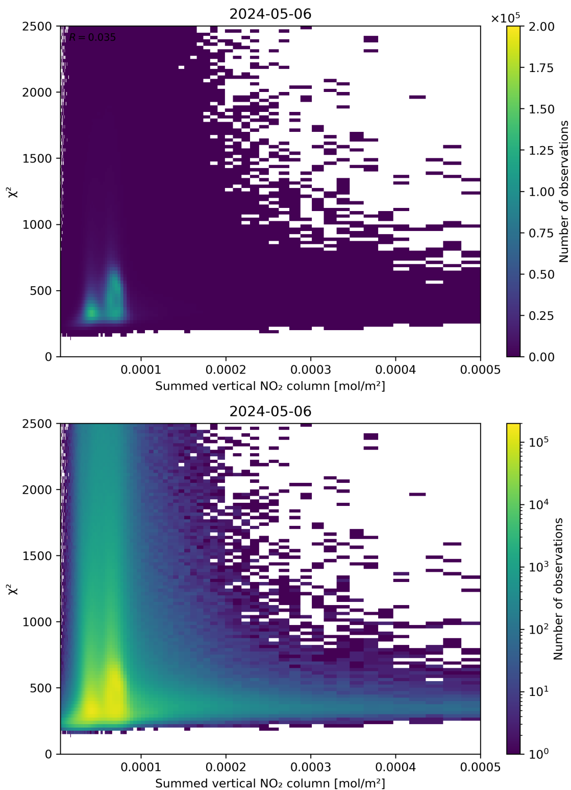
Figure 104: Scatter density plot of “Summed vertical NO 2 column” against “ \chi^2 ” for 2024-05-05 to 2024-05-07.
