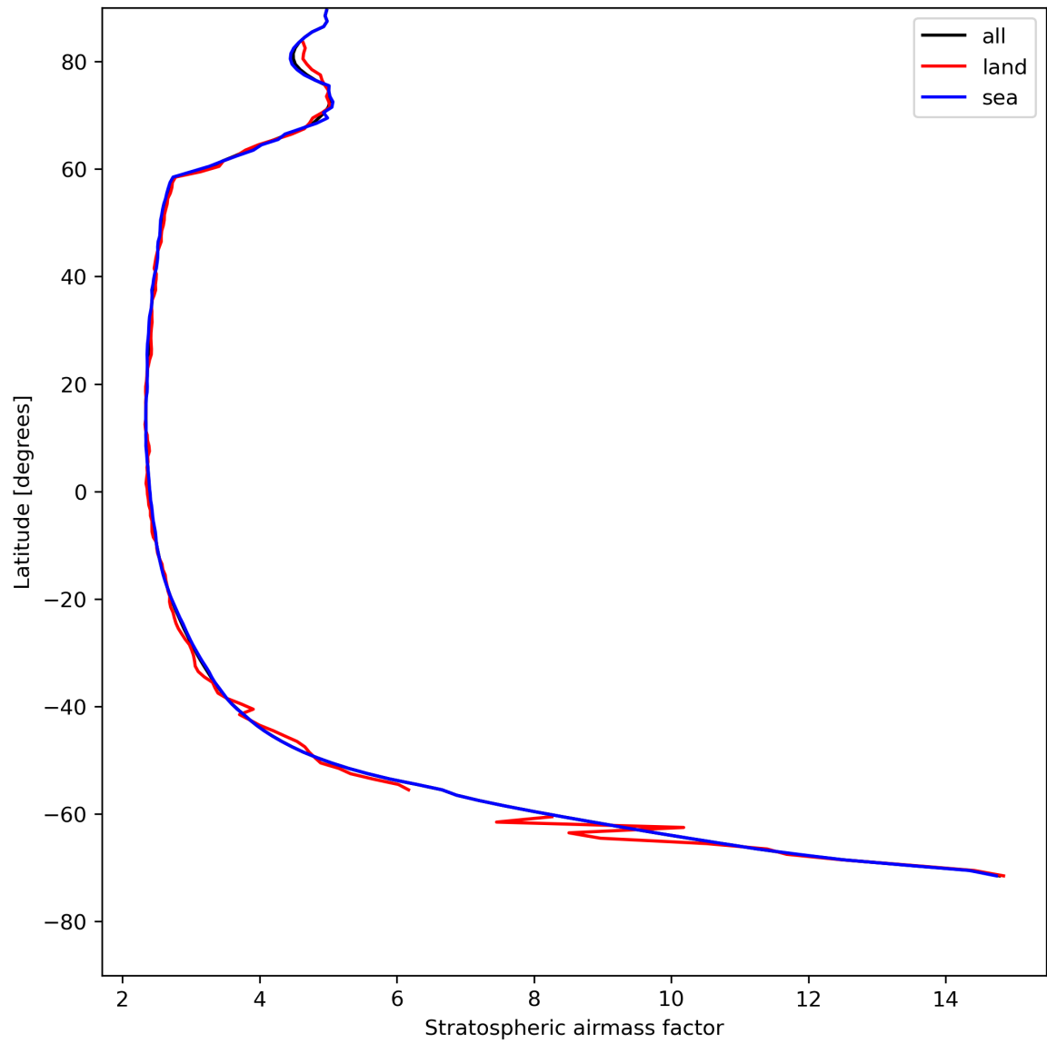
Figure 27: Zonal average of “Stratospheric airmass factor” for 2024-05-05 to 2024-05-07.
