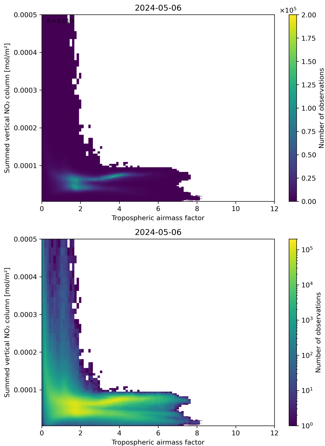
Figure 75: Scatter density plot of “Tropospheric air mass factor” against “Summed vertical NO 2 column” for 2024-05-05 to 2024-05-07.
