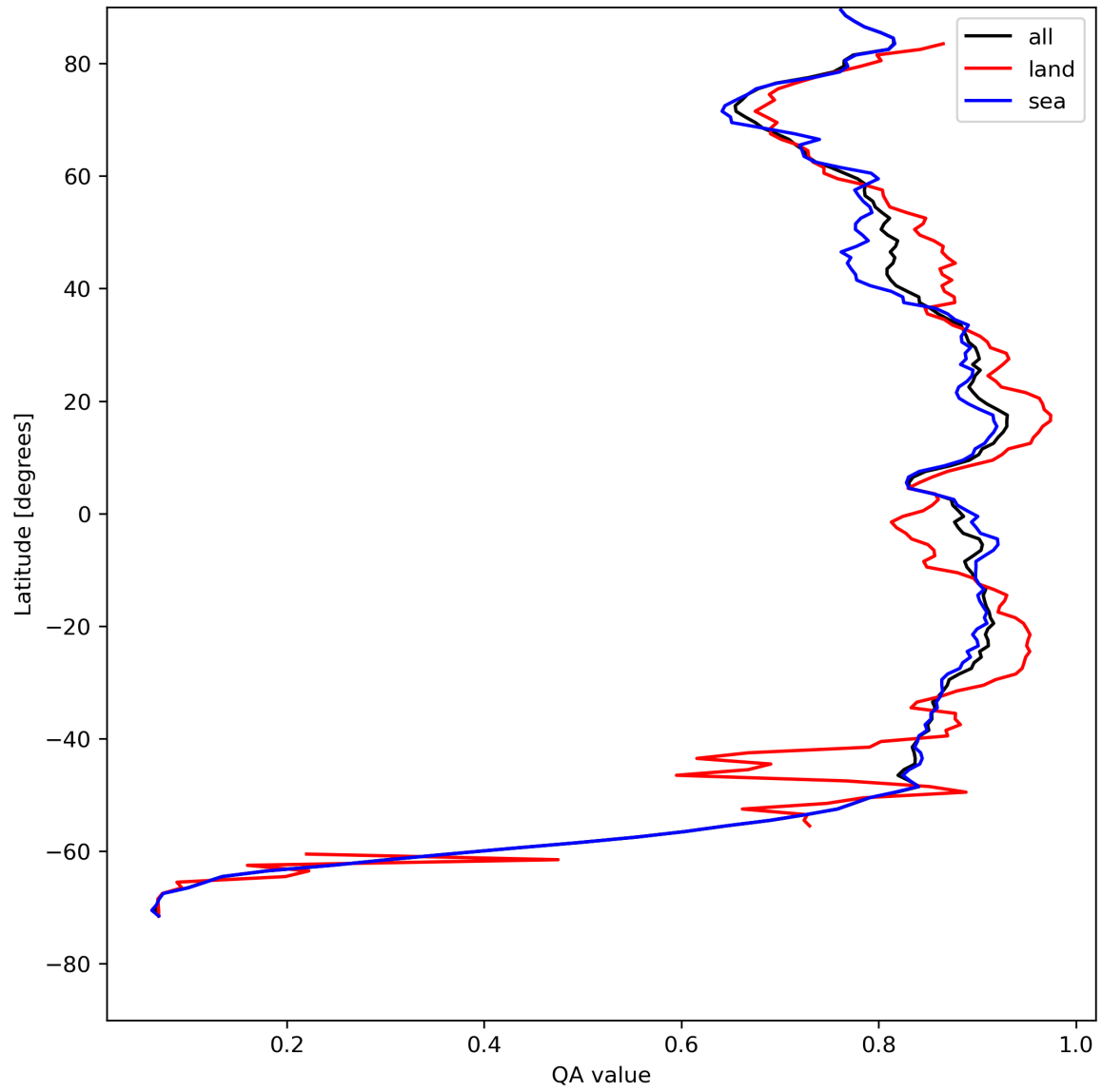
Figure 11: Zonal average of “QA value” for 2024-05-05 to 2024-05-07.
