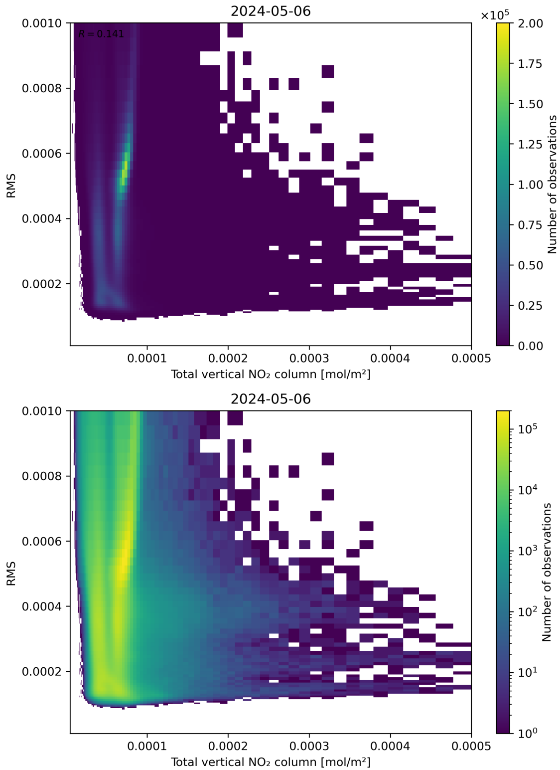
Figure 120: Scatter density plot of “Total vertical NO 2 column” against “RMS” for 2024-05-05 to 2024-05-07.
