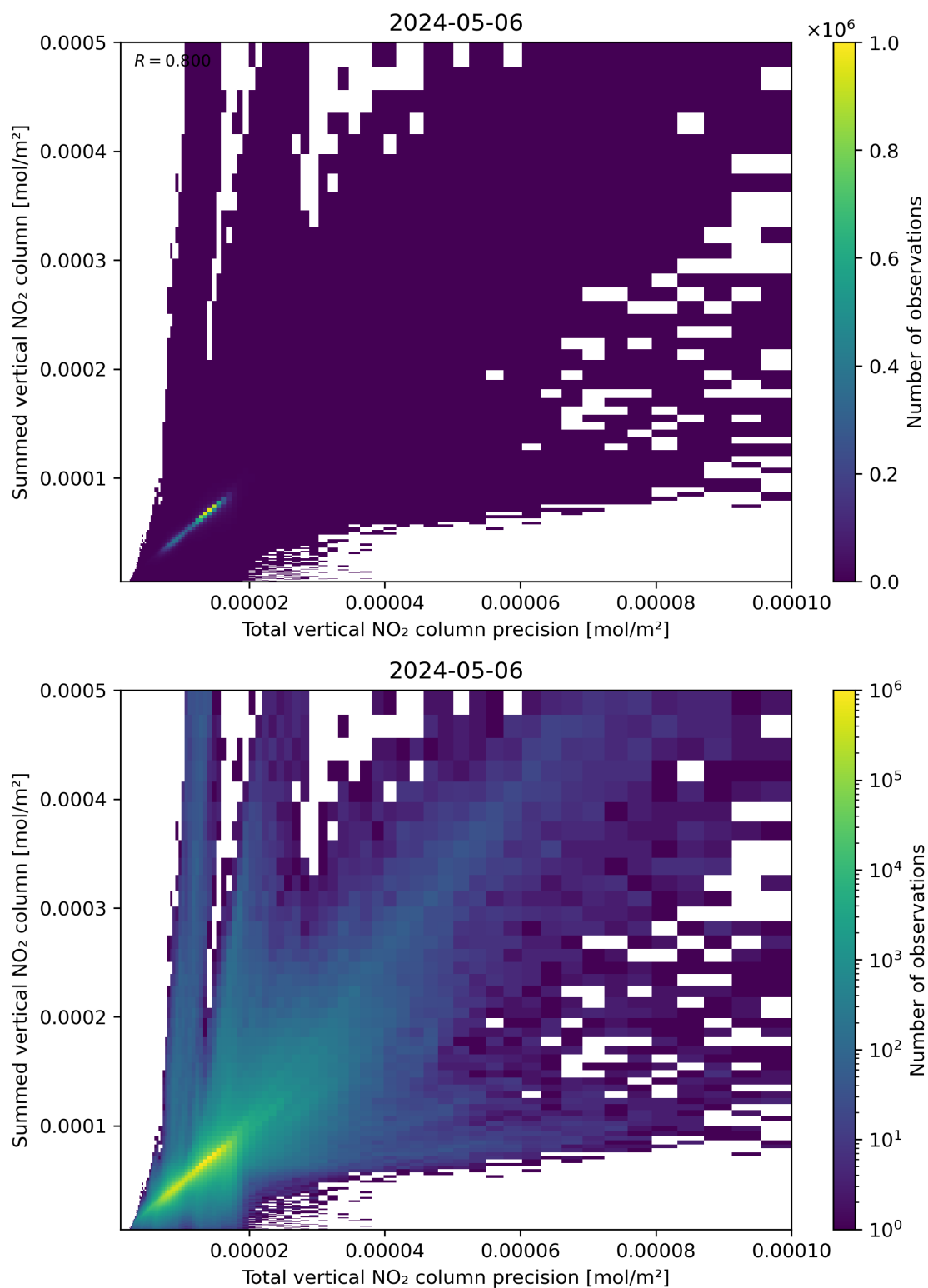
Figure 117: Scatter density plot of “Total vertical NO 2 column precision” against “Summed vertical NO 2 column” for 2024-05-05 to 2024-05-07.
