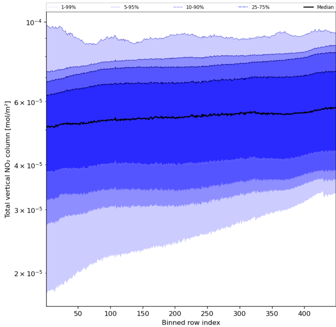
Figure 55: Along track statistics of “Total vertical NO 2 column” for 2024-05-05 to 2024-05-07
