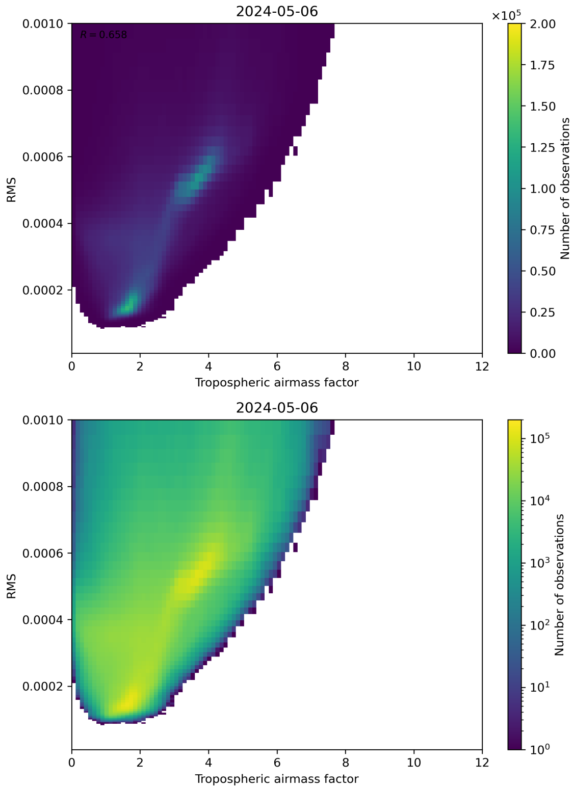
Figure 79: Scatter density plot of “Tropospheric airmass factor” against “RMS” for 2024-05-05 to 2024-05-07.
