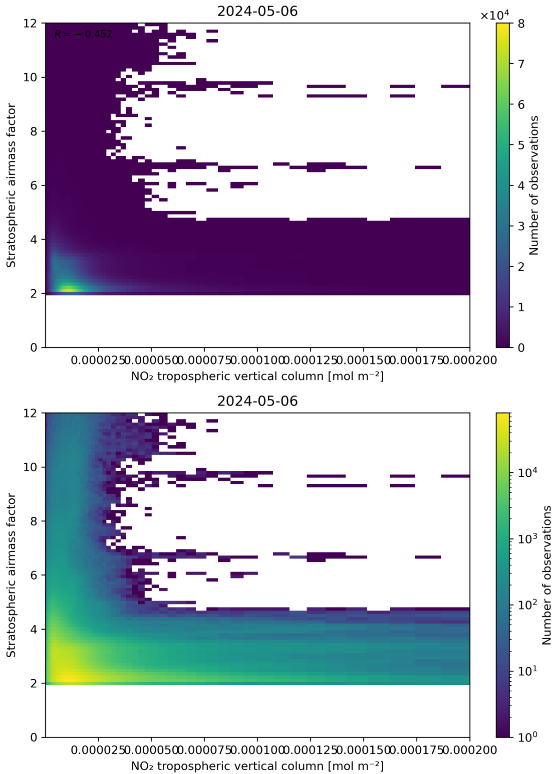
Figure 121: Scatter density plot of “NO 2 tropospheric vertical column” against “Stratospheric air mass factor” for 2024-05-05 to 2024-05-07.
