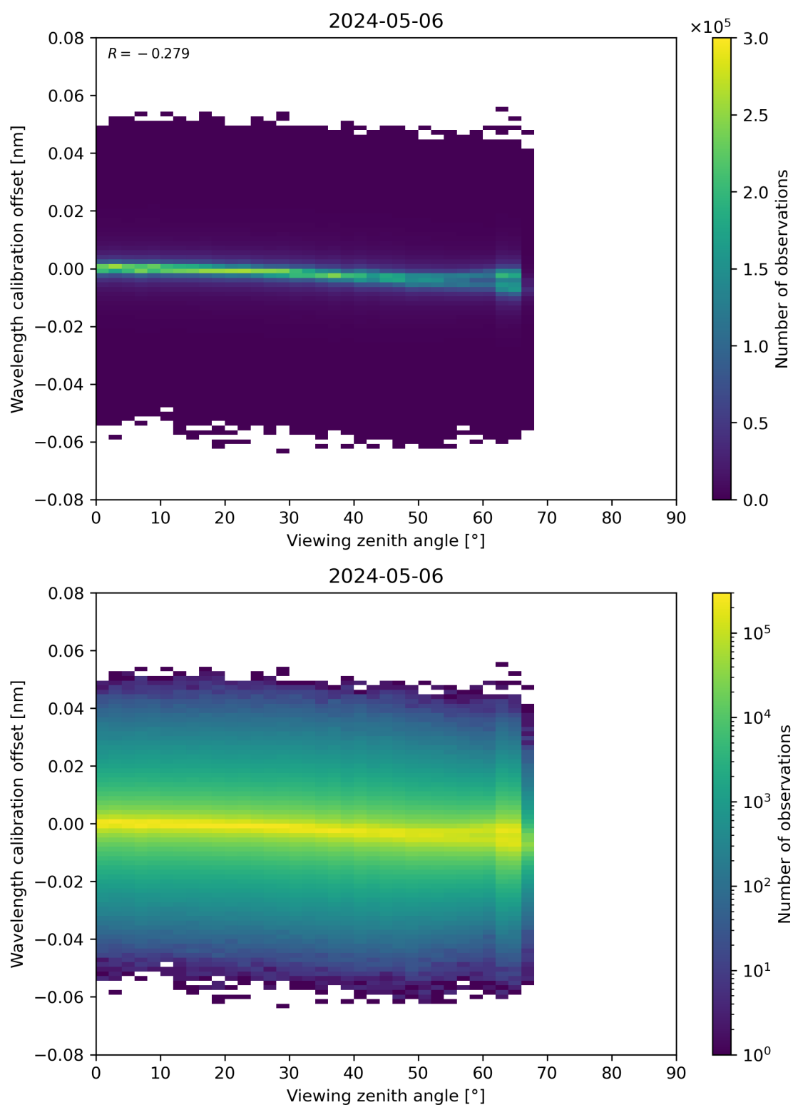
Figure 173: Scatter density plot of “Viewing zenith angle” against “Wavelength calibration offset” for 2024-05-05 to 2024-05-07.
