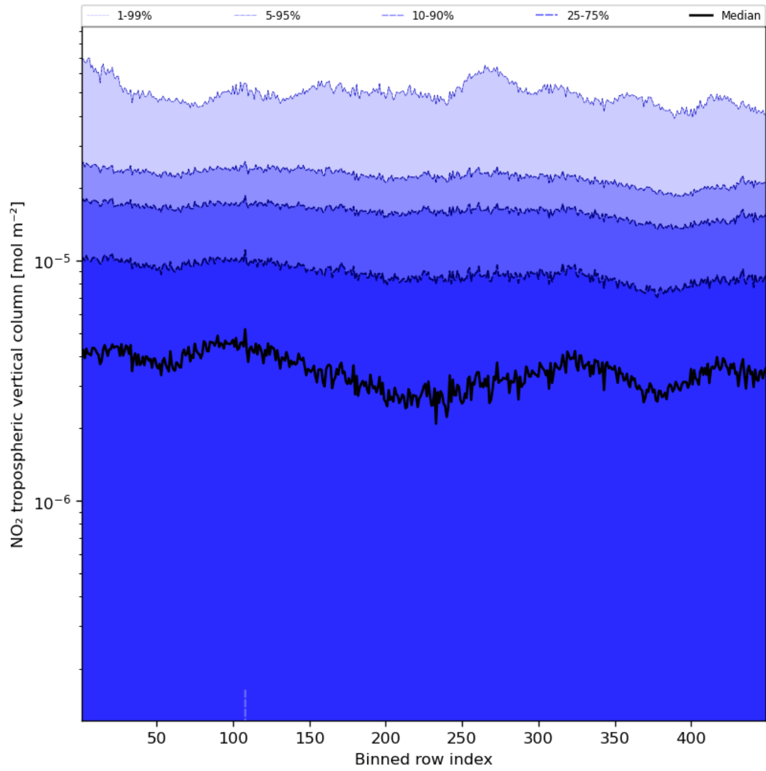
Figure 46: Along track statistics of “NO 2 tropospheric vertical column” for 2024-05-05 to 2024-05-07
