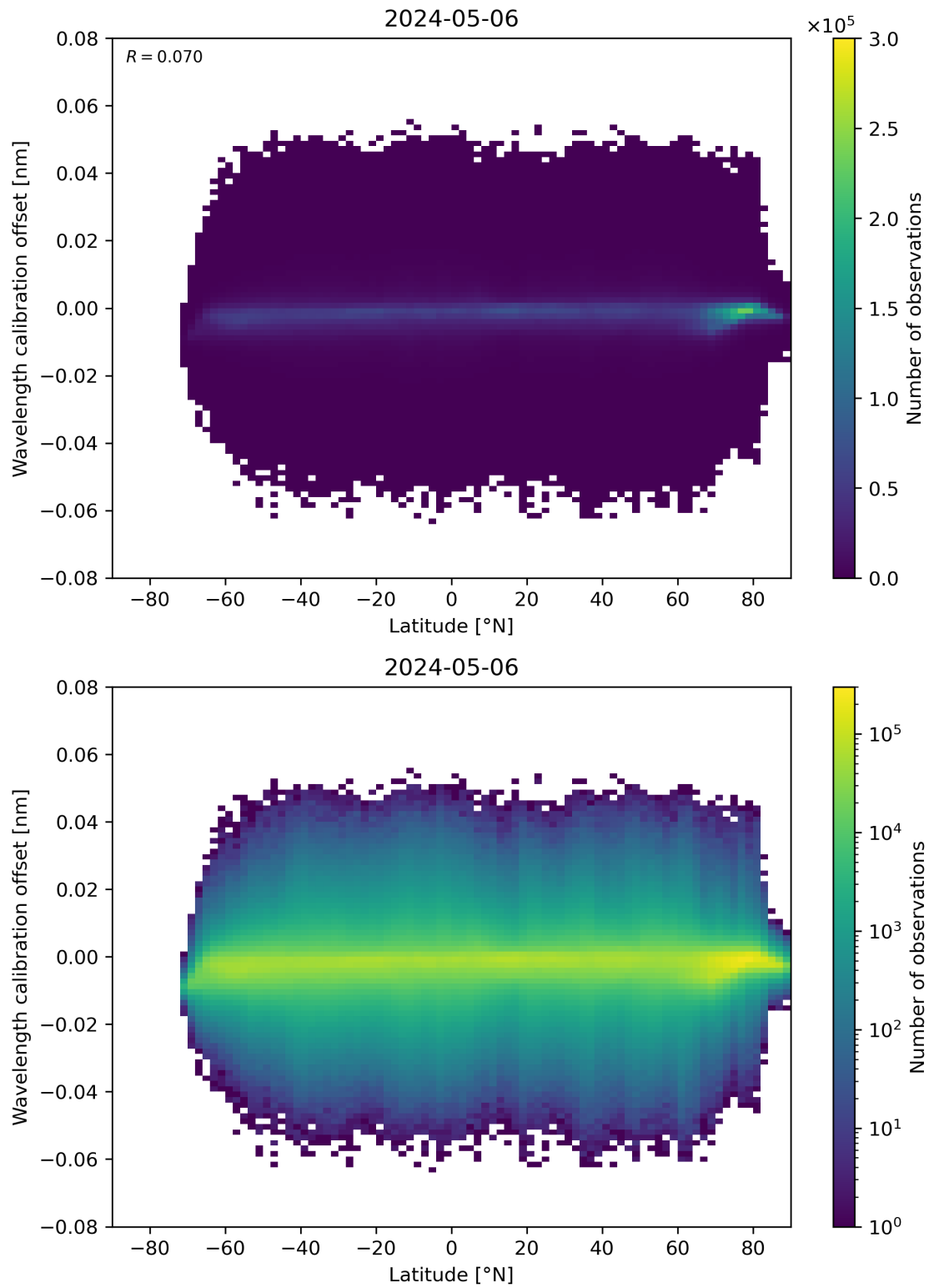
Figure 95: Scatter density plot of “Latitude” against “Wavelength calibration offset” for 2024-05-05 to 2024-05-07.
