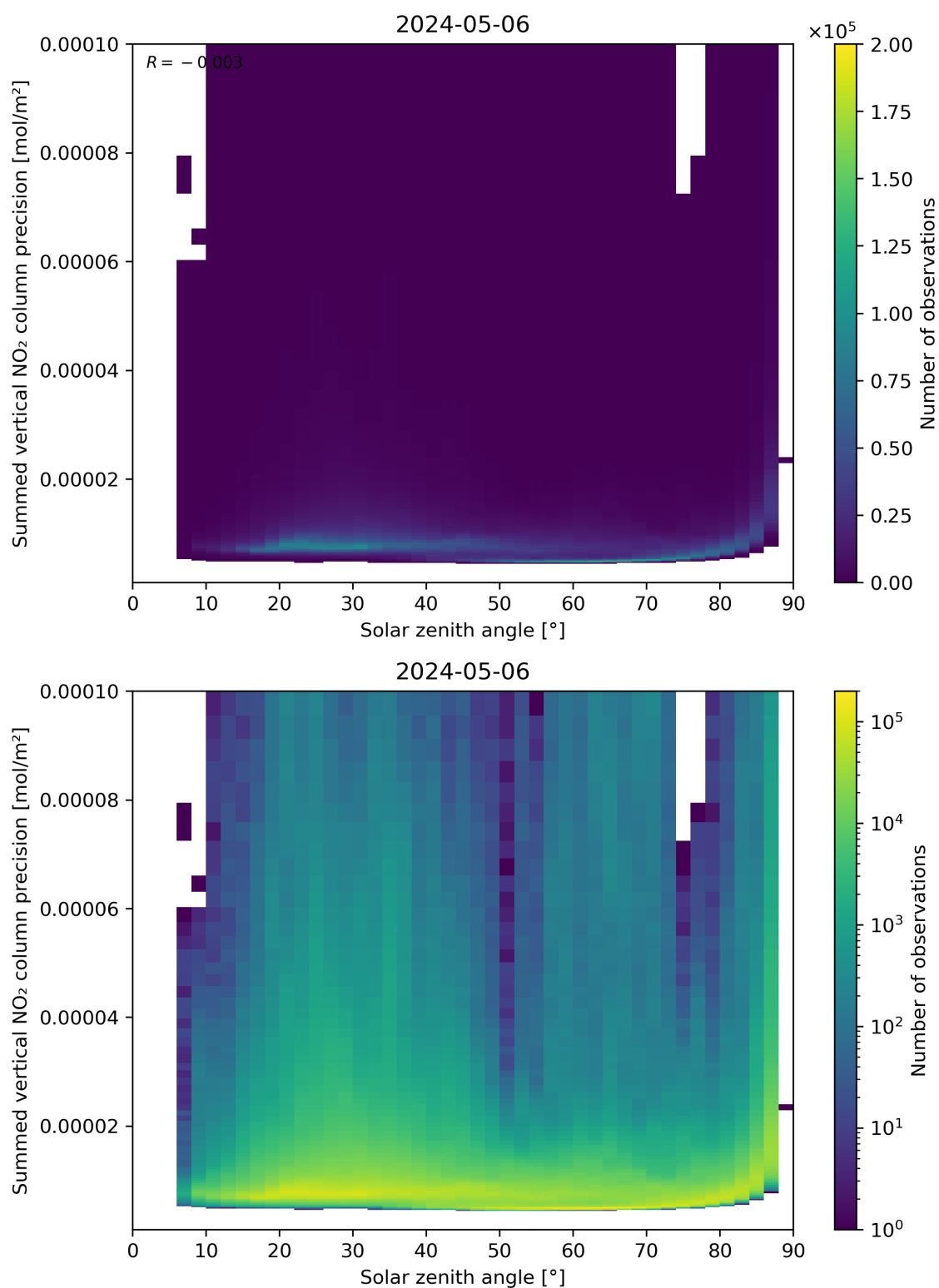
Figure 152: Scatter density plot of “Solar zenith angle” against “Summed vertical NO 2 column precision” for 2024-05-05 to 2024-05-07.
