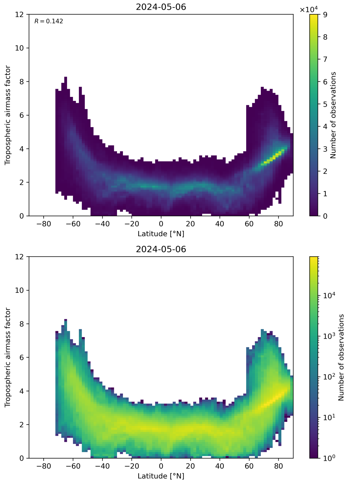
Figure 85: Scatter density plot of “Latitude” against “Tropospheric air mass factor” for 2024-05-05 to 2024-05-07.
