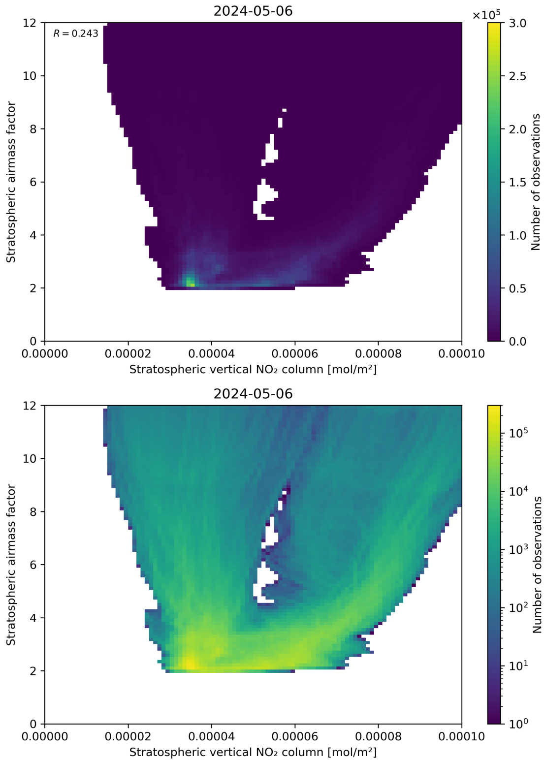
Figure 96: Scatter density plot of “Stratospheric vertical NO 2 column” against “Stratospheric airmass factor” for 2024-05-05 to 2024-05-07.
