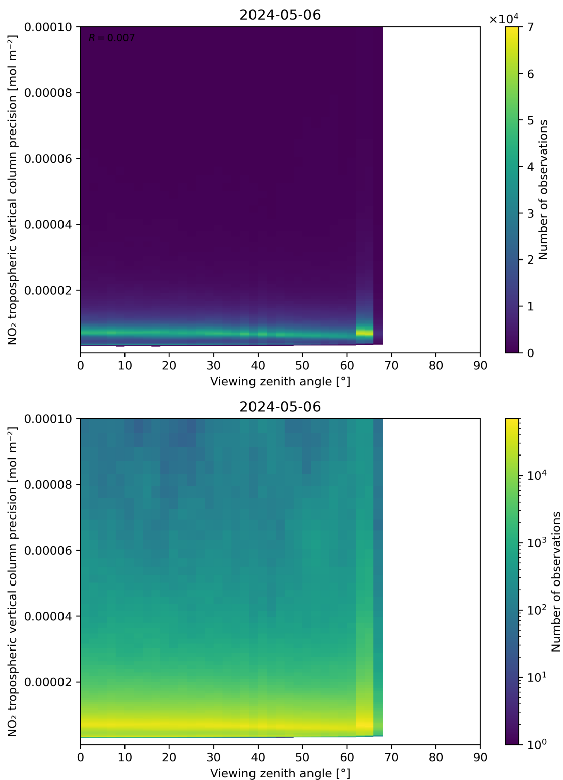
Figure 170: Scatter density plot of “Viewing zenith angle” against “NO 2 tropospheric vertical column precision” for 2024-05-05 to 2024-05-07.
