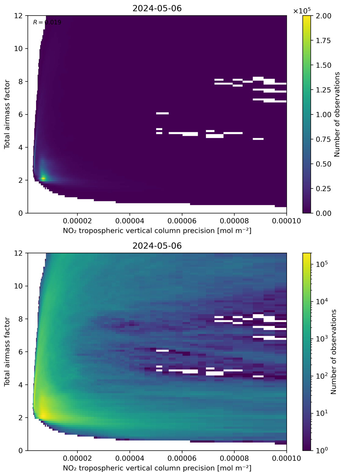
Figure 132: Scatter density plot of “NO 2 tropospheric vertical column precision” against “Total air mass factor” for 2024-05-05 to 2024-05-07.
