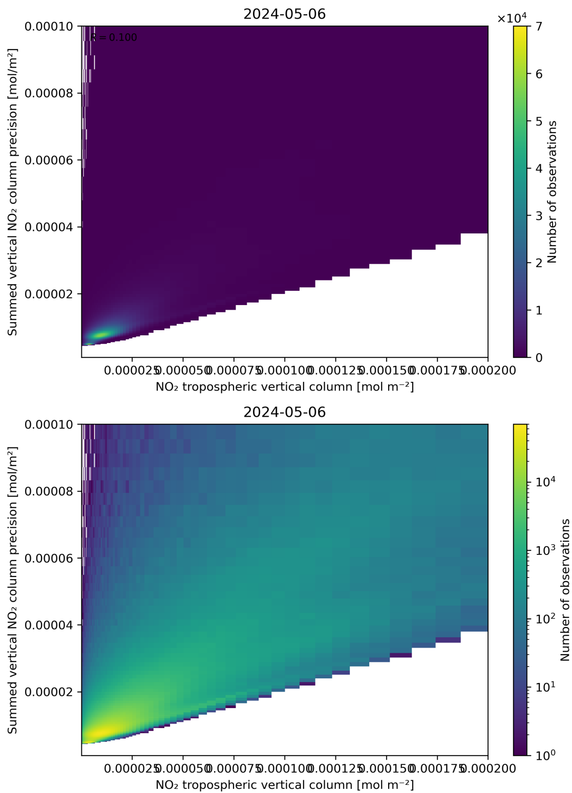
Figure 127: Scatter density plot of “NO 2 tropospheric vertical column” against “Summed vertical NO 2 column precision” for 2024-05-05 to 2024-05-07.
