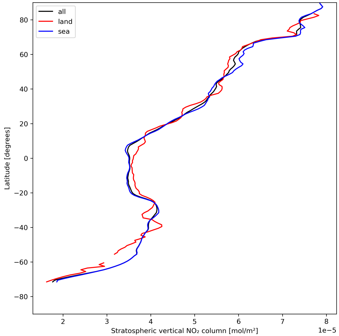
Figure 19: Zonal average of “Stratospheric vertical NO 2 column” for 2024-05-05 to 2024-05-07.
