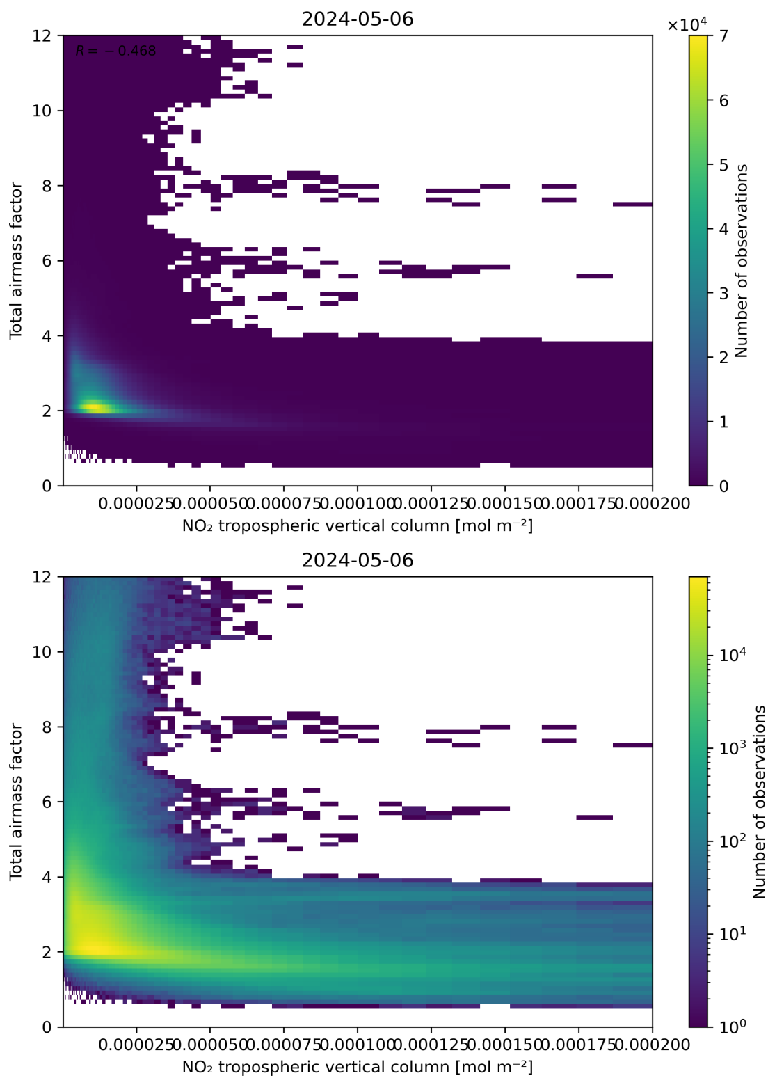
Figure 122: Scatter density plot of “NO 2 tropospheric vertical column” against “Total air mass factor” for 2024-05-05 to 2024-05-07.
