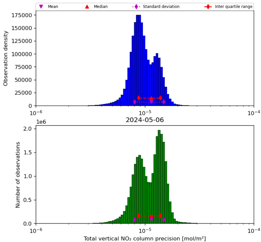
Figure 39: Histogram of “Total vertical NO 2 column precision” for 2024-05-05 to 2024-05-07
