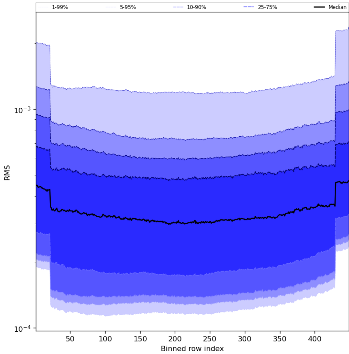
Figure 60: Along track statistics of “RMS” for 2024-05-05 to 2024-05-07
