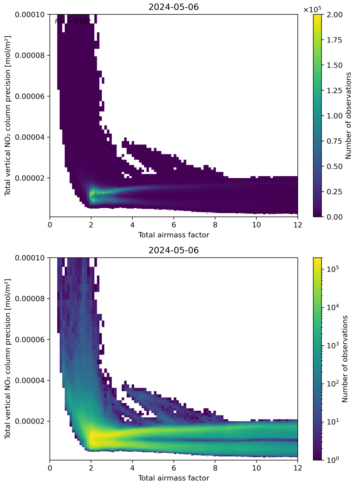
Figure 68: Scatter density plot of “Total airmass factor” against “Total vertical NO 2 column precision” for 2024-05-05 to 2024-05-07.
