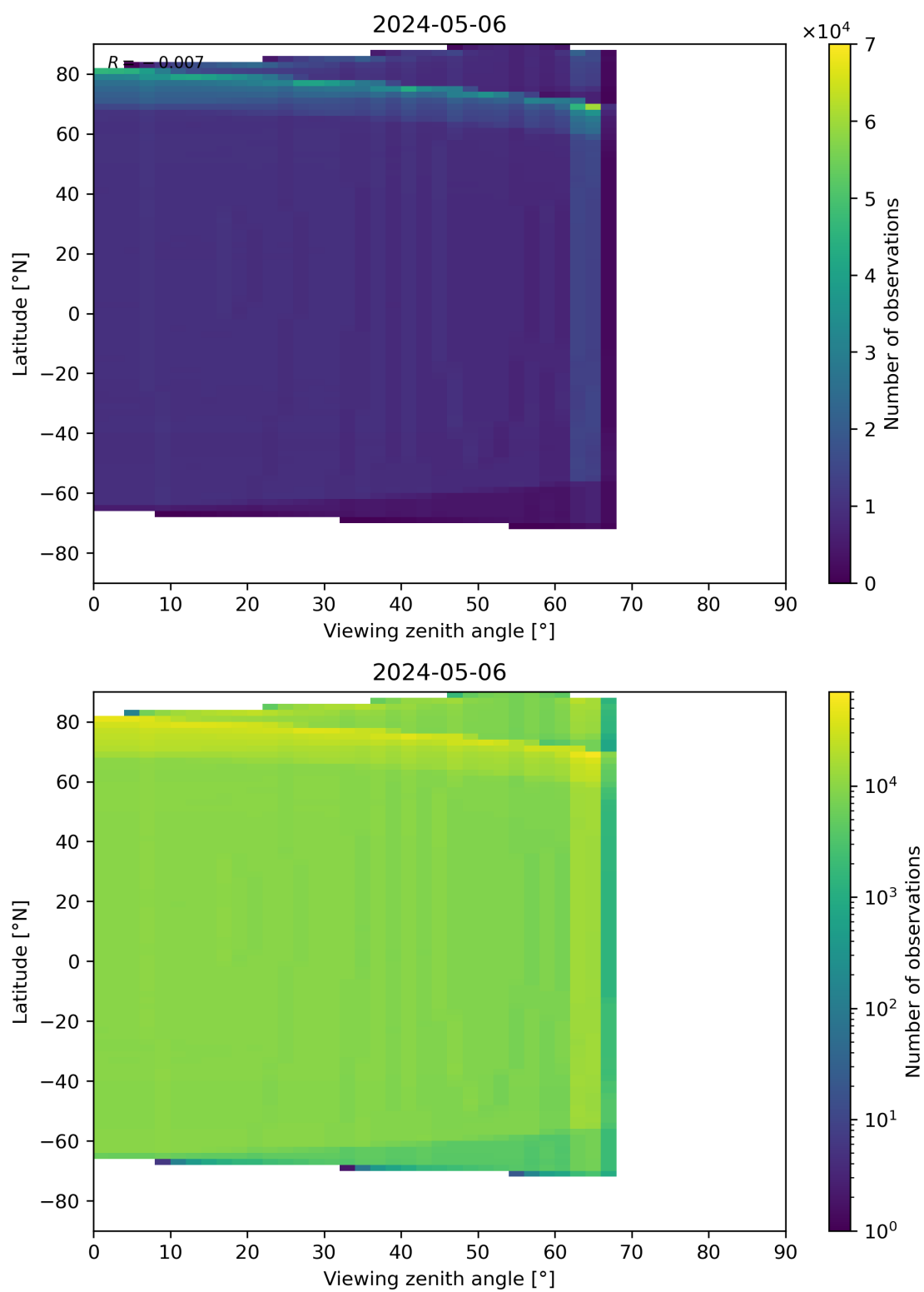
Figure 163: Scatter density plot of “Viewing zenith angle” against “Latitude” for 2024-05-05 to 2024-05-07.
