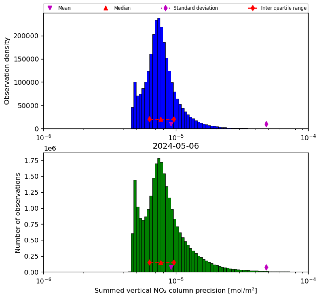
Figure 41: Histogram of “Summed vertical NO 2 column precision” for 2024-05-05 to 2024-05-07
