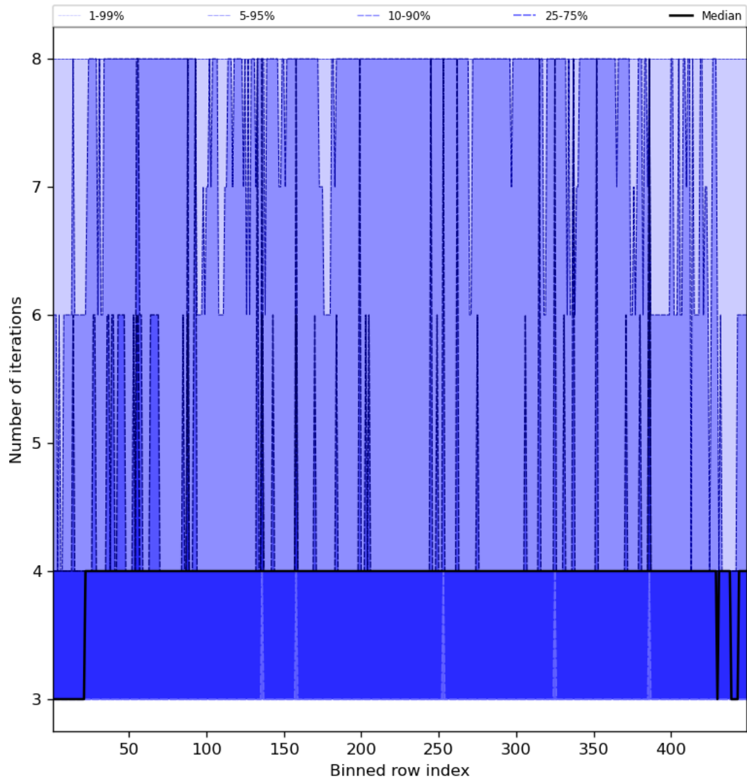
Figure 51: Along track statistics of “Number of iterations” for 2024-05-05 to 2024-05-07
