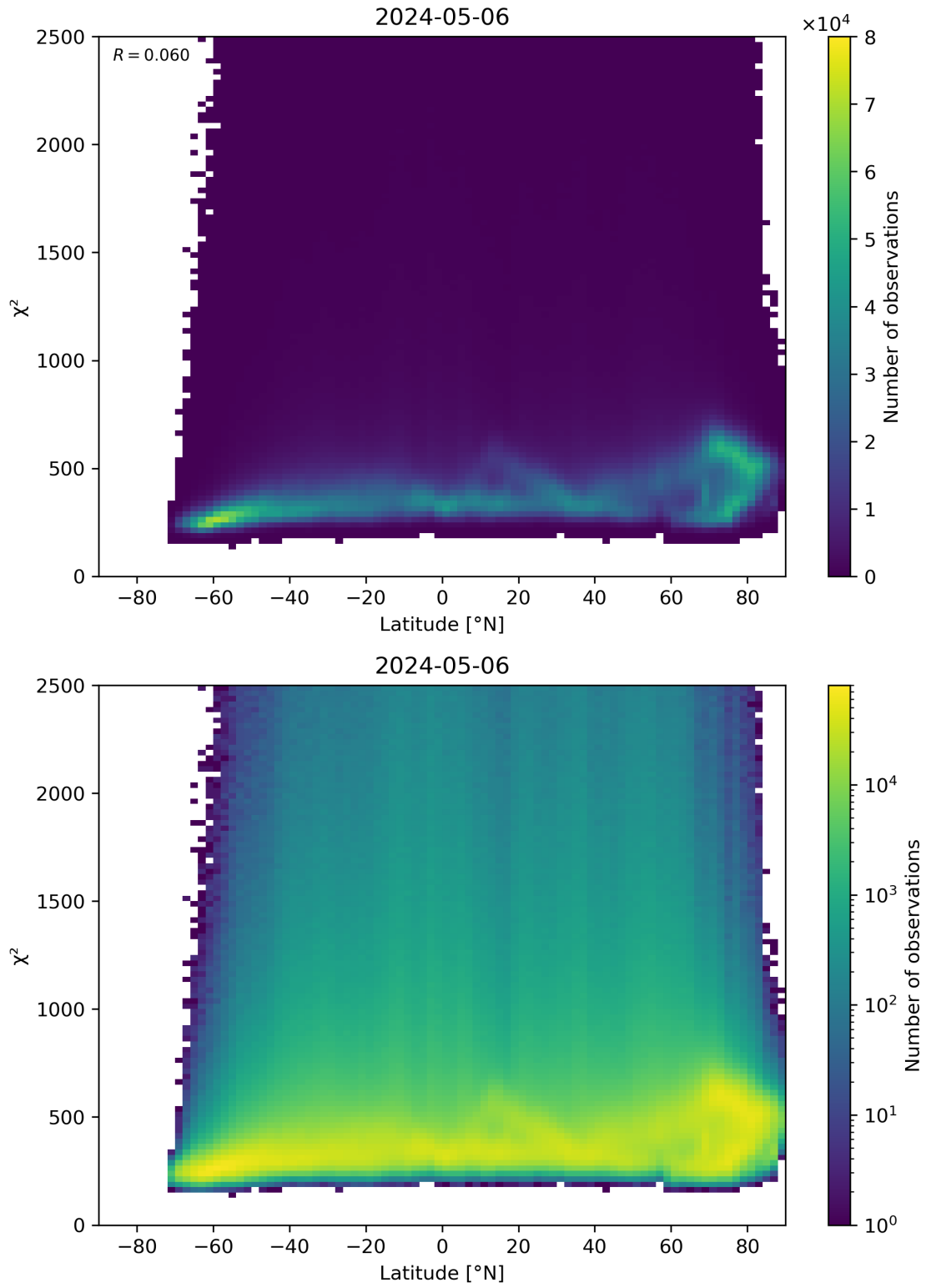
Figure 86: Scatter density plot of “Latitude” against “ \chi^2 ” for 2024-05-05 to 2024-05-07.
