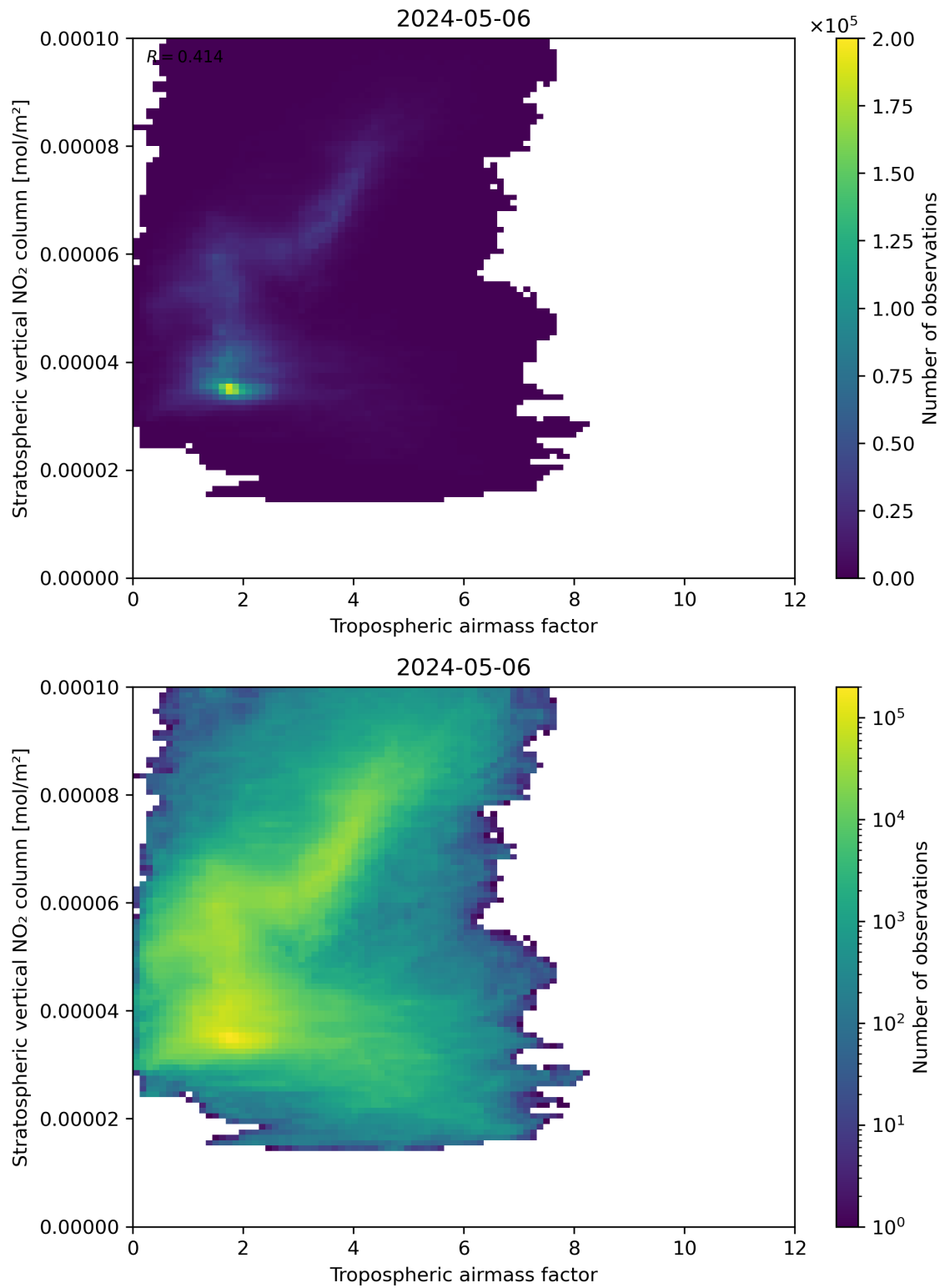
Figure 74: Scatter density plot of “Tropospheric air mass factor” against “Stratospheric vertical NO 2 column” for 2024-05-05 to 2024-05-07.
