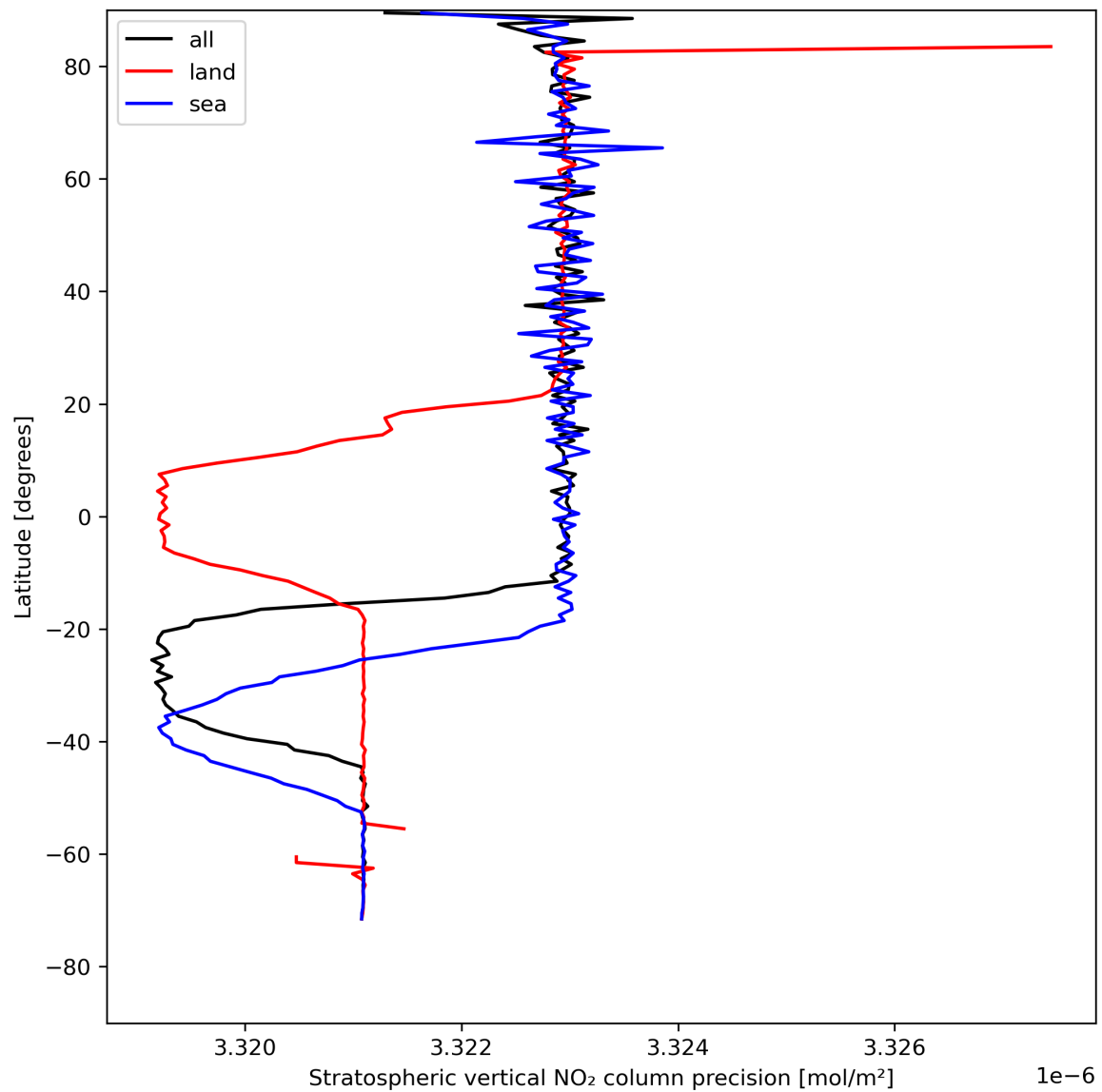
Figure 20: Zonal average of “Stratospheric vertical NO 2 column precision” for 2024-05-05 to 2024-05-07.
