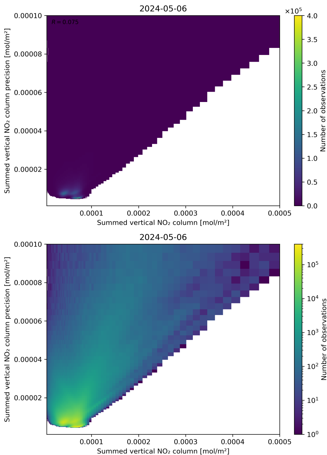
Figure 105: Scatter density plot of “Summed vertical NO 2 column” against “Summed vertical NO 2 column precision” for 2024-05-05 to 2024-05-07.
