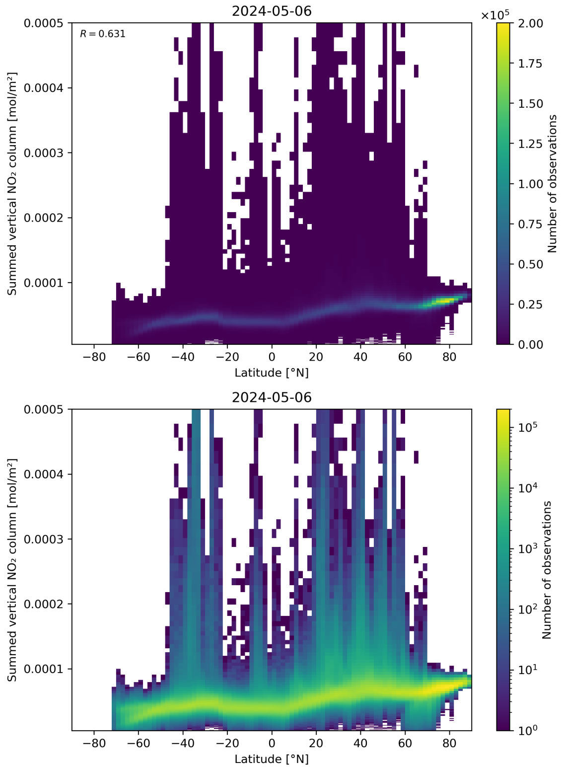
Figure 88: Scatter density plot of “Latitude” against “Summed vertical NO 2 column” for 2024-05-05 to 2024-05-07.
