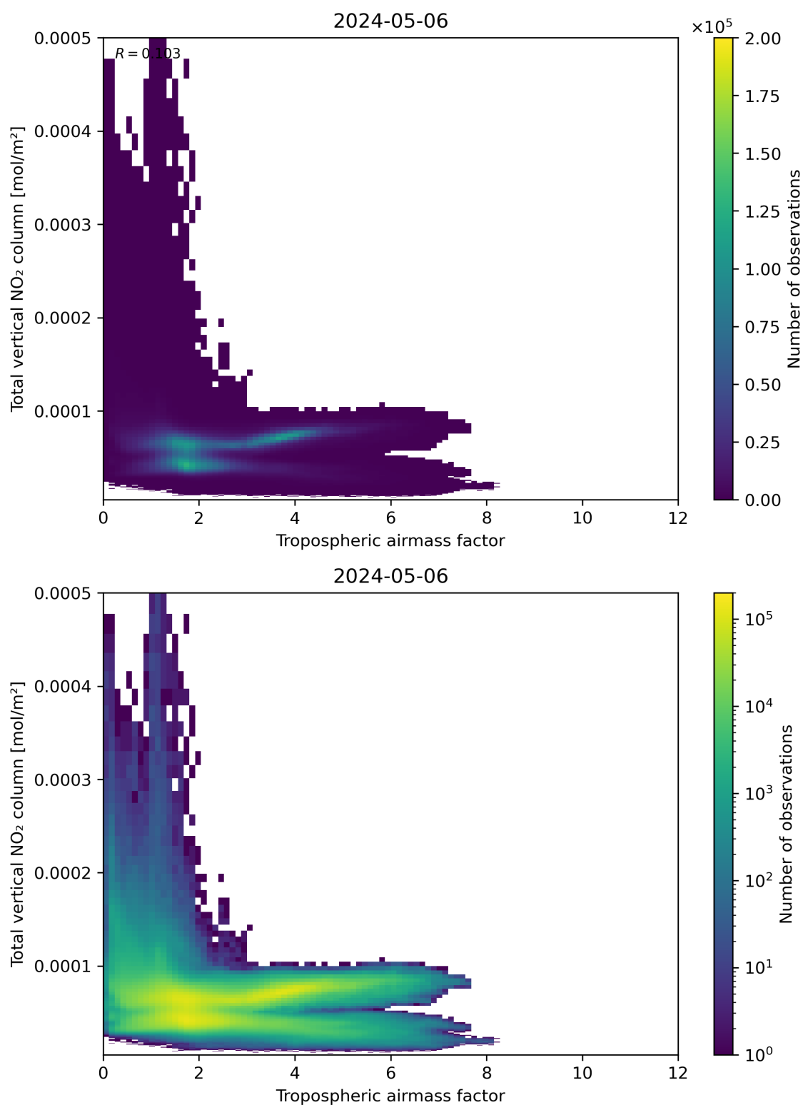
Figure 77: Scatter density plot of “Tropospheric airmass factor” against “Total vertical NO 2 column” for 2024-05-05 to 2024-05-07.
