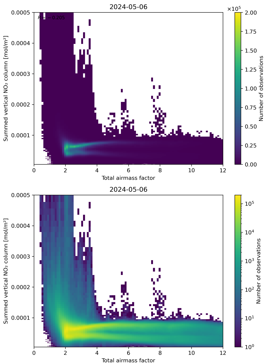
Figure 65: Scatter density plot of “Total airmass factor” against “Summed vertical NO 2 column” for 2024-05-05 to 2024-05-07.
