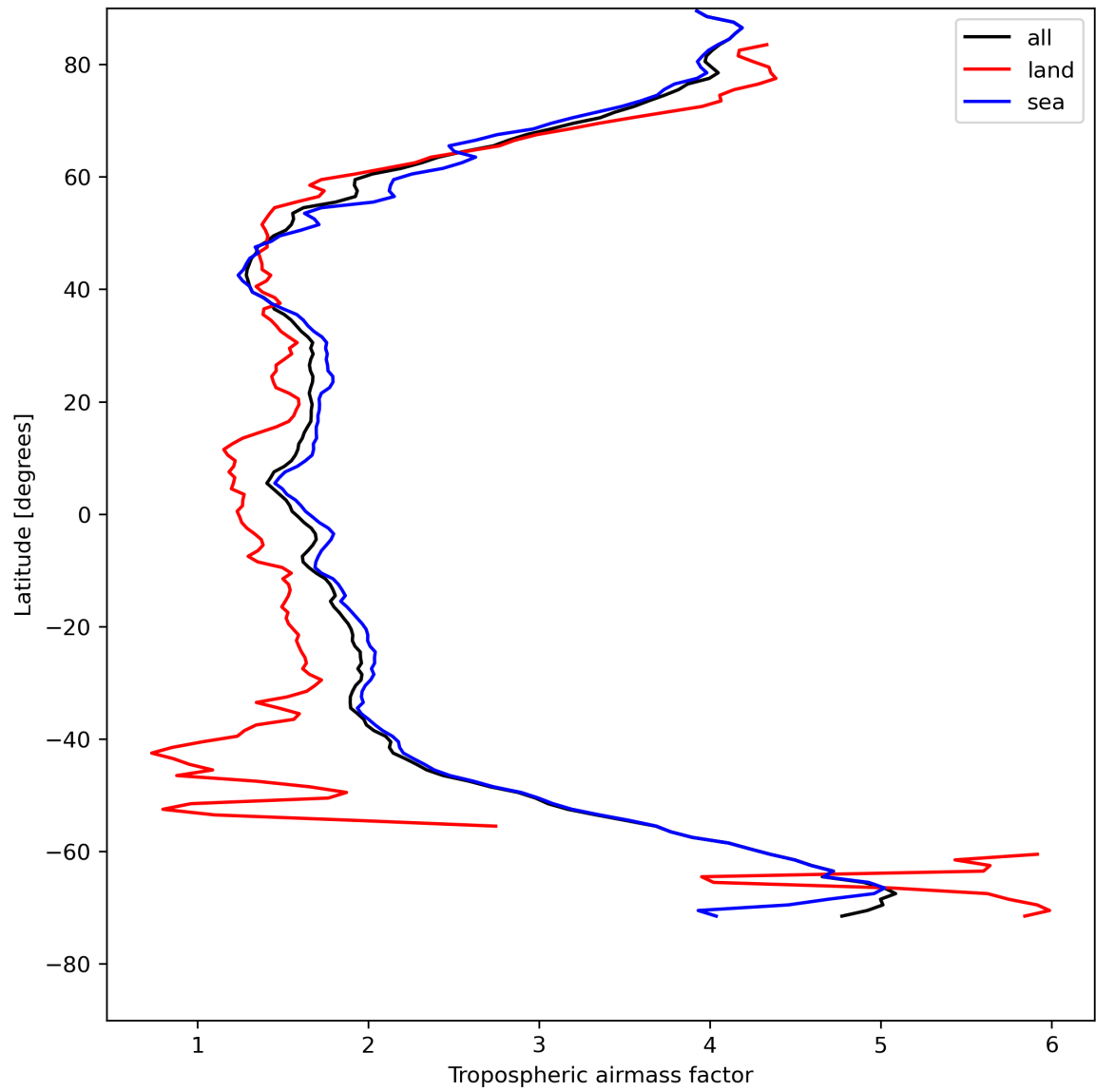
Figure 14: Zonal average of “Tropospheric airmass factor” for 2024-05-05 to 2024-05-07.
