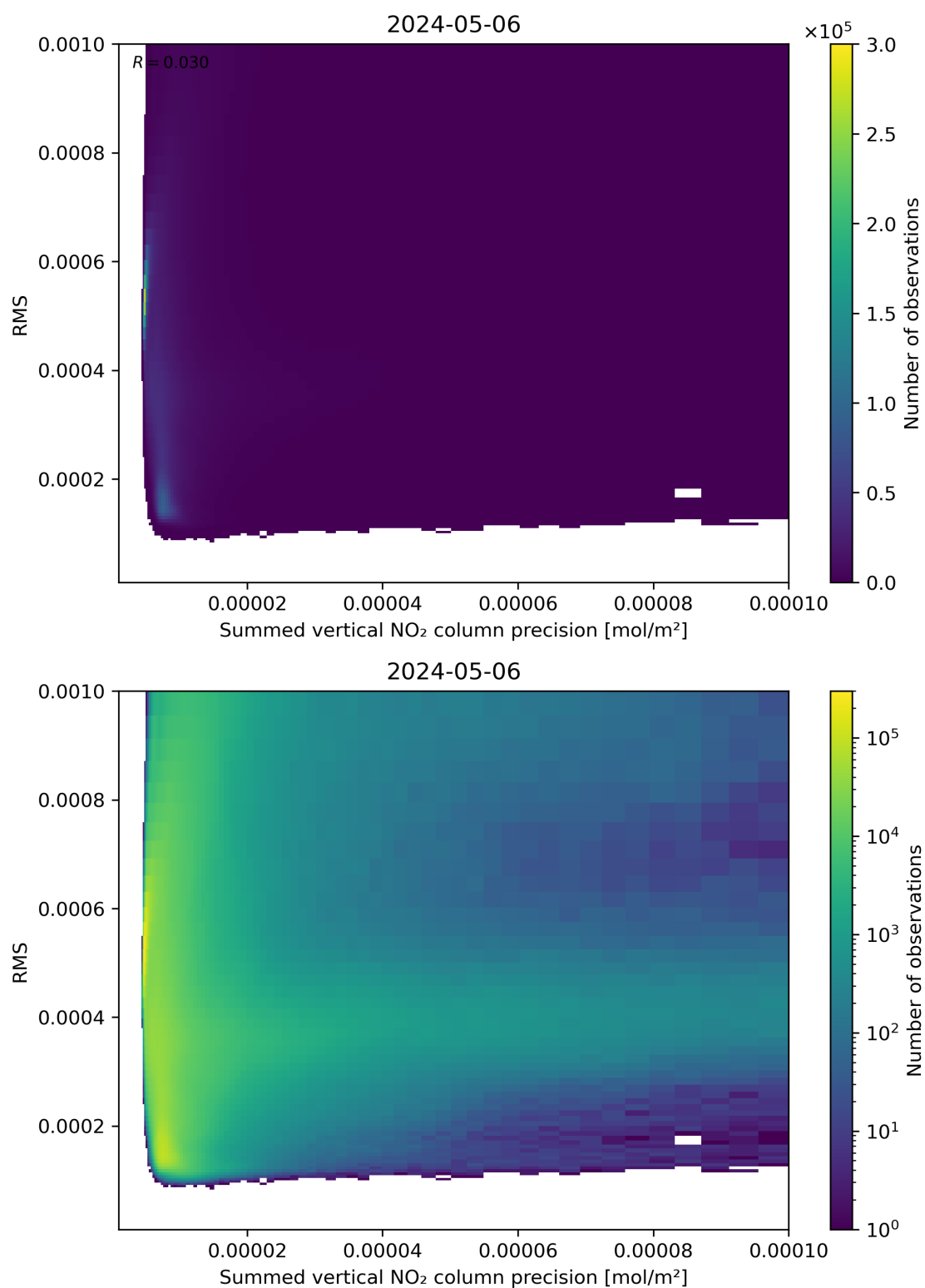
Figure 108: Scatter density plot of “Summed vertical NO 2 column precision” against “RMS” for 2024-05-05 to 2024-05-07.
