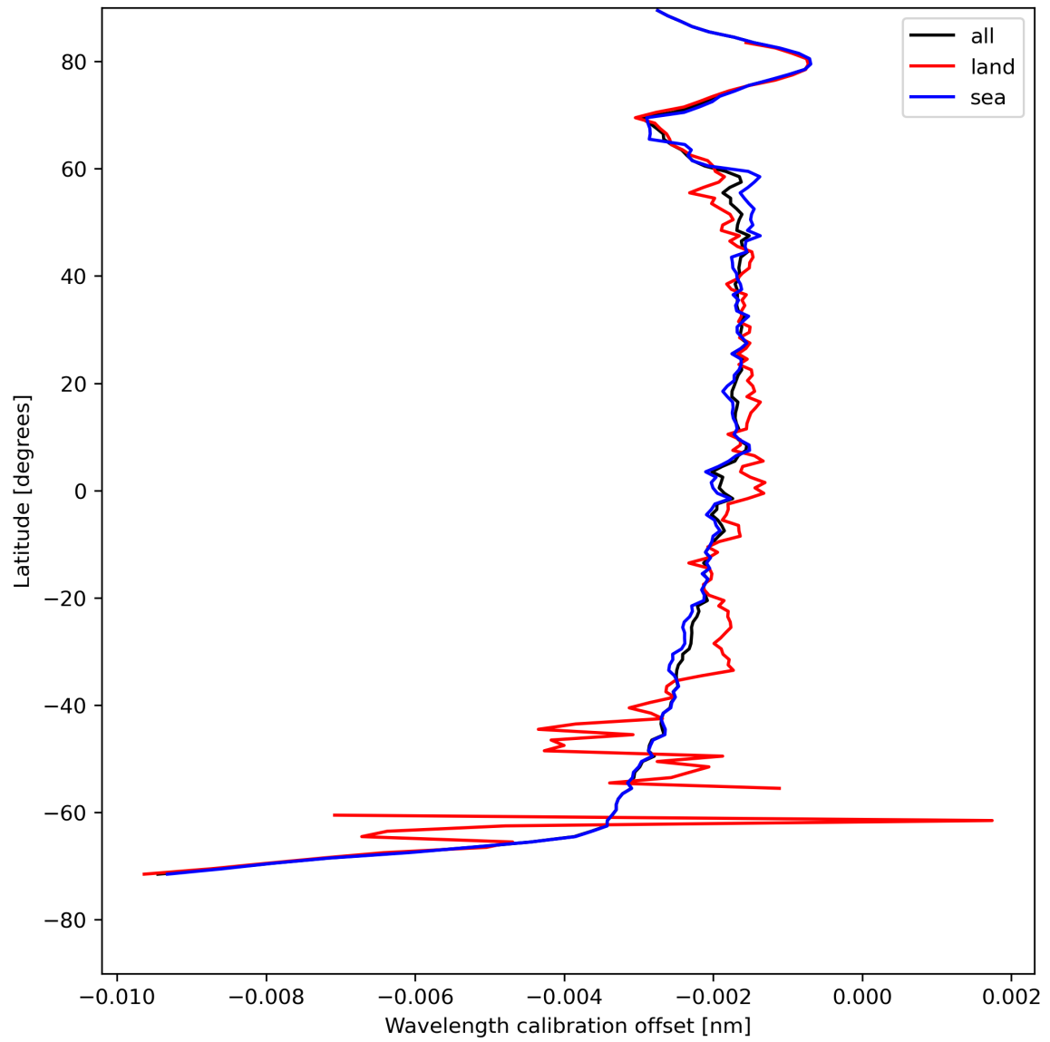
Figure 18: Zonal average of “Wavelength calibration offset” for 2024-05-05 to 2024-05-07.
