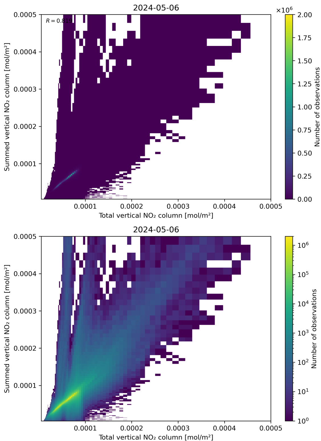
Figure 112: Scatter density plot of “Total vertical NO 2 column” against “Summed vertical NO 2 column” for 2024-05-05 to 2024-05-07.
