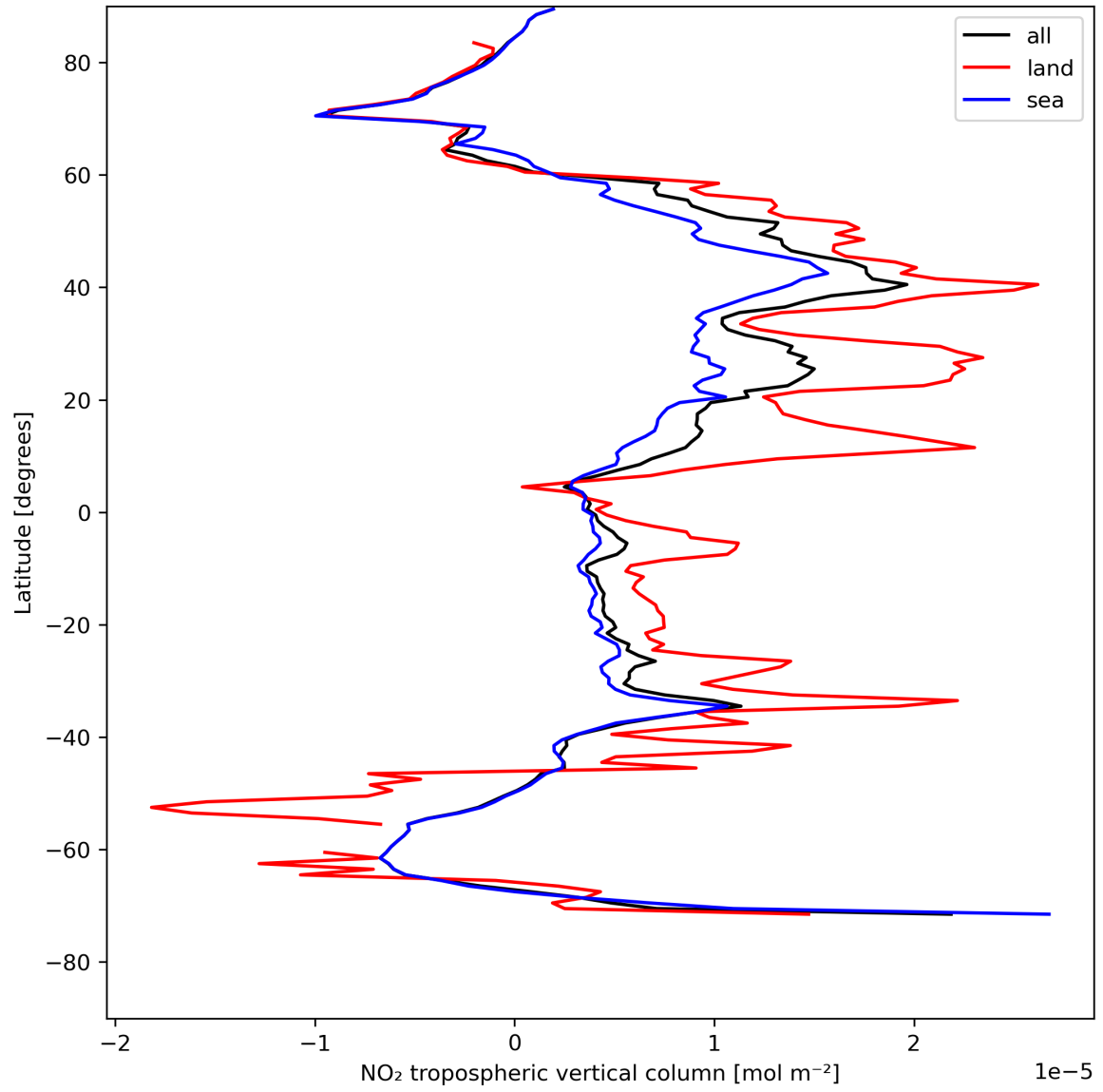
Figure 12: Zonal average of “NO 2 tropospheric vertical column” for 2024-05-05 to 2024-05-07.
