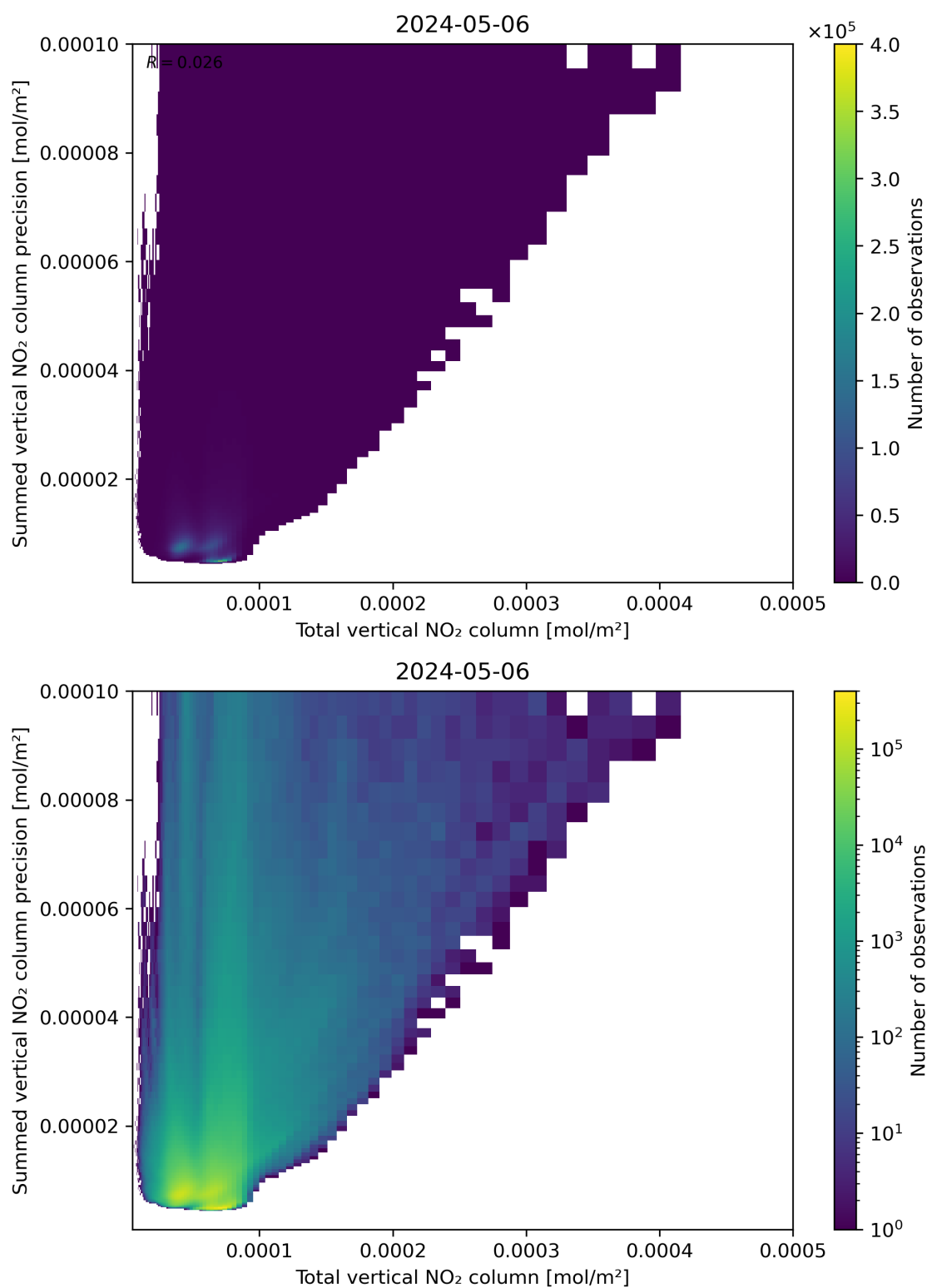
Figure 113: Scatter density plot of “Total vertical NO 2 column” against “Summed vertical NO 2 column precision” for 2024-05-05 to 2024-05-07.
