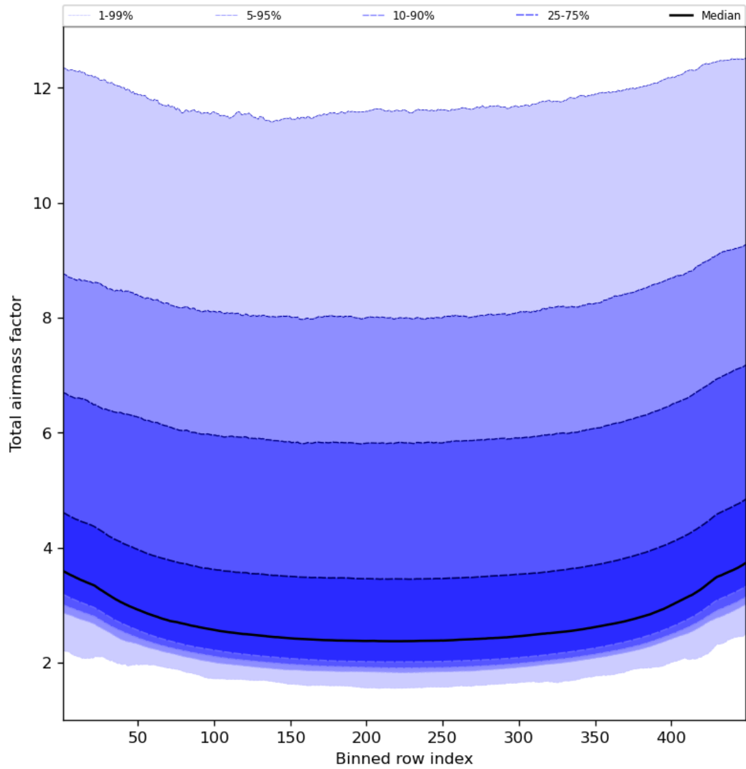
Figure 49: Along track statistics of “Total airmass factor” for 2024-05-05 to 2024-05-07
