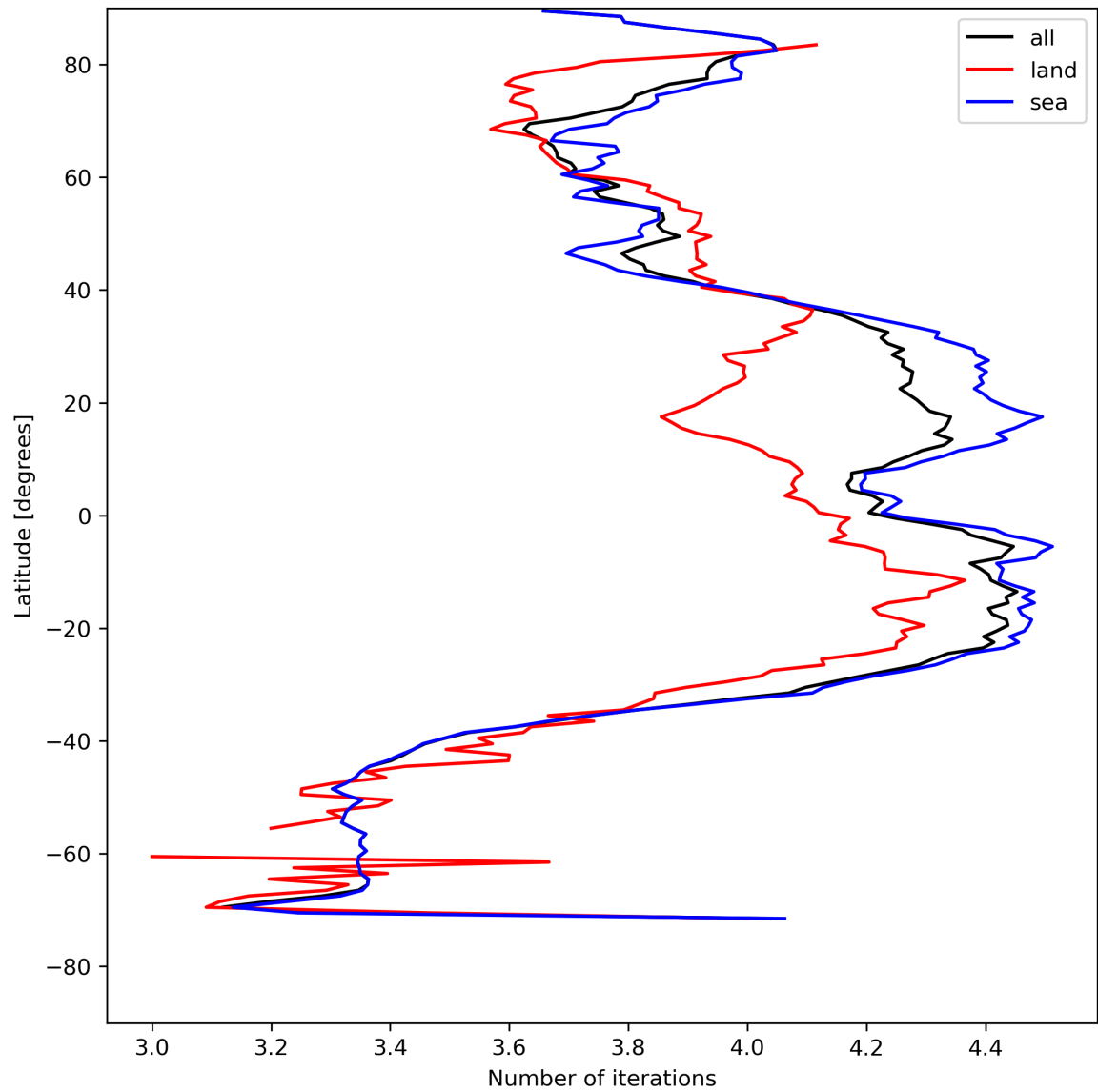
Figure 17: Zonal average of “Number of iterations” for 2024-05-05 to 2024-05-07.
