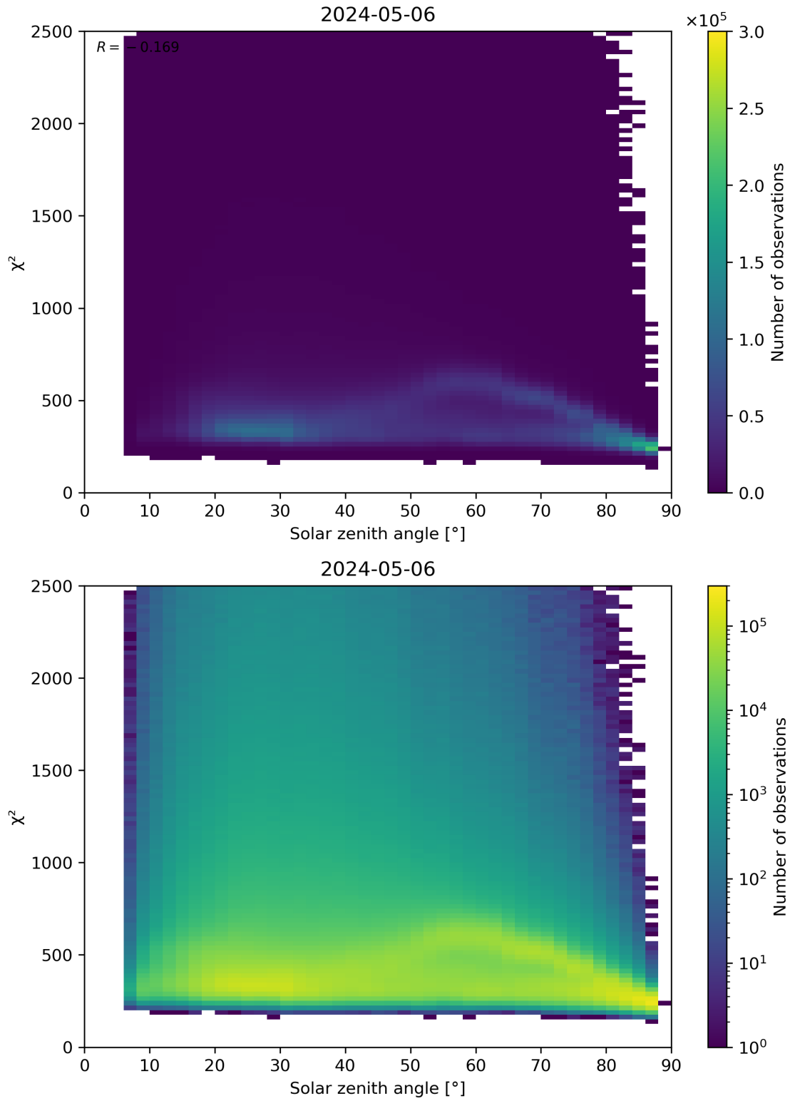
Figure 148: Scatter density plot of “Solar zenith angle” against “ \chi^2 ” for 2024-05-05 to 2024-05-07.
