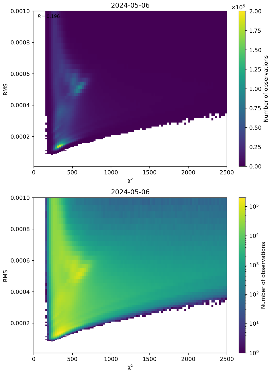
Figure 82: Scatter density plot of “ \chi^2 ” against “RMS” for 2024-05-05 to 2024-05-07.
