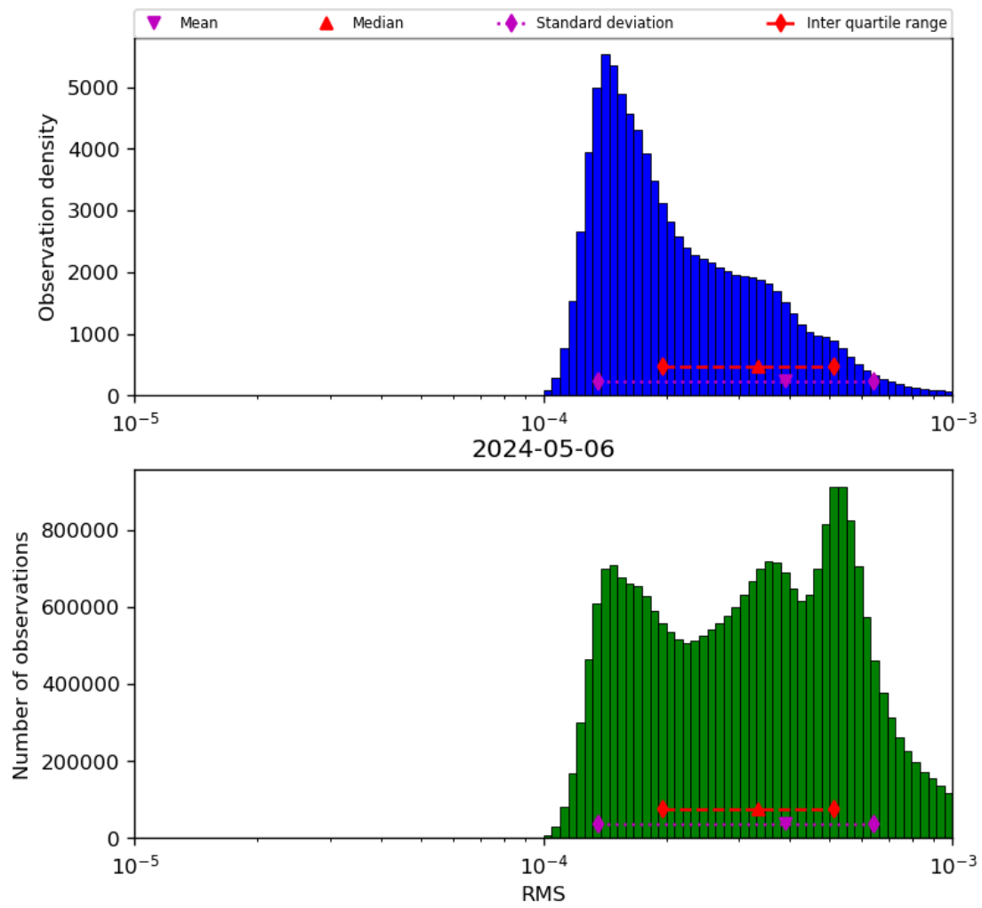
Figure 43: Histogram of “RMS” for 2024-05-05 to 2024-05-07
