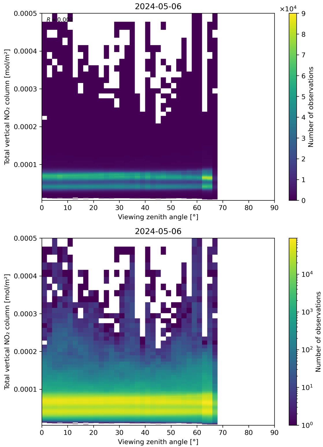
Figure 167: Scatter density plot of “Viewing zenith angle” against “Total vertical NO 2 column” for 2024-05-05 to 2024-05-07.
