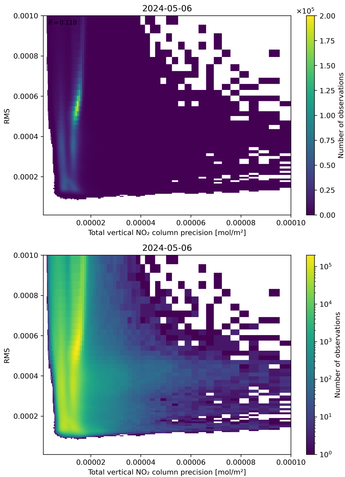
Figure 119: Scatter density plot of “Total vertical NO 2 column precision” against “RMS” for 2024-05-05 to 2024-05-07.
