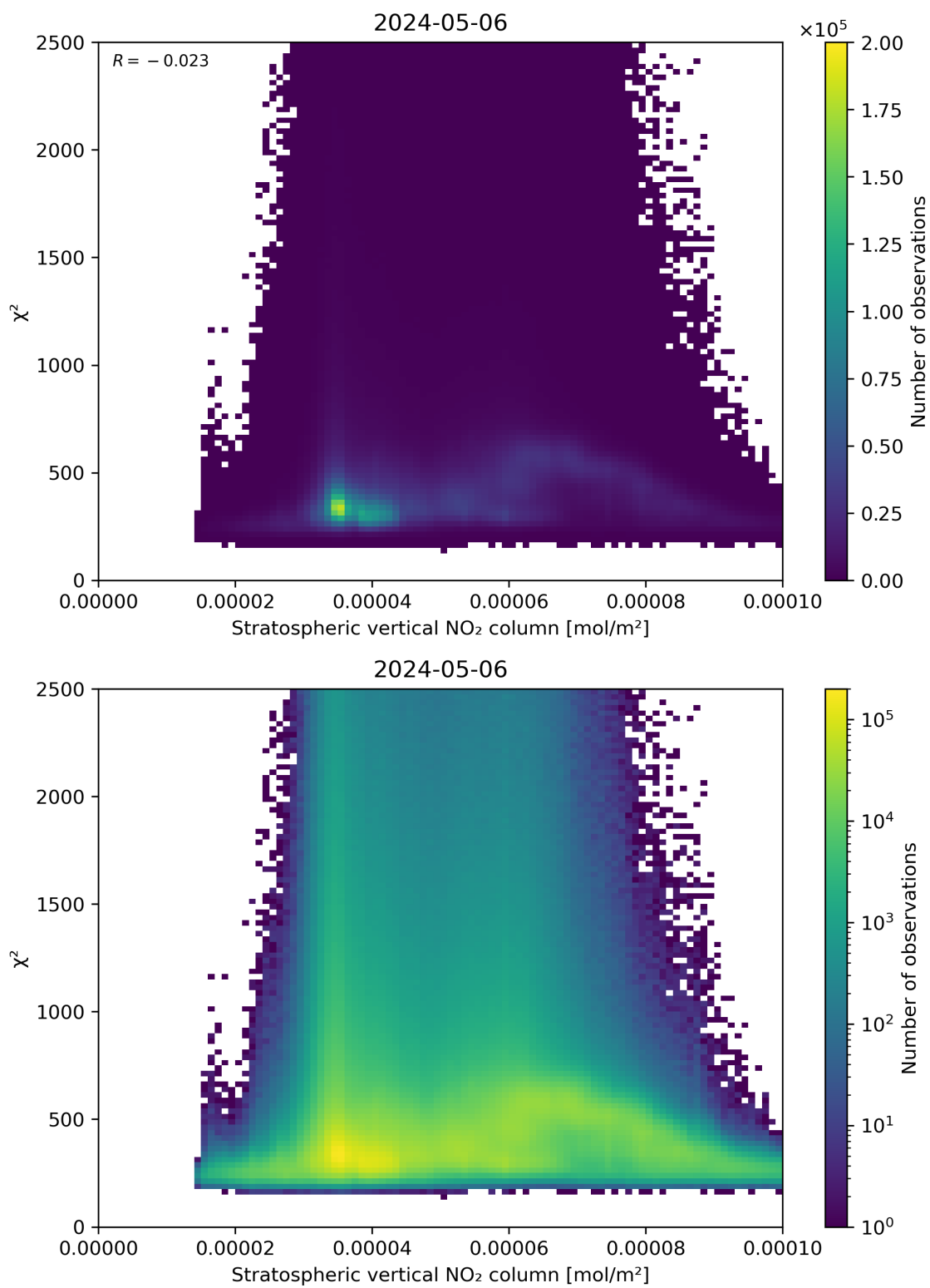
Figure 97: Scatter density plot of “Stratospheric vertical NO 2 column” against “ \chi^2 ” for 2024-05-05 to 2024-05-07.
