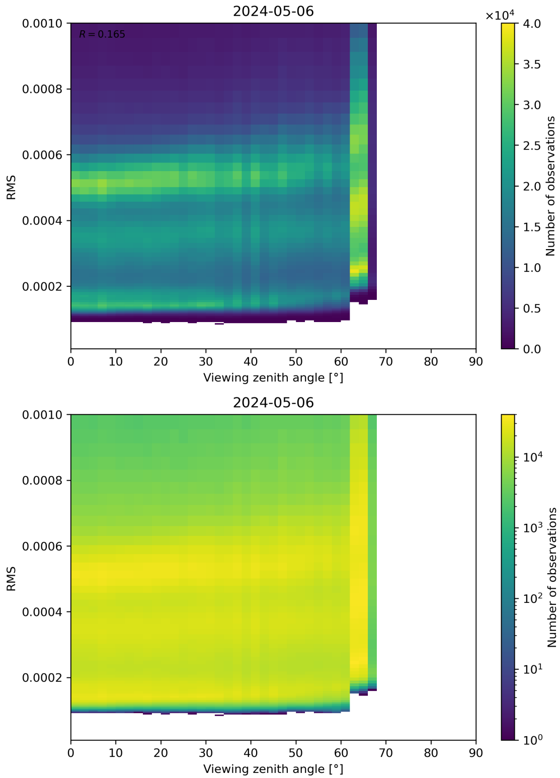
Figure 171: Scatter density plot of “Viewing zenith angle” against “RMS” for 2024-05-05 to 2024-05-07.
