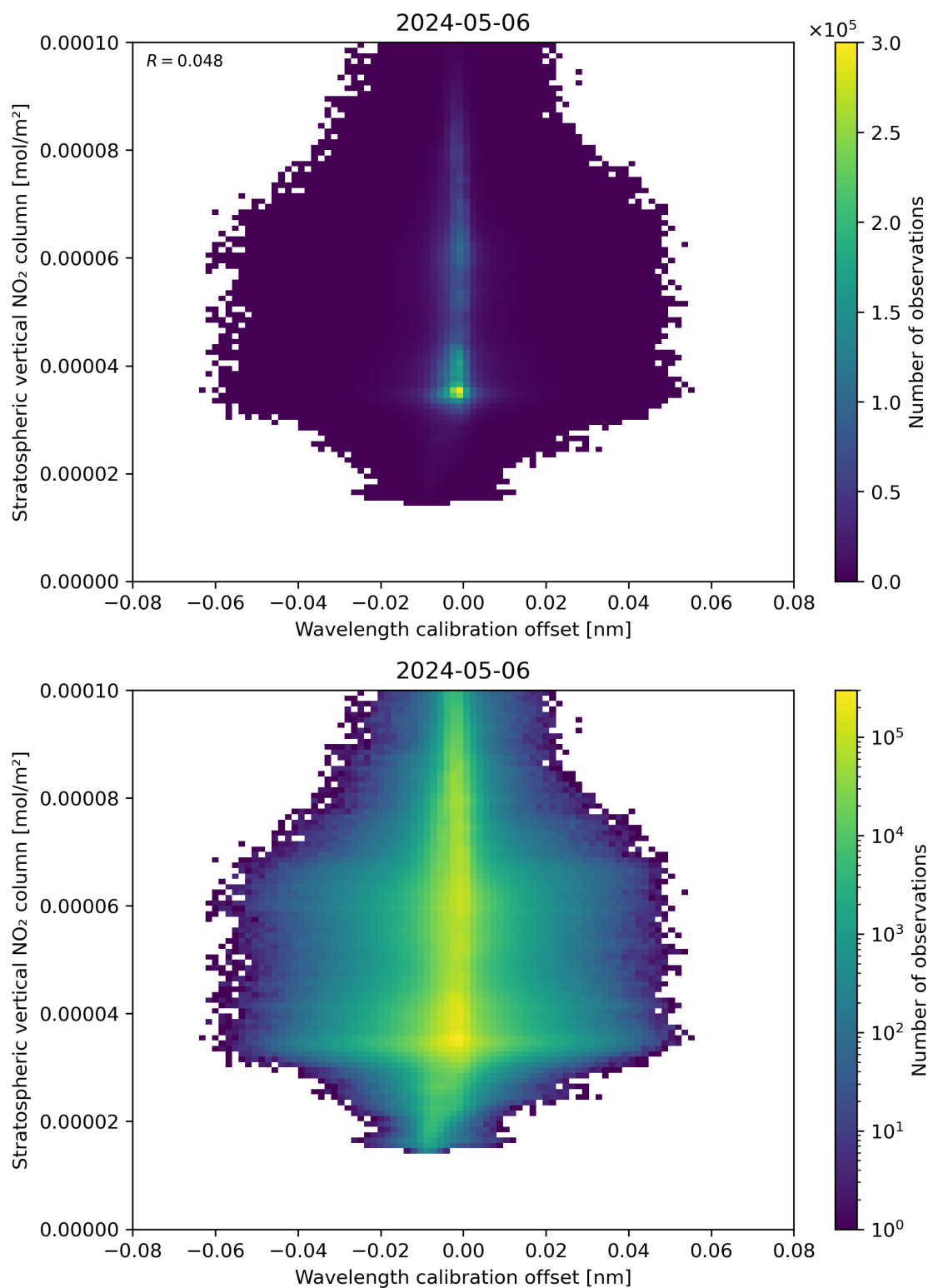
Figure 176: Scatter density plot of “Wavelength calibration offset” against “Stratospheric vertical NO 2 column” for 2024-05-05 to 2024-05-07.
