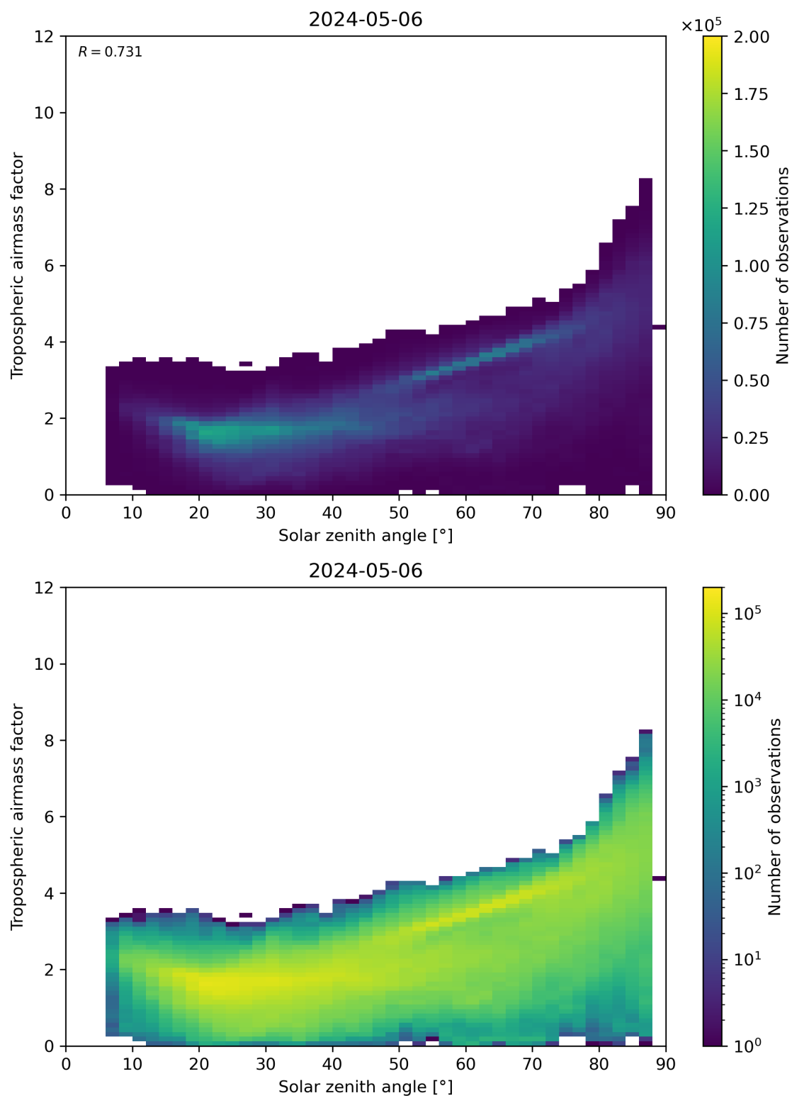
Figure 147: Scatter density plot of “Solar zenith angle” against “Tropospheric airmass factor” for 2024-05-05 to 2024-05-07.
