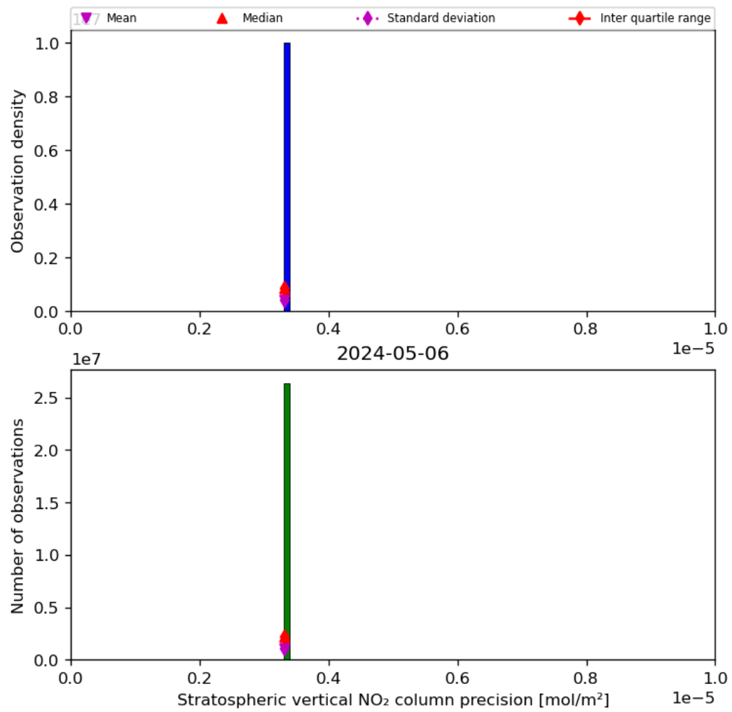
Figure 37: Histogram of “Stratospheric vertical NO 2 column precision” for 2024-05-05 to 2024-05-07
