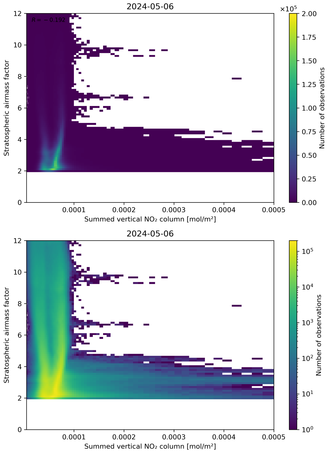
Figure 103: Scatter density plot of “Summed vertical NO 2 column” against “Stratospheric air mass factor” for 2024-05-05 to 2024-05-07.
