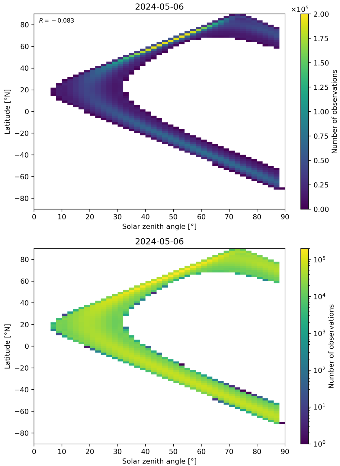
Figure 149: Scatter density plot of “Solar zenith angle” against “Latitude” for 2024-05-05 to 2024-05-07.
