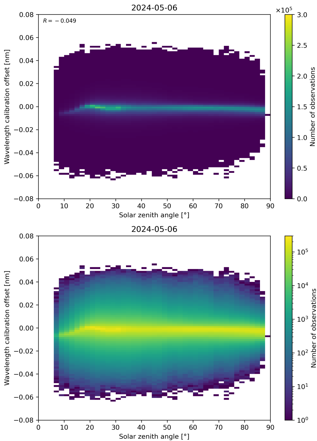
Figure 158: Scatter density plot of “Solar zenith angle” against “Wavelength calibration offset” for 2024-05-05 to 2024-05-07.
