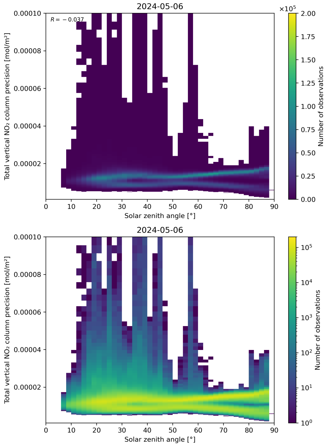
Figure 154: Scatter density plot of “Solar zenith angle” against “Total vertical NO 2 column precision” for 2024-05-05 to 2024-05-07.
