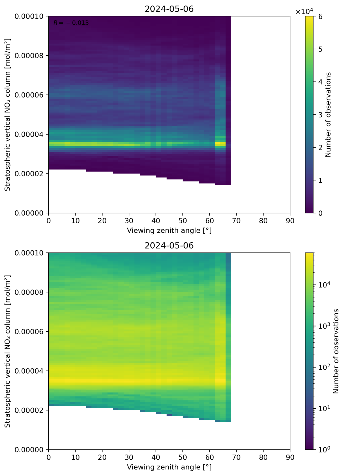
Figure 164: Scatter density plot of “Viewing zenith angle” against “Stratospheric vertical NO 2 column” for 2024-05-05 to 2024-05-07.
