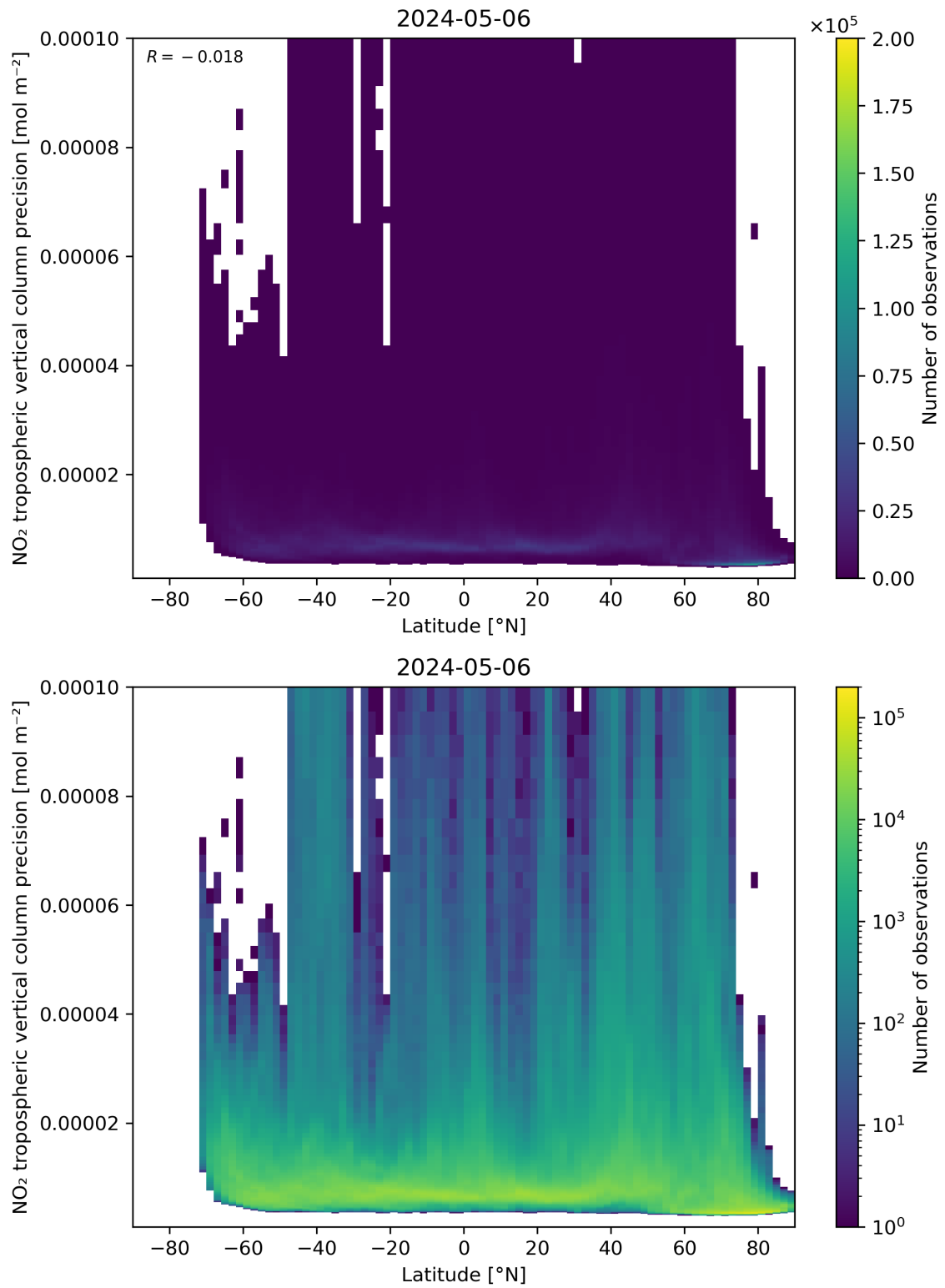
Figure 93: Scatter density plot of “Latitude” against “NO 2 tropospheric vertical column precision” for 2024-05-05 to 2024-05-07.
