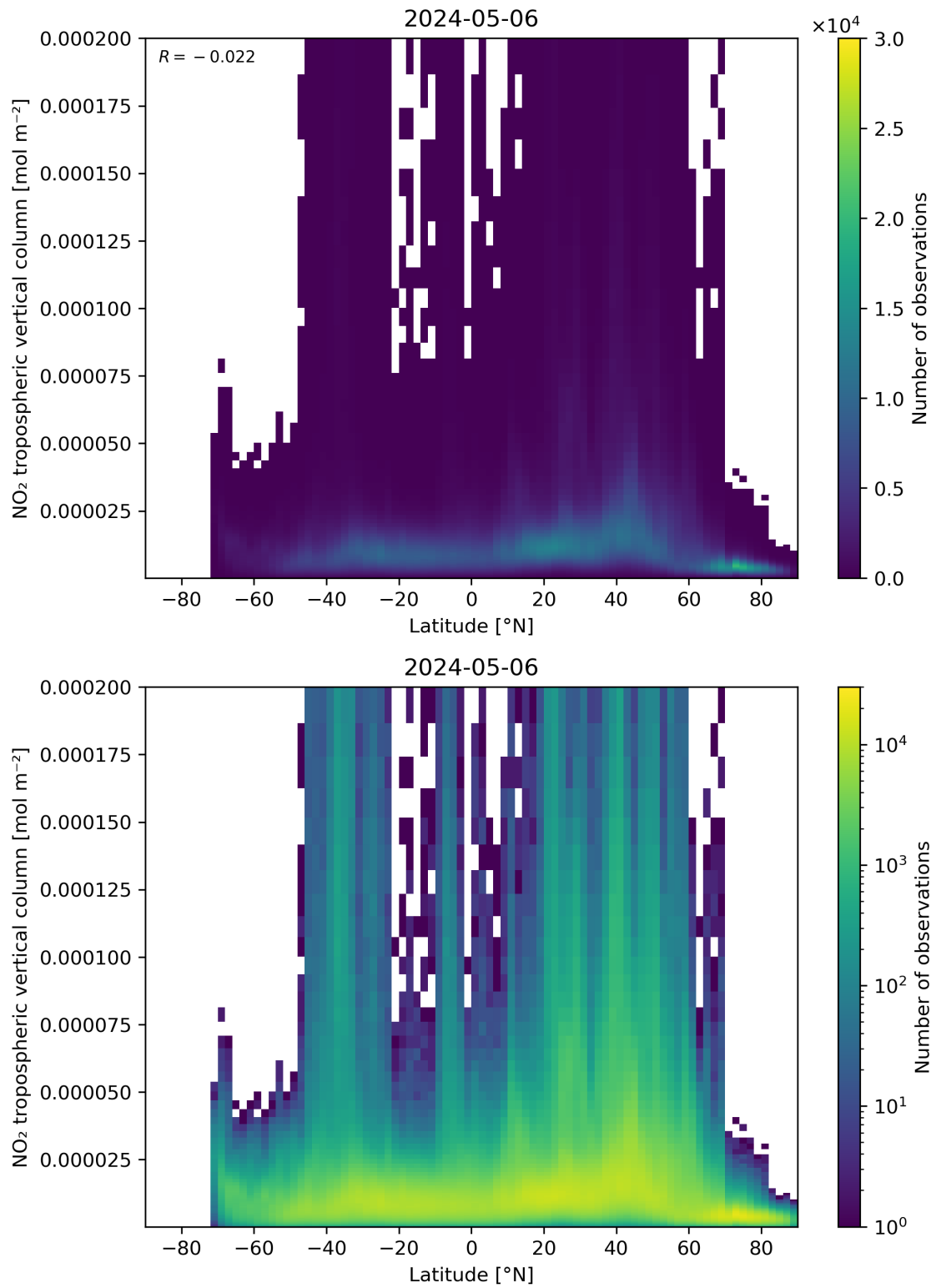
Figure 92: Scatter density plot of “Latitude” against “NO 2 tropospheric vertical column” for 2024-05-05 to 2024-05-07.
