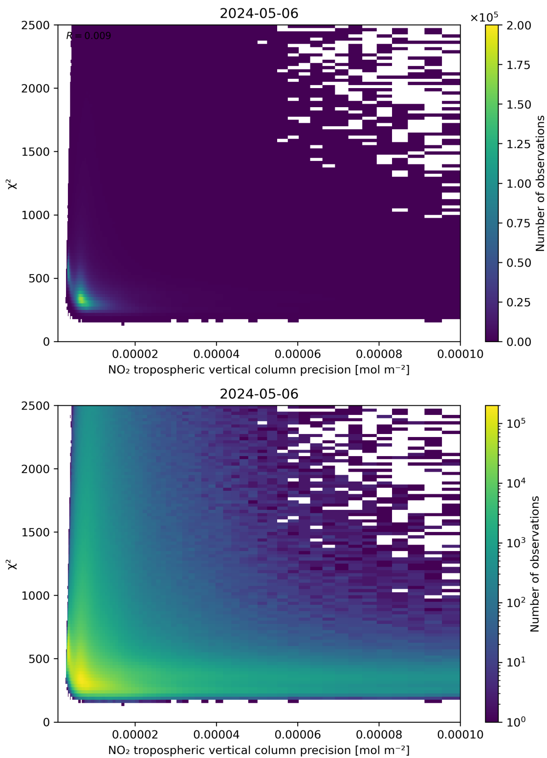
Figure 134: Scatter density plot of “NO 2 tropospheric vertical column precision” against “ \chi^2 ” for 2024-05-05 to 2024-05-07.
