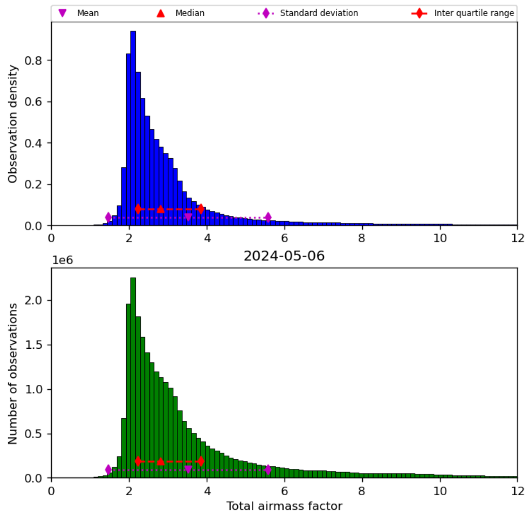
Figure 32: Histogram of “Total airmass factor” for 2024-05-05 to 2024-05-07
