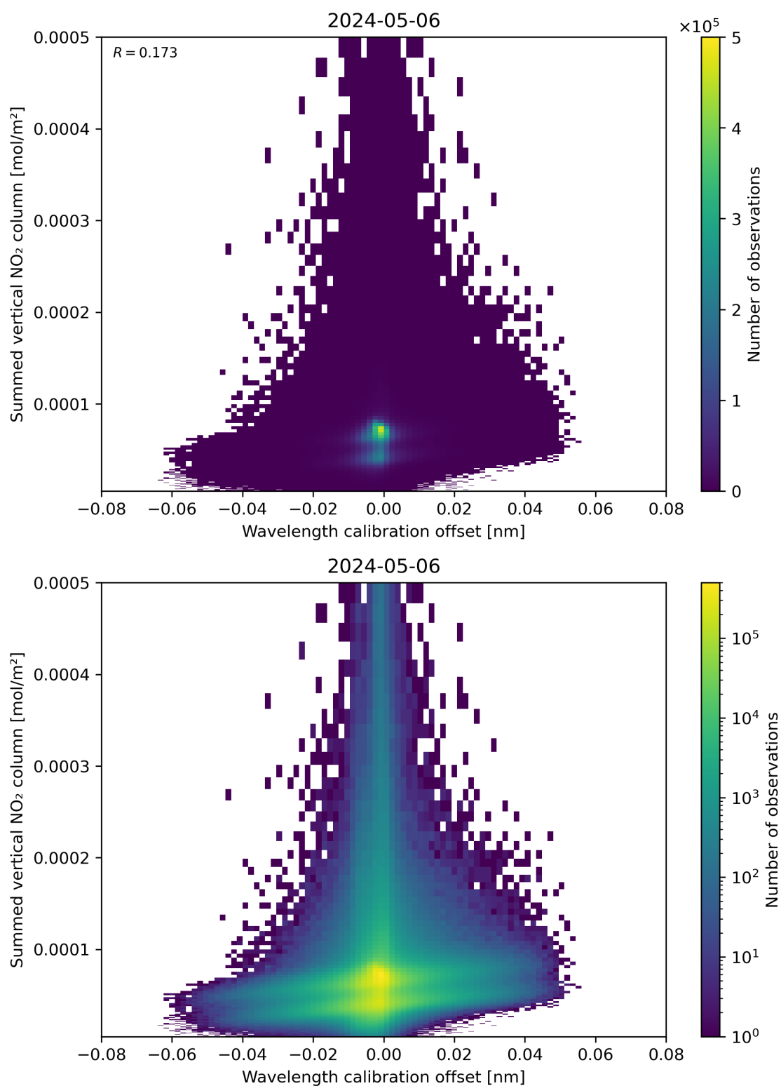
Figure 177: Scatter density plot of “Wavelength calibration offset” against “Summed vertical NO 2 column” for 2024-05-05 to 2024-05-07.
