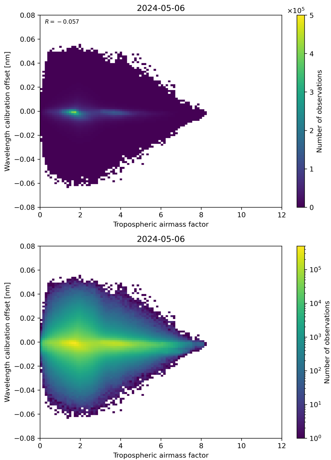
Figure 80: Scatter density plot of “Tropospheric airmass factor” against “Wavelength calibration offset” for 2024-05-05 to 2024-05-07.
