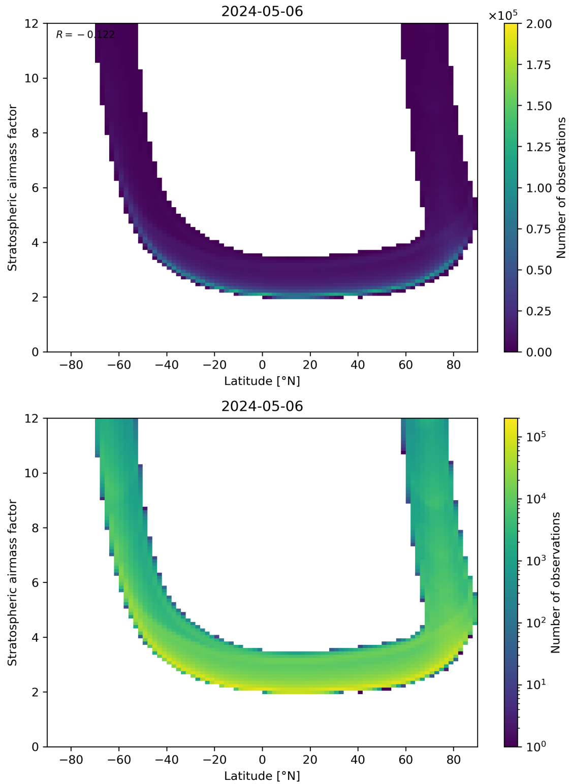
Figure 83: Scatter density plot of “Latitude” against “Stratospheric air mass factor” for 2024-05-05 to 2024-05-07.
