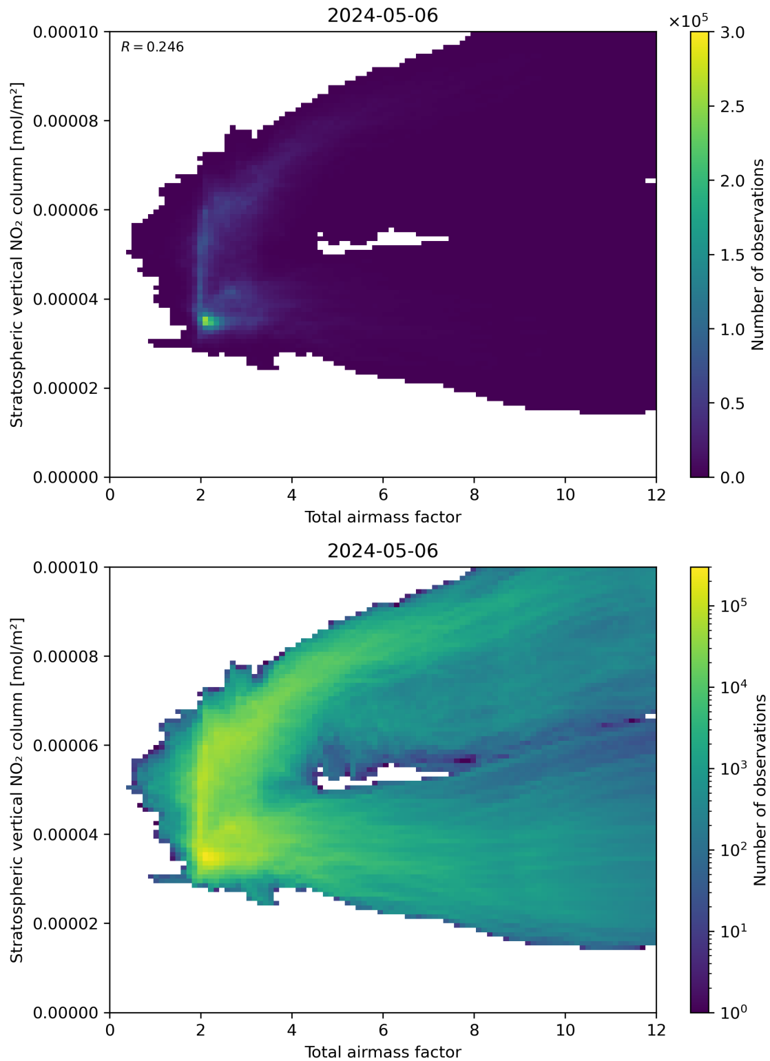
Figure 64: Scatter density plot of “Total airmass factor” against “Stratospheric vertical \text{NO}_2 column” for 2024-05-05 to 2024-05-07.
