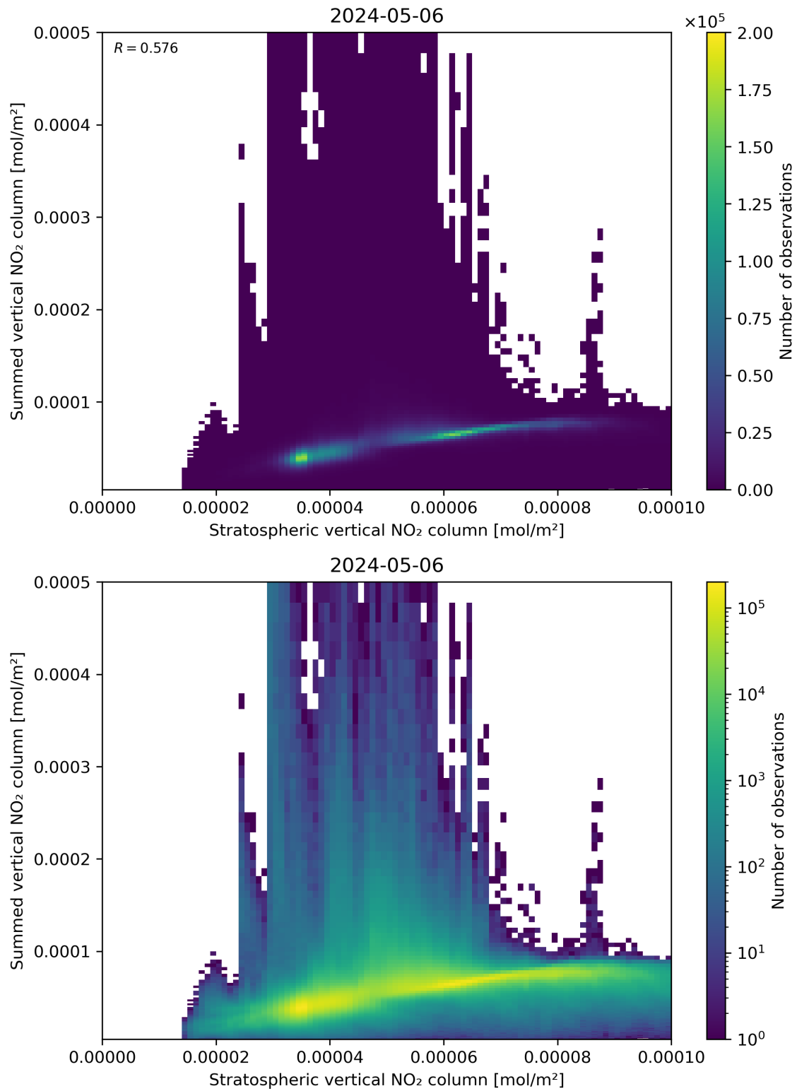
Figure 98: Scatter density plot of “Stratospheric vertical NO 2 column” against “Summed vertical NO 2 column” for 2024-05-05 to 2024-05-07.
