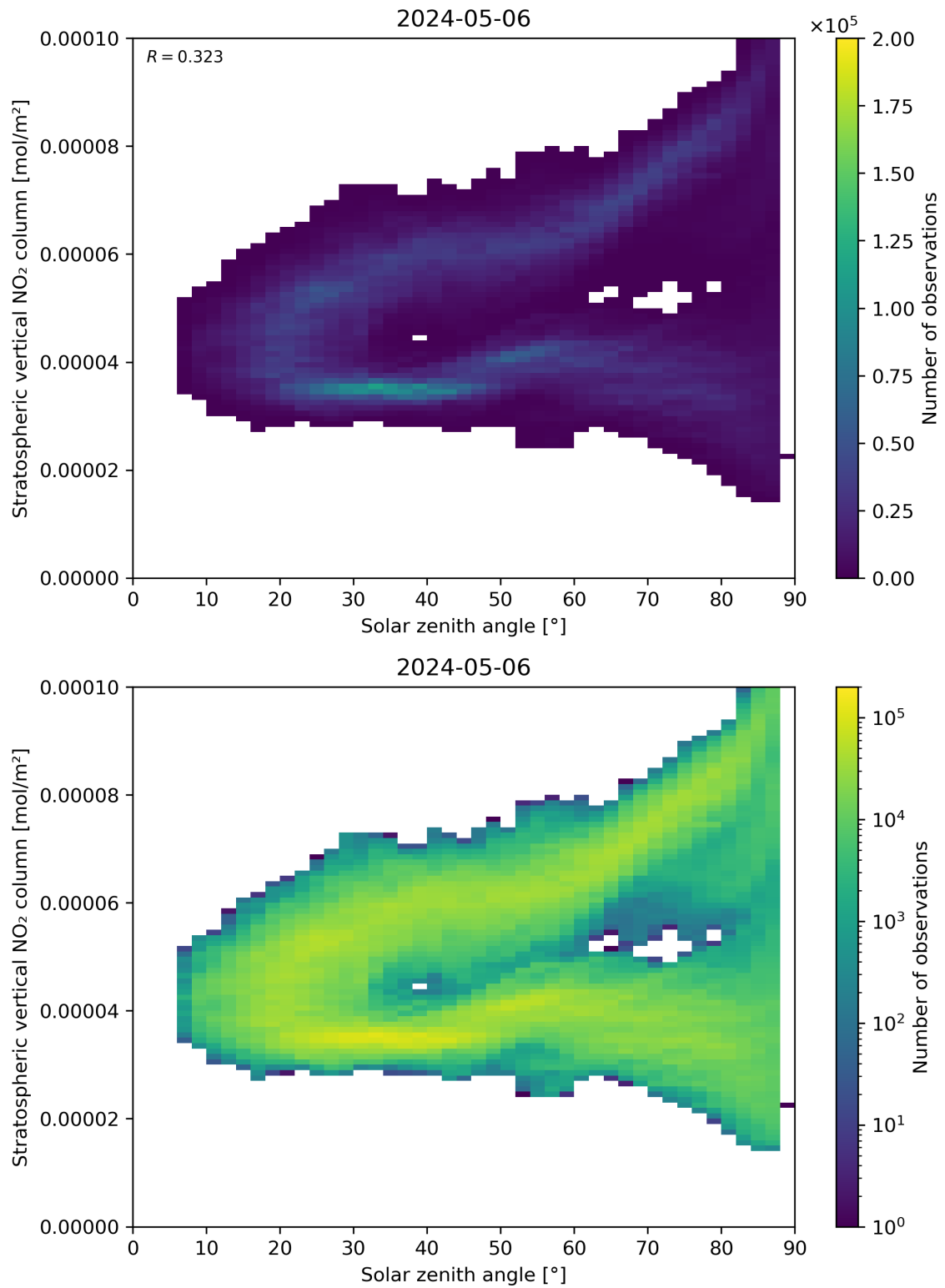
Figure 150: Scatter density plot of “Solar zenith angle” against “Stratospheric vertical NO 2 column” for 2024-05-05 to 2024-05-07.
