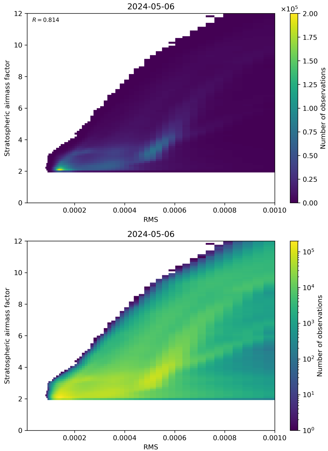
Figure 144: Scatter density plot of “RMS” against “Stratospheric airmass factor” for 2024-05-05 to 2024-05-07.
